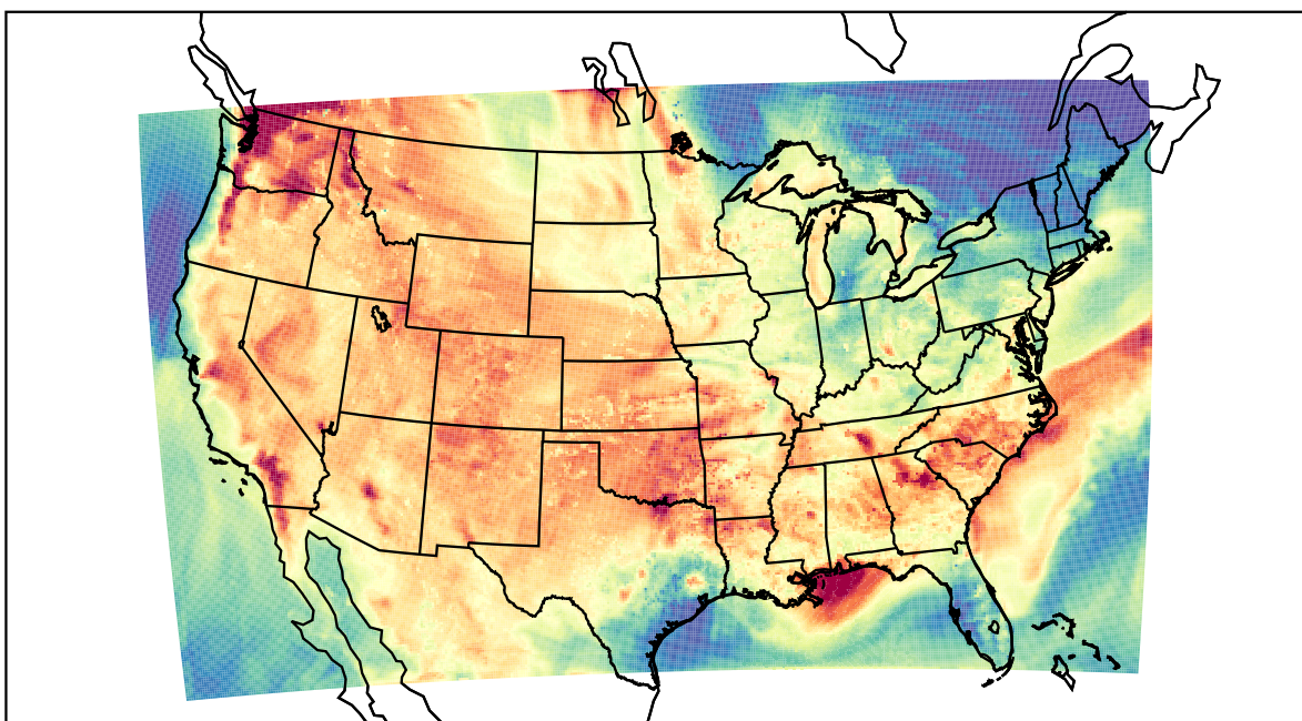
WRF (2021-08-01_00:00:00)
