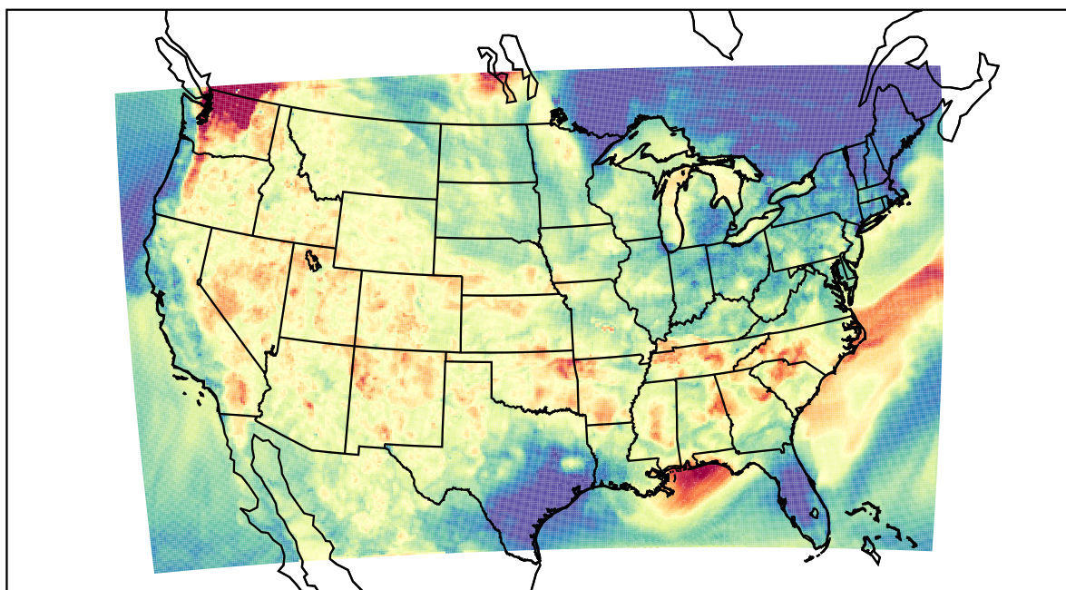
WRF (2021-08-01_04:00:00)
