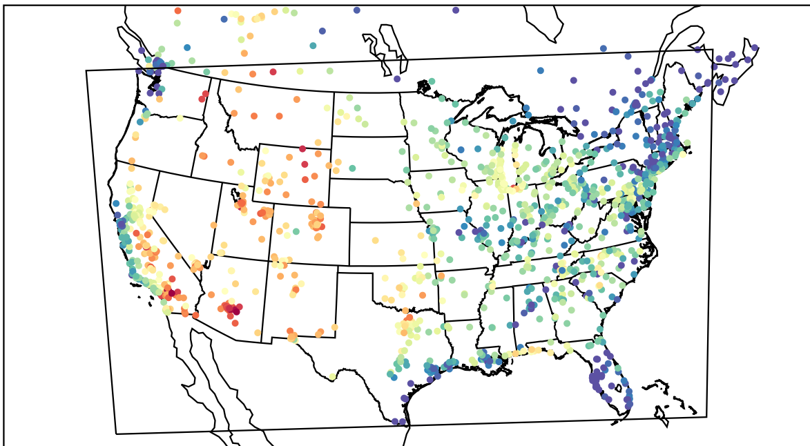
AirNOW (2021-08-01_00:00:00)
