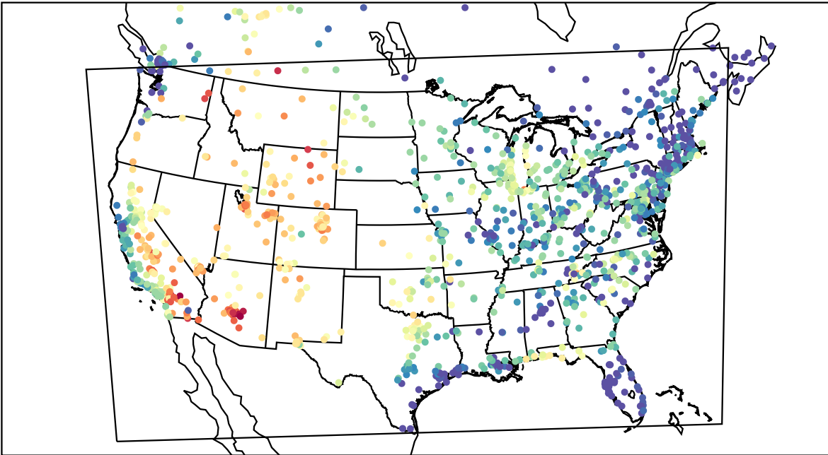
AirNOW (2021-08-01_01:00:00)
