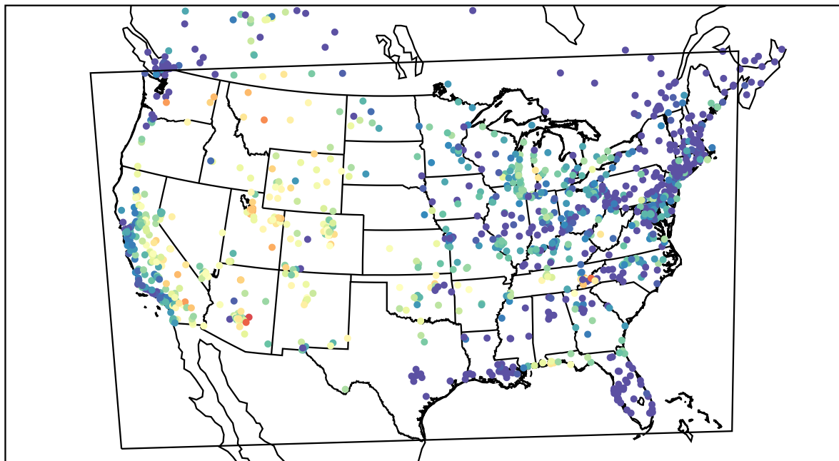
AirNOW (2021-08-01_04:00:00)
