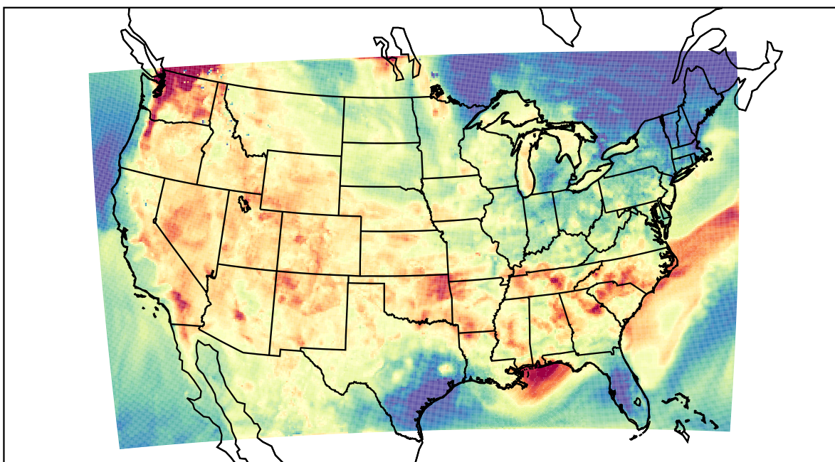
WRF (2021-08-01_02:00:00)
