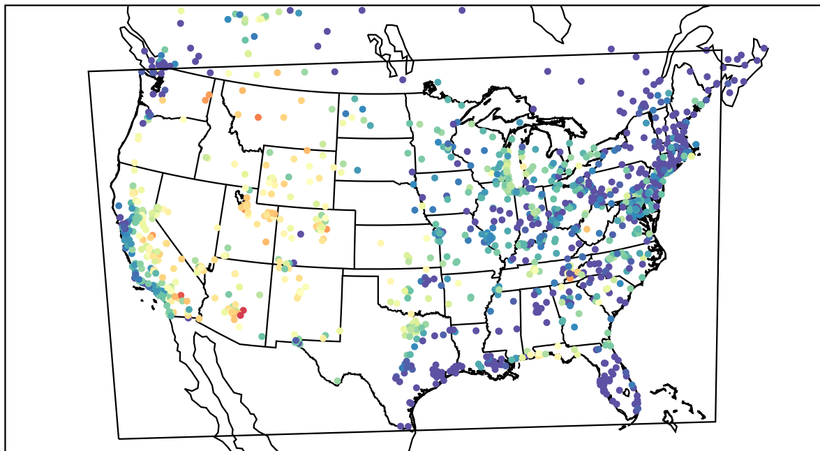
AirNOW (2021-08-01_03:00:00)
