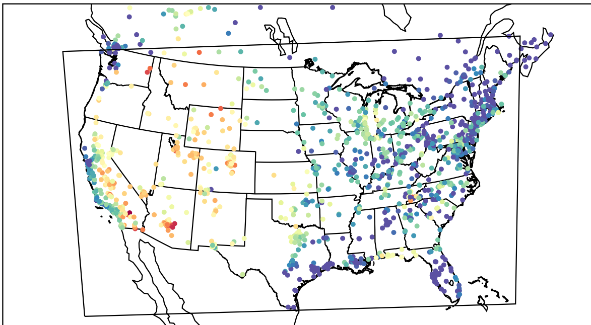
AirNOW (2021-08-01_02:00:00)
