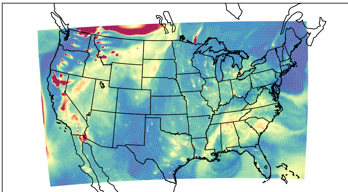
WRF 2021-08-17_02:00:00
