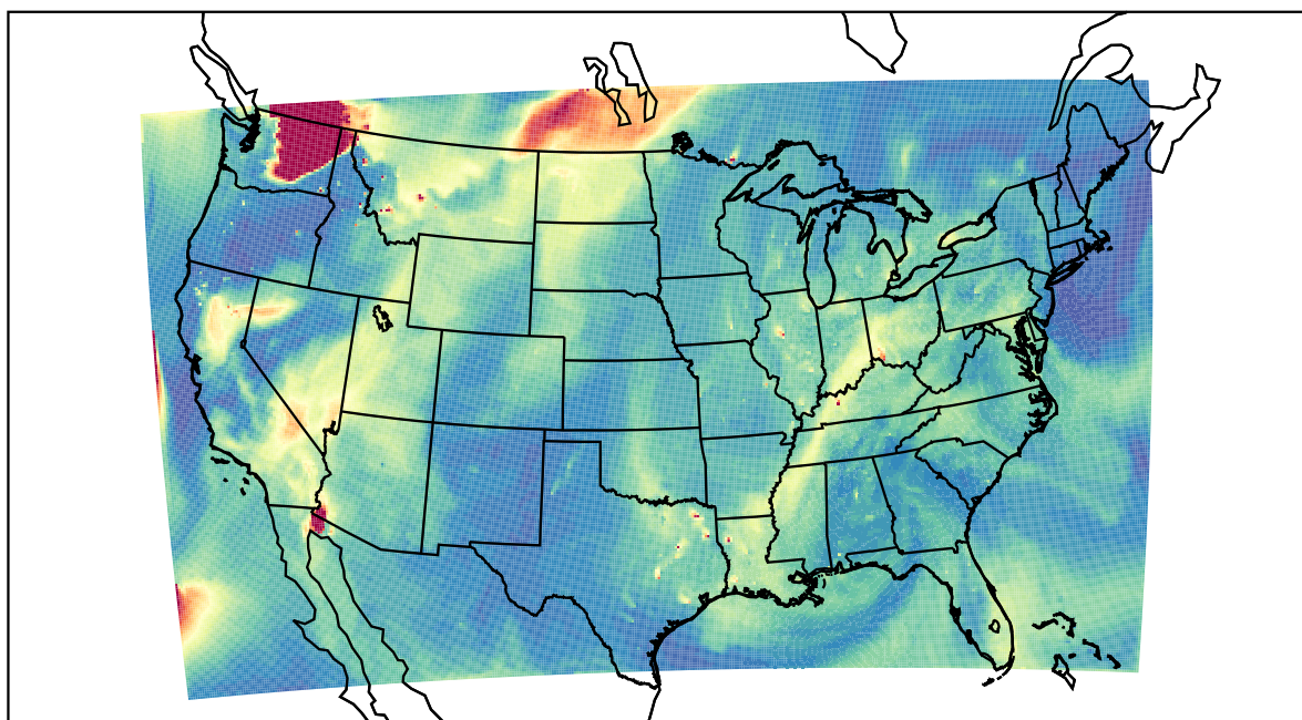
WRF 2021-08-17_19:00:00
