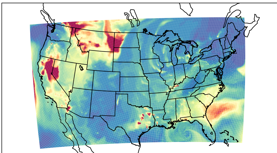
WRF 2021-08-16_09:00:00
