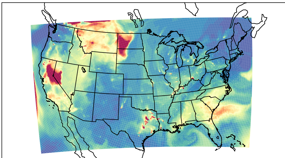
WRF 2021-08-16_14:00:00
