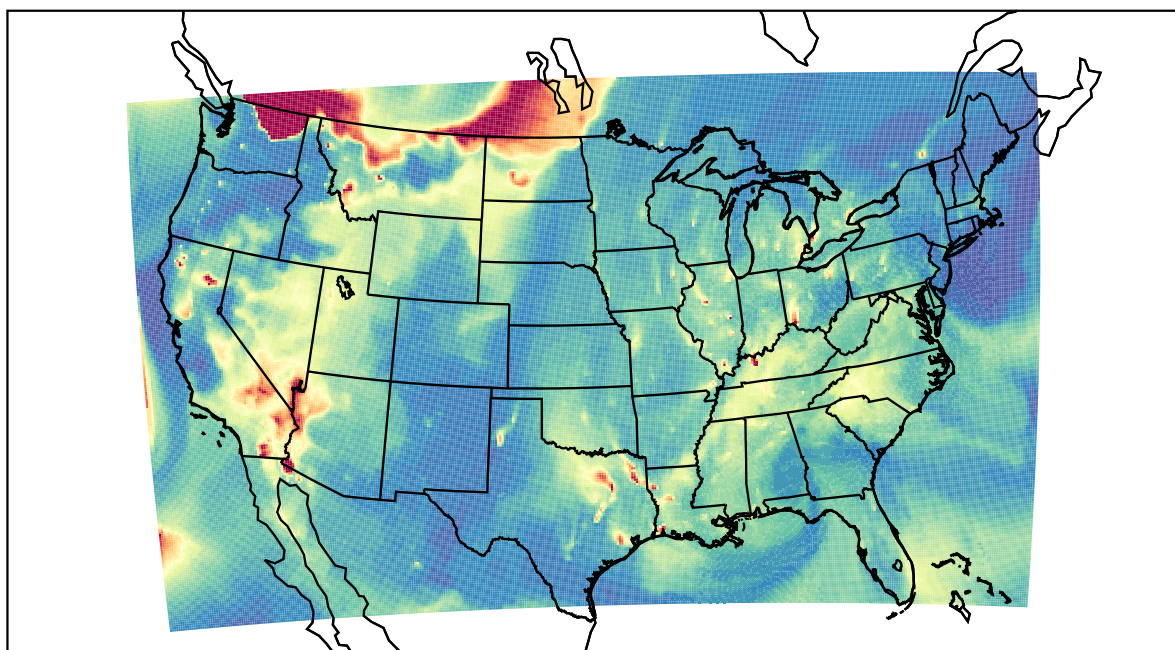
WRF 2021-08-17_13:00:00
