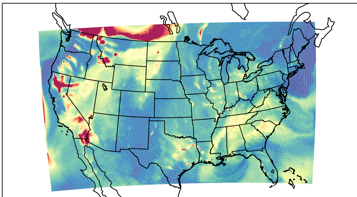
WRF 2021-08-17_05:00:00
