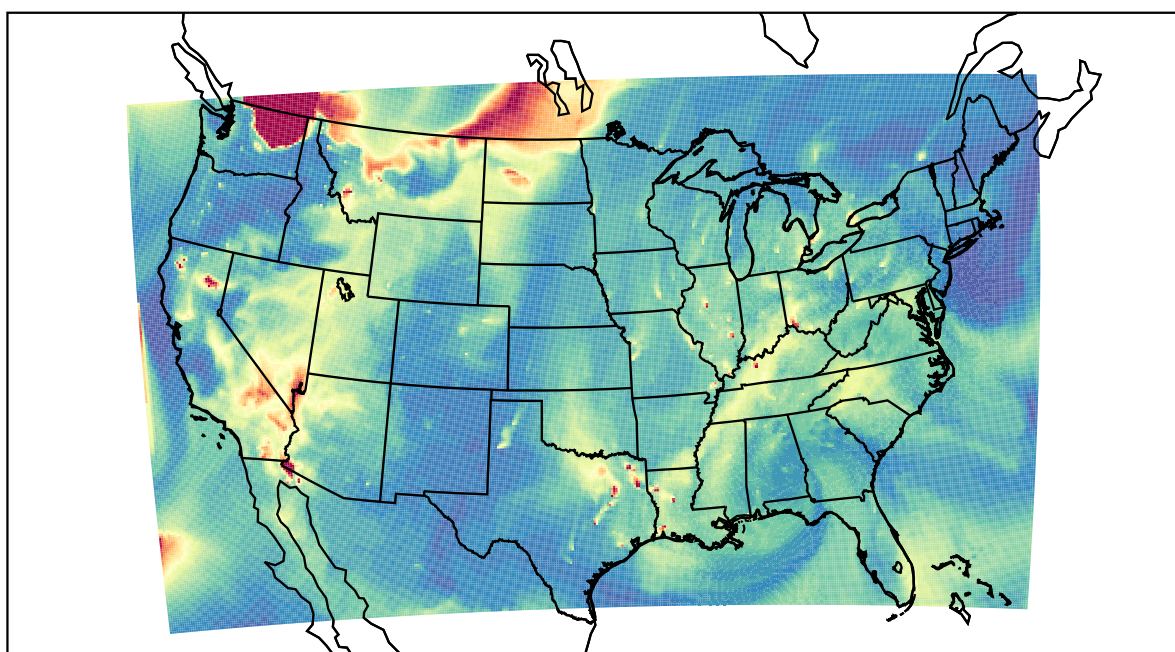
WRF 2021-08-17_15:00:00
