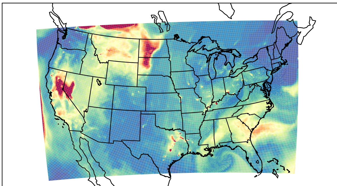
WRF 2021-08-16_16:00:00
