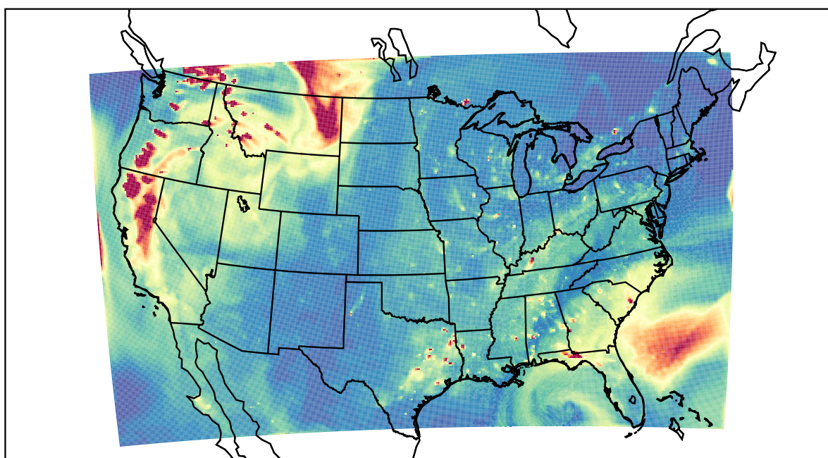
WRF 2021-08-16_01:00:00
