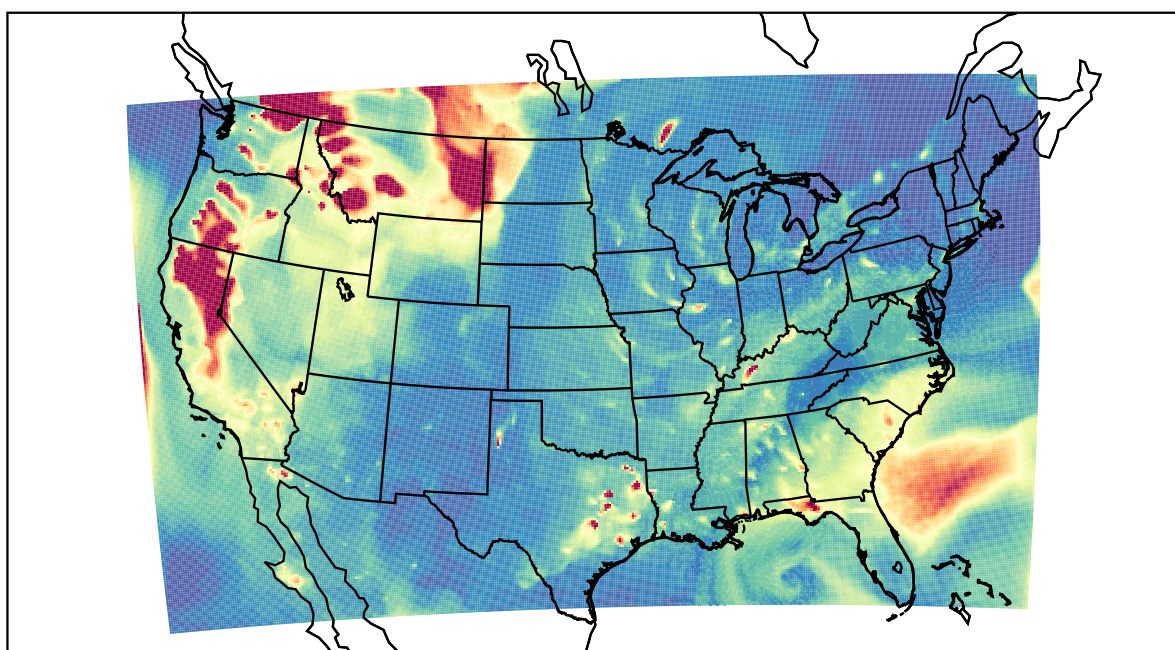
WRF 2021-08-16_04:00:00
