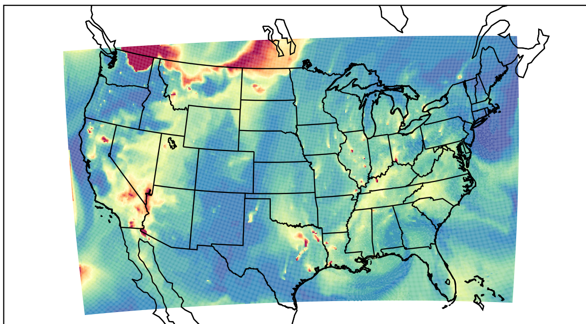
WRF 2021-08-17_14:00:00
