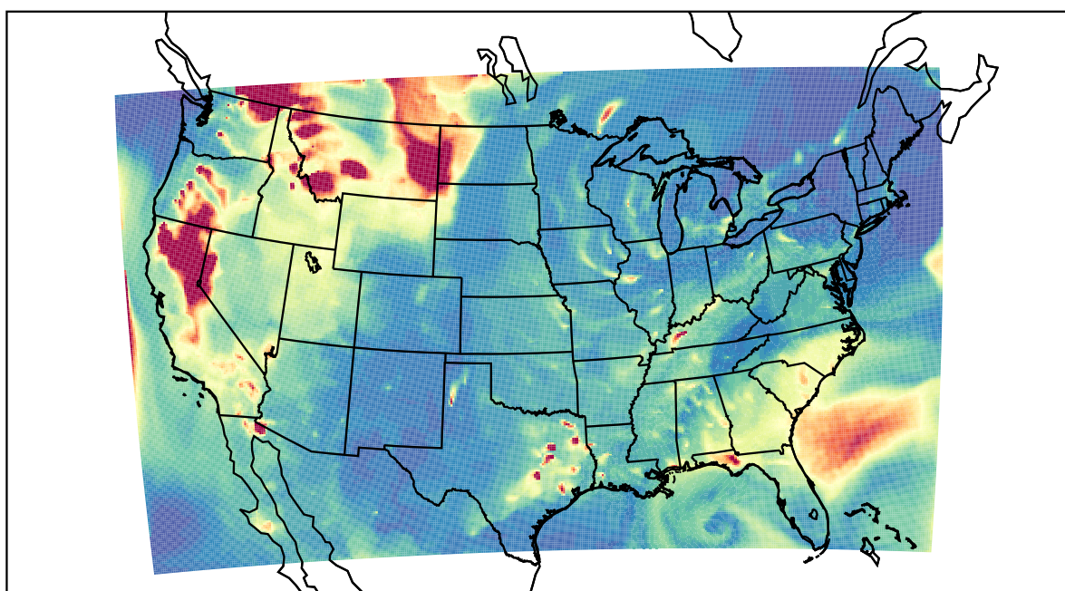
WRF 2021-08-16_05:00:00
