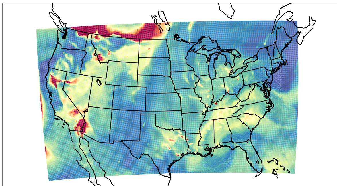
WRF 2021-08-17_07:00:00
