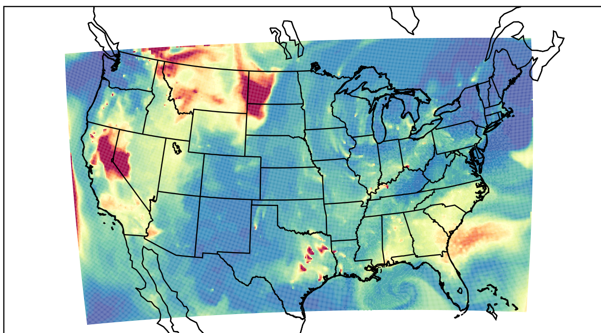
WRF 2021-08-16_12:00:00
