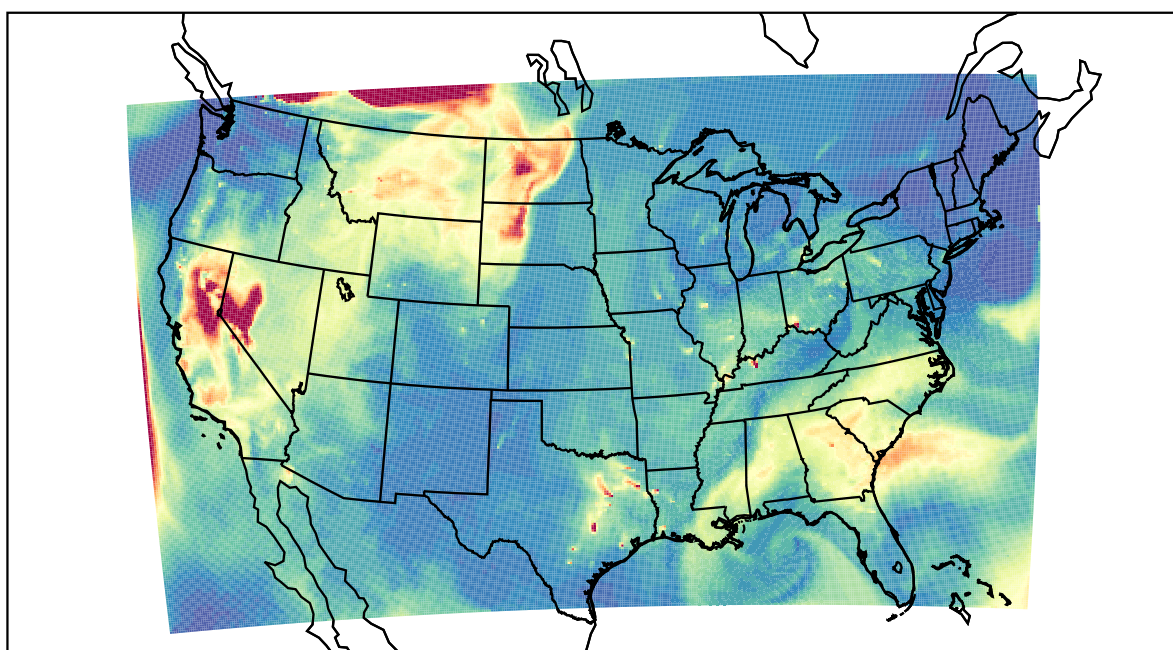
WRF 2021-08-16_17:00:00
