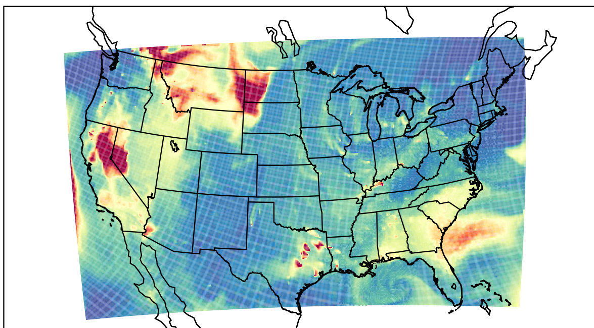
WRF 2021-08-16_11:00:00
