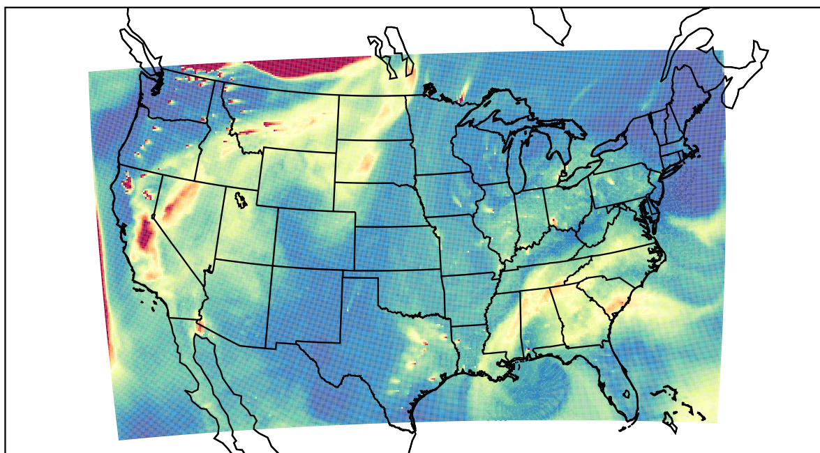
WRF 2021-08-16_22:00:00
