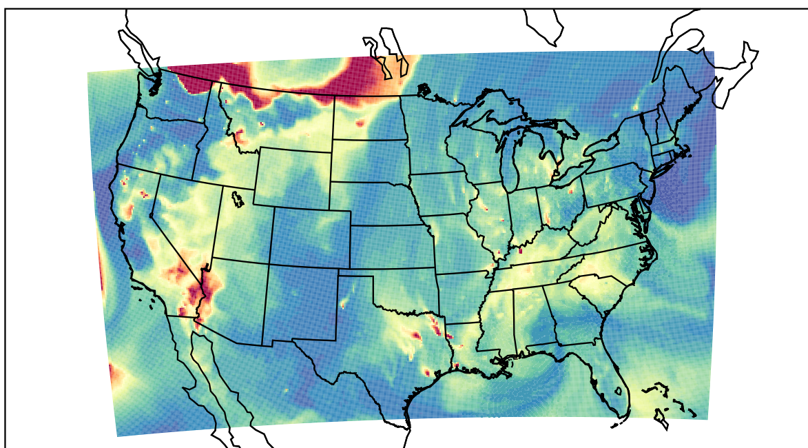
WRF 2021-08-17_11:00:00
