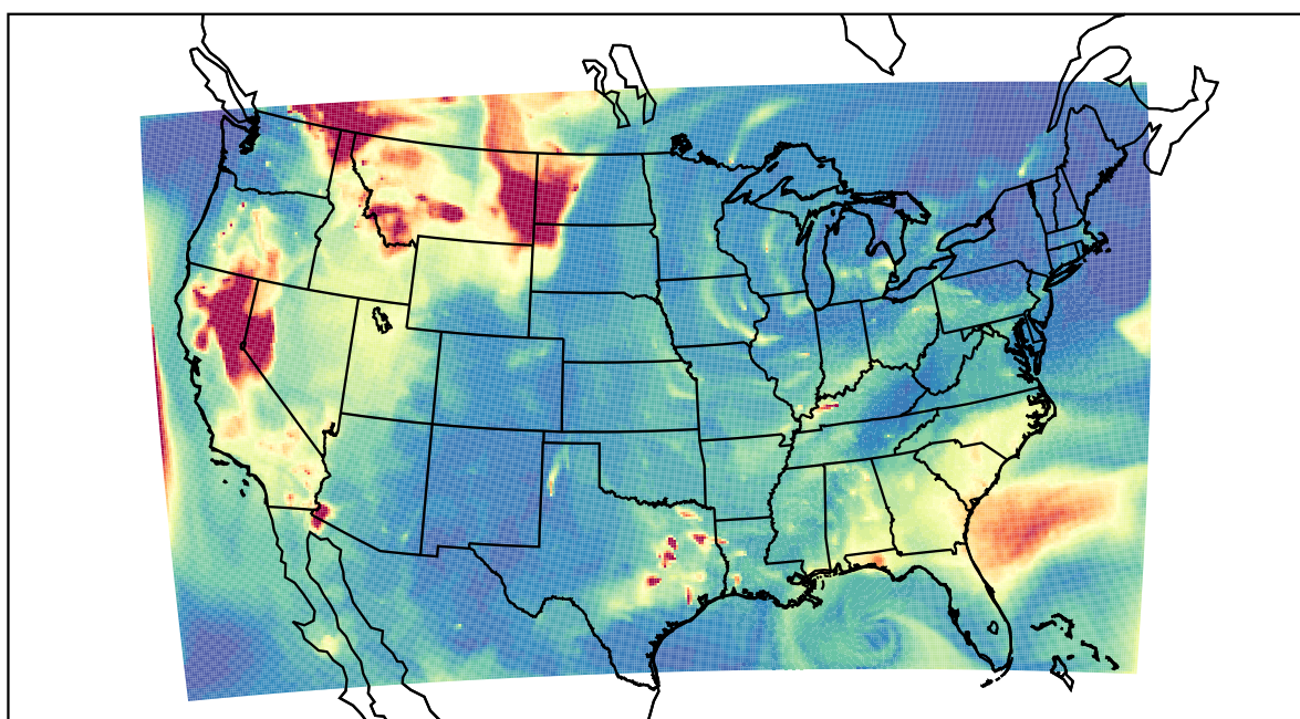
WRF 2021-08-16_08:00:00
