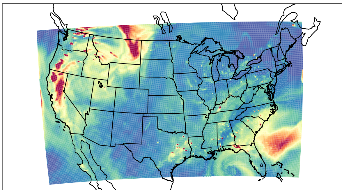
WRF 2021-08-16_00:00:00
