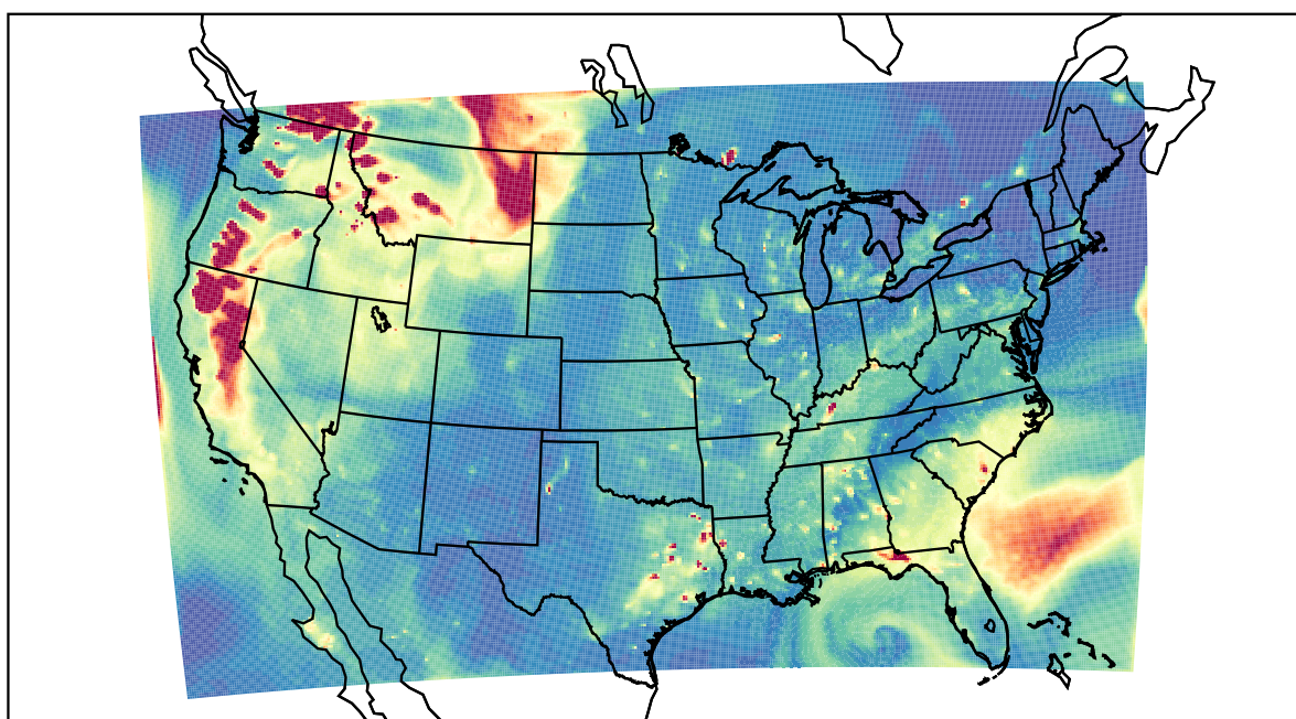
WRF 2021-08-16_02:00:00
