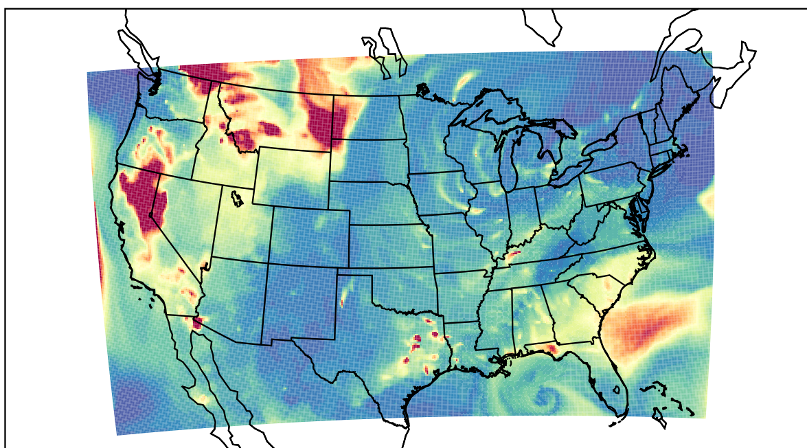
WRF 2021-08-16_06:00:00
