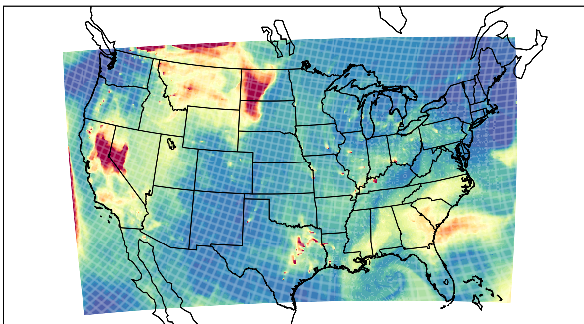
WRF 2021-08-16_15:00:00
