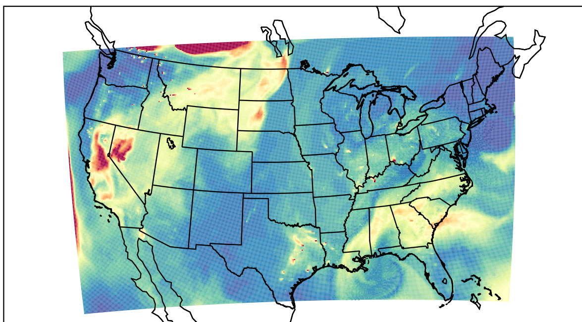
WRF 2021-08-16_19:00:00
