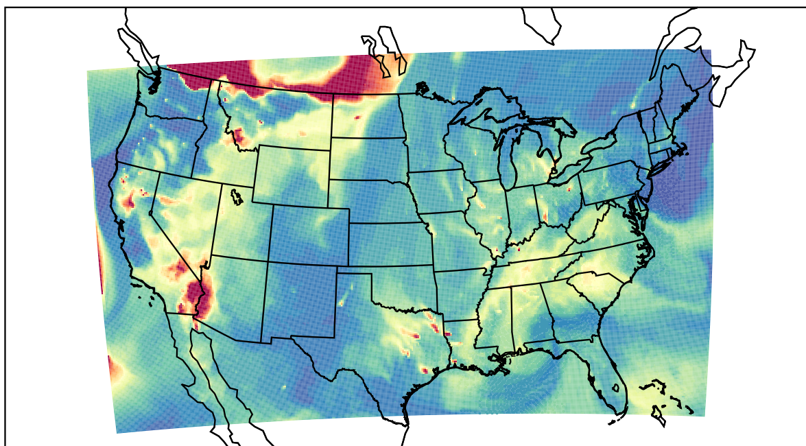
WRF 2021-08-17_09:00:00
