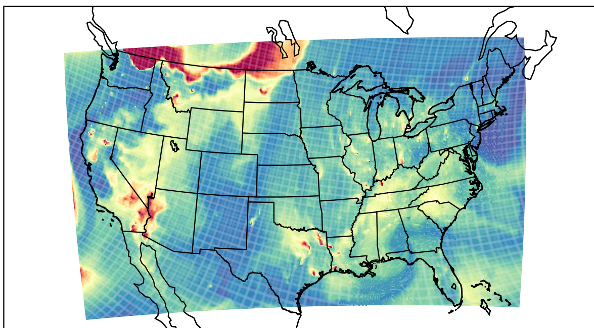
WRF 2021-08-17_12:00:00
