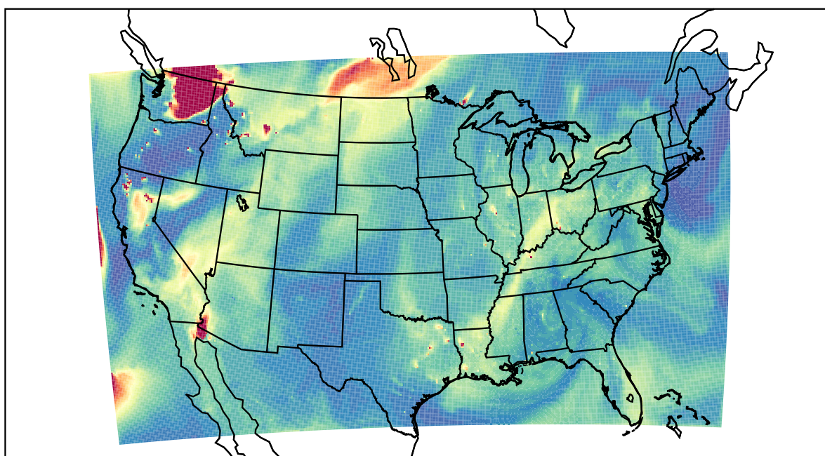
WRF 2021-08-17_21:00:00
