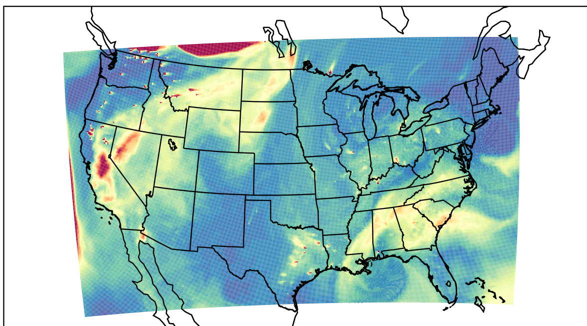
WRF 2021-08-16_21:00:00
