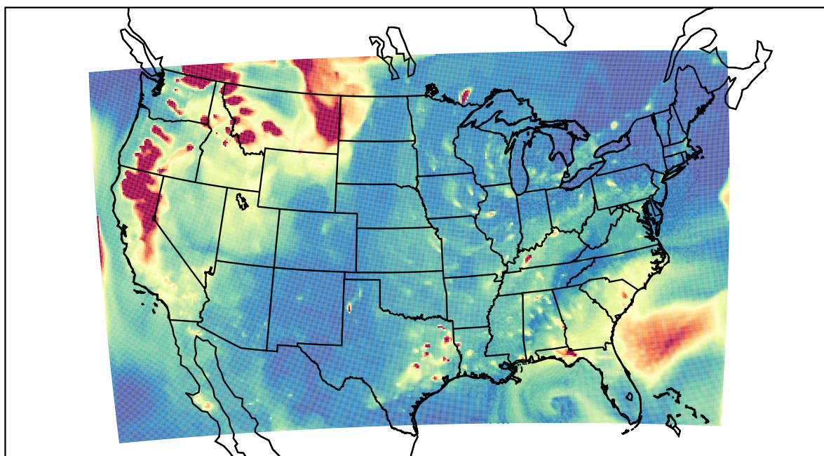
WRF 2021-08-16_03:00:00
