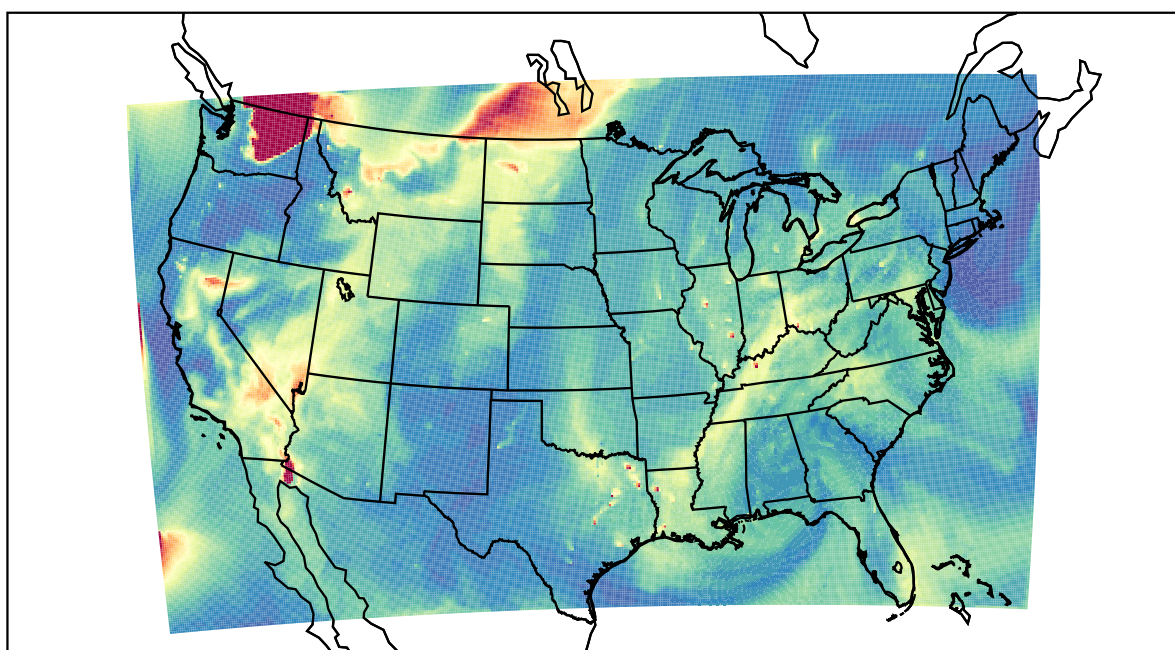
WRF 2021-08-17_17:00:00
