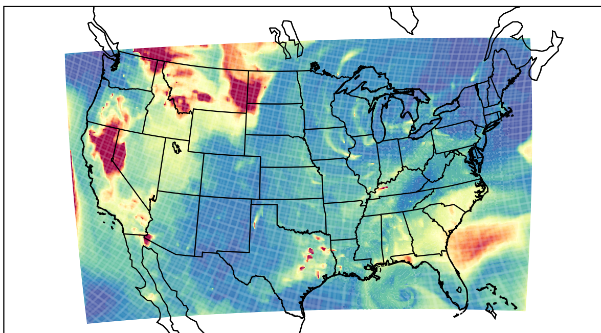
WRF 2021-08-16_07:00:00
