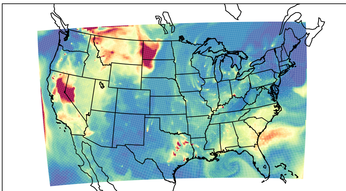
WRF 2021-08-16_13:00:00
