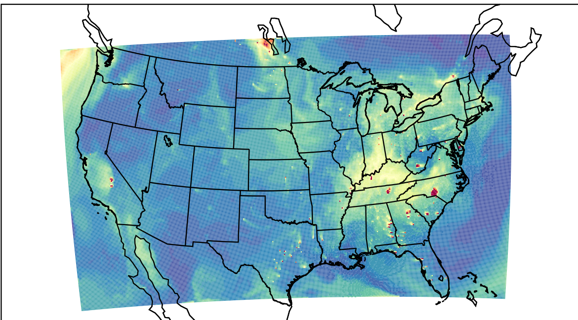
WRF 2021-10-02_22:00:00
