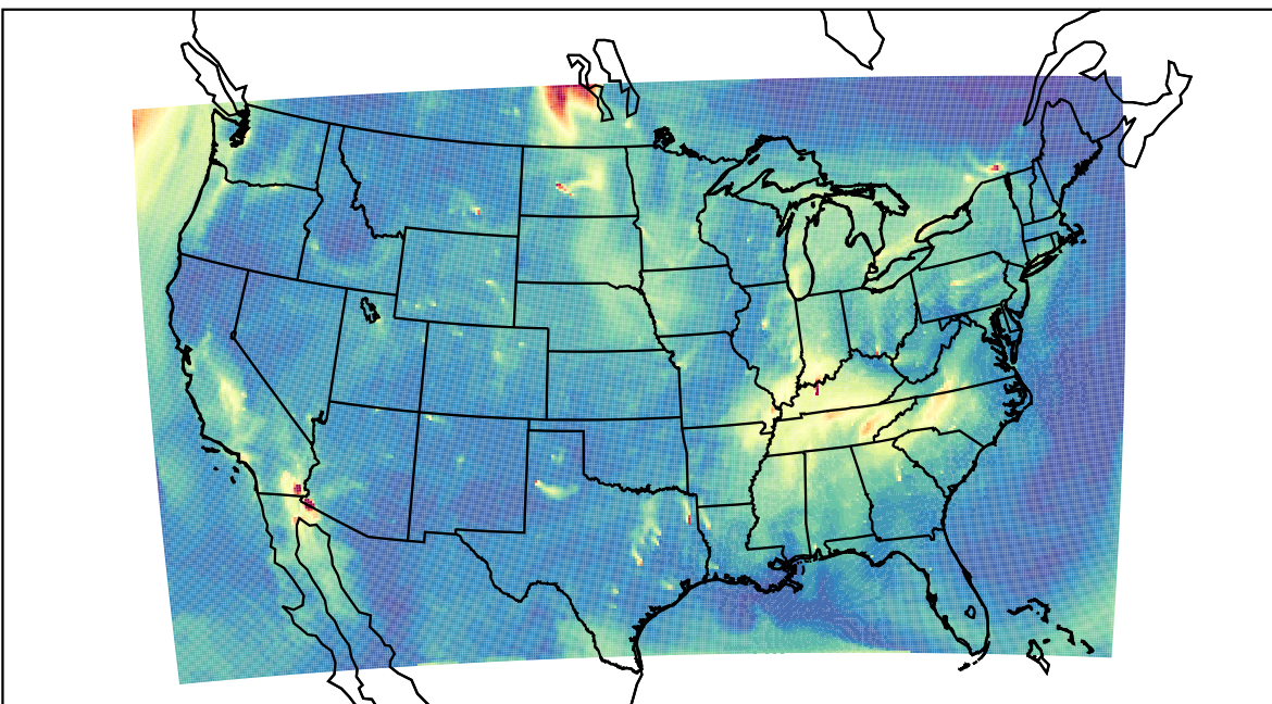
WRF 2021-10-02_16:00:00
