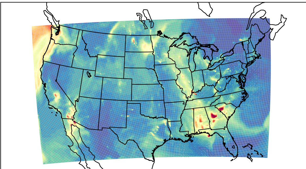
WRF 2021-10-01_09:00:00
