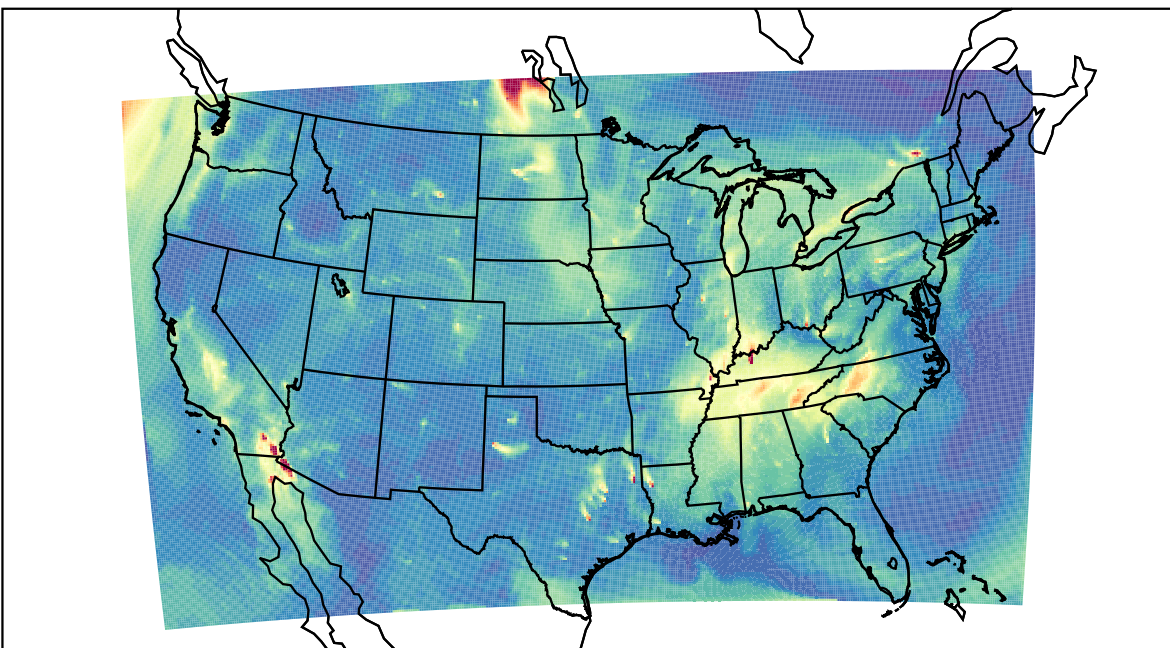
WRF 2021-10-02_15:00:00
