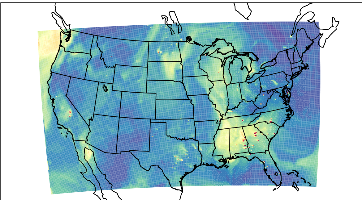
WRF 2021-10-01_21:00:00
