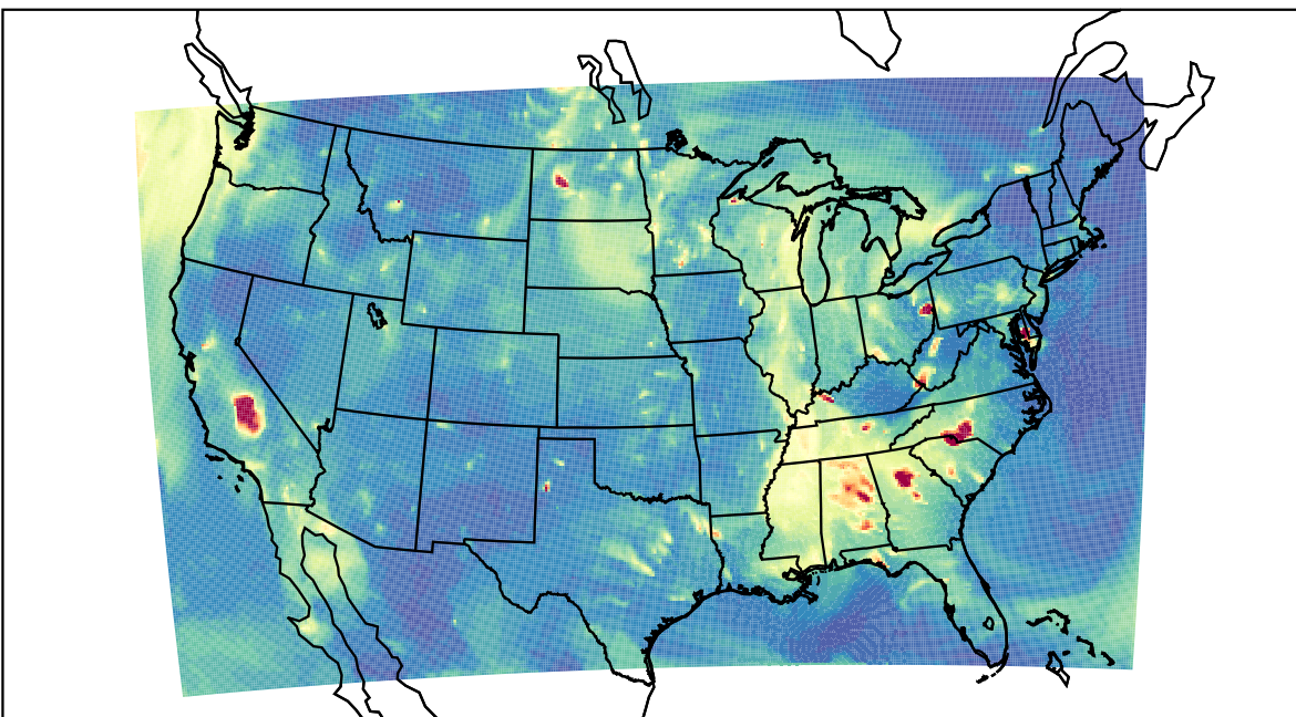
WRF 2021-10-02_04:00:00
