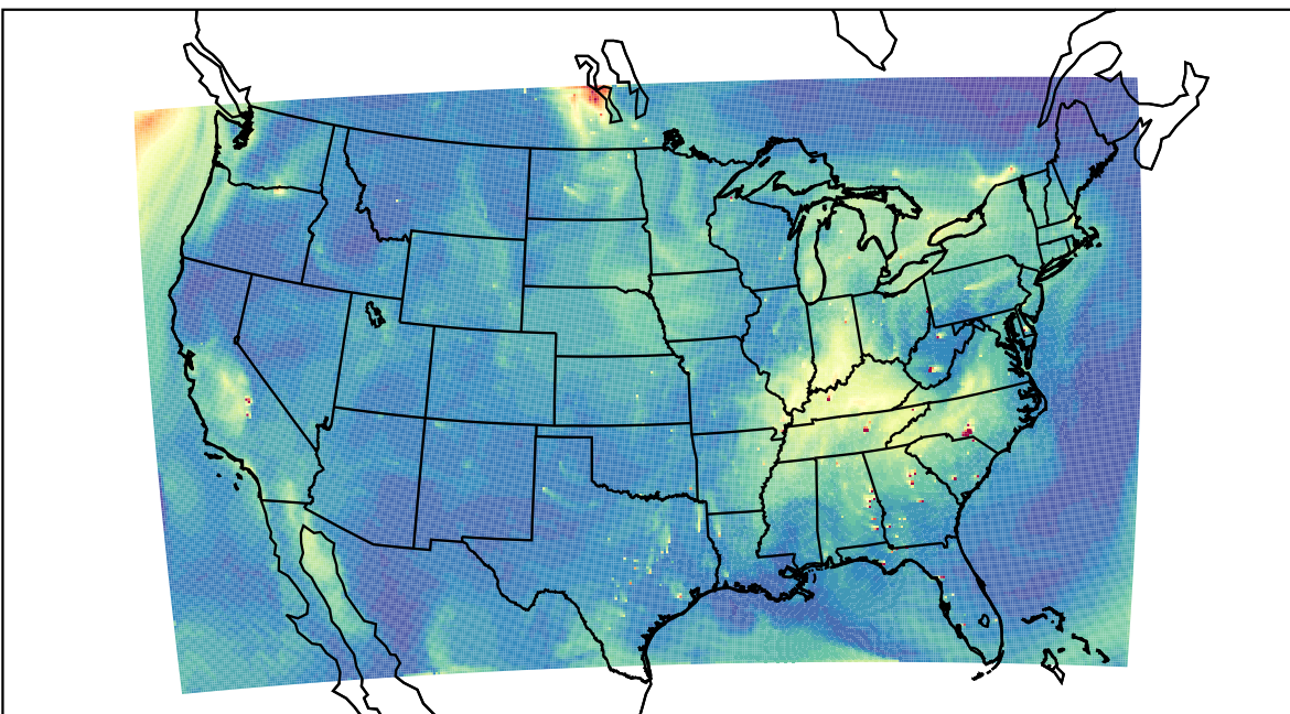
WRF 2021-10-02_20:00:00
