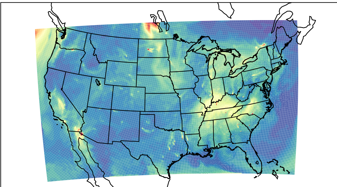
WRF 2021-10-02_17:00:00
