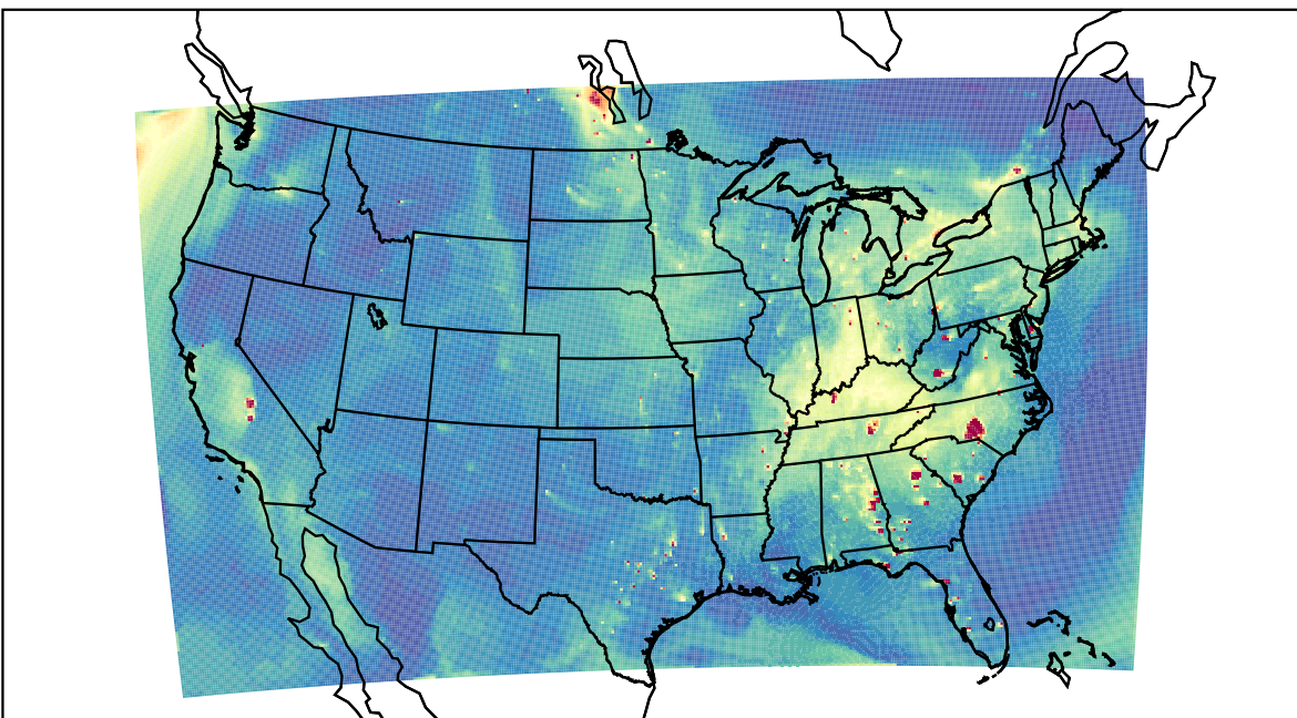
WRF 2021-10-02_23:00:00
