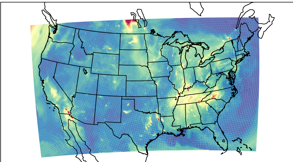
WRF 2021-10-02_14:00:00
