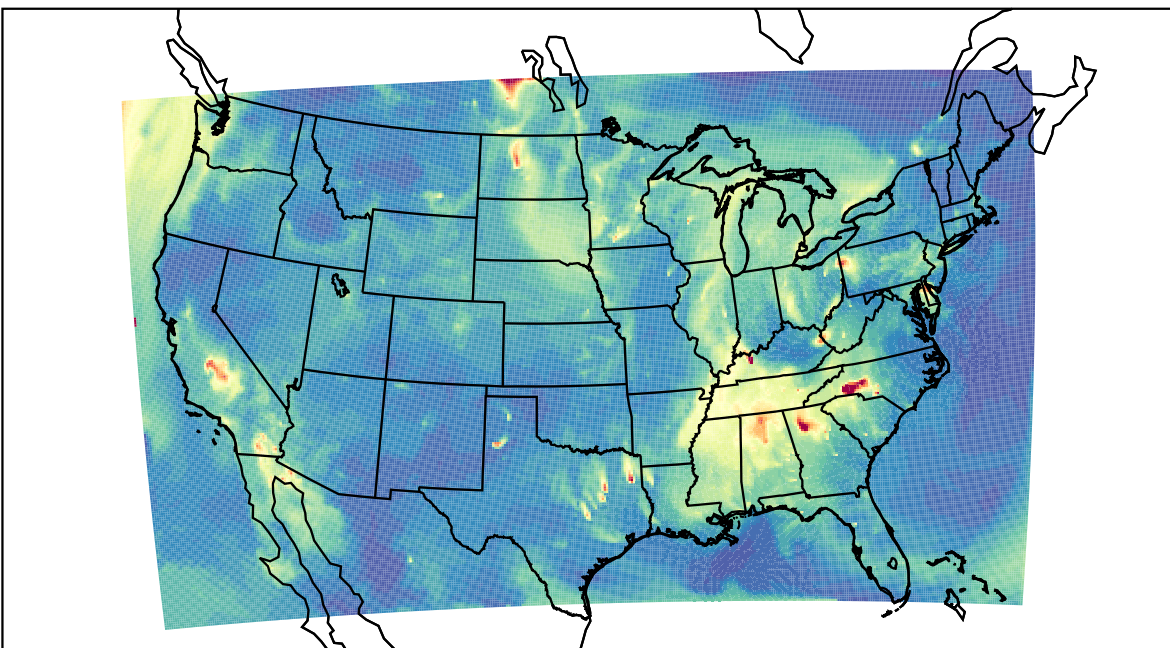
WRF 2021-10-02_09:00:00
