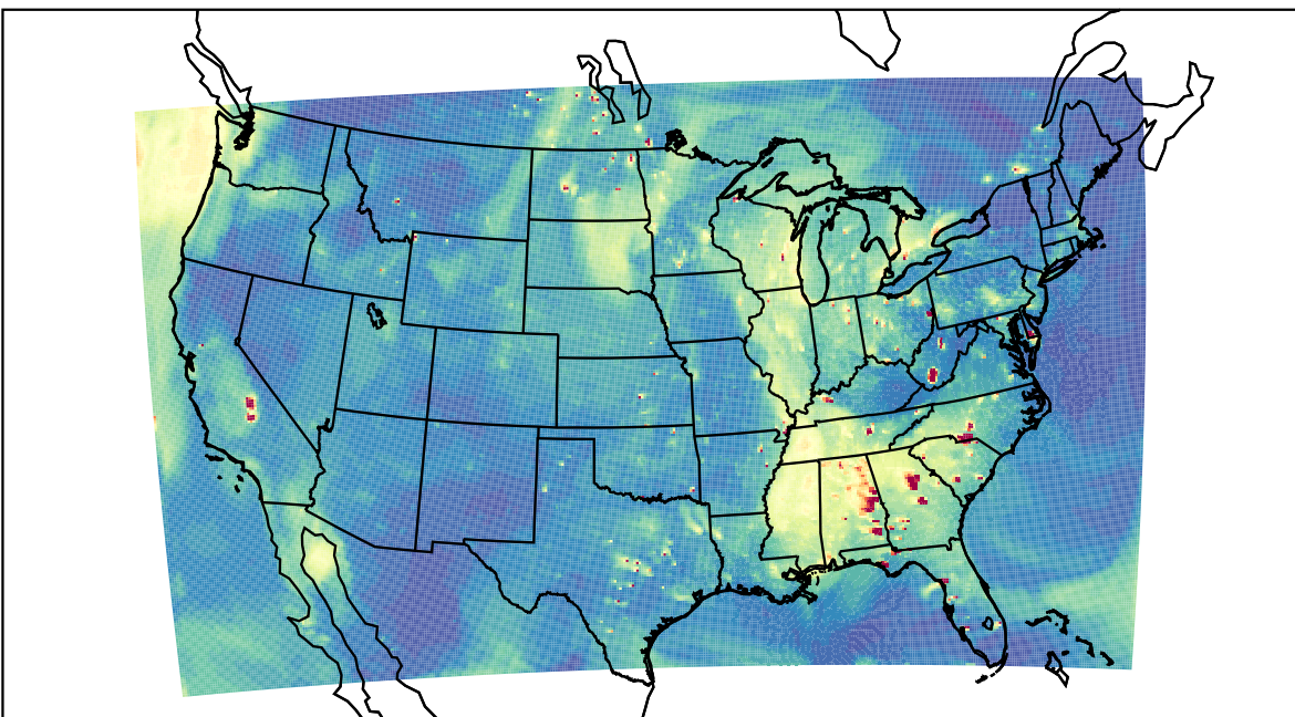
WRF 2021-10-02_00:00:00
