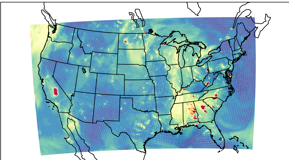
WRF 2021-10-02_02:00:00
