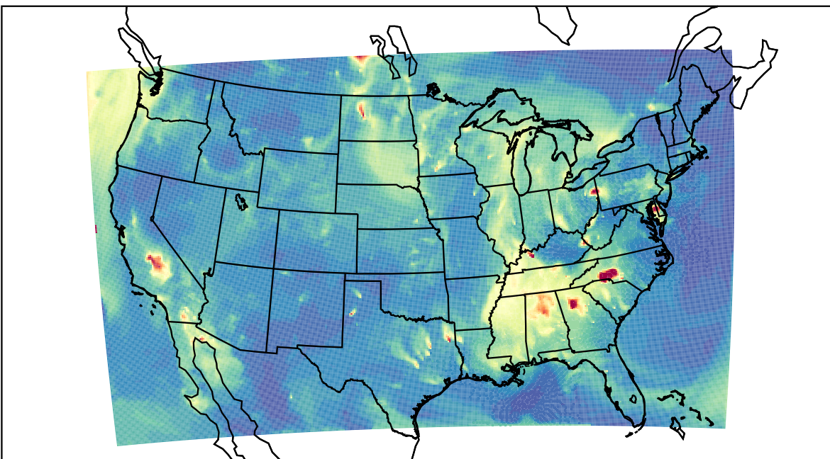
WRF 2021-10-02_07:00:00
