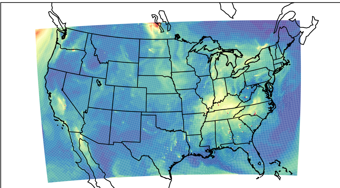
WRF 2021-10-02_19:00:00
