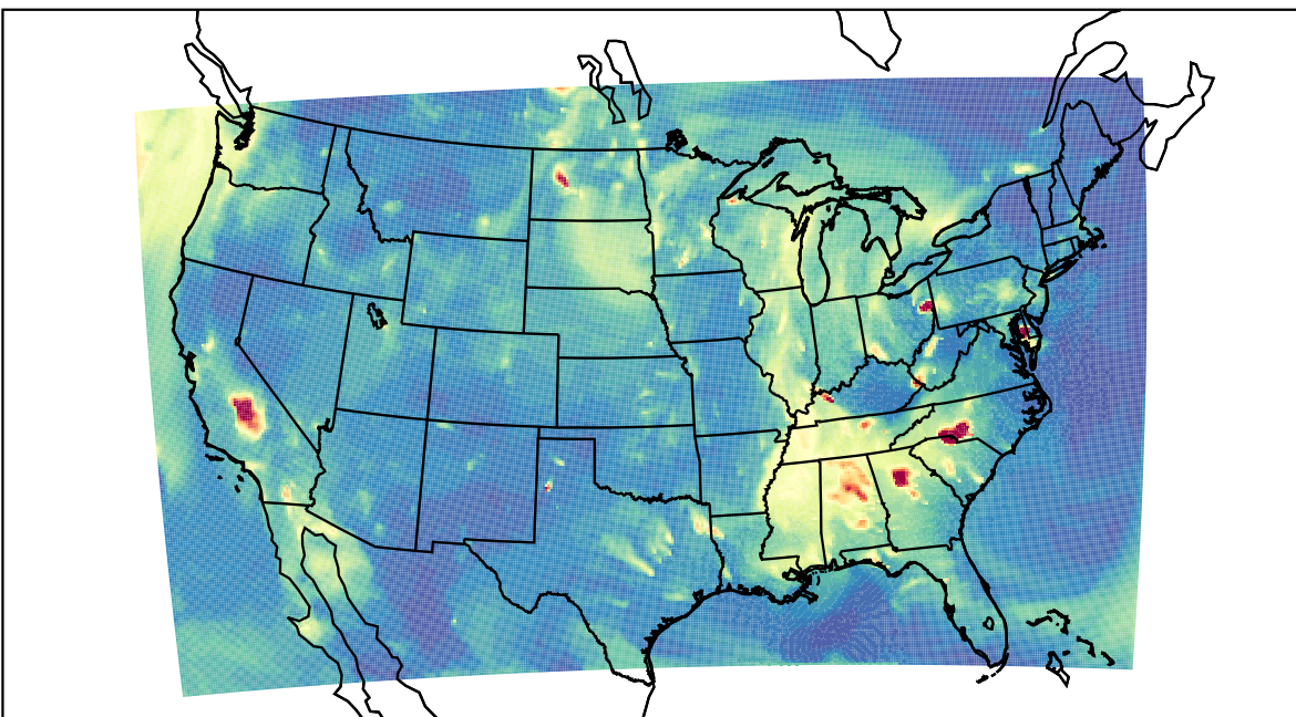
WRF 2021-10-02_05:00:00
