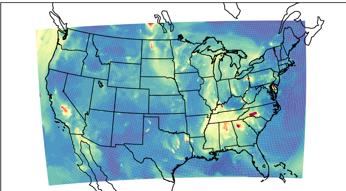
WRF 2021-10-02_08:00:00
