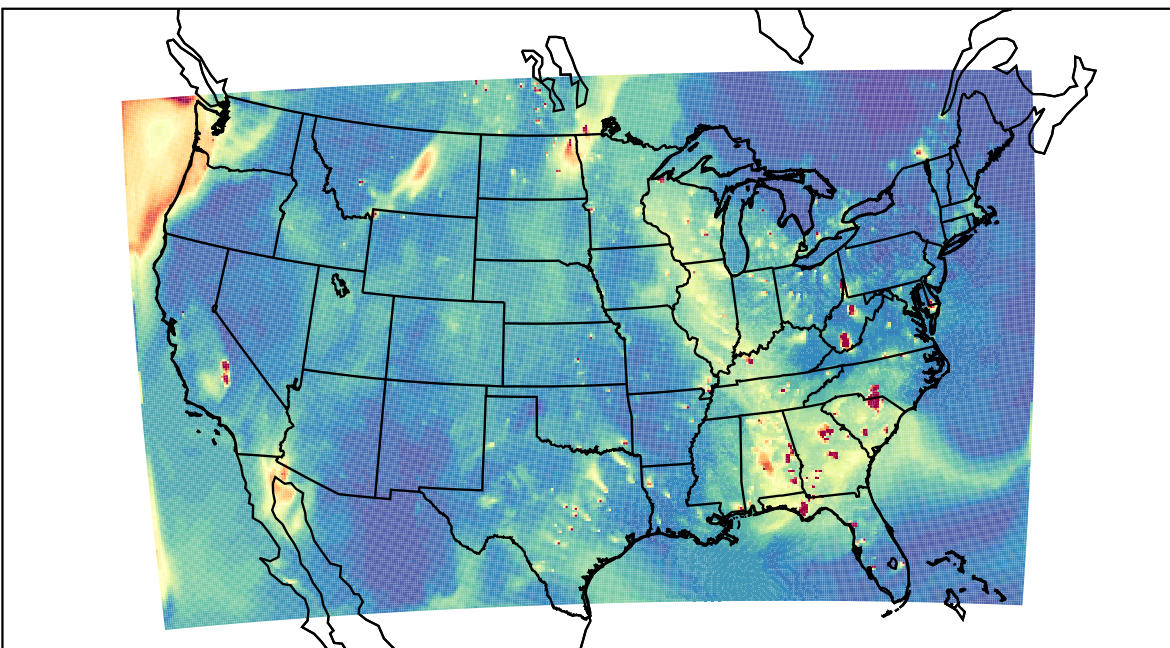
WRF 2021-10-01_00:00:00
