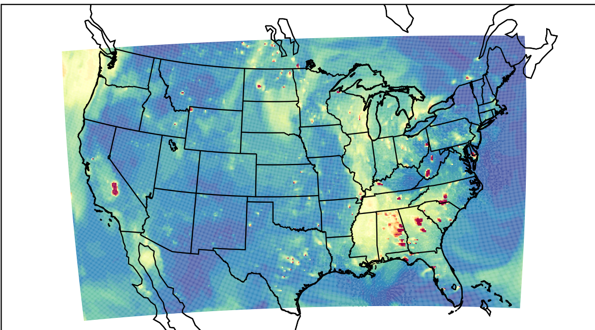
WRF 2021-10-02_01:00:00
