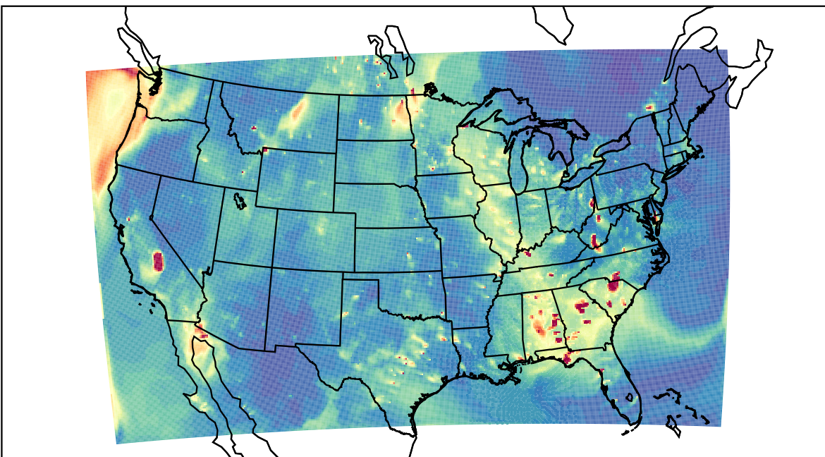
WRF 2021-10-01_02:00:00
