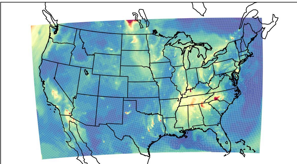
WRF 2021-10-02_12:00:00
