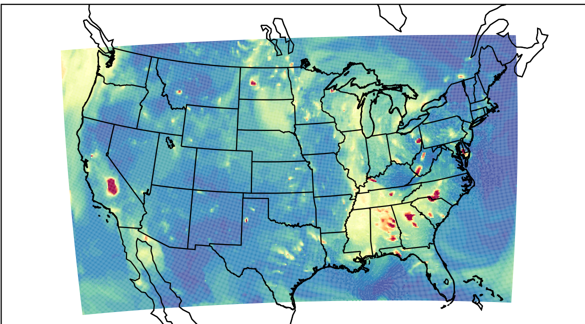
WRF 2021-10-02_03:00:00
