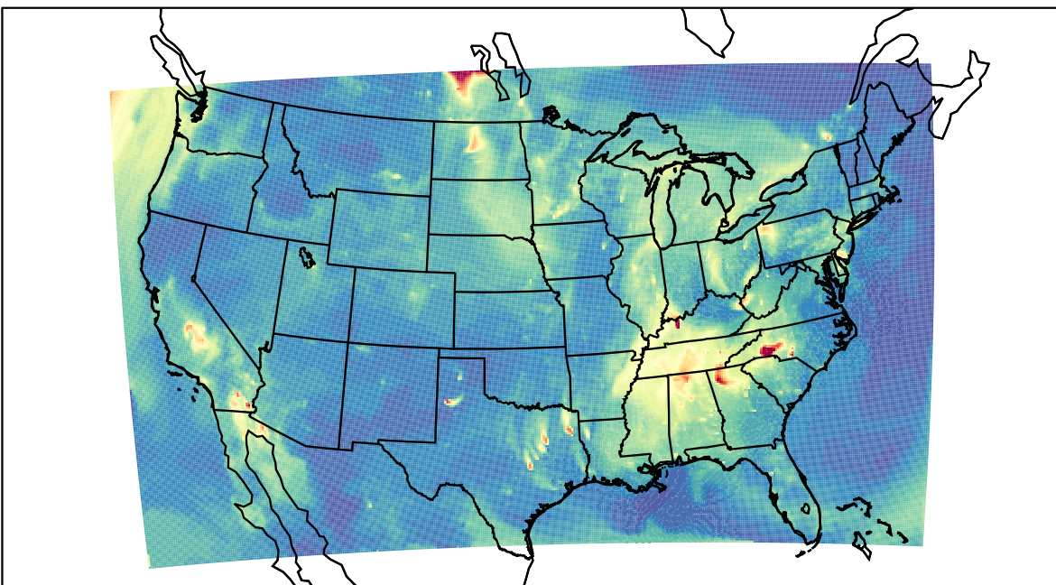
WRF 2021-10-02_11:00:00
