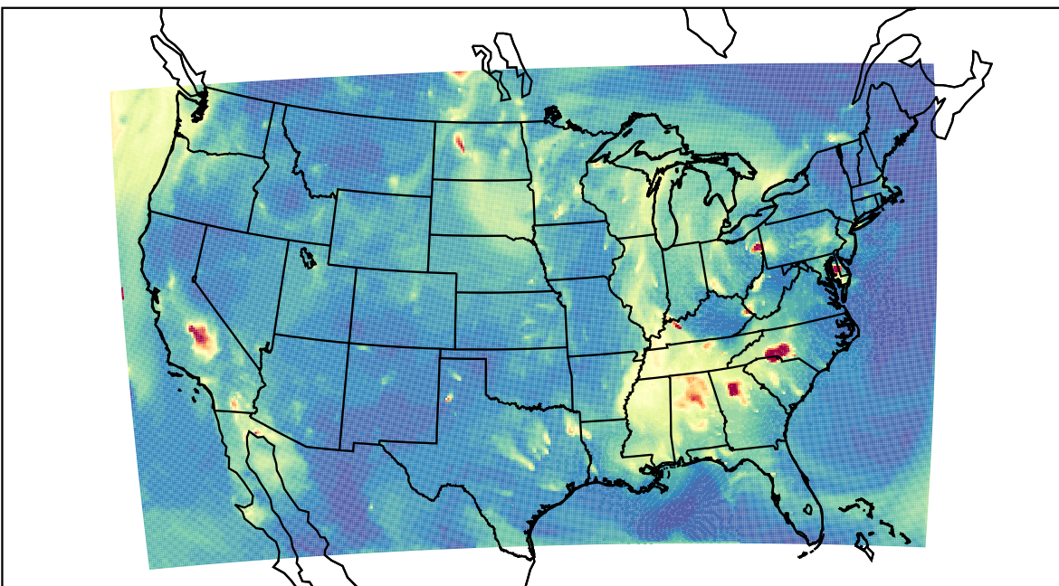
WRF 2021-10-02_06:00:00
