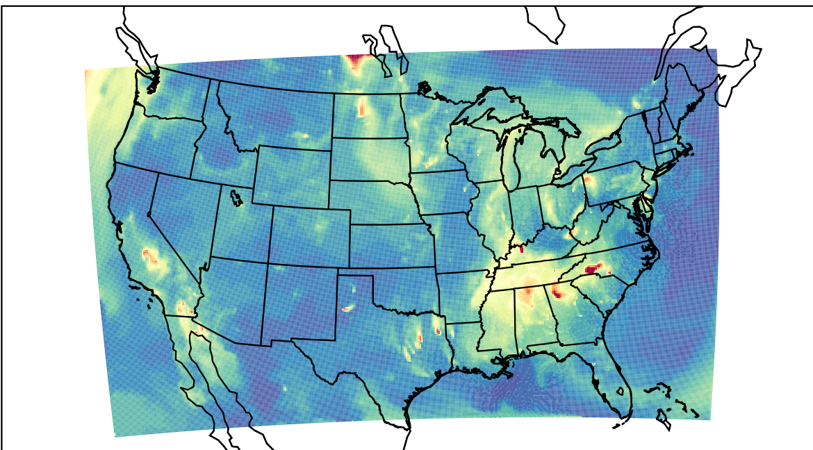
WRF 2021-10-02_10:00:00
