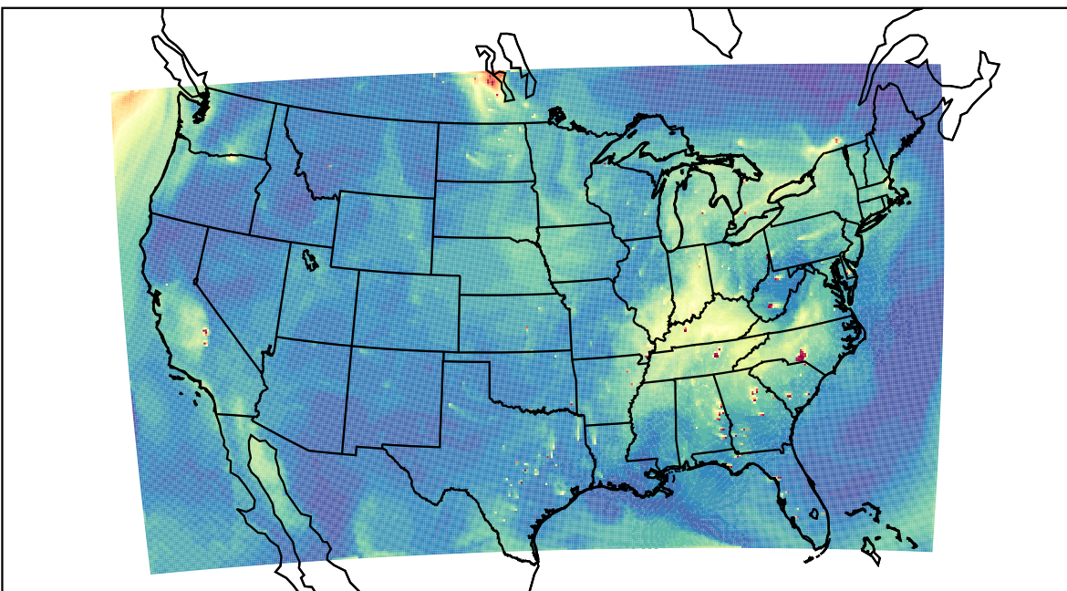
WRF 2021-10-02_21:00:00
