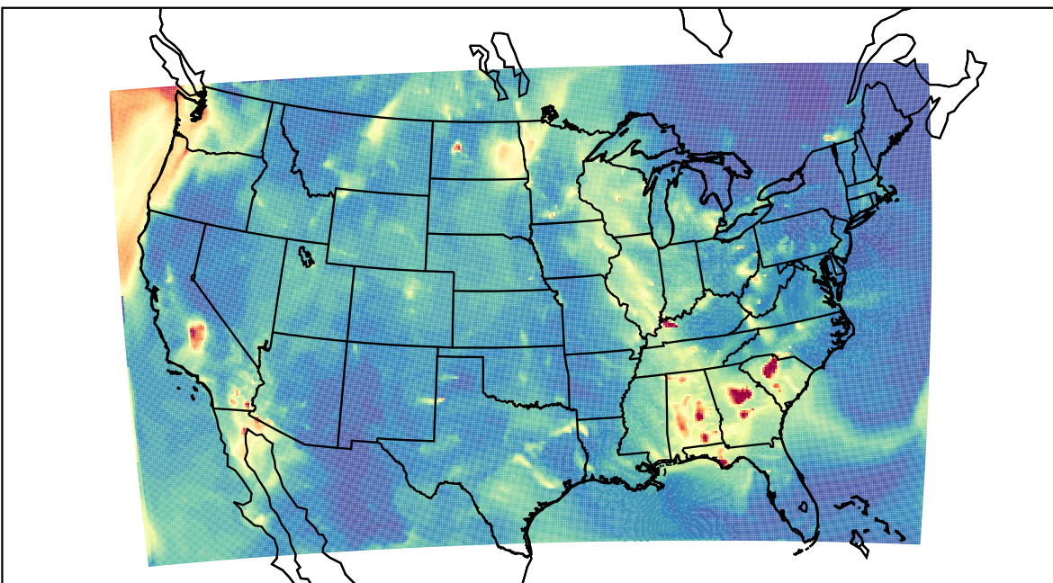
WRF 2021-10-01_06:00:00
