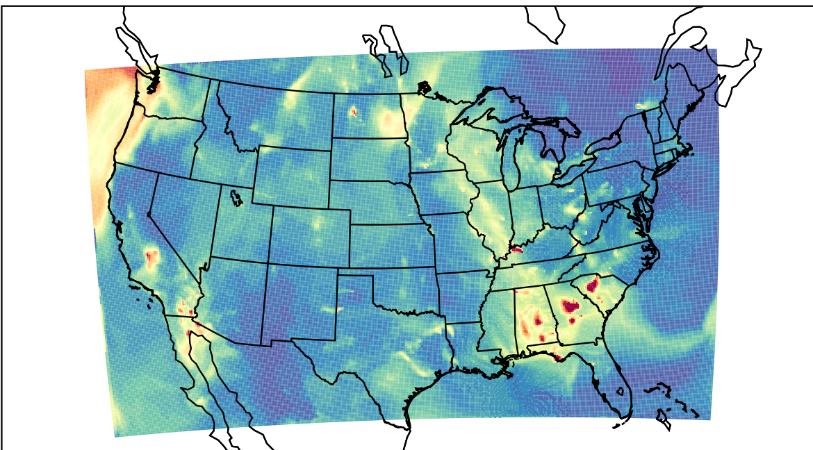
WRF 2021-10-01_07:00:00
