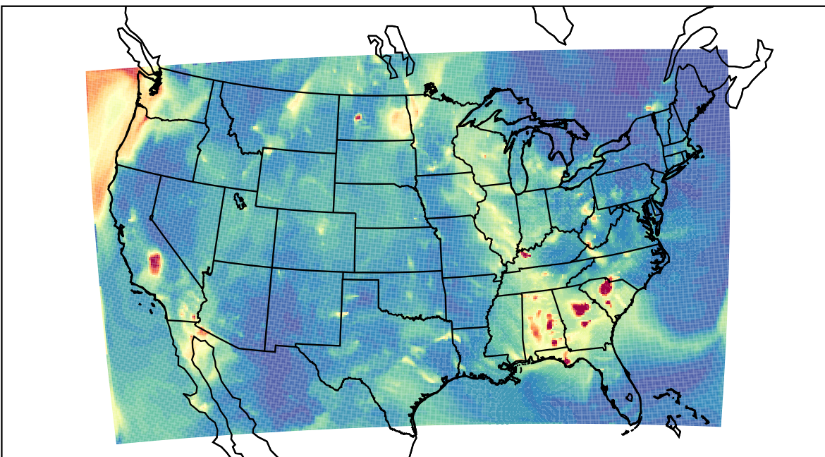
WRF 2021-10-01_05:00:00
