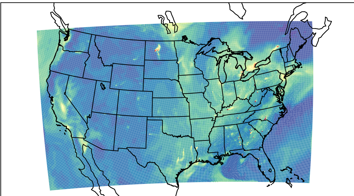
WRF 2021-10-04_18:00:00
