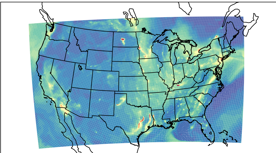
WRF 2021-10-04_13:00:00
