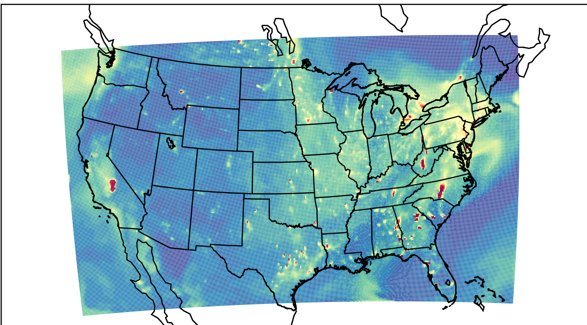
WRF 2021-10-04_01:00:00
