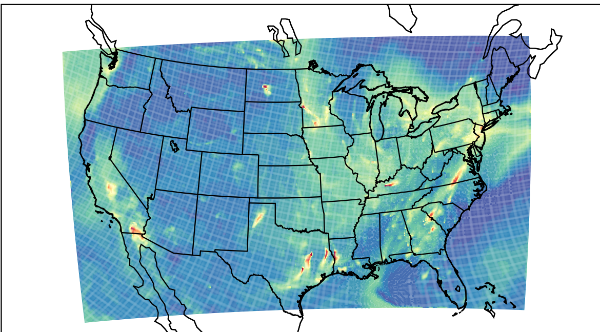
WRF 2021-10-04_09:00:00
