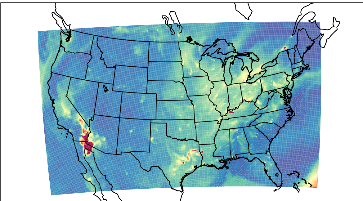
WRF 2021-10-05_14:00:00
