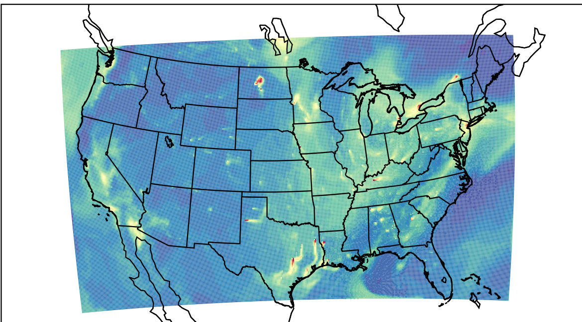
WRF 2021-10-04_16:00:00
