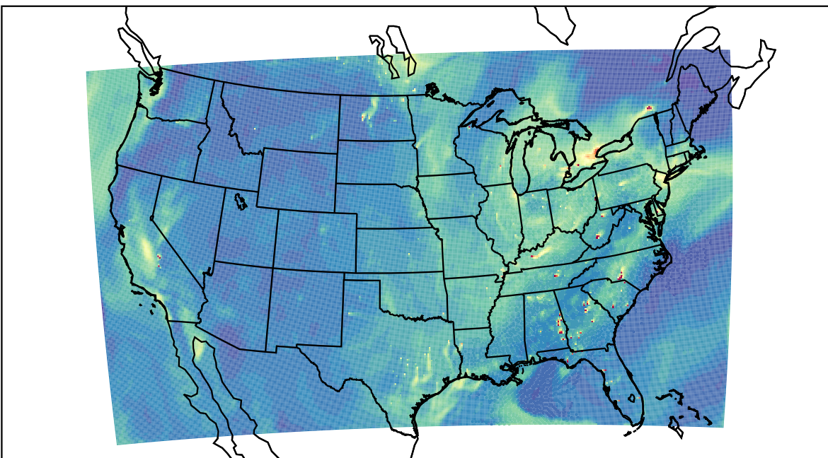
WRF 2021-10-04_20:00:00
