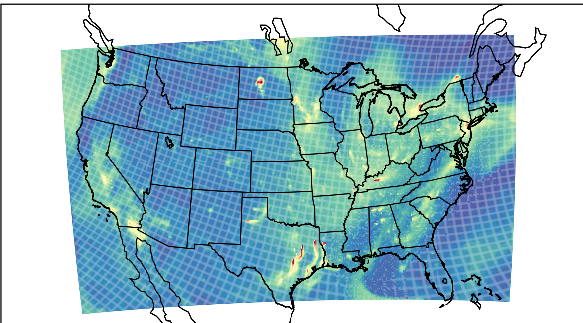
WRF 2021-10-04_15:00:00
