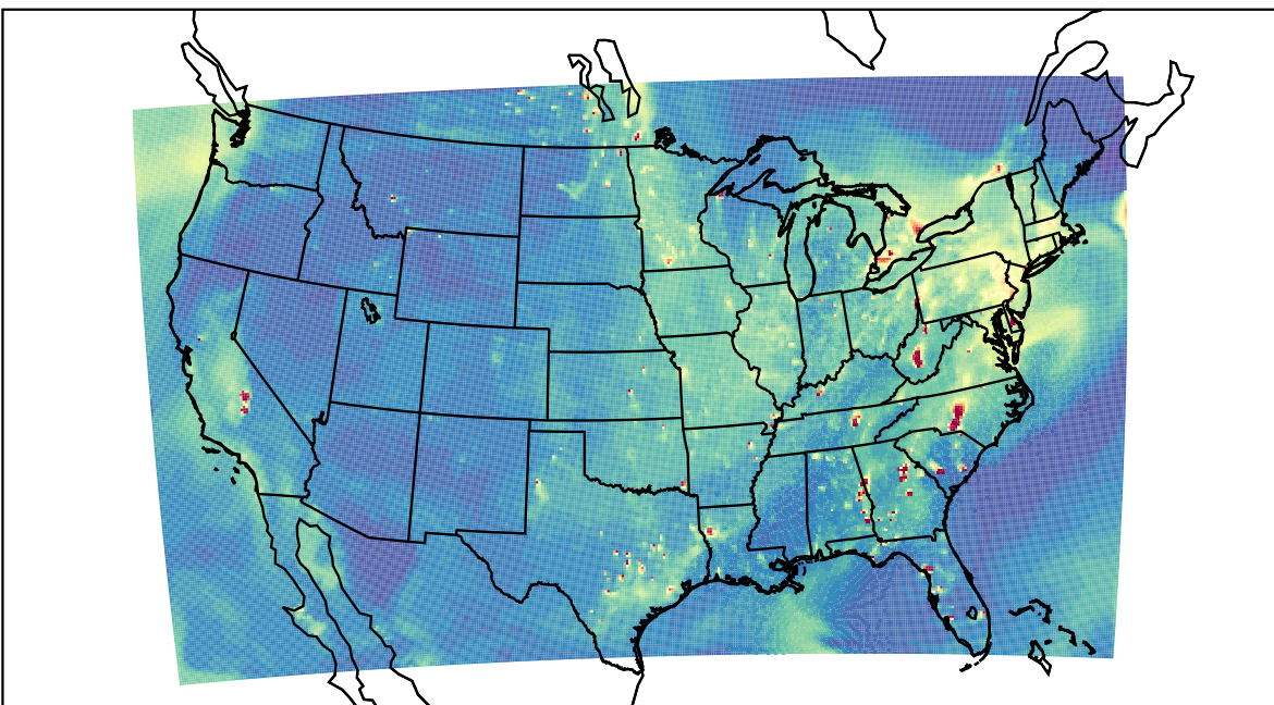
WRF 2021-10-04_00:00:00
