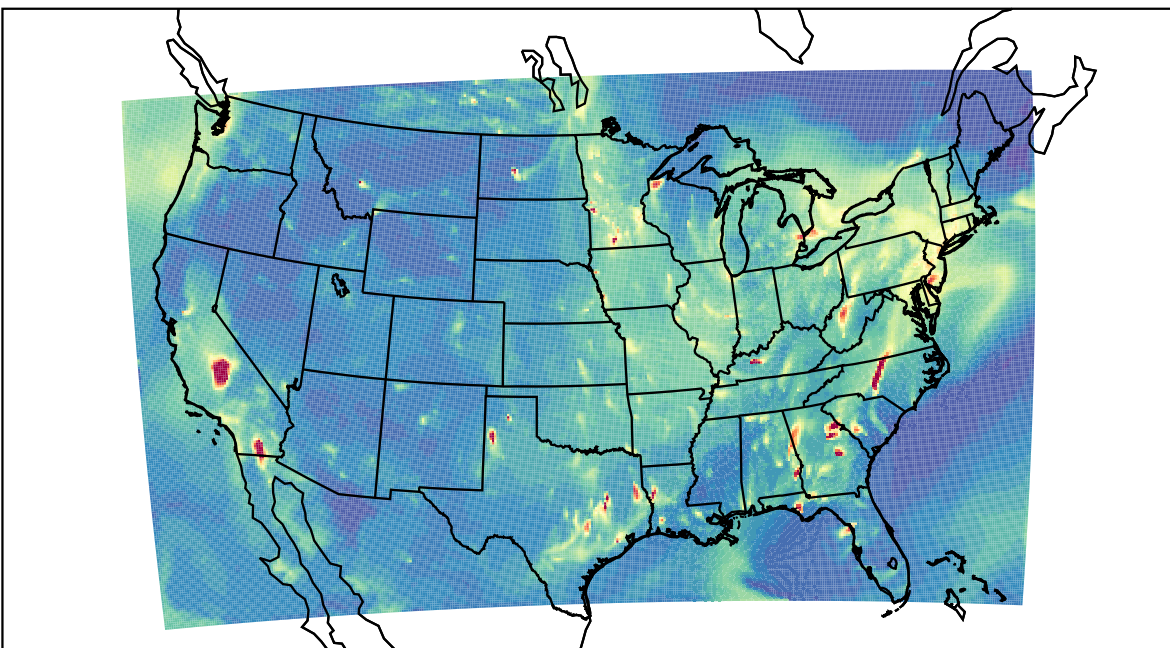
WRF 2021-10-04_04:00:00
