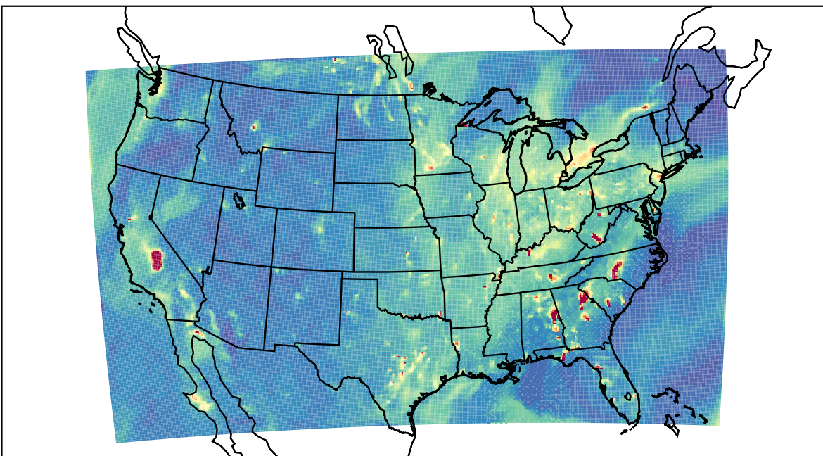
WRF 2021-10-05_02:00:00
