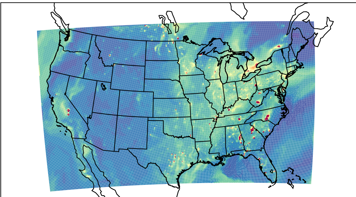
WRF 2021-10-05_00:00:00
