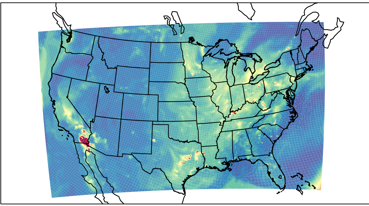
WRF 2021-10-05_10:00:00
