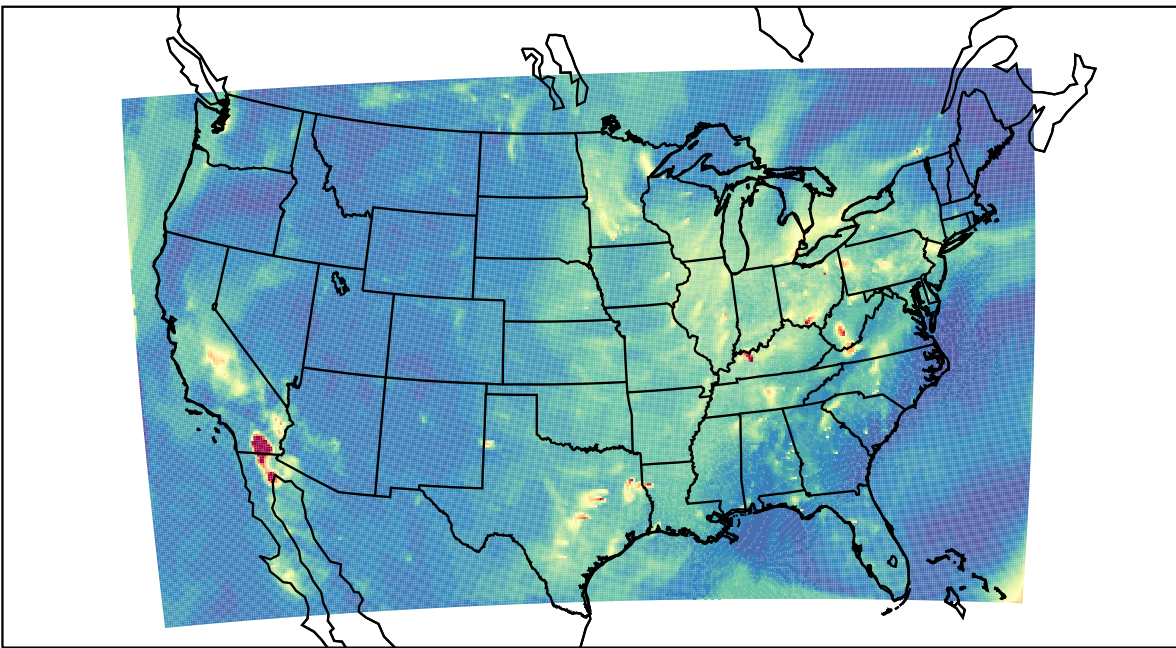
WRF 2021-10-05_08:00:00
