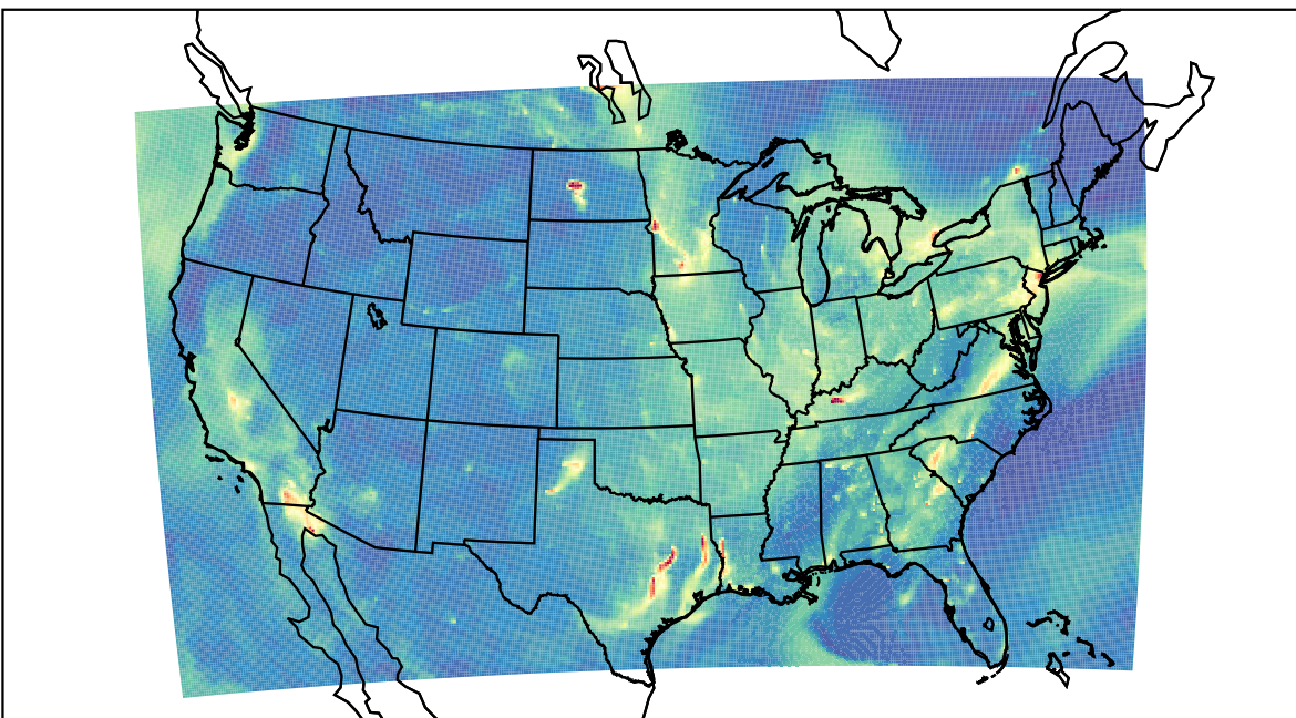
WRF 2021-10-04_12:00:00
