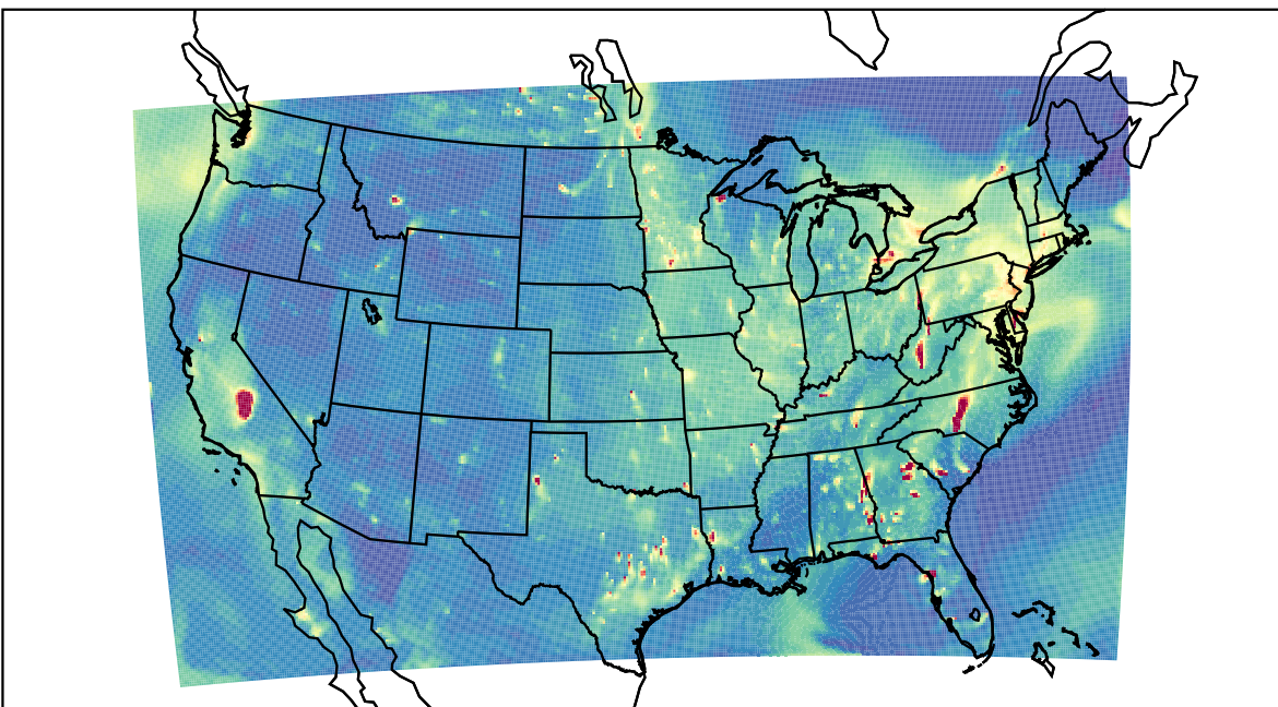
WRF 2021-10-04_02:00:00
