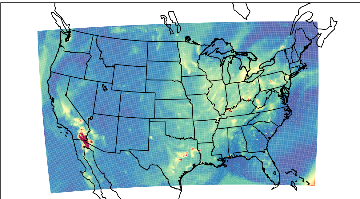
WRF 2021-10-05_11:00:00
