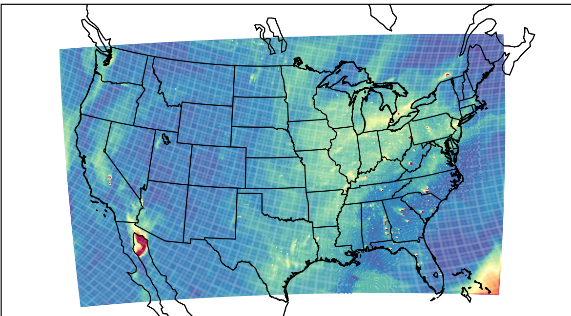
WRF 2021-10-05_20:00:00
