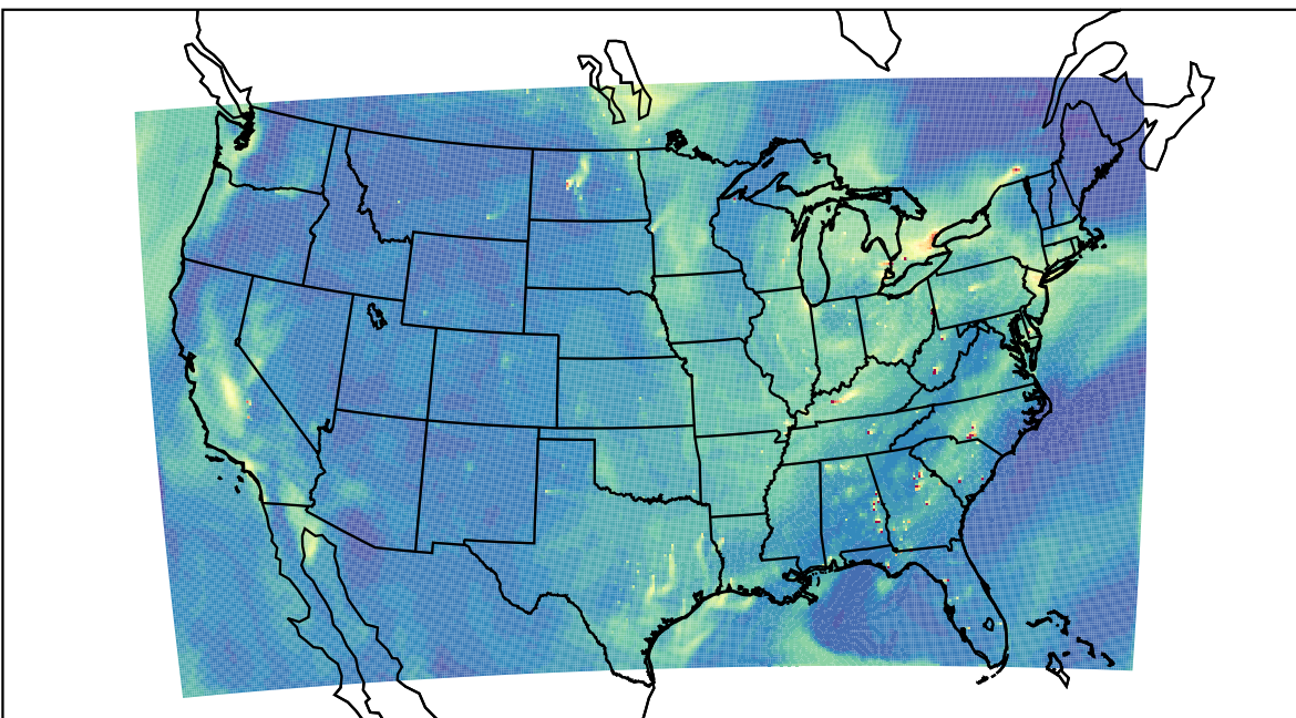
WRF 2021-10-04_19:00:00
