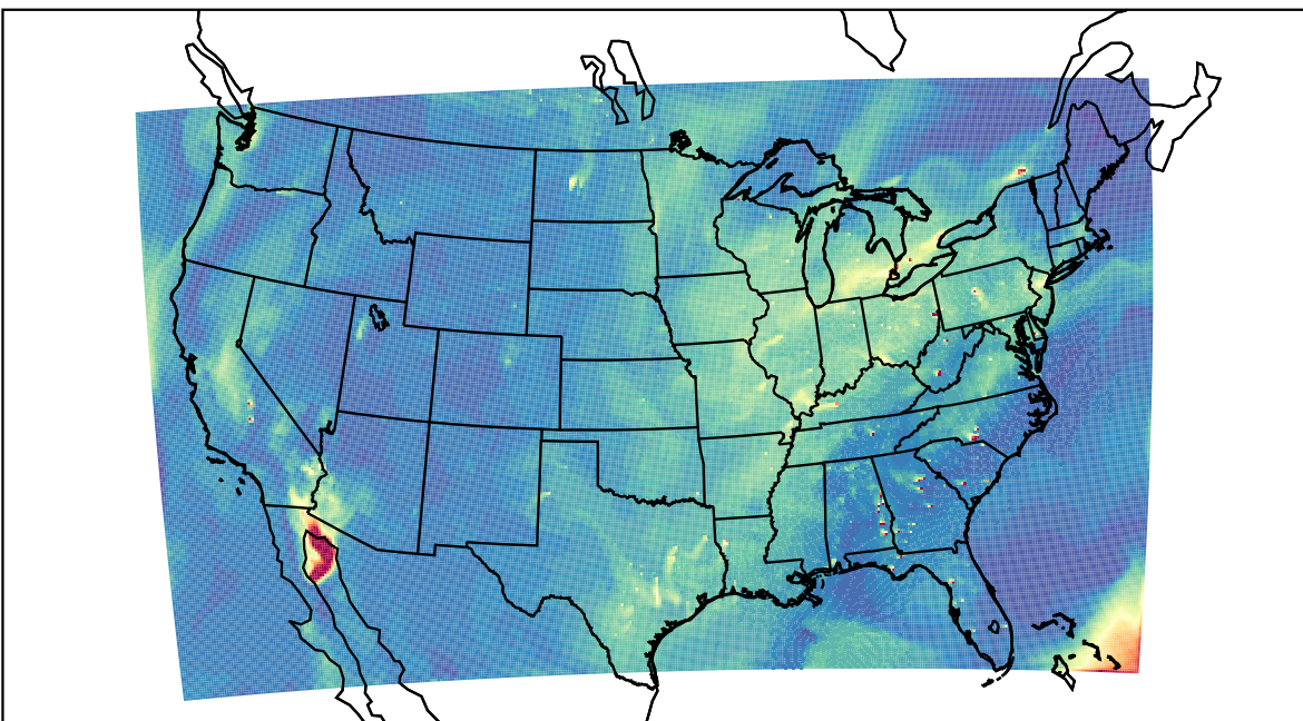
WRF 2021-10-05_19:00:00
