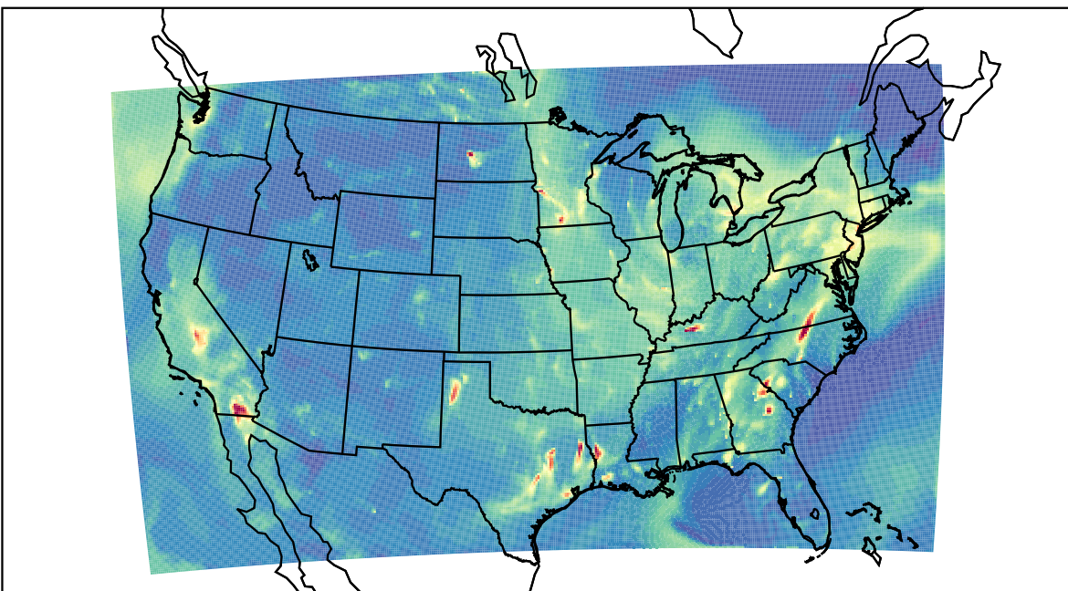
WRF 2021-10-04_07:00:00
