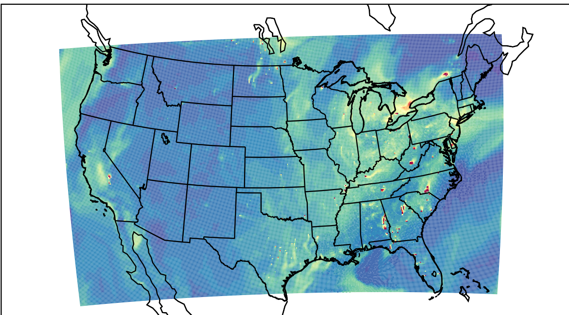
WRF 2021-10-04_22:00:00
