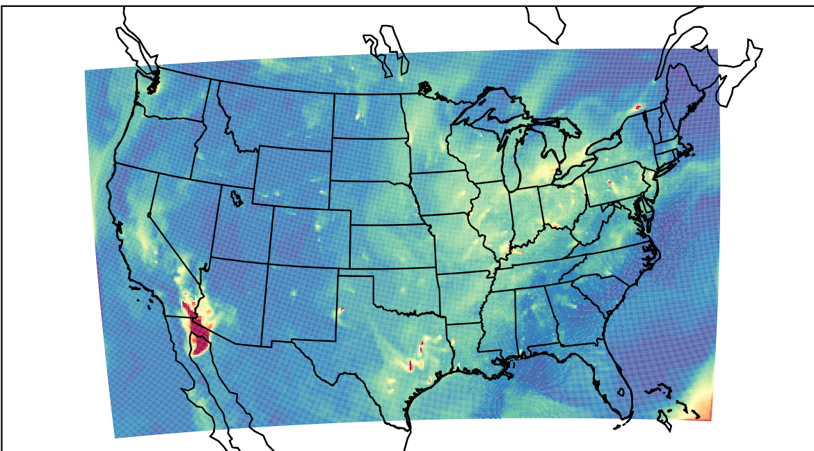
WRF 2021-10-05_16:00:00
