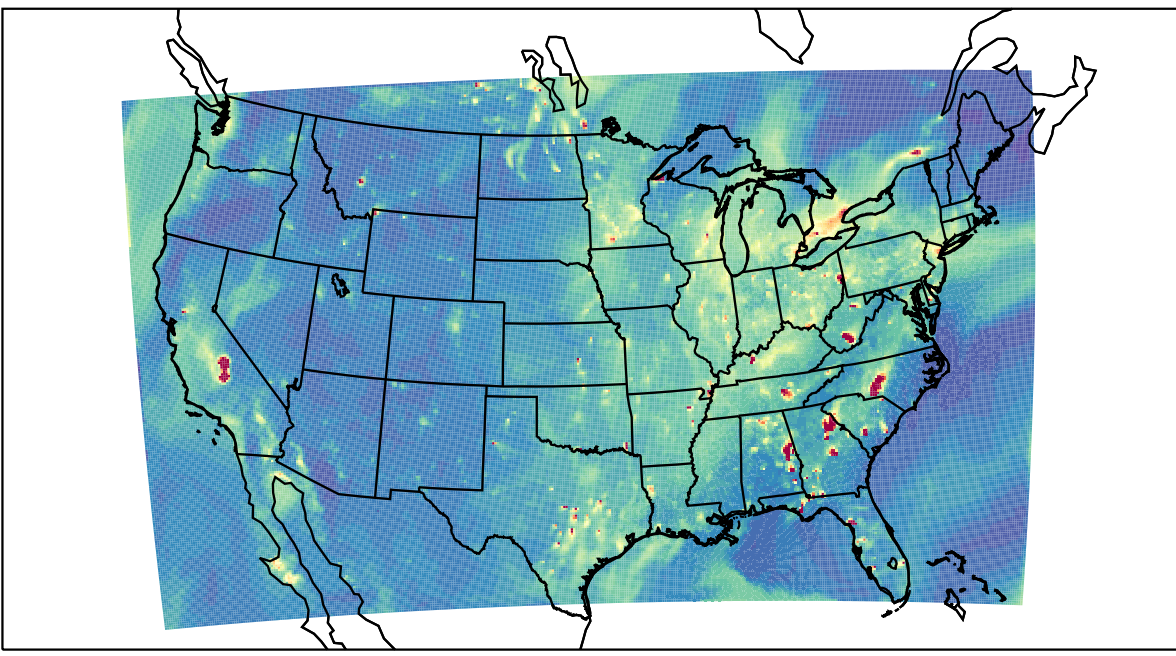
WRF 2021-10-05_01:00:00
