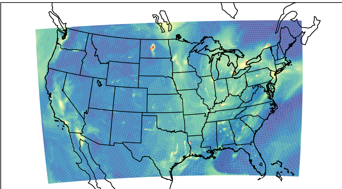
WRF 2021-10-04_17:00:00
