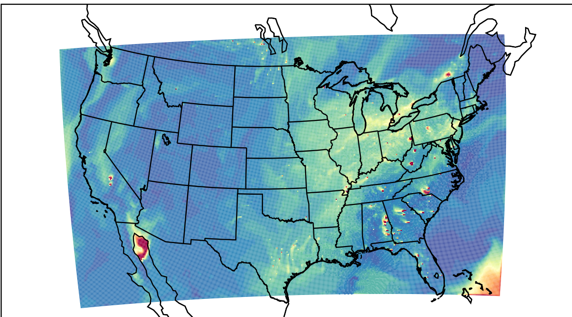
WRF 2021-10-05_22:00:00
