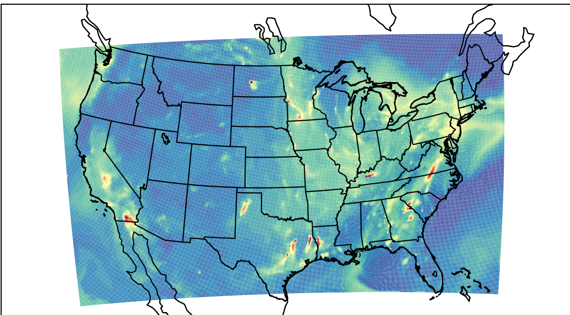
WRF 2021-10-04_08:00:00
