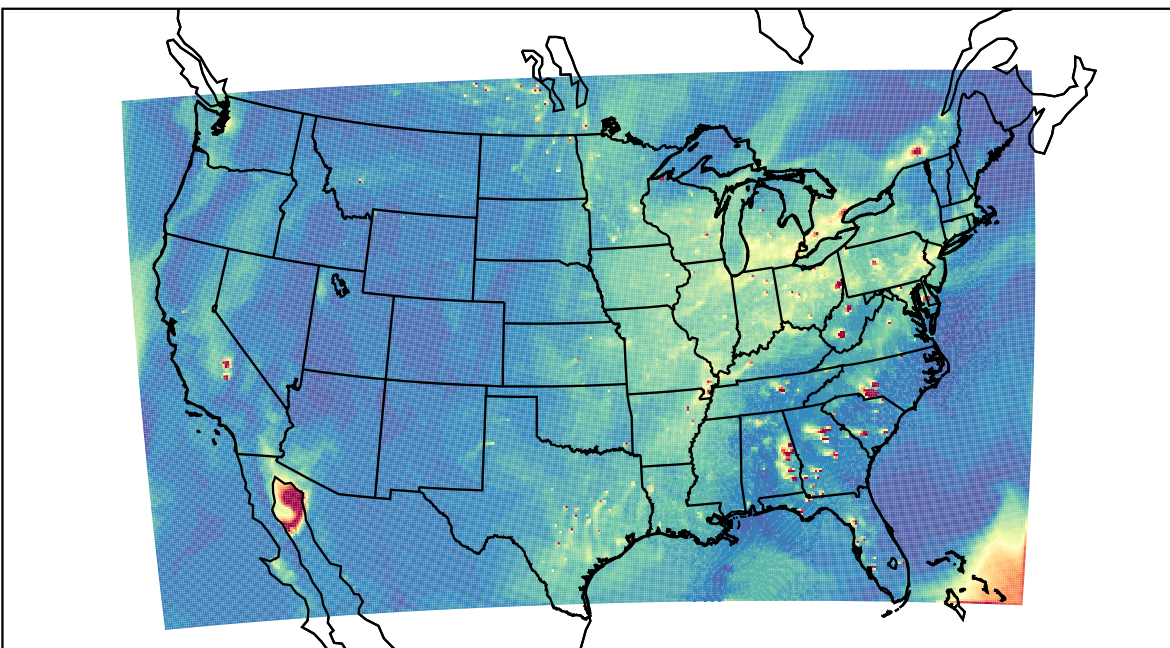
WRF 2021-10-05_23:00:00
