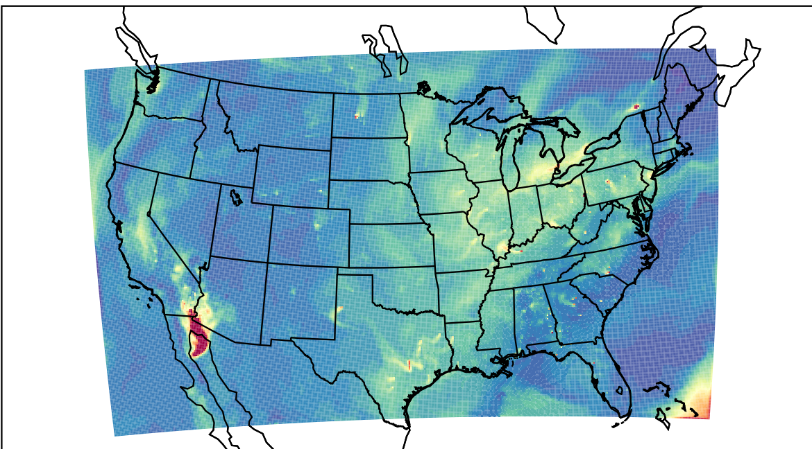
WRF 2021-10-05_17:00:00
