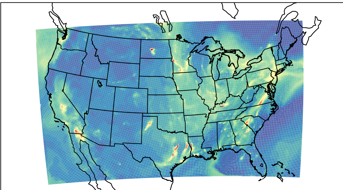
WRF 2021-10-04_10:00:00
