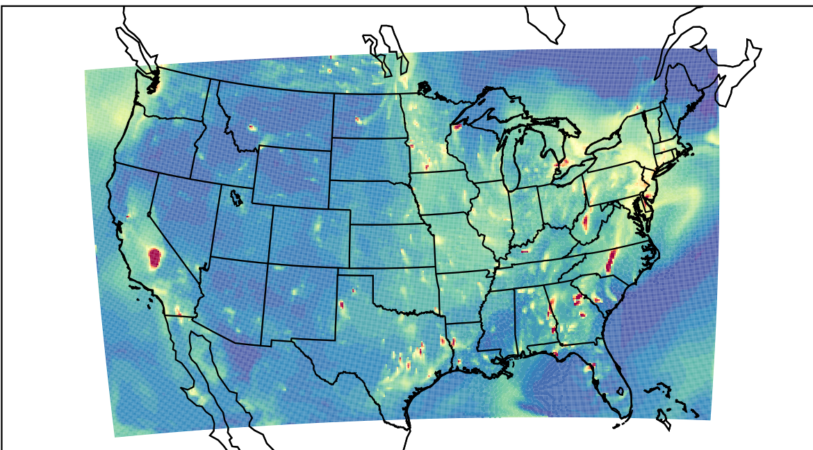
WRF 2021-10-04_03:00:00
