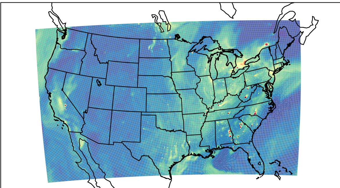
WRF 2021-10-04_21:00:00
