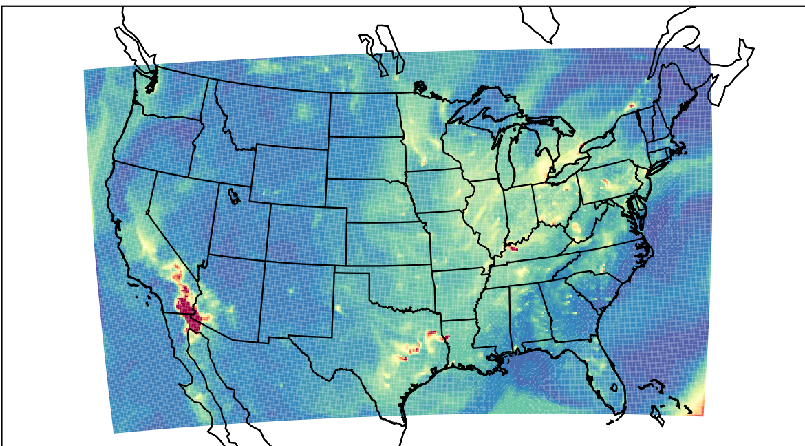
WRF 2021-10-05_12:00:00
