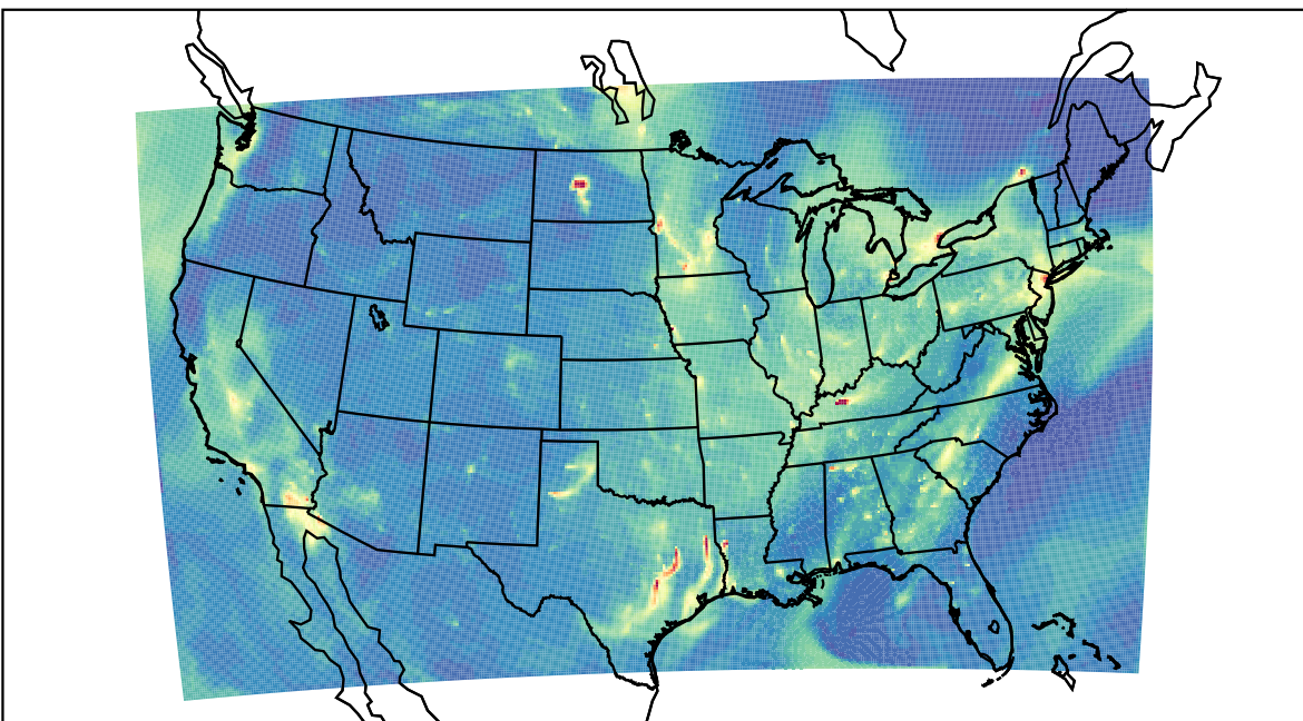
WRF 2021-10-04_14:00:00
