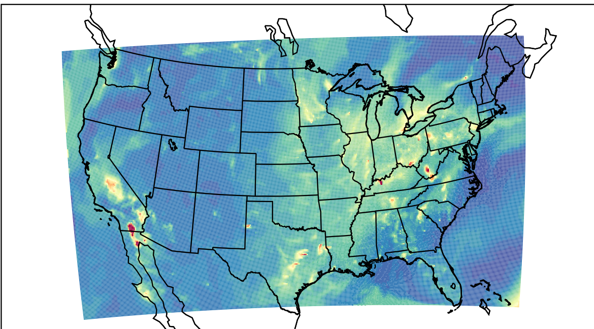
WRF 2021-10-05_07:00:00
