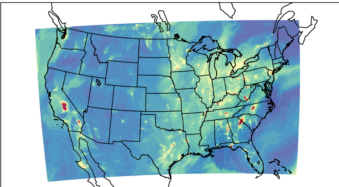
WRF 2021-10-05_04:00:00
