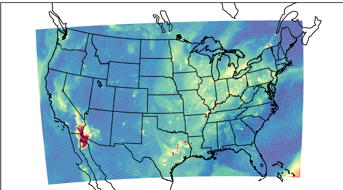
WRF 2021-10-05_15:00:00
