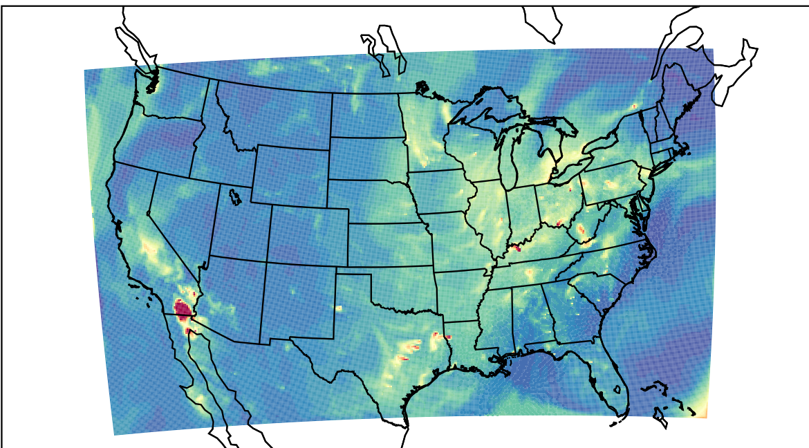
WRF 2021-10-05_09:00:00
