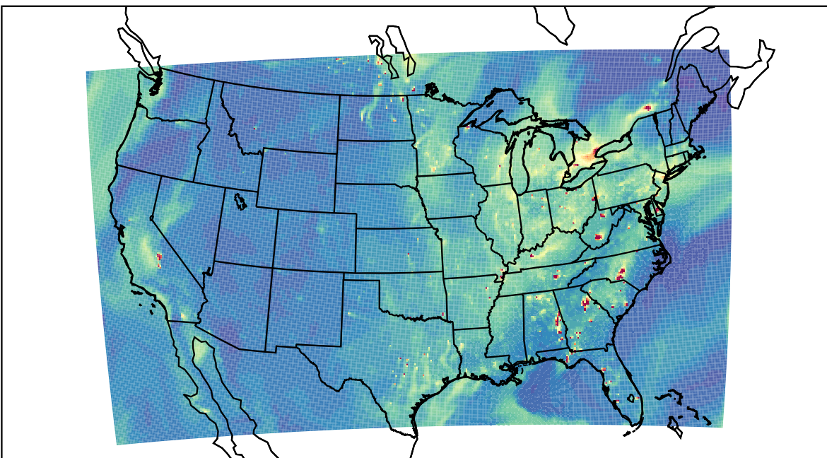
WRF 2021-10-04_23:00:00
