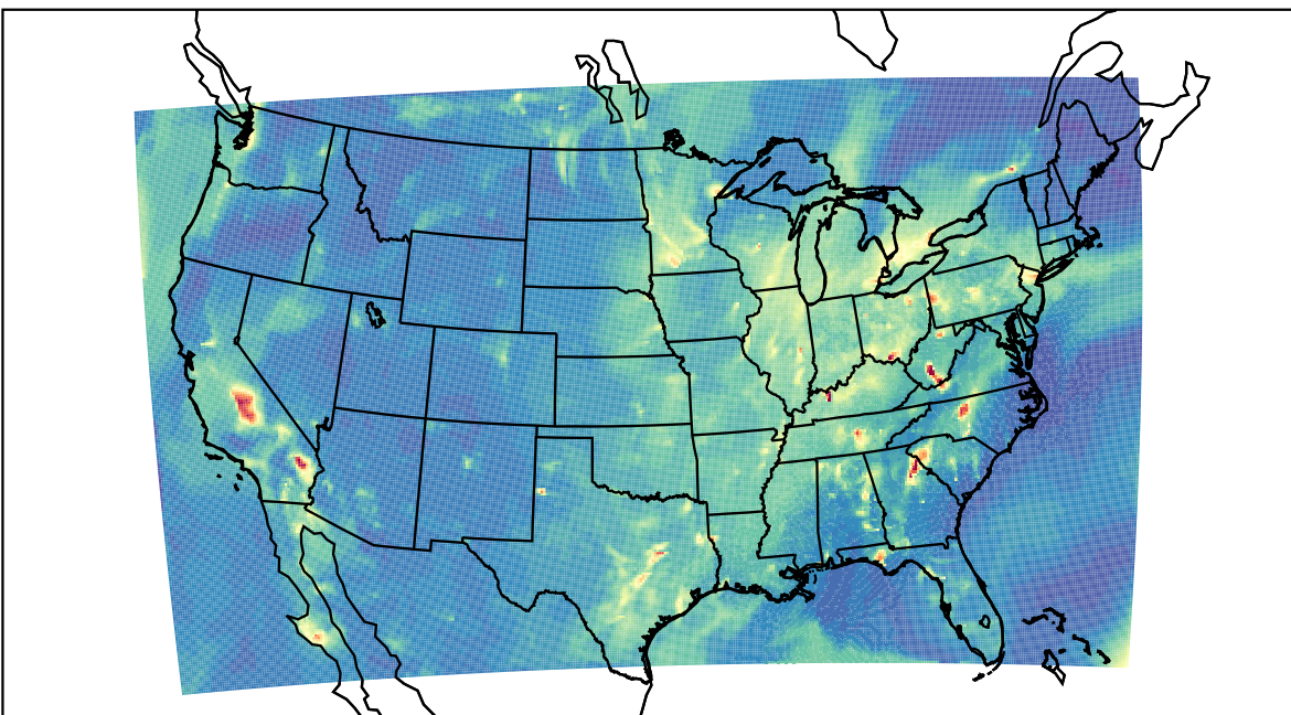
WRF 2021-10-05_05:00:00
