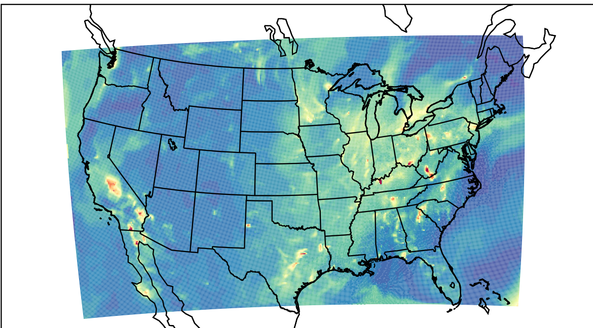
WRF 2021-10-05_06:00:00
