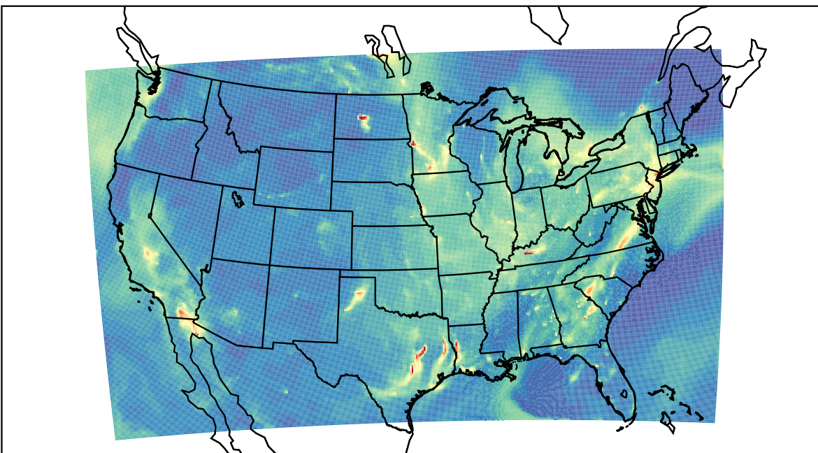
WRF 2021-10-04_11:00:00
