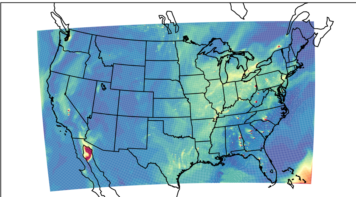
WRF 2021-10-05_21:00:00
