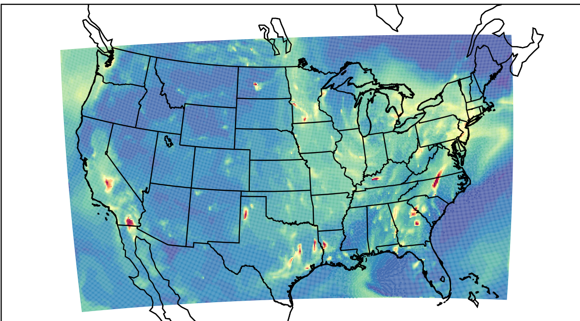
WRF 2021-10-04_06:00:00
