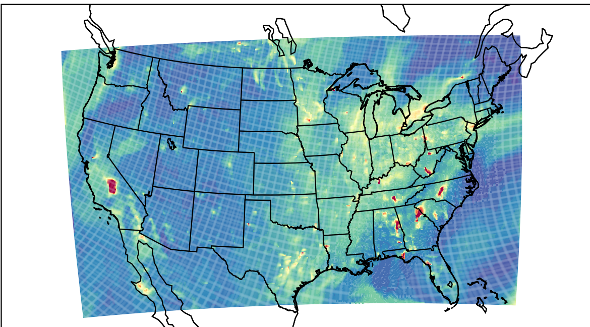
WRF 2021-10-05_03:00:00
