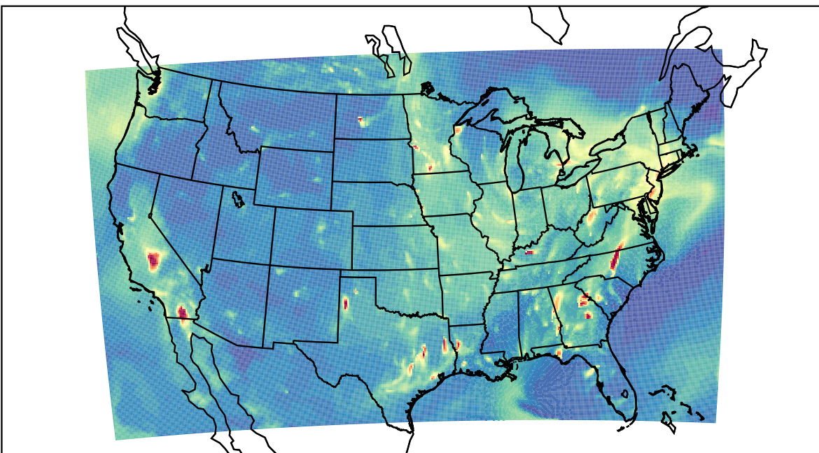
WRF 2021-10-04_05:00:00
