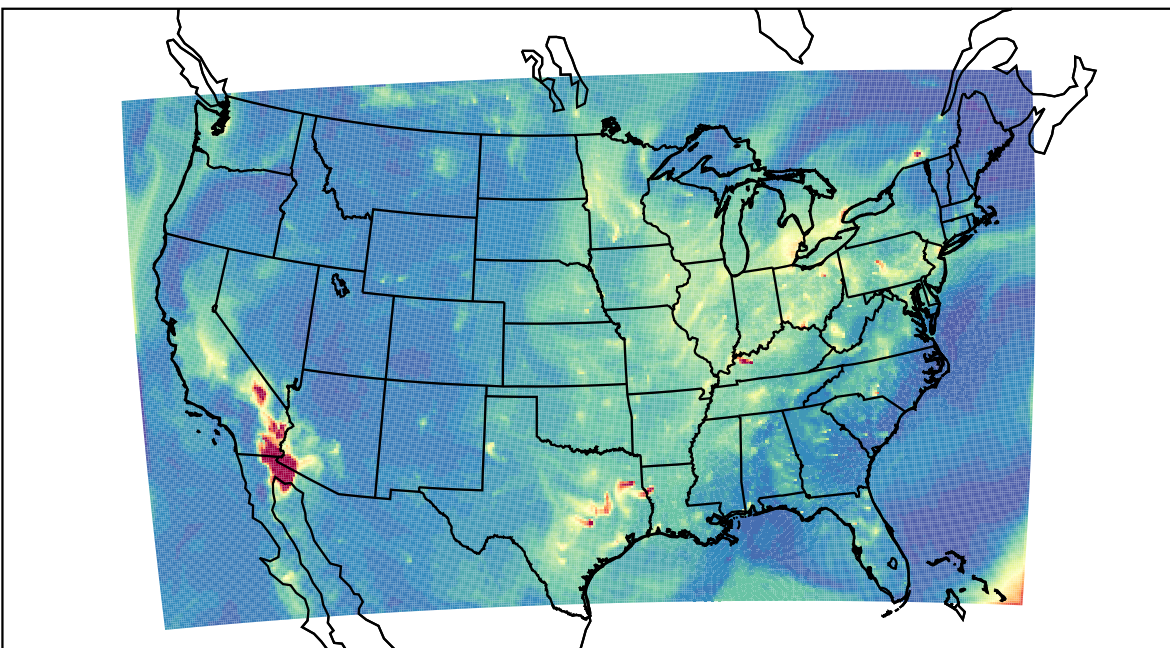
WRF 2021-10-05_13:00:00
