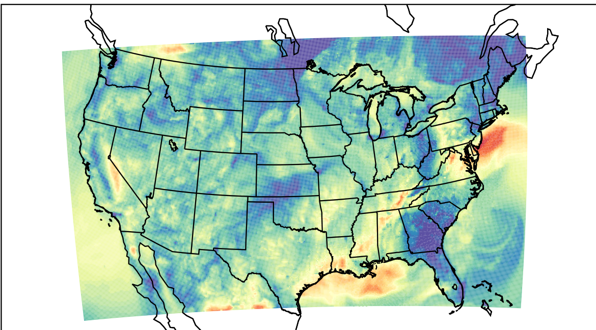
WRF (2021-10-09_11:00:00)
