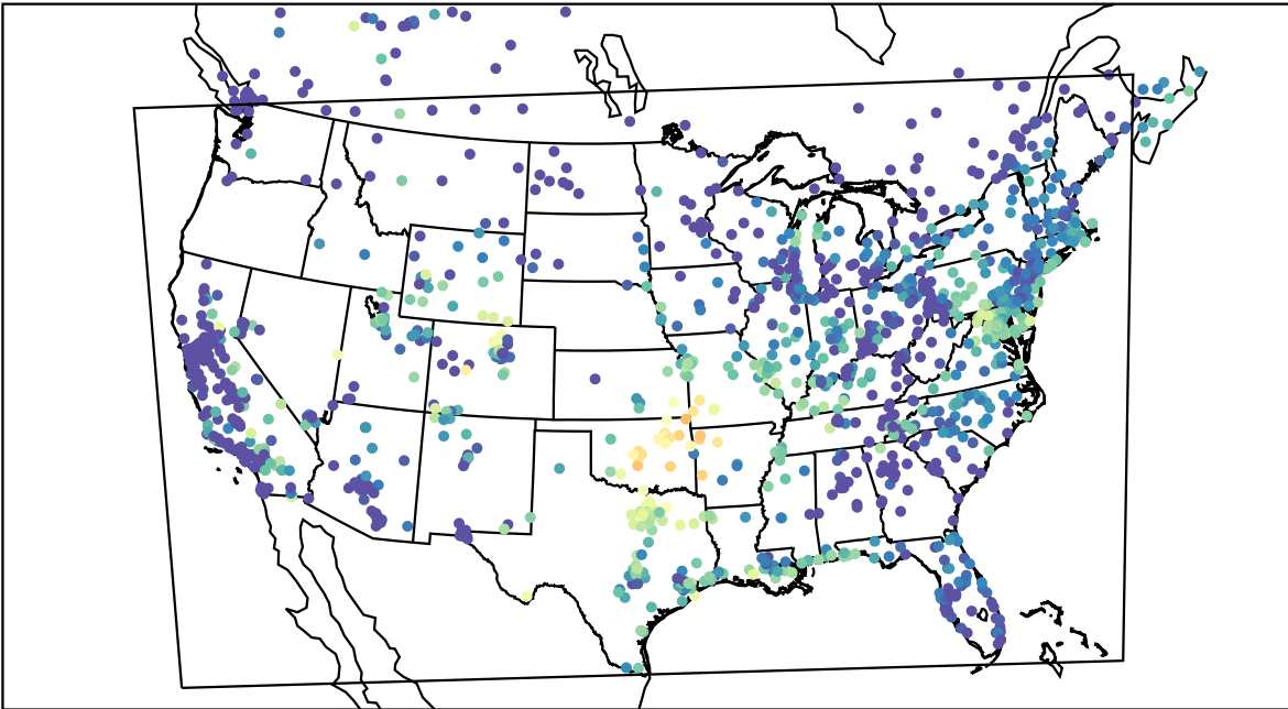
AirNOW (2021-10-09_14:00:00)
