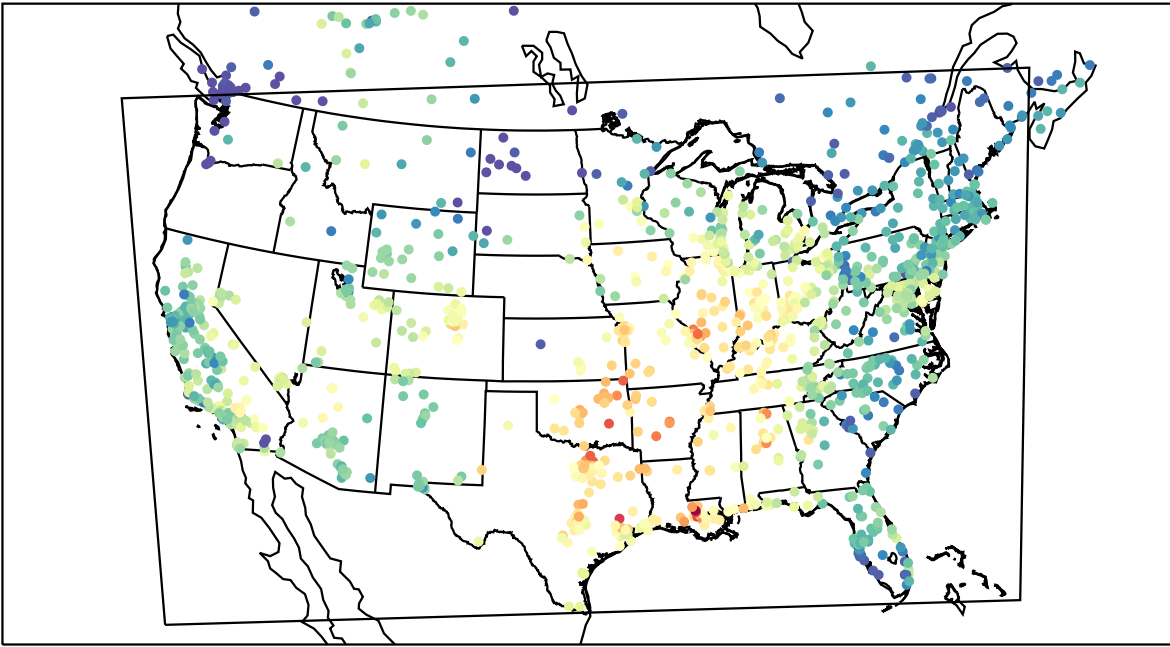
AirNOW (2021-10-09_18:00:00)
