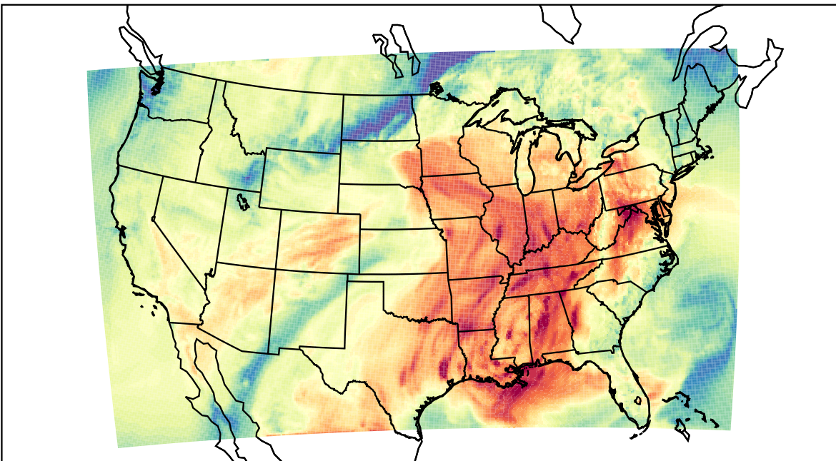
WRF (2021-10-09_20:00:00)
