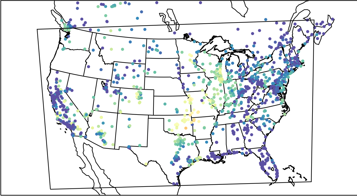
AirNOW (2021-10-10_08:00:00)
