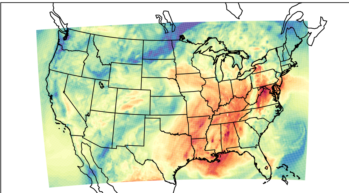
WRF (2021-10-09_17:00:00)
