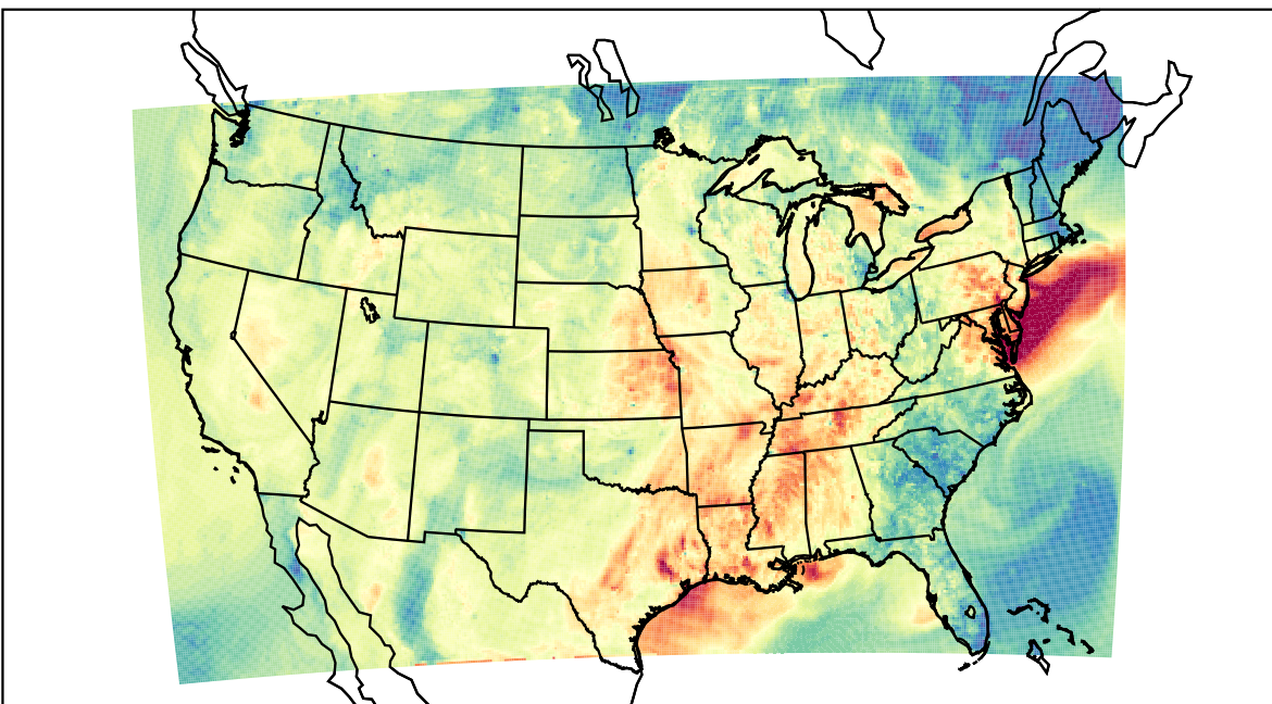
WRF (2021-10-09_00:00:00)
