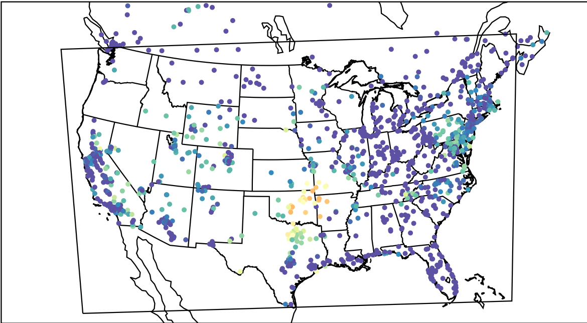
AirNOW (2021-10-09_10:00:00)
