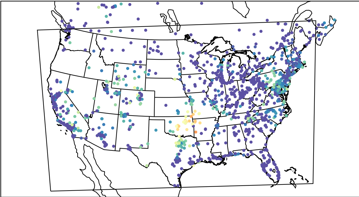
AirNOW (2021-10-09_12:00:00)
