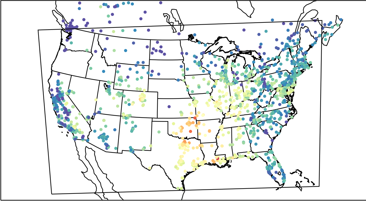
AirNOW (2021-10-09_16:00:00)
