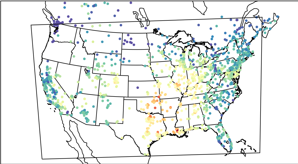
AirNOW (2021-10-09_17:00:00)
