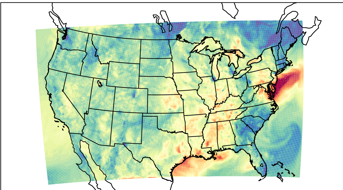
WRF (2021-10-09_03:00:00)
