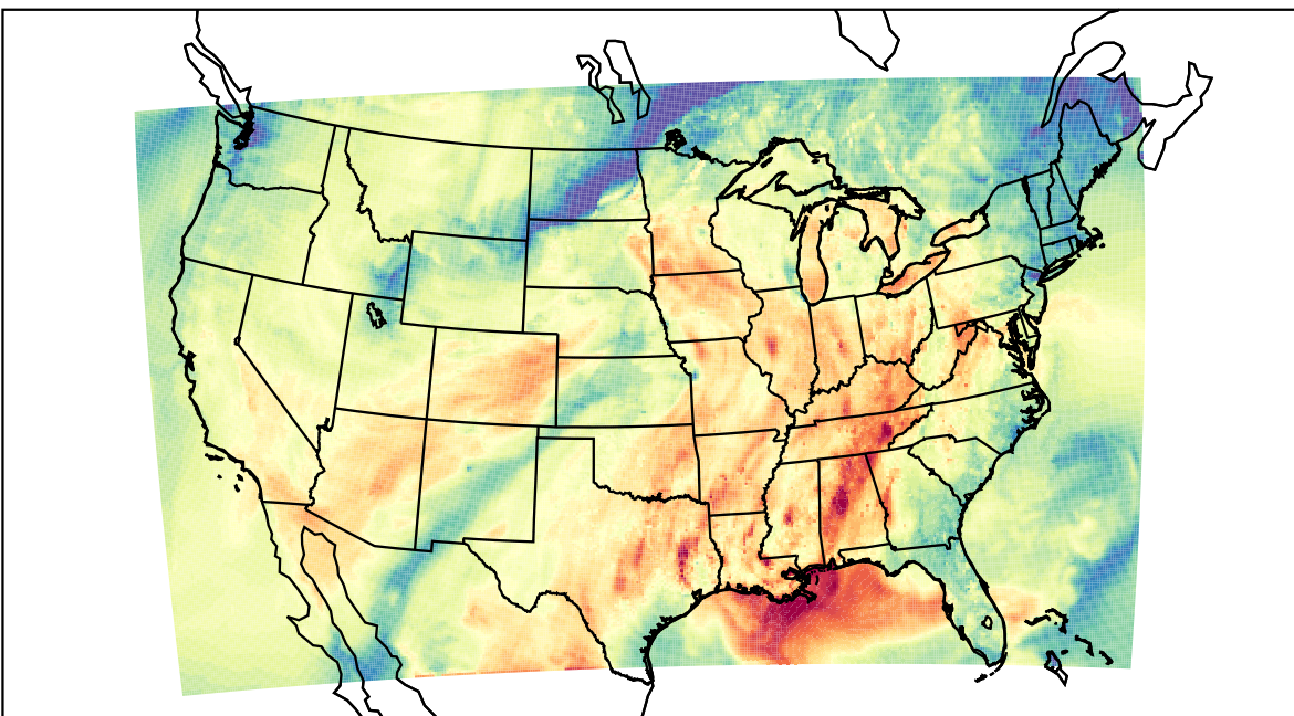
WRF (2021-10-09_23:00:00)
