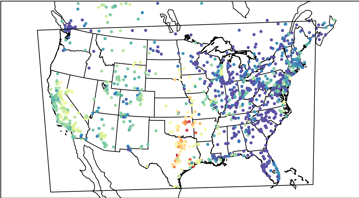
AirNOW (2021-10-09_00:00:00)
