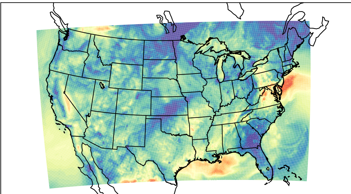
WRF (2021-10-09_13:00:00)
