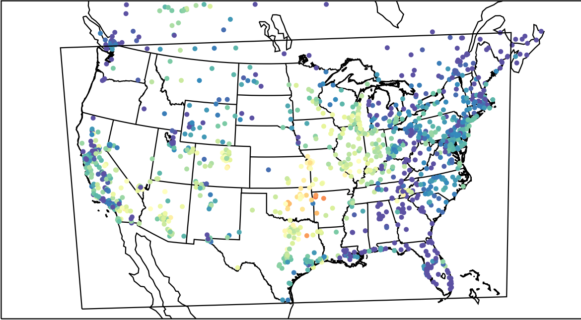
AirNOW (2021-10-10_03:00:00)
