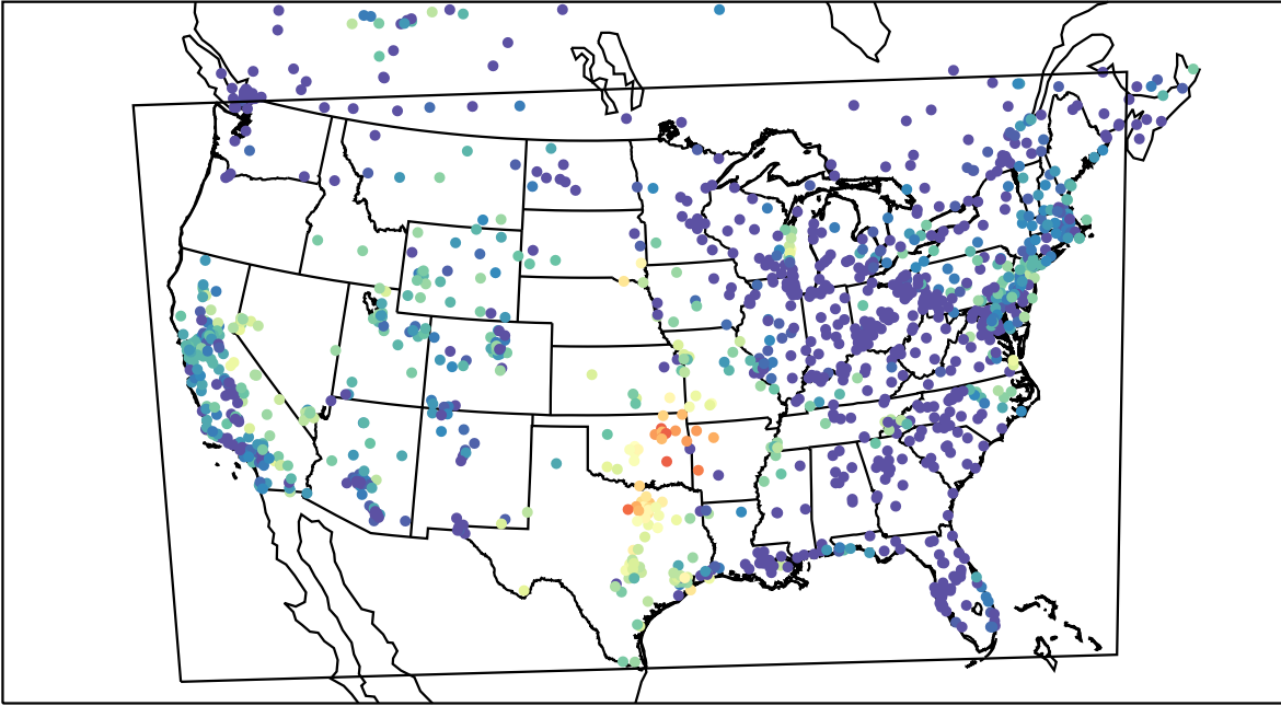
AirNOW (2021-10-09_04:00:00)
