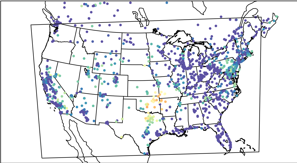
AirNOW (2021-10-09_09:00:00)
