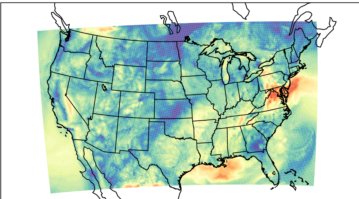
WRF (2021-10-09_14:00:00)
