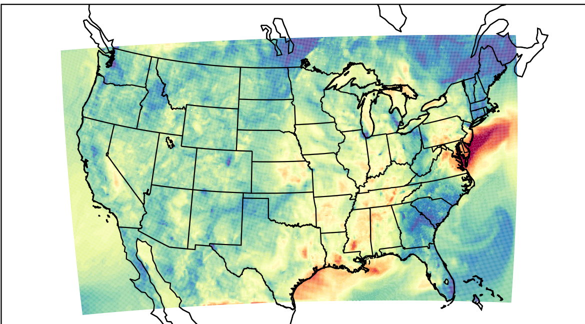
WRF (2021-10-09_04:00:00)
