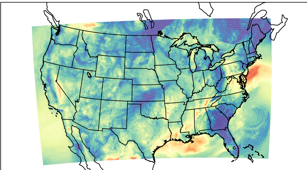
WRF (2021-10-09_12:00:00)
