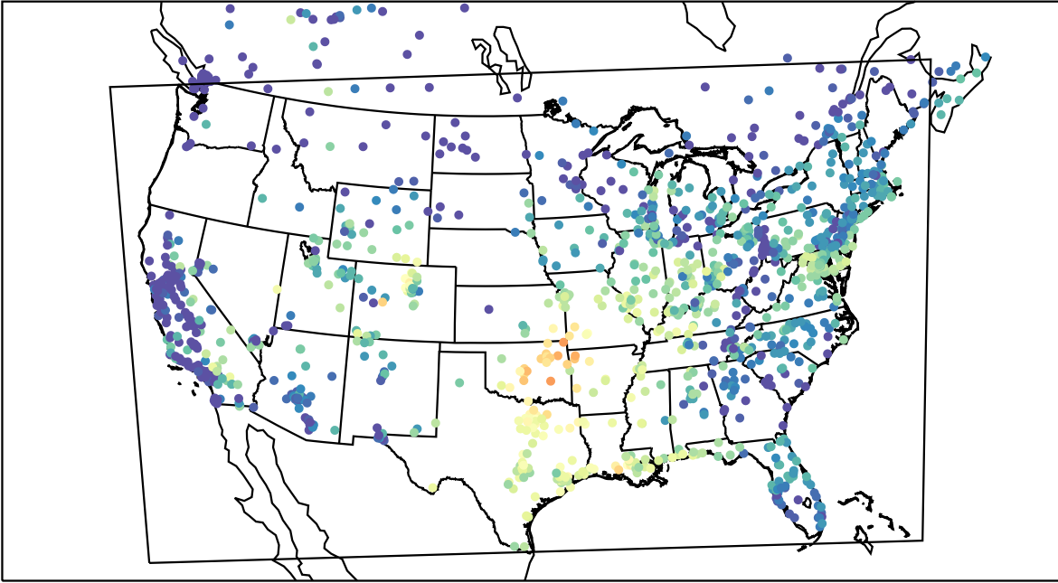
AirNOW (2021-10-09_15:00:00)
