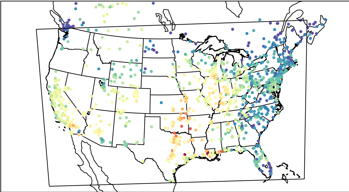
AirNOW (2021-10-09_22:00:00)
