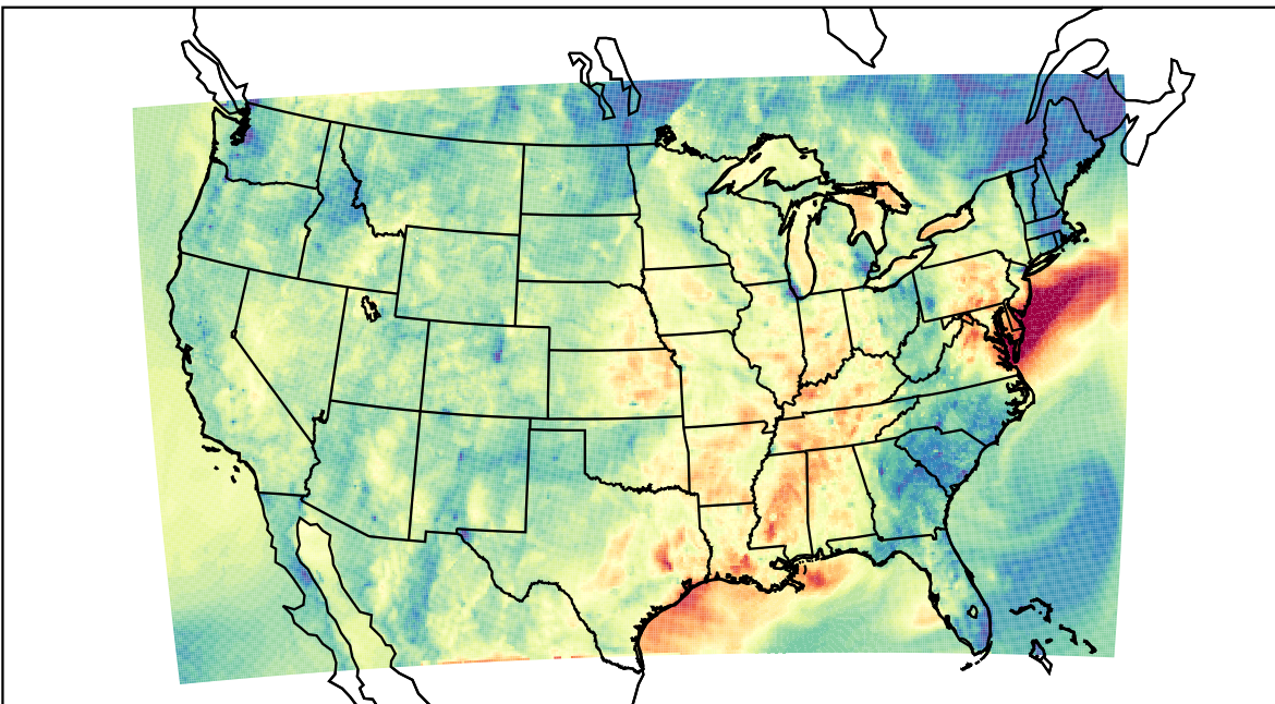
WRF (2021-10-09_02:00:00)
