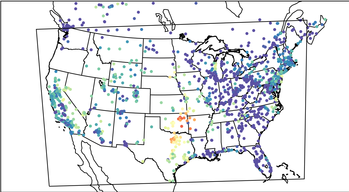
AirNOW (2021-10-09_03:00:00)
