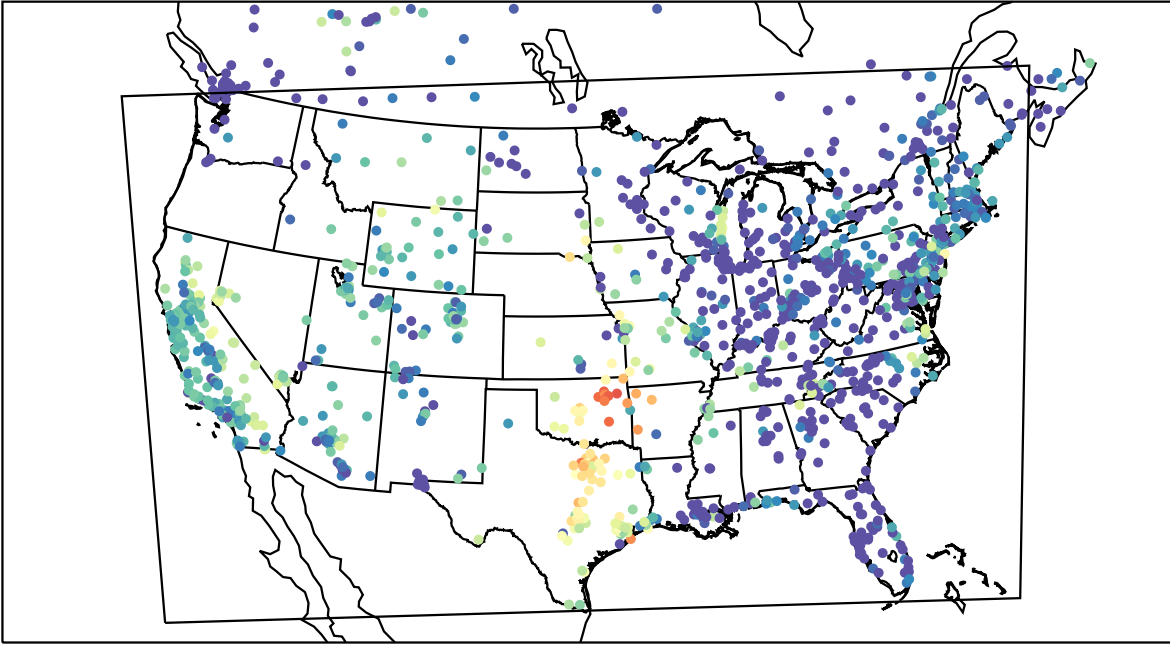
AirNOW (2021-10-09_02:00:00)
