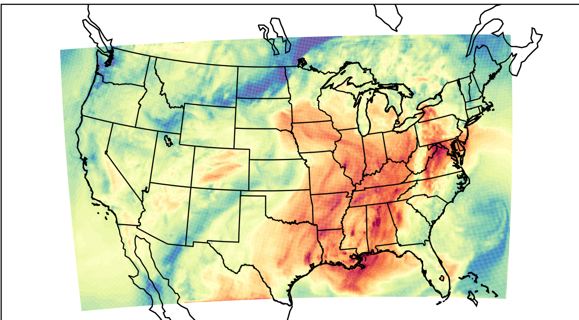
WRF (2021-10-09_18:00:00)
