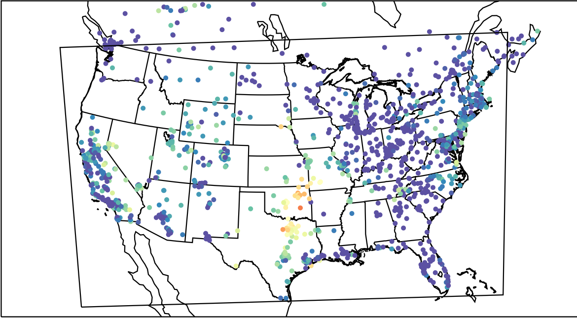
AirNOW (2021-10-09_06:00:00)
