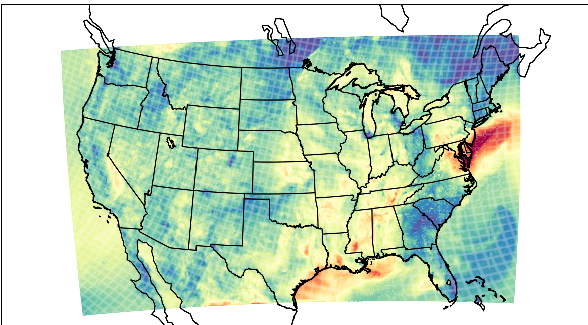
WRF (2021-10-09_05:00:00)
