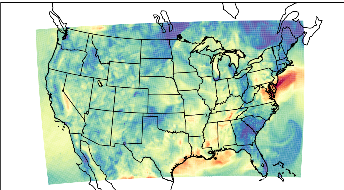
WRF (2021-10-09_07:00:00)
