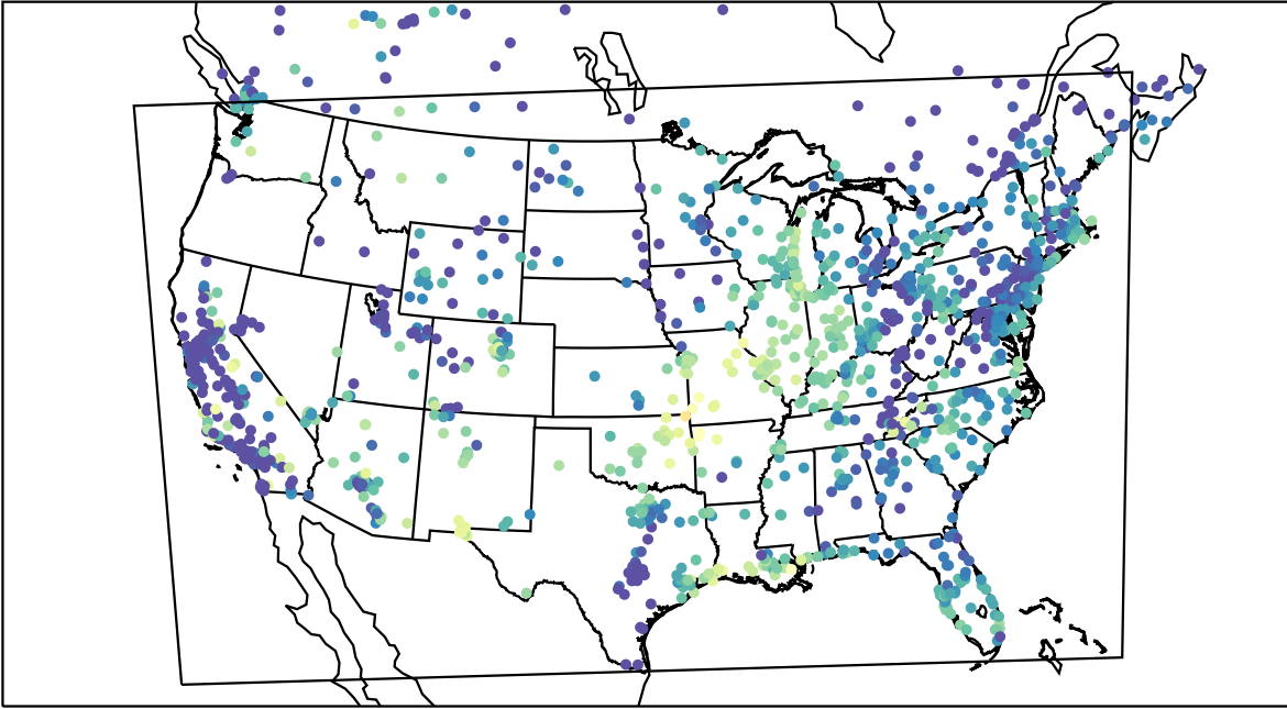
AirNOW (2021-10-10_14:00:00)
