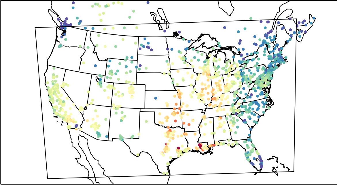
AirNOW (2021-10-09_21:00:00)
