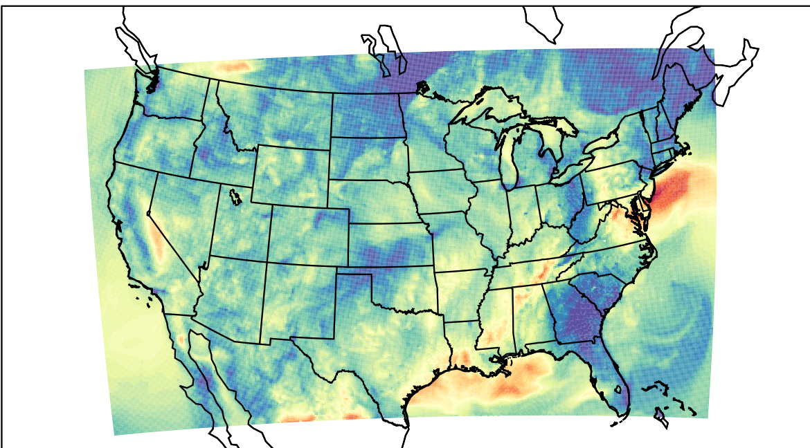
WRF (2021-10-09_10:00:00)
