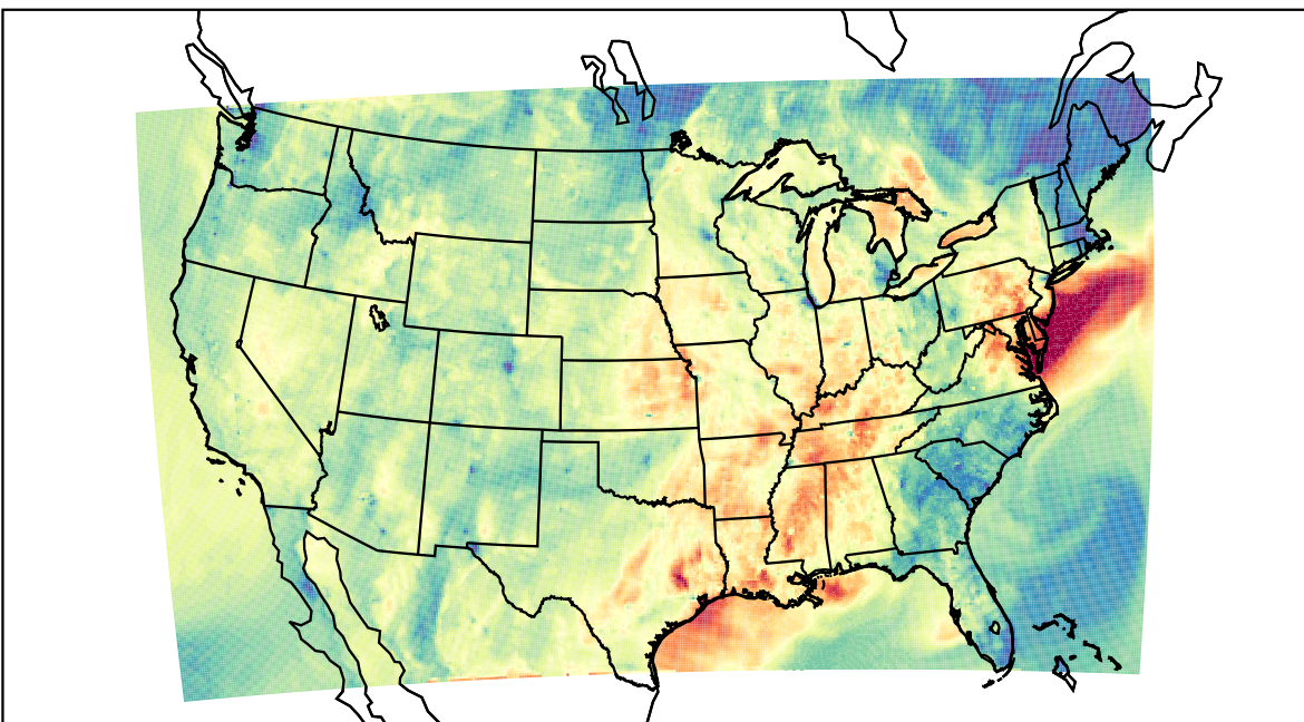
WRF (2021-10-09_01:00:00)
