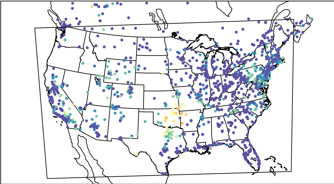
AirNOW (2021-10-09_11:00:00)
