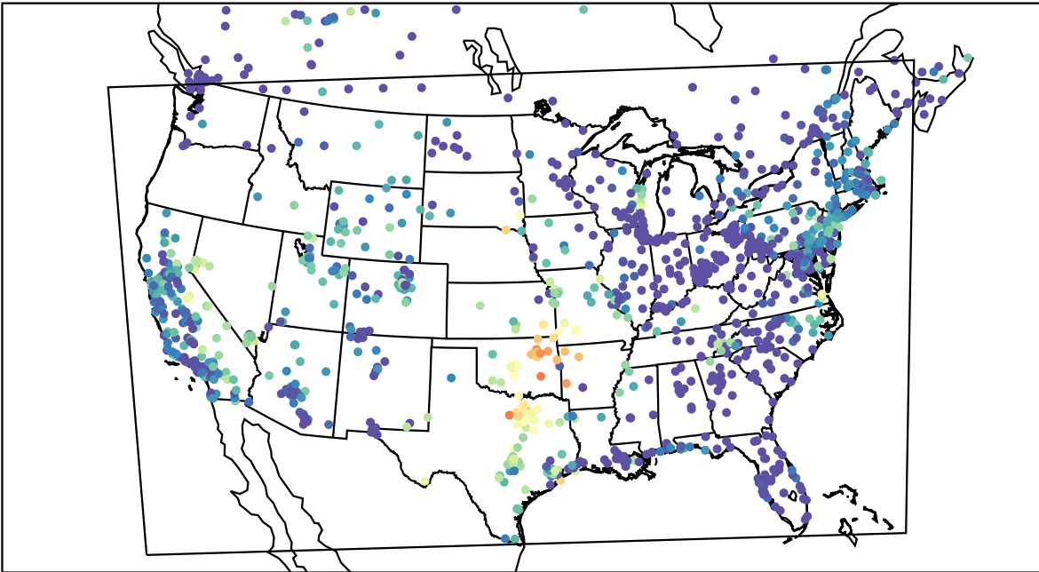
AirNOW (2021-10-09_05:00:00)
