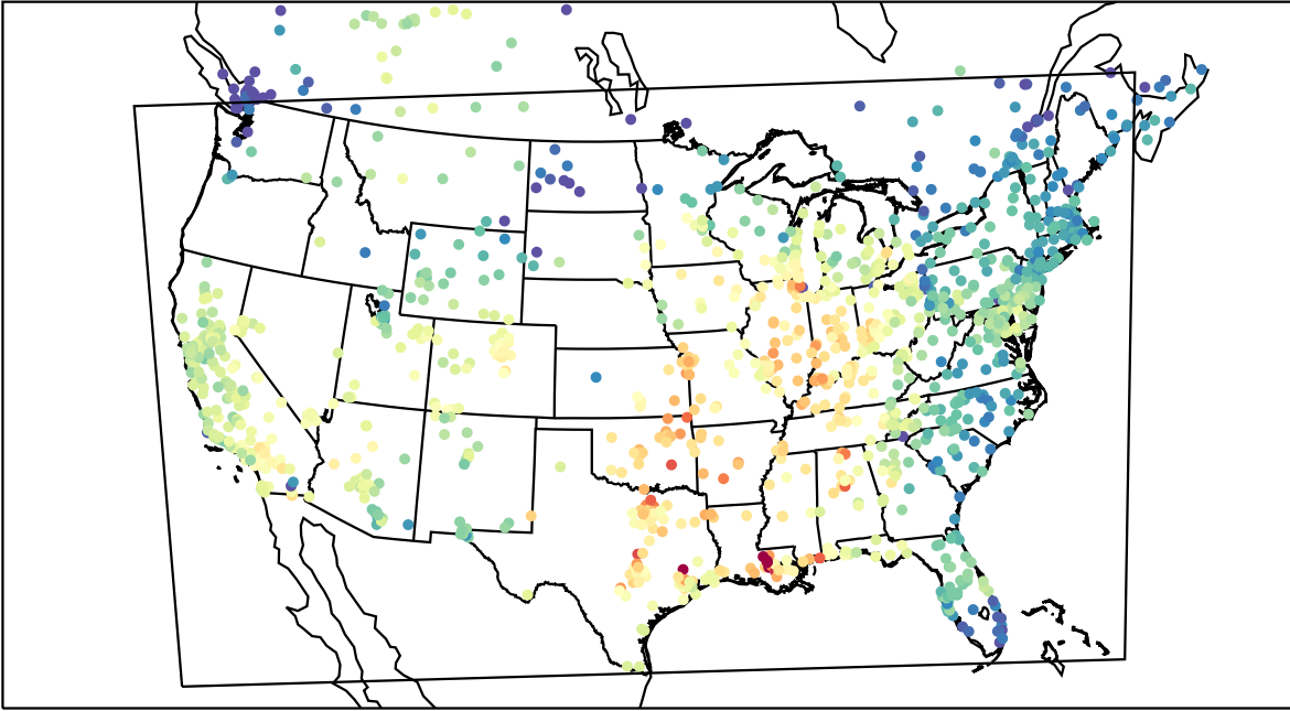
AirNOW (2021-10-09_20:00:00)
