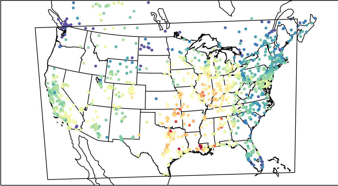
AirNOW (2021-10-09_19:00:00)
