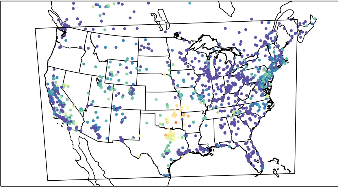
AirNOW (2021-10-09_07:00:00)
