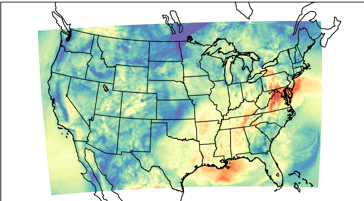
WRF (2021-10-09_15:00:00)
