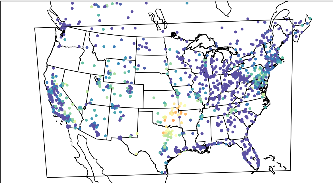
AirNOW (2021-10-09_08:00:00)
