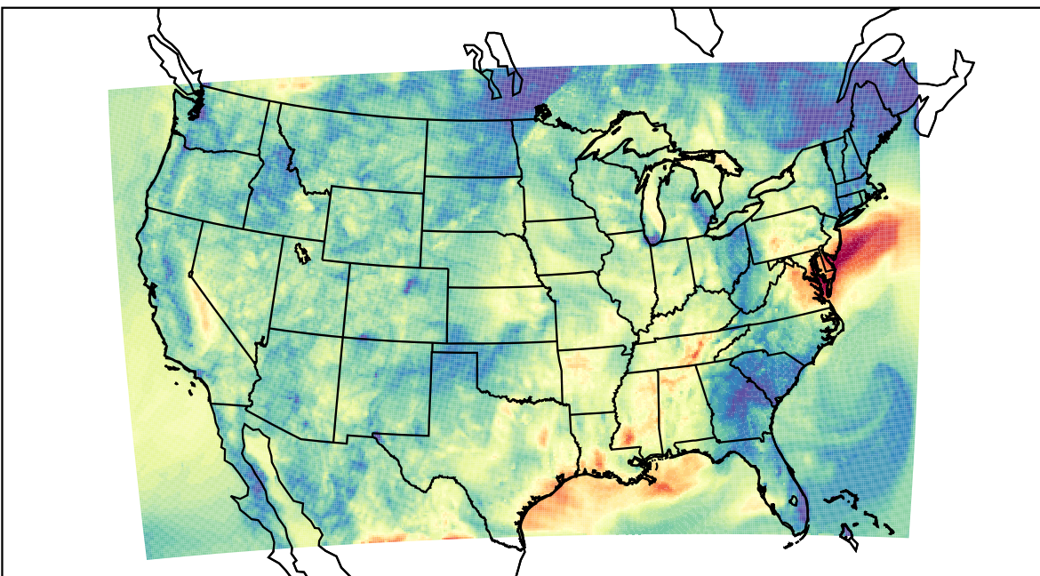
WRF (2021-10-09_06:00:00)
