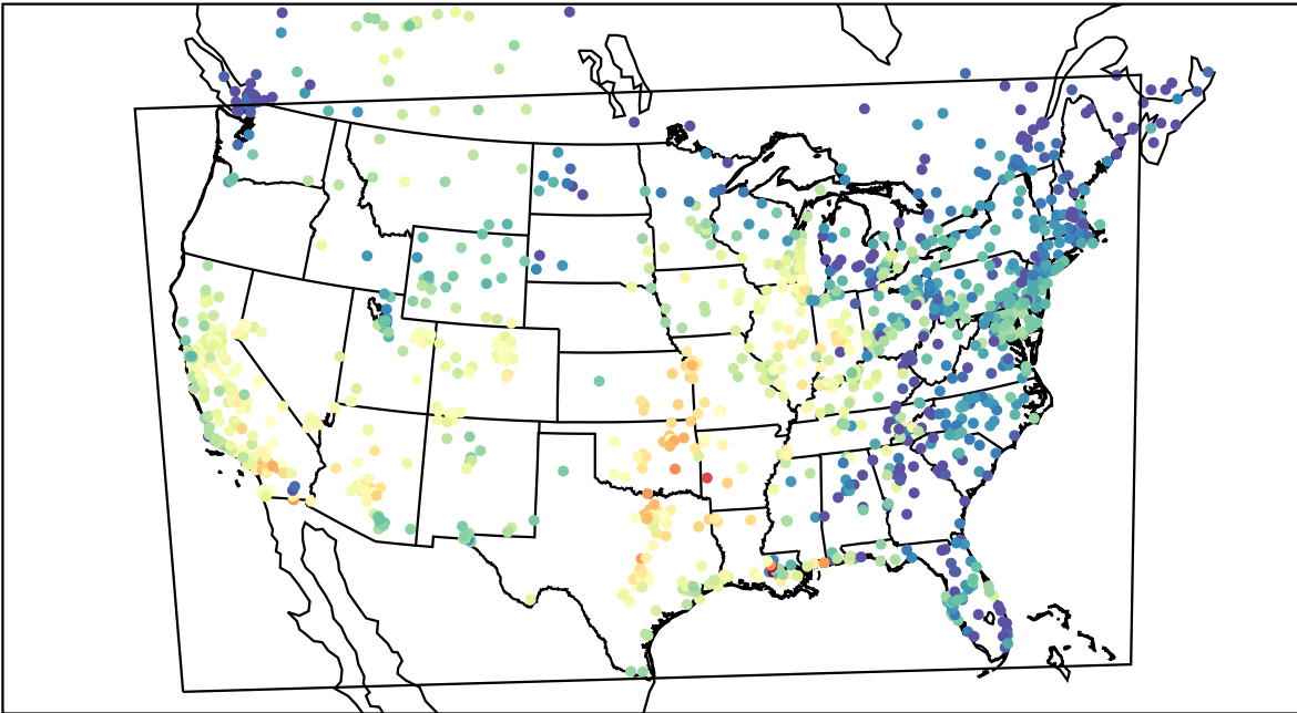
AirNOW (2021-10-09_23:00:00)
