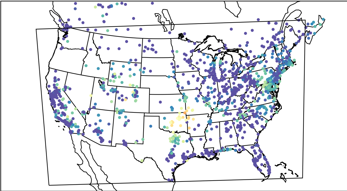
AirNOW (2021-10-09_13:00:00)
