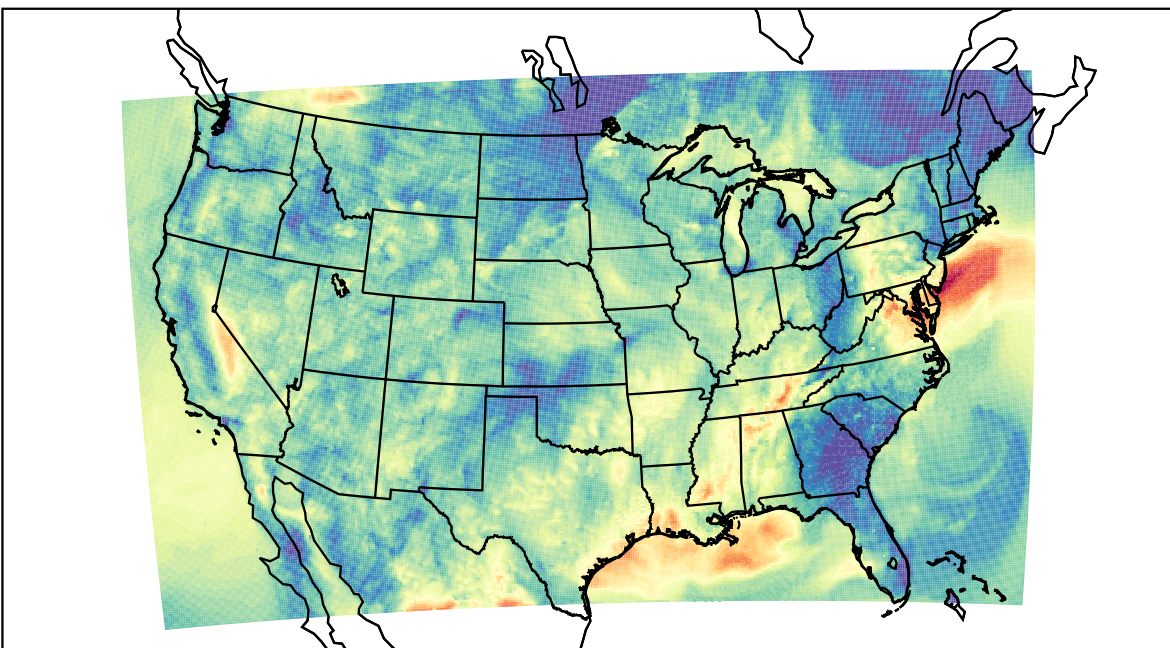
WRF (2021-10-09_09:00:00)
