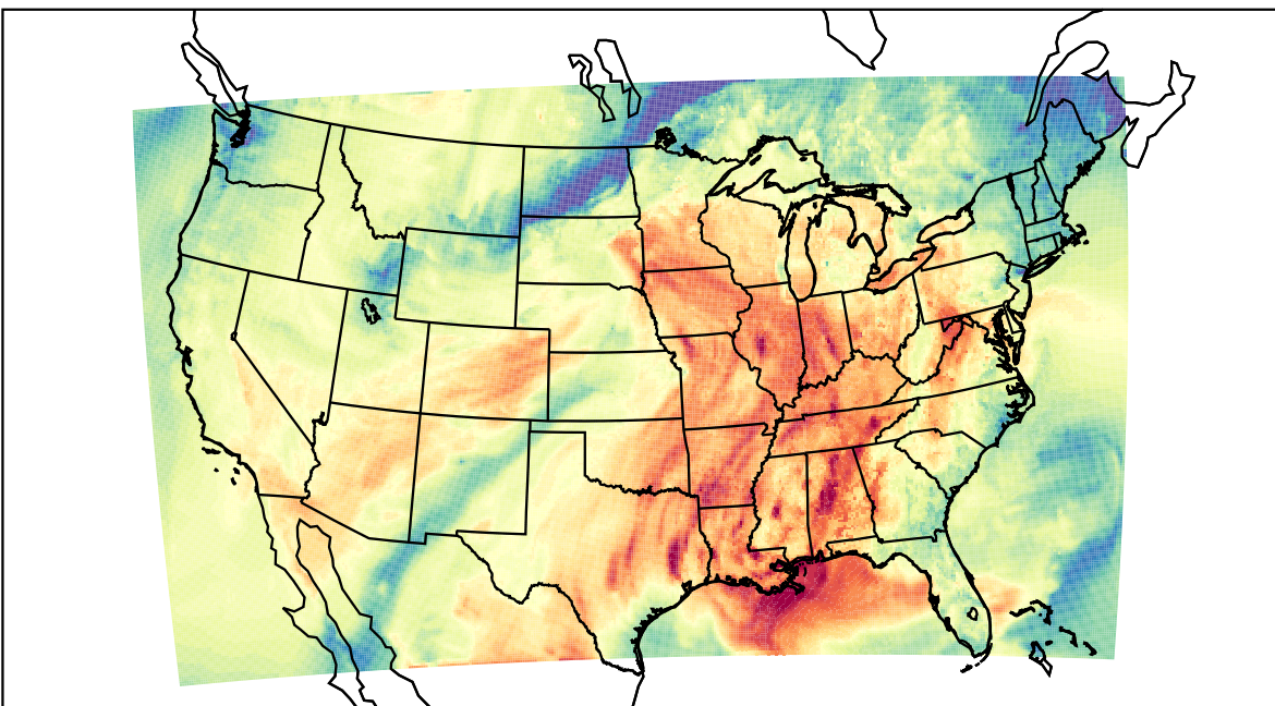
WRF (2021-10-09_22:00:00)
