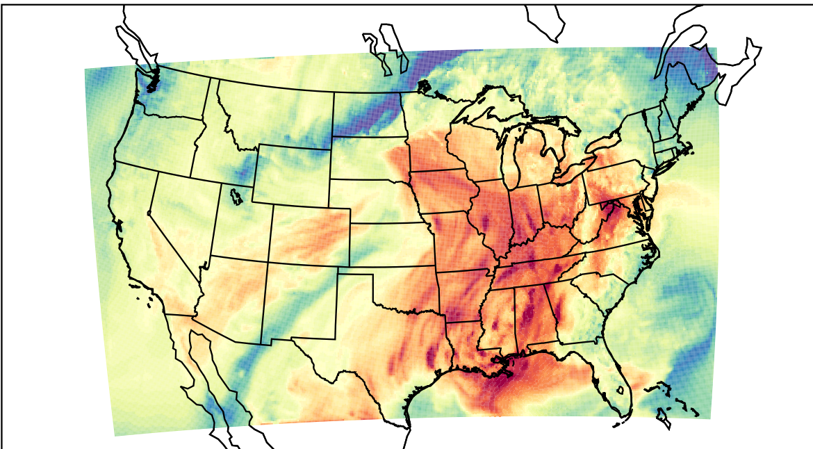
WRF (2021-10-09_21:00:00)
