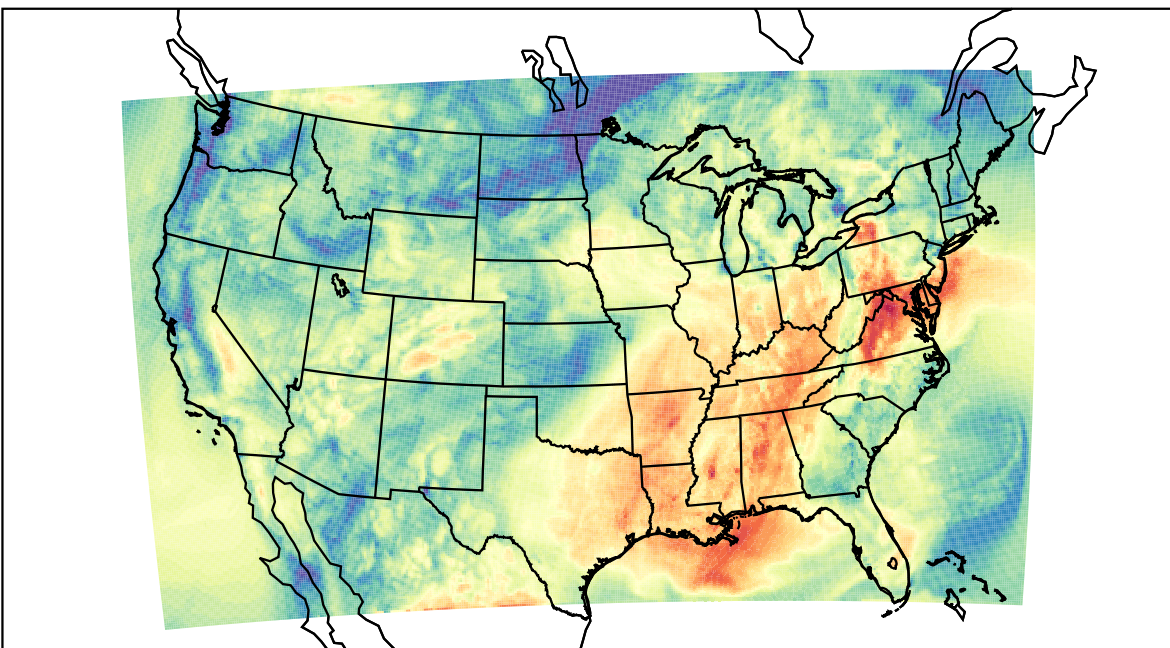
WRF (2021-10-09_16:00:00)
