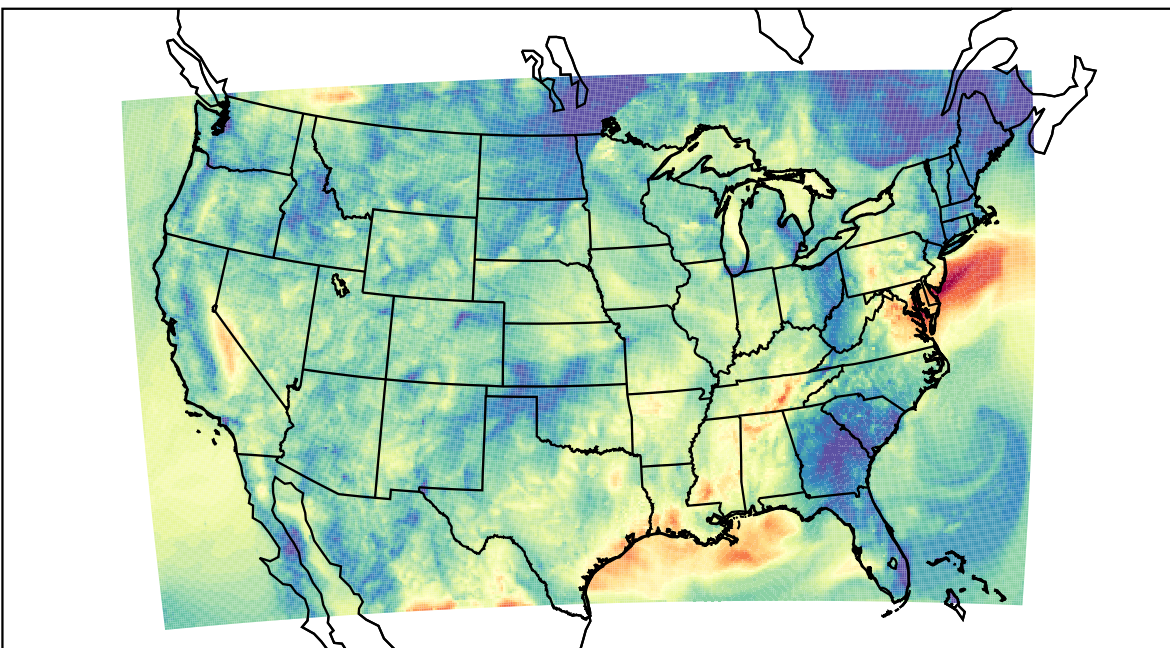
WRF (2021-10-09_08:00:00)
