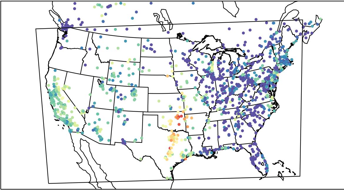
AirNOW (2021-10-09_01:00:00)
