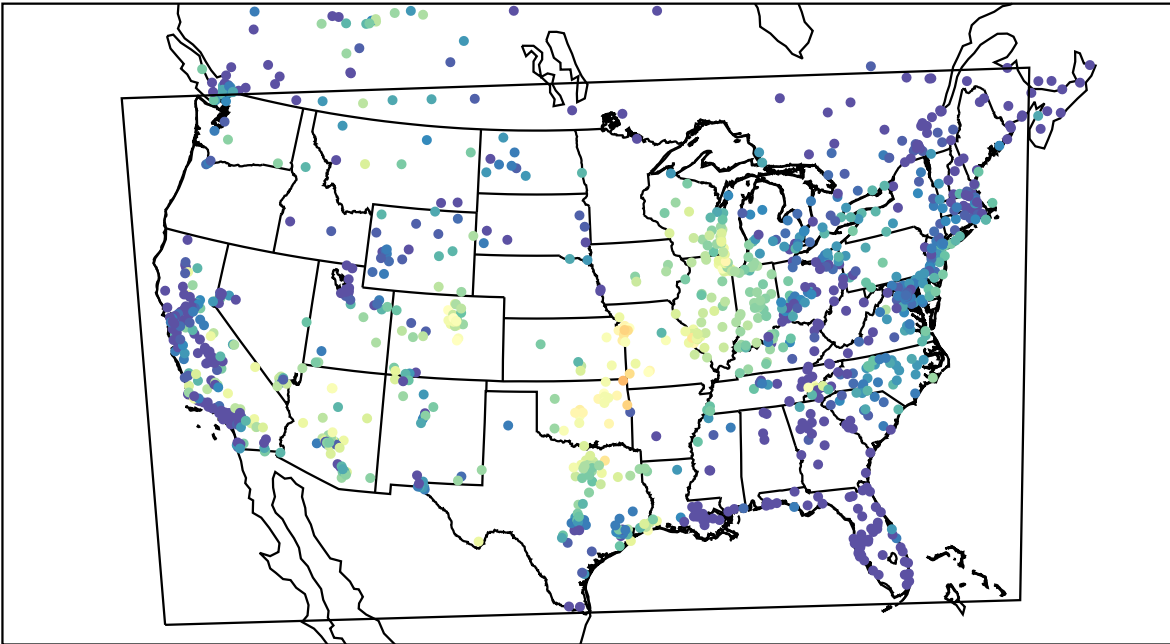
AirNOW (2021-10-10_06:00:00)
