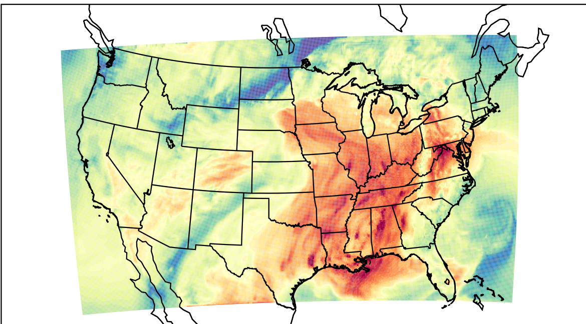
WRF (2021-10-09_19:00:00)
