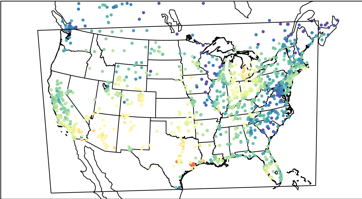
AirNOW (2021-10-11_21:00:00)
