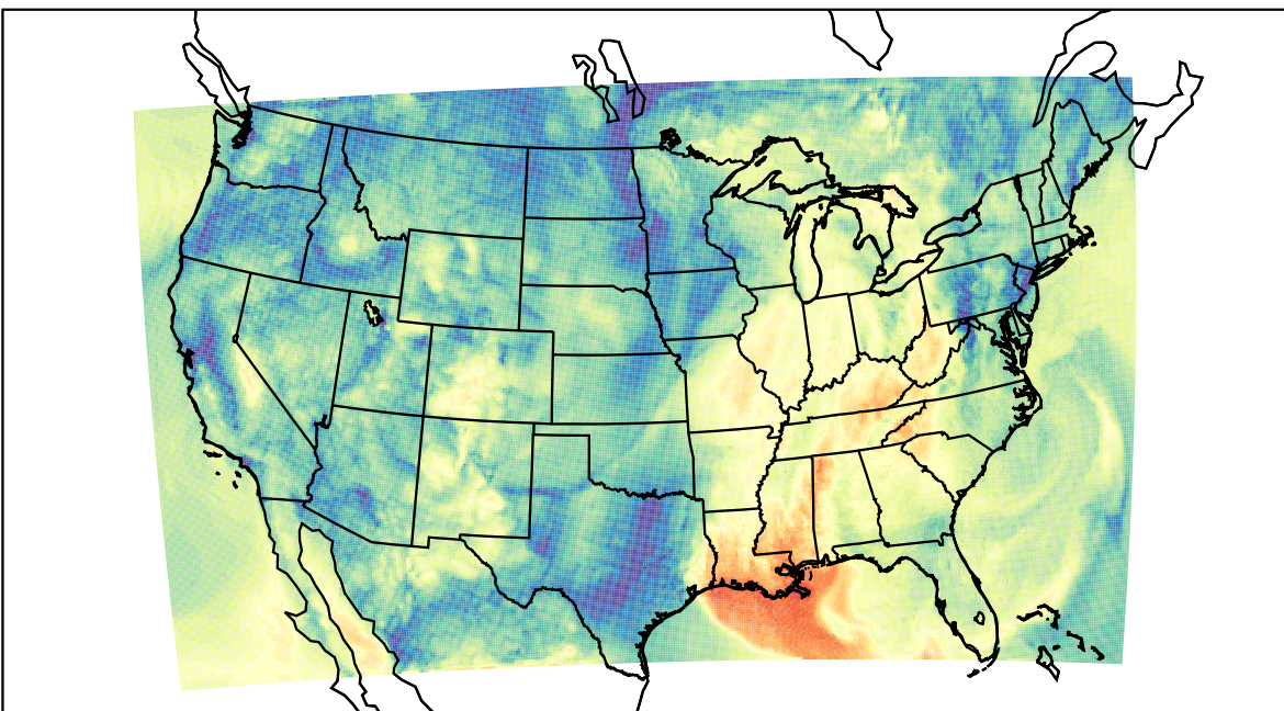
WRF (2021-10-10_15:00:00)
