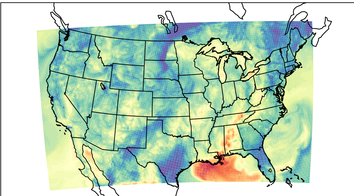
WRF (2021-10-10_07:00:00)
