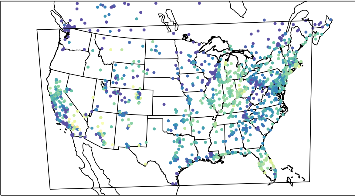
AirNOW (2021-10-11_15:00:00)
