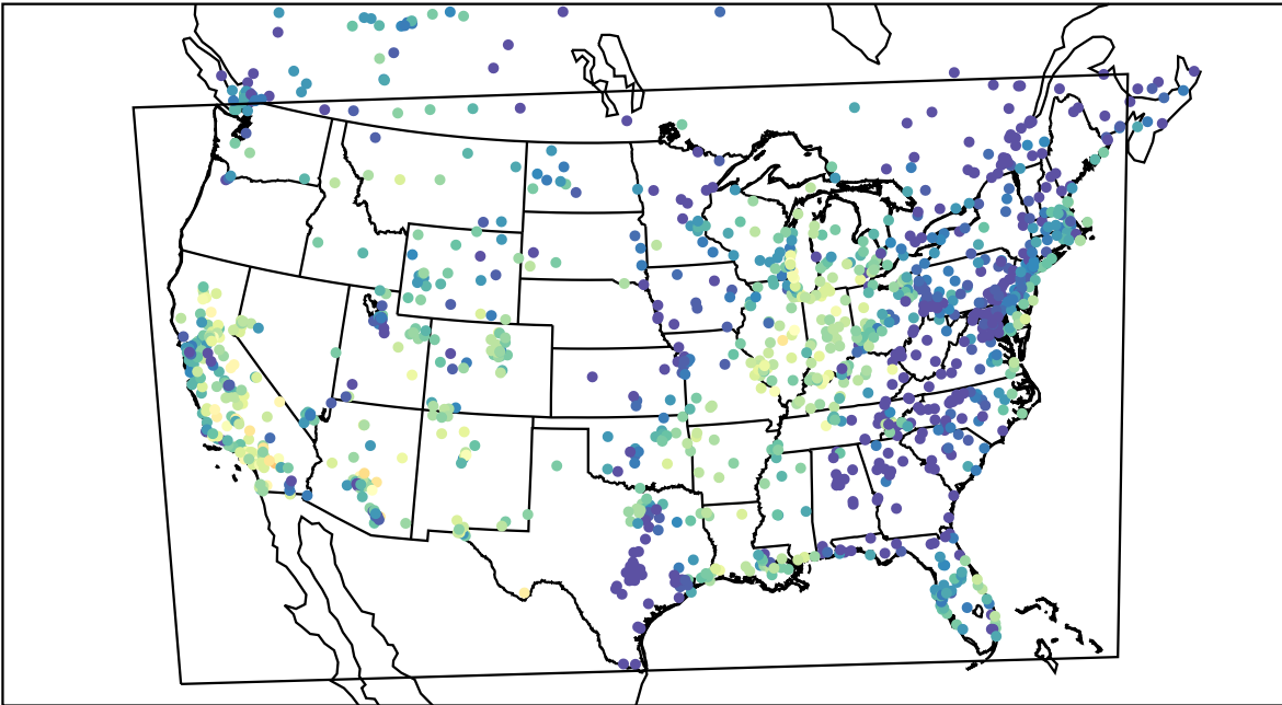
AirNOW (2021-10-11_02:00:00)
