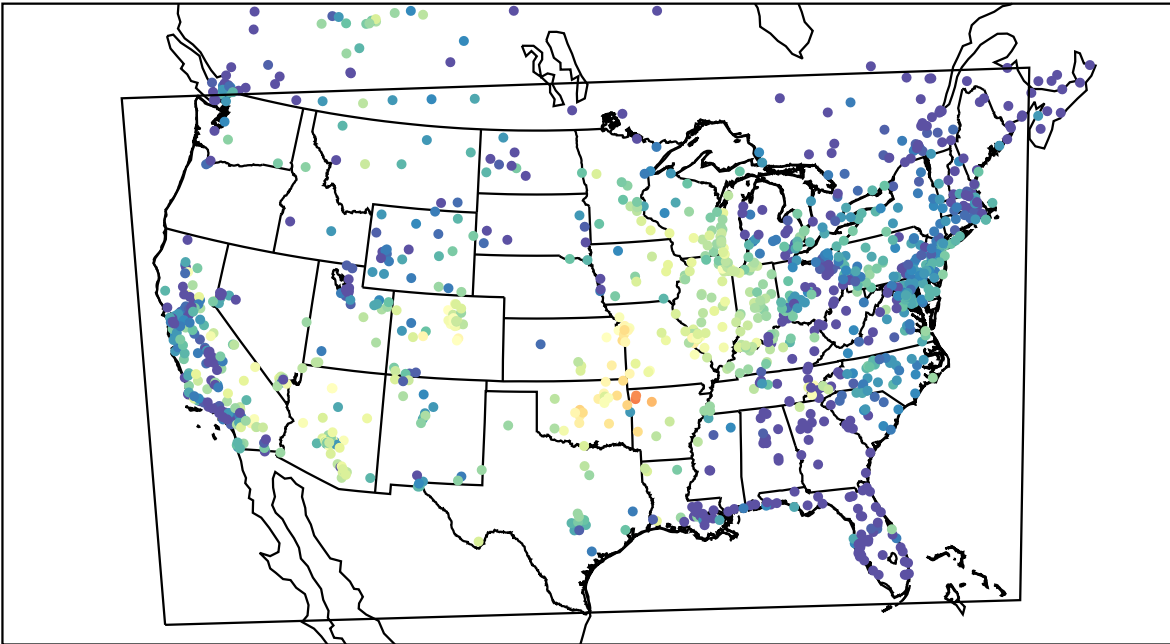
AirNOW (2021-10-10_04:00:00)
