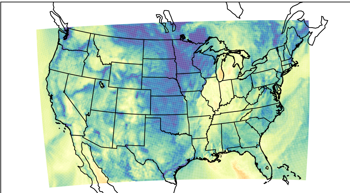
WRF (2021-10-11_14:00:00)
