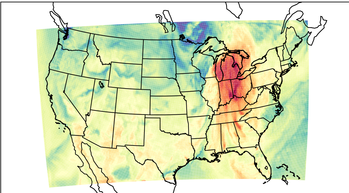
WRF (2021-10-11_18:00:00)
