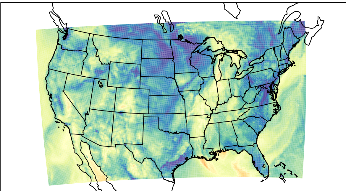
WRF (2021-10-11_10:00:00)
