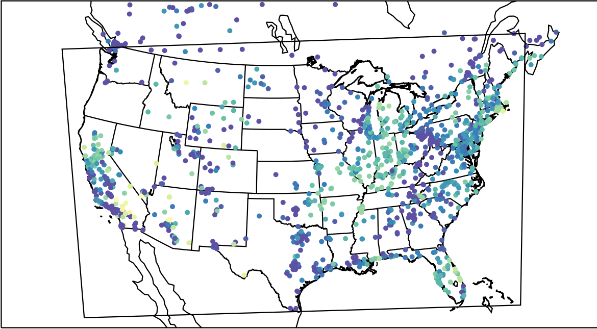
AirNOW (2021-10-11_14:00:00)
