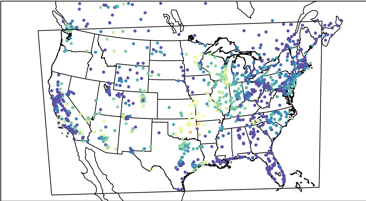
AirNOW (2021-10-10_09:00:00)
