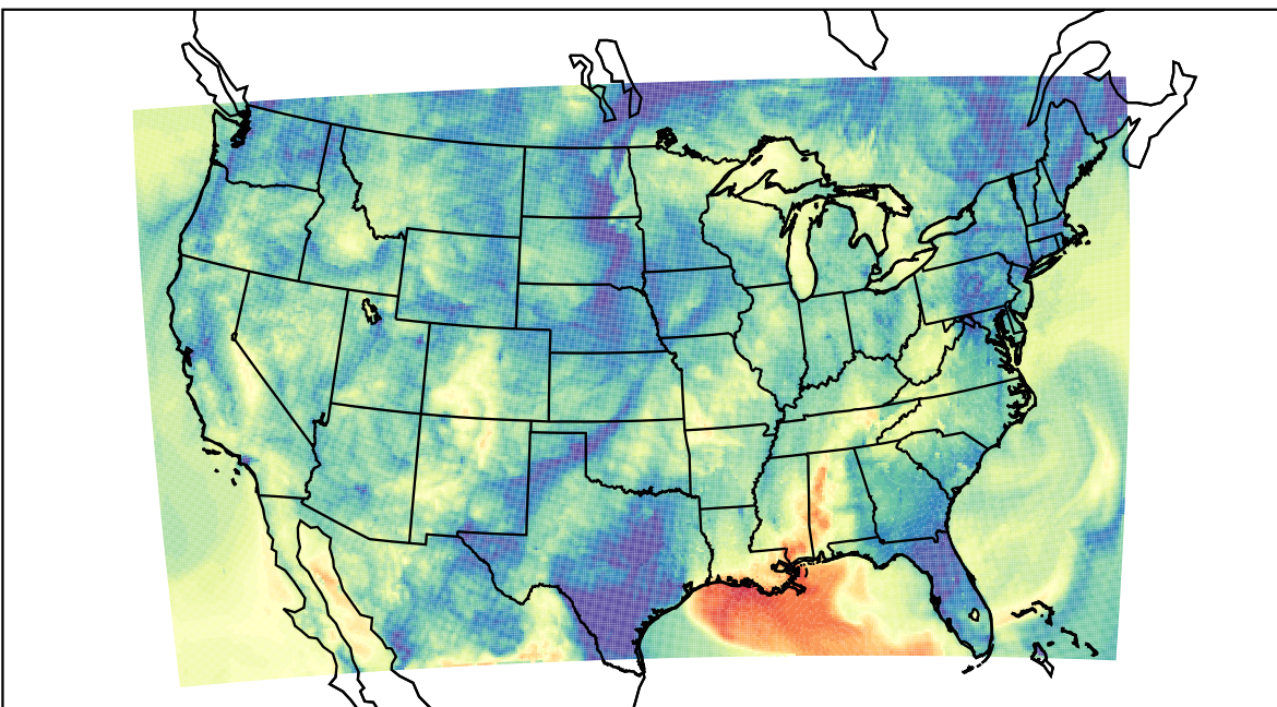
WRF (2021-10-10_10:00:00)
