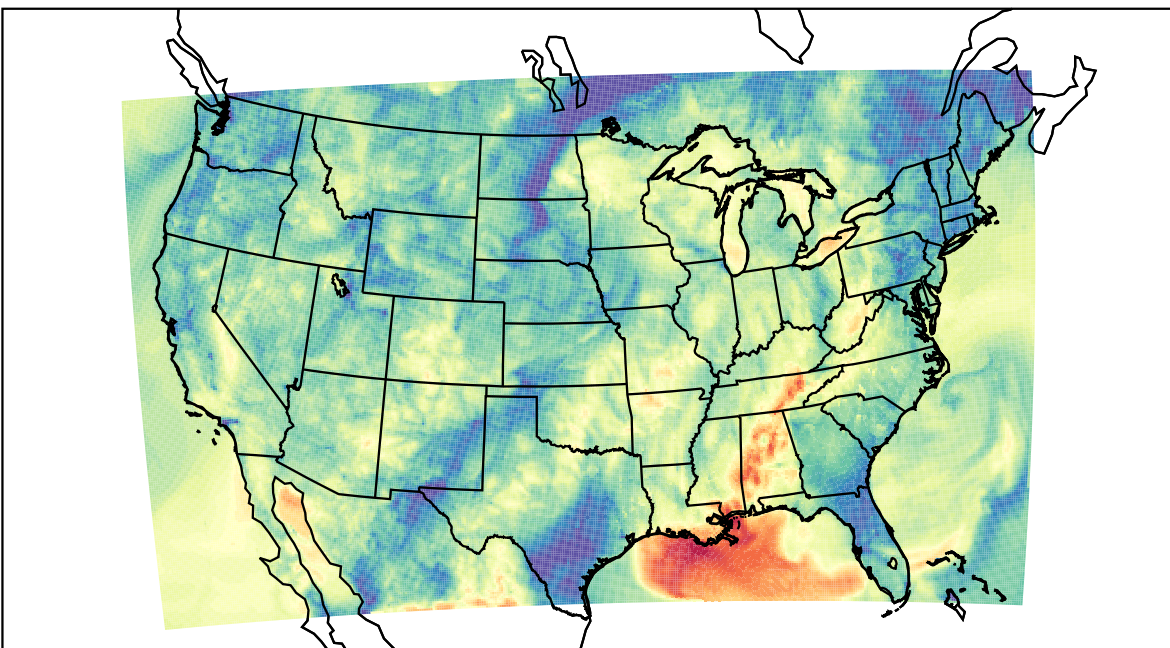
WRF (2021-10-10_06:00:00)
