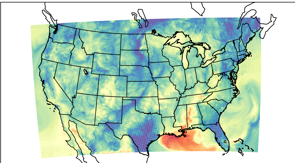
WRF (2021-10-10_09:00:00)
