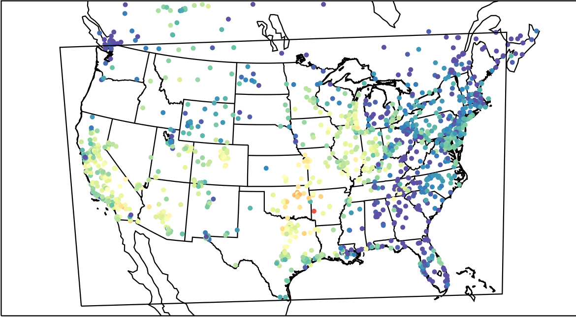
AirNOW (2021-10-10_01:00:00)
