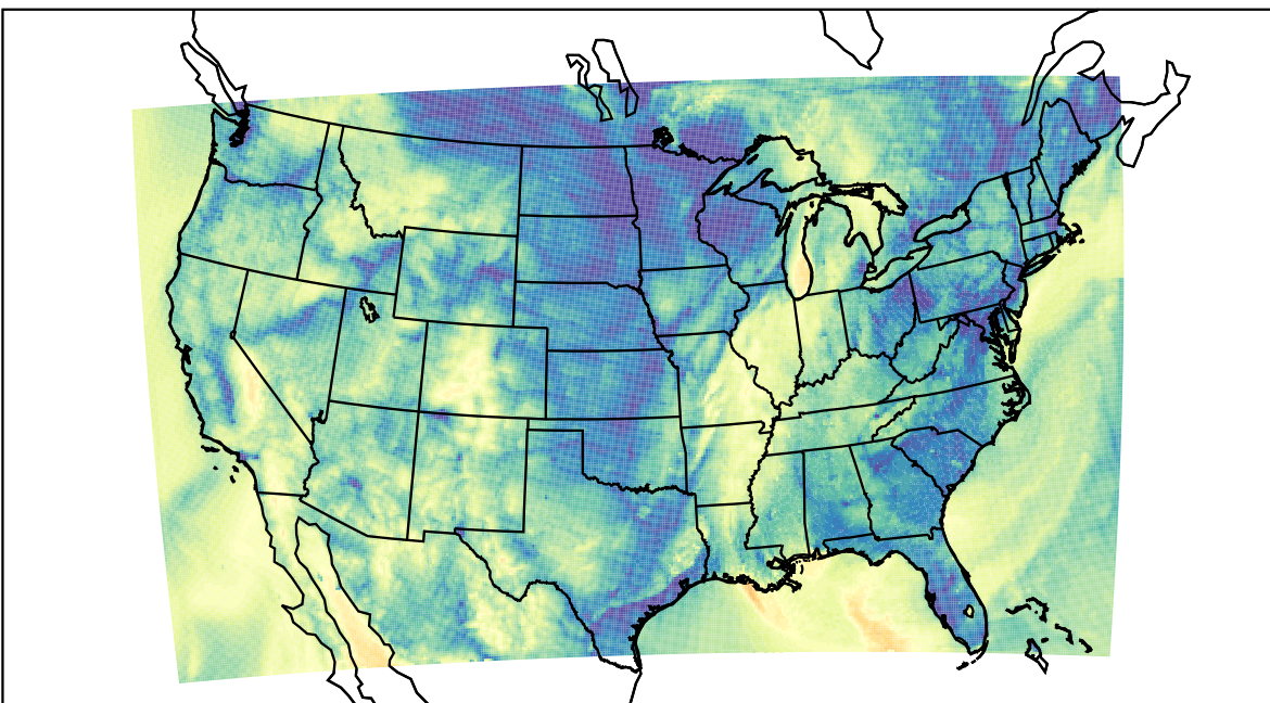
WRF (2021-10-11_12:00:00)
