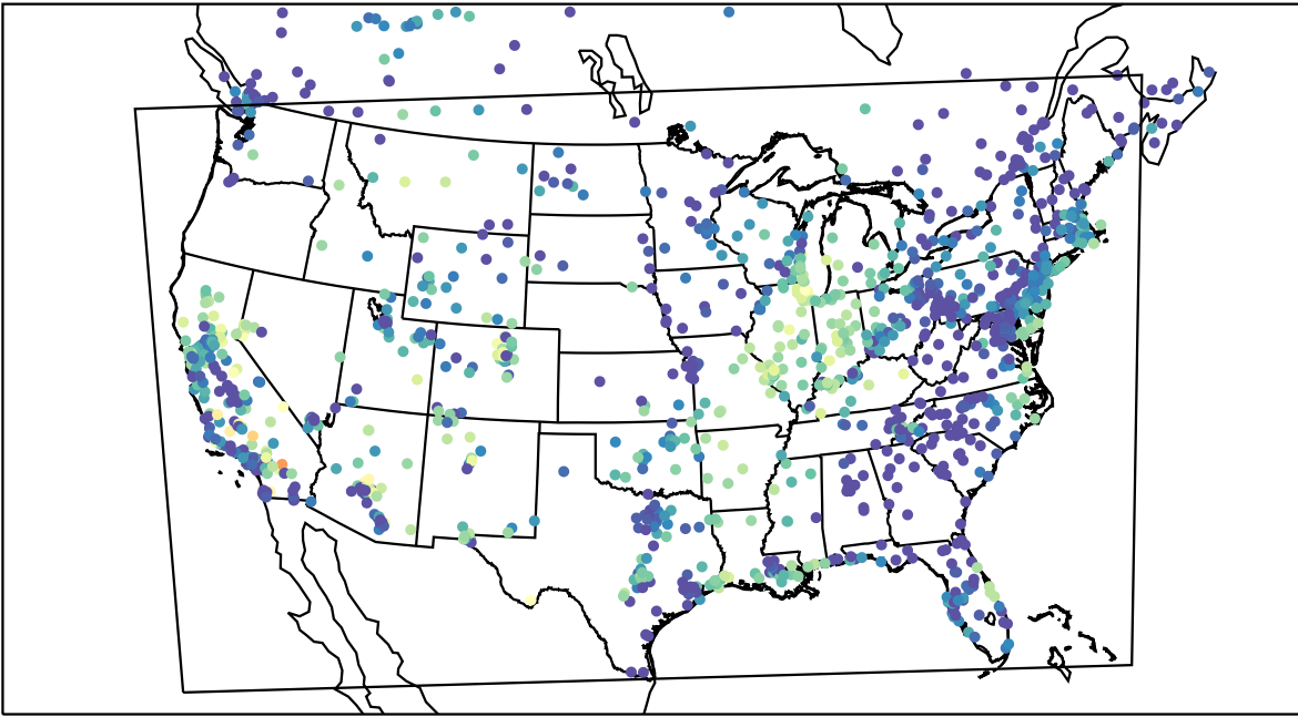
AirNOW (2021-10-11_05:00:00)
