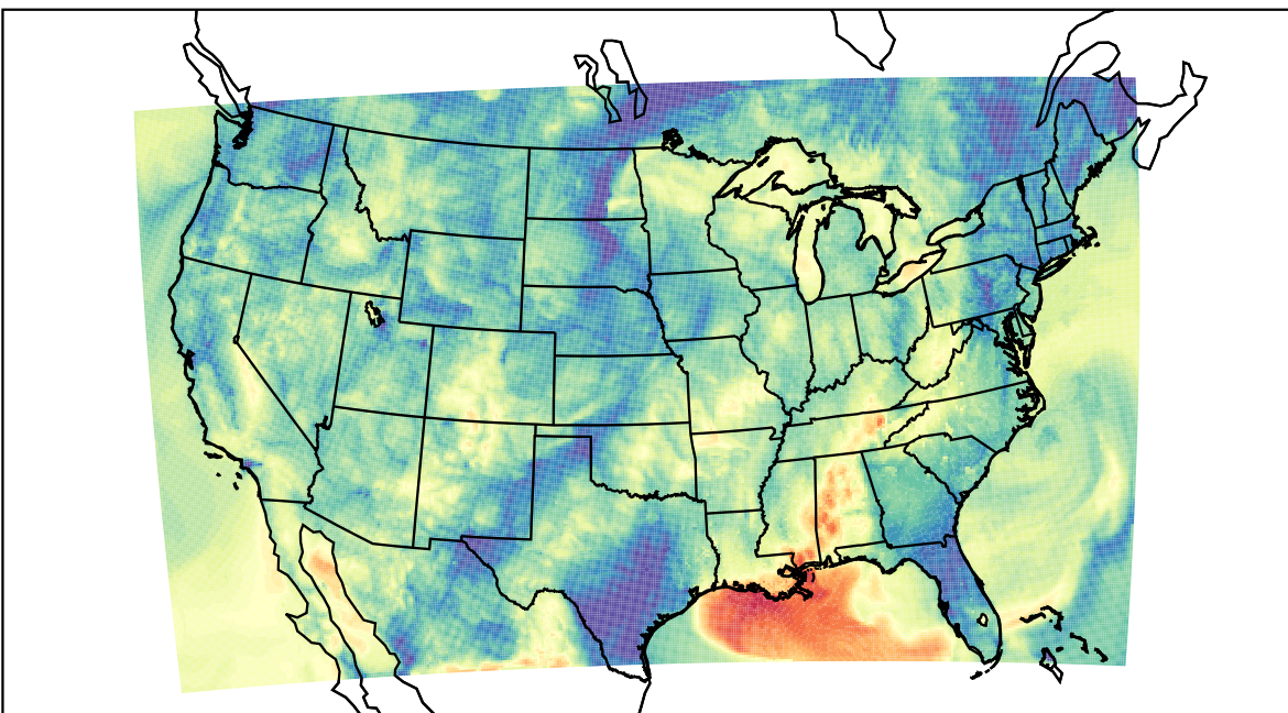
WRF (2021-10-10_08:00:00)
