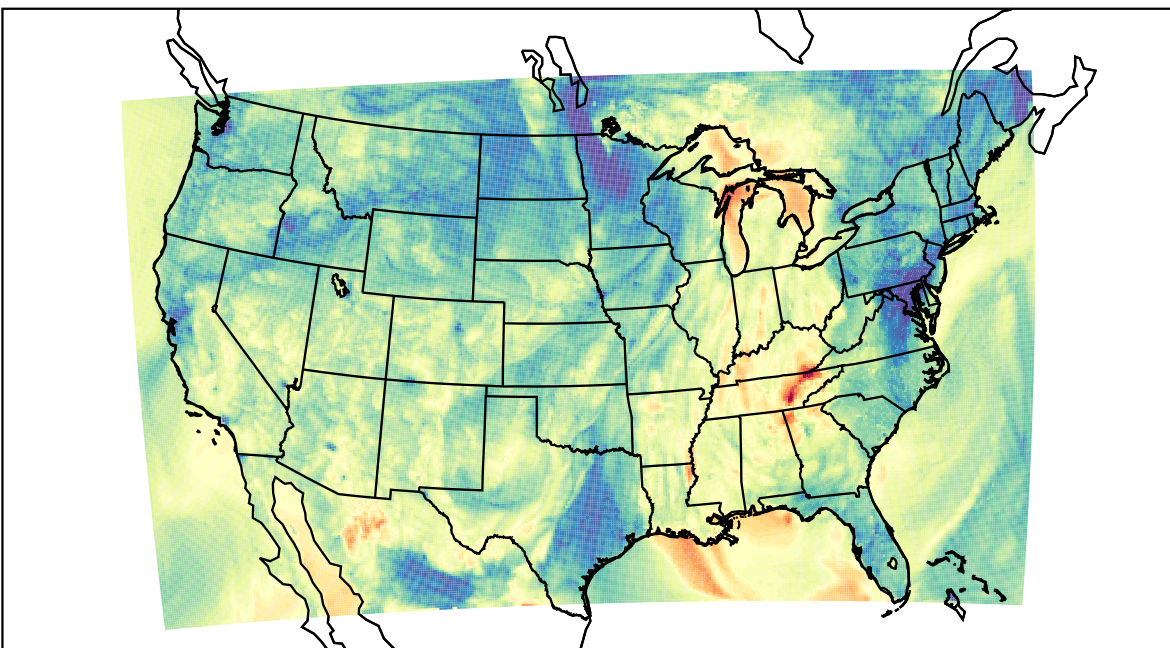
WRF (2021-10-11_03:00:00)
