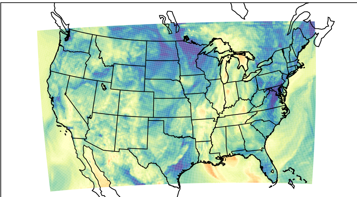
WRF (2021-10-11_07:00:00)
