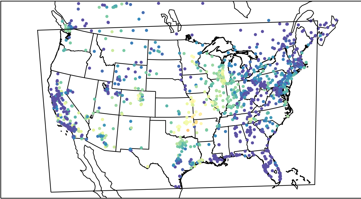
AirNOW (2021-10-10_08:00:00)
