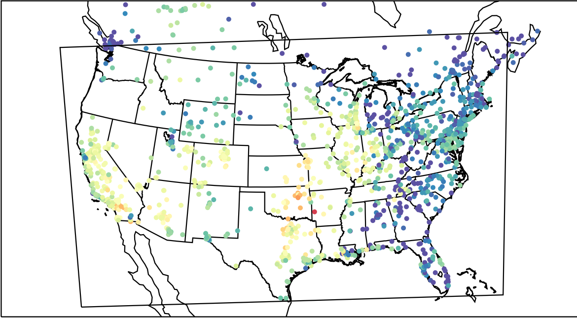
AirNOW (2021-10-10_00:00:00)
