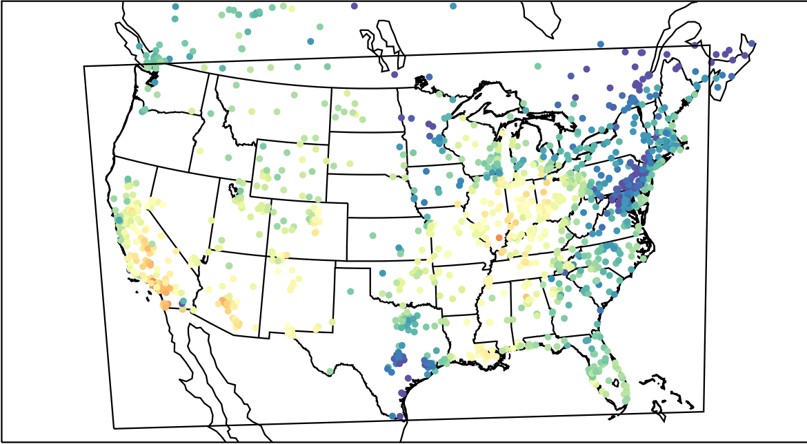
AirNOW (2021-10-10_21:00:00)
