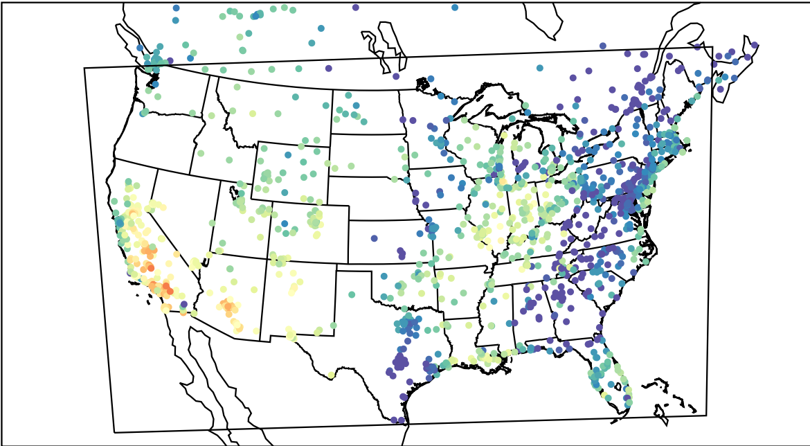
AirNOW (2021-10-11_00:00:00)
