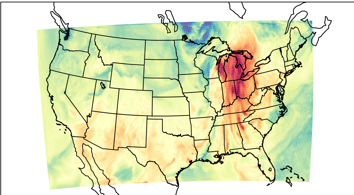
WRF (2021-10-11_20:00:00)
