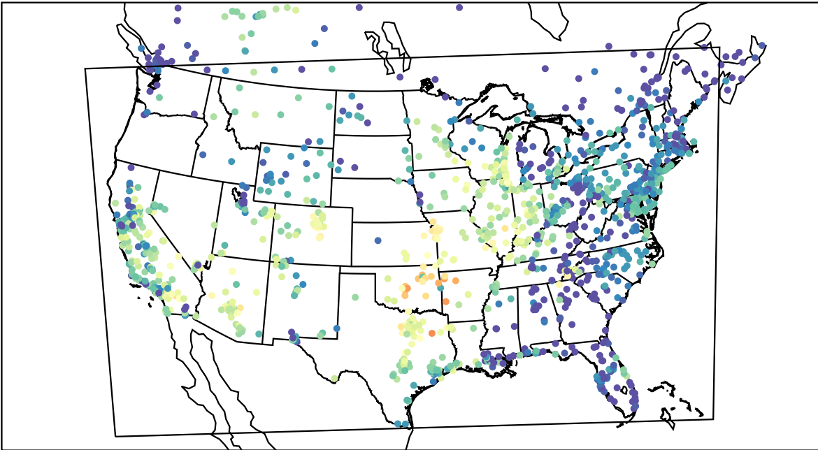
AirNOW (2021-10-10_02:00:00)
