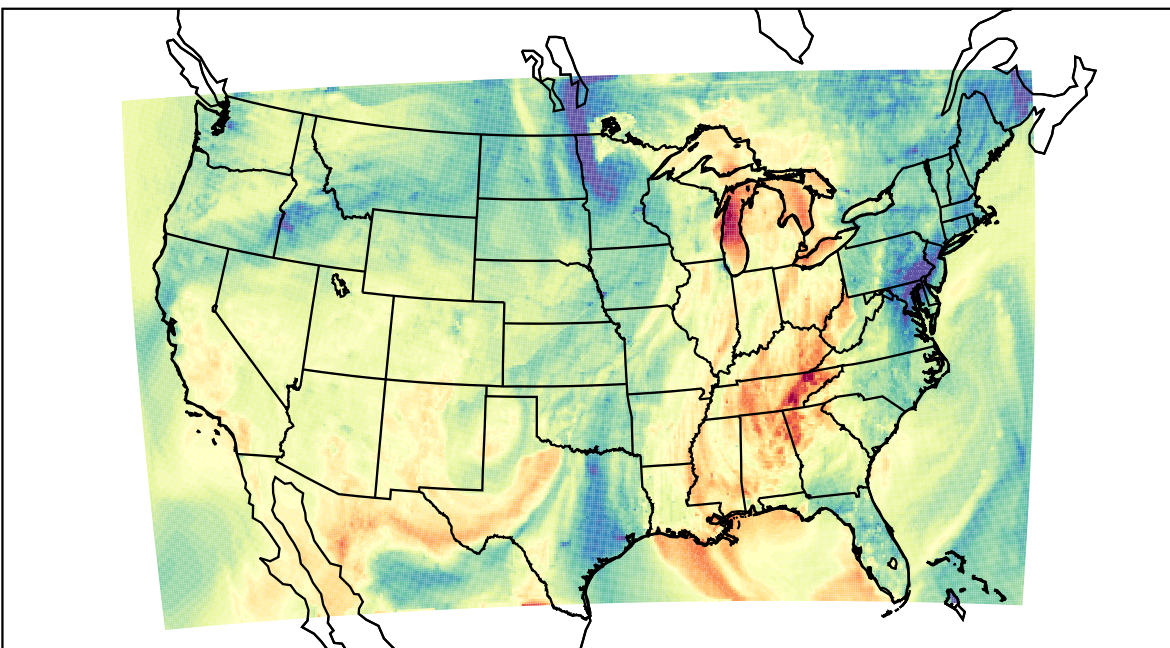
WRF (2021-10-11_00:00:00)
