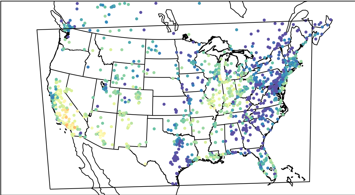
AirNOW (2021-10-11_01:00:00)
