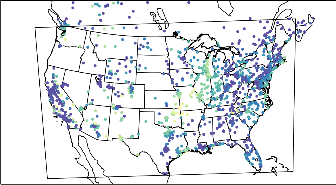
AirNOW (2021-10-10_13:00:00)
