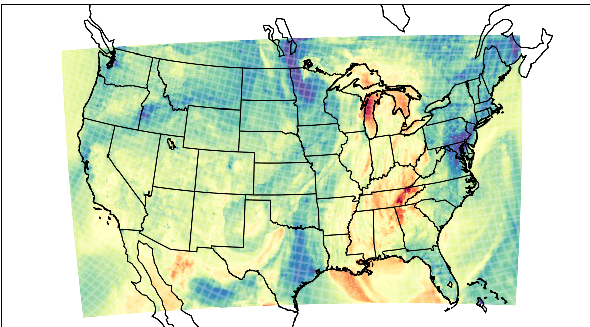
WRF (2021-10-11_01:00:00)
