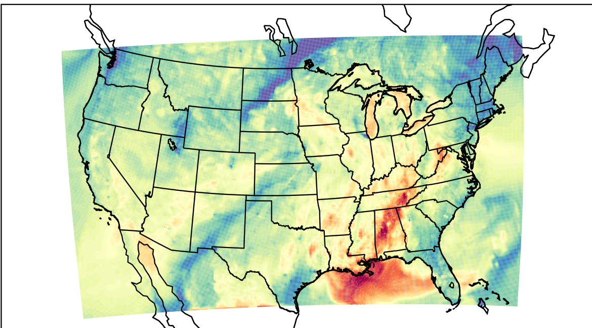
WRF (2021-10-10_01:00:00)
