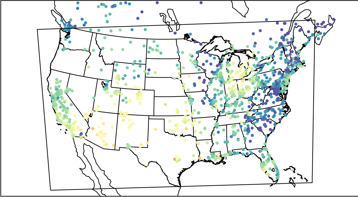
AirNOW (2021-10-11_22:00:00)
