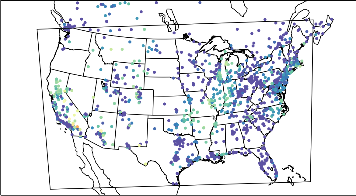
AirNOW (2021-10-11_11:00:00)
