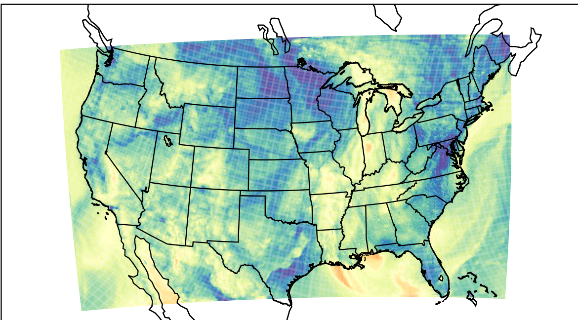
WRF (2021-10-11_08:00:00)
