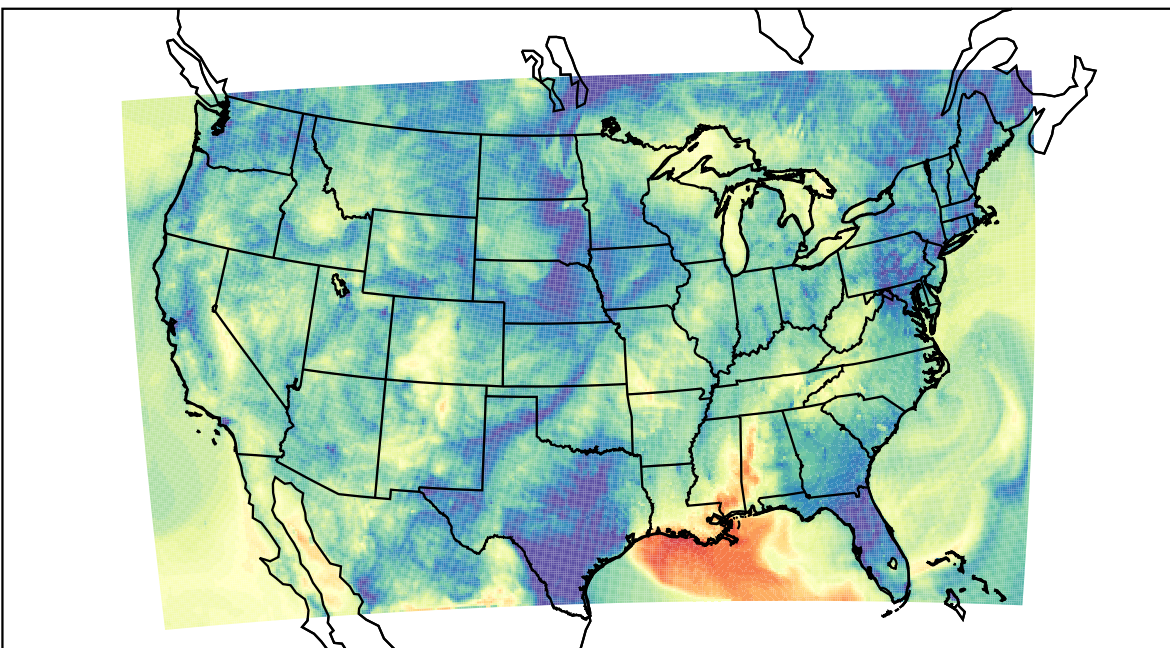
WRF (2021-10-10_11:00:00)
