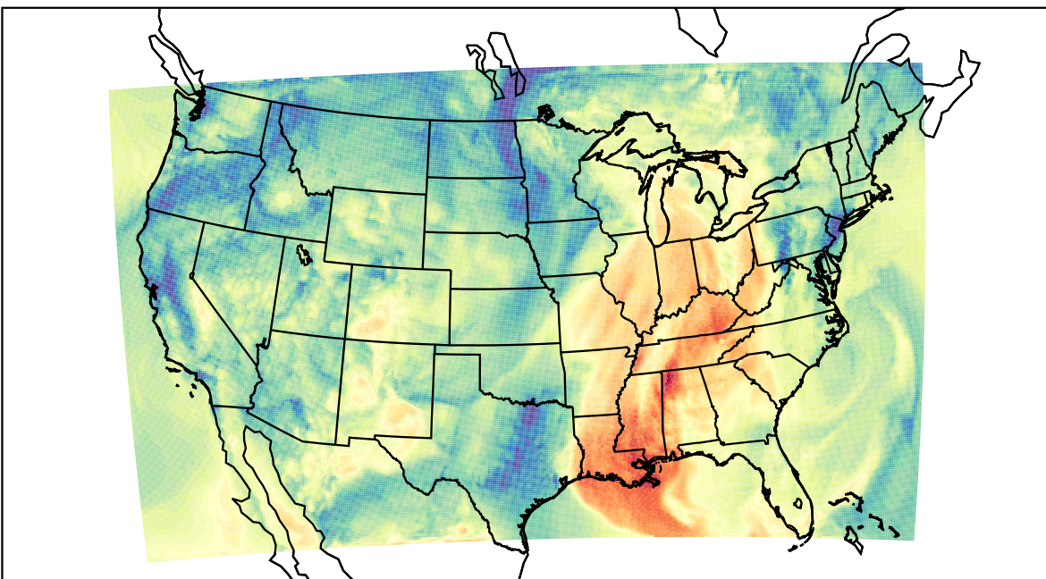
WRF (2021-10-10_16:00:00)
