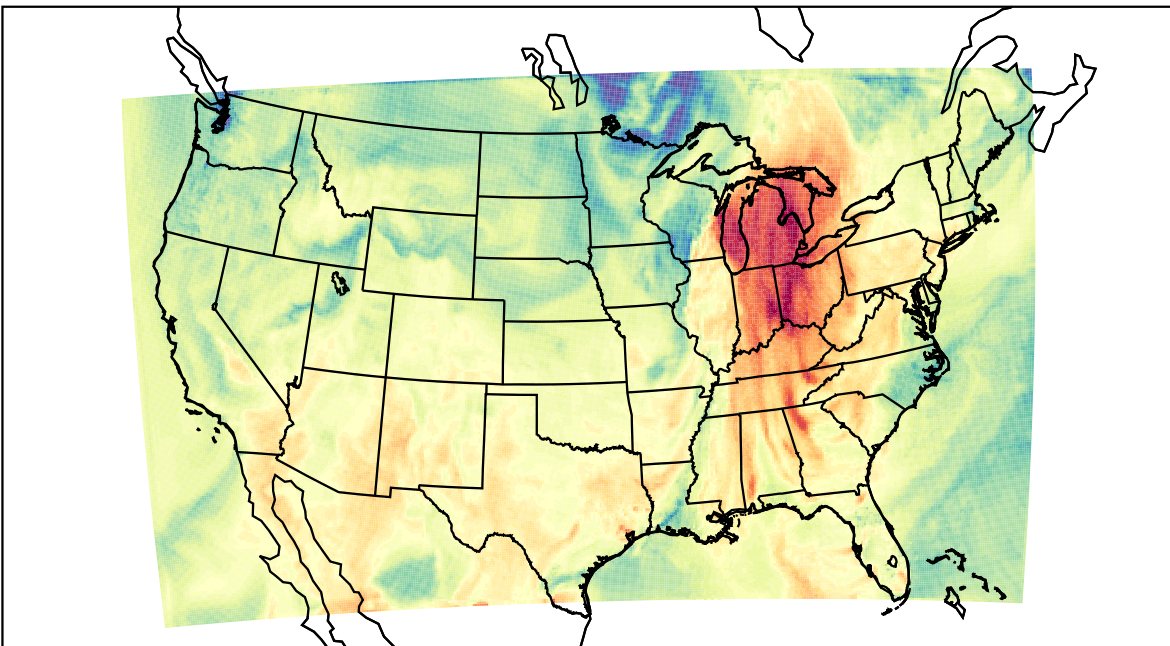
WRF (2021-10-11_19:00:00)
