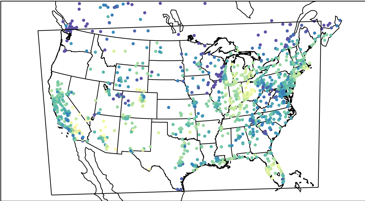
AirNOW (2021-10-11_16:00:00)
