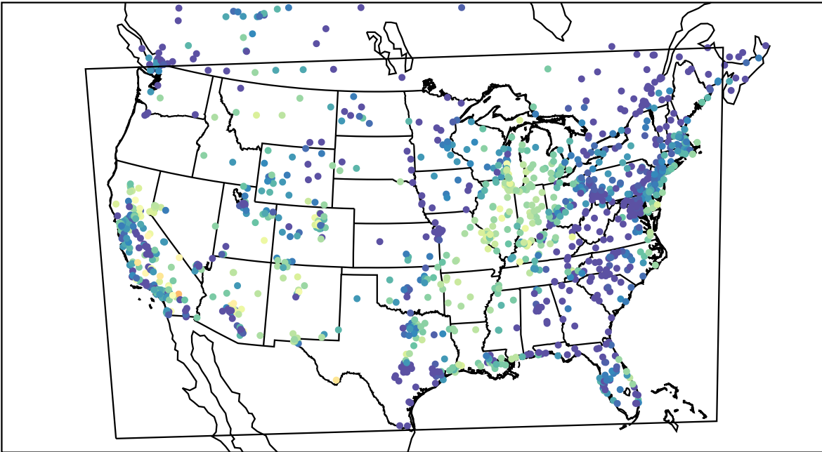
AirNOW (2021-10-11_04:00:00)
