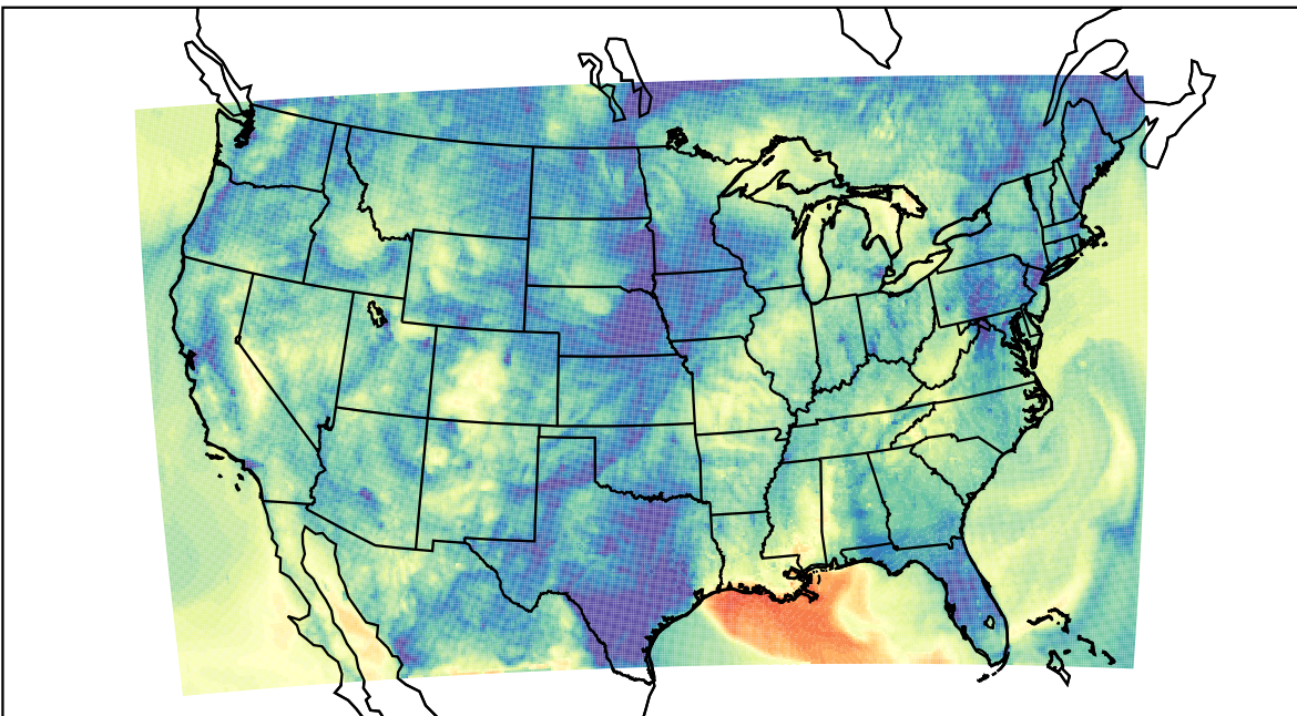
WRF (2021-10-10_13:00:00)
