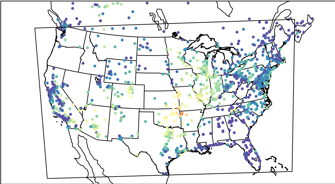
AirNOW (2021-10-10_05:00:00)
