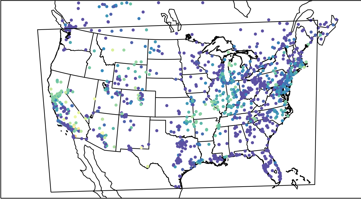
AirNOW (2021-10-11_12:00:00)
