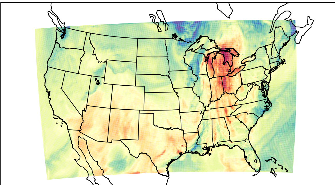
WRF (2021-10-11_22:00:00)
