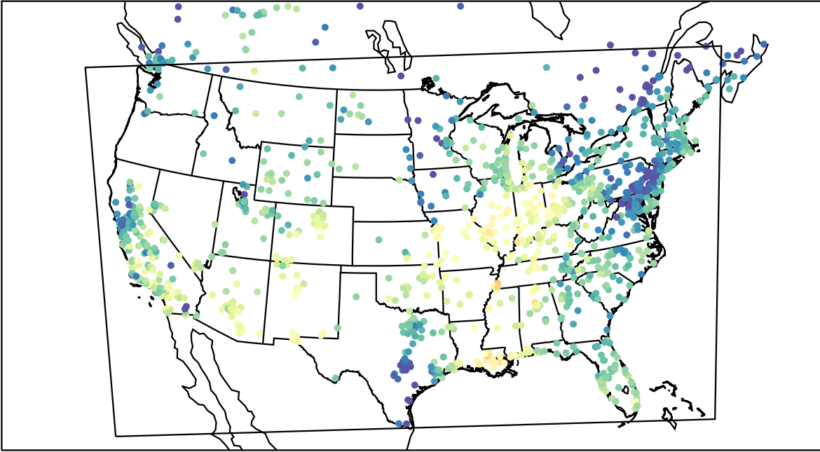
AirNOW (2021-10-10_17:00:00)
