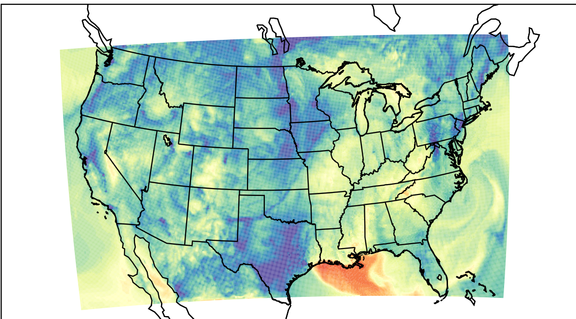
WRF (2021-10-10_14:00:00)
