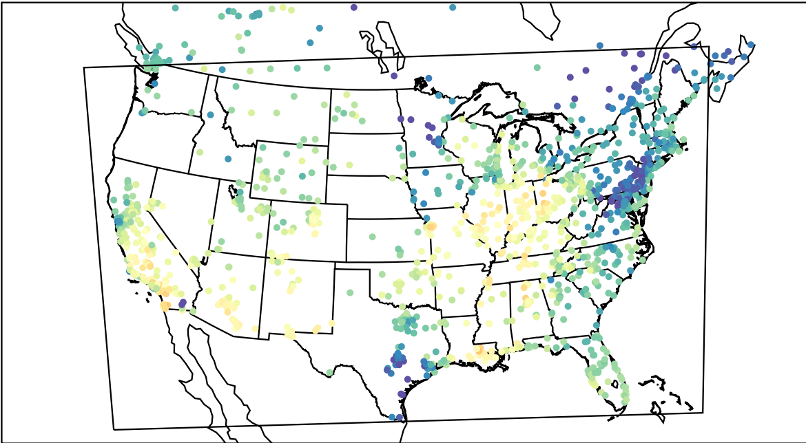
AirNOW (2021-10-10_19:00:00)
