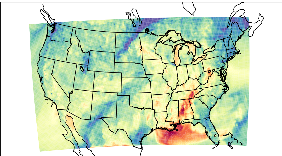
WRF (2021-10-10_02:00:00)
