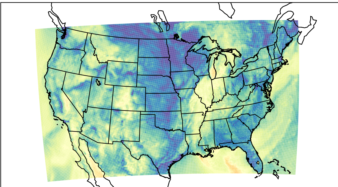
WRF (2021-10-11_13:00:00)
