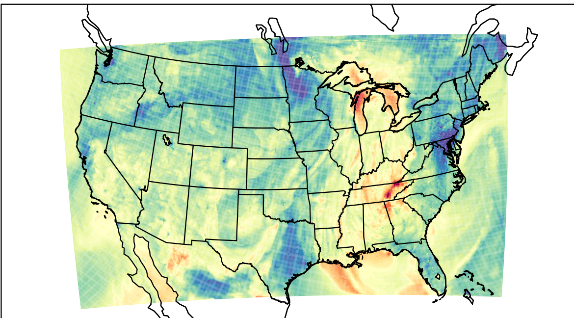
WRF (2021-10-11_02:00:00)
