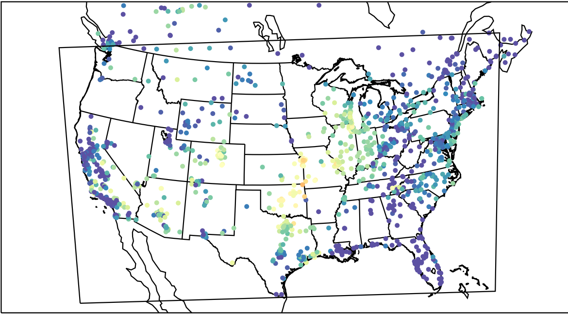
AirNOW (2021-10-10_06:00:00)
