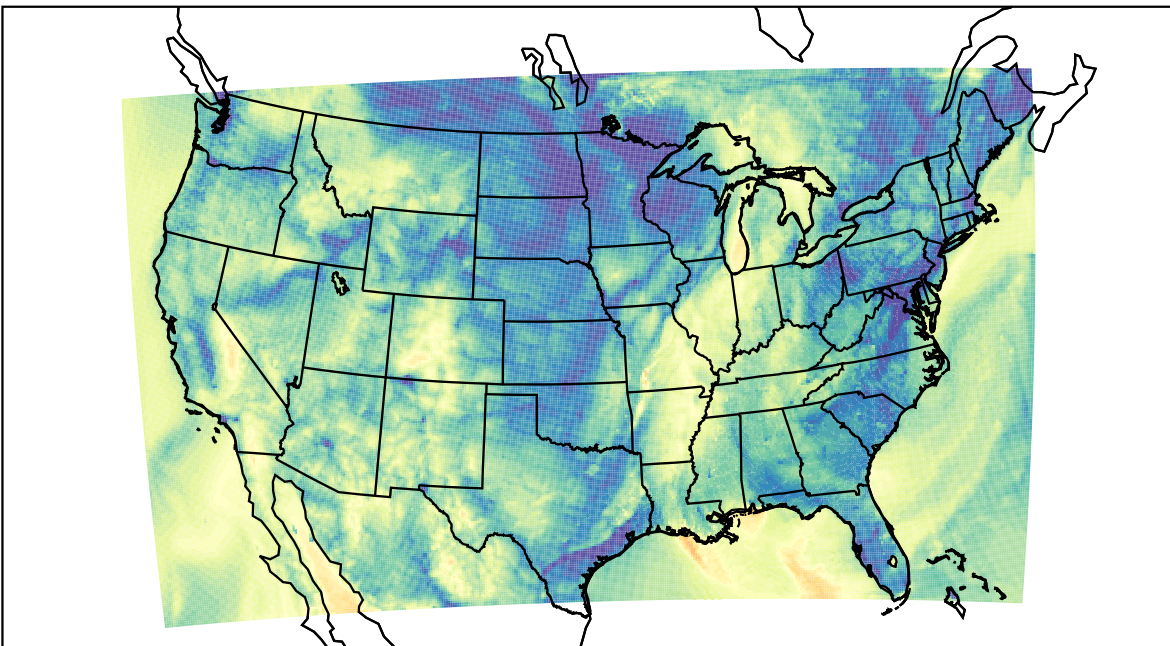
WRF (2021-10-11_11:00:00)
