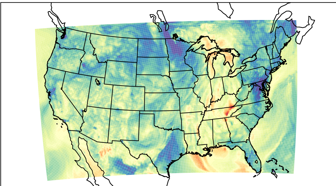
WRF (2021-10-11_04:00:00)
