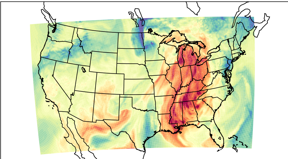
WRF (2021-10-10_21:00:00)
