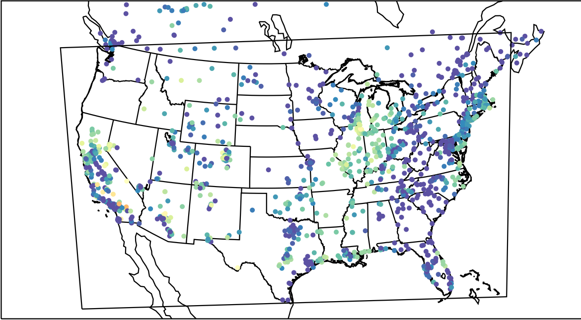
AirNOW (2021-10-11_06:00:00)
