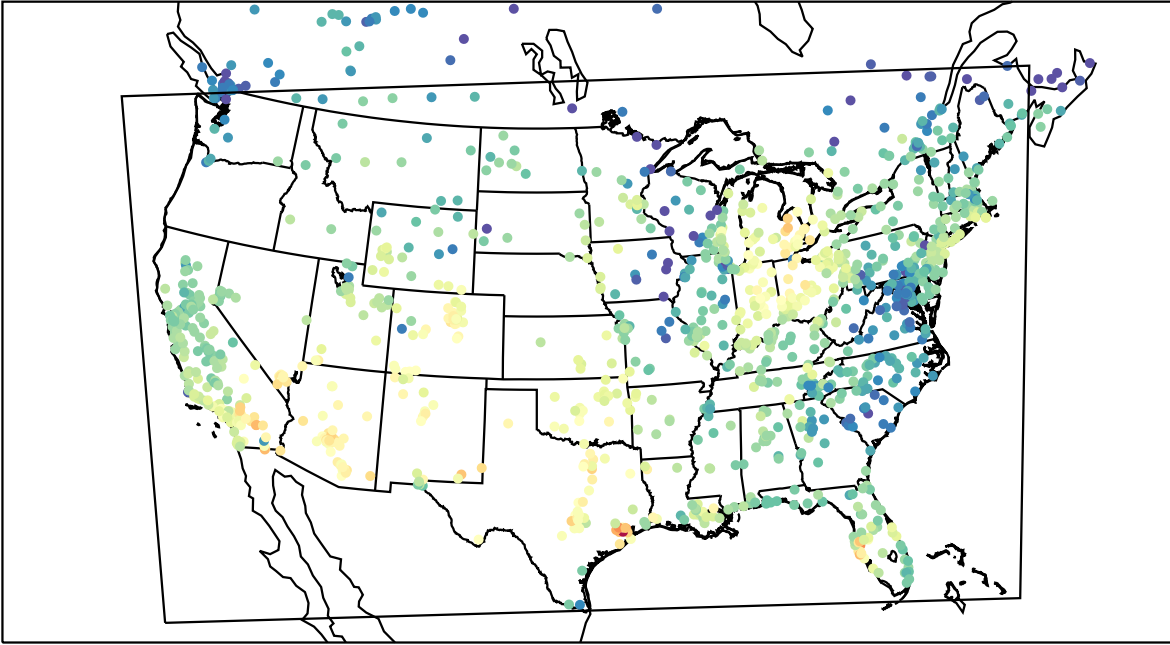
AirNOW (2021-10-11_20:00:00)
