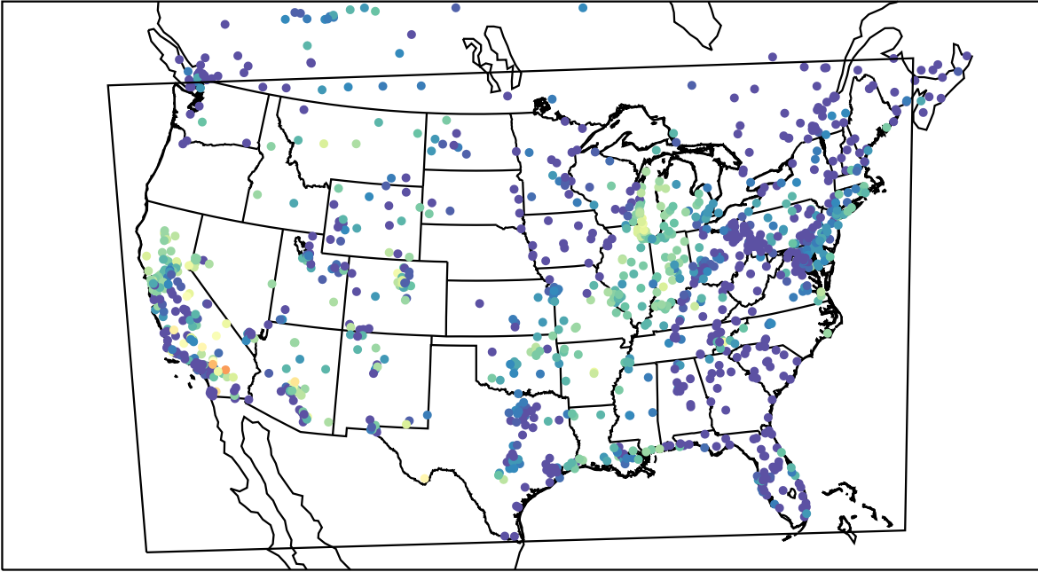
AirNOW (2021-10-11_08:00:00)
