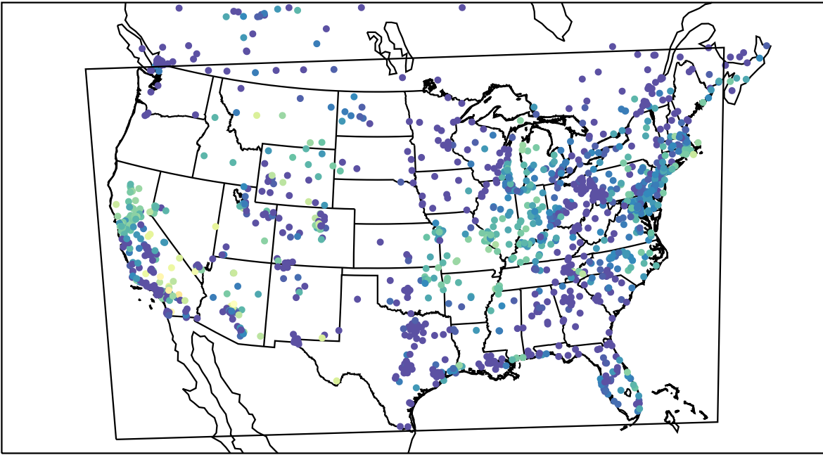
AirNOW (2021-10-11_13:00:00)
