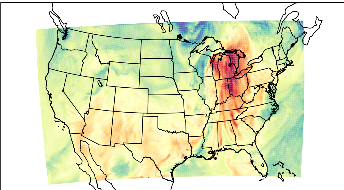
WRF (2021-10-11_21:00:00)
