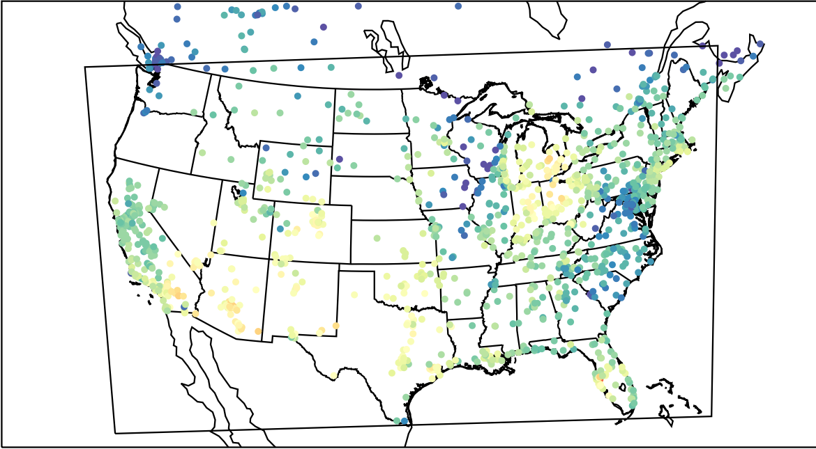
AirNOW (2021-10-11_19:00:00)
