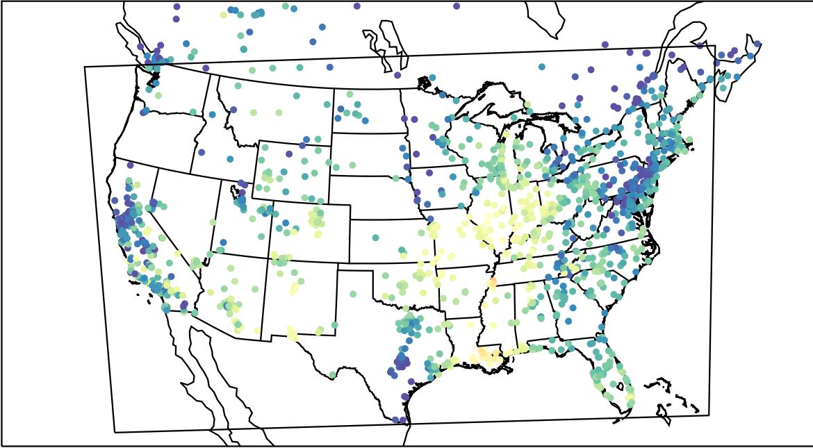
AirNOW (2021-10-10_16:00:00)
