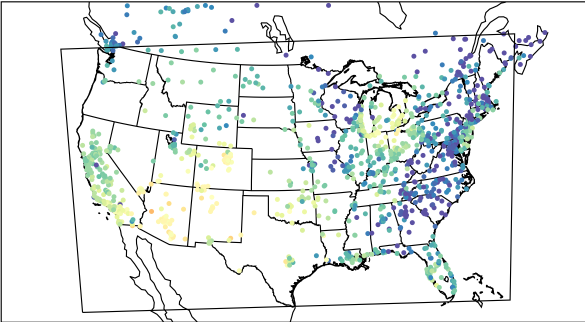
AirNOW (2021-10-11_23:00:00)
