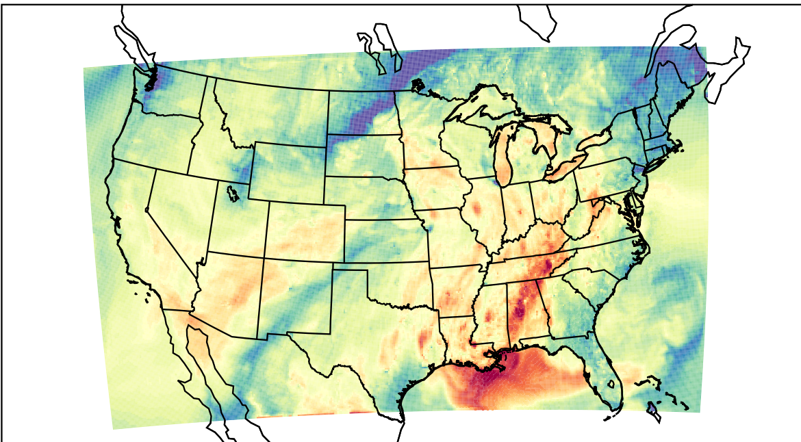
WRF (2021-10-10_00:00:00)
