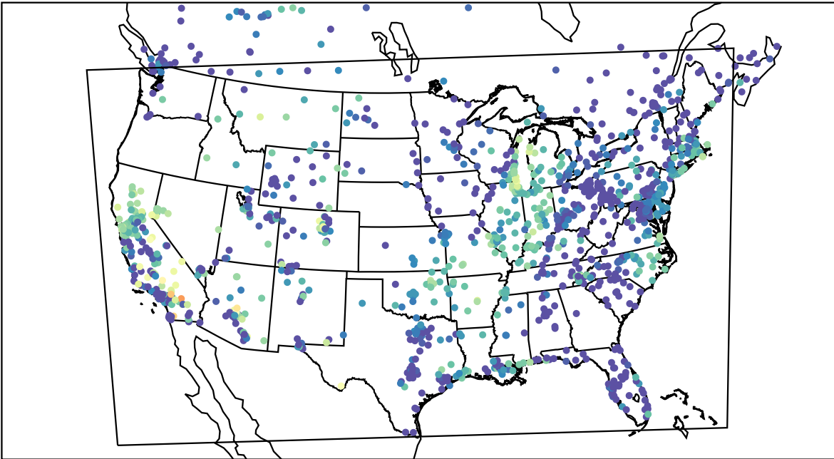
AirNOW (2021-10-11_09:00:00)
