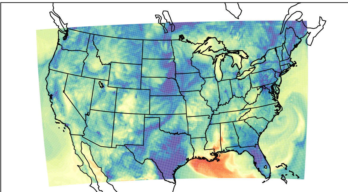
WRF (2021-10-10_12:00:00)
