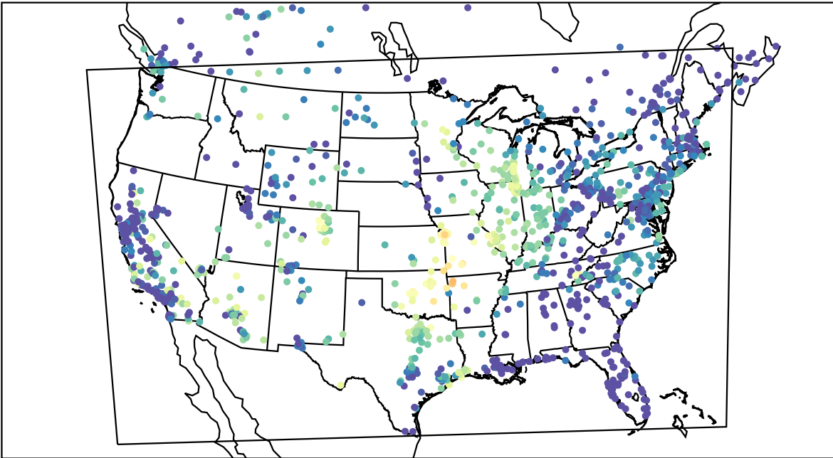
AirNOW (2021-10-10_07:00:00)
