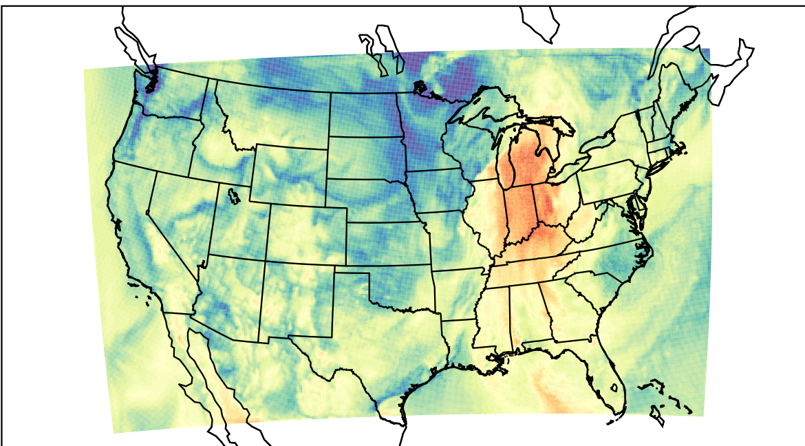
WRF (2021-10-11_16:00:00)
