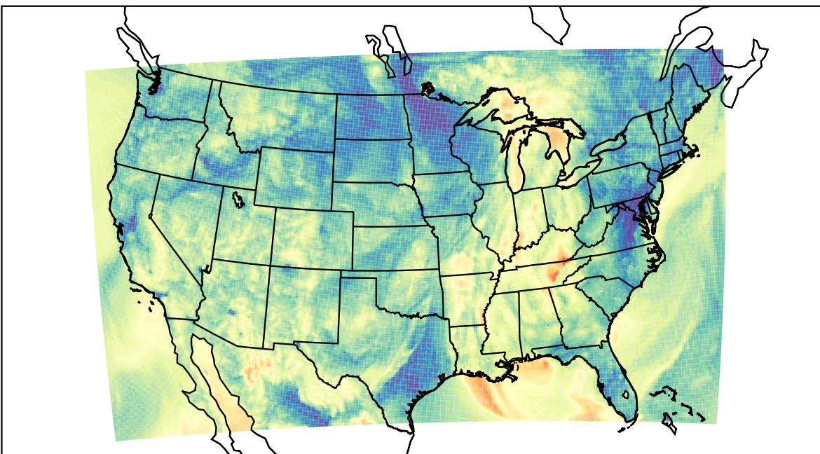
WRF (2021-10-11_05:00:00)
