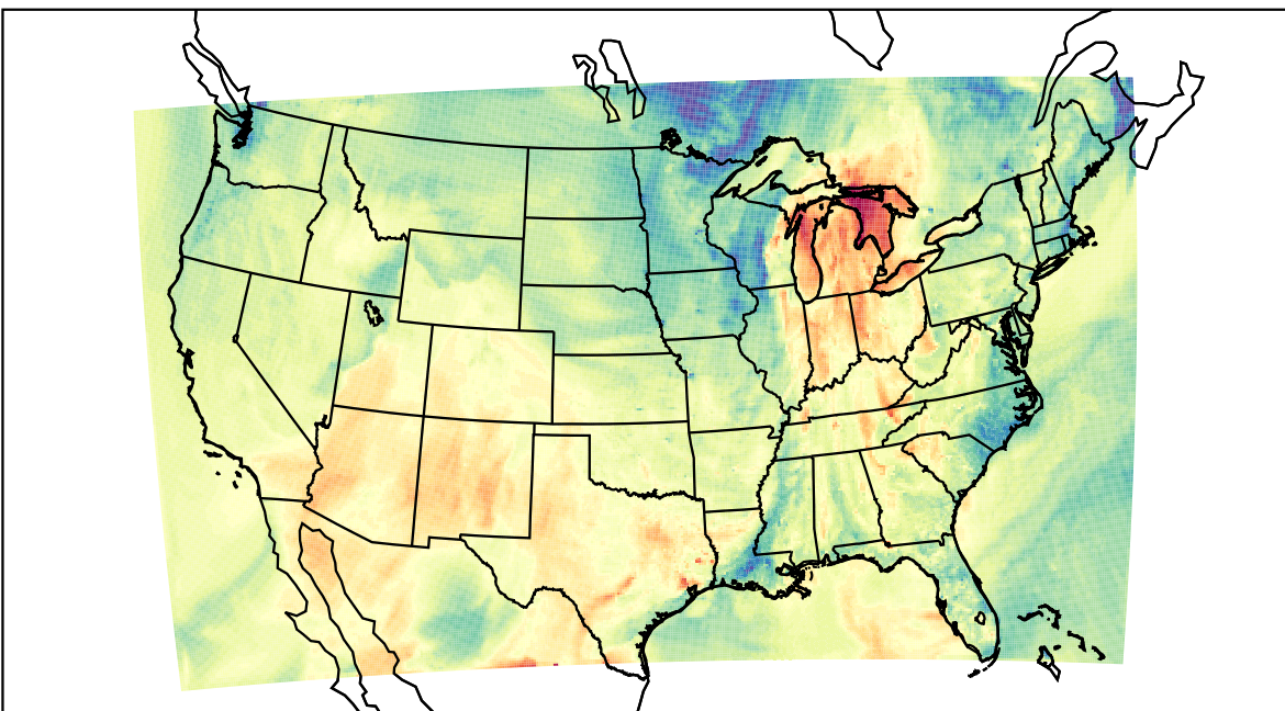
WRF (2021-10-11_23:00:00)
