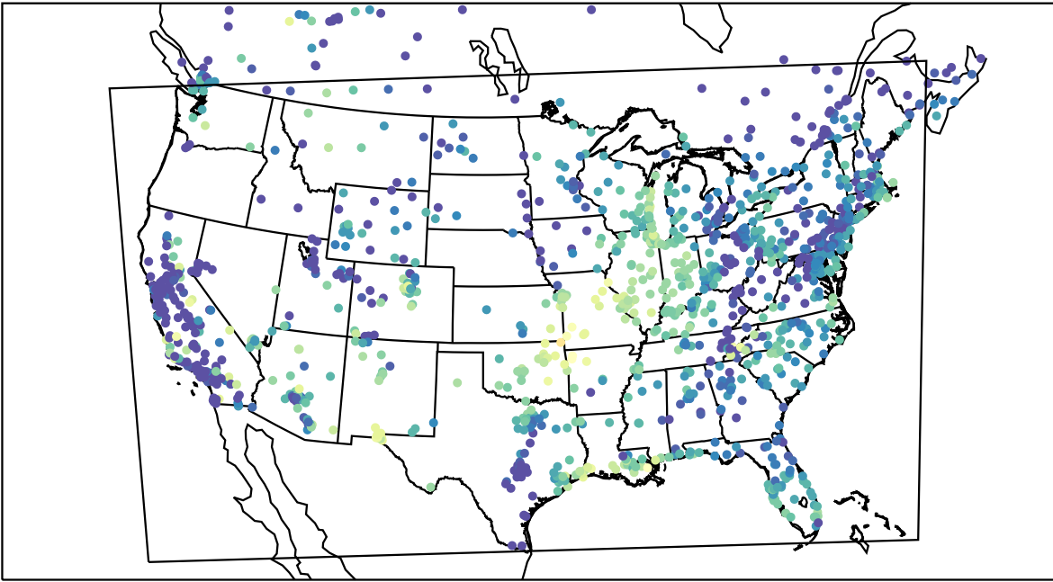
AirNOW (2021-10-10_14:00:00)
