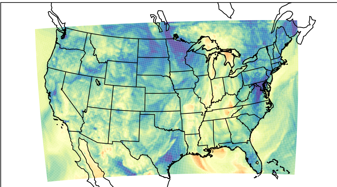
WRF (2021-10-11_06:00:00)
