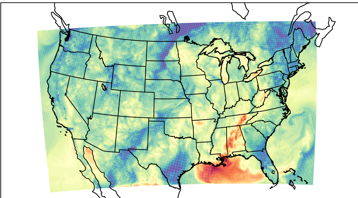
WRF (2021-10-10_05:00:00)
