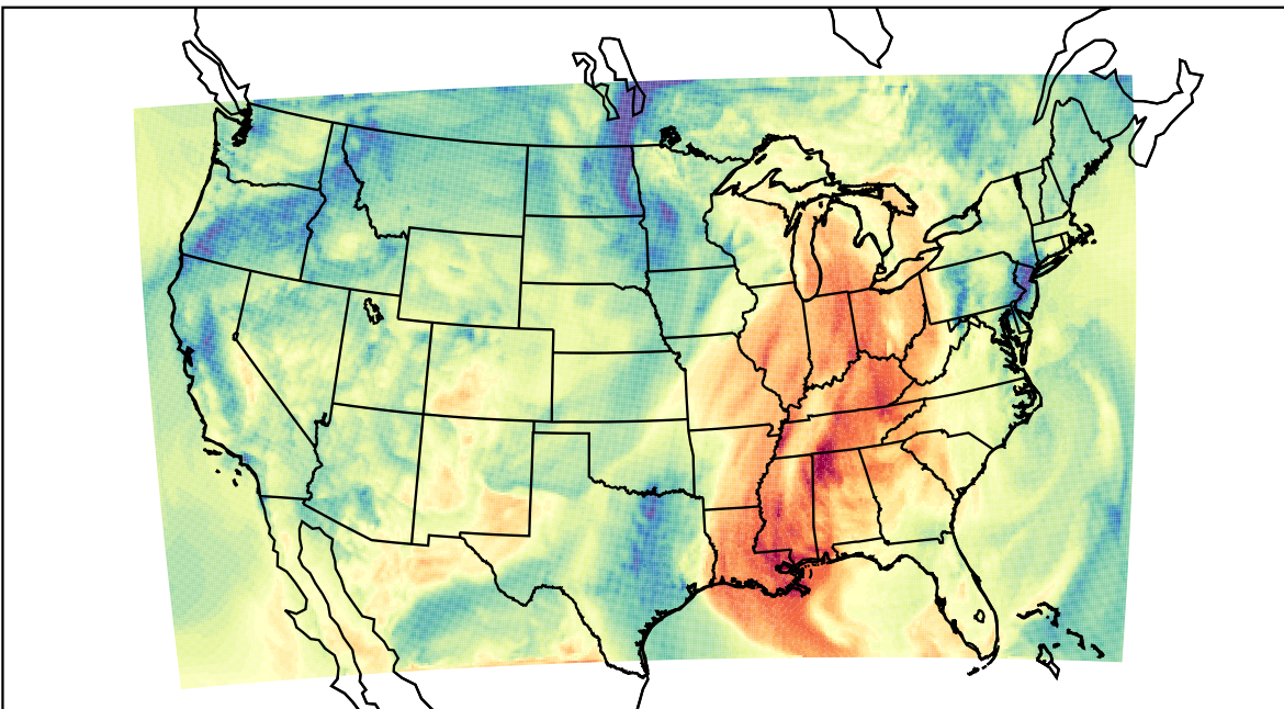
WRF (2021-10-10_17:00:00)
