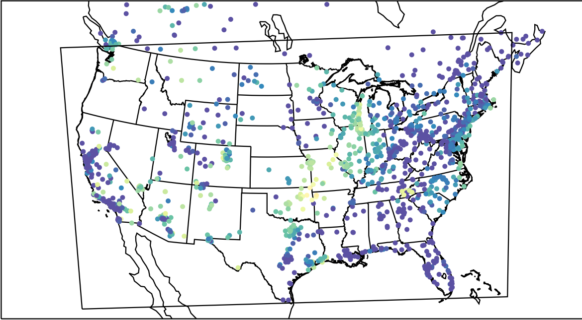
AirNOW (2021-10-10_12:00:00)
