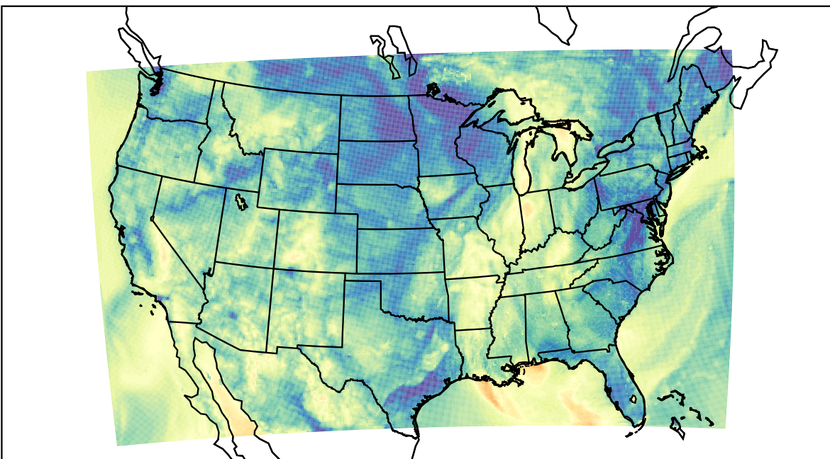
WRF (2021-10-11_09:00:00)
