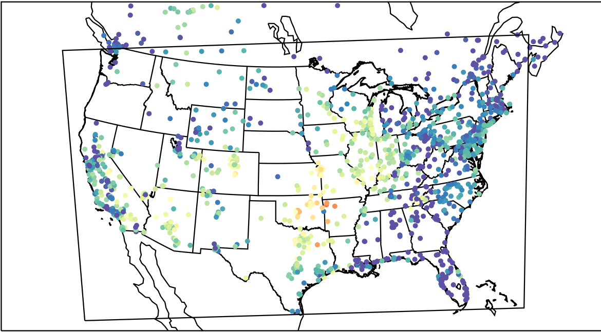
AirNOW (2021-10-10_03:00:00)
