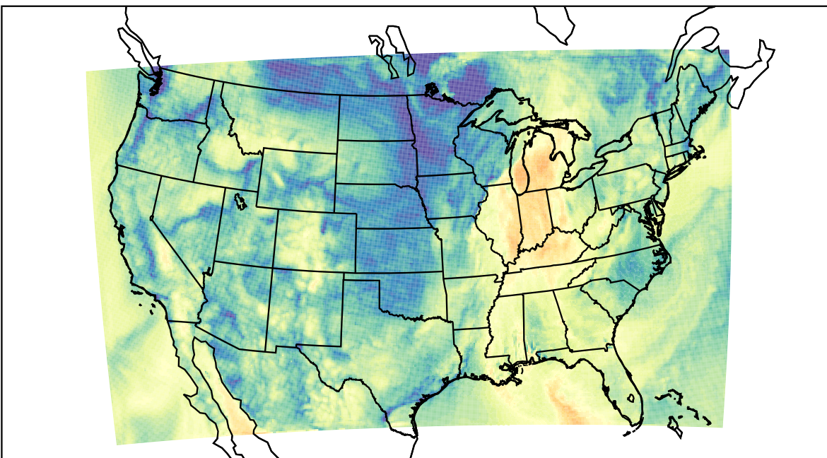
WRF (2021-10-11_15:00:00)
