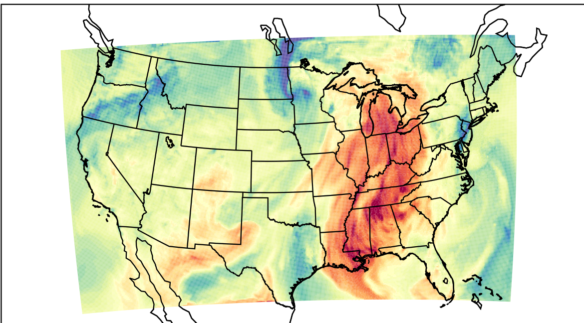
WRF (2021-10-10_19:00:00)
