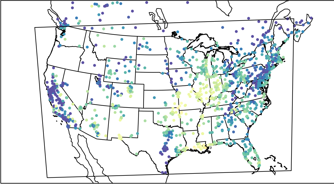
AirNOW (2021-10-10_15:00:00)
