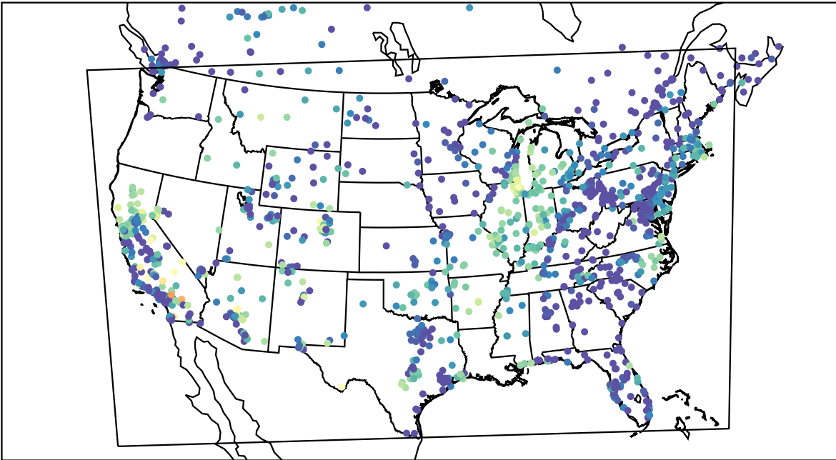
AirNOW (2021-10-11_07:00:00)
