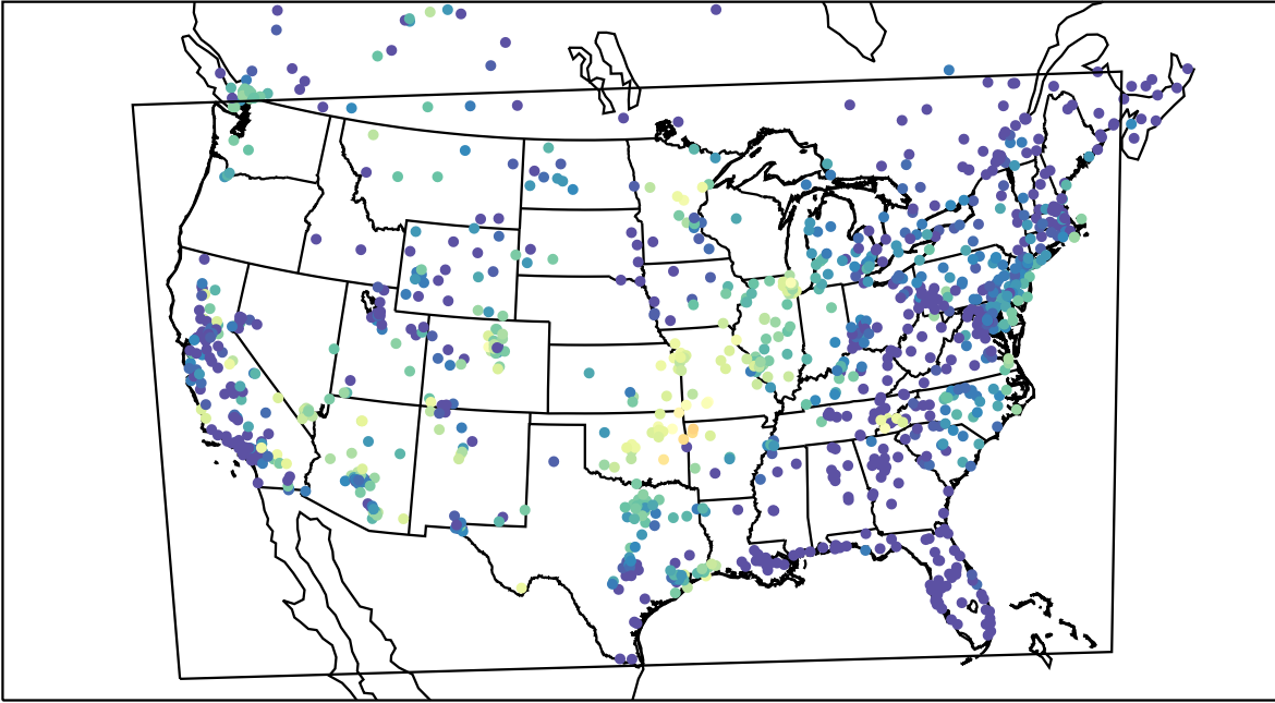
AirNOW (2021-10-10_10:00:00)
