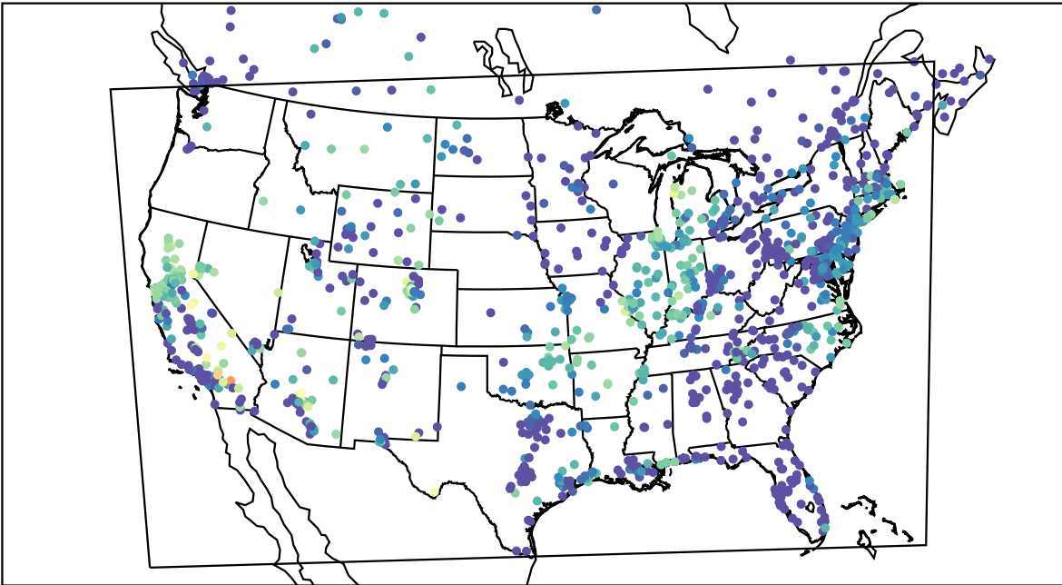
AirNOW (2021-10-11_10:00:00)
