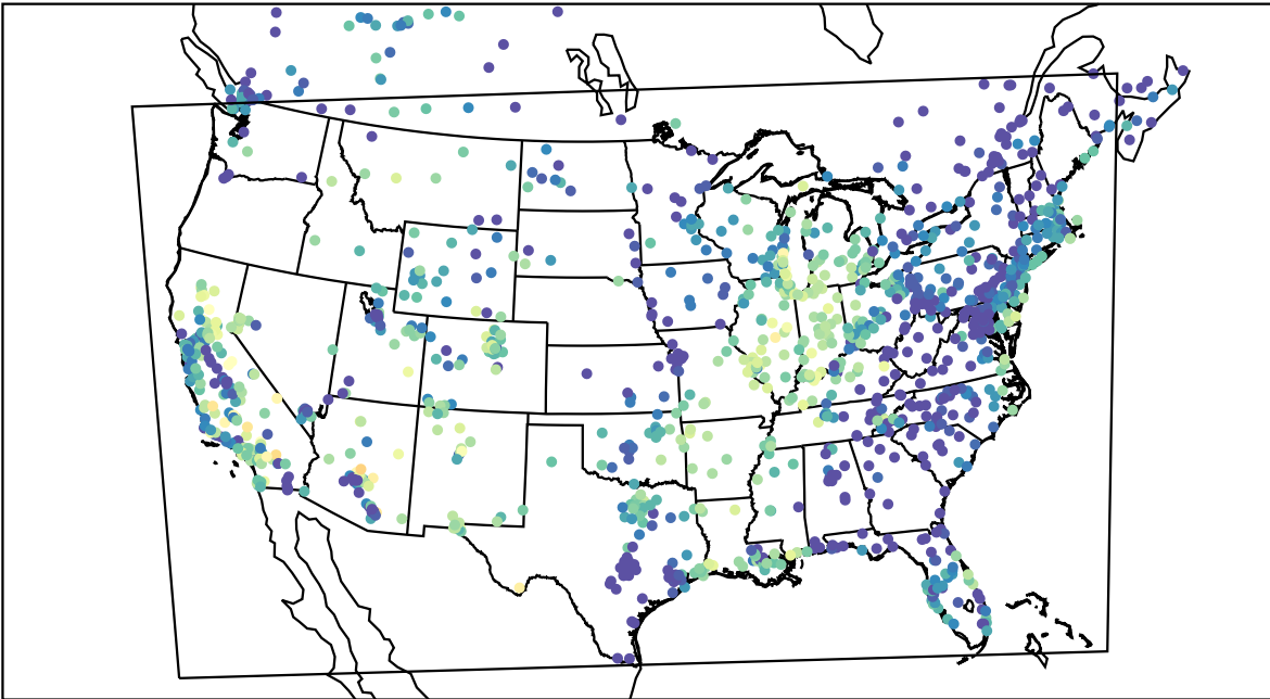
AirNOW (2021-10-11_03:00:00)
