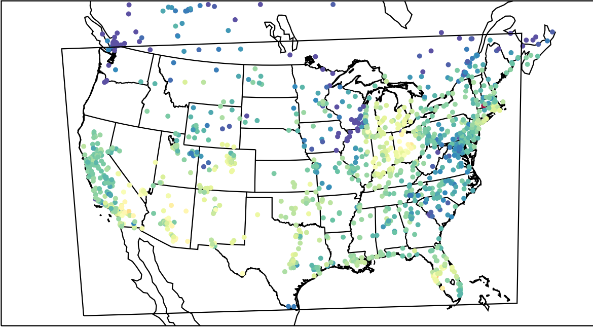
AirNOW (2021-10-11_17:00:00)
