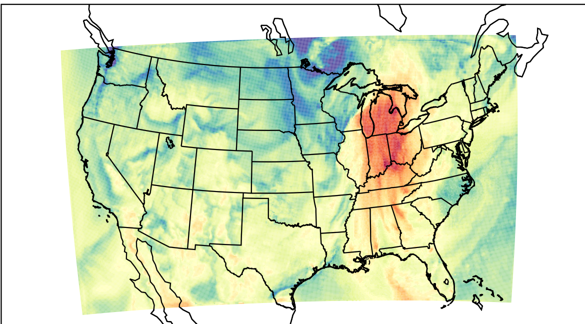
WRF (2021-10-11_17:00:00)
