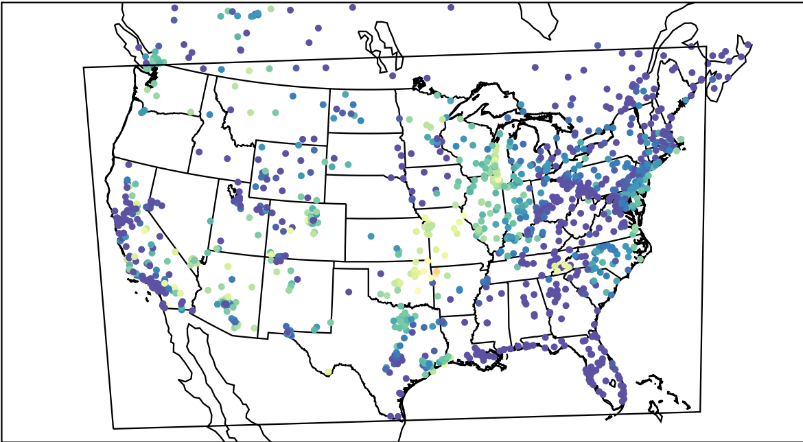
AirNOW (2021-10-10_11:00:00)
