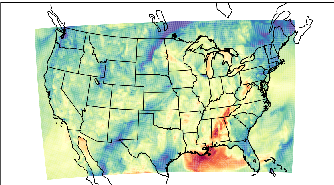
WRF (2021-10-10_03:00:00)
