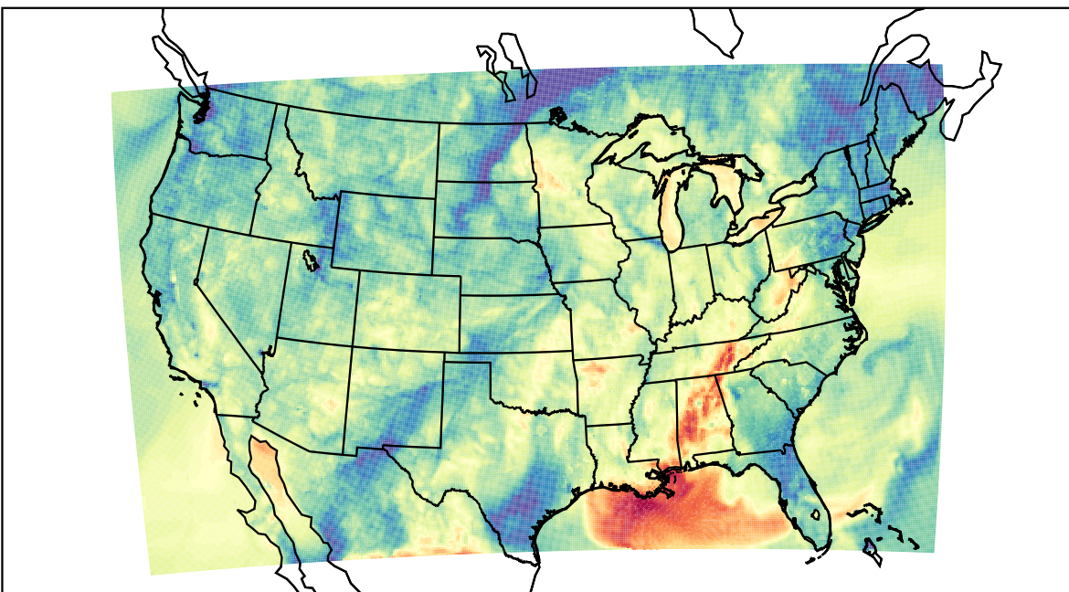
WRF (2021-10-10_04:00:00)
