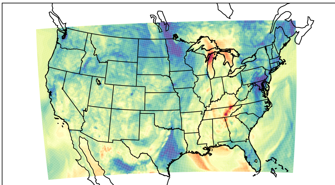
WRF (2021-10-11_03:00:00)
