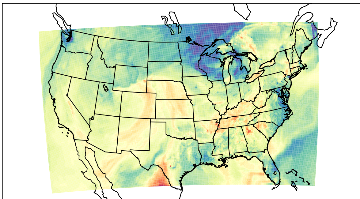
WRF (2021-10-12_23:00:00)
