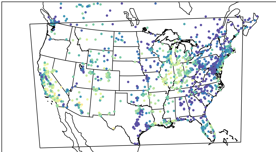
AirNOW (2021-10-11_02:00:00)
