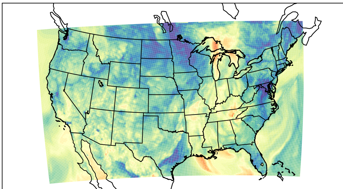
WRF (2021-10-11_06:00:00)
