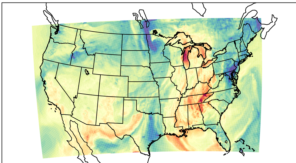
WRF (2021-10-11_00:00:00)
