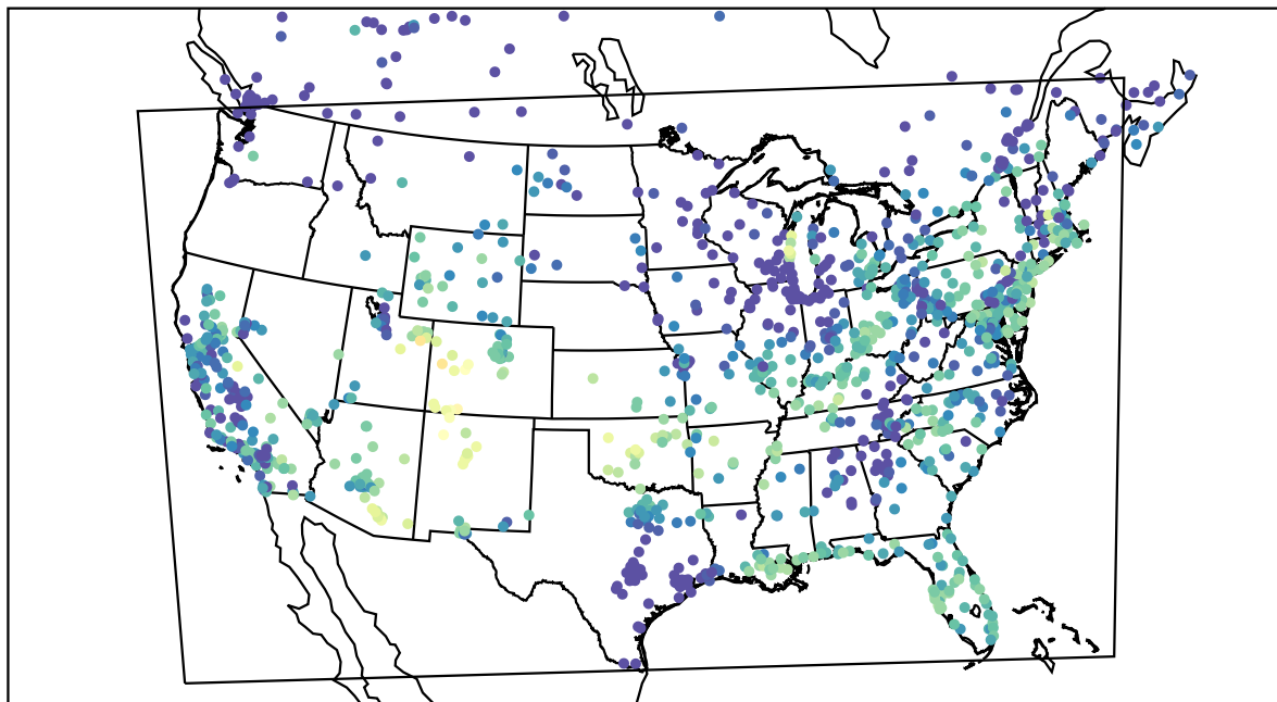
AirNOW (2021-10-12_15:00:00)
