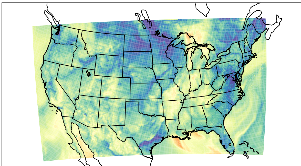
WRF (2021-10-11_08:00:00)
