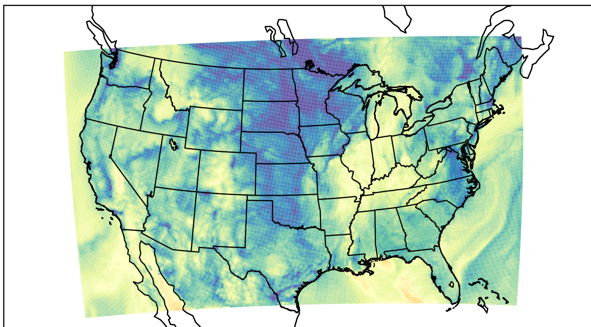
WRF (2021-10-11_14:00:00)
