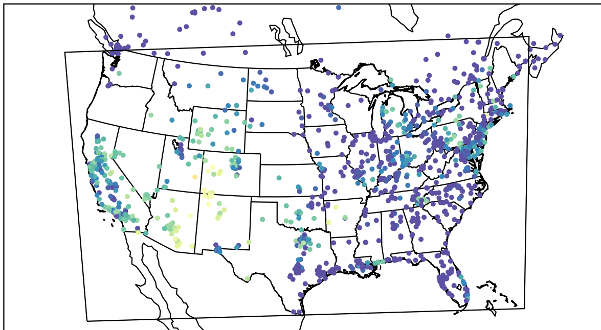
AirNOW (2021-10-12_10:00:00)
