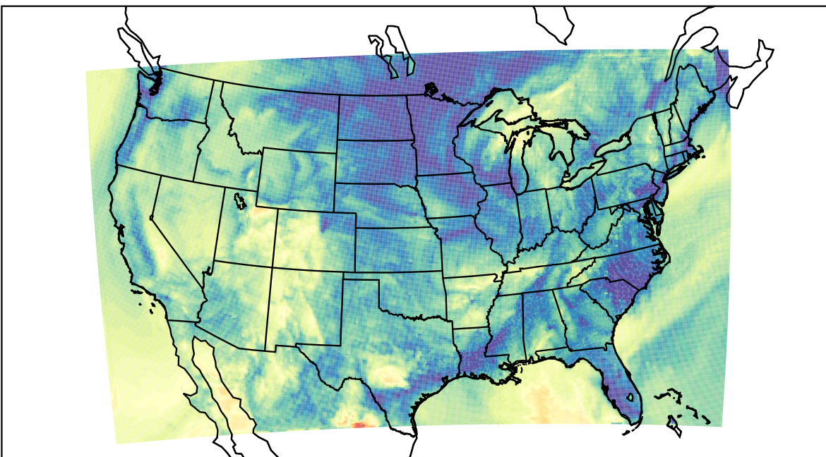
WRF (2021-10-12_11:00:00)
