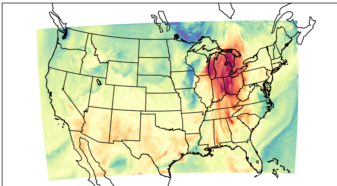
WRF (2021-10-11_20:00:00)
