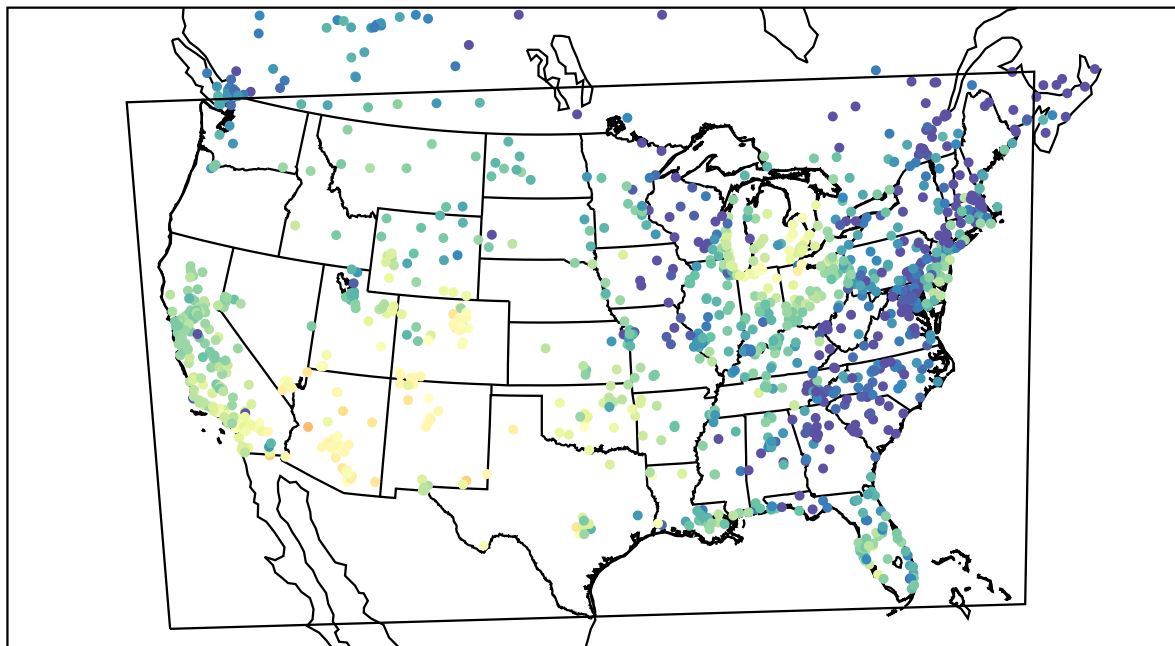
AirNOW (2021-10-11_23:00:00)
