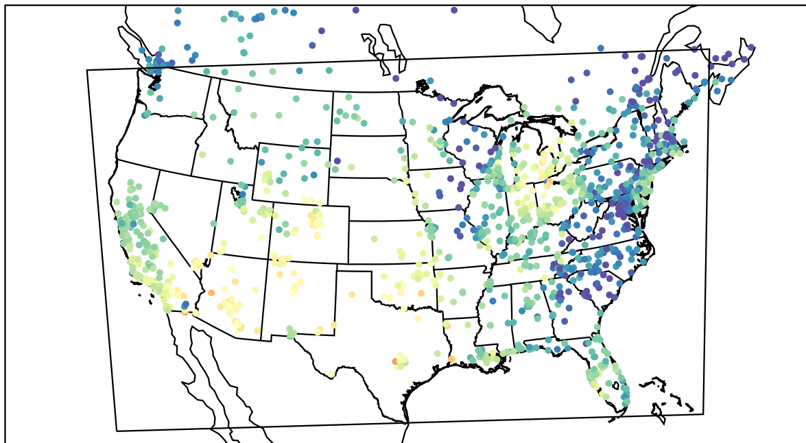
AirNOW (2021-10-11_22:00:00)
