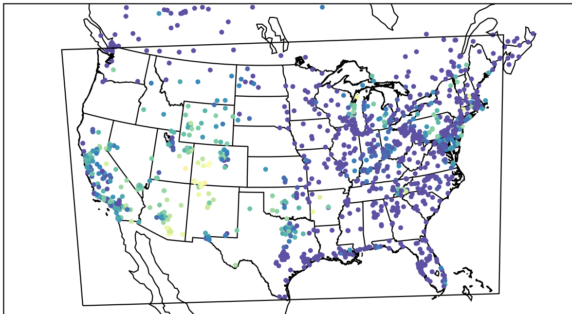
AirNOW (2021-10-12_12:00:00)
