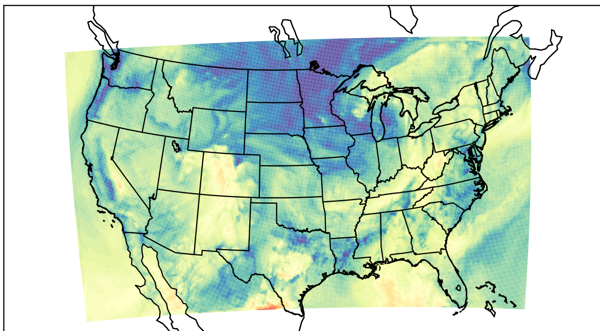
WRF (2021-10-12_15:00:00)
