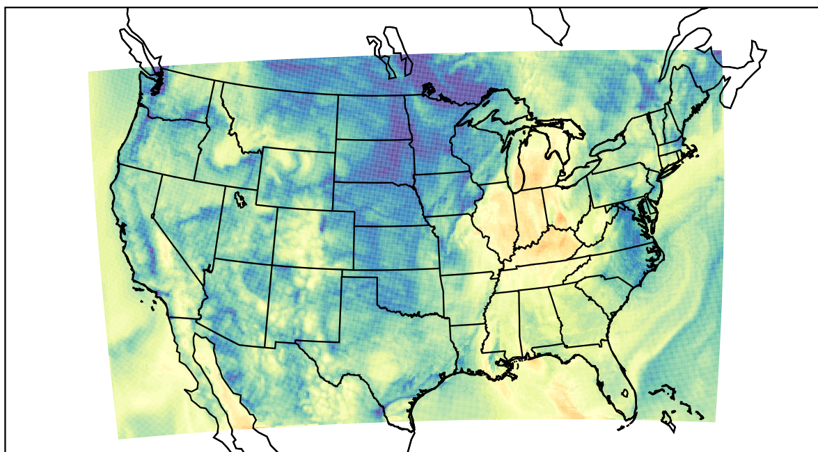
WRF (2021-10-11_15:00:00)
