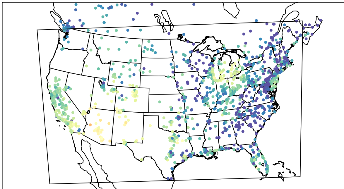
AirNOW (2021-10-12_00:00:00)
