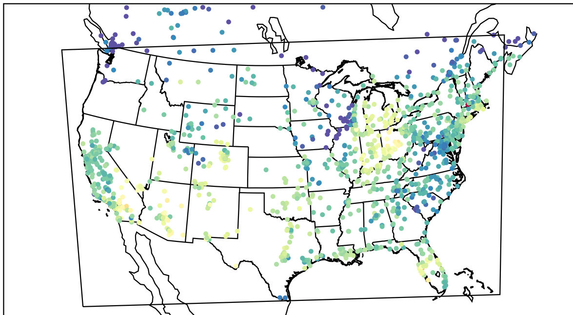
AirNOW (2021-10-11_17:00:00)
