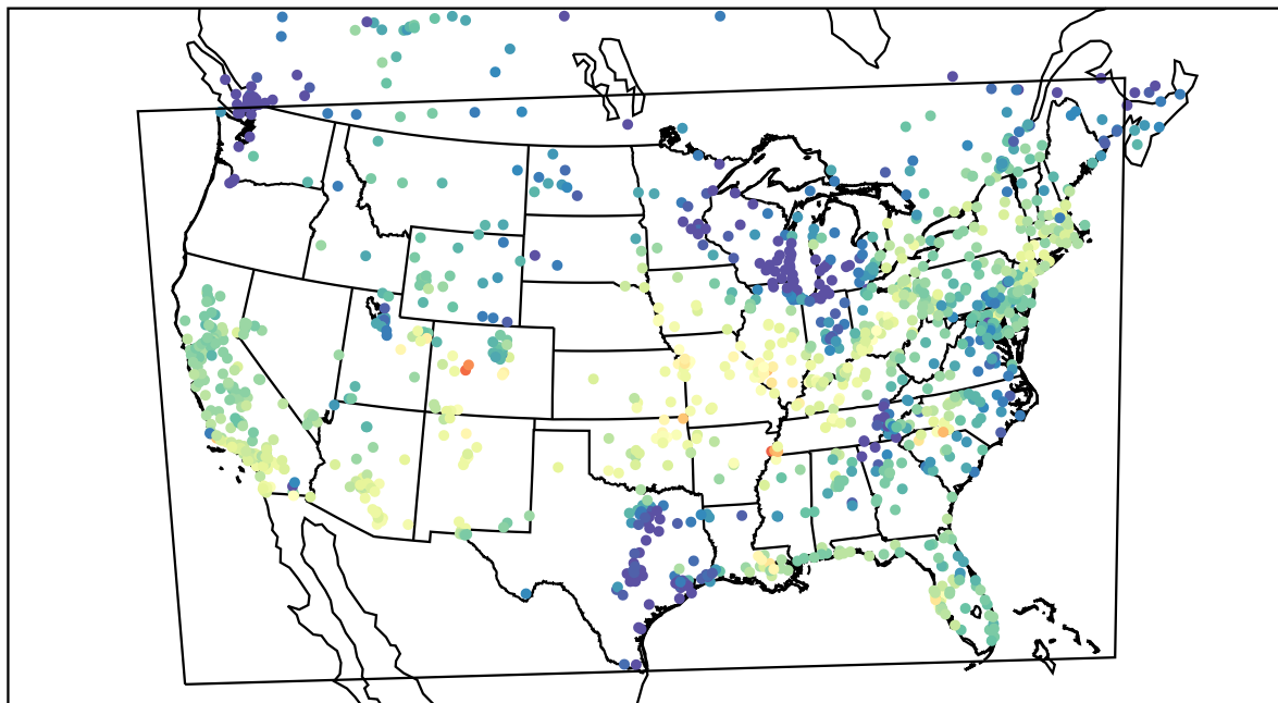
AirNOW (2021-10-12_20:00:00)
