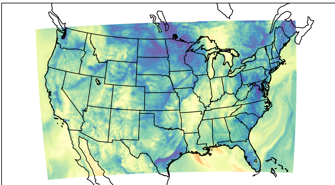
WRF (2021-10-11_09:00:00)
