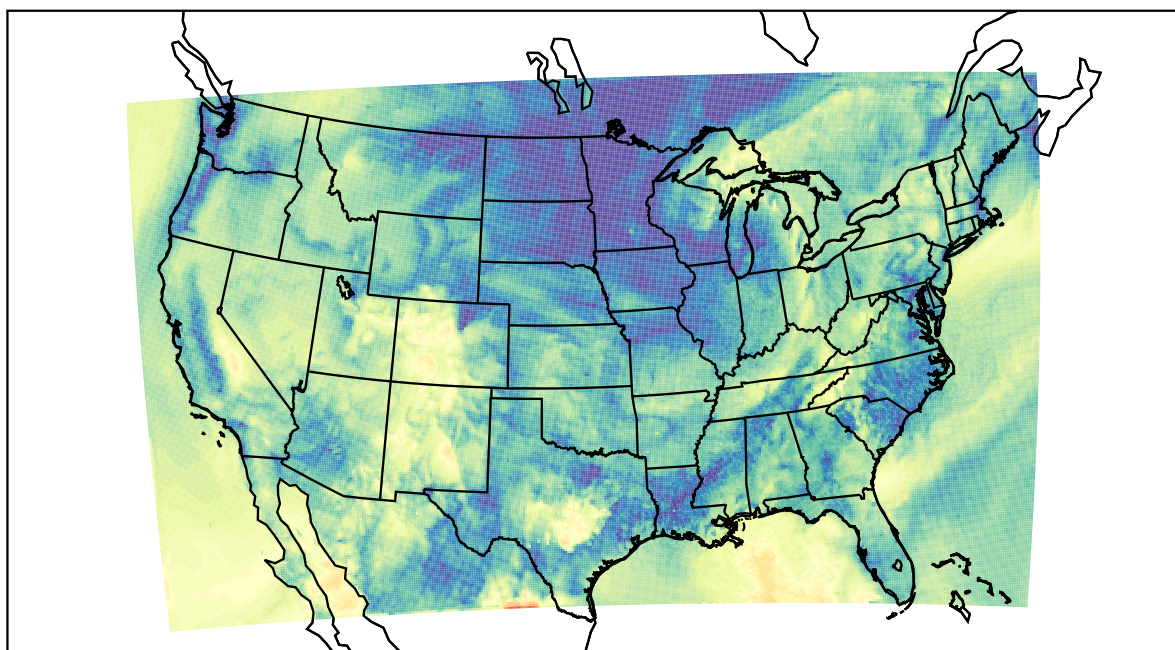
WRF (2021-10-12_14:00:00)
