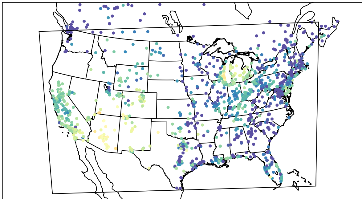
AirNOW (2021-10-12_02:00:00)
