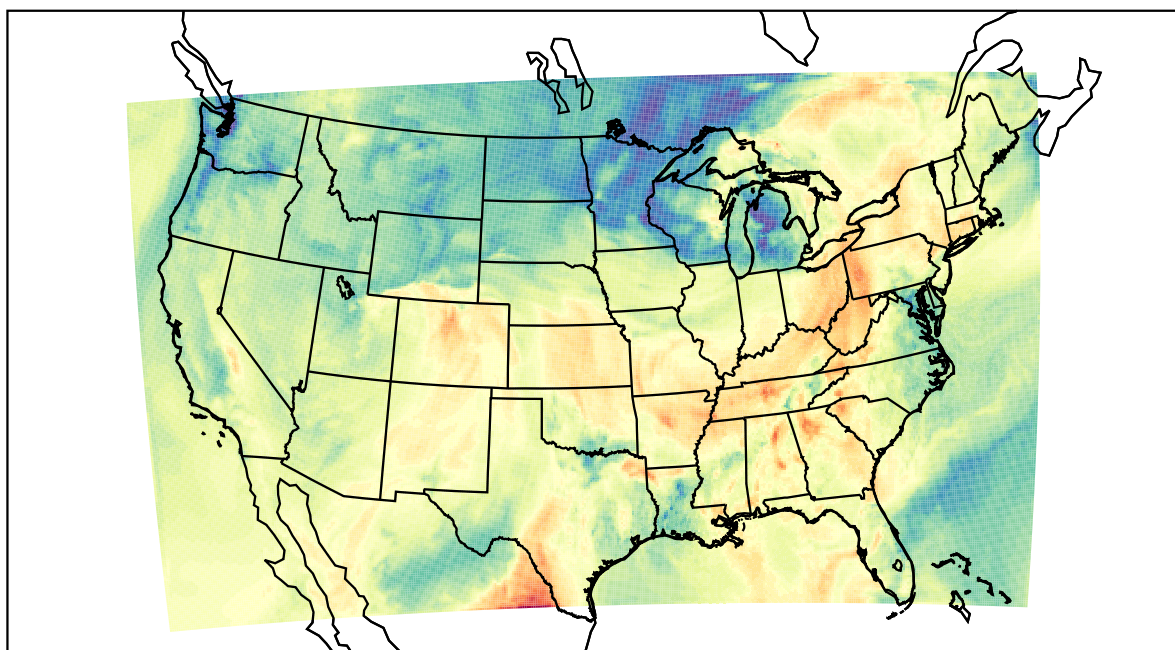
WRF (2021-10-12_18:00:00)
