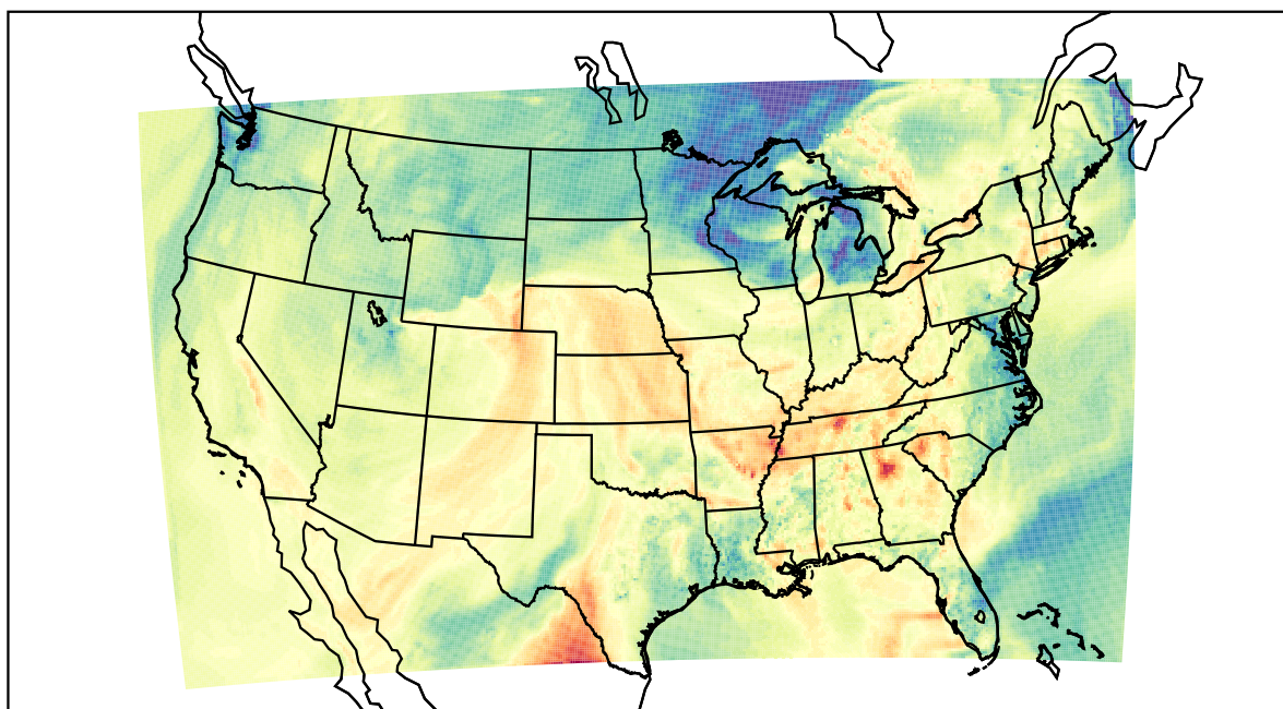
WRF (2021-10-12_22:00:00)
