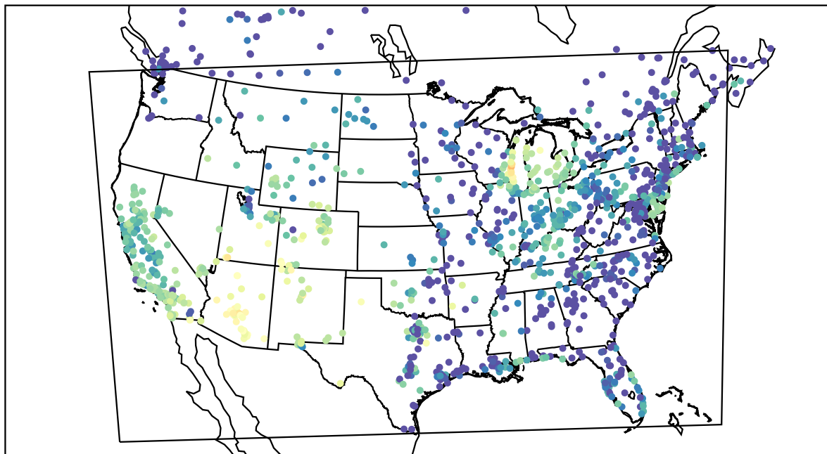
AirNOW (2021-10-12_03:00:00)
