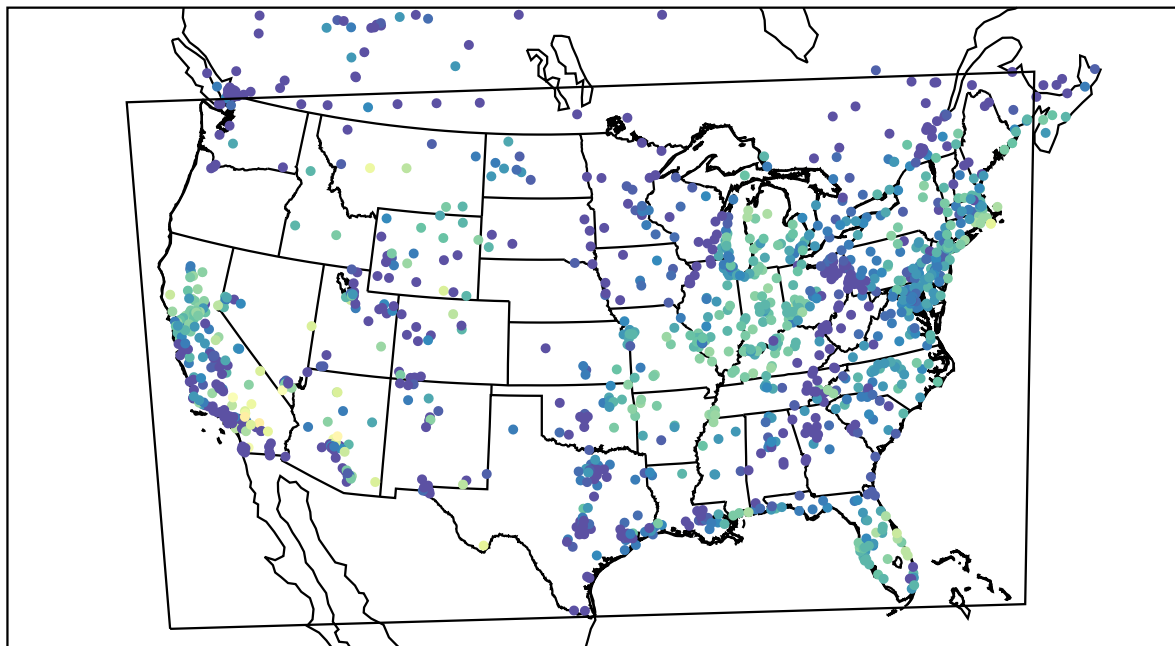
AirNOW (2021-10-11_14:00:00)
