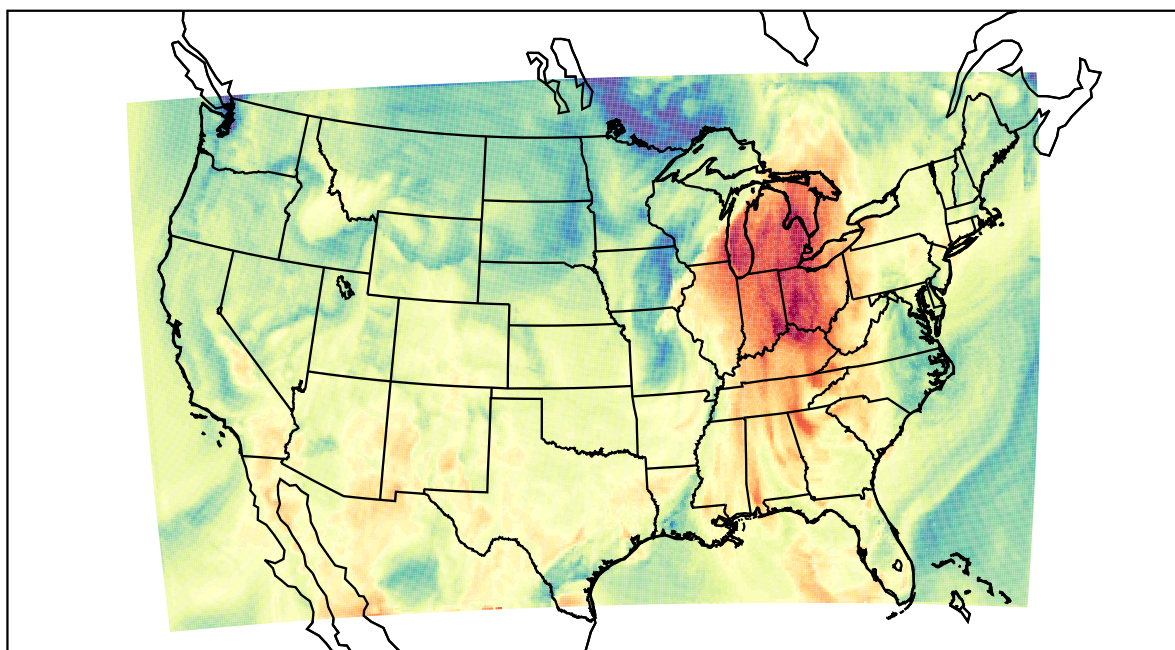
WRF (2021-10-11_18:00:00)
