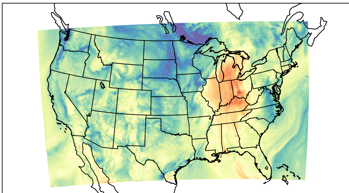
WRF (2021-10-11_16:00:00)
