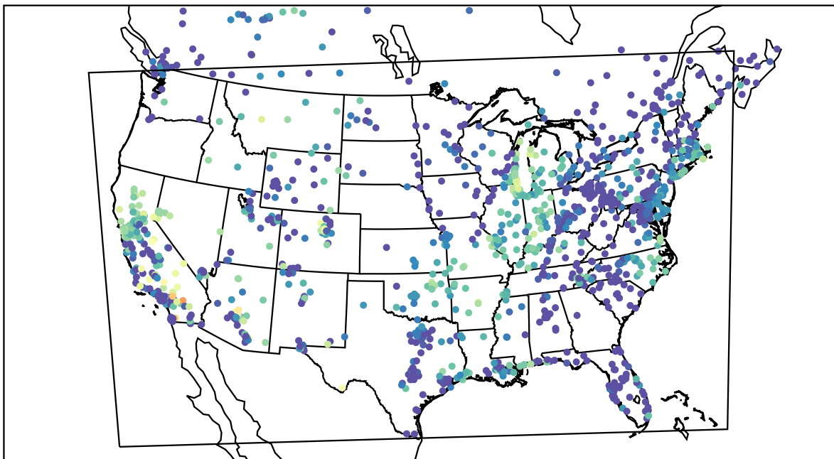
AirNOW (2021-10-11_09:00:00)
