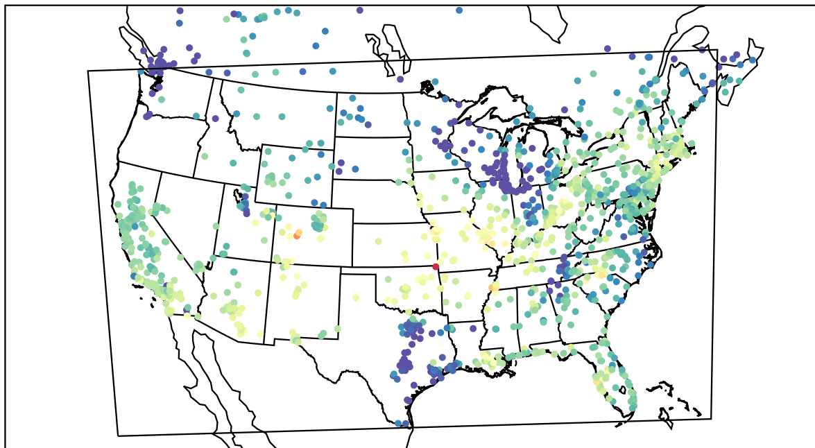
AirNOW (2021-10-12_19:00:00)
