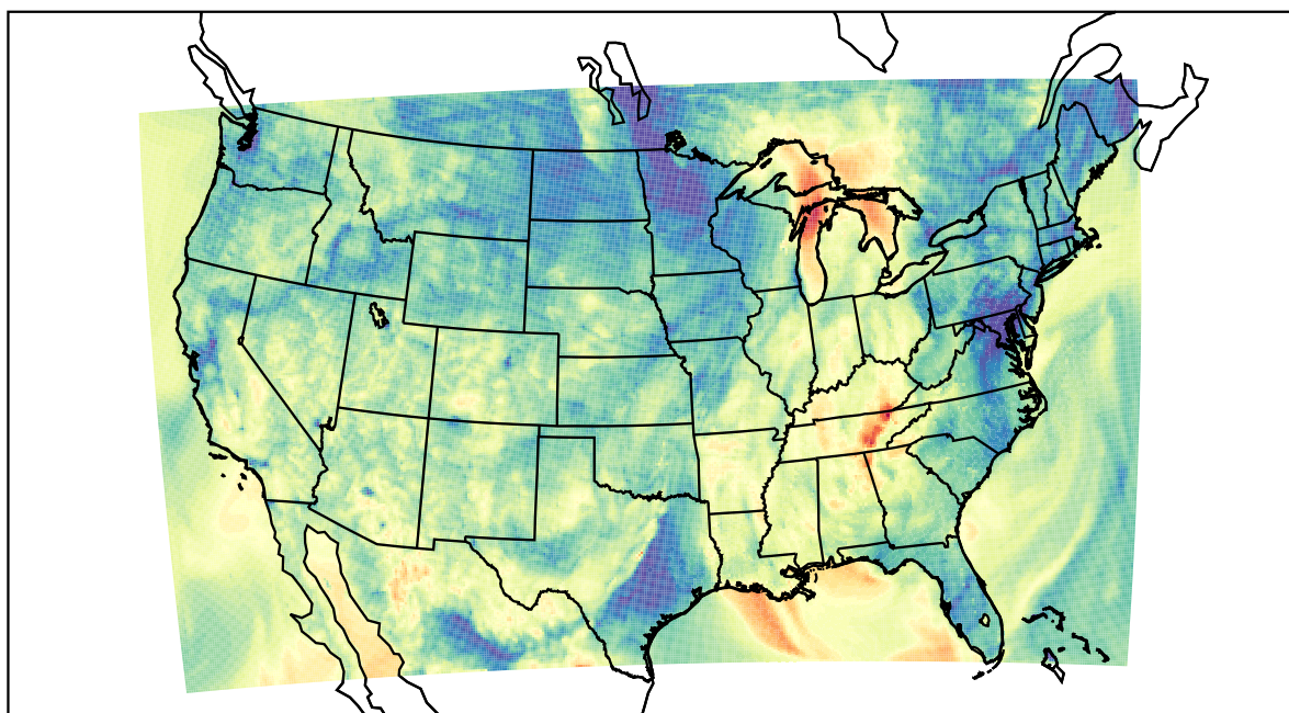
WRF (2021-10-11_04:00:00)
