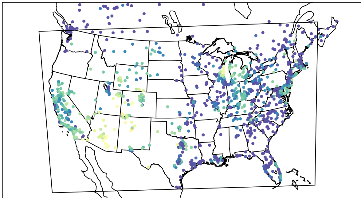
AirNOW (2021-10-12_06:00:00)
