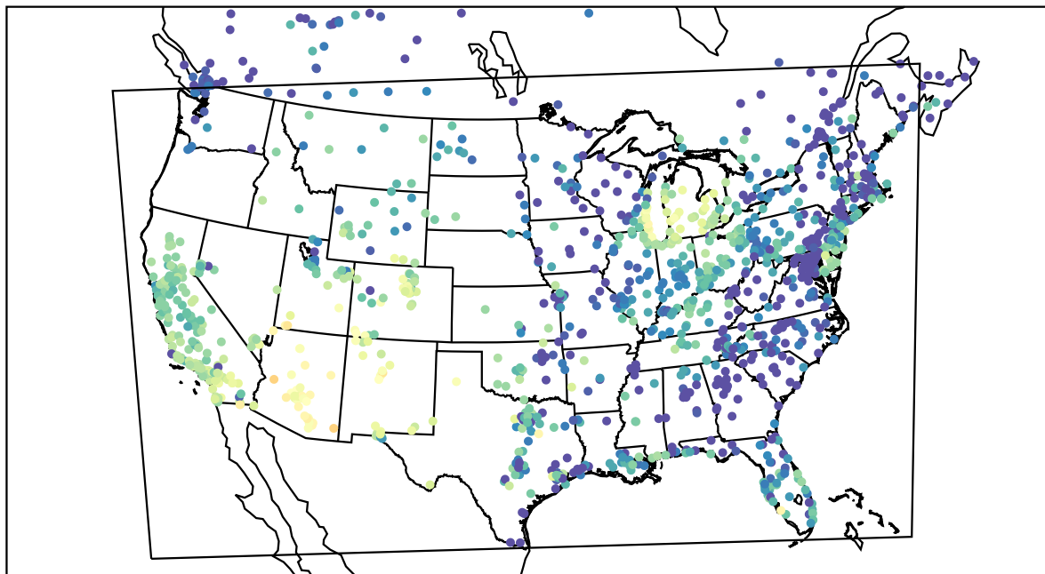
AirNOW (2021-10-12_01:00:00)
