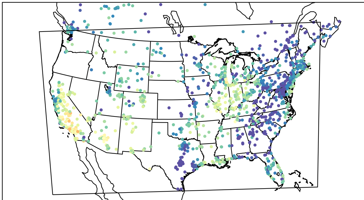
AirNOW (2021-10-11_01:00:00)
