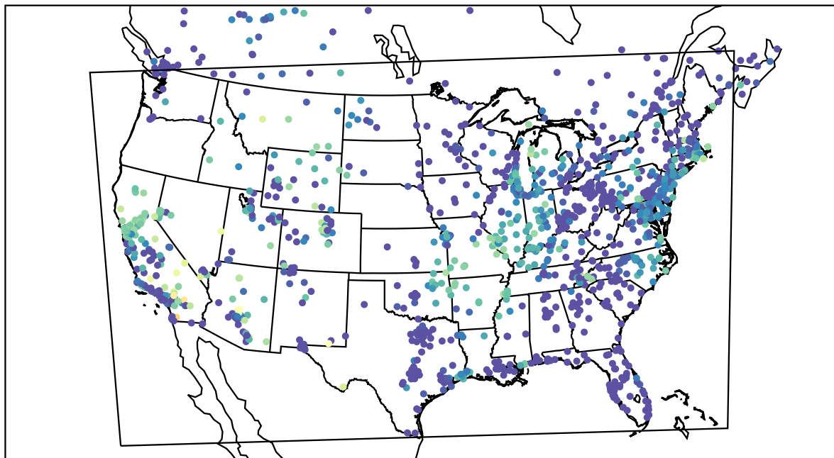
AirNOW (2021-10-11_12:00:00)
