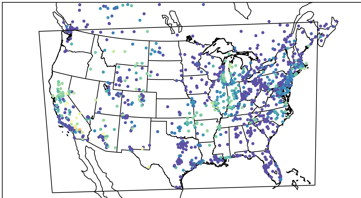
AirNOW (2021-10-11_11:00:00)
