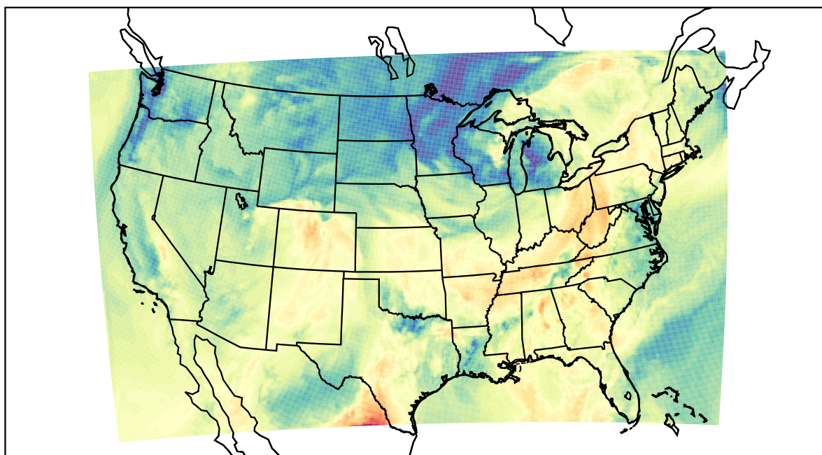
WRF (2021-10-12_17:00:00)
