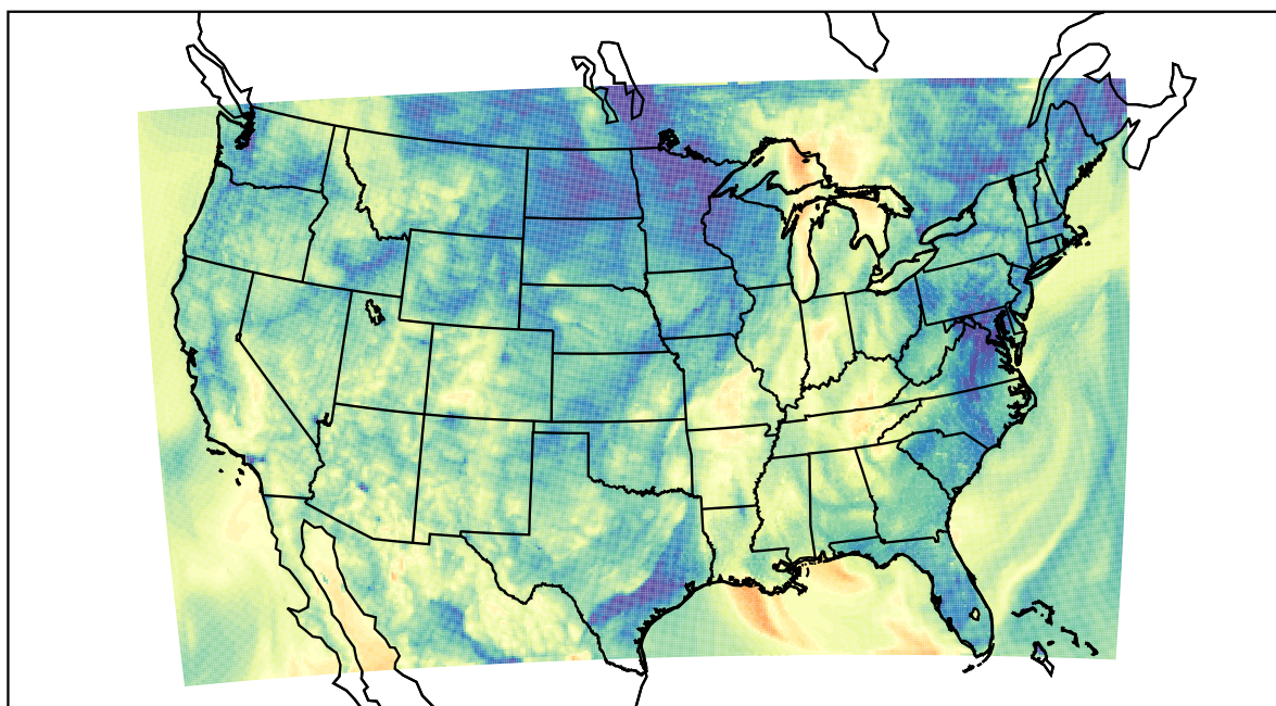
WRF (2021-10-11_07:00:00)
