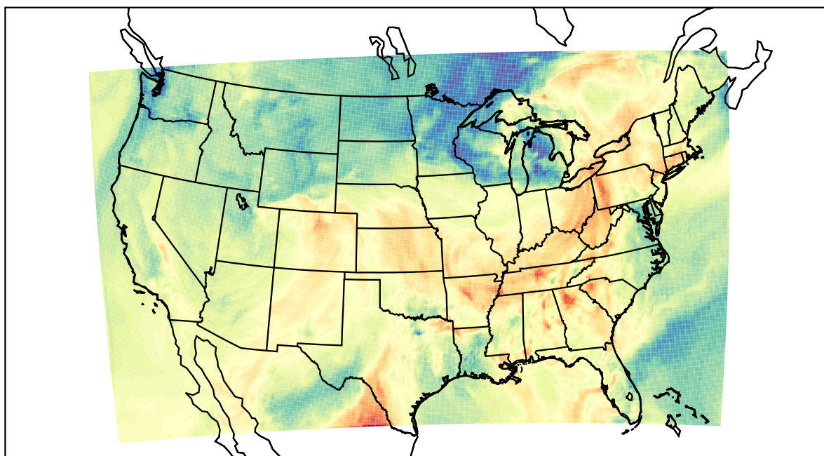
WRF (2021-10-12_19:00:00)
