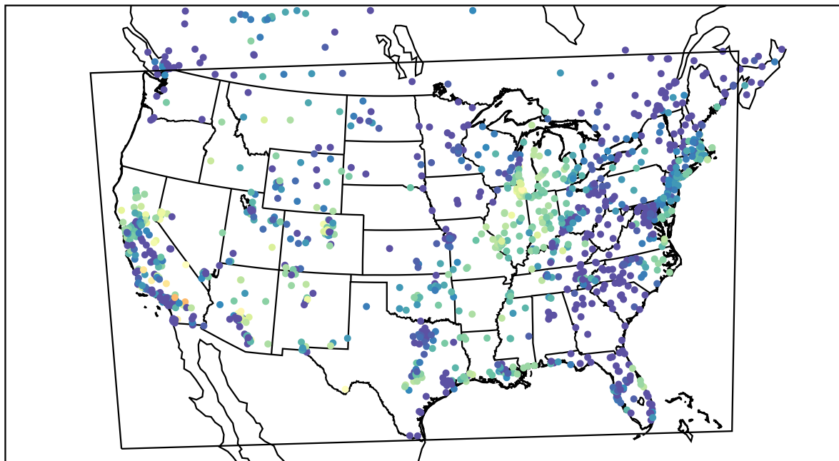
AirNOW (2021-10-11_06:00:00)
