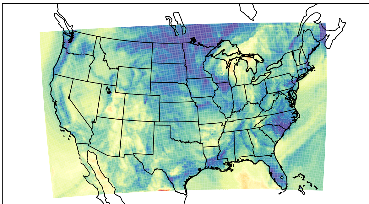
WRF (2021-10-12_08:00:00)
