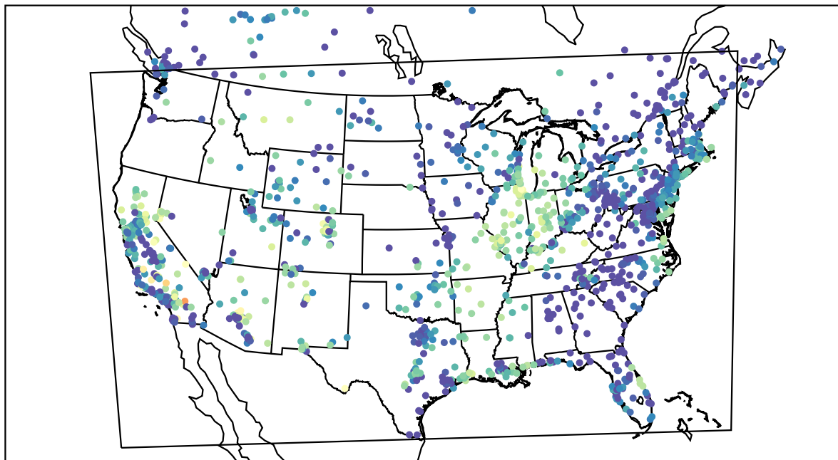
AirNOW (2021-10-11_05:00:00)
