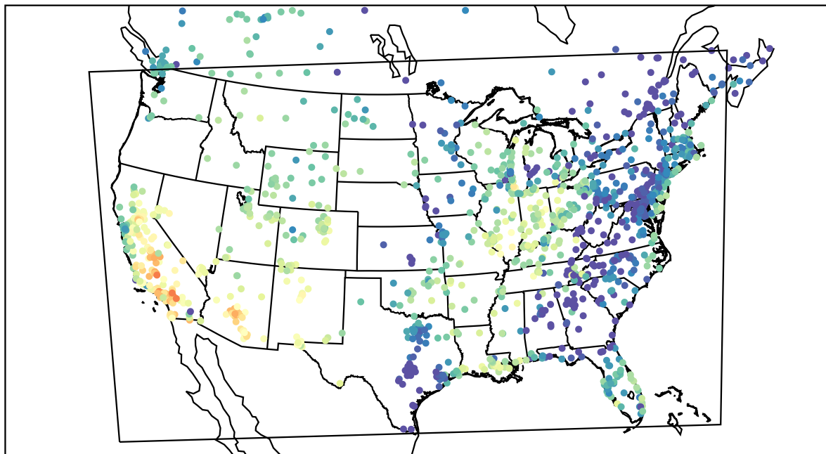
AirNOW (2021-10-11_00:00:00)
