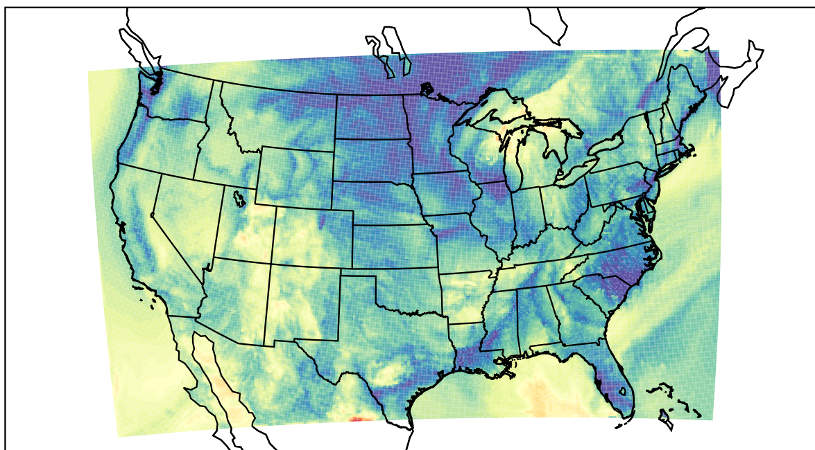
WRF (2021-10-12_09:00:00)
