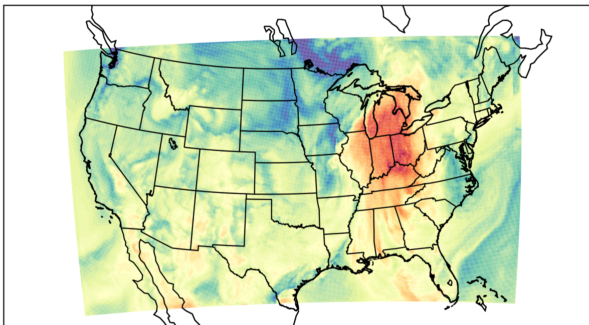
WRF (2021-10-11_17:00:00)
