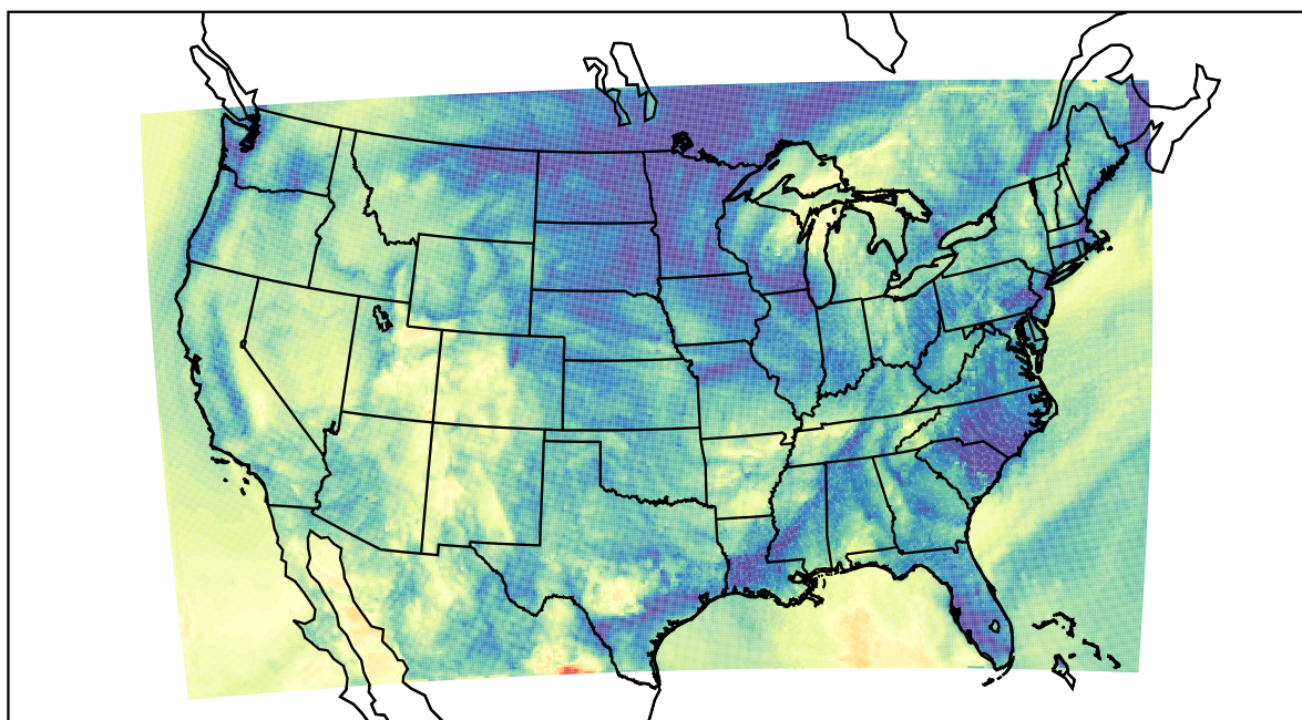
WRF (2021-10-12_10:00:00)
