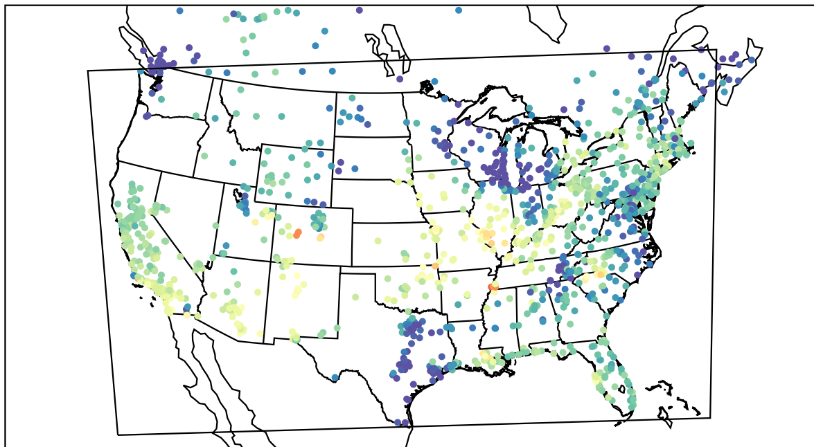
AirNOW (2021-10-12_21:00:00)
