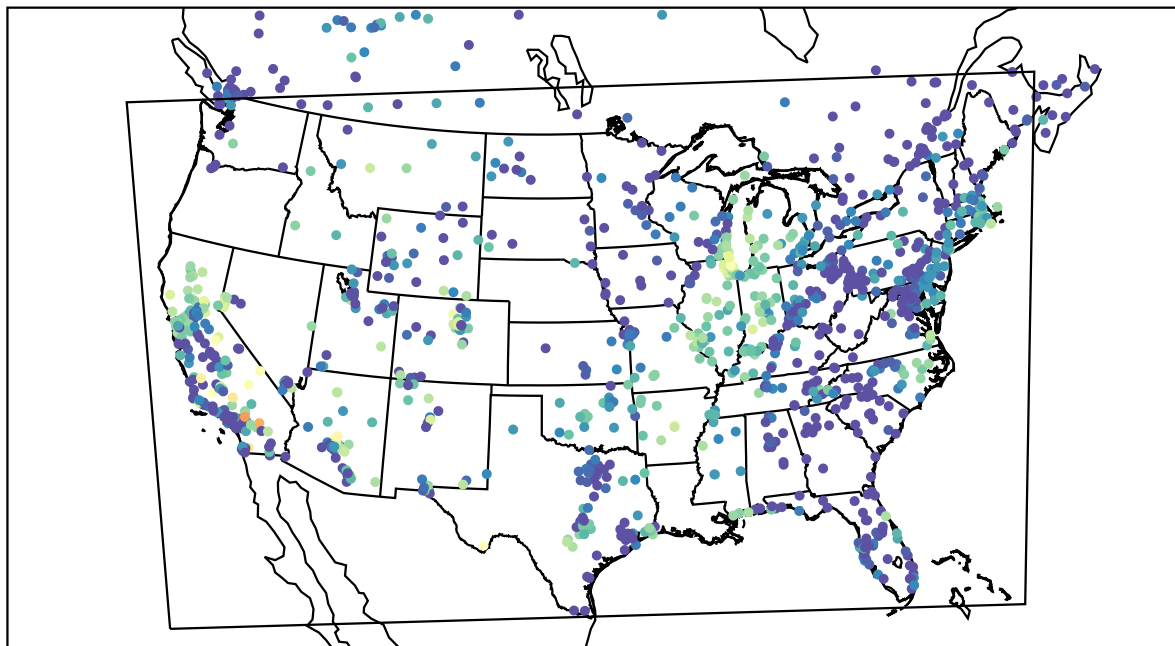
AirNOW (2021-10-11_07:00:00)
