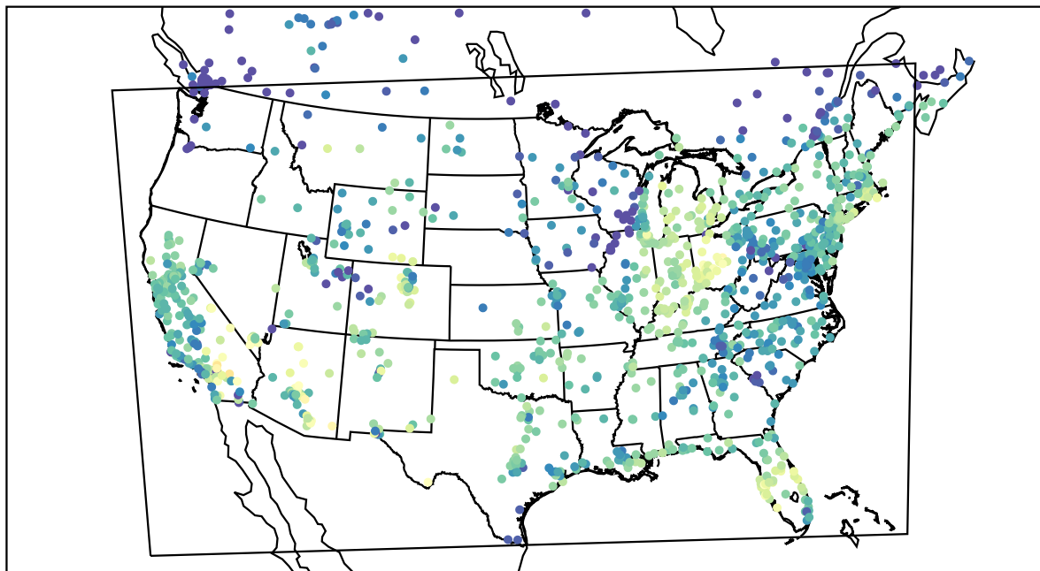
AirNOW (2021-10-11_16:00:00)
