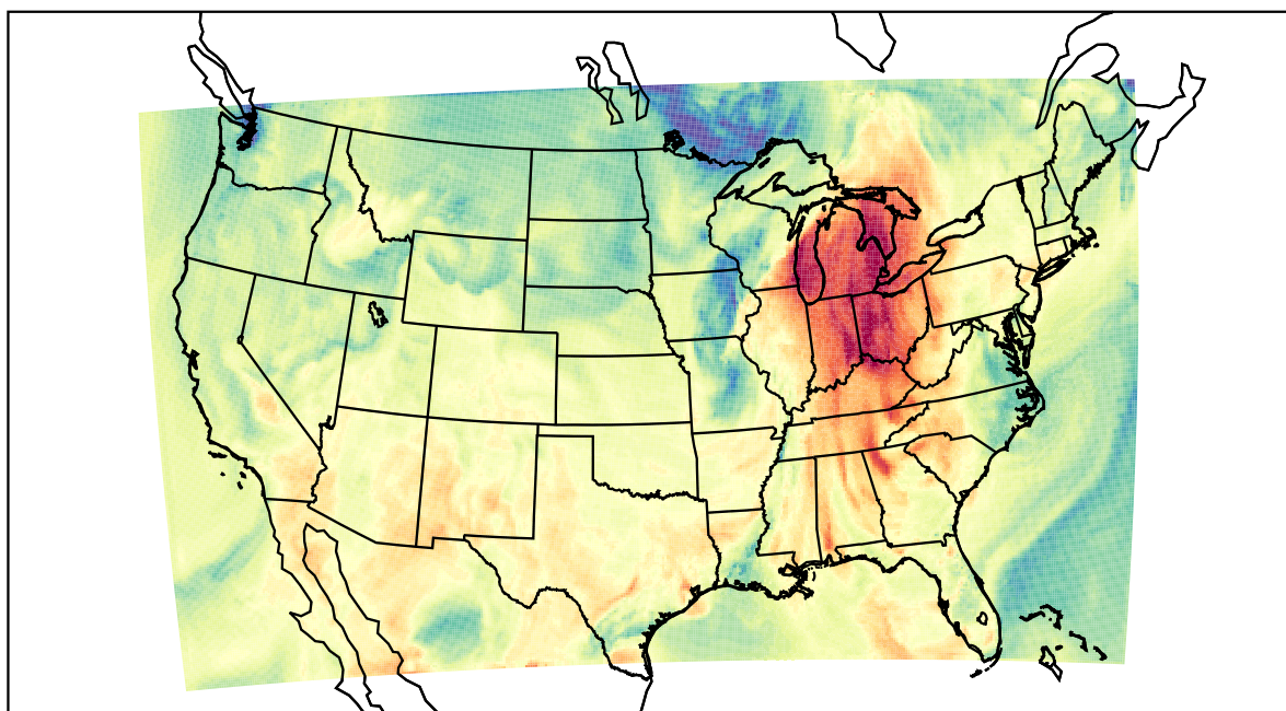
WRF (2021-10-11_19:00:00)
