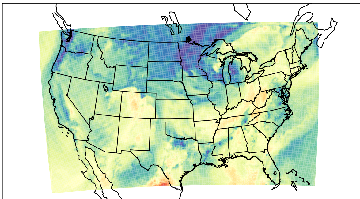
WRF (2021-10-12_16:00:00)
