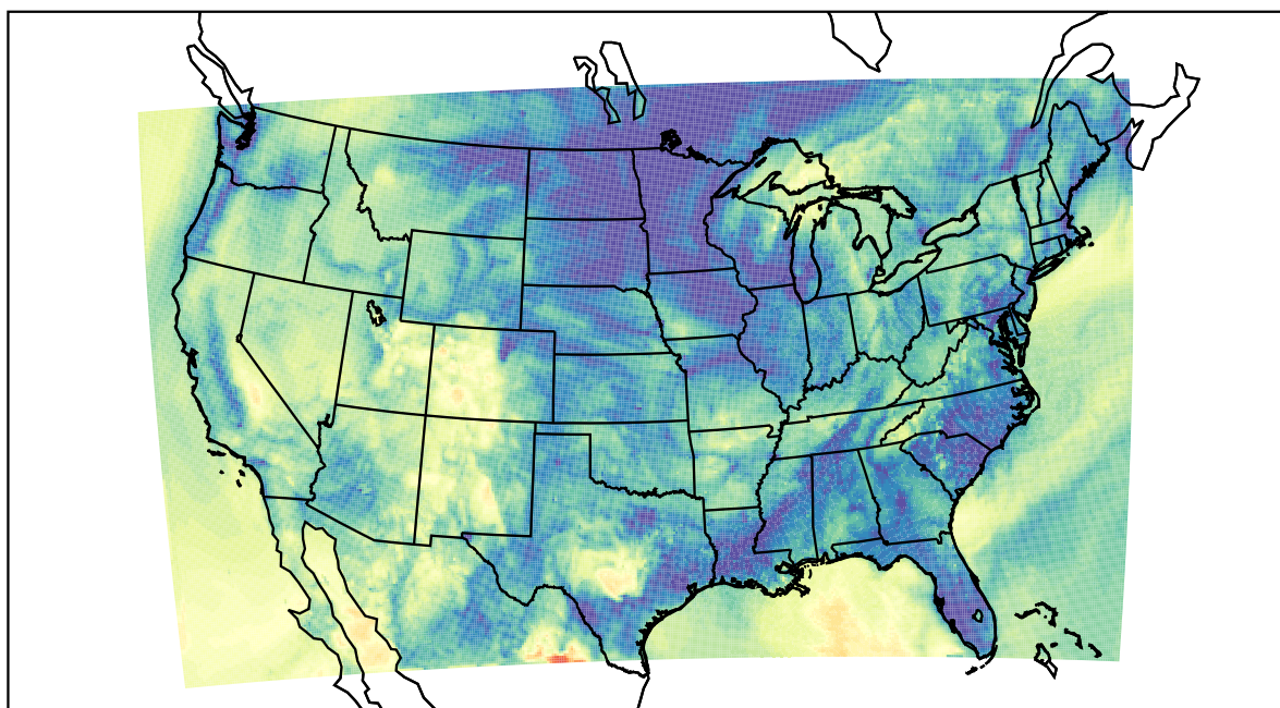
WRF (2021-10-12_13:00:00)
