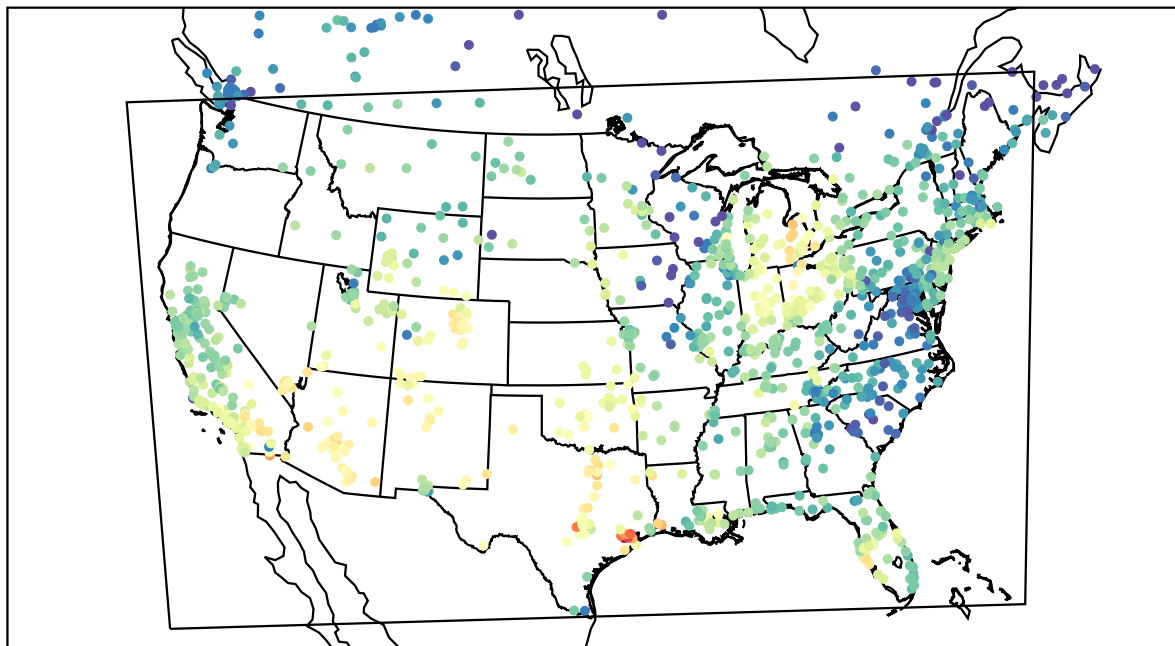
AirNOW (2021-10-11_21:00:00)
