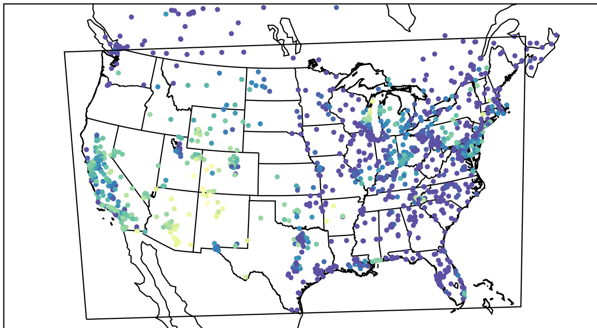
AirNOW (2021-10-12_09:00:00)
