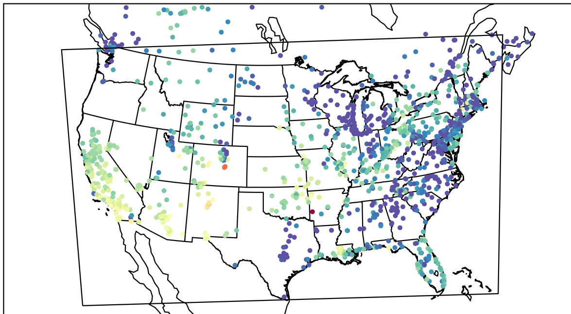
AirNOW (2021-10-12_23:00:00)
