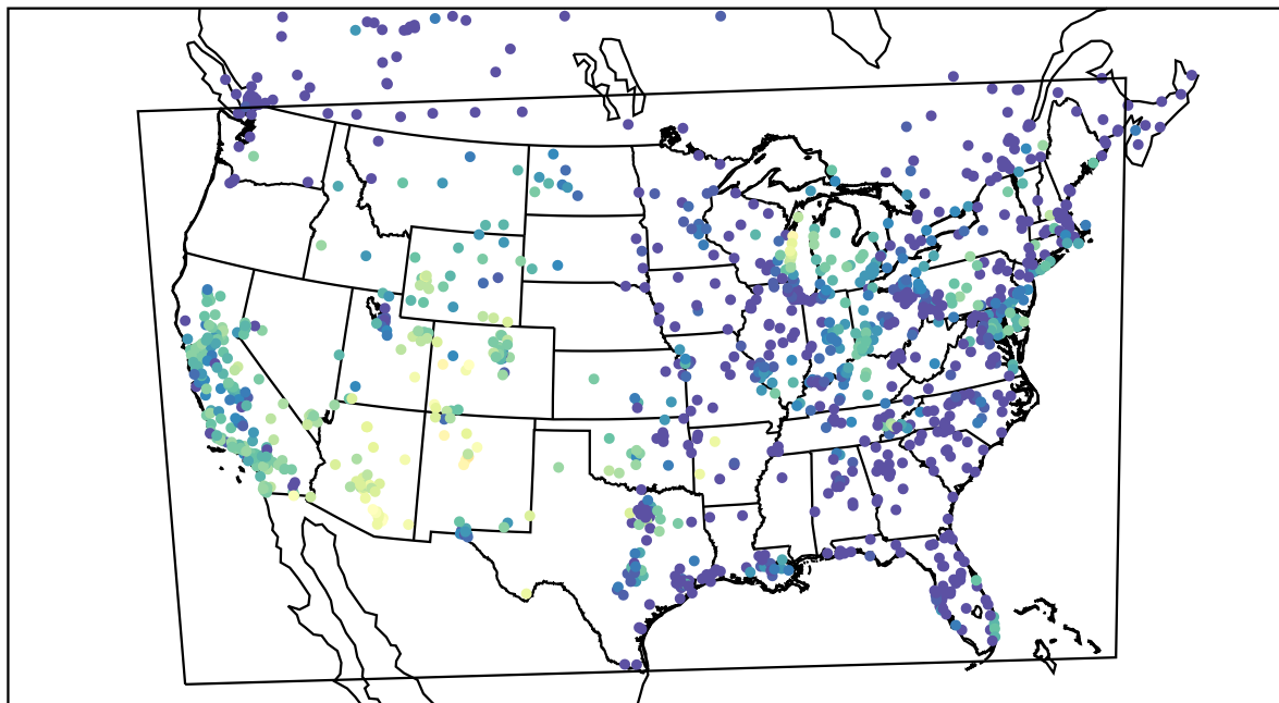
AirNOW (2021-10-12_07:00:00)
