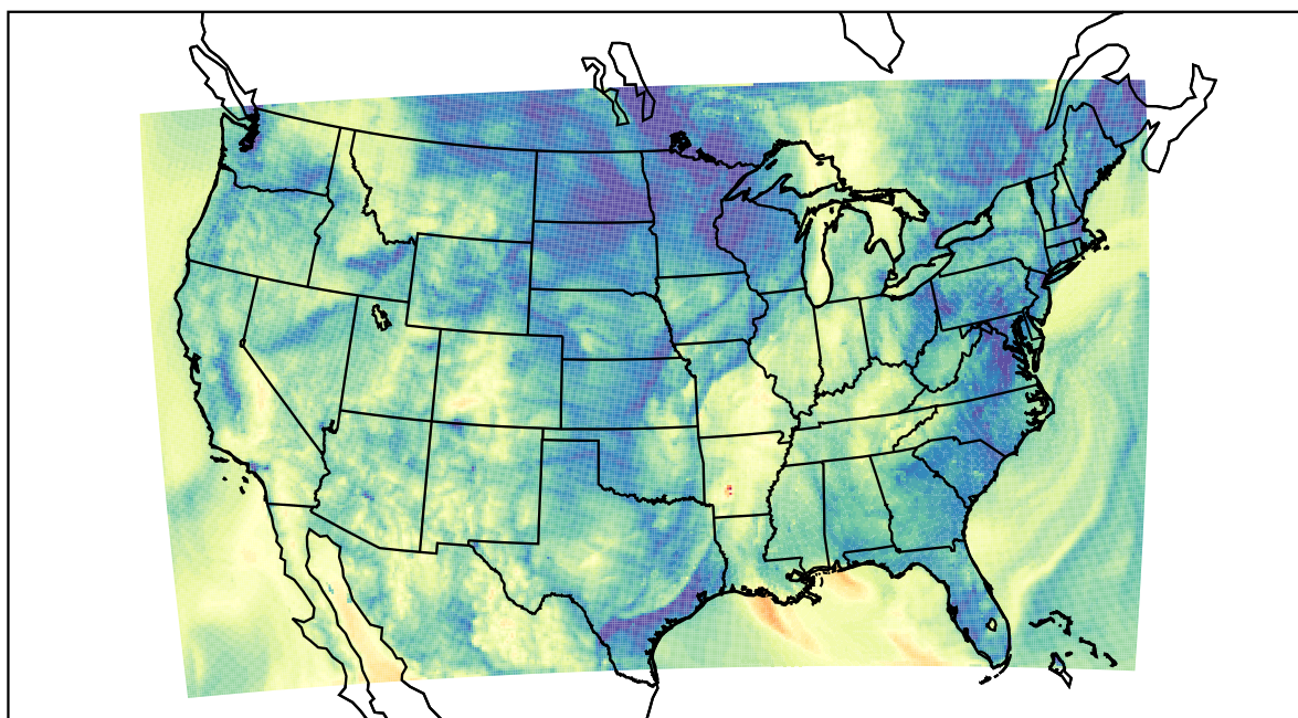
WRF (2021-10-11_10:00:00)
