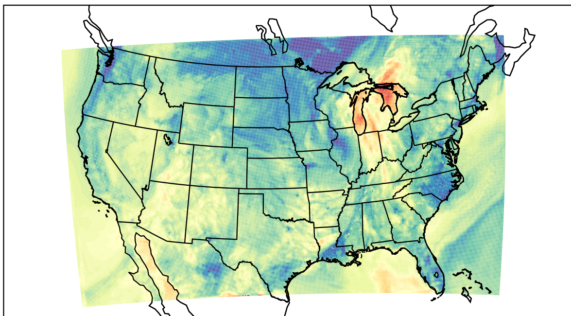
WRF (2021-10-12_03:00:00)
