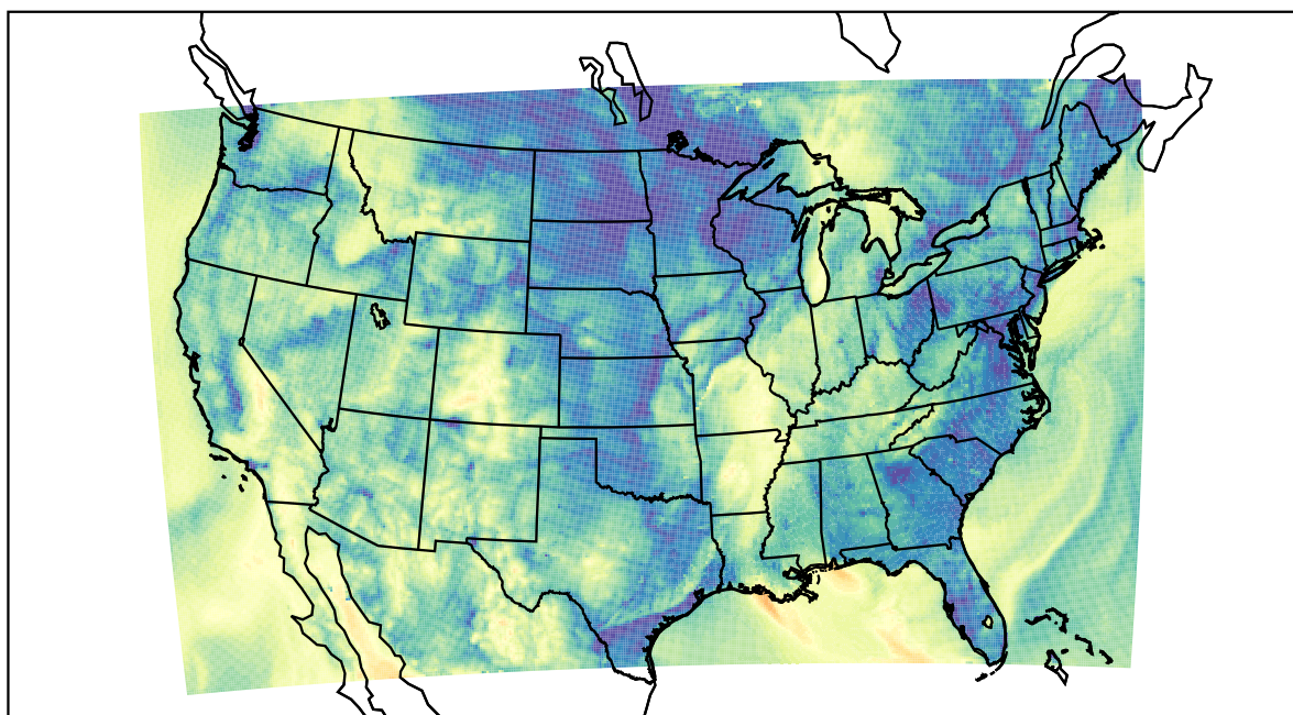
WRF (2021-10-11_12:00:00)
