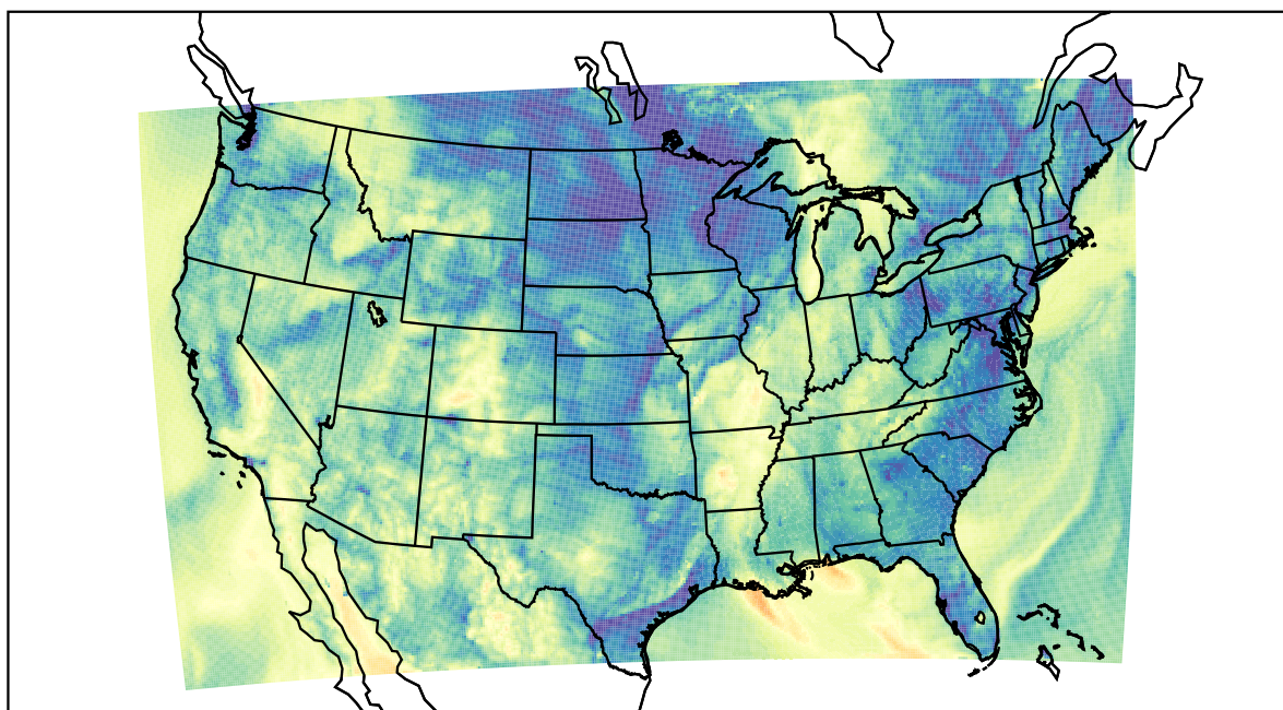
WRF (2021-10-11_11:00:00)
