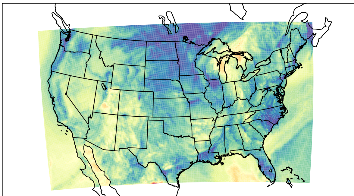
WRF (2021-10-12_07:00:00)
