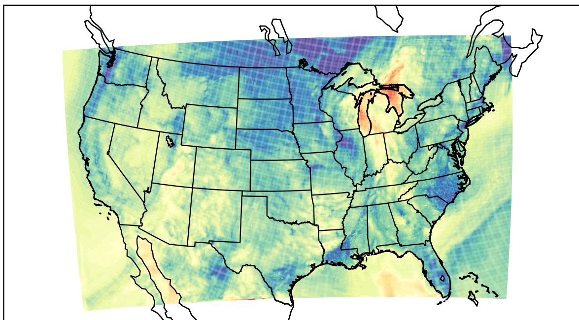
WRF (2021-10-12_04:00:00)
