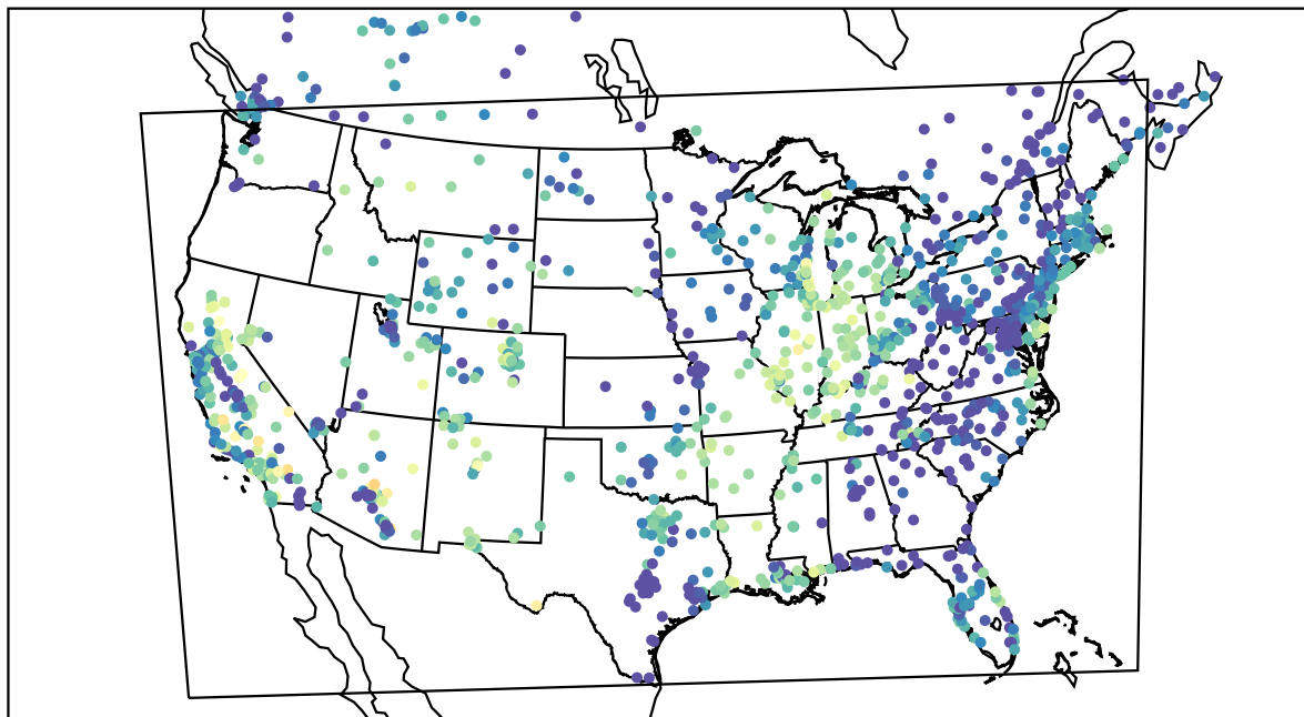
AirNOW (2021-10-11_03:00:00)
