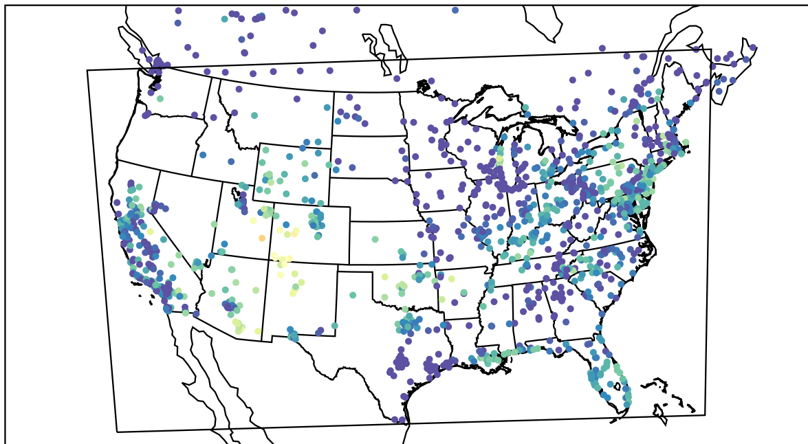
AirNOW (2021-10-12_14:00:00)
