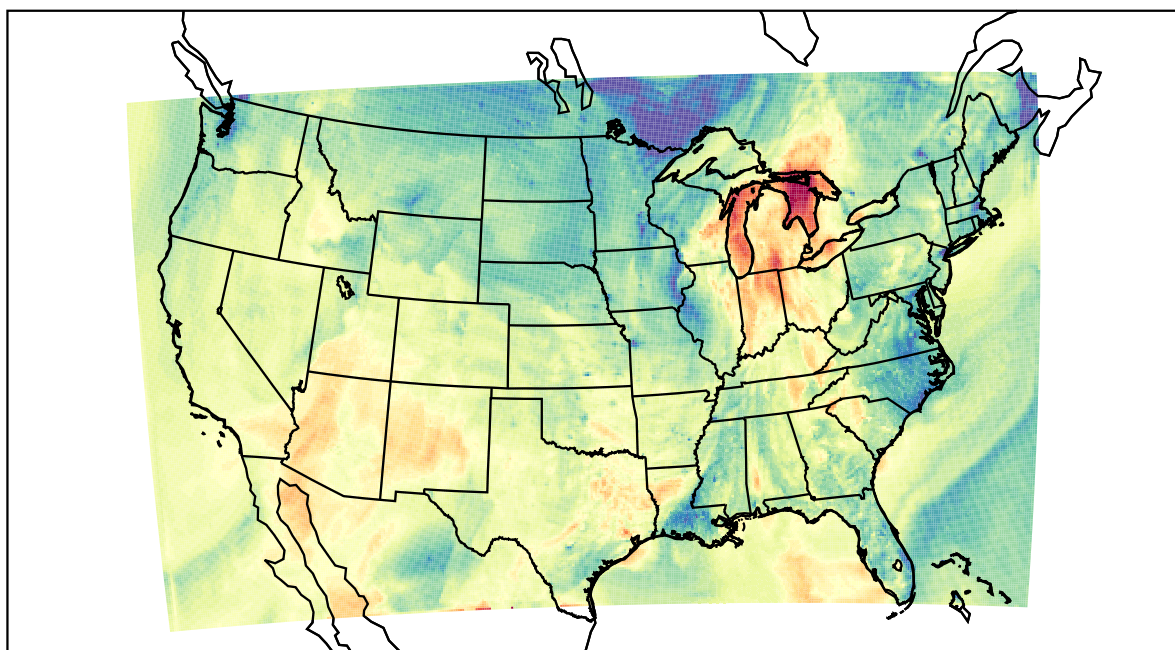
WRF (2021-10-12_00:00:00)
