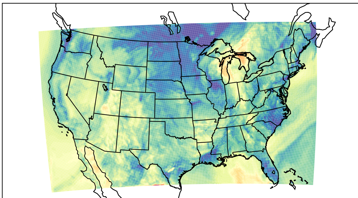
WRF (2021-10-12_06:00:00)
