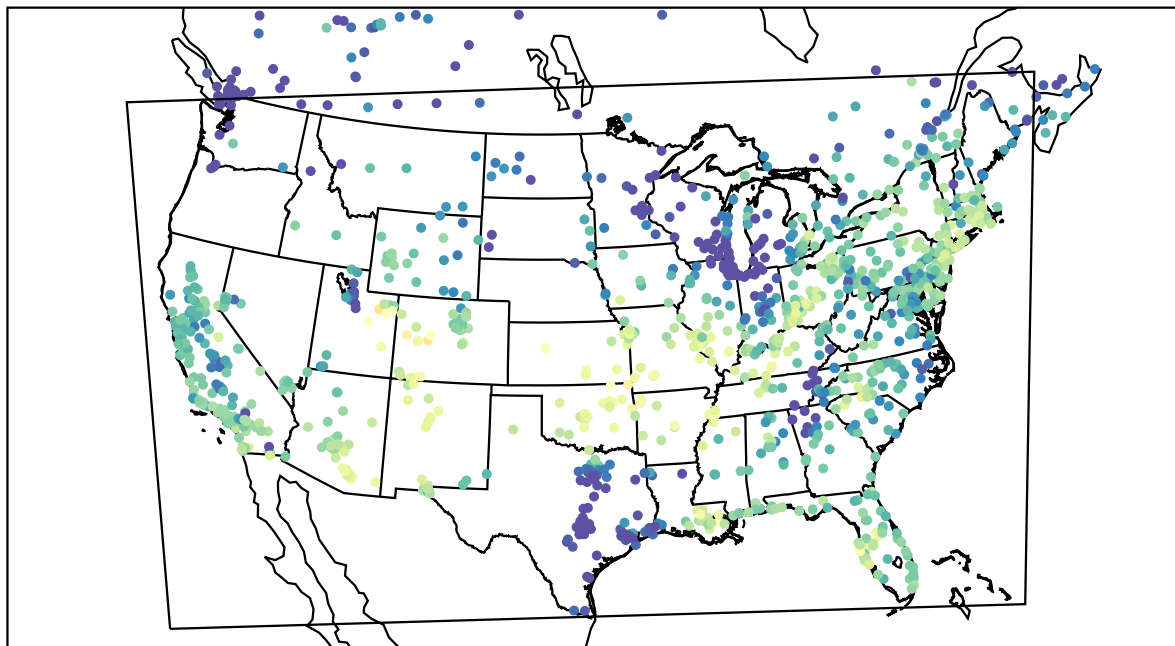
AirNOW (2021-10-12_17:00:00)
