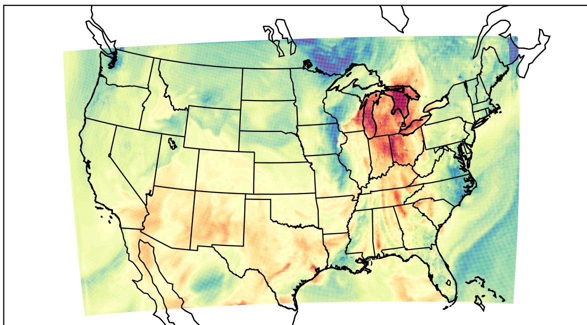
WRF (2021-10-11_22:00:00)
