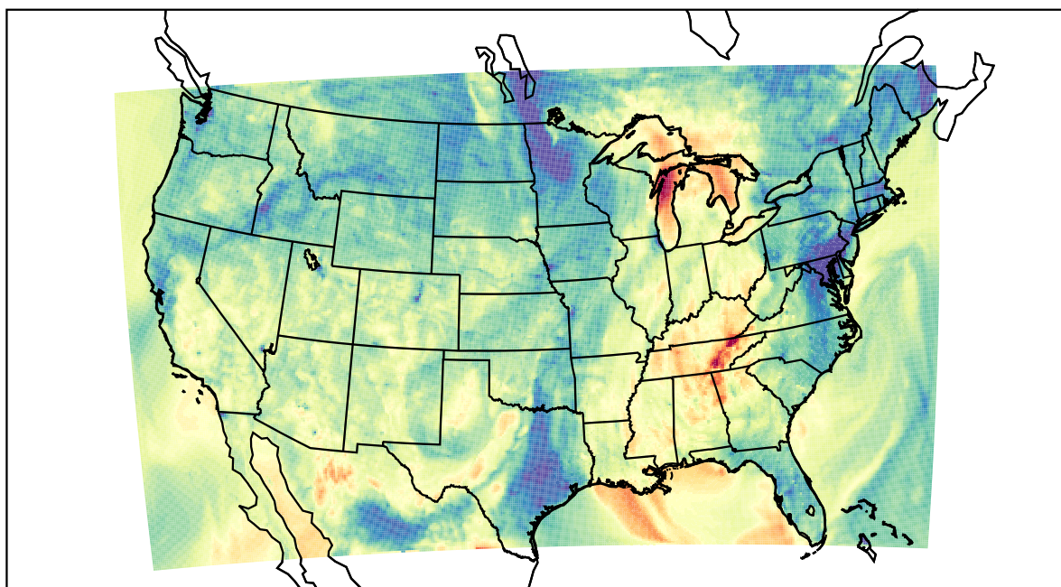
WRF (2021-10-11_02:00:00)
