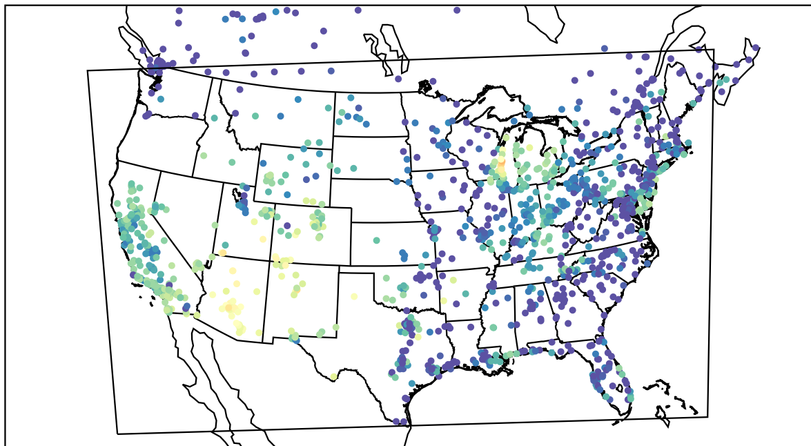
AirNOW (2021-10-12_04:00:00)
