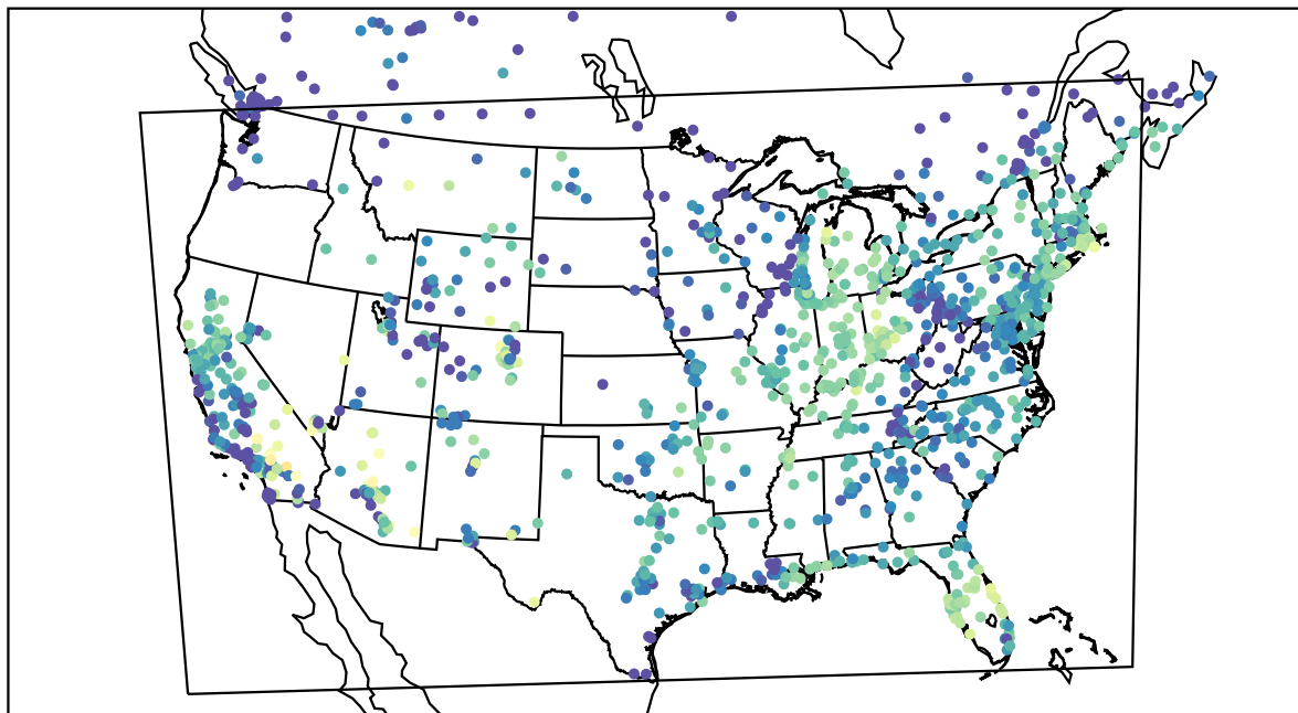
AirNOW (2021-10-11_15:00:00)
