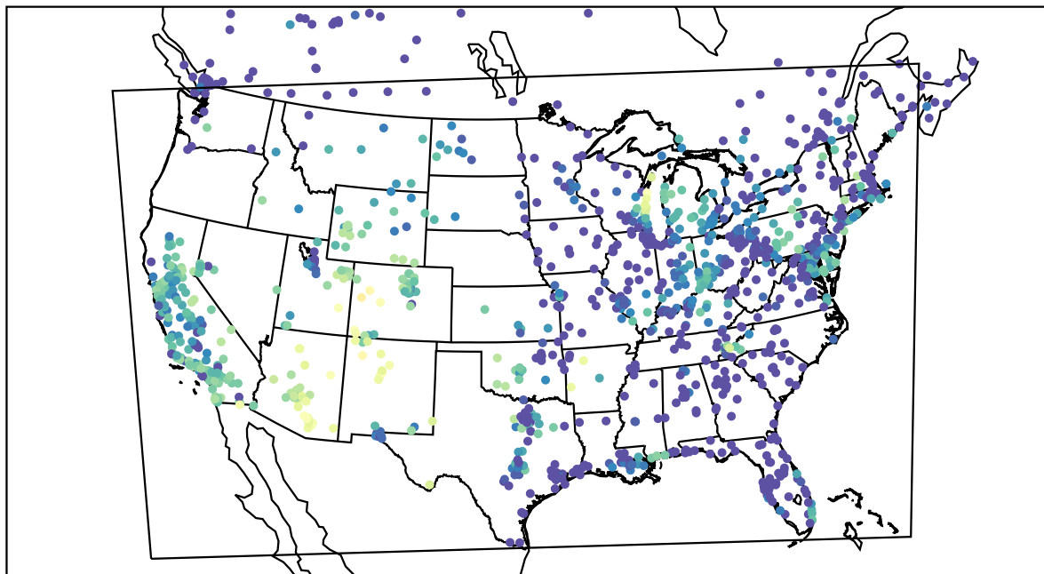
AirNOW (2021-10-12_08:00:00)
