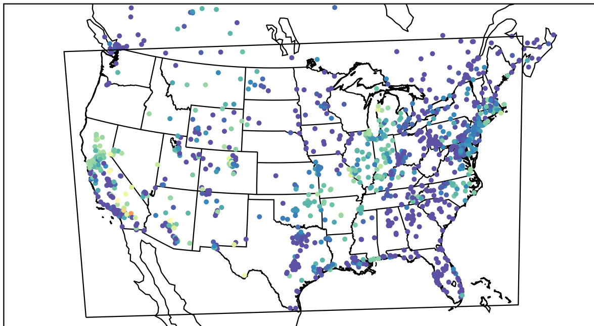
AirNOW (2021-10-11_10:00:00)
