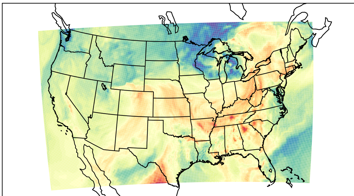
WRF (2021-10-12_20:00:00)
