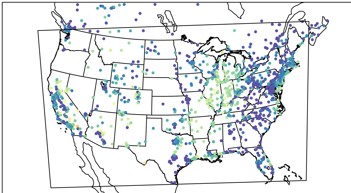
AirNOW (2021-10-11_04:00:00)
