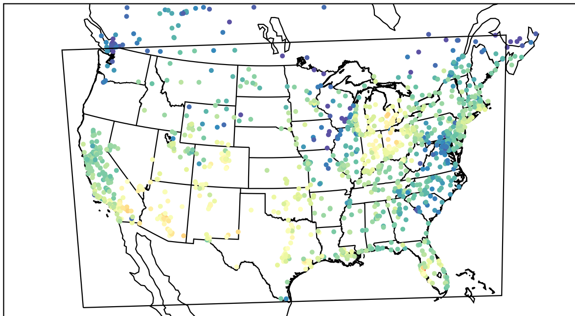
AirNOW (2021-10-11_19:00:00)
