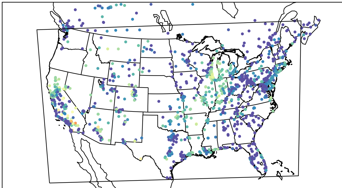
AirNOW (2021-10-11_08:00:00)
