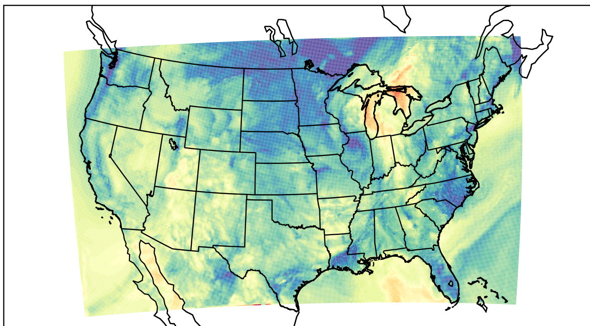
WRF (2021-10-12_05:00:00)
