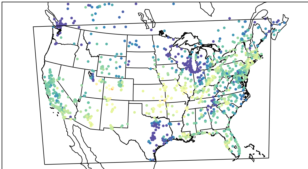
AirNOW (2021-10-12_18:00:00)
