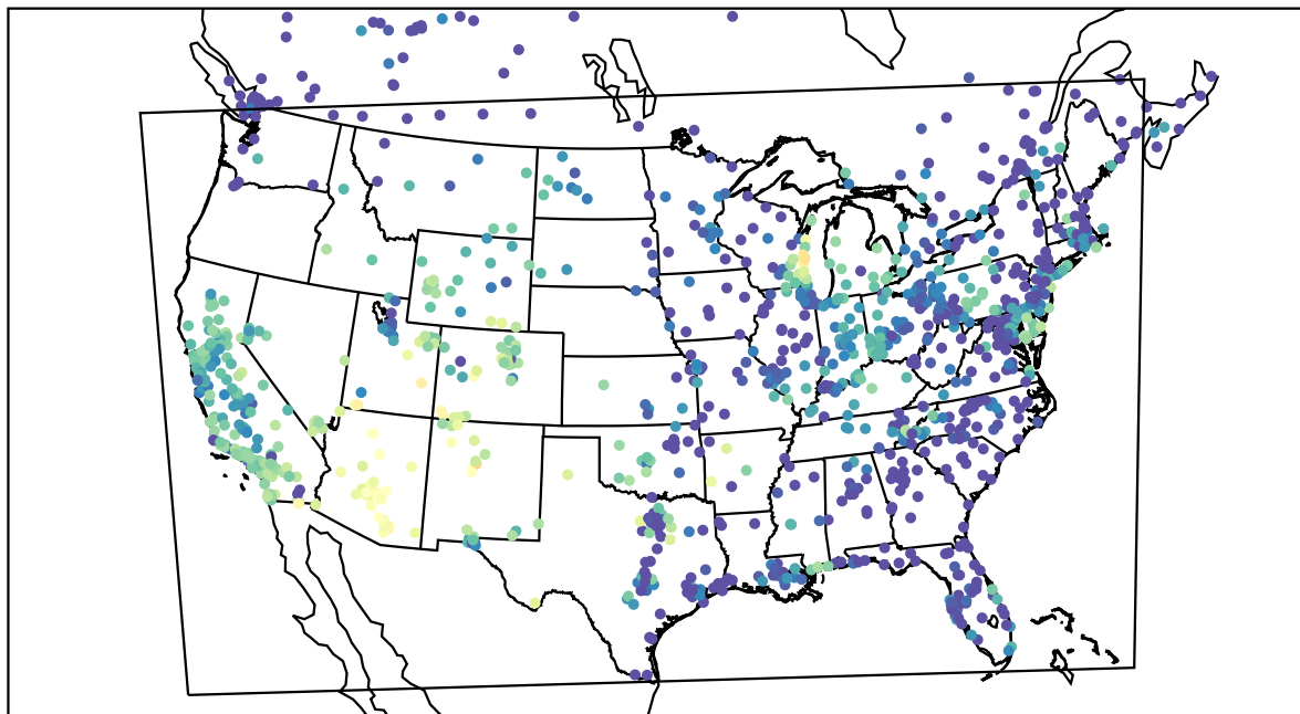
AirNOW (2021-10-12_05:00:00)
