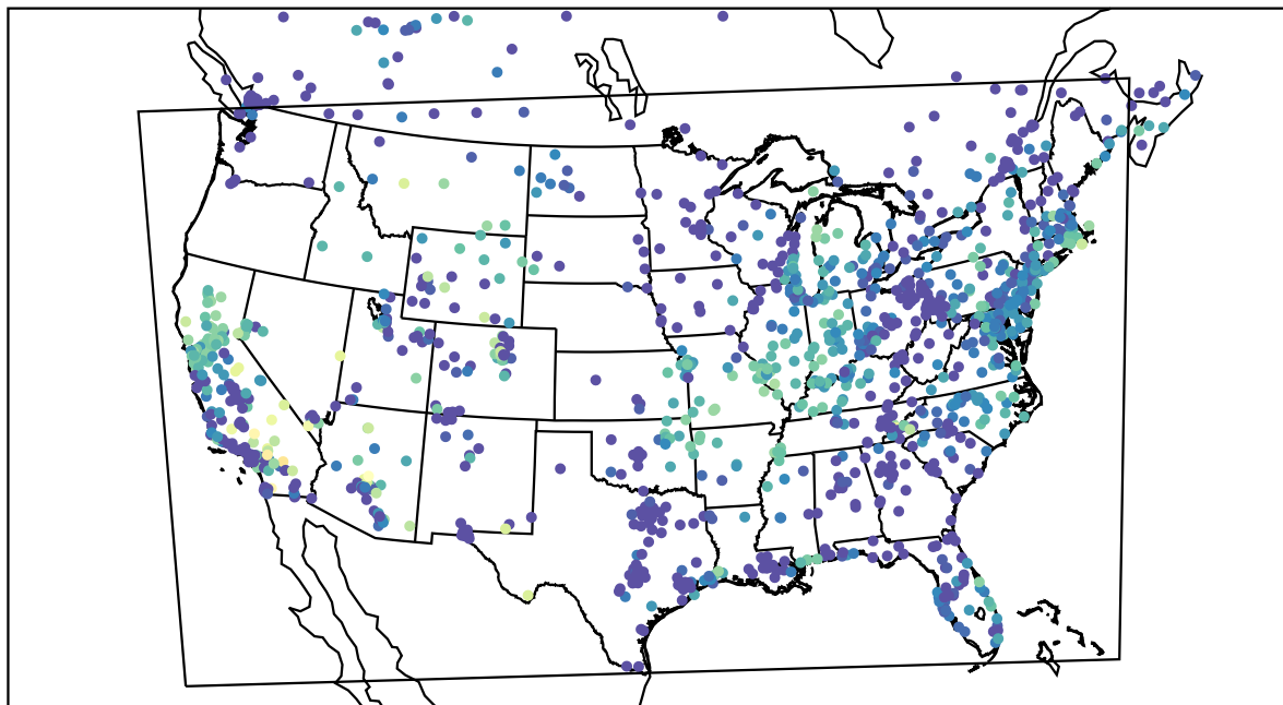
AirNOW (2021-10-11_13:00:00)
