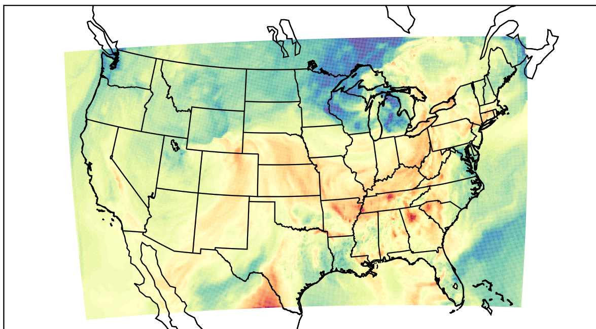
WRF (2021-10-12_21:00:00)
