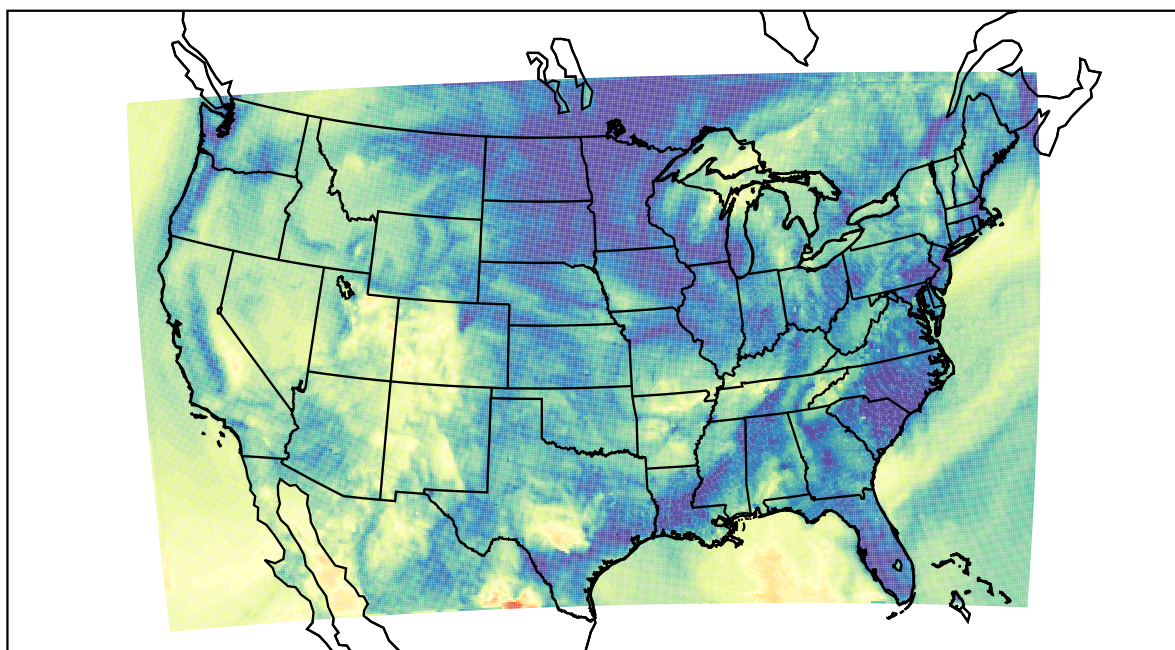
WRF (2021-10-12_12:00:00)
