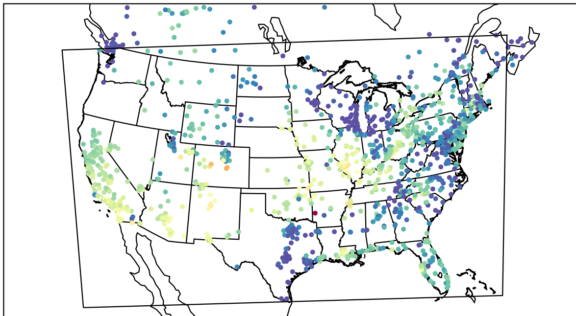
AirNOW (2021-10-12_22:00:00)
