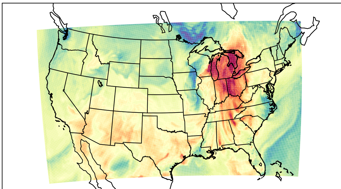
WRF (2021-10-11_21:00:00)
