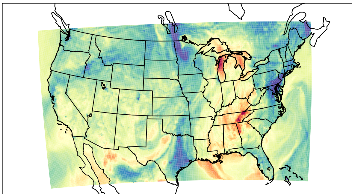
WRF (2021-10-11_01:00:00)
