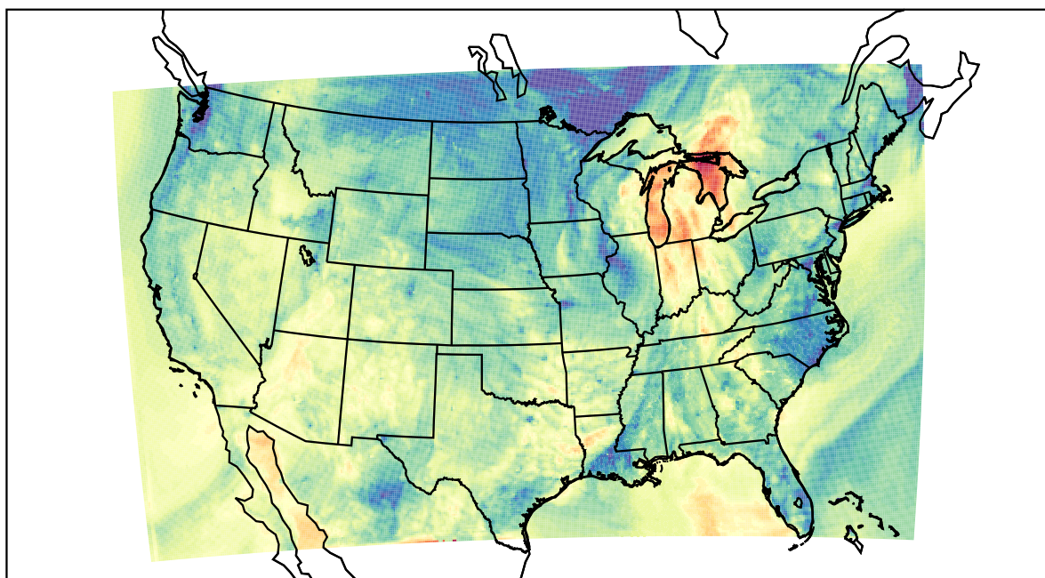
WRF (2021-10-12_02:00:00)
