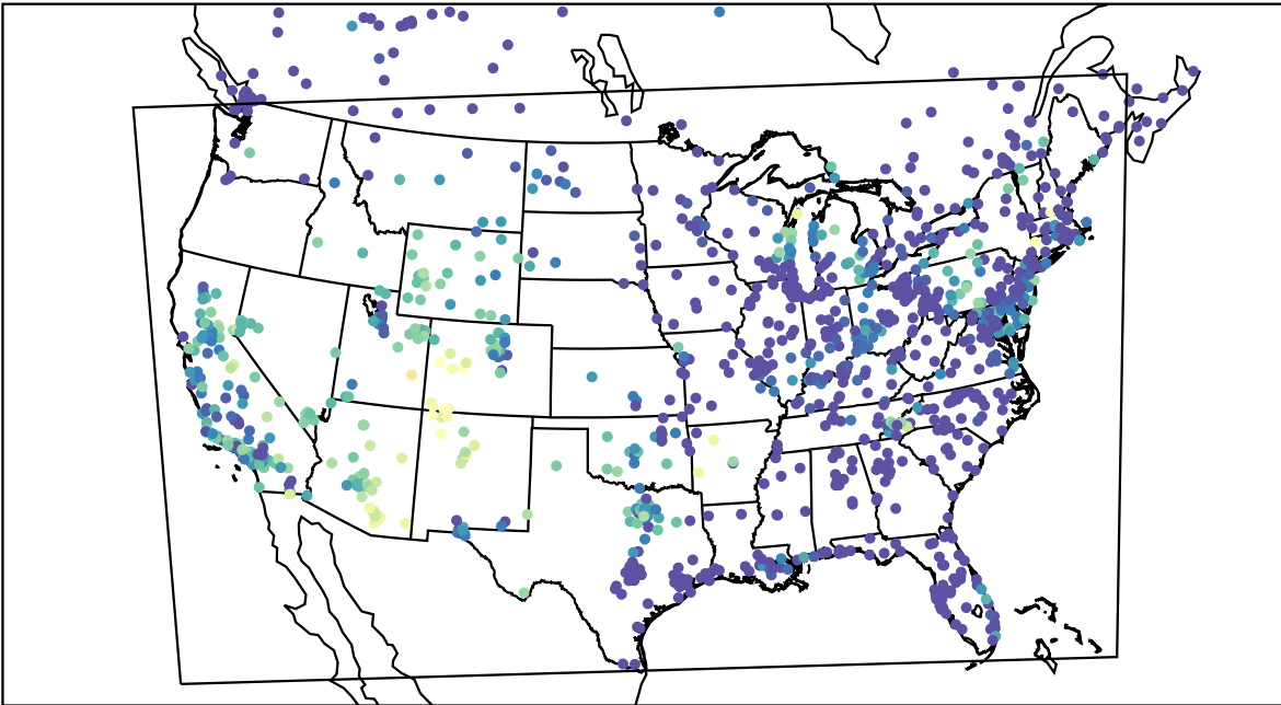
AirNOW (2021-10-12_11:00:00)
