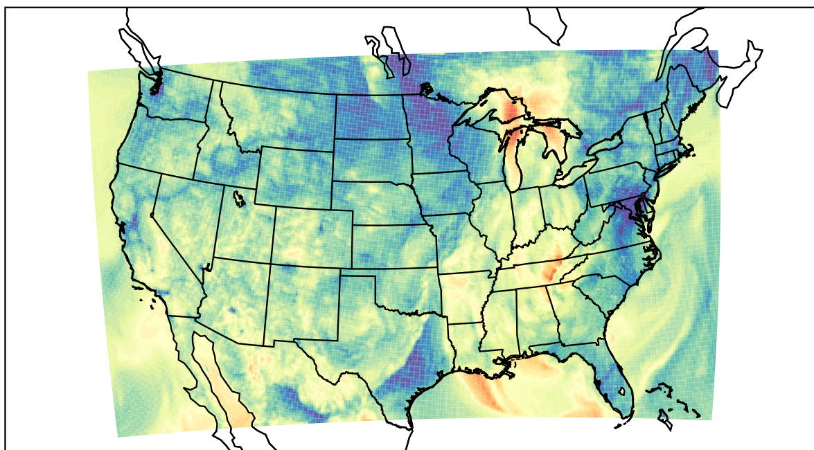
WRF (2021-10-11_05:00:00)
