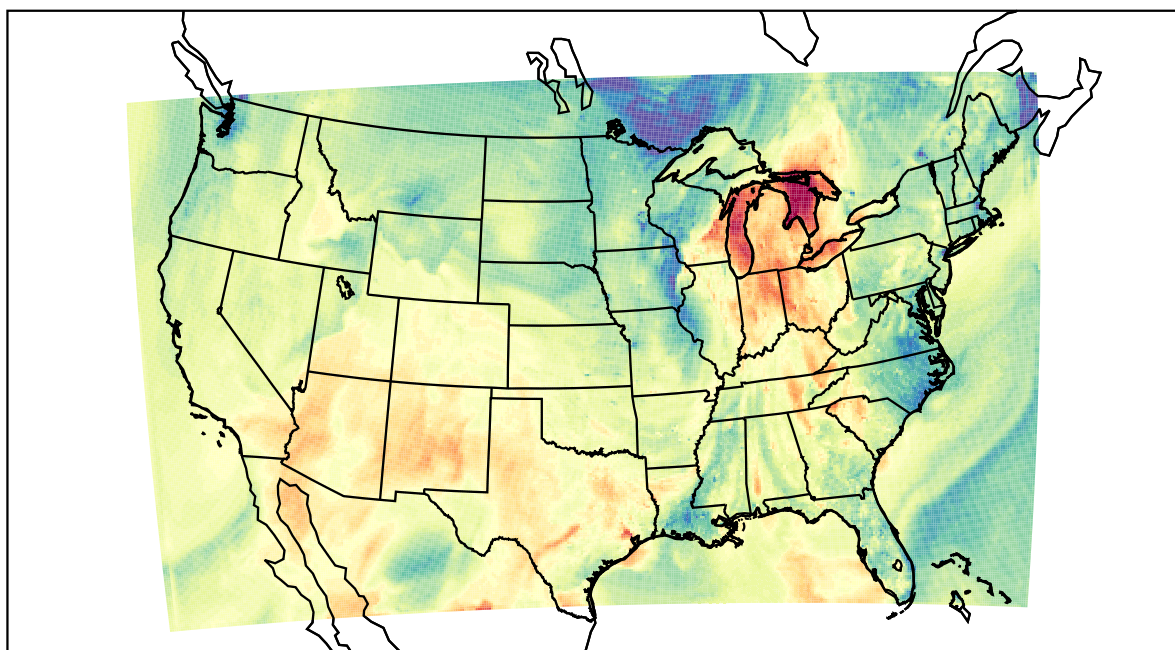
WRF (2021-10-11_23:00:00)
