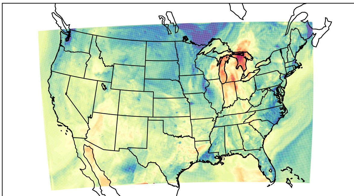
WRF (2021-10-12_01:00:00)
