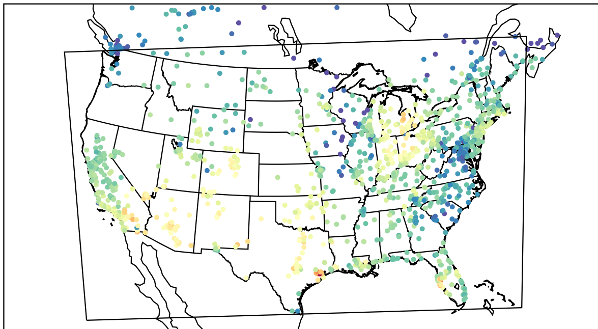
AirNOW (2021-10-11_20:00:00)
