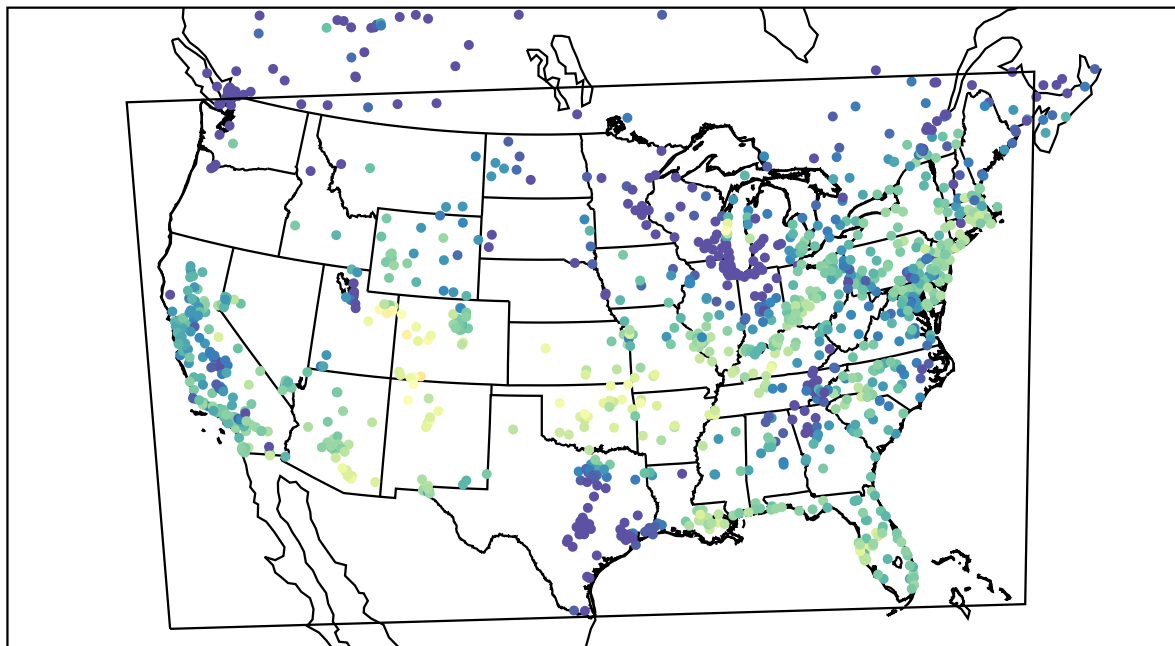
AirNOW (2021-10-12_16:00:00)
