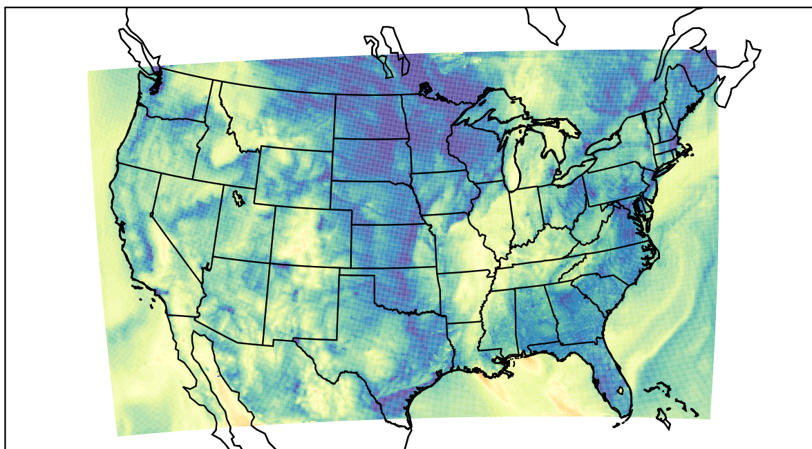
WRF (2021-10-11_13:00:00)
