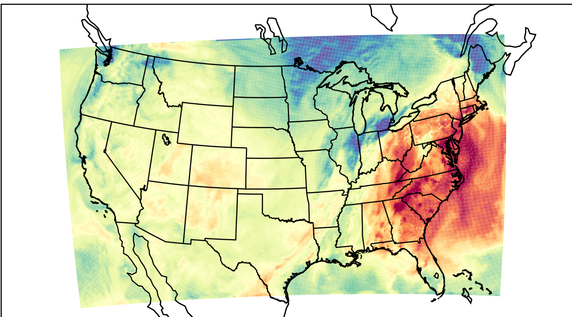
WRF (2021-10-15_19:00:00)
