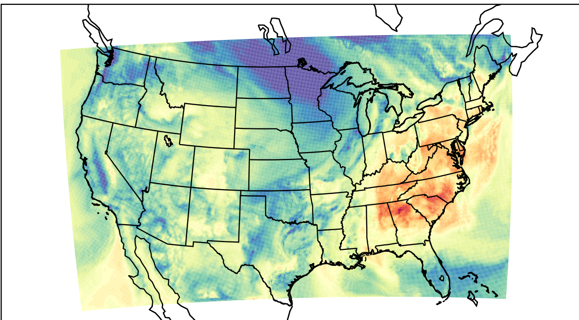
WRF (2021-10-14_16:00:00)
