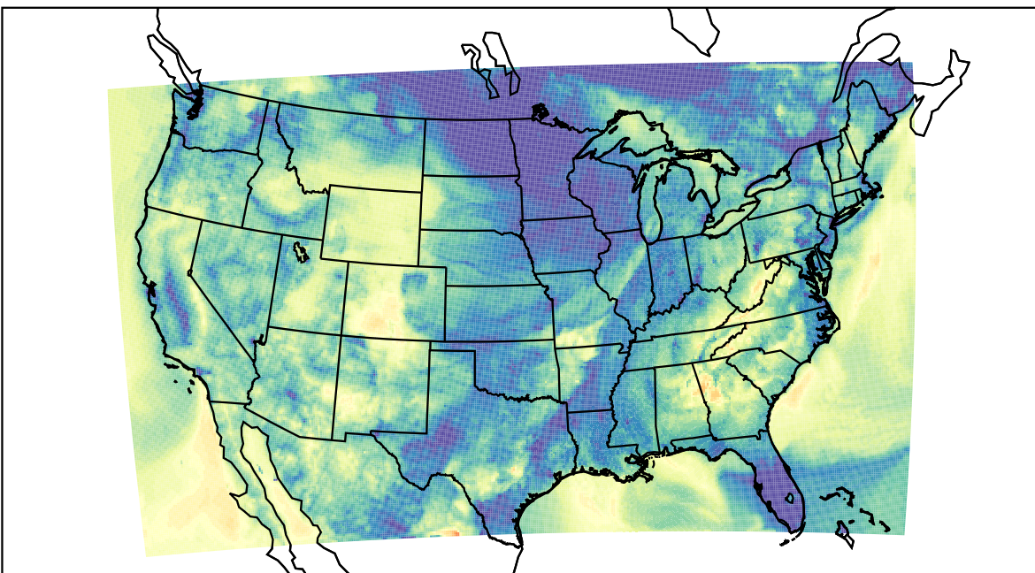
WRF (2021-10-14_11:00:00)
