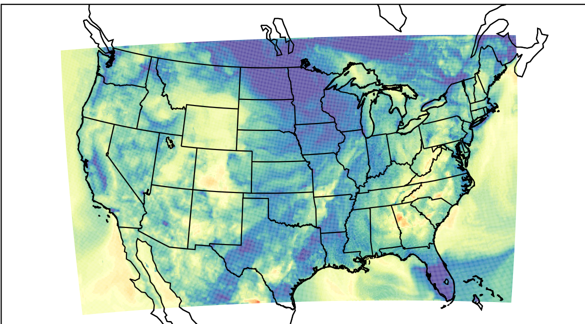
WRF (2021-10-14_09:00:00)
