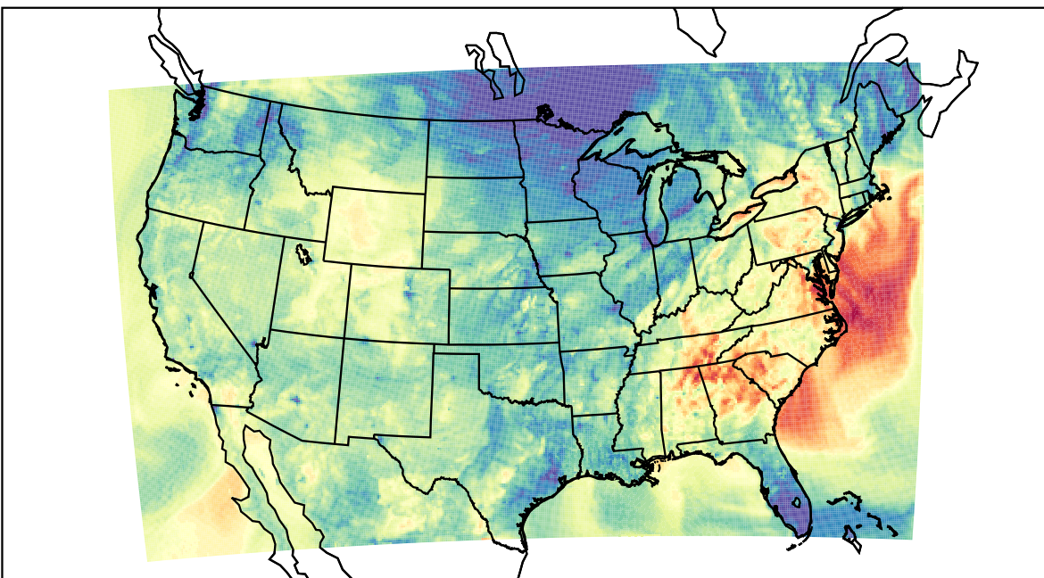
WRF (2021-10-15_02:00:00)
