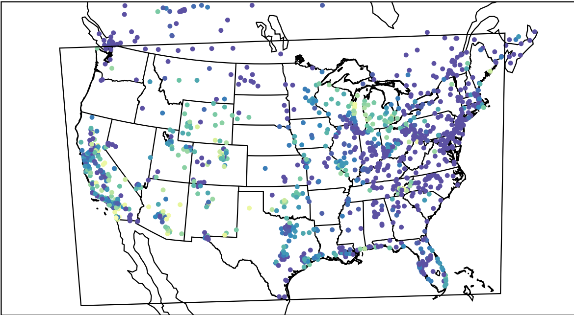
AirNOW (2021-10-14_03:00:00)
