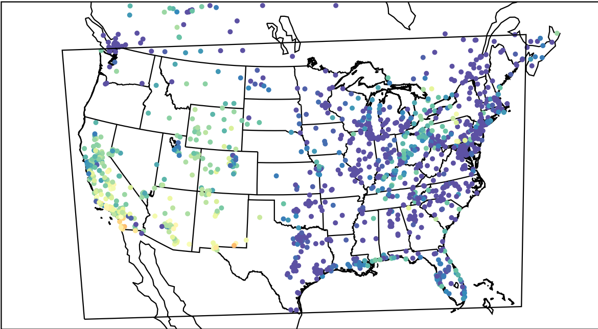
AirNOW (2021-10-15_01:00:00)
