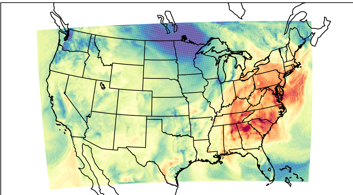
WRF (2021-10-14_18:00:00)
