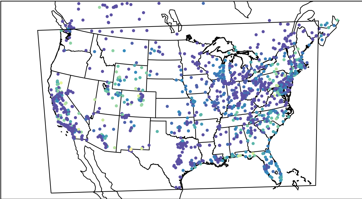
AirNOW (2021-10-14_14:00:00)
