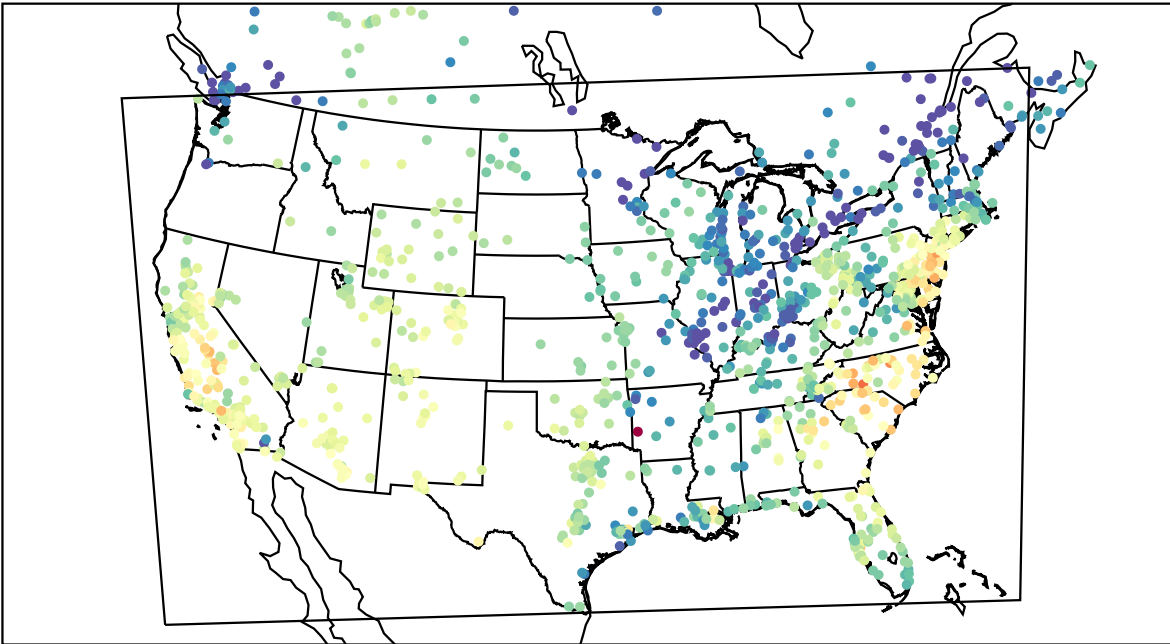
AirNOW (2021-10-15_20:00:00)
