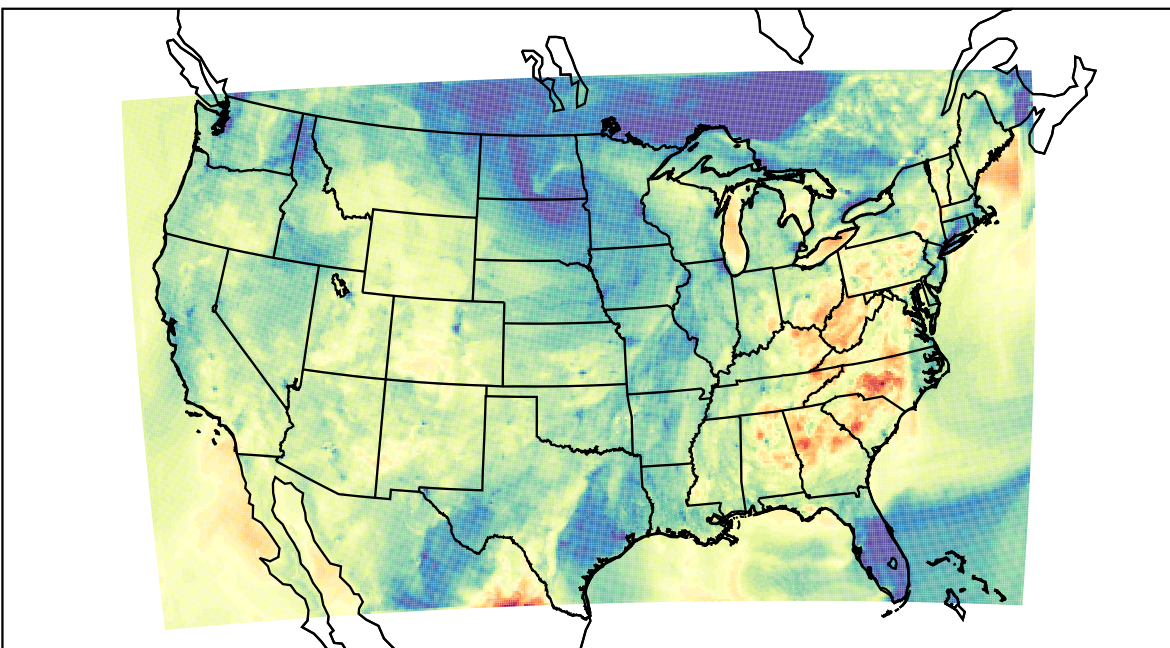
WRF (2021-10-14_01:00:00)
