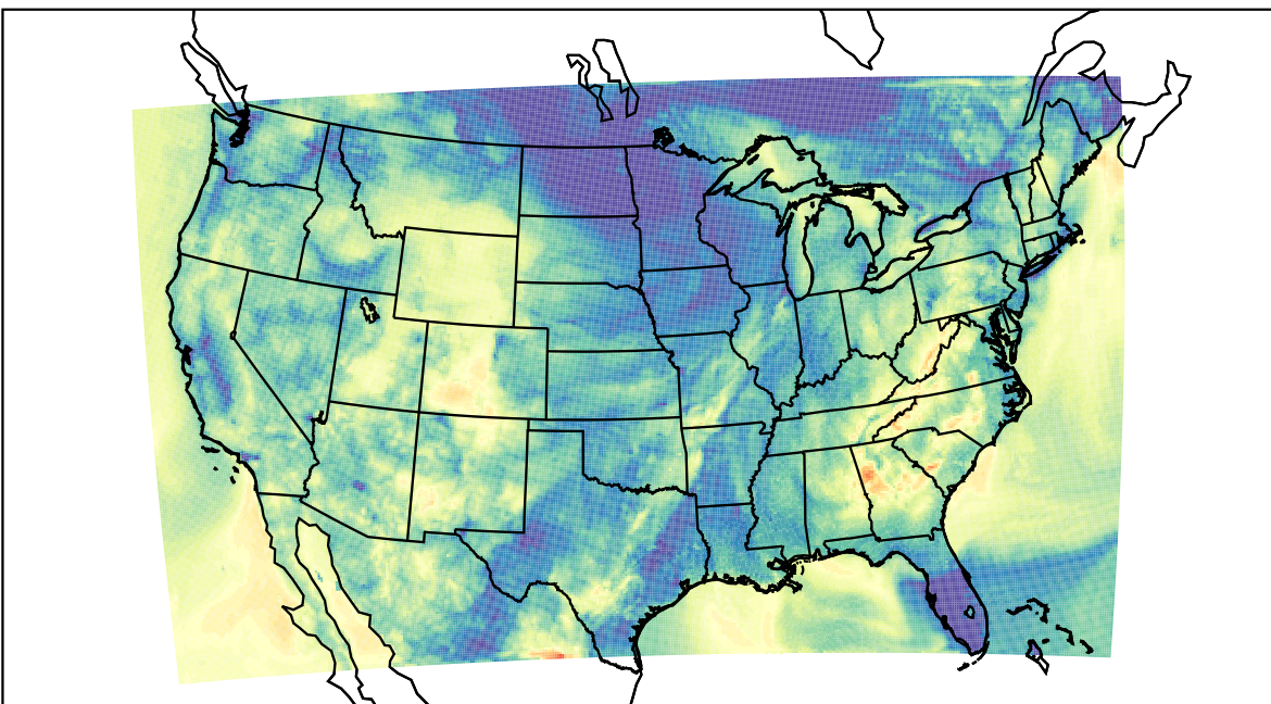
WRF (2021-10-14_08:00:00)
