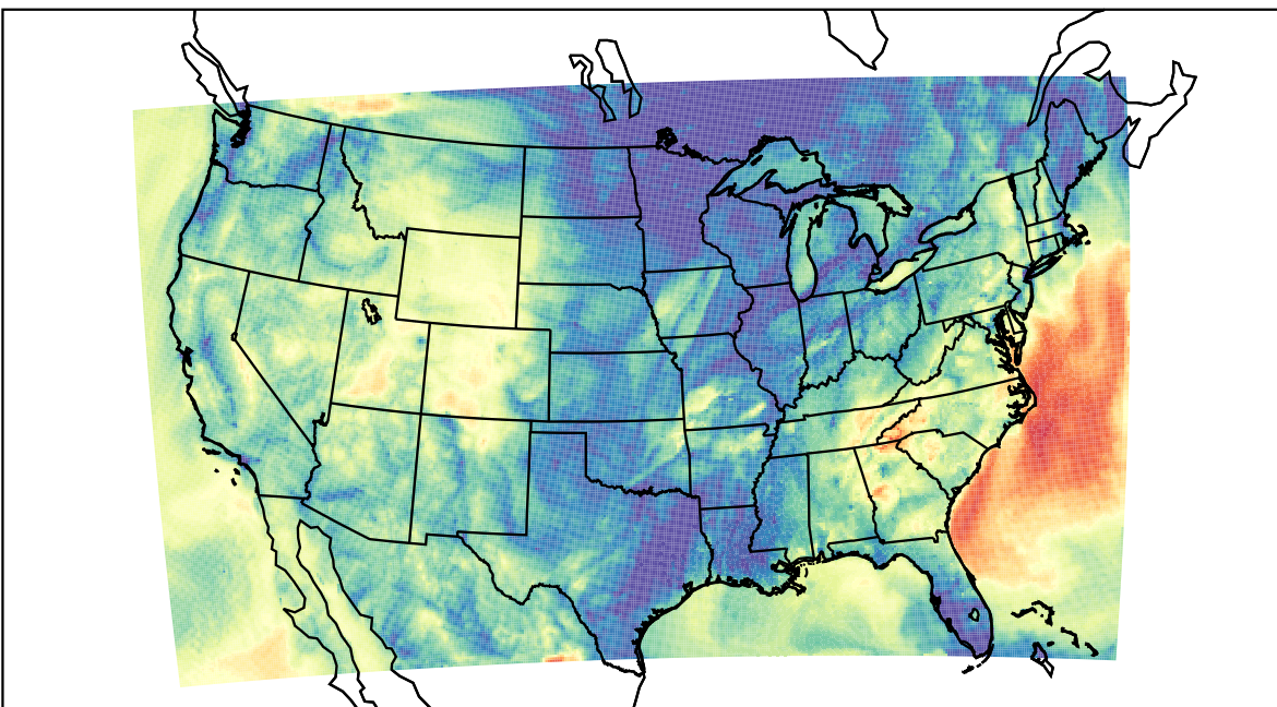
WRF (2021-10-15_11:00:00)
