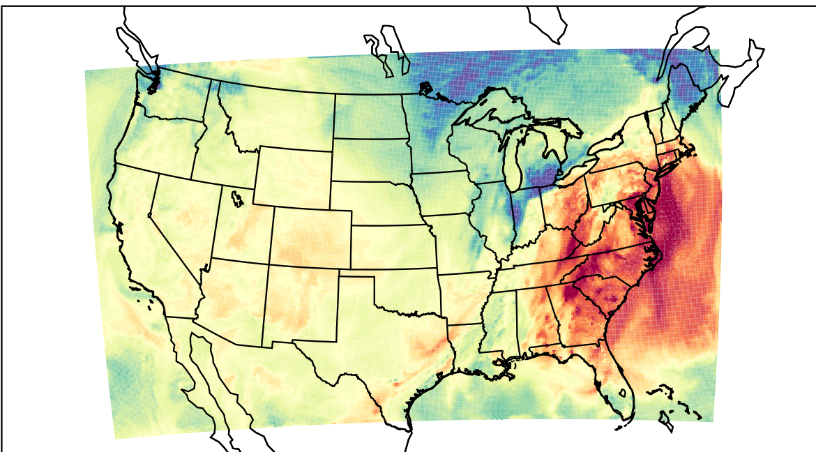
WRF (2021-10-15_21:00:00)
