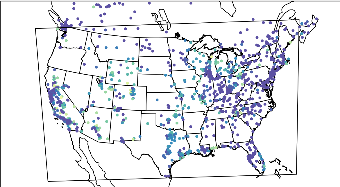
AirNOW (2021-10-14_06:00:00)
