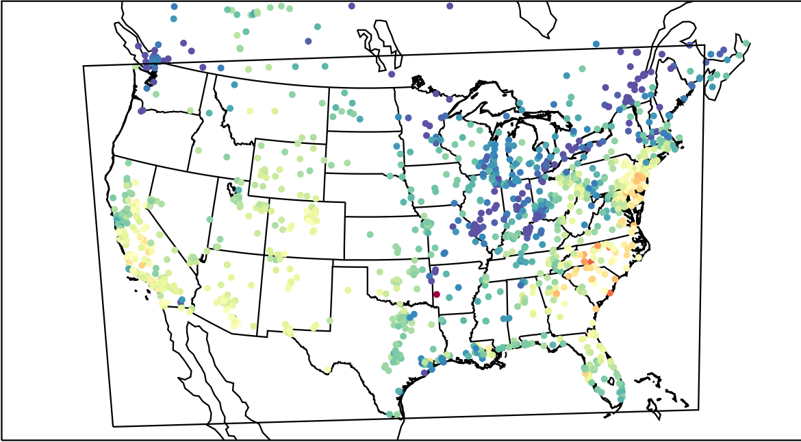
AirNOW (2021-10-15_19:00:00)
