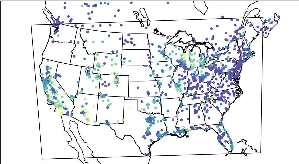
AirNOW (2021-10-14_02:00:00)
