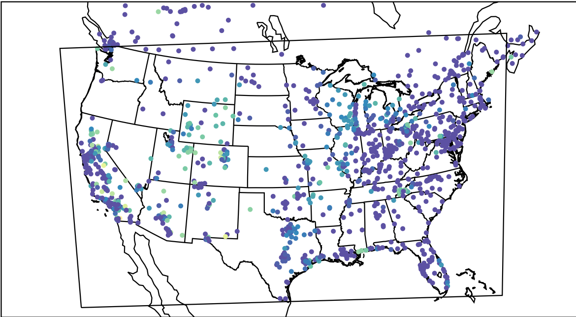
AirNOW (2021-10-14_09:00:00)
