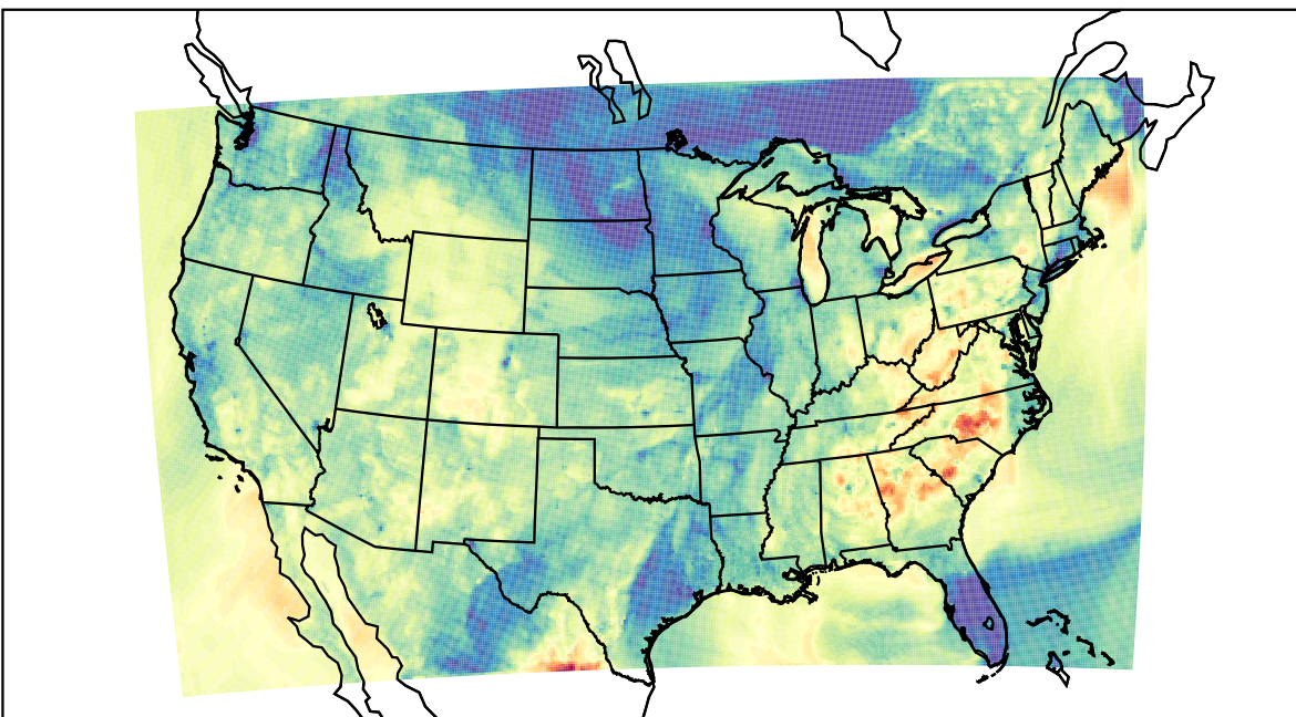
WRF (2021-10-14_02:00:00)
