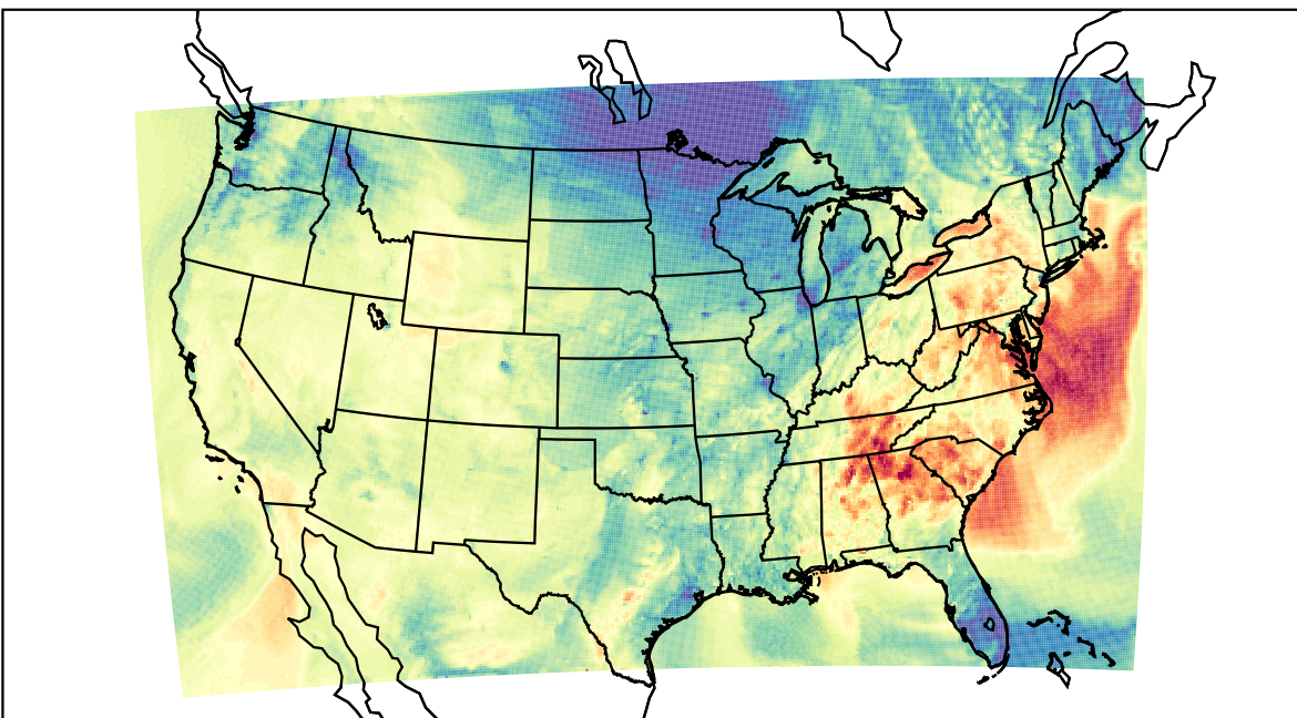
WRF (2021-10-15_00:00:00)
