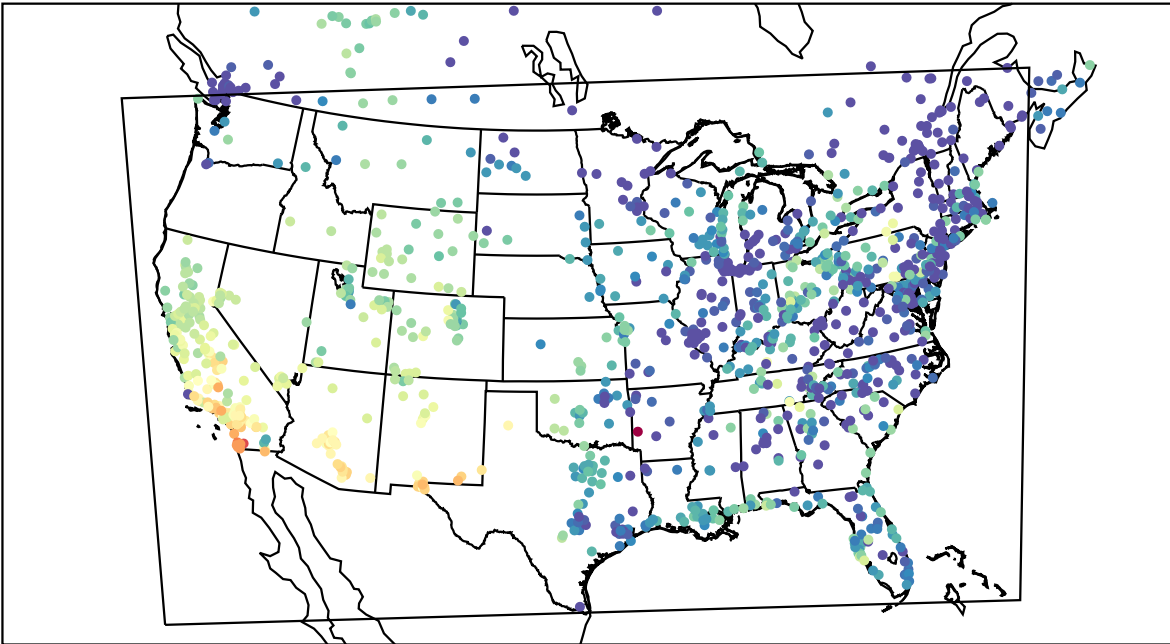
AirNOW (2021-10-14_23:00:00)
