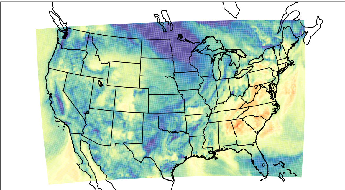
WRF (2021-10-14_15:00:00)
