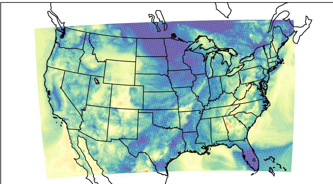
WRF (2021-10-14_10:00:00)
