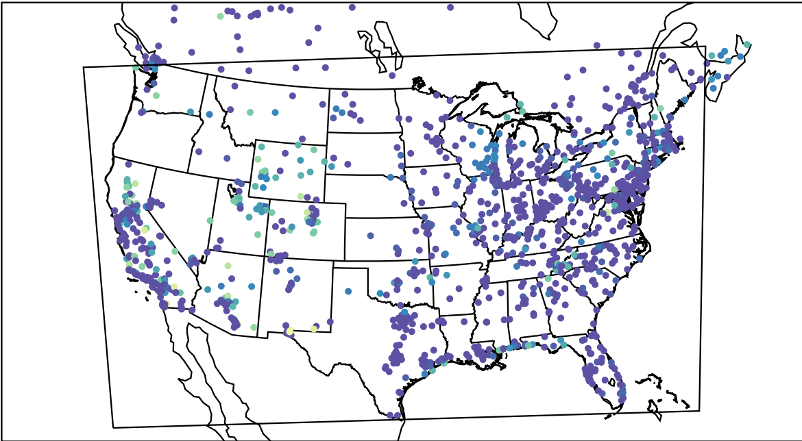
AirNOW (2021-10-14_13:00:00)
