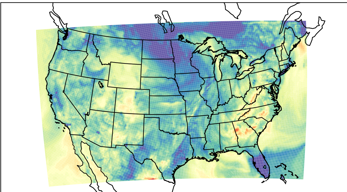
WRF (2021-10-14_06:00:00)
