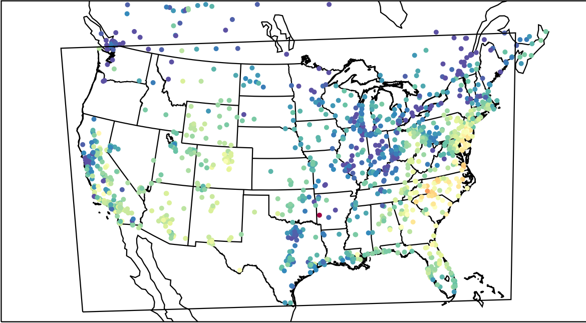
AirNOW (2021-10-15_17:00:00)
