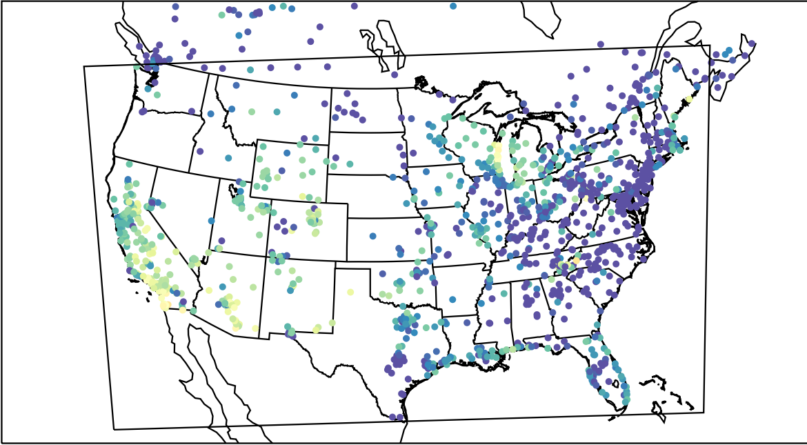
AirNOW (2021-10-14_01:00:00)
