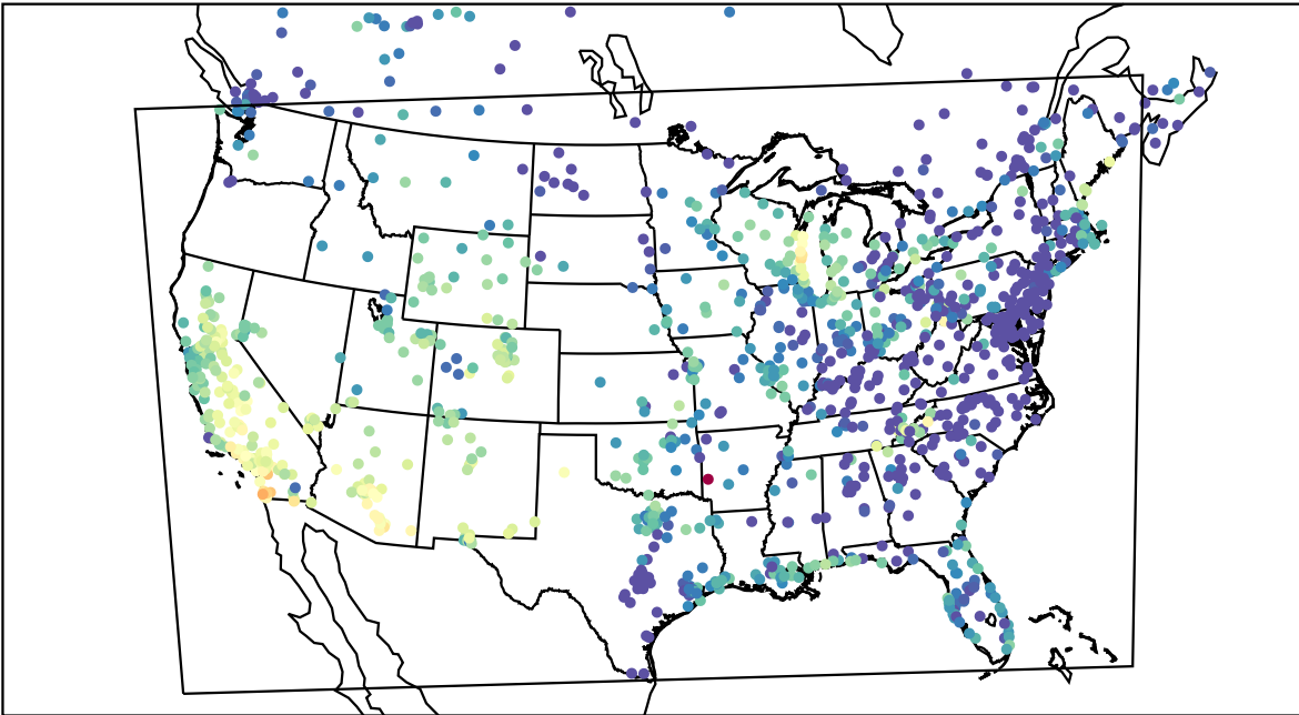
AirNOW (2021-10-14_00:00:00)
