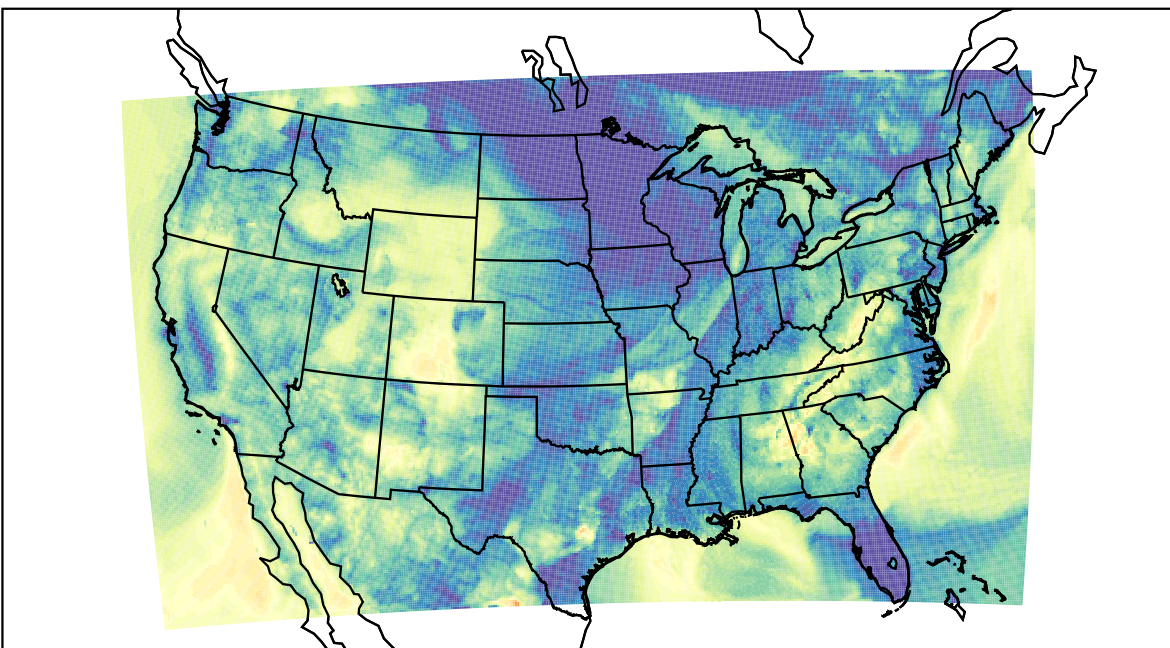
WRF (2021-10-14_12:00:00)
