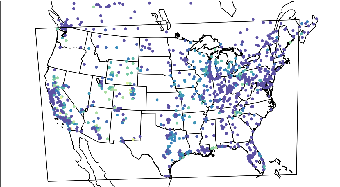
AirNOW (2021-10-14_08:00:00)
