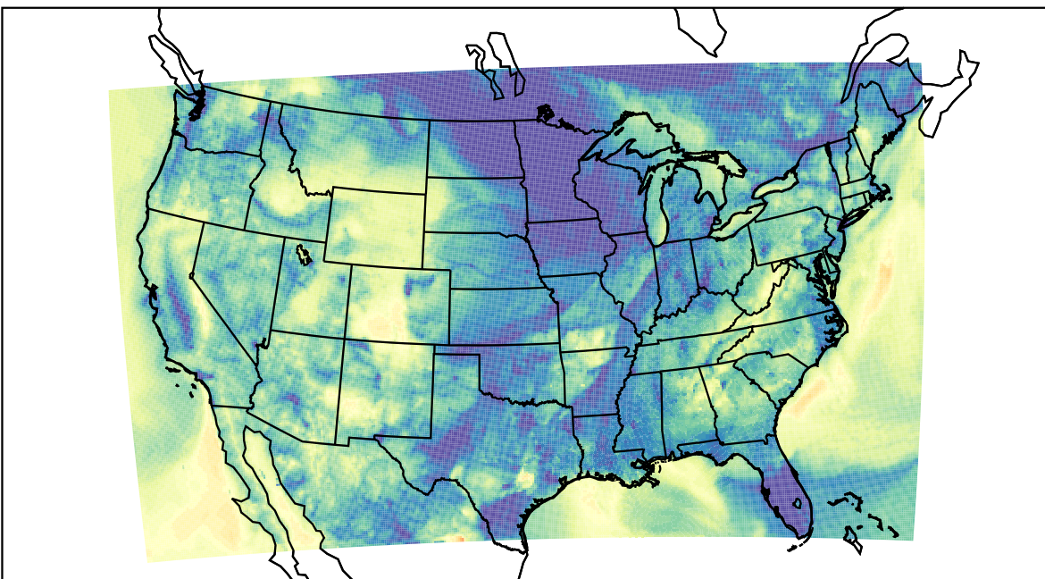
WRF (2021-10-14_13:00:00)
