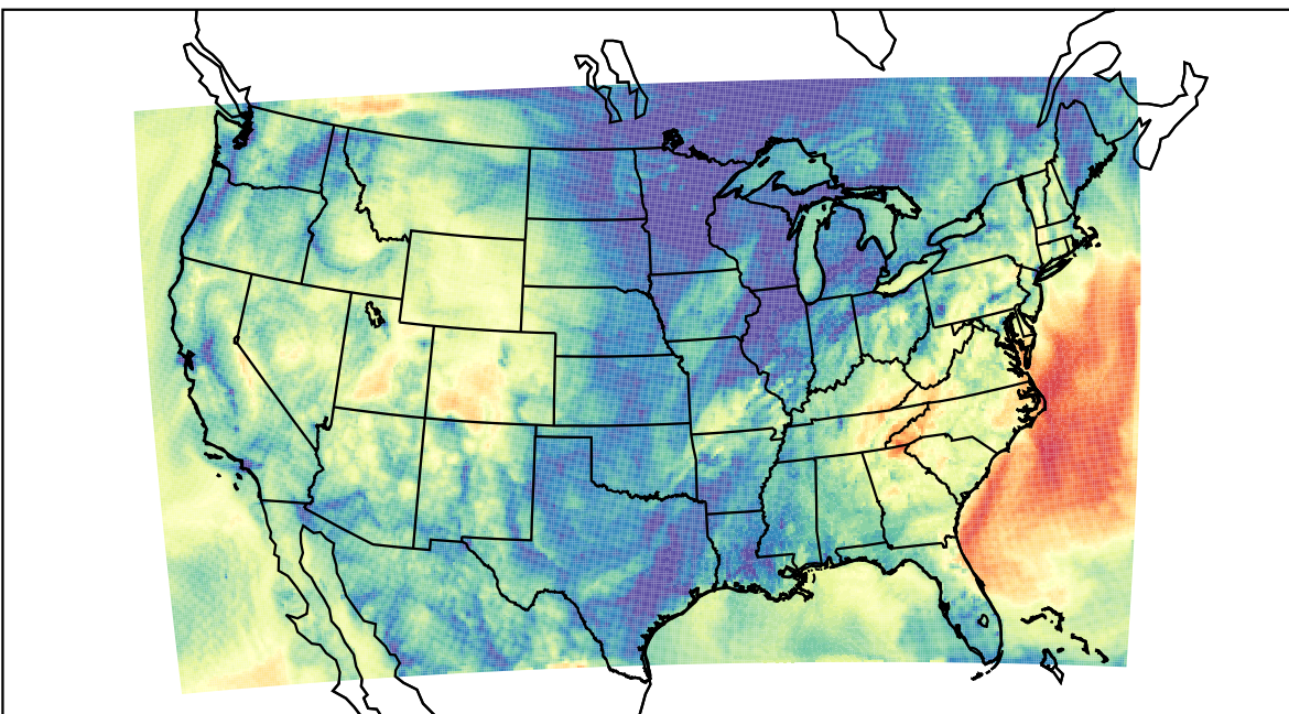
WRF (2021-10-15_14:00:00)
