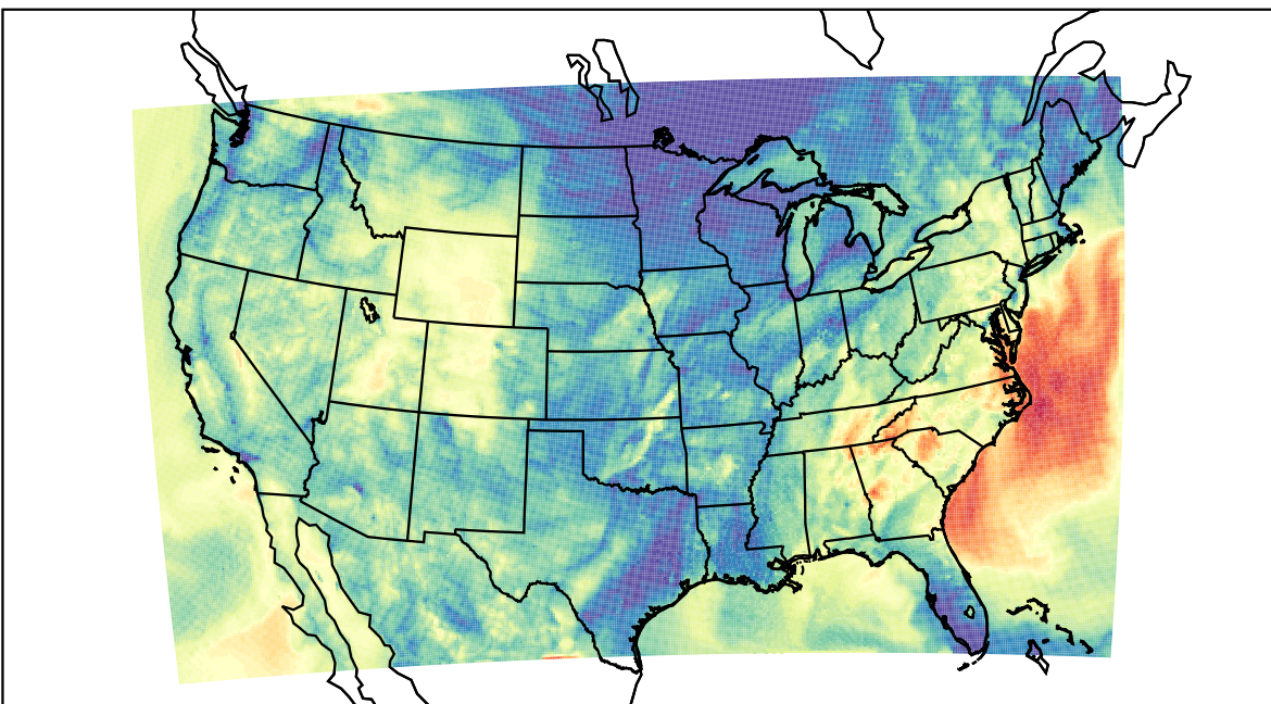
WRF (2021-10-15_07:00:00)
