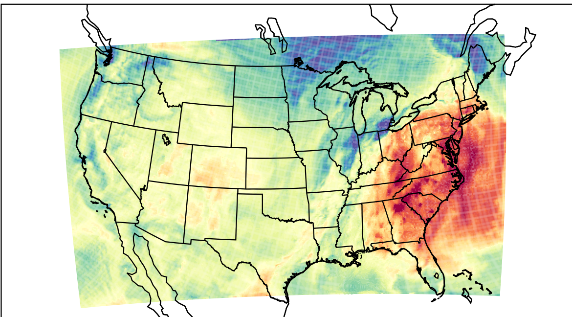
WRF (2021-10-15_18:00:00)
