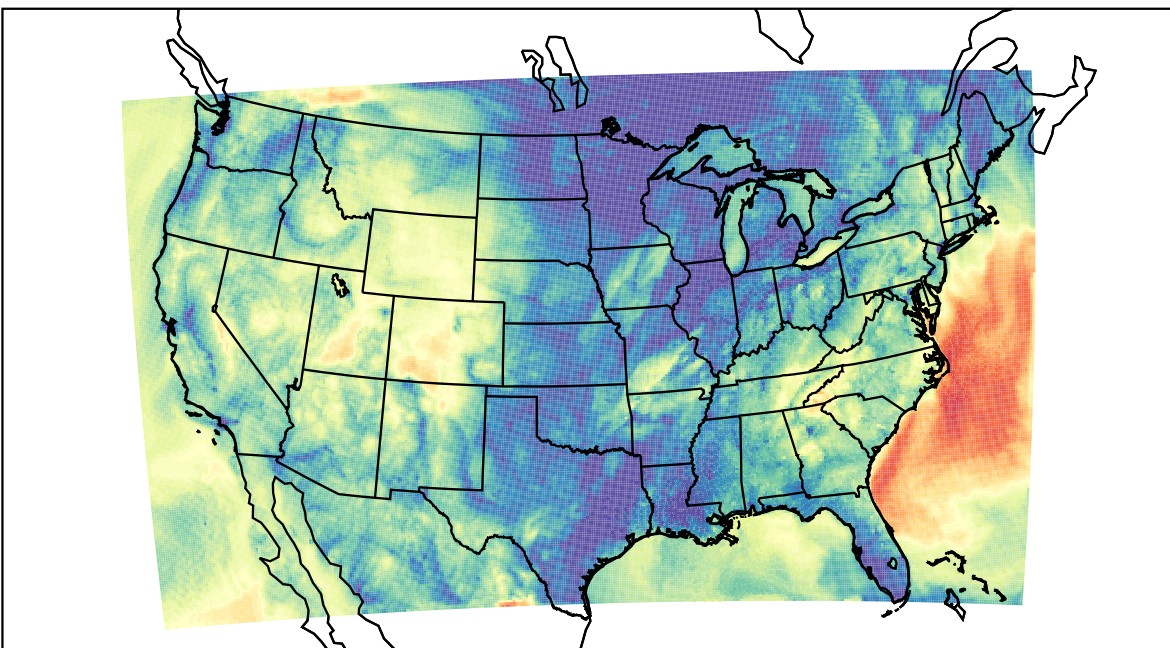
WRF (2021-10-15_13:00:00)
