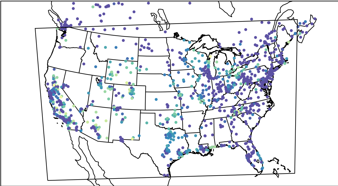
AirNOW (2021-10-14_05:00:00)
