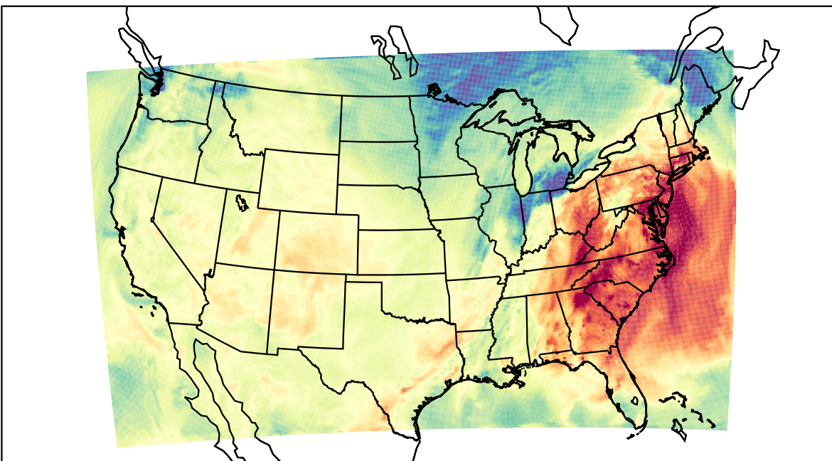
WRF (2021-10-15_20:00:00)
