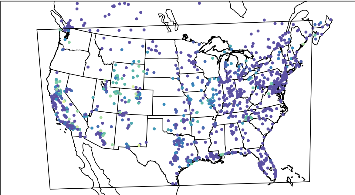
AirNOW (2021-10-14_10:00:00)
