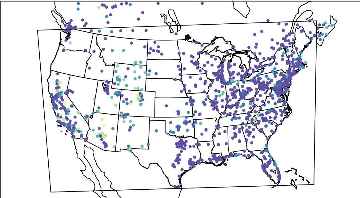
AirNOW (2021-10-15_13:00:00)
