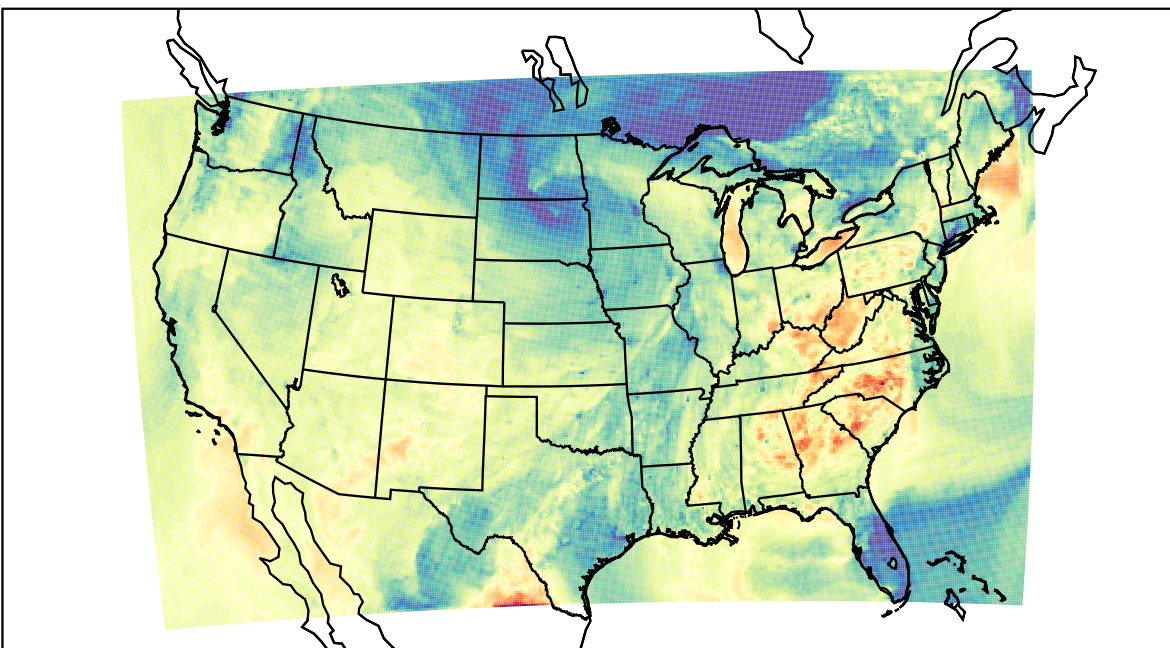
WRF (2021-10-14_00:00:00)
