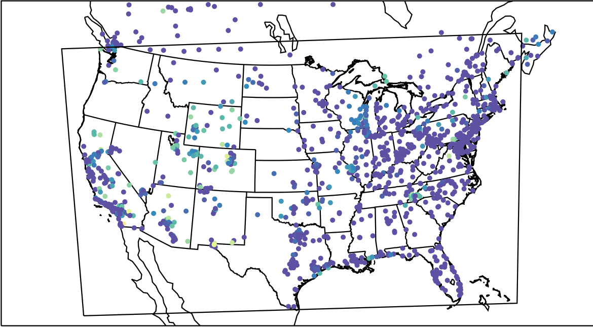
AirNOW (2021-10-14_12:00:00)
