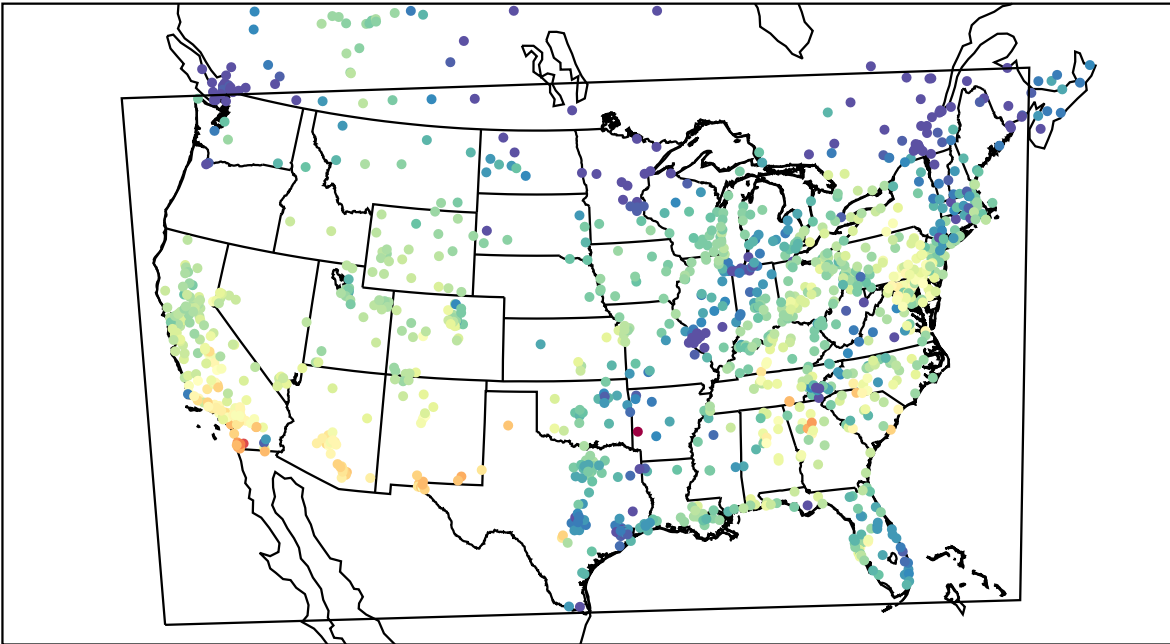
AirNOW (2021-10-14_21:00:00)
