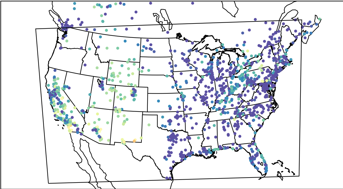
AirNOW (2021-10-15_02:00:00)
