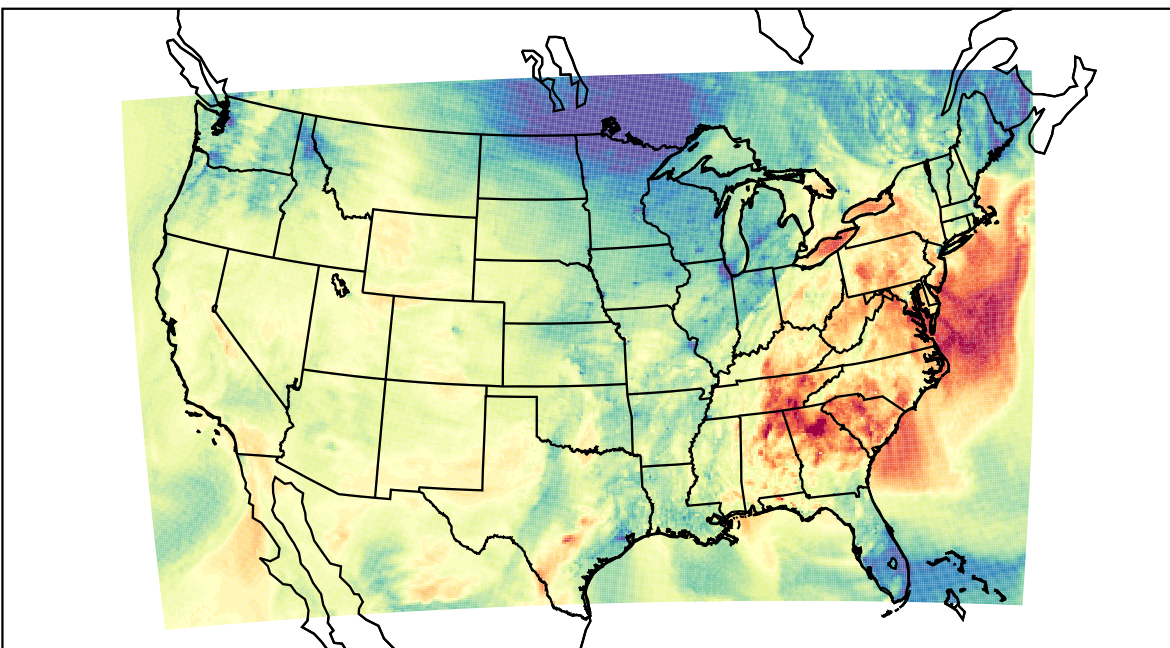
WRF (2021-10-14_23:00:00)
