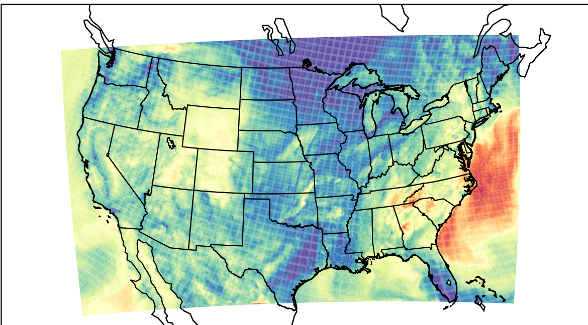
WRF (2021-10-15_08:00:00)
