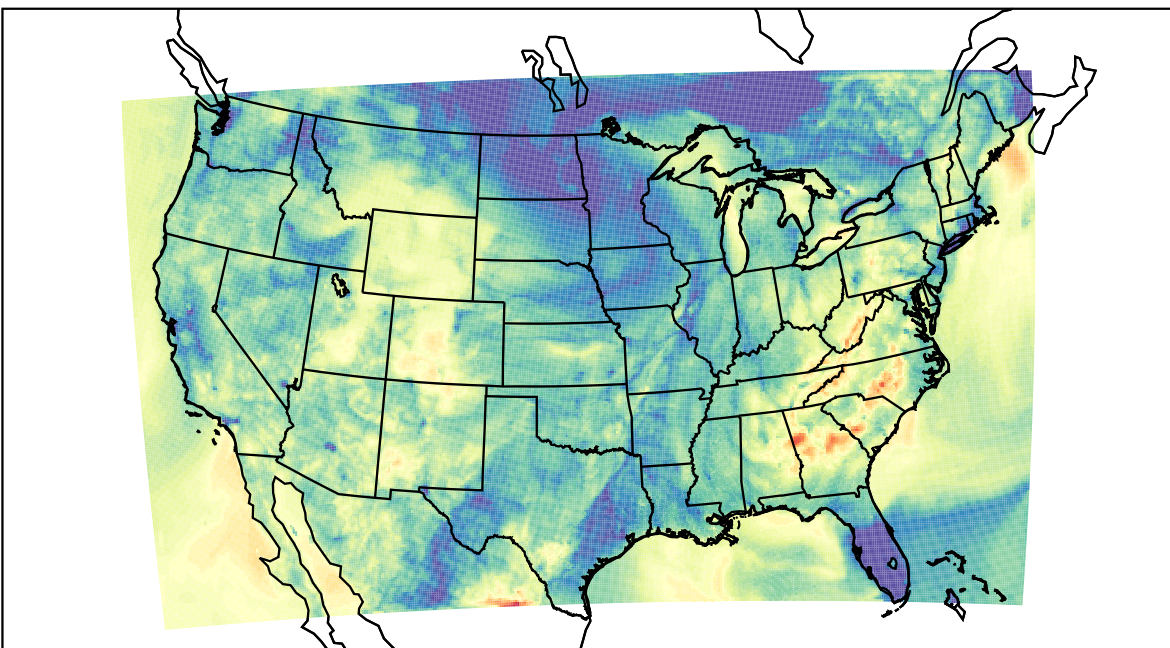
WRF (2021-10-14_05:00:00)
