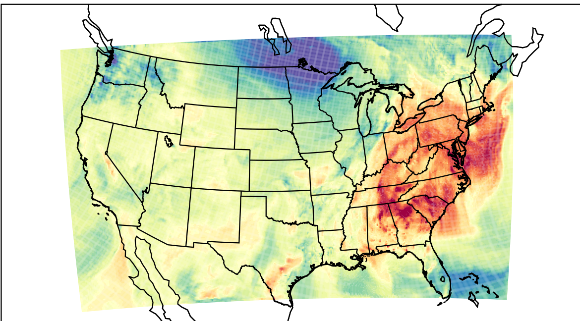
WRF (2021-10-14_20:00:00)
