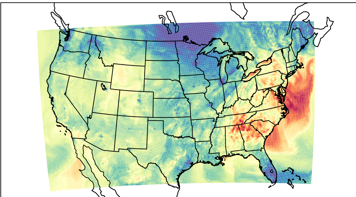
WRF (2021-10-15_01:00:00)
