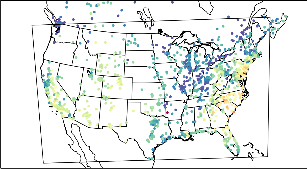
AirNOW (2021-10-15_18:00:00)
