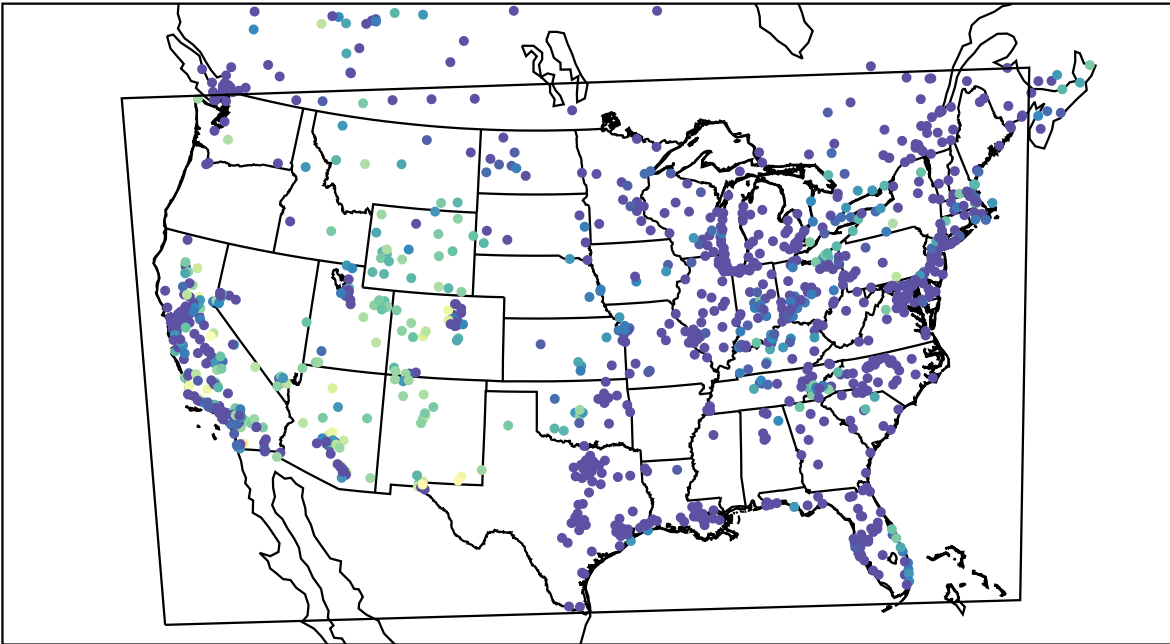
AirNOW (2021-10-15_06:00:00)
