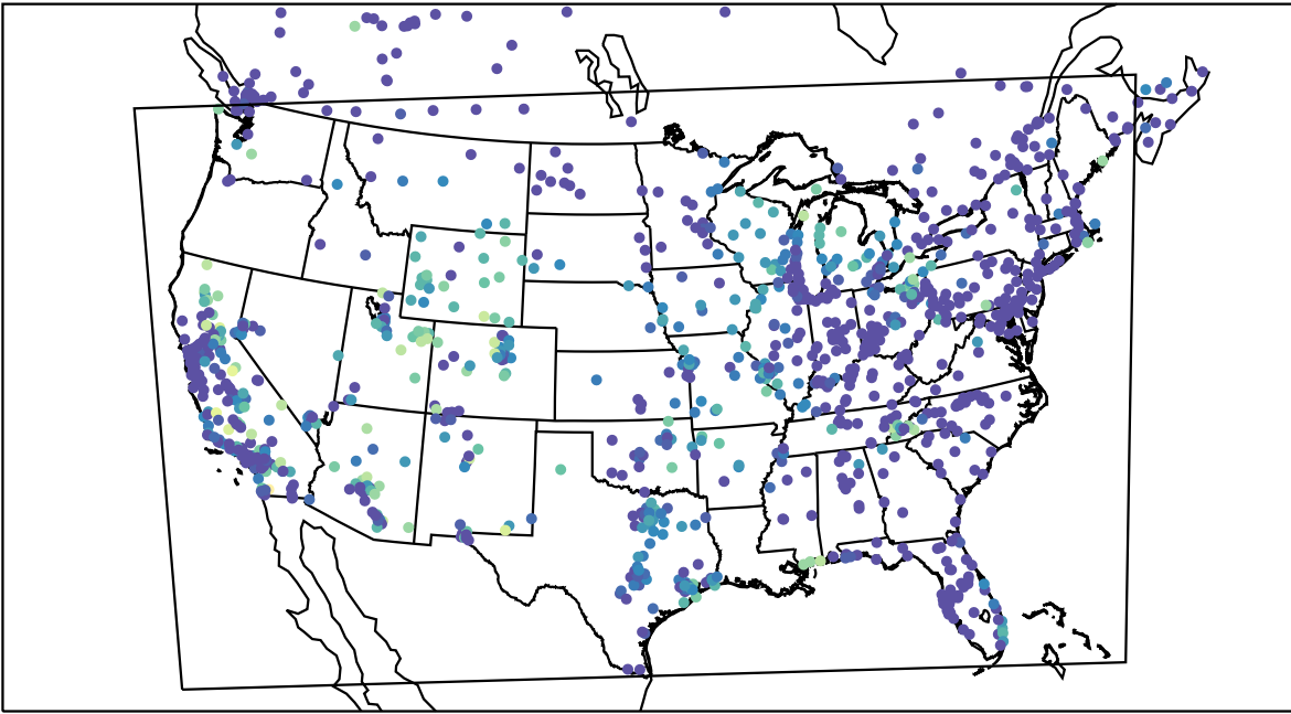
AirNOW (2021-10-14_07:00:00)
