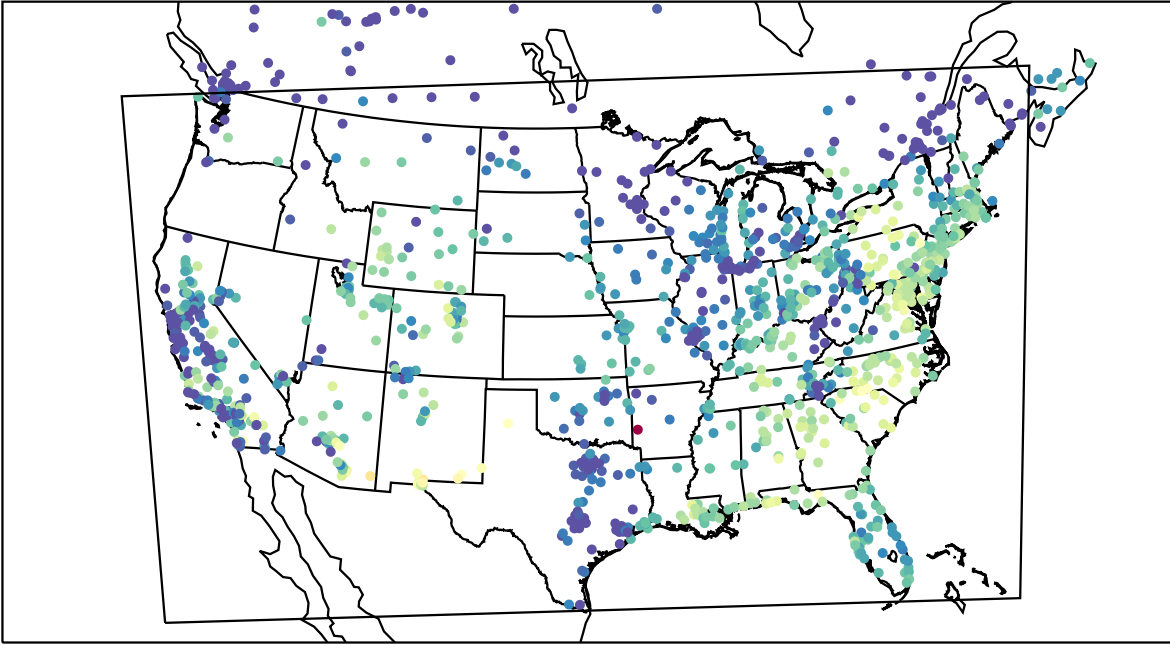
AirNOW (2021-10-14_16:00:00)
