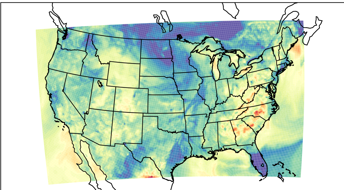
WRF (2021-10-14_03:00:00)
