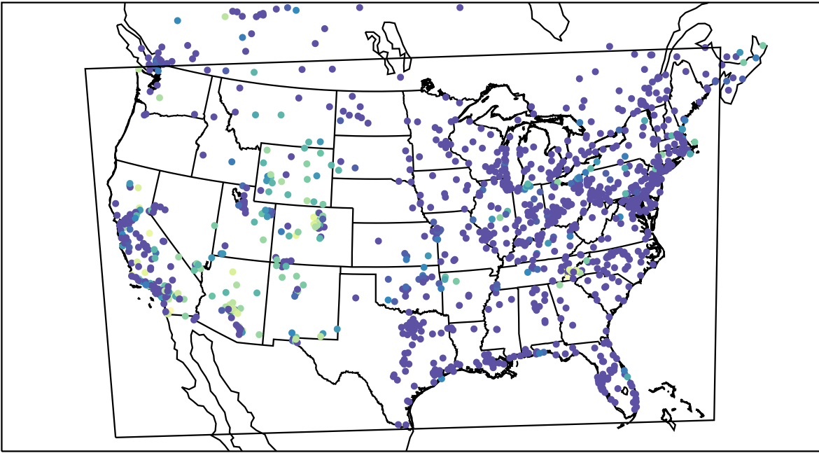
AirNOW (2021-10-15_12:00:00)
