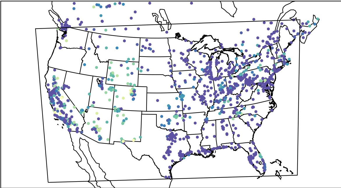
AirNOW (2021-10-15_08:00:00)
