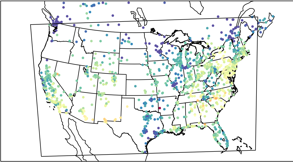
AirNOW (2021-10-14_18:00:00)
