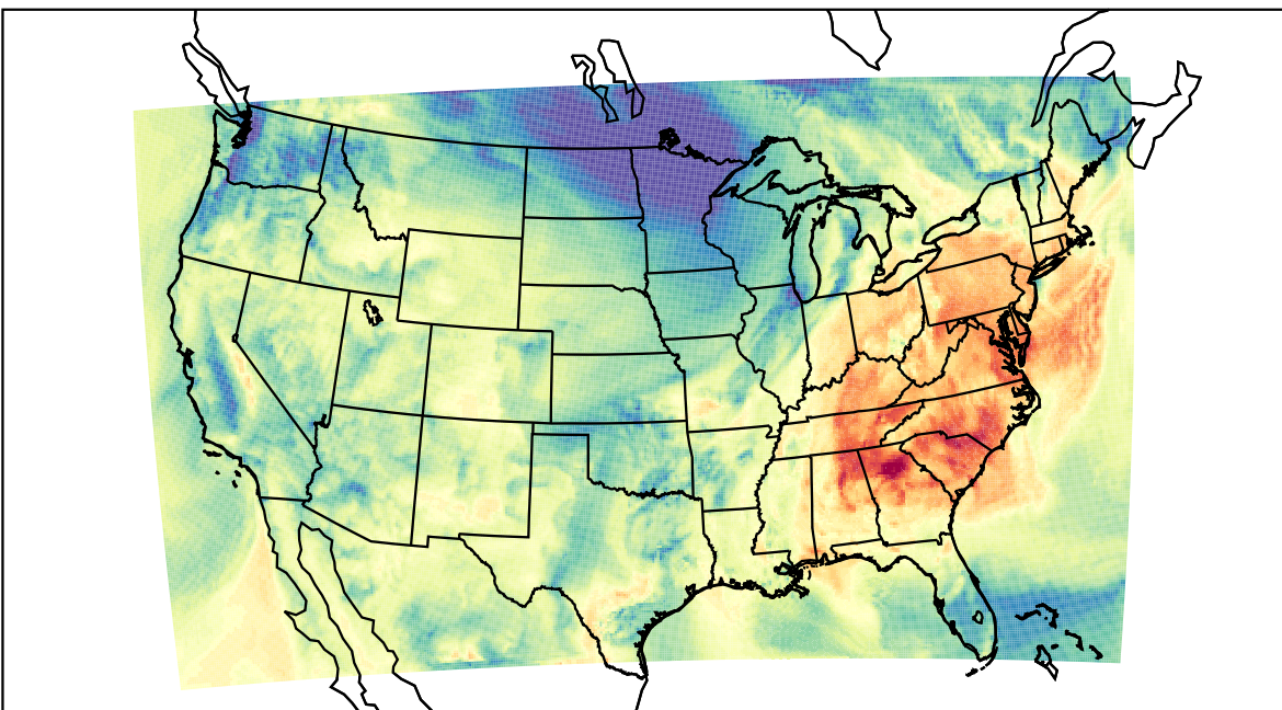
WRF (2021-10-14_17:00:00)
