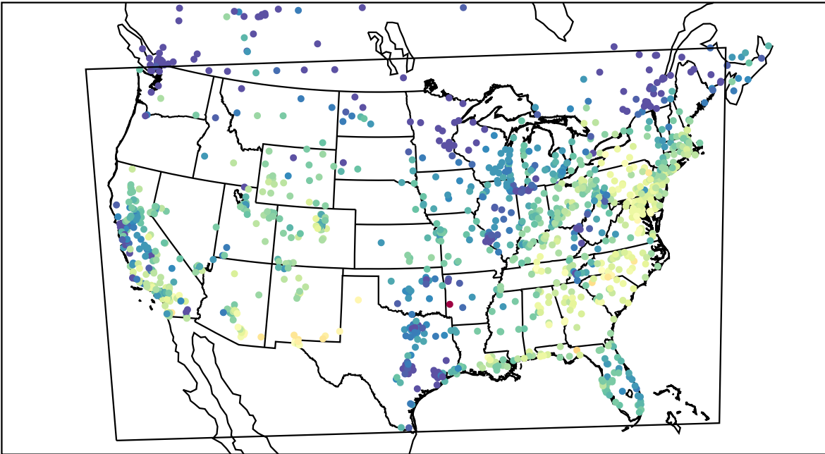
AirNOW (2021-10-14_17:00:00)
