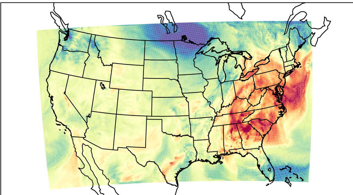
WRF (2021-10-14_21:00:00)
