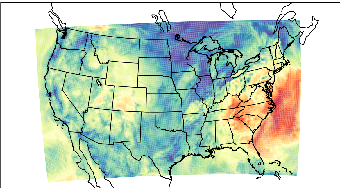
WRF (2021-10-15_15:00:00)
