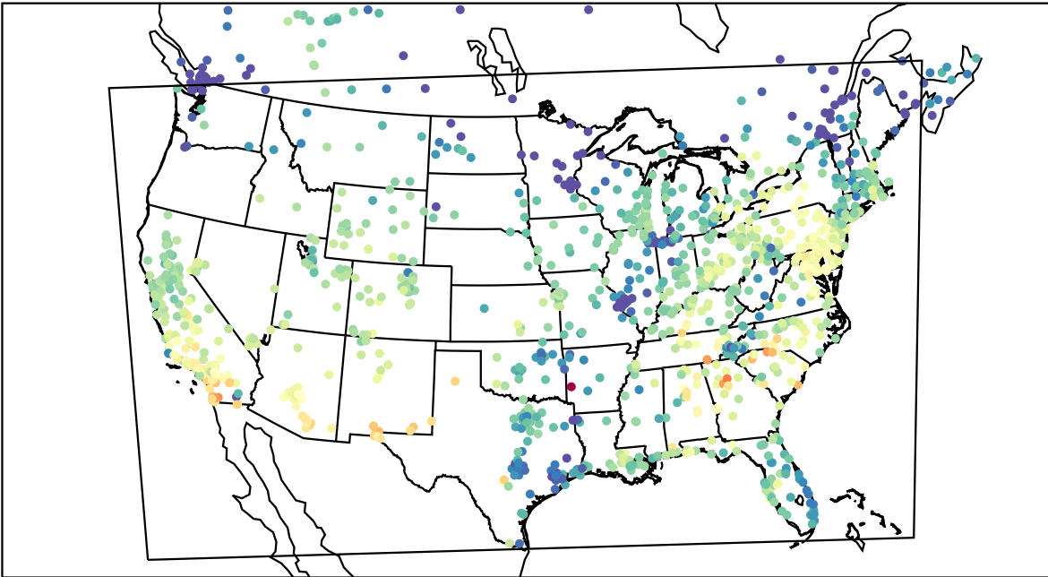
AirNOW (2021-10-14_20:00:00)
