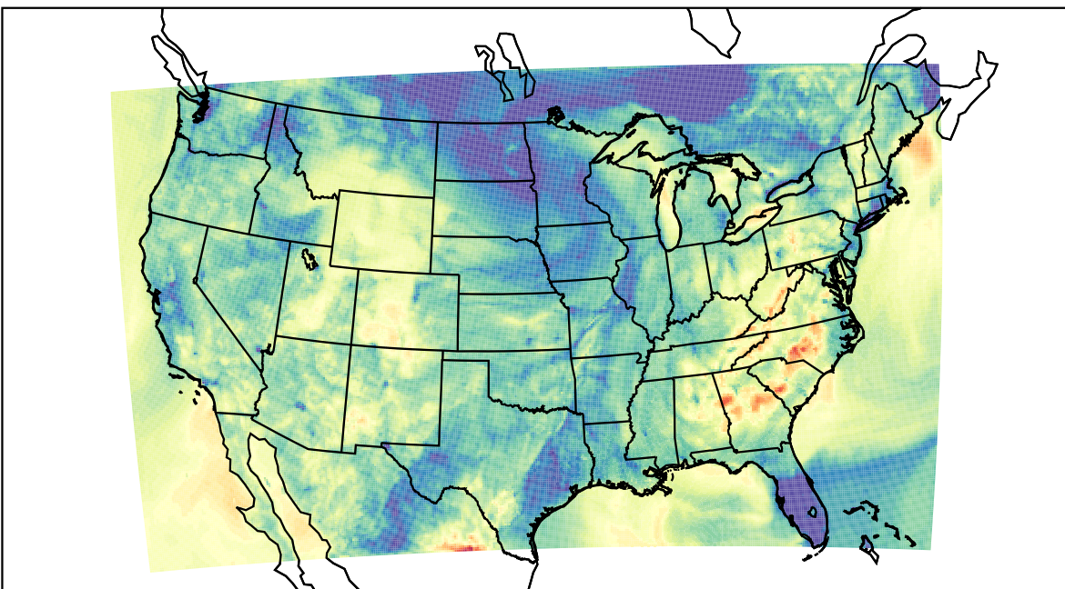
WRF (2021-10-14_04:00:00)
