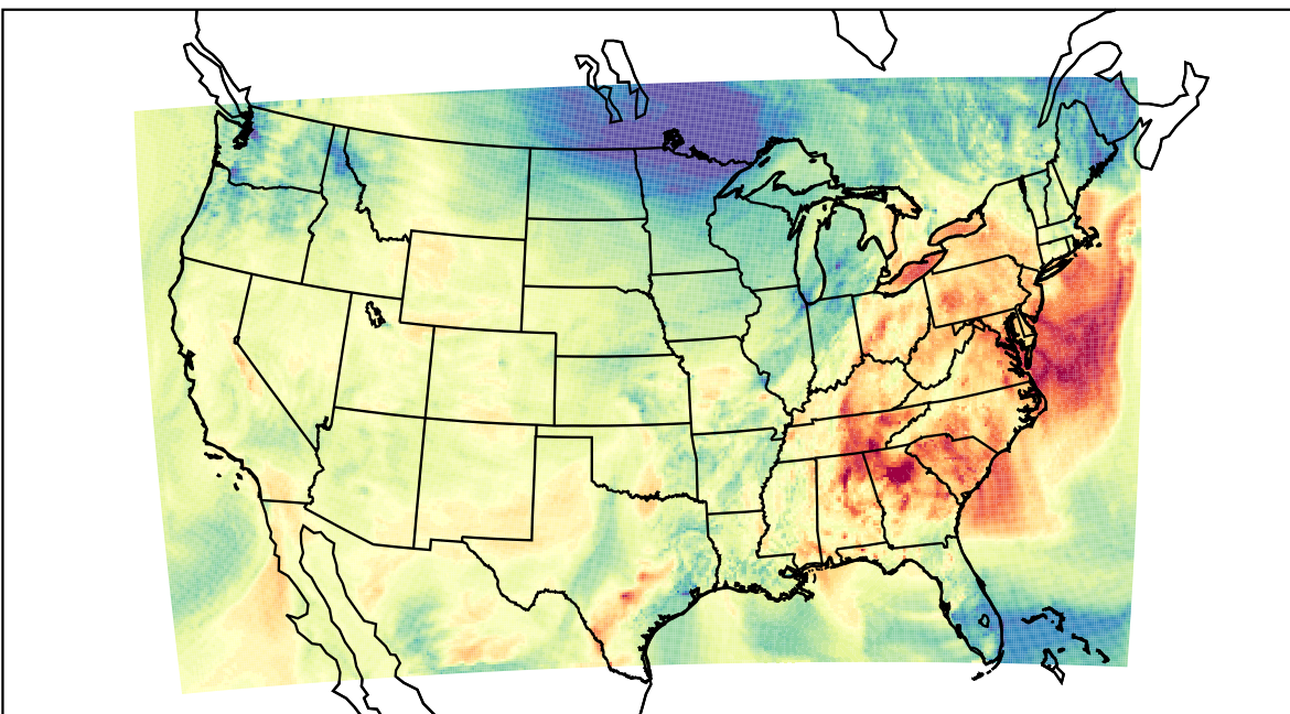
WRF (2021-10-14_22:00:00)
