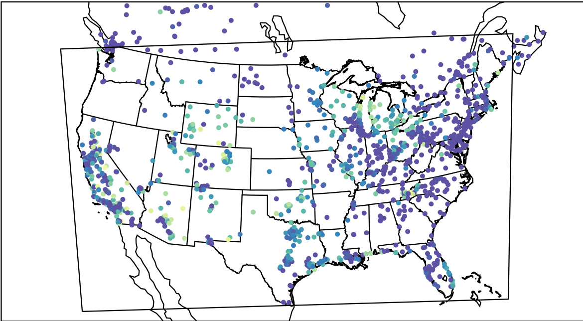
AirNOW (2021-10-14_04:00:00)
