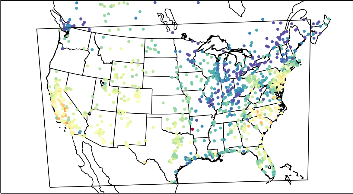
AirNOW (2021-10-15_21:00:00)
