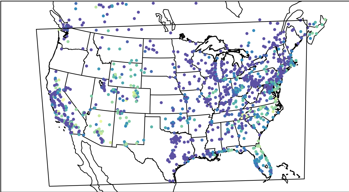
AirNOW (2021-10-15_14:00:00)
