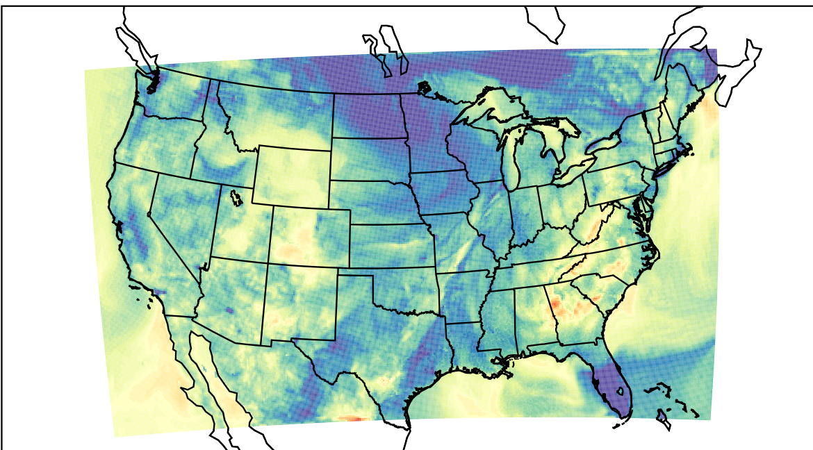
WRF (2021-10-14_07:00:00)
