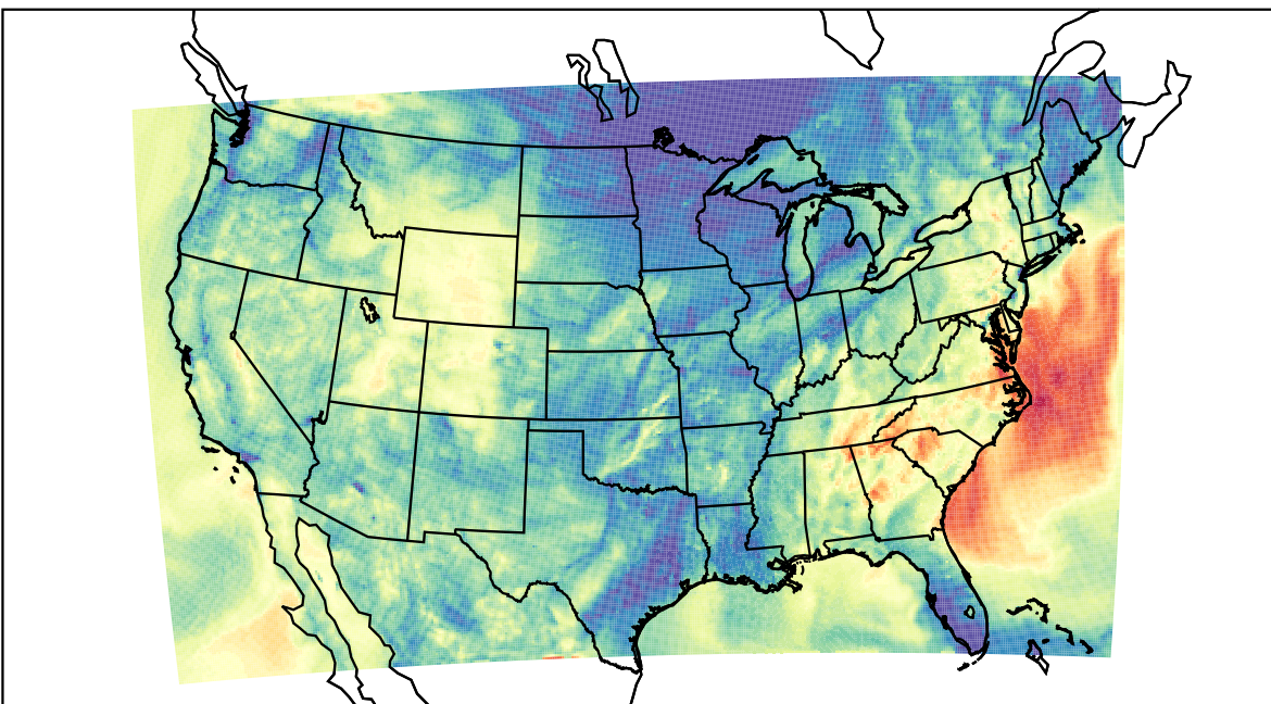
WRF (2021-10-15_06:00:00)
