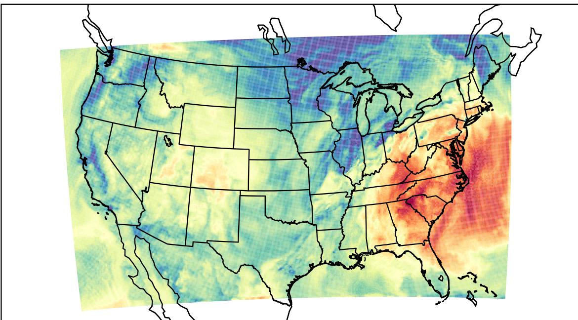
WRF (2021-10-15_16:00:00)
