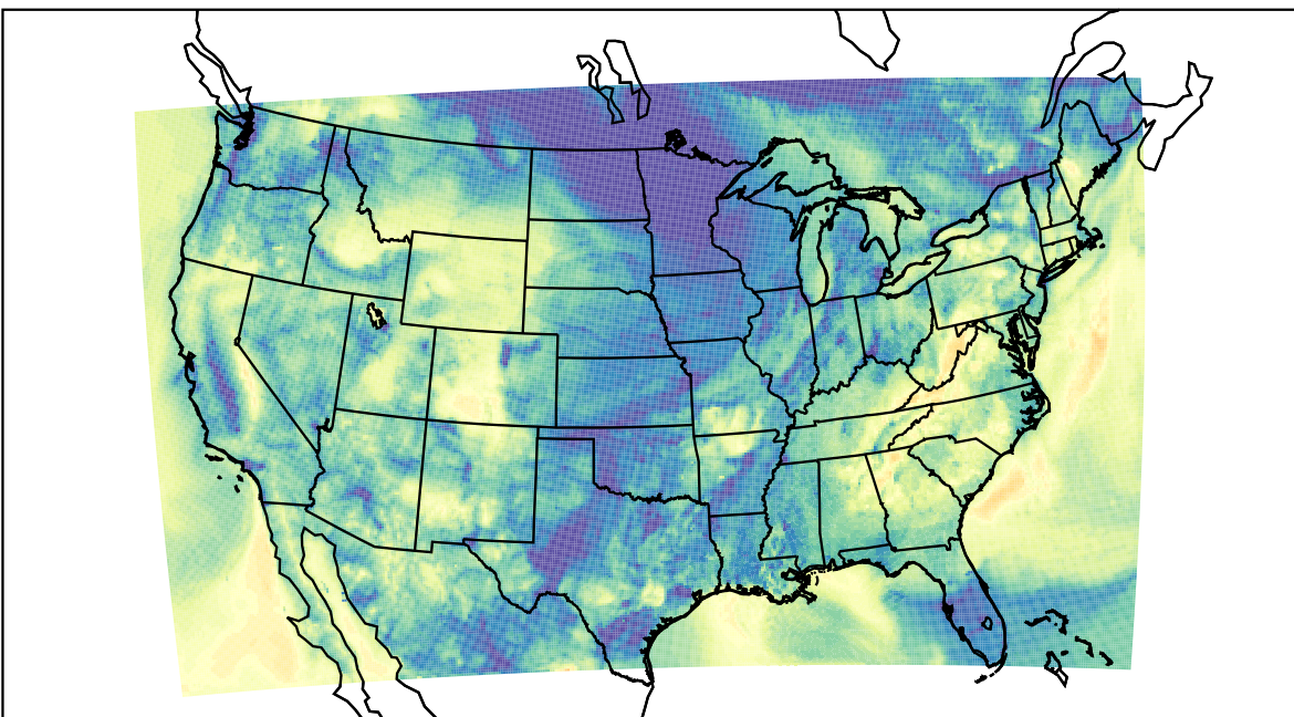
WRF (2021-10-14_14:00:00)
