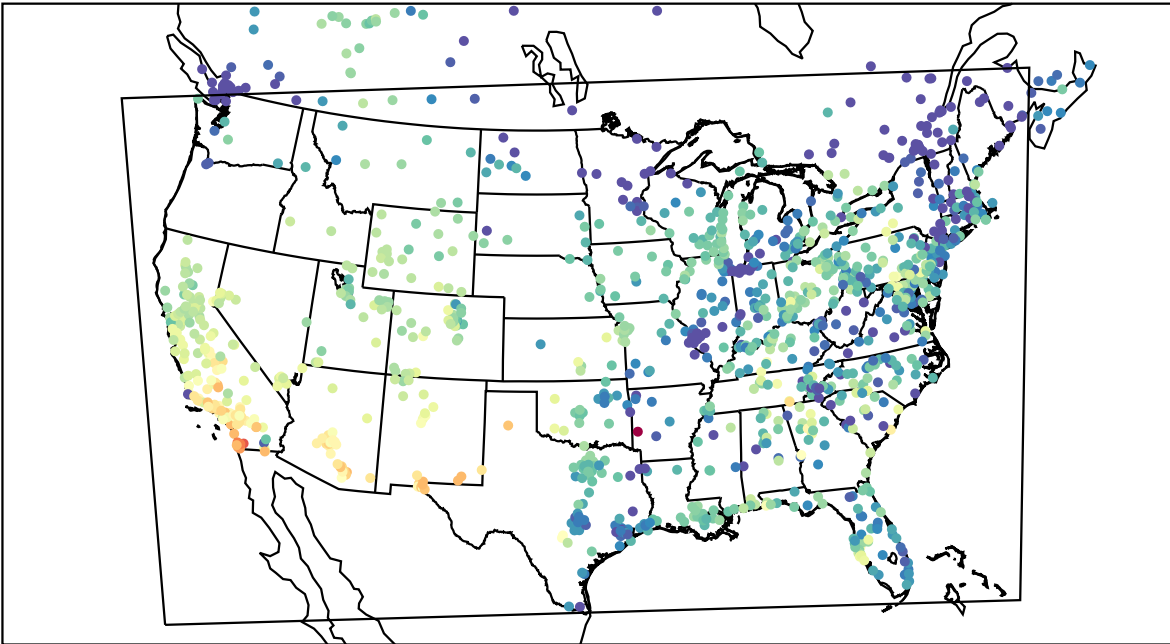
AirNOW (2021-10-14_22:00:00)
