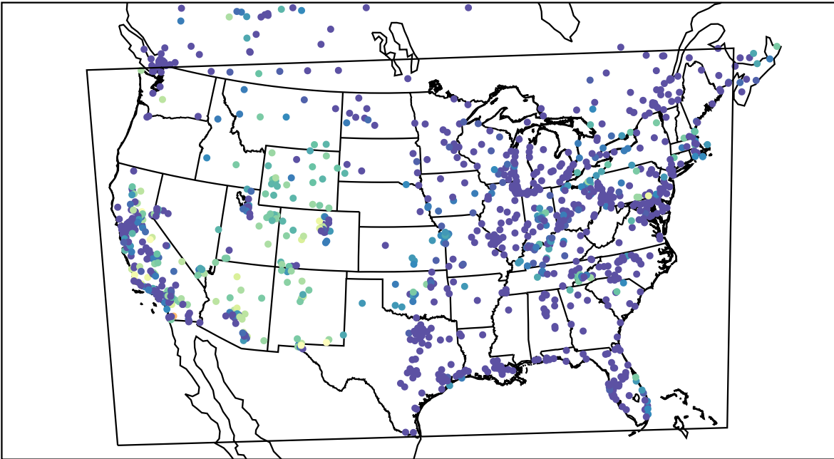
AirNOW (2021-10-15_07:00:00)
