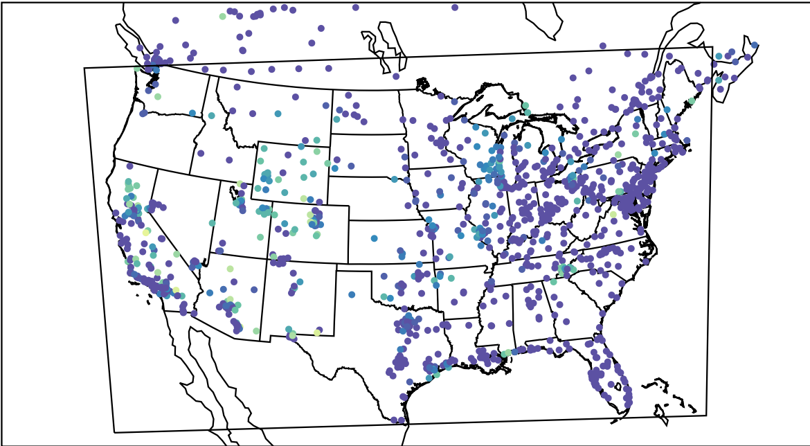
AirNOW (2021-10-14_11:00:00)
