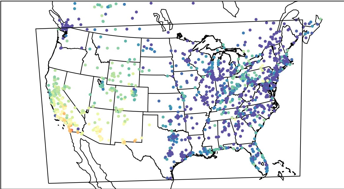
AirNOW (2021-10-15_00:00:00)
