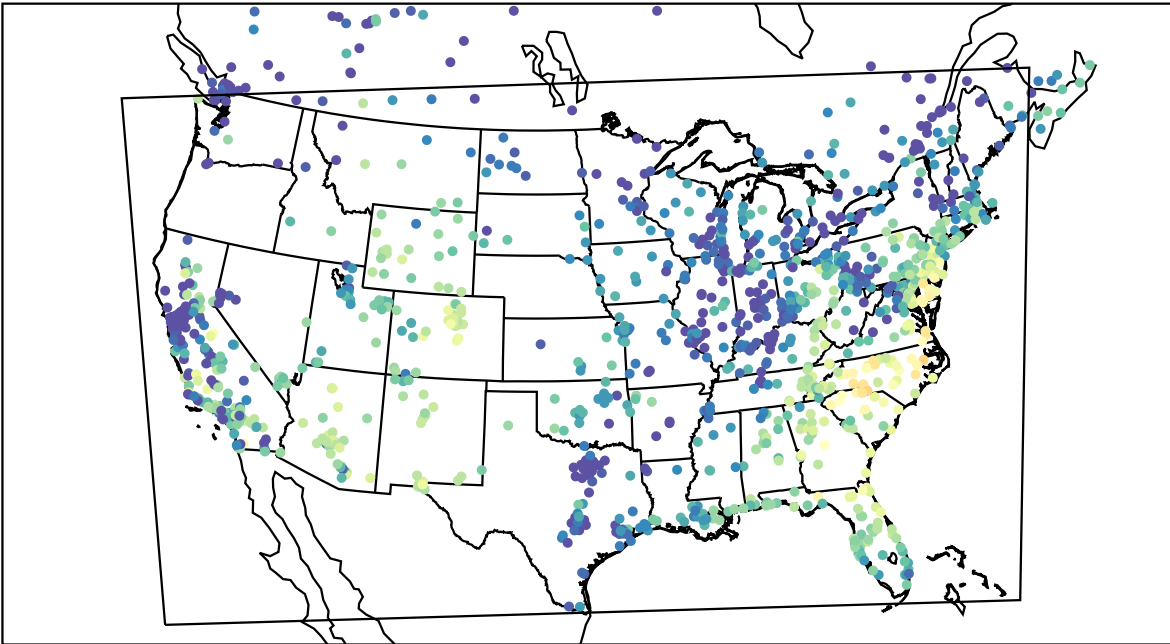
AirNOW (2021-10-15_16:00:00)
