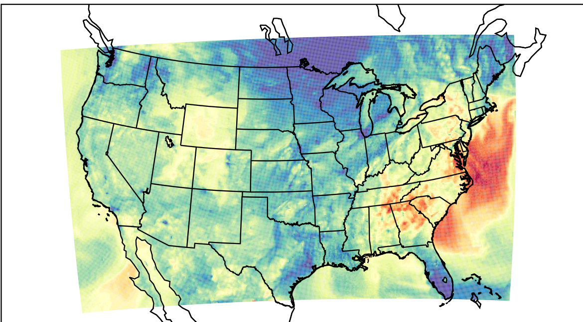
WRF (2021-10-15_03:00:00)
