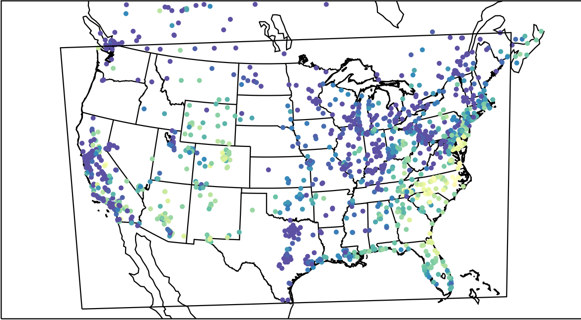
AirNOW (2021-10-15_15:00:00)
