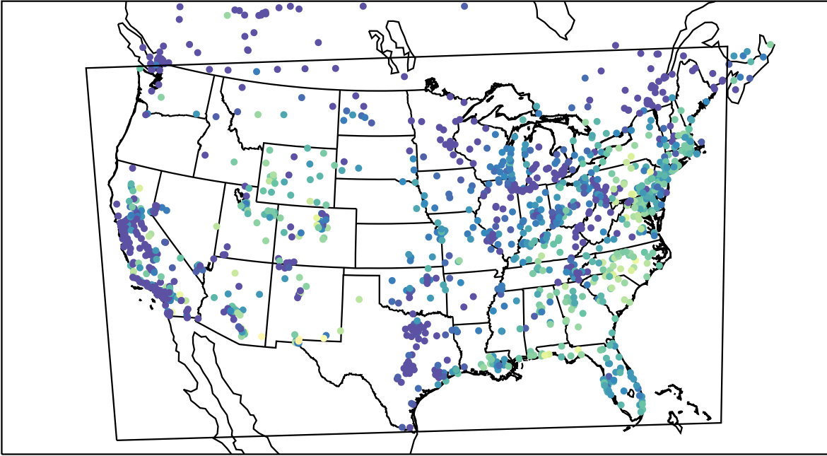
AirNOW (2021-10-14_15:00:00)
