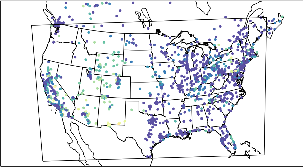
AirNOW (2021-10-15_04:00:00)
