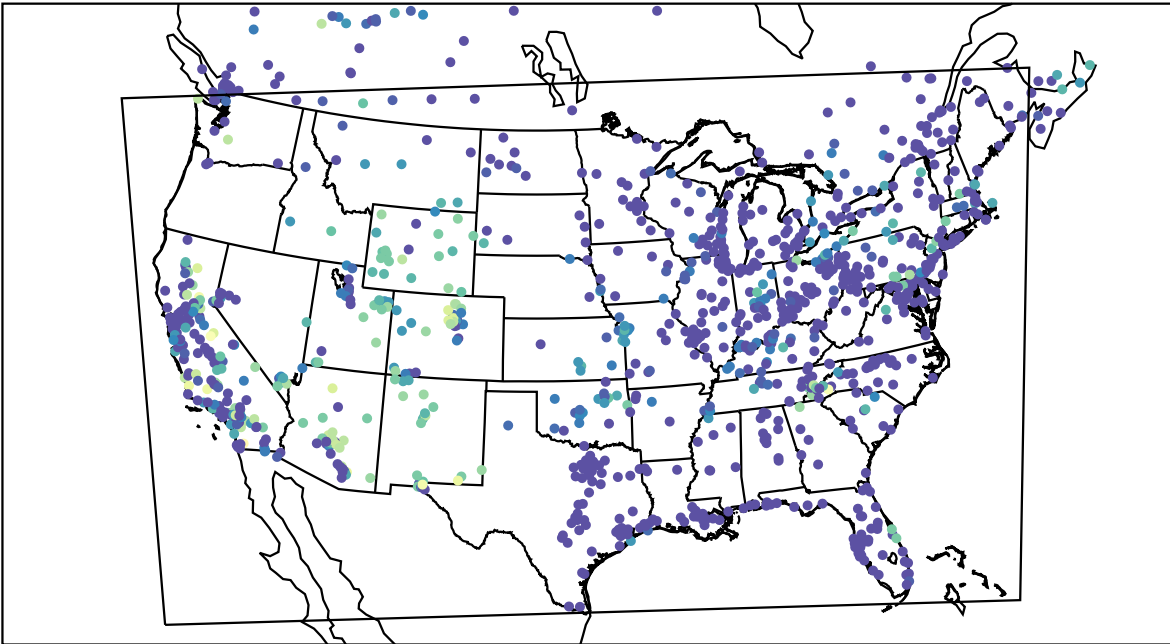
AirNOW (2021-10-15_09:00:00)
