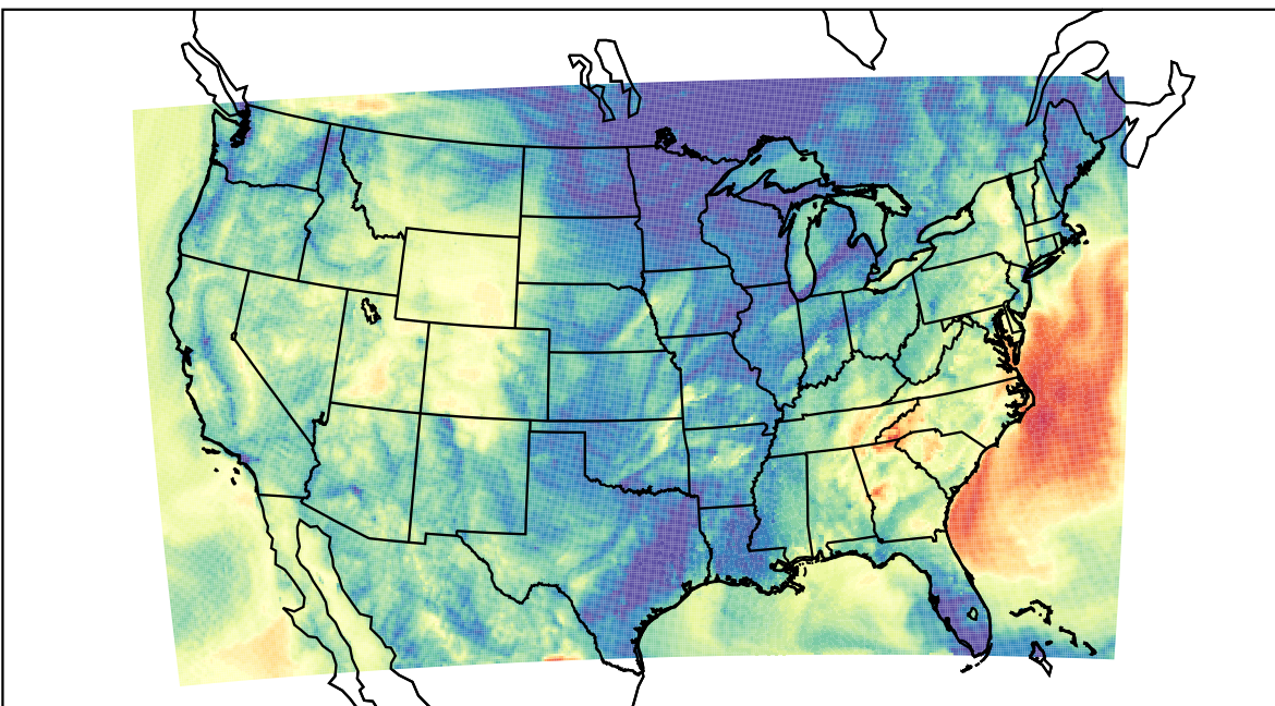
WRF (2021-10-15_09:00:00)
