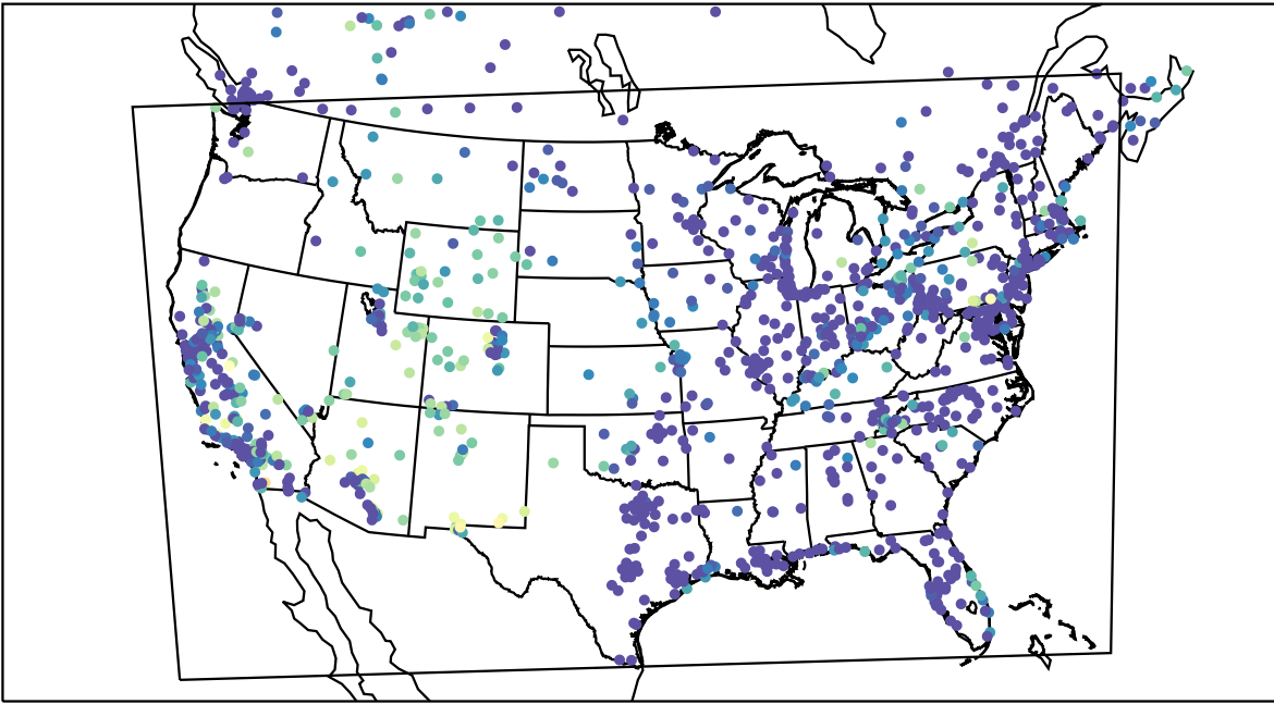
AirNOW (2021-10-15_05:00:00)
