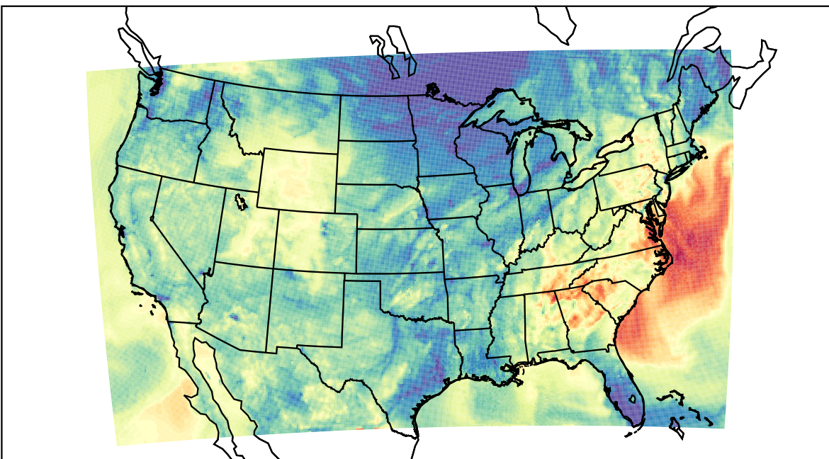
WRF (2021-10-15_04:00:00)
