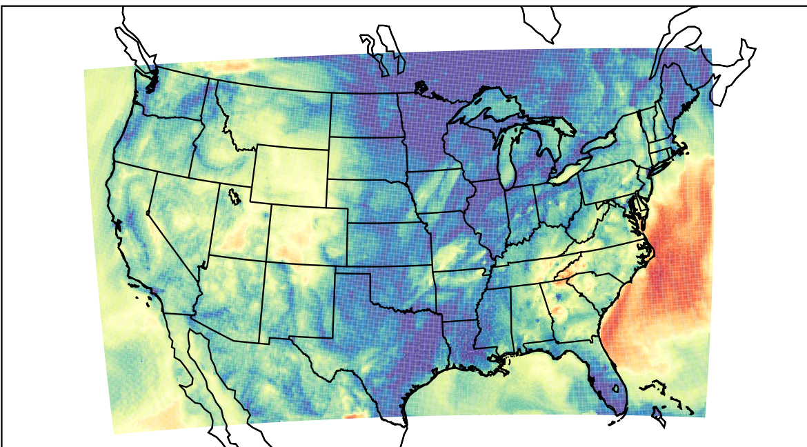
WRF (2021-10-15_12:00:00)
