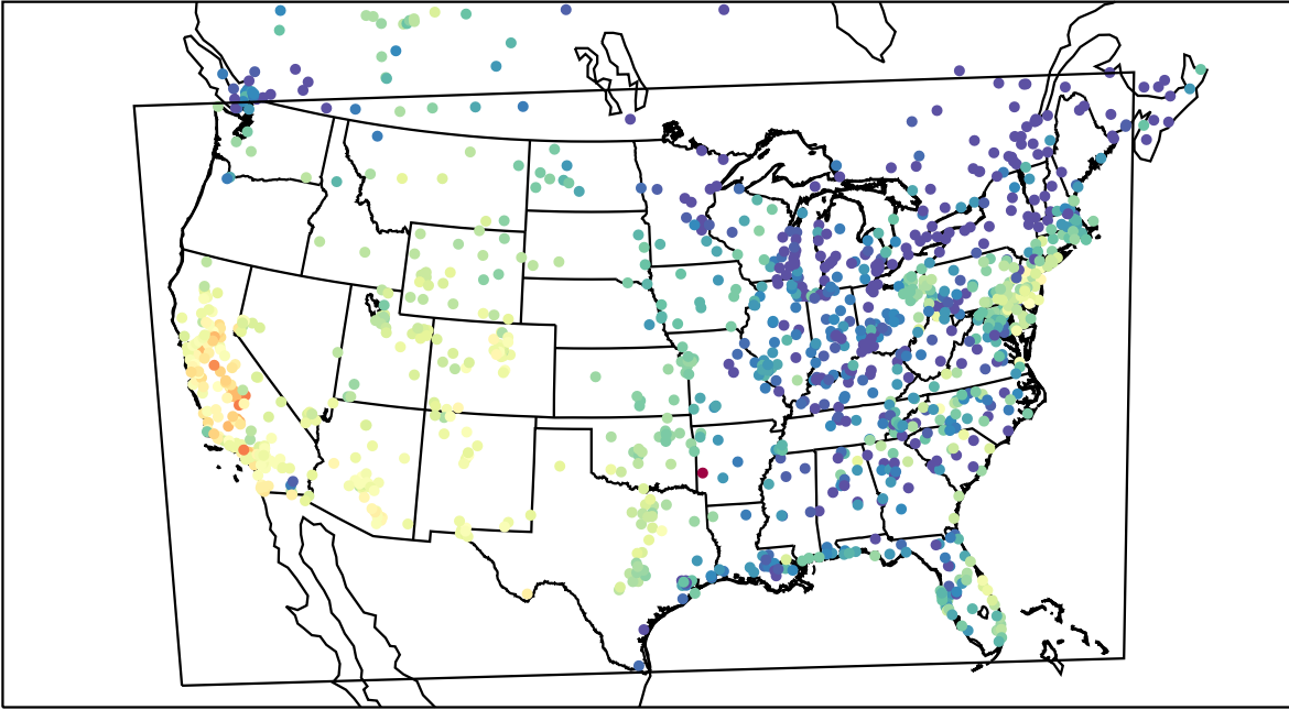
AirNOW (2021-10-15_23:00:00)
