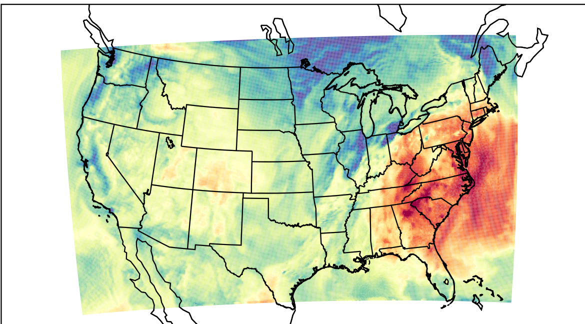
WRF (2021-10-15_17:00:00)
