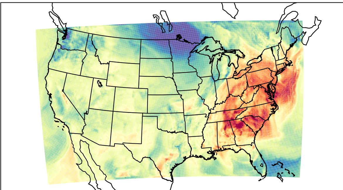
WRF (2021-10-14_19:00:00)
