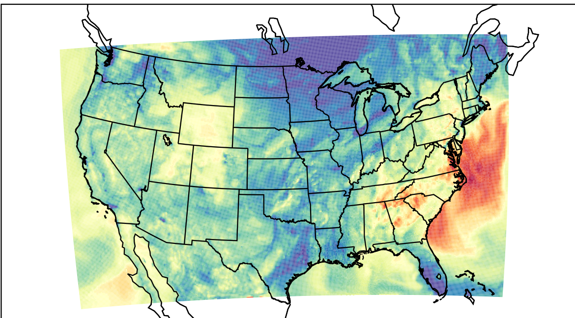
WRF (2021-10-15_05:00:00)
