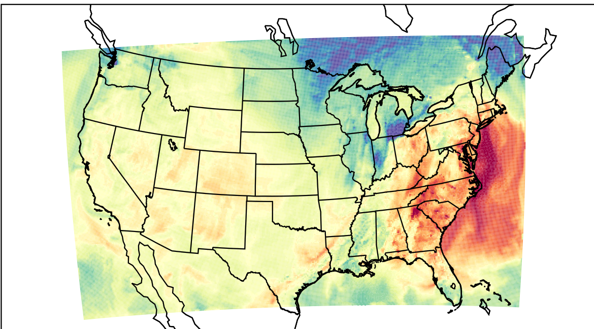
WRF (2021-10-15_22:00:00)
