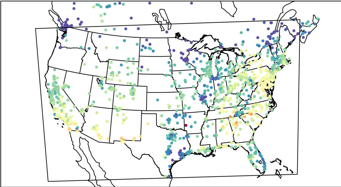
AirNOW (2021-10-14_19:00:00)
