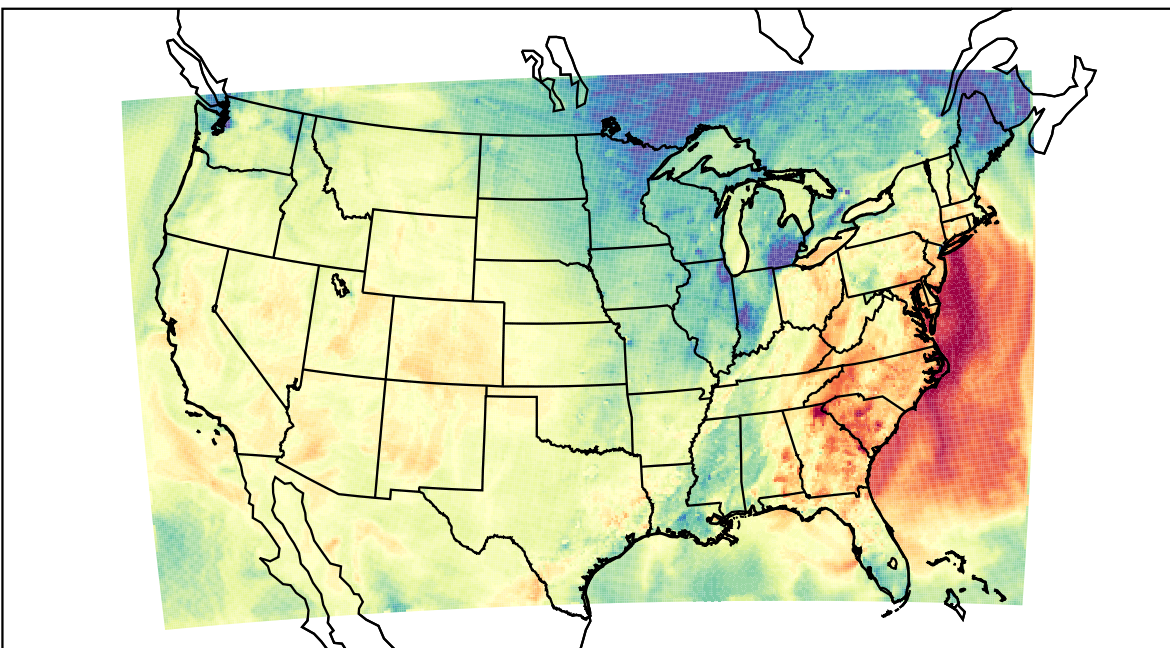
WRF (2021-10-15_23:00:00)
