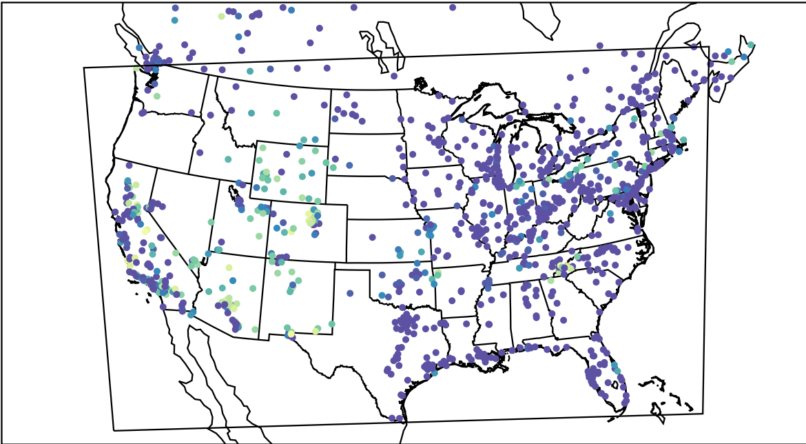
AirNOW (2021-10-15_11:00:00)
