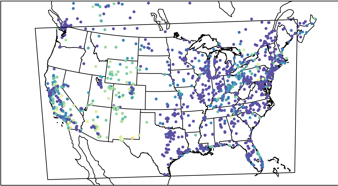
AirNOW (2021-10-15_03:00:00)
