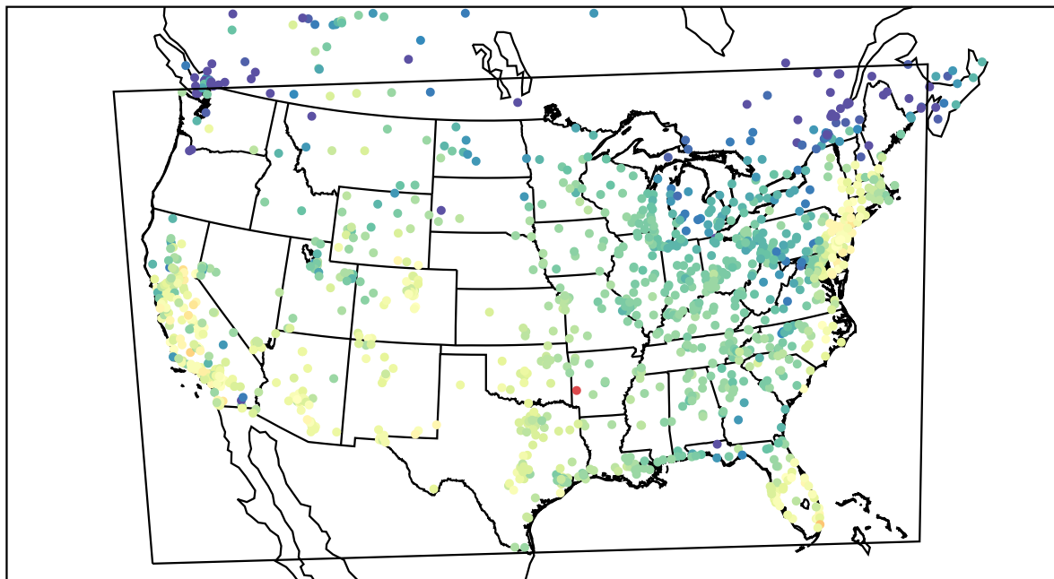
AirNOW (2021-10-16_18:00:00)
