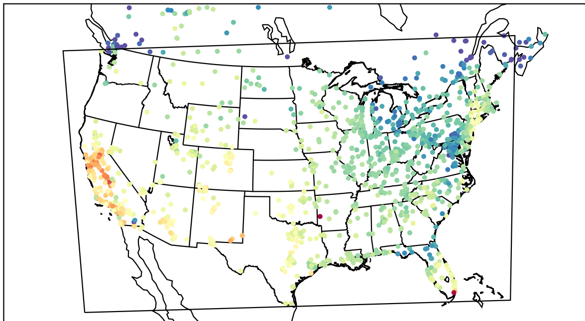
AirNOW (2021-10-16_21:00:00)
