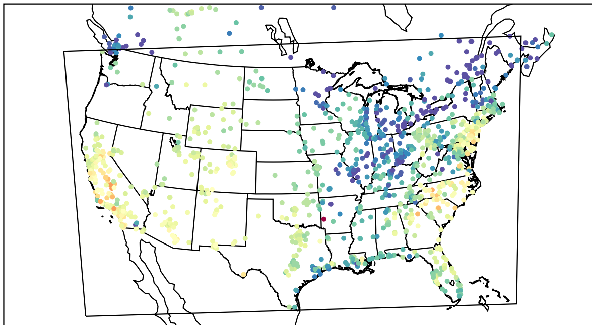
AirNOW (2021-10-15_21:00:00)
