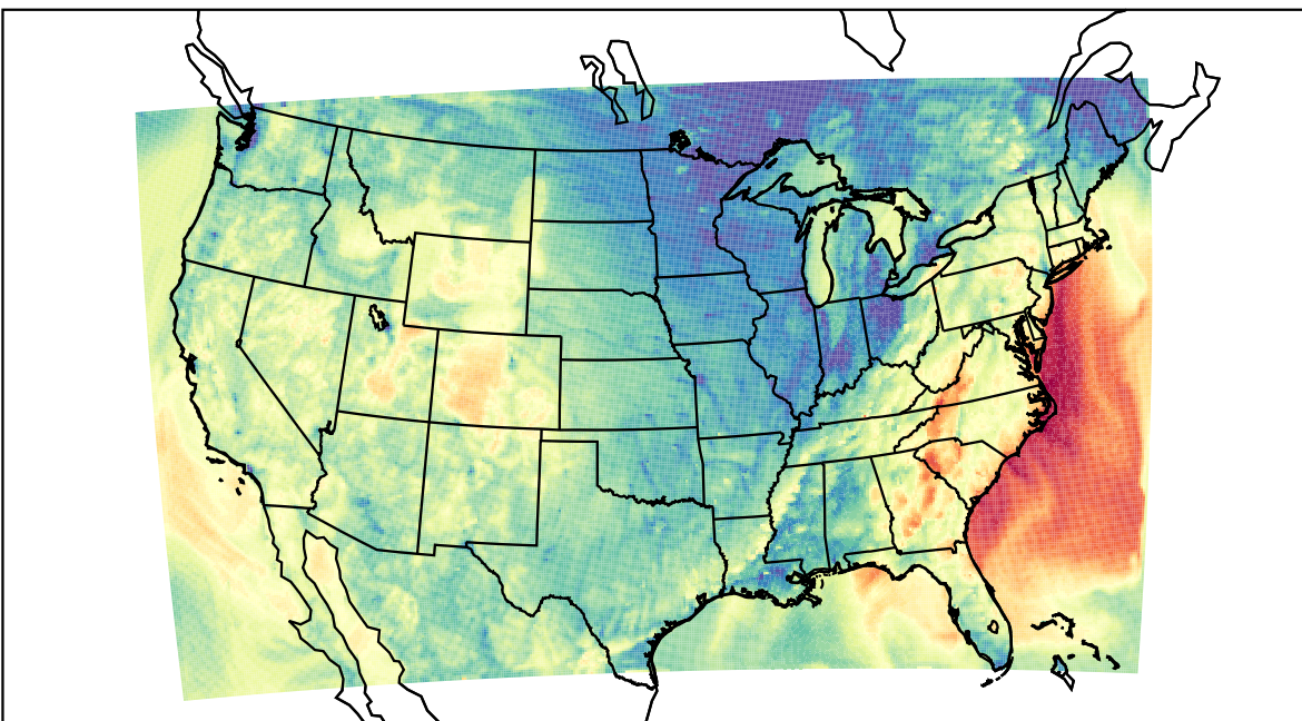
WRF (2021-10-16_03:00:00)
