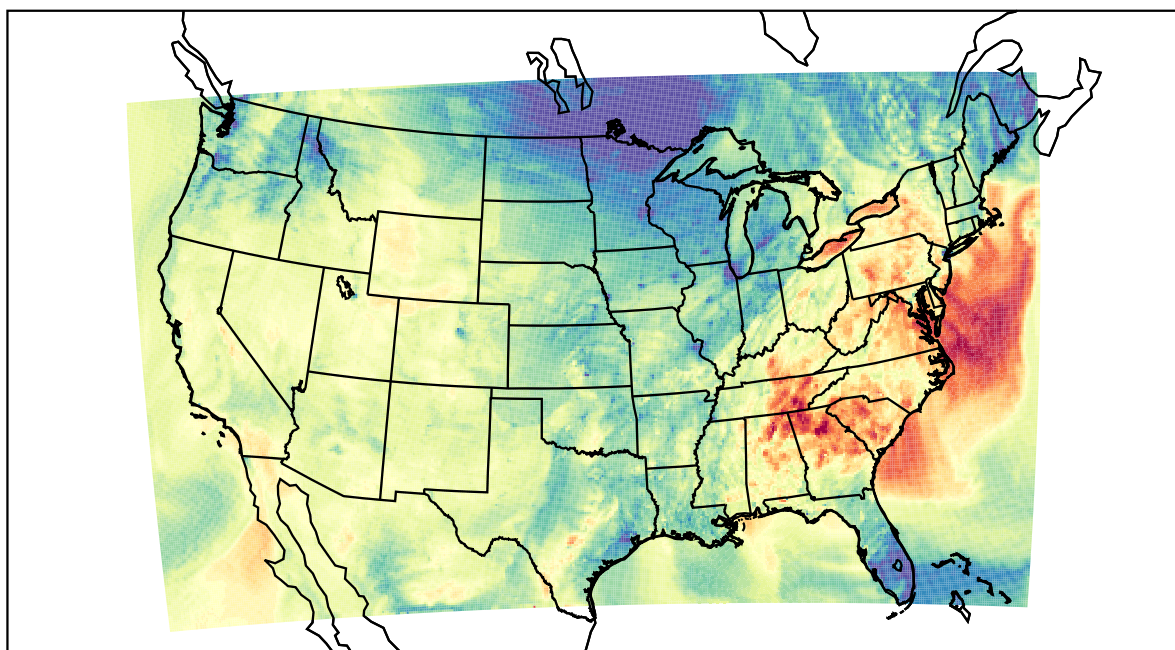
WRF (2021-10-15_00:00:00)
