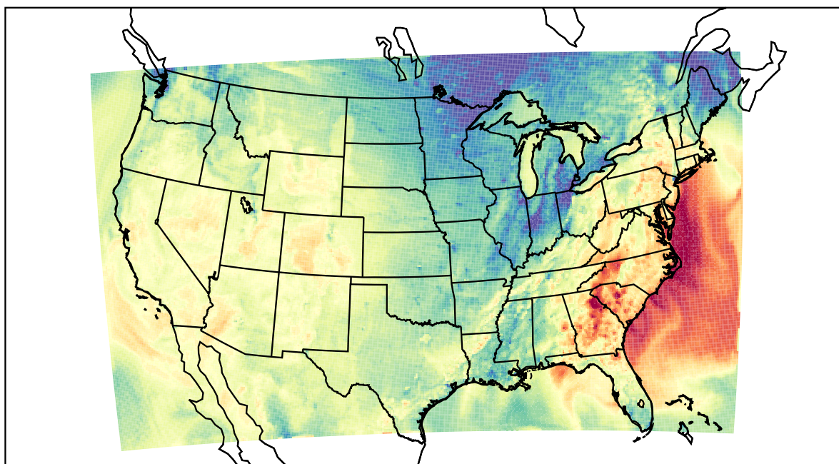
WRF (2021-10-16_00:00:00)
