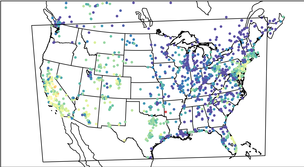
AirNOW (2021-10-16_01:00:00)
