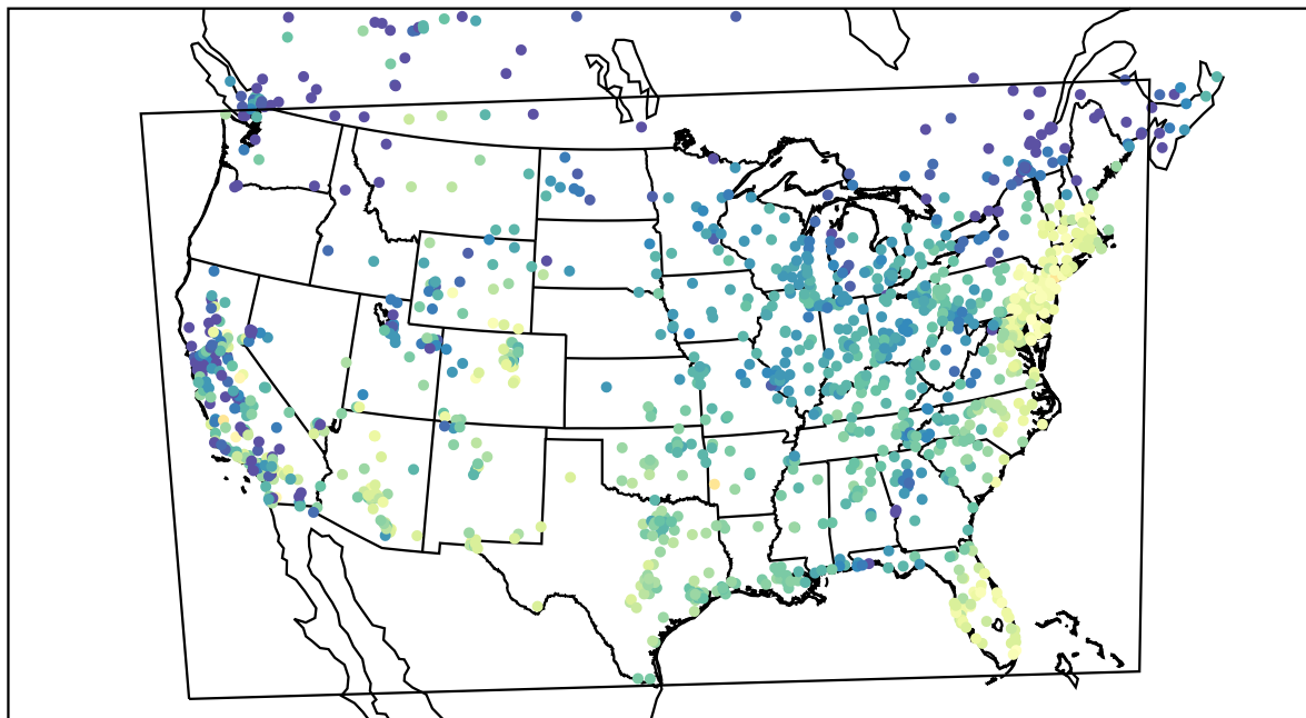
AirNOW (2021-10-16_16:00:00)
