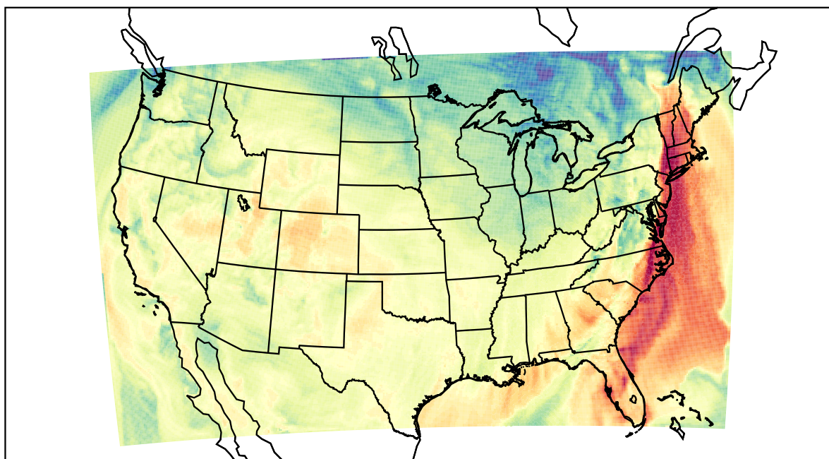
WRF (2021-10-16_19:00:00)
