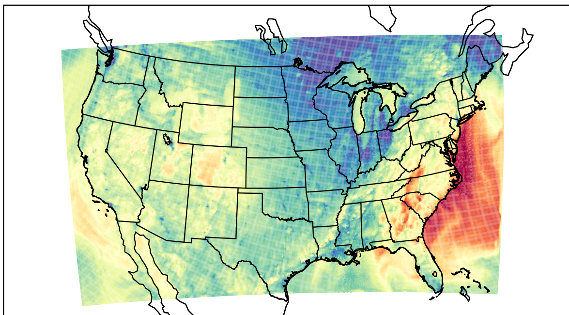
WRF (2021-10-16_02:00:00)
