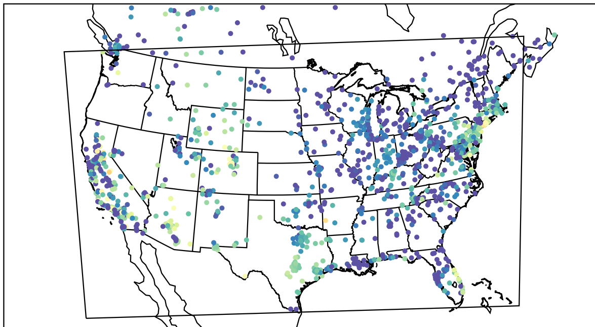
AirNOW (2021-10-16_04:00:00)
