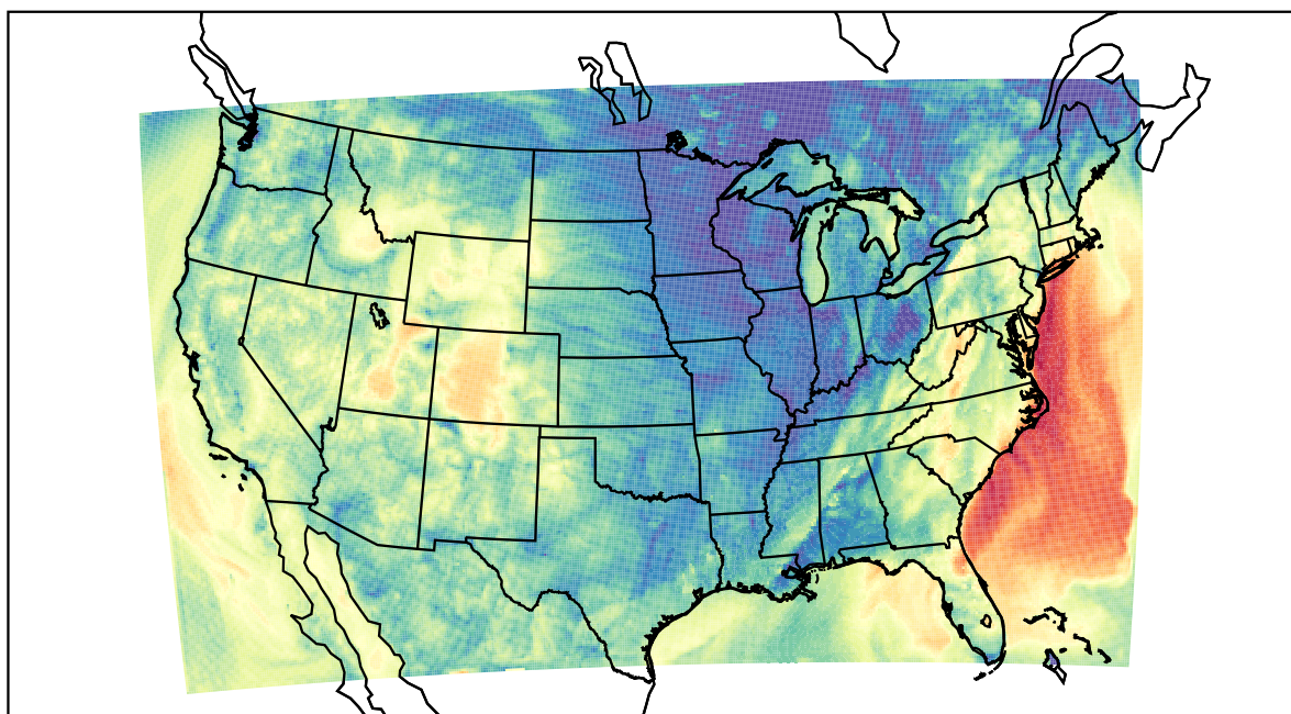
WRF (2021-10-16_08:00:00)
