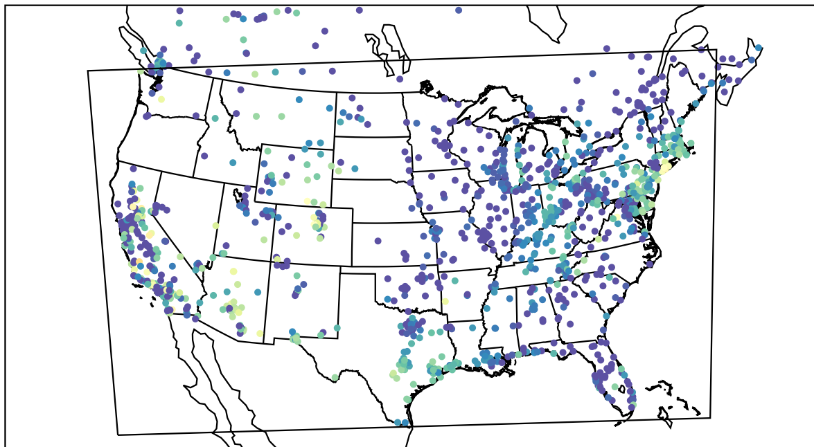
AirNOW (2021-10-16_08:00:00)
