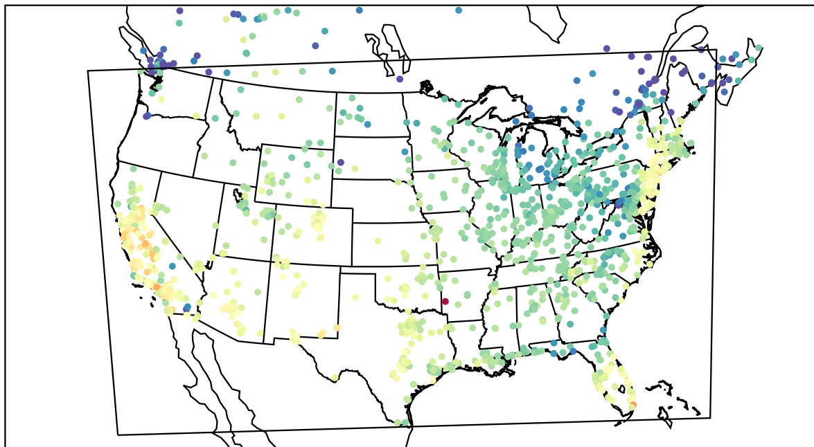
AirNOW (2021-10-16_19:00:00)
