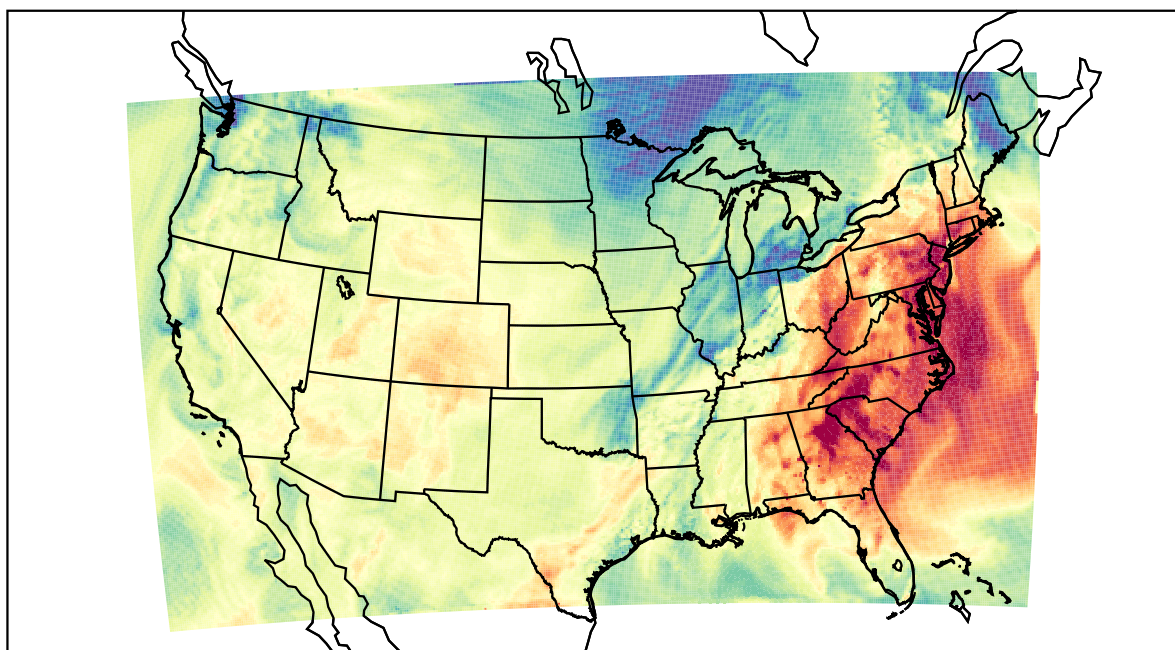
WRF (2021-10-15_19:00:00)
