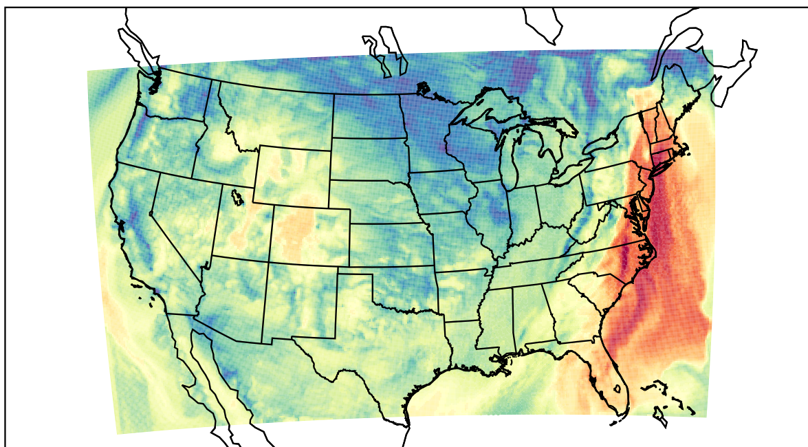
WRF (2021-10-16_16:00:00)
