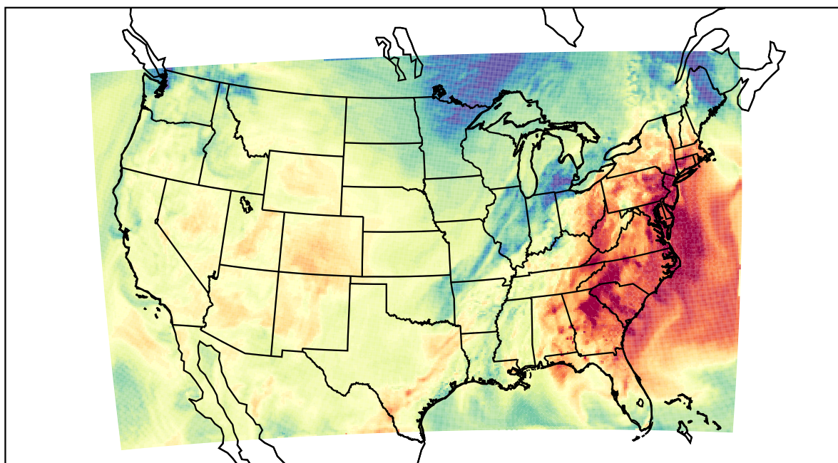
WRF (2021-10-15_20:00:00)
