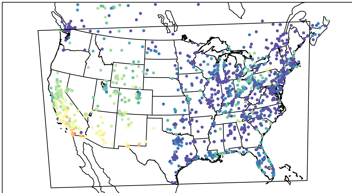
AirNOW (2021-10-15_00:00:00)
