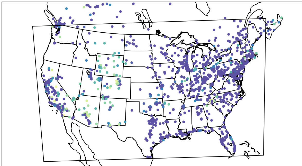
AirNOW (2021-10-15_12:00:00)
