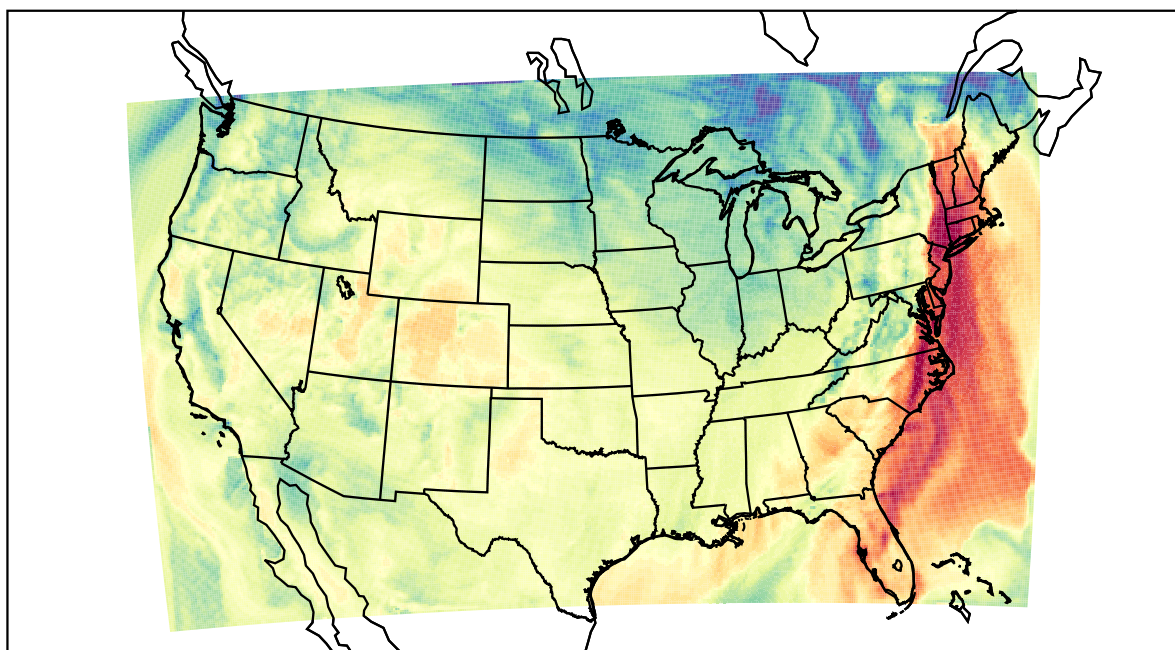
WRF (2021-10-16_18:00:00)
