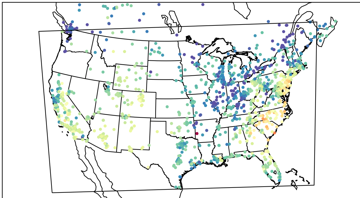
AirNOW (2021-10-15_18:00:00)
