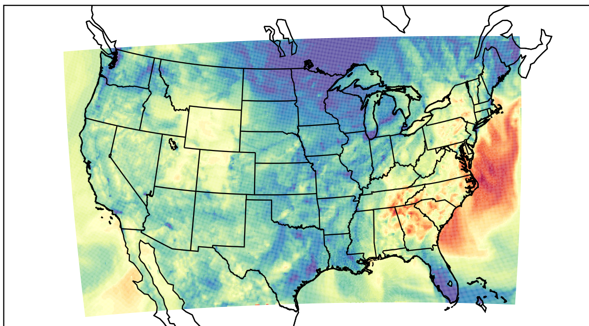
WRF (2021-10-15_04:00:00)
