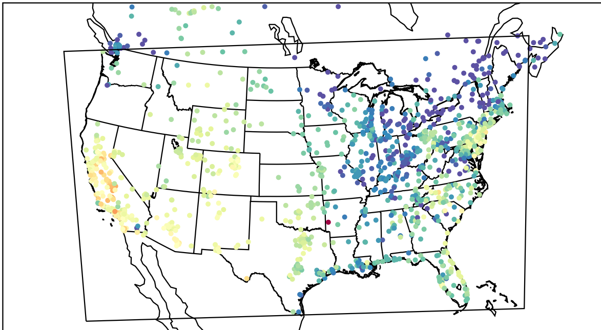
AirNOW (2021-10-15_22:00:00)
