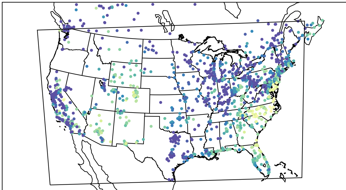
AirNOW (2021-10-15_15:00:00)
