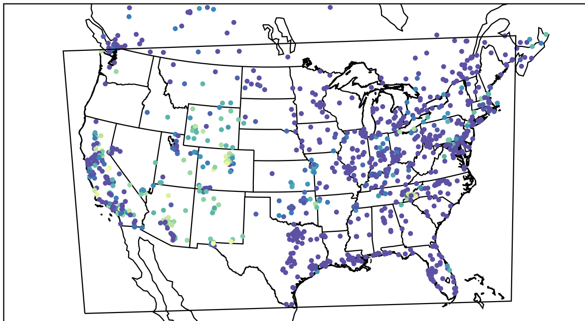
AirNOW (2021-10-15_10:00:00)
