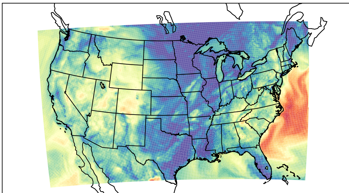
WRF (2021-10-15_13:00:00)
