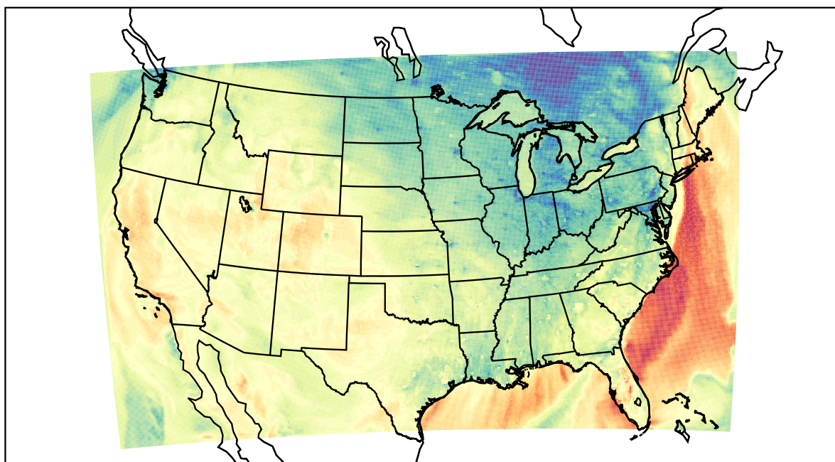
WRF (2021-10-16_23:00:00)
