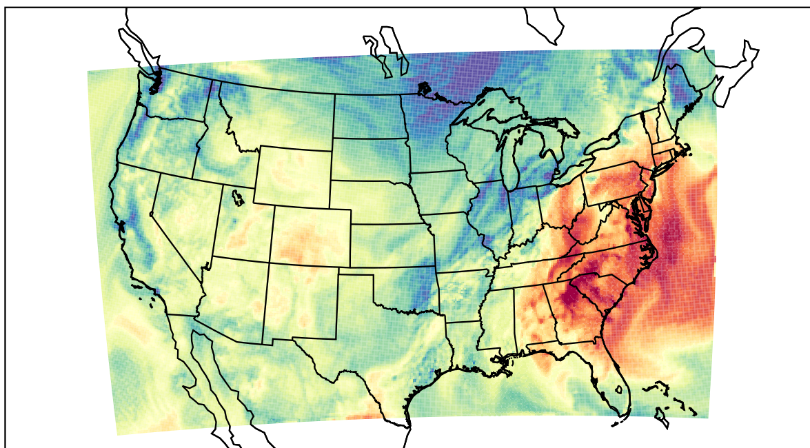
WRF (2021-10-15_17:00:00)
