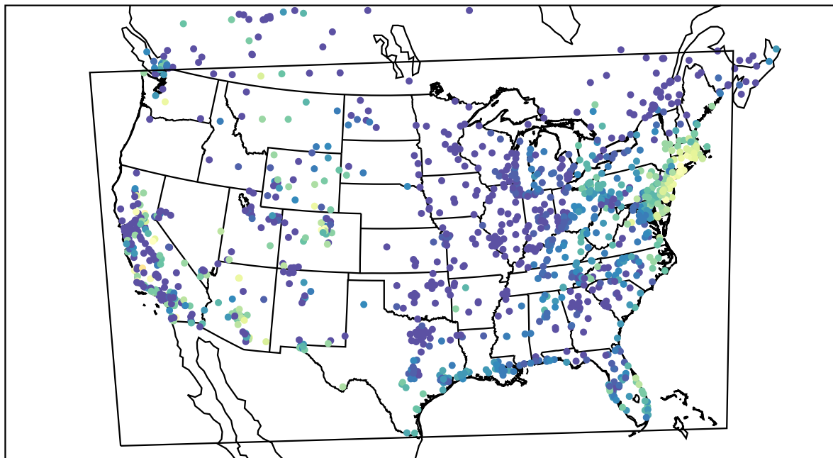
AirNOW (2021-10-16_13:00:00)
