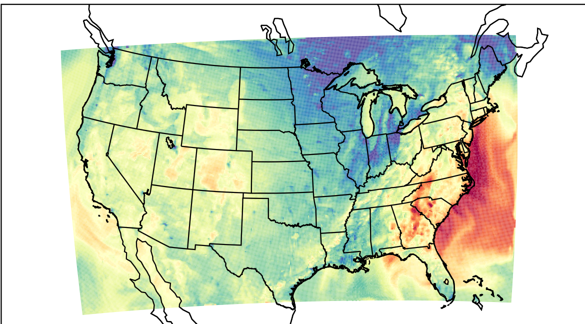
WRF (2021-10-16_01:00:00)
