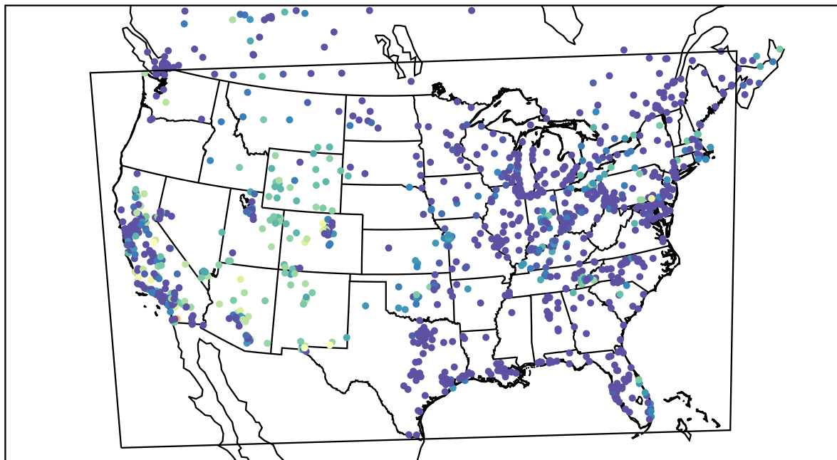
AirNOW (2021-10-15_07:00:00)
