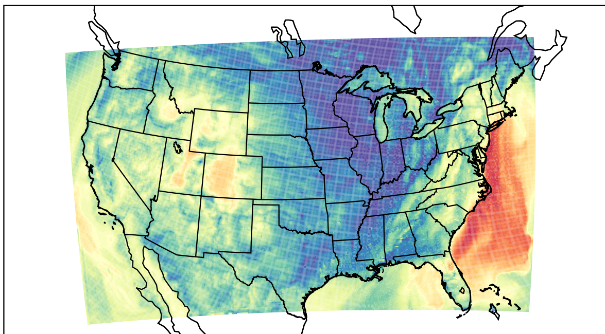
WRF (2021-10-16_11:00:00)
