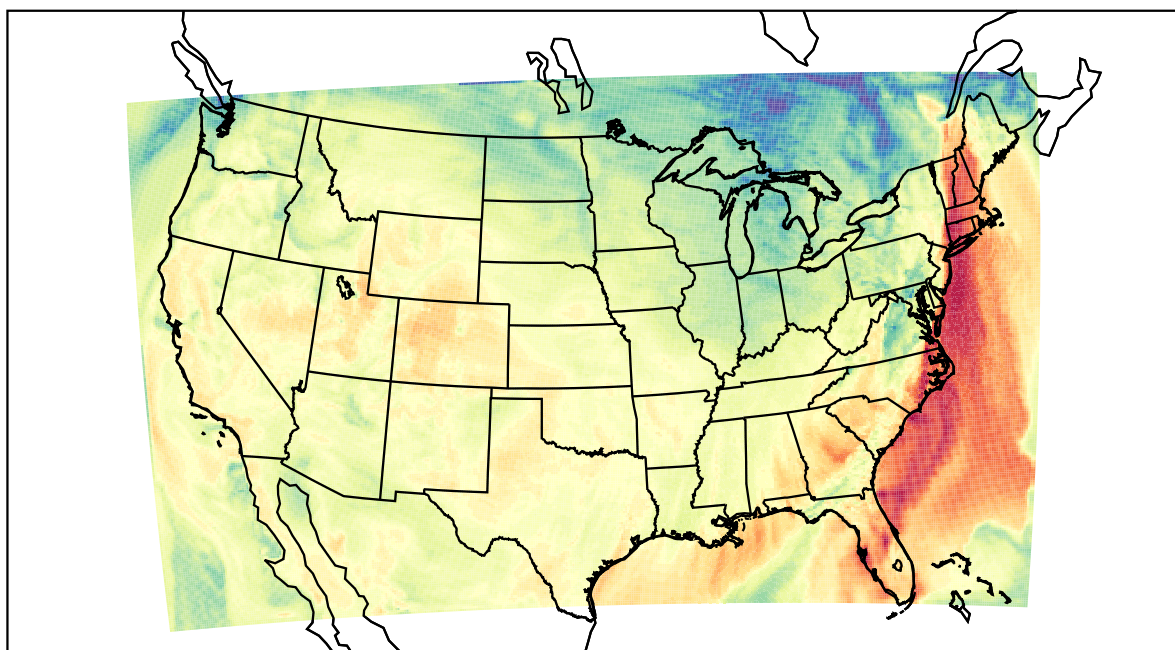
WRF (2021-10-16_20:00:00)
