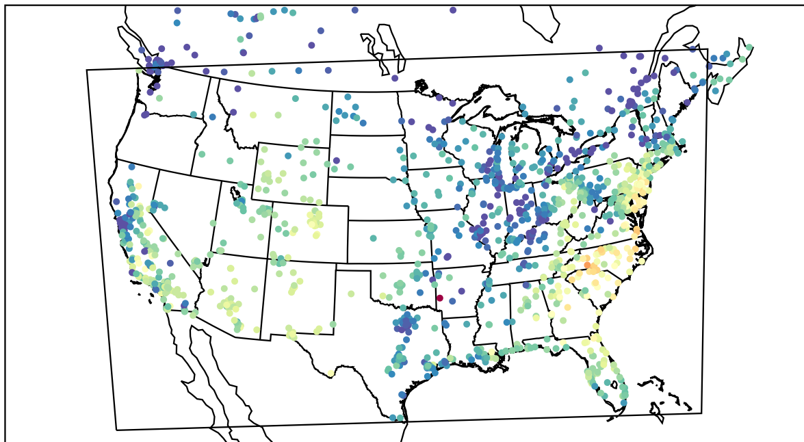
AirNOW (2021-10-15_17:00:00)
