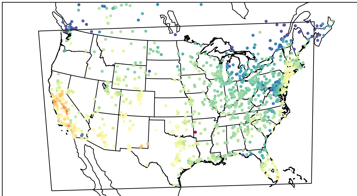
AirNOW (2021-10-16_20:00:00)
