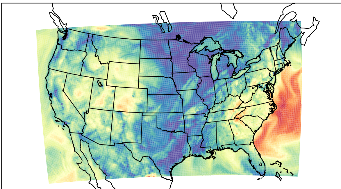
WRF (2021-10-15_14:00:00)
