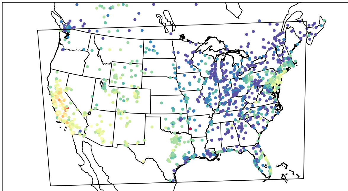
AirNOW (2021-10-16_00:00:00)
