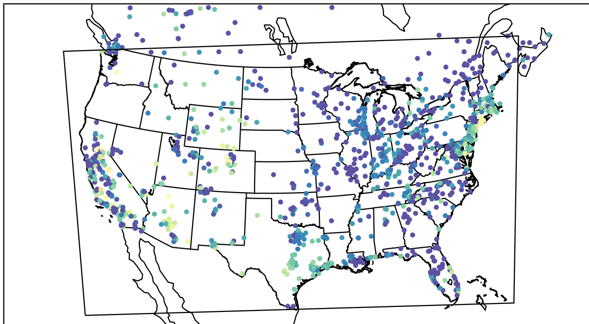
AirNOW (2021-10-16_06:00:00)
