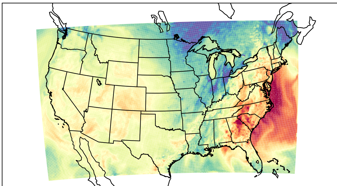
WRF (2021-10-15_23:00:00)
