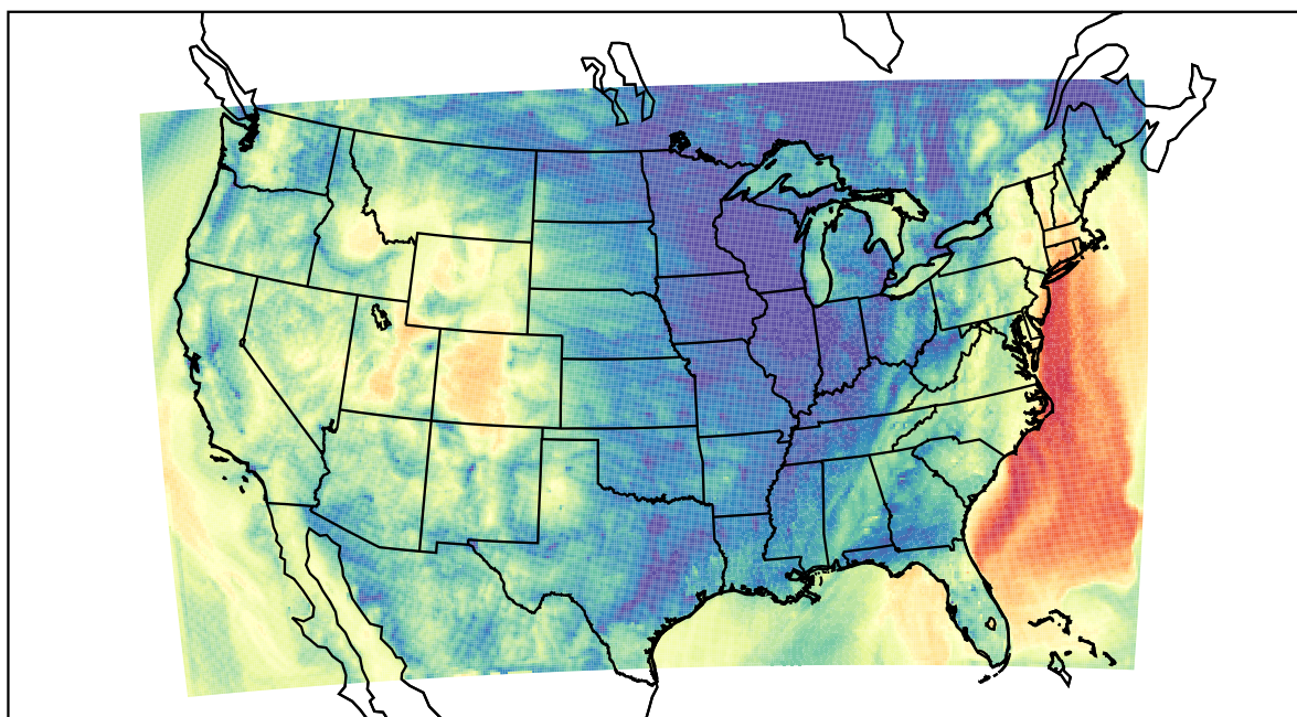
WRF (2021-10-16_13:00:00)
