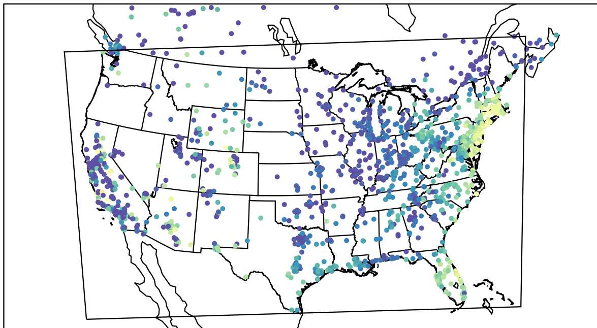
AirNOW (2021-10-16_14:00:00)
