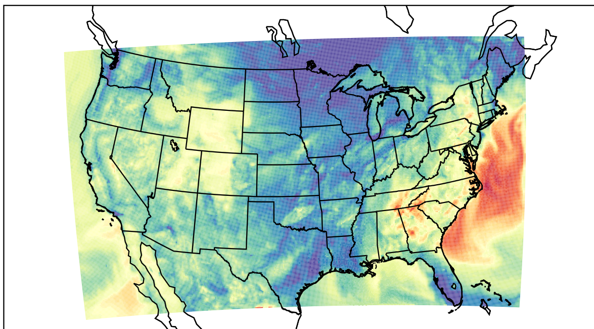
WRF (2021-10-15_07:00:00)
