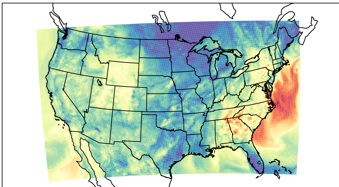
WRF (2021-10-15_05:00:00)
