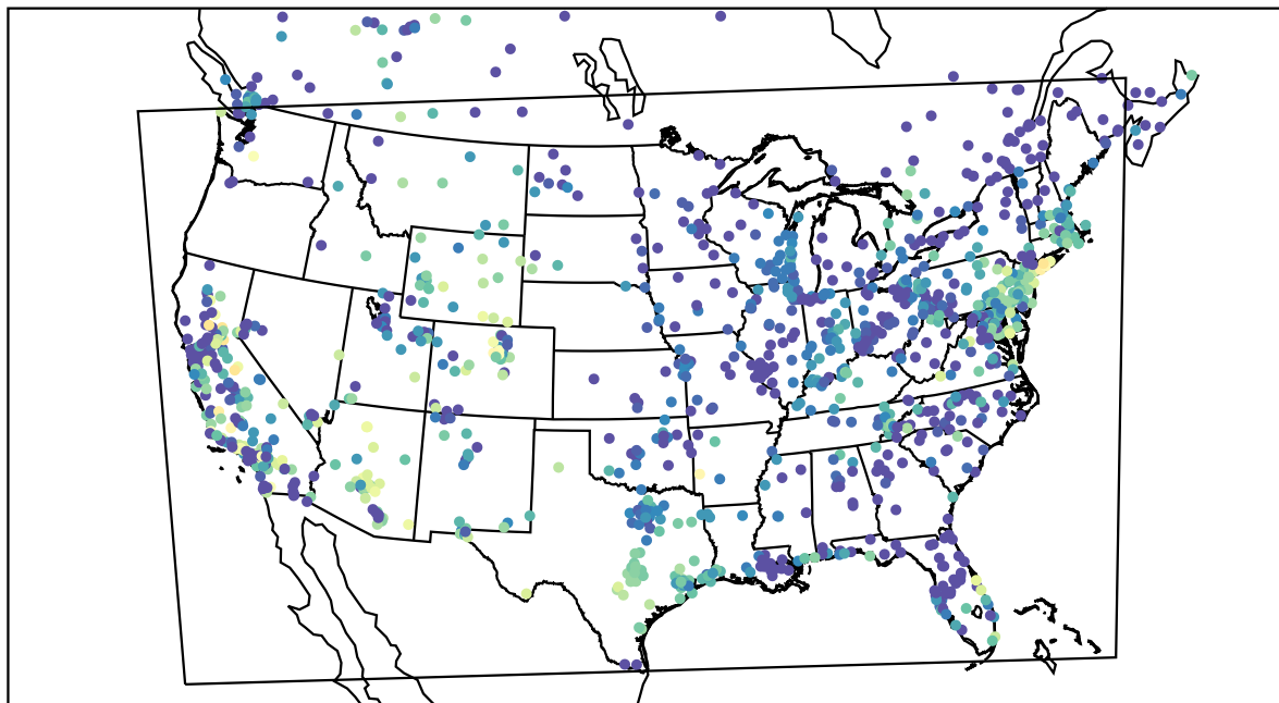
AirNOW (2021-10-16_05:00:00)
