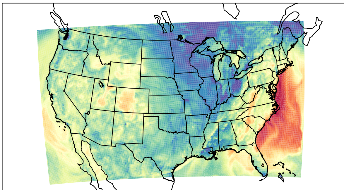
WRF (2021-10-16_05:00:00)
