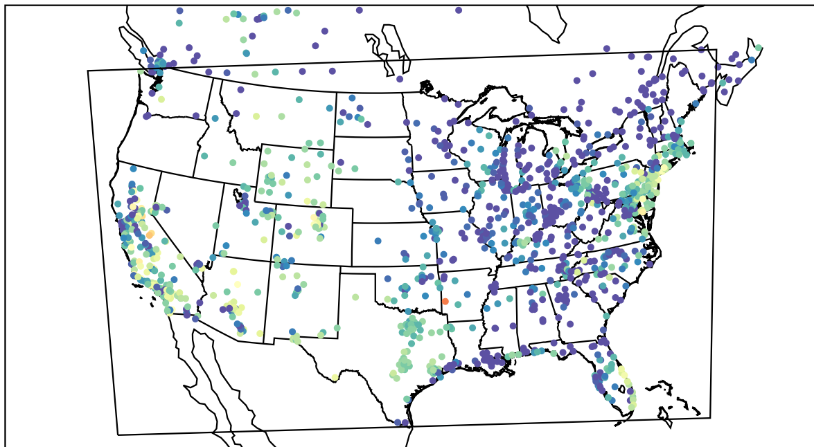
AirNOW (2021-10-16_02:00:00)
