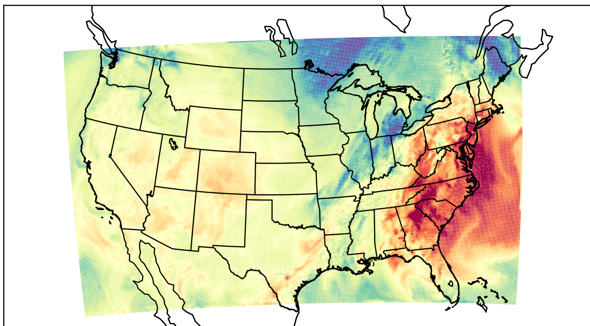
WRF (2021-10-15_21:00:00)
