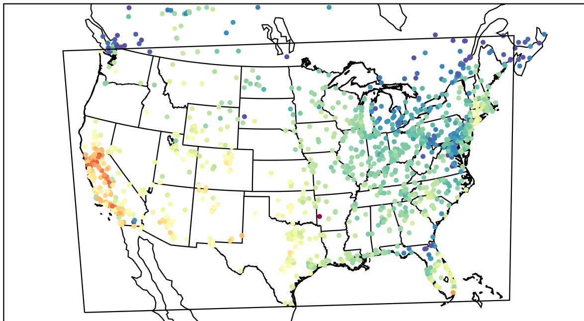
AirNOW (2021-10-16_22:00:00)
