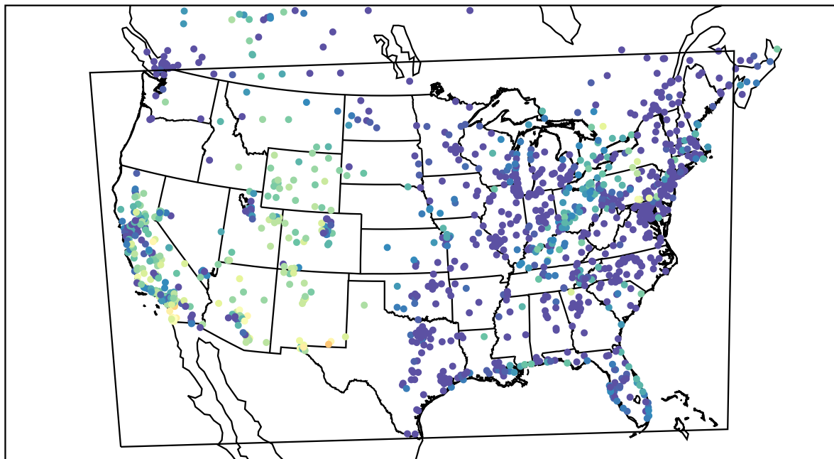
AirNOW (2021-10-15_02:00:00)
