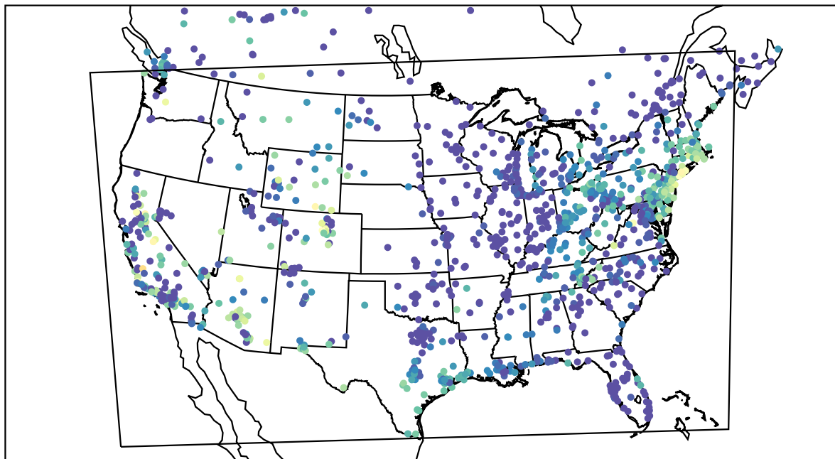
AirNOW (2021-10-16_11:00:00)
