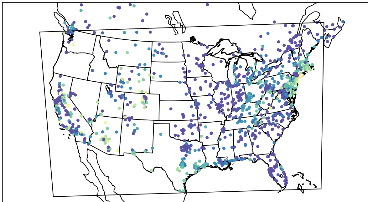
AirNOW (2021-10-16_10:00:00)
