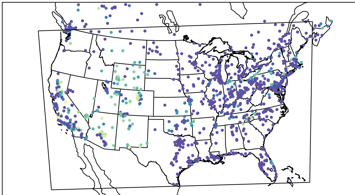
AirNOW (2021-10-15_11:00:00)
