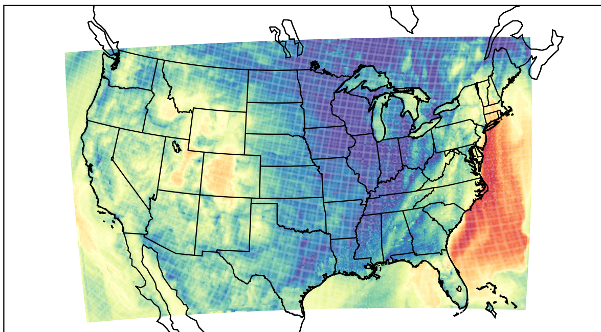
WRF (2021-10-16_12:00:00)
