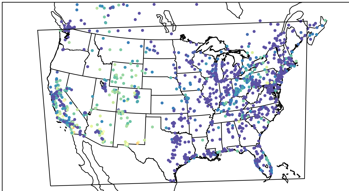
AirNOW (2021-10-15_03:00:00)
