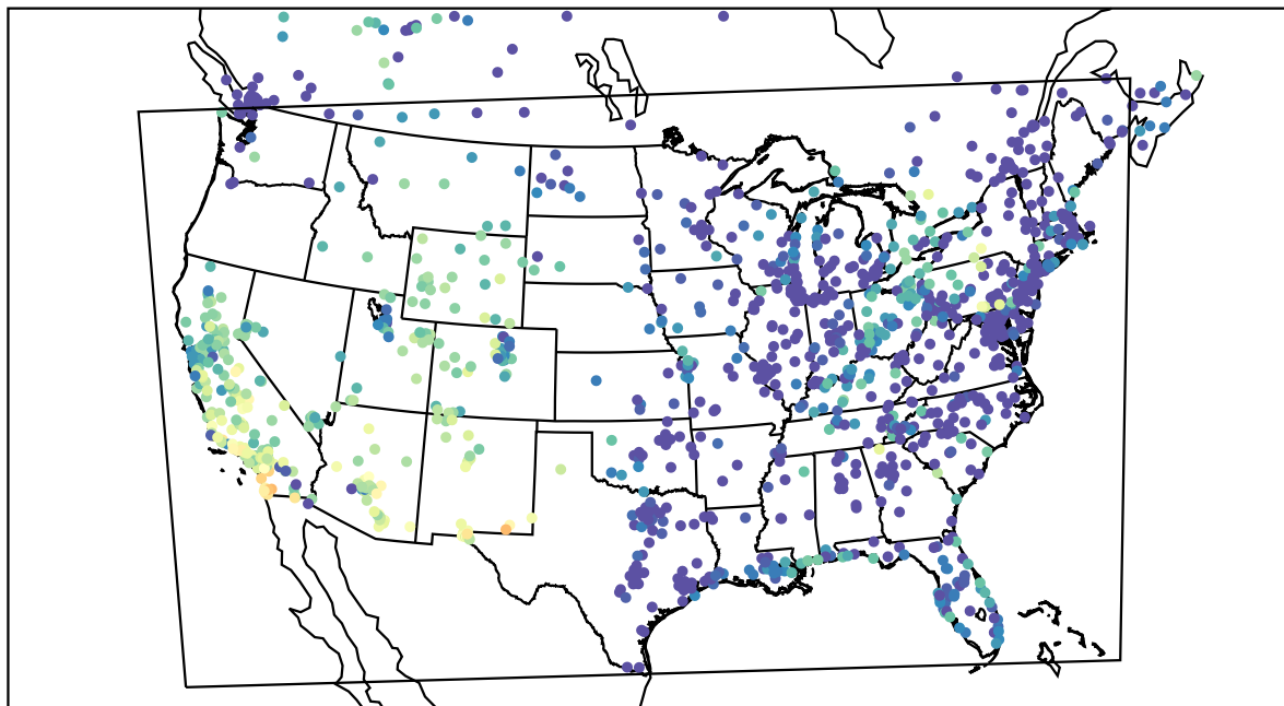
AirNOW (2021-10-15_01:00:00)
