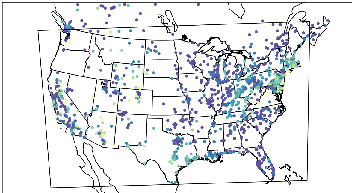
AirNOW (2021-10-16_09:00:00)
