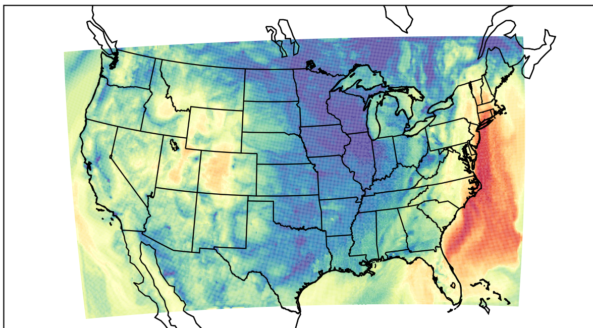
WRF (2021-10-16_14:00:00)
