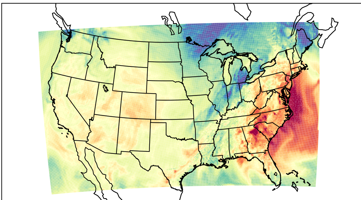
WRF (2021-10-15_22:00:00)
