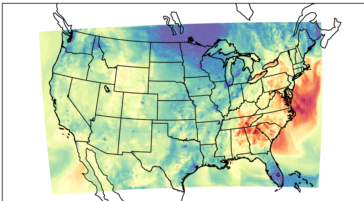
WRF (2021-10-15_01:00:00)
