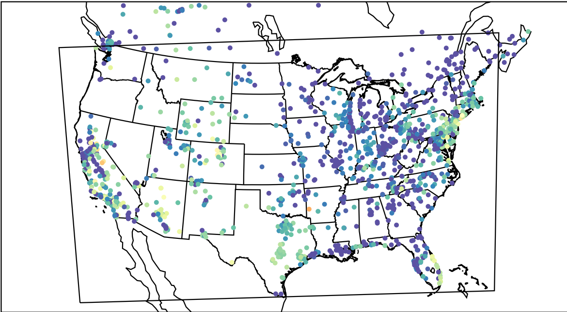
AirNOW (2021-10-16_03:00:00)
