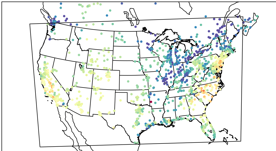
AirNOW (2021-10-15_20:00:00)
