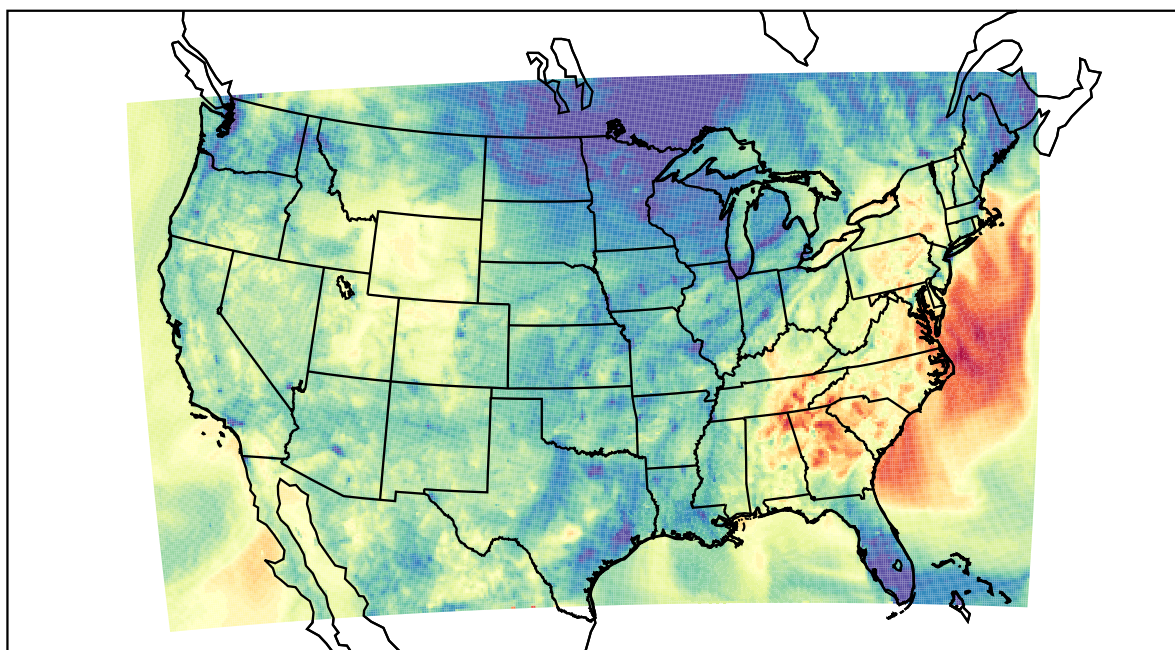
WRF (2021-10-15_03:00:00)
