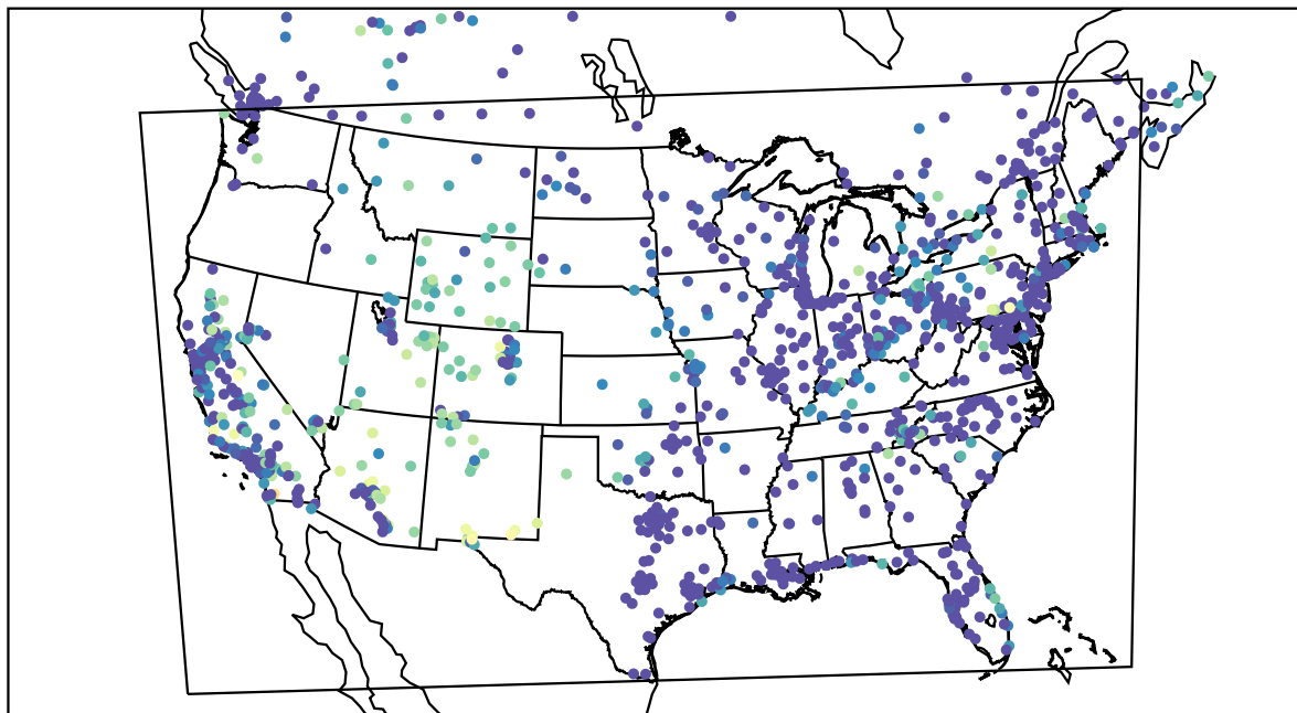
AirNOW (2021-10-15_05:00:00)
