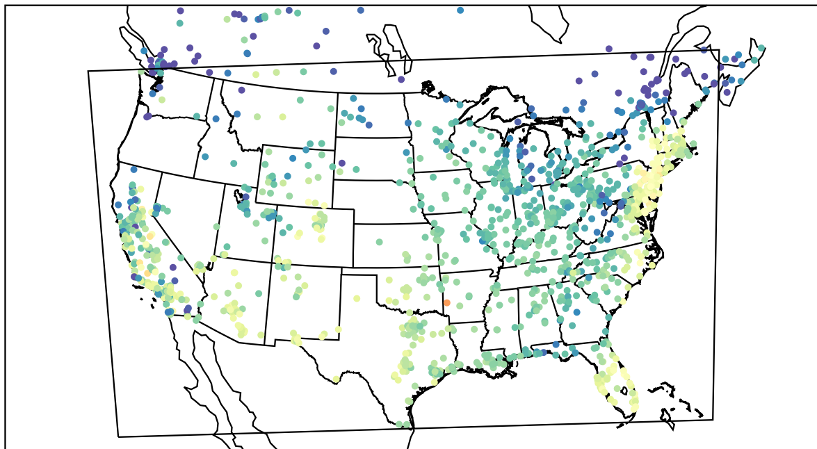
AirNOW (2021-10-16_17:00:00)
