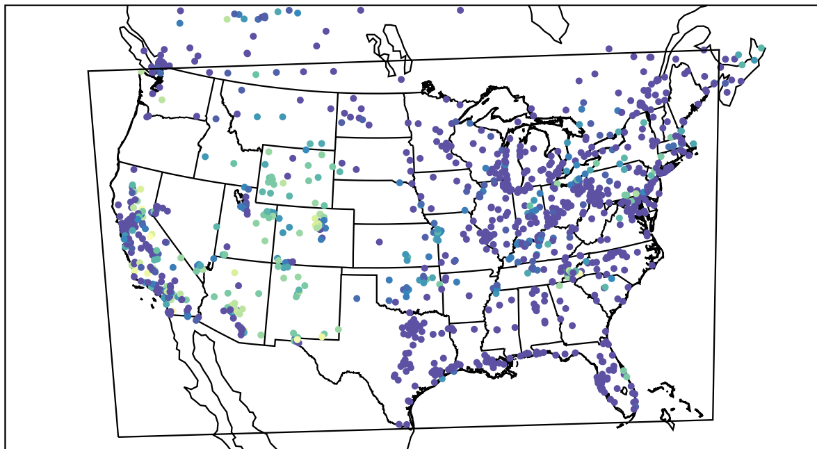
AirNOW (2021-10-15_09:00:00)
