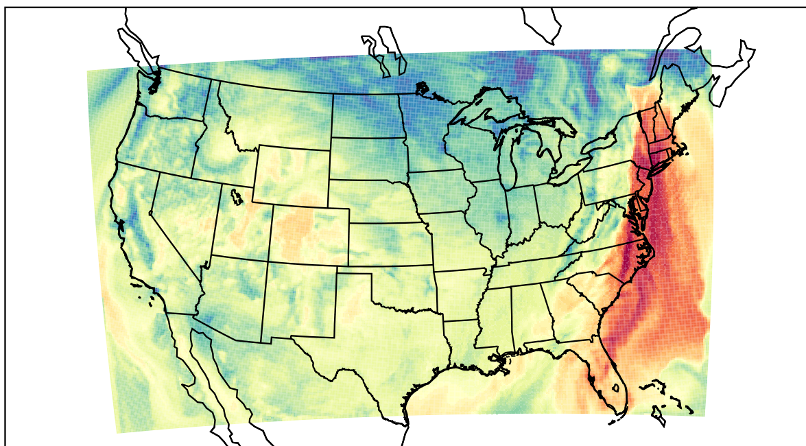
WRF (2021-10-16_17:00:00)
