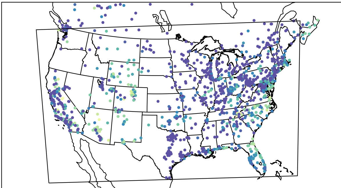
AirNOW (2021-10-15_14:00:00)
