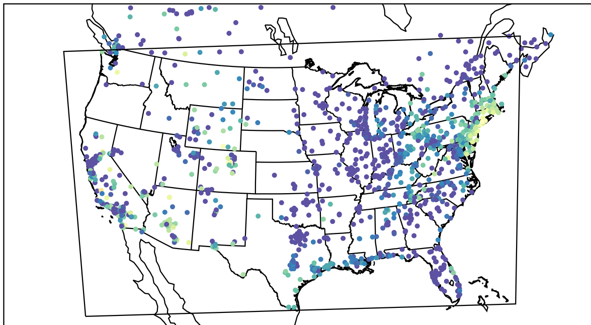
AirNOW (2021-10-16_12:00:00)
