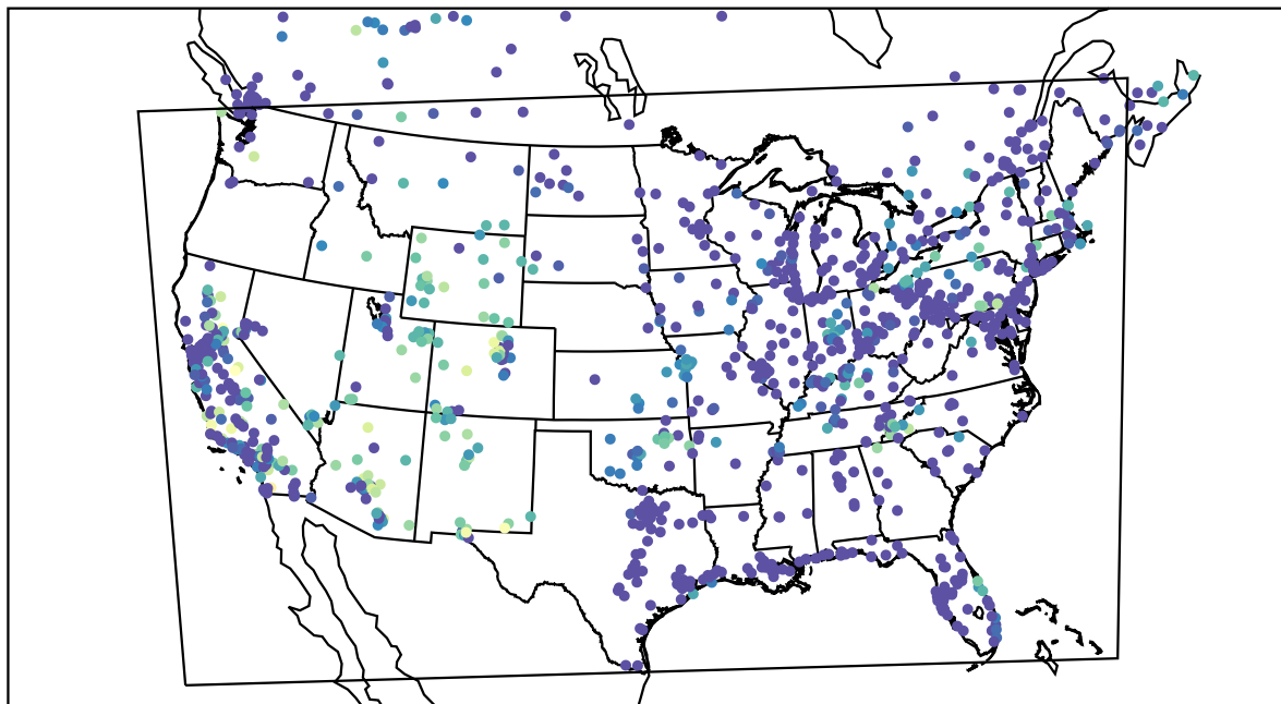
AirNOW (2021-10-15_08:00:00)
