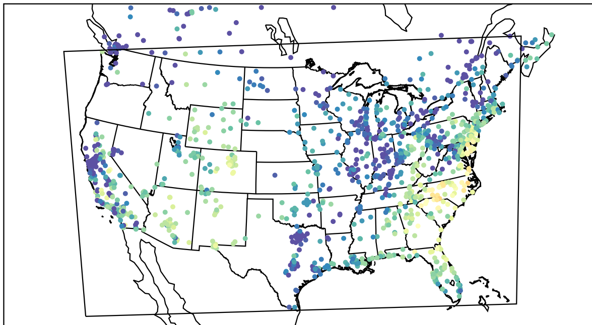
AirNOW (2021-10-15_16:00:00)
