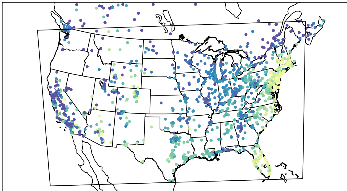
AirNOW (2021-10-16_15:00:00)
