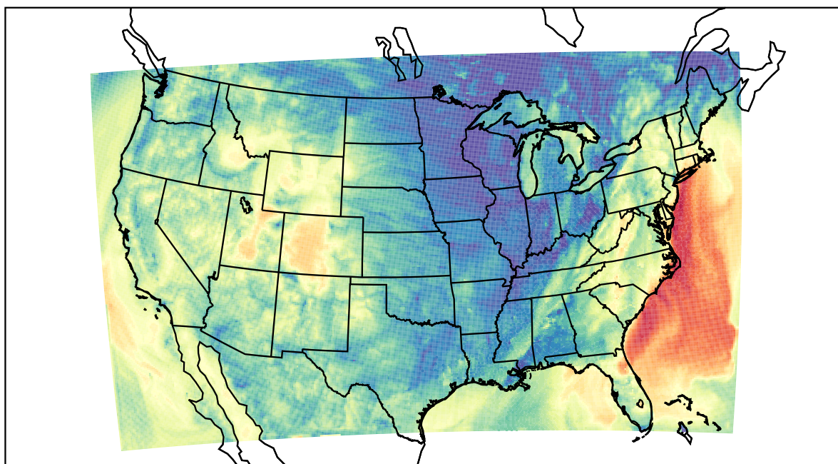
WRF (2021-10-16_09:00:00)
