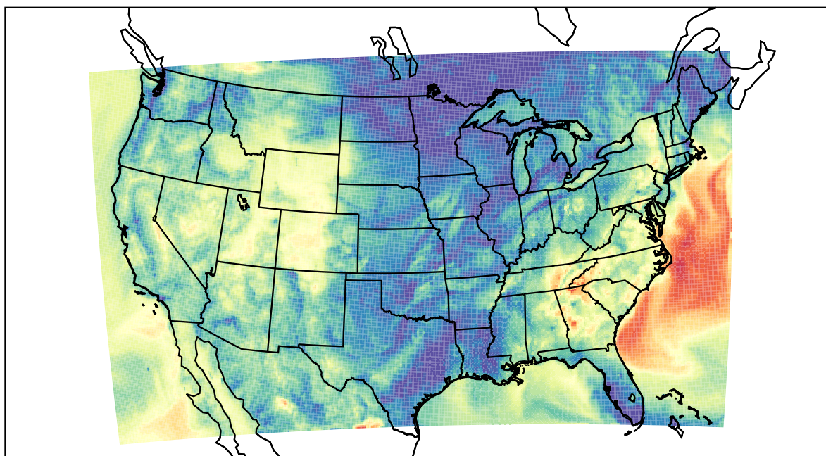
WRF (2021-10-15_10:00:00)
