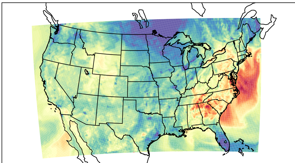
WRF (2021-10-15_02:00:00)
