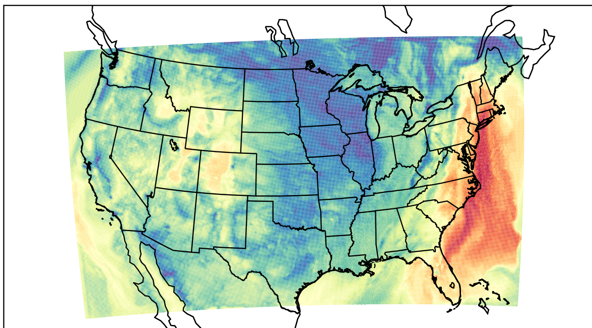
WRF (2021-10-16_15:00:00)
