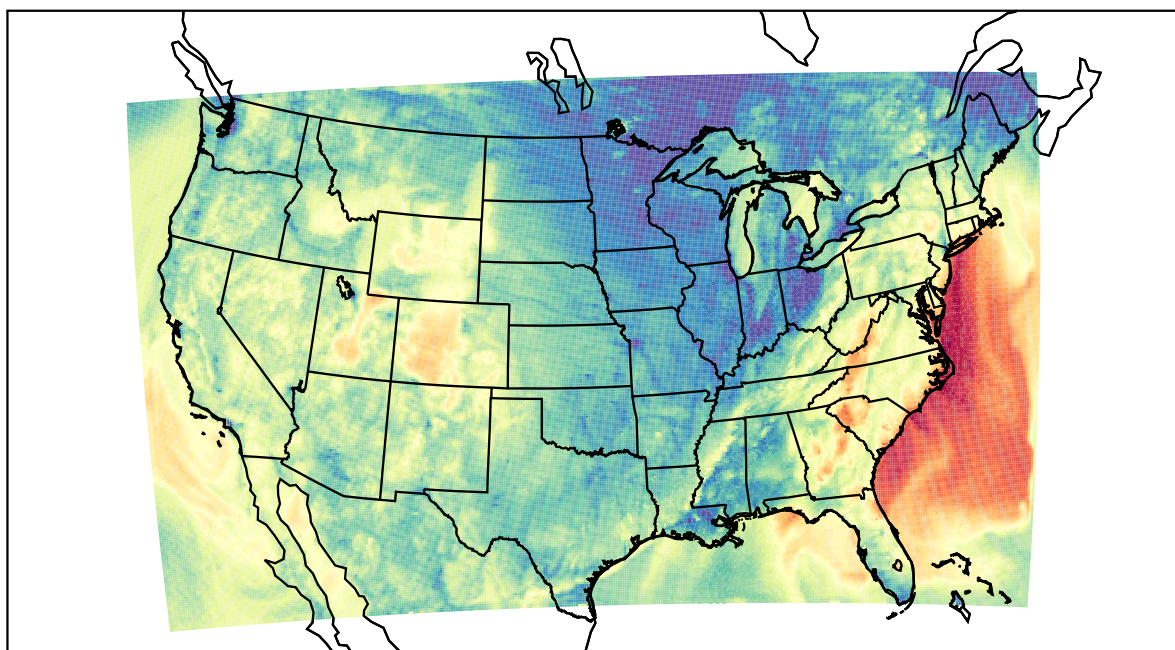
WRF (2021-10-16_04:00:00)
