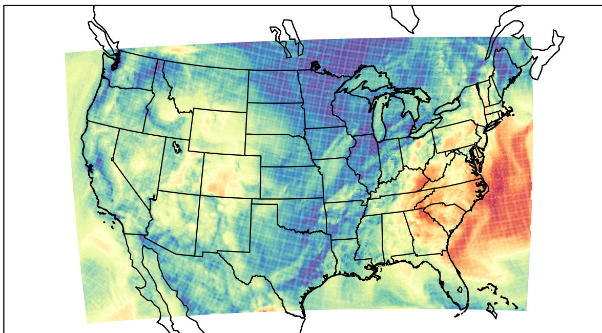
WRF (2021-10-15_15:00:00)
