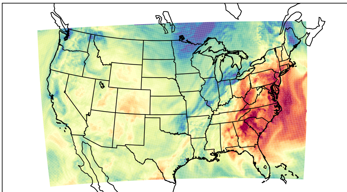
WRF (2021-10-15_18:00:00)
