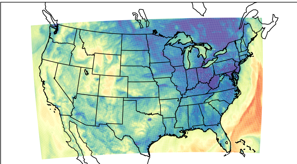
WRF (2021-10-17_09:00:00)
