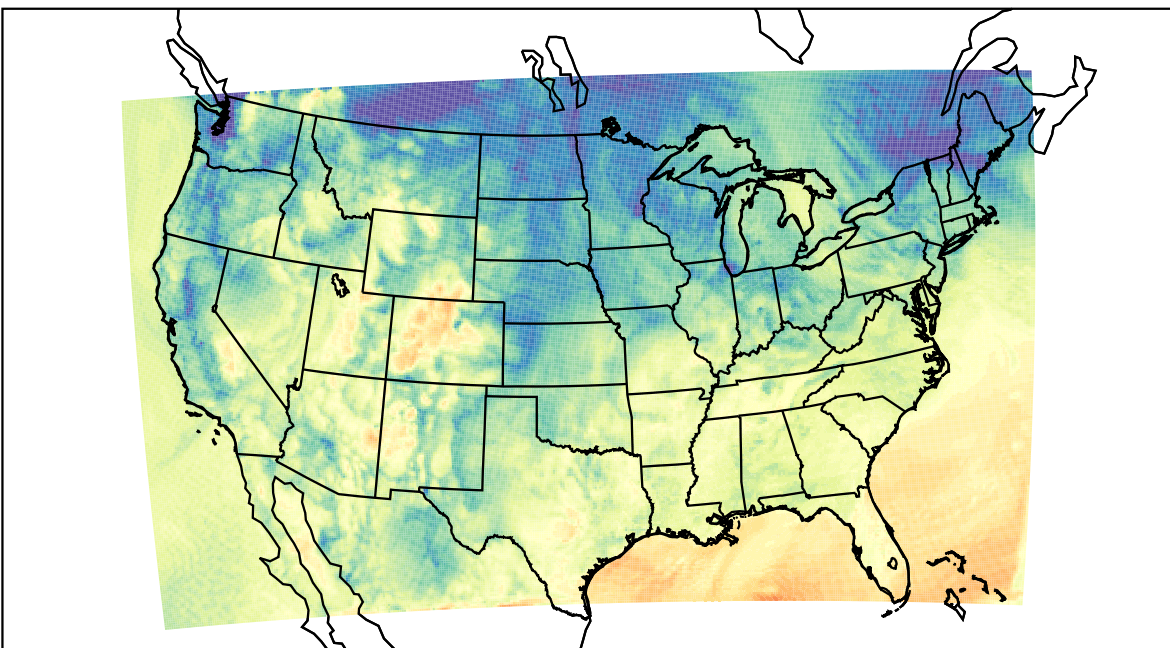
WRF (2021-10-18_16:00:00)
