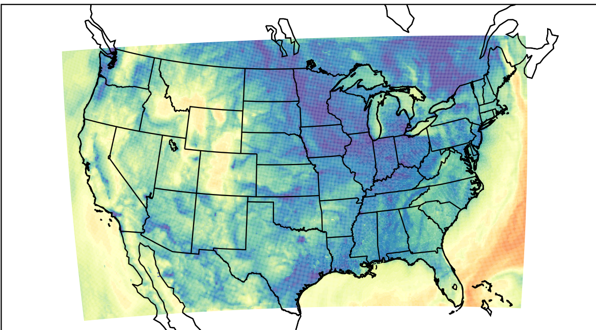
WRF (2021-10-17_14:00:00)
