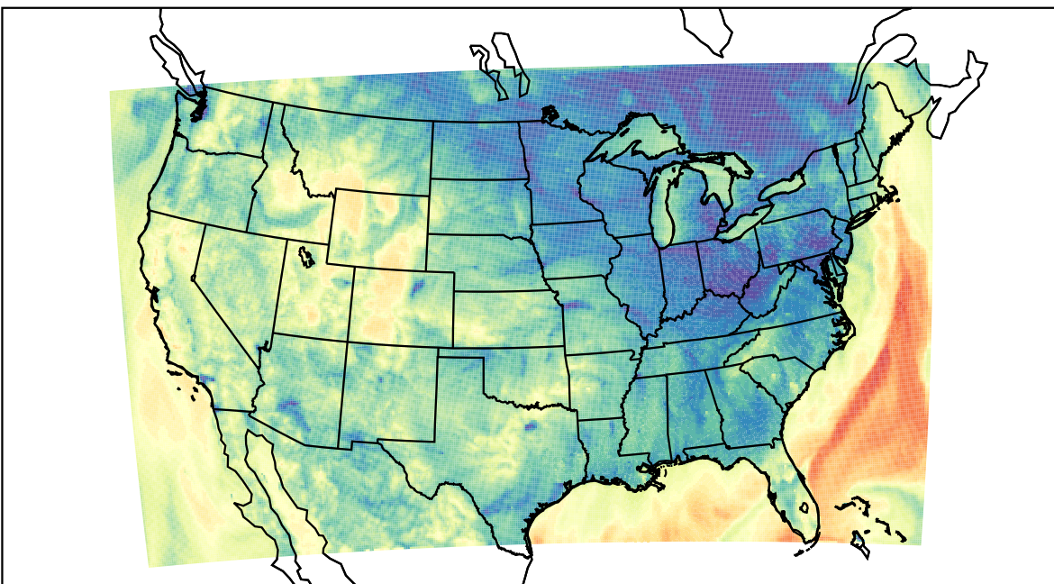
WRF (2021-10-17_06:00:00)
