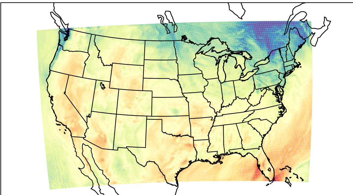
WRF (2021-10-17_21:00:00)
