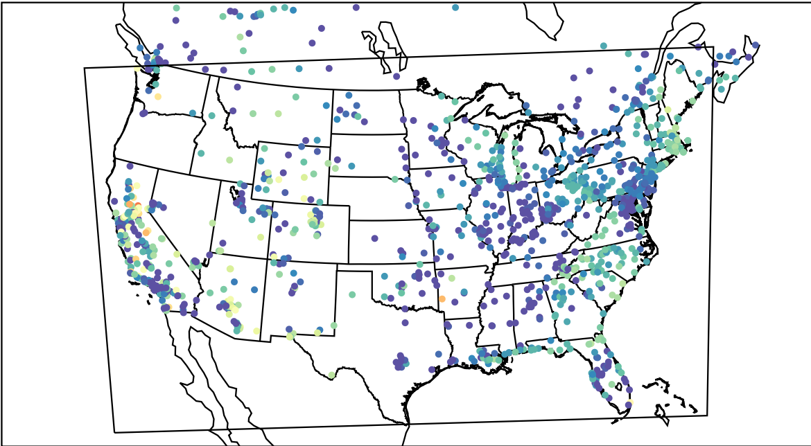
AirNOW (2021-10-17_05:00:00)
