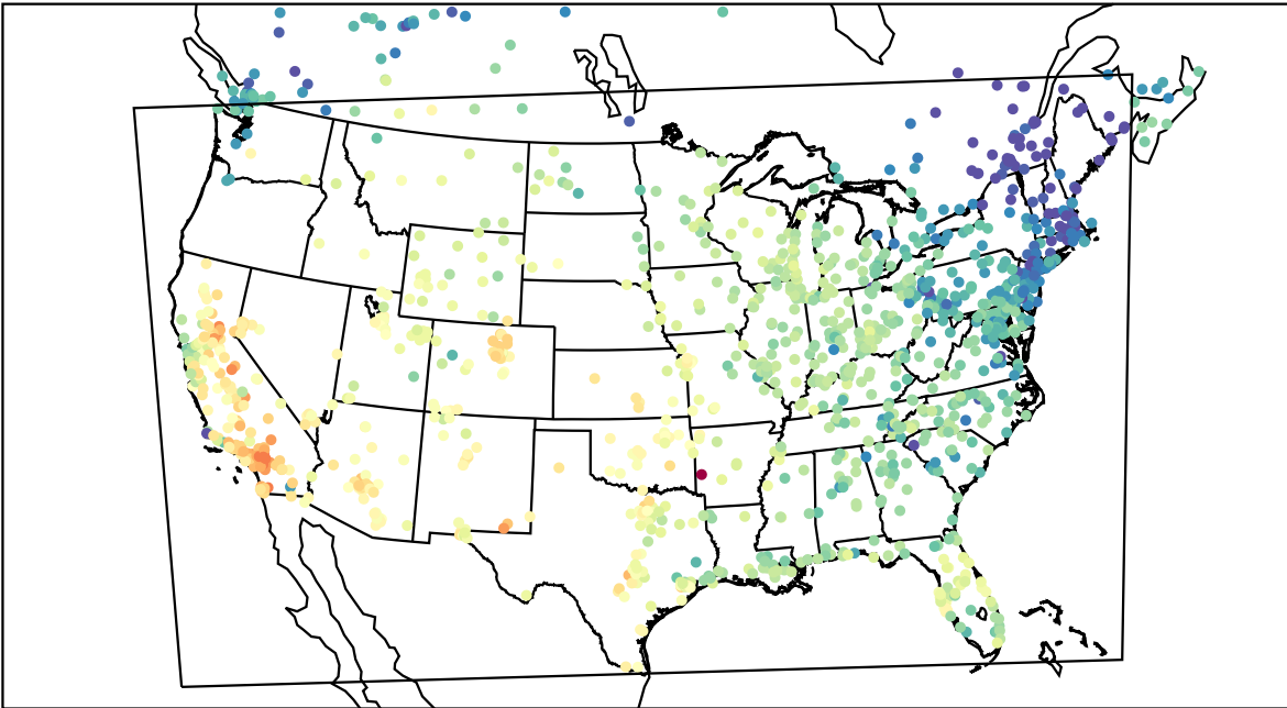
AirNOW (2021-10-17_22:00:00)
