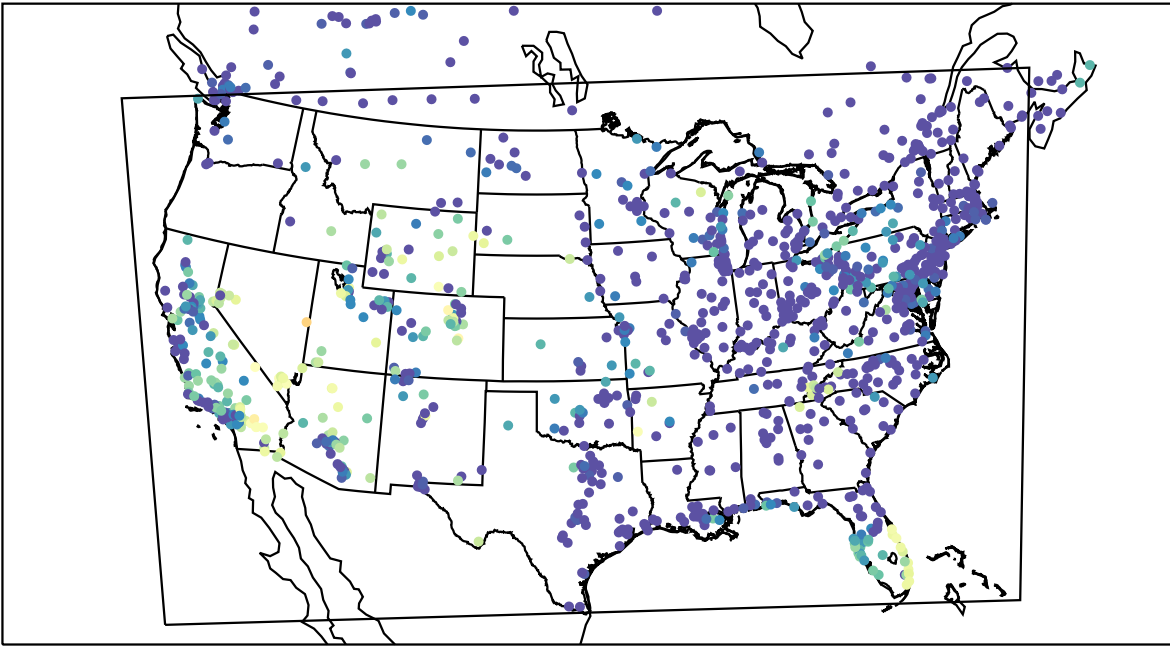
AirNOW (2021-10-18_11:00:00)
