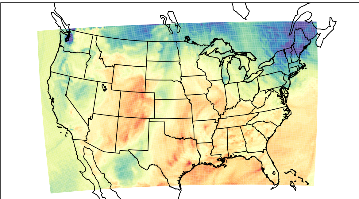
WRF (2021-10-18_21:00:00)
