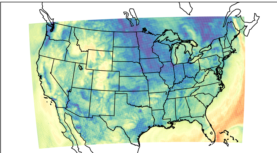
WRF (2021-10-17_15:00:00)
