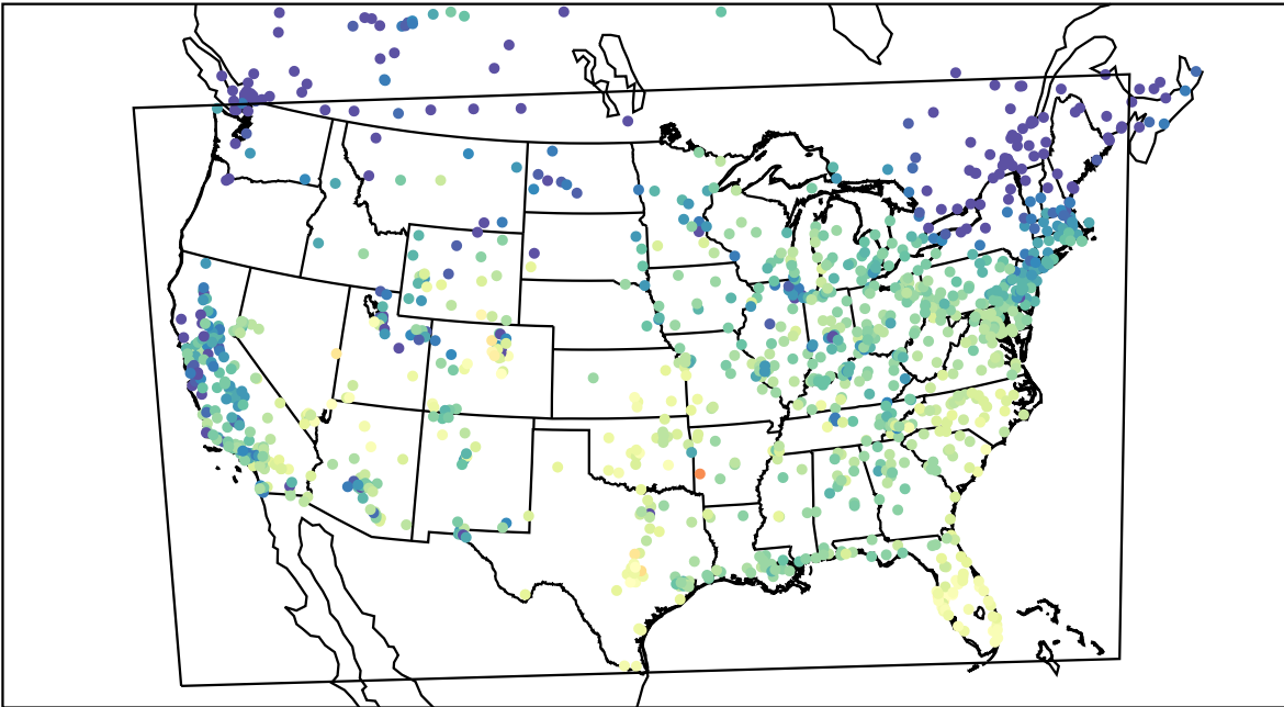
AirNOW (2021-10-18_16:00:00)
