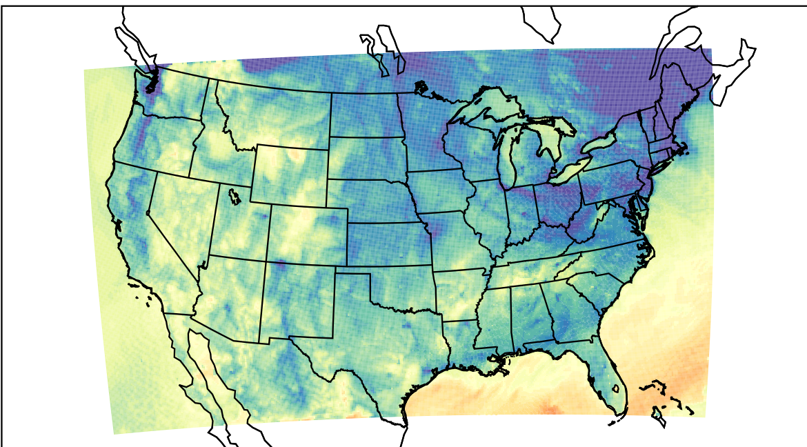
WRF (2021-10-18_10:00:00)
