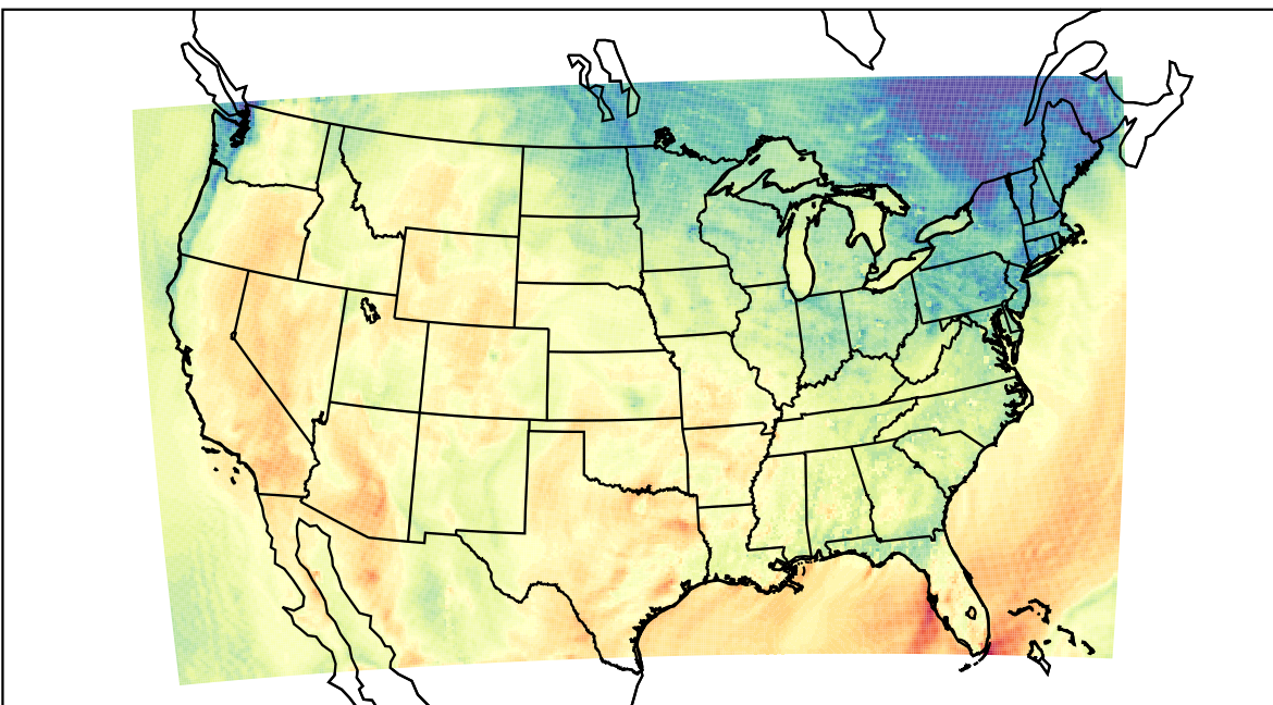
WRF (2021-10-17_22:00:00)
