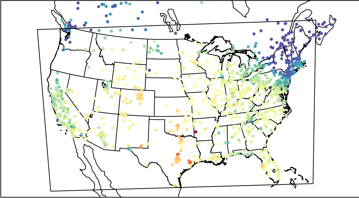
AirNOW (2021-10-18_21:00:00)
