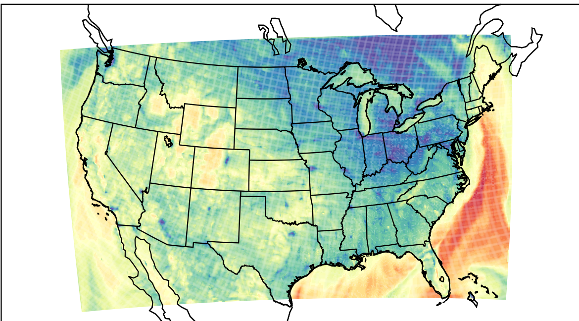
WRF (2021-10-17_03:00:00)
