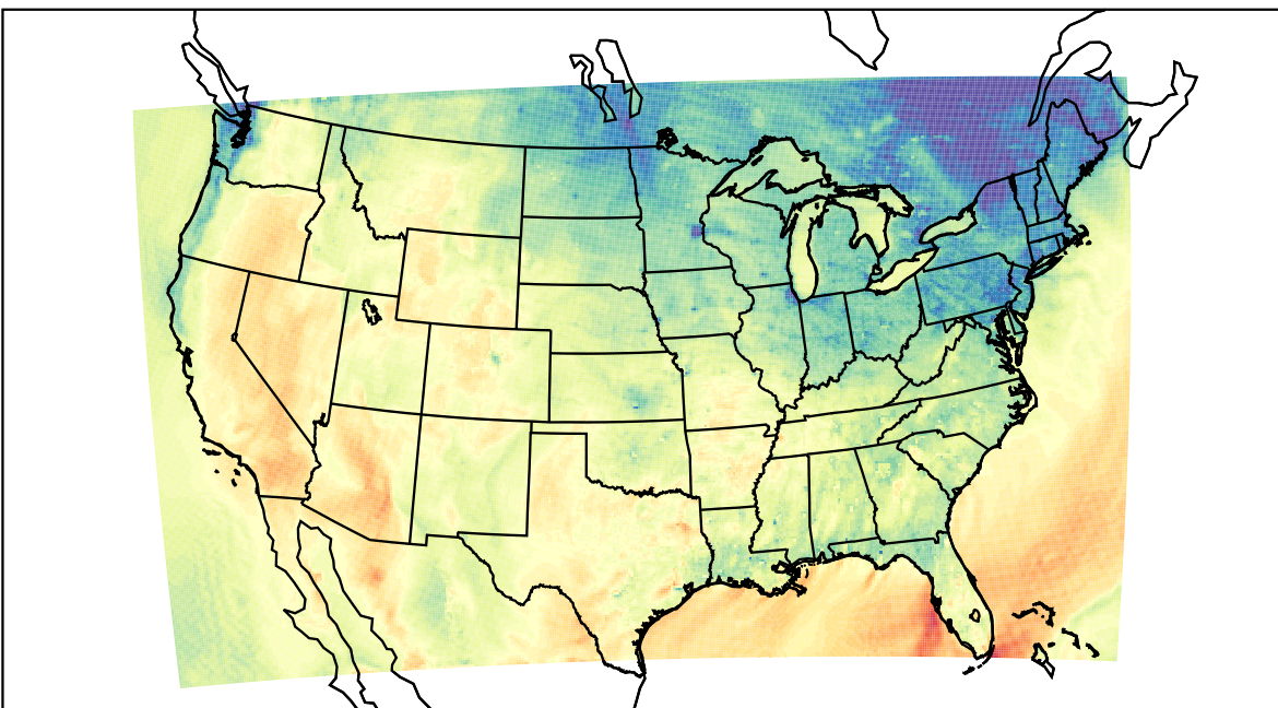
WRF (2021-10-17_23:00:00)
