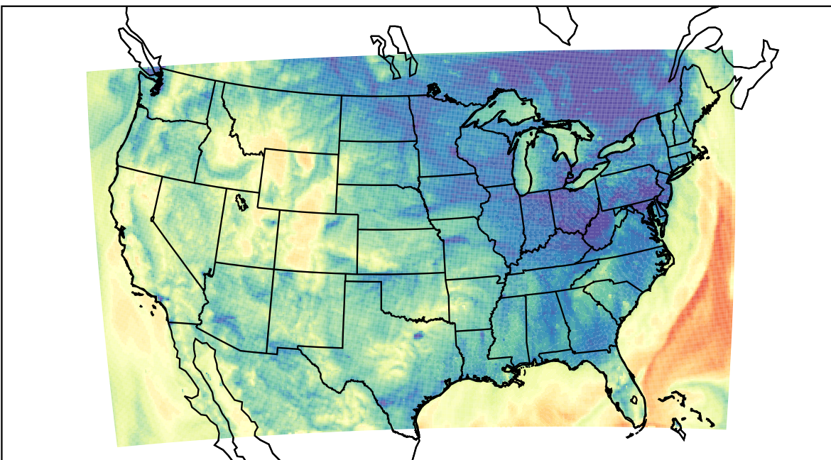
WRF (2021-10-17_08:00:00)
