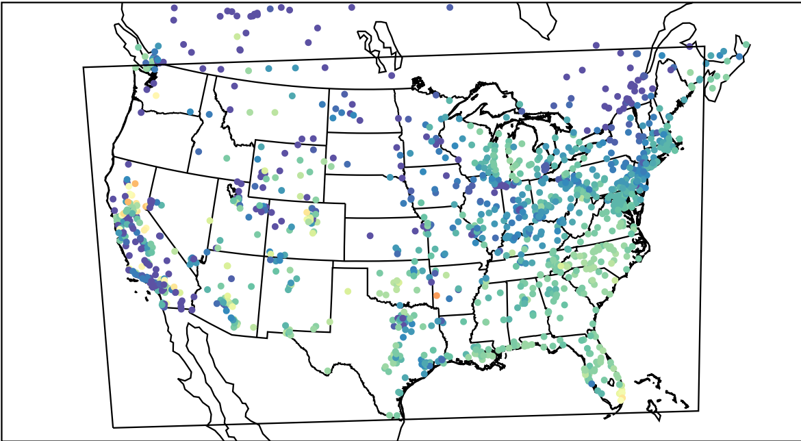
AirNOW (2021-10-17_15:00:00)
