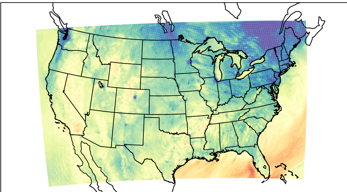
WRF (2021-10-18_01:00:00)
