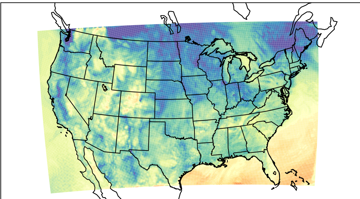
WRF (2021-10-18_15:00:00)
