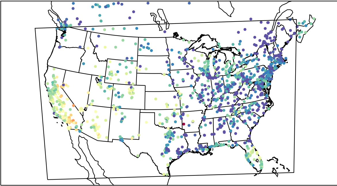
AirNOW (2021-10-18_01:00:00)
