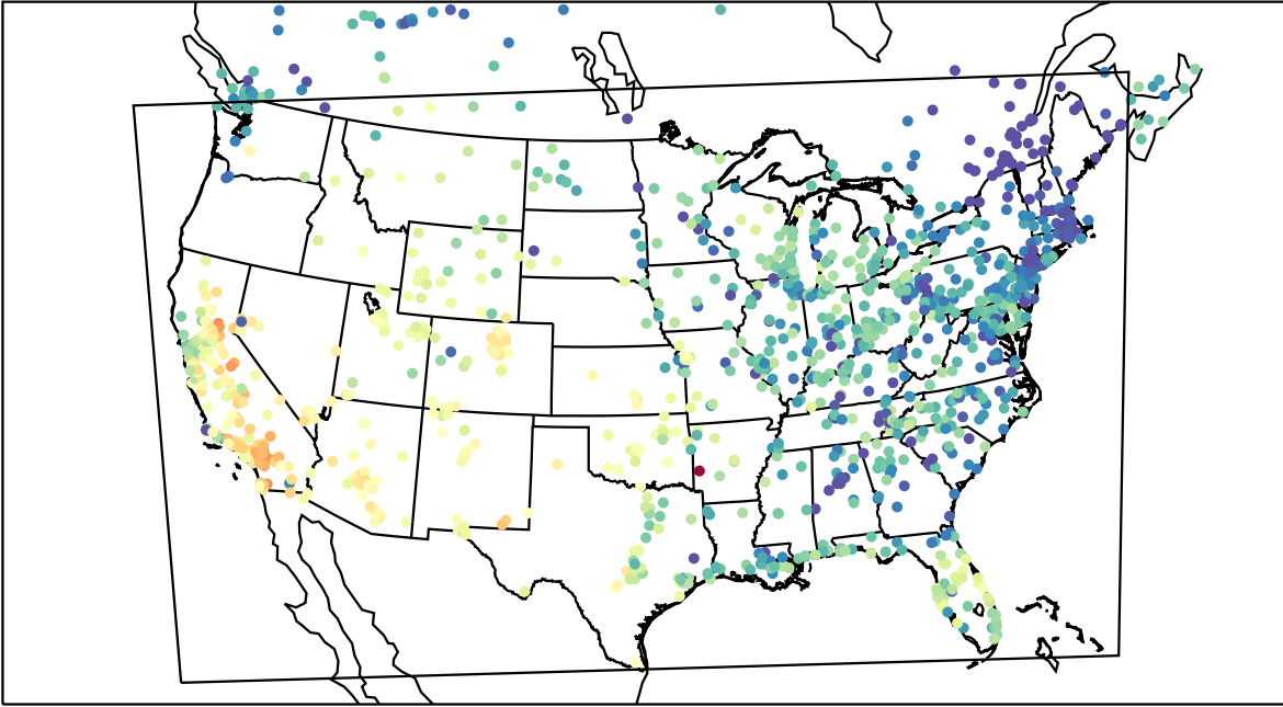
AirNOW (2021-10-17_23:00:00)
