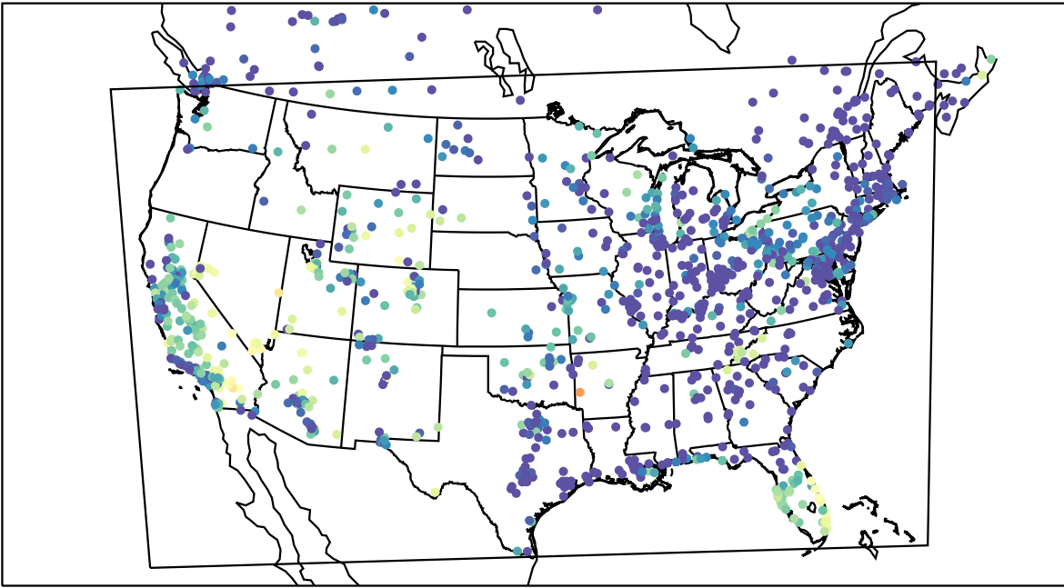
AirNOW (2021-10-18_08:00:00)
