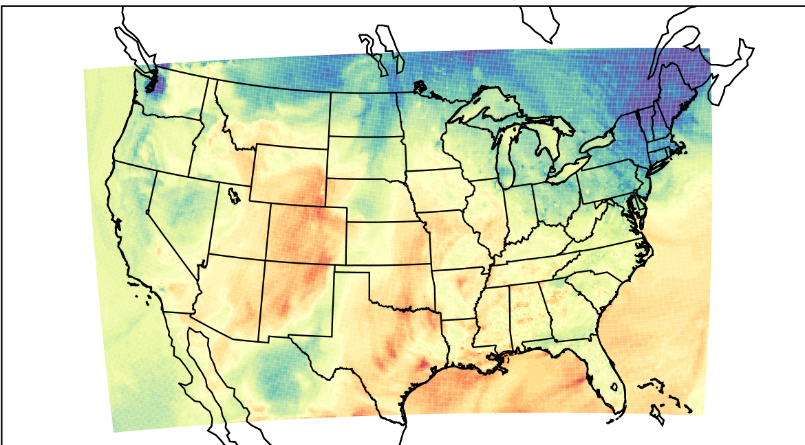
WRF (2021-10-18_22:00:00)
