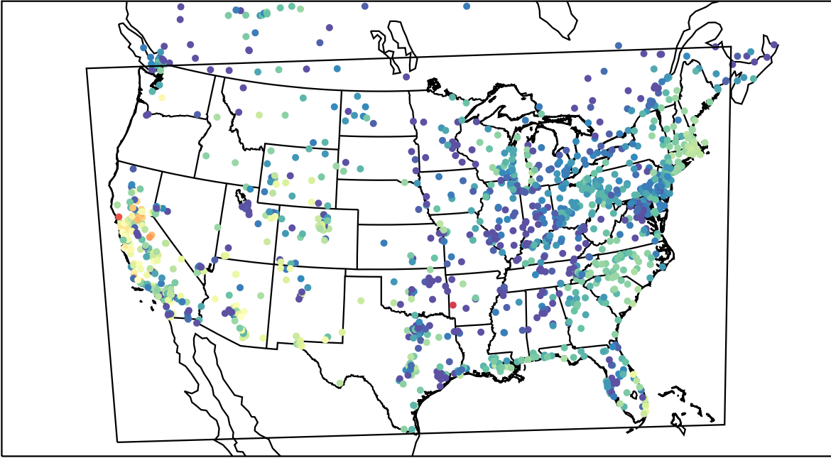
AirNOW (2021-10-17_02:00:00)
