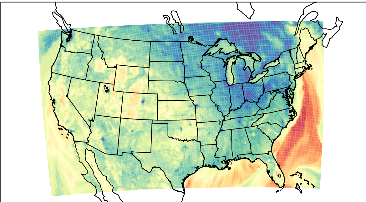
WRF (2021-10-17_02:00:00)
