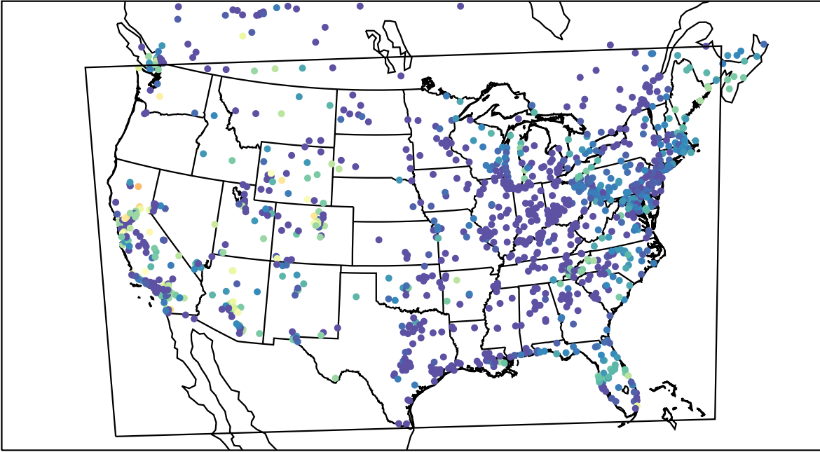
AirNOW (2021-10-17_12:00:00)
