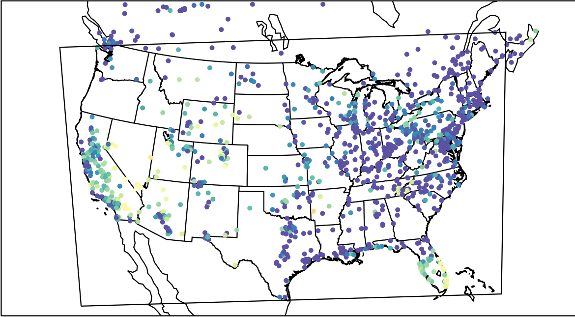
AirNOW (2021-10-18_09:00:00)
