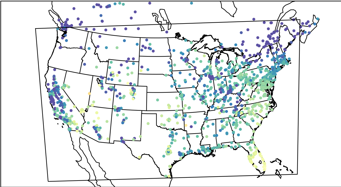
AirNOW (2021-10-18_15:00:00)
