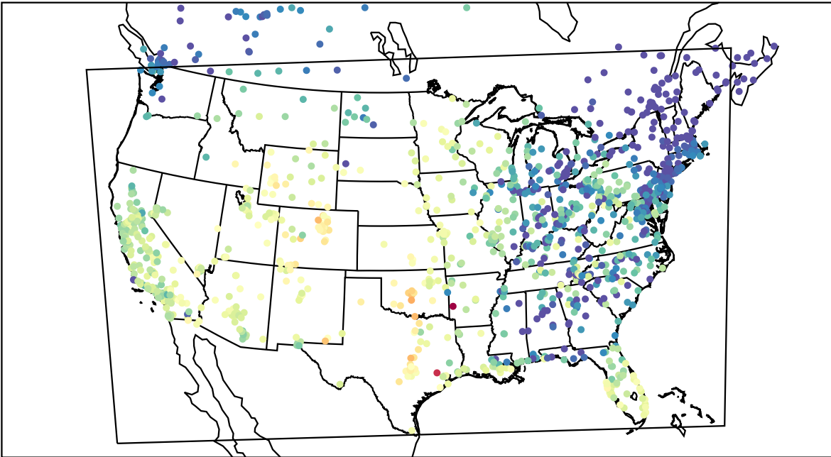
AirNOW (2021-10-18_23:00:00)
