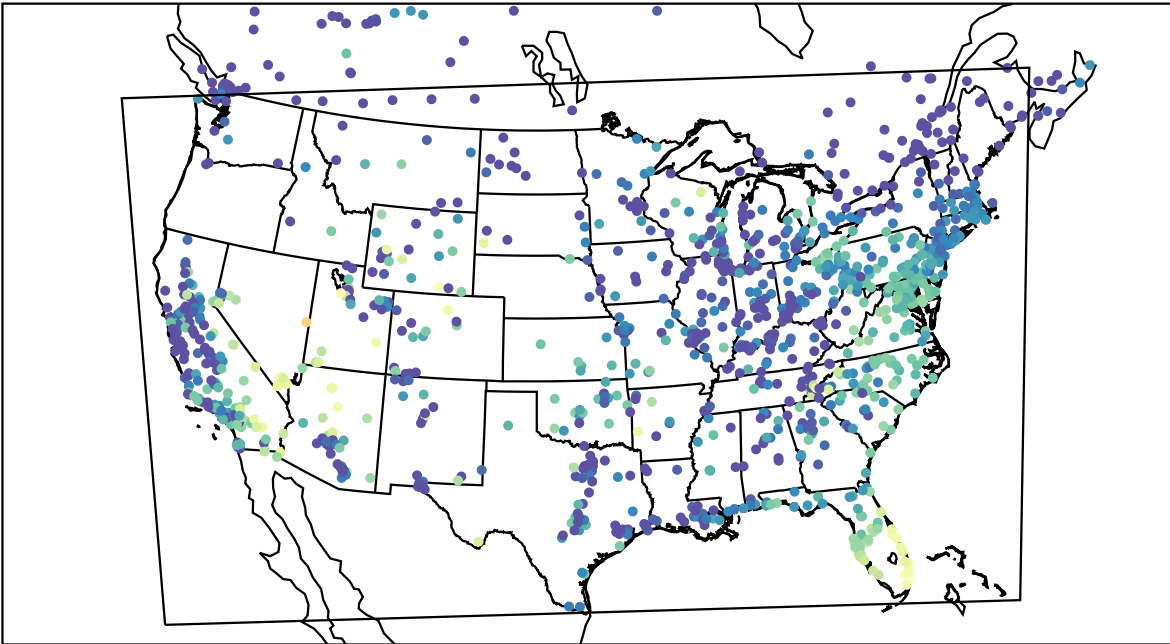
AirNOW (2021-10-18_14:00:00)
