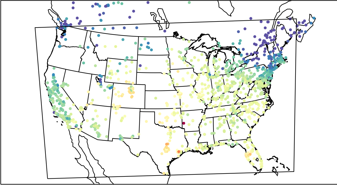
AirNOW (2021-10-18_18:00:00)
