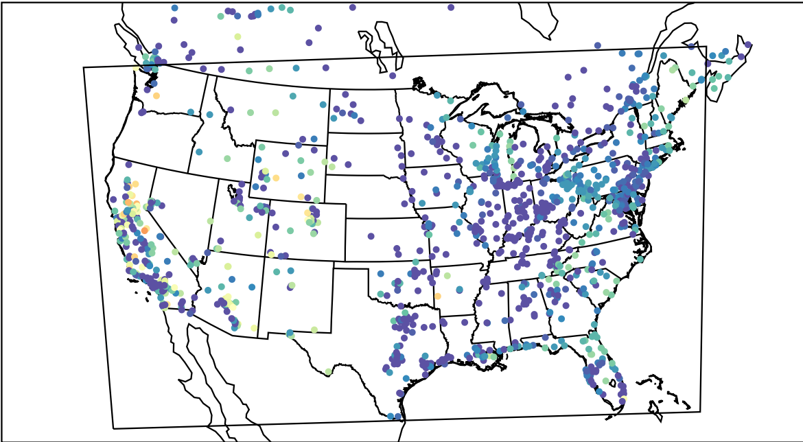
AirNOW (2021-10-17_08:00:00)
