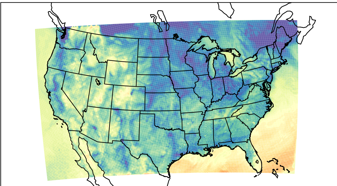
WRF (2021-10-18_14:00:00)
