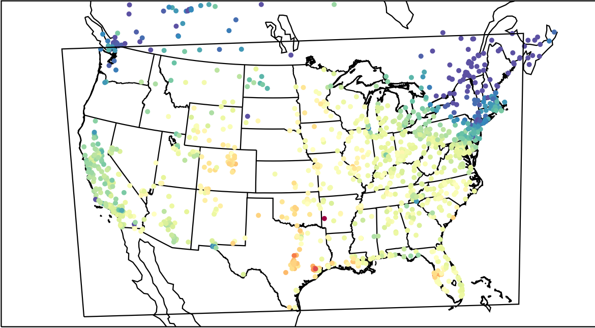
AirNOW (2021-10-18_20:00:00)
