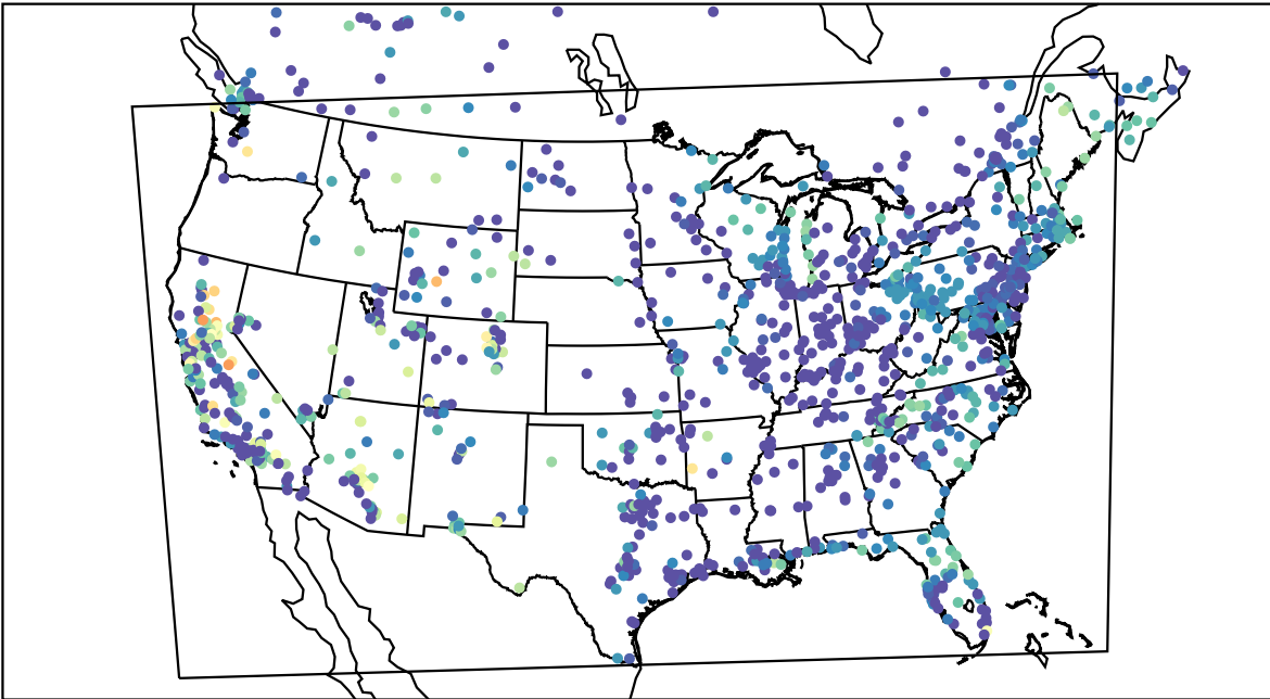
AirNOW (2021-10-17_09:00:00)
