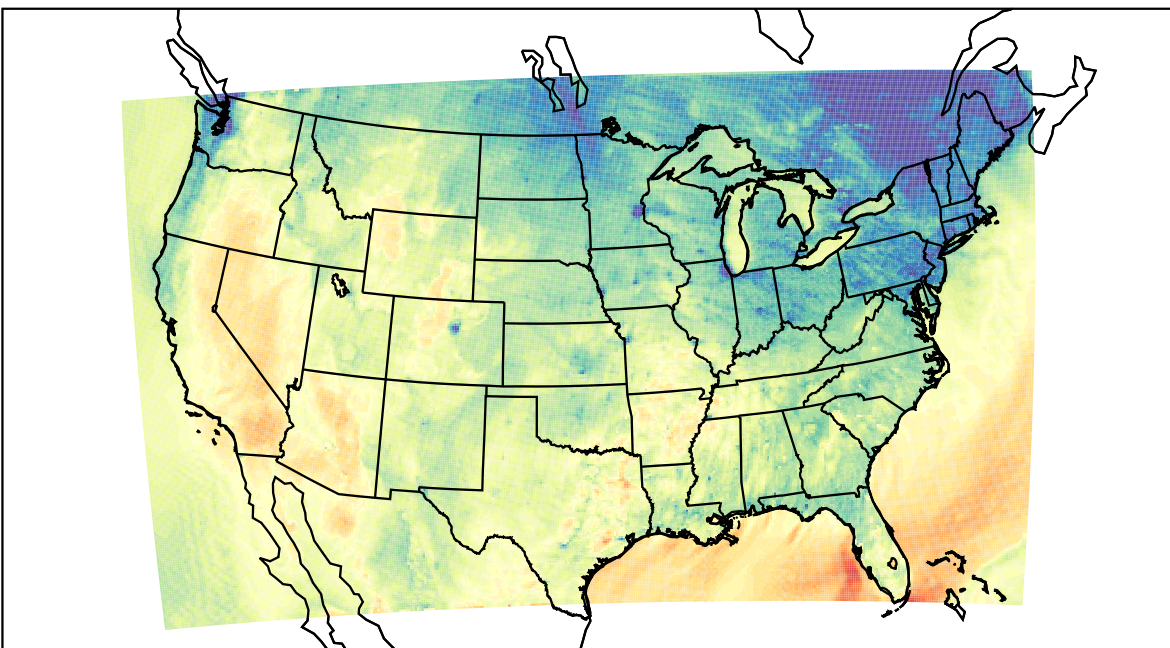
WRF (2021-10-18_00:00:00)
