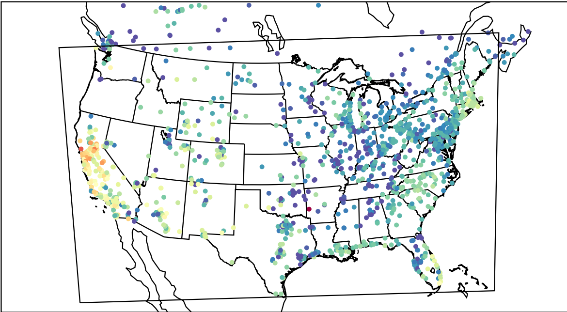
AirNOW (2021-10-17_01:00:00)
