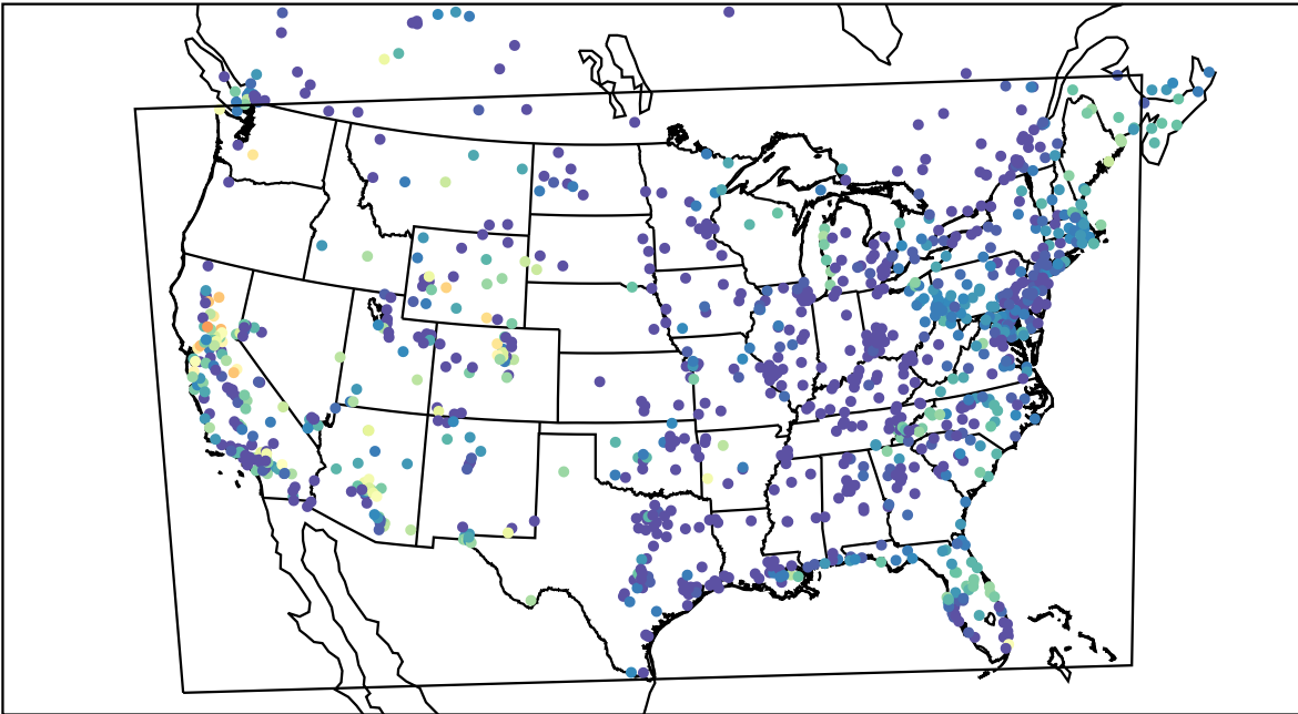
AirNOW (2021-10-17_10:00:00)
