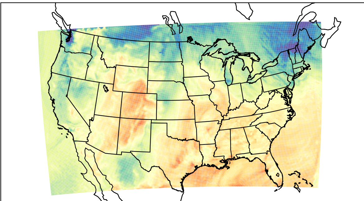
WRF (2021-10-18_19:00:00)
