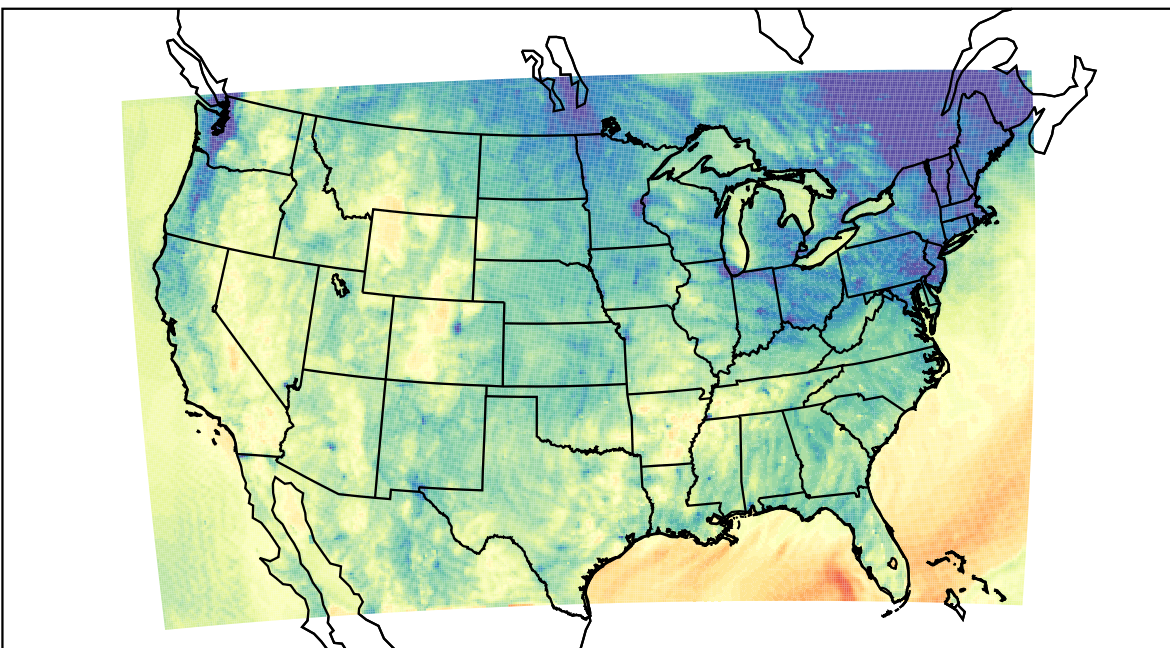
WRF (2021-10-18_03:00:00)
