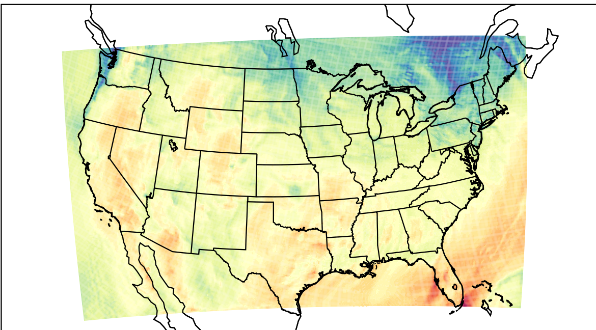
WRF (2021-10-17_20:00:00)
