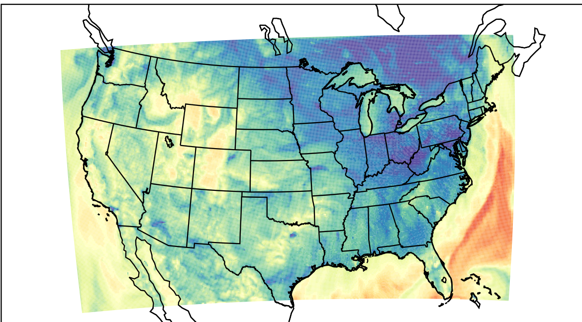
WRF (2021-10-17_07:00:00)
