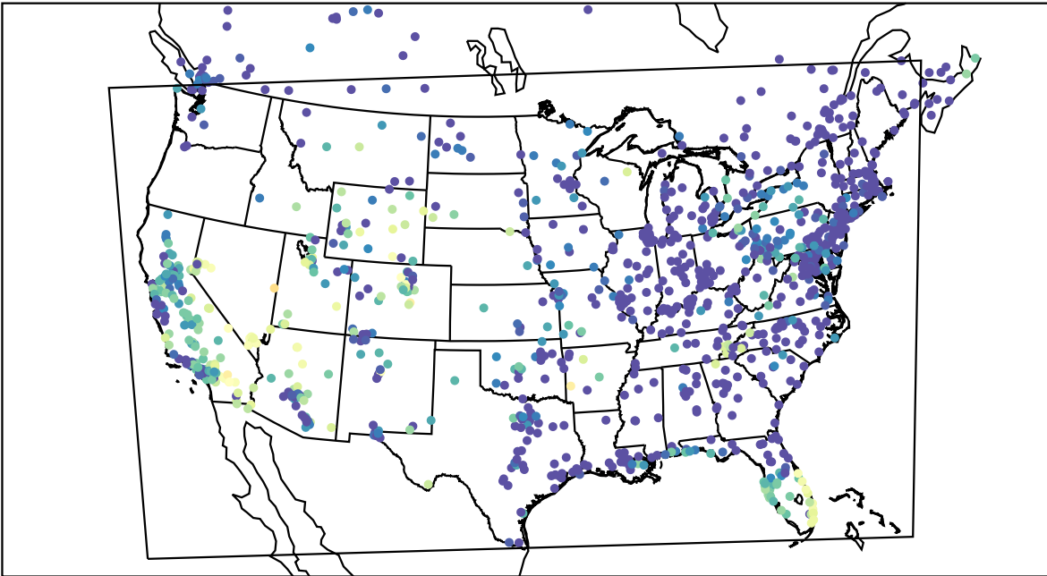
AirNOW (2021-10-18_10:00:00)
