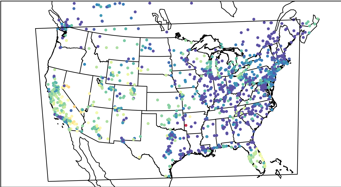
AirNOW (2021-10-18_04:00:00)
