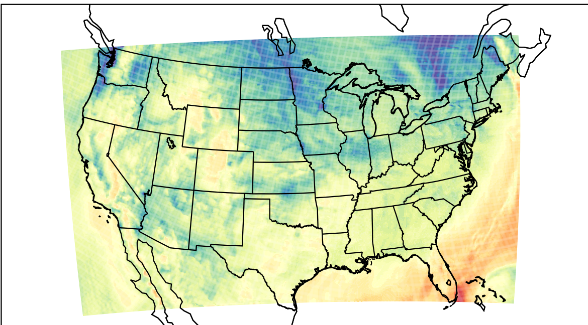
WRF (2021-10-17_17:00:00)
