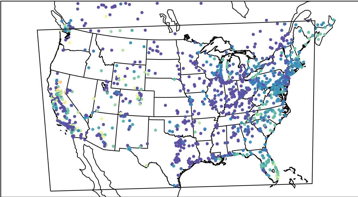
AirNOW (2021-10-17_13:00:00)
