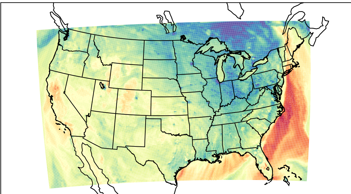
WRF (2021-10-17_00:00:00)
