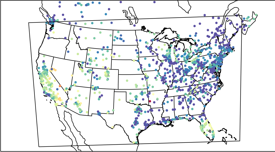
AirNOW (2021-10-18_03:00:00)
