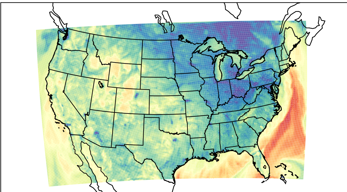
WRF (2021-10-17_04:00:00)
