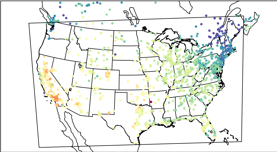
AirNOW (2021-10-17_21:00:00)
