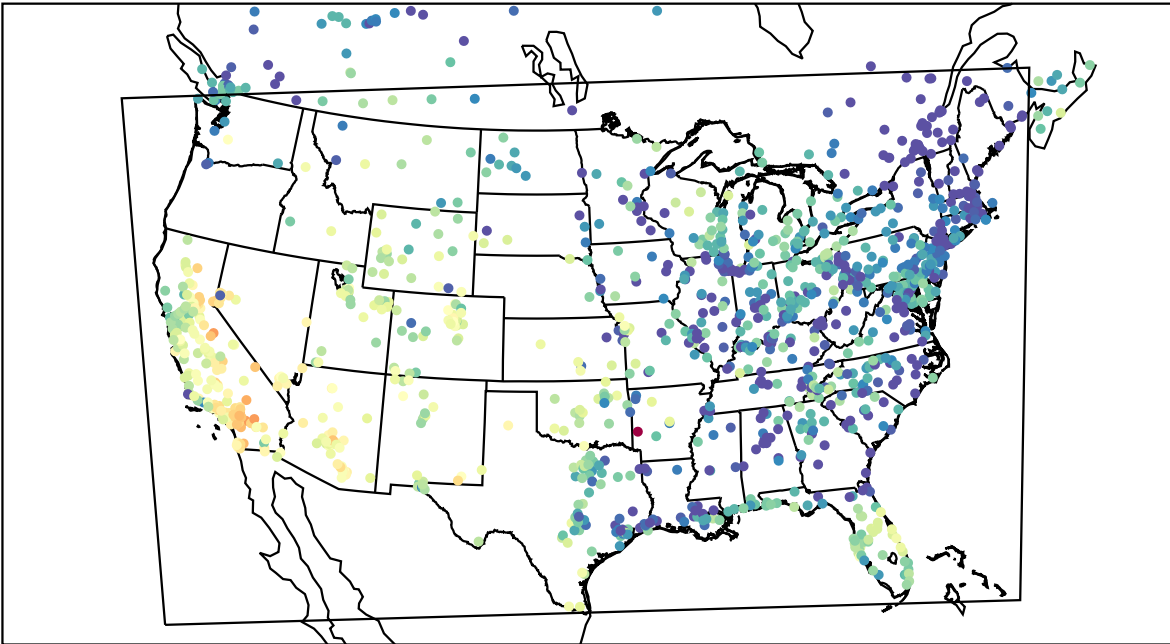
AirNOW (2021-10-18_00:00:00)
