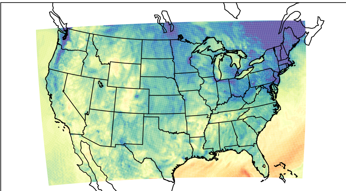
WRF (2021-10-18_05:00:00)
