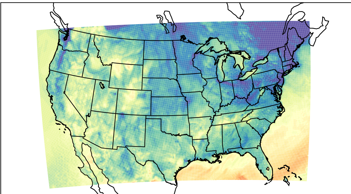
WRF (2021-10-18_09:00:00)
