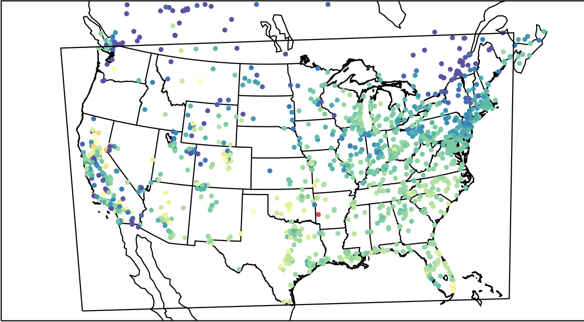
AirNOW (2021-10-17_16:00:00)
