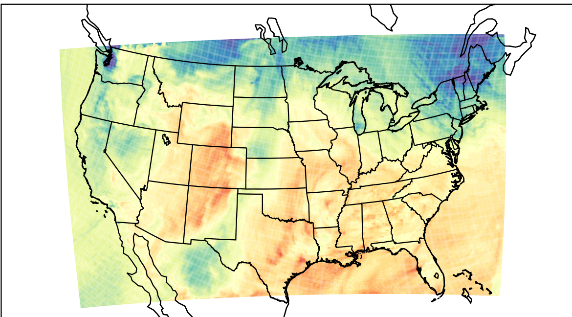
WRF (2021-10-18_20:00:00)
