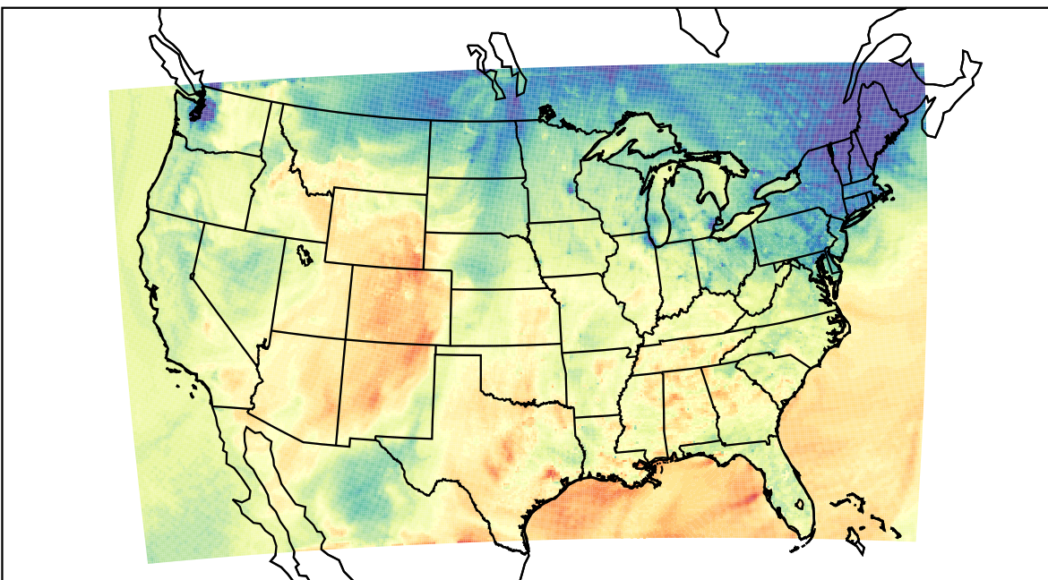
WRF (2021-10-18_23:00:00)
