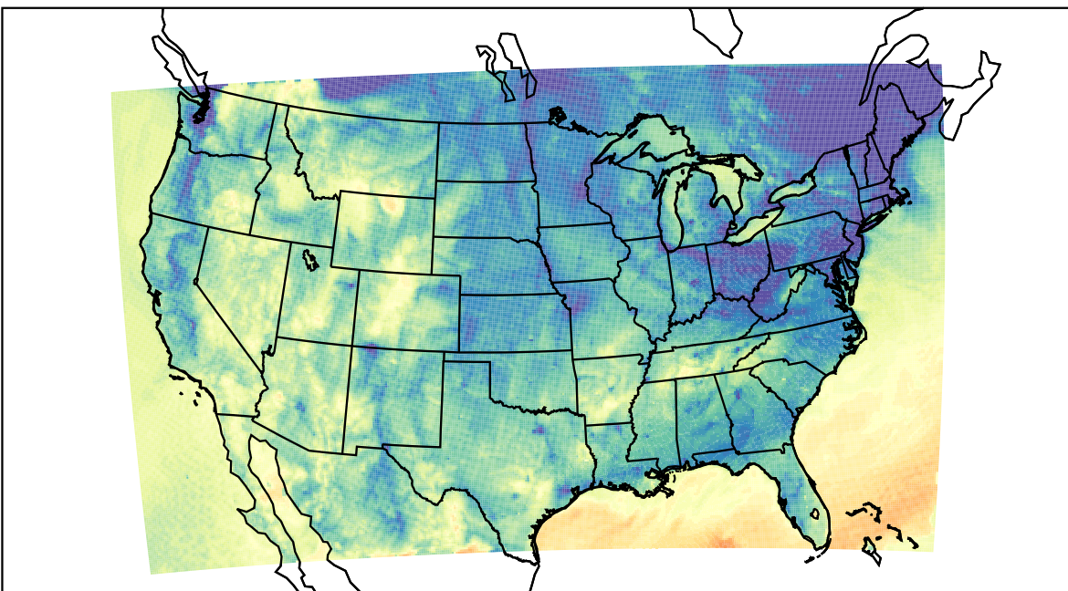
WRF (2021-10-18_11:00:00)
