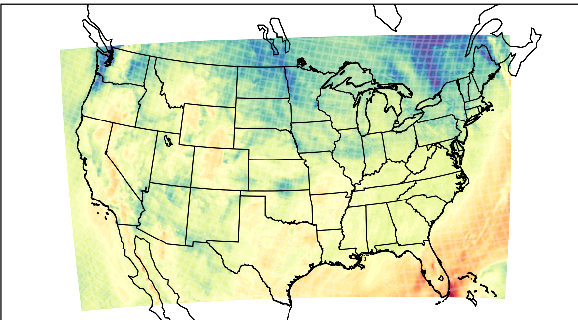
WRF (2021-10-17_18:00:00)
