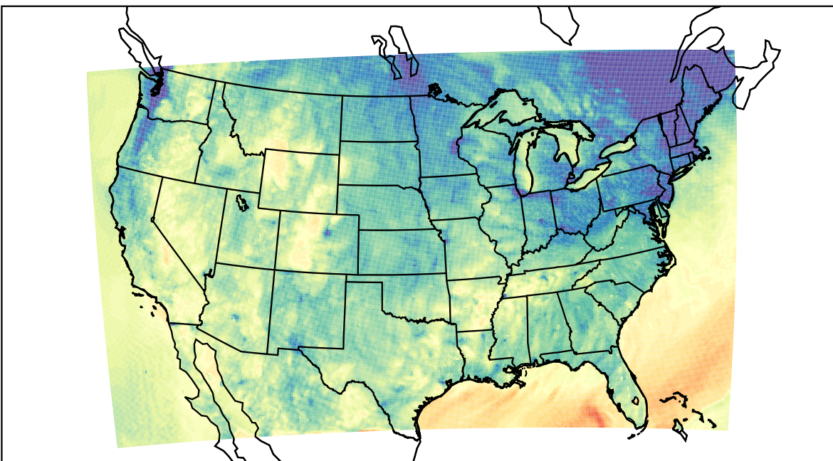
WRF (2021-10-18_04:00:00)
