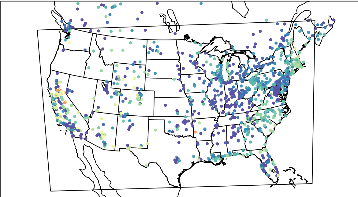
AirNOW (2021-10-17_04:00:00)
