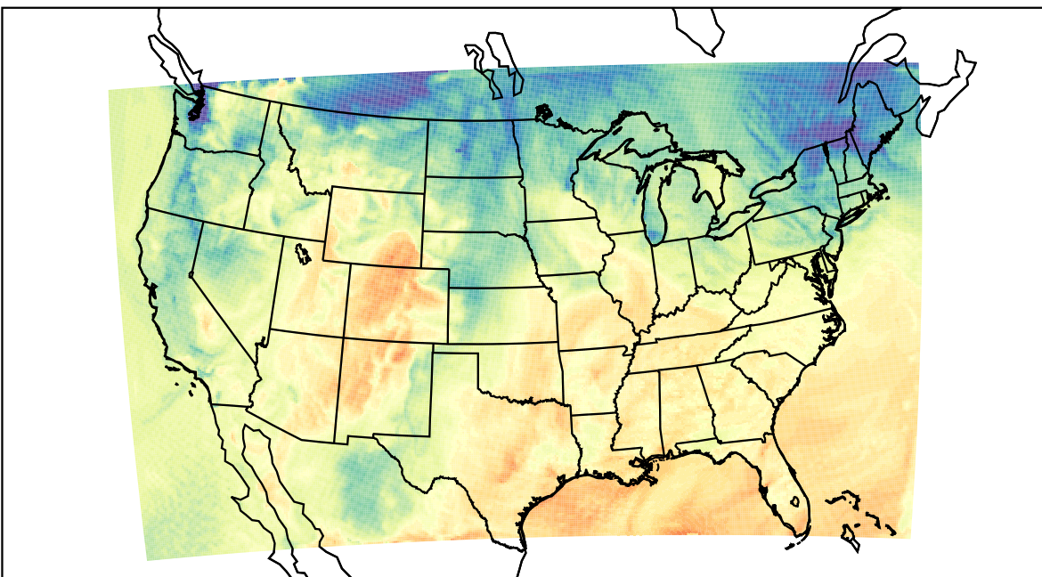
WRF (2021-10-18_18:00:00)
