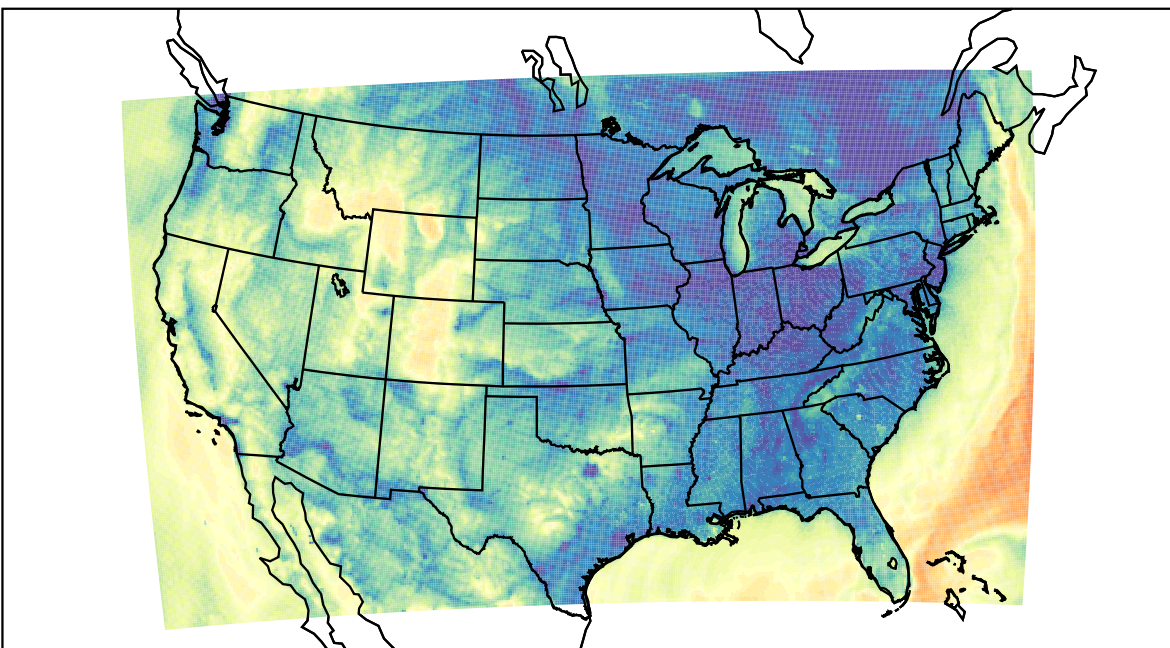
WRF (2021-10-17_13:00:00)
