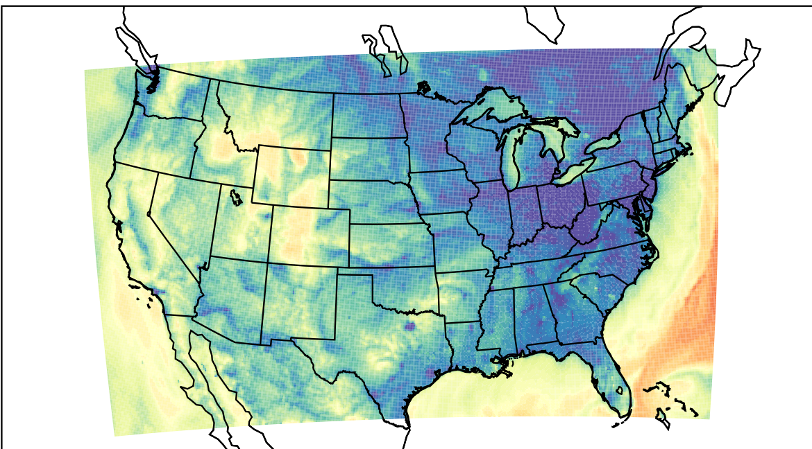
WRF (2021-10-17_12:00:00)
