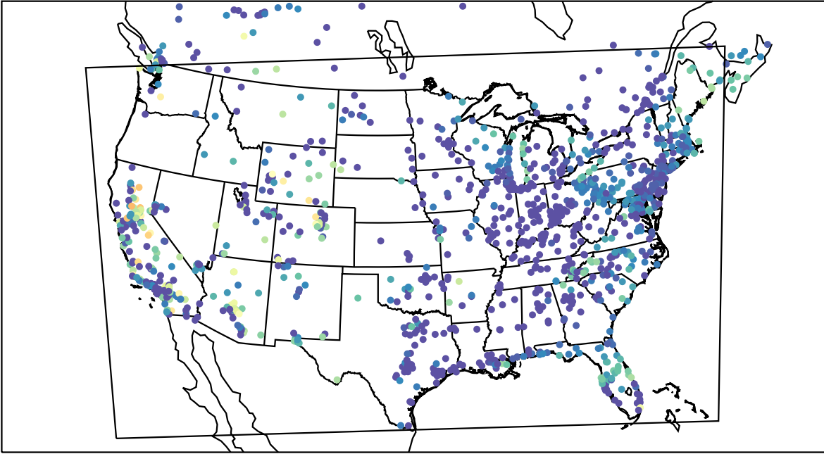
AirNOW (2021-10-17_11:00:00)
