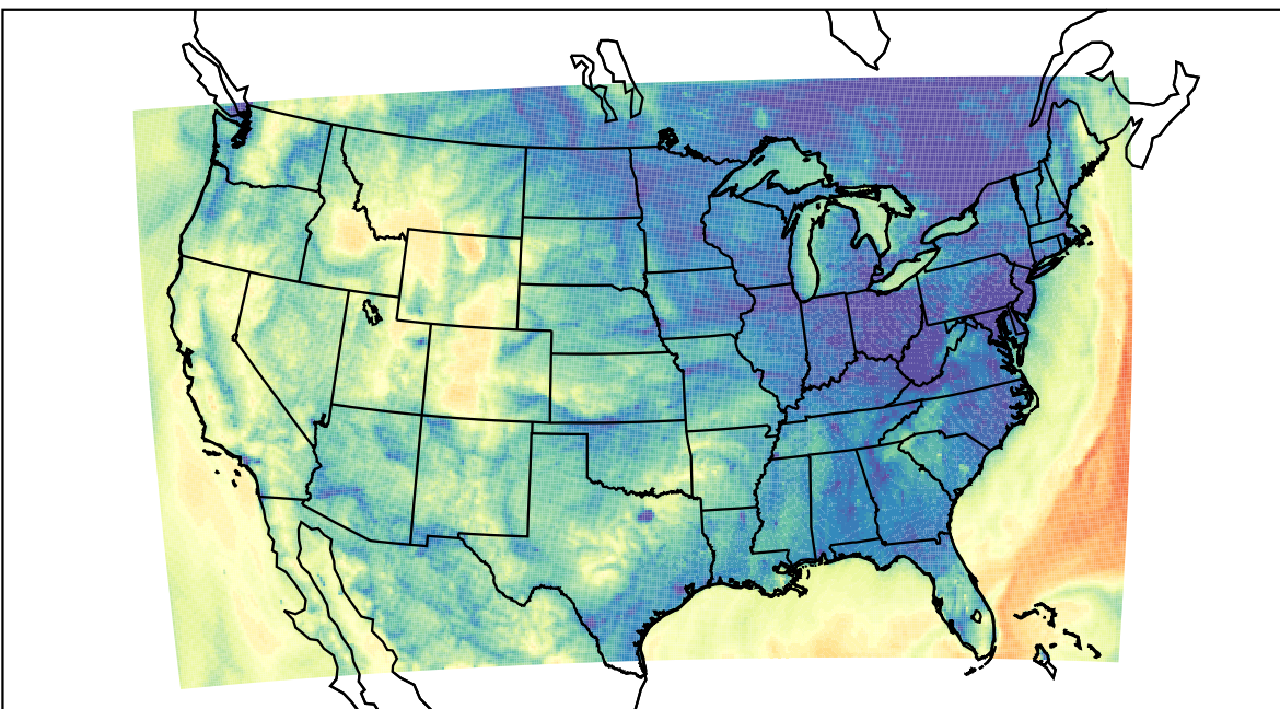
WRF (2021-10-17_11:00:00)
