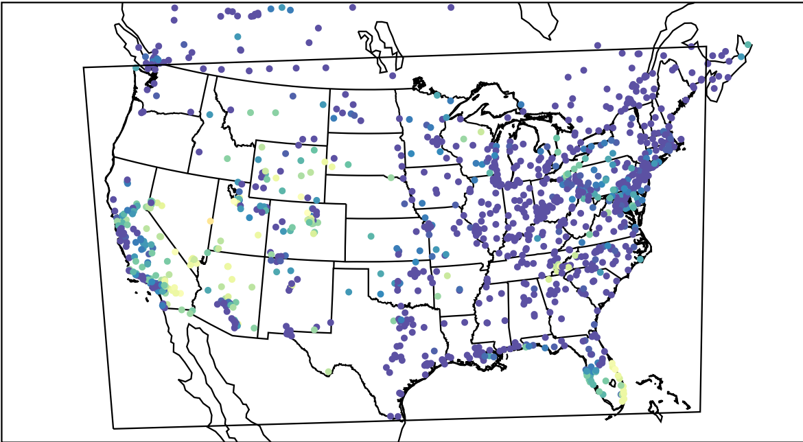
AirNOW (2021-10-18_12:00:00)
