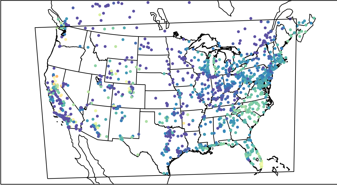
AirNOW (2021-10-17_14:00:00)
