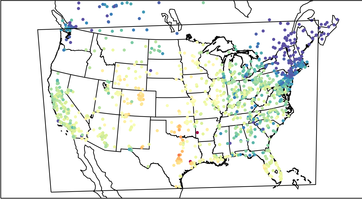
AirNOW (2021-10-18_22:00:00)
