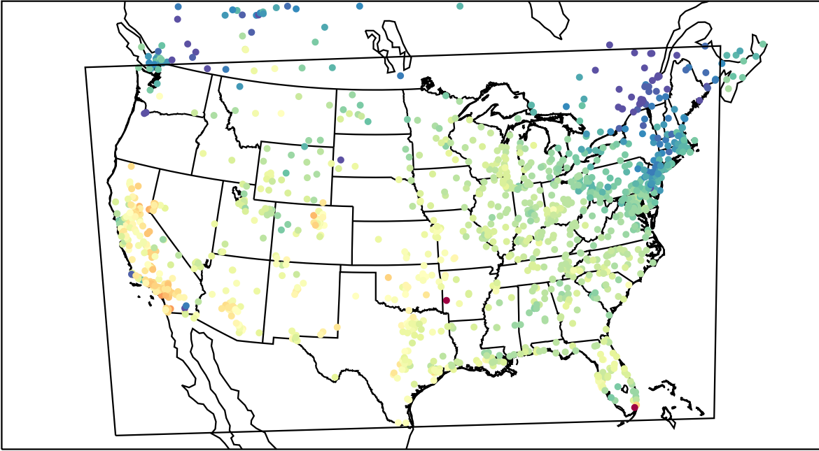
AirNOW (2021-10-17_19:00:00)
