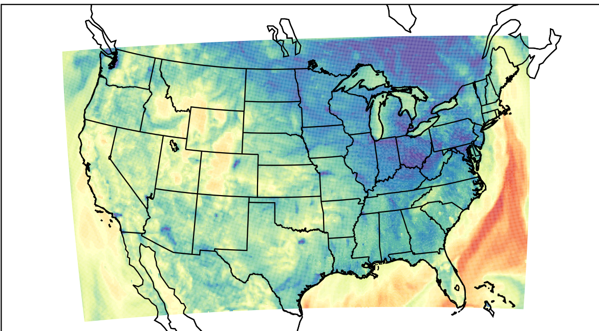
WRF (2021-10-17_05:00:00)
