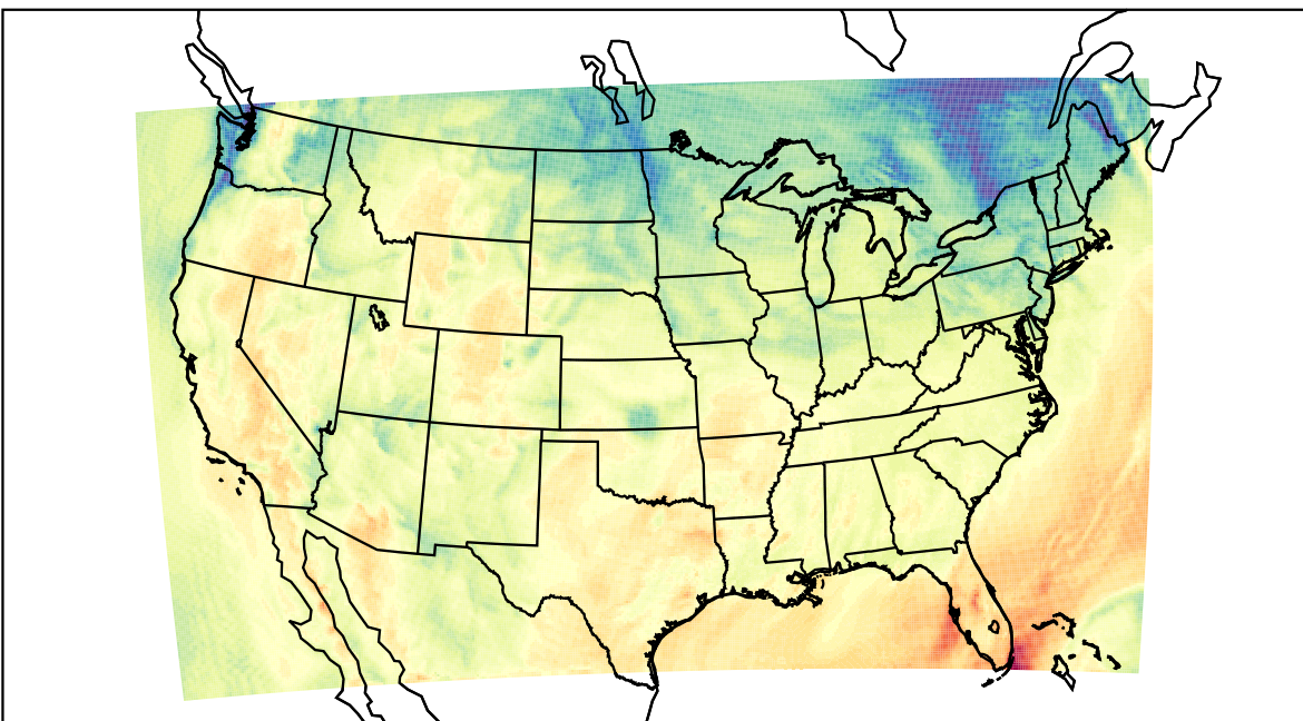
WRF (2021-10-17_19:00:00)
