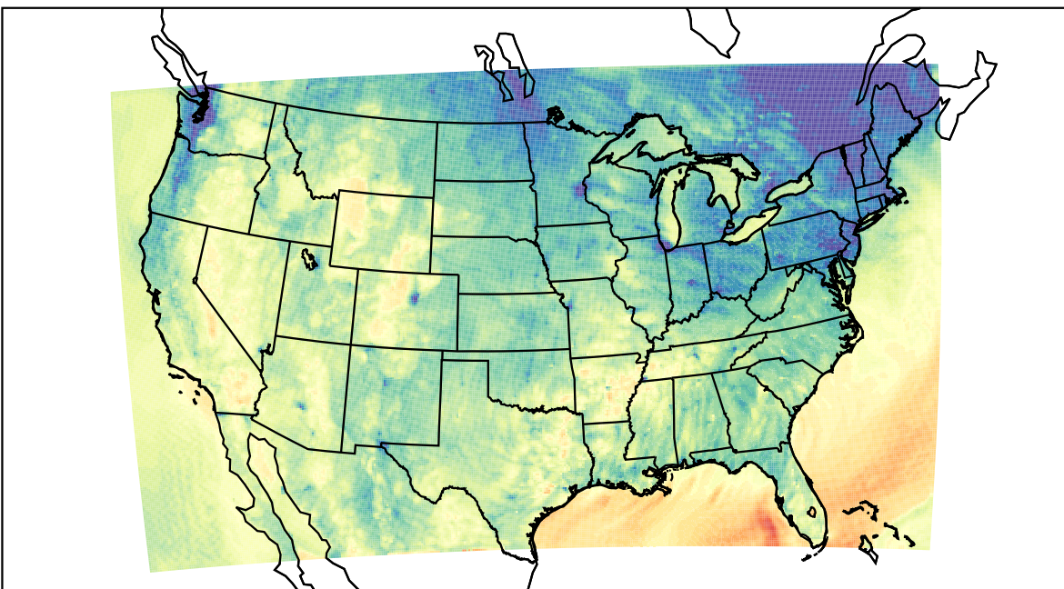
WRF (2021-10-18_02:00:00)
