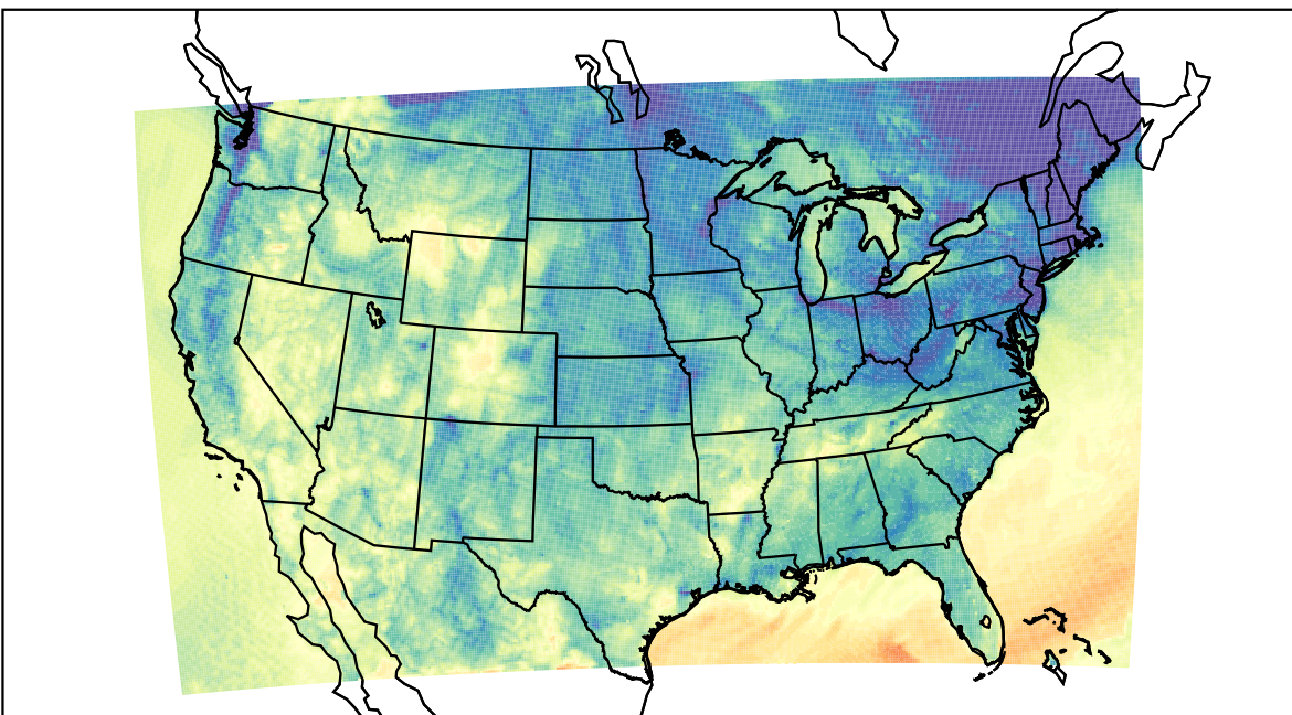
WRF (2021-10-18_08:00:00)
