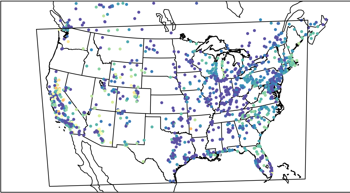
AirNOW (2021-10-17_07:00:00)
