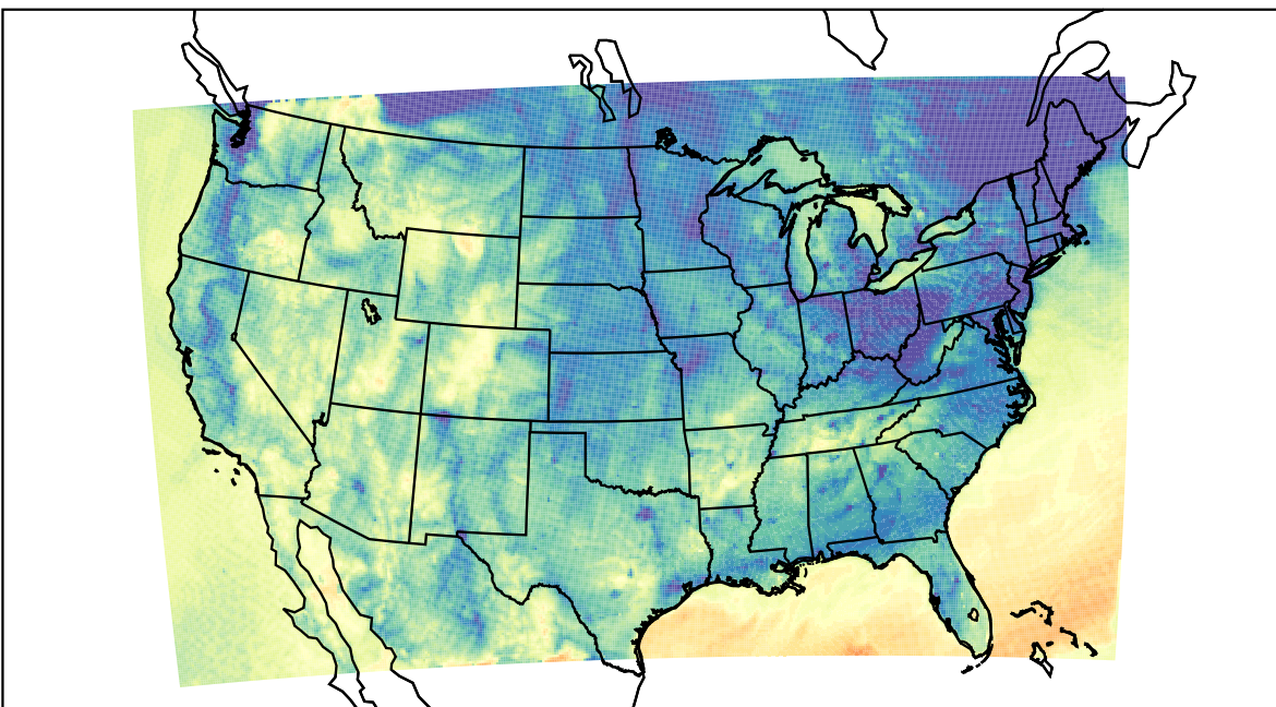
WRF (2021-10-18_12:00:00)
