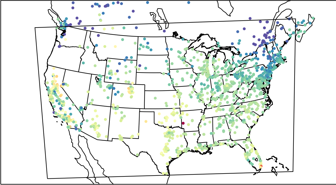
AirNOW (2021-10-17_17:00:00)
