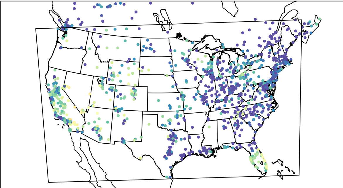
AirNOW (2021-10-18_06:00:00)
