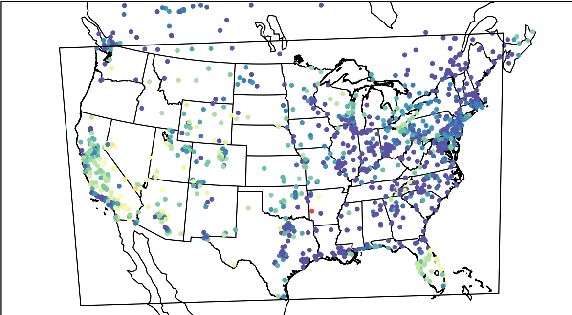
AirNOW (2021-10-18_05:00:00)
