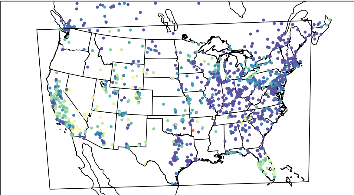
AirNOW (2021-10-18_07:00:00)
