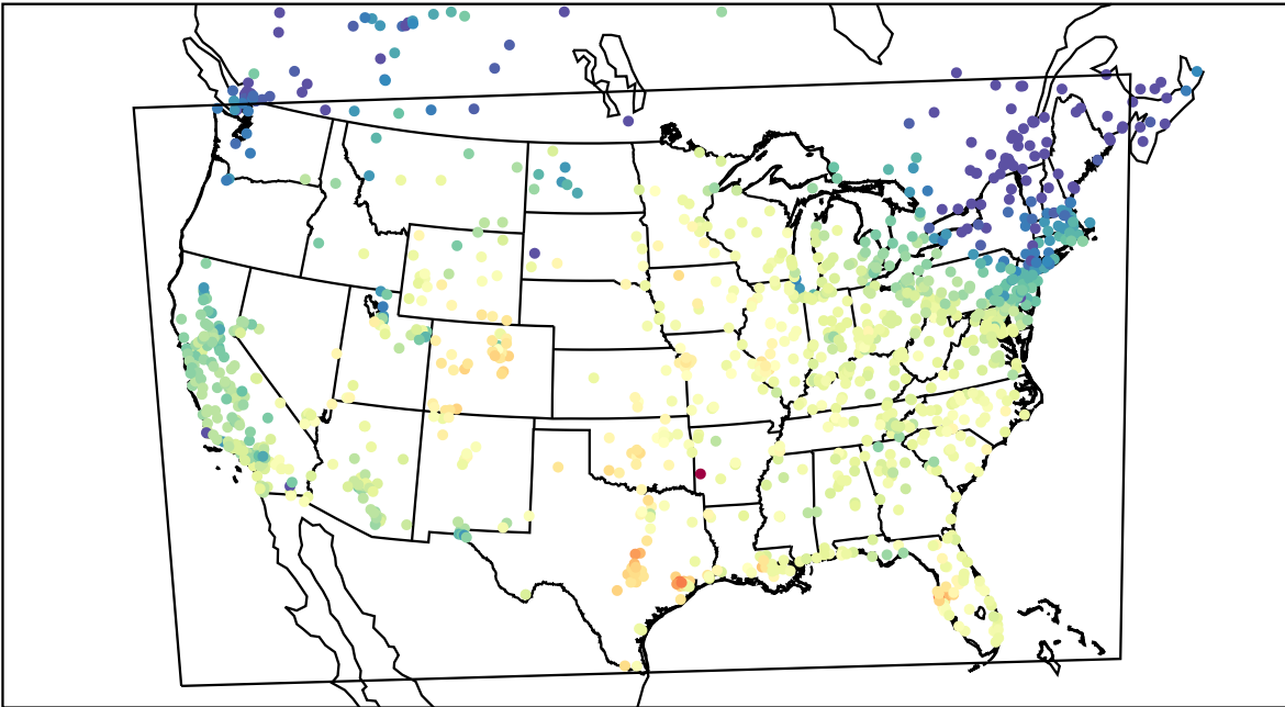
AirNOW (2021-10-18_19:00:00)
