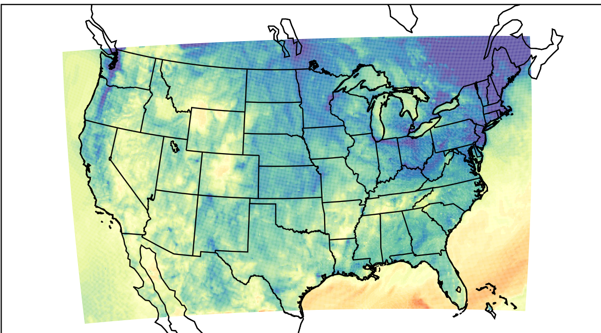
WRF (2021-10-18_07:00:00)
