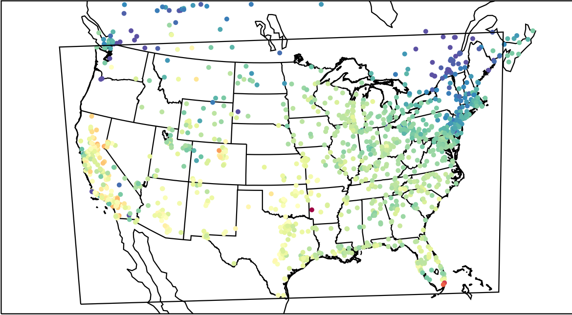
AirNOW (2021-10-17_18:00:00)
