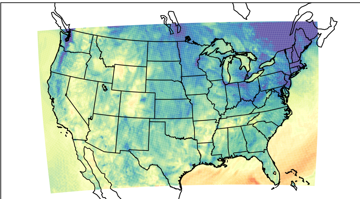
WRF (2021-10-18_06:00:00)
