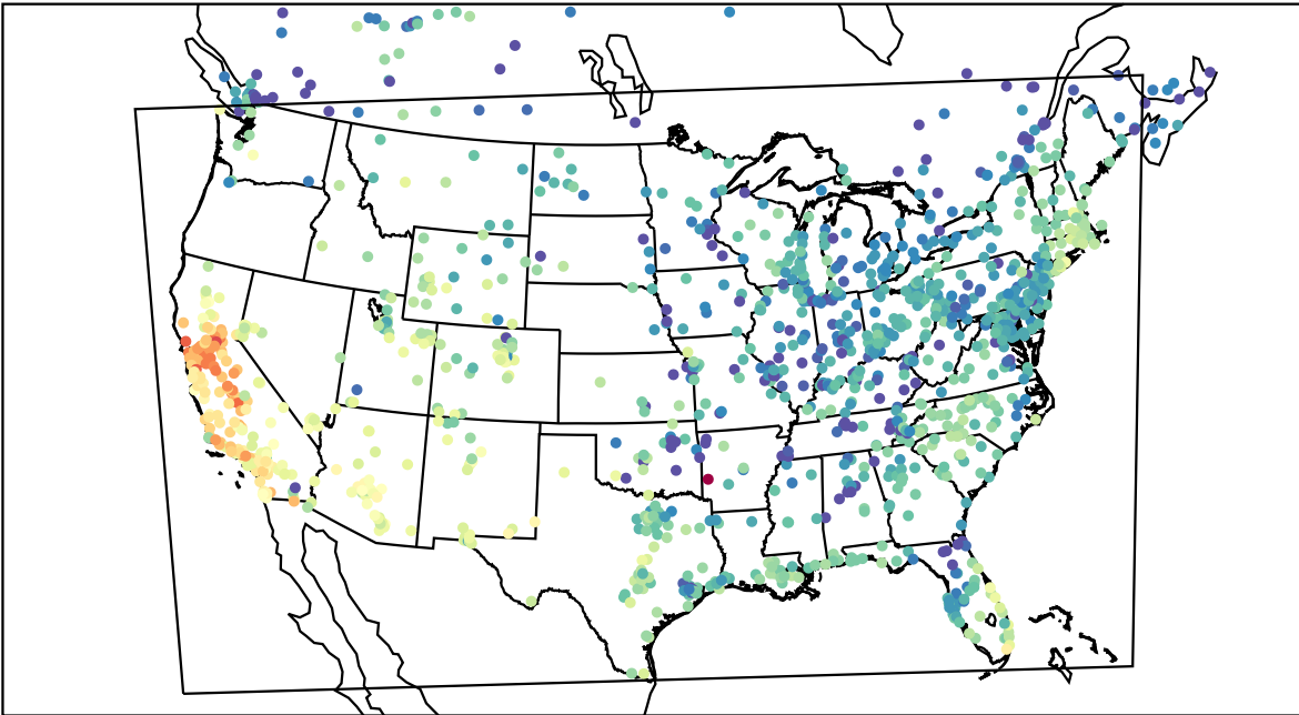
AirNOW (2021-10-17_00:00:00)
