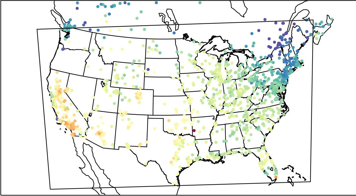
AirNOW (2021-10-17_20:00:00)
