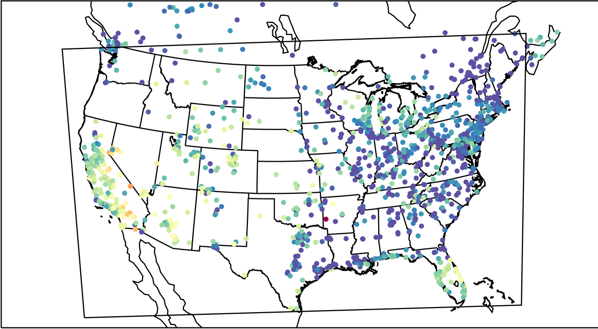
AirNOW (2021-10-18_02:00:00)
