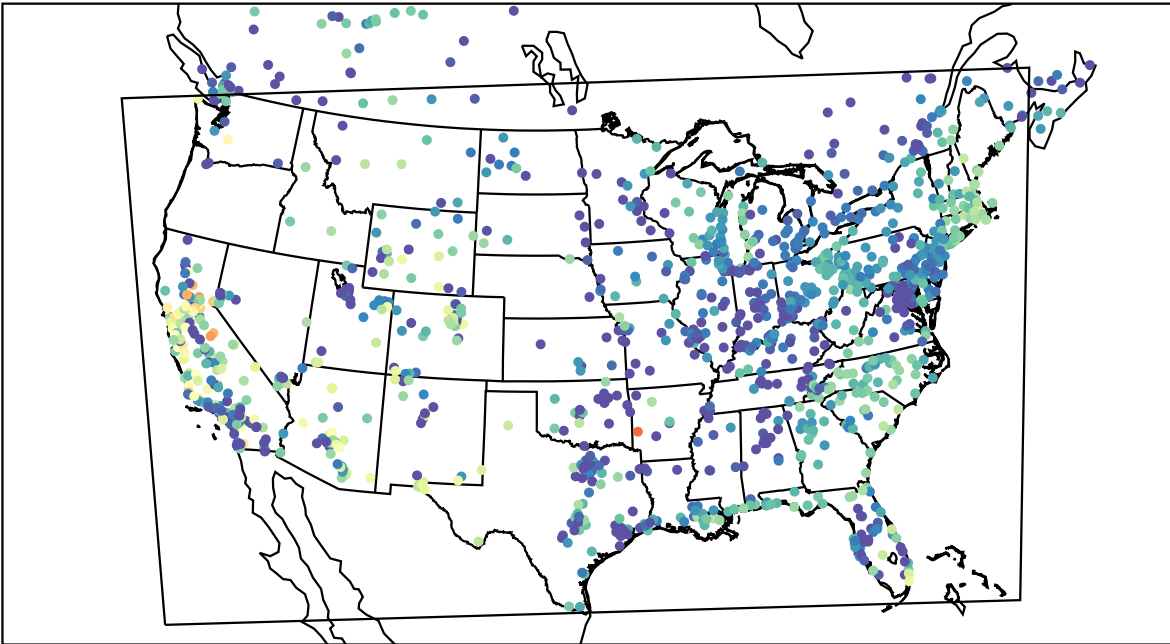
AirNOW (2021-10-17_03:00:00)
