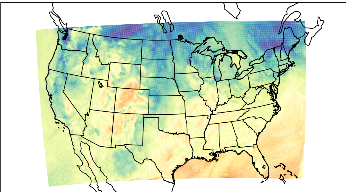
WRF (2021-10-18_17:00:00)
