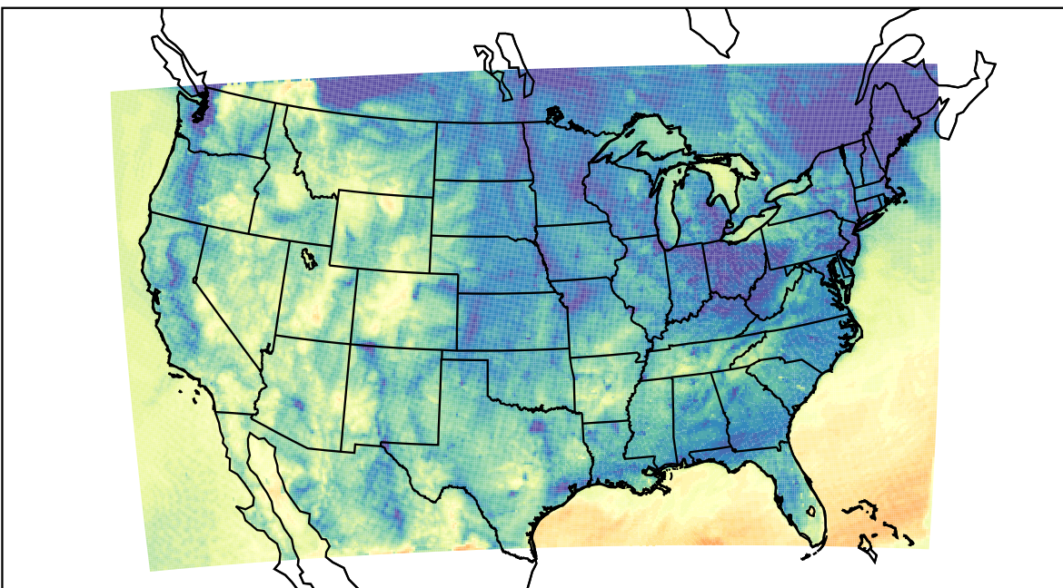
WRF (2021-10-18_13:00:00)
