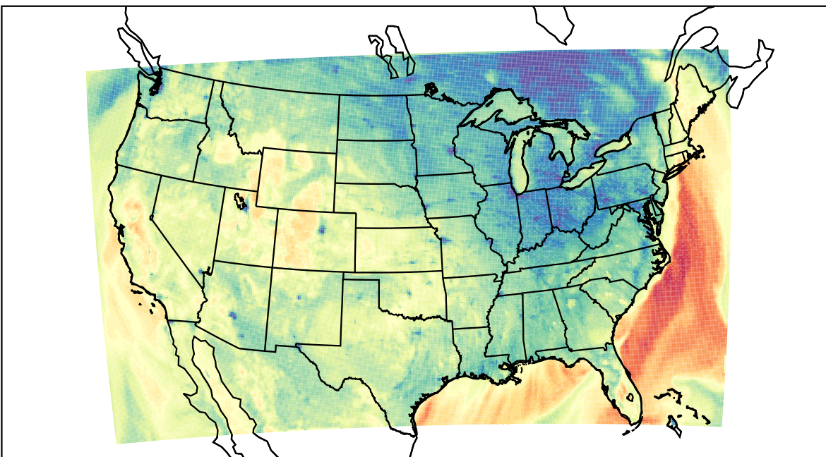
WRF (2021-10-17_01:00:00)
