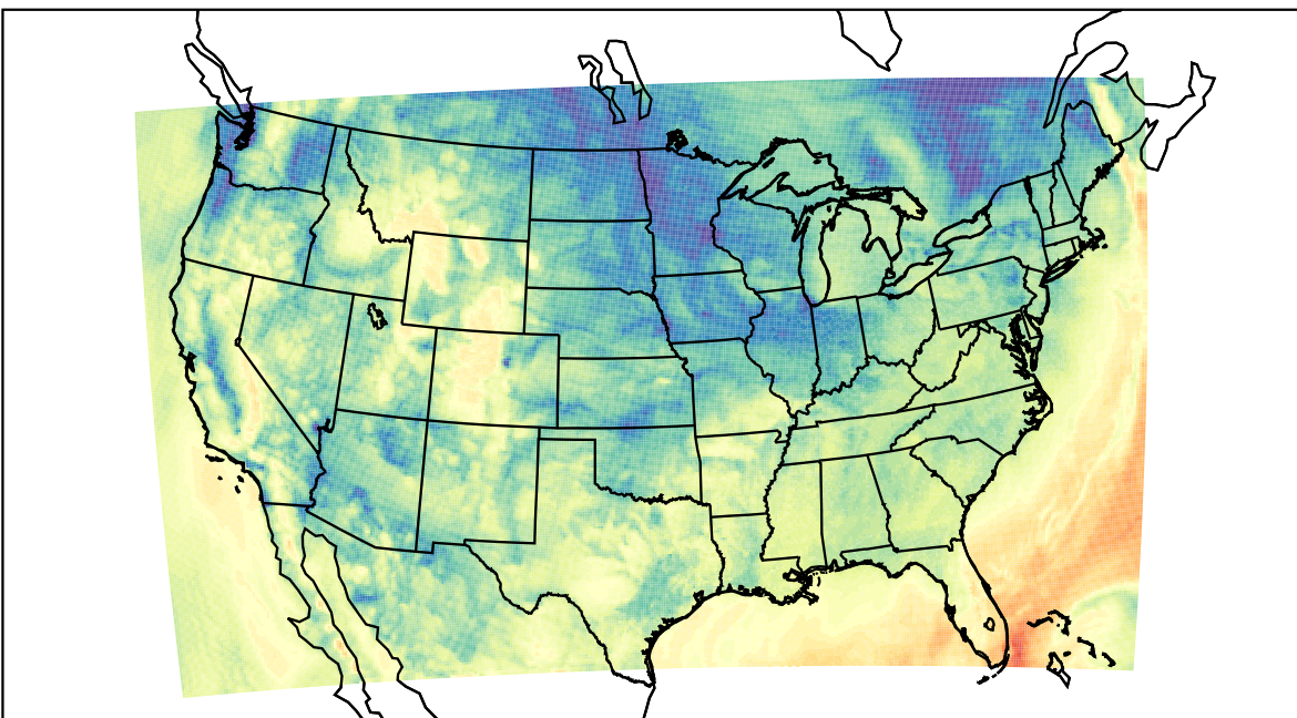
WRF (2021-10-17_16:00:00)
