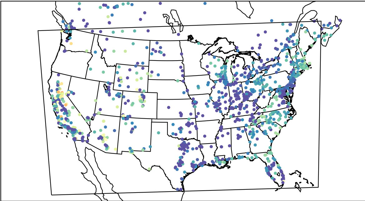
AirNOW (2021-10-17_06:00:00)
