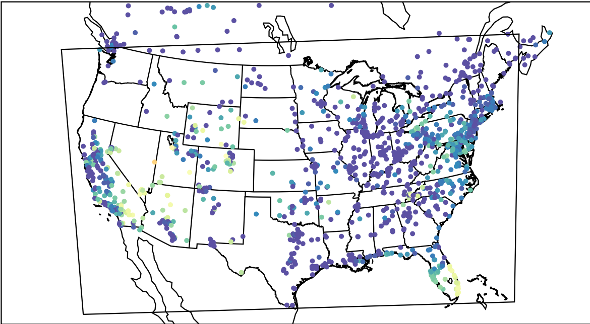
AirNOW (2021-10-18_13:00:00)
