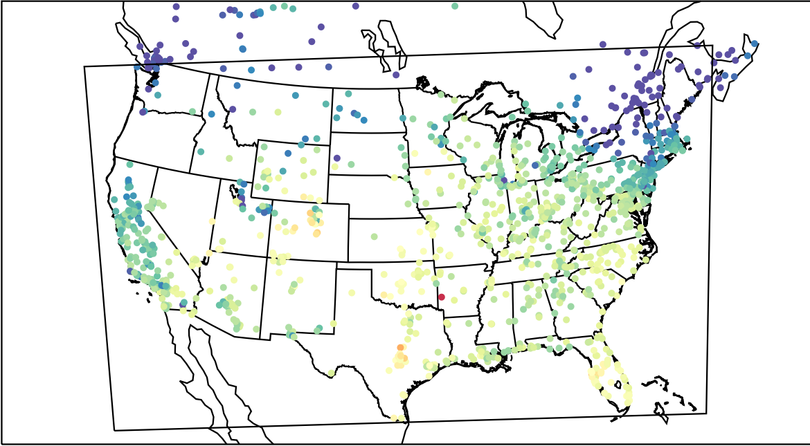
AirNOW (2021-10-18_17:00:00)
