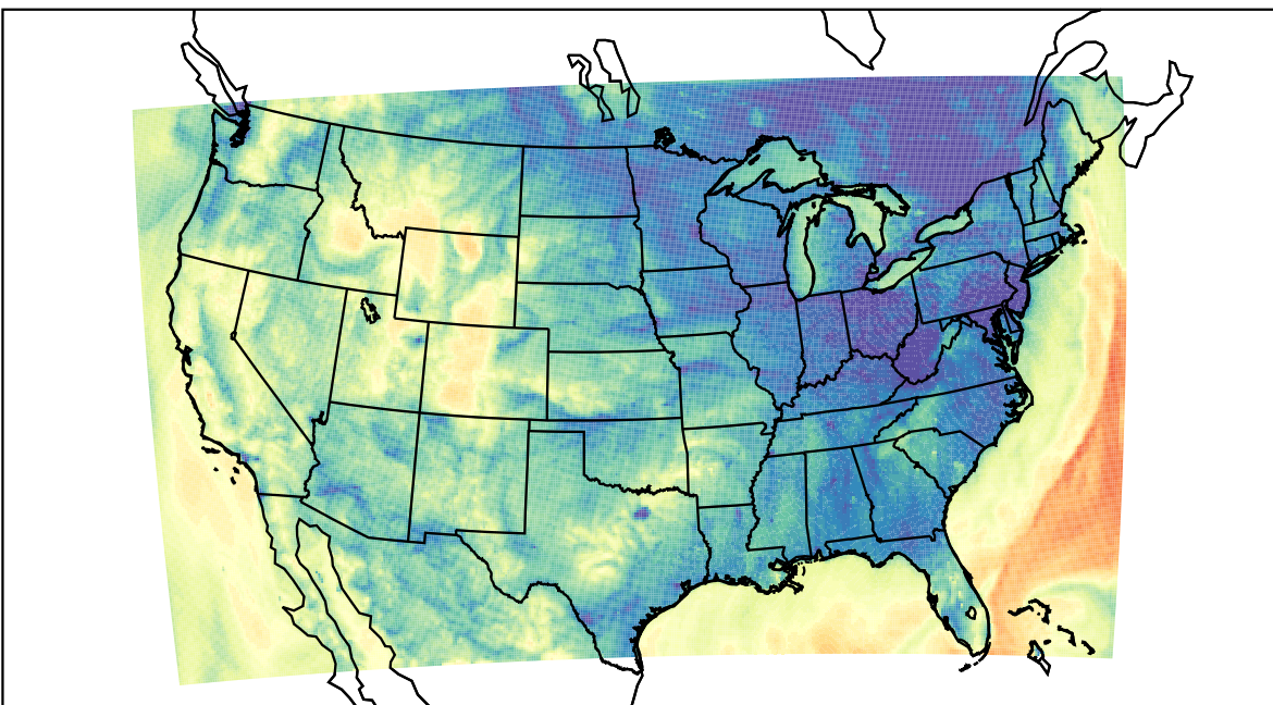
WRF (2021-10-17_10:00:00)
