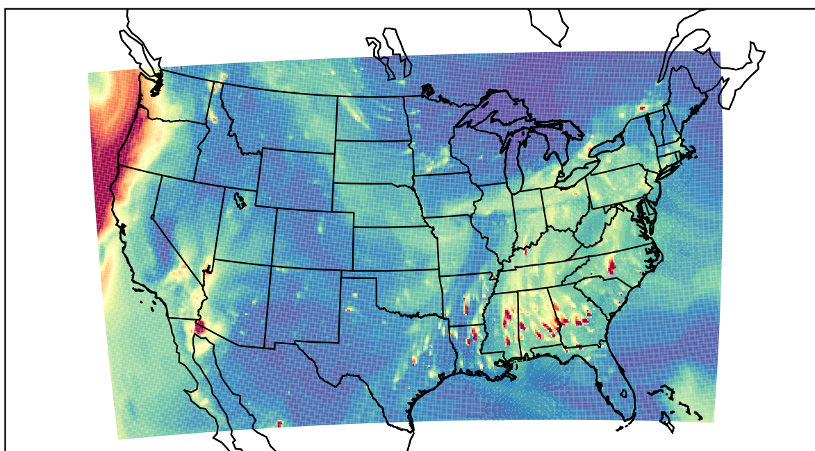
WRF 2021-10-25_01:00:00
