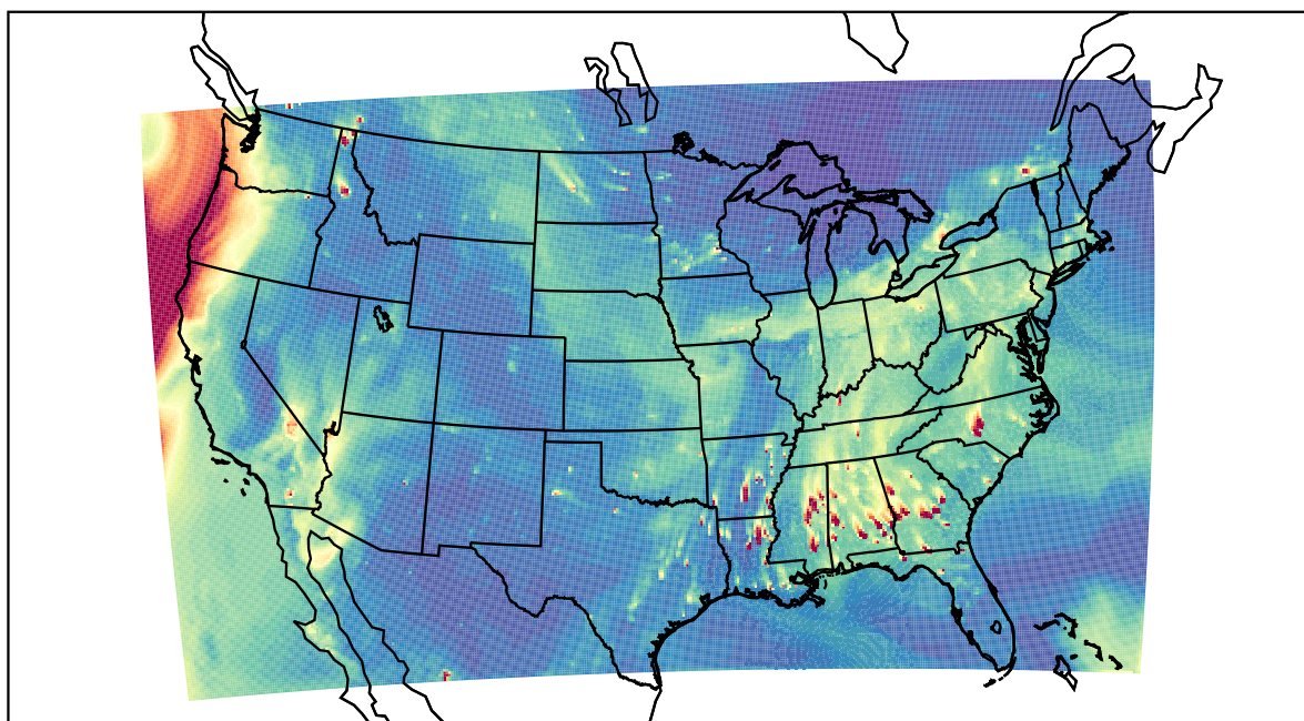
WRF 2021-10-25_00:00:00
