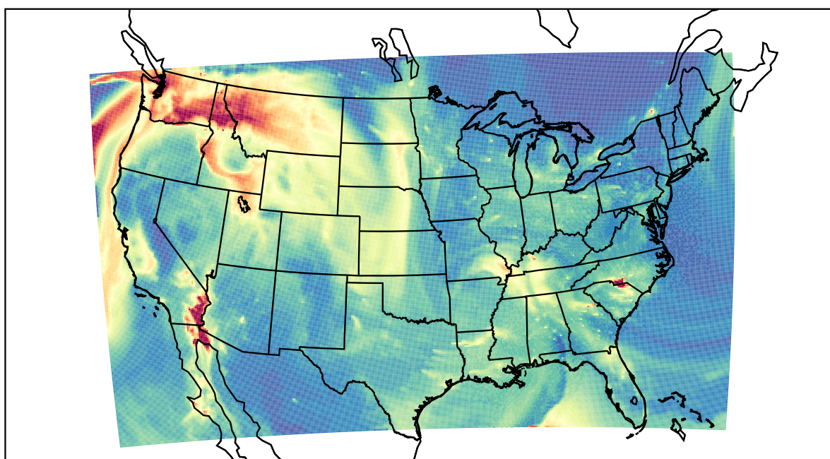
WRF 2021-10-28_12:00:00
