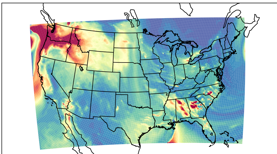
WRF 2021-10-28_05:00:00
