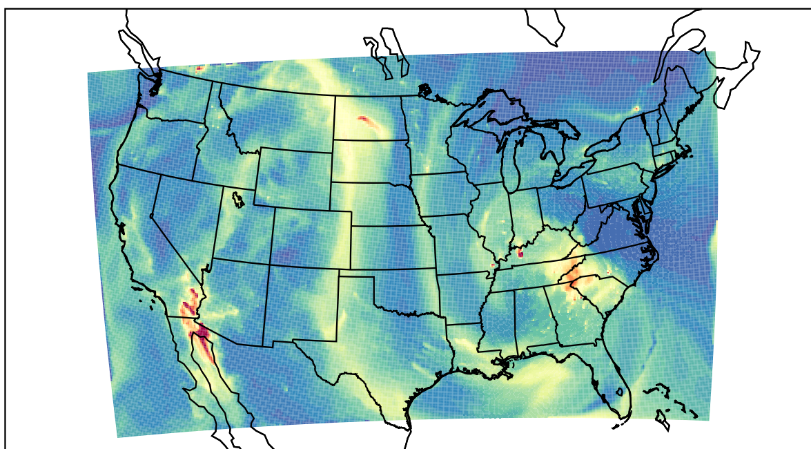
WRF 2021-10-29_09:00:00
