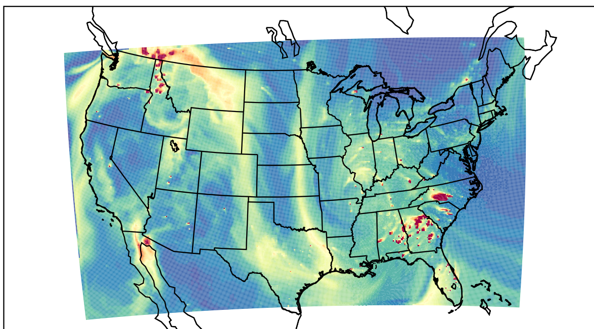
WRF 2021-10-28_22:00:00
