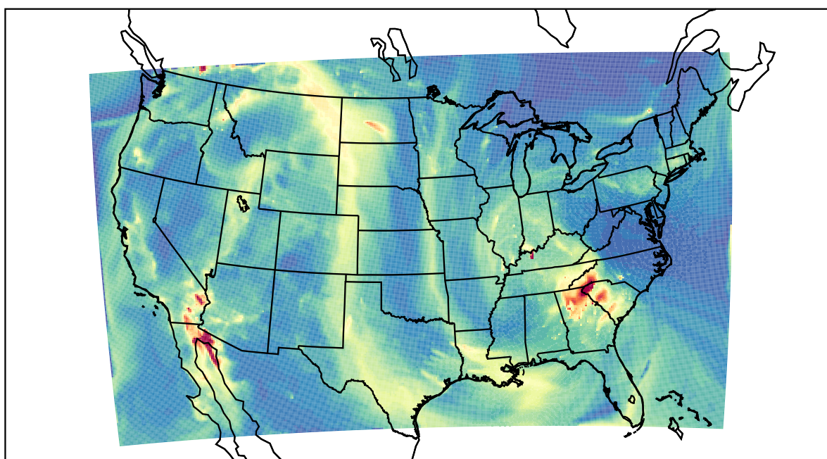
WRF 2021-10-29_06:00:00
