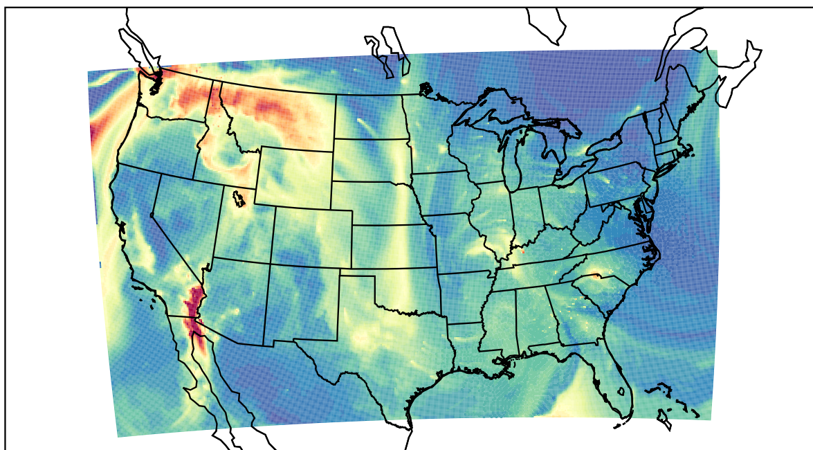
WRF 2021-10-28_16:00:00
