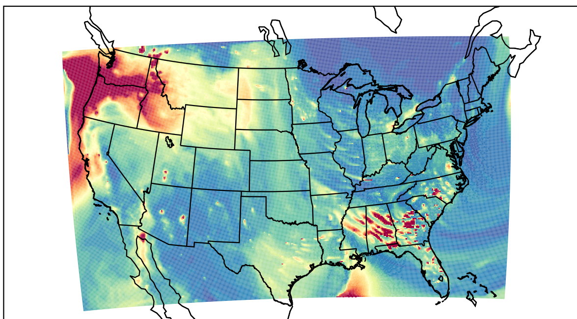
WRF 2021-10-28_02:00:00
