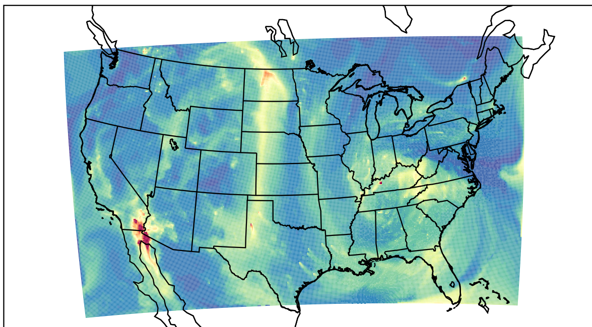
WRF 2021-10-29_15:00:00
