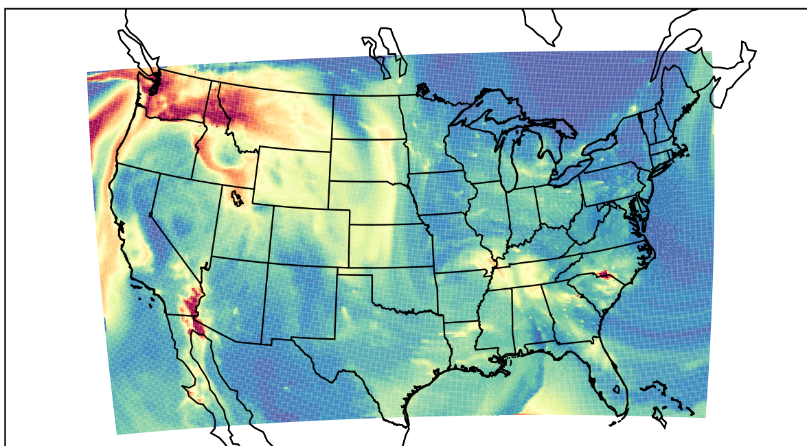
WRF 2021-10-28_11:00:00
