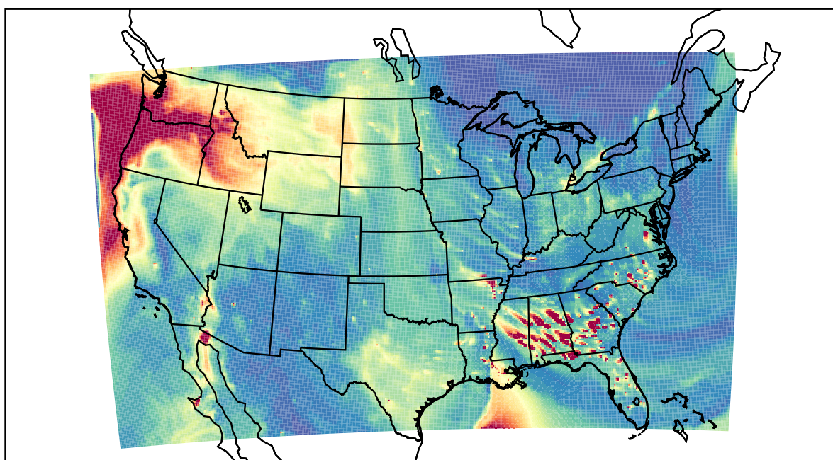
WRF 2021-10-28_00:00:00
