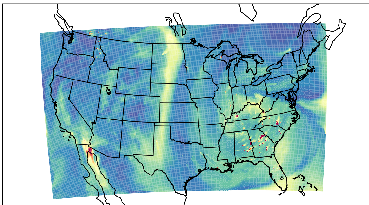
WRF 2021-10-29_19:00:00
