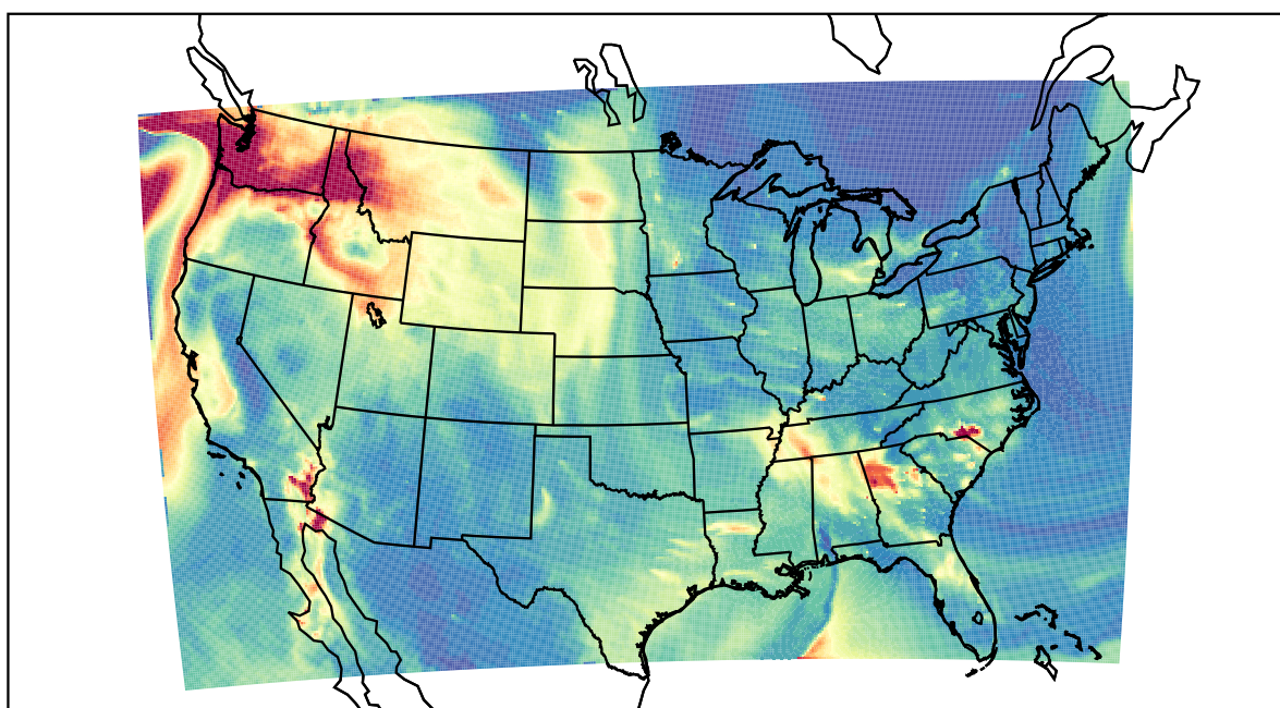
WRF 2021-10-28_08:00:00
