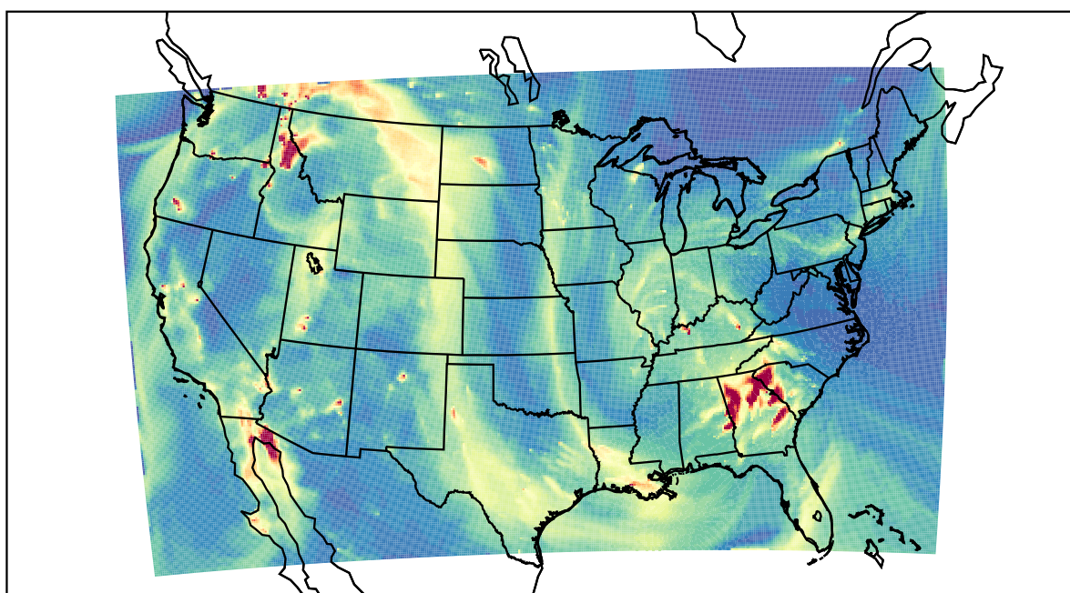
WRF 2021-10-29_03:00:00
