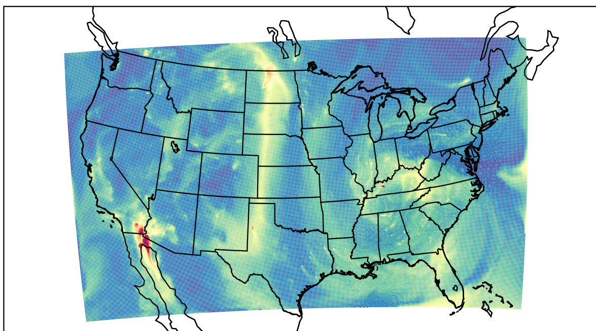
WRF 2021-10-29_16:00:00
