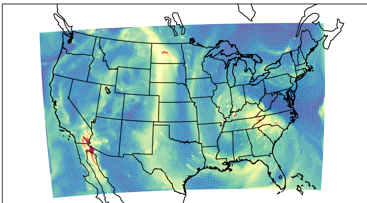
WRF 2021-10-29_11:00:00
