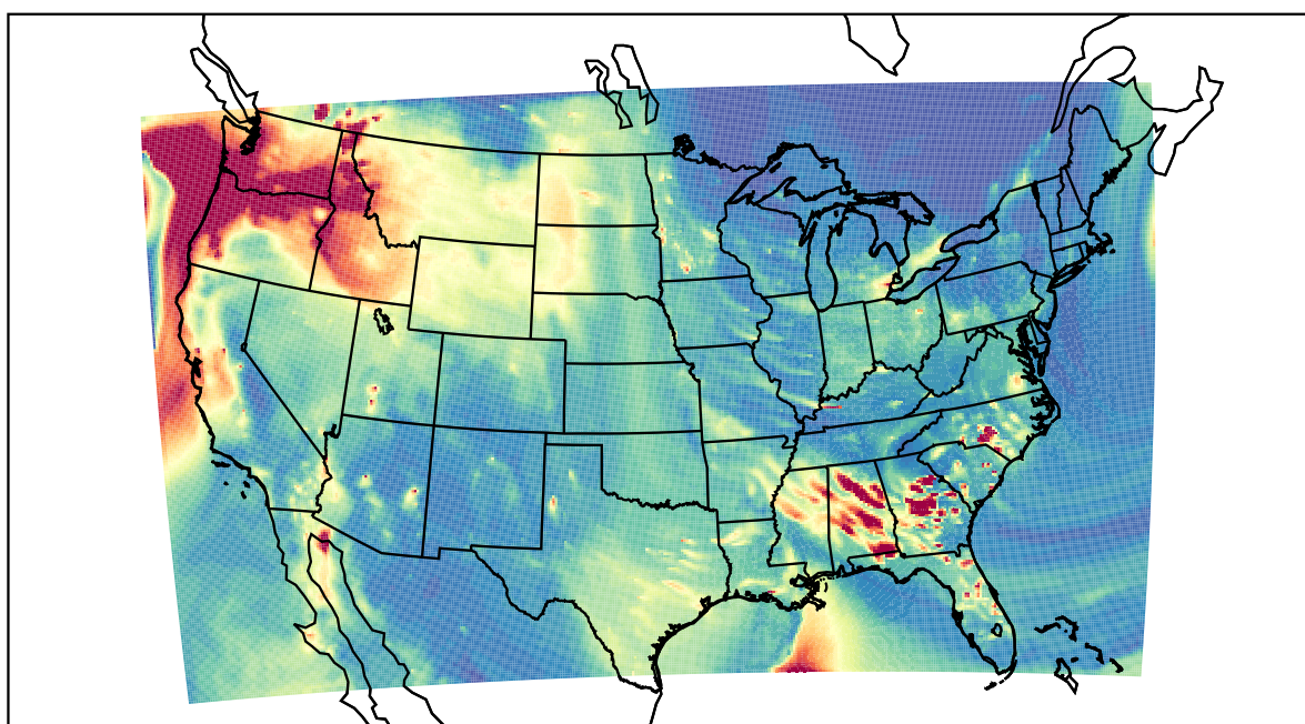
WRF 2021-10-28_03:00:00
