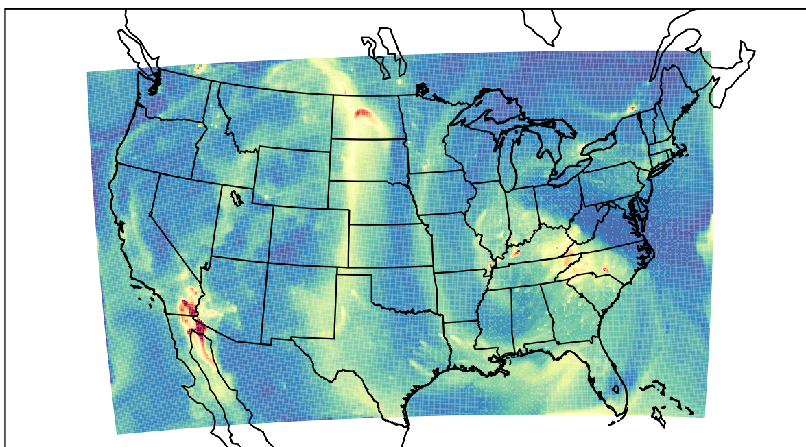
WRF 2021-10-29_12:00:00
