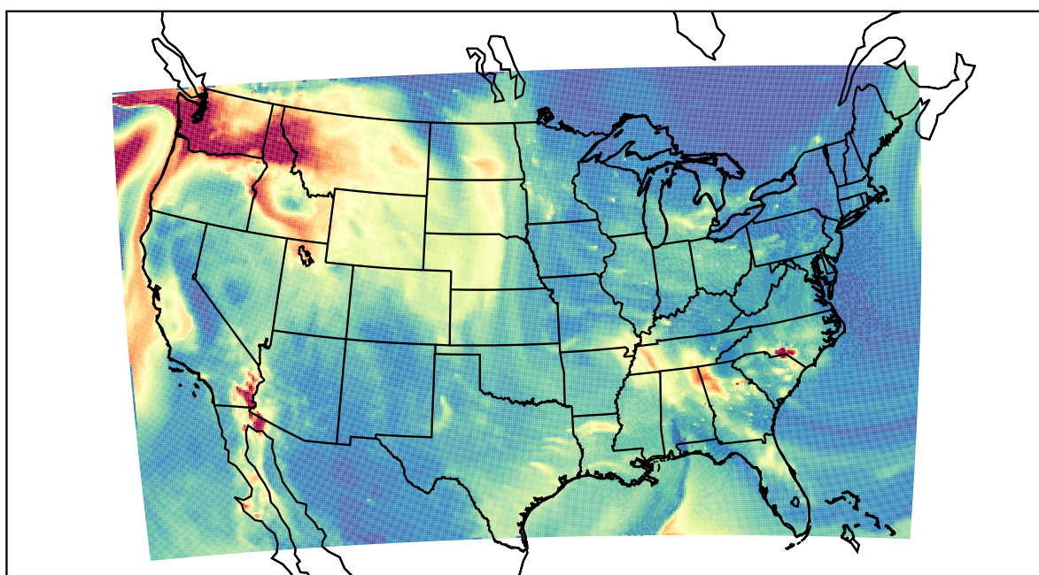
WRF 2021-10-28_09:00:00
