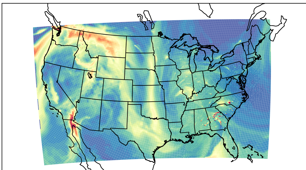
WRF 2021-10-28_18:00:00
