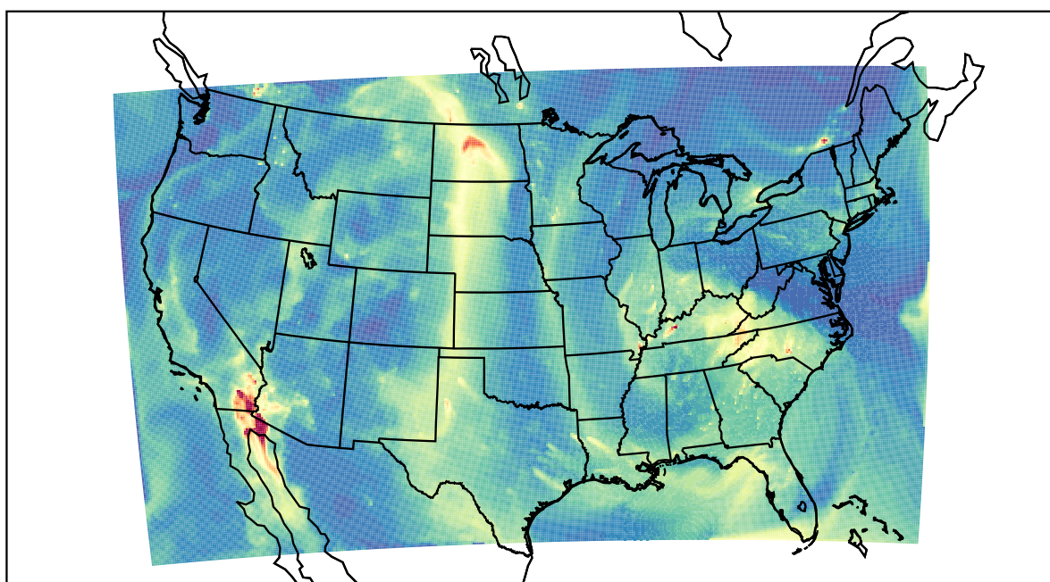
WRF 2021-10-29_13:00:00
