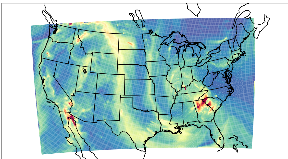
WRF 2021-10-29_05:00:00
