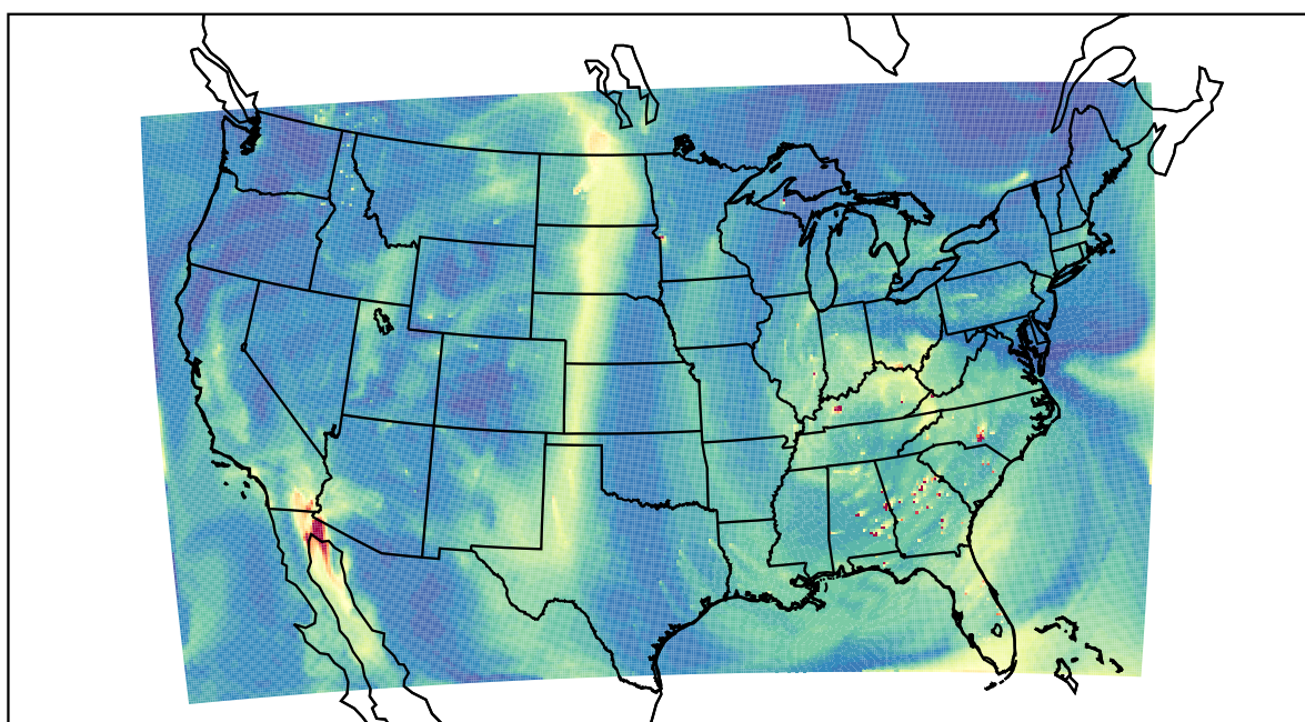
WRF 2021-10-29_18:00:00
