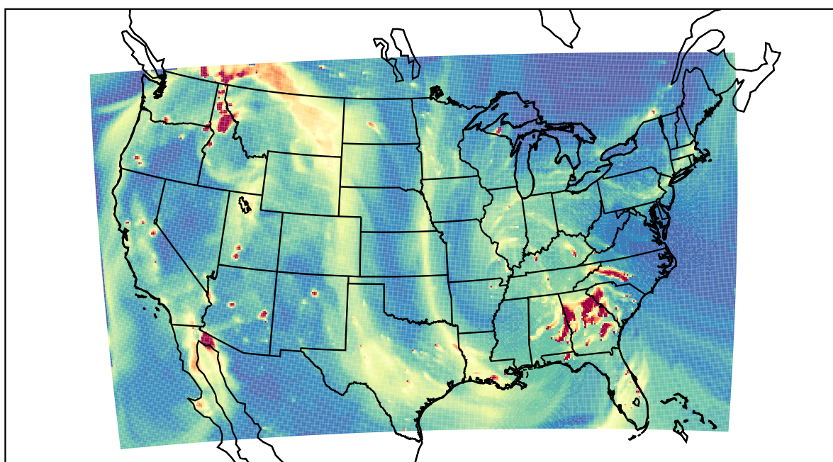
WRF 2021-10-29_01:00:00
