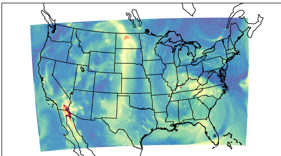
WRF 2021-10-29_14:00:00
