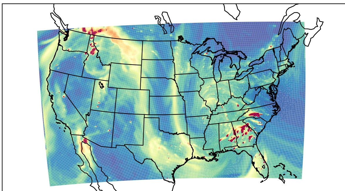
WRF 2021-10-28_23:00:00
