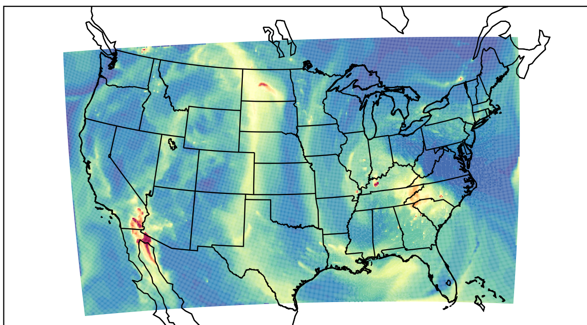
WRF 2021-10-29_10:00:00
