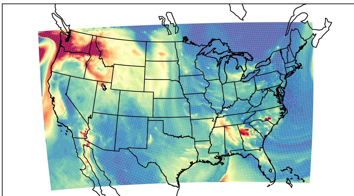
WRF 2021-10-28_07:00:00
