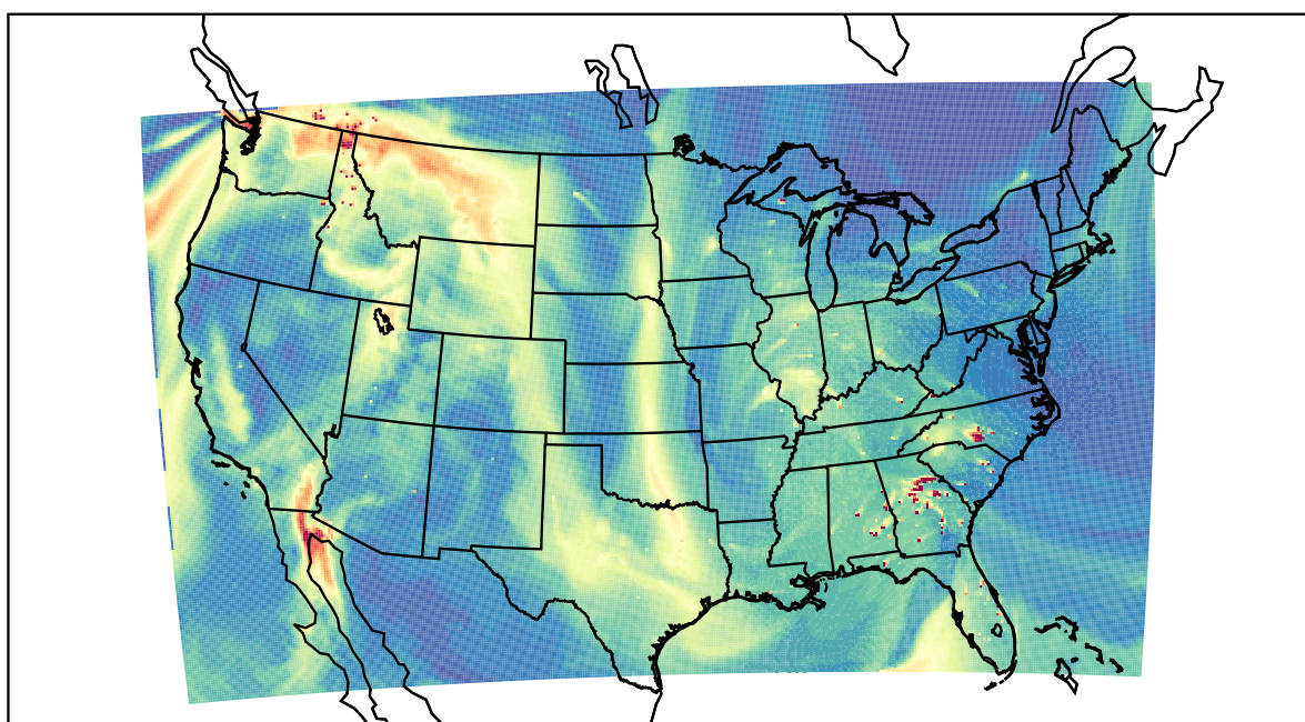
WRF 2021-10-28_19:00:00
