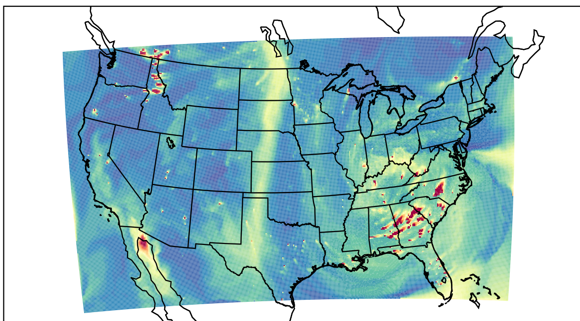
WRF 2021-10-29_23:00:00
