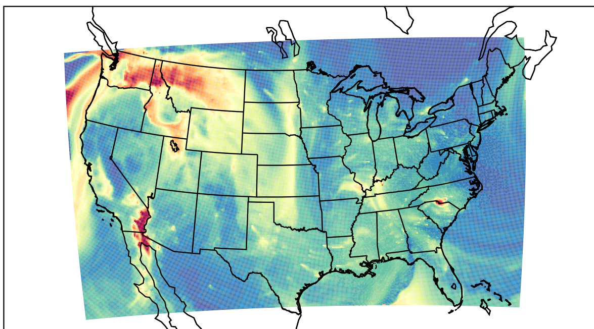
WRF 2021-10-28_14:00:00
