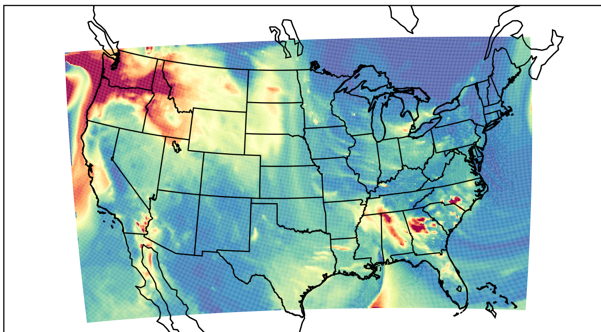
WRF 2021-10-28_06:00:00
