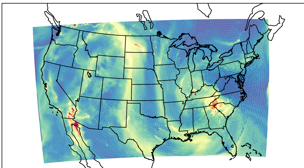
WRF 2021-10-29_08:00:00
