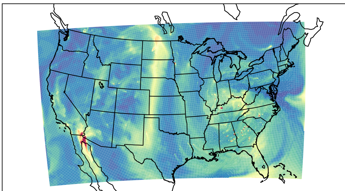
WRF 2021-10-29_17:00:00
