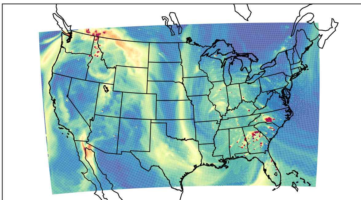
WRF 2021-10-28_21:00:00
