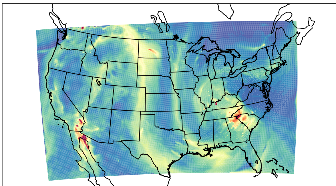
WRF 2021-10-29_07:00:00
