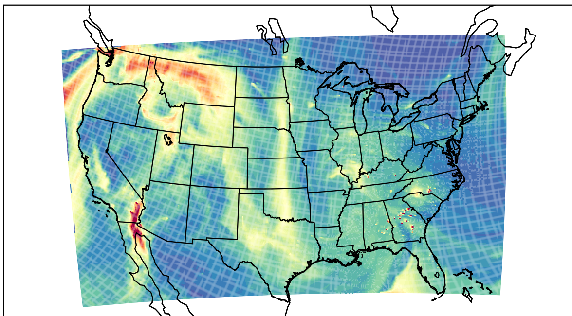
WRF 2021-10-28_17:00:00
