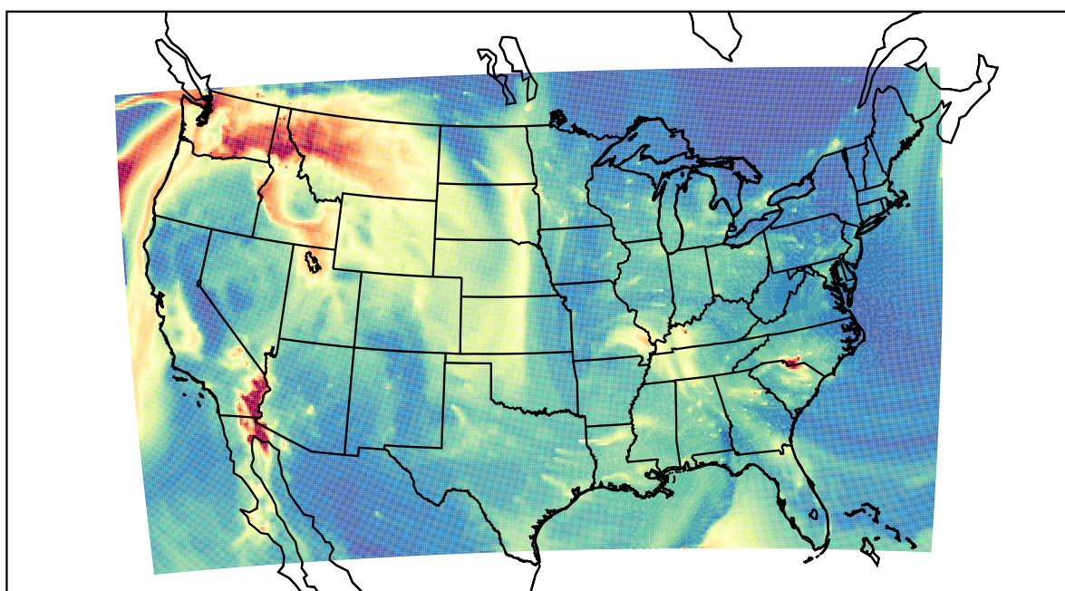
WRF 2021-10-28_13:00:00
