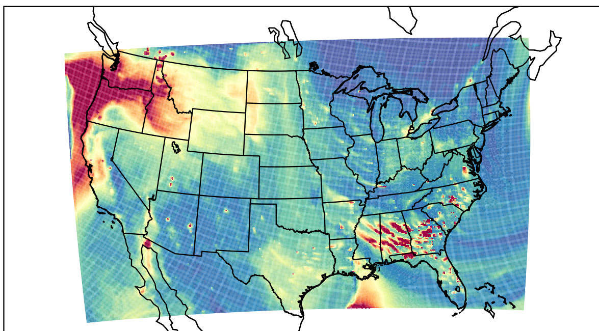
WRF 2021-10-28_01:00:00
