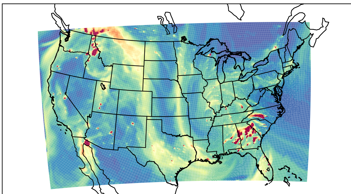
WRF 2021-10-29_00:00:00
