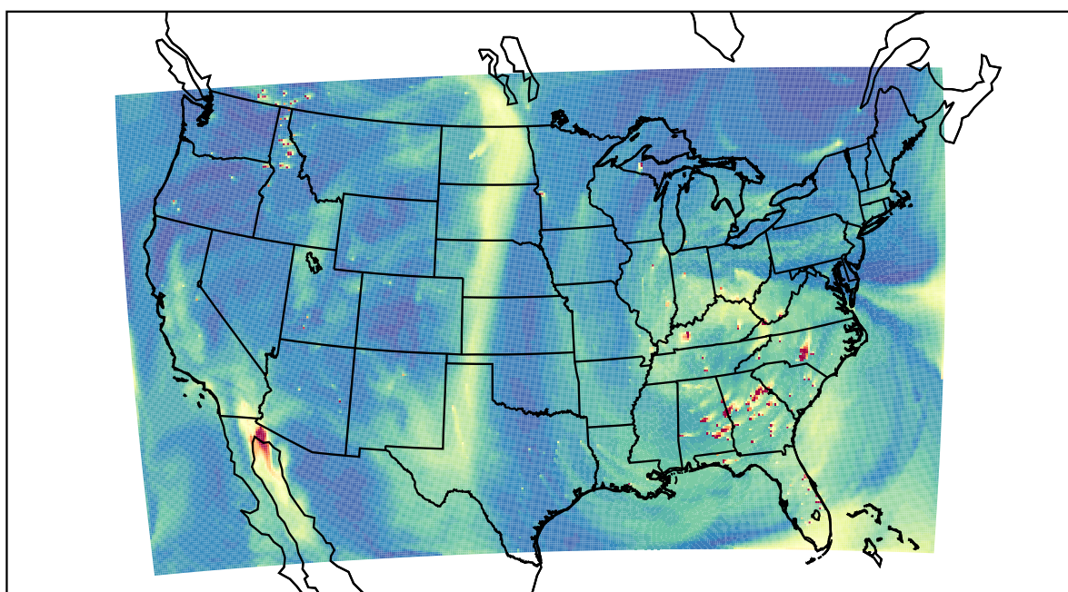
WRF 2021-10-29_20:00:00
