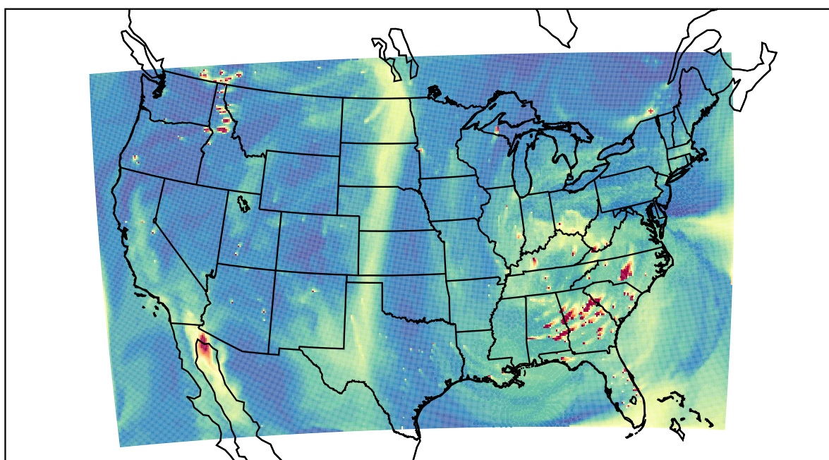
WRF 2021-10-29_22:00:00
