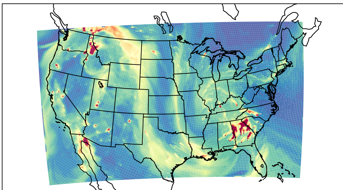
WRF 2021-10-29_02:00:00
