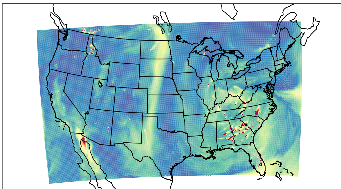
WRF 2021-10-29_21:00:00
