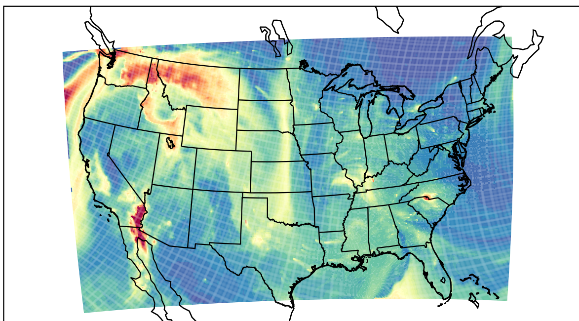
WRF 2021-10-28_15:00:00
