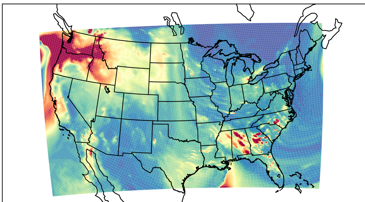
WRF 2021-10-28_04:00:00
