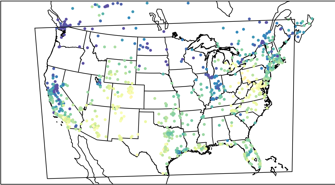
AirNOW (2021-11-11_20:00:00)
