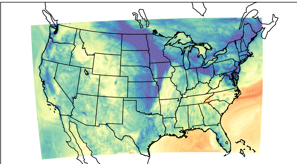
WRF (2021-11-11_04:00:00)
