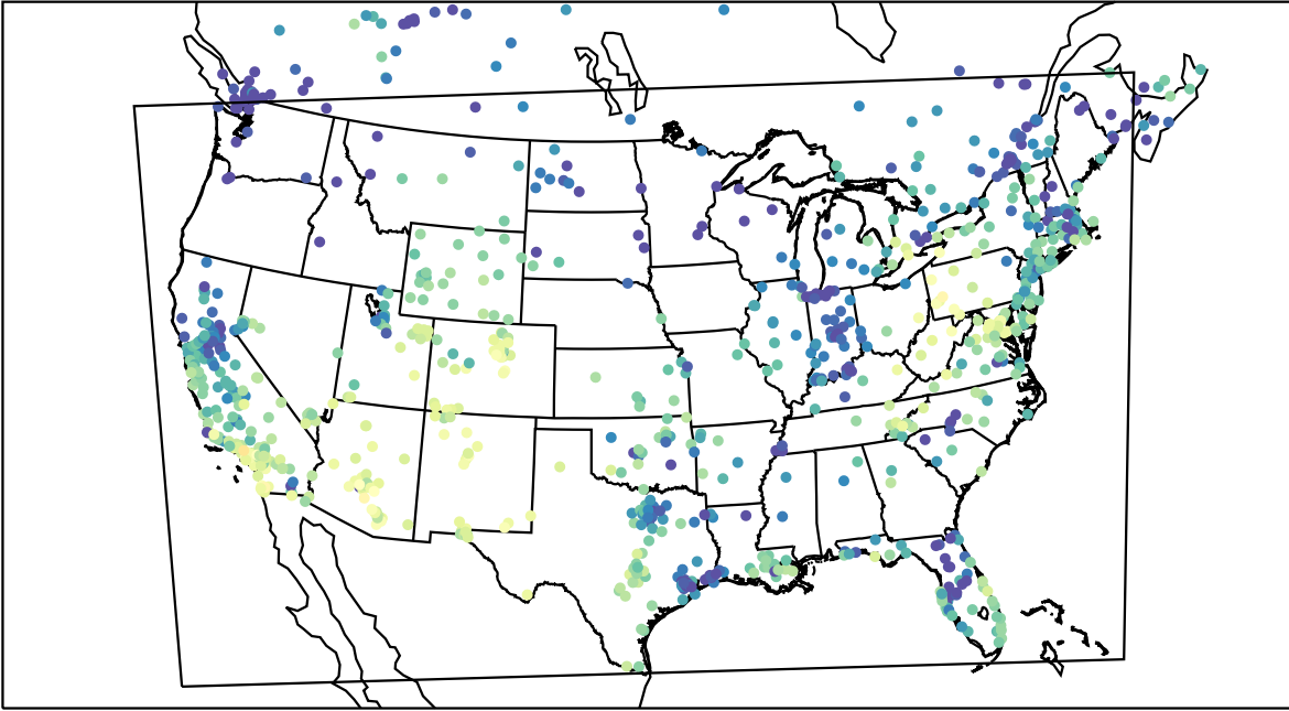
AirNOW (2021-11-11_23:00:00)
