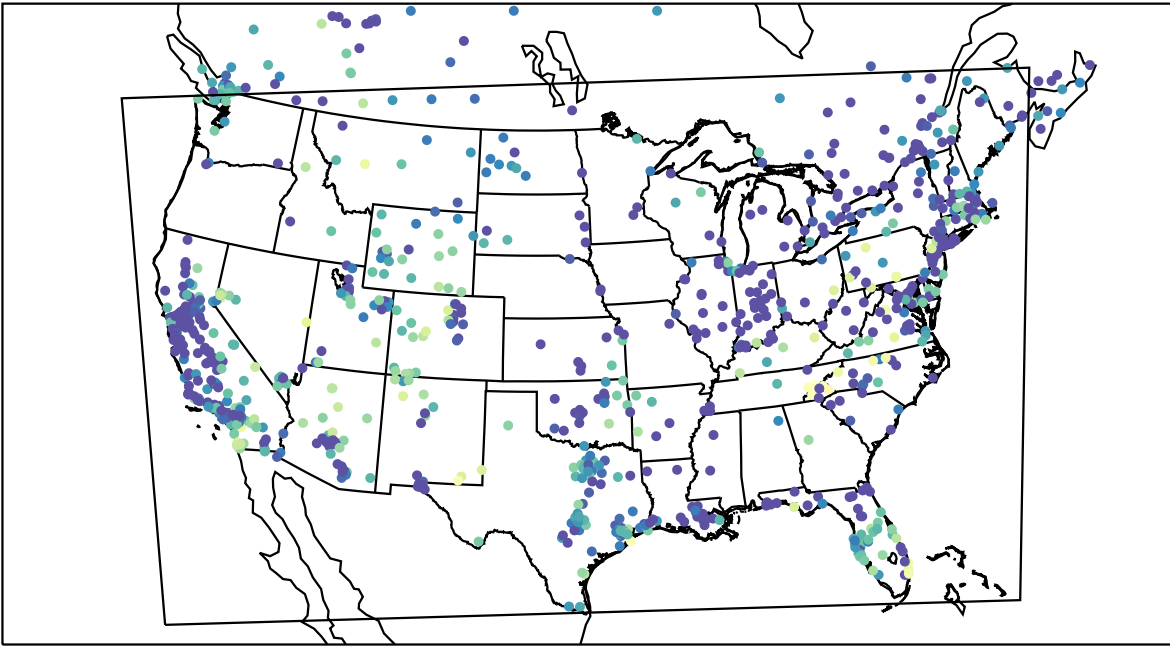
AirNOW (2021-11-10_04:00:00)
