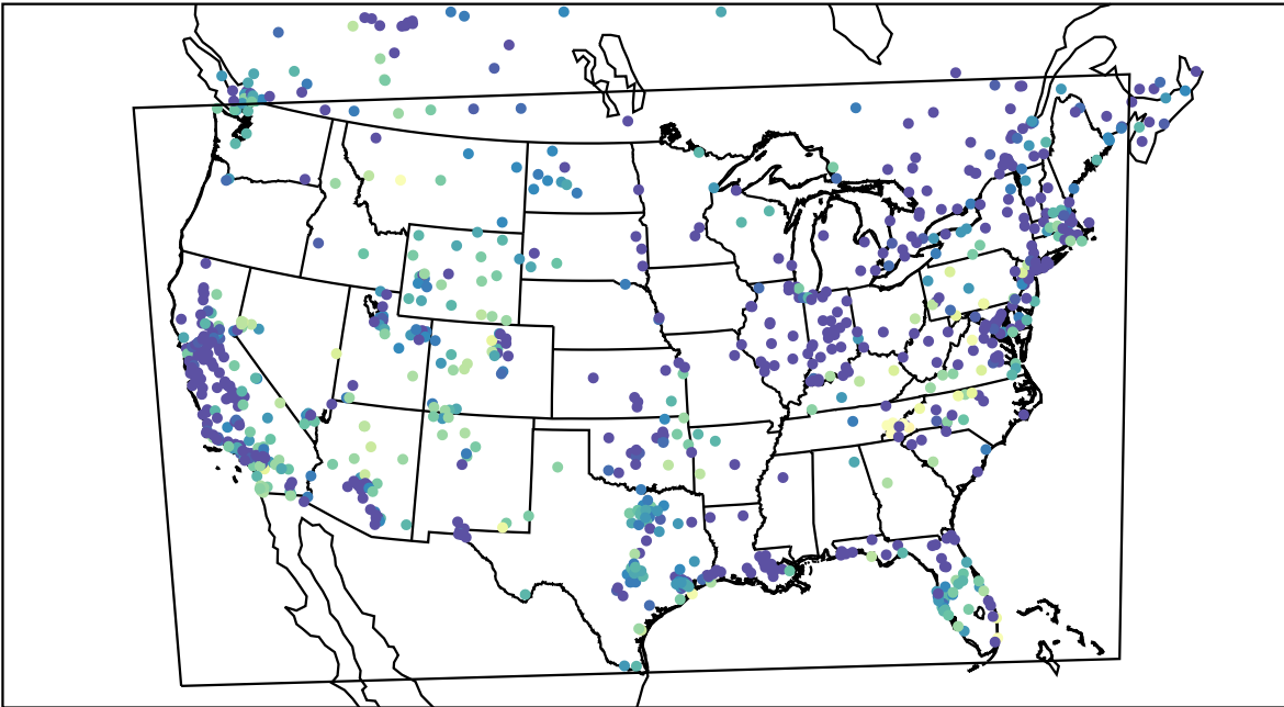
AirNOW (2021-11-10_05:00:00)
