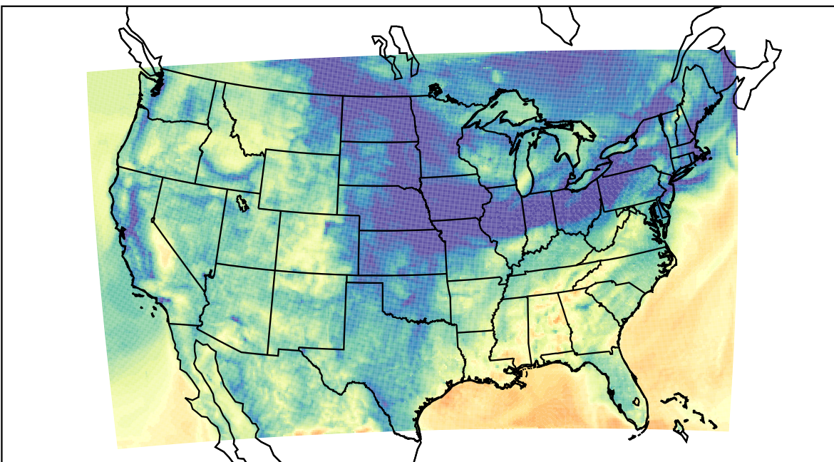
WRF (2021-11-10_08:00:00)
