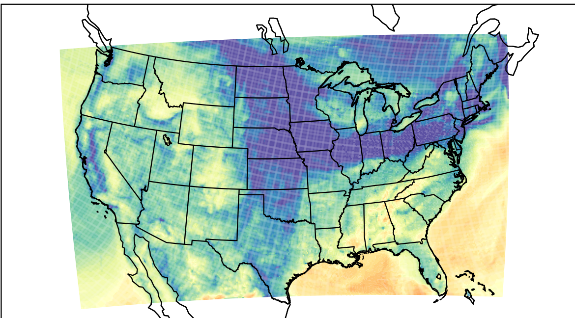
WRF (2021-11-10_11:00:00)
