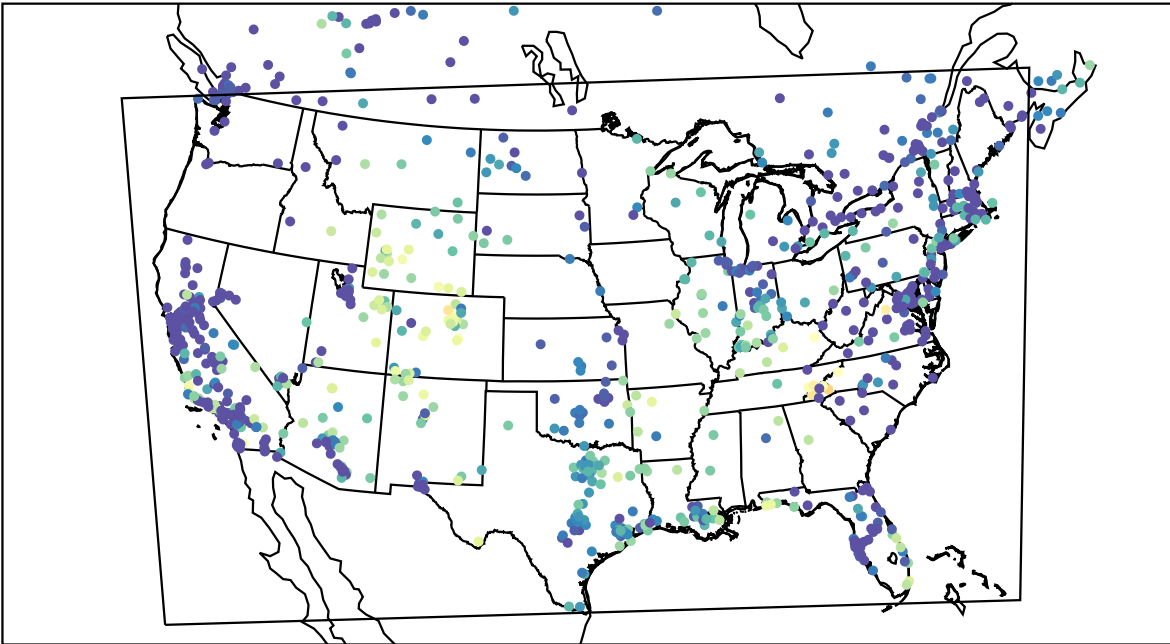
AirNOW (2021-11-11_05:00:00)
