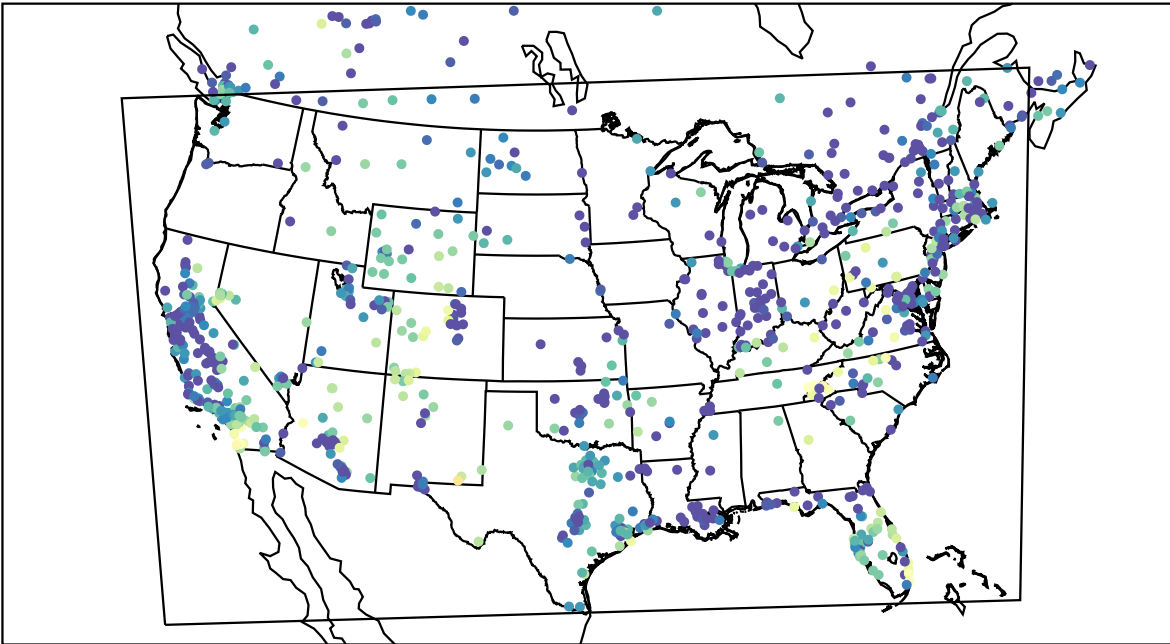
AirNOW (2021-11-10_02:00:00)
