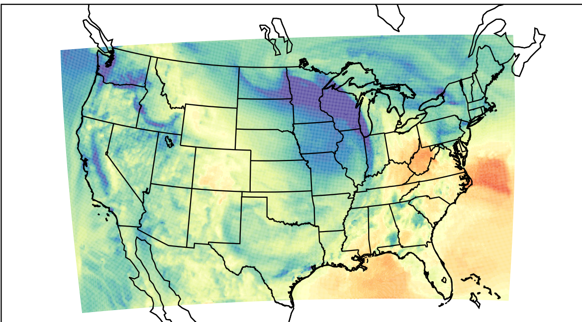
WRF (2021-11-11_17:00:00)
