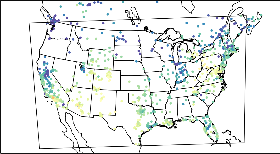
AirNOW (2021-11-11_21:00:00)
