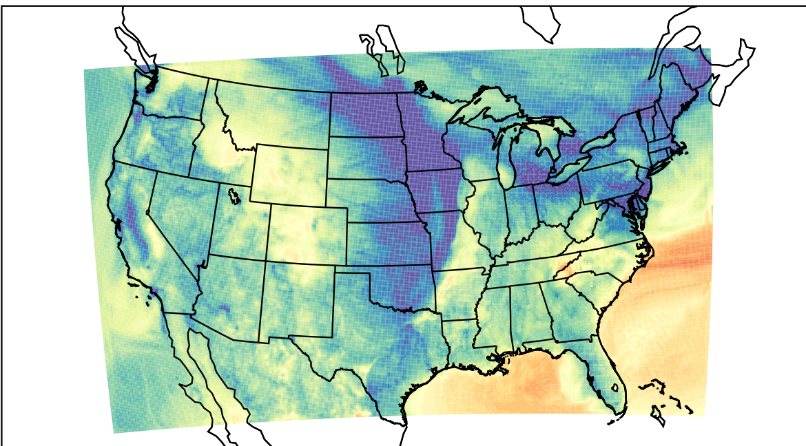
WRF (2021-11-11_07:00:00)
