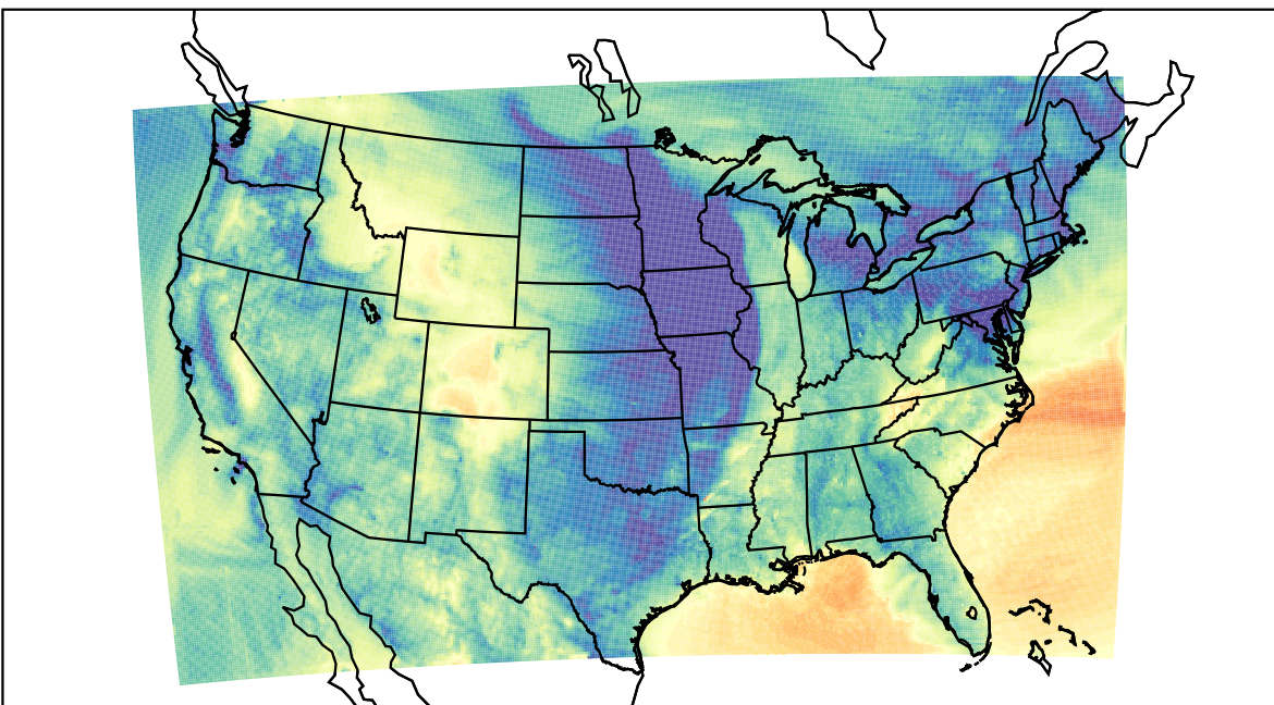
WRF (2021-11-11_11:00:00)
