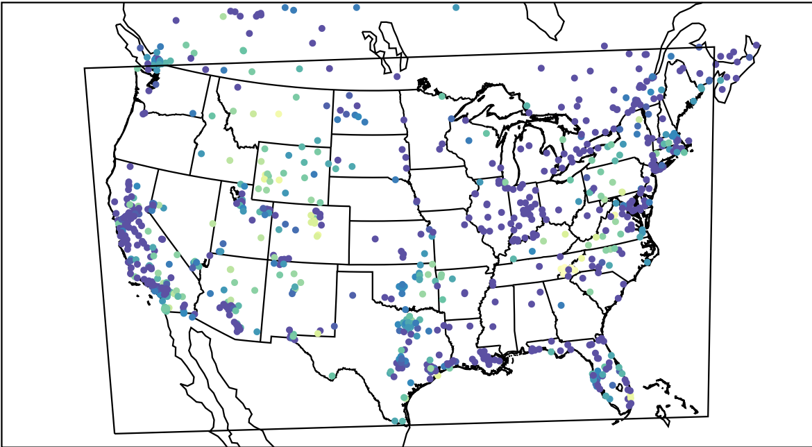
AirNOW (2021-11-10_09:00:00)
