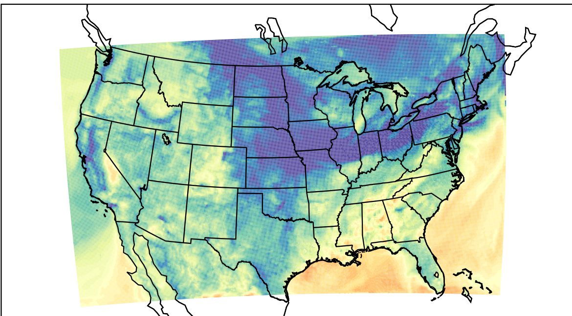
WRF (2021-11-10_07:00:00)
