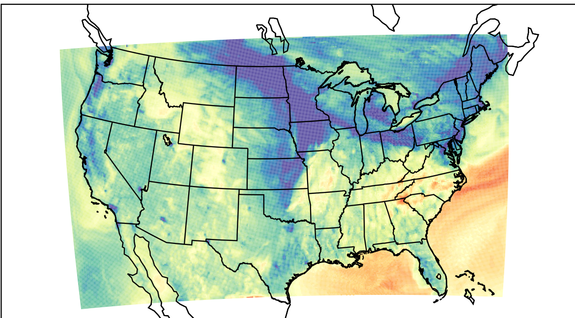
WRF (2021-11-11_02:00:00)
