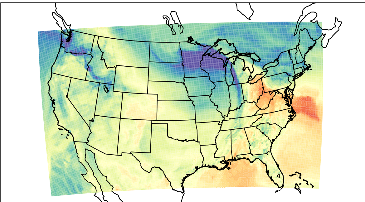
WRF (2021-11-11_20:00:00)
