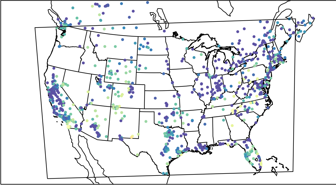
AirNOW (2021-11-10_03:00:00)
