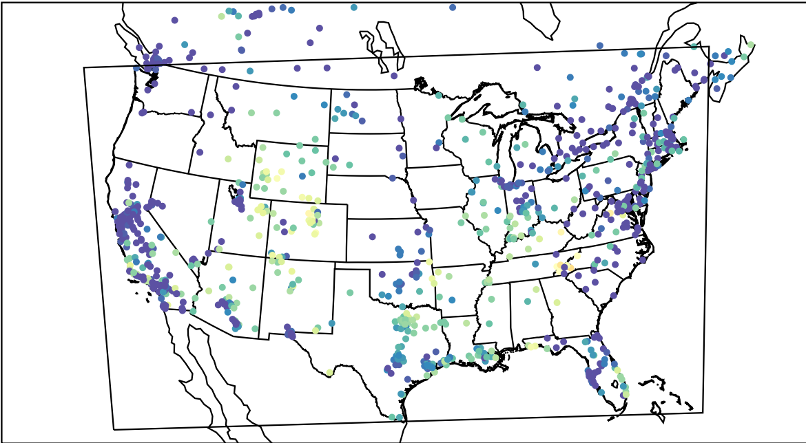
AirNOW (2021-11-11_04:00:00)
