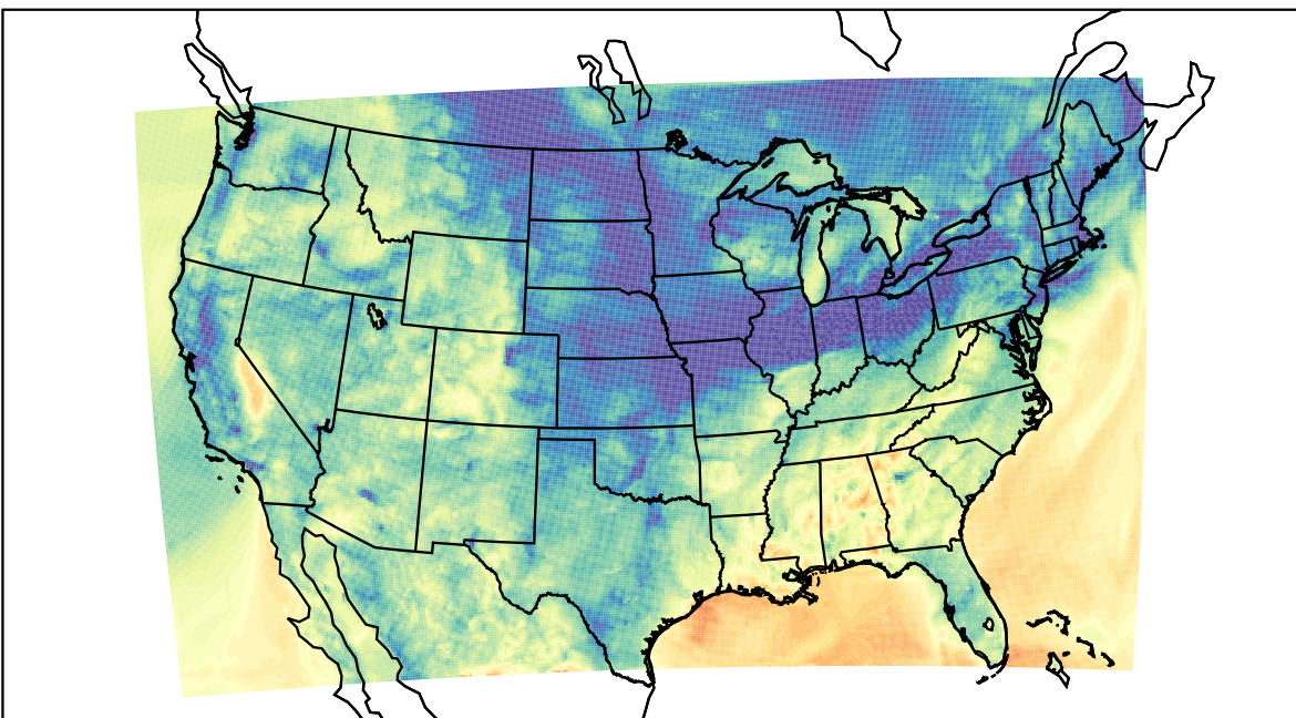
WRF (2021-11-10_05:00:00)
