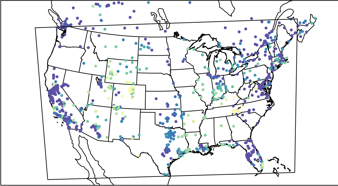
AirNOW (2021-11-11_08:00:00)
