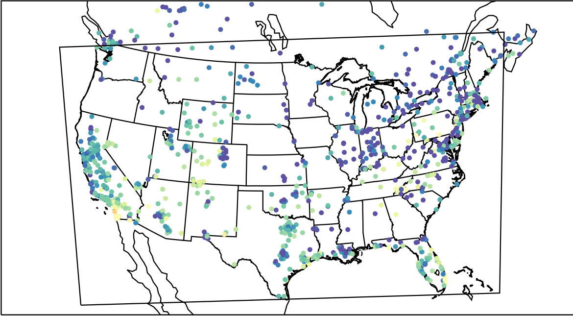
AirNOW (2021-11-10_00:00:00)
