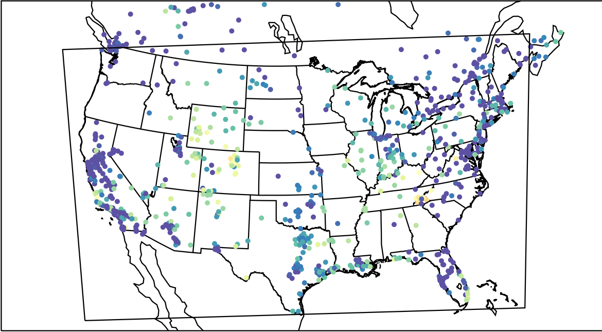
AirNOW (2021-11-11_06:00:00)
