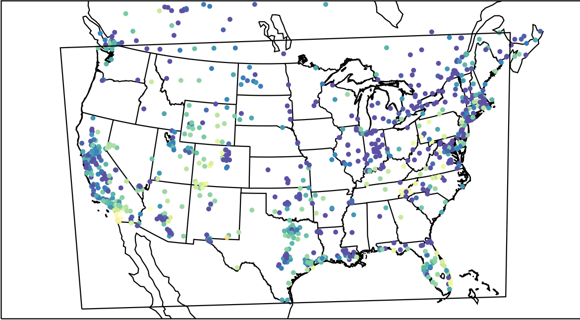
AirNOW (2021-11-10_01:00:00)
