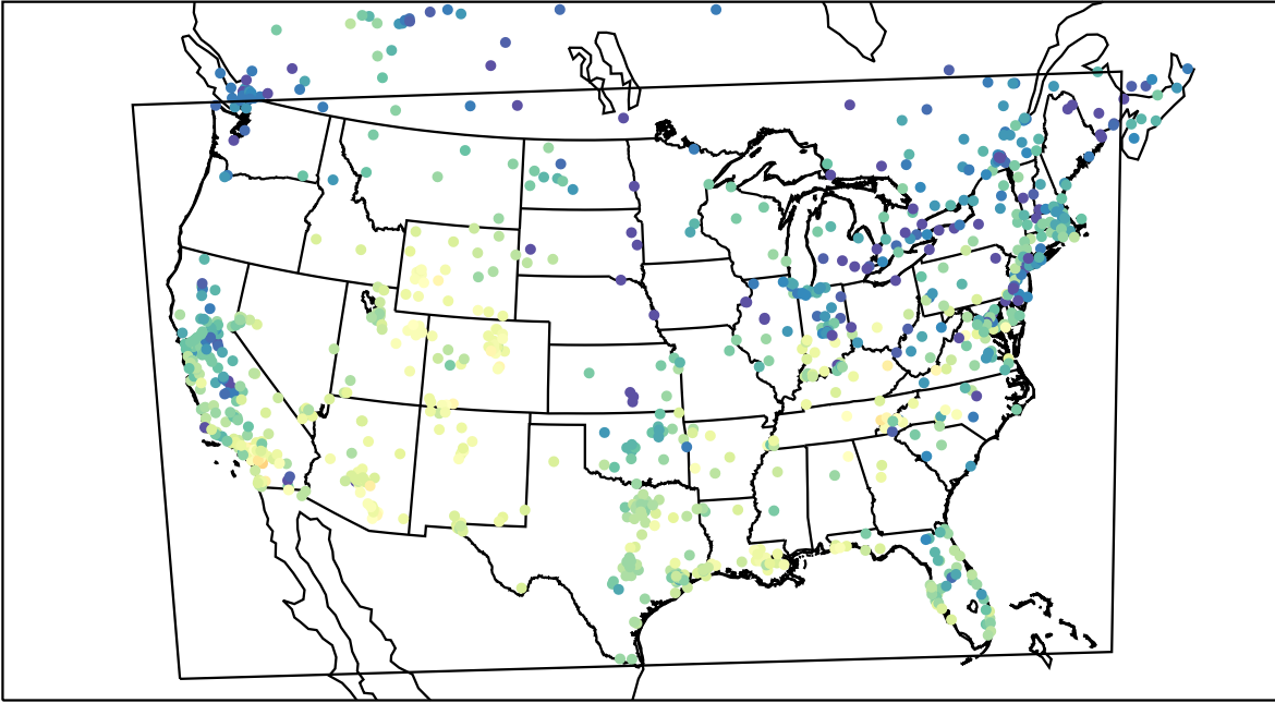
AirNOW (2021-11-10_22:00:00)
