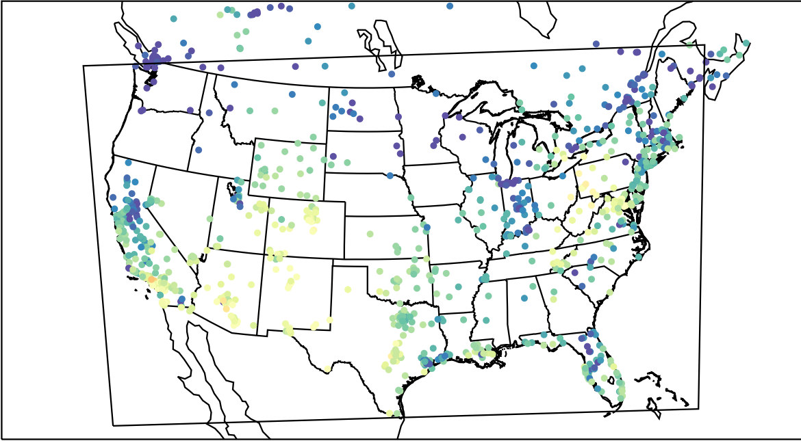
AirNOW (2021-11-11_22:00:00)
