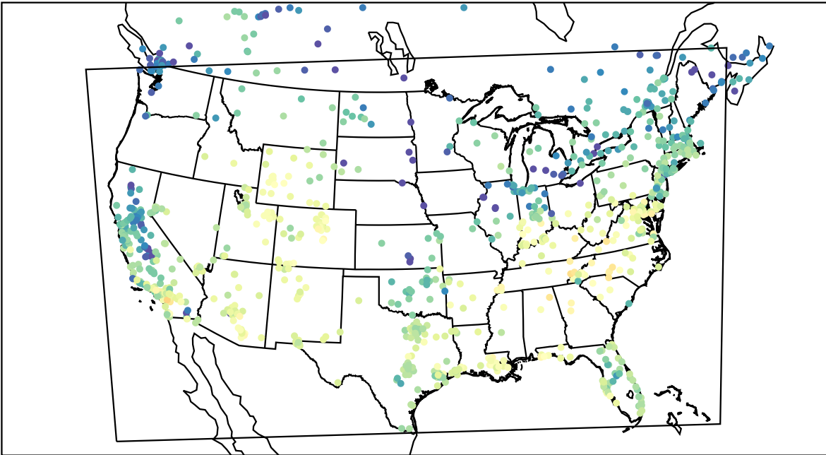
AirNOW (2021-11-10_21:00:00)
