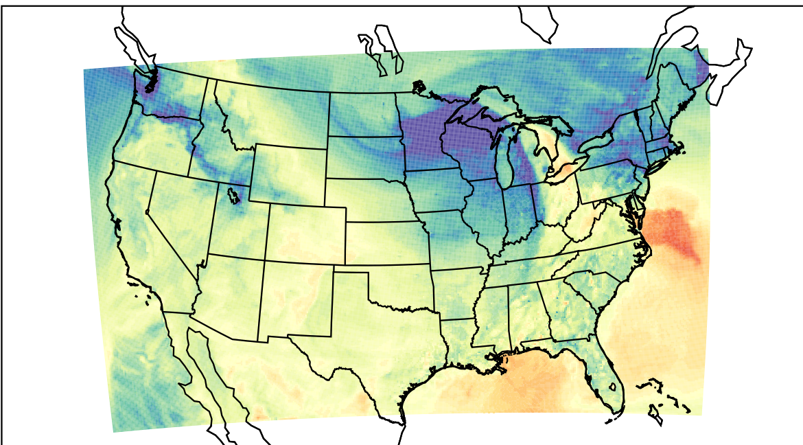
WRF (2021-11-11_22:00:00)
