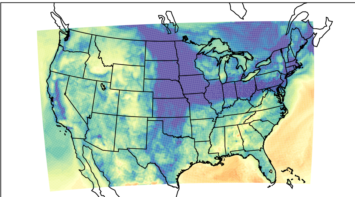
WRF (2021-11-10_13:00:00)
