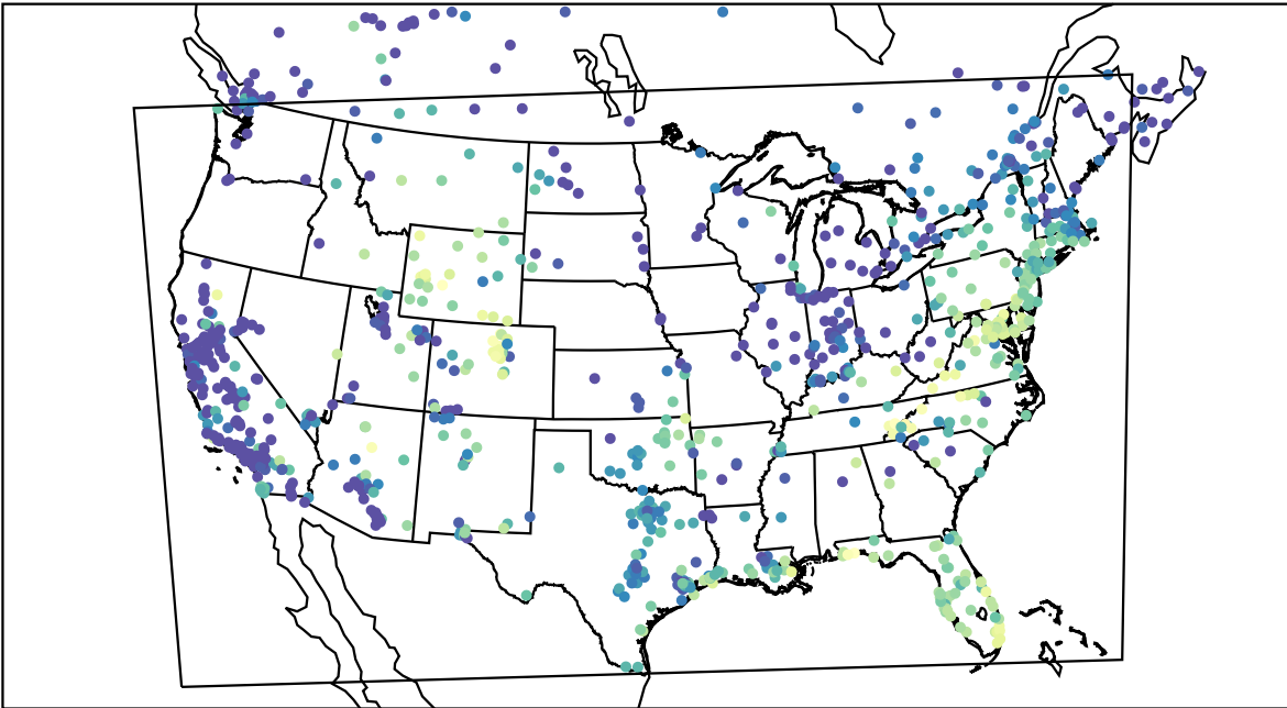
AirNOW (2021-11-10_15:00:00)
