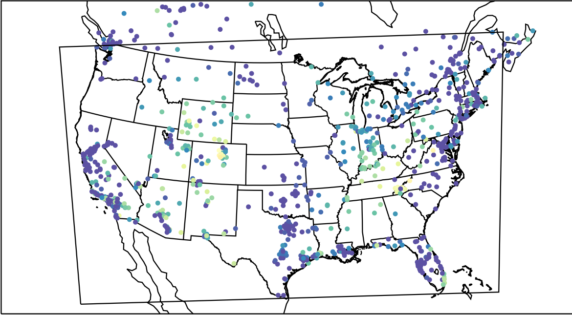
AirNOW (2021-11-11_12:00:00)
