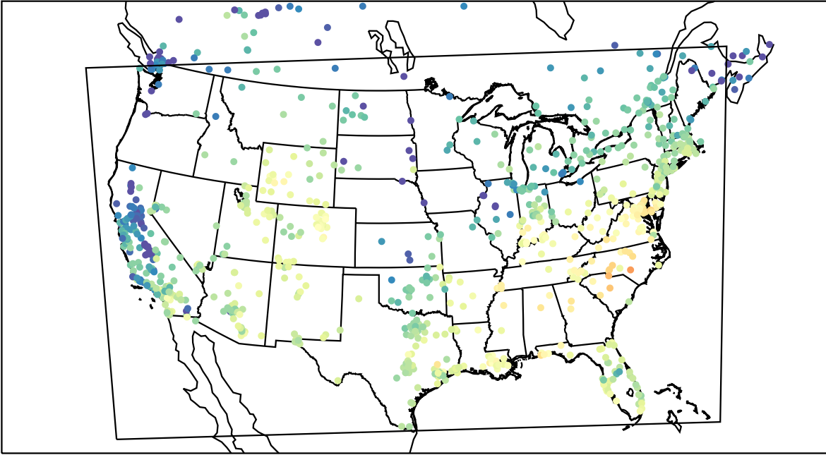
AirNOW (2021-11-10_19:00:00)
