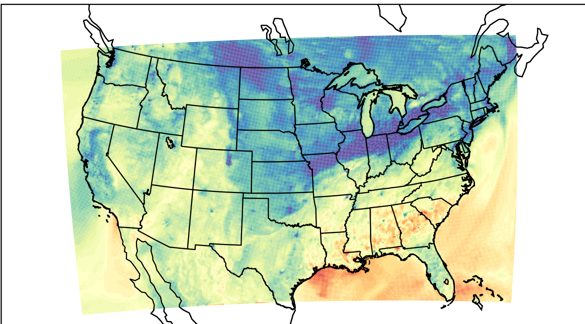
WRF (2021-11-10_00:00:00)
