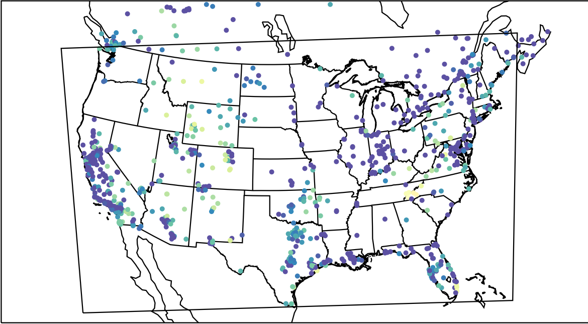
AirNOW (2021-11-10_08:00:00)
