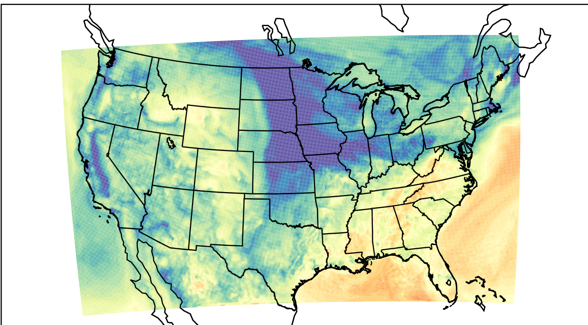
WRF (2021-11-10_16:00:00)
