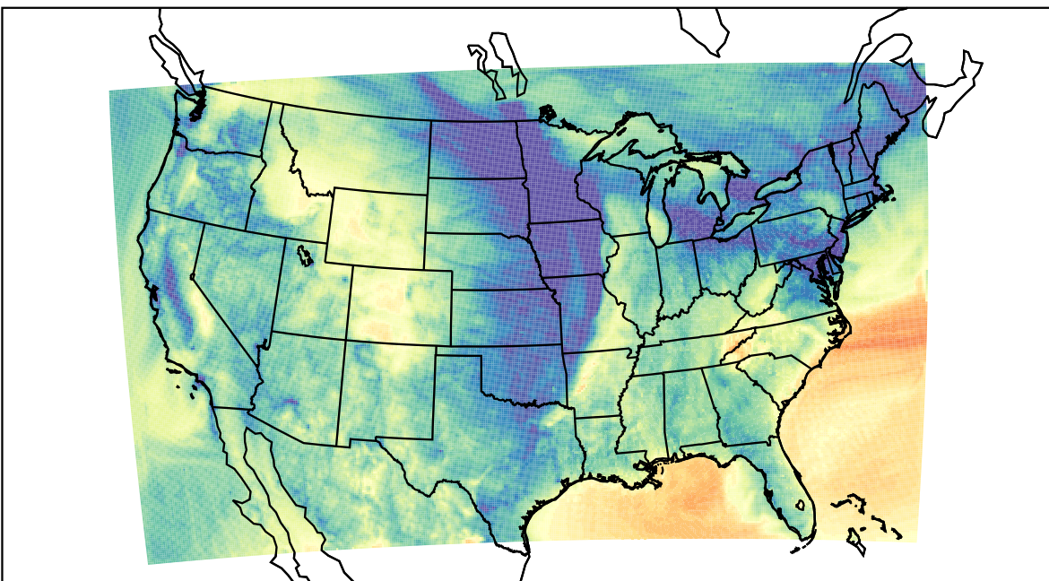
WRF (2021-11-11_08:00:00)
