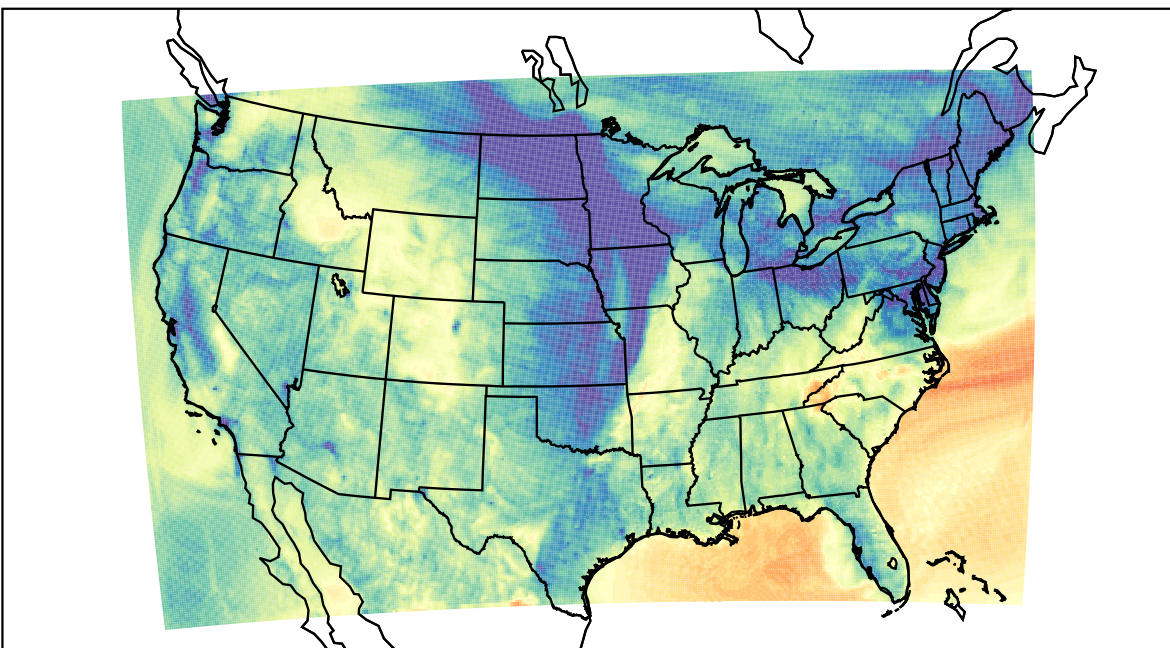
WRF (2021-11-11_05:00:00)
