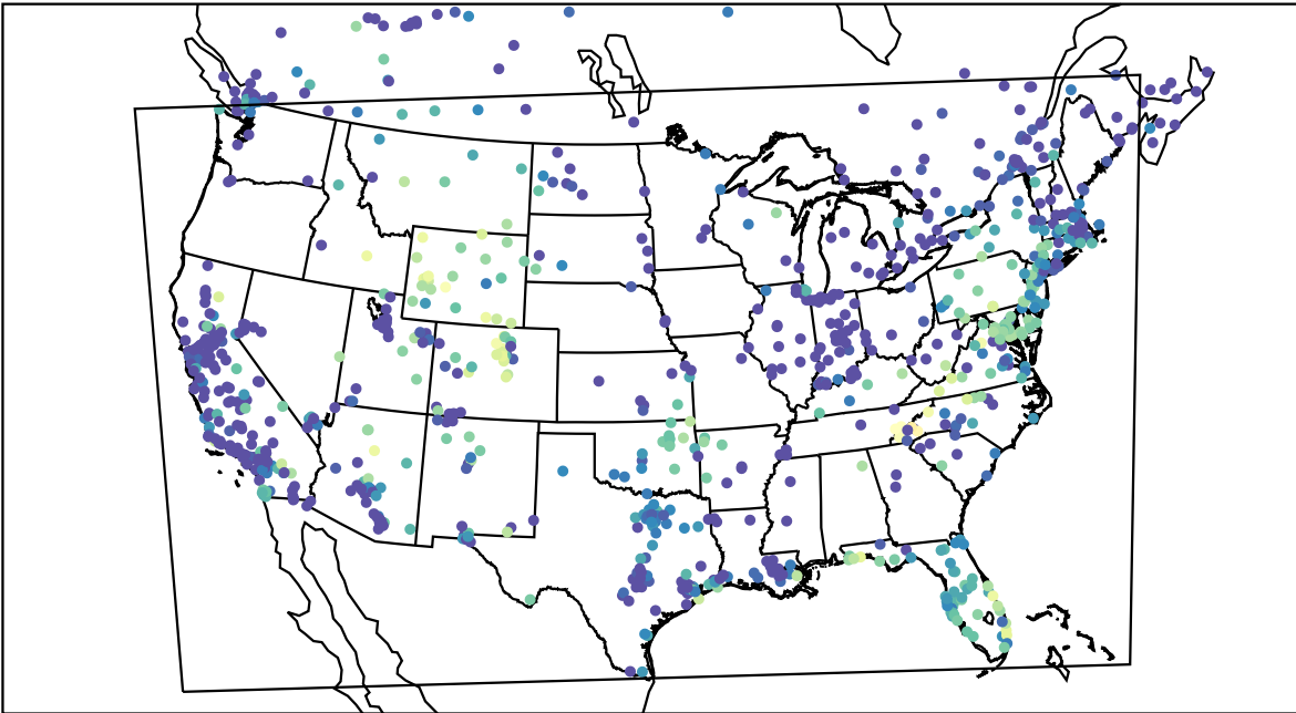
AirNOW (2021-11-10_14:00:00)
