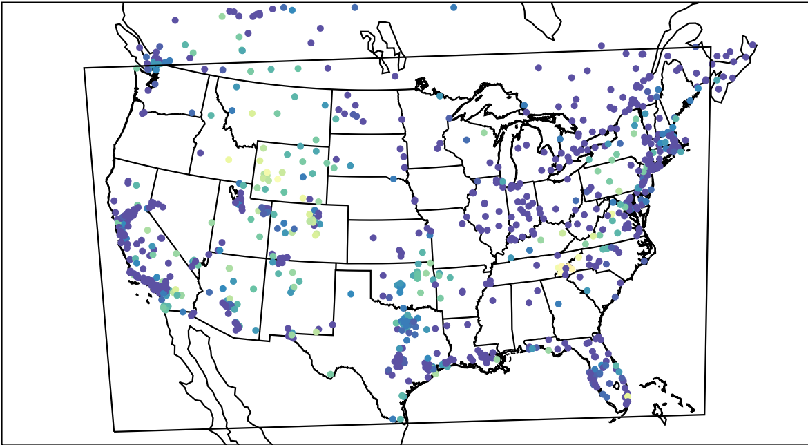
AirNOW (2021-11-10_12:00:00)
