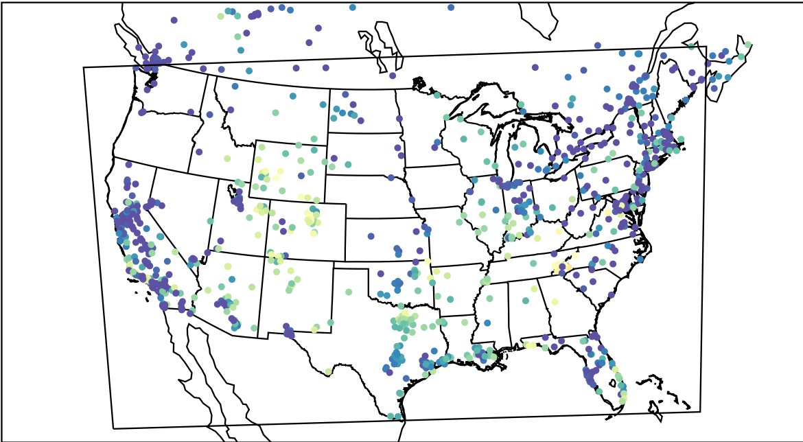
AirNOW (2021-11-11_03:00:00)
