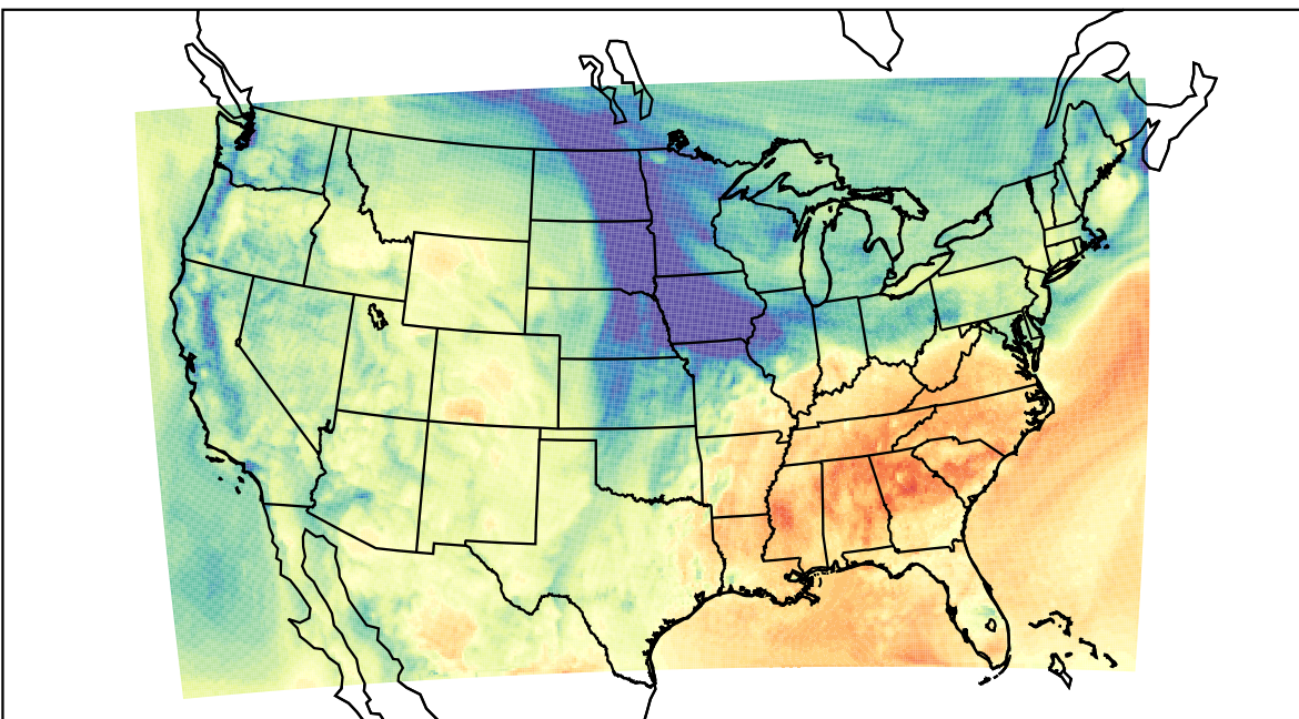
WRF (2021-11-10_18:00:00)
