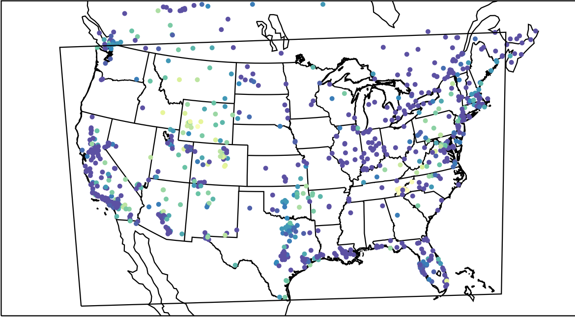
AirNOW (2021-11-10_11:00:00)
