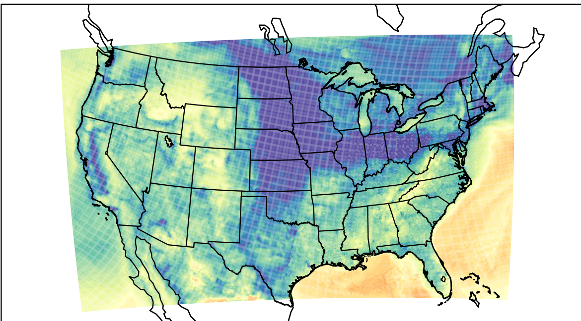
WRF (2021-11-10_14:00:00)
