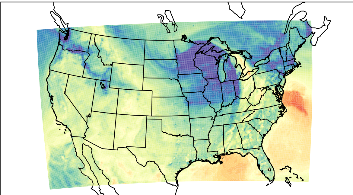
WRF (2021-11-11_23:00:00)
