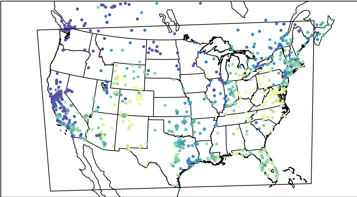
AirNOW (2021-11-11_17:00:00)
