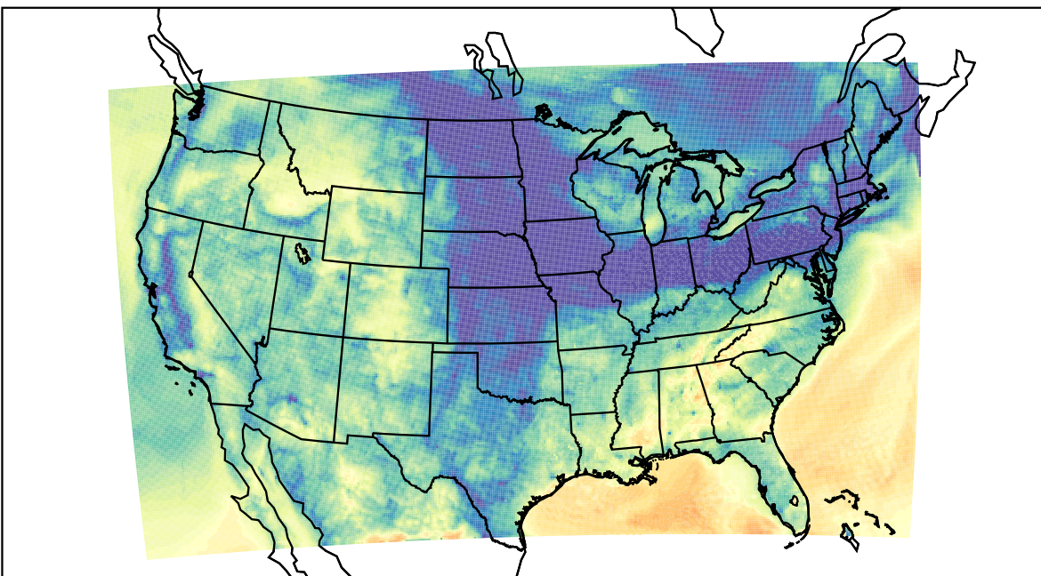
WRF (2021-11-10_12:00:00)
