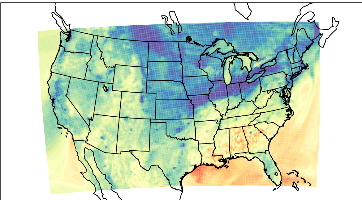
WRF (2021-11-10_01:00:00)
