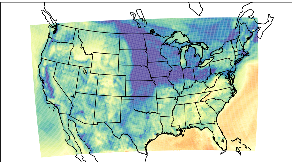
WRF (2021-11-10_15:00:00)
