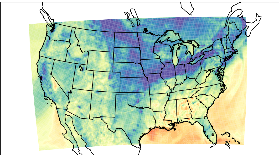
WRF (2021-11-10_03:00:00)
