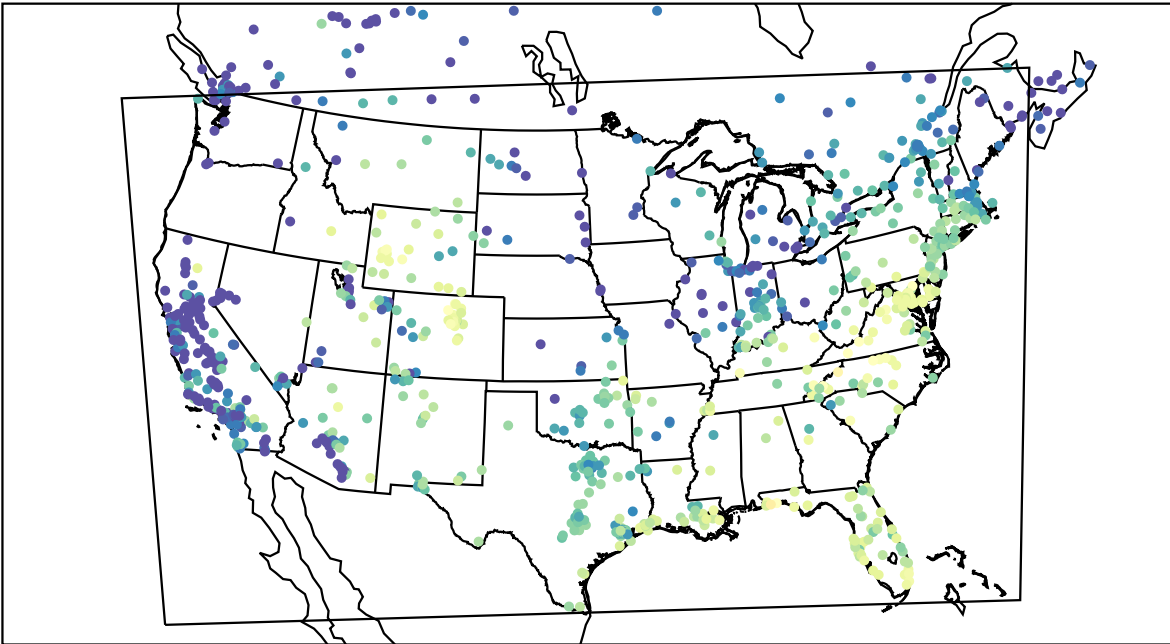
AirNOW (2021-11-10_16:00:00)
