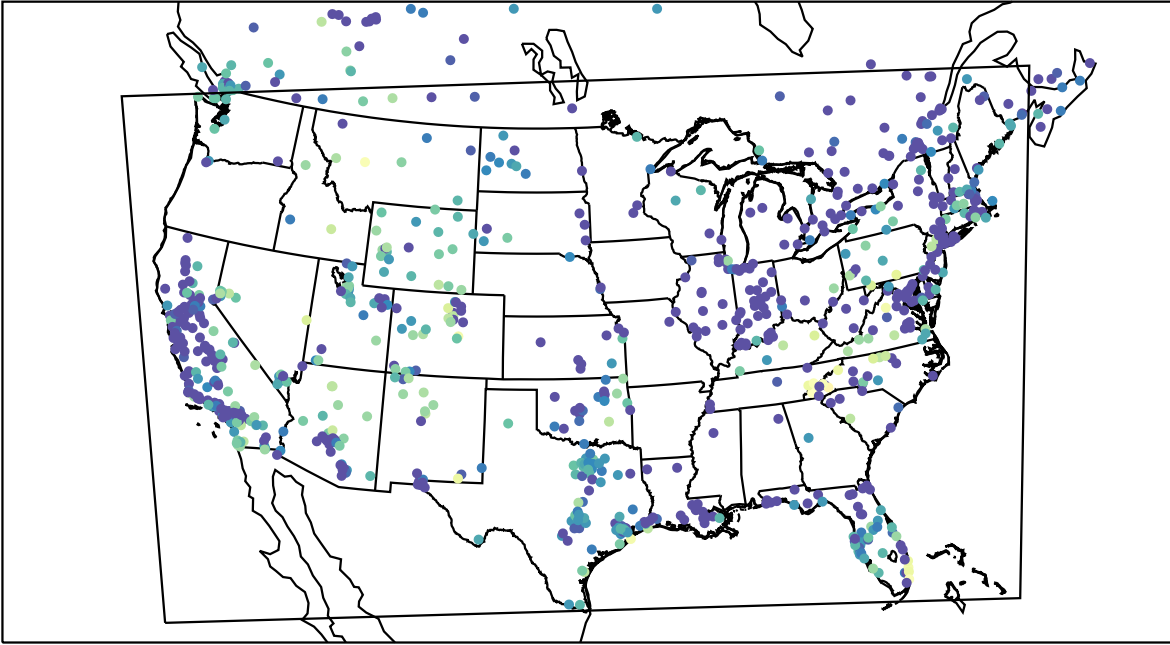
AirNOW (2021-11-10_06:00:00)
