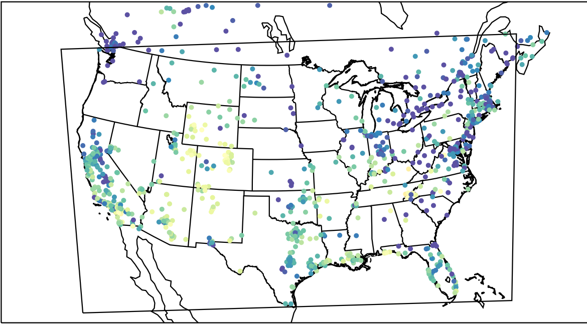
AirNOW (2021-11-11_00:00:00)
