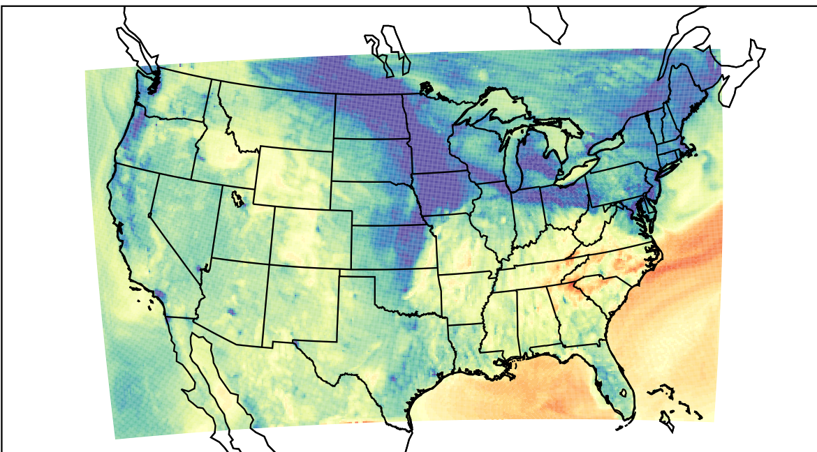
WRF (2021-11-11_01:00:00)
