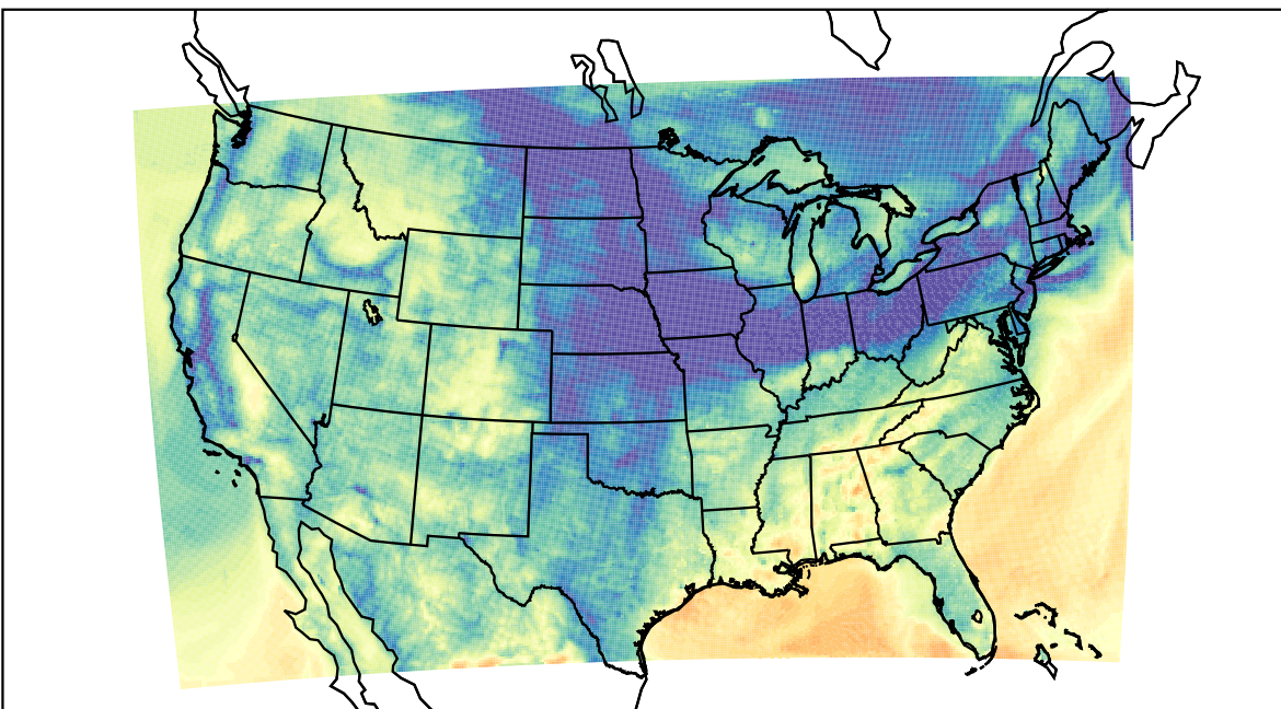
WRF (2021-11-10_09:00:00)
