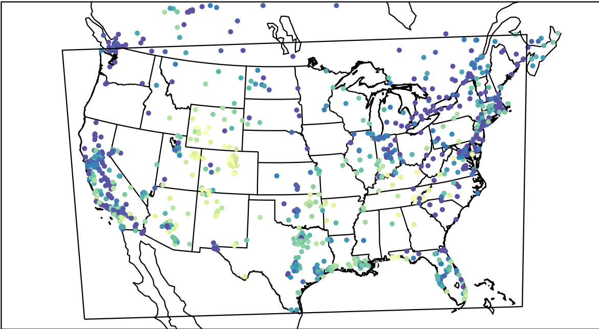
AirNOW (2021-11-11_01:00:00)
