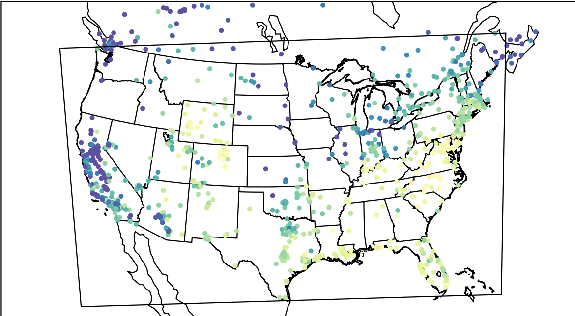
AirNOW (2021-11-10_17:00:00)
