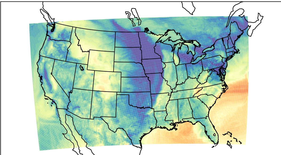
WRF (2021-11-11_09:00:00)
