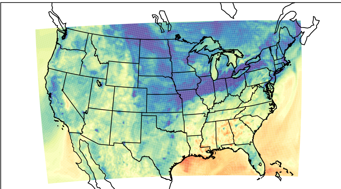
WRF (2021-11-10_02:00:00)
