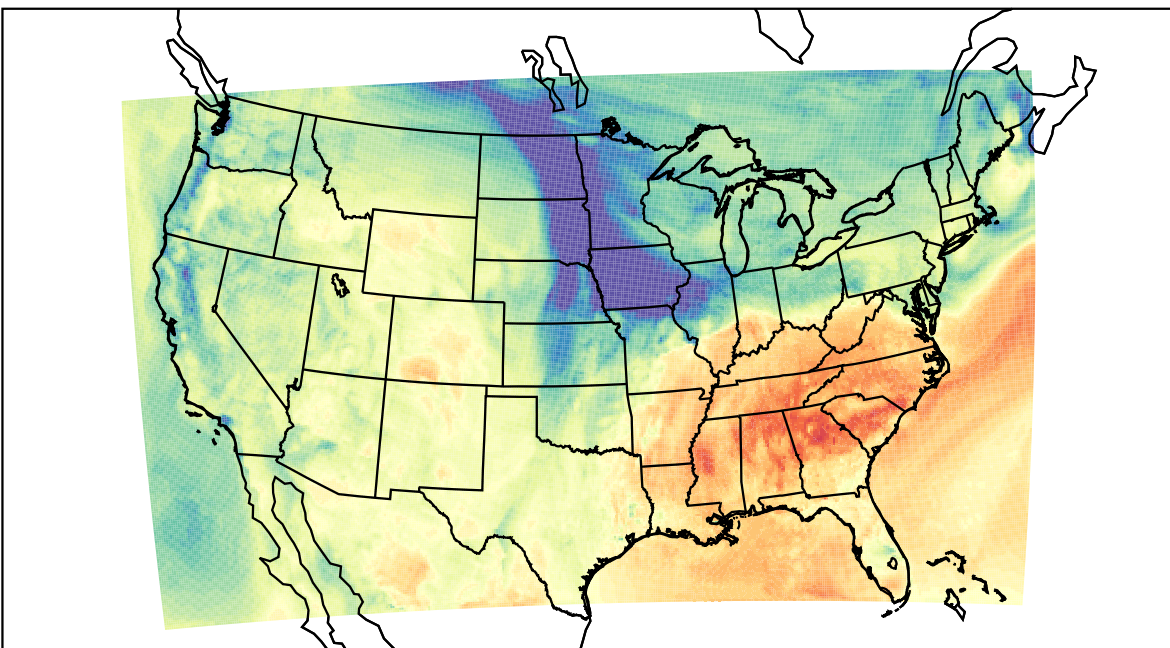
WRF (2021-11-10_19:00:00)
