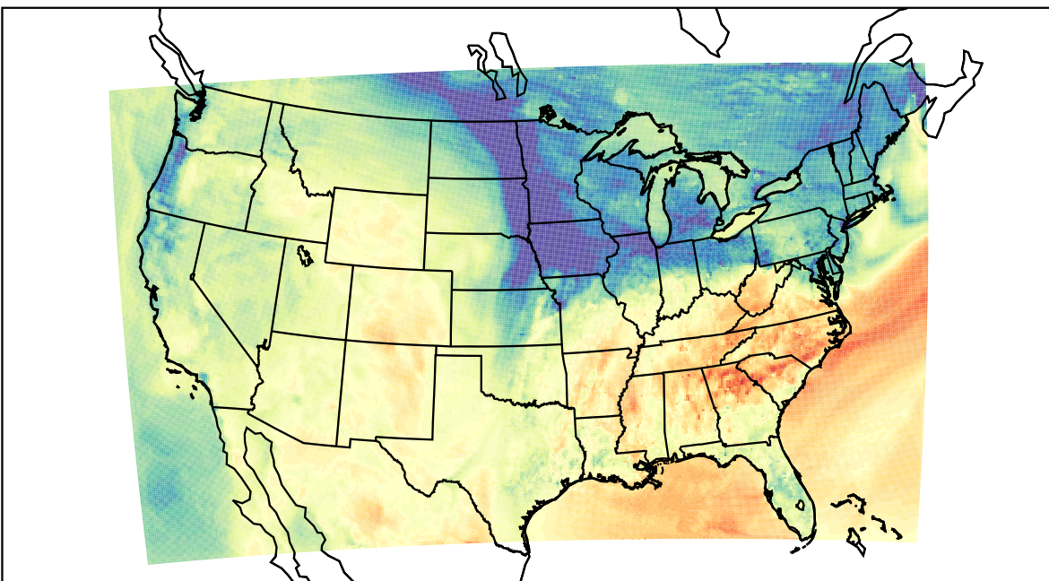
WRF (2021-11-10_22:00:00)
