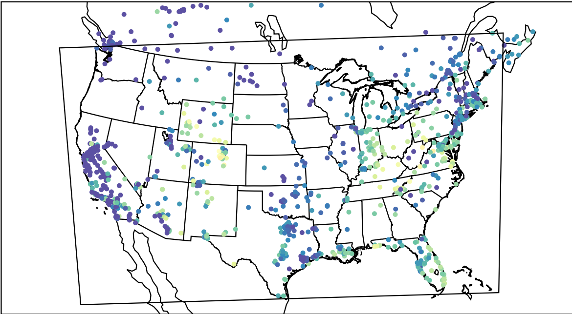
AirNOW (2021-11-11_15:00:00)
