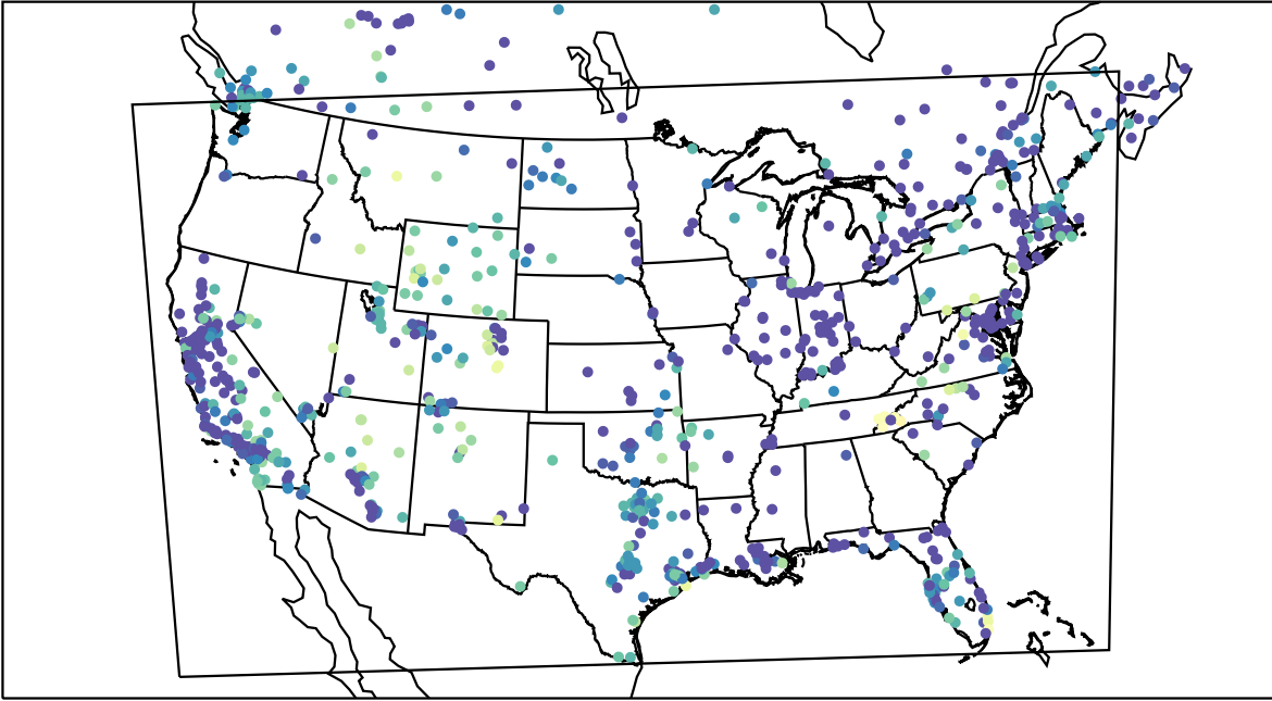
AirNOW (2021-11-10_07:00:00)
