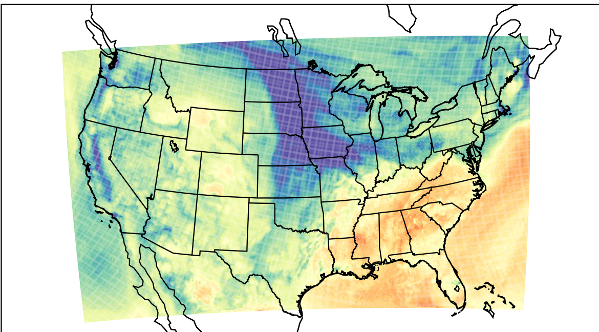
WRF (2021-11-10_17:00:00)
