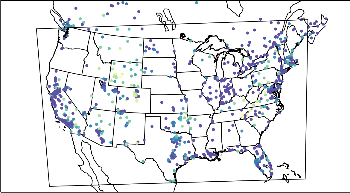
AirNOW (2021-11-10_10:00:00)
