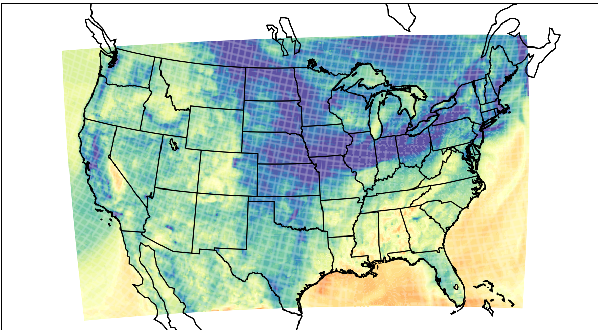
WRF (2021-11-10_06:00:00)
