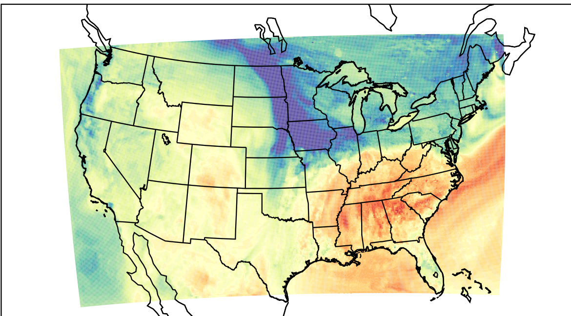
WRF (2021-11-10_21:00:00)
