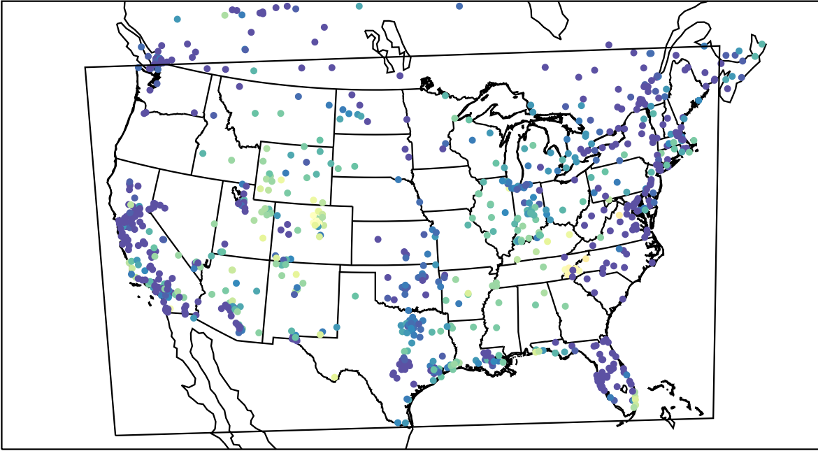
AirNOW (2021-11-11_09:00:00)
