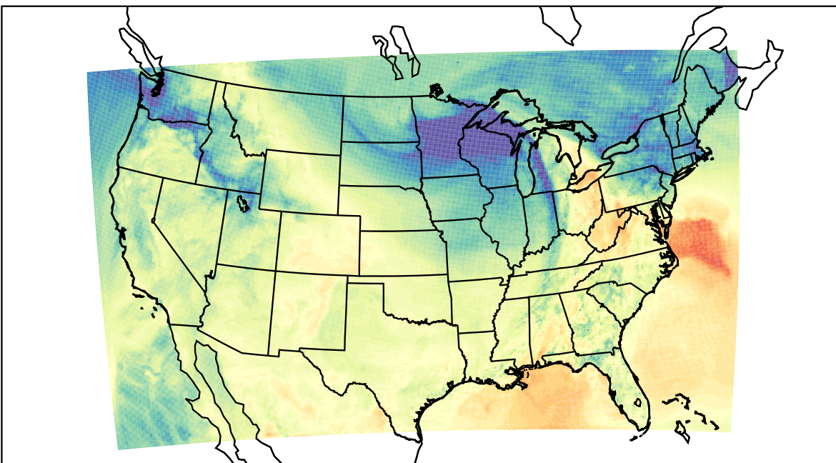
WRF (2021-11-11_21:00:00)
