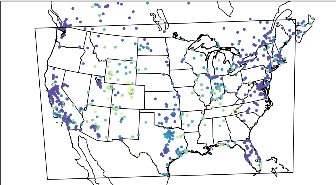
AirNOW (2021-11-11_07:00:00)
