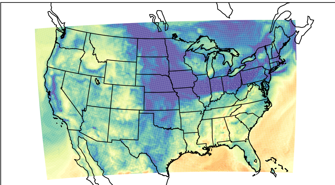
WRF (2021-11-10_10:00:00)
