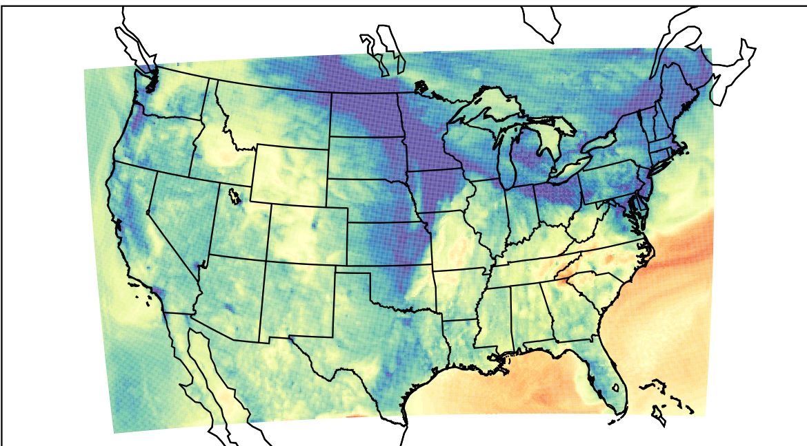
WRF (2021-11-11_03:00:00)
