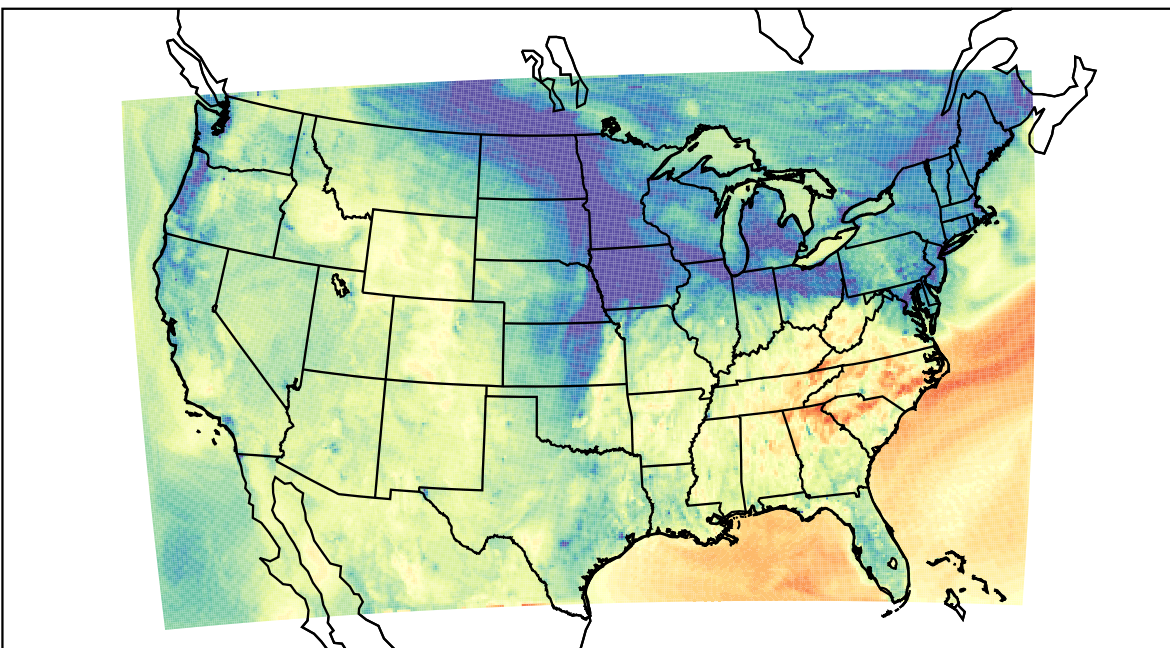
WRF (2021-11-11_00:00:00)
