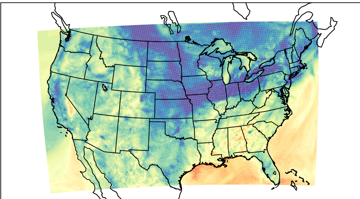
WRF (2021-11-10_04:00:00)
