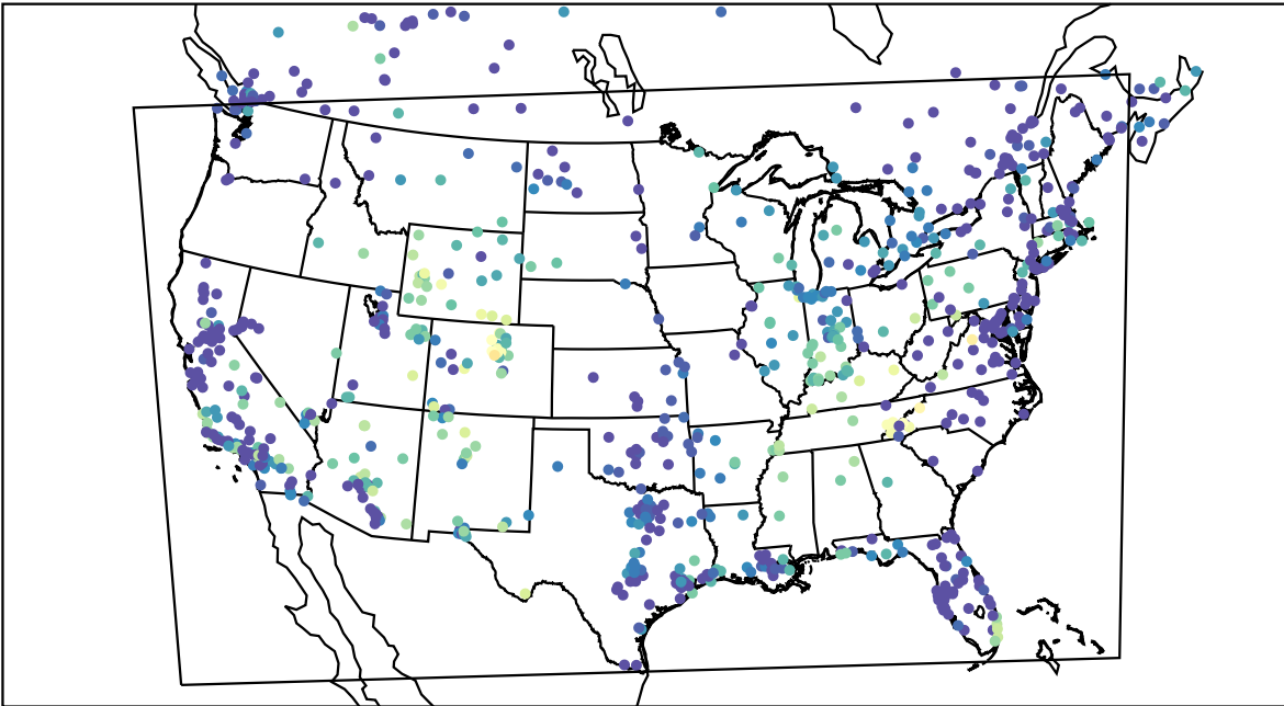
AirNOW (2021-11-11_11:00:00)
