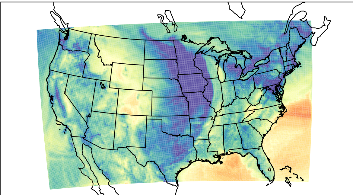
WRF (2021-11-11_12:00:00)
