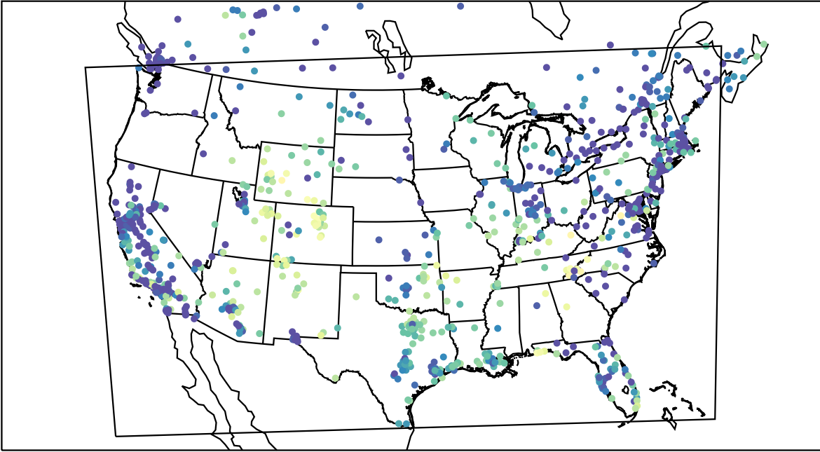
AirNOW (2021-11-11_02:00:00)
