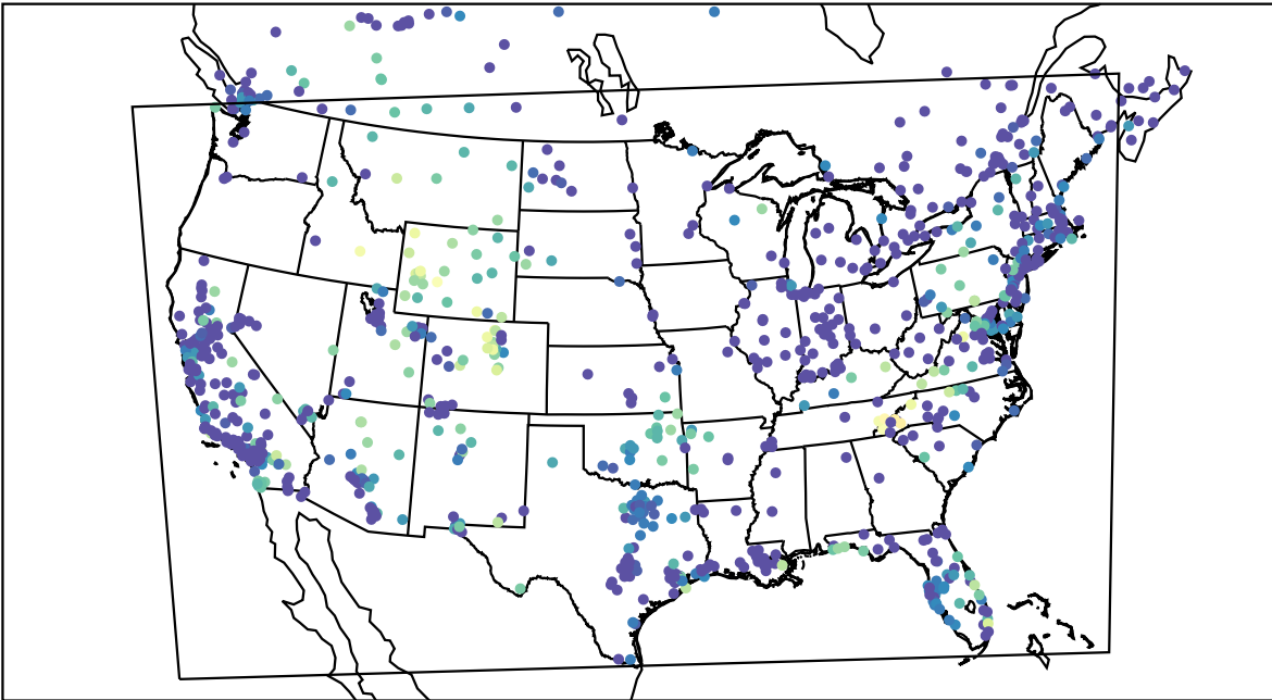
AirNOW (2021-11-10_13:00:00)
