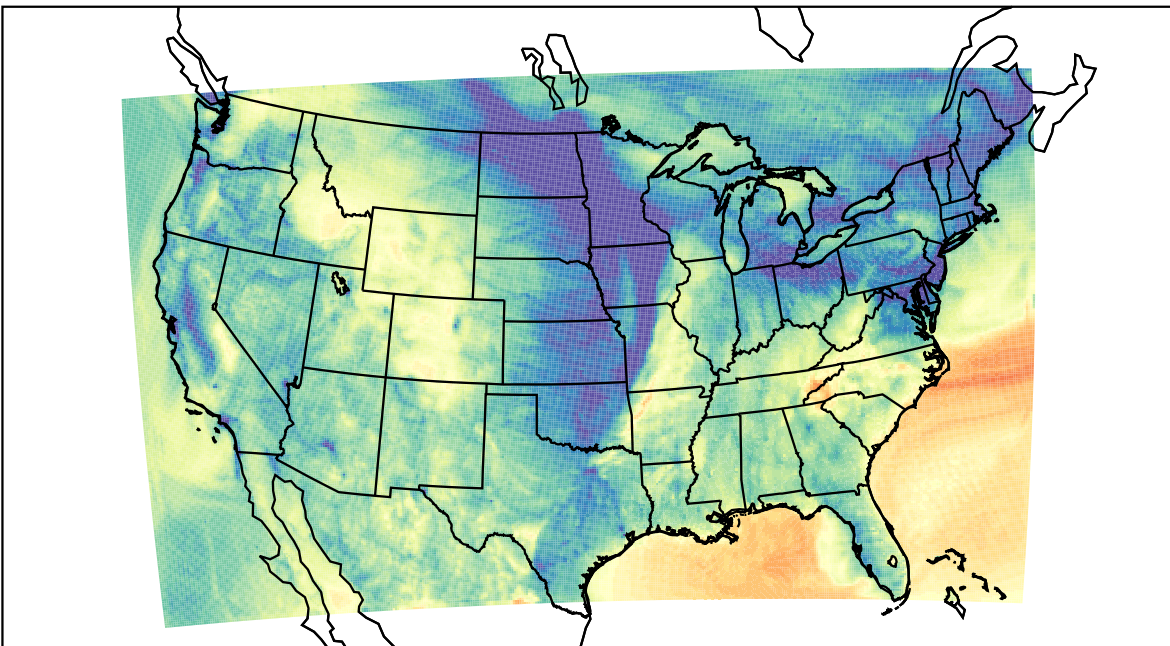
WRF (2021-11-11_06:00:00)
