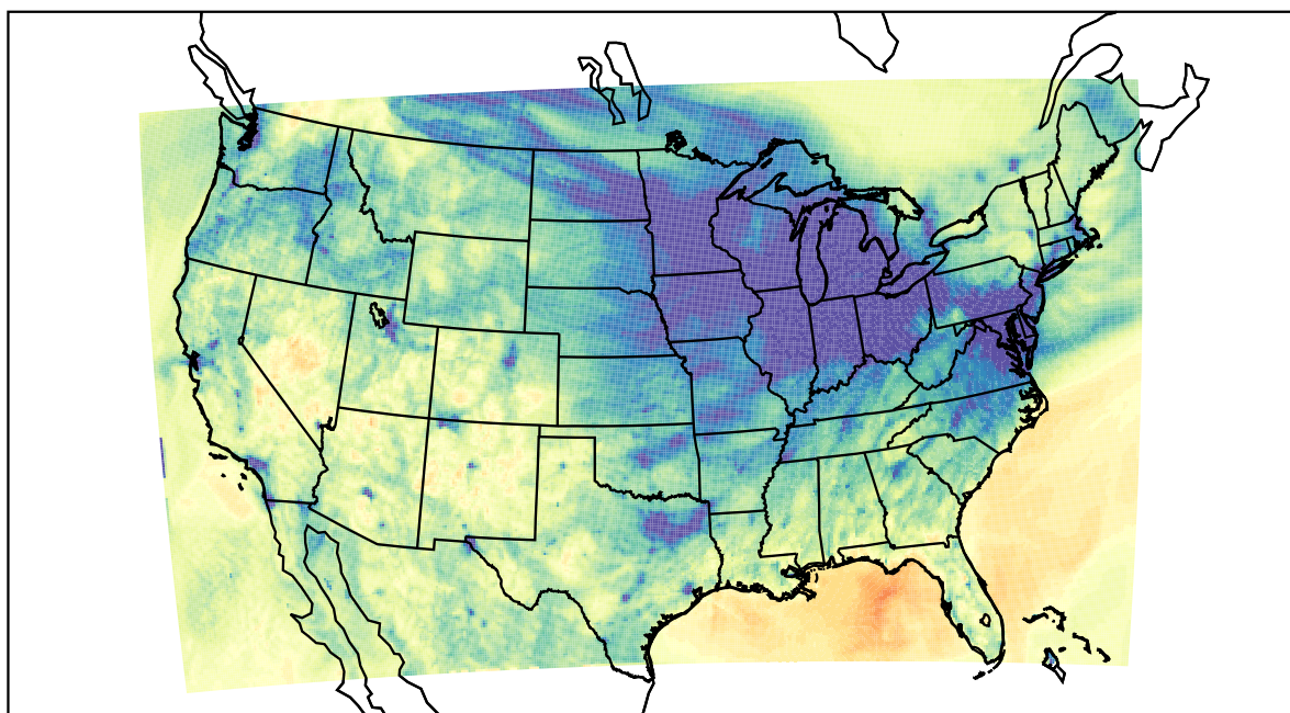
WRF (2021-12-02_01:00:00)
