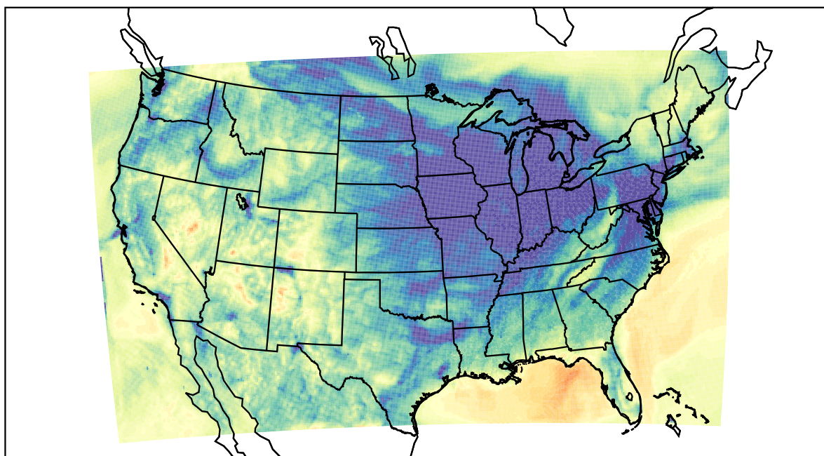
WRF (2021-12-02_06:00:00)
