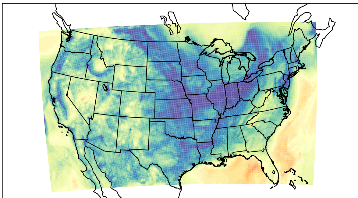
WRF (2021-12-02_16:00:00)
