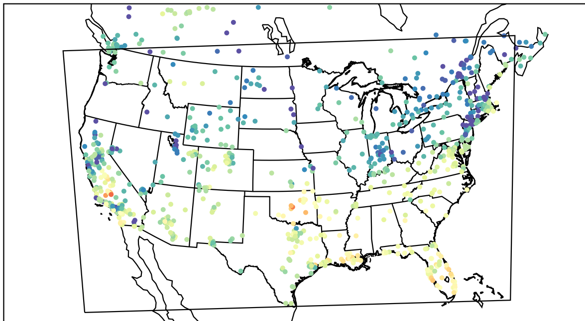
AirNOW (2021-12-02_21:00:00)
