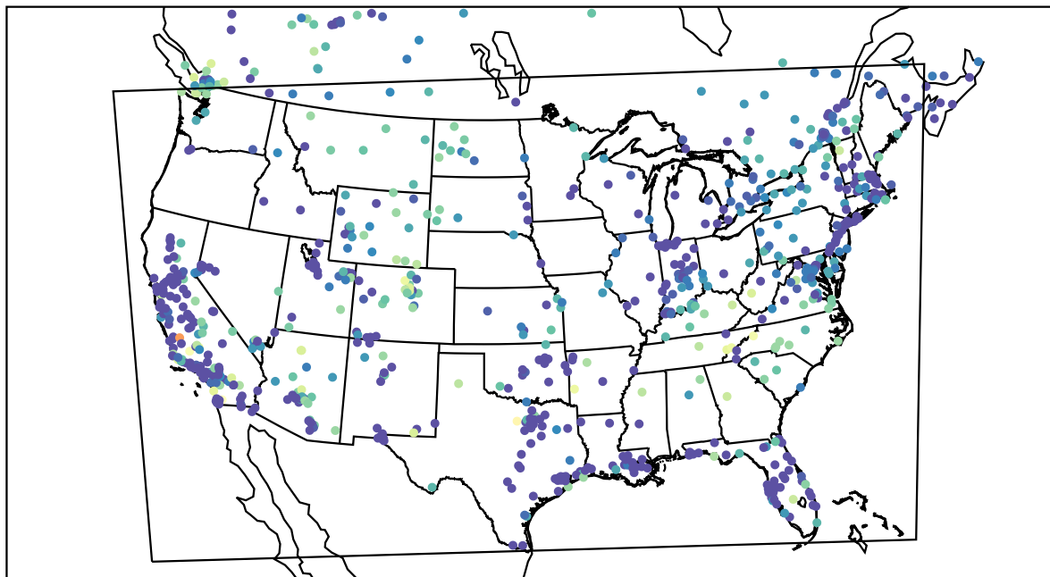
AirNOW (2021-12-02_05:00:00)
