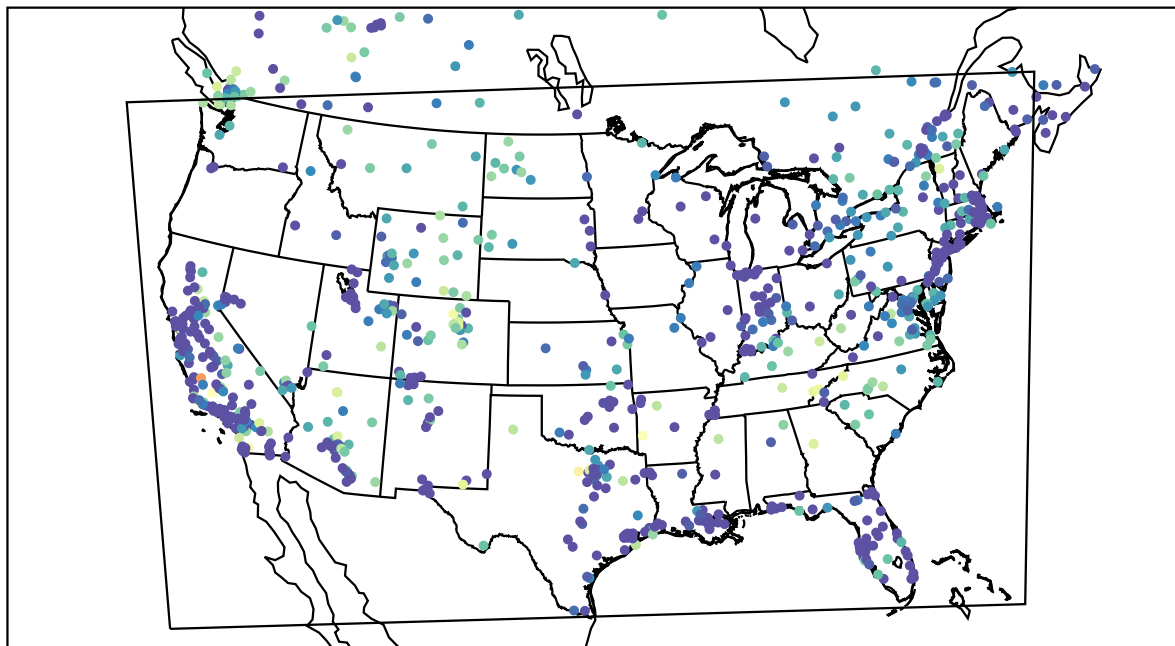
AirNOW (2021-12-02_04:00:00)
