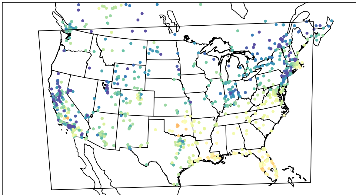
AirNOW (2021-12-02_19:00:00)
