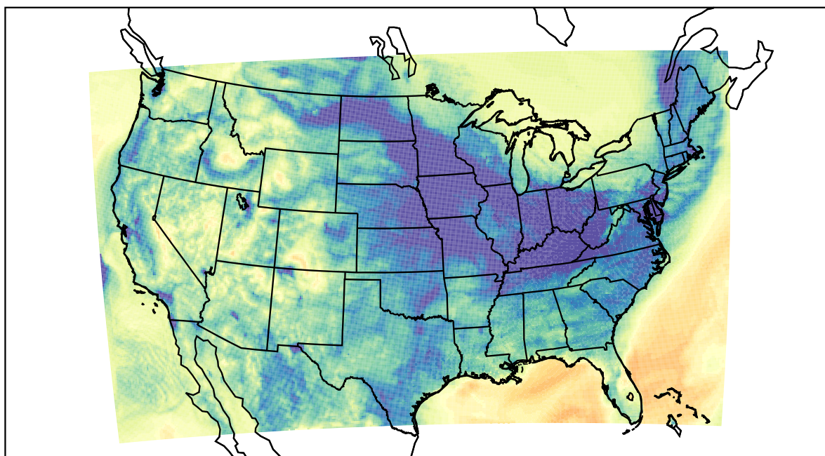
WRF (2021-12-03_07:00:00)
