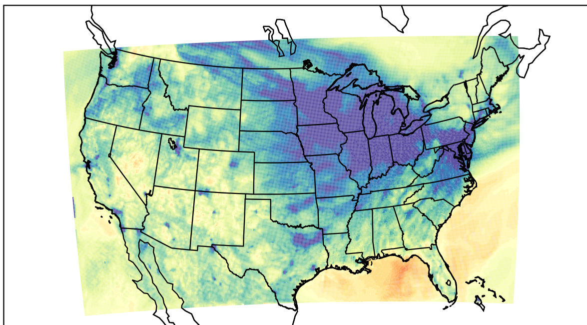
WRF (2021-12-02_02:00:00)
