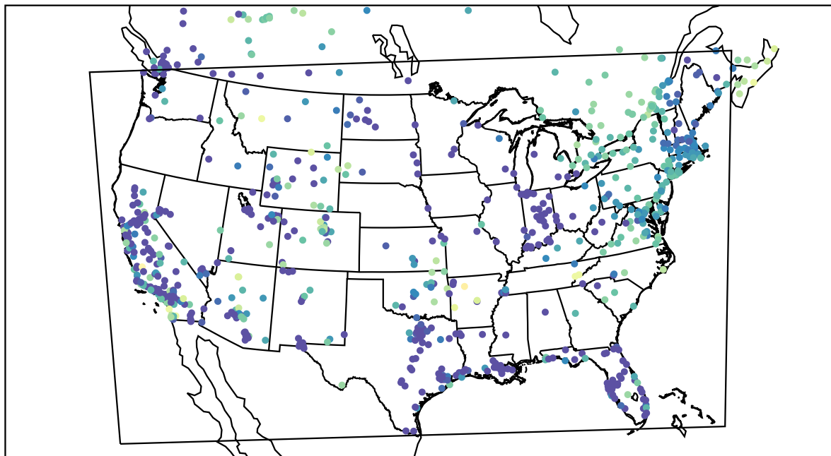
AirNOW (2021-12-03_08:00:00)
