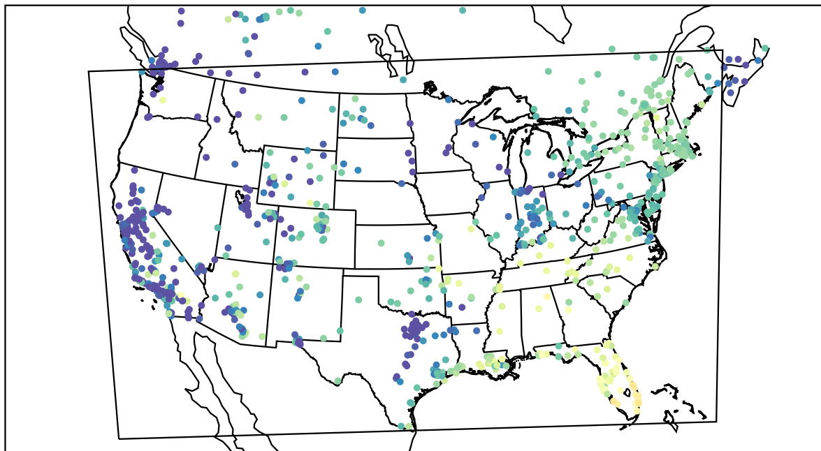
AirNOW (2021-12-03_17:00:00)
