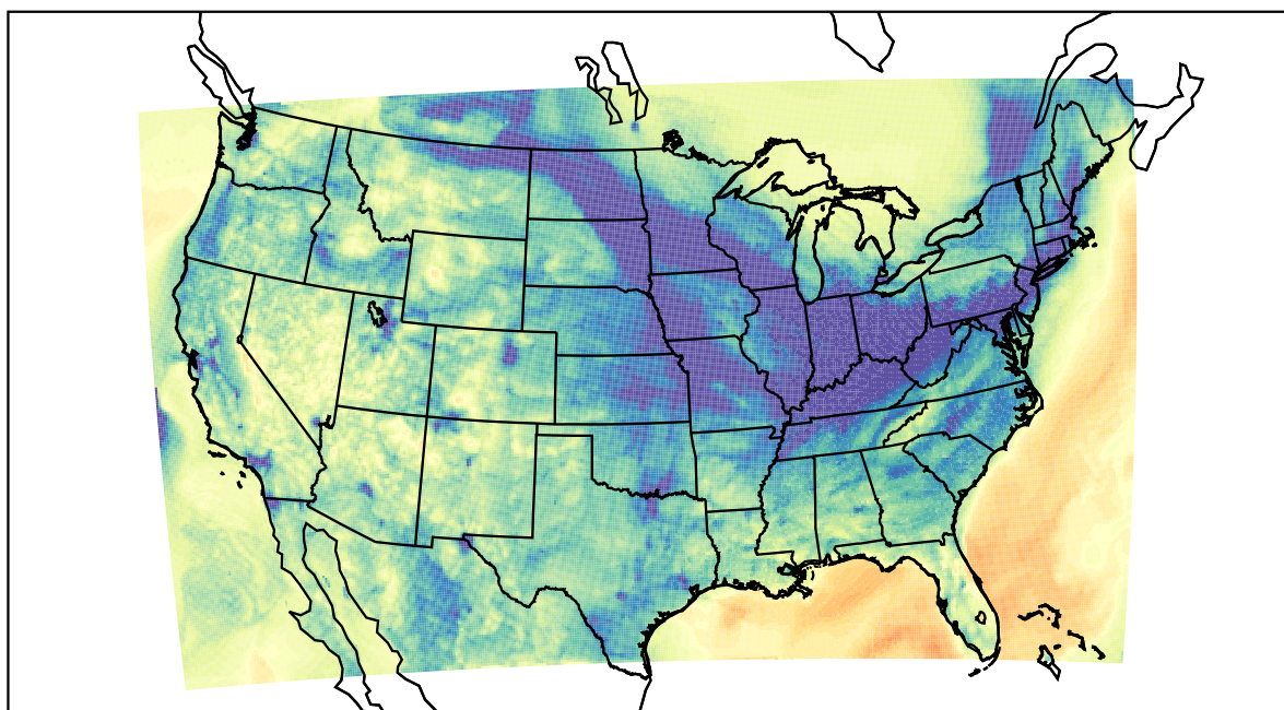
WRF (2021-12-03_03:00:00)
