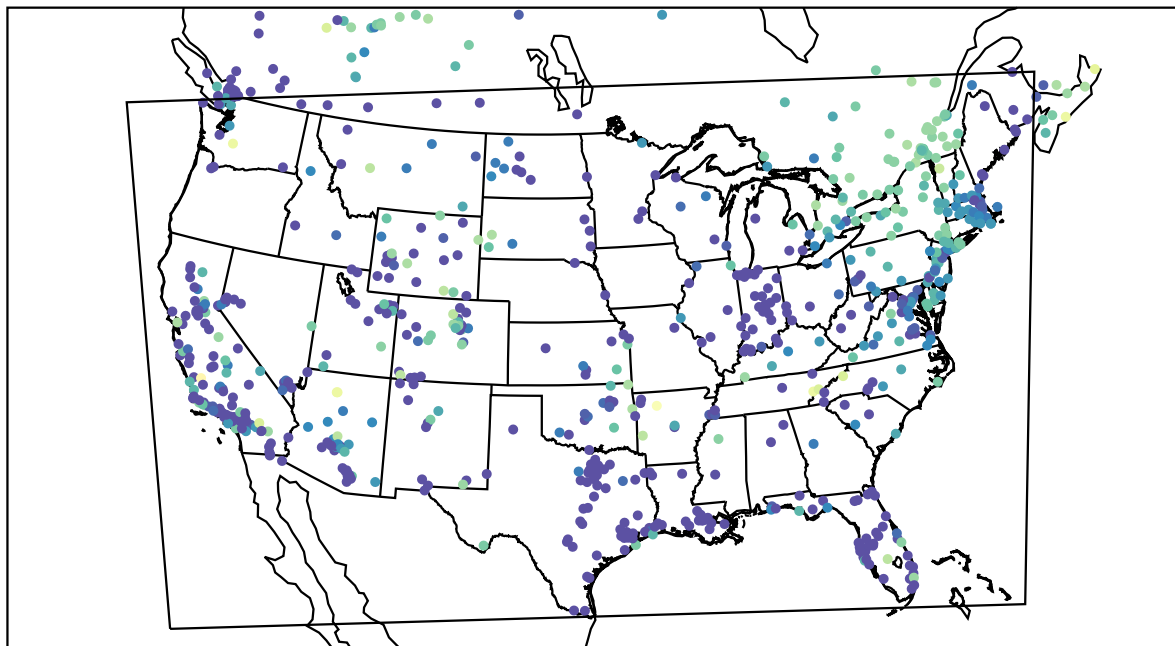
AirNOW (2021-12-03_11:00:00)
