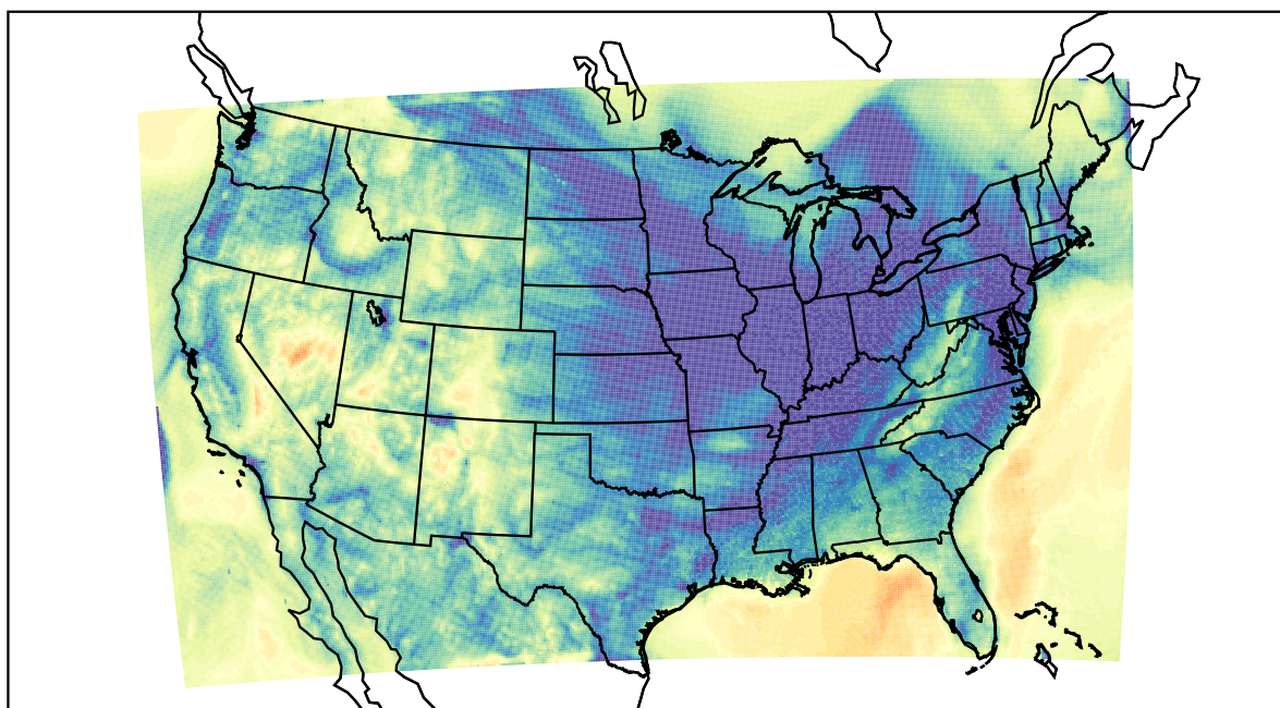
WRF (2021-12-02_12:00:00)
