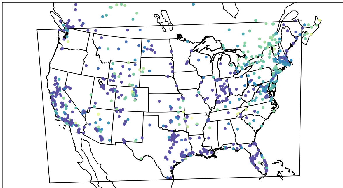
AirNOW (2021-12-03_10:00:00)
