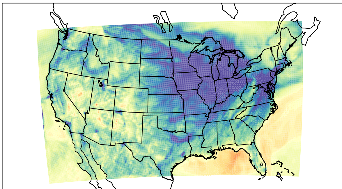
WRF (2021-12-02_05:00:00)
