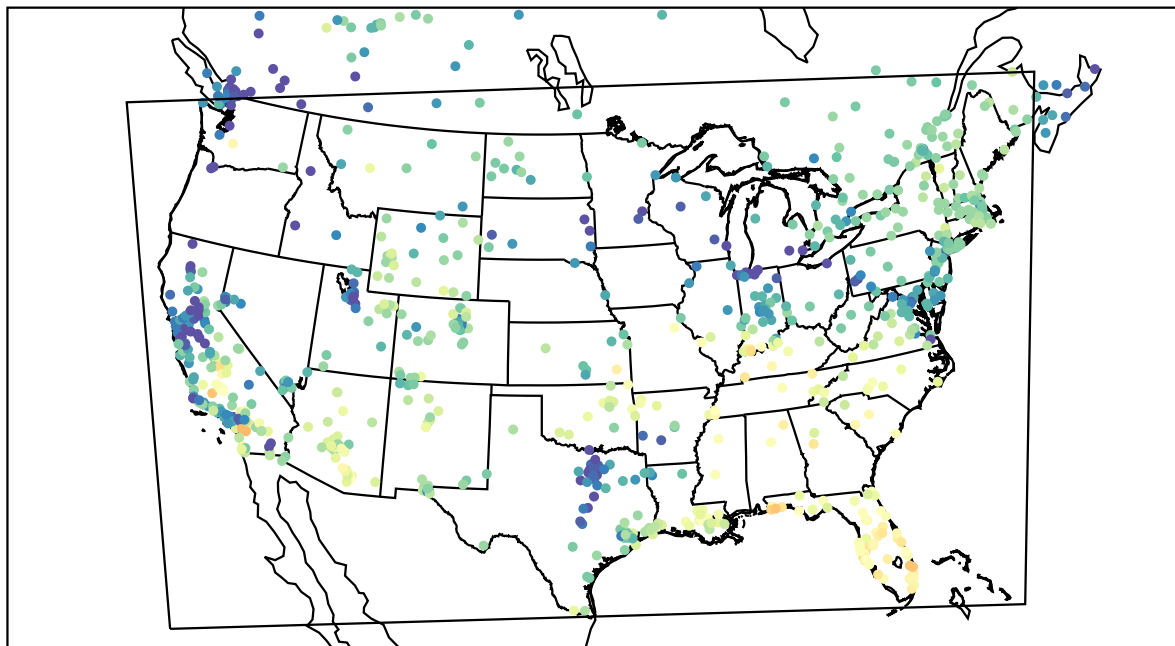
AirNOW (2021-12-03_20:00:00)
