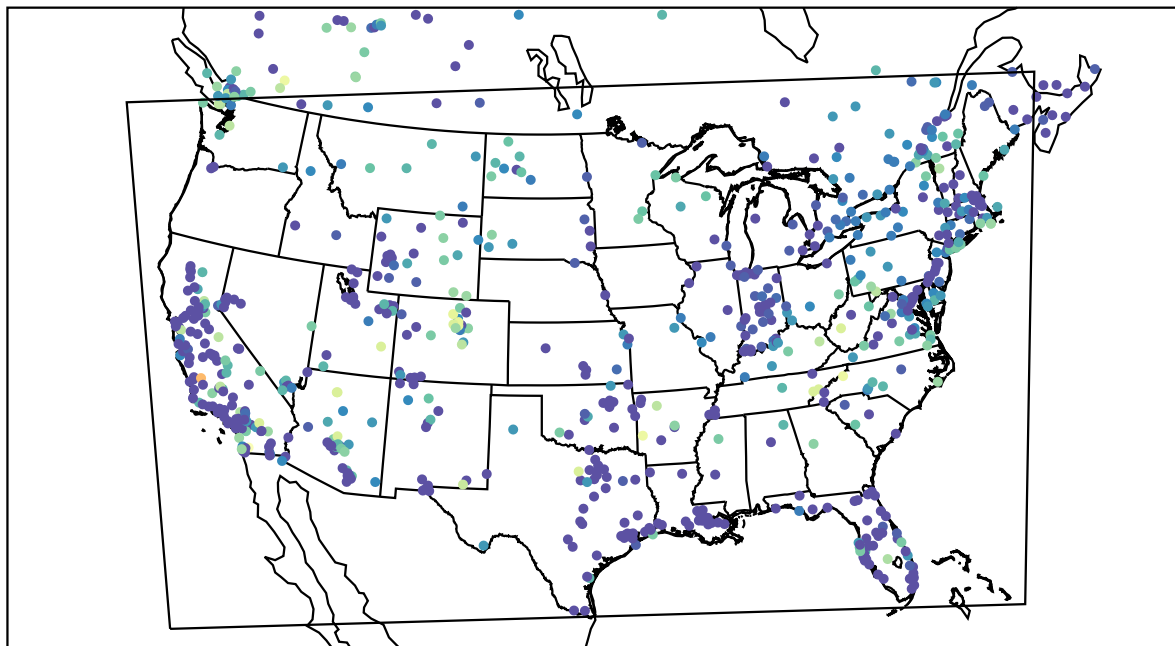
AirNOW (2021-12-02_09:00:00)
