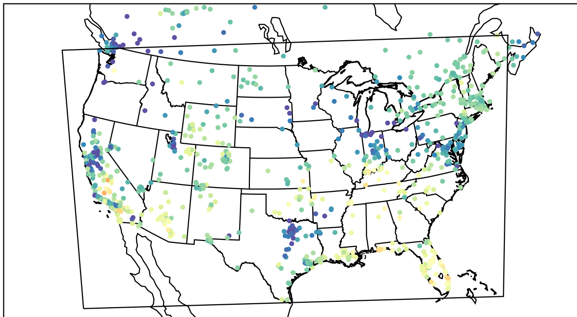
AirNOW (2021-12-03_21:00:00)
