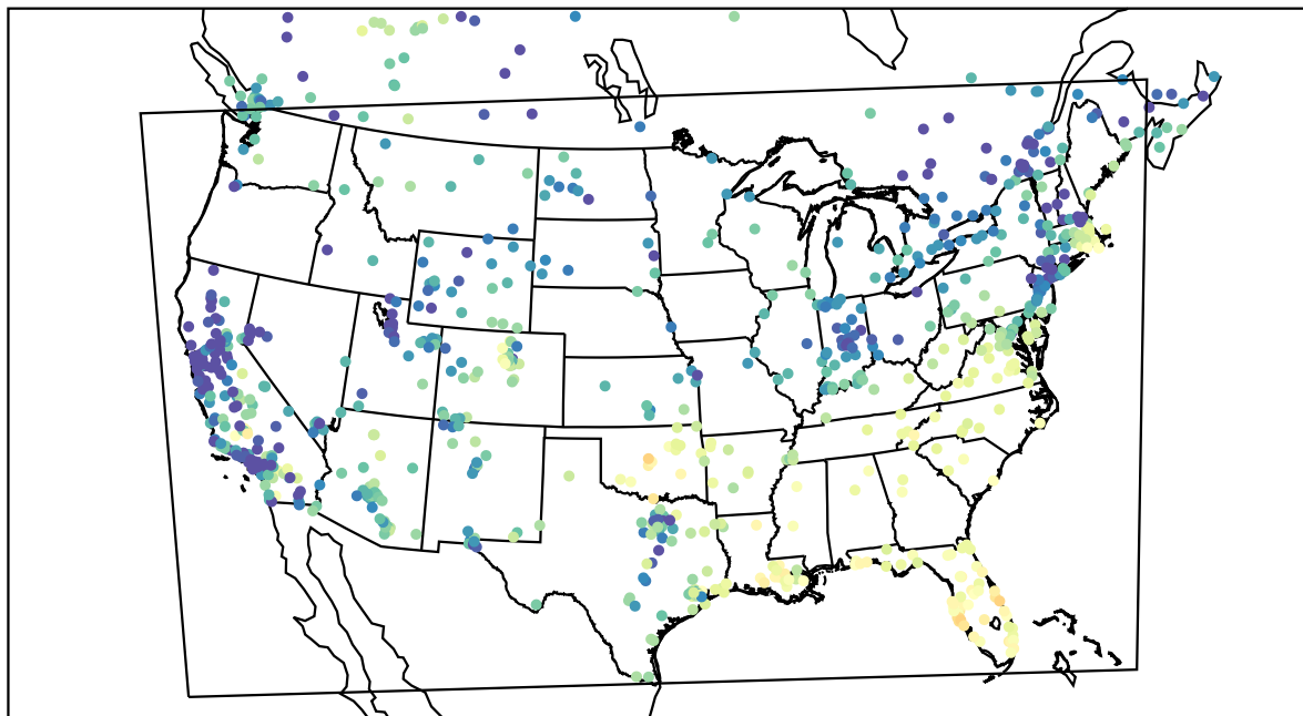
AirNOW (2021-12-02_18:00:00)
