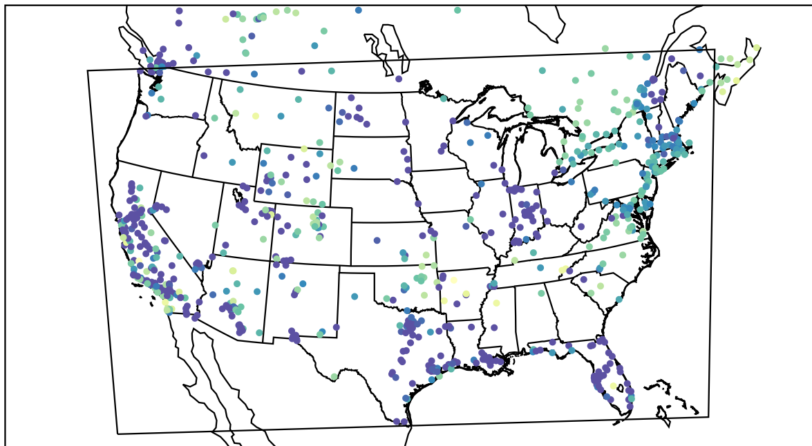
AirNOW (2021-12-03_07:00:00)
