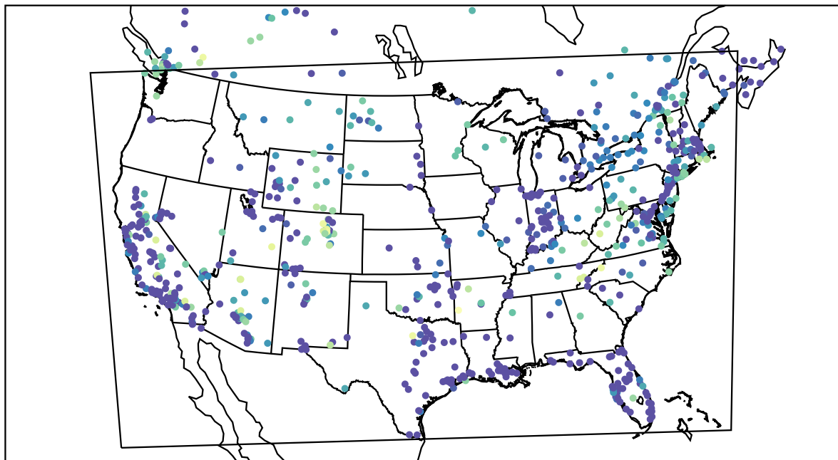
AirNOW (2021-12-02_10:00:00)
