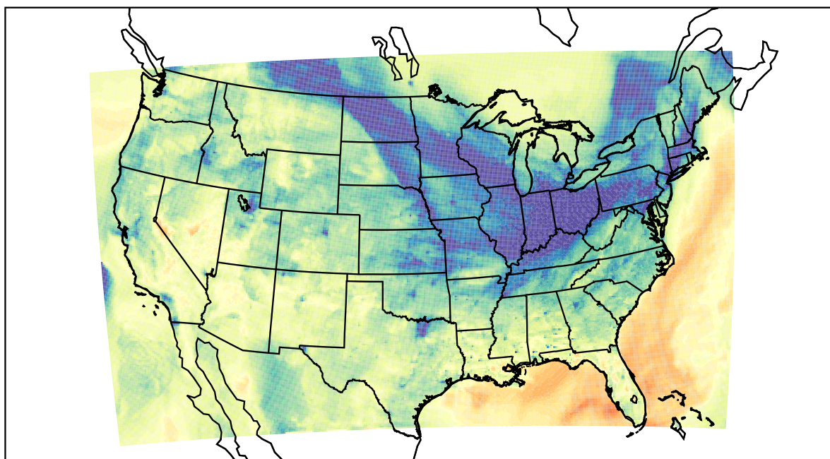
WRF (2021-12-02_23:00:00)
