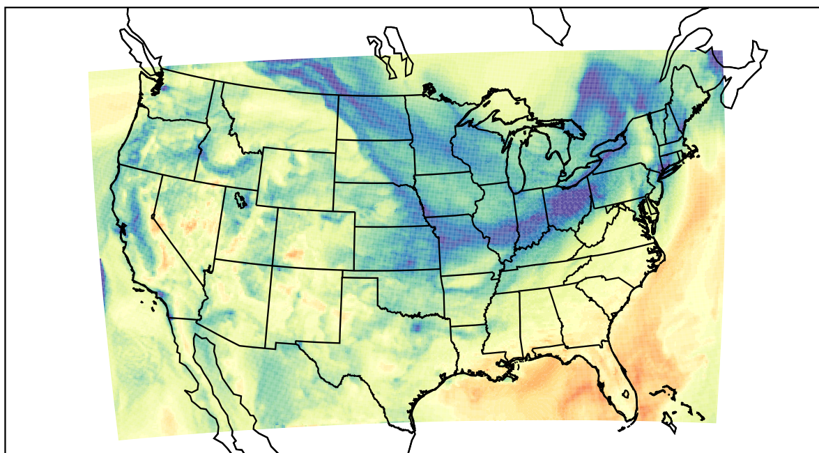
WRF (2021-12-02_19:00:00)
