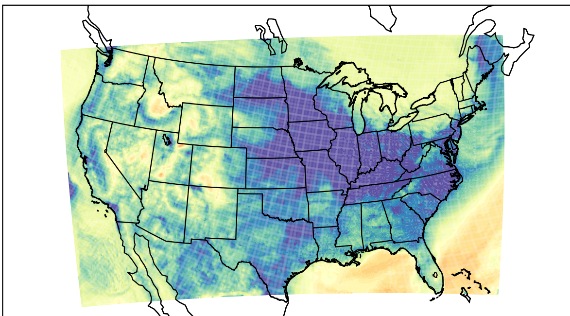
WRF (2021-12-03_12:00:00)
