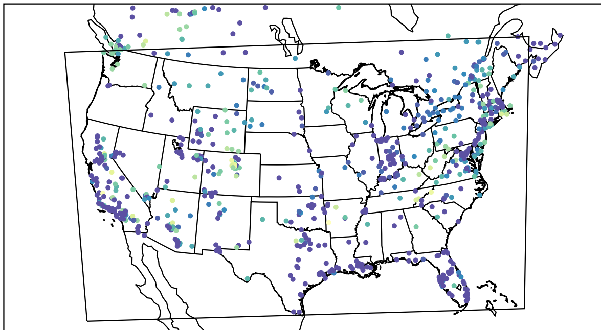
AirNOW (2021-12-02_11:00:00)
