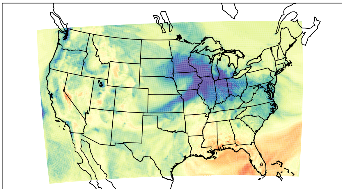
WRF (2021-12-03_21:00:00)
