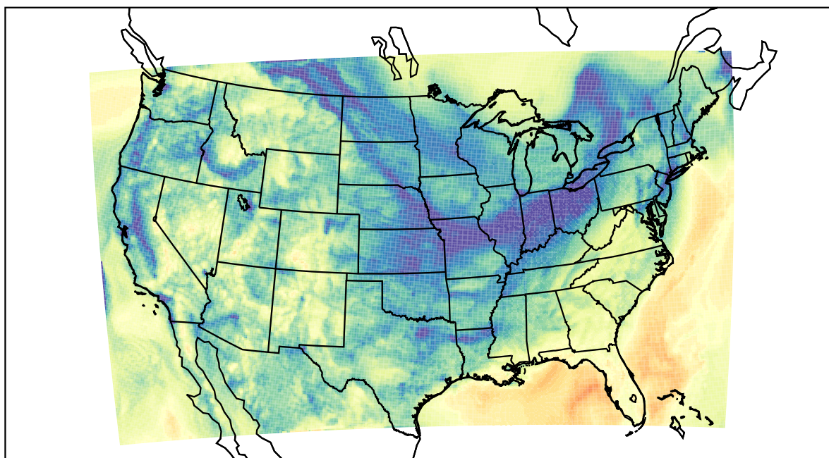
WRF (2021-12-02_17:00:00)
