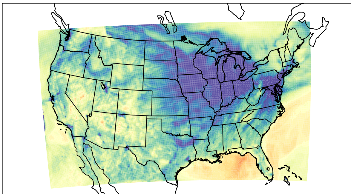
WRF (2021-12-02_04:00:00)
