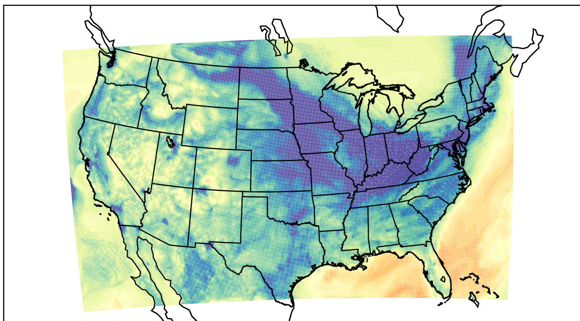
WRF (2021-12-03_05:00:00)
