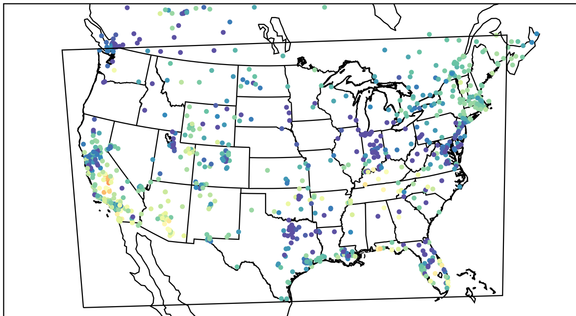
AirNOW (2021-12-03_23:00:00)
