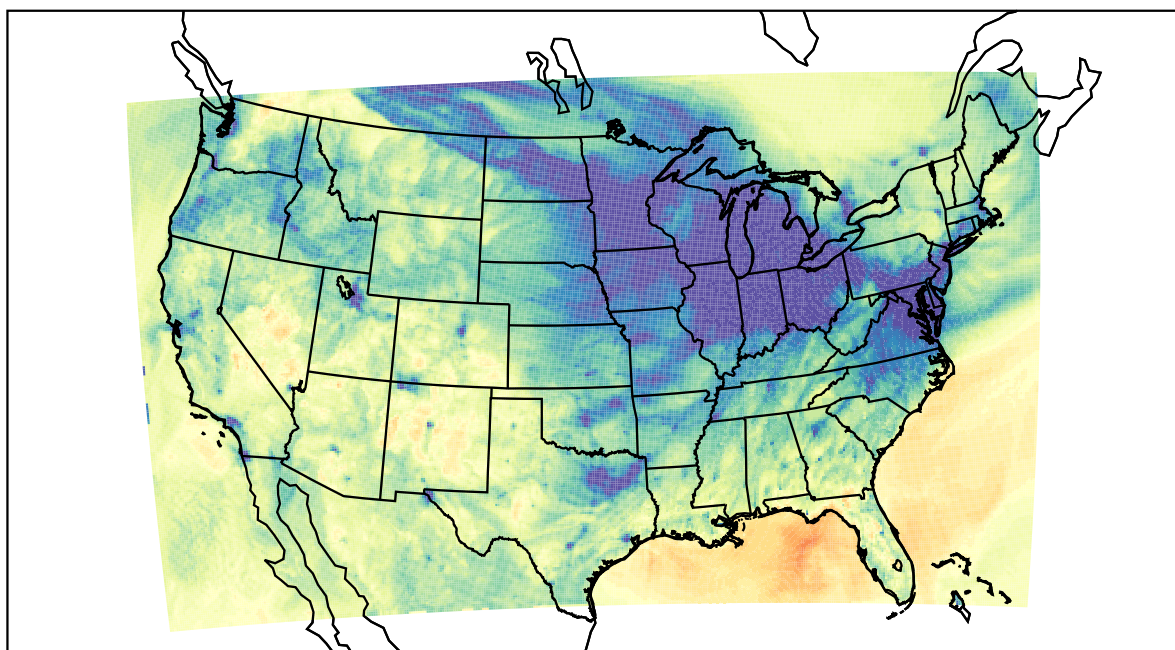
WRF (2021-12-02_00:00:00)
