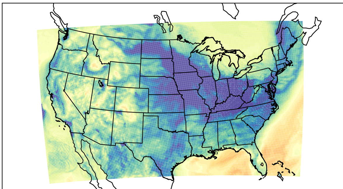
WRF (2021-12-03_08:00:00)
