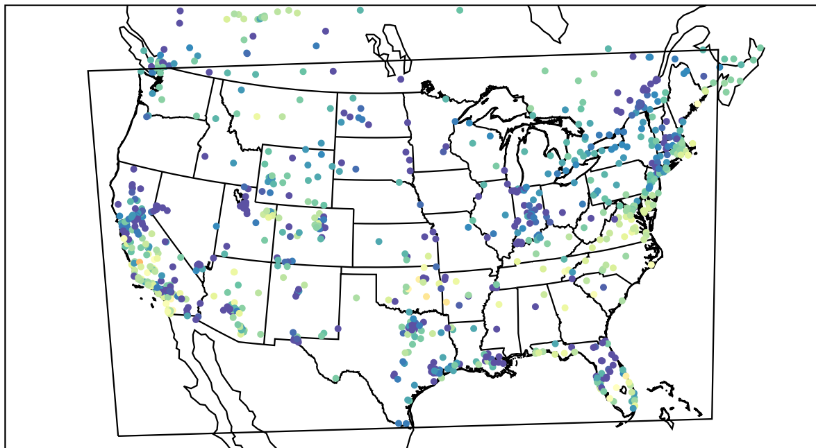
AirNOW (2021-12-03_00:00:00)
