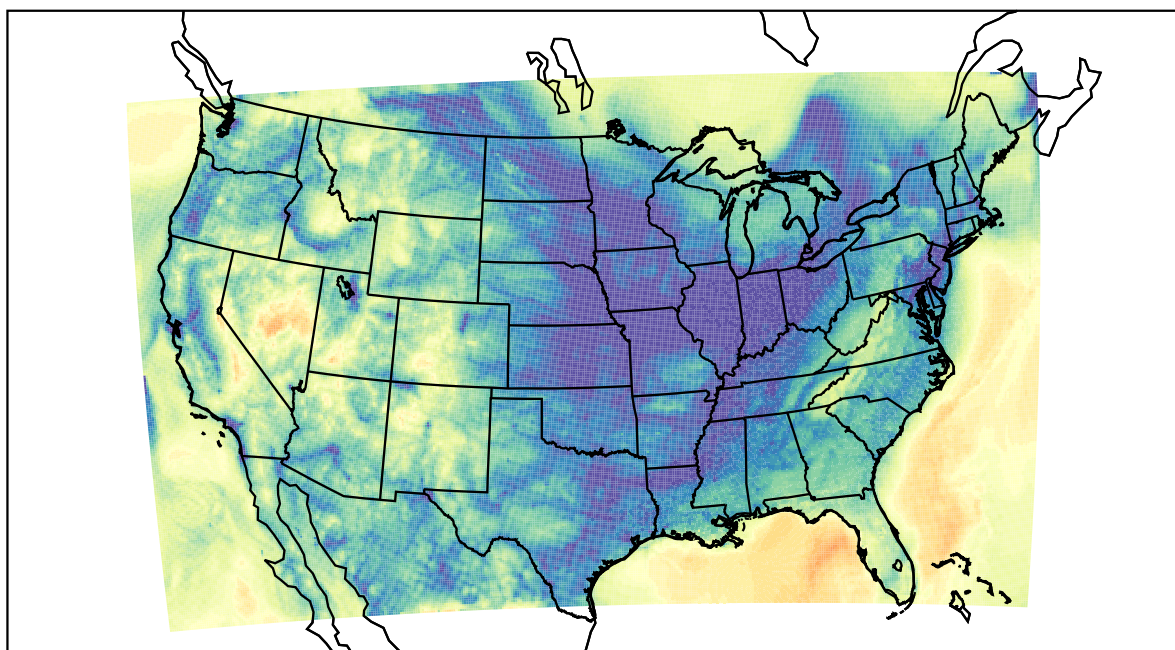
WRF (2021-12-02_15:00:00)
