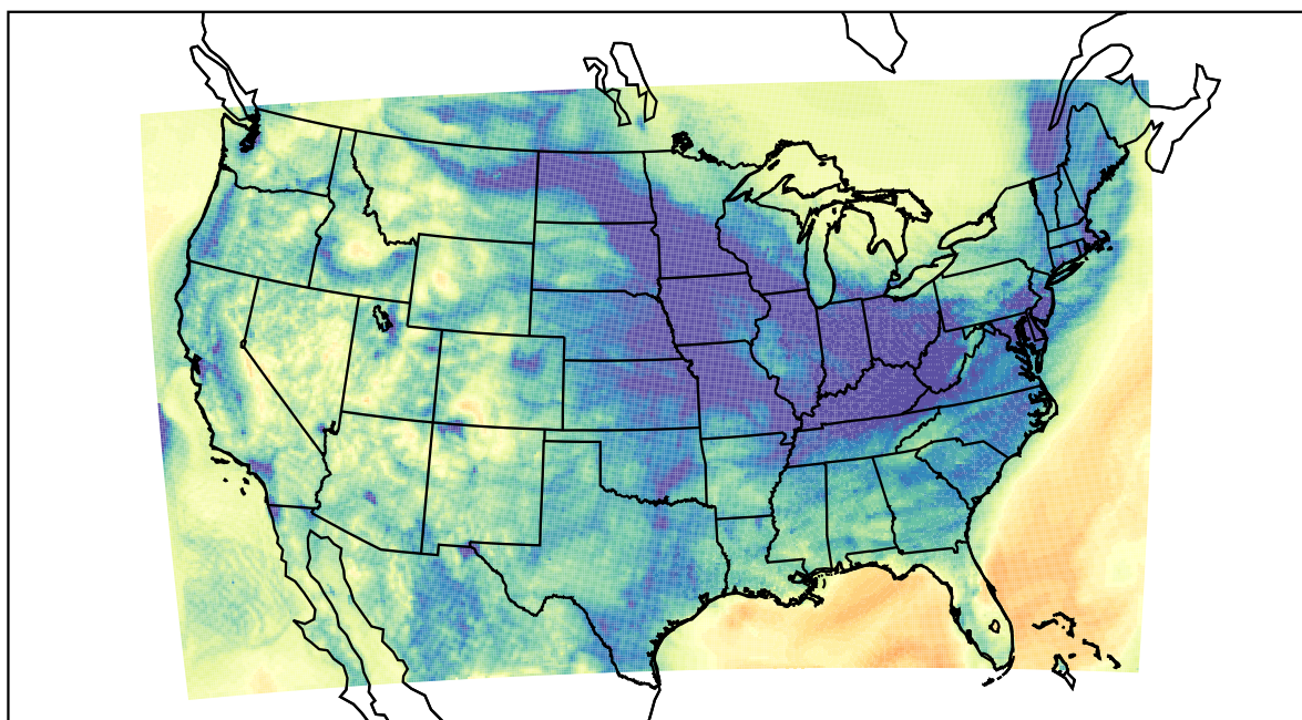
WRF (2021-12-03_06:00:00)
