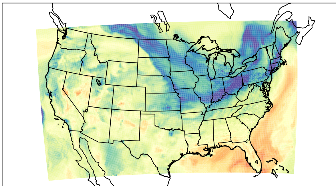
WRF (2021-12-02_21:00:00)
