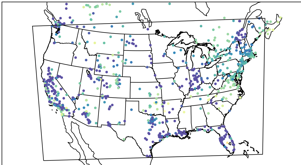
AirNOW (2021-12-03_05:00:00)
