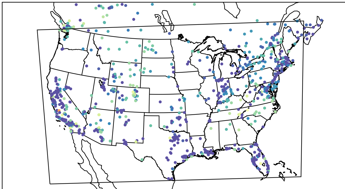
AirNOW (2021-12-02_06:00:00)
