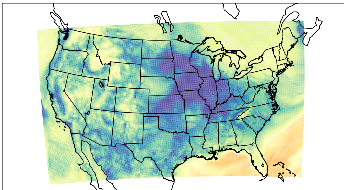
WRF (2021-12-03_16:00:00)
