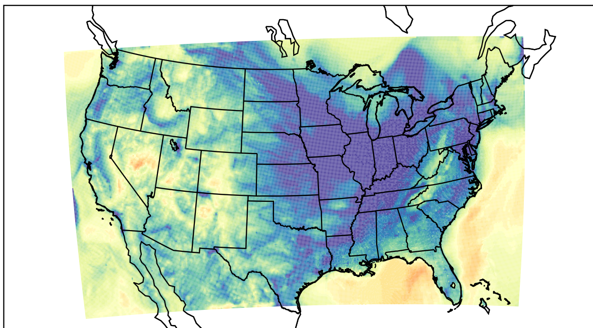
WRF (2021-12-02_13:00:00)
