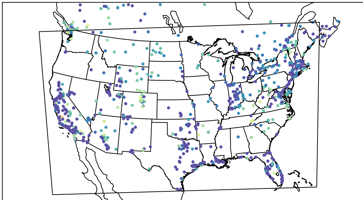
AirNOW (2021-12-02_08:00:00)
