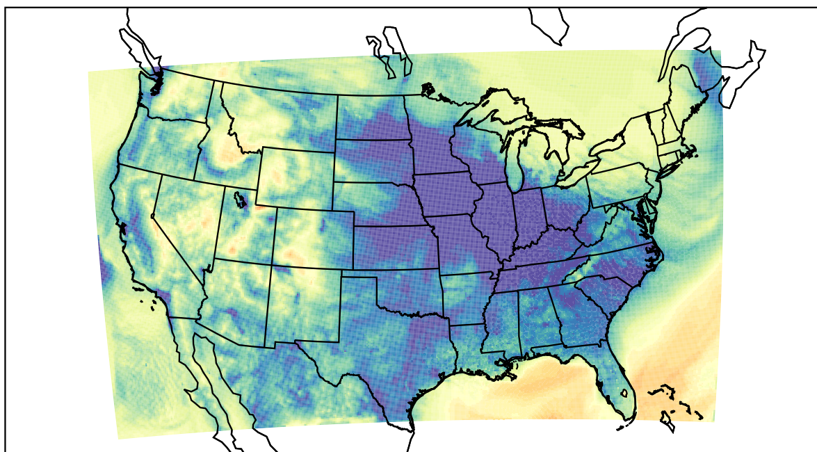
WRF (2021-12-03_14:00:00)
