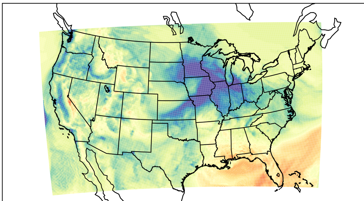
WRF (2021-12-03_19:00:00)
