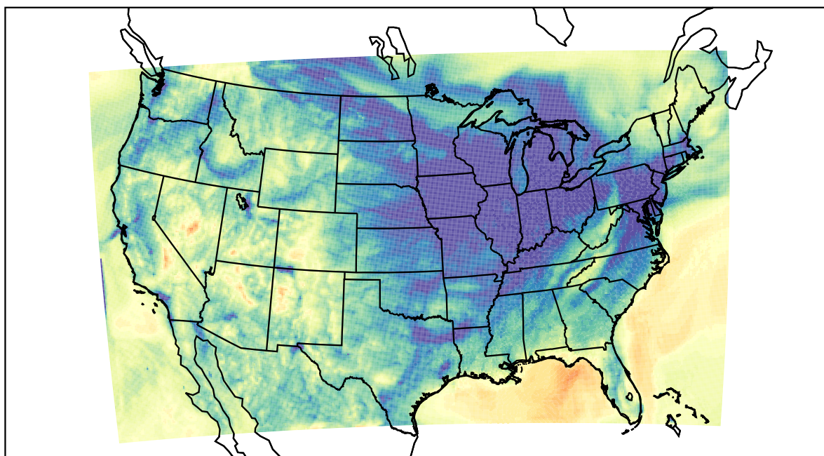
WRF (2021-12-02_07:00:00)
