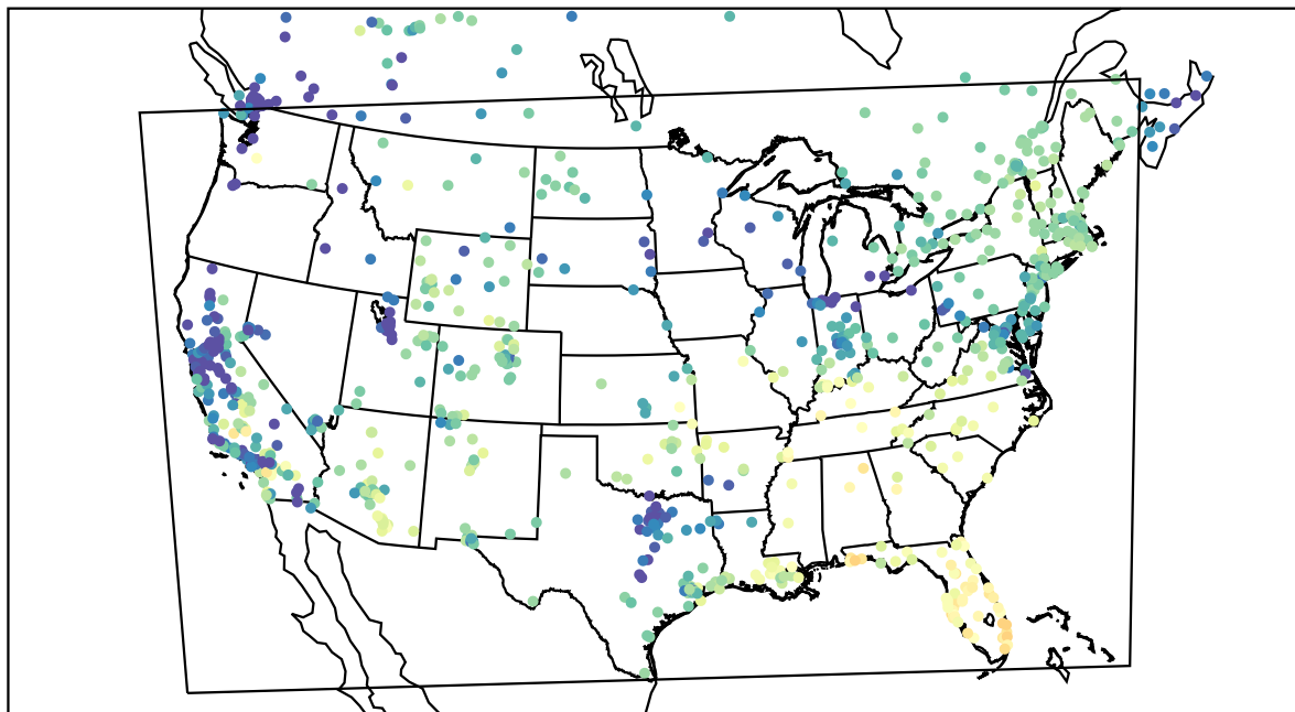
AirNOW (2021-12-03_19:00:00)
