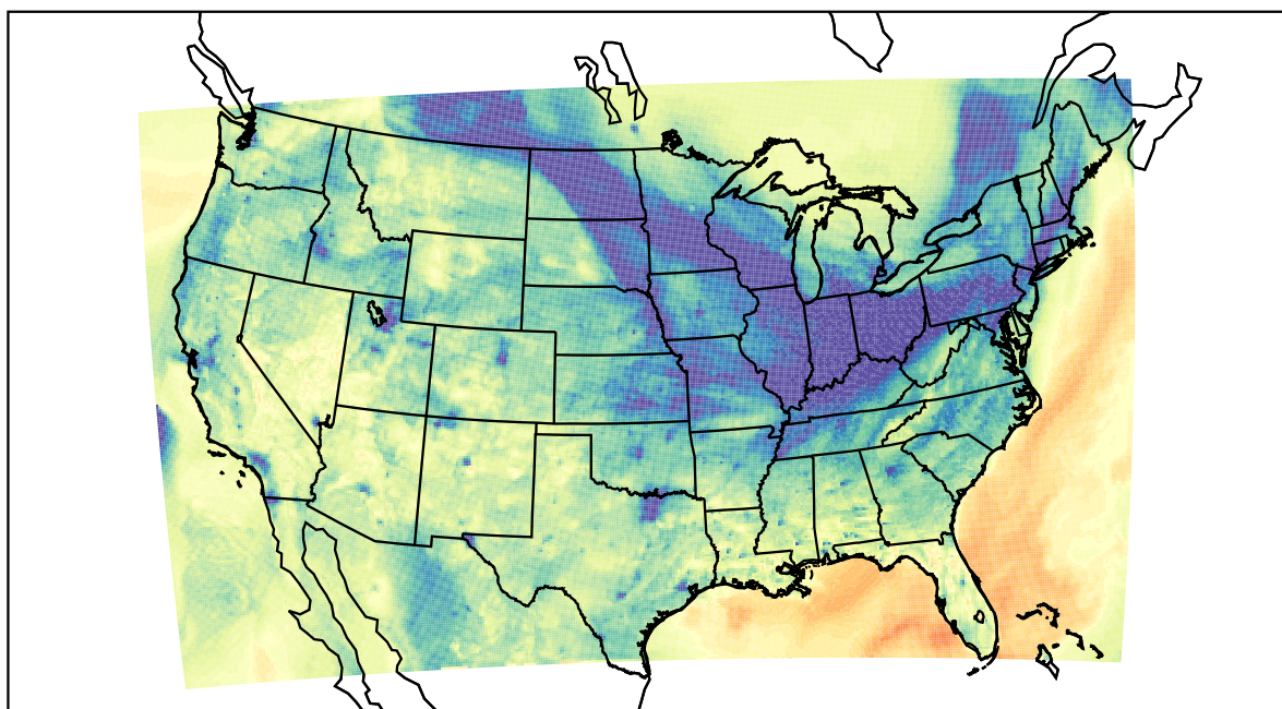
WRF (2021-12-03_00:00:00)
