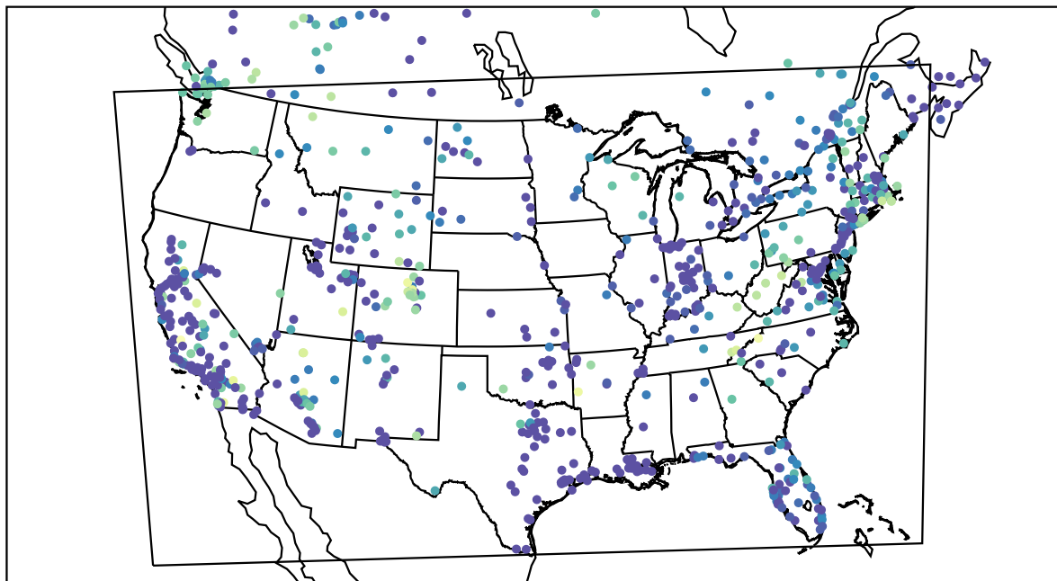
AirNOW (2021-12-02_13:00:00)
