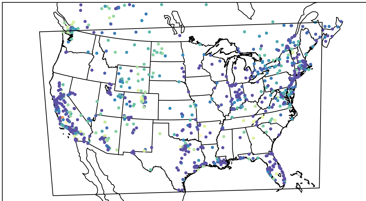
AirNOW (2021-12-02_03:00:00)
