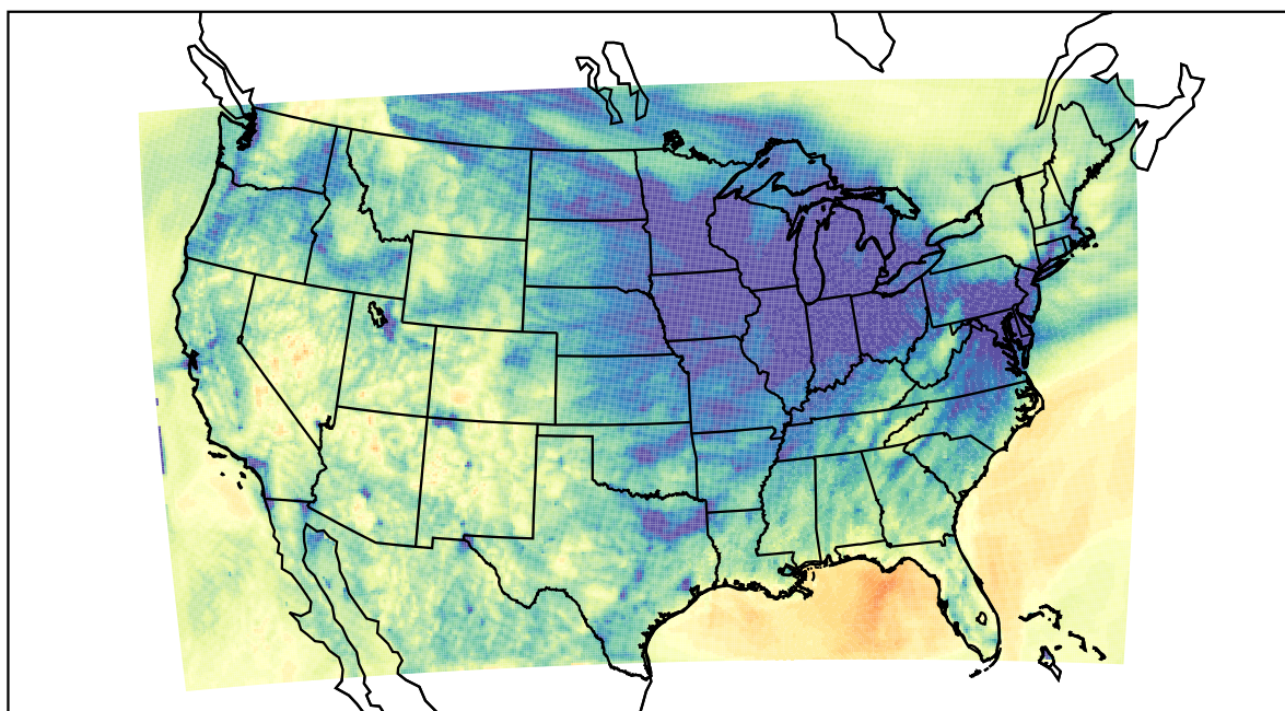
WRF (2021-12-02_03:00:00)
