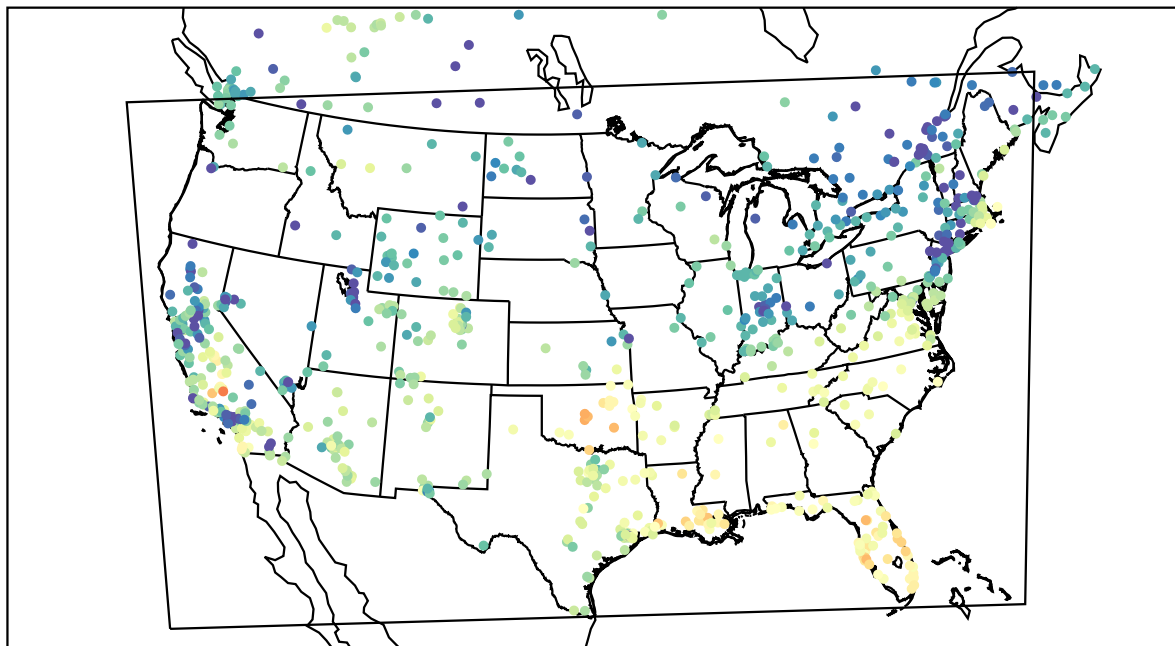
AirNOW (2021-12-02_20:00:00)
