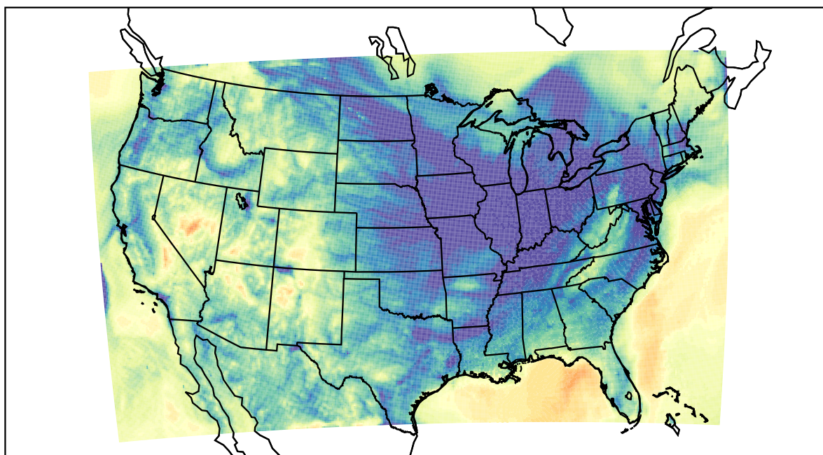
WRF (2021-12-02_11:00:00)
