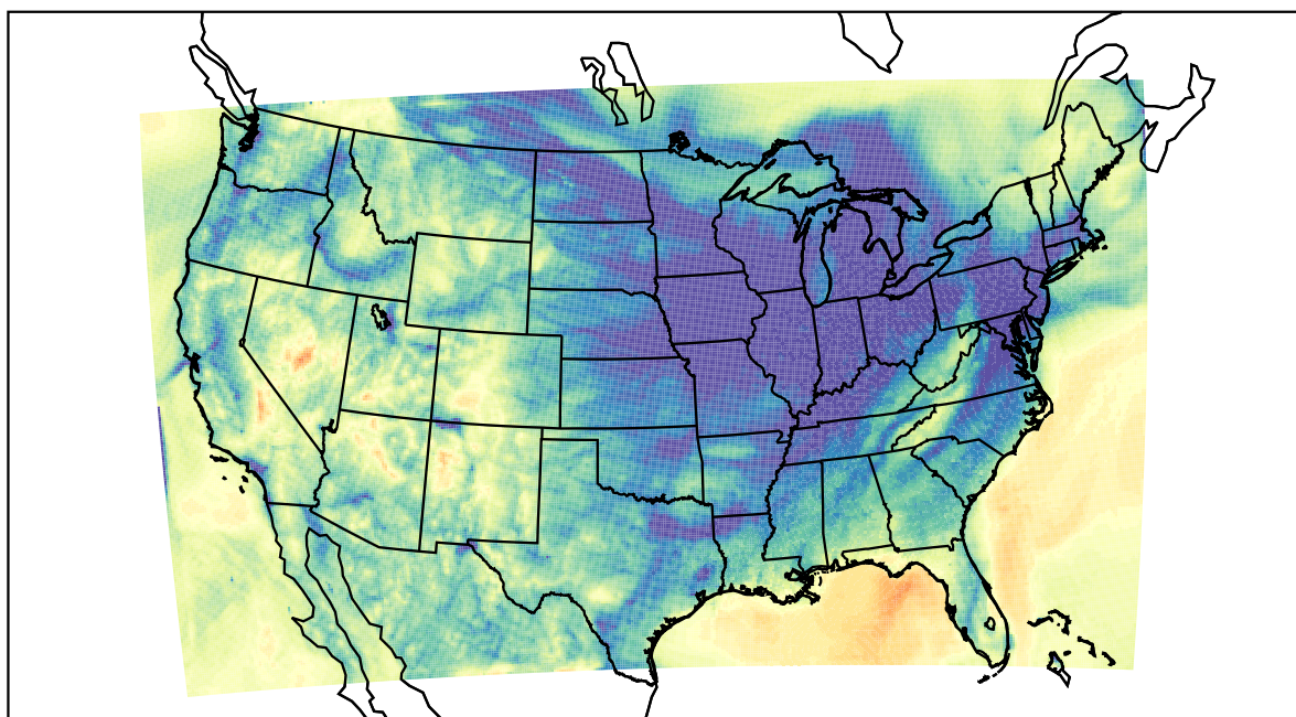
WRF (2021-12-02_08:00:00)
