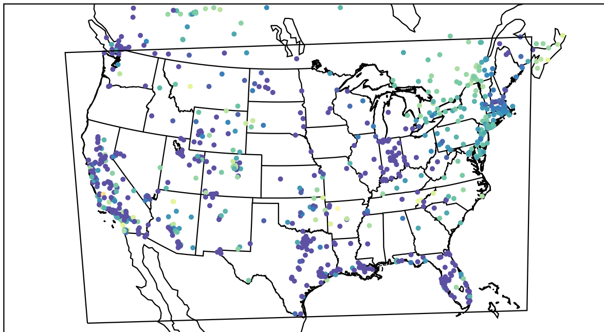
AirNOW (2021-12-03_09:00:00)
