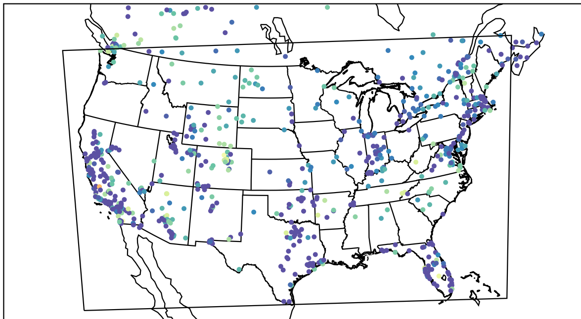
AirNOW (2021-12-02_07:00:00)
