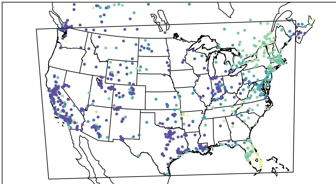
AirNOW (2021-12-03_15:00:00)
