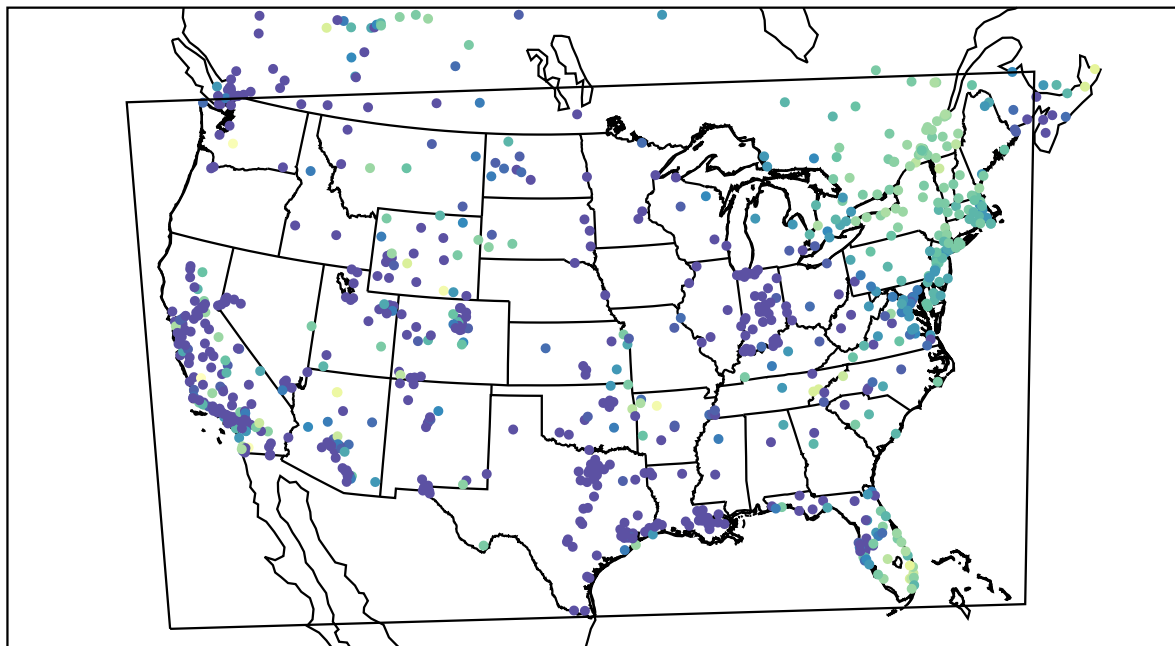
AirNOW (2021-12-03_14:00:00)
