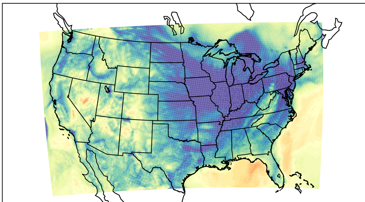
WRF (2021-12-02_10:00:00)
