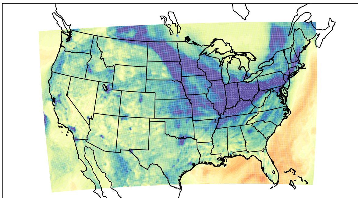
WRF (2021-12-03_01:00:00)
