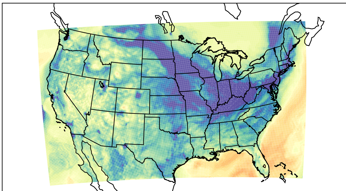
WRF (2021-12-03_04:00:00)
