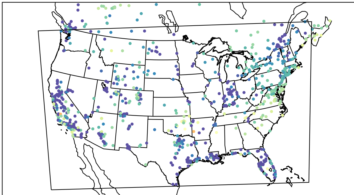
AirNOW (2021-12-03_03:00:00)
