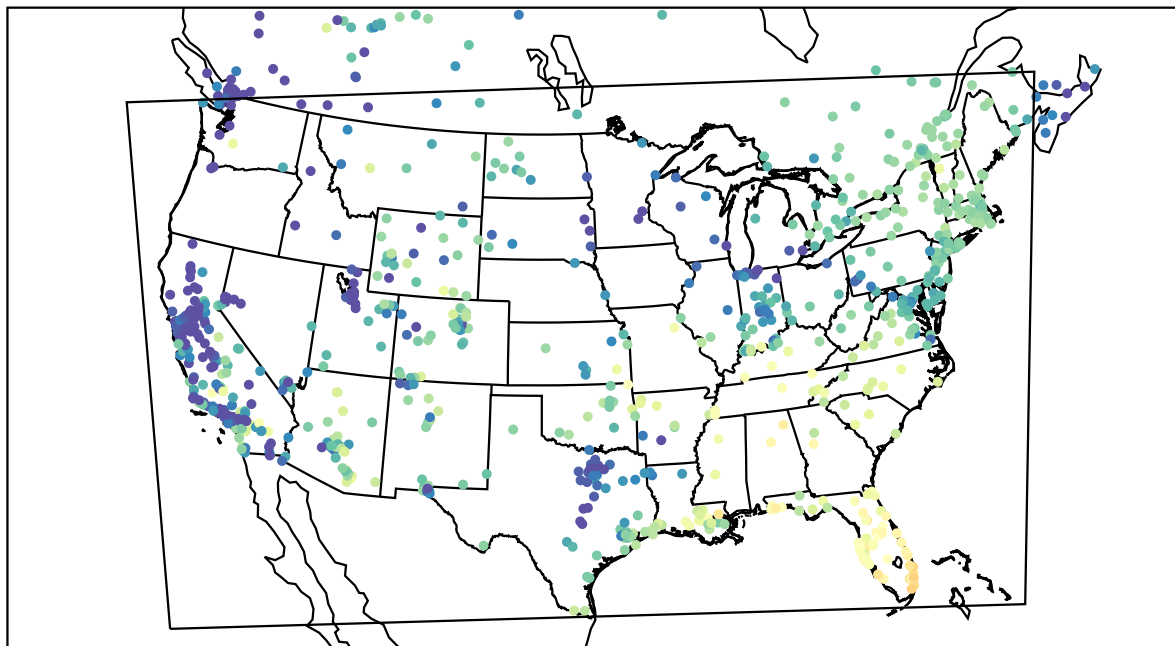
AirNOW (2021-12-03_18:00:00)
