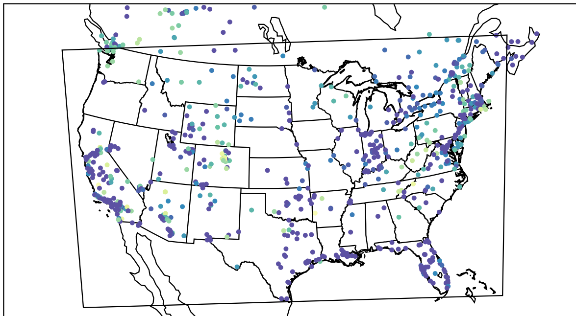
AirNOW (2021-12-02_12:00:00)
