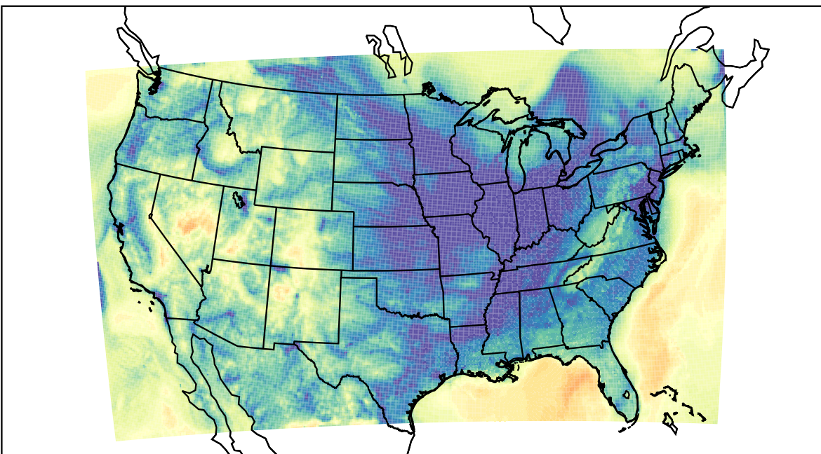
WRF (2021-12-02_14:00:00)
