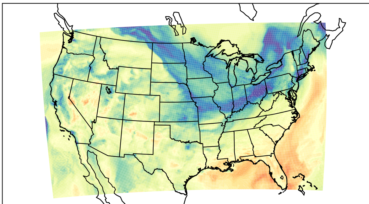
WRF (2021-12-02_20:00:00)
