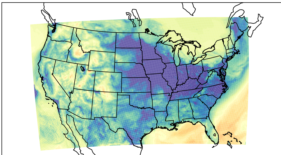
WRF (2021-12-03_11:00:00)
