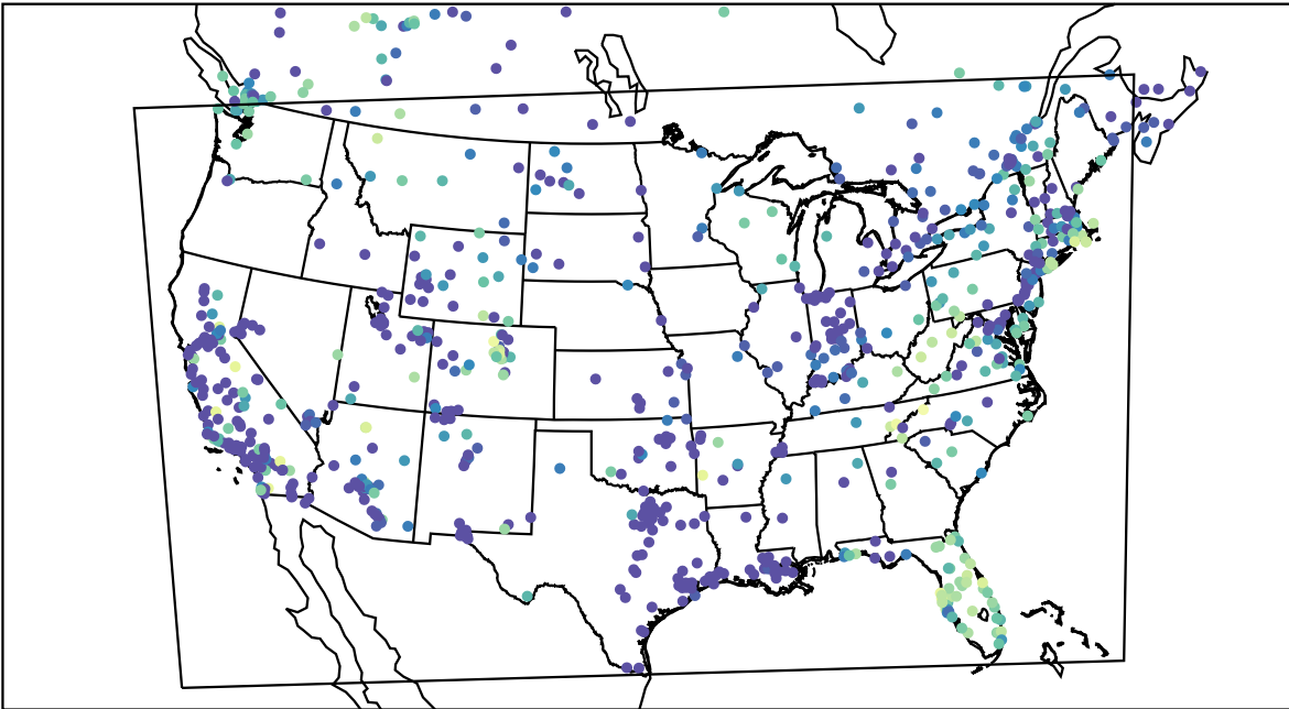
AirNOW (2021-12-02_14:00:00)
