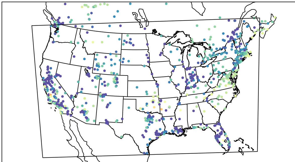
AirNOW (2021-12-03_02:00:00)
