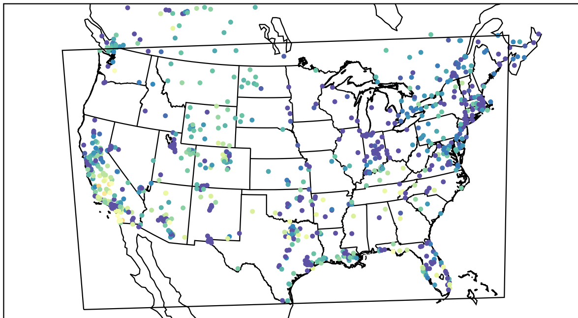
AirNOW (2021-12-02_00:00:00)
