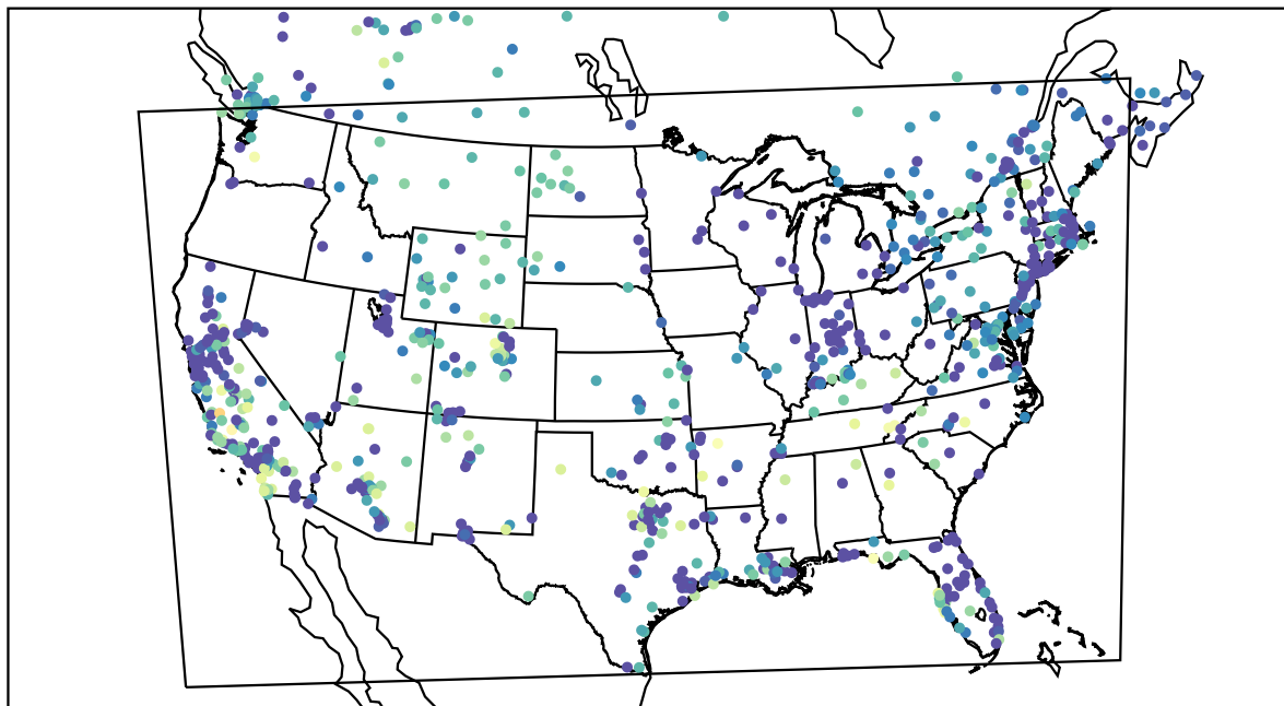
AirNOW (2021-12-02_01:00:00)
