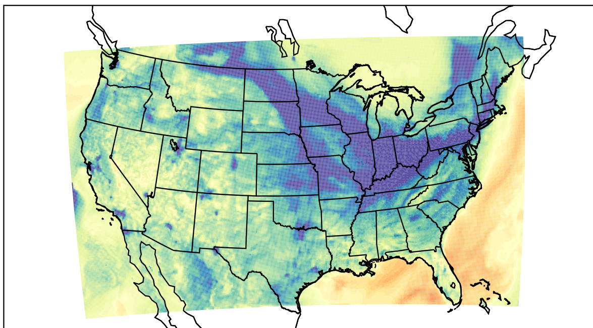
WRF (2021-12-03_02:00:00)
