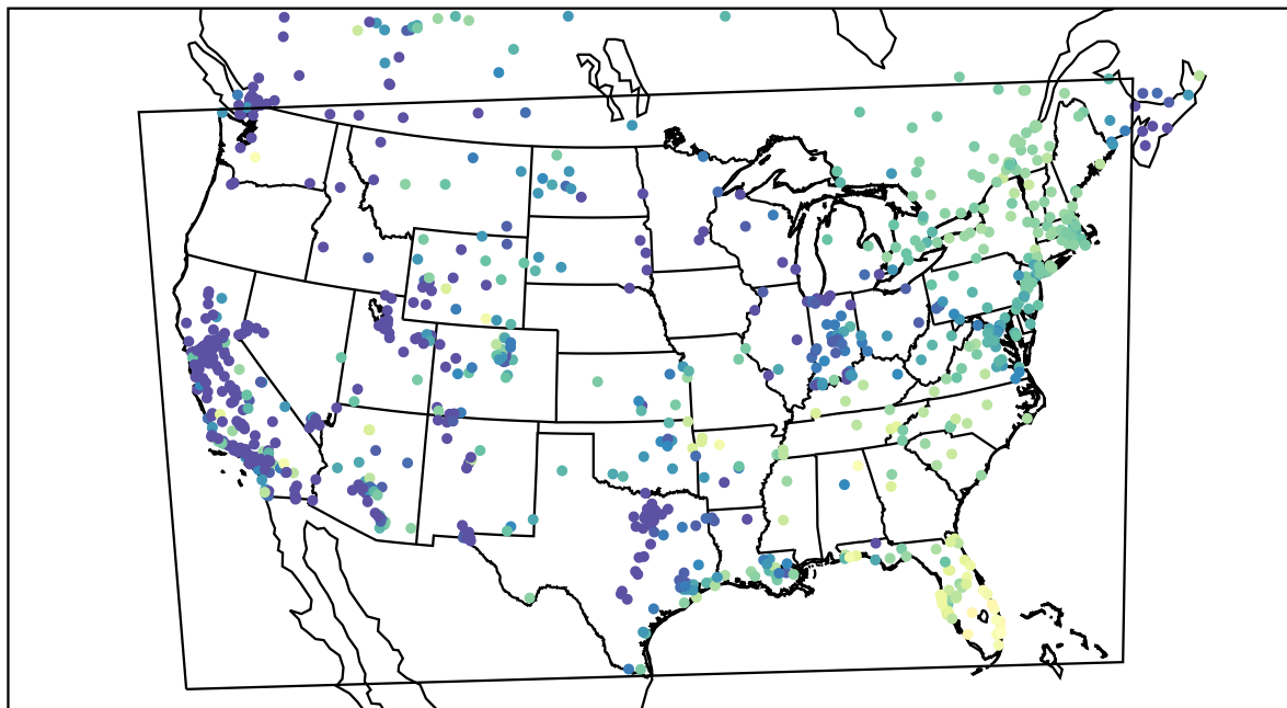
AirNOW (2021-12-03_16:00:00)
