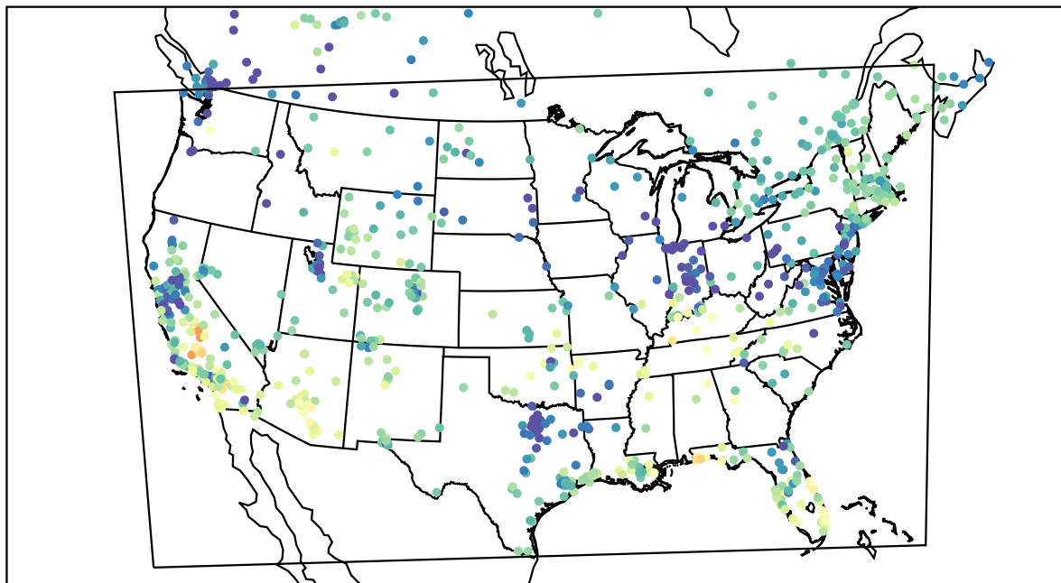
AirNOW (2021-12-03_22:00:00)
