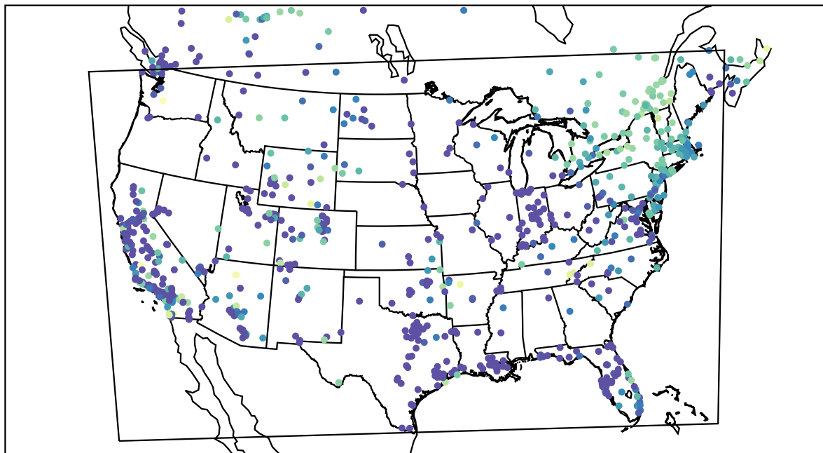
AirNOW (2021-12-03_13:00:00)
