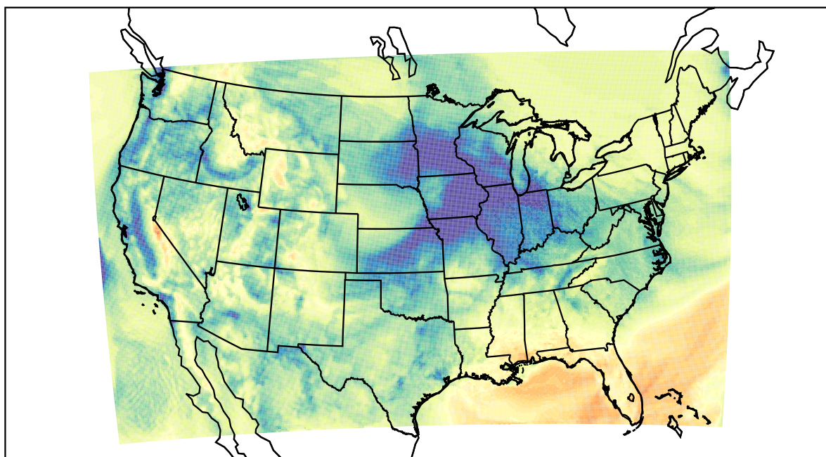
WRF (2021-12-03_18:00:00)
