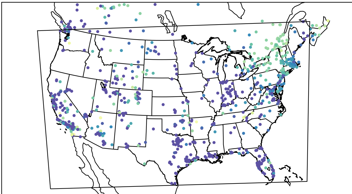
AirNOW (2021-12-03_12:00:00)
