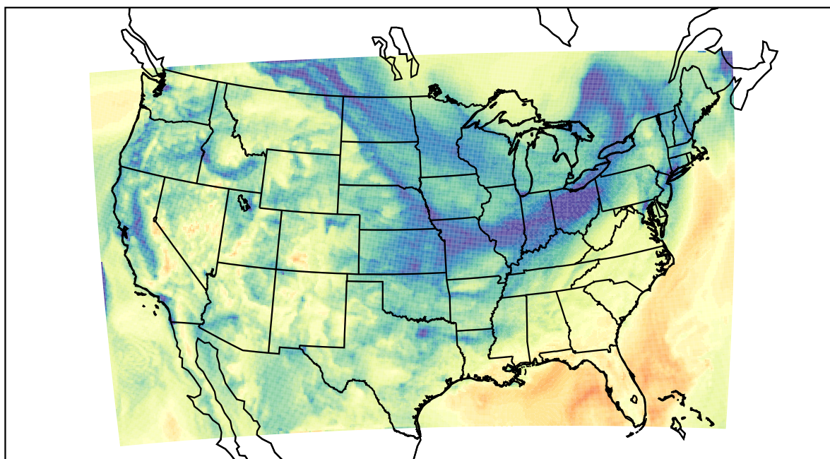
WRF (2021-12-02_18:00:00)
