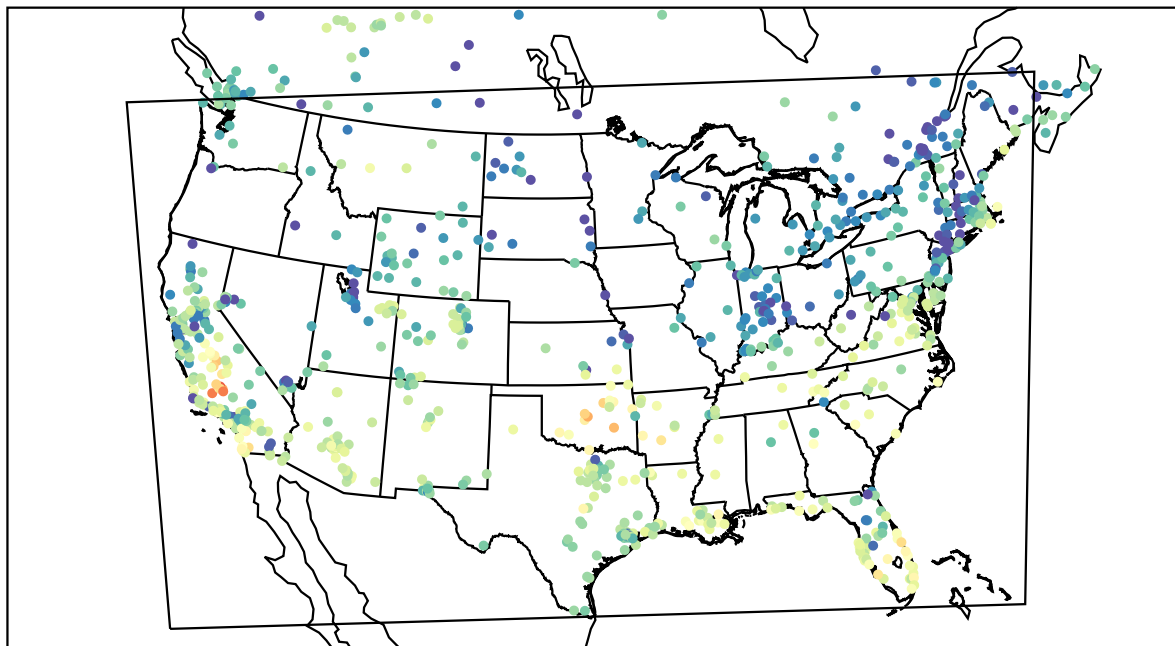
AirNOW (2021-12-02_22:00:00)
