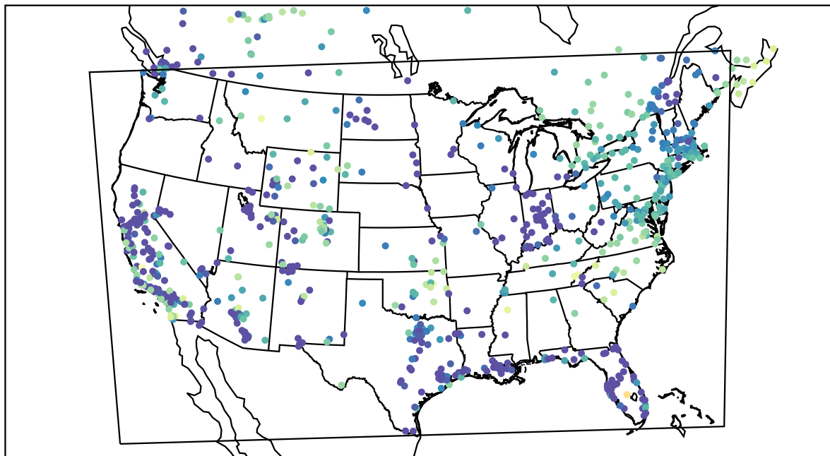
AirNOW (2021-12-03_06:00:00)
