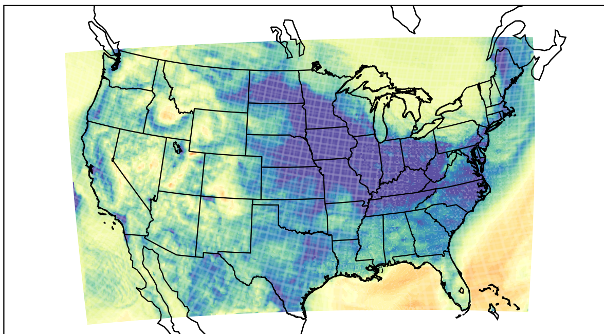
WRF (2021-12-03_10:00:00)
