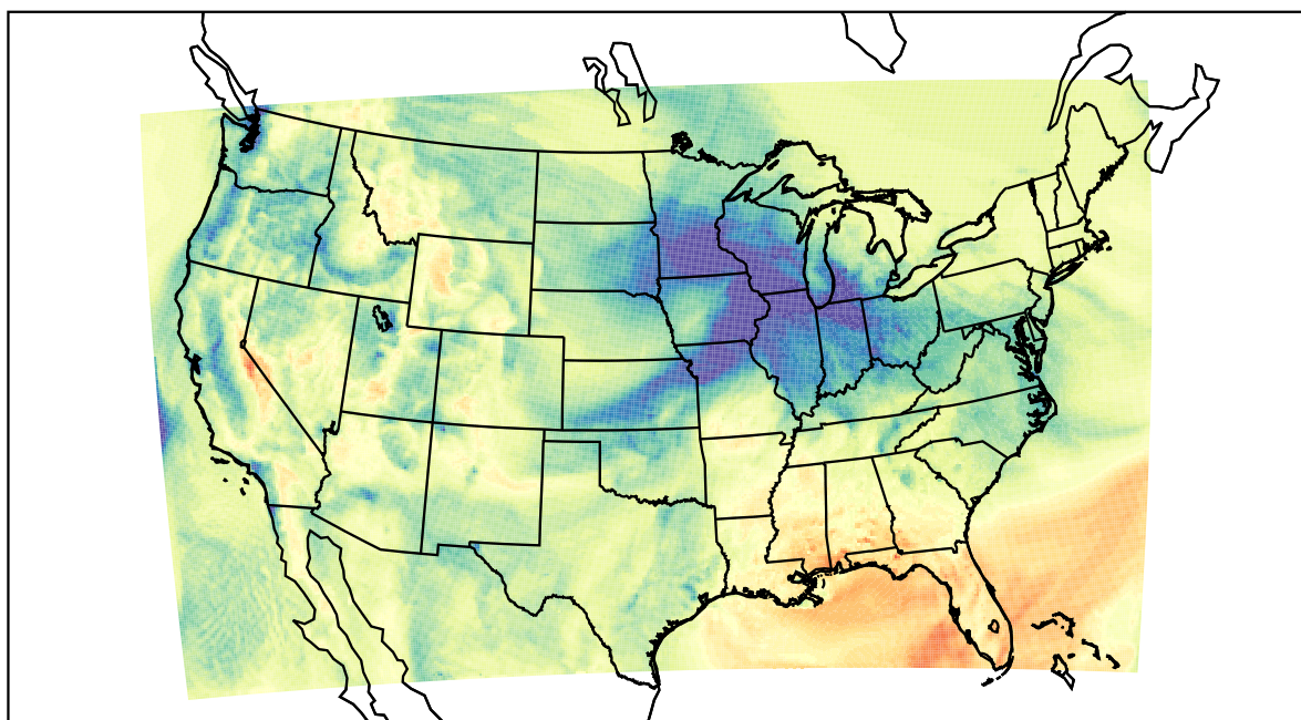
WRF (2021-12-03_20:00:00)
