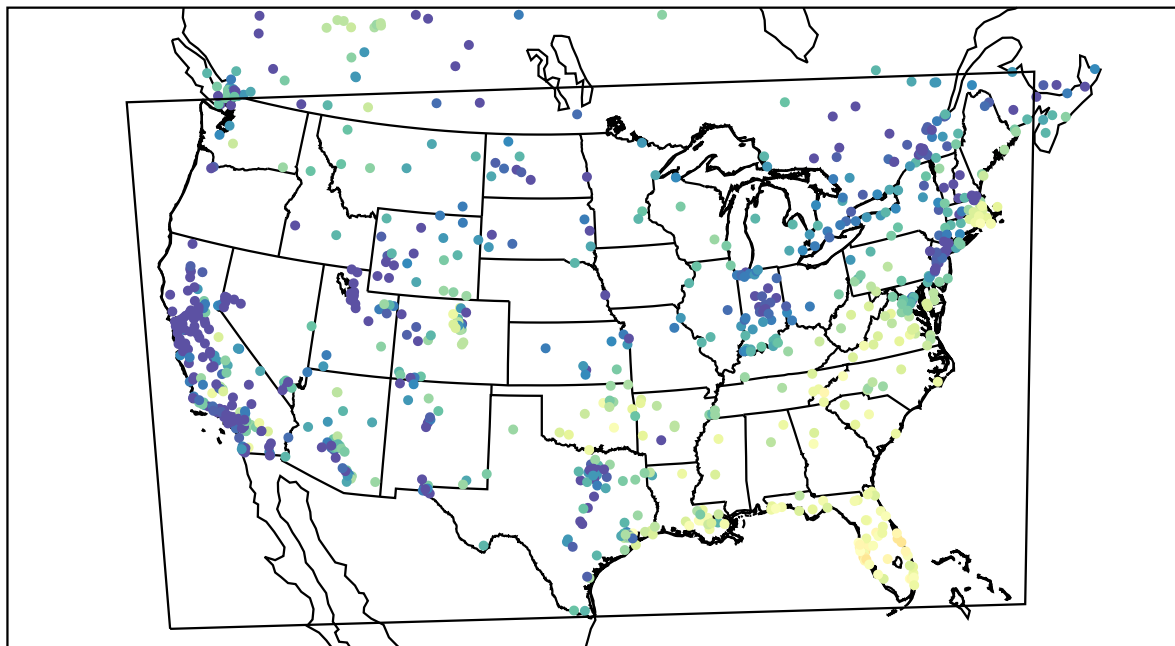
AirNOW (2021-12-02_17:00:00)
