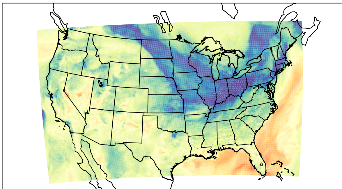
WRF (2021-12-02_22:00:00)
