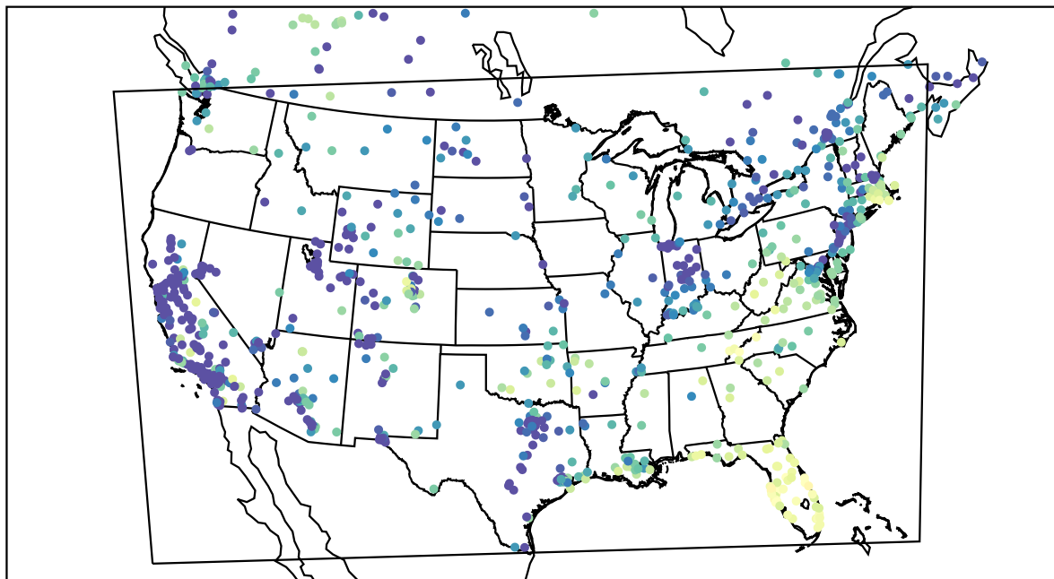
AirNOW (2021-12-02_16:00:00)
