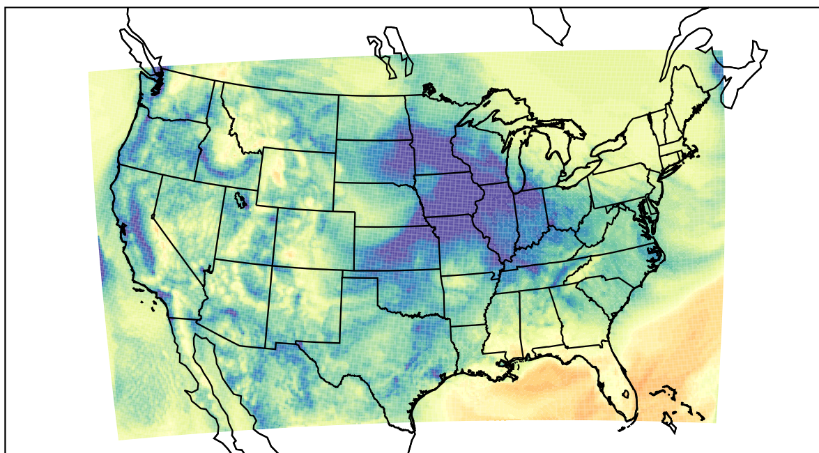
WRF (2021-12-03_17:00:00)
