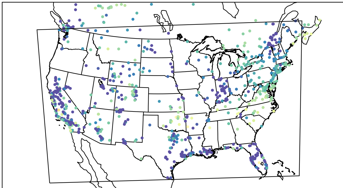
AirNOW (2021-12-03_04:00:00)
