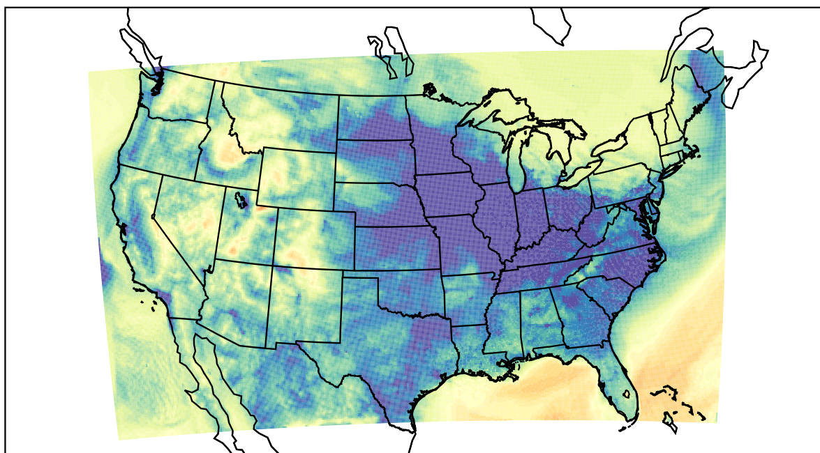
WRF (2021-12-03_13:00:00)
