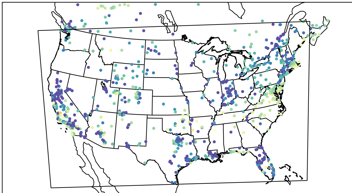
AirNOW (2021-12-03_01:00:00)
