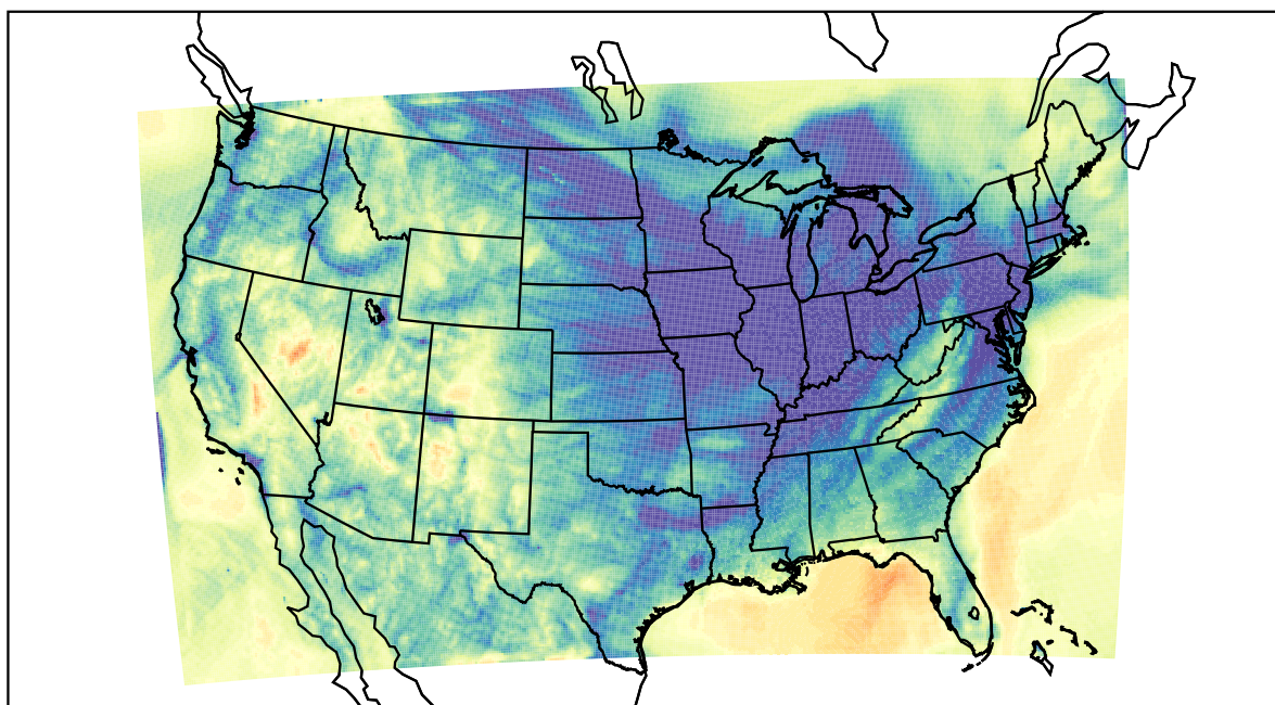
WRF (2021-12-02_09:00:00)
