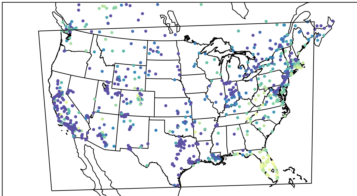
AirNOW (2021-12-02_15:00:00)
