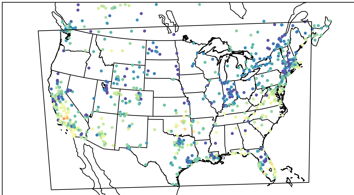
AirNOW (2021-12-02_23:00:00)
