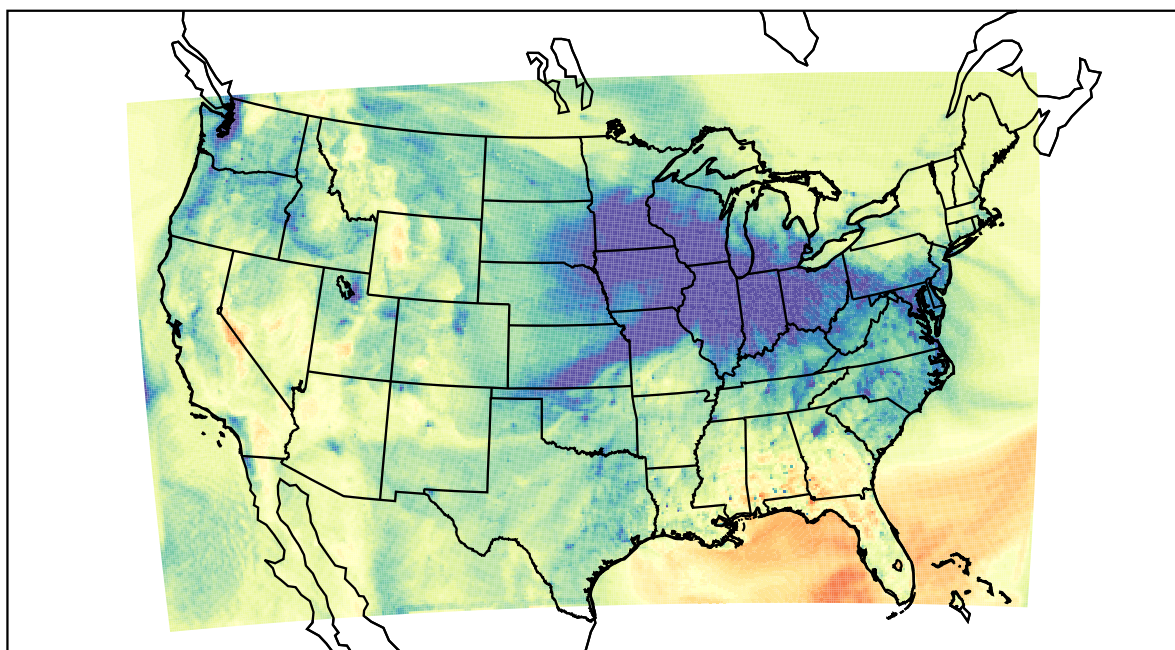
WRF (2021-12-03_23:00:00)
