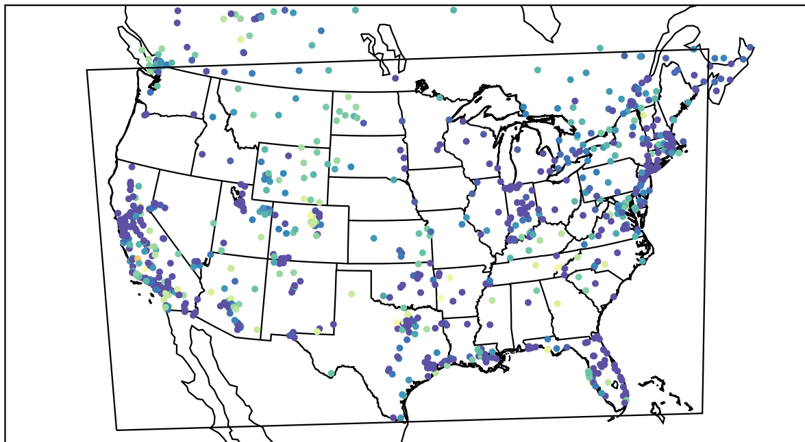
AirNOW (2021-12-02_02:00:00)
