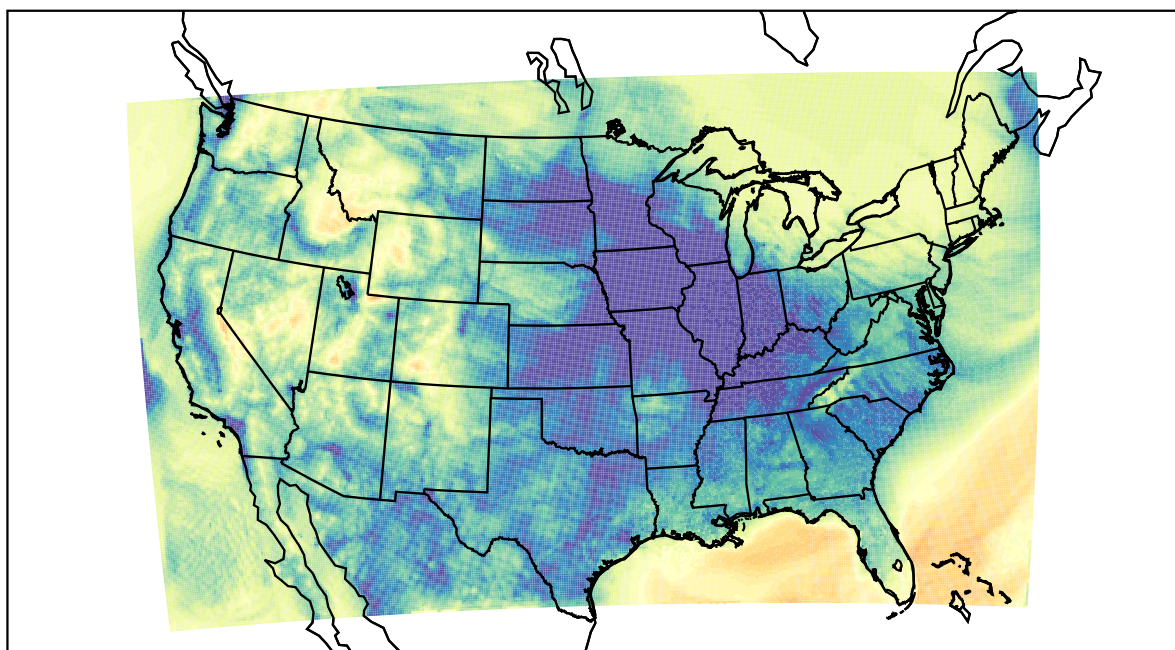
WRF (2021-12-03_15:00:00)
