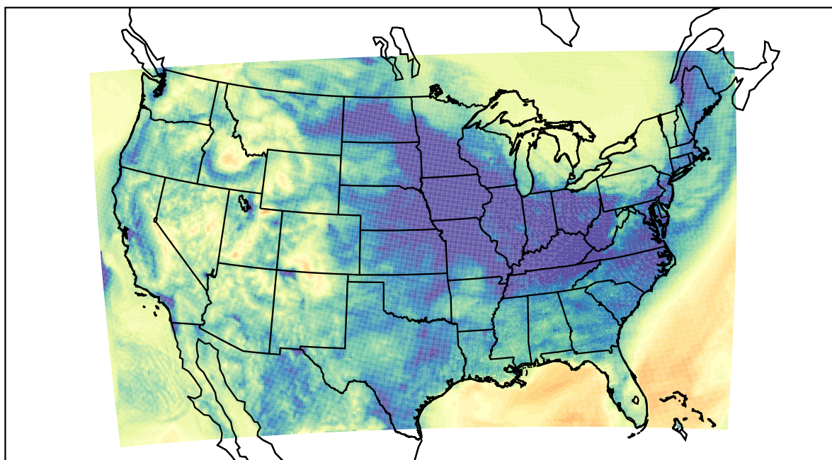
WRF (2021-12-03_09:00:00)
