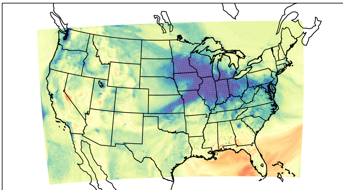
WRF (2021-12-03_22:00:00)
