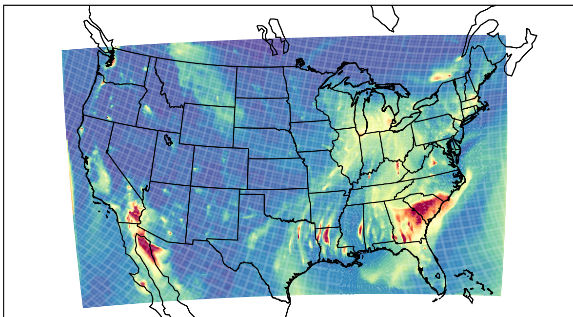
WRF 2021-12-06_04:00:00
