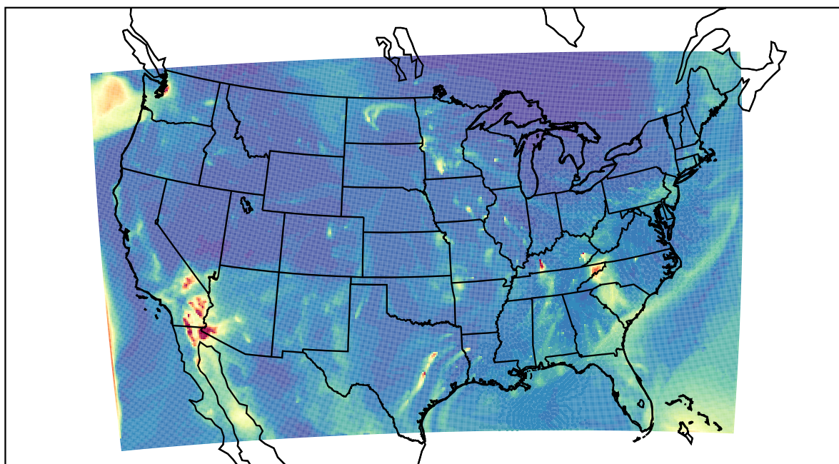
WRF 2021-12-07_08:00:00
