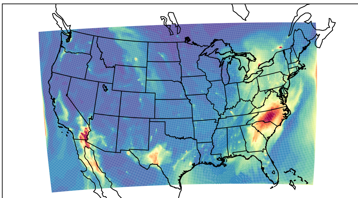
WRF 2021-12-06_13:00:00
