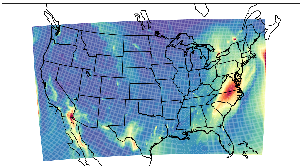
WRF 2021-12-06_16:00:00
