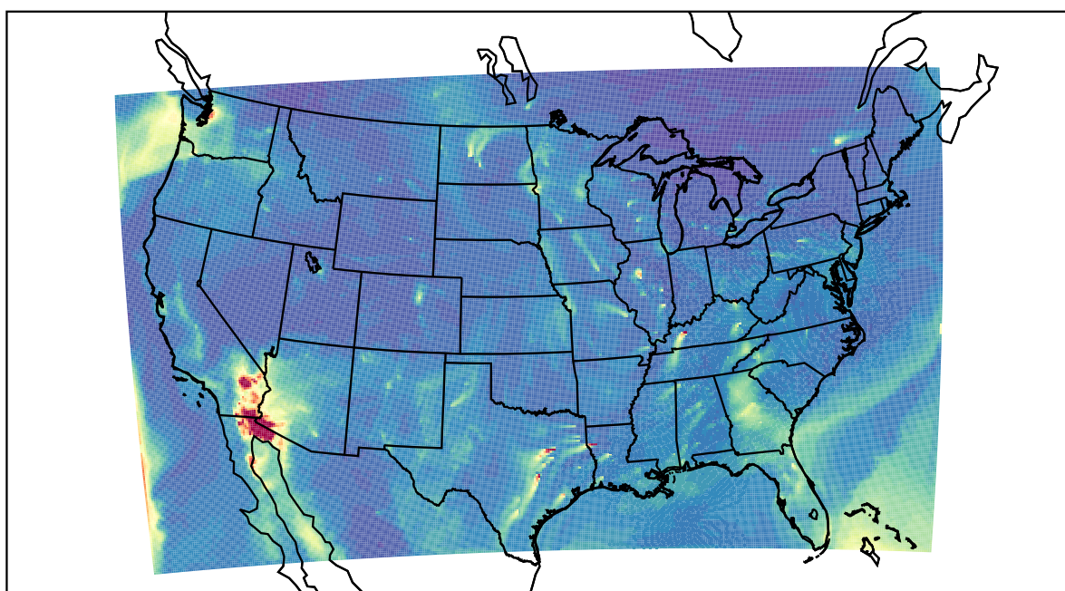
WRF 2021-12-07_15:00:00
