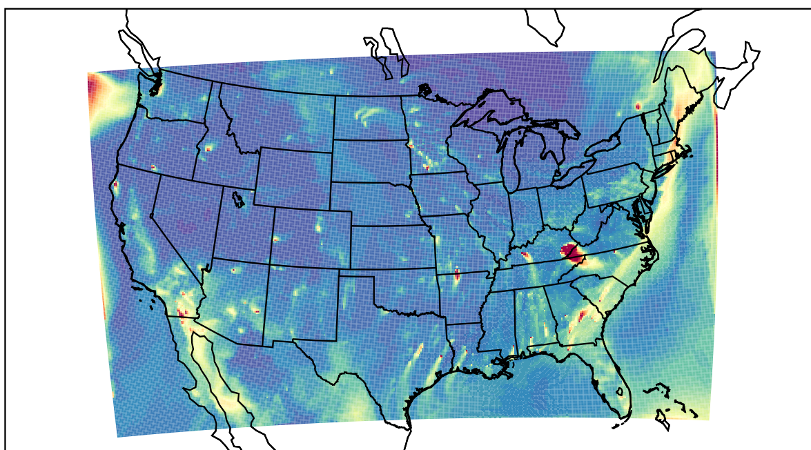
WRF 2021-12-07_02:00:00
