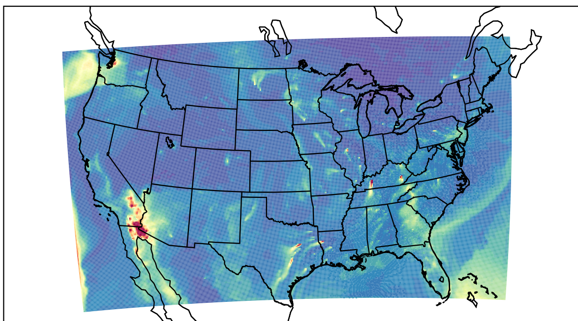
WRF 2021-12-07_13:00:00
