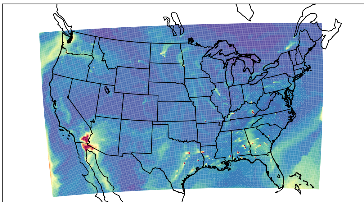
WRF 2021-12-07_19:00:00
