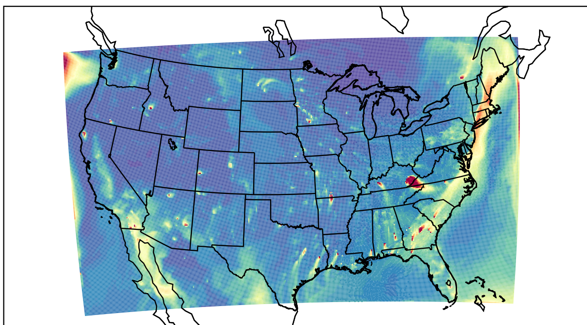
WRF 2021-12-07_01:00:00
