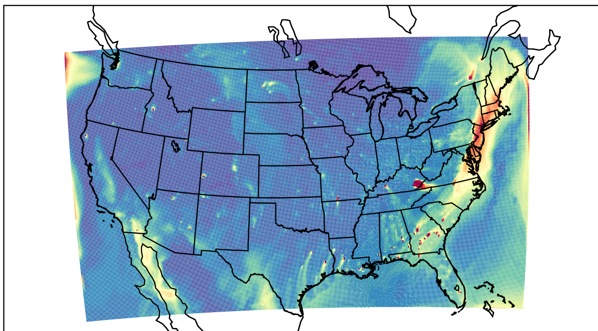
WRF 2021-12-06_23:00:00
