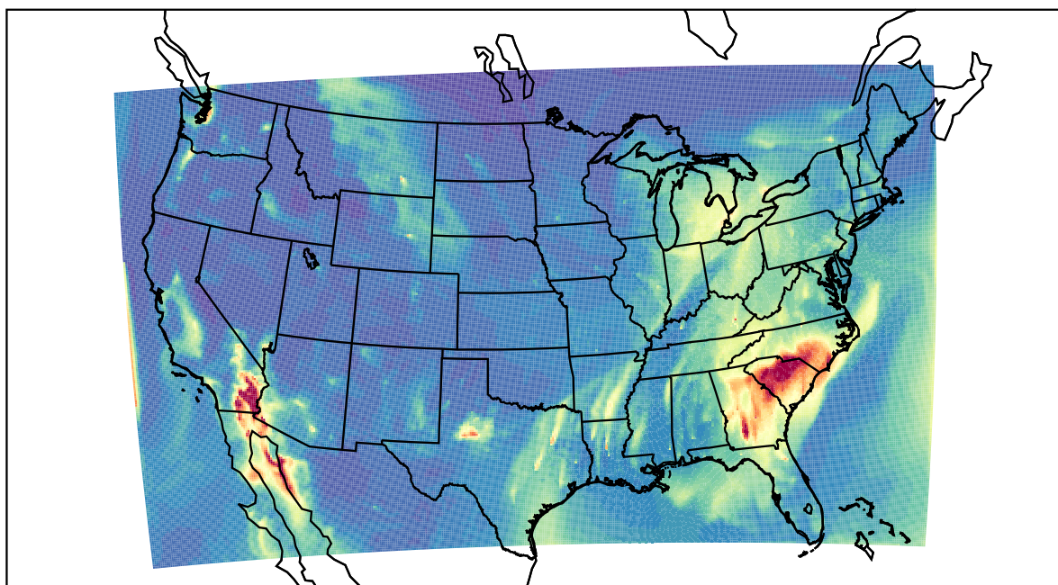
WRF 2021-12-06_08:00:00
