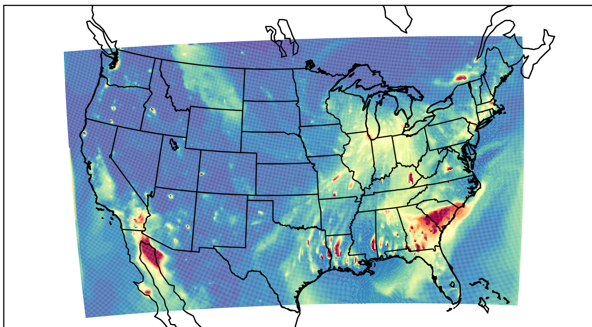
WRF 2021-12-06_02:00:00
