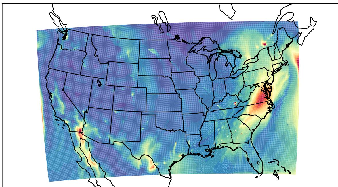
WRF 2021-12-06_17:00:00
