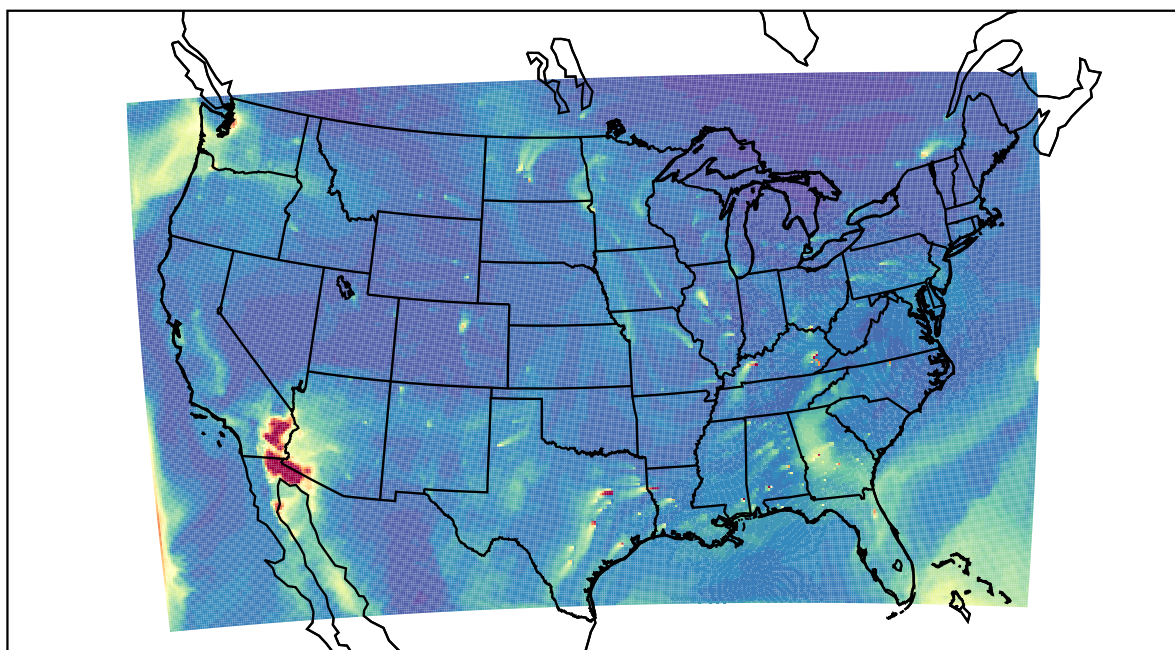
WRF 2021-12-07_17:00:00
