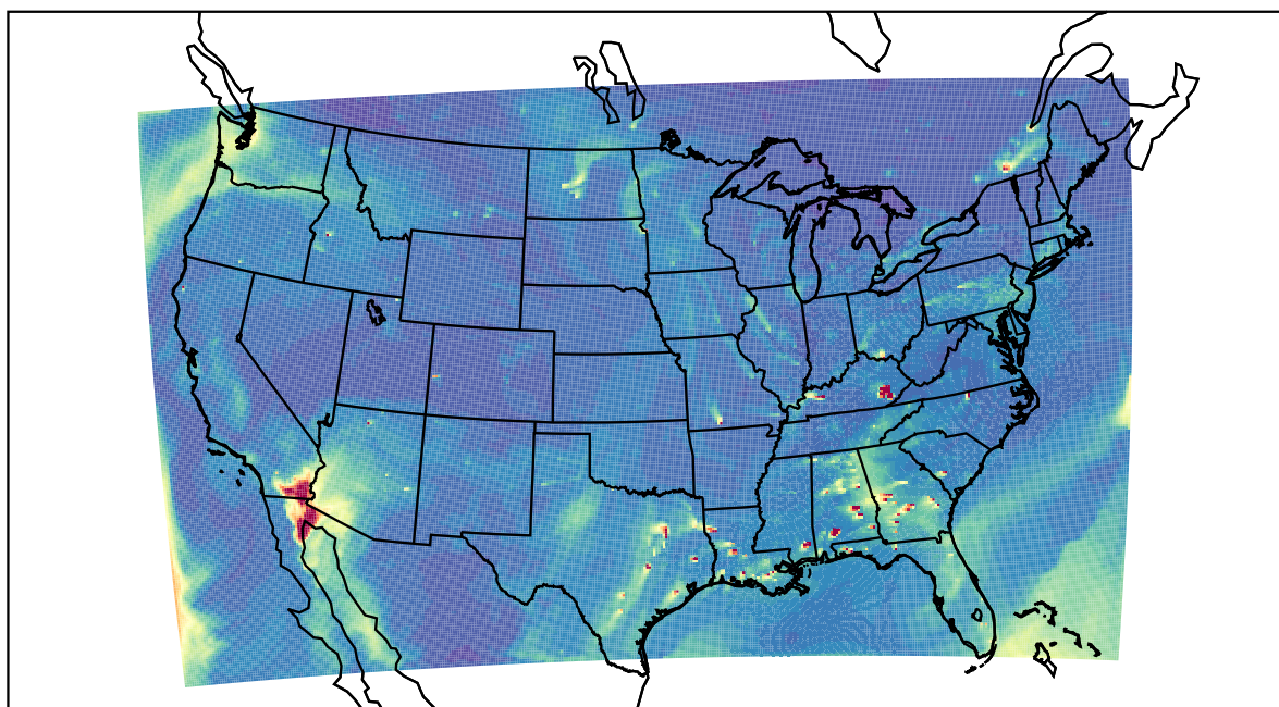
WRF 2021-12-07_21:00:00
