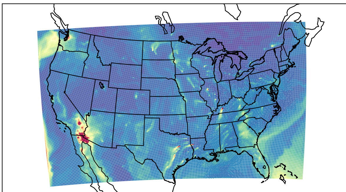
WRF 2021-12-07_14:00:00
