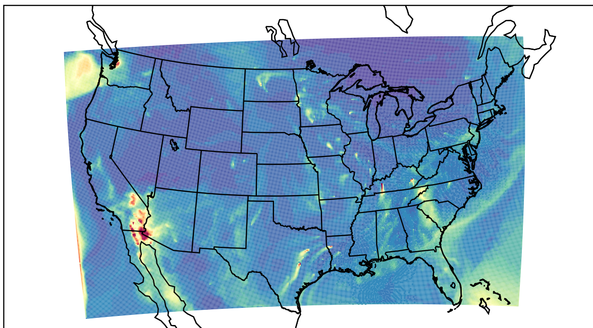
WRF 2021-12-07_10:00:00
