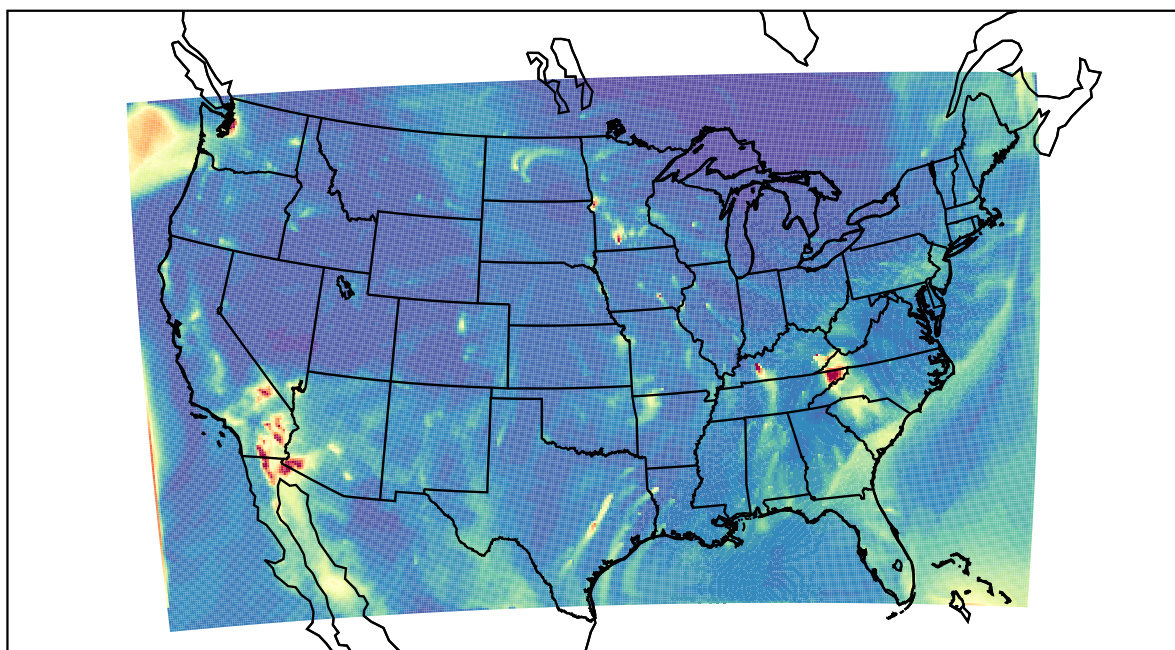
WRF 2021-12-07_06:00:00
