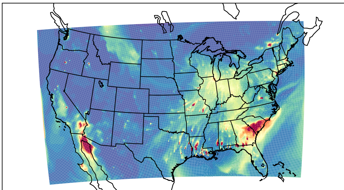
WRF 2021-12-06_00:00:00
