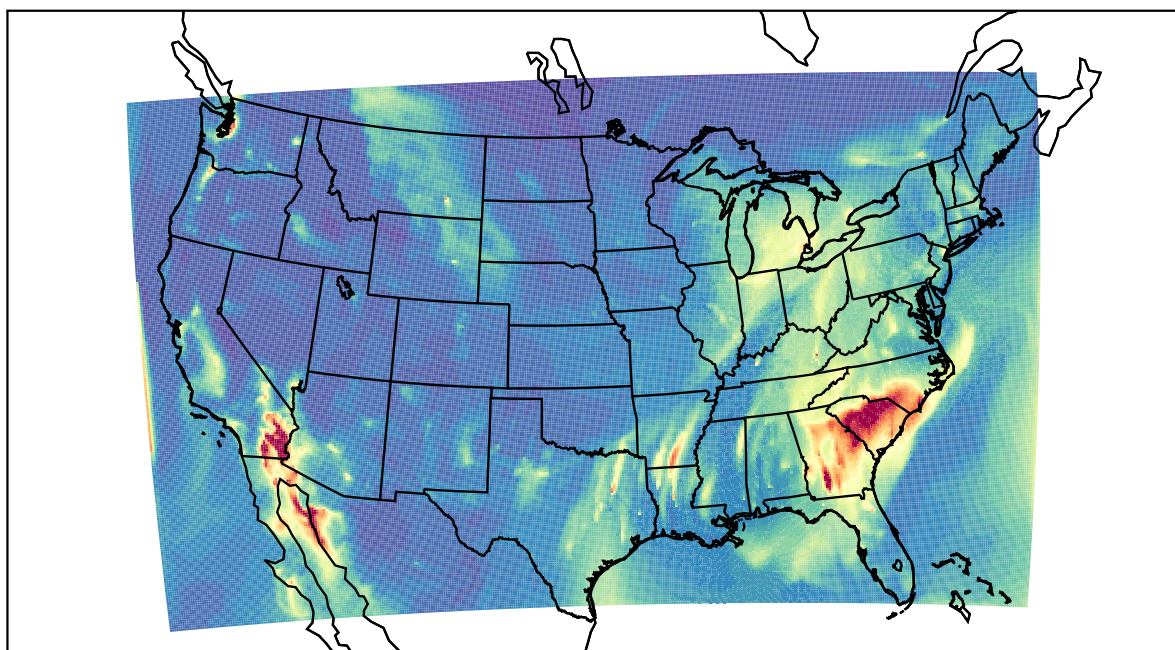
WRF 2021-12-06_07:00:00
