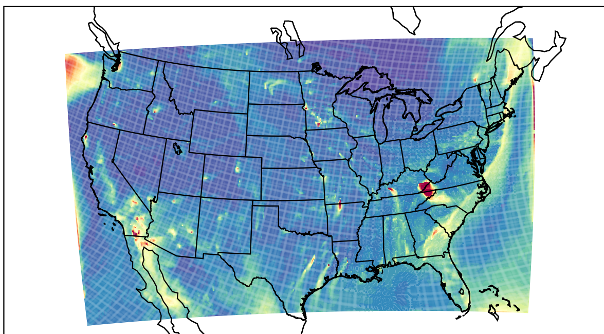
WRF 2021-12-07_03:00:00
