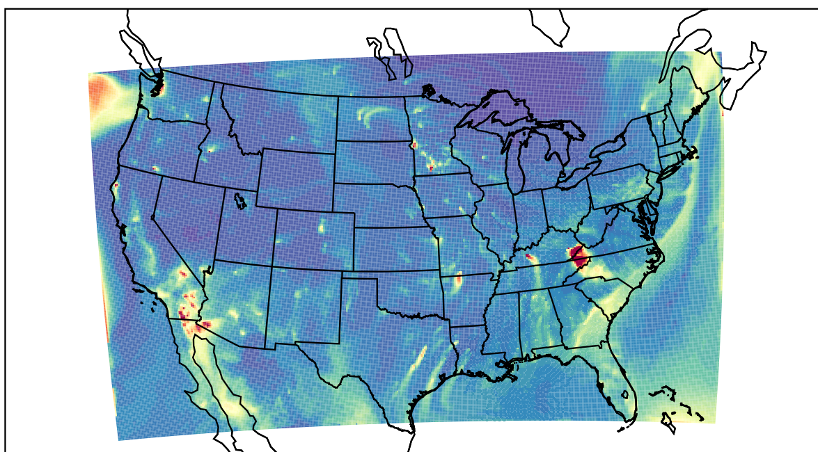
WRF 2021-12-07_04:00:00
