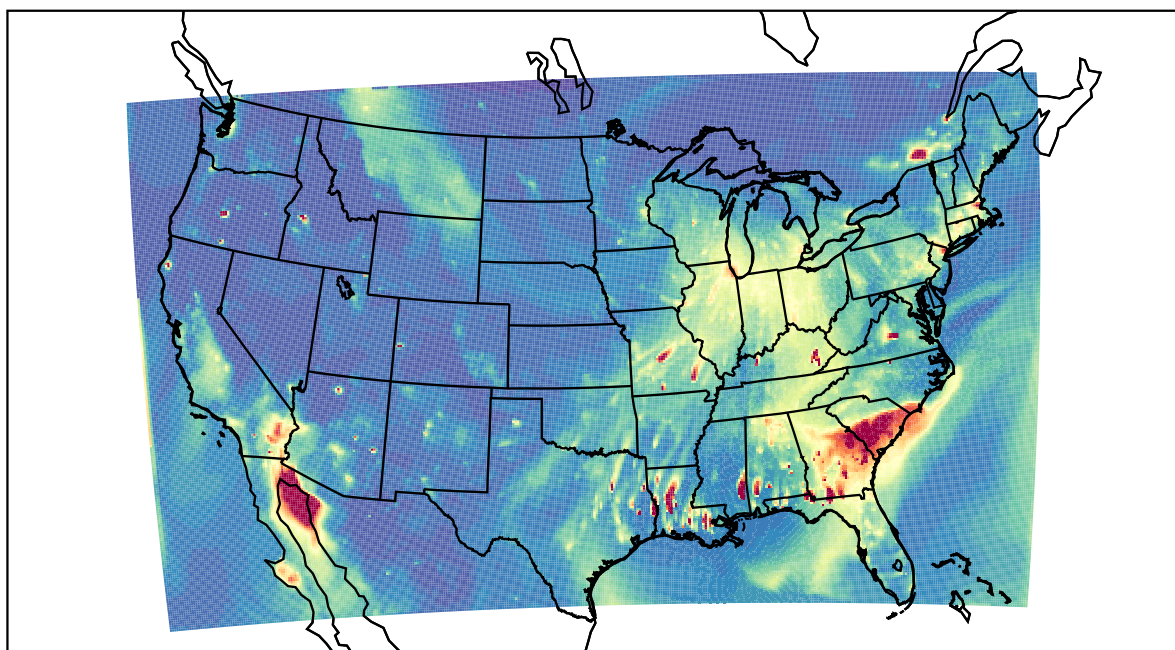
WRF 2021-12-06_01:00:00
