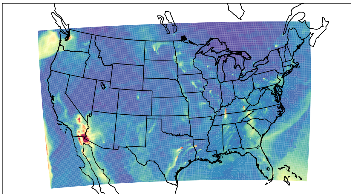
WRF 2021-12-07_12:00:00
