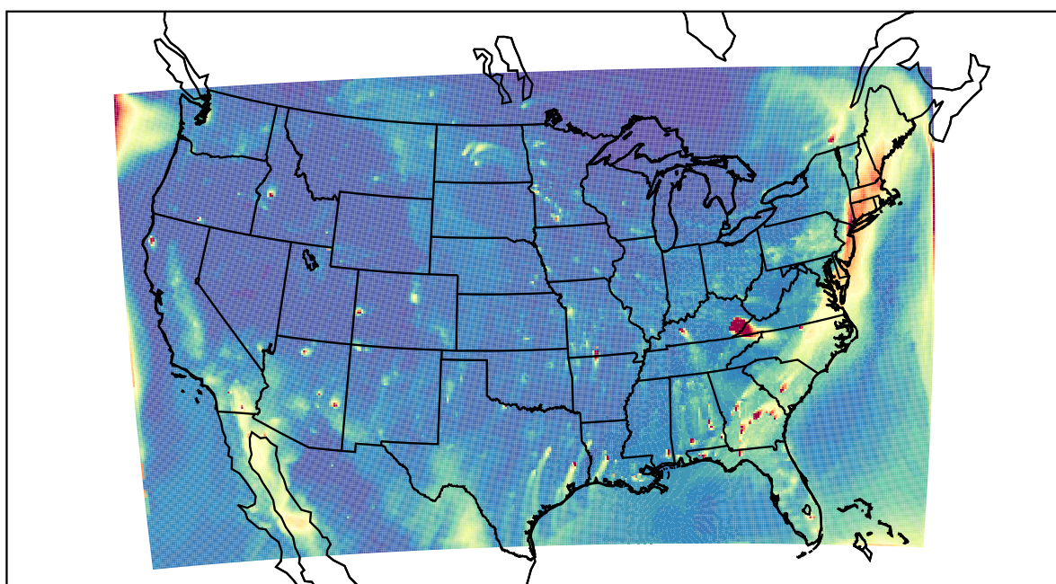
WRF 2021-12-07_00:00:00
