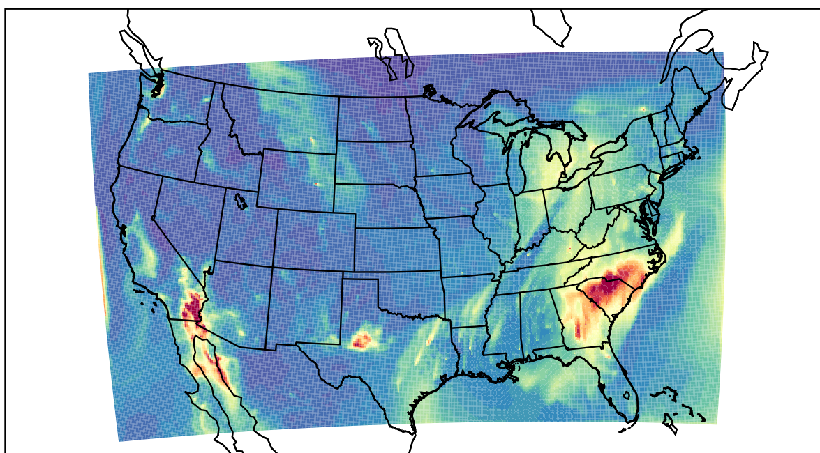
WRF 2021-12-06_09:00:00
