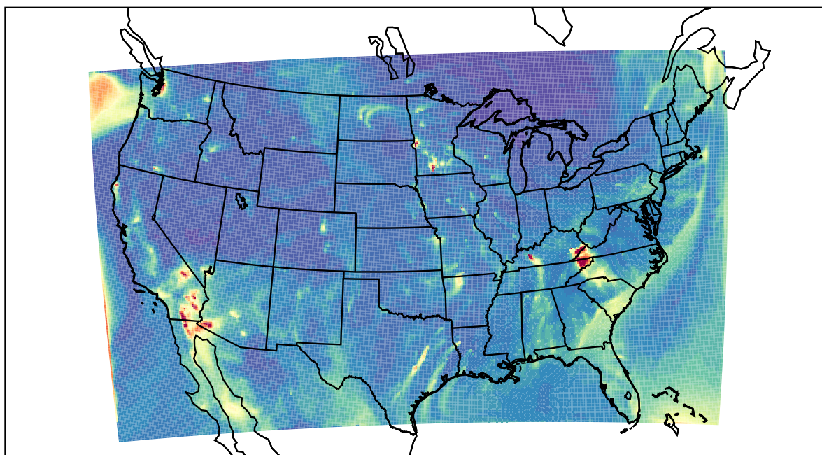
WRF 2021-12-07_05:00:00
