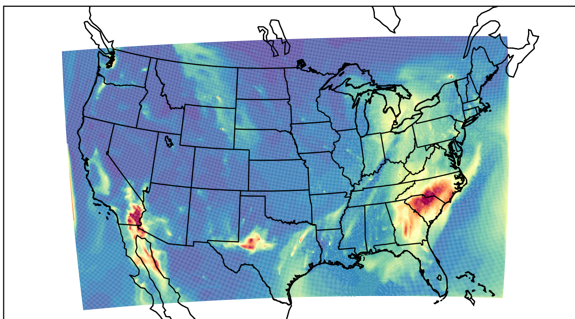
WRF 2021-12-06_10:00:00
