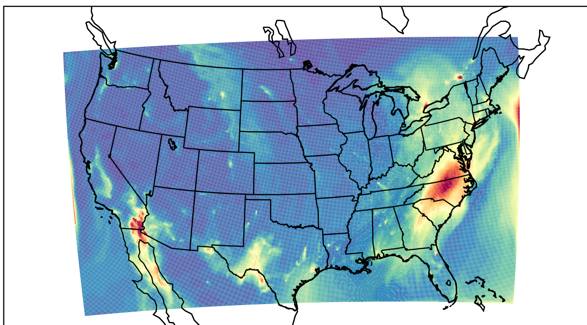
WRF 2021-12-06_15:00:00
