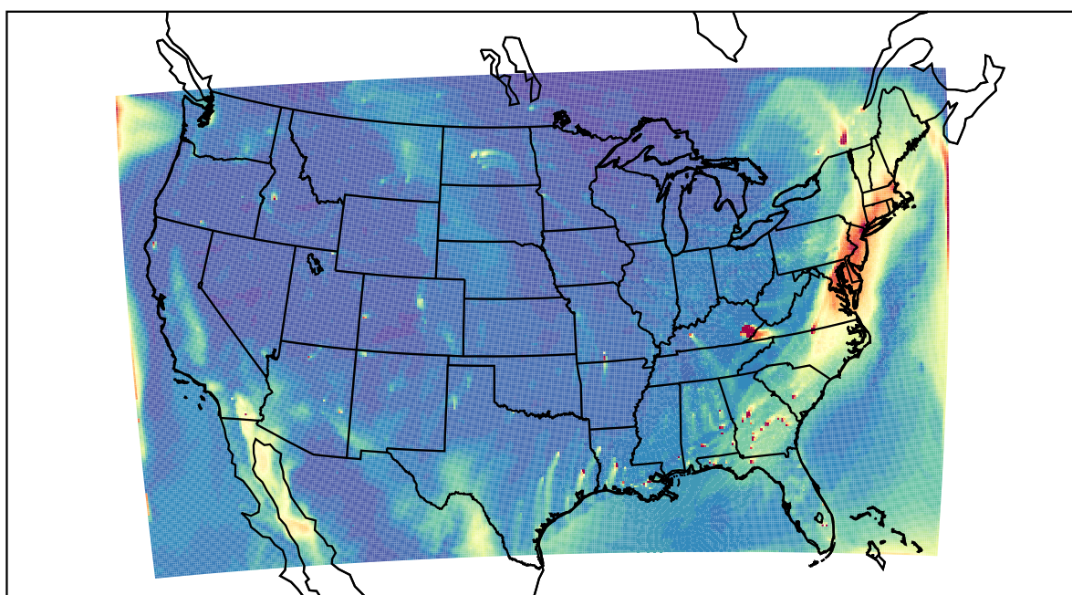
WRF 2021-12-06_22:00:00
