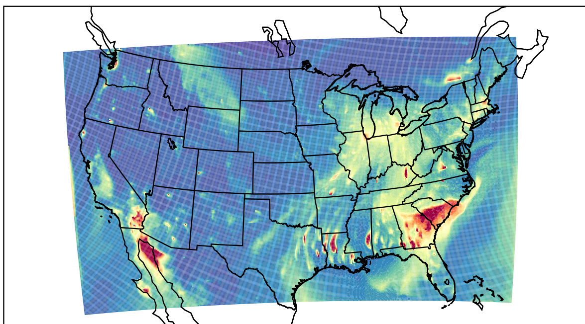
WRF 2021-12-06_03:00:00
