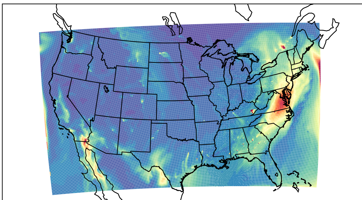
WRF 2021-12-06_18:00:00
