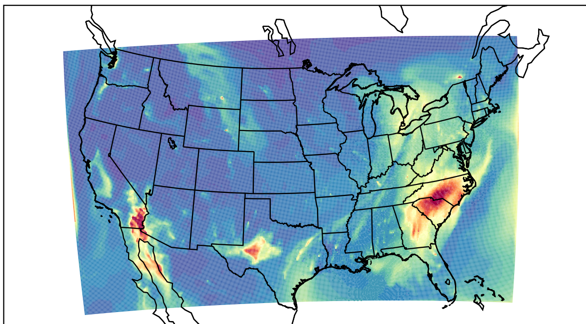
WRF 2021-12-06_11:00:00
