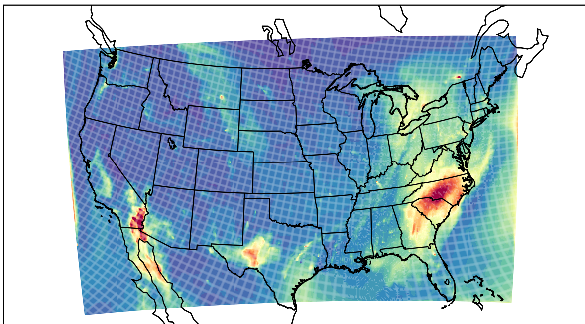
WRF 2021-12-06_12:00:00
