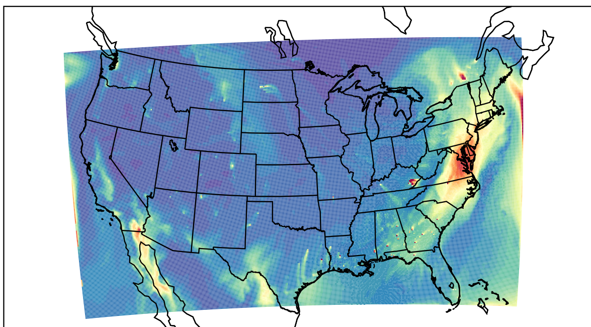
WRF 2021-12-06_19:00:00
