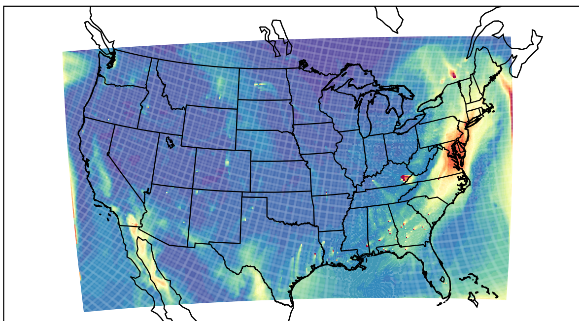
WRF 2021-12-06_20:00:00
