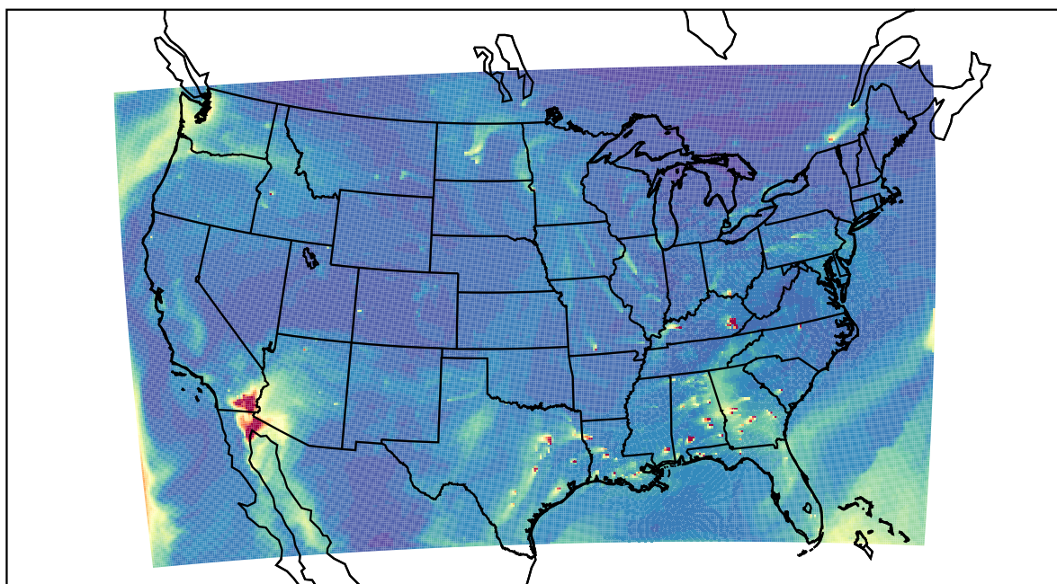
WRF 2021-12-07_20:00:00
