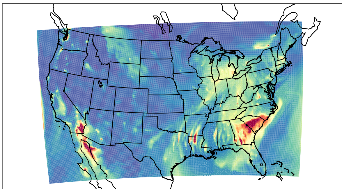
WRF 2021-12-06_05:00:00
