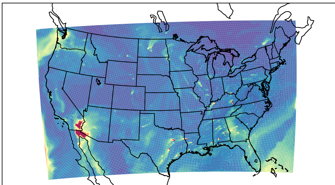
WRF 2021-12-07_18:00:00
