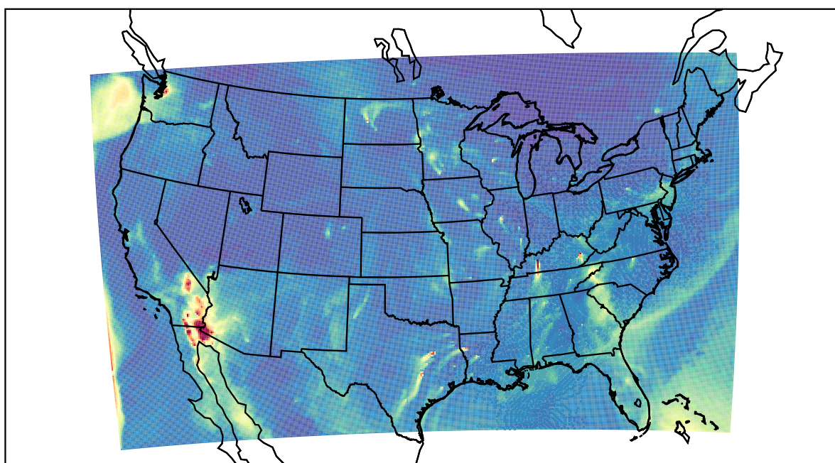
WRF 2021-12-07_11:00:00
