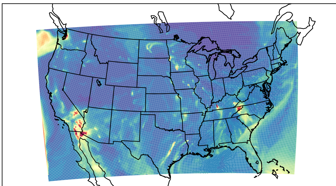
WRF 2021-12-07_07:00:00
