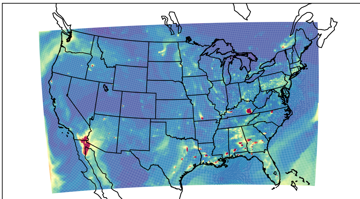
WRF 2021-12-07_23:00:00
