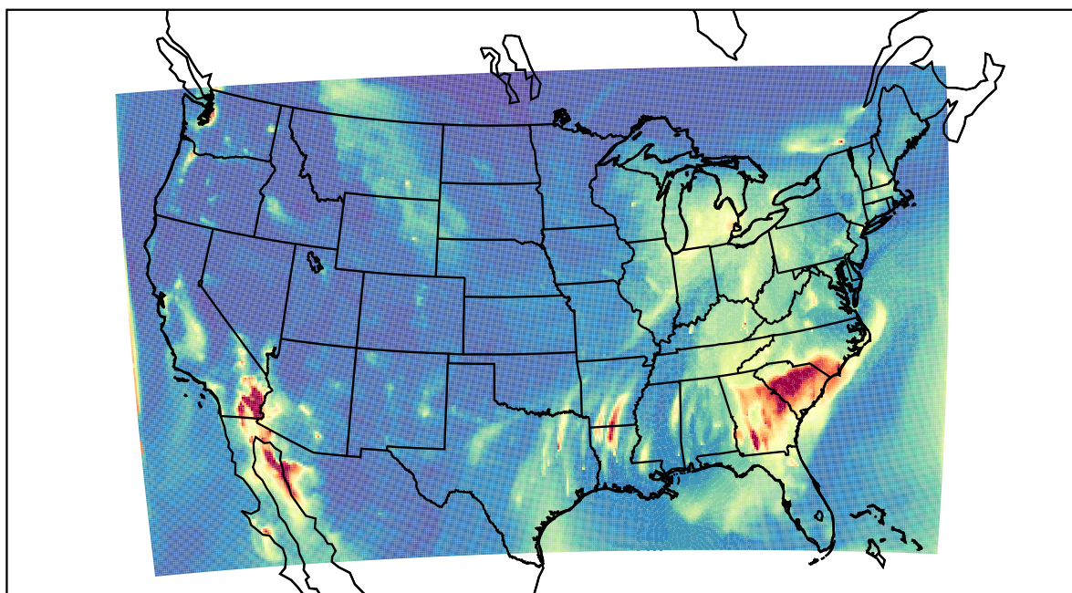
WRF 2021-12-06_06:00:00
