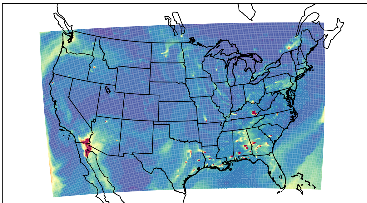
WRF 2021-12-07_22:00:00
