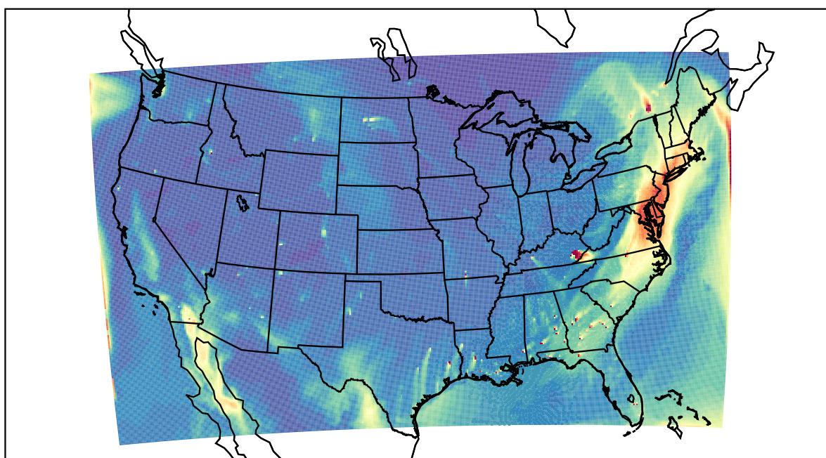
WRF 2021-12-06_21:00:00
