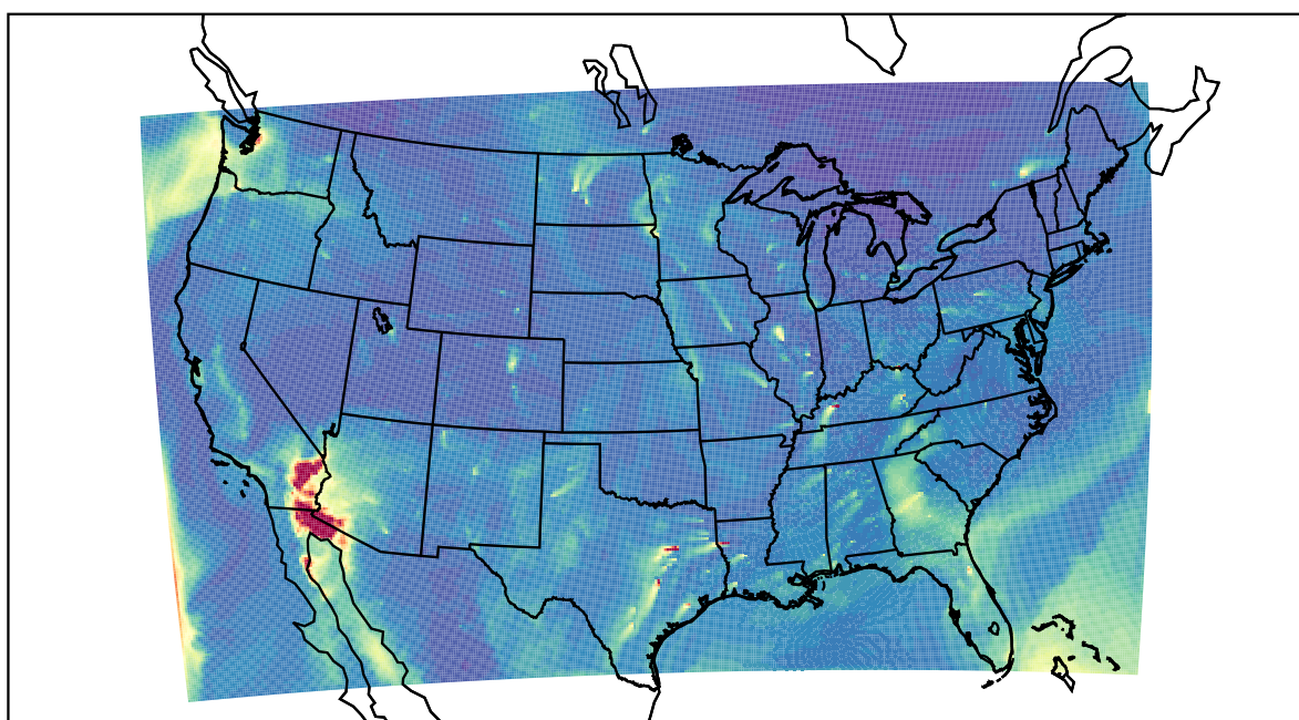
WRF 2021-12-07_16:00:00
