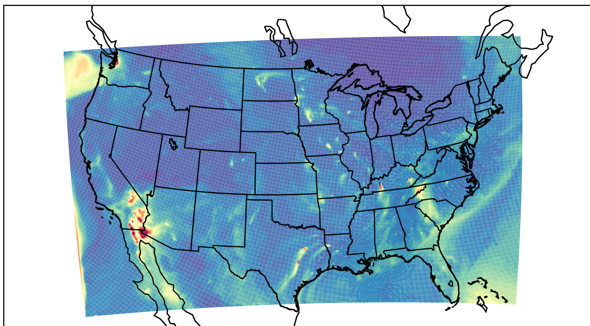
WRF 2021-12-07_09:00:00
