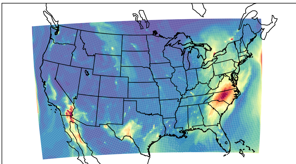
WRF 2021-12-06_14:00:00
