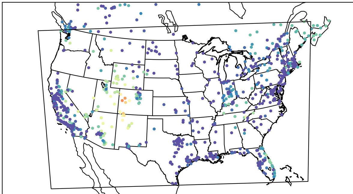
AirNOW (2021-12-15_13:00:00)
