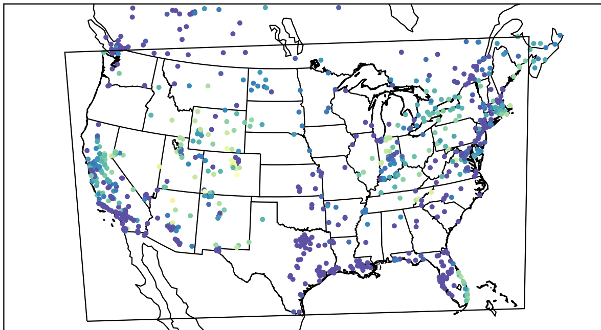
AirNOW (2021-12-16_13:00:00)
