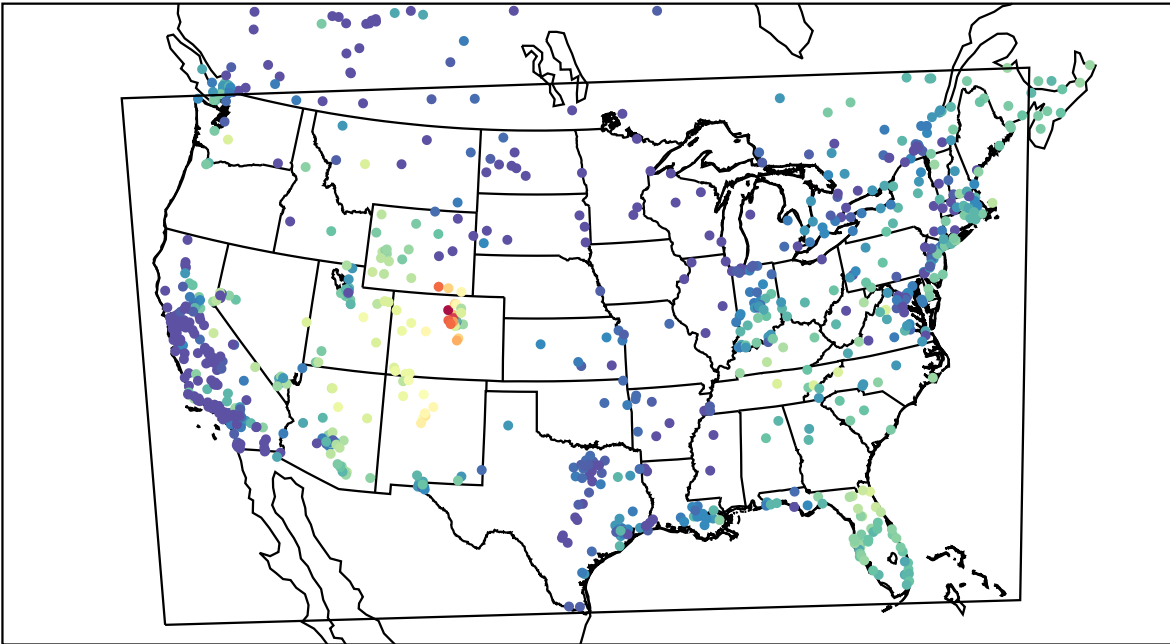
AirNOW (2021-12-15_16:00:00)
