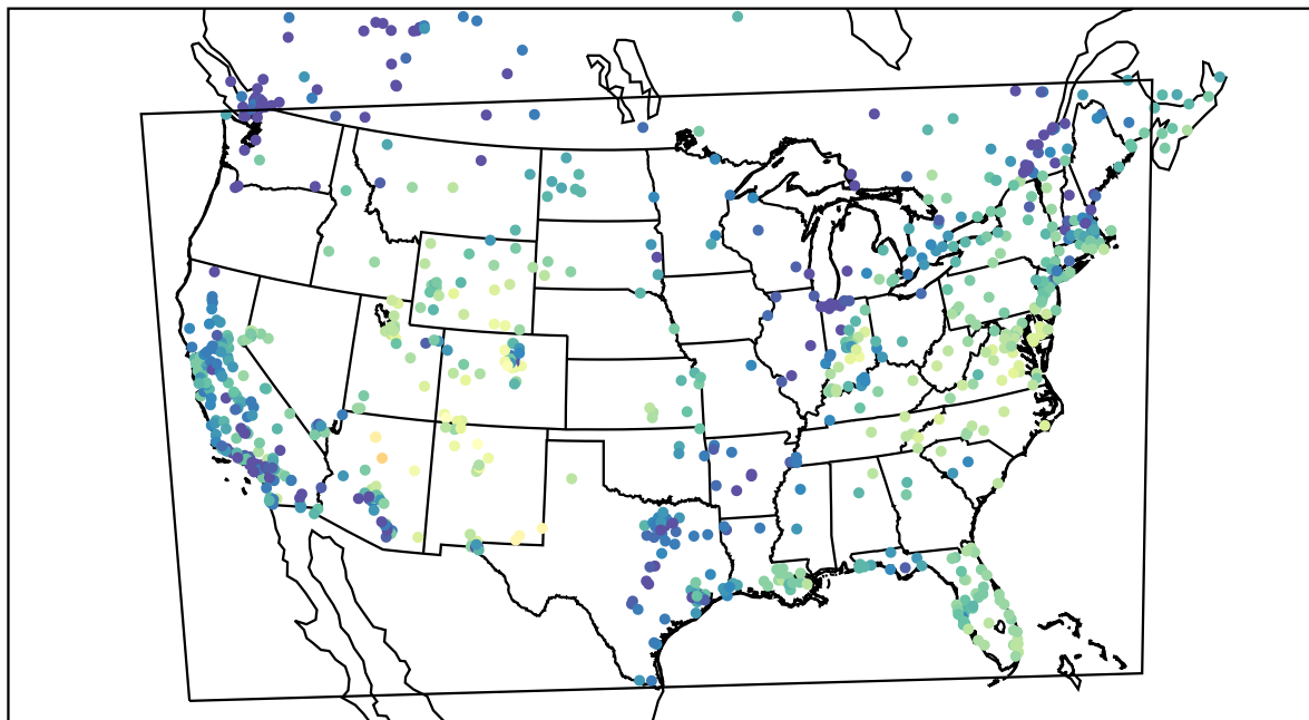
AirNOW (2021-12-16_18:00:00)
