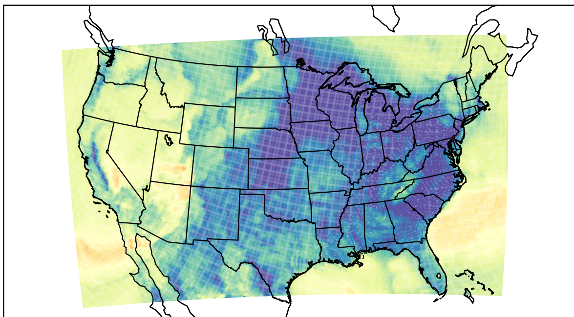
WRF (2021-12-15_10:00:00)
