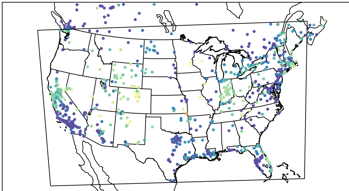
AirNOW (2021-12-16_04:00:00)
