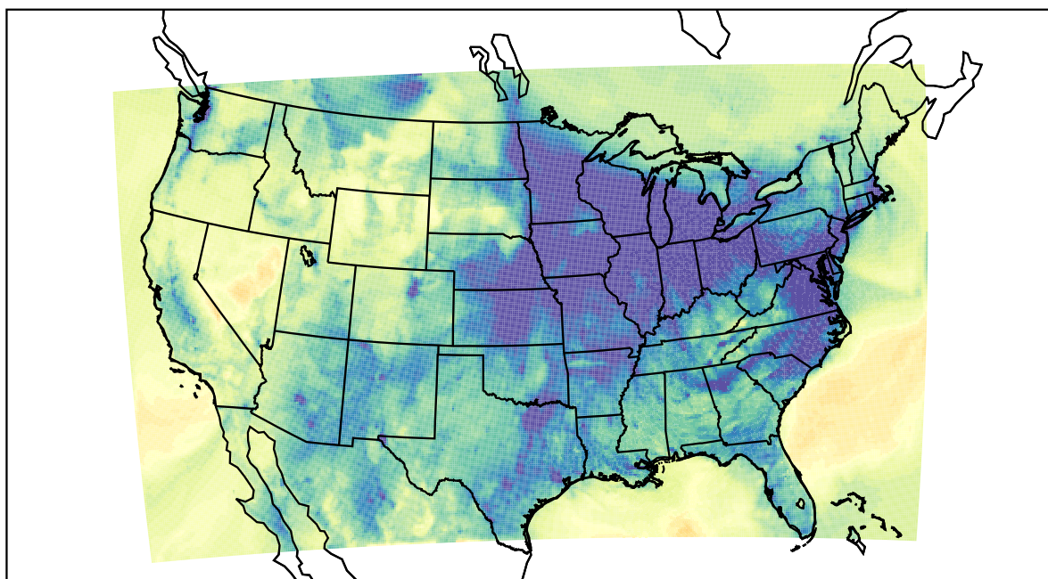
WRF (2021-12-15_01:00:00)
