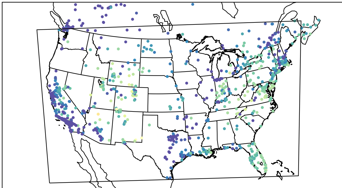
AirNOW (2021-12-16_16:00:00)
