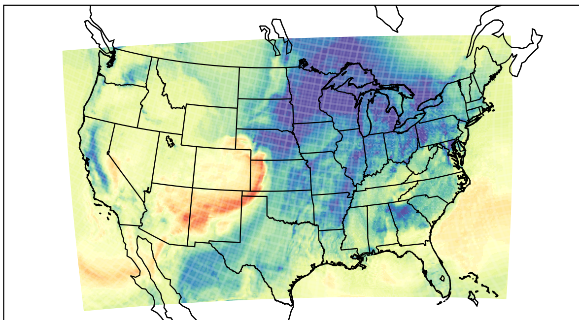
WRF (2021-12-15_18:00:00)
