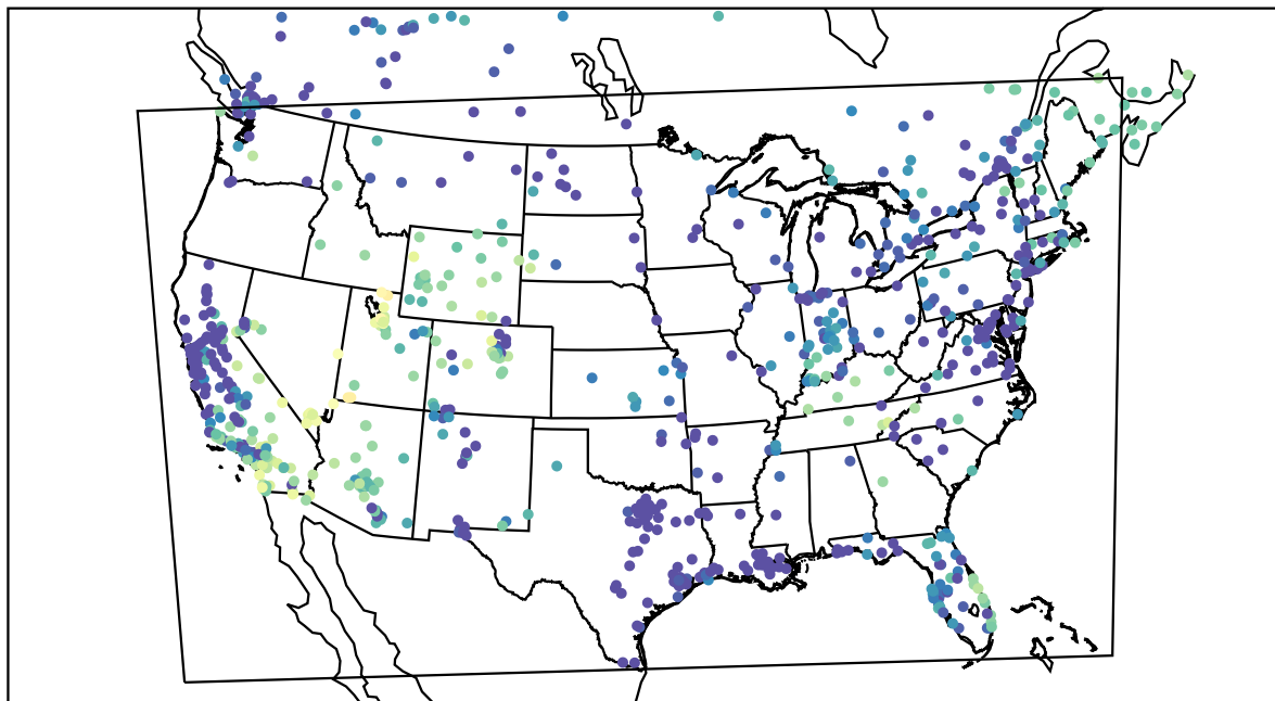
AirNOW (2021-12-15_04:00:00)
