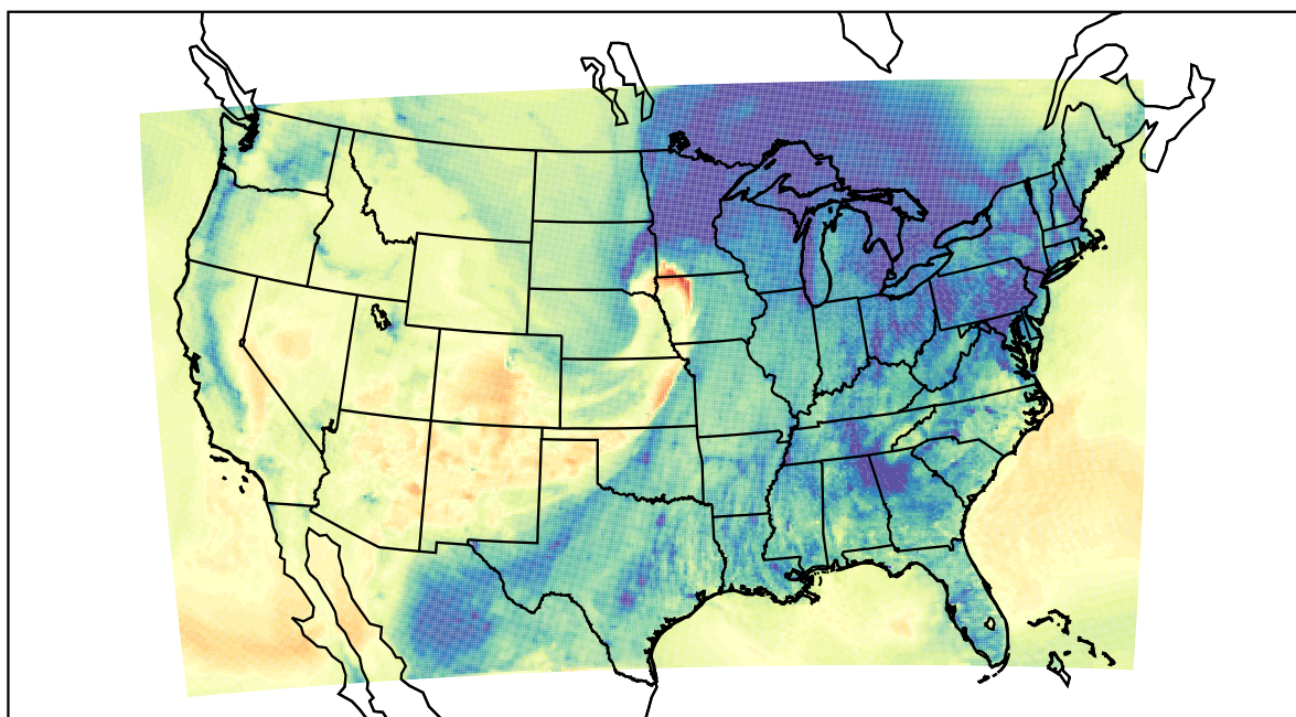
WRF (2021-12-16_00:00:00)
