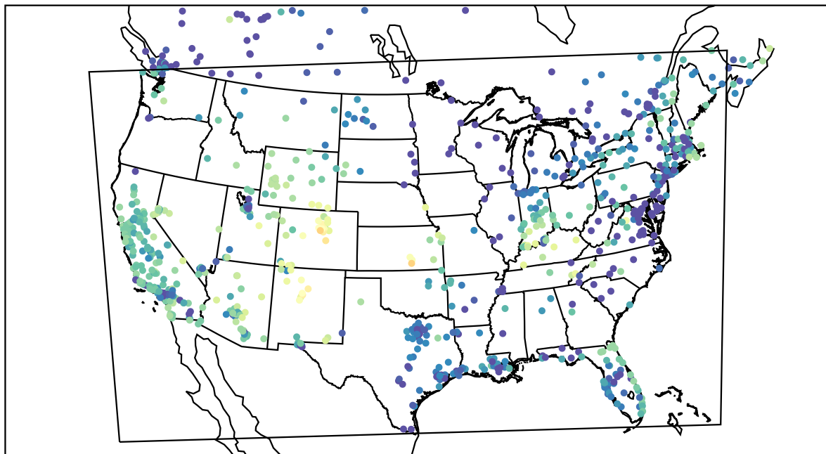
AirNOW (2021-12-16_00:00:00)
