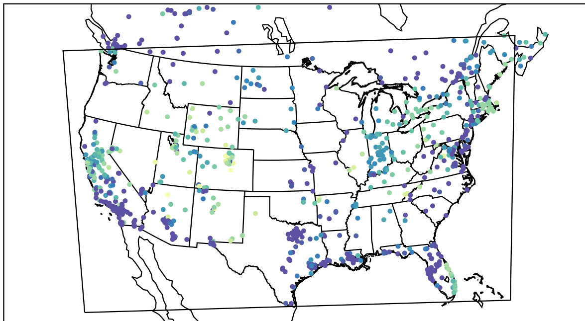
AirNOW (2021-12-16_09:00:00)
