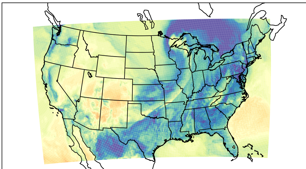
WRF (2021-12-16_08:00:00)
