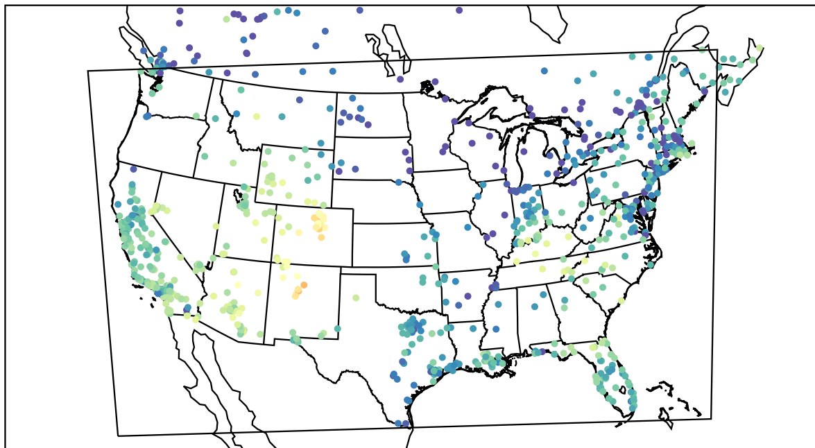
AirNOW (2021-12-15_21:00:00)
