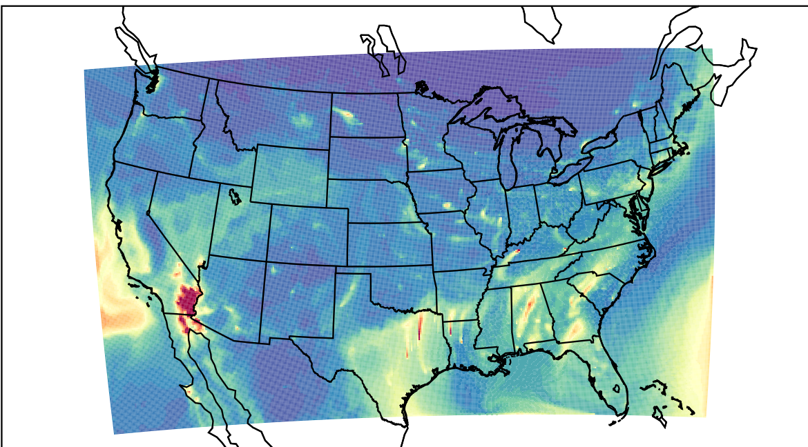
WRF 2021-12-17_12:00:00
