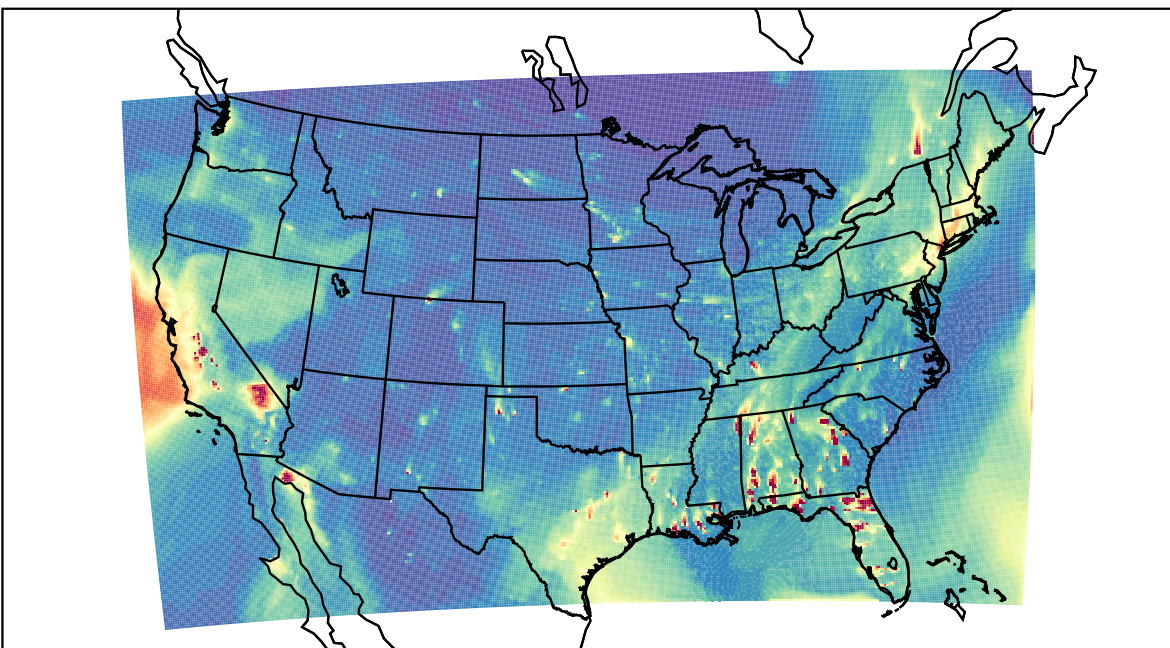
WRF 2021-12-17_00:00:00
