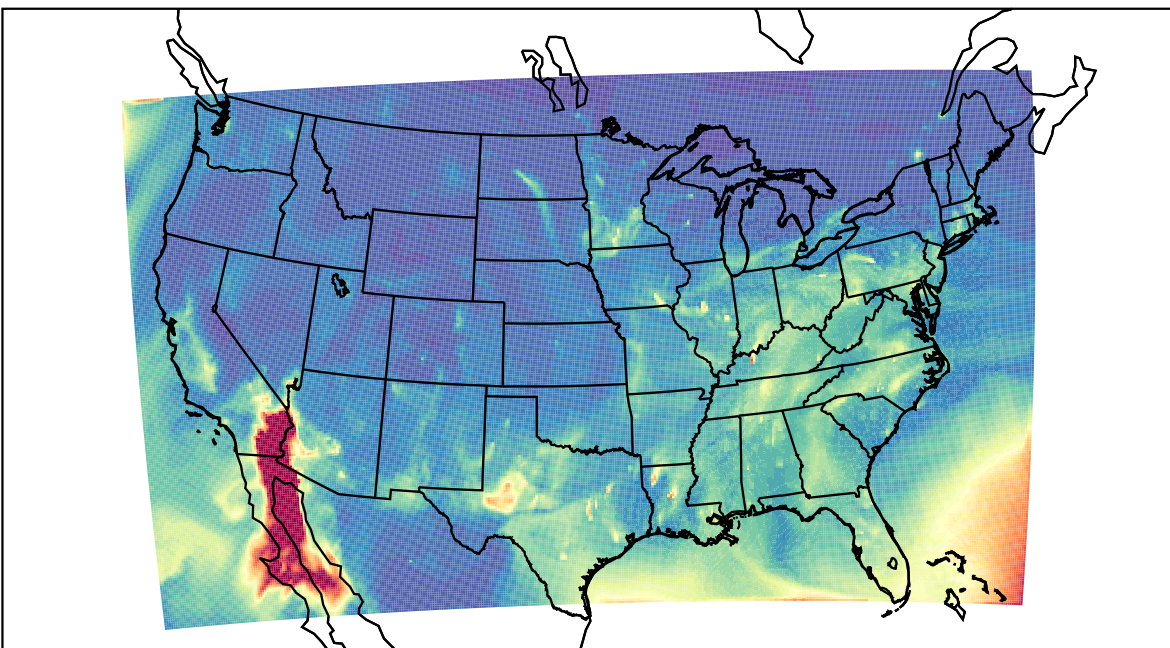
WRF 2021-12-18_12:00:00
