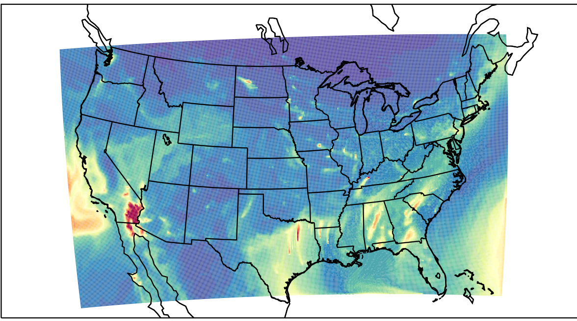
WRF 2021-12-17_11:00:00
