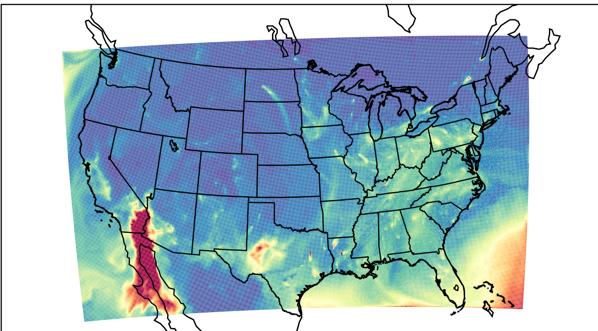
WRF 2021-12-18_15:00:00
