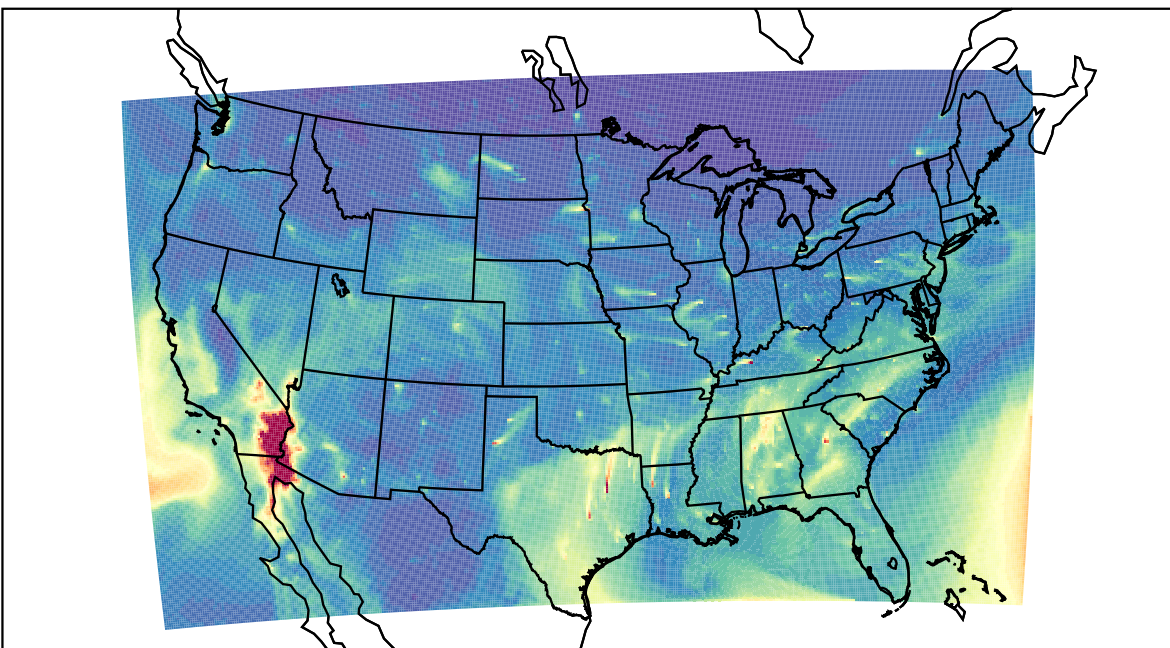
WRF 2021-12-17_16:00:00
