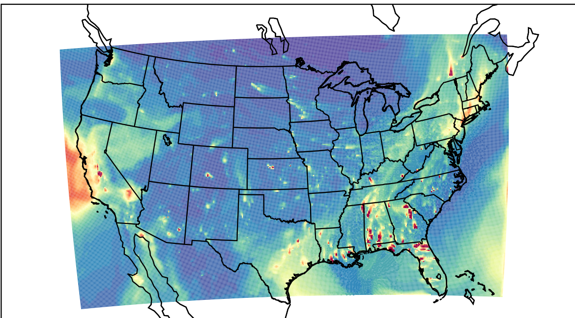
WRF 2021-12-17_01:00:00
