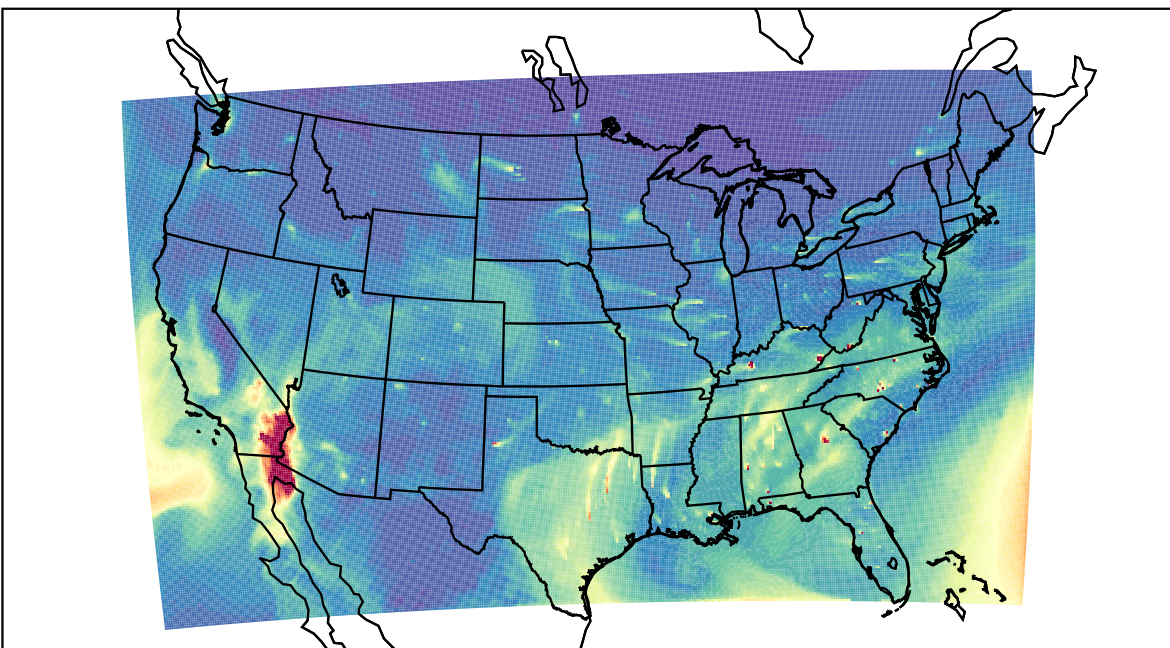
WRF 2021-12-17_18:00:00
