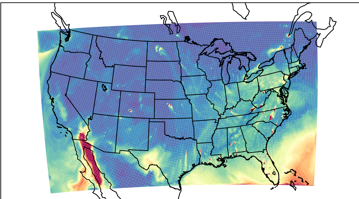
WRF 2021-12-18_22:00:00
