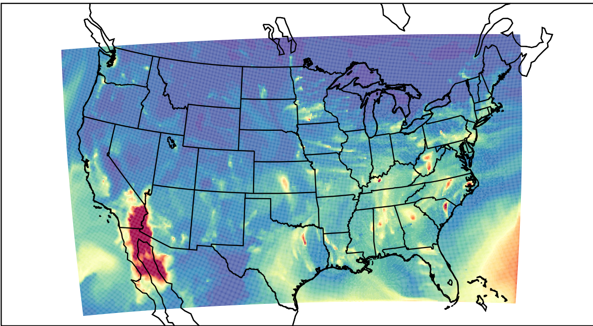
WRF 2021-12-18_05:00:00
