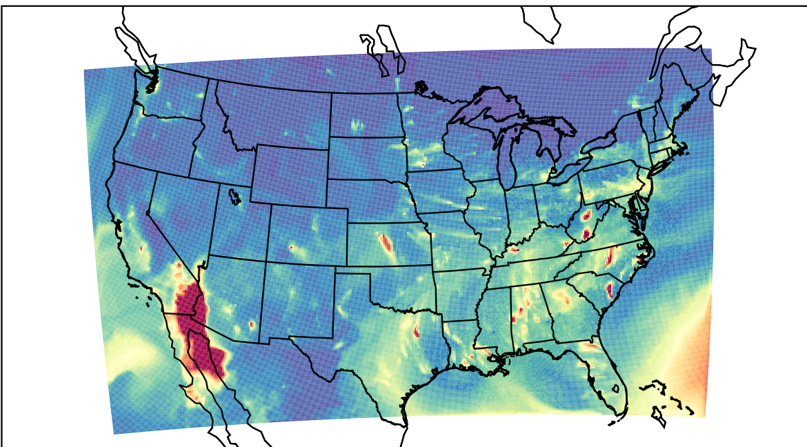
WRF 2021-12-18_03:00:00
