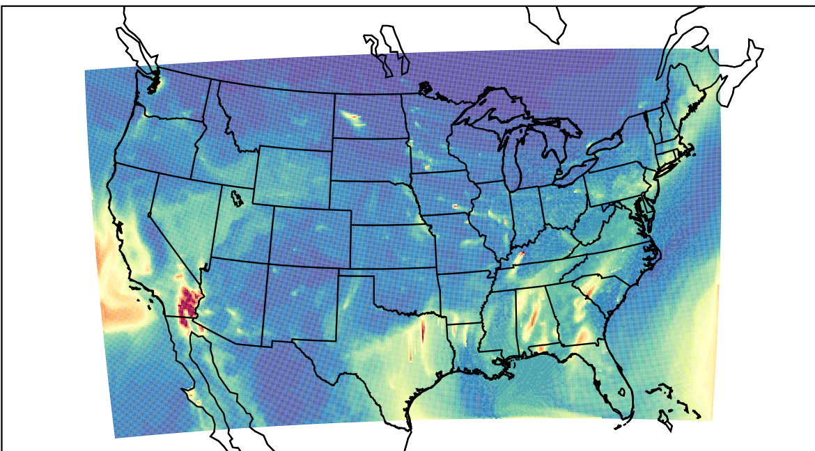
WRF 2021-12-17_10:00:00
