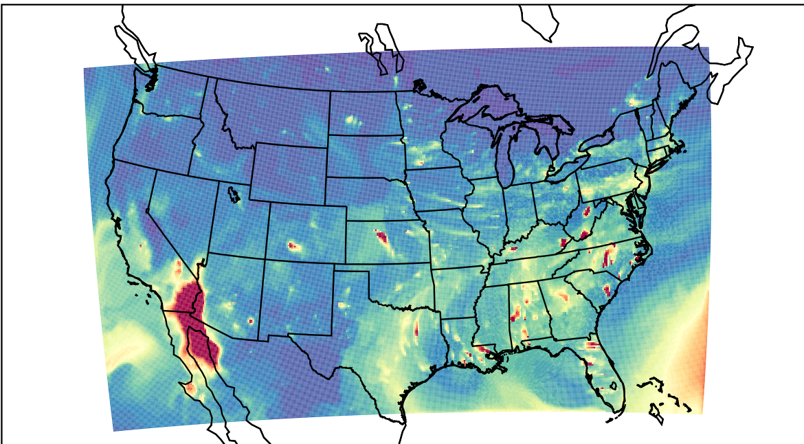
WRF 2021-12-18_01:00:00
