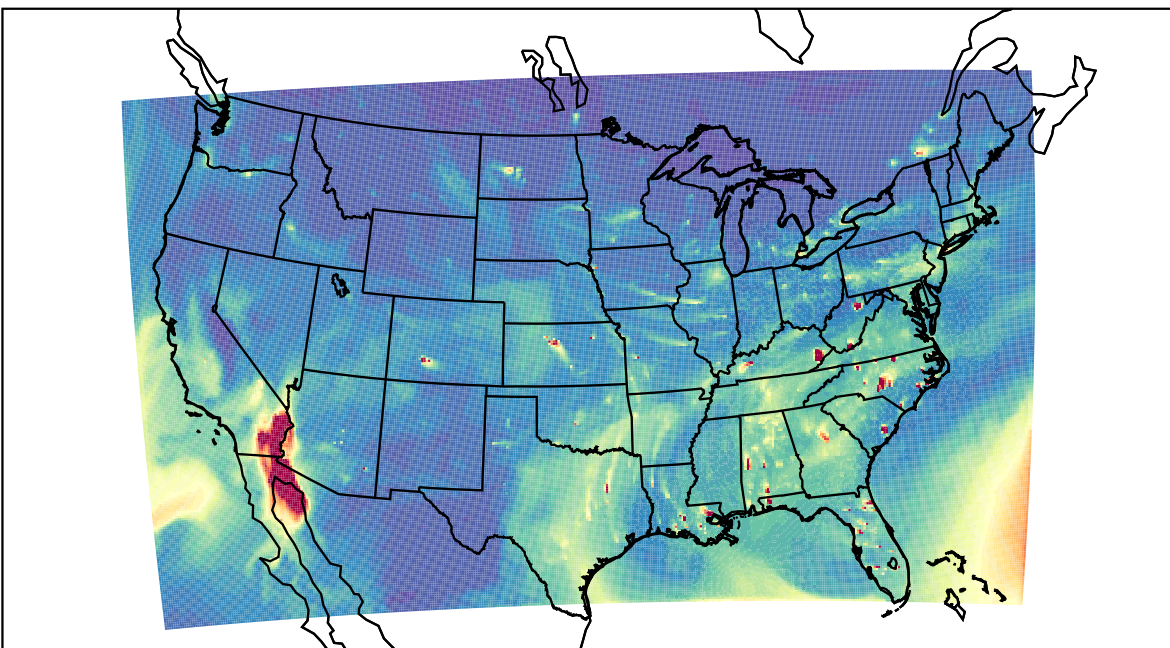
WRF 2021-12-17_22:00:00
