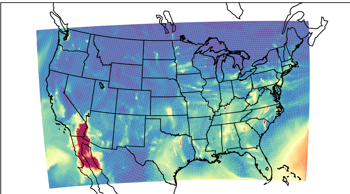
WRF 2021-12-18_06:00:00
