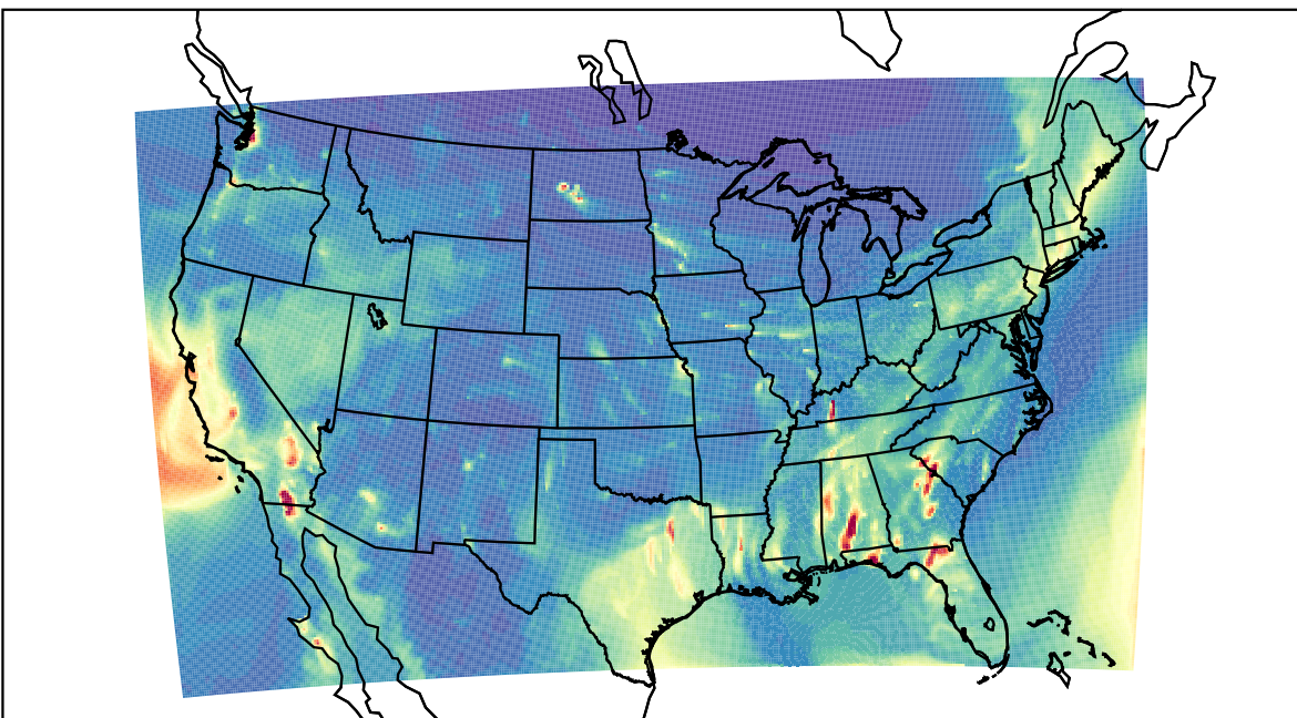
WRF 2021-12-17_06:00:00
