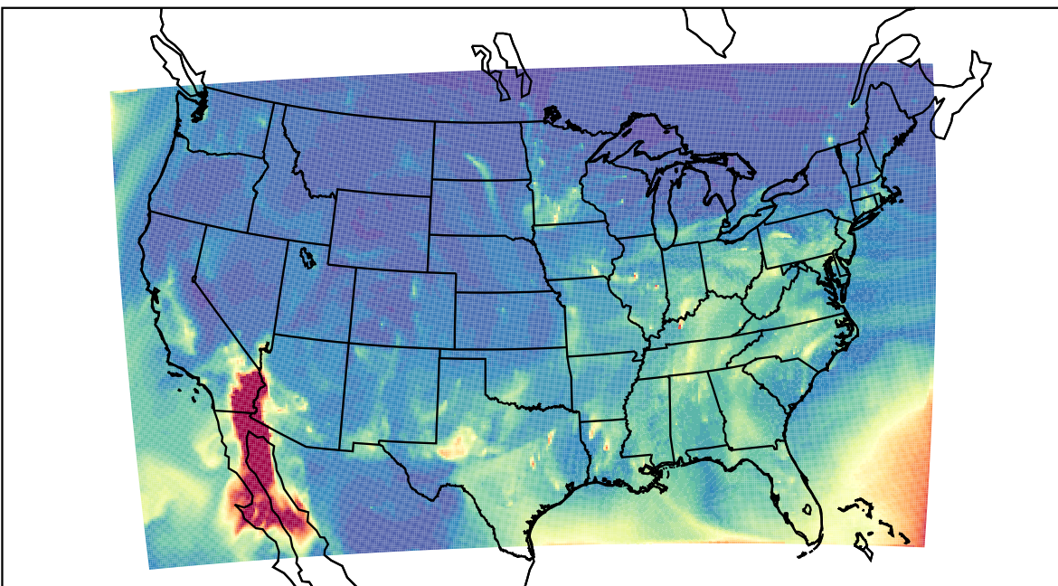
WRF 2021-12-18_11:00:00
