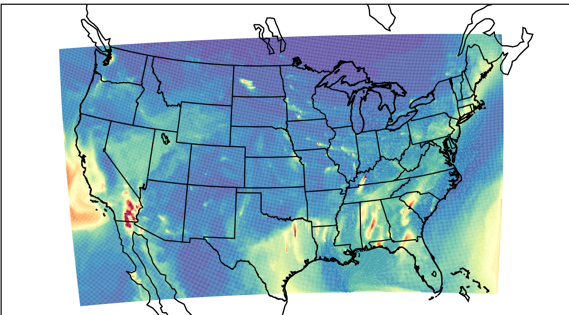
WRF 2021-12-17_09:00:00
