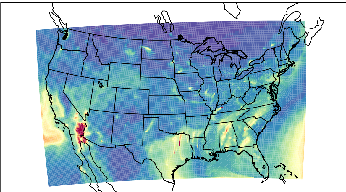
WRF 2021-12-17_13:00:00
