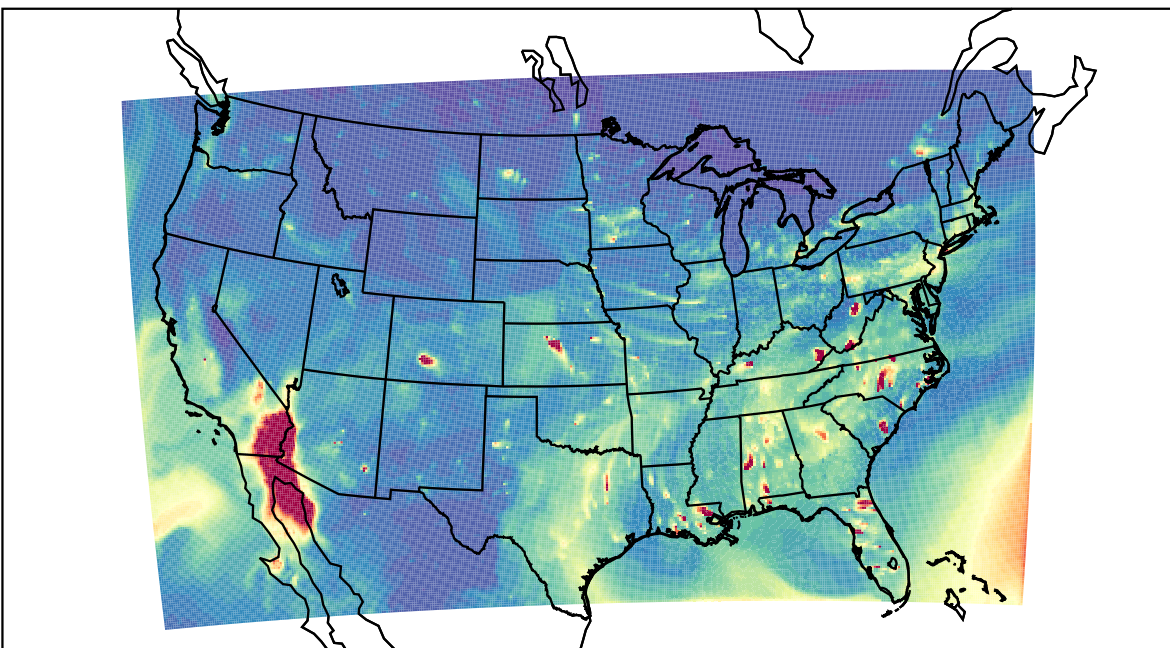
WRF 2021-12-18_00:00:00
