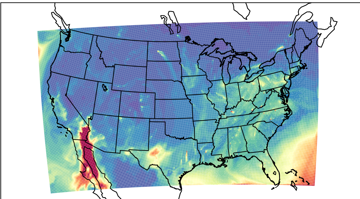
WRF 2021-12-18_17:00:00
