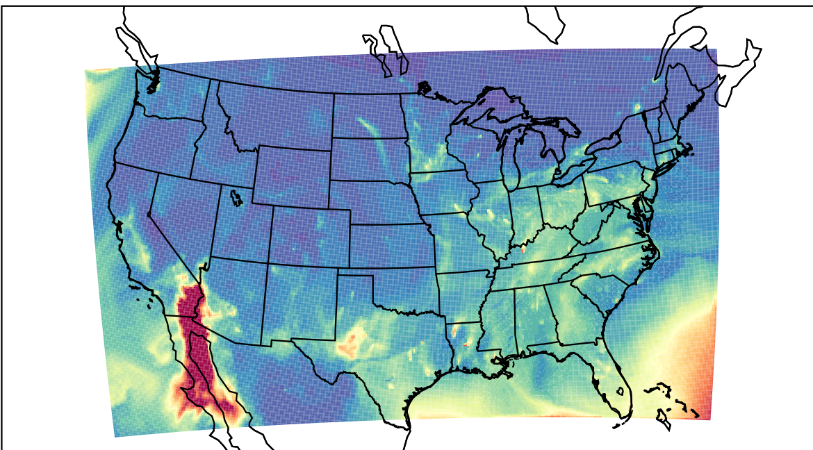
WRF 2021-12-18_13:00:00
