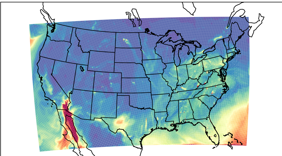
WRF 2021-12-18_19:00:00
