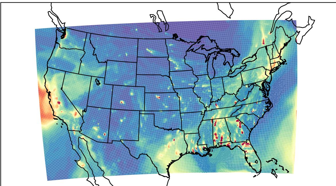
WRF 2021-12-17_02:00:00
