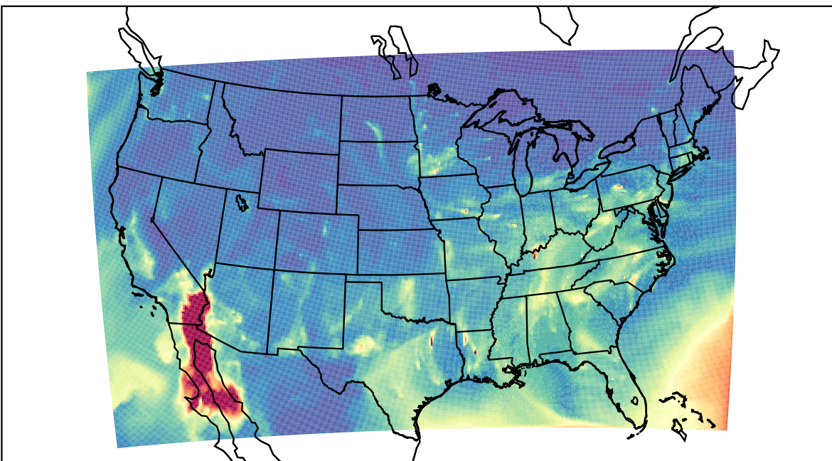
WRF 2021-12-18_09:00:00
