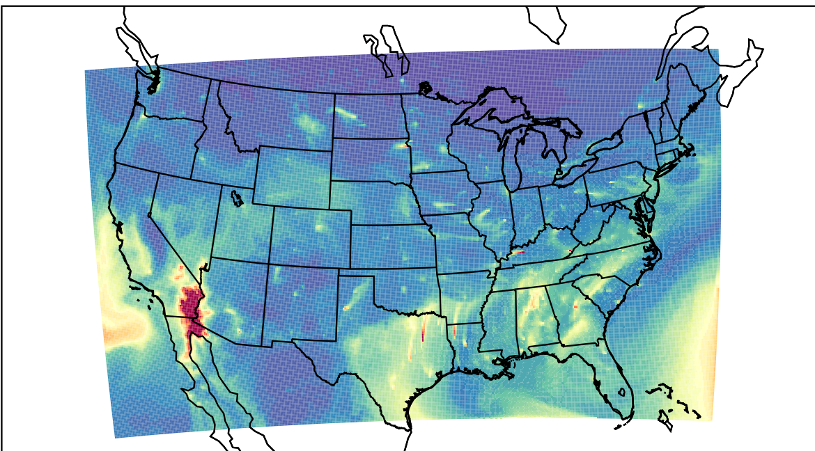
WRF 2021-12-17_15:00:00
