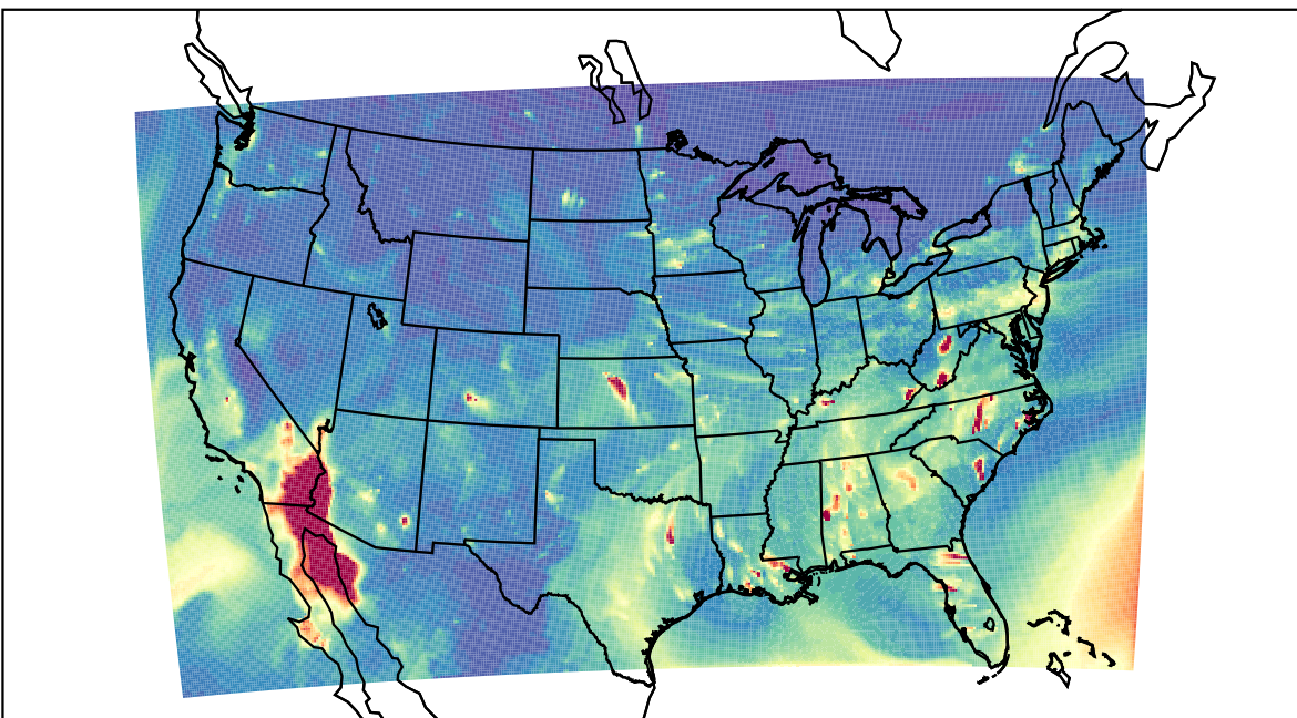
WRF 2021-12-18_02:00:00
