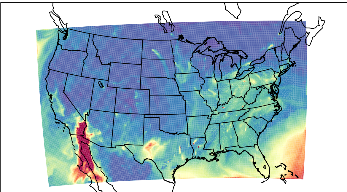
WRF 2021-12-18_16:00:00
