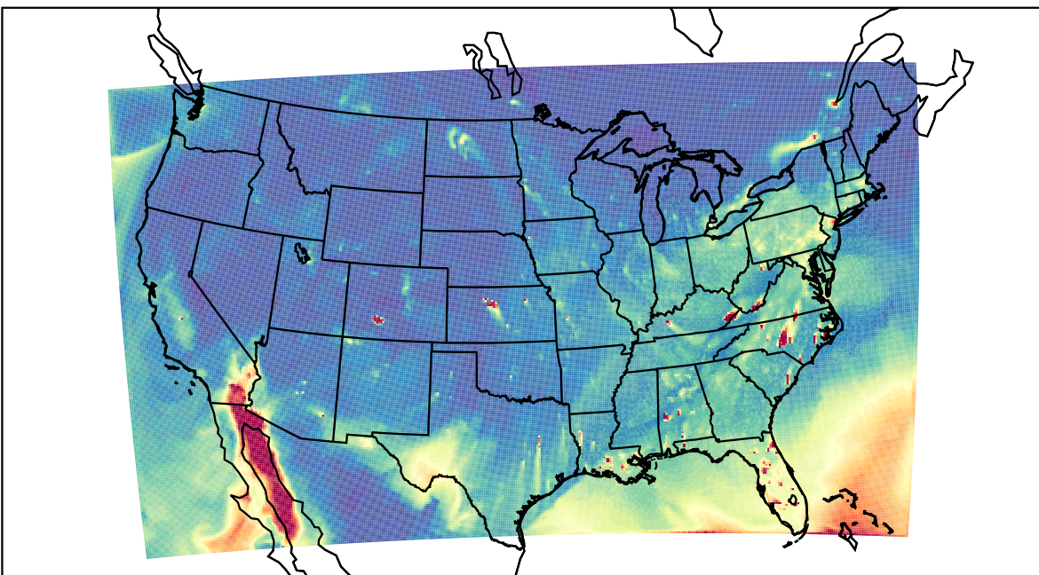
WRF 2021-12-18_23:00:00
