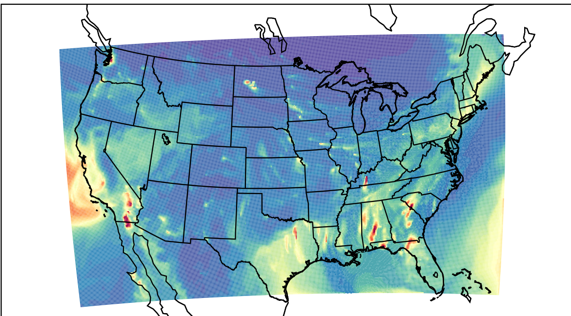
WRF 2021-12-17_07:00:00
