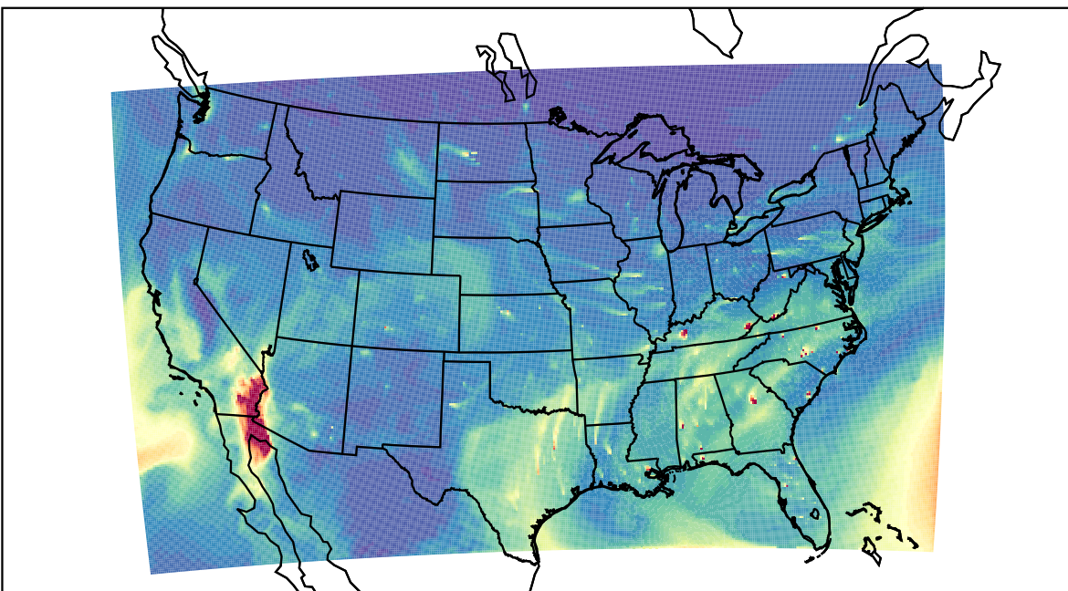
WRF 2021-12-17_19:00:00
