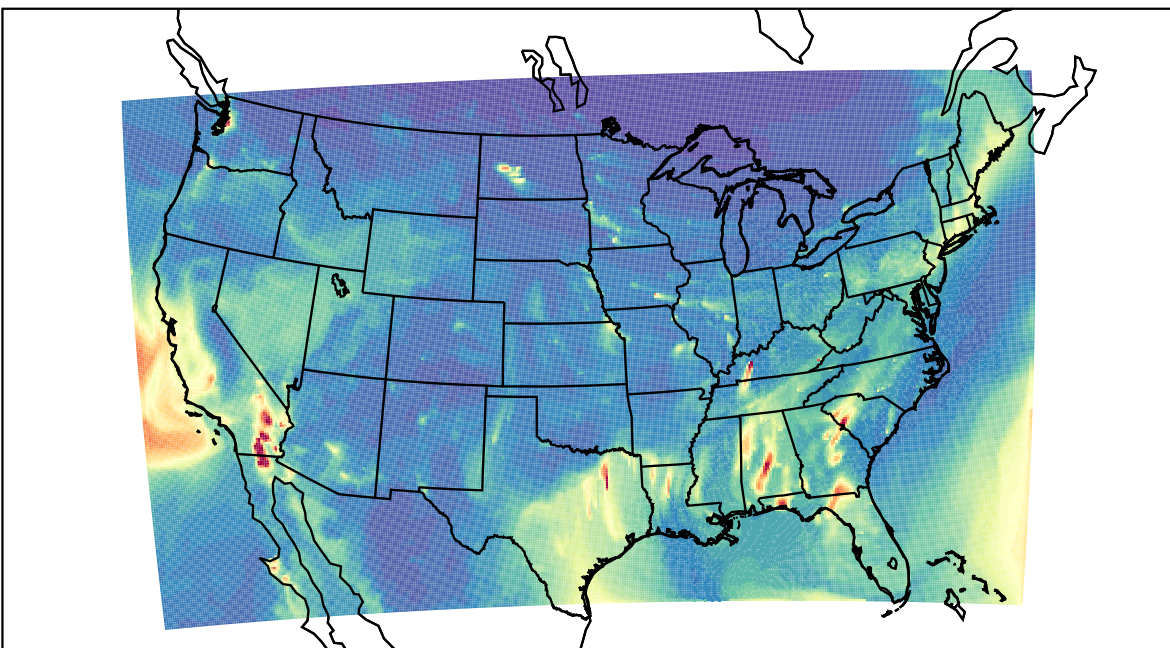
WRF 2021-12-17_08:00:00
