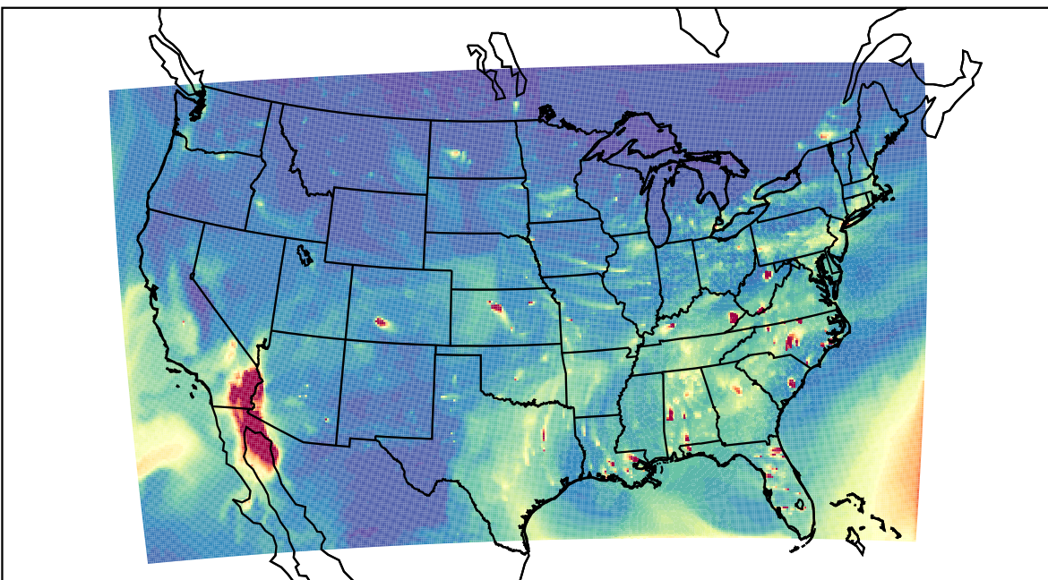
WRF 2021-12-17_23:00:00
