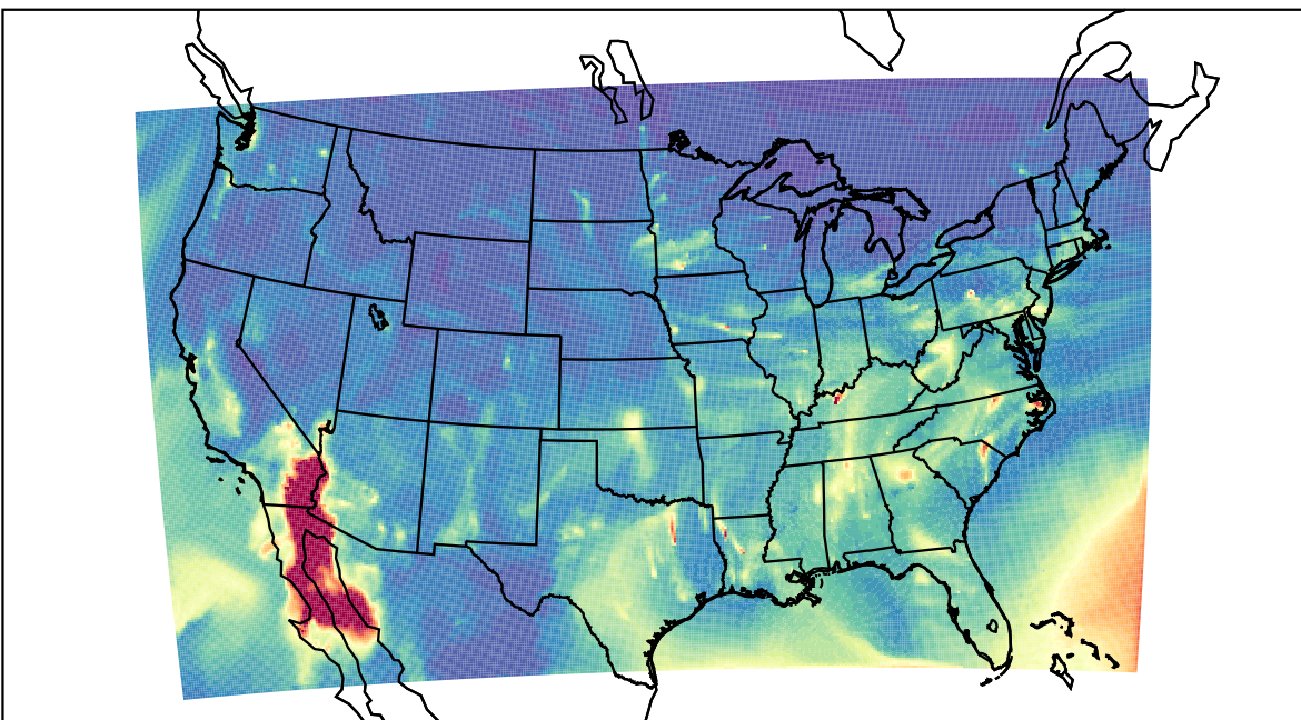
WRF 2021-12-18_07:00:00
