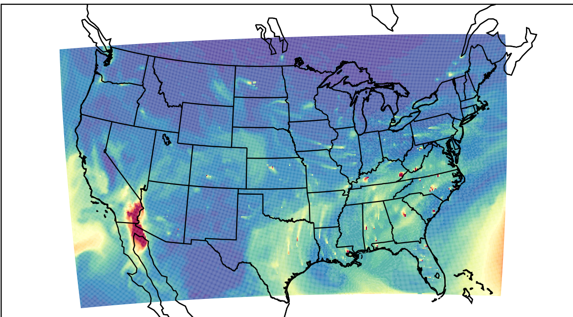
WRF 2021-12-17_20:00:00
