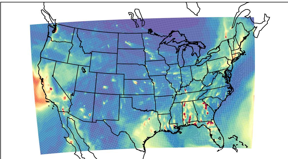
WRF 2021-12-17_03:00:00
