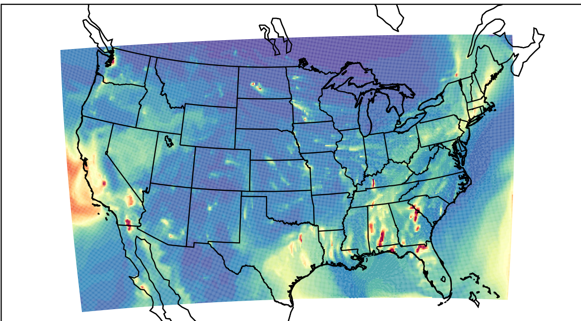
WRF 2021-12-17_05:00:00
