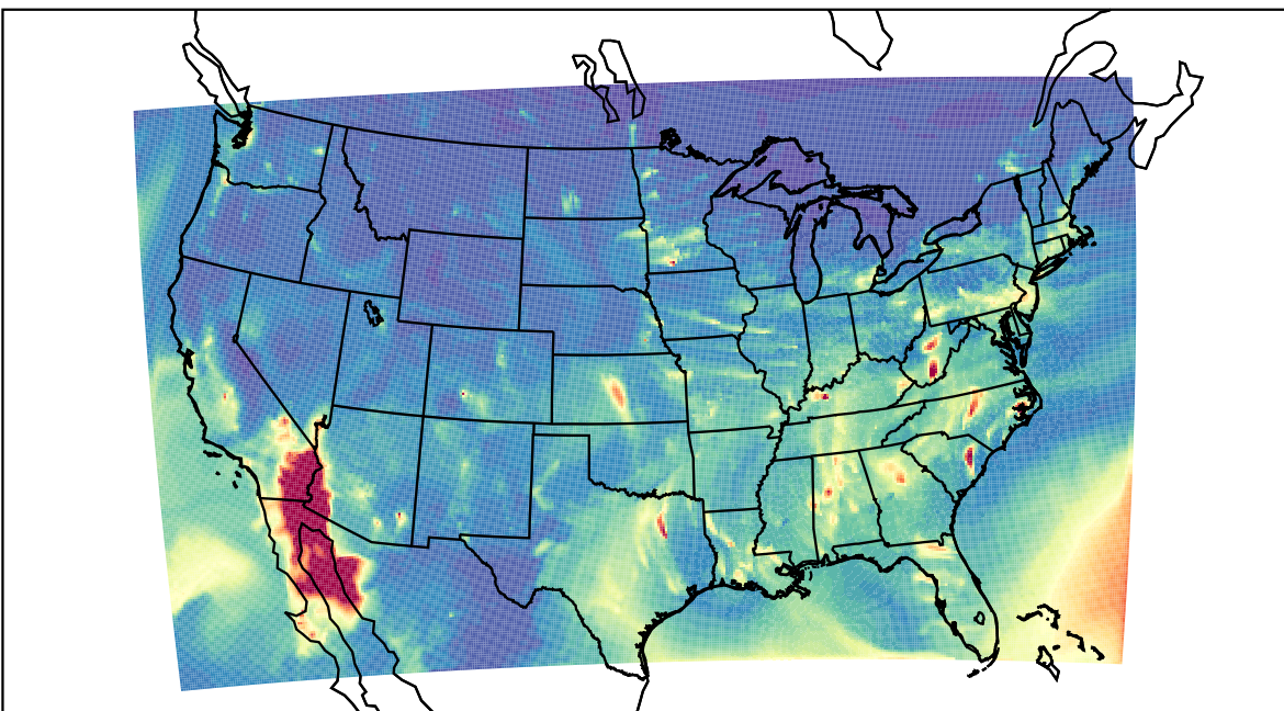
WRF 2021-12-18_04:00:00
