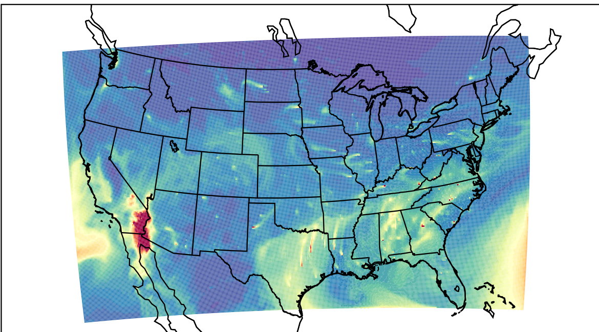
WRF 2021-12-17_17:00:00
