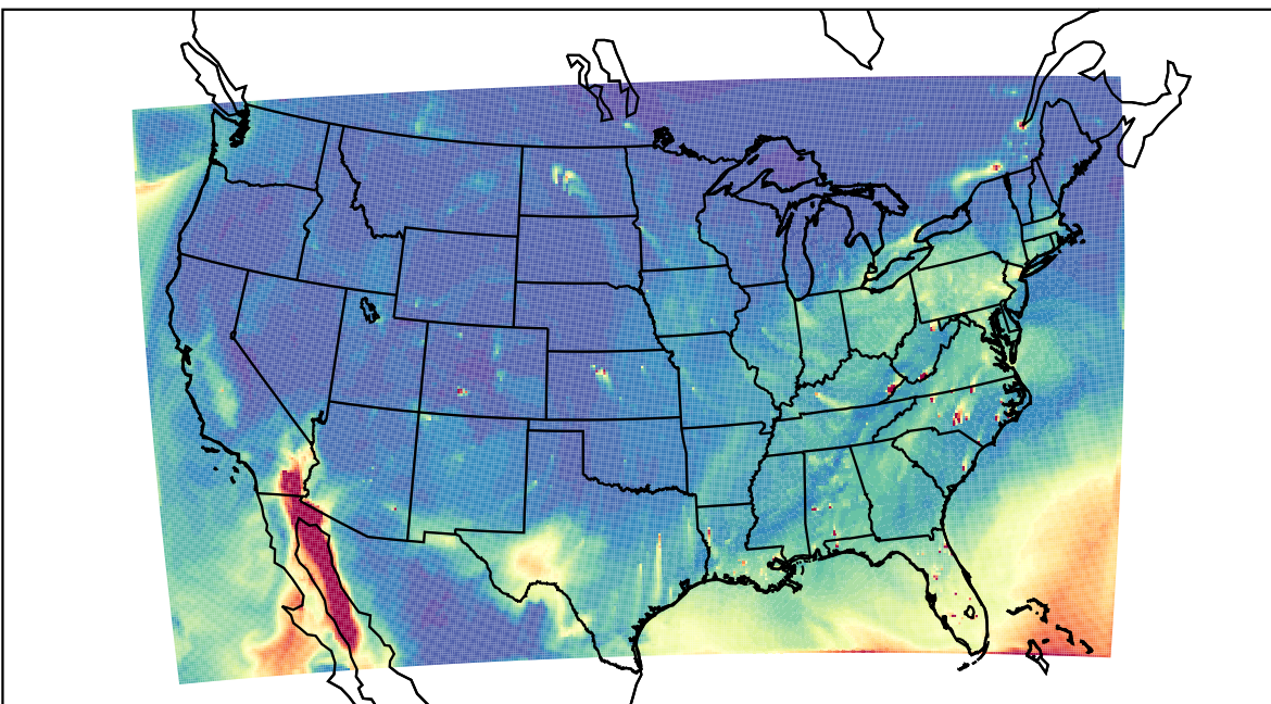
WRF 2021-12-18_21:00:00
