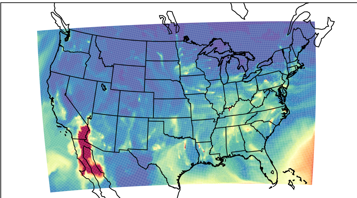
WRF 2021-12-18_08:00:00
