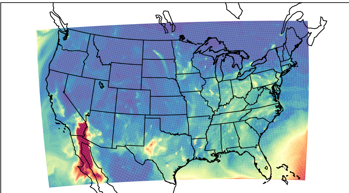
WRF 2021-12-18_14:00:00
