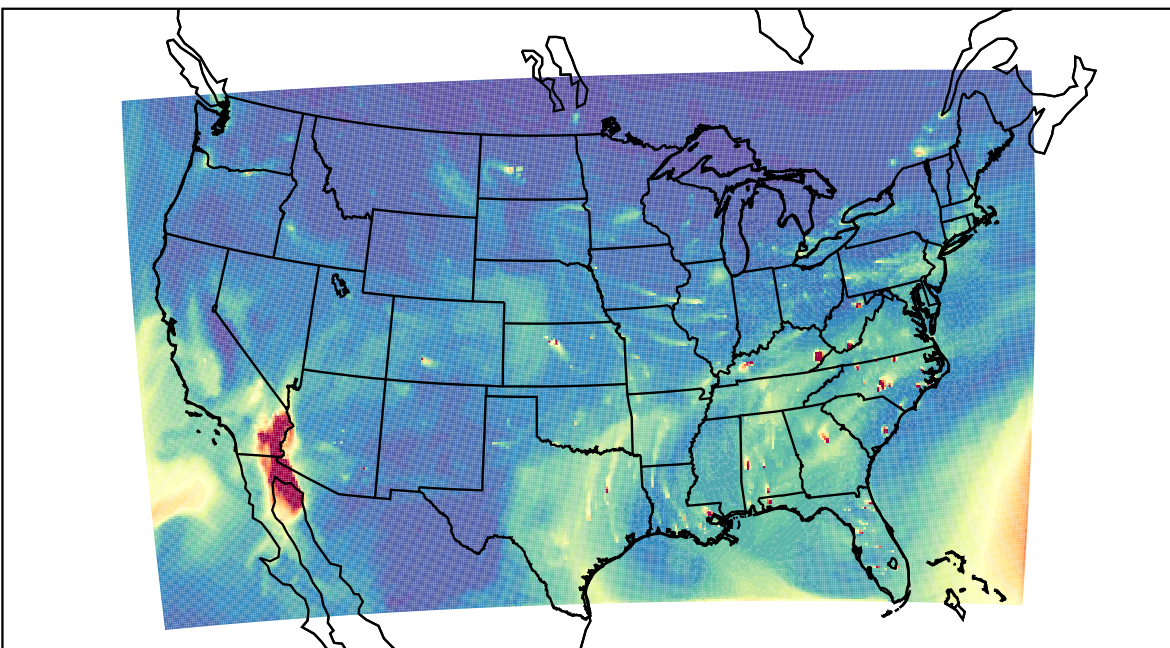
WRF 2021-12-17_21:00:00
