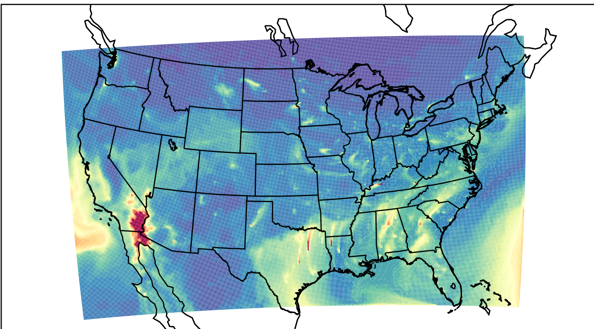
WRF 2021-12-17_14:00:00
