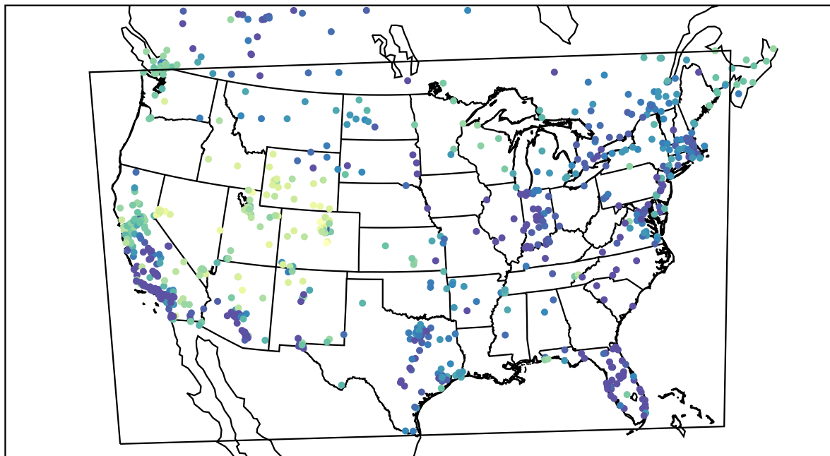
AirNOW (2021-12-27_07:00:00)
