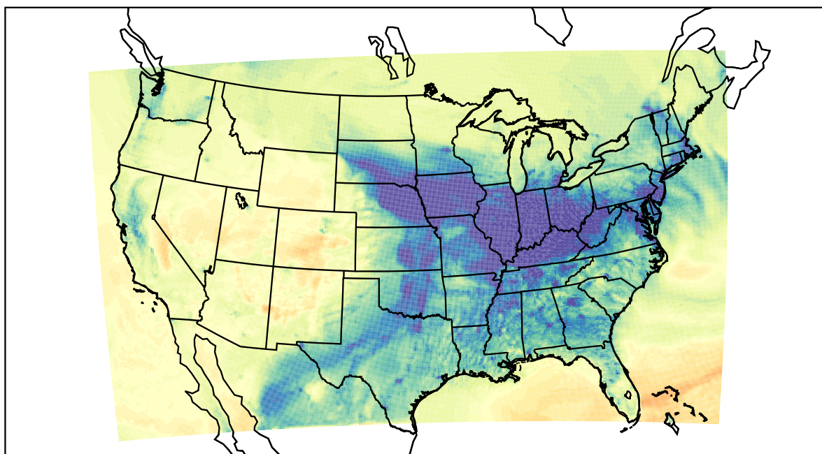
WRF (2021-12-27_00:00:00)
