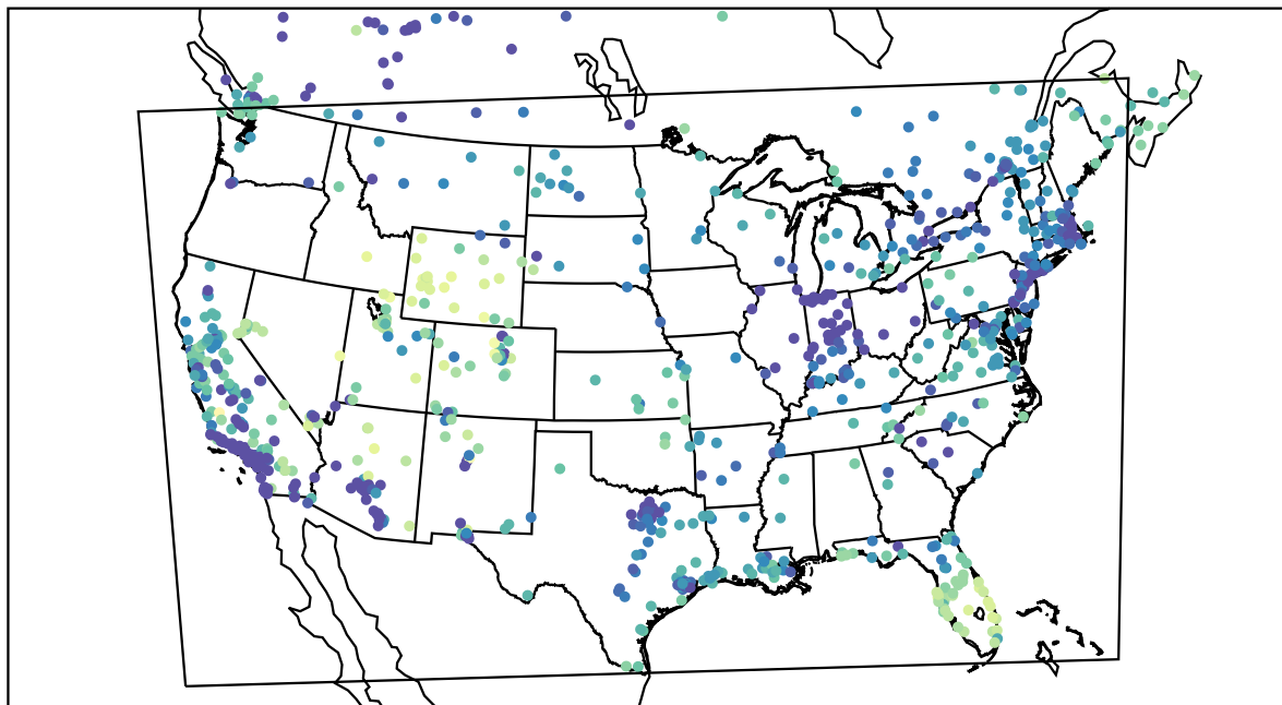
AirNOW (2021-12-27_16:00:00)
