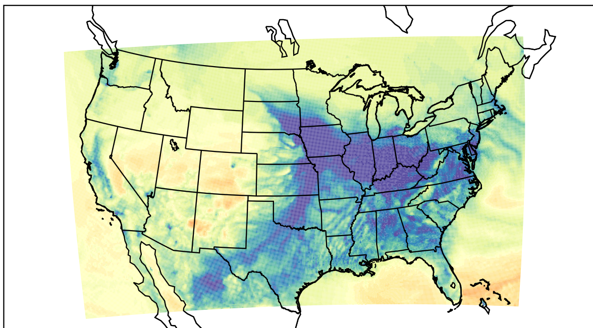
WRF (2021-12-27_04:00:00)
