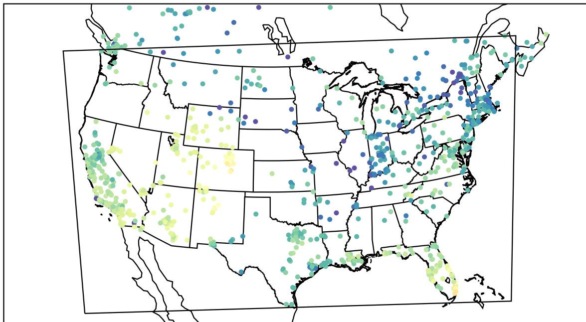
AirNOW (2021-12-26_21:00:00)
