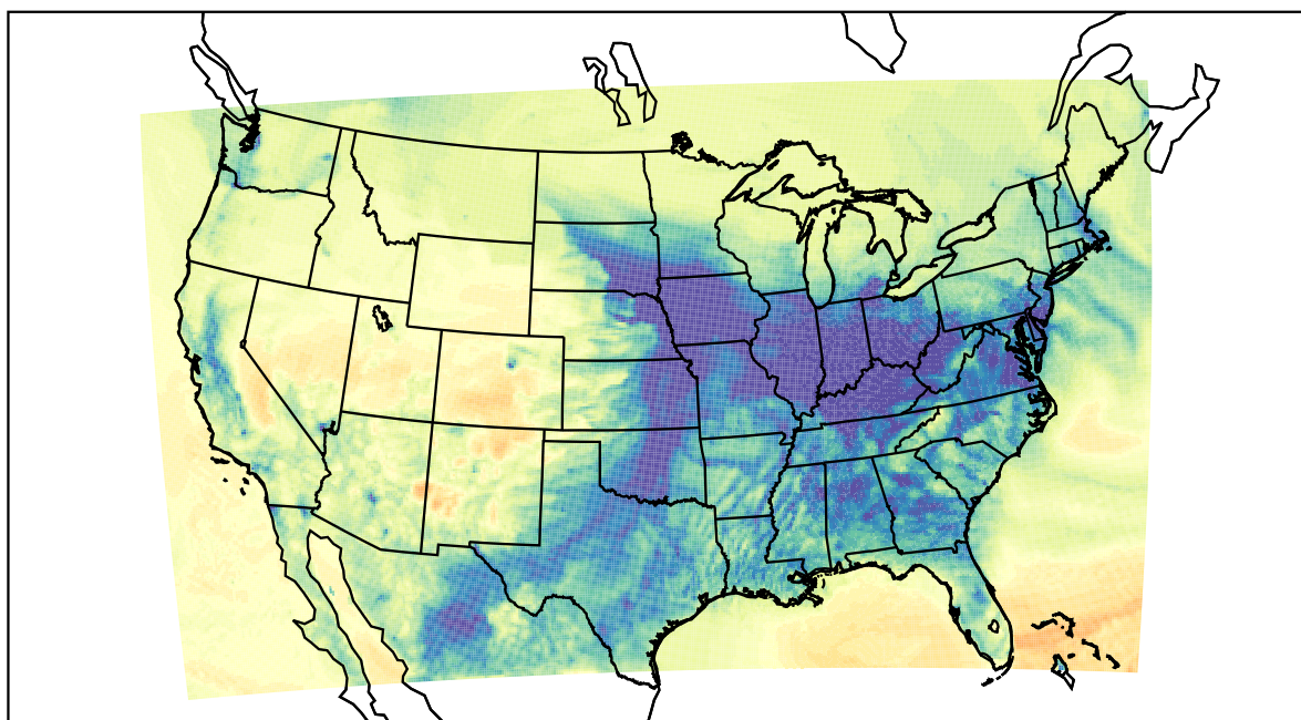
WRF (2021-12-27_03:00:00)
