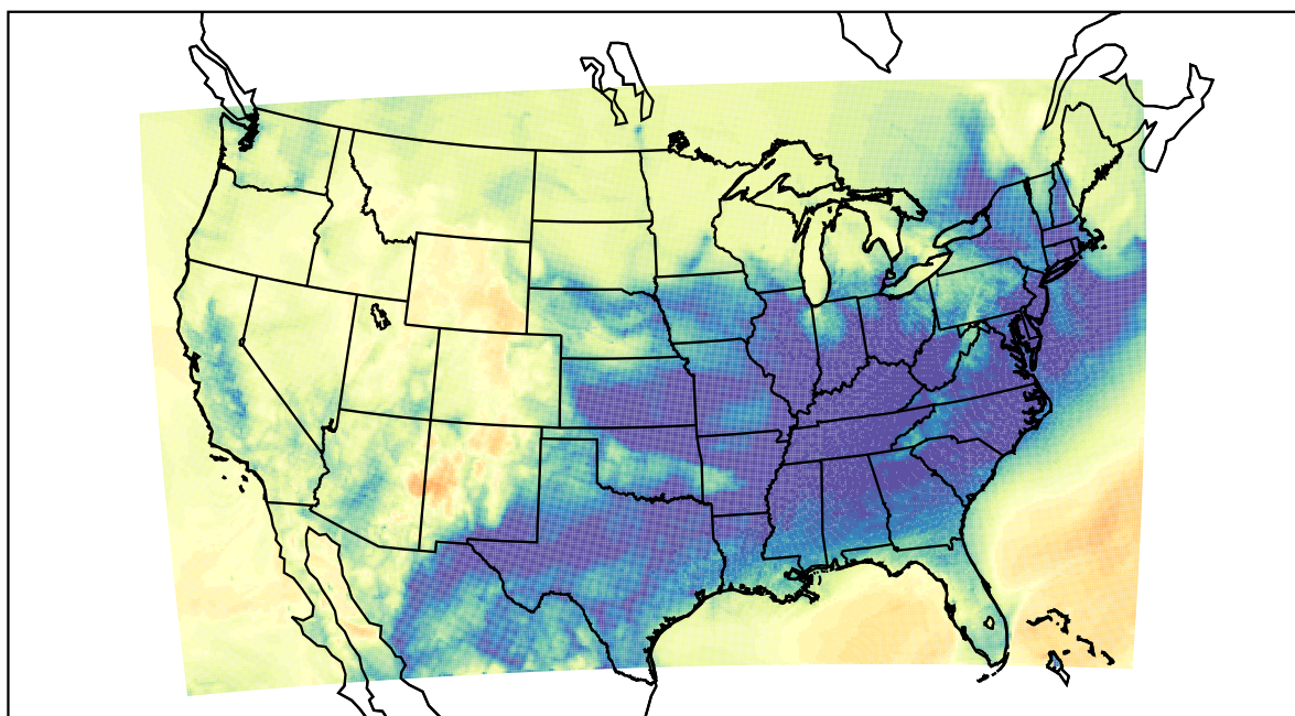
WRF (2021-12-26_11:00:00)
