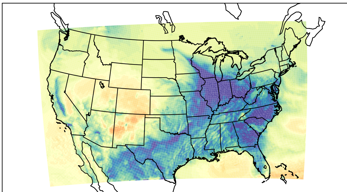
WRF (2021-12-27_12:00:00)
