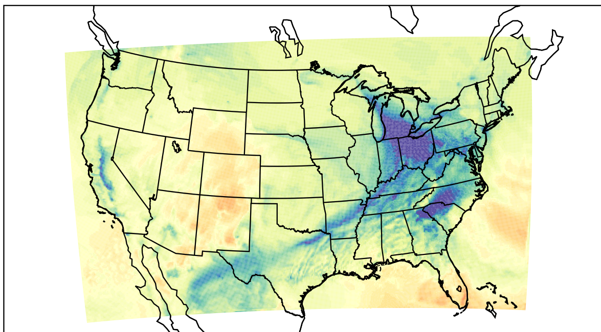
WRF (2021-12-27_19:00:00)
