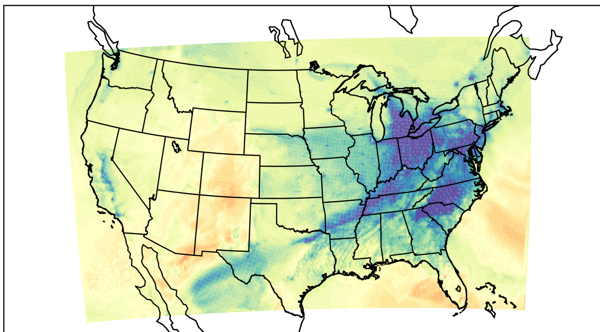
WRF (2021-12-27_22:00:00)
