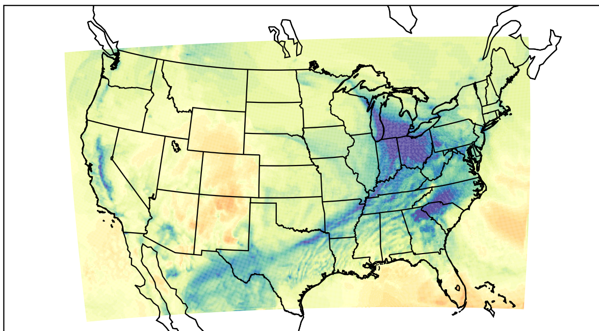
WRF (2021-12-27_18:00:00)
