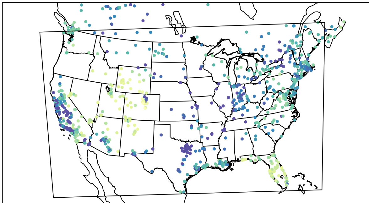
AirNOW (2021-12-26_16:00:00)
