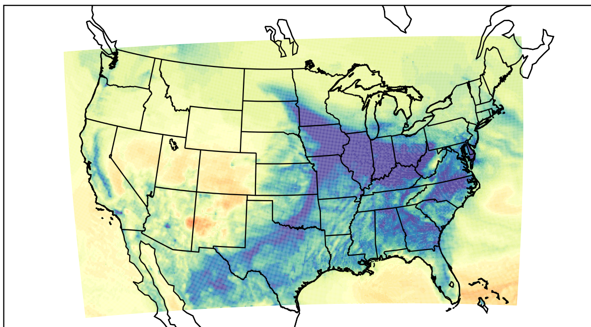
WRF (2021-12-27_07:00:00)
