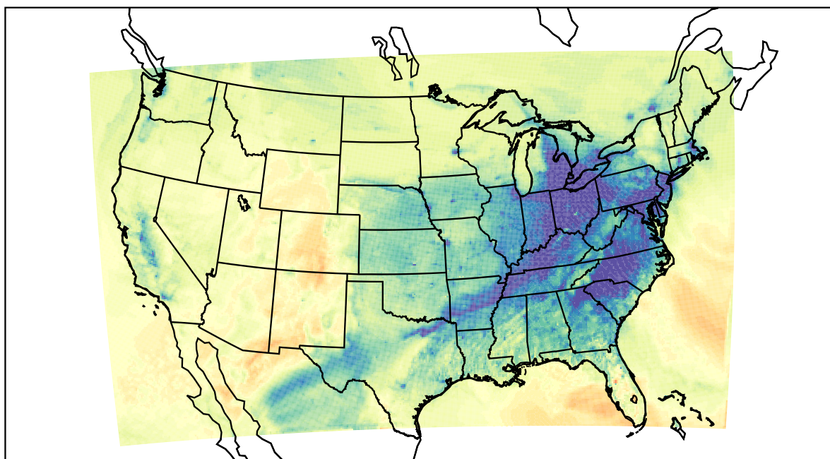
WRF (2021-12-27_23:00:00)
