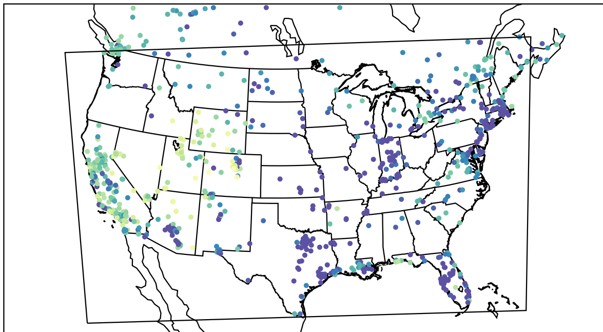
AirNOW (2021-12-26_07:00:00)
