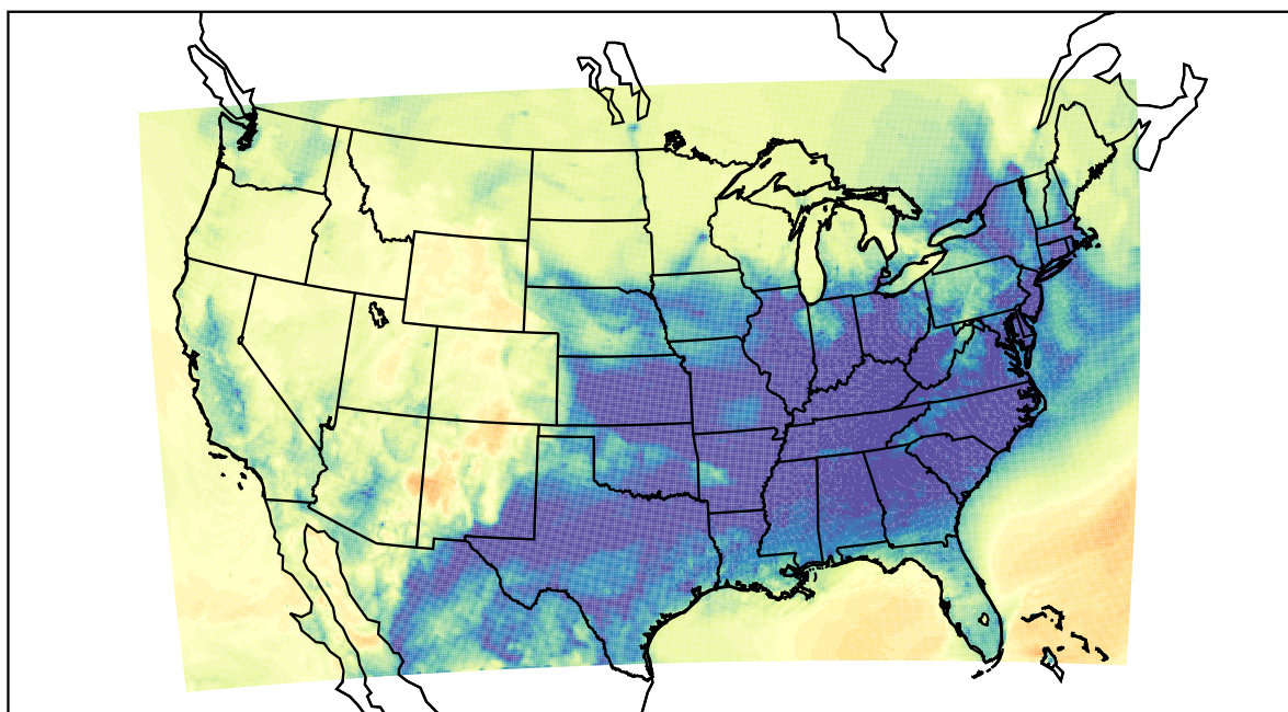
WRF (2021-12-26_13:00:00)
