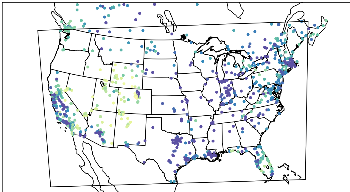
AirNOW (2021-12-26_14:00:00)
