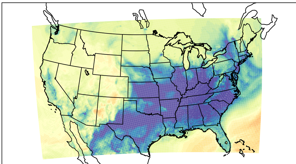
WRF (2021-12-26_14:00:00)
