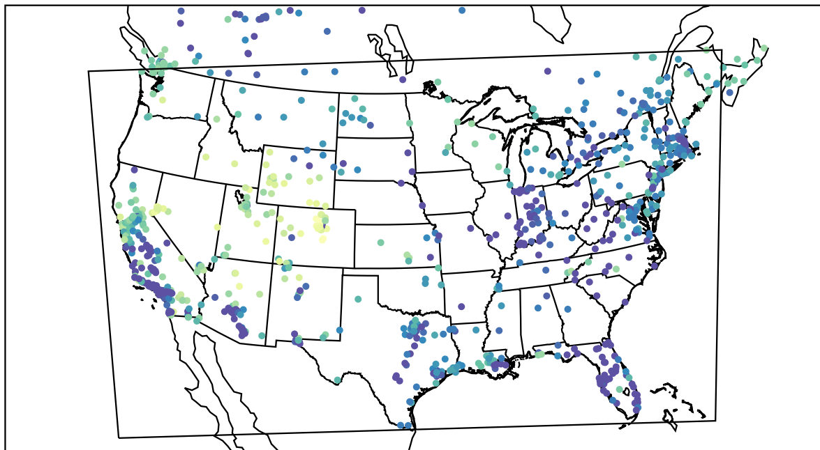
AirNOW (2021-12-27_06:00:00)
