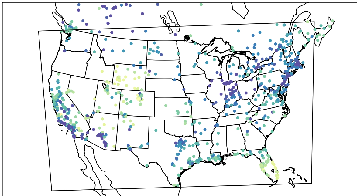
AirNOW (2021-12-27_17:00:00)
