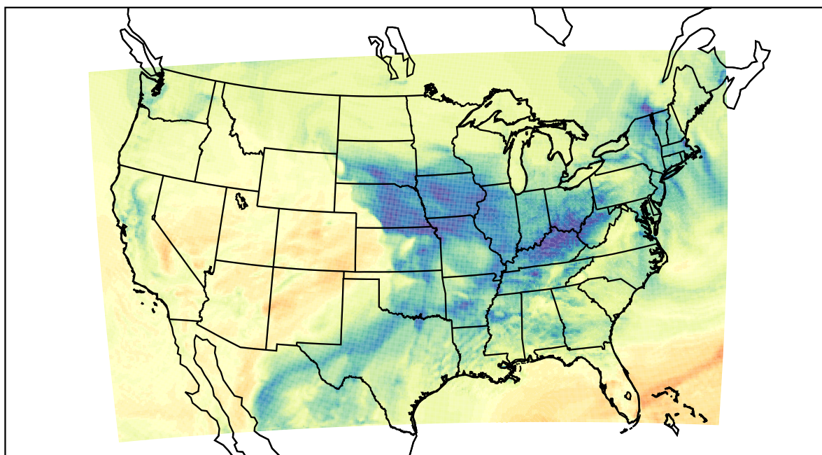
WRF (2021-12-26_20:00:00)
