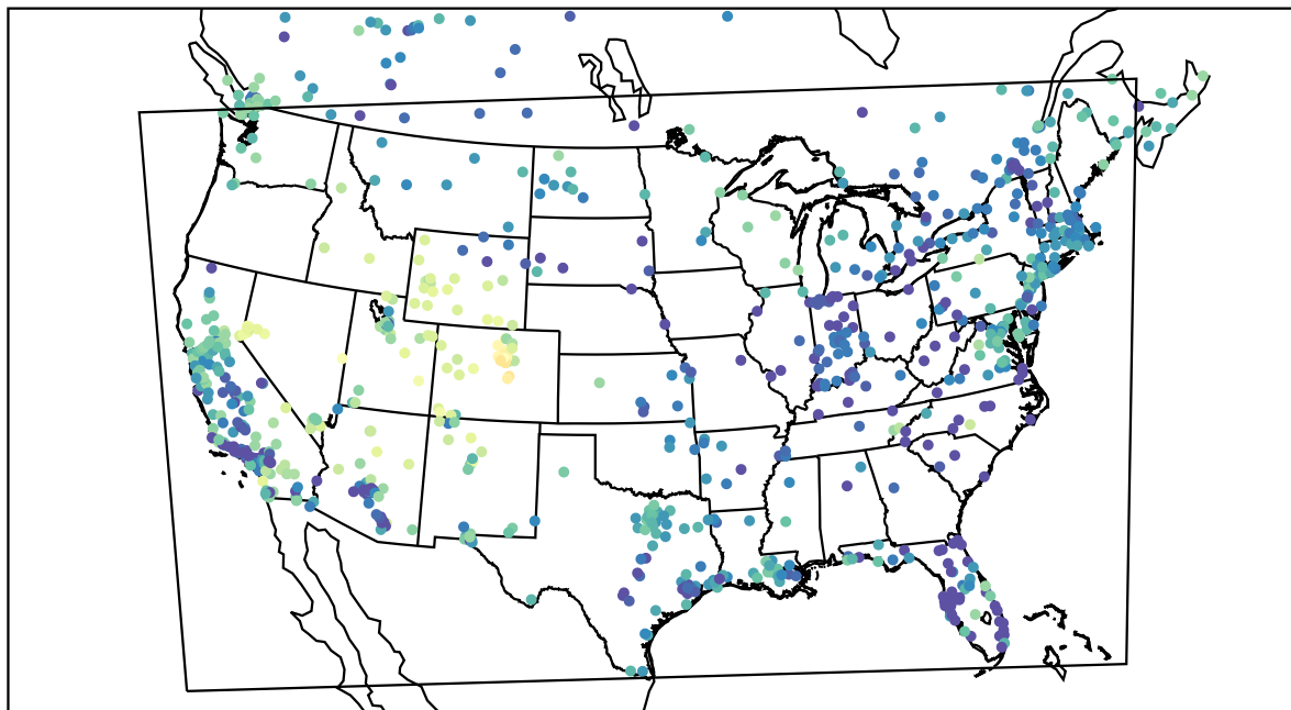
AirNOW (2021-12-27_02:00:00)
