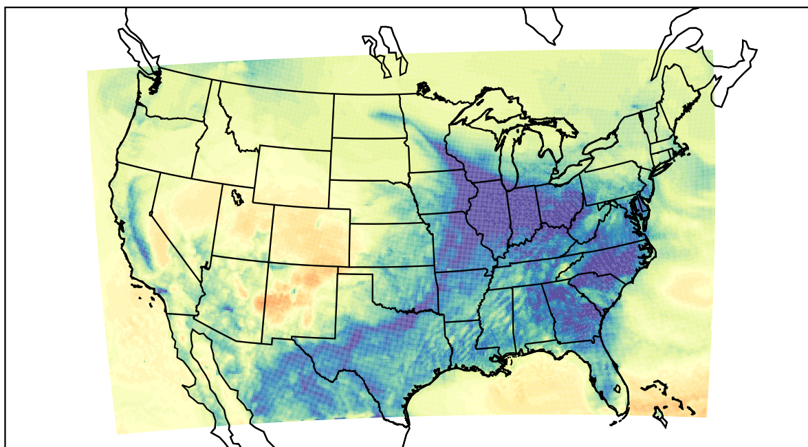
WRF (2021-12-27_11:00:00)
