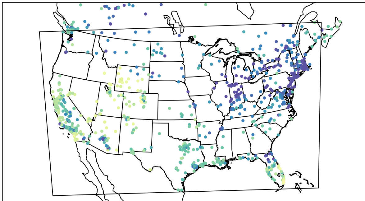
AirNOW (2021-12-27_22:00:00)
