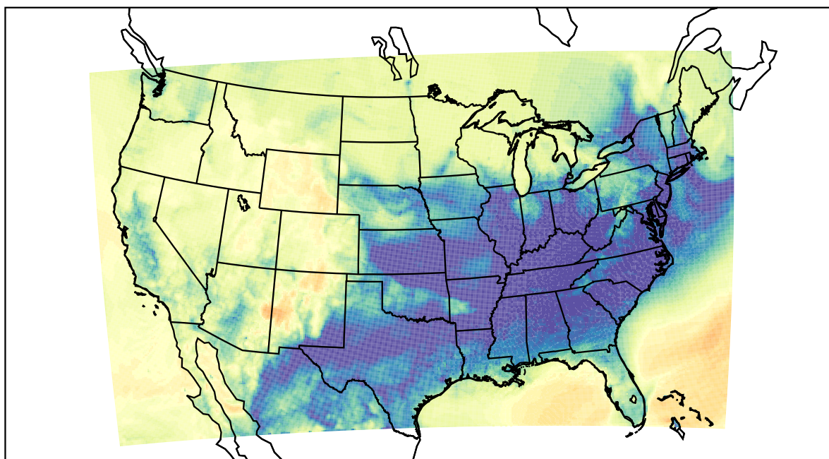
WRF (2021-12-26_12:00:00)
