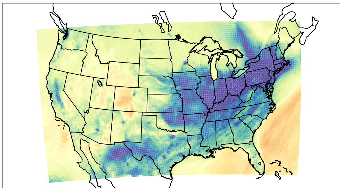
WRF (2021-12-26_01:00:00)
