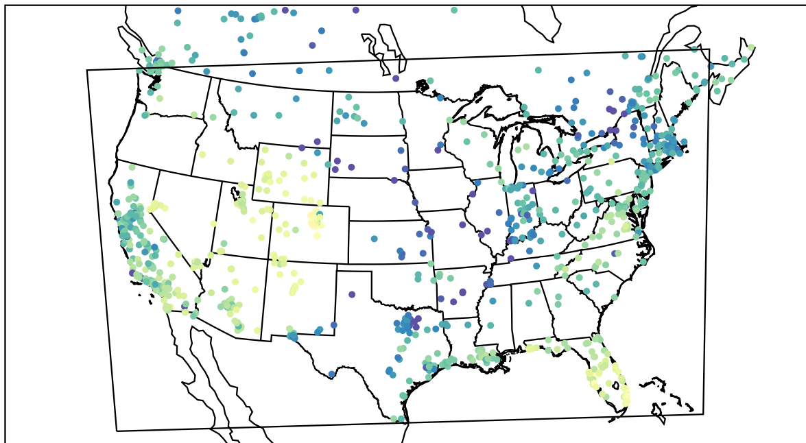
AirNOW (2021-12-26_18:00:00)
