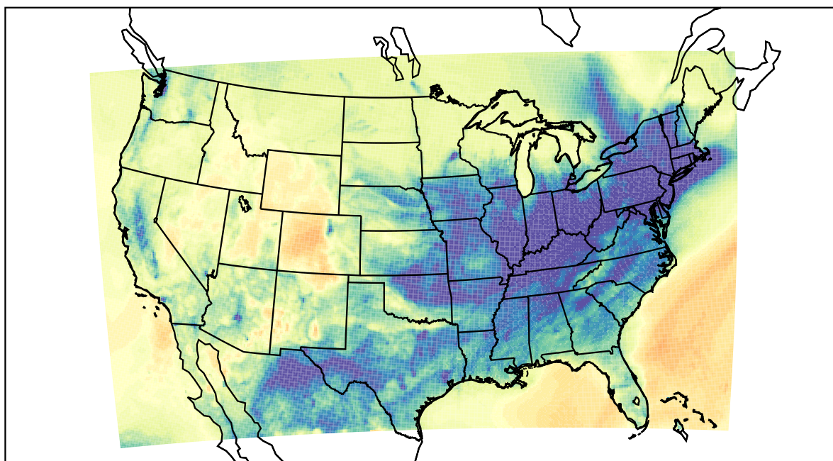
WRF (2021-12-26_03:00:00)
