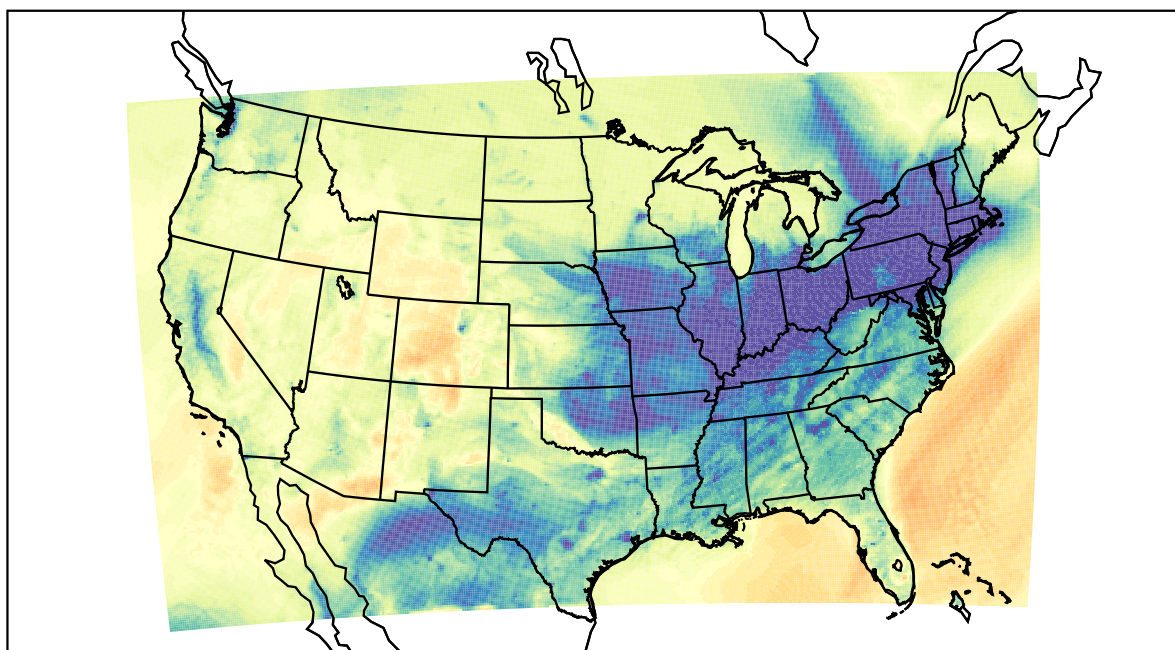
WRF (2021-12-26_00:00:00)
