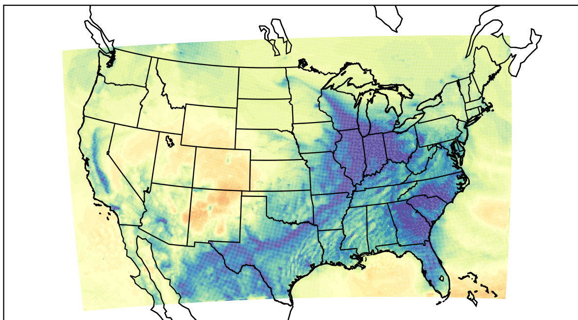
WRF (2021-12-27_14:00:00)
