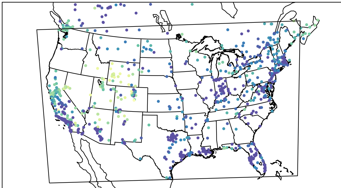
AirNOW (2021-12-27_13:00:00)
