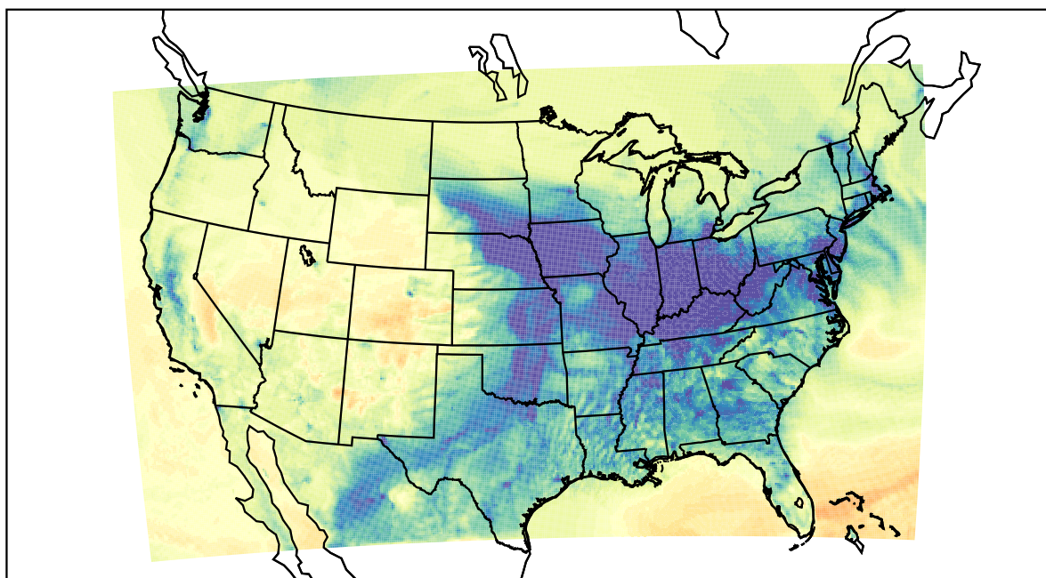
WRF (2021-12-27_01:00:00)
