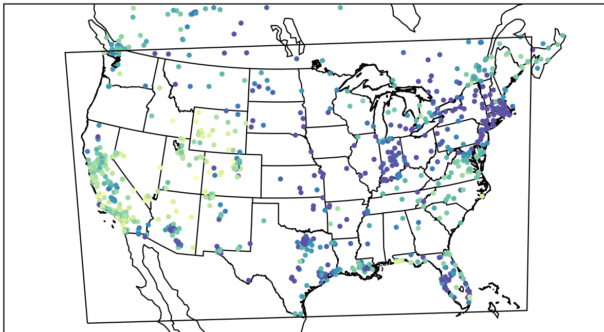
AirNOW (2021-12-26_01:00:00)
