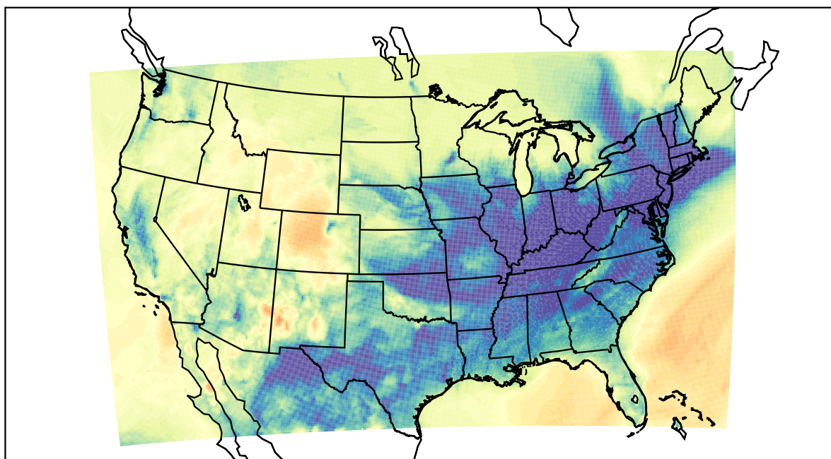
WRF (2021-12-26_05:00:00)
