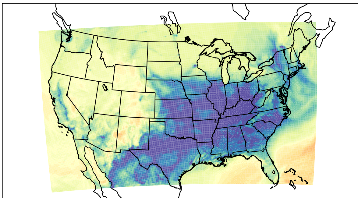
WRF (2021-12-26_15:00:00)
