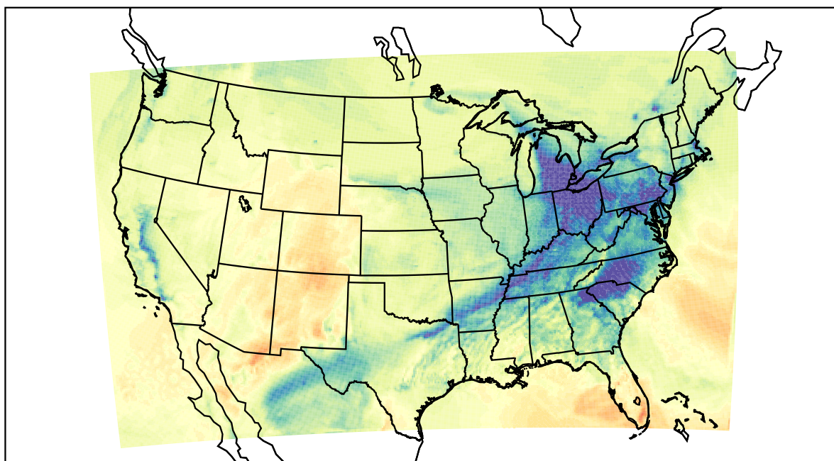
WRF (2021-12-27_21:00:00)
