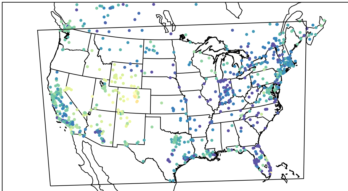
AirNOW (2021-12-27_01:00:00)
