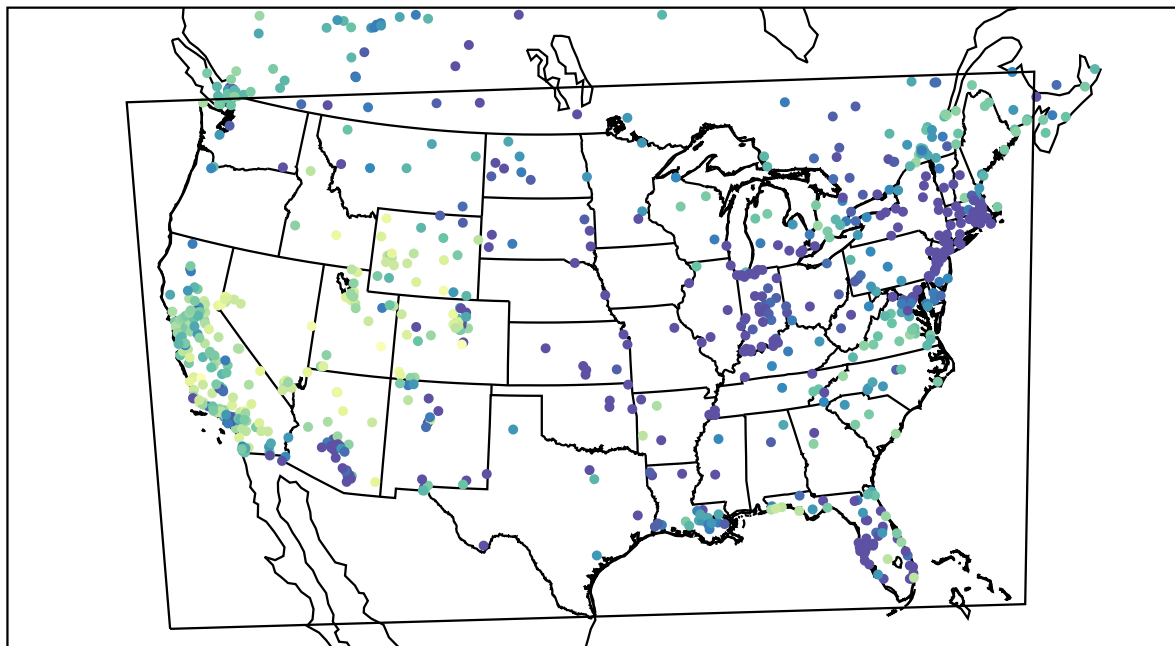
AirNOW (2021-12-26_04:00:00)
