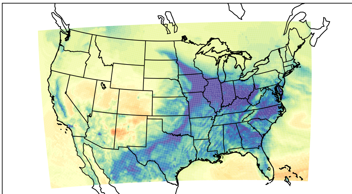
WRF (2021-12-27_08:00:00)
