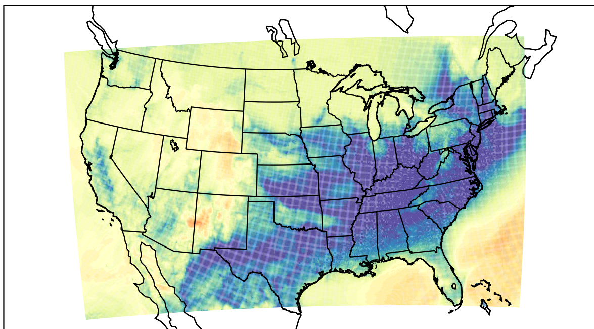
WRF (2021-12-26_10:00:00)
