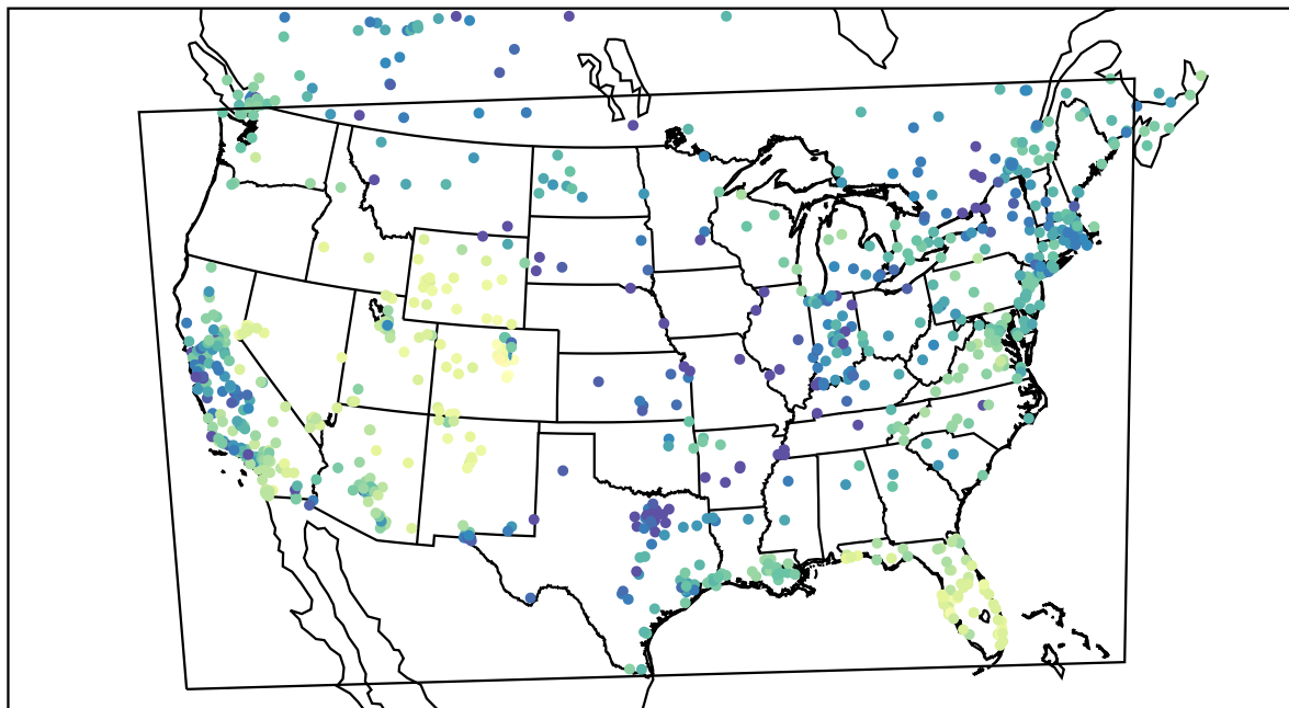
AirNOW (2021-12-26_17:00:00)
