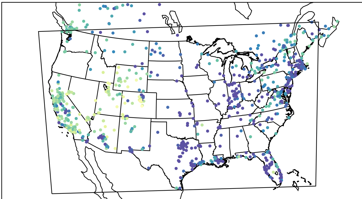
AirNOW (2021-12-26_09:00:00)
