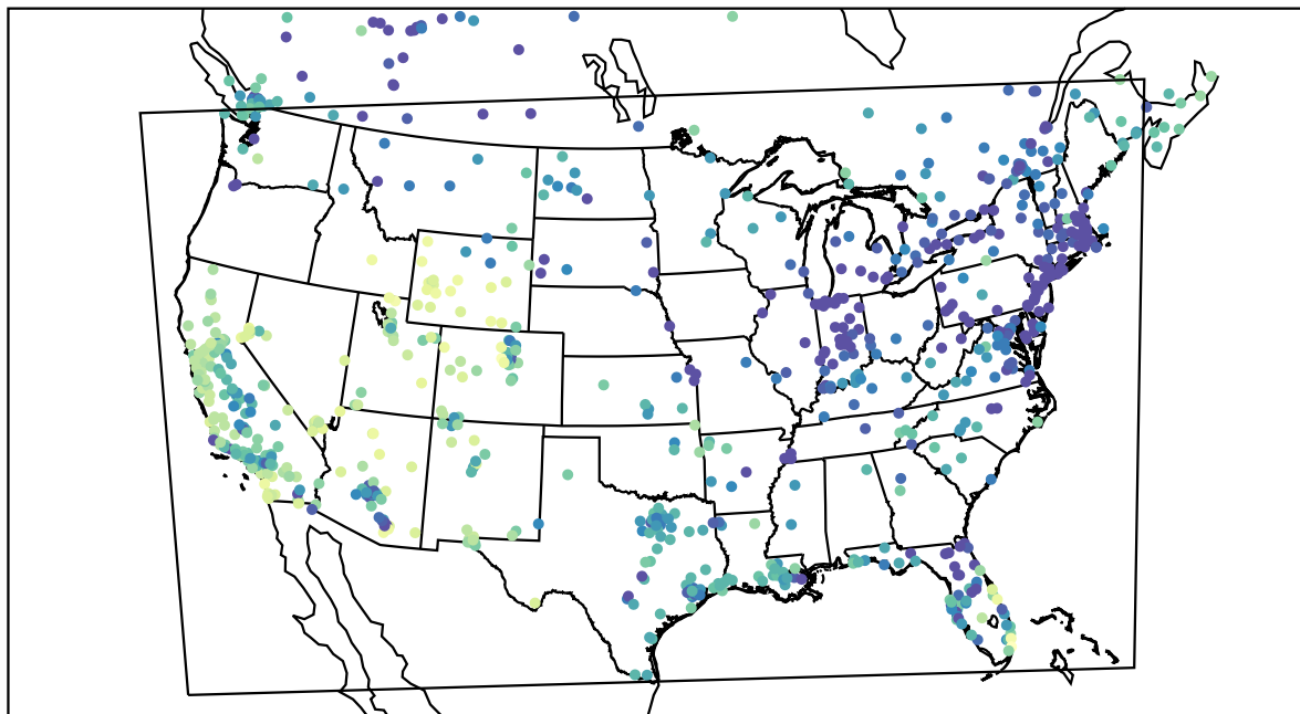
AirNOW (2021-12-27_23:00:00)
