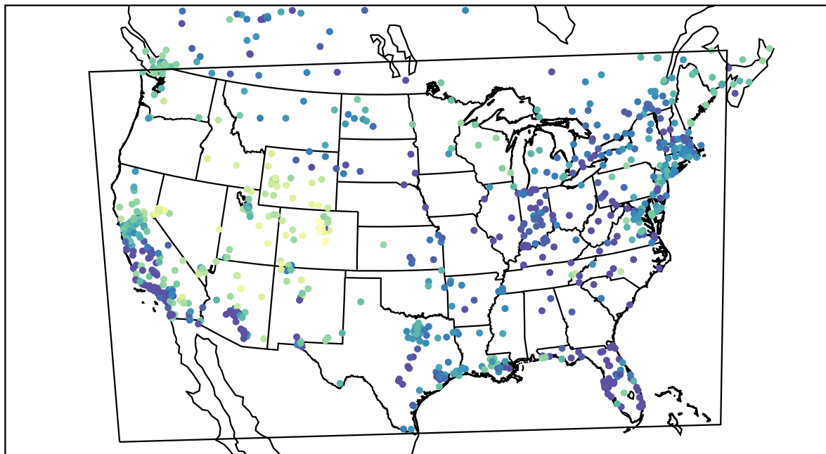
AirNOW (2021-12-27_04:00:00)
