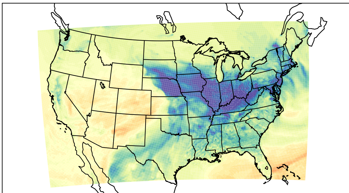
WRF (2021-12-26_22:00:00)
