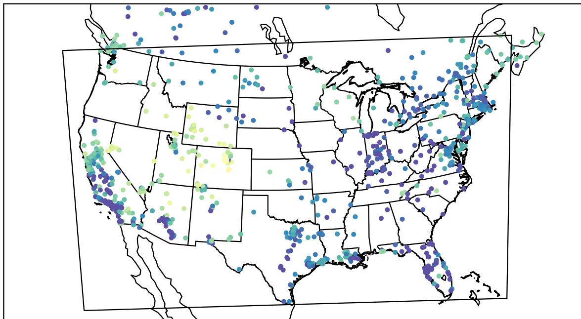
AirNOW (2021-12-27_05:00:00)
