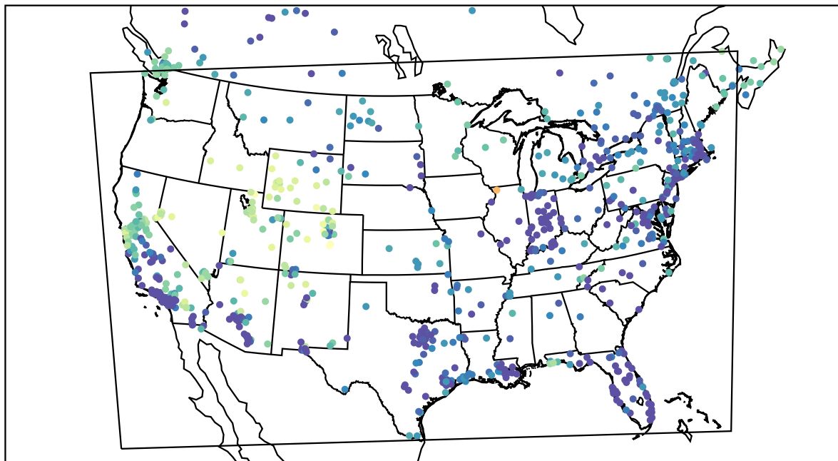
AirNOW (2021-12-27_10:00:00)
