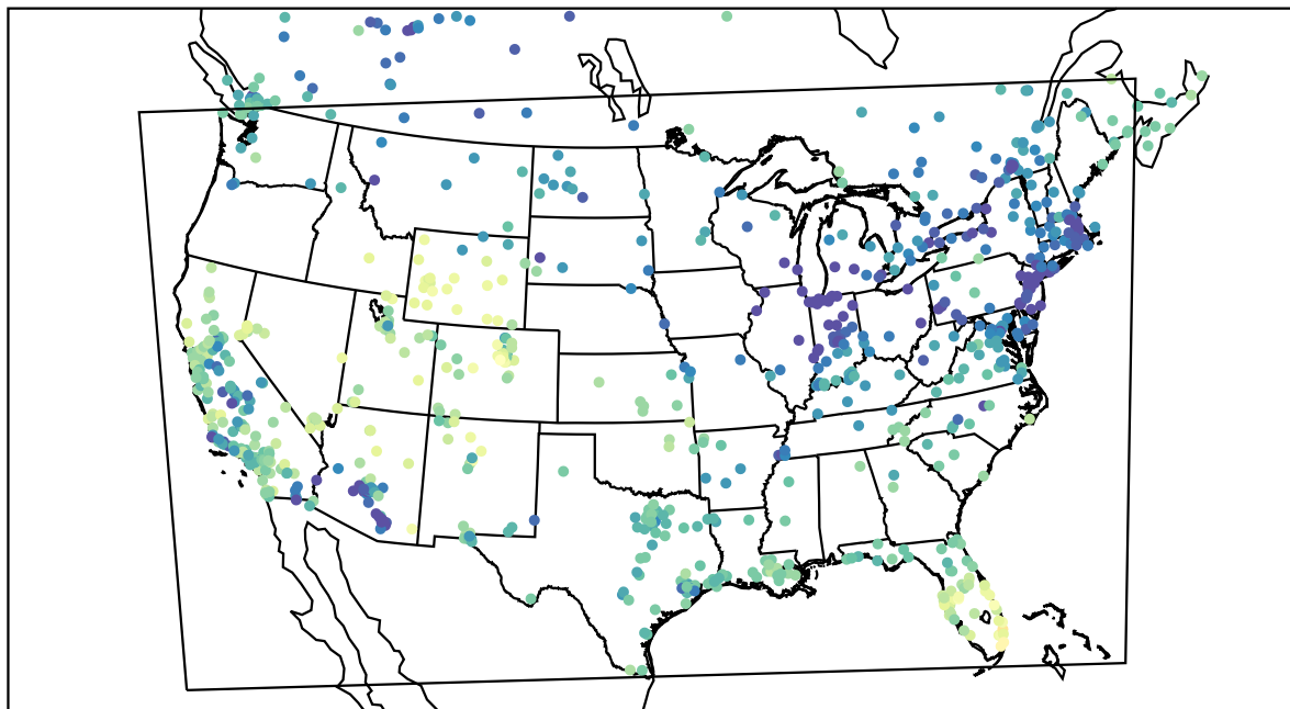
AirNOW (2021-12-27_19:00:00)
