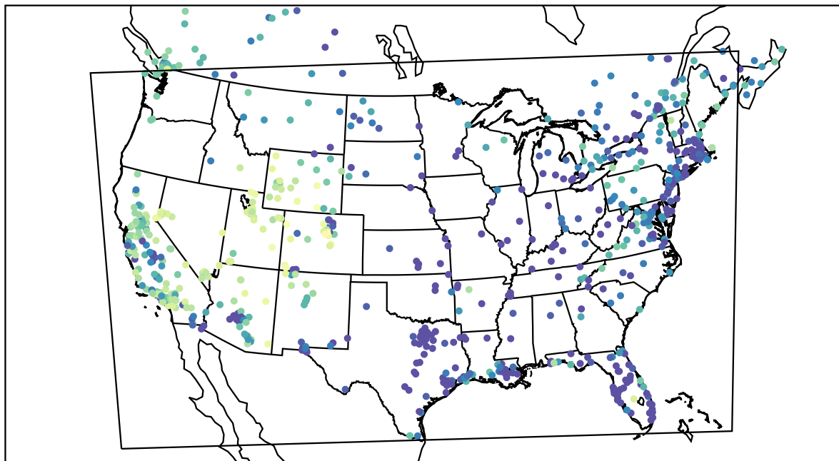
AirNOW (2021-12-26_10:00:00)
