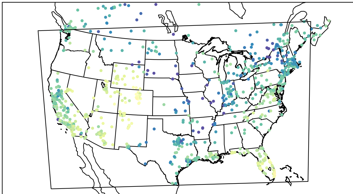
AirNOW (2021-12-26_19:00:00)
