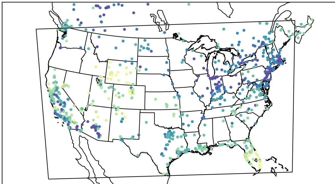
AirNOW (2021-12-27_18:00:00)
