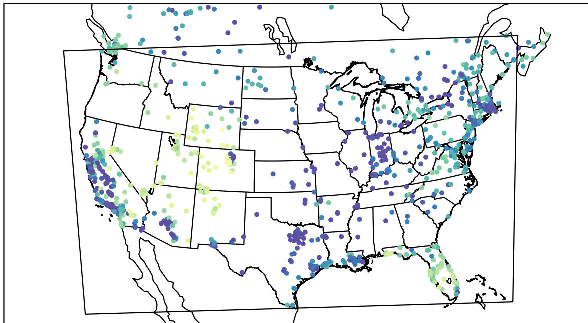
AirNOW (2021-12-26_15:00:00)
