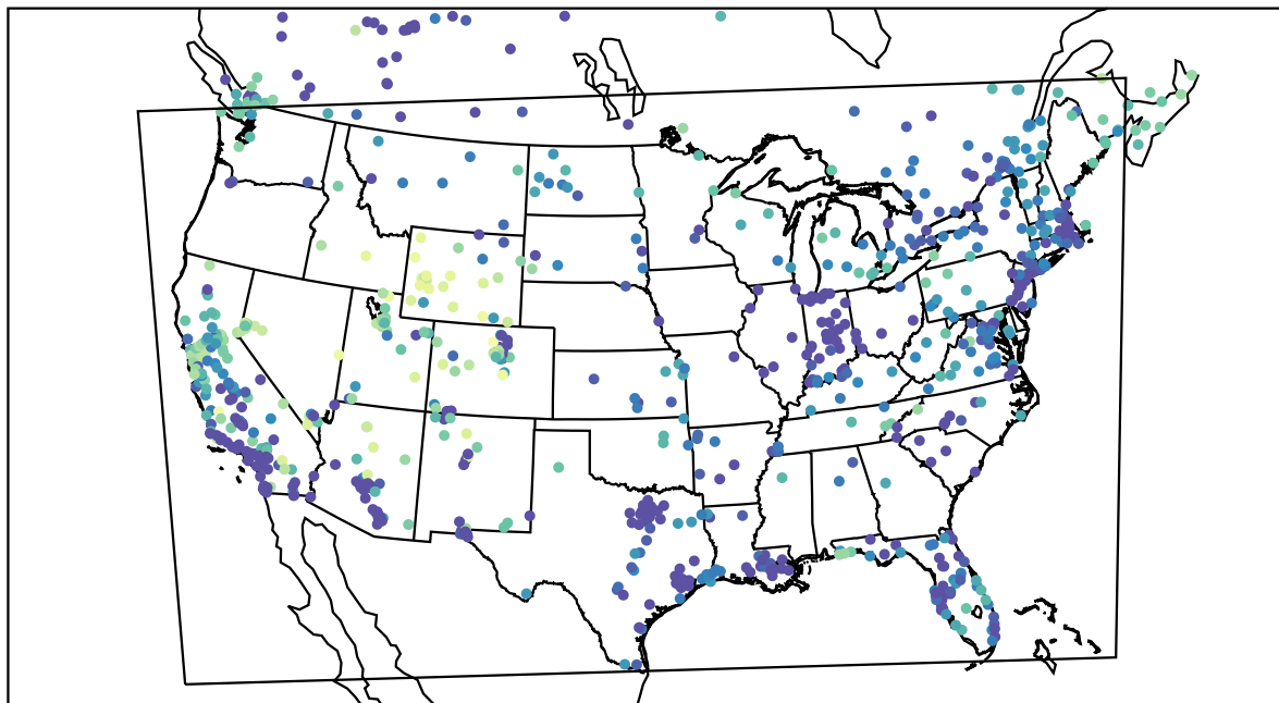
AirNOW (2021-12-27_14:00:00)
