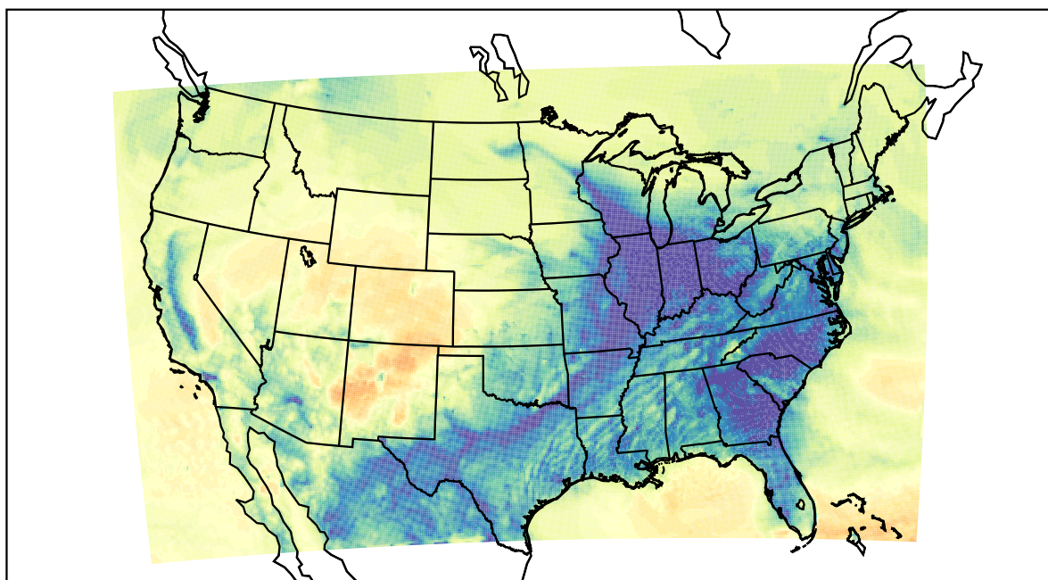
WRF (2021-12-27_13:00:00)
