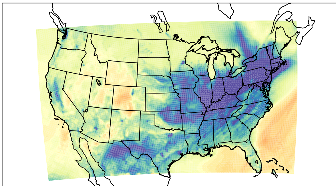
WRF (2021-12-26_02:00:00)
