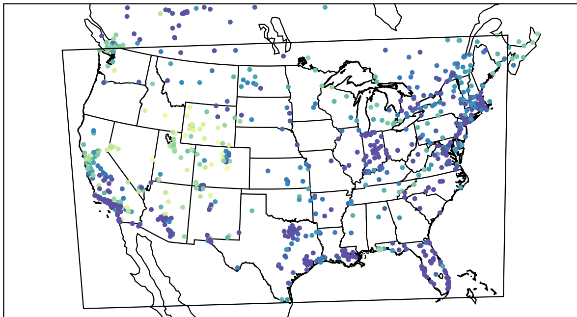
AirNOW (2021-12-27_12:00:00)
