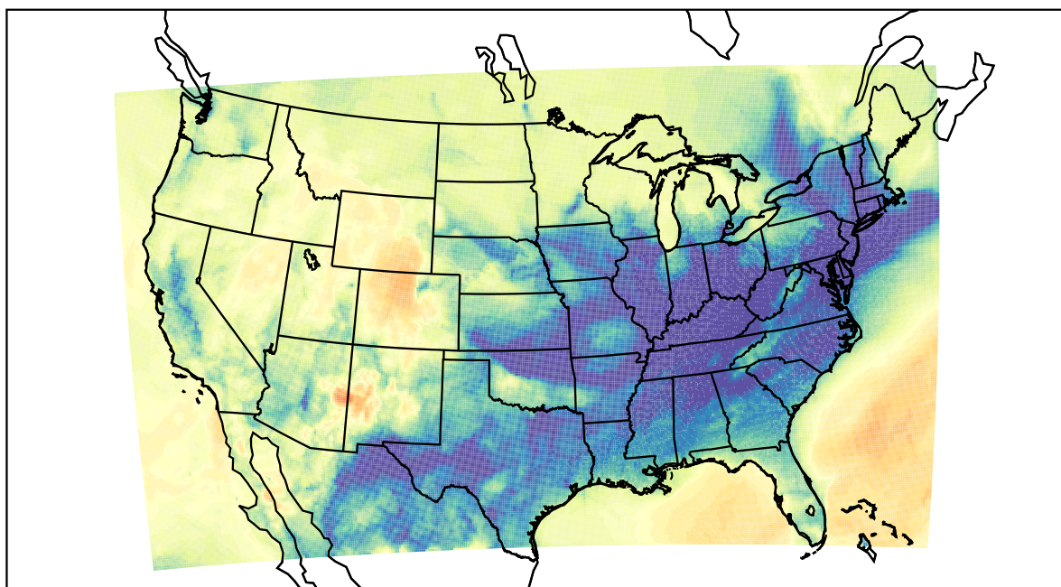
WRF (2021-12-26_07:00:00)
