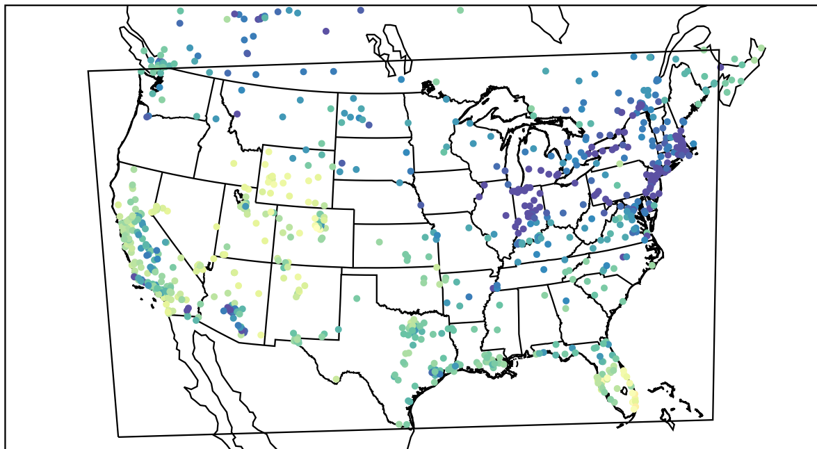
AirNOW (2021-12-27_21:00:00)
