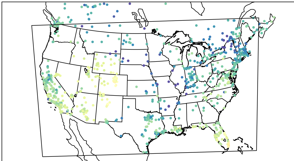
AirNOW (2021-12-26_20:00:00)
