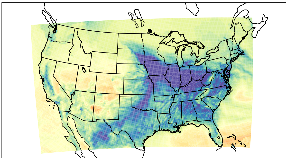
WRF (2021-12-27_05:00:00)
