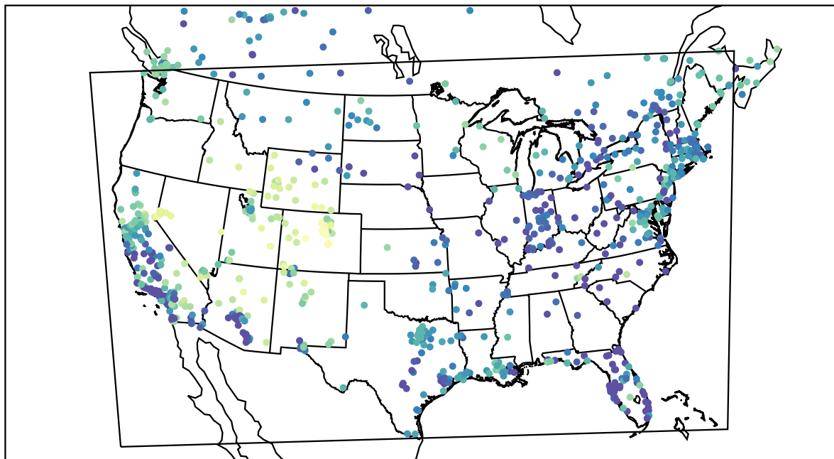
AirNOW (2021-12-27_03:00:00)
