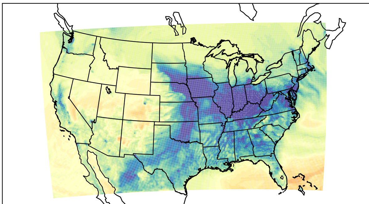
WRF (2021-12-27_02:00:00)
