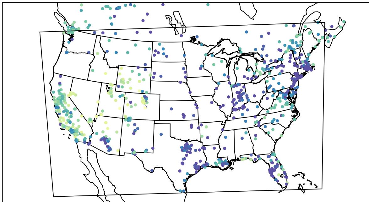
AirNOW (2021-12-26_05:00:00)
