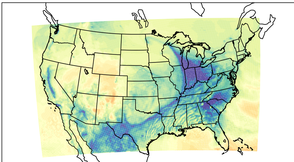
WRF (2021-12-27_16:00:00)
