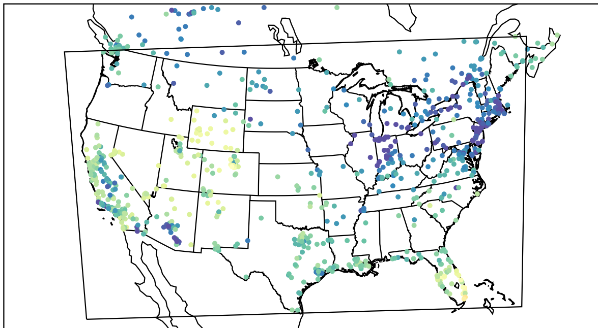
AirNOW (2021-12-27_20:00:00)
