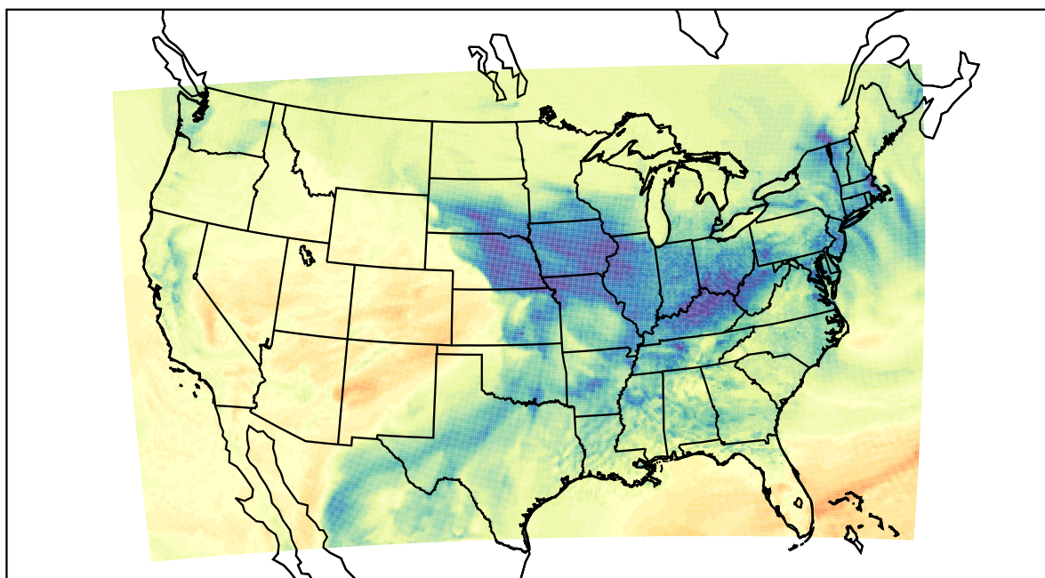
WRF (2021-12-26_21:00:00)
