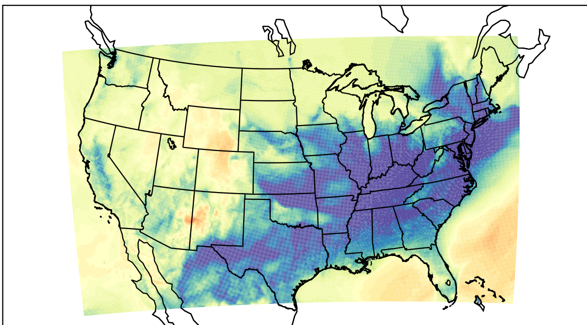
WRF (2021-12-26_09:00:00)
