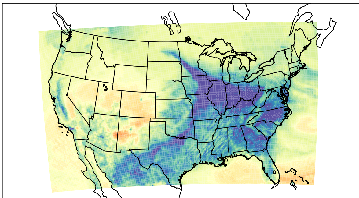
WRF (2021-12-27_09:00:00)
