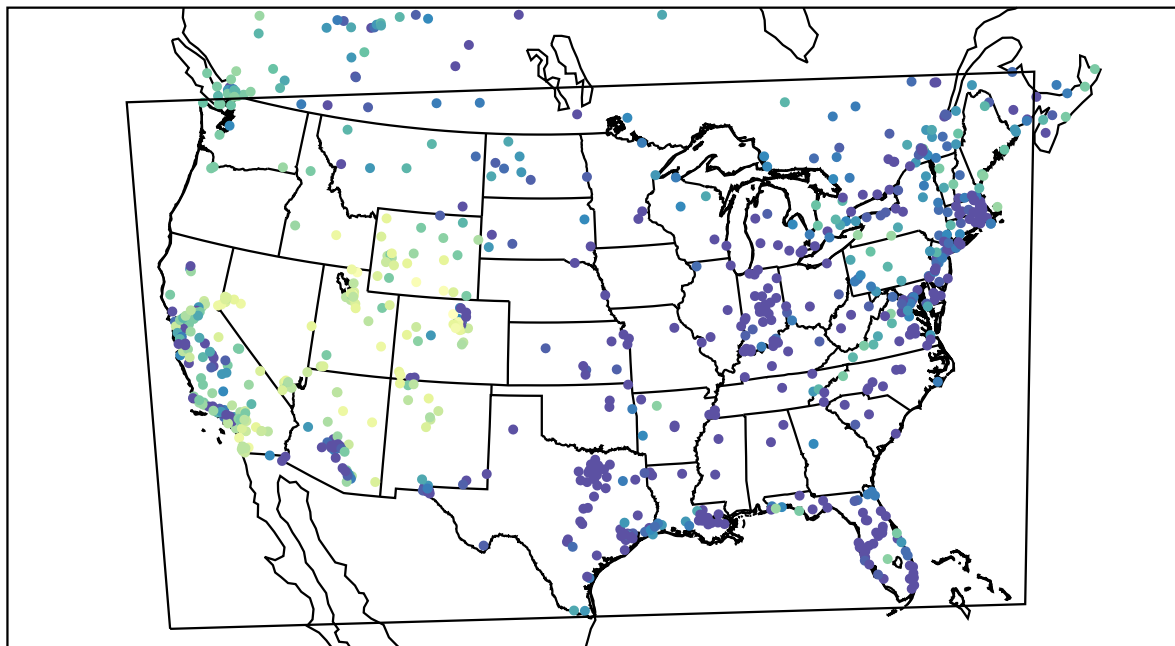
AirNOW (2021-12-26_12:00:00)
