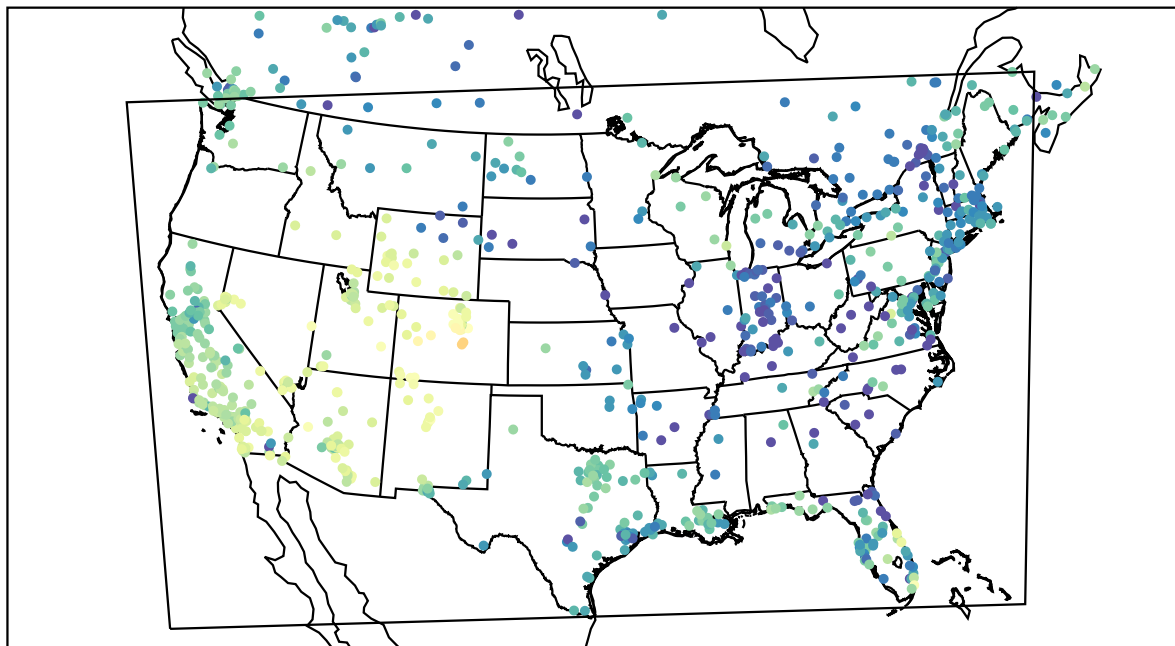
AirNOW (2021-12-26_23:00:00)
