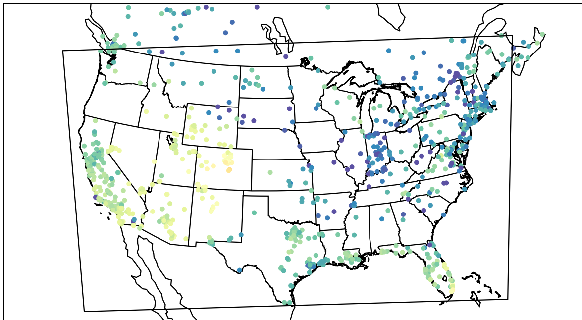
AirNOW (2021-12-26_22:00:00)
