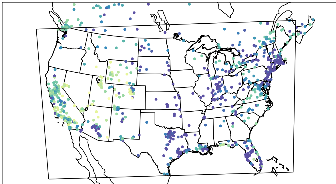
AirNOW (2021-12-26_06:00:00)
