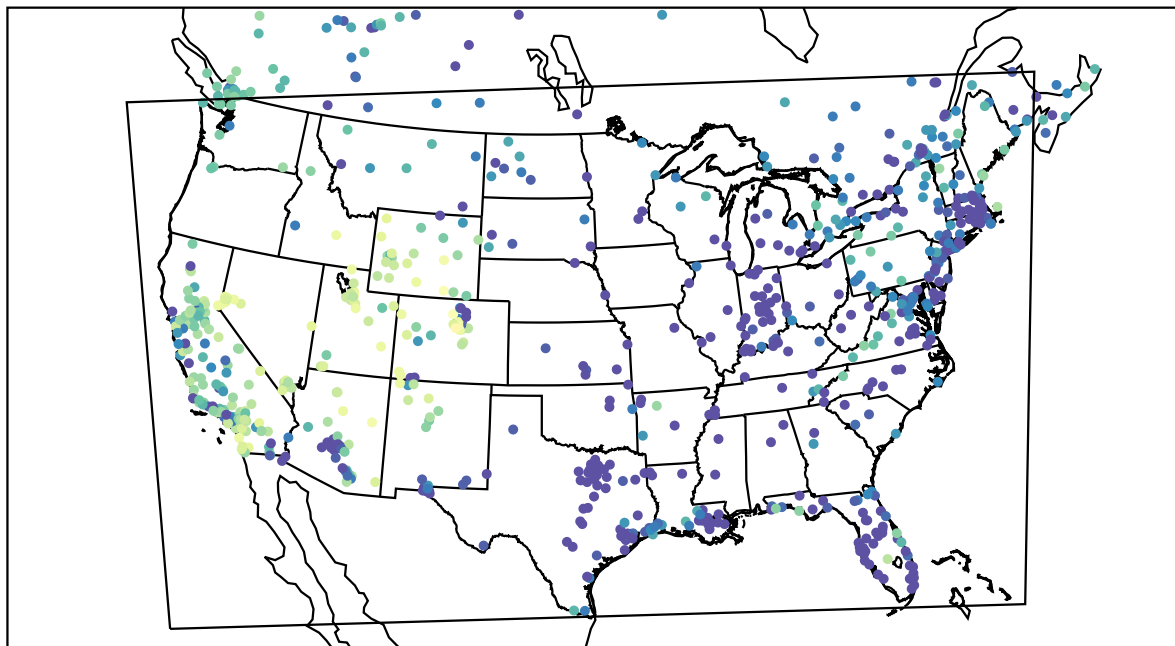
AirNOW (2021-12-26_11:00:00)
