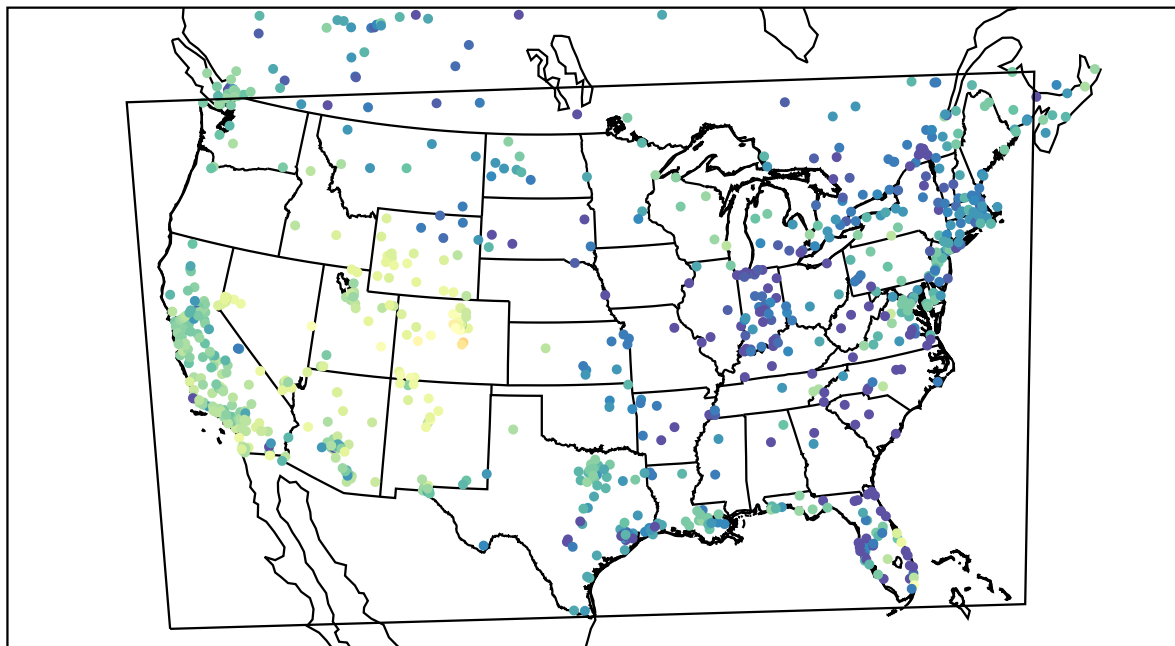
AirNOW (2021-12-27_00:00:00)
