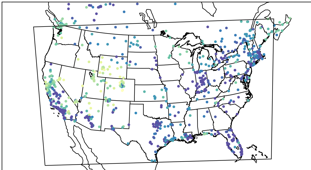
AirNOW (2021-12-27_09:00:00)
