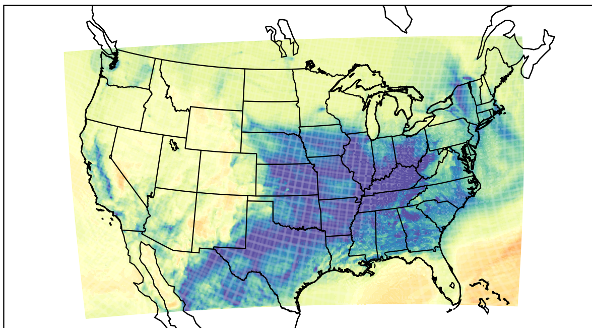
WRF (2021-12-26_16:00:00)
