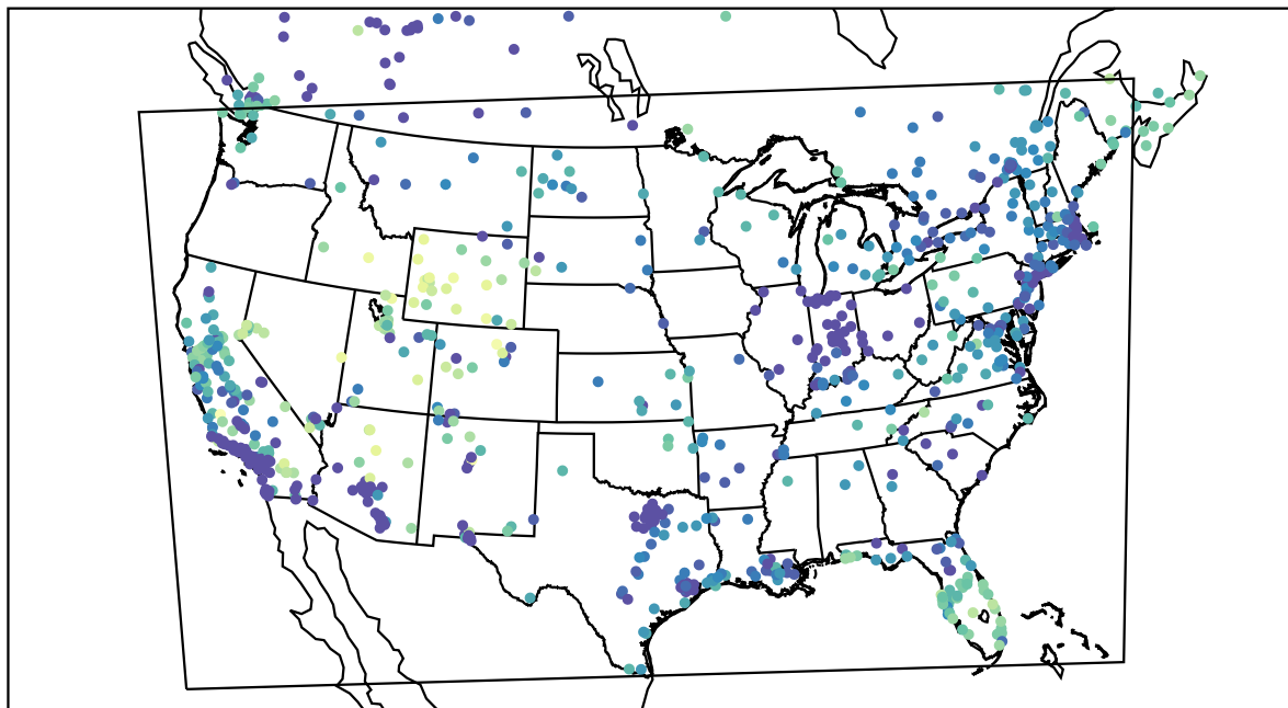
AirNOW (2021-12-27_15:00:00)
