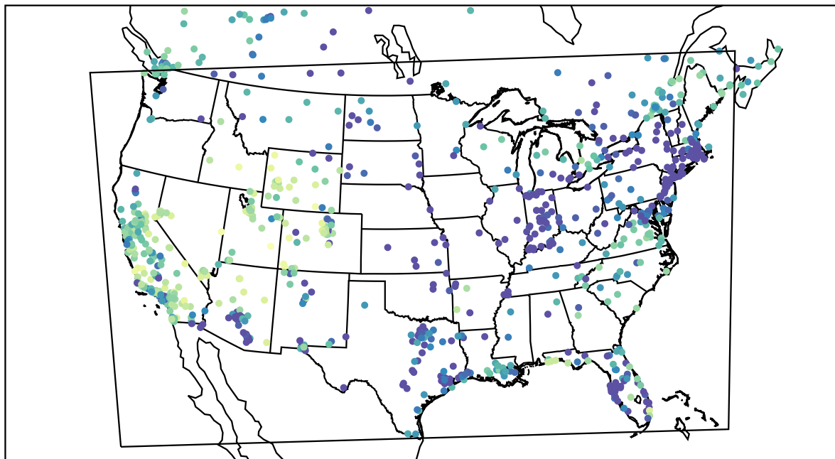
AirNOW (2021-12-26_03:00:00)
