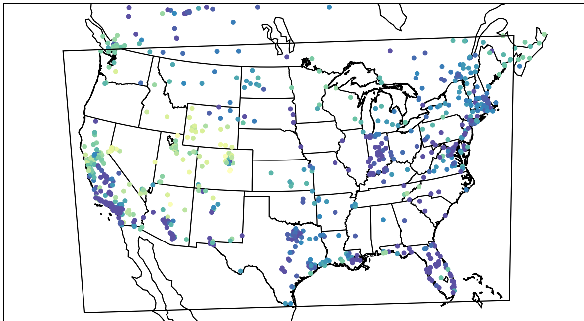
AirNOW (2021-12-27_08:00:00)
