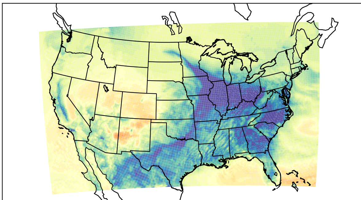
WRF (2021-12-27_10:00:00)
