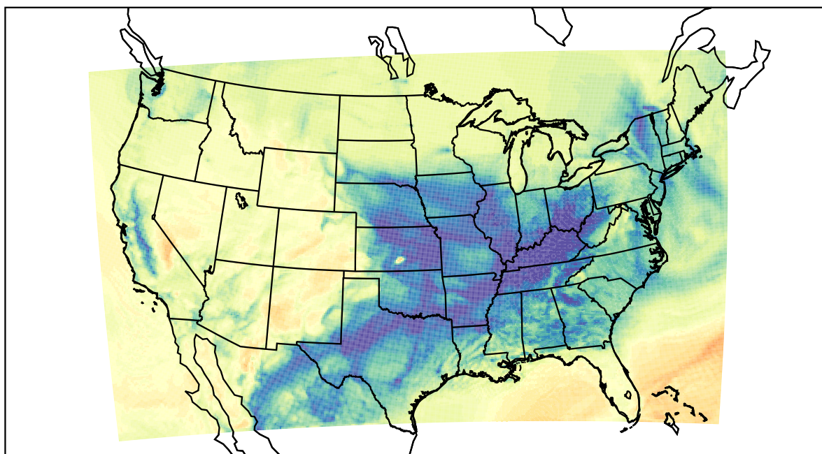
WRF (2021-12-26_17:00:00)
