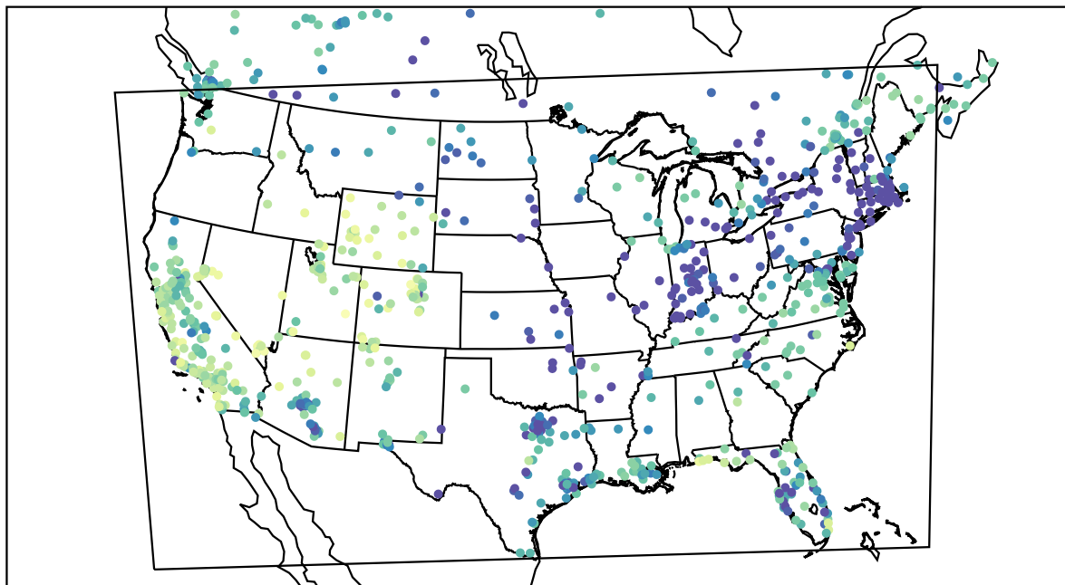
AirNOW (2021-12-26_00:00:00)
