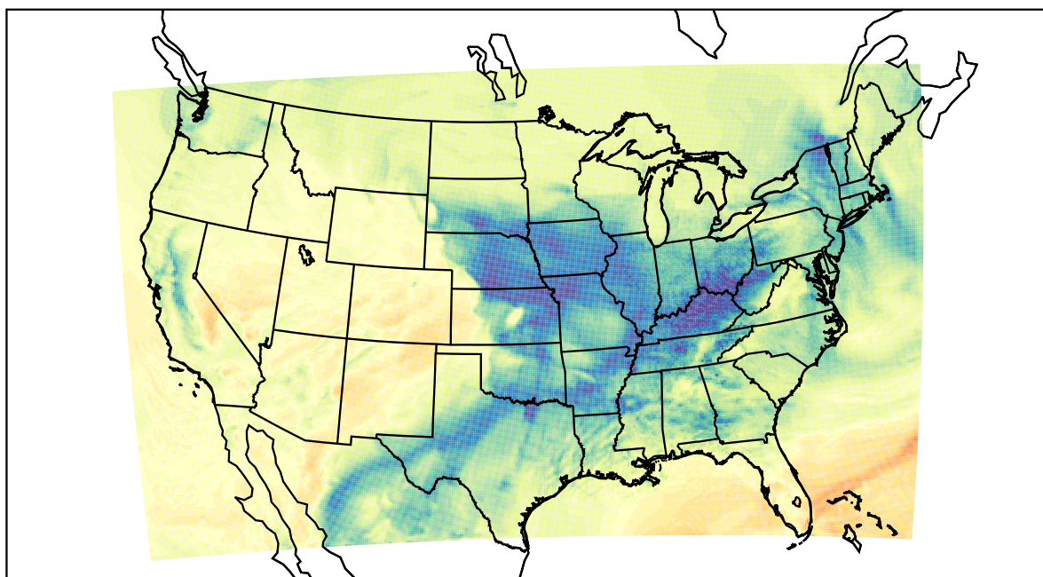
WRF (2021-12-26_19:00:00)
