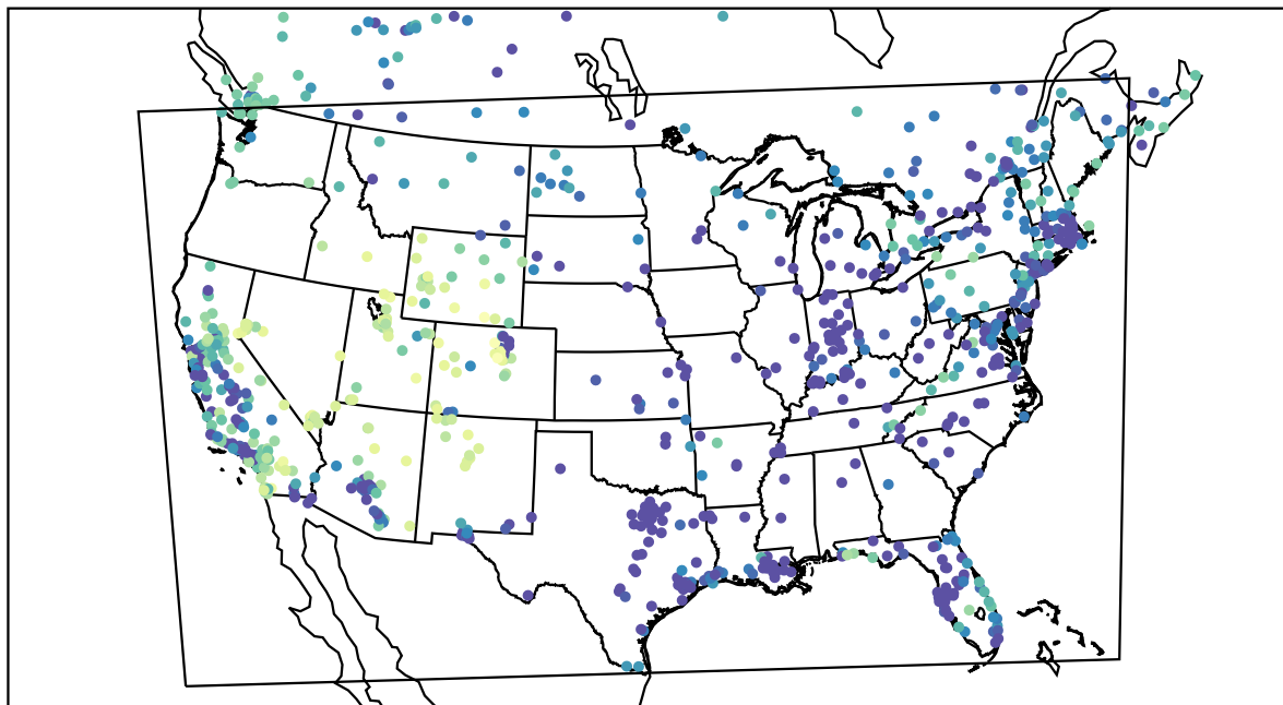
AirNOW (2021-12-26_13:00:00)
