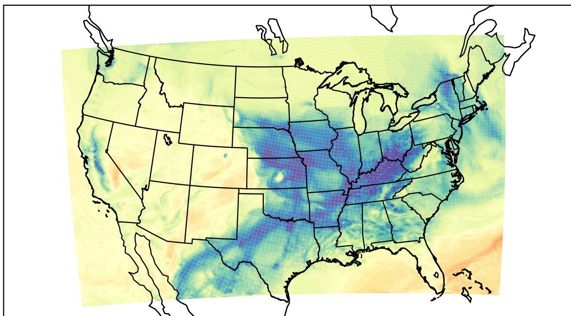
WRF (2021-12-26_18:00:00)
