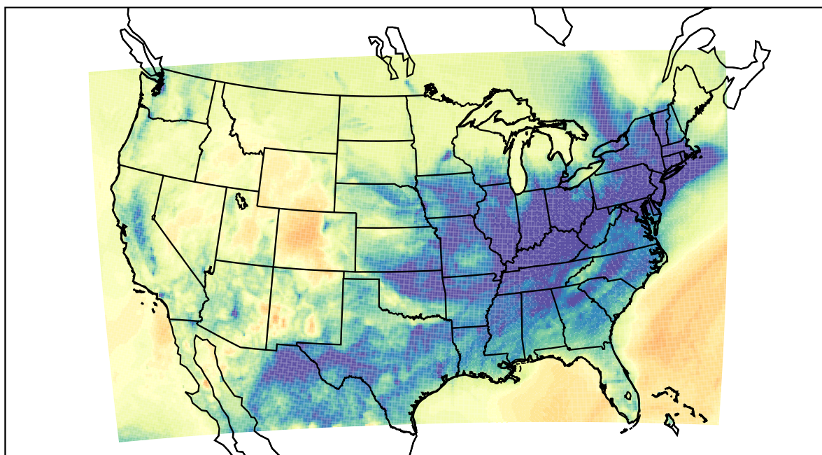
WRF (2021-12-26_04:00:00)
