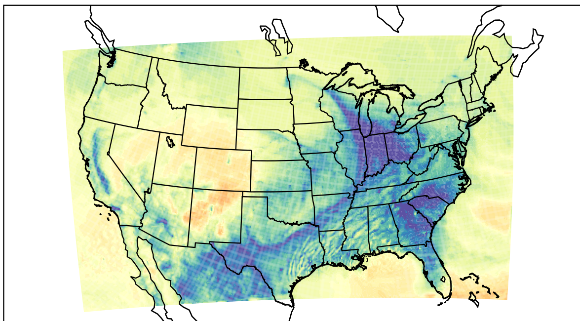
WRF (2021-12-27_15:00:00)
