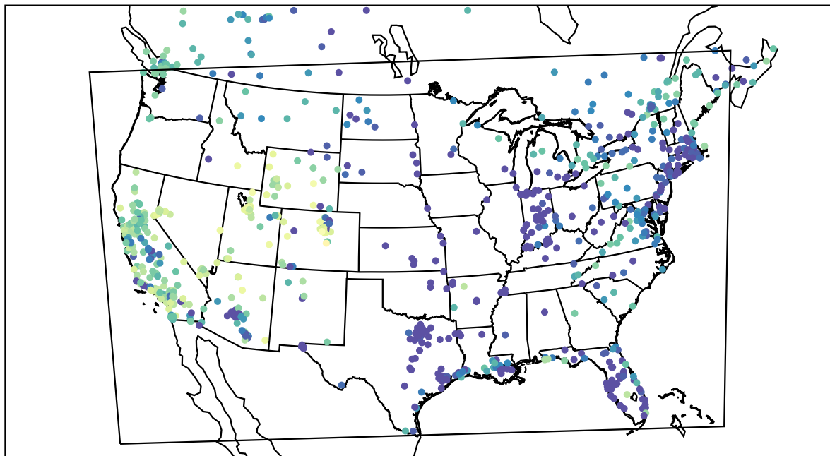
AirNOW (2021-12-26_08:00:00)
