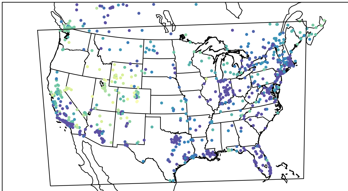
AirNOW (2021-12-27_11:00:00)
