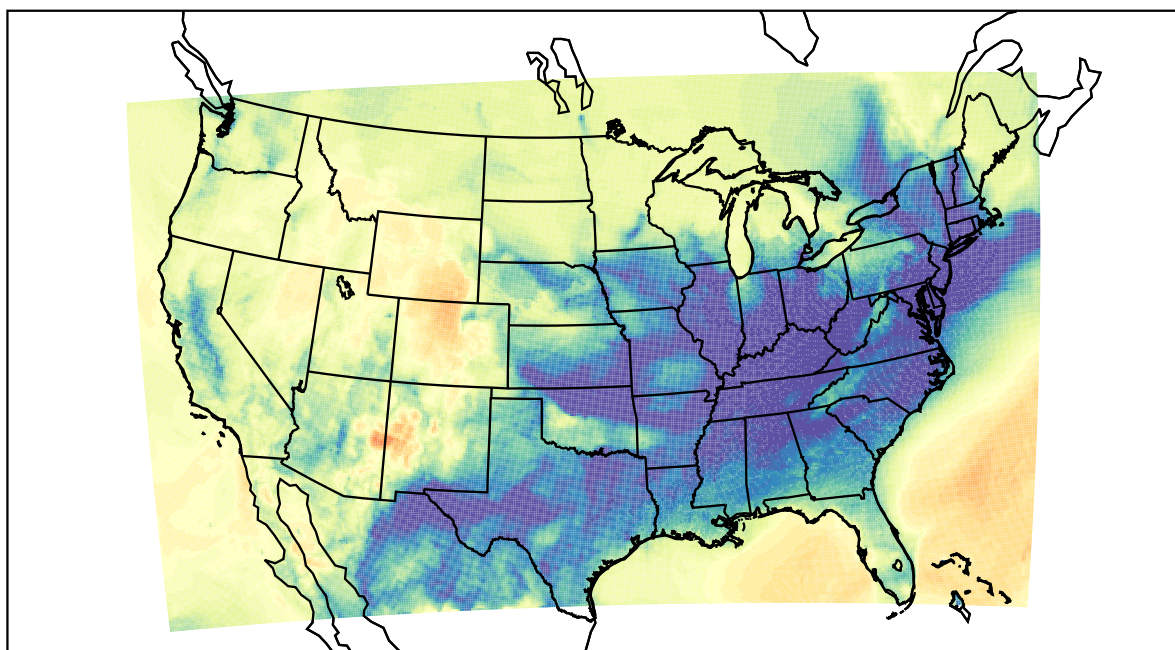
WRF (2021-12-26_08:00:00)
