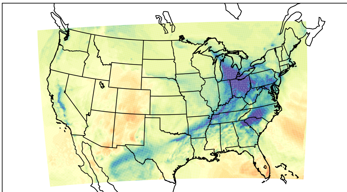
WRF (2021-12-27_20:00:00)
