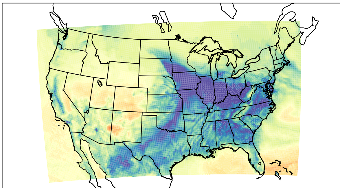
WRF (2021-12-27_06:00:00)
