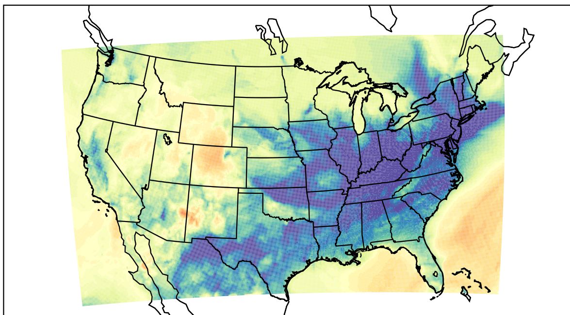
WRF (2021-12-26_06:00:00)
