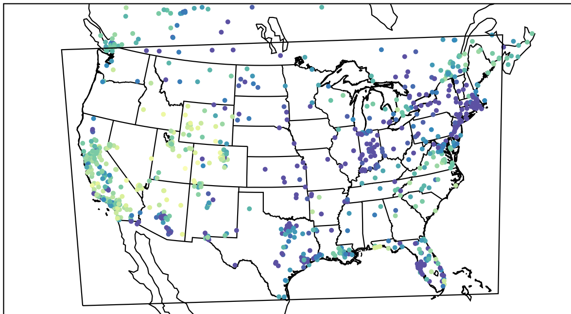
AirNOW (2021-12-26_02:00:00)
