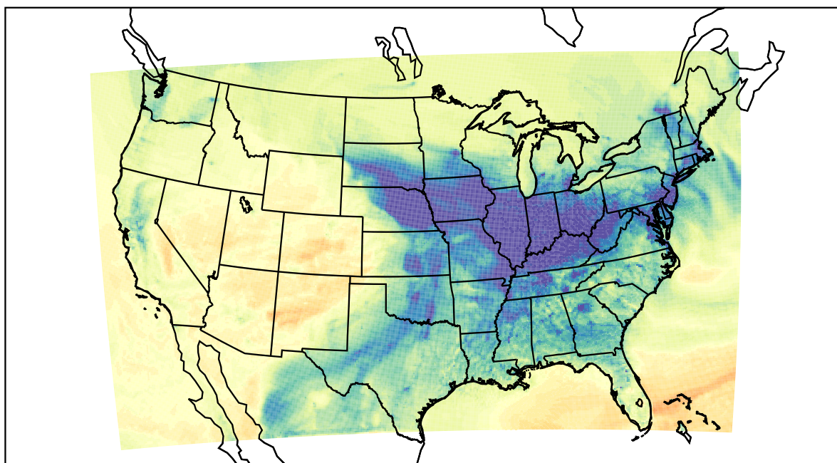
WRF (2021-12-26_23:00:00)
