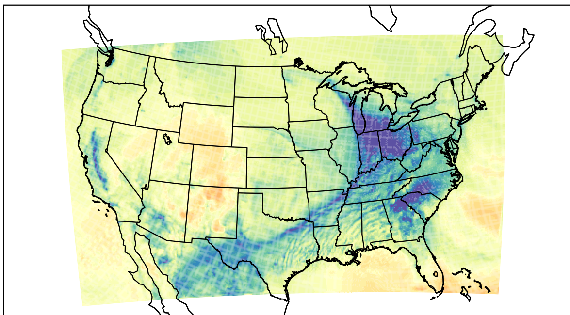
WRF (2021-12-27_17:00:00)
