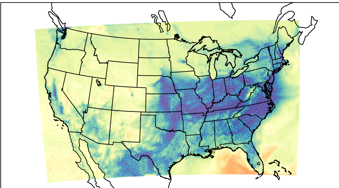
WRF (2021-12-28_14:00:00)
