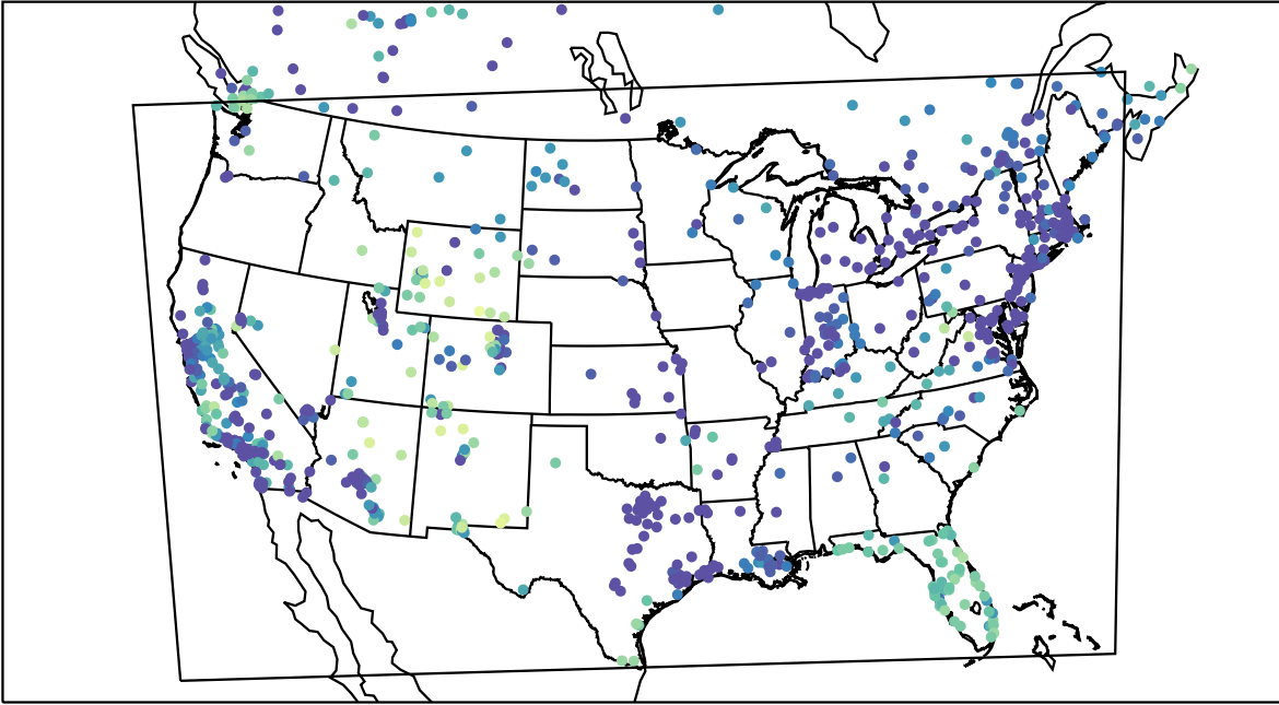
AirNOW (2021-12-29_15:00:00)
