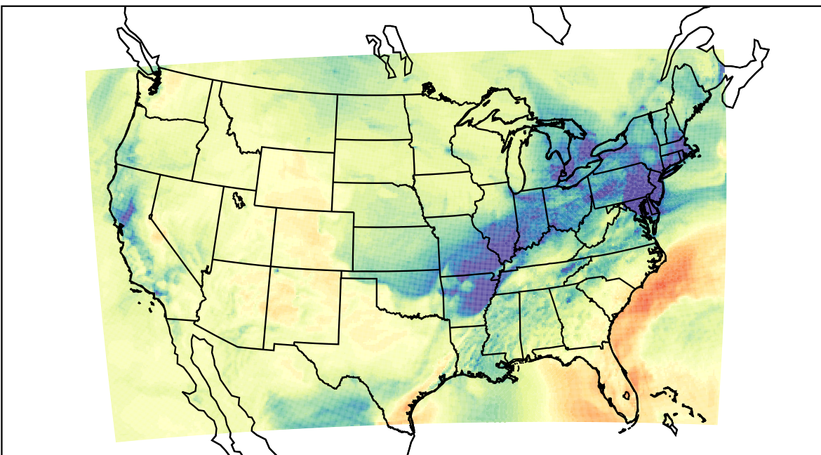
WRF (2021-12-29_21:00:00)
