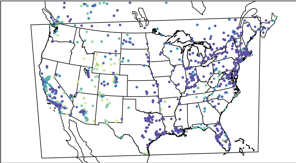
AirNOW (2021-12-29_12:00:00)
