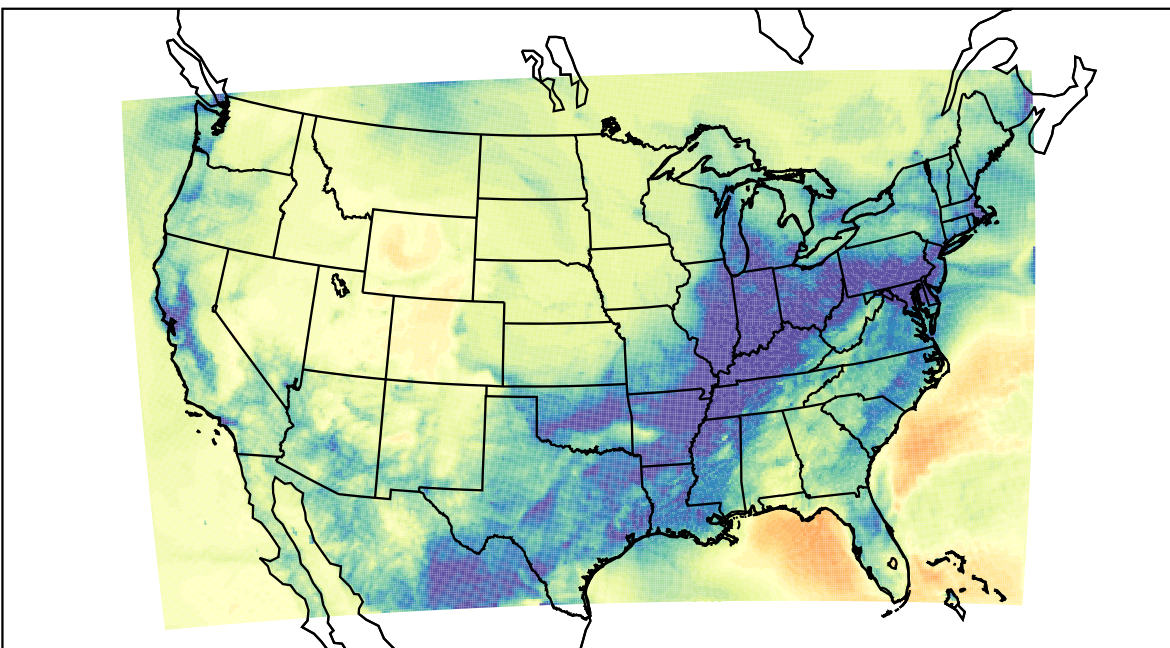
WRF (2021-12-29_12:00:00)
