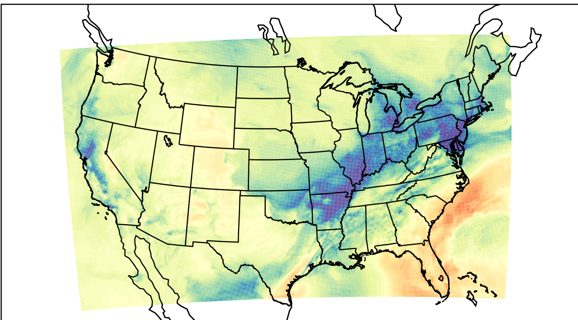
WRF (2021-12-29_19:00:00)
