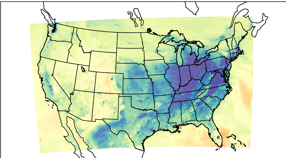
WRF (2021-12-28_01:00:00)
