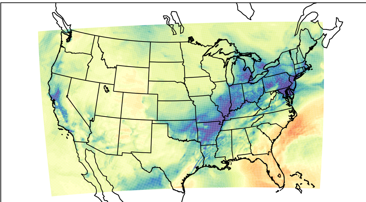
WRF (2021-12-29_18:00:00)
