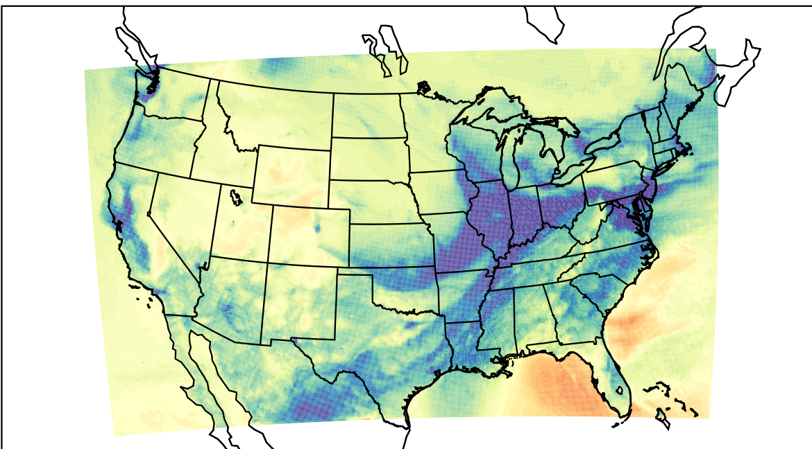
WRF (2021-12-29_05:00:00)
