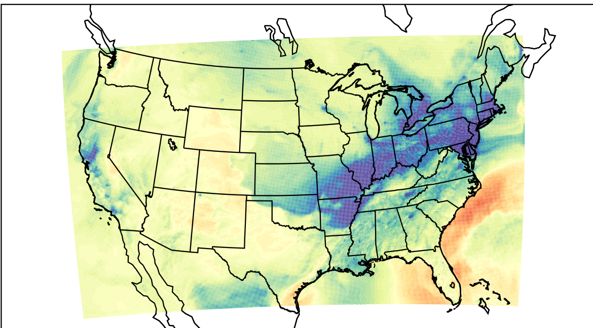
WRF (2021-12-29_22:00:00)
