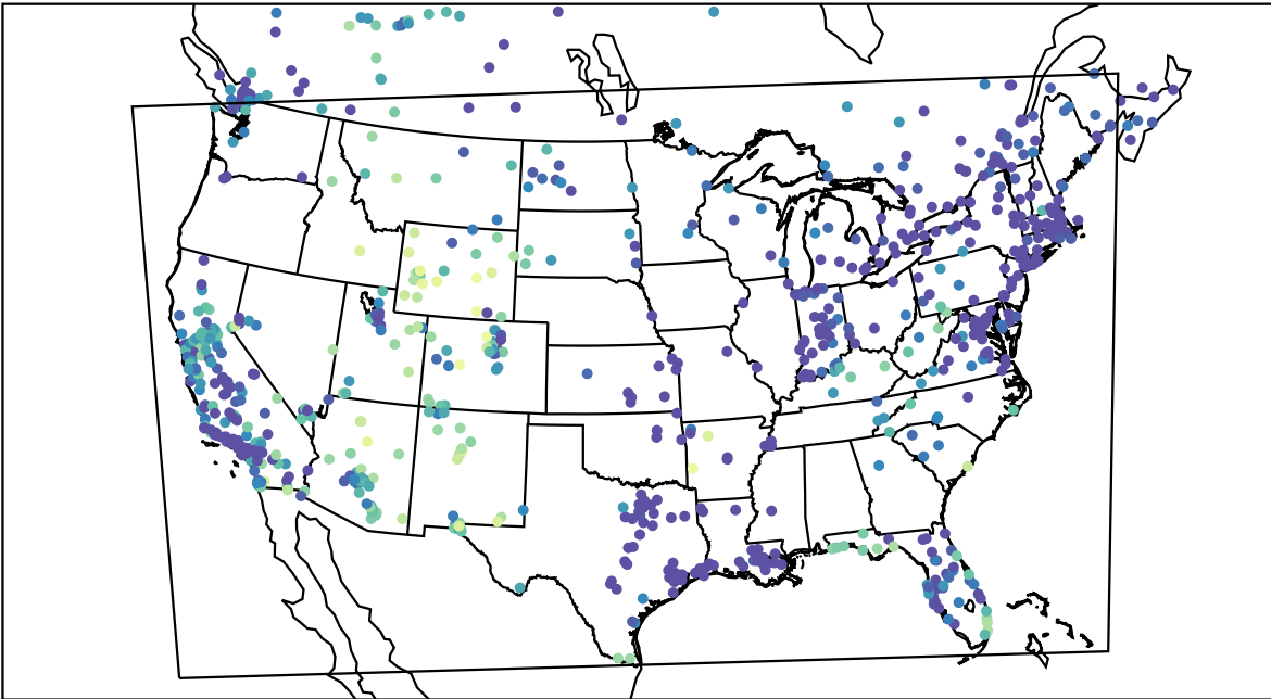
AirNOW (2021-12-29_08:00:00)
