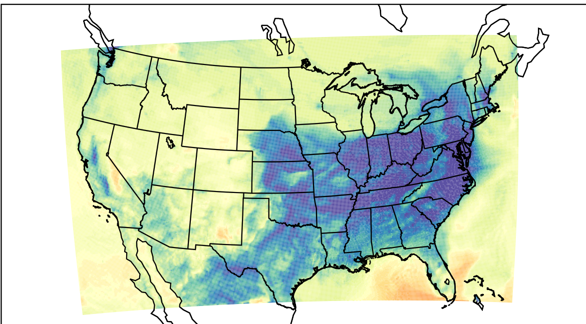
WRF (2021-12-28_10:00:00)
