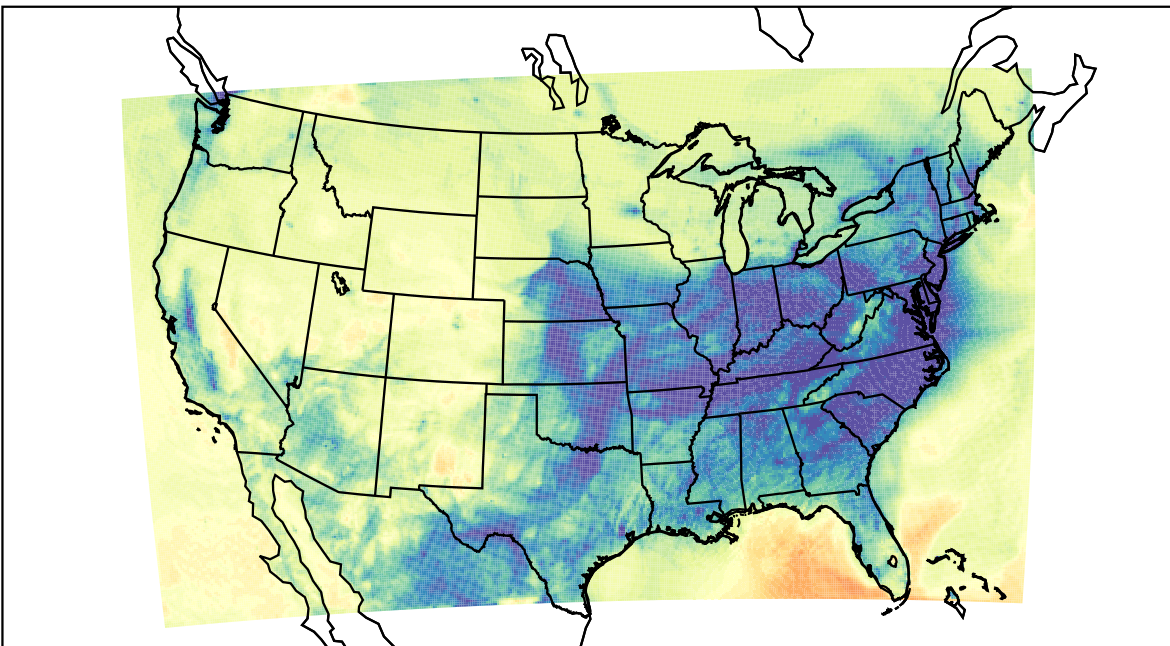
WRF (2021-12-28_13:00:00)
