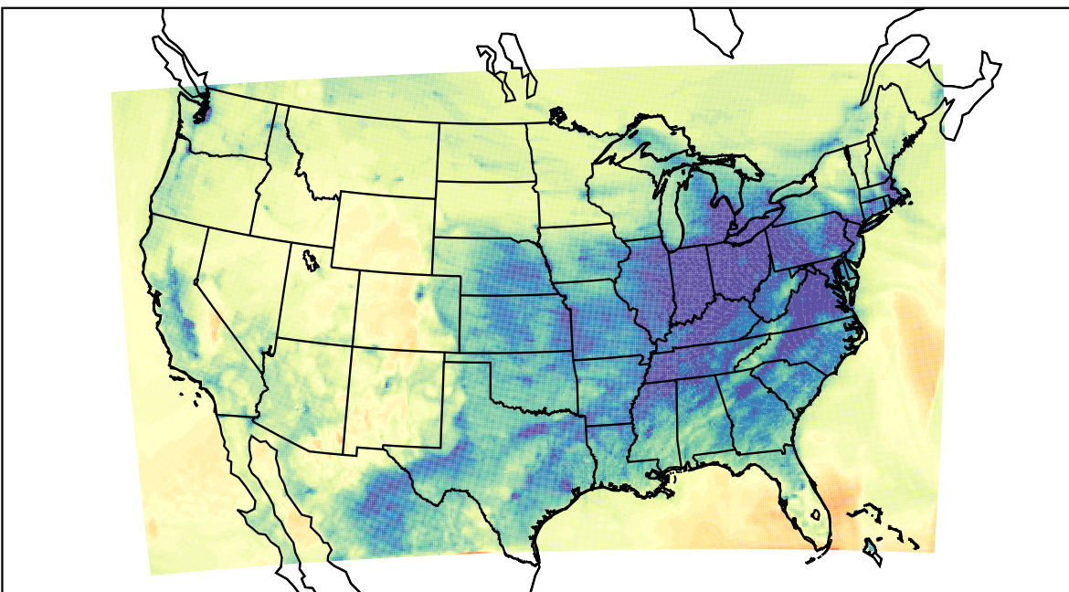
WRF (2021-12-28_02:00:00)
