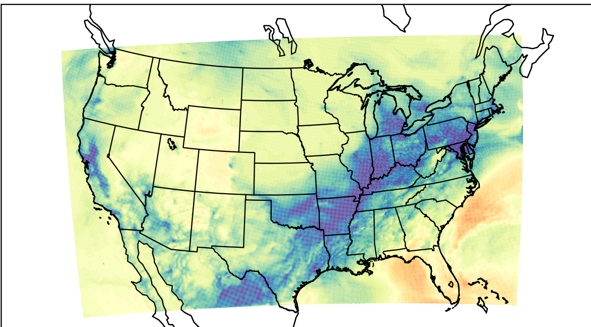
WRF (2021-12-29_16:00:00)
