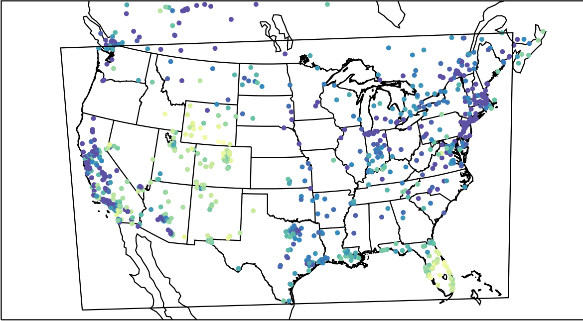
AirNOW (2021-12-28_16:00:00)
