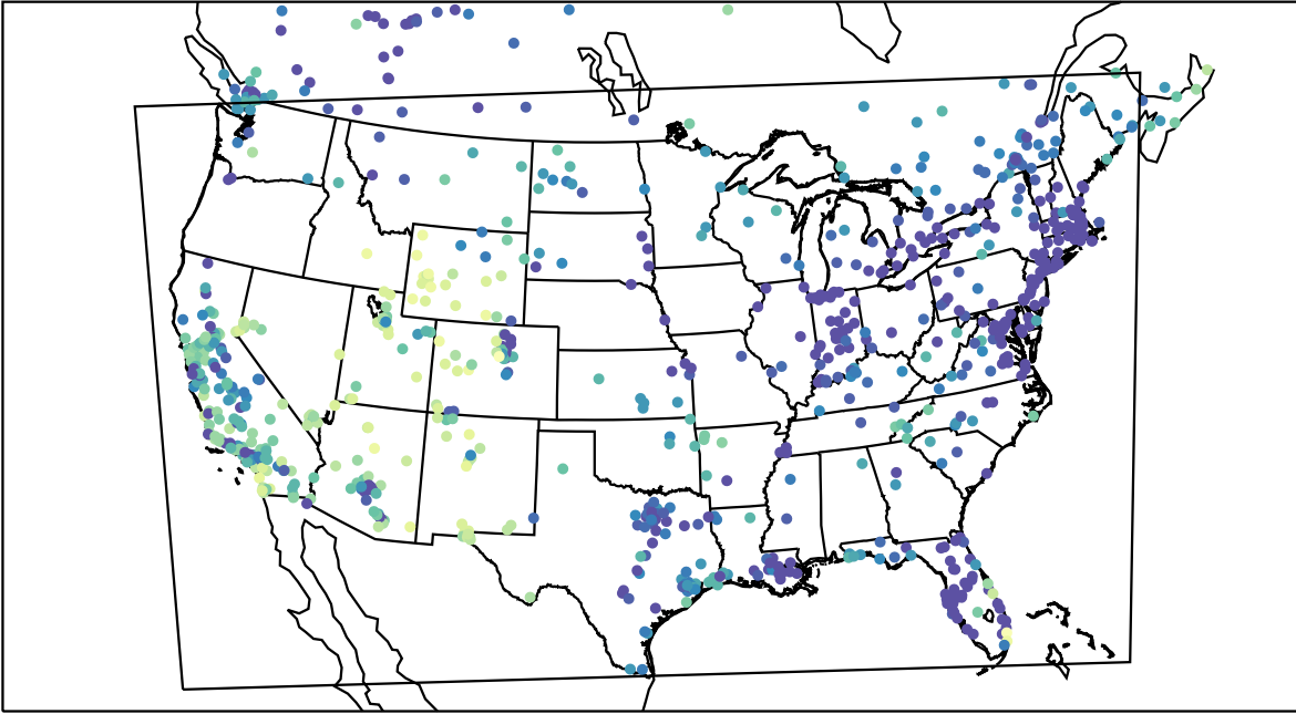
AirNOW (2021-12-28_02:00:00)
