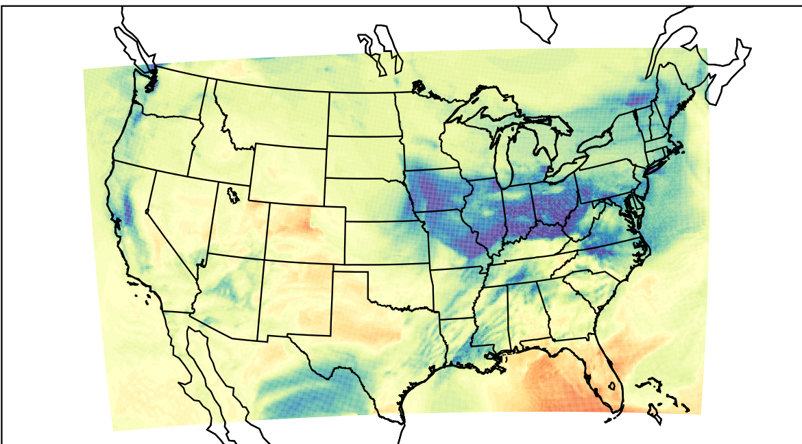
WRF (2021-12-28_19:00:00)
