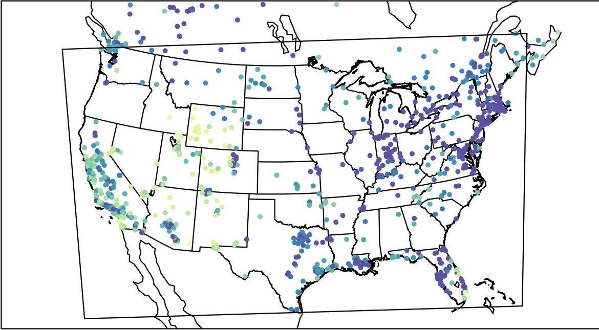
AirNOW (2021-12-28_01:00:00)
