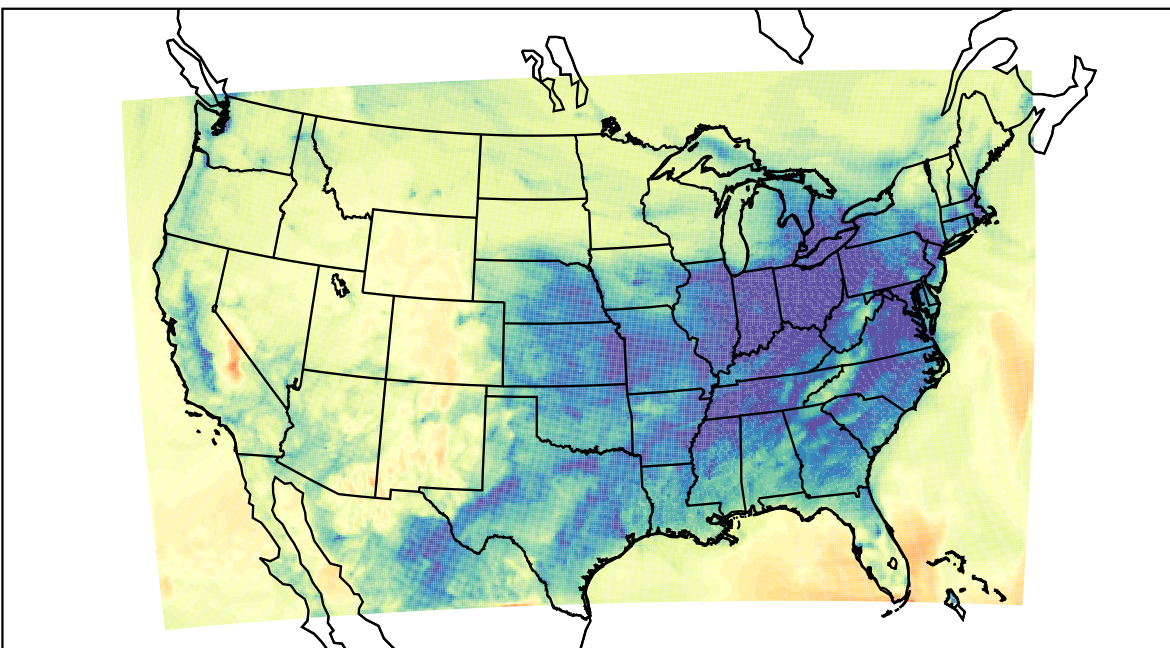
WRF (2021-12-28_04:00:00)
