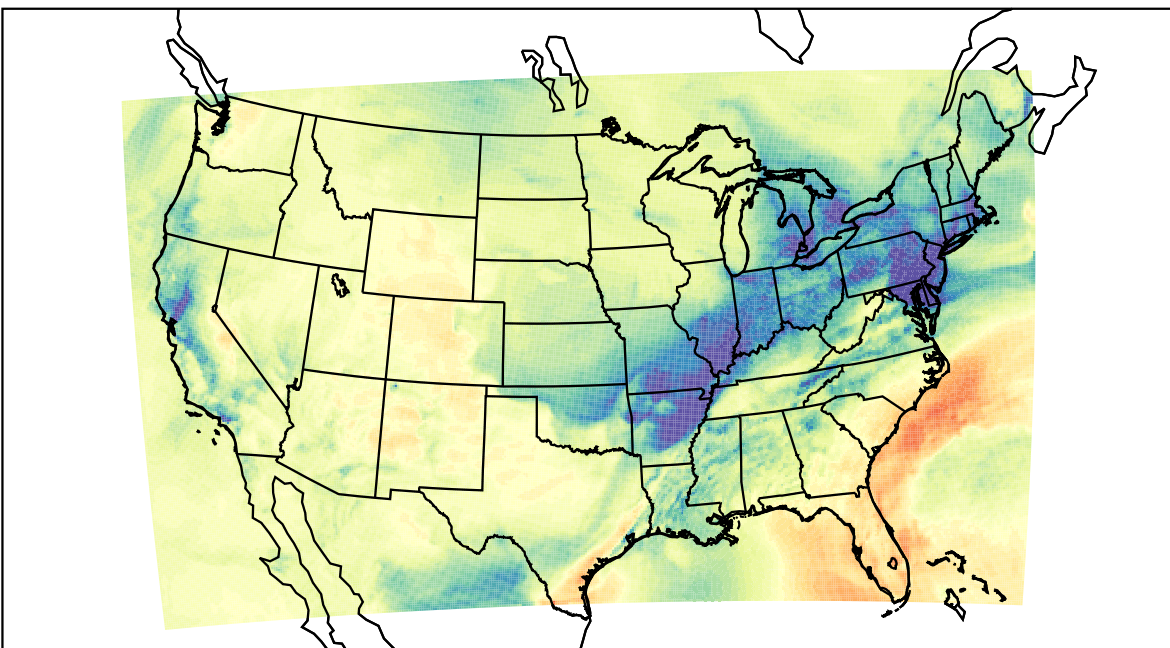
WRF (2021-12-29_20:00:00)
