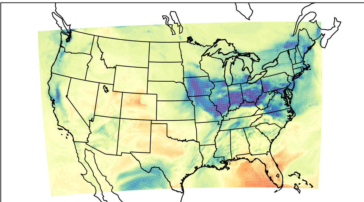
WRF (2021-12-28_20:00:00)
