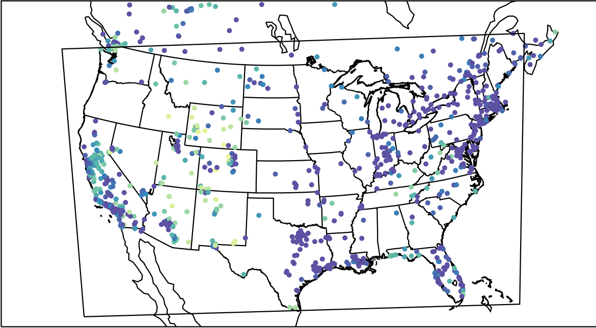
AirNOW (2021-12-29_13:00:00)
