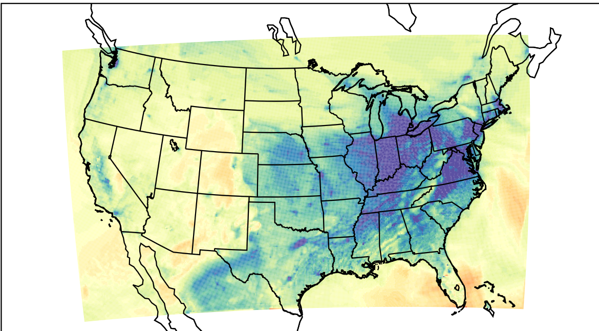
WRF (2021-12-28_00:00:00)
