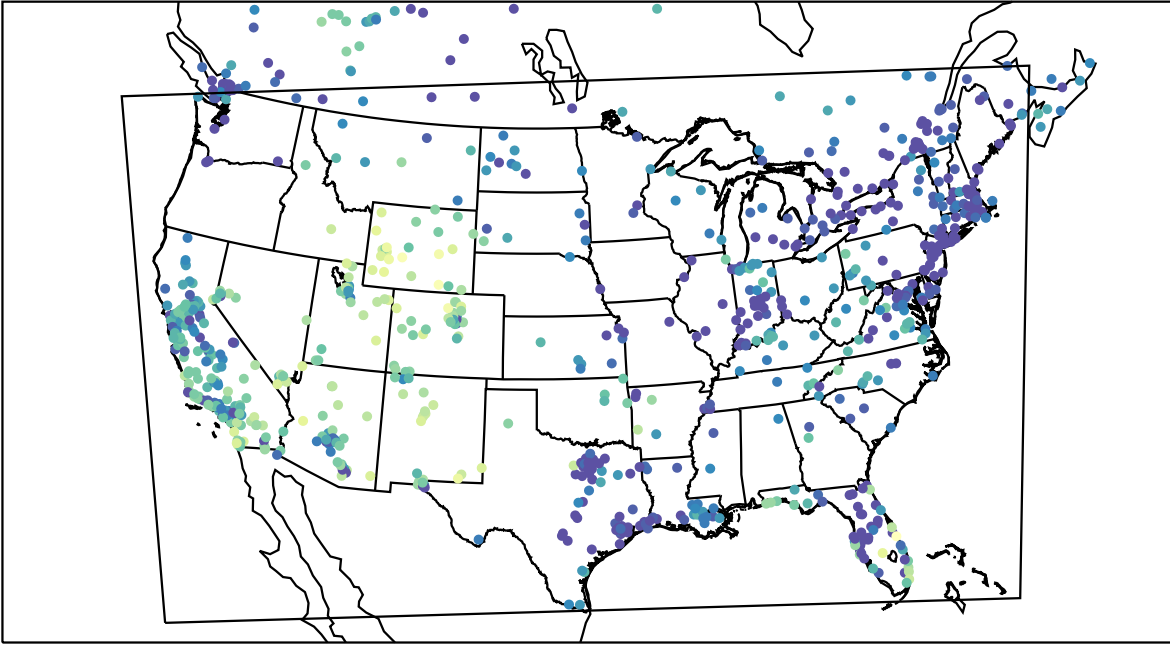
AirNOW (2021-12-29_01:00:00)
