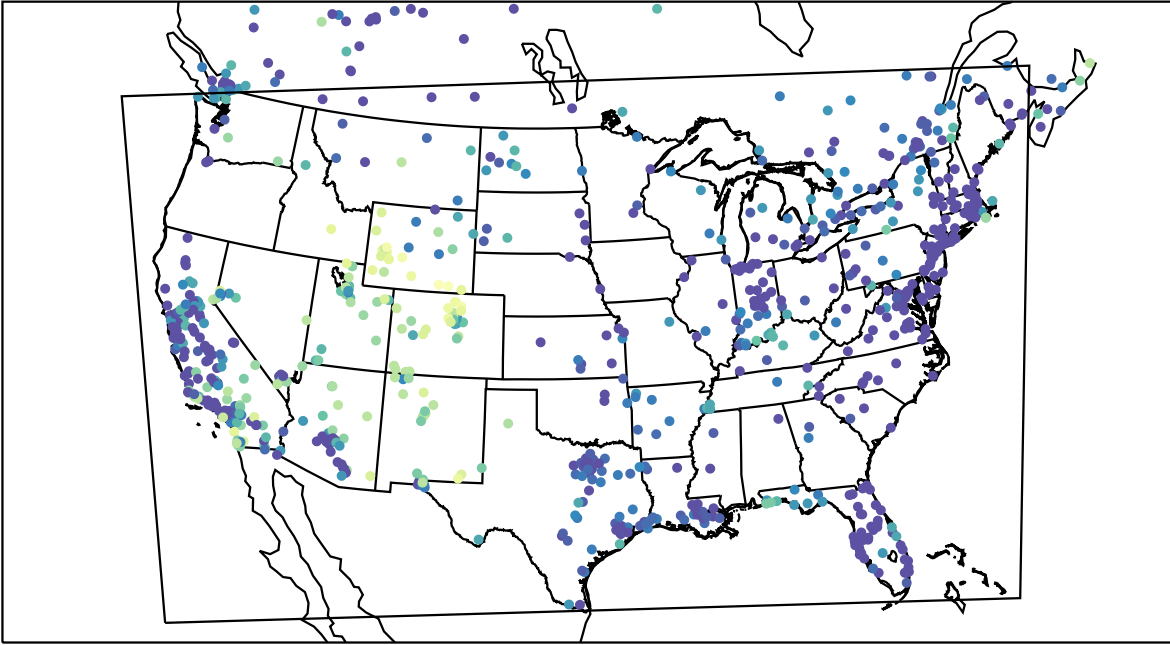
AirNOW (2021-12-28_13:00:00)
