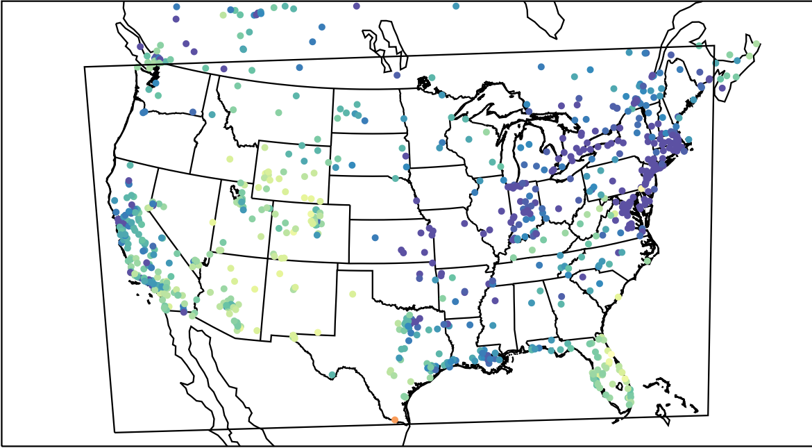
AirNOW (2021-12-29_19:00:00)
