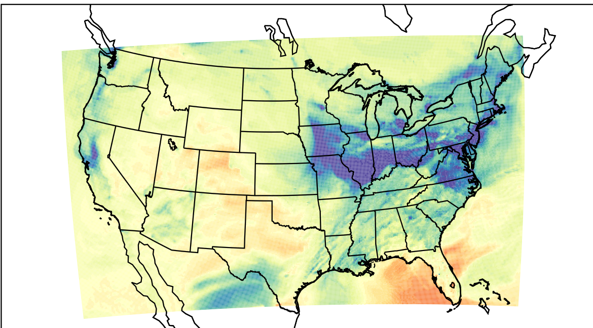
WRF (2021-12-28_22:00:00)
