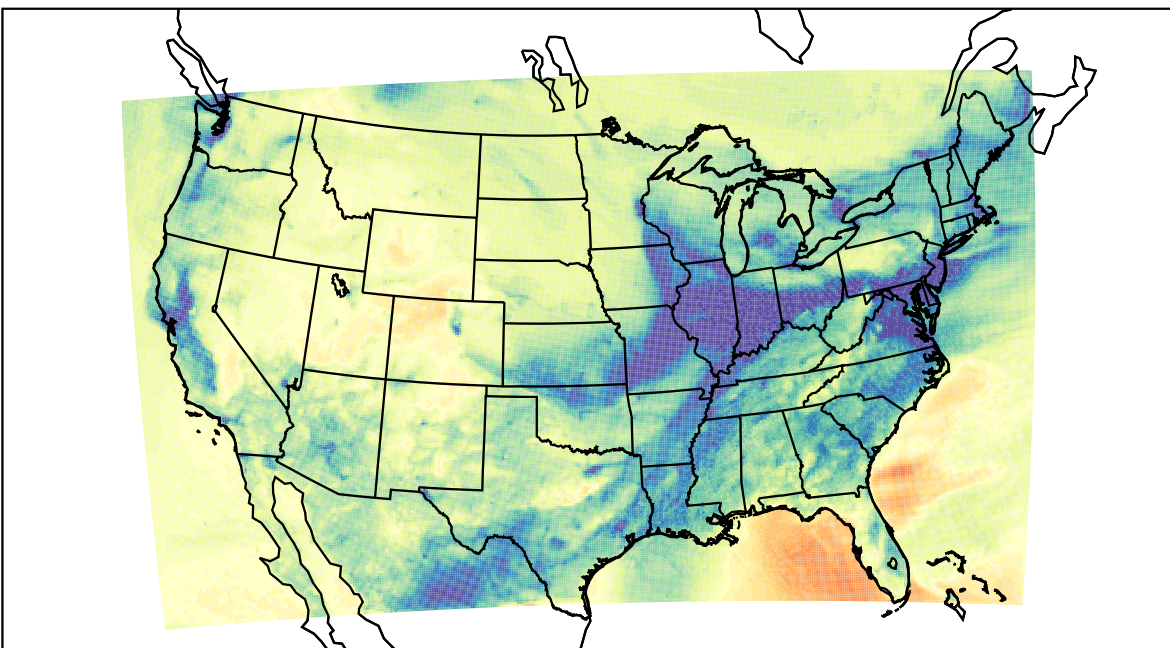
WRF (2021-12-29_03:00:00)
