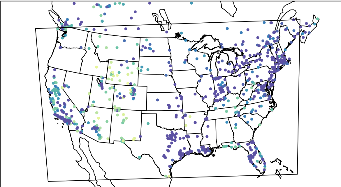
AirNOW (2021-12-29_11:00:00)
