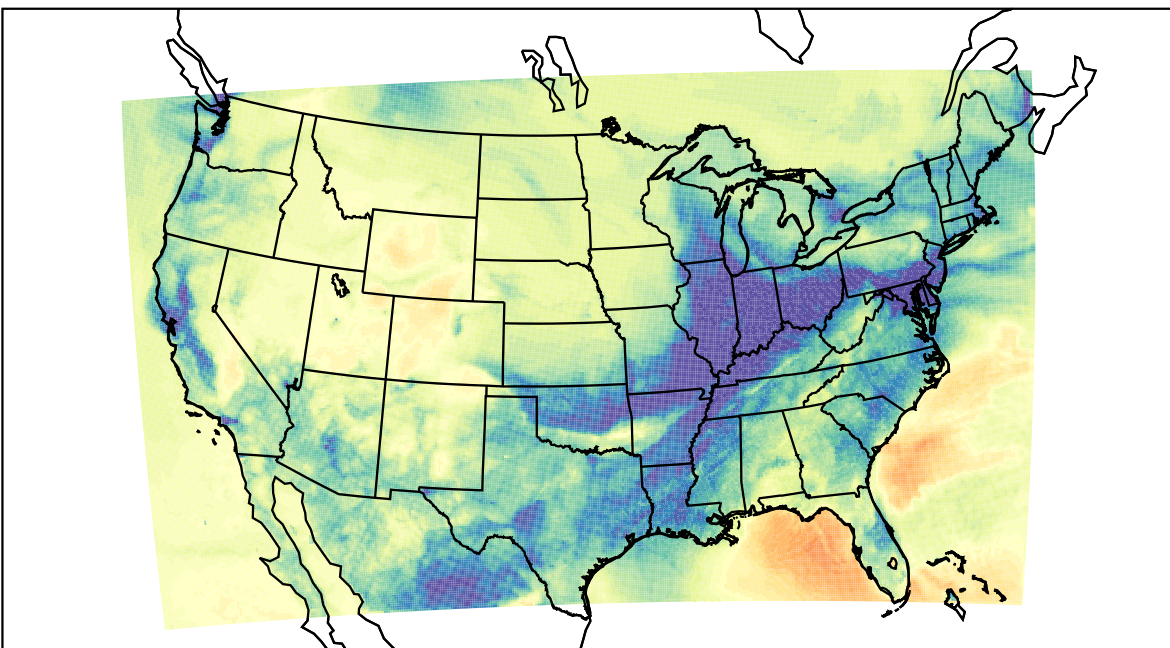
WRF (2021-12-29_08:00:00)
