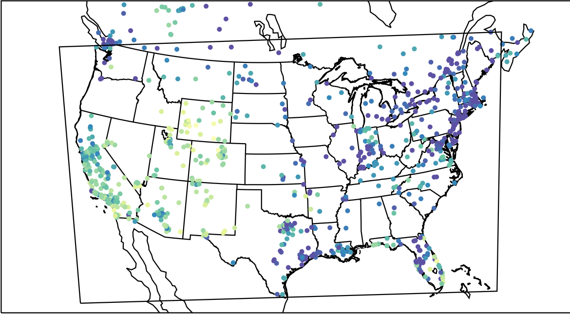
AirNOW (2021-12-29_00:00:00)
