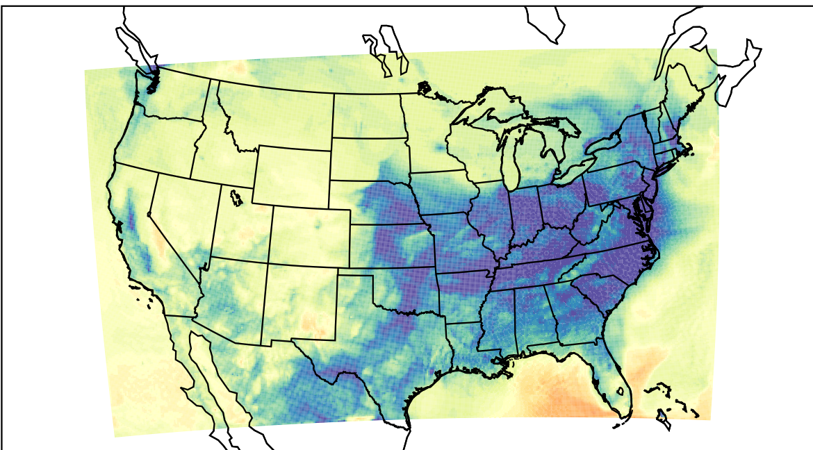
WRF (2021-12-28_12:00:00)
