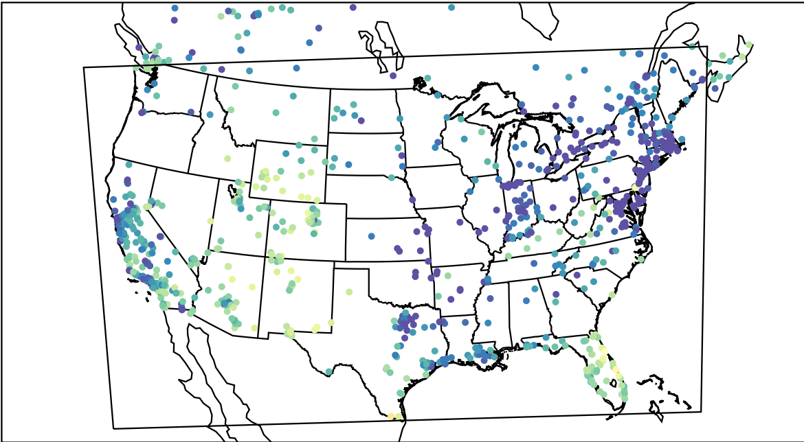
AirNOW (2021-12-29_18:00:00)
