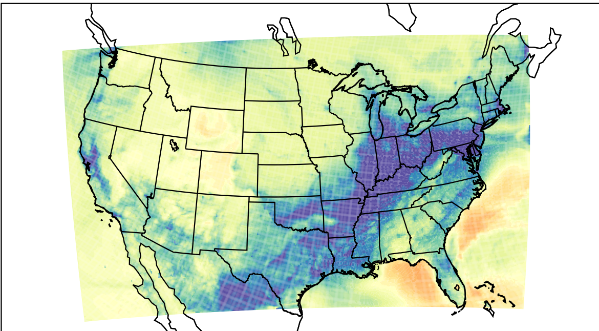
WRF (2021-12-29_13:00:00)
