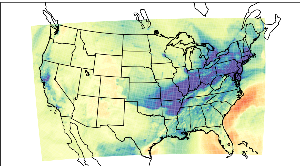
WRF (2021-12-29_23:00:00)
