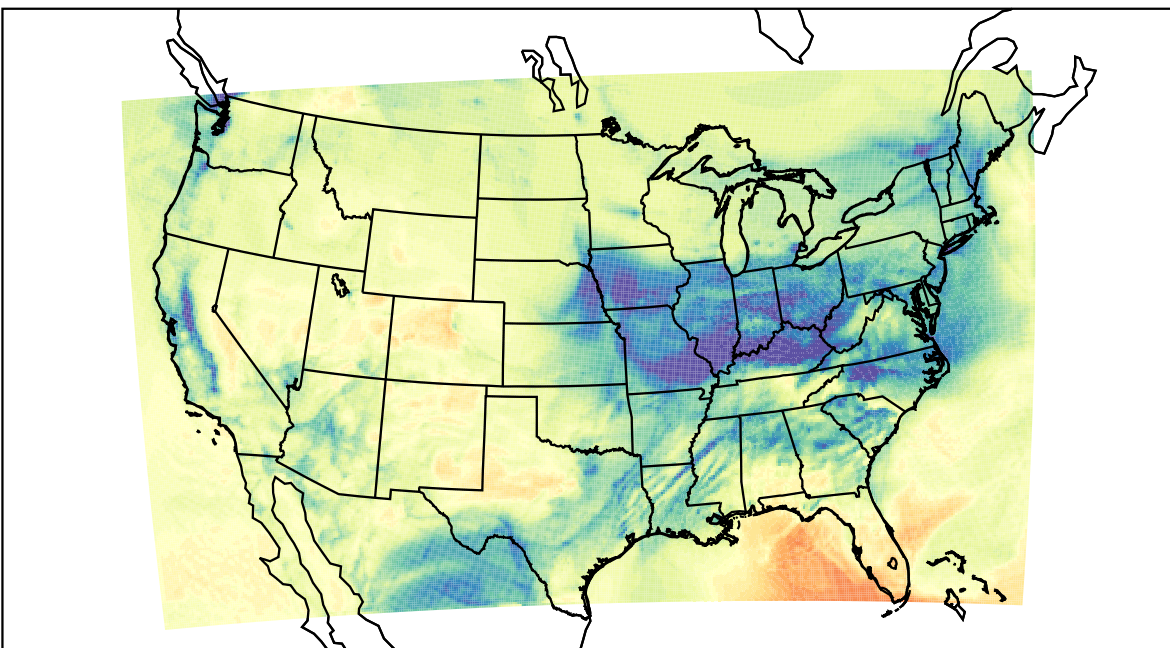
WRF (2021-12-28_17:00:00)
