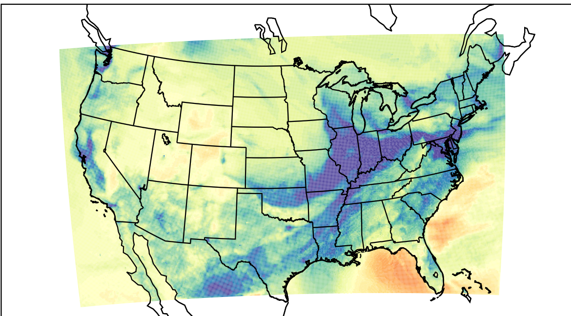
WRF (2021-12-29_06:00:00)
