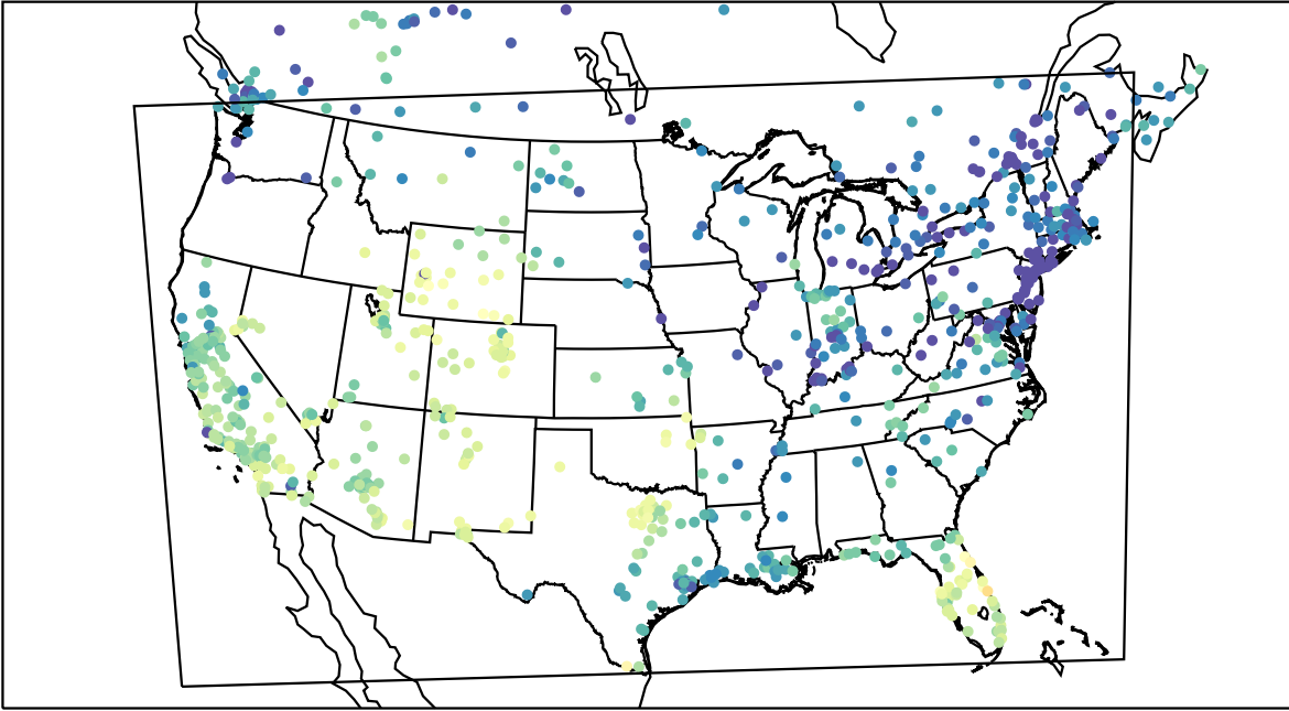
AirNOW (2021-12-28_21:00:00)
