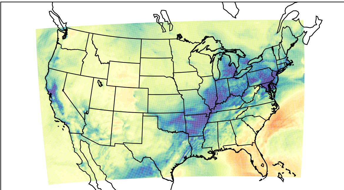
WRF (2021-12-29_17:00:00)
