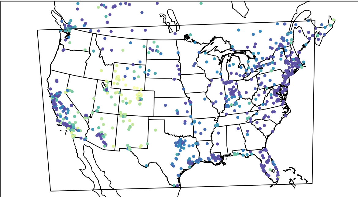
AirNOW (2021-12-28_12:00:00)
