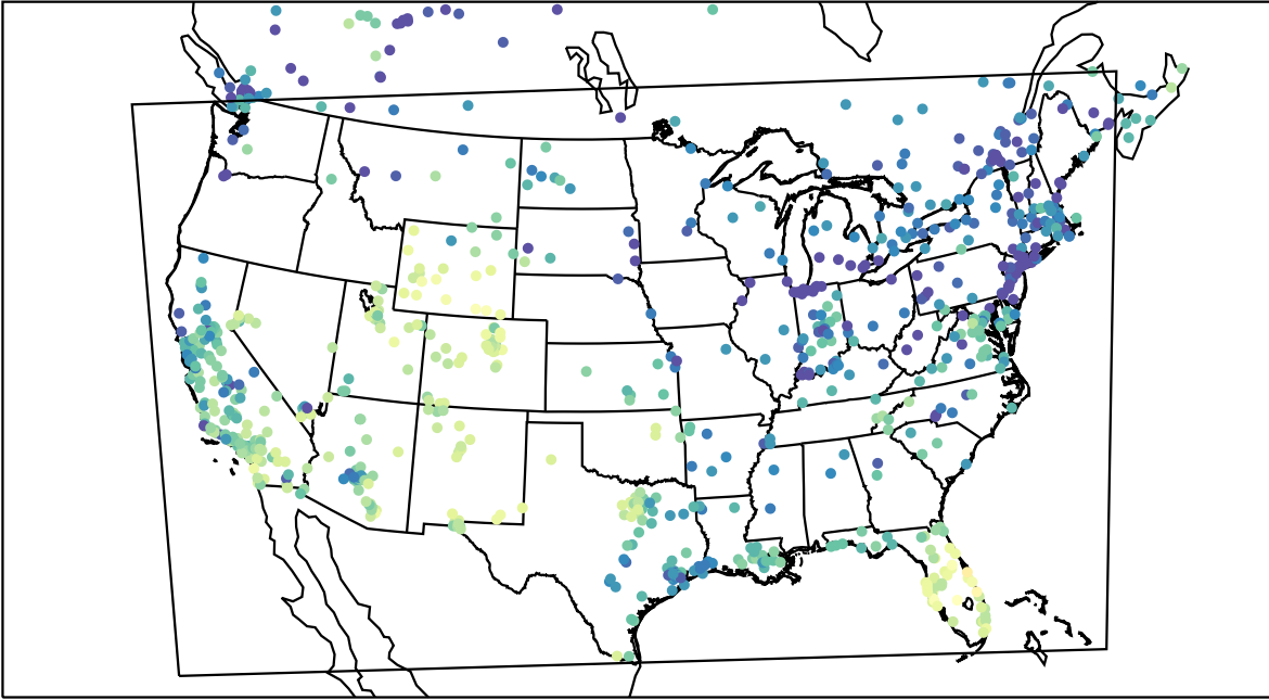
AirNOW (2021-12-28_18:00:00)
