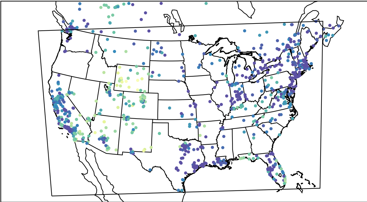
AirNOW (2021-12-29_03:00:00)
