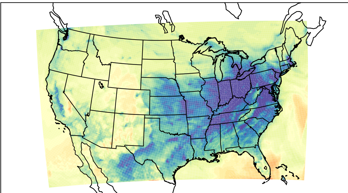
WRF (2021-12-28_03:00:00)
