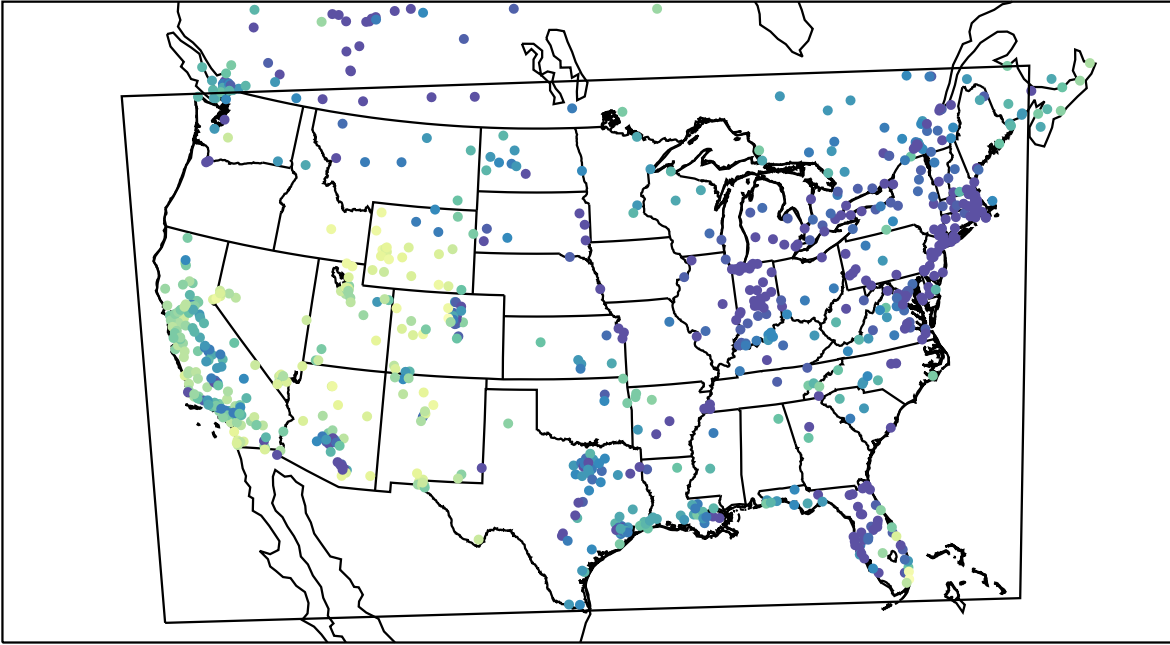
AirNOW (2021-12-28_00:00:00)
