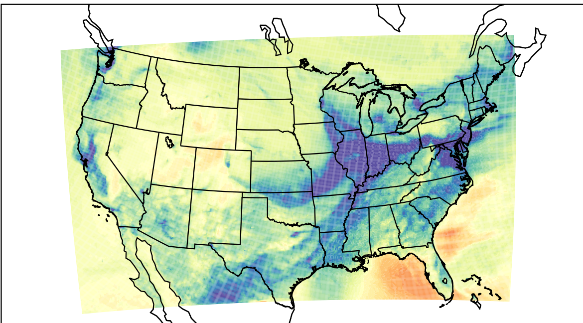
WRF (2021-12-29_04:00:00)
