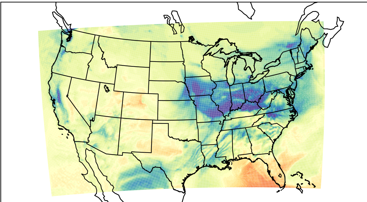
WRF (2021-12-28_18:00:00)
