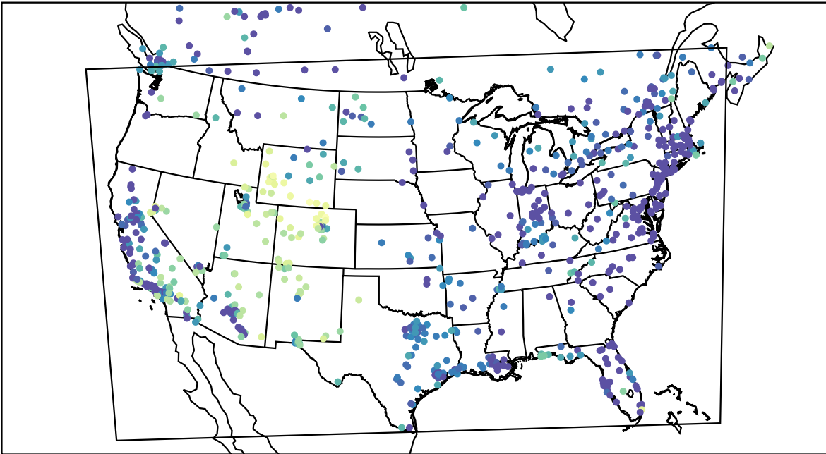
AirNOW (2021-12-28_11:00:00)
