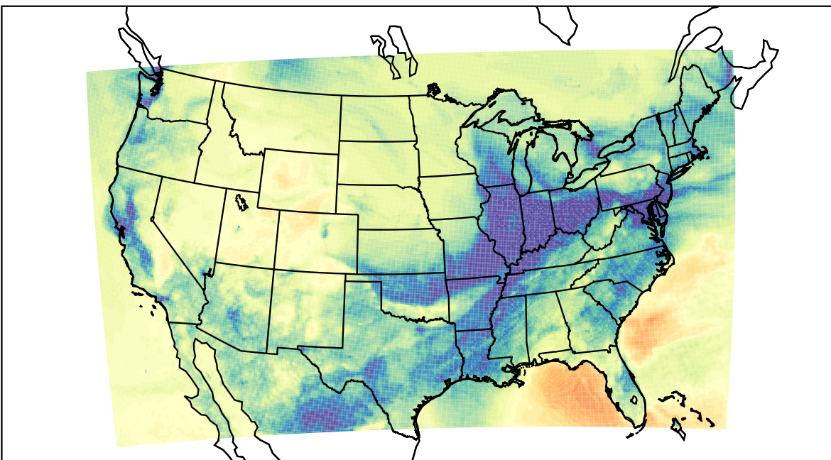
WRF (2021-12-29_07:00:00)
