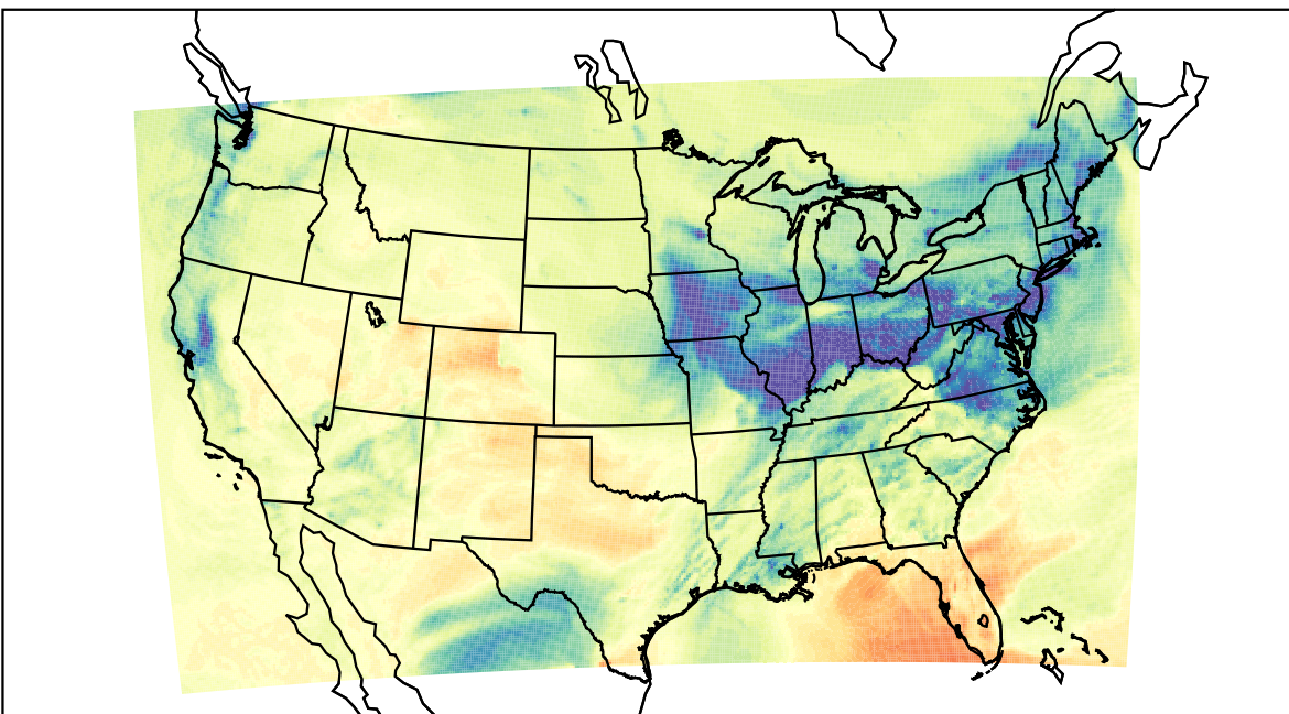
WRF (2021-12-28_21:00:00)
