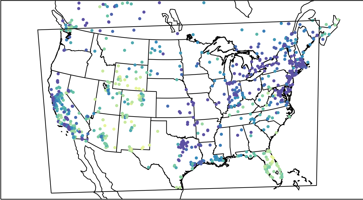
AirNOW (2021-12-29_17:00:00)
