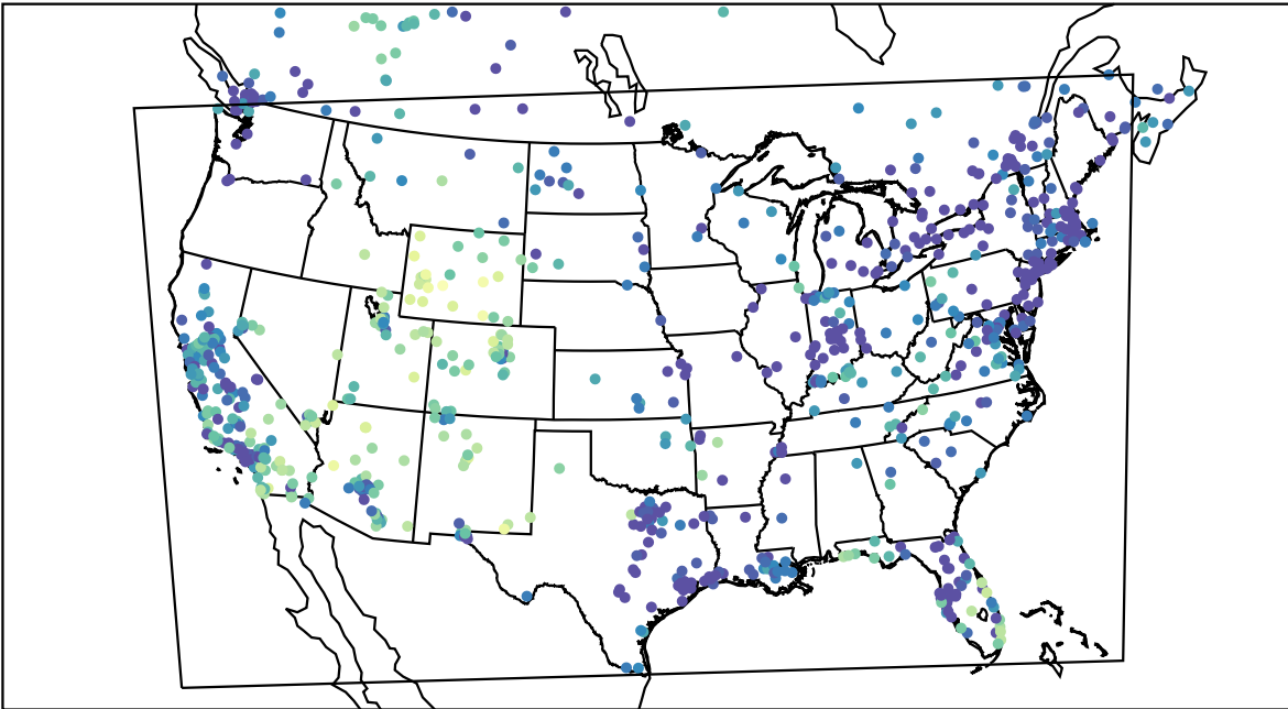
AirNOW (2021-12-29_02:00:00)
