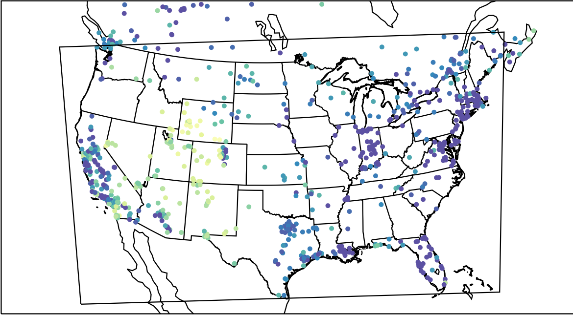
AirNOW (2021-12-28_07:00:00)
