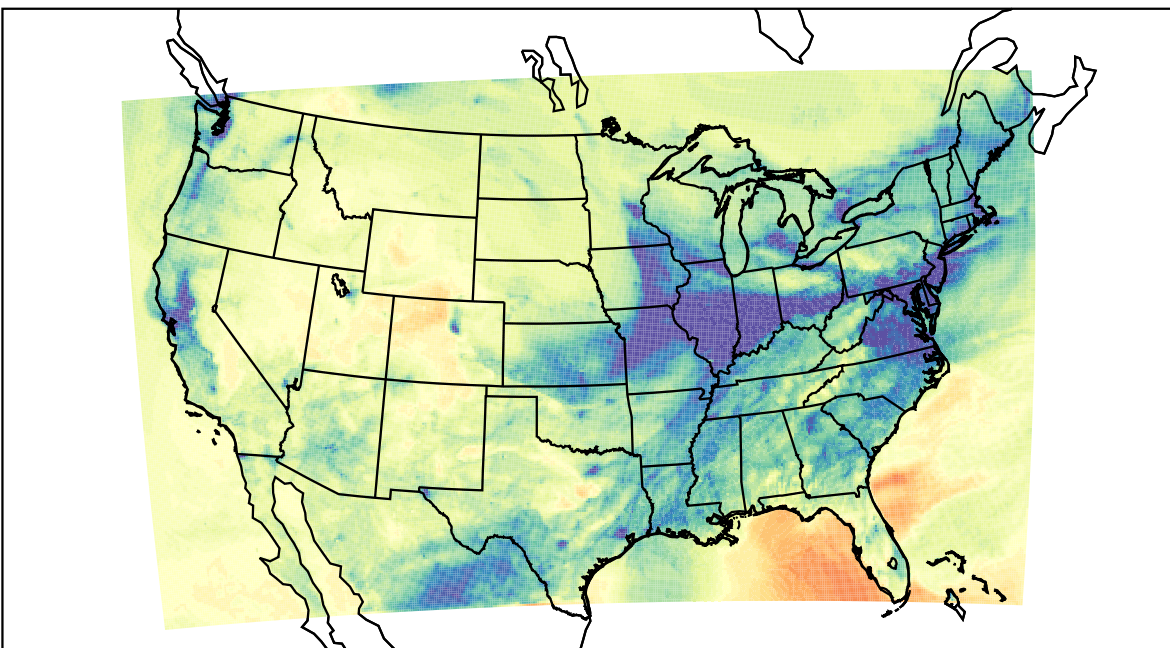
WRF (2021-12-29_01:00:00)
