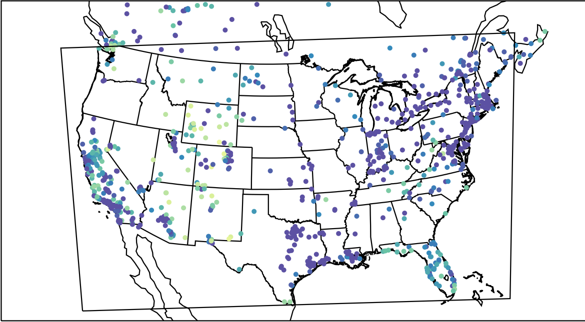
AirNOW (2021-12-29_14:00:00)
