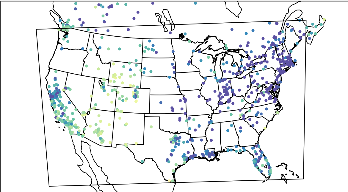
AirNOW (2021-12-29_23:00:00)
