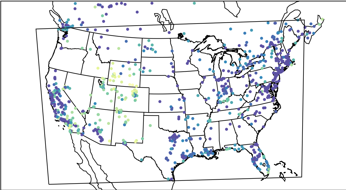
AirNOW (2021-12-28_14:00:00)
