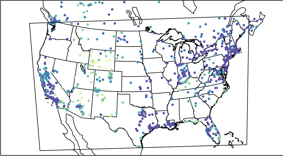
AirNOW (2021-12-29_06:00:00)
