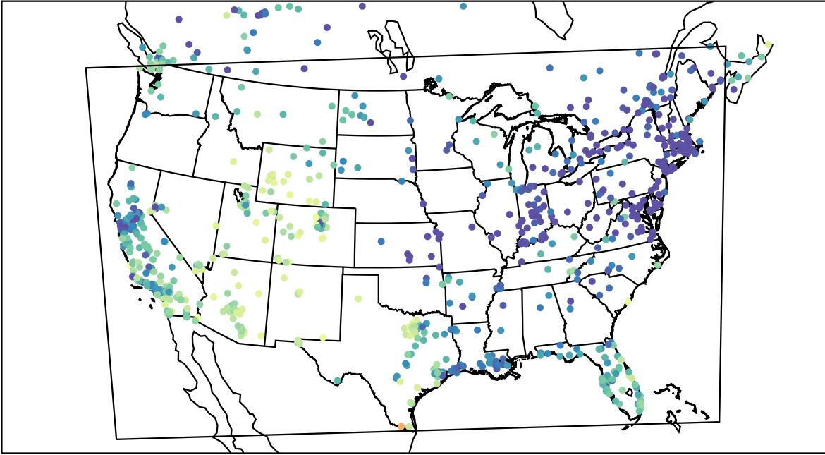
AirNOW (2021-12-29_22:00:00)
