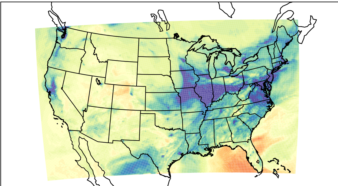
WRF (2021-12-29_00:00:00)
