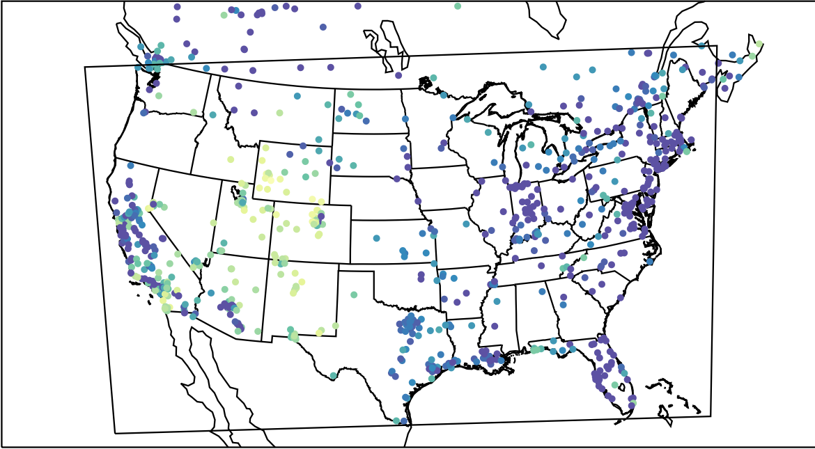
AirNOW (2021-12-28_09:00:00)
