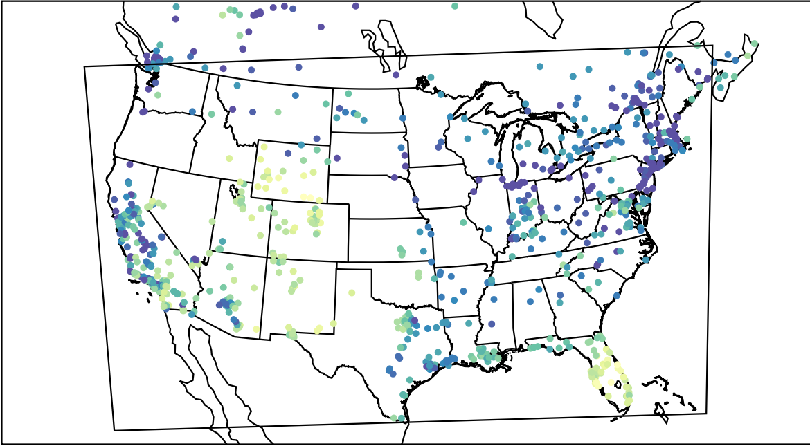
AirNOW (2021-12-28_17:00:00)
