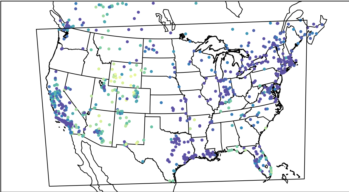
AirNOW (2021-12-29_07:00:00)
