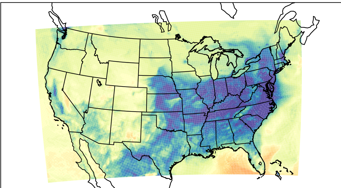
WRF (2021-12-28_11:00:00)
