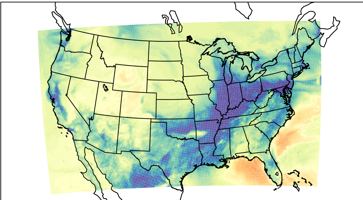
WRF (2021-12-29_10:00:00)
