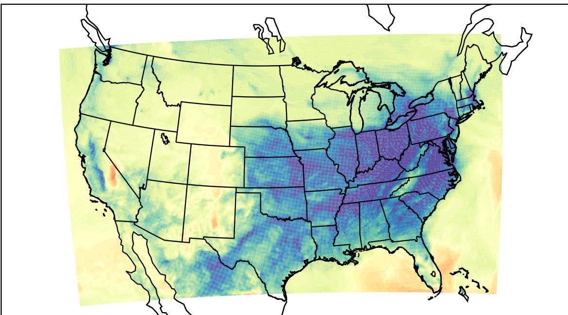
WRF (2021-12-28_06:00:00)
