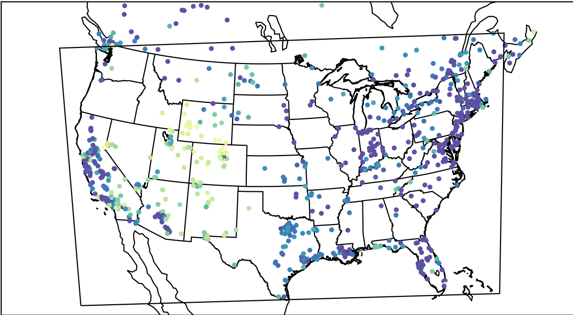
AirNOW (2021-12-28_10:00:00)
