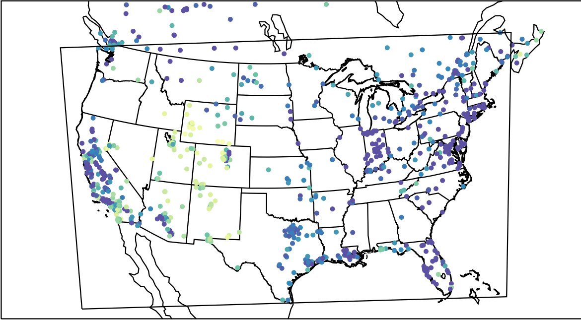
AirNOW (2021-12-28_08:00:00)
