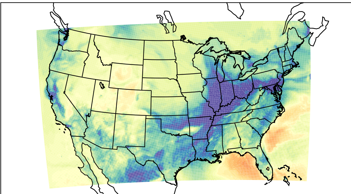
WRF (2021-12-29_09:00:00)
