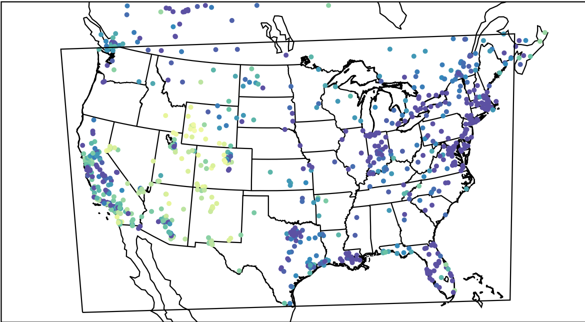
AirNOW (2021-12-28_05:00:00)
