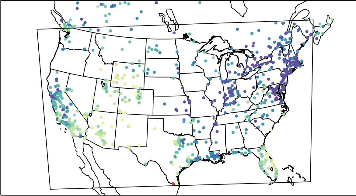
AirNOW (2021-12-29_20:00:00)
