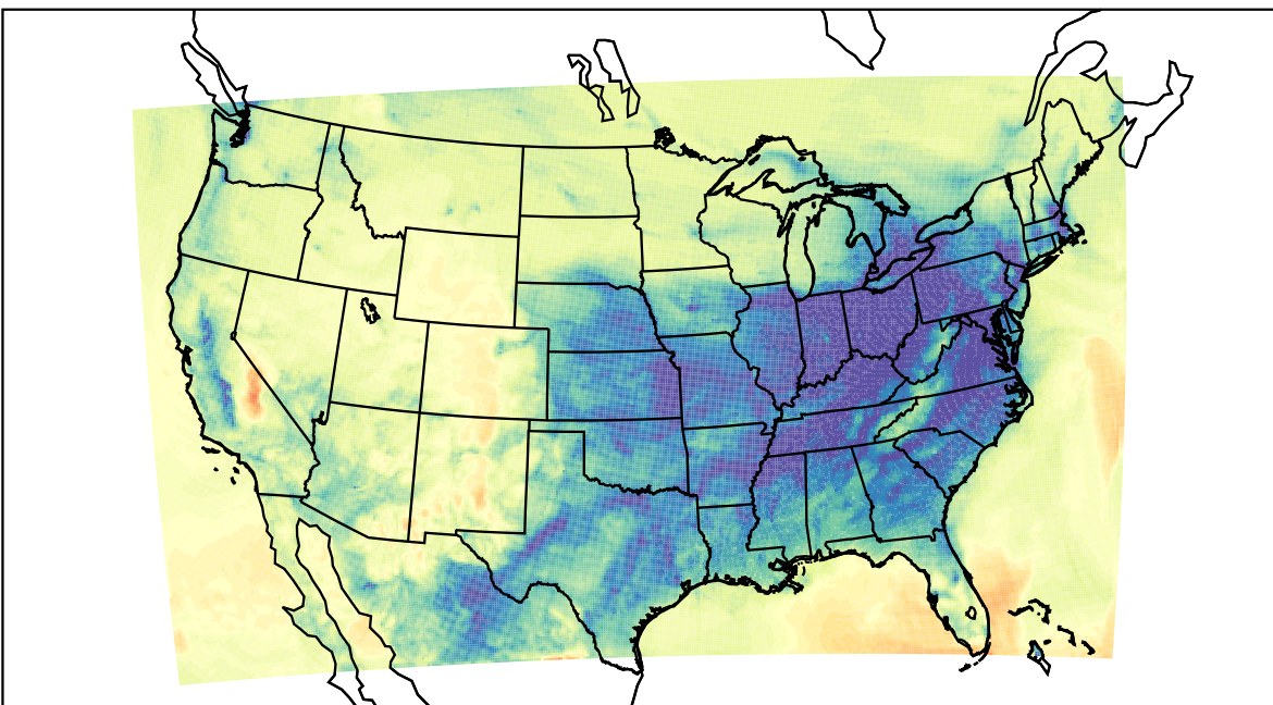
WRF (2021-12-28_05:00:00)
