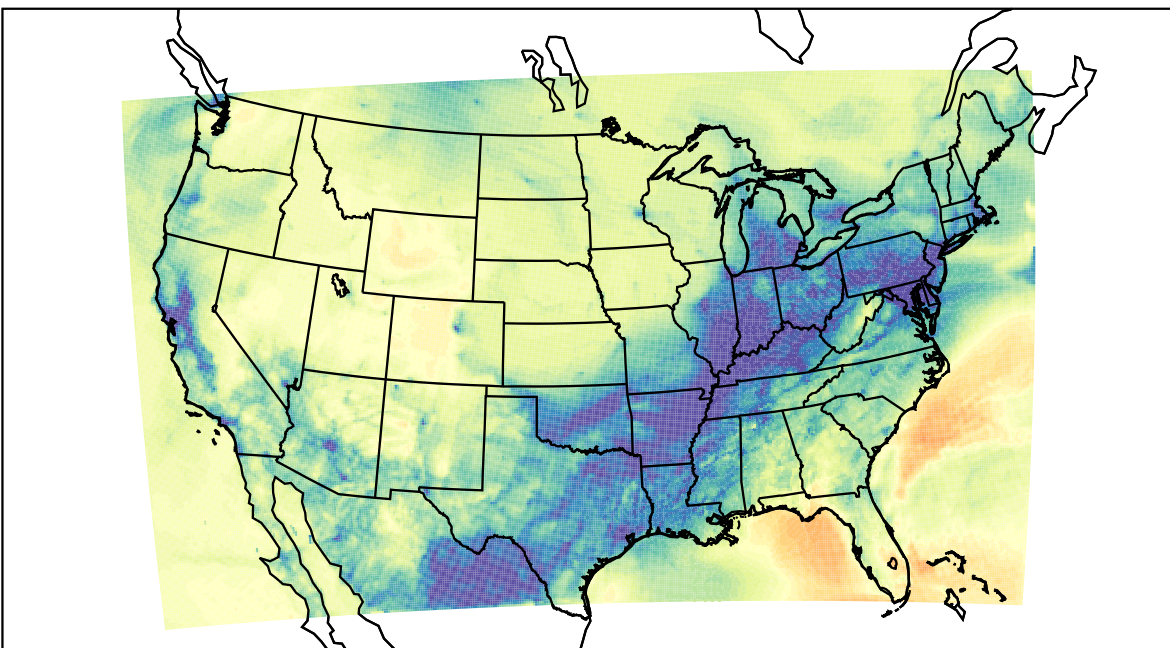
WRF (2021-12-29_15:00:00)
