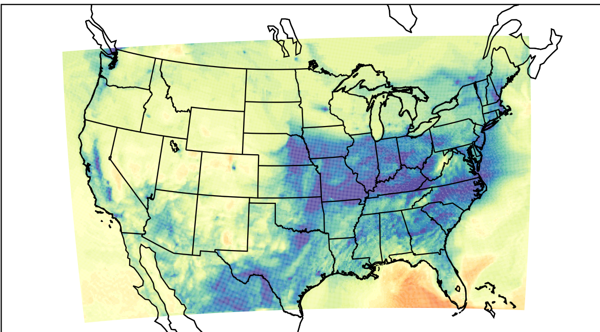
WRF (2021-12-28_15:00:00)
