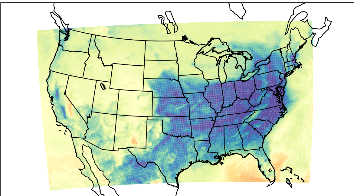
WRF (2021-12-28_09:00:00)
