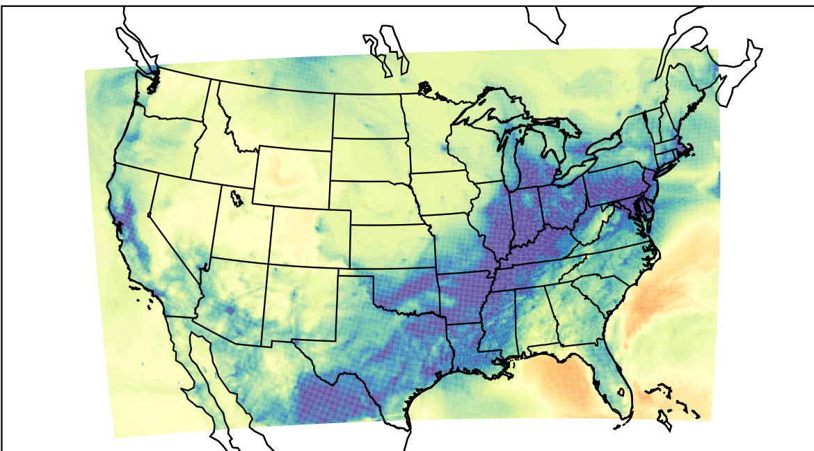
WRF (2021-12-29_14:00:00)
