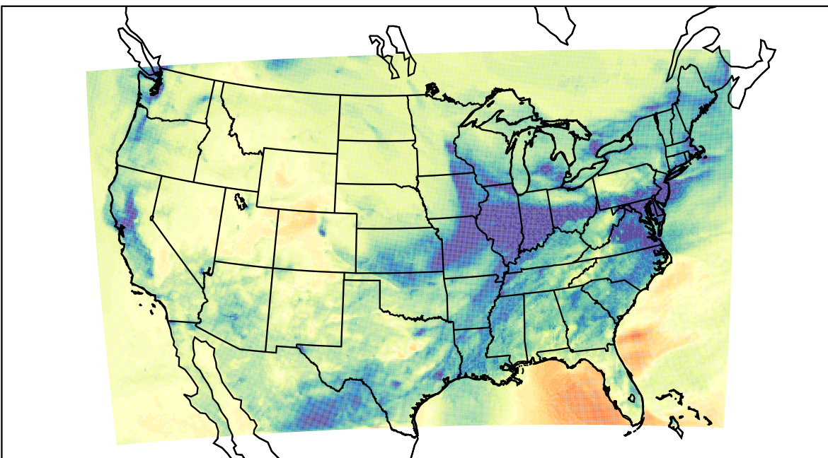
WRF (2021-12-29_02:00:00)
