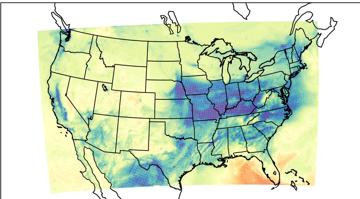
WRF (2021-12-28_16:00:00)
