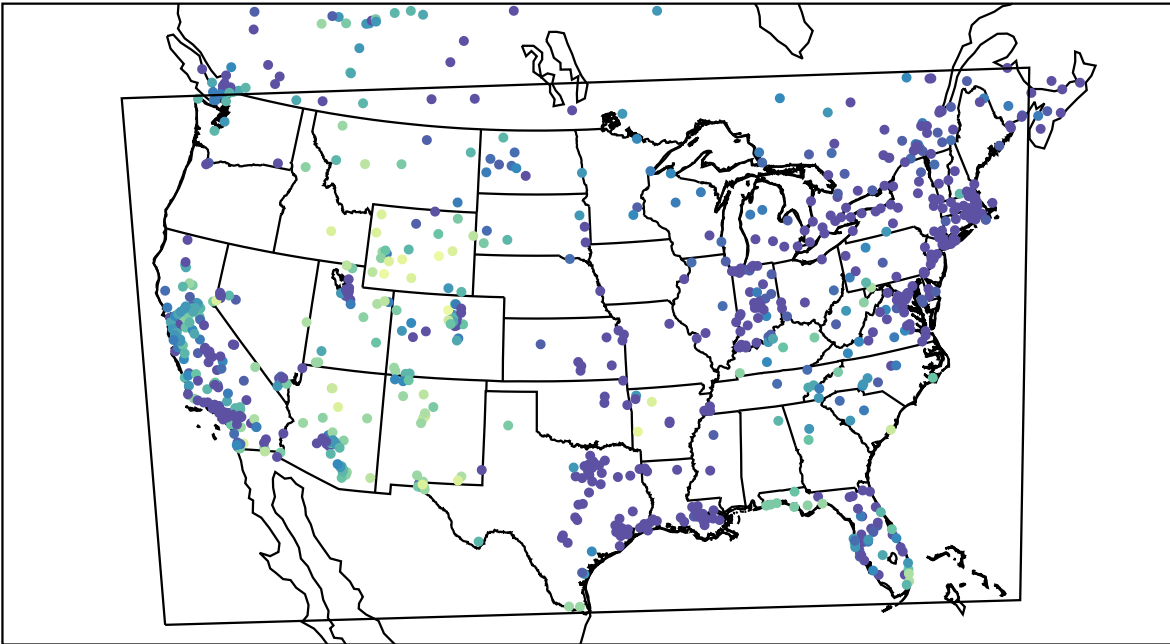
AirNOW (2021-12-29_09:00:00)
