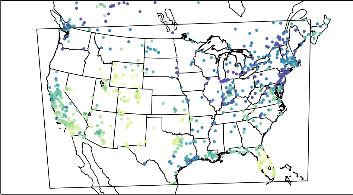
AirNOW (2021-12-28_19:00:00)
