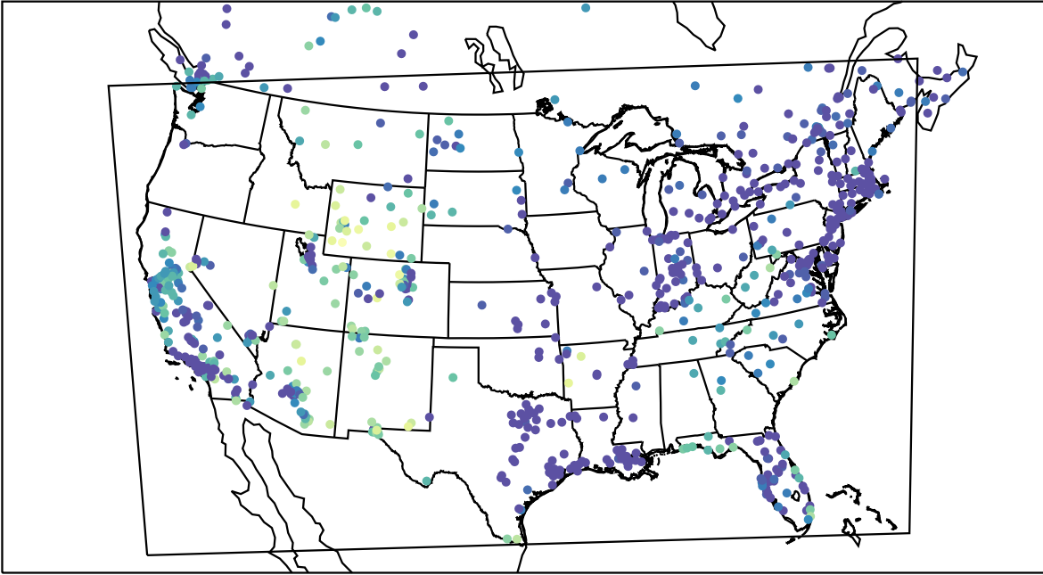
AirNOW (2021-12-29_10:00:00)
