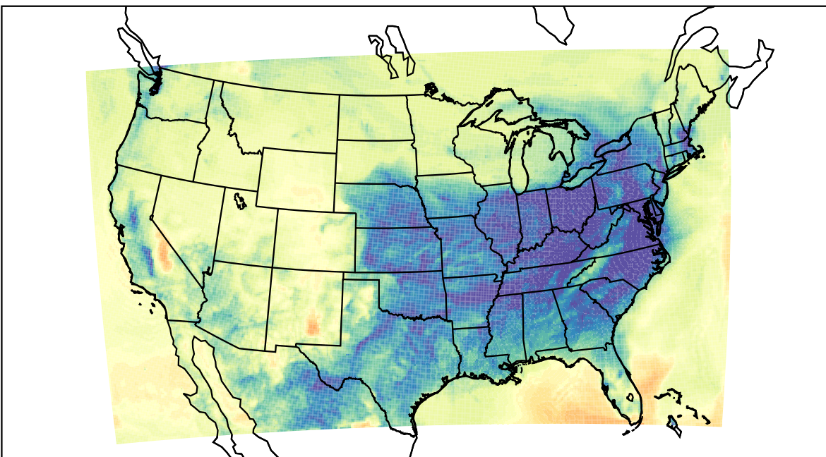
WRF (2021-12-28_08:00:00)
