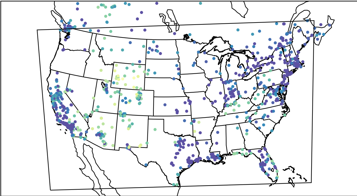
AirNOW (2021-12-29_05:00:00)
