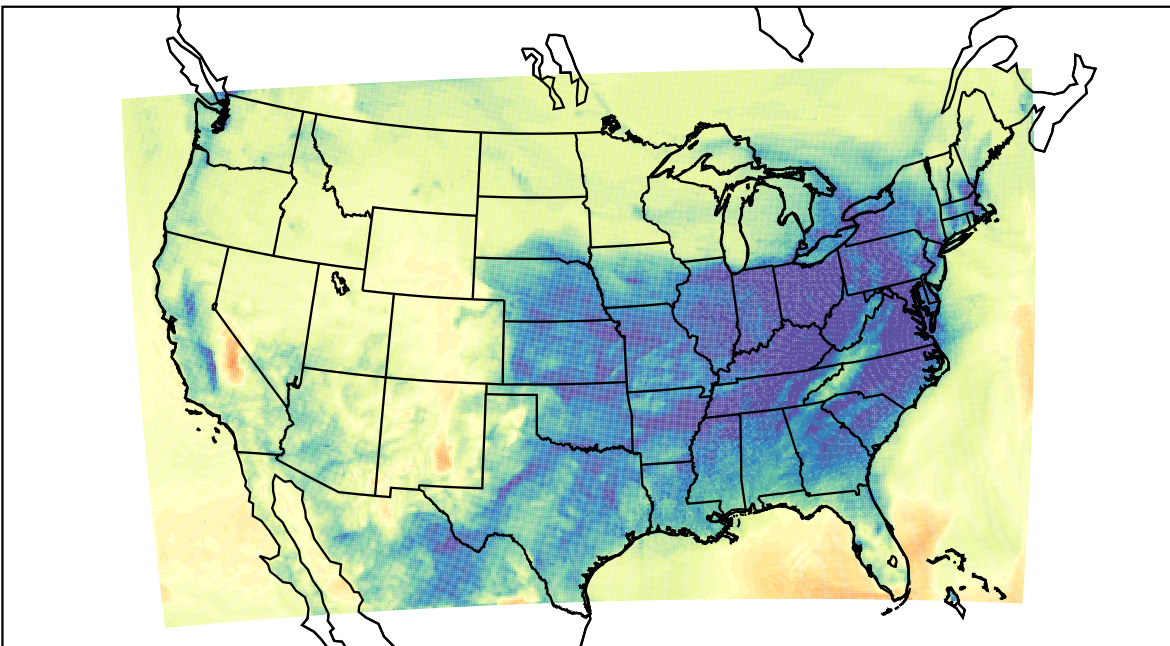
WRF (2021-12-28_07:00:00)
