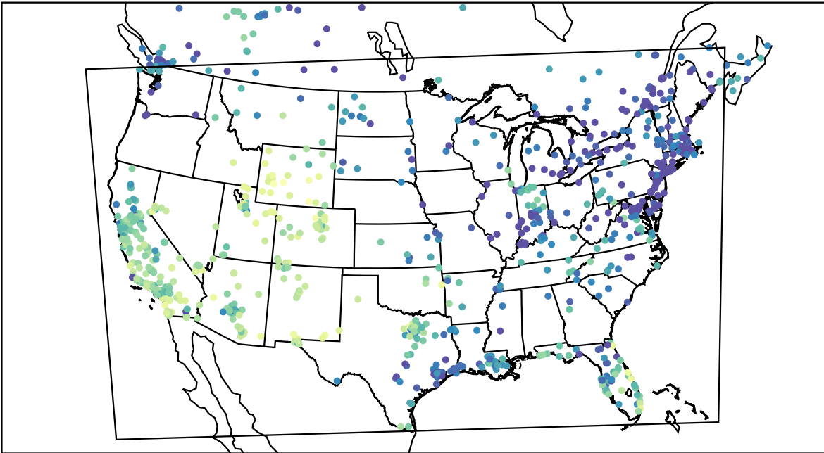
AirNOW (2021-12-28_23:00:00)
