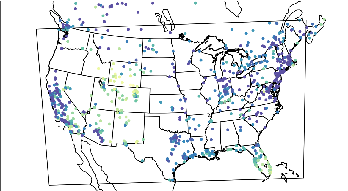
AirNOW (2021-12-28_15:00:00)
