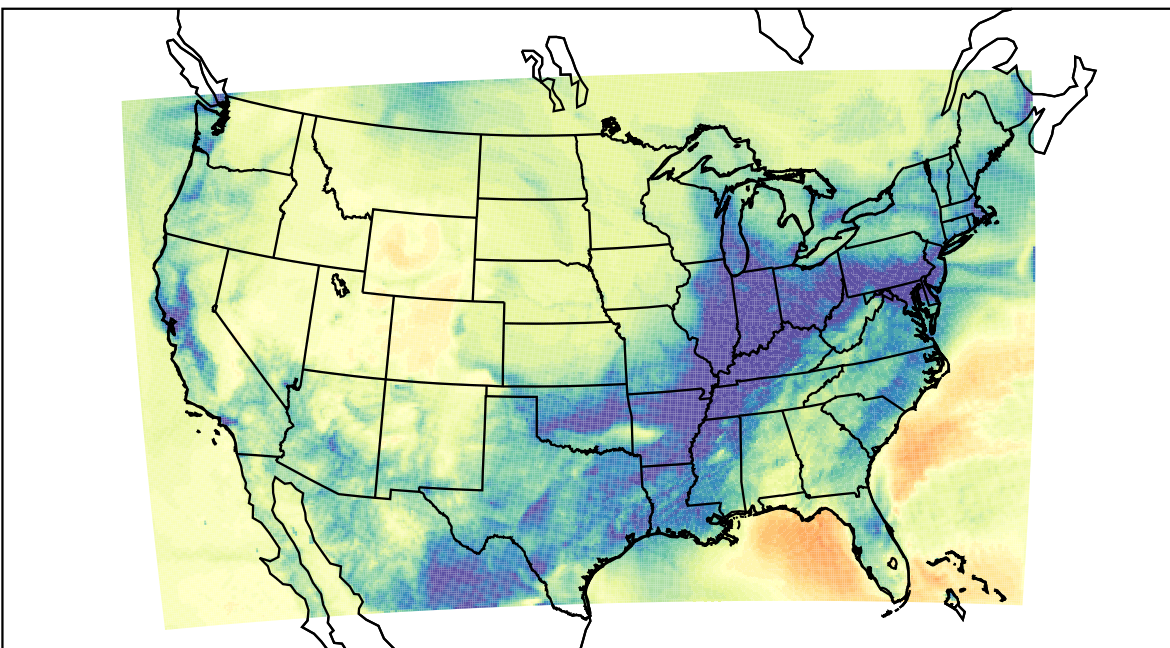
WRF (2021-12-29_11:00:00)
