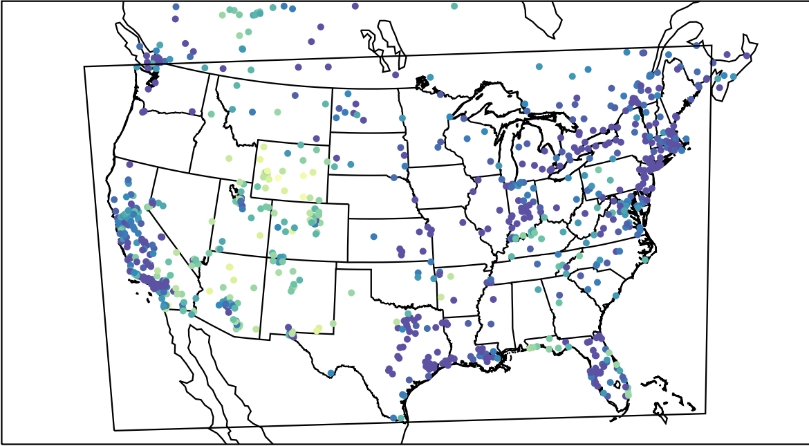
AirNOW (2021-12-29_04:00:00)
