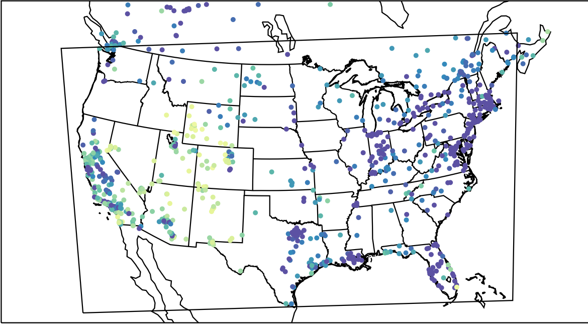
AirNOW (2021-12-28_04:00:00)
