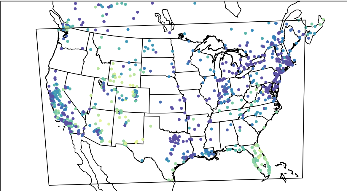
AirNOW (2021-12-29_16:00:00)
