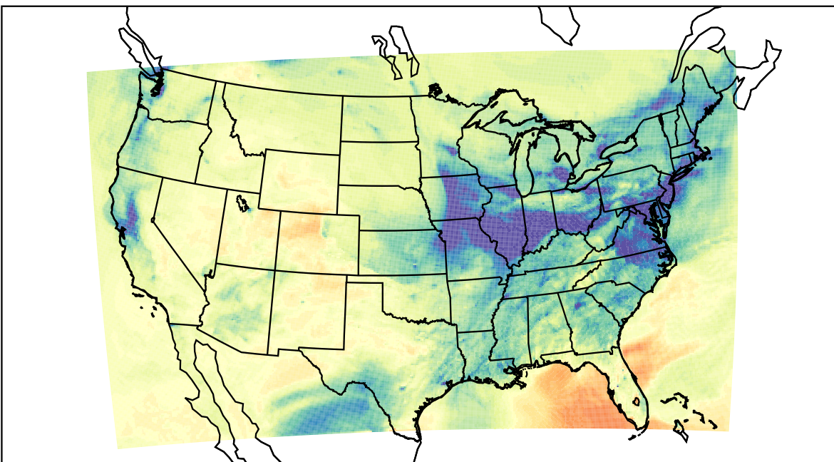
WRF (2021-12-28_23:00:00)
