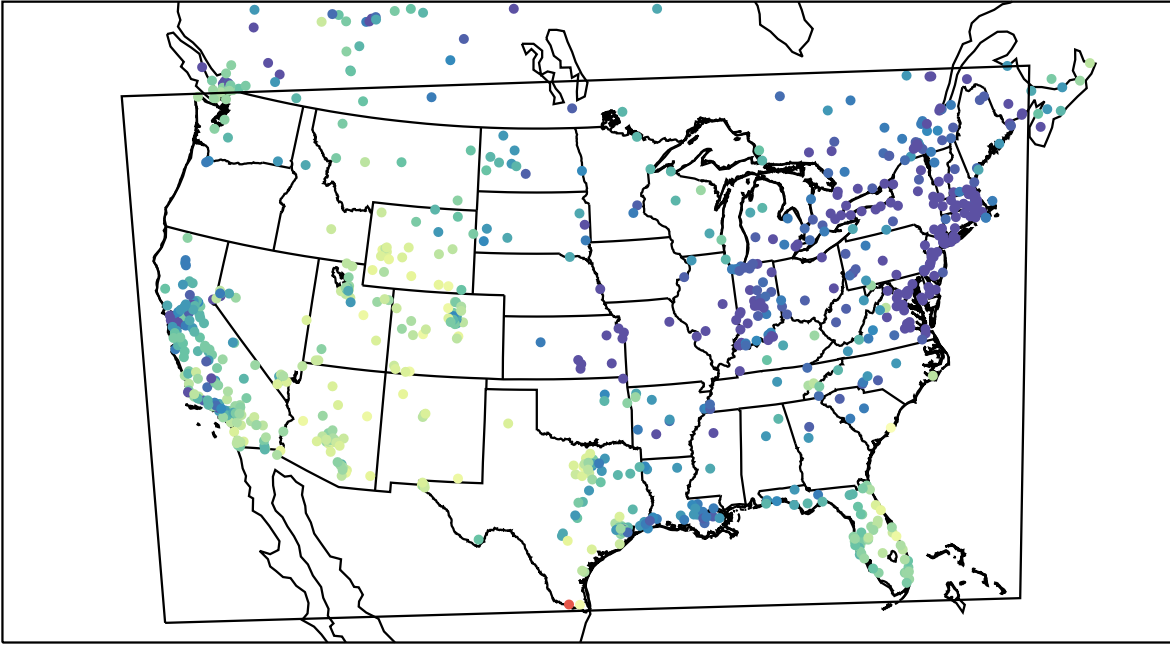
AirNOW (2021-12-29_21:00:00)
