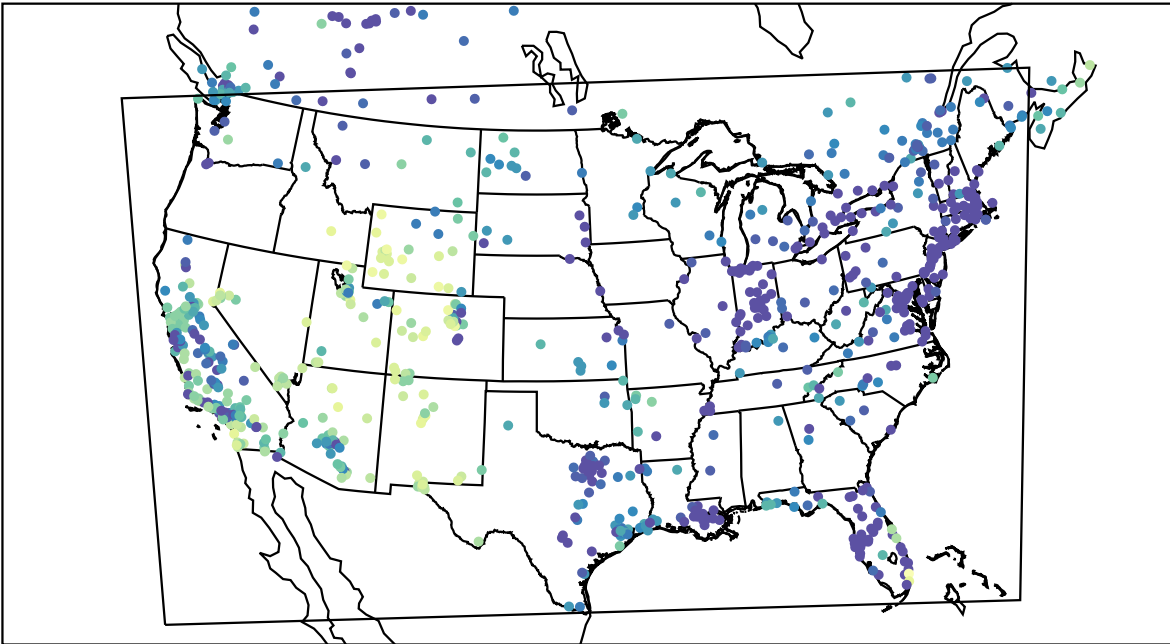
AirNOW (2021-12-28_03:00:00)
