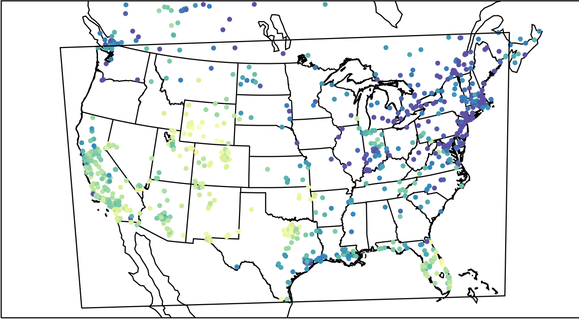
AirNOW (2021-12-28_22:00:00)
