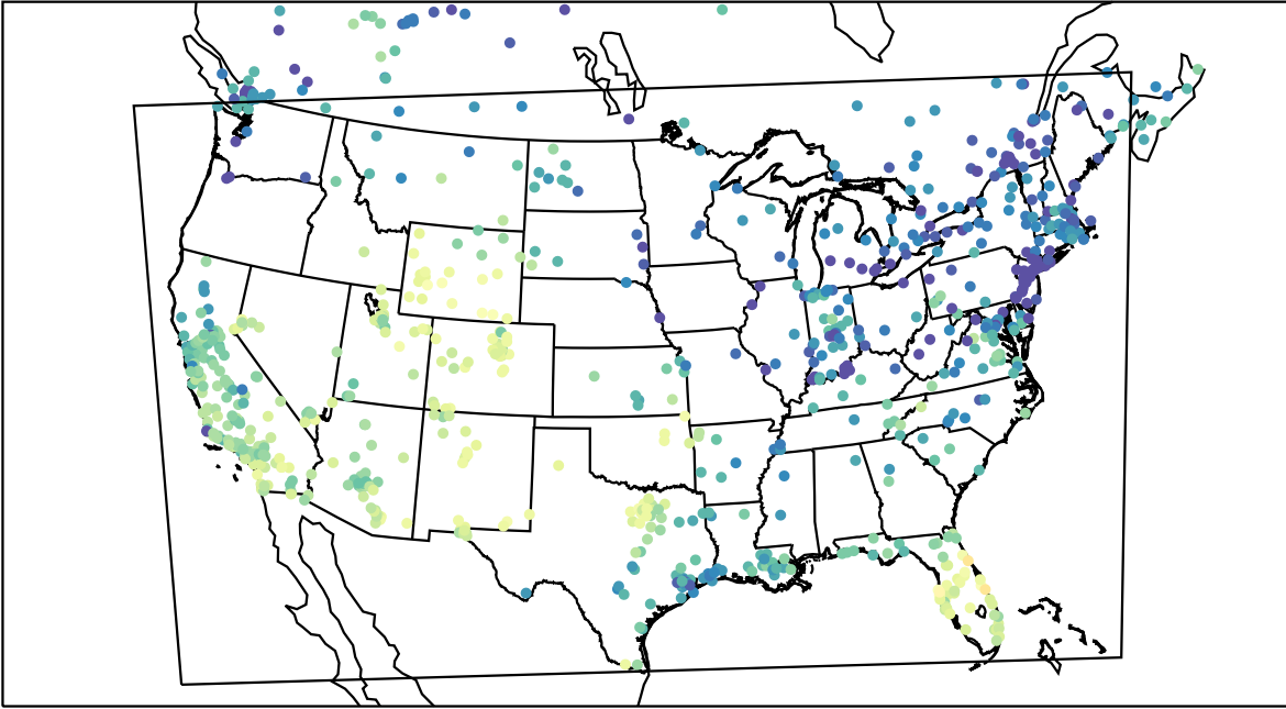
AirNOW (2021-12-28_20:00:00)
