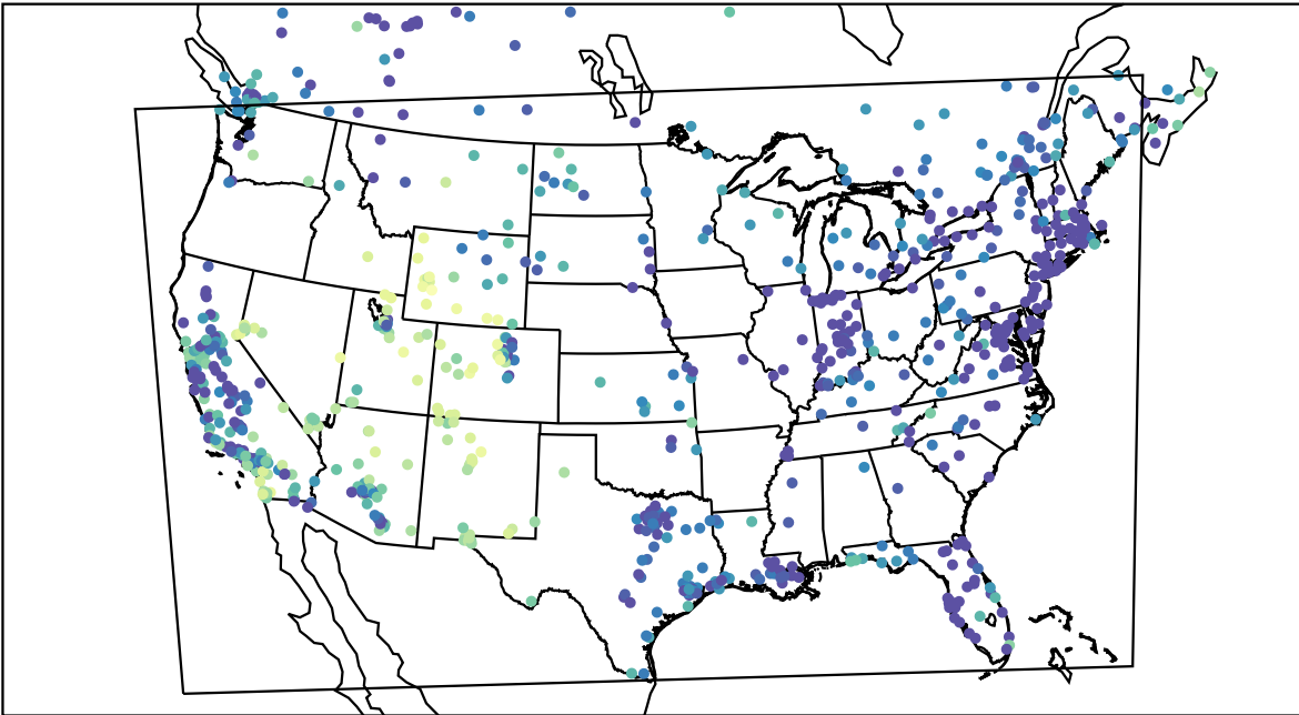
AirNOW (2021-12-28_06:00:00)
