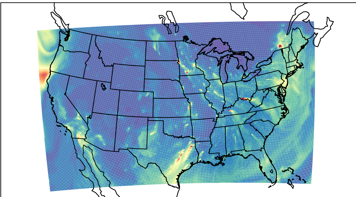
WRF 2022-01-07_14:00:00
