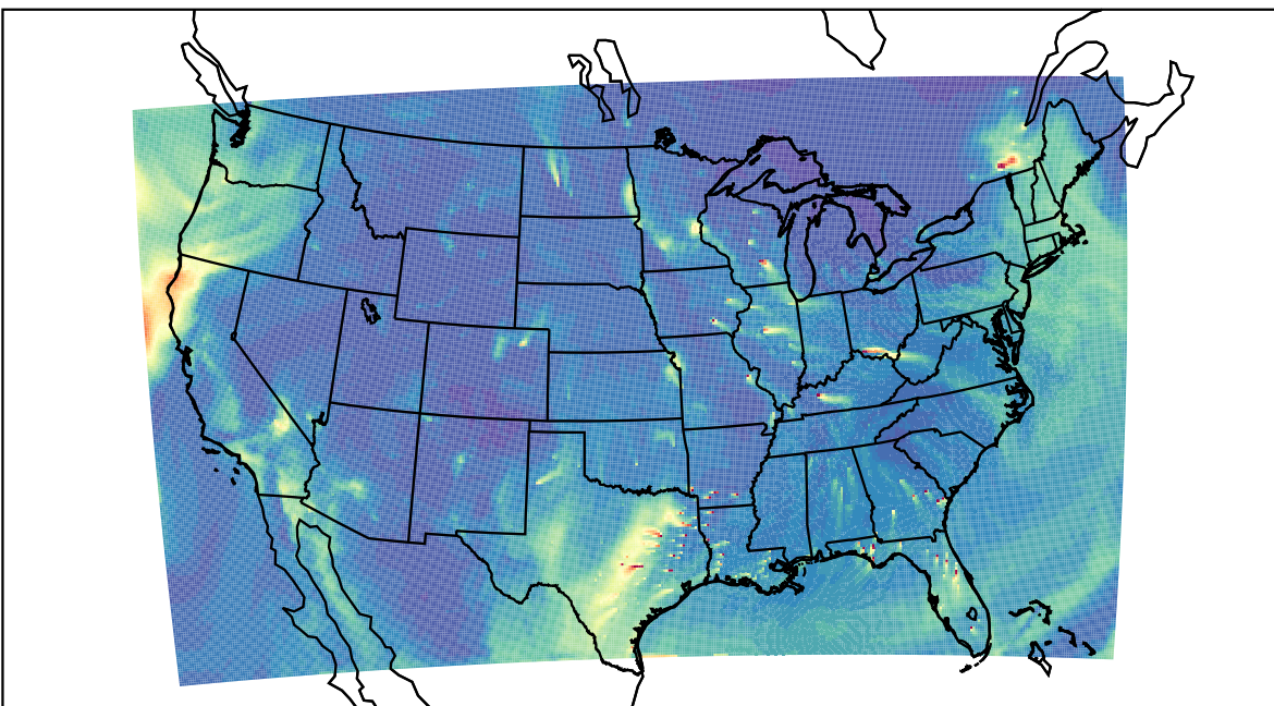
WRF 2022-01-07_19:00:00
