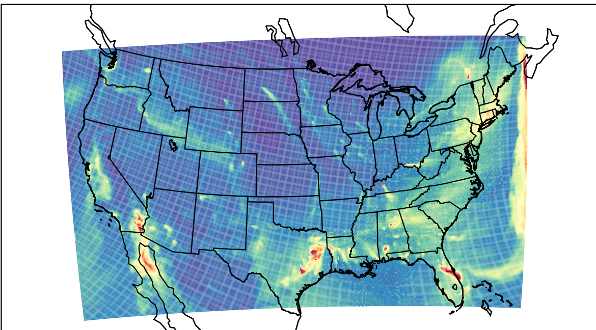
WRF 2022-01-06_07:00:00
