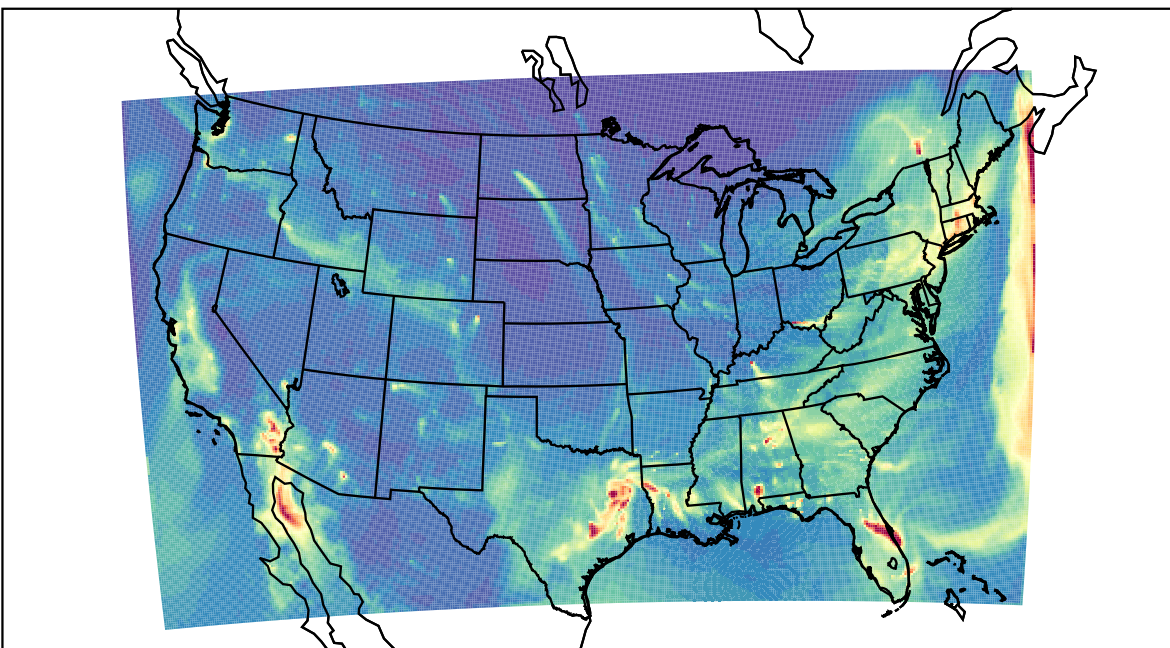
WRF 2022-01-06_06:00:00
