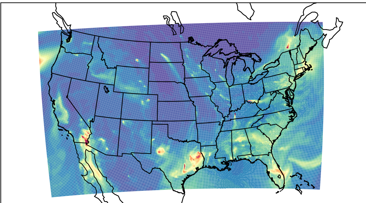
WRF 2022-01-06_12:00:00
