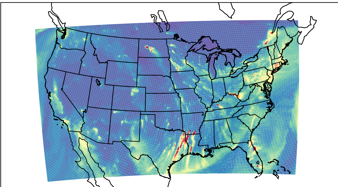
WRF 2022-01-07_03:00:00
