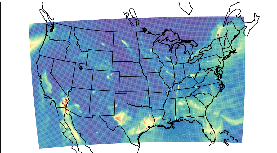
WRF 2022-01-06_15:00:00
