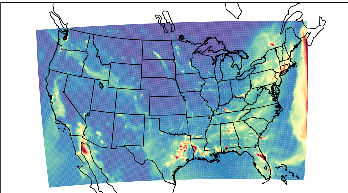
WRF 2022-01-06_04:00:00
