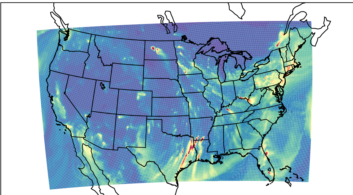
WRF 2022-01-07_04:00:00
