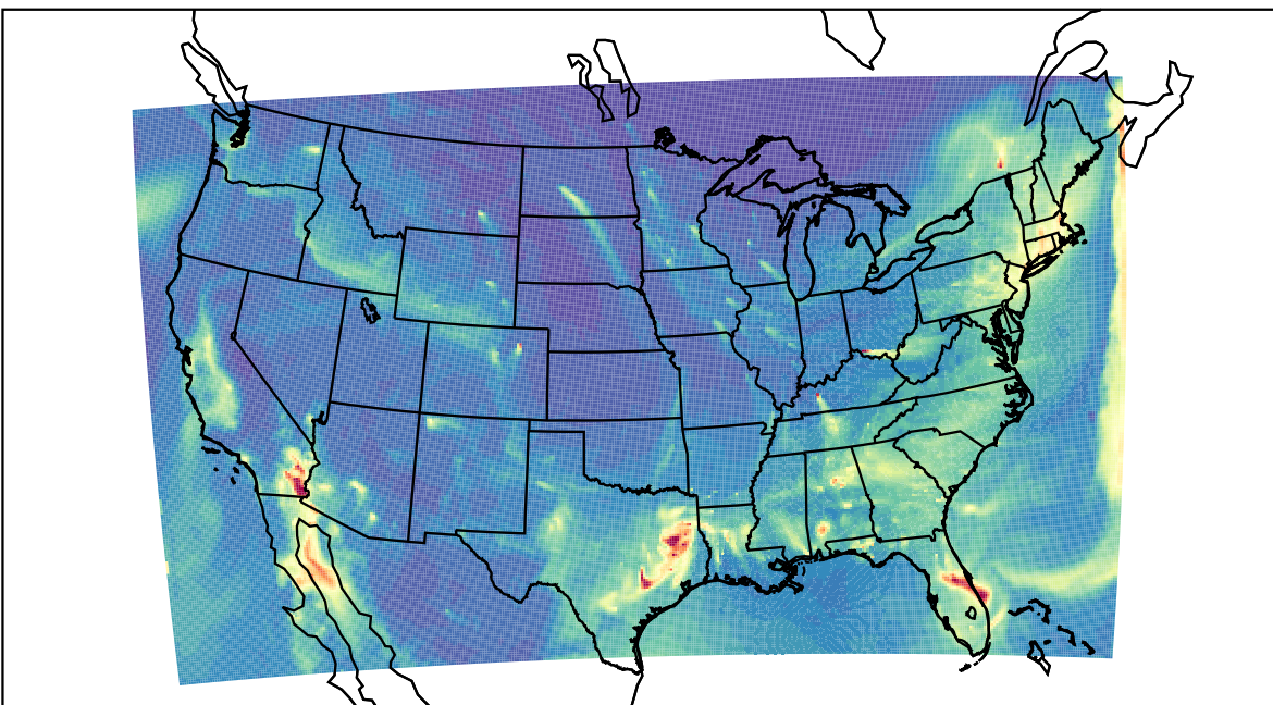
WRF 2022-01-06_08:00:00
