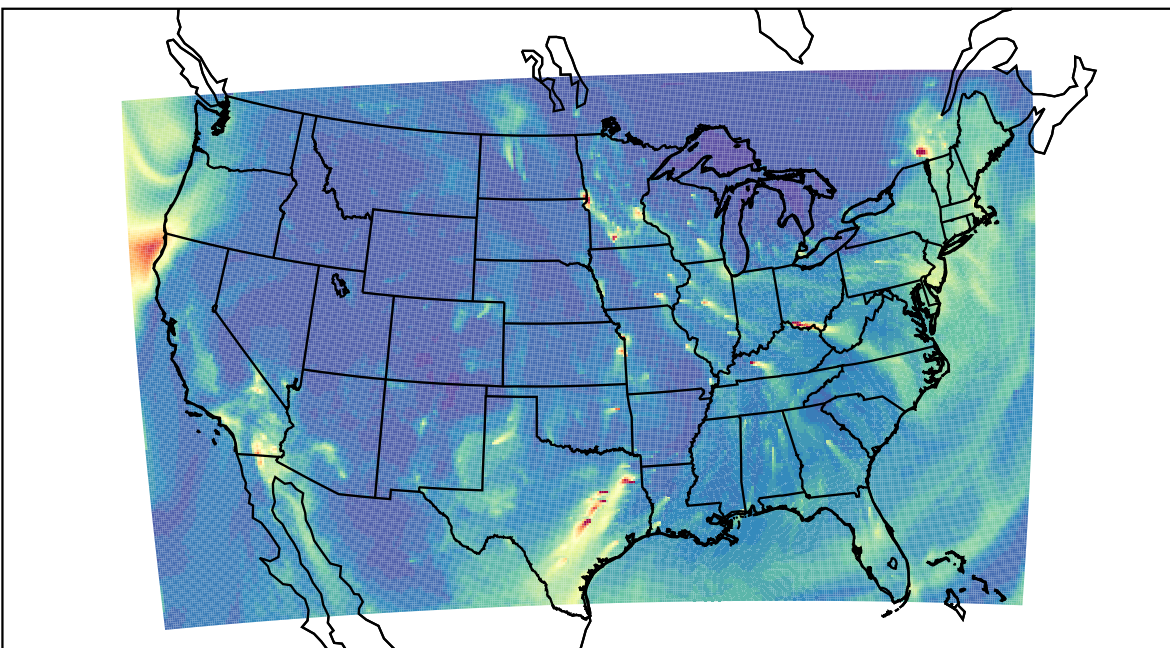
WRF 2022-01-07_15:00:00
