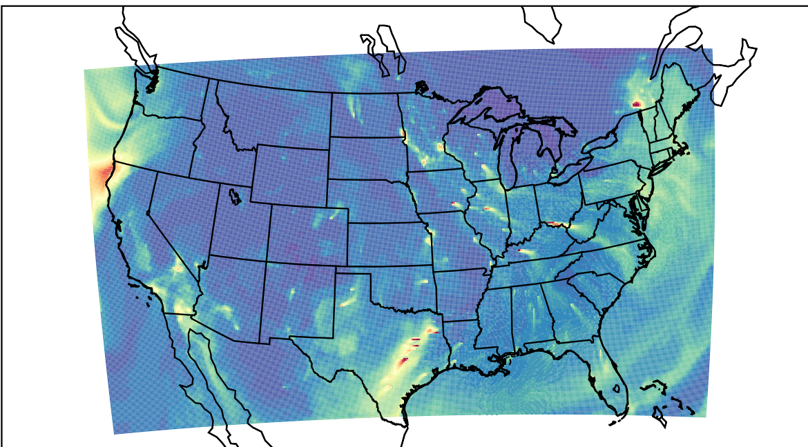
WRF 2022-01-07_16:00:00
