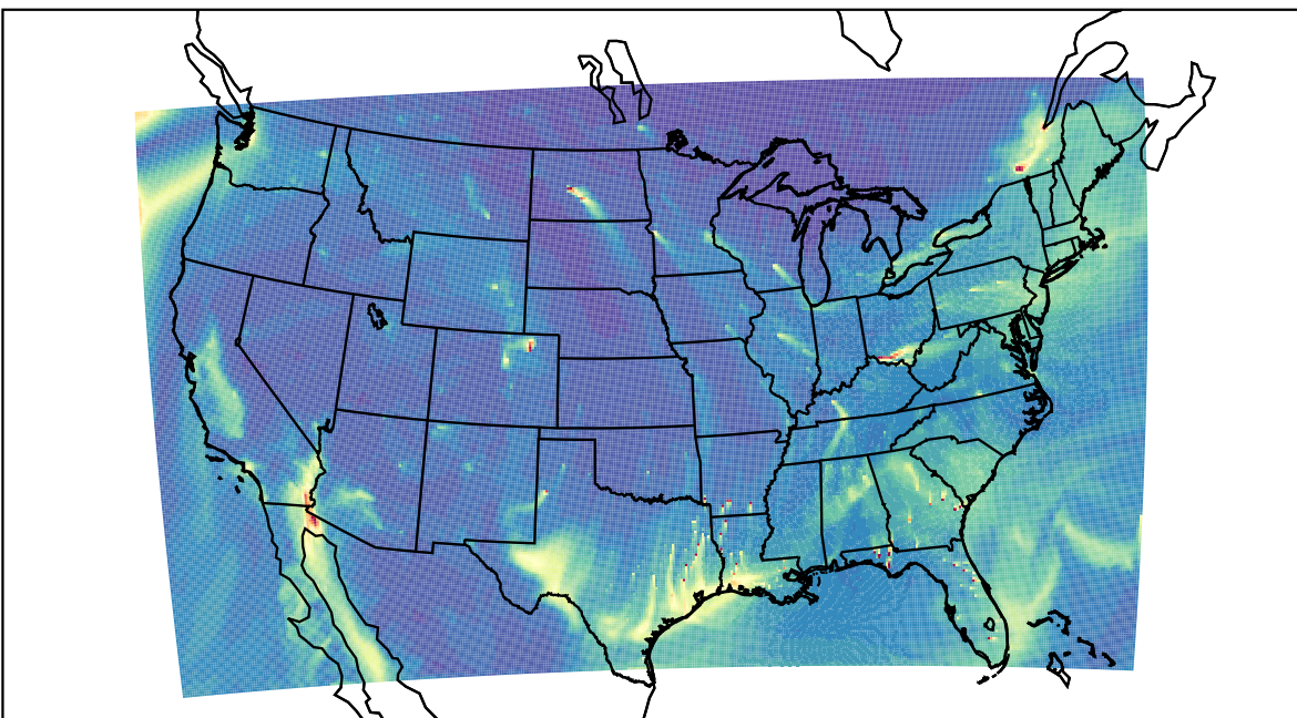
WRF 2022-01-06_19:00:00
