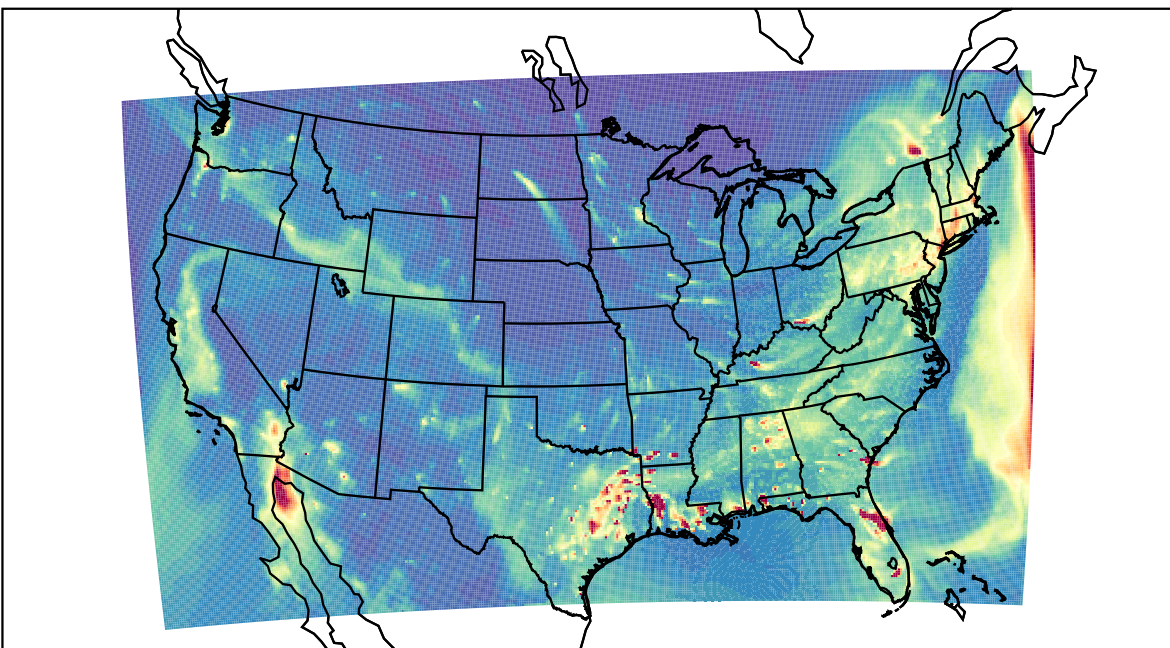
WRF 2022-01-06_02:00:00
