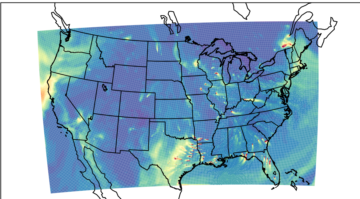
WRF 2022-01-07_22:00:00
