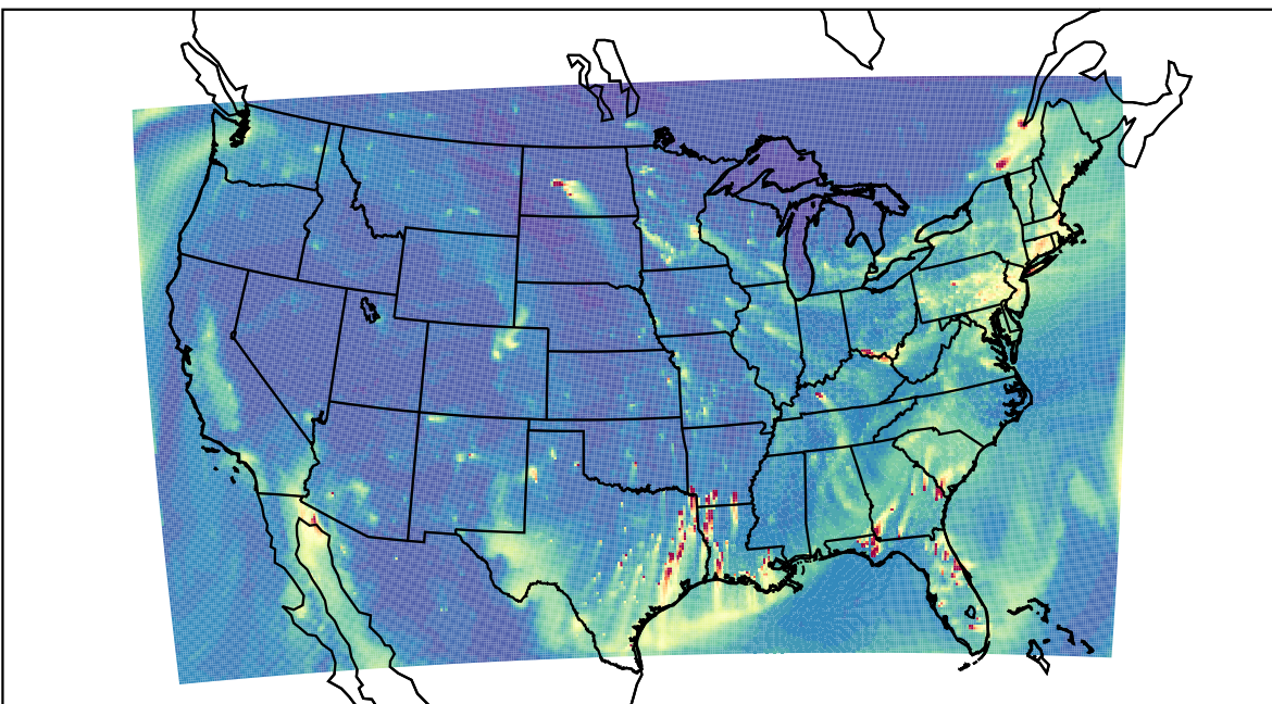
WRF 2022-01-07_00:00:00
