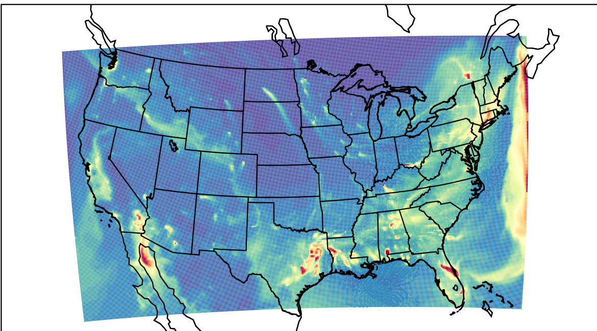
WRF 2022-01-06_05:00:00
