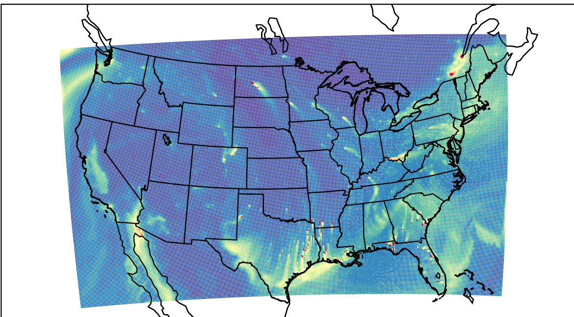
WRF 2022-01-06_21:00:00
