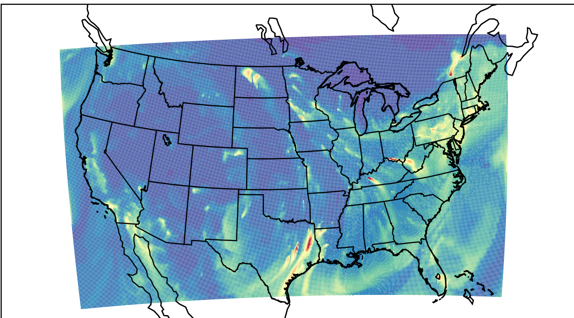
WRF 2022-01-07_07:00:00
