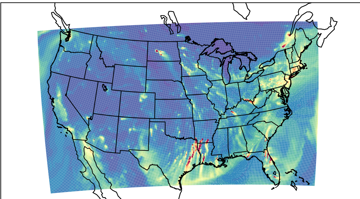
WRF 2022-01-07_02:00:00
