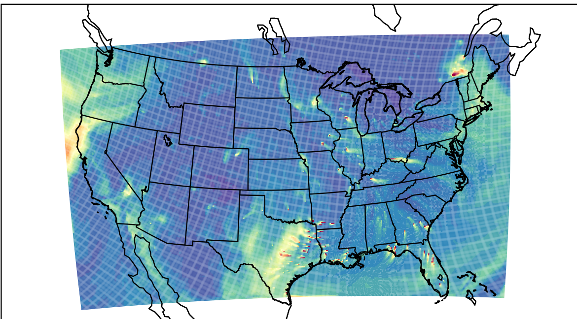
WRF 2022-01-07_21:00:00
