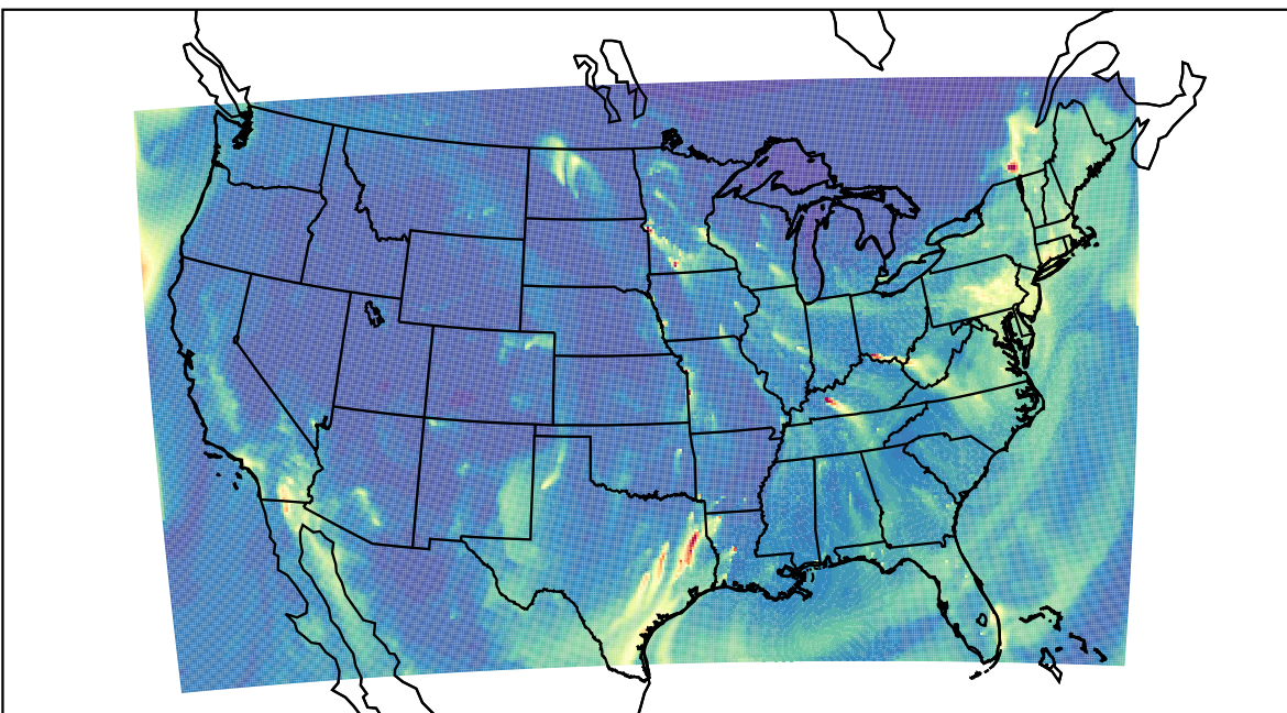
WRF 2022-01-07_10:00:00
