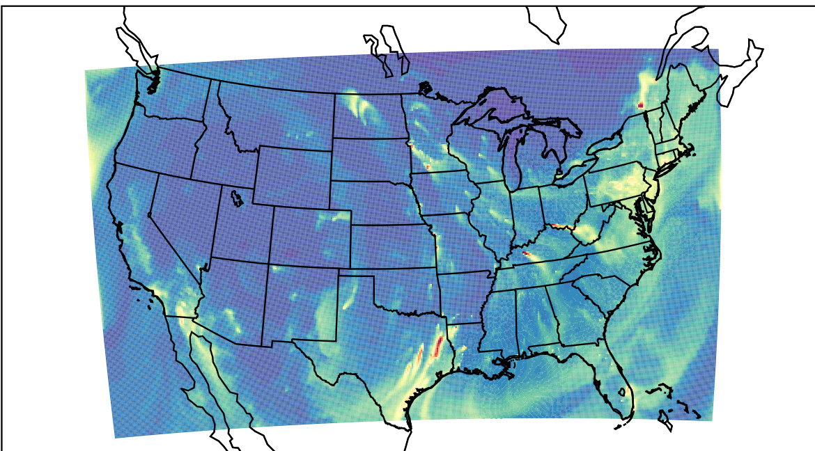
WRF 2022-01-07_09:00:00
