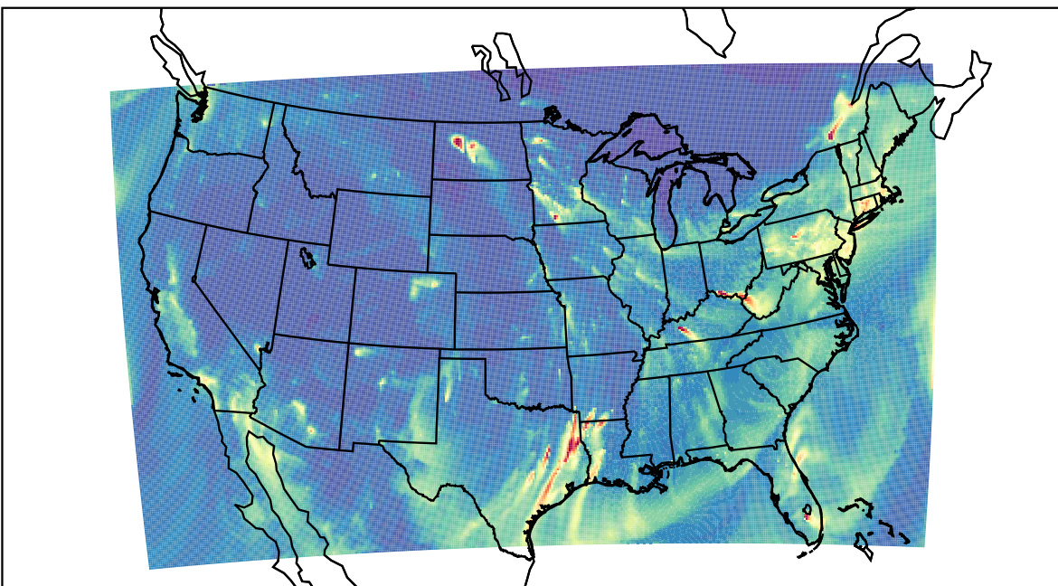
WRF 2022-01-07_05:00:00
