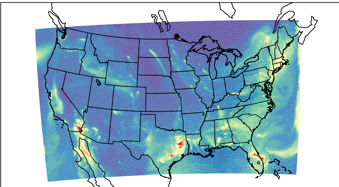
WRF 2022-01-06_09:00:00
