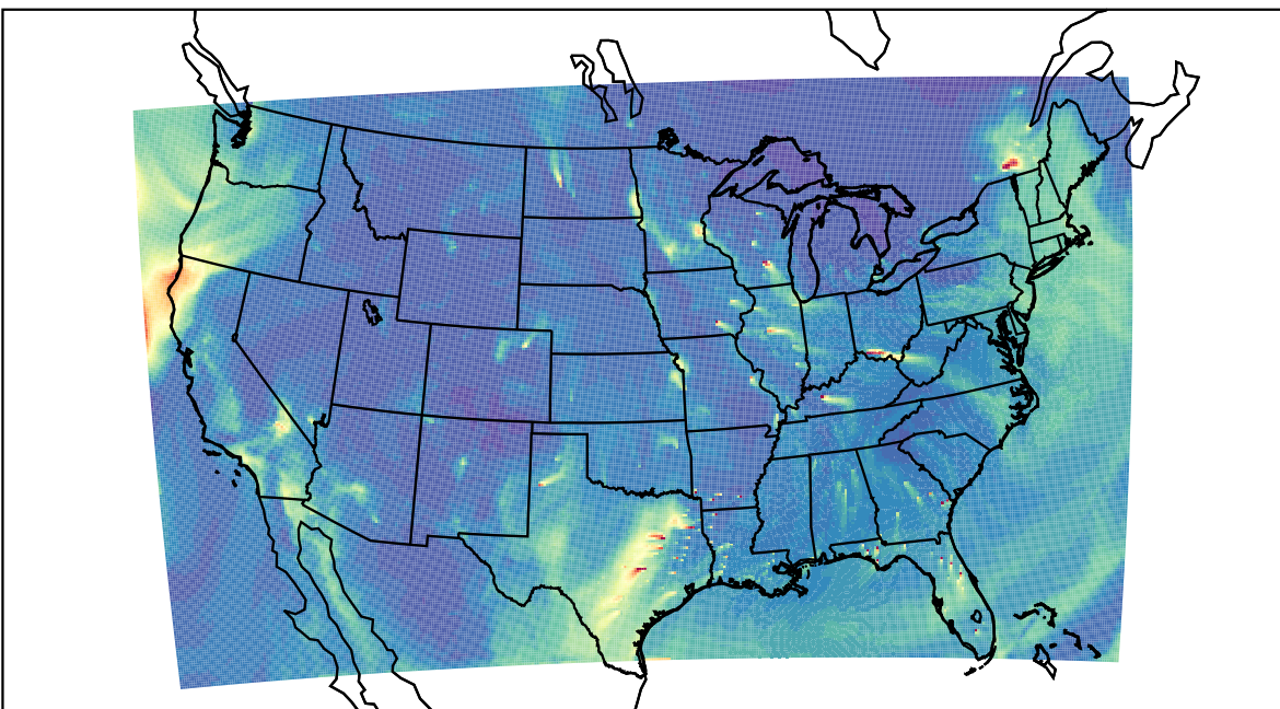
WRF 2022-01-07_18:00:00
