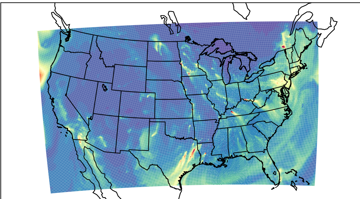
WRF 2022-01-07_11:00:00
