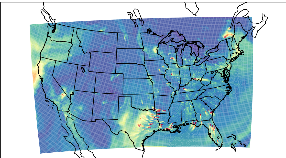
WRF 2022-01-07_23:00:00
