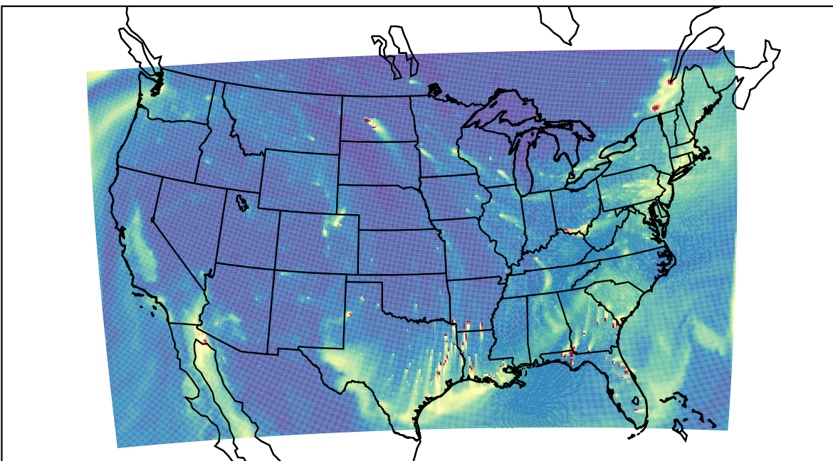
WRF 2022-01-06_22:00:00
