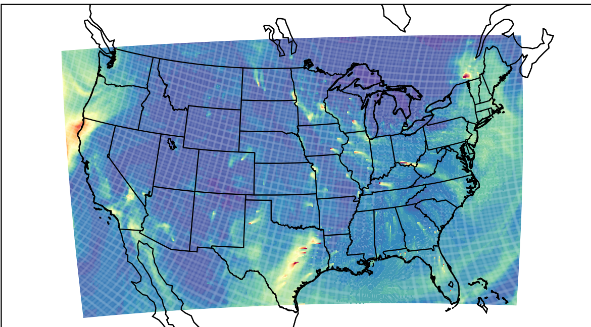
WRF 2022-01-07_17:00:00
