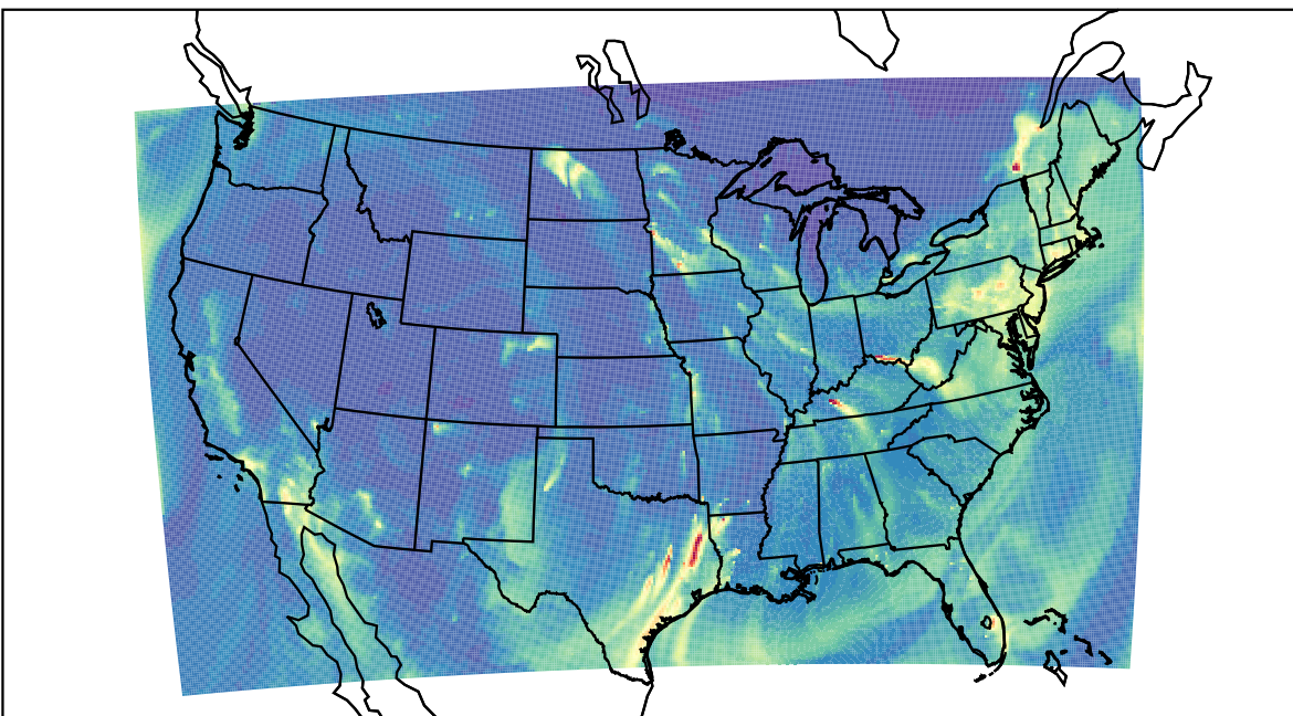
WRF 2022-01-07_08:00:00
