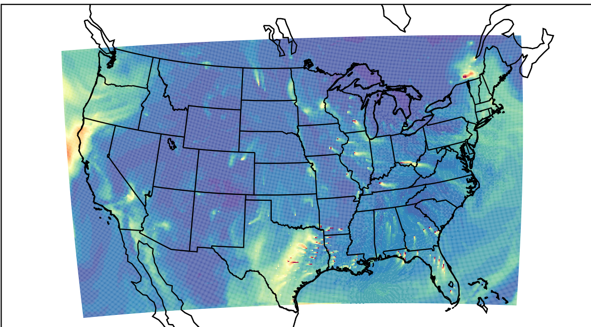
WRF 2022-01-07_20:00:00
