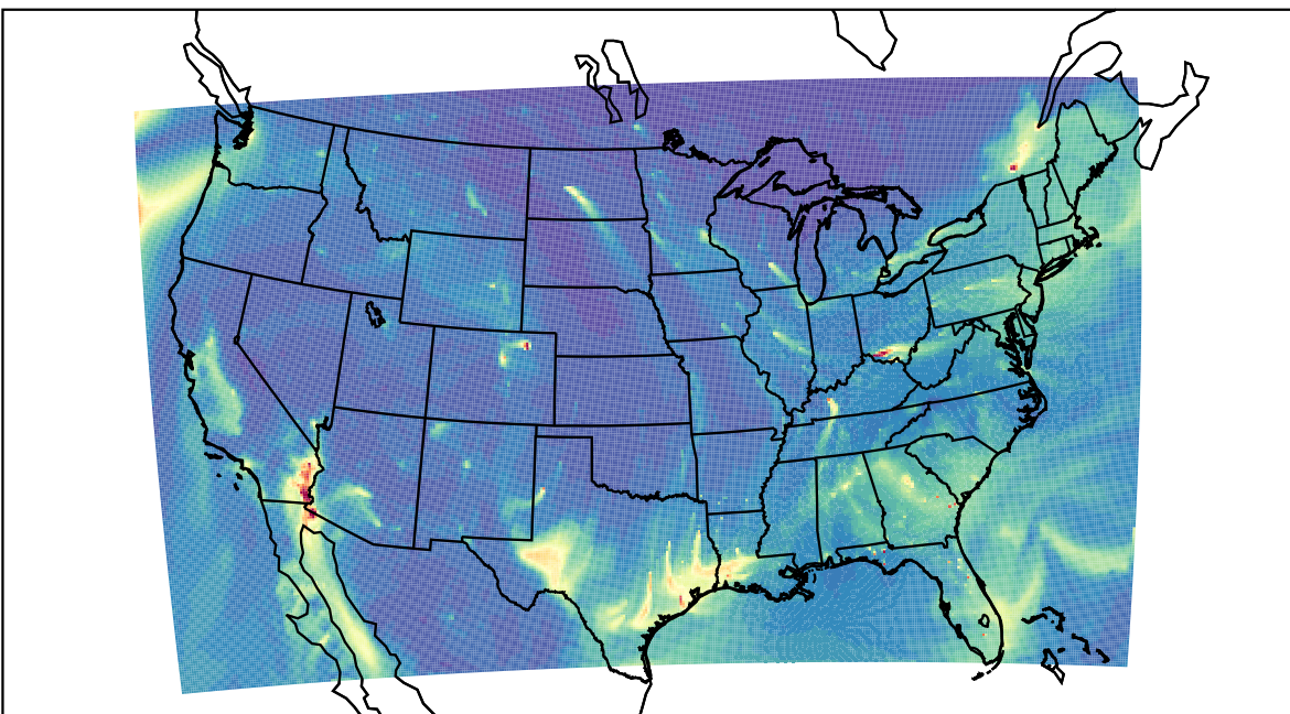
WRF 2022-01-06_17:00:00
