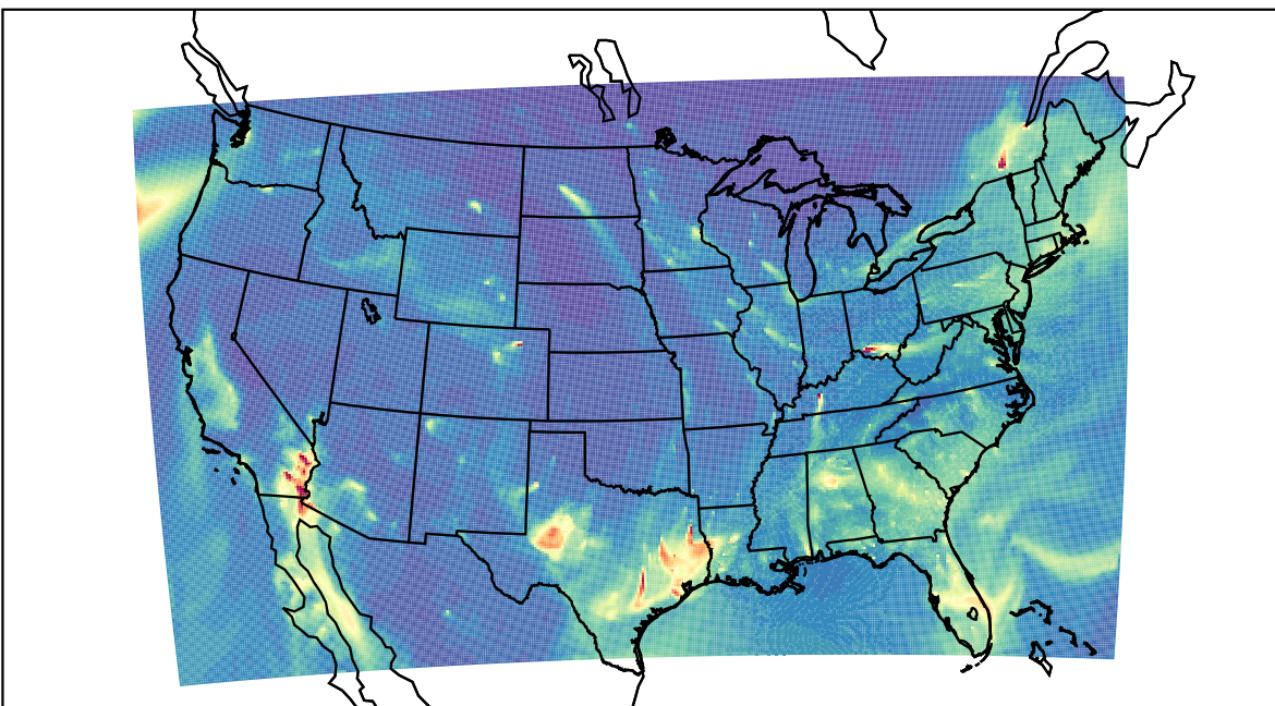
WRF 2022-01-06_14:00:00
