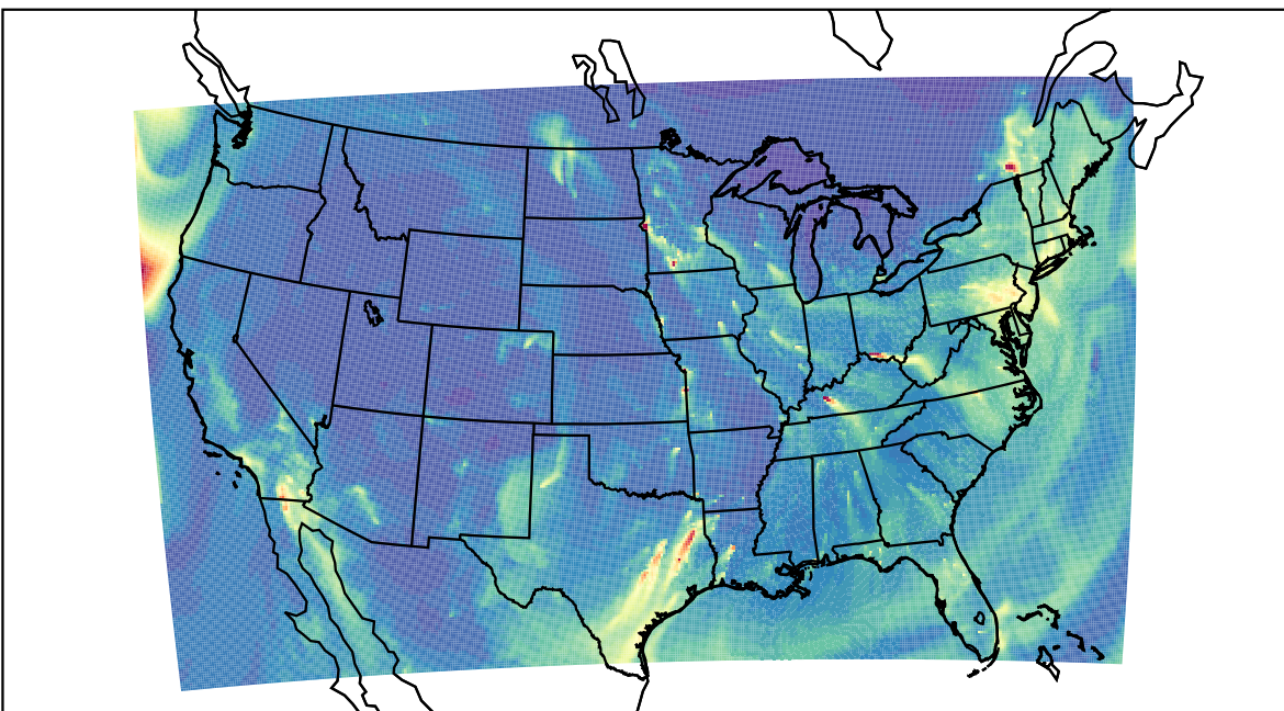
WRF 2022-01-07_12:00:00
