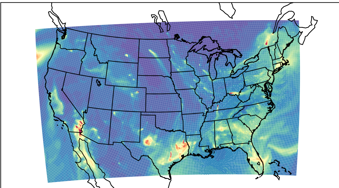
WRF 2022-01-06_13:00:00
