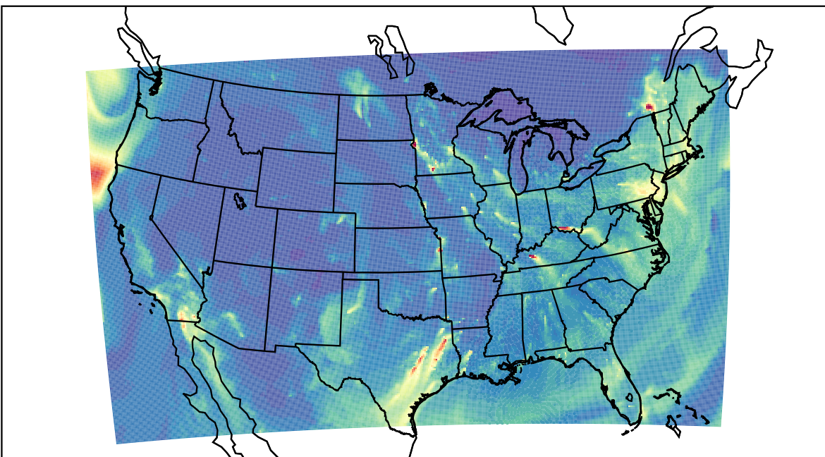
WRF 2022-01-07_13:00:00
