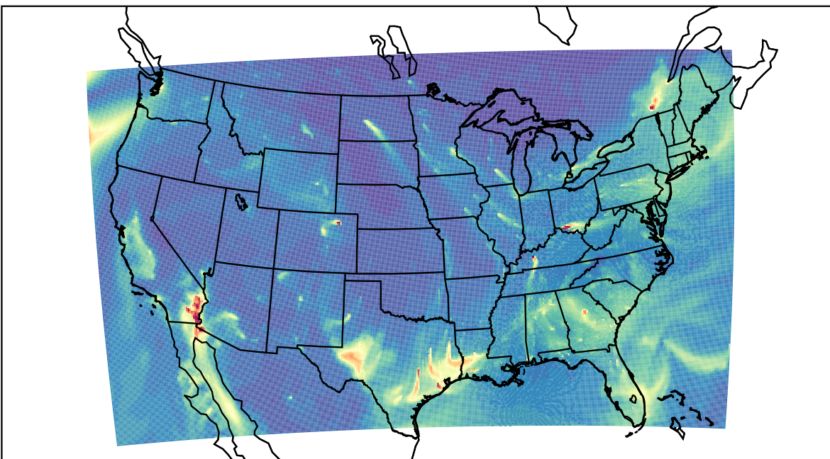
WRF 2022-01-06_16:00:00
