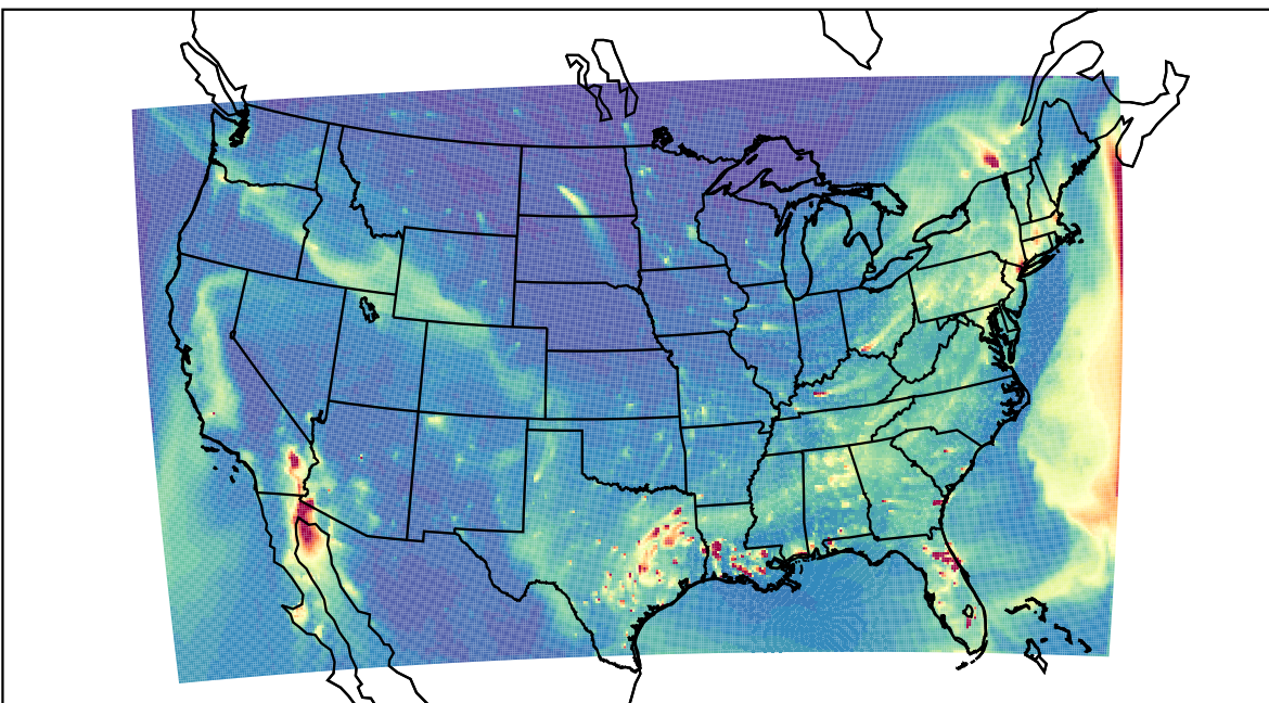
WRF 2022-01-06_00:00:00
