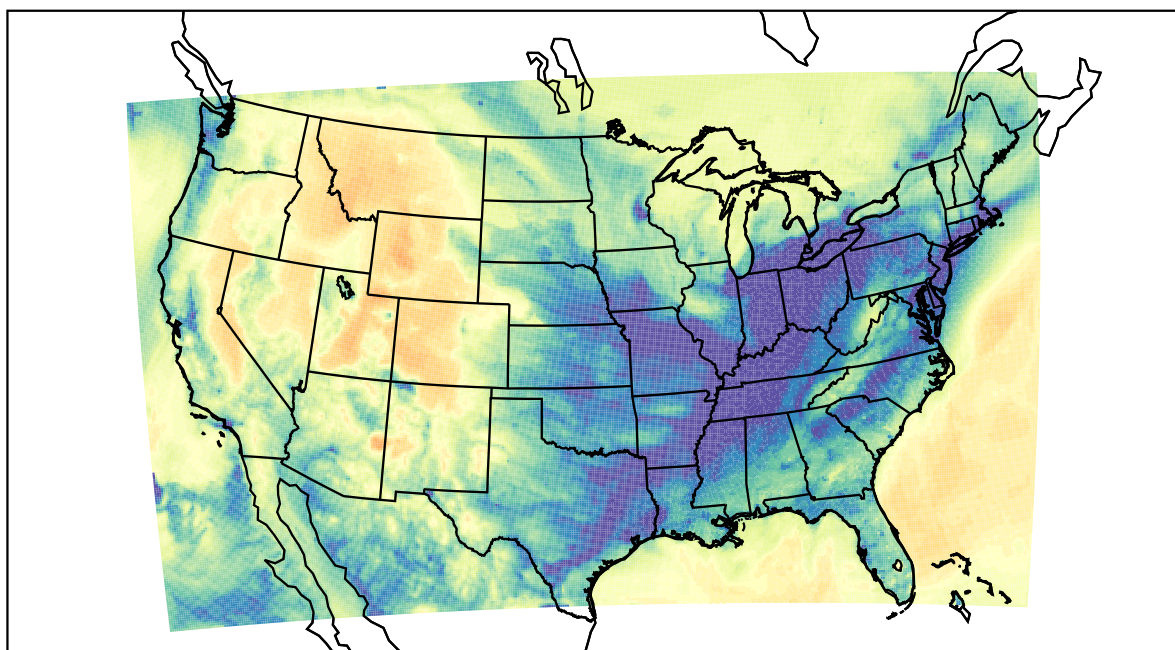
WRF (2022-01-13_13:00:00)
