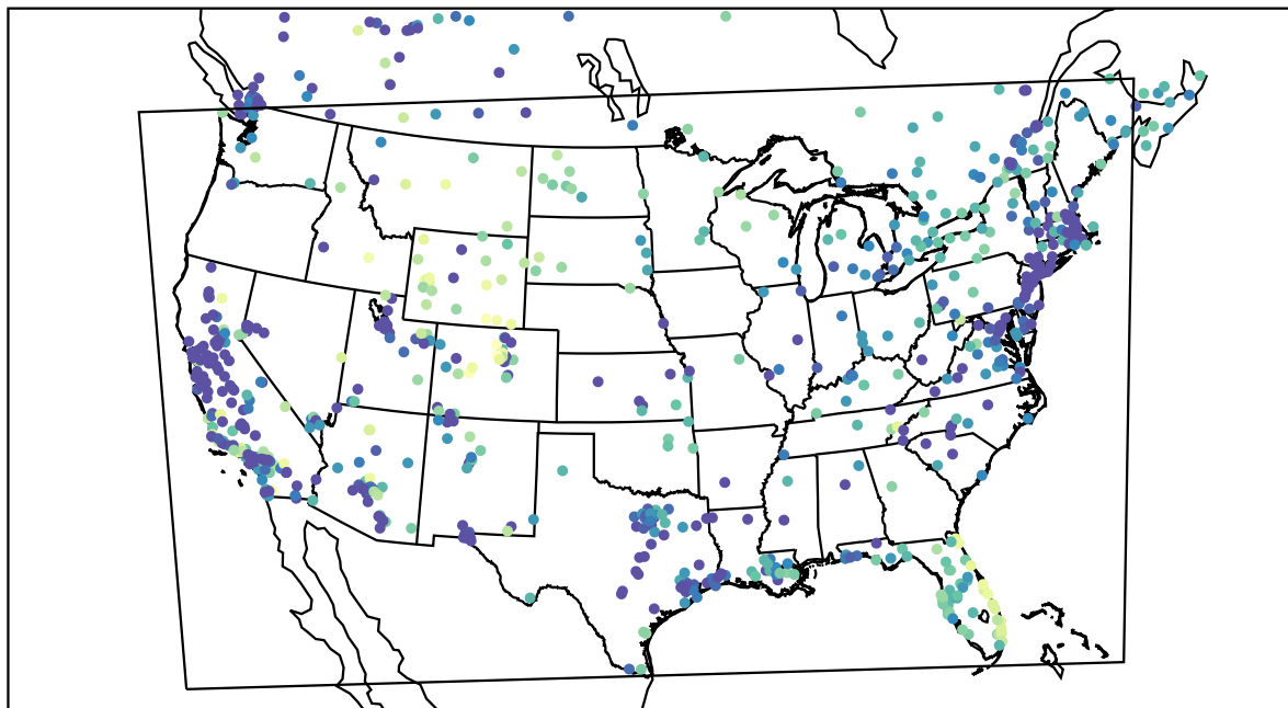
AirNOW (2022-01-12_06:00:00)
