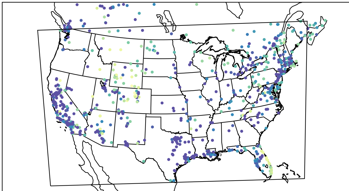
AirNOW (2022-01-12_13:00:00)
