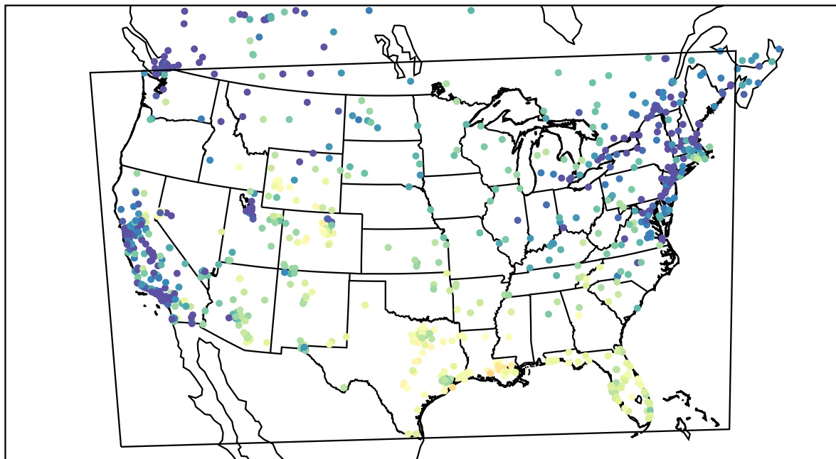
AirNOW (2022-01-13_20:00:00)
