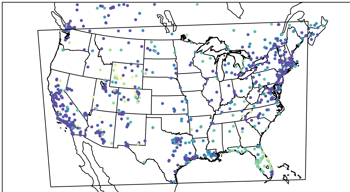
AirNOW (2022-01-13_15:00:00)
