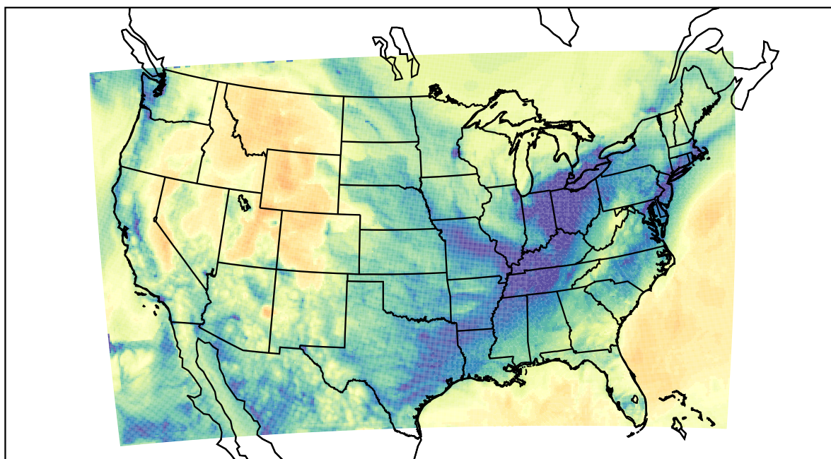
WRF (2022-01-13_16:00:00)
