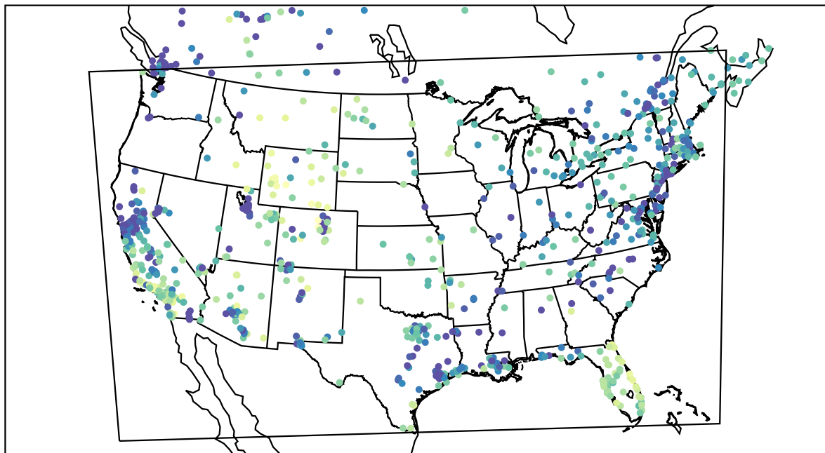
AirNOW (2022-01-12_00:00:00)
