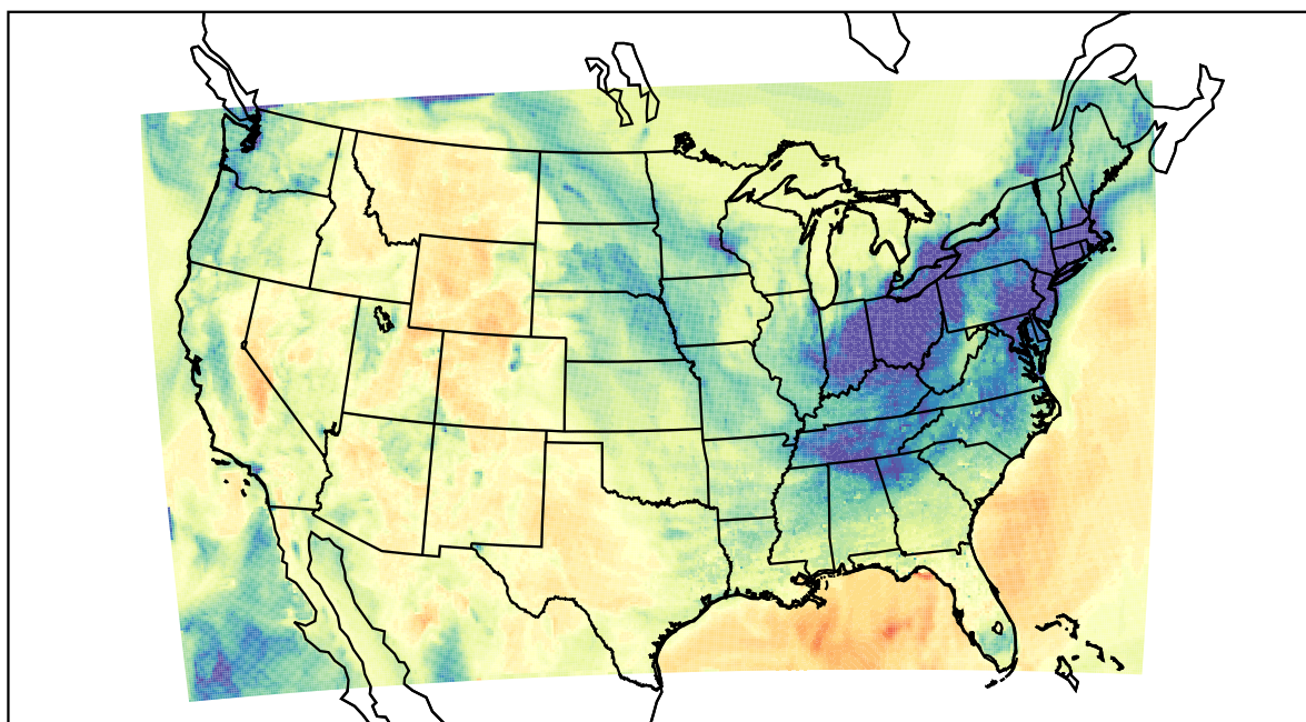
WRF (2022-01-13_22:00:00)
