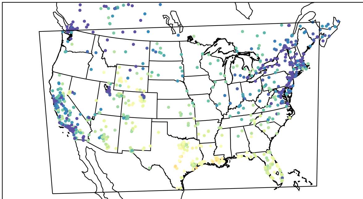
AirNOW (2022-01-13_21:00:00)
