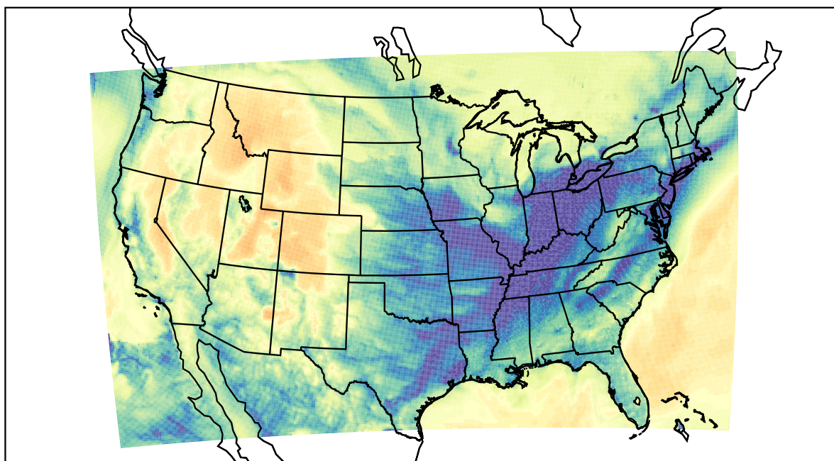
WRF (2022-01-13_11:00:00)
