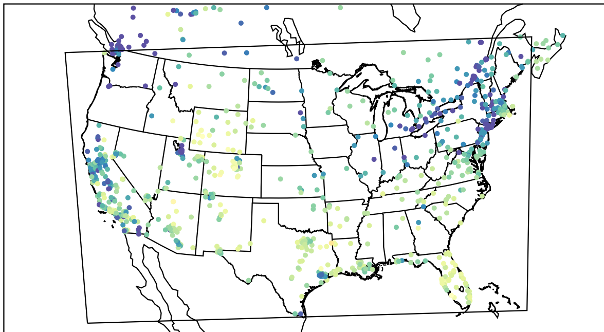
AirNOW (2022-01-12_21:00:00)
