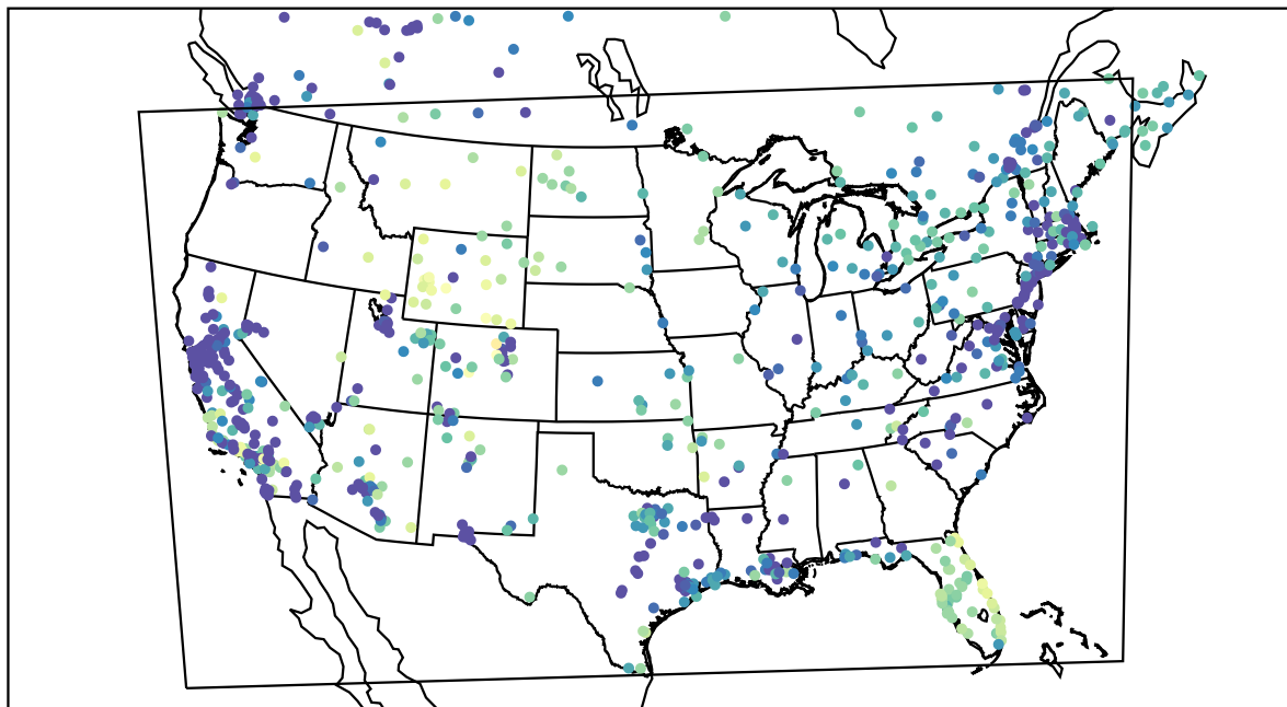
AirNOW (2022-01-12_02:00:00)
