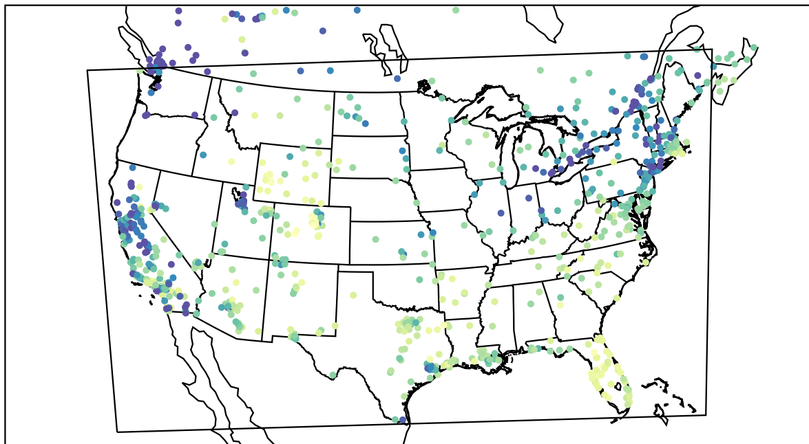
AirNOW (2022-01-12_20:00:00)
