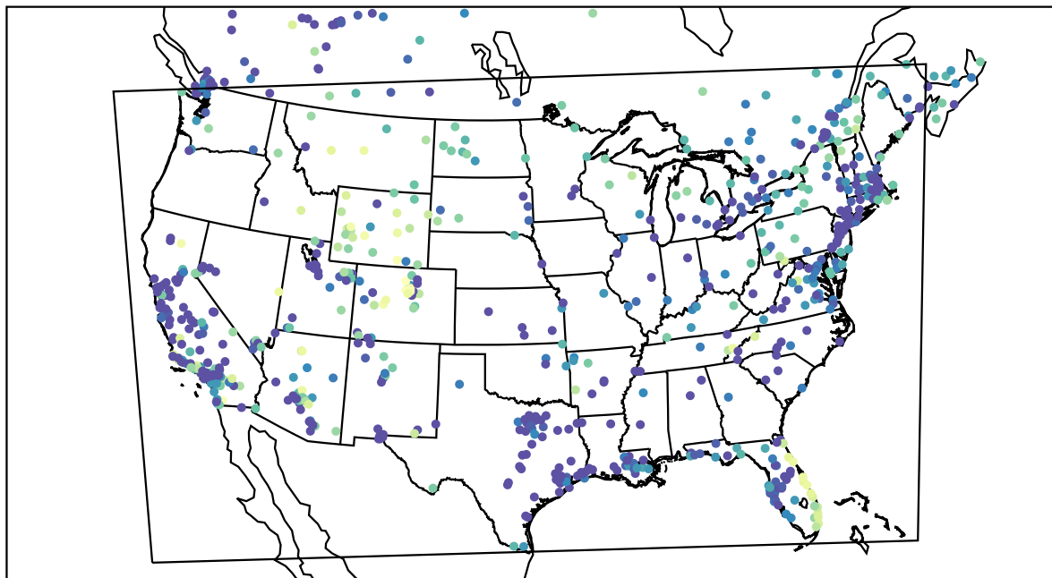
AirNOW (2022-01-12_12:00:00)
