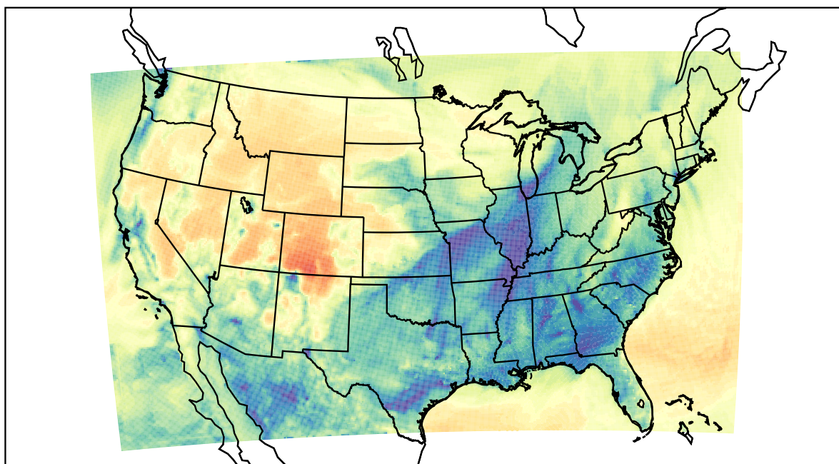
WRF (2022-01-12_06:00:00)
