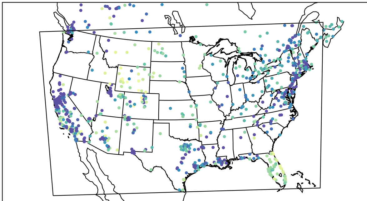
AirNOW (2022-01-12_01:00:00)
