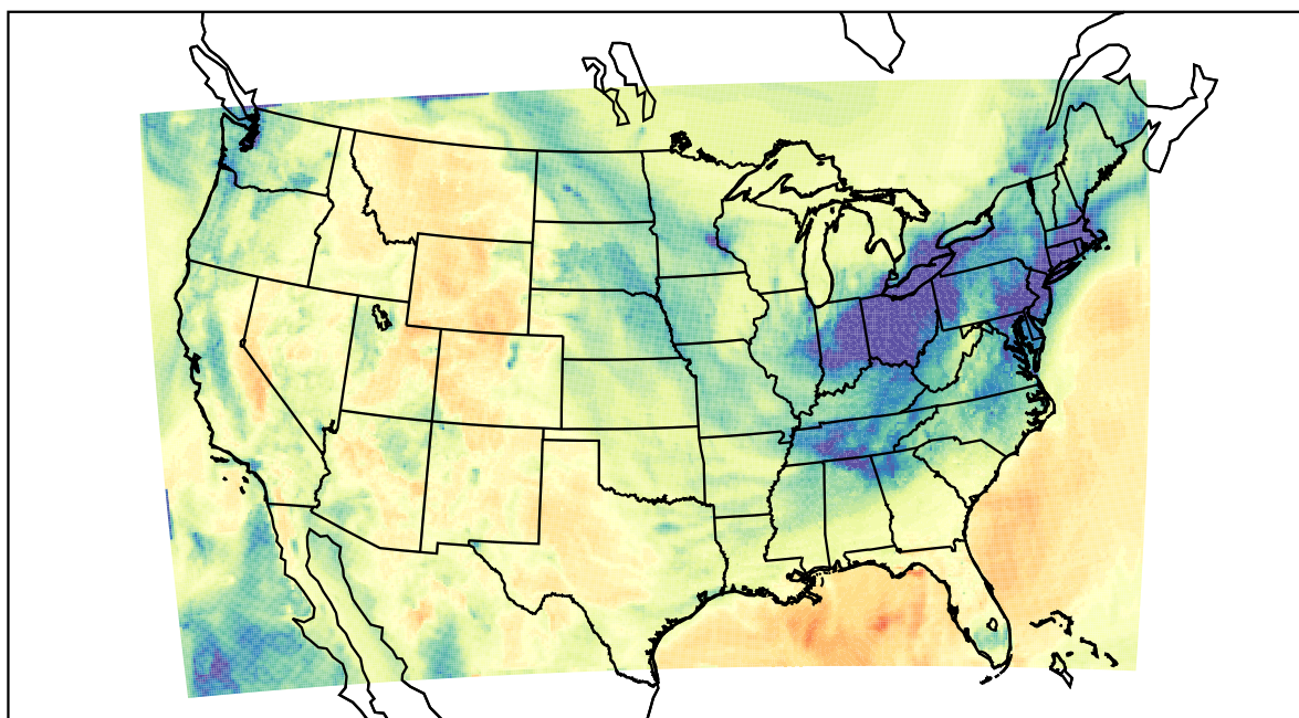
WRF (2022-01-13_21:00:00)
