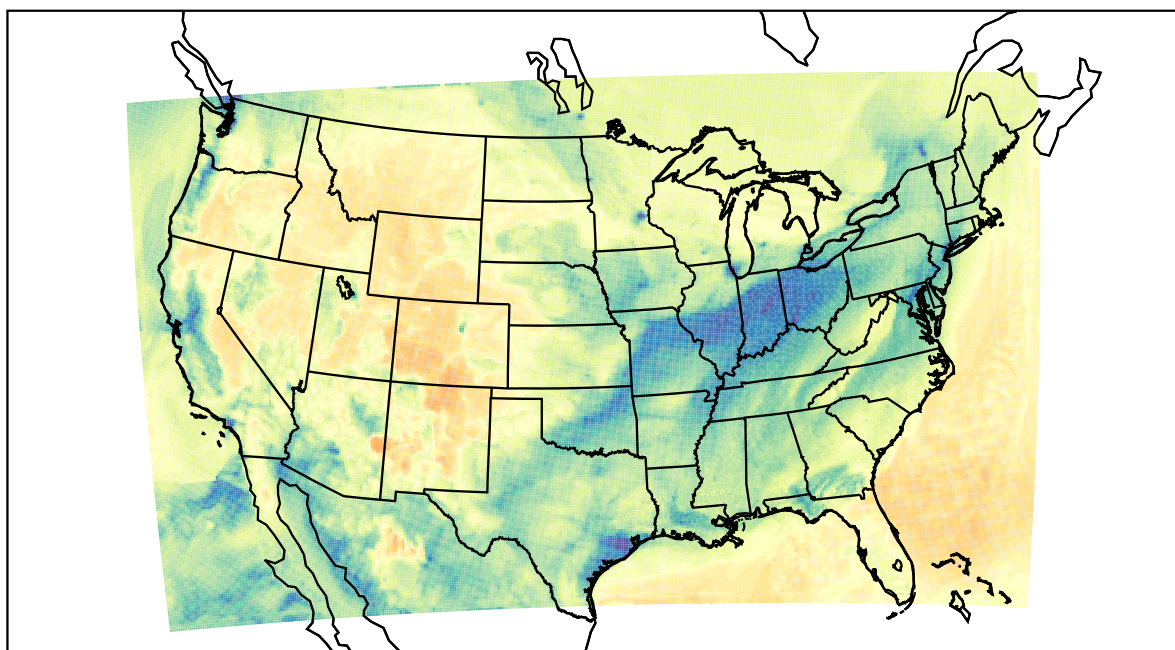
WRF (2022-01-12_18:00:00)
