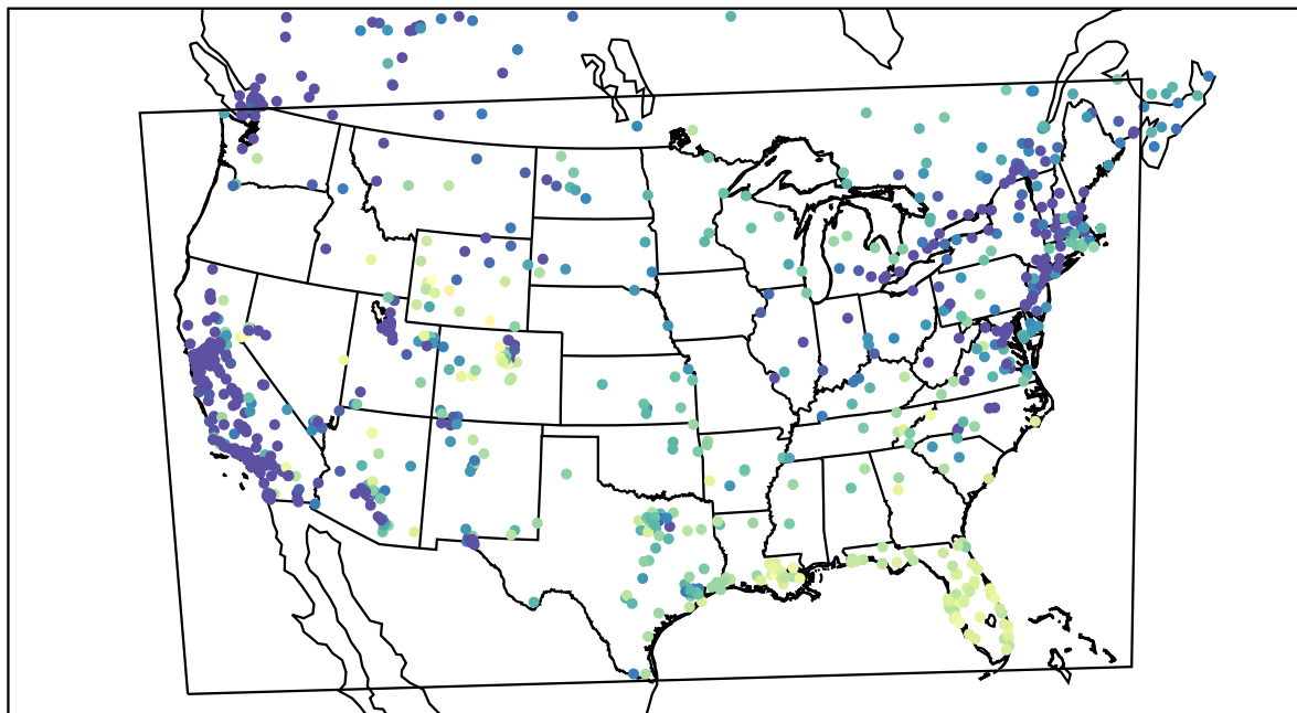
AirNOW (2022-01-13_17:00:00)
