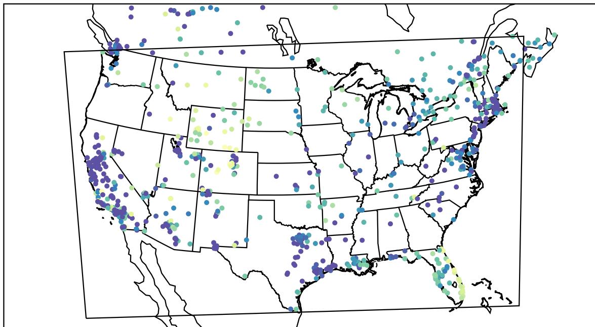
AirNOW (2022-01-12_07:00:00)
