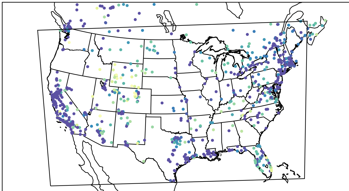
AirNOW (2022-01-13_04:00:00)
