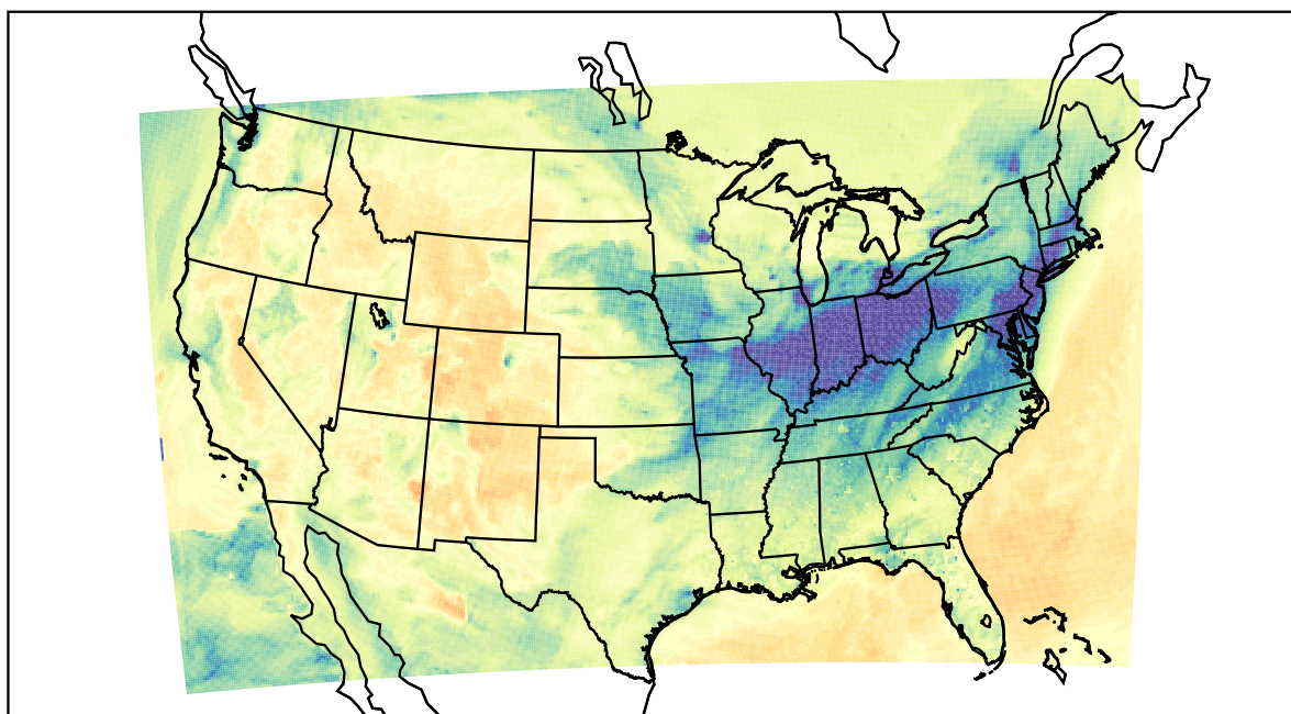
WRF (2022-01-12_22:00:00)
