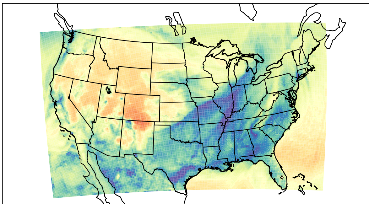
WRF (2022-01-12_09:00:00)
