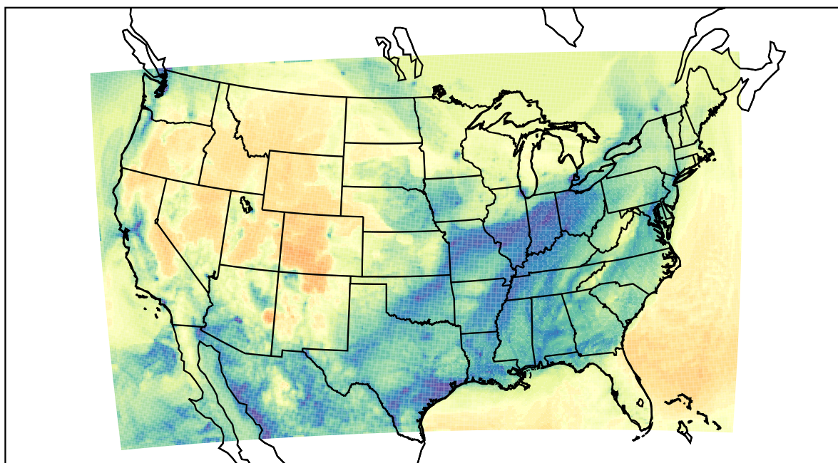
WRF (2022-01-12_16:00:00)
