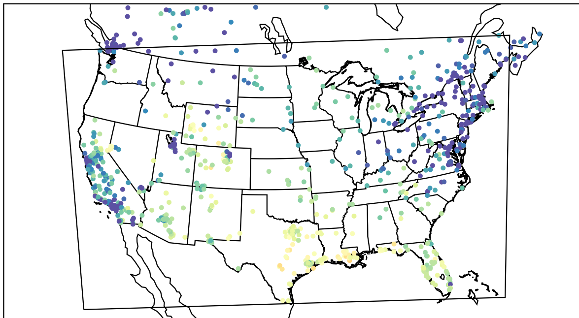
AirNOW (2022-01-13_22:00:00)
