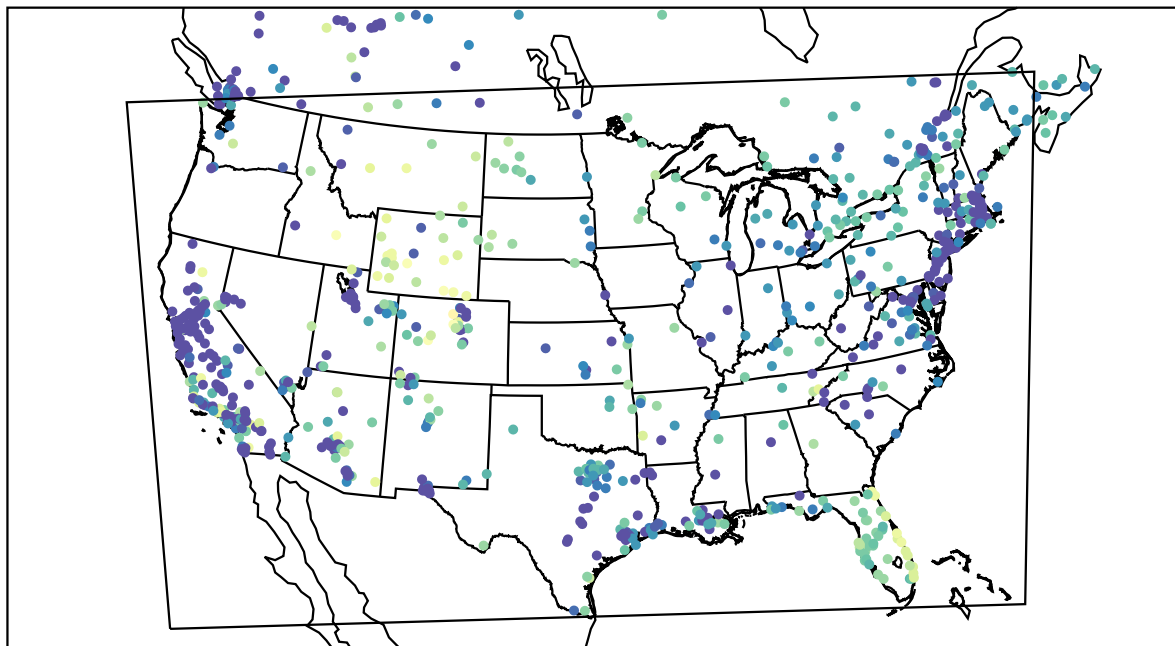
AirNOW (2022-01-12_04:00:00)
