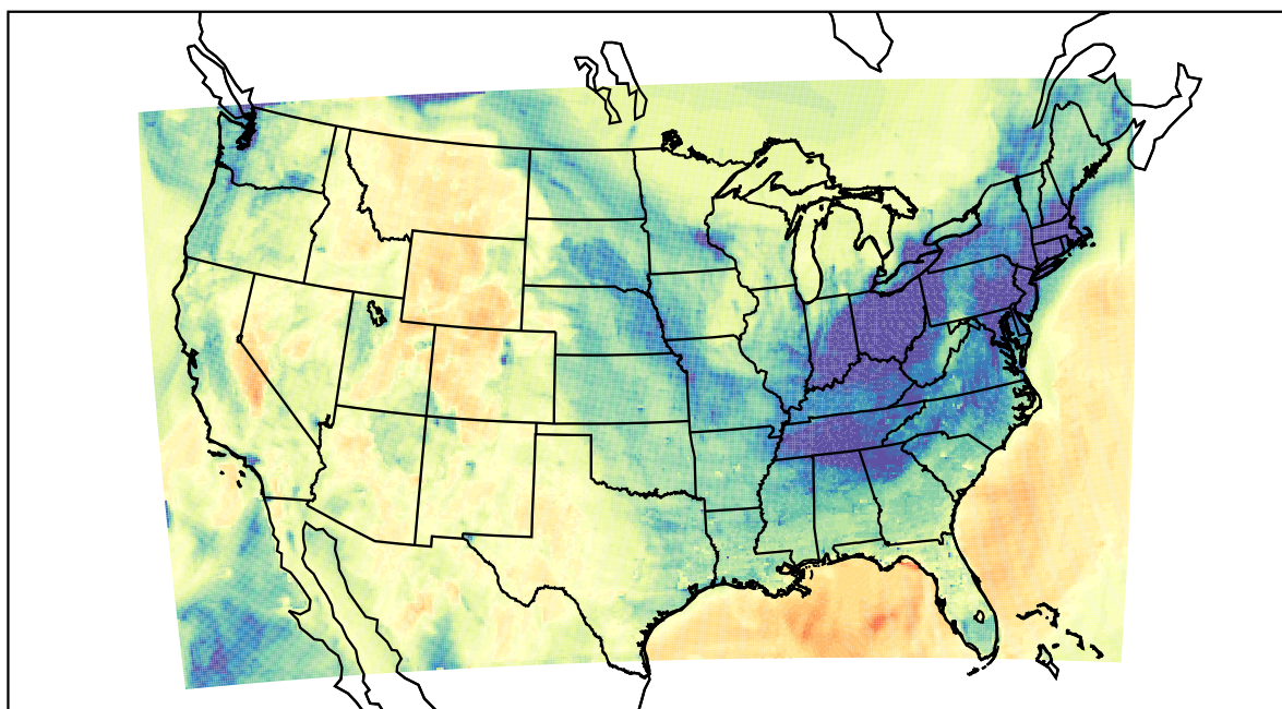
WRF (2022-01-13_23:00:00)
