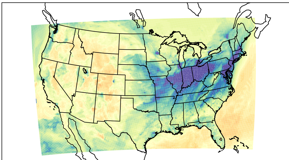
WRF (2022-01-12_23:00:00)
