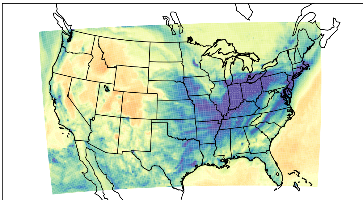
WRF (2022-01-13_06:00:00)
