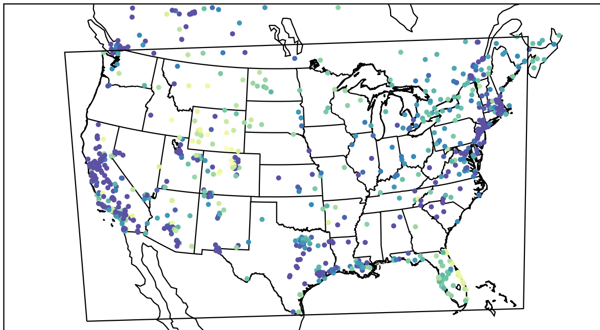
AirNOW (2022-01-12_05:00:00)
