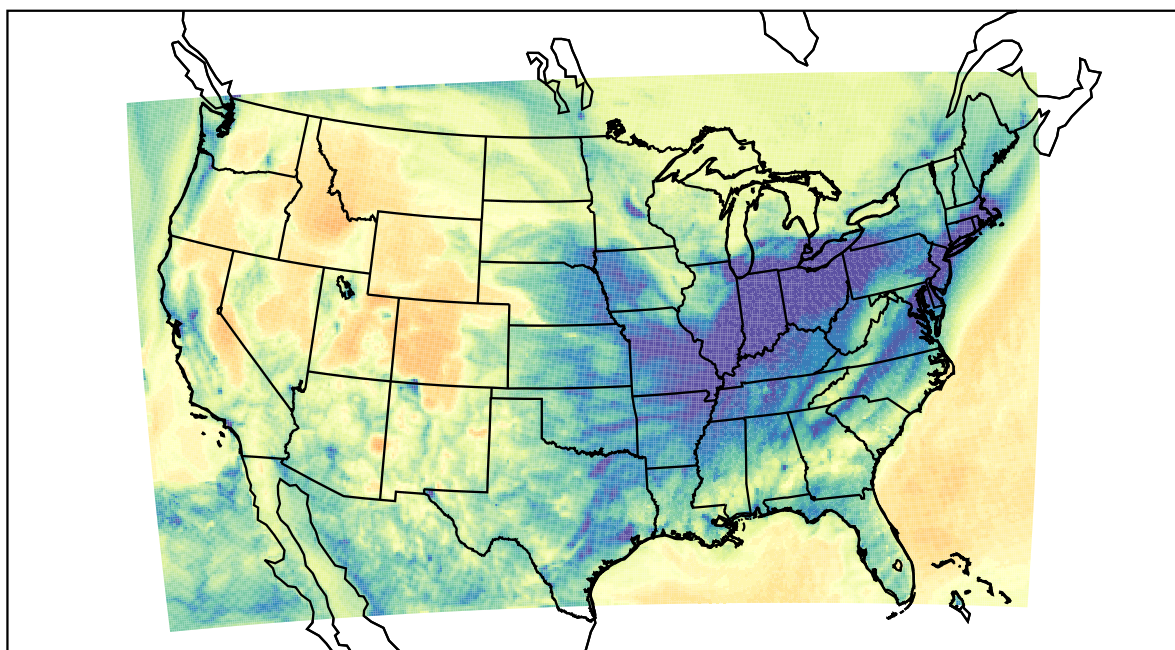
WRF (2022-01-13_05:00:00)
