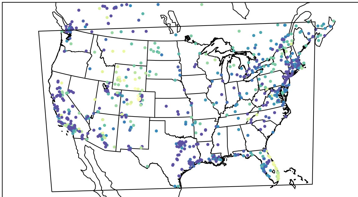
AirNOW (2022-01-12_11:00:00)
