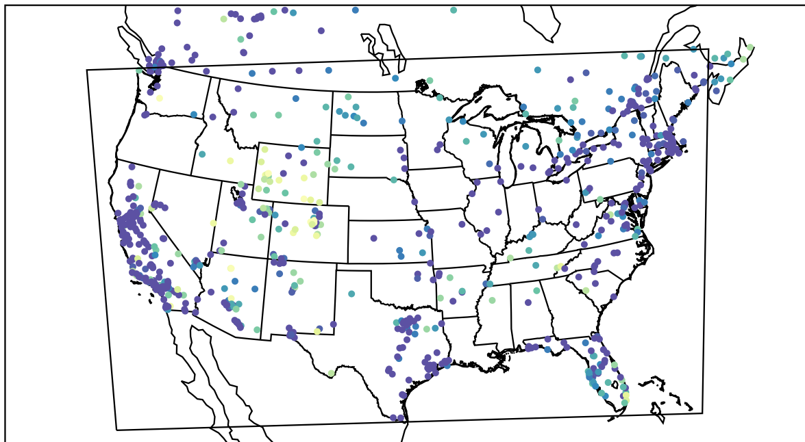
AirNOW (2022-01-13_07:00:00)
