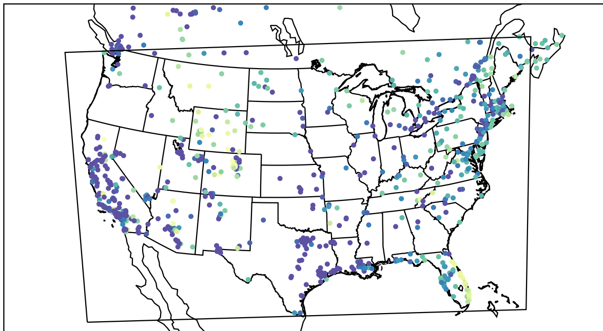
AirNOW (2022-01-12_14:00:00)
