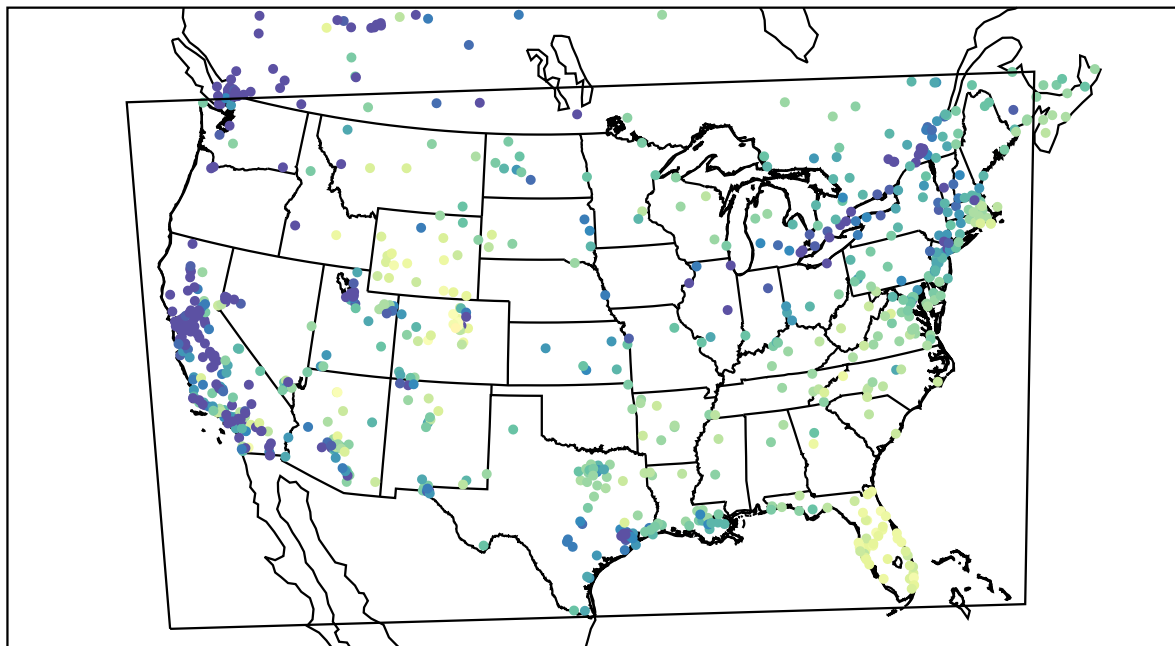
AirNOW (2022-01-12_18:00:00)
