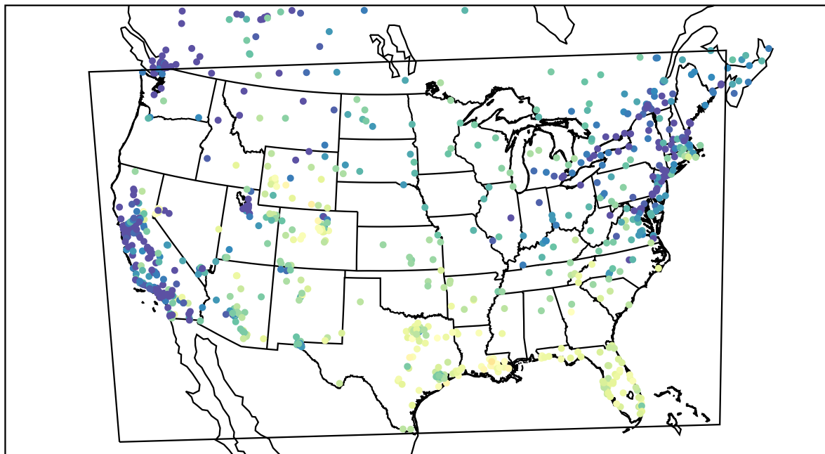
AirNOW (2022-01-13_19:00:00)
