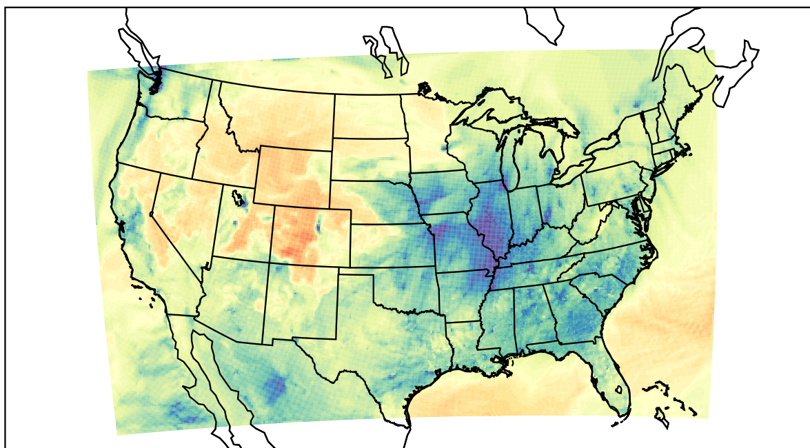
WRF (2022-01-12_00:00:00)
