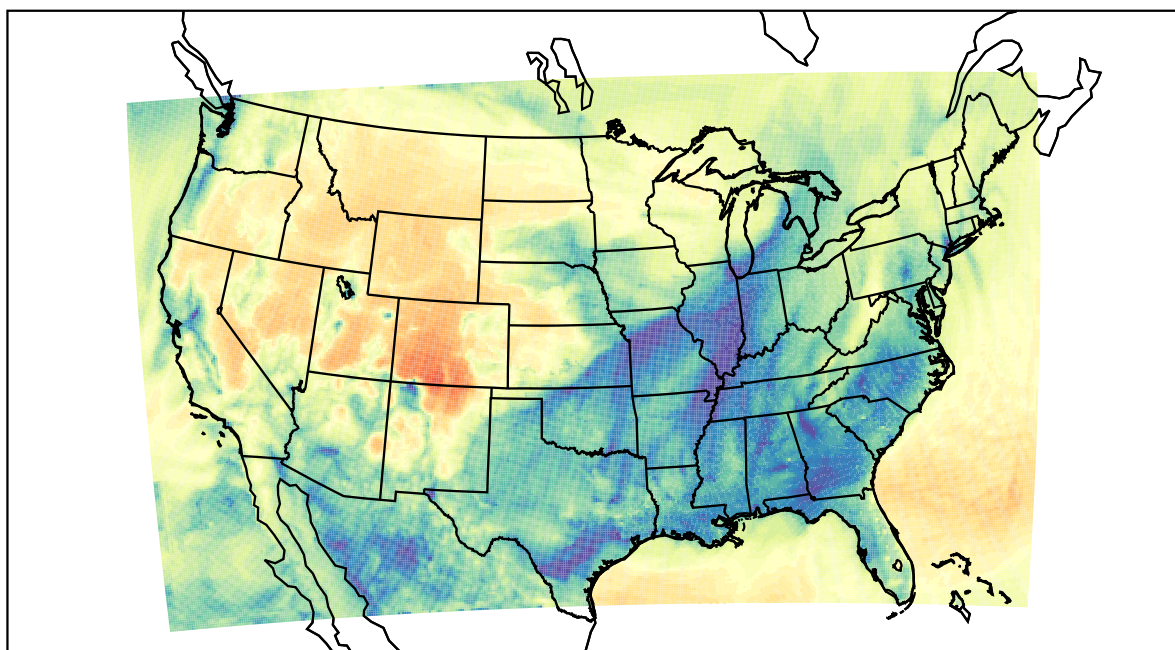
WRF (2022-01-12_07:00:00)
