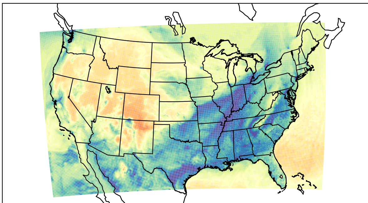
WRF (2022-01-12_13:00:00)
