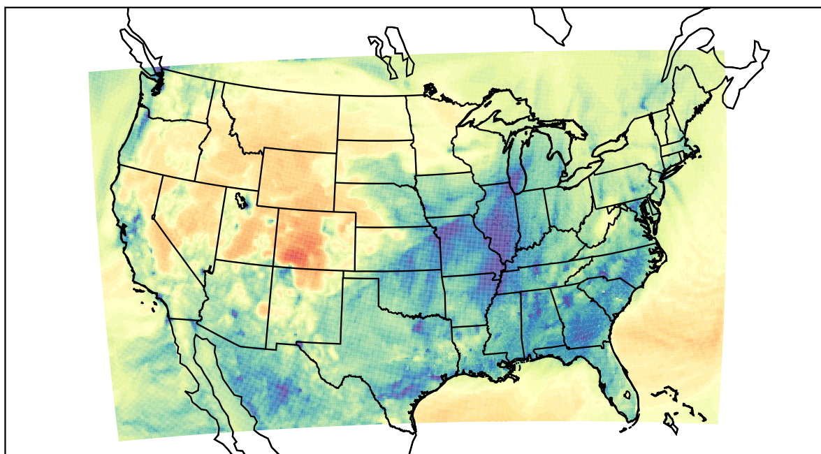
WRF (2022-01-12_03:00:00)
