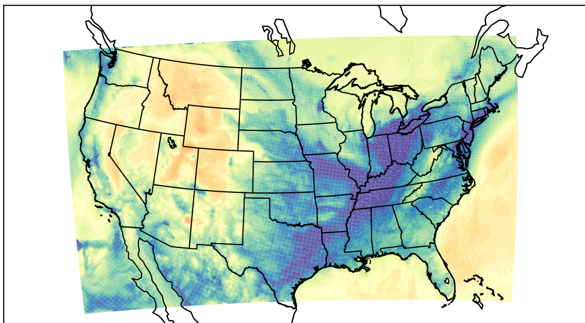
WRF (2022-01-13_15:00:00)
