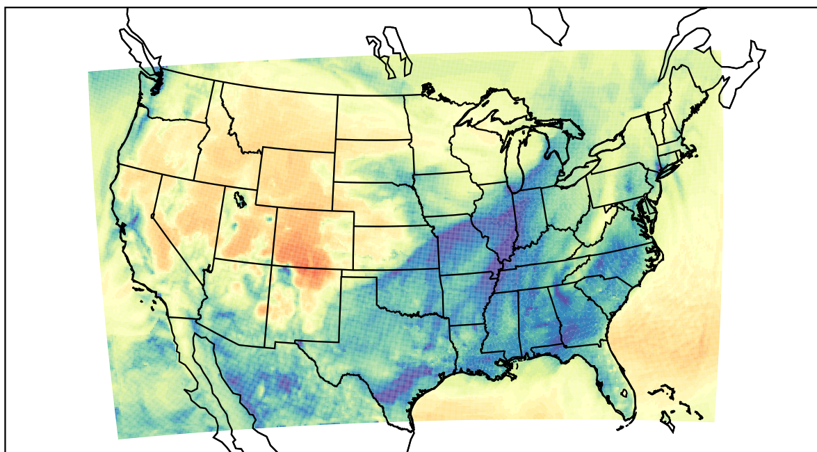
WRF (2022-01-12_08:00:00)
