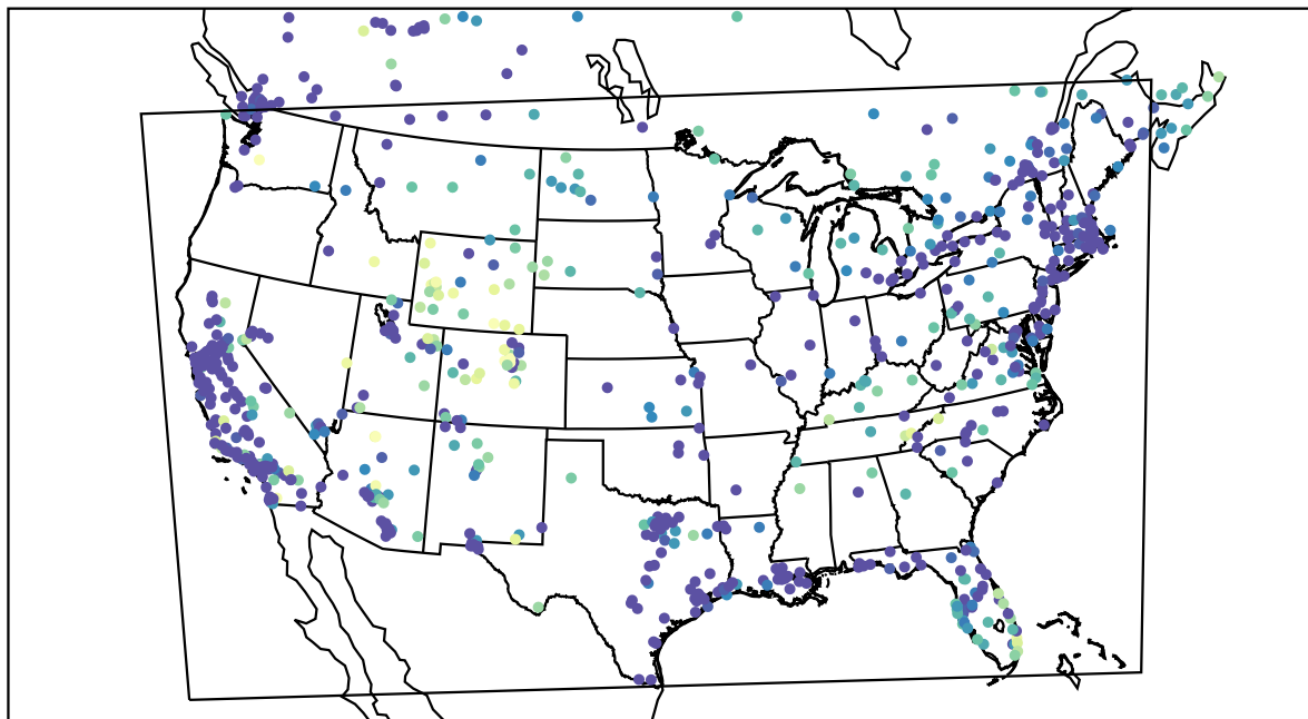
AirNOW (2022-01-13_06:00:00)
