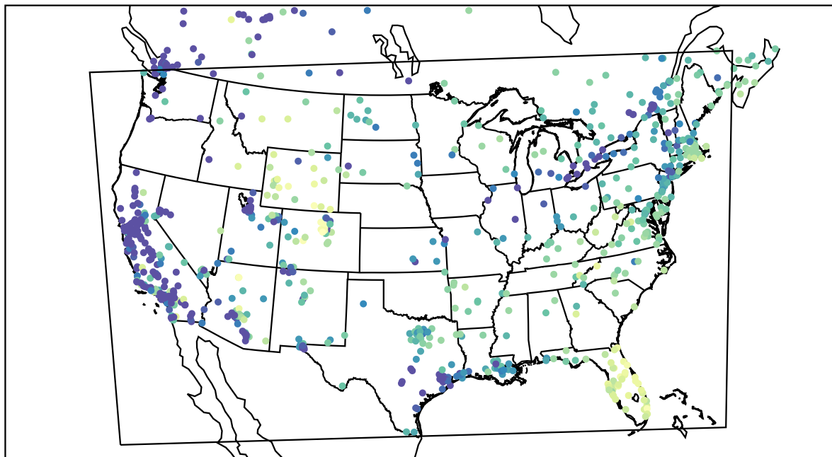
AirNOW (2022-01-12_17:00:00)
