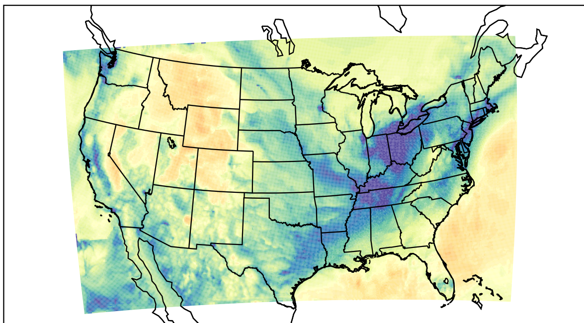
WRF (2022-01-13_17:00:00)
