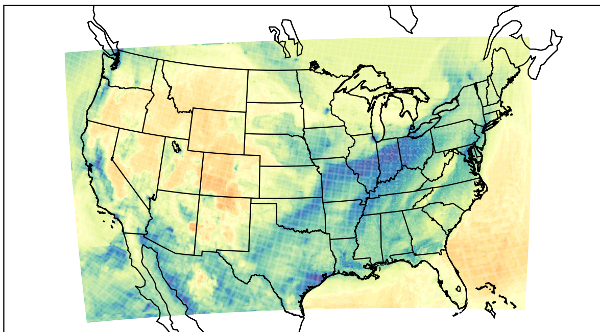
WRF (2022-01-12_17:00:00)
