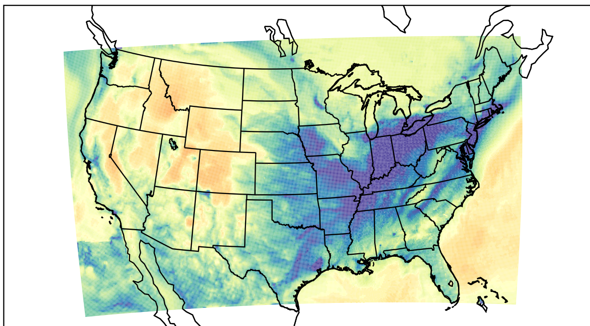
WRF (2022-01-13_08:00:00)
