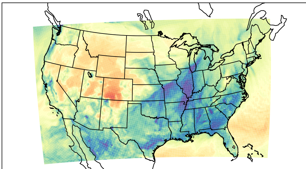
WRF (2022-01-12_05:00:00)
