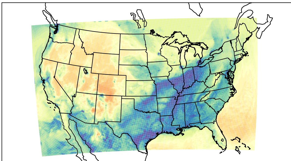
WRF (2022-01-12_15:00:00)
