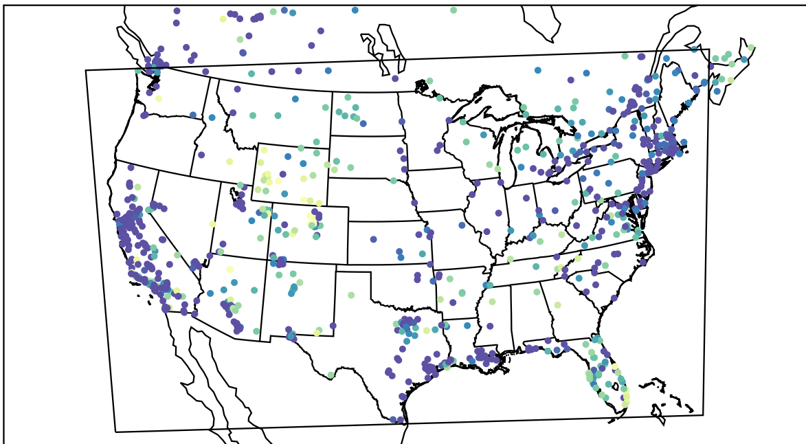
AirNOW (2022-01-13_03:00:00)
