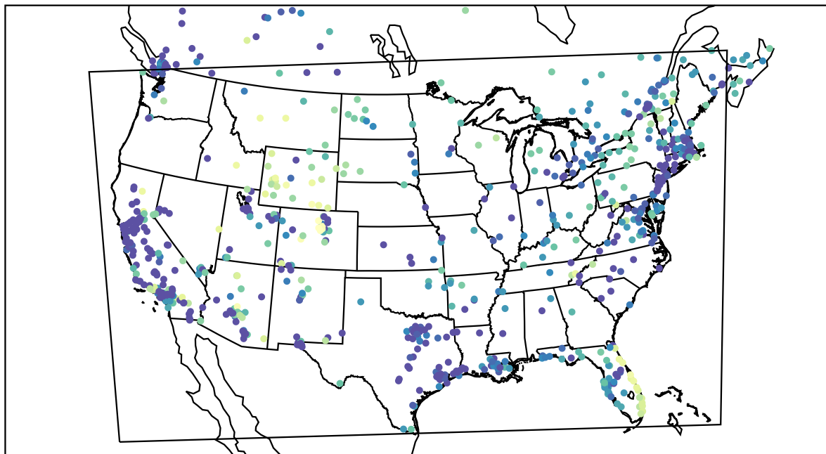
AirNOW (2022-01-12_10:00:00)
