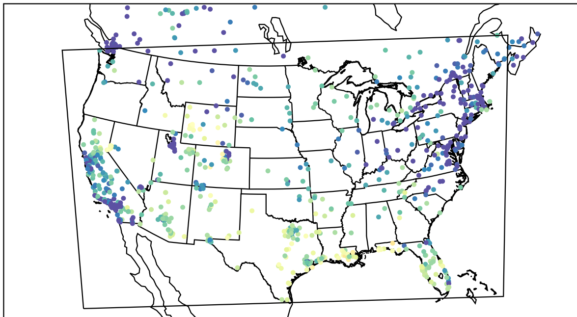
AirNOW (2022-01-13_23:00:00)
