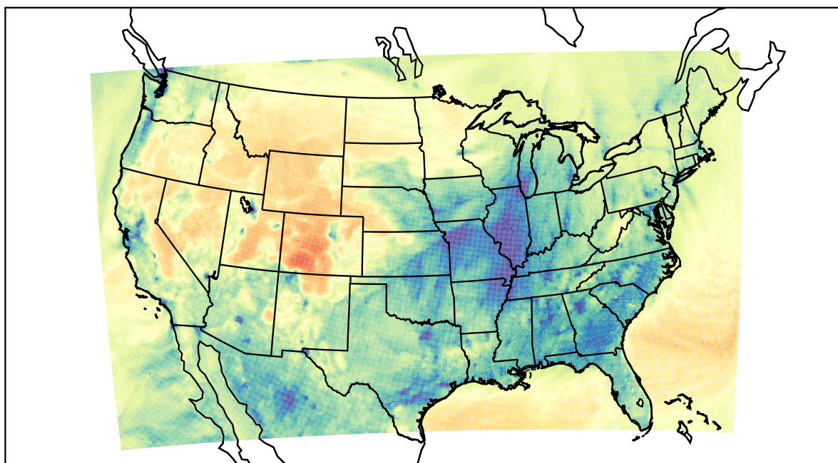
WRF (2022-01-12_02:00:00)
