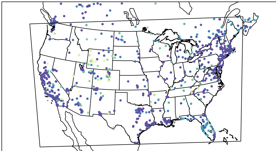
AirNOW (2022-01-13_14:00:00)
