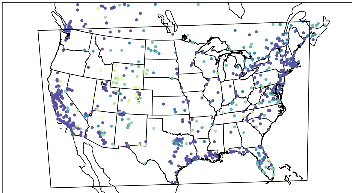
AirNOW (2022-01-13_05:00:00)
