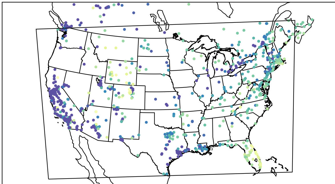
AirNOW (2022-01-12_16:00:00)
