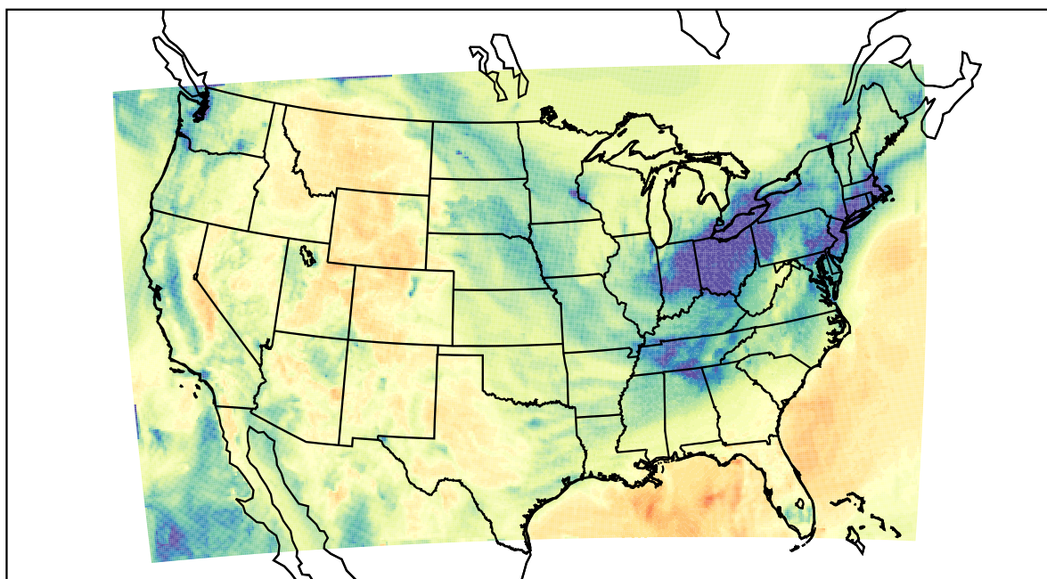
WRF (2022-01-13_20:00:00)
