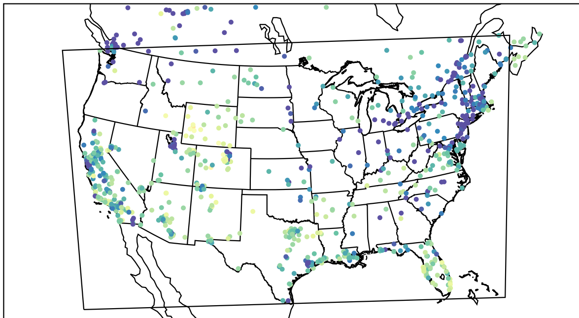
AirNOW (2022-01-12_23:00:00)
