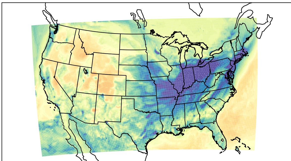
WRF (2022-01-13_04:00:00)
