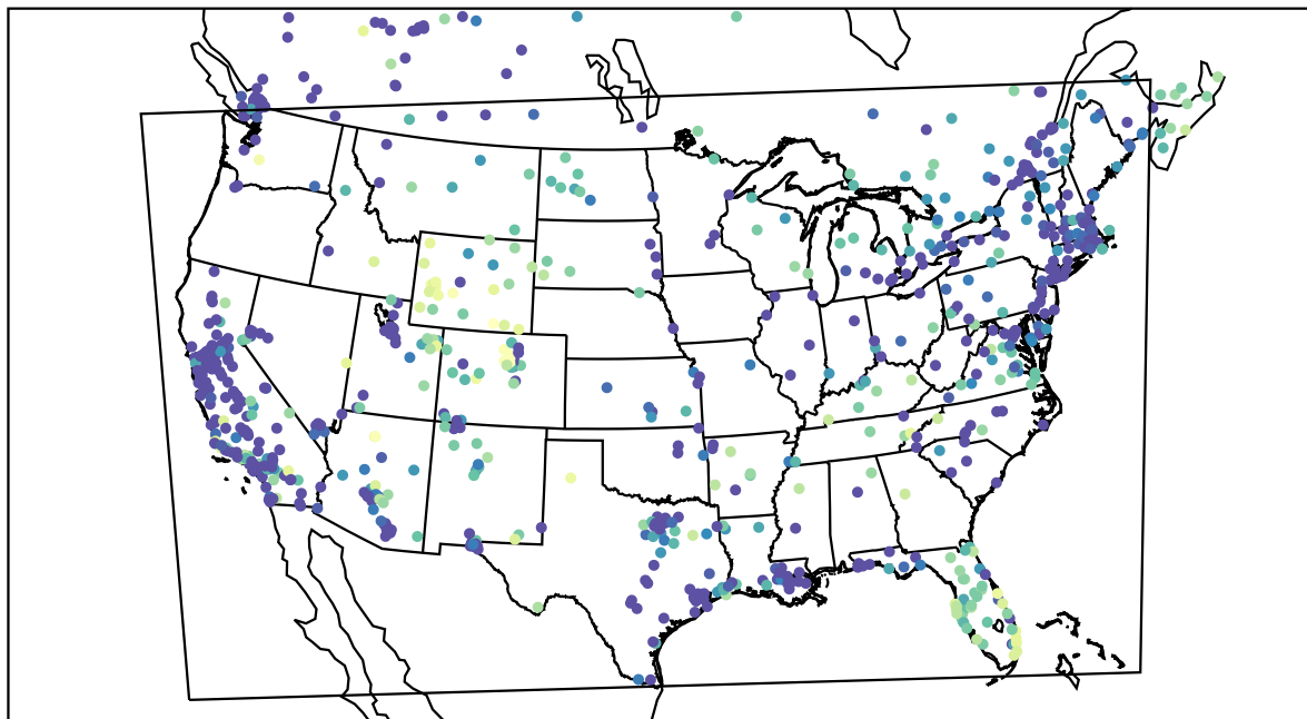
AirNOW (2022-01-13_02:00:00)
