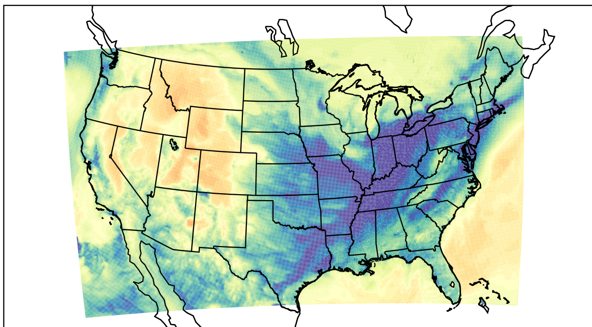
WRF (2022-01-13_12:00:00)
