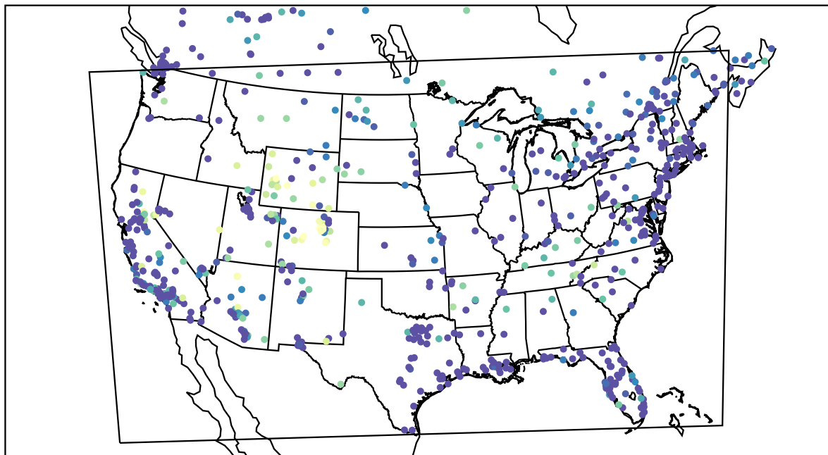
AirNOW (2022-01-13_11:00:00)
