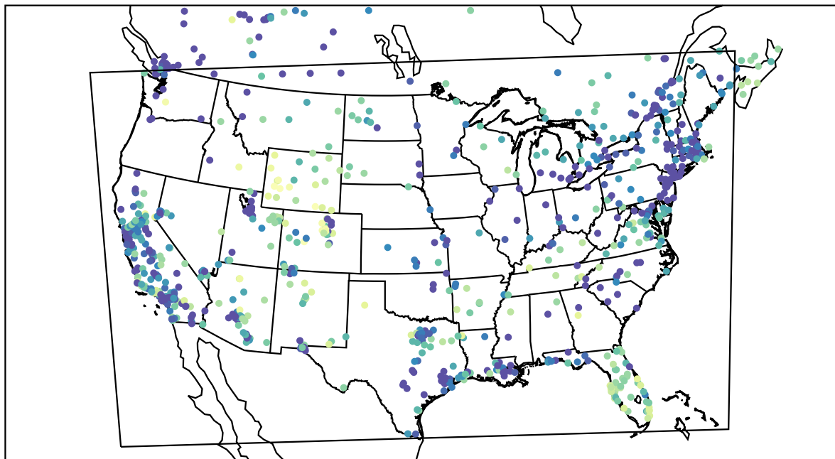
AirNOW (2022-01-13_00:00:00)
