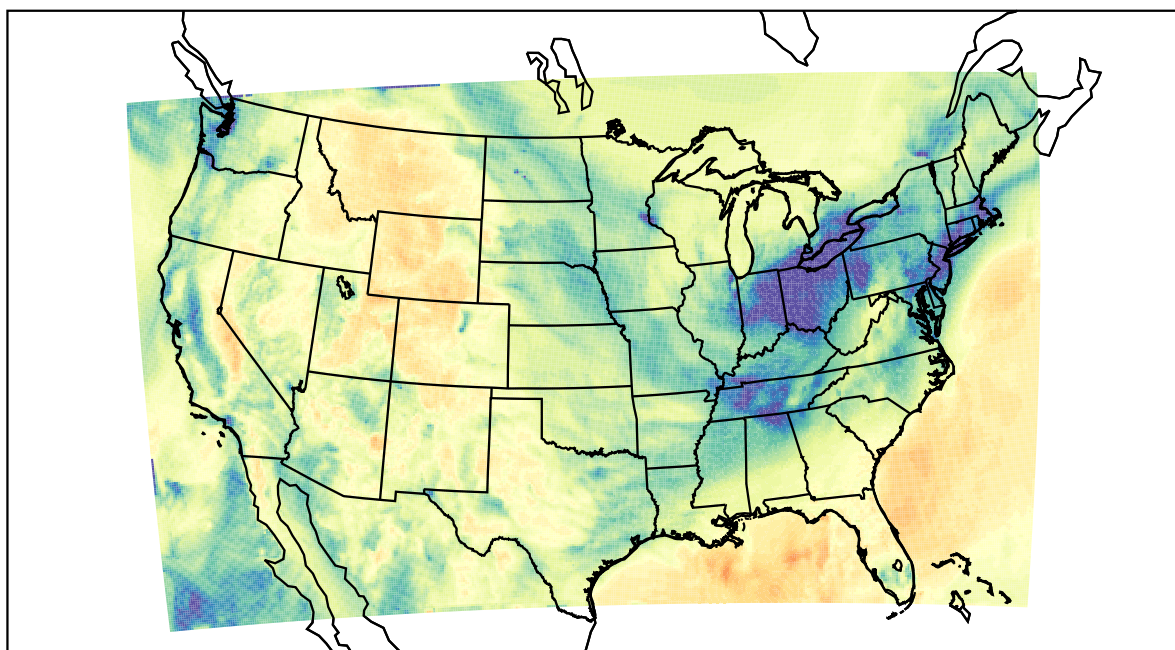
WRF (2022-01-13_19:00:00)
