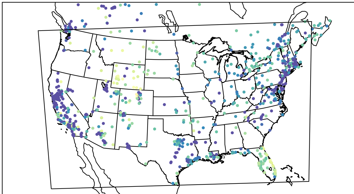
AirNOW (2022-01-12_03:00:00)
