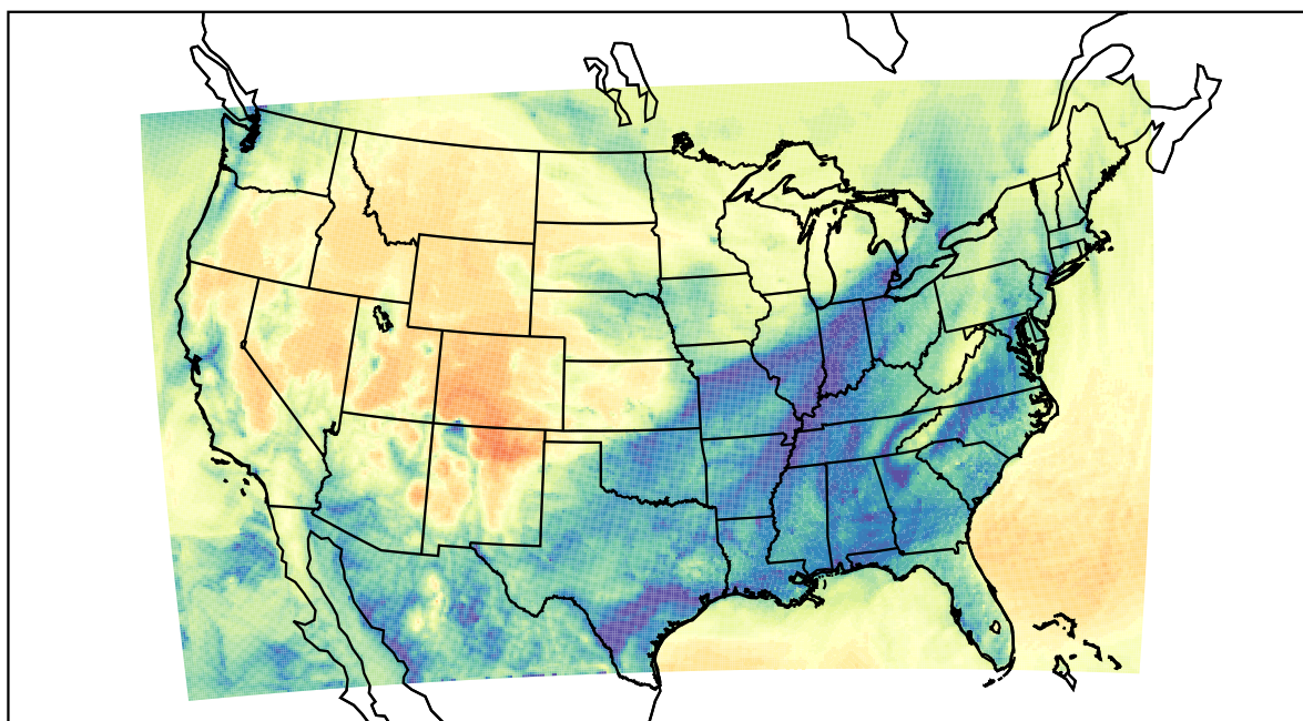
WRF (2022-01-12_12:00:00)
