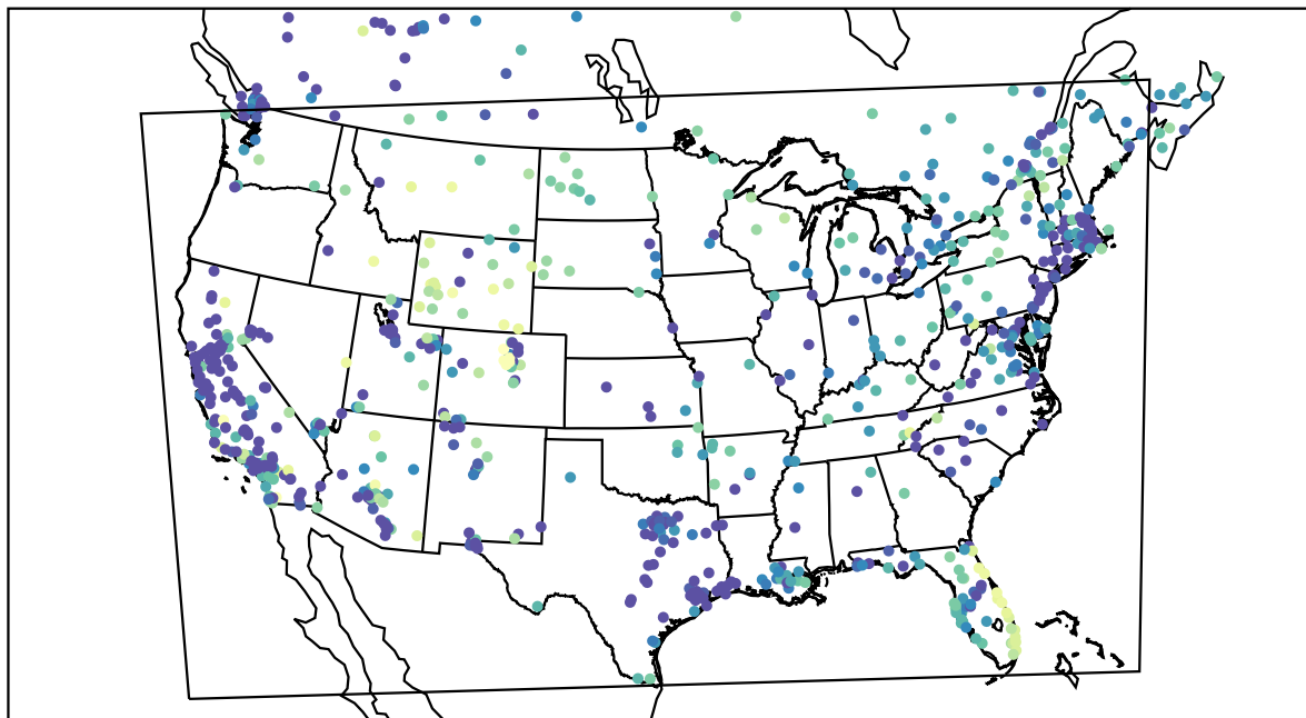
AirNOW (2022-01-12_09:00:00)
