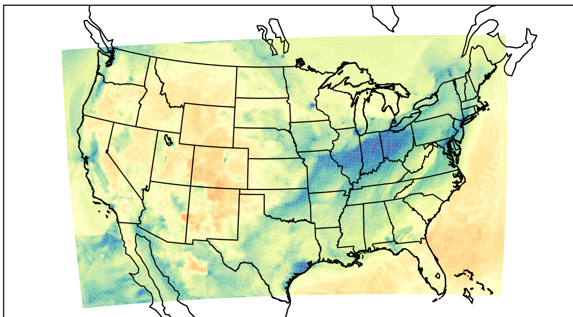
WRF (2022-01-12_19:00:00)
