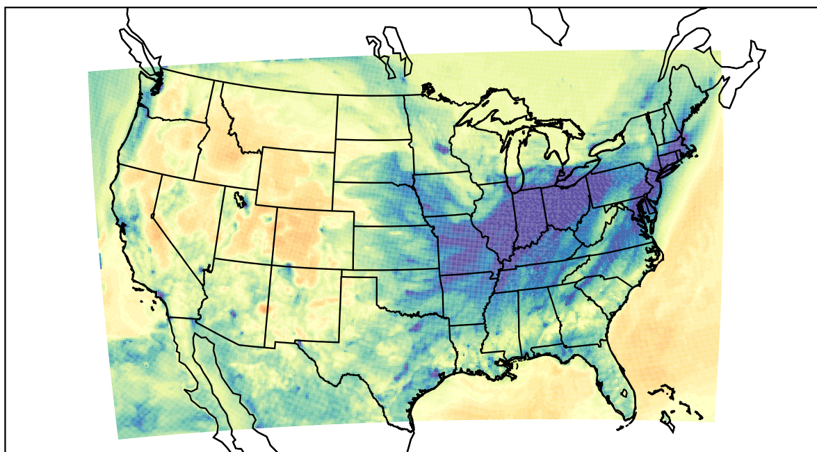
WRF (2022-01-13_02:00:00)
