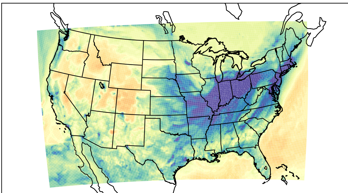
WRF (2022-01-13_03:00:00)
