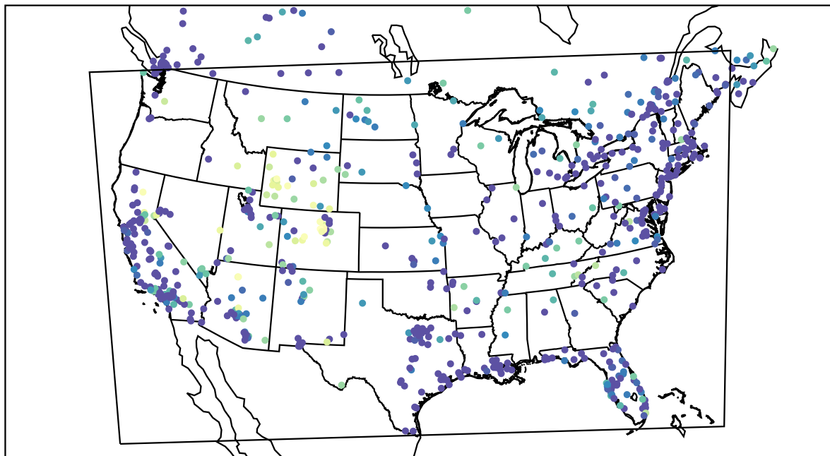
AirNOW (2022-01-13_10:00:00)
