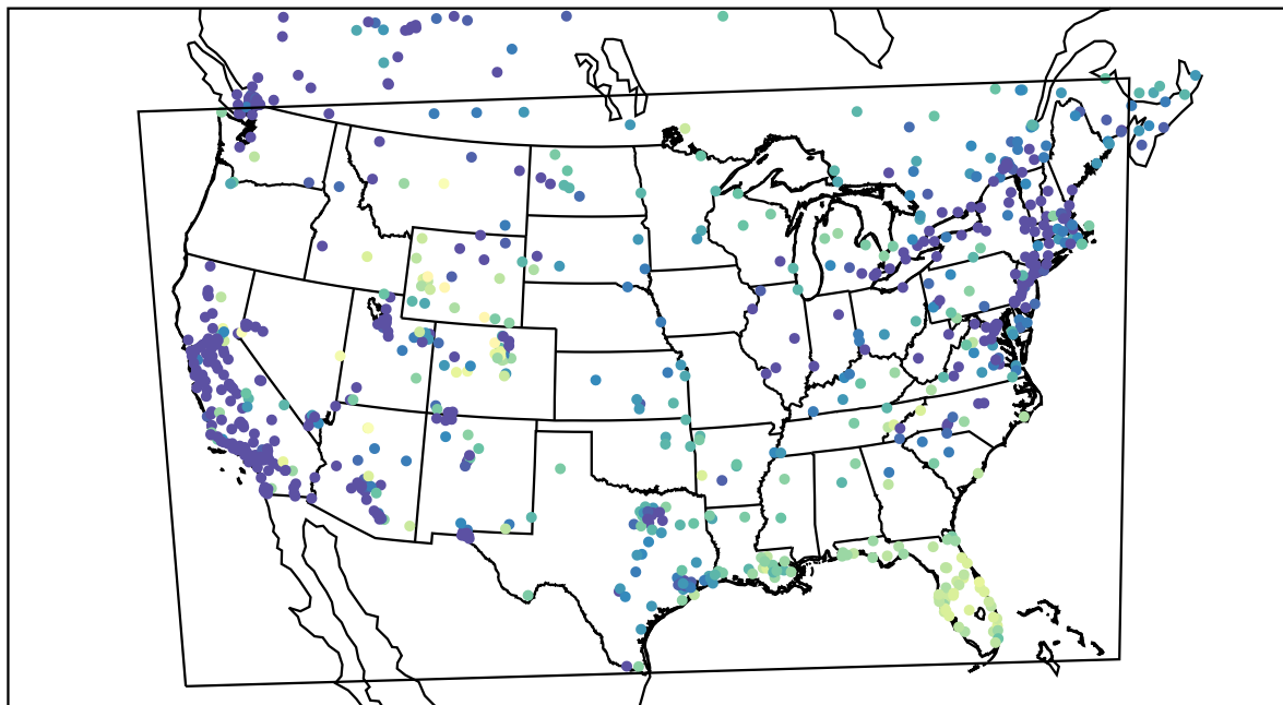
AirNOW (2022-01-13_16:00:00)
