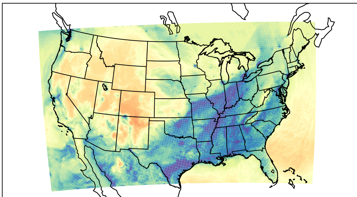
WRF (2022-01-12_14:00:00)
