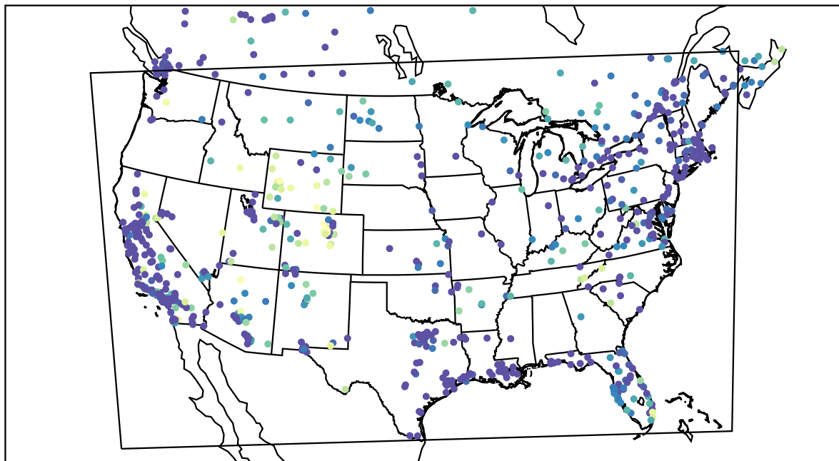
AirNOW (2022-01-13_08:00:00)
