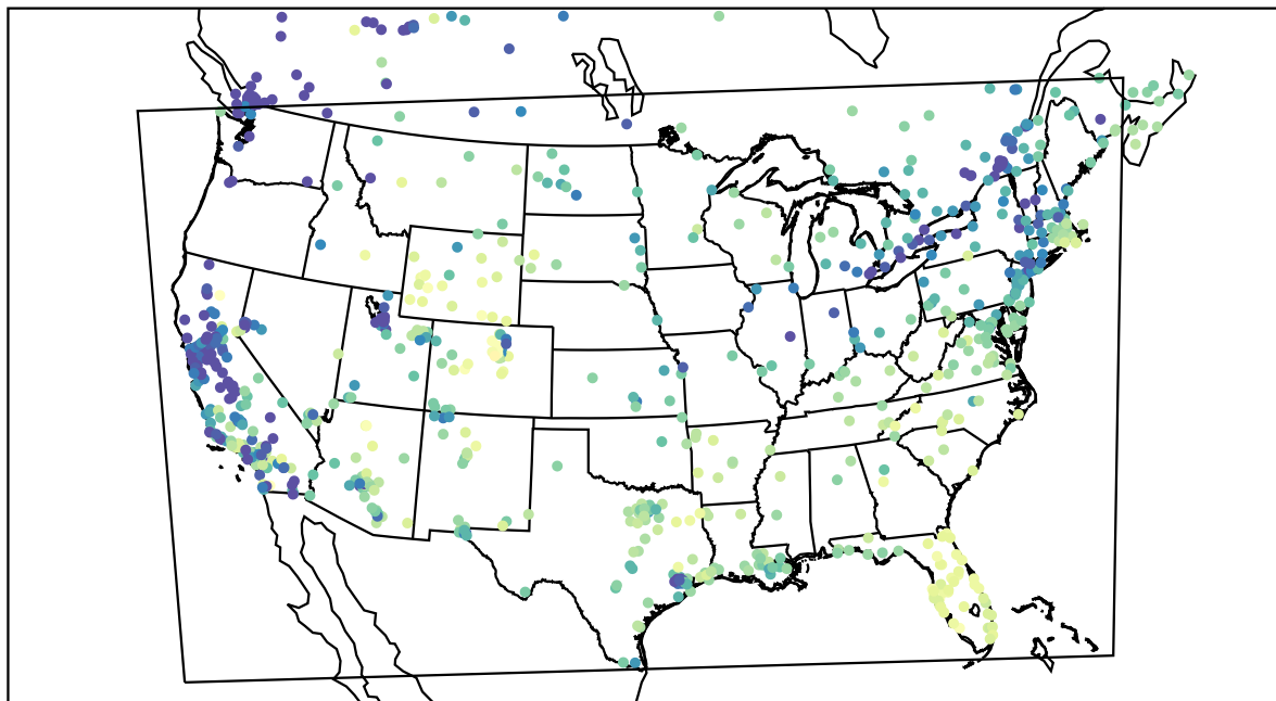
AirNOW (2022-01-12_19:00:00)
