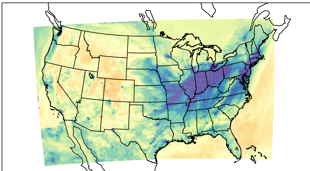
WRF (2022-01-13_01:00:00)
