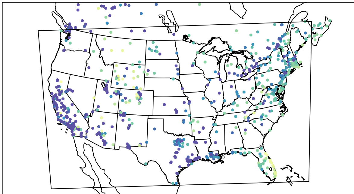
AirNOW (2022-01-12_15:00:00)
