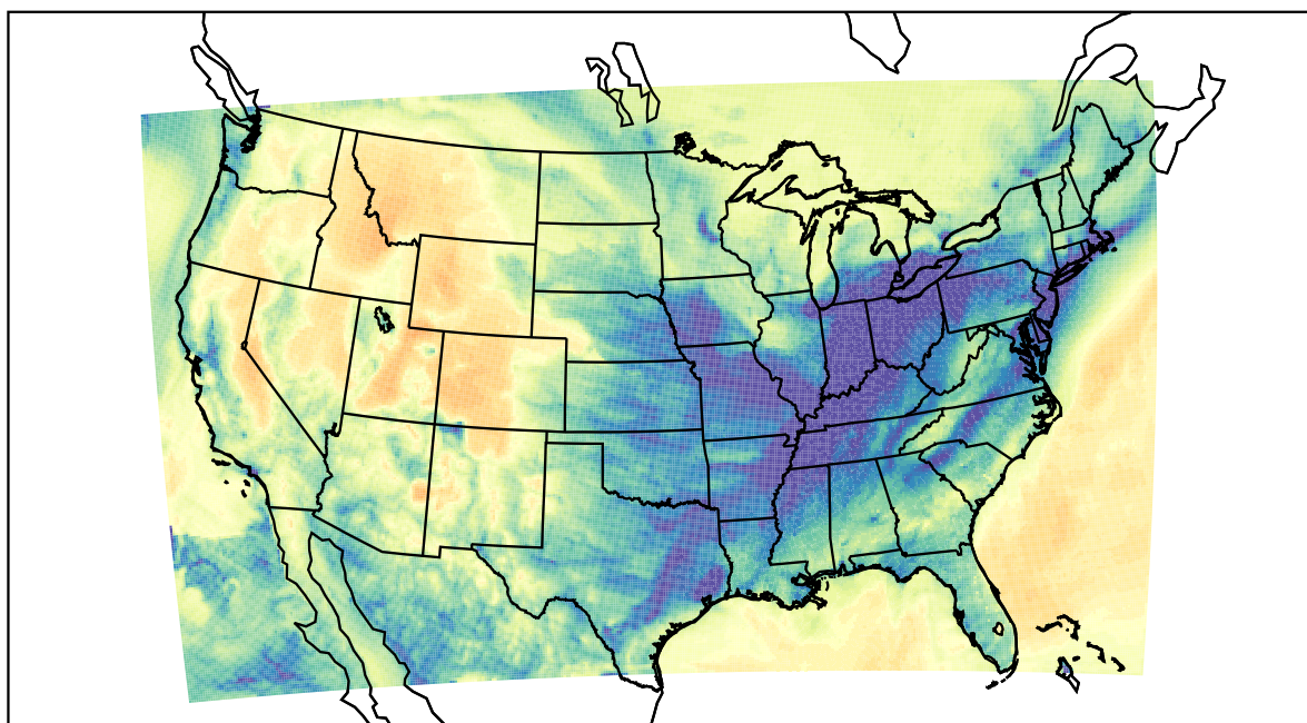
WRF (2022-01-13_10:00:00)
