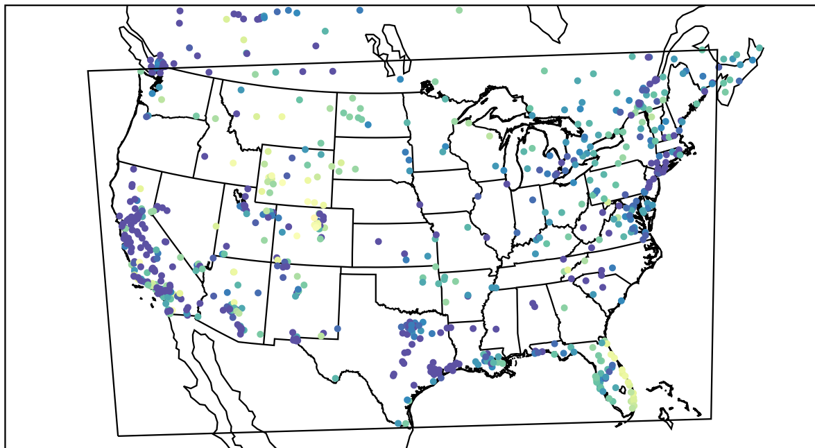
AirNOW (2022-01-12_08:00:00)
