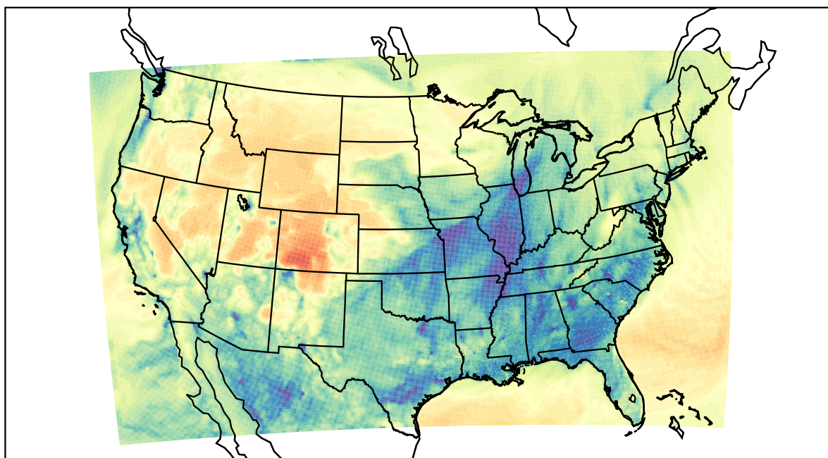
WRF (2022-01-12_04:00:00)
