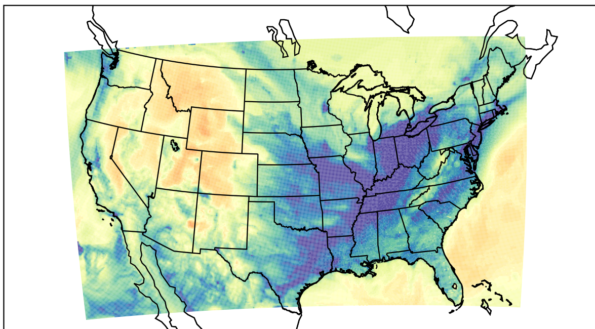
WRF (2022-01-13_14:00:00)
