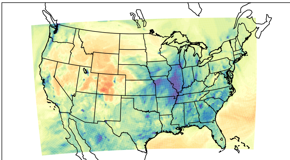
WRF (2022-01-12_01:00:00)
