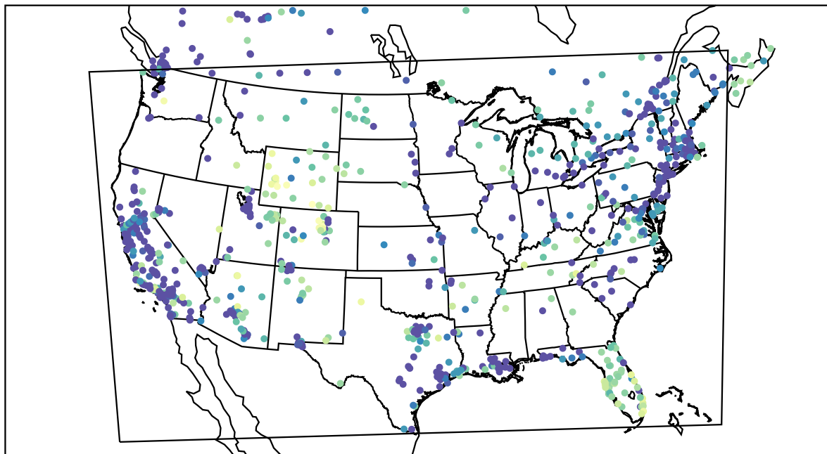
AirNOW (2022-01-13_01:00:00)
