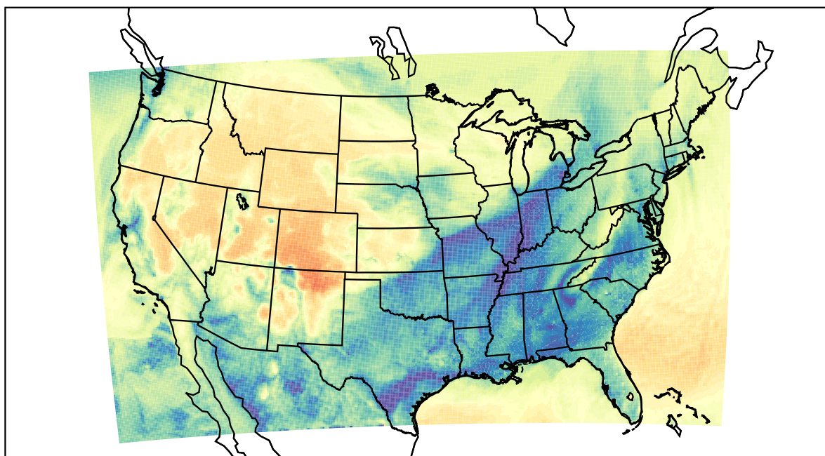
WRF (2022-01-12_11:00:00)
