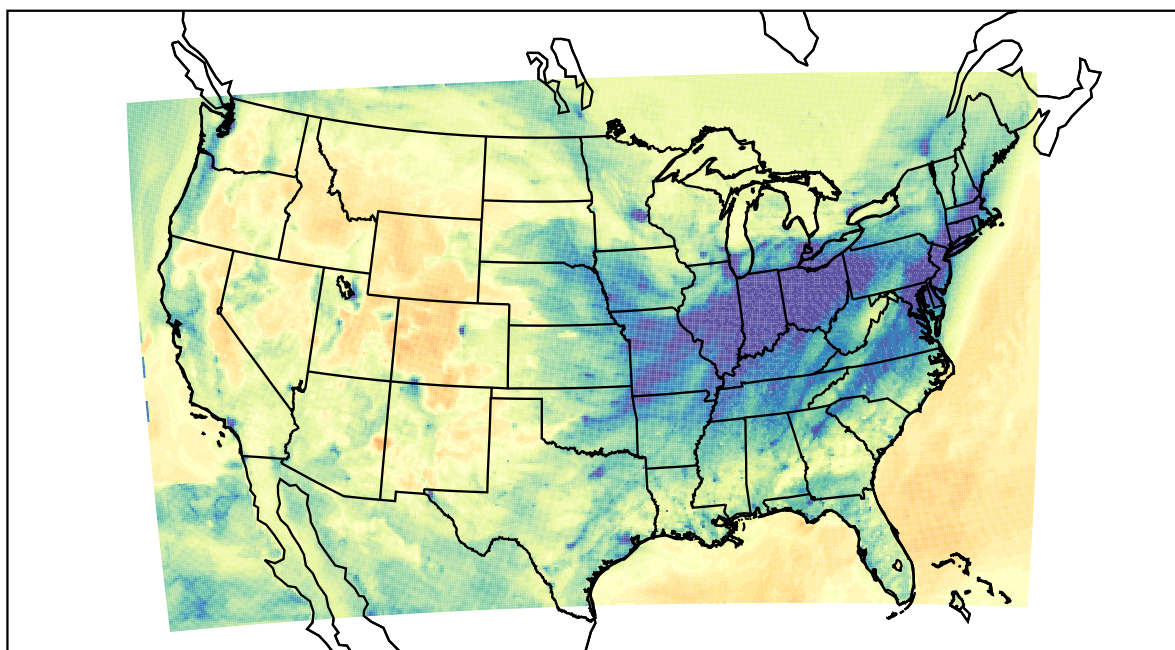
WRF (2022-01-13_00:00:00)
