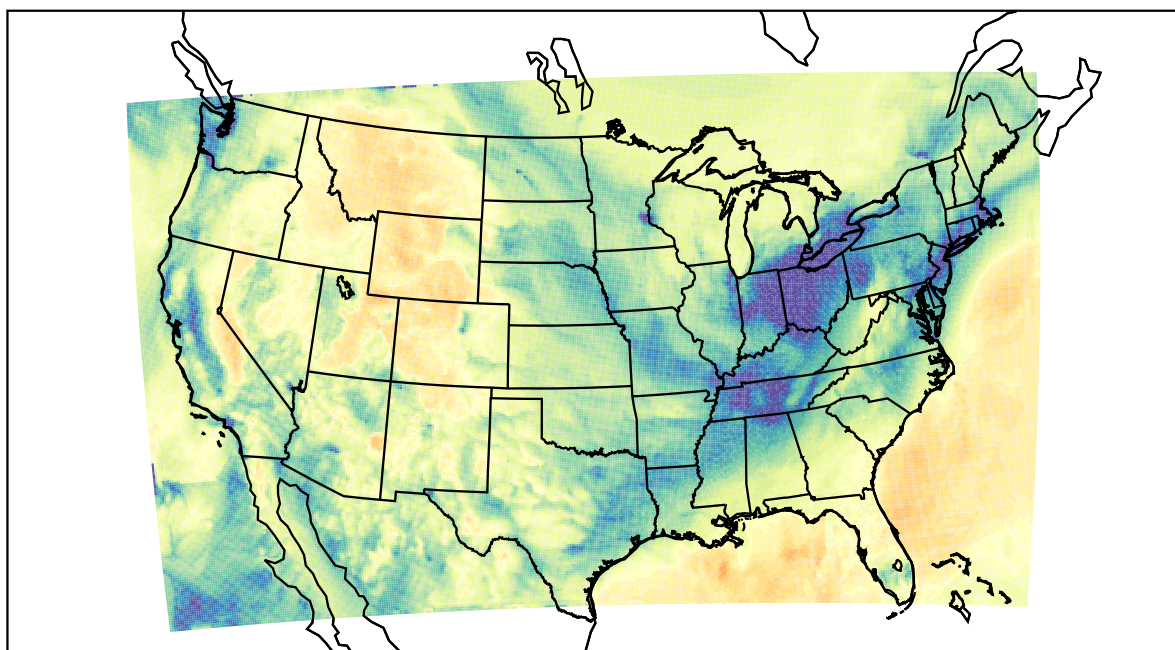
WRF (2022-01-13_18:00:00)
