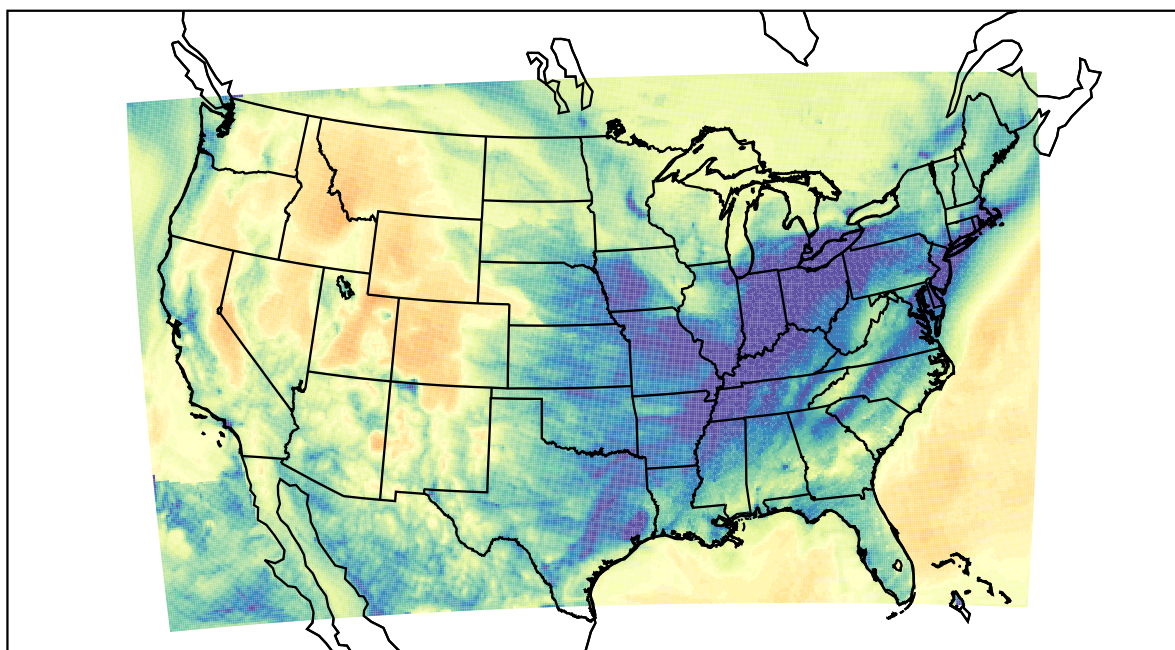
WRF (2022-01-13_09:00:00)
