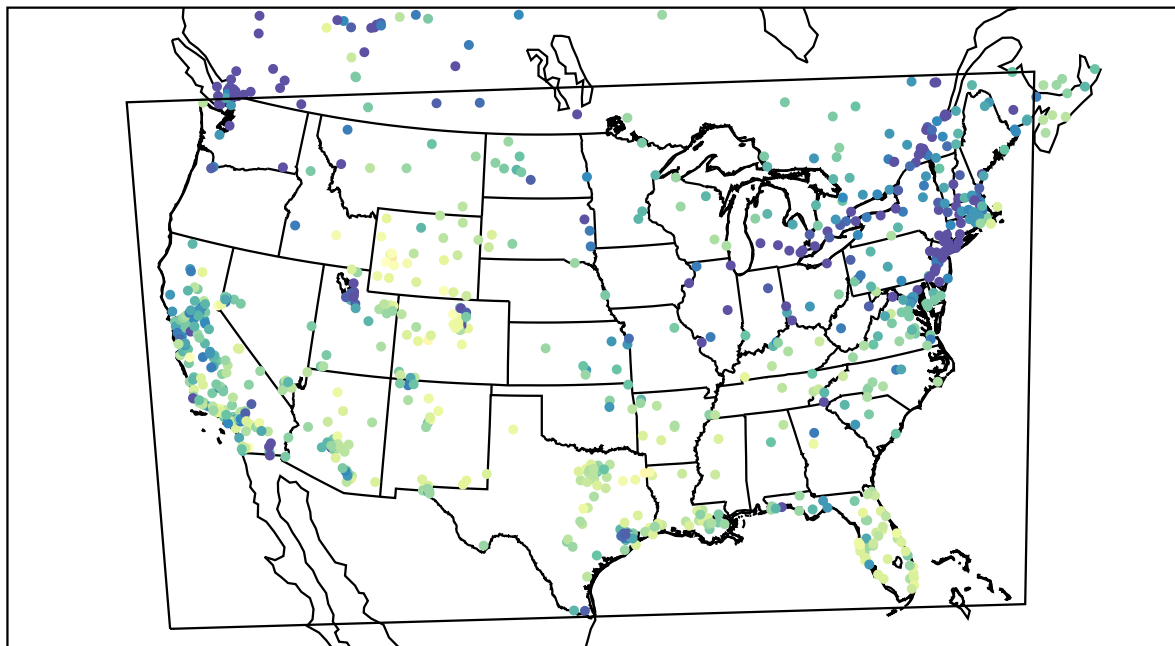
AirNOW (2022-01-12_22:00:00)
