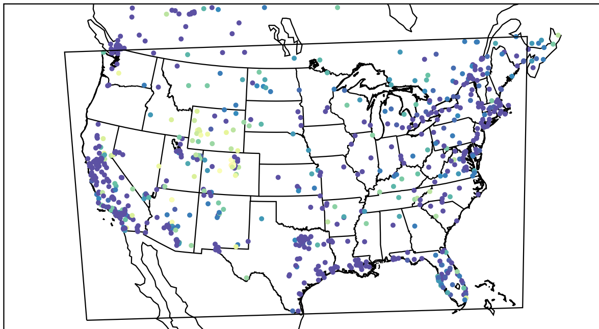
AirNOW (2022-01-13_09:00:00)
