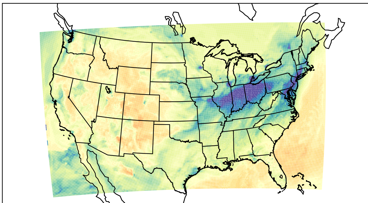
WRF (2022-01-12_21:00:00)
