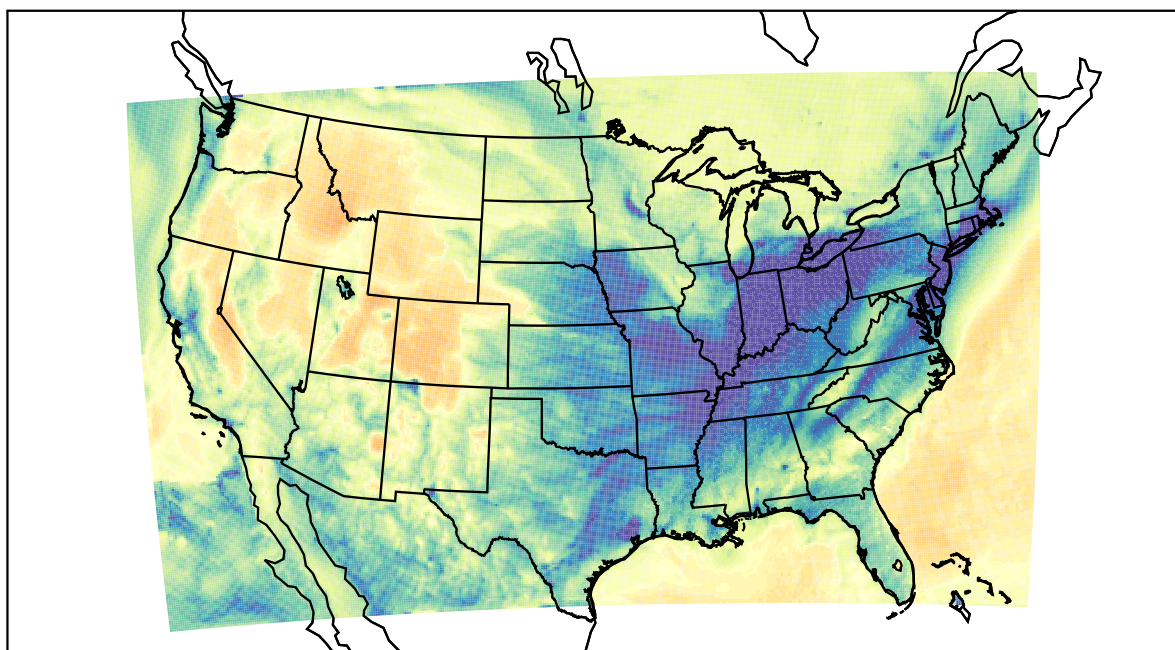
WRF (2022-01-13_07:00:00)
