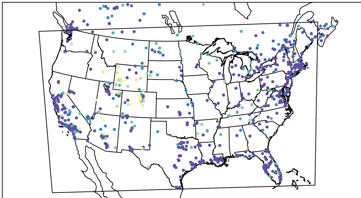
AirNOW (2022-01-13_12:00:00)
