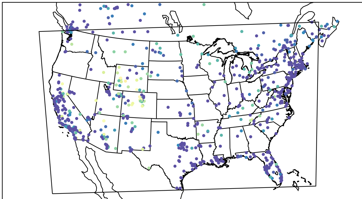
AirNOW (2022-01-13_13:00:00)
