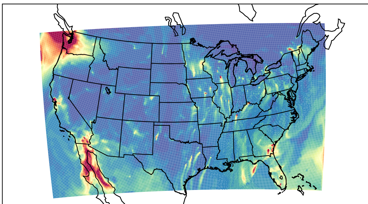
WRF 2022-01-21_06:00:00
