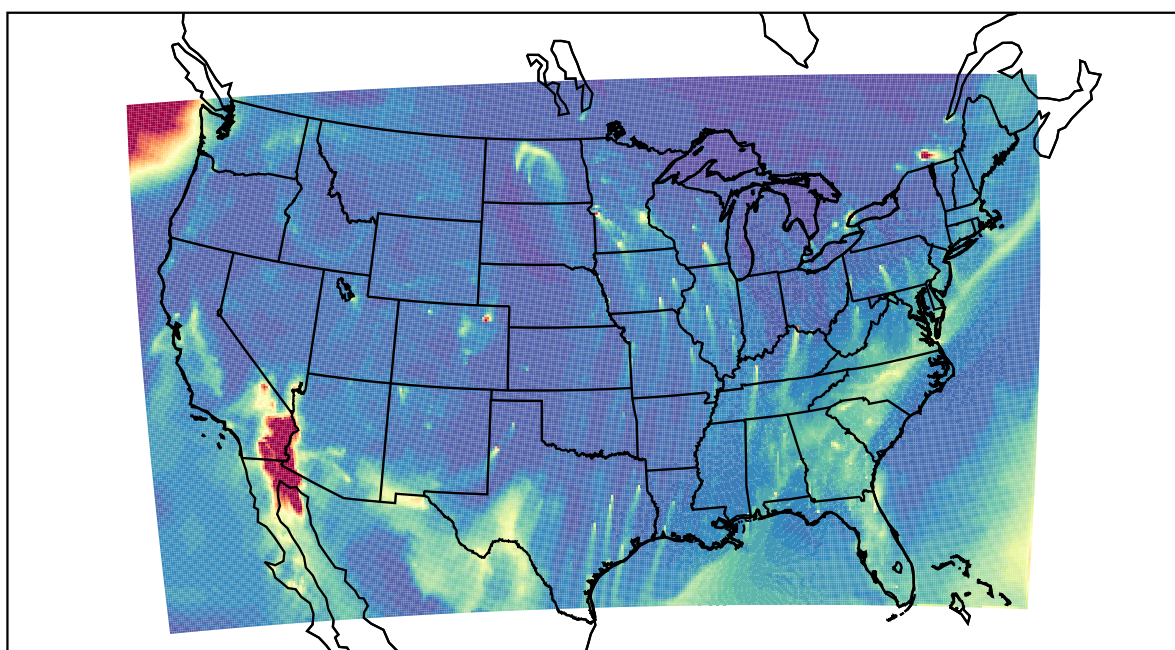
WRF 2022-01-20_16:00:00
