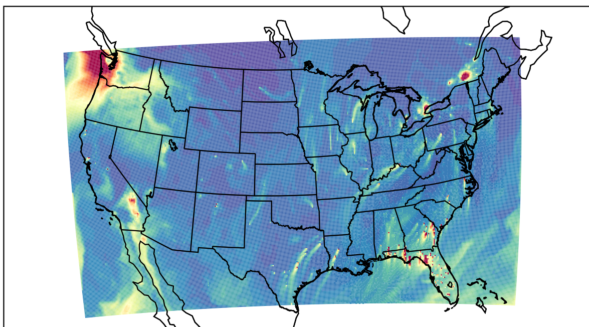
WRF 2022-01-21_21:00:00
