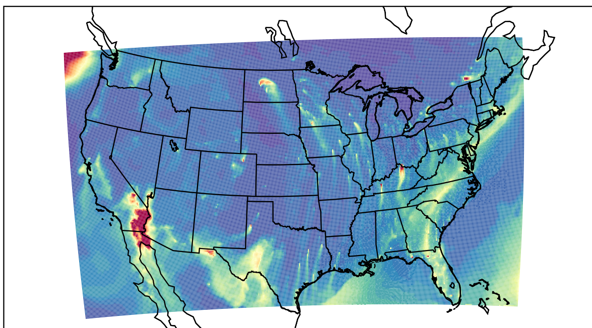
WRF 2022-01-20_13:00:00
