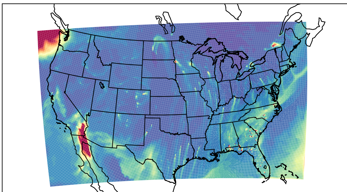
WRF 2022-01-20_19:00:00
