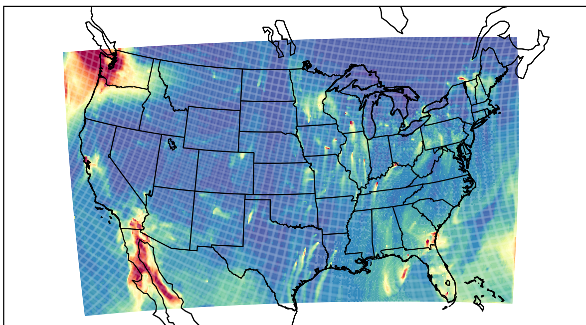
WRF 2022-01-21_07:00:00
