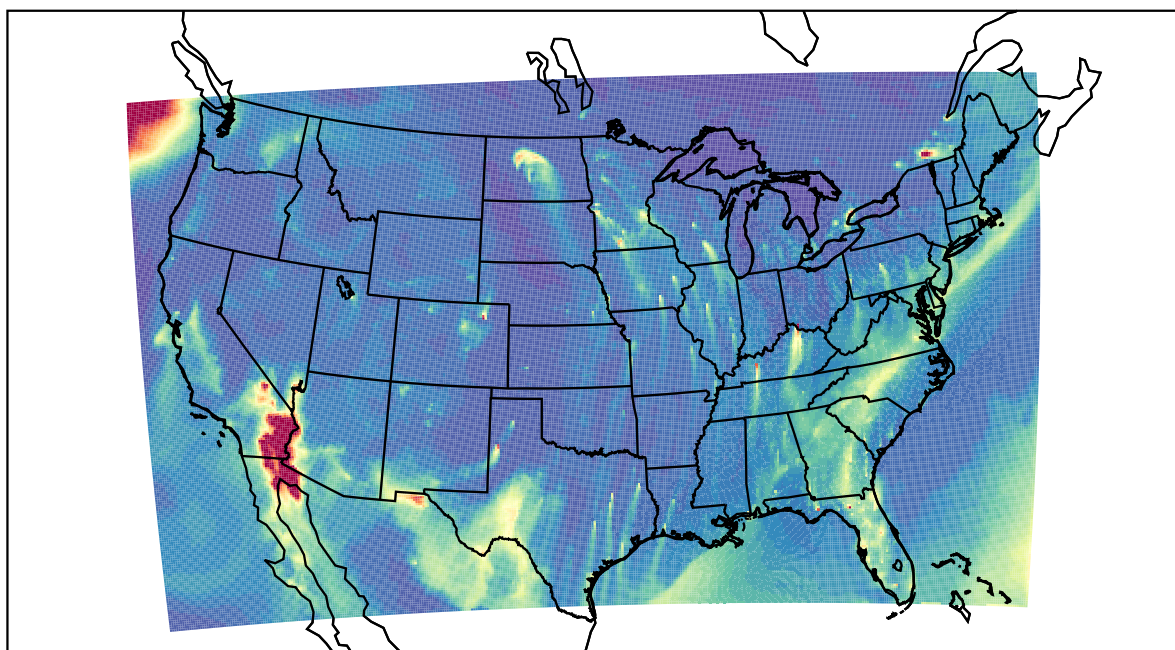
WRF 2022-01-20_14:00:00
