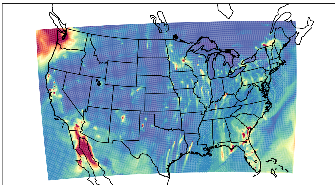
WRF 2022-01-21_03:00:00
