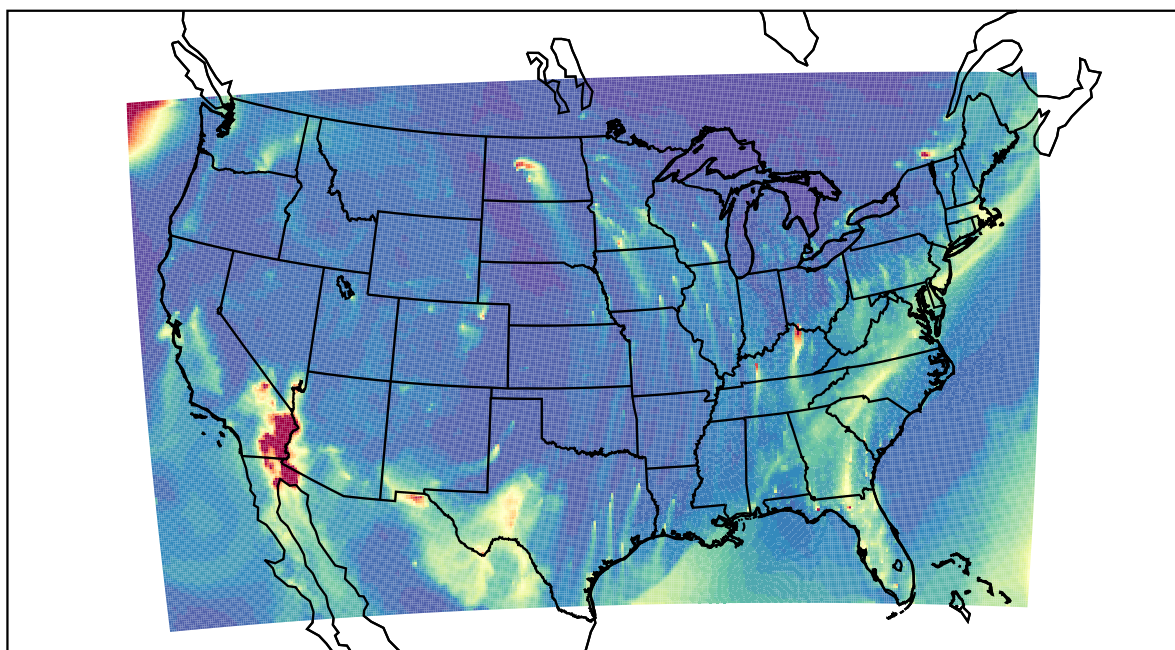
WRF 2022-01-20_12:00:00
