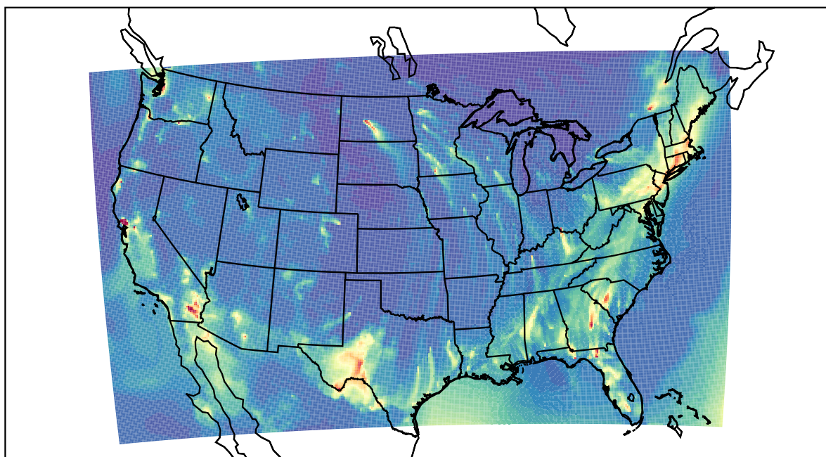
WRF 2022-01-20_05:00:00
