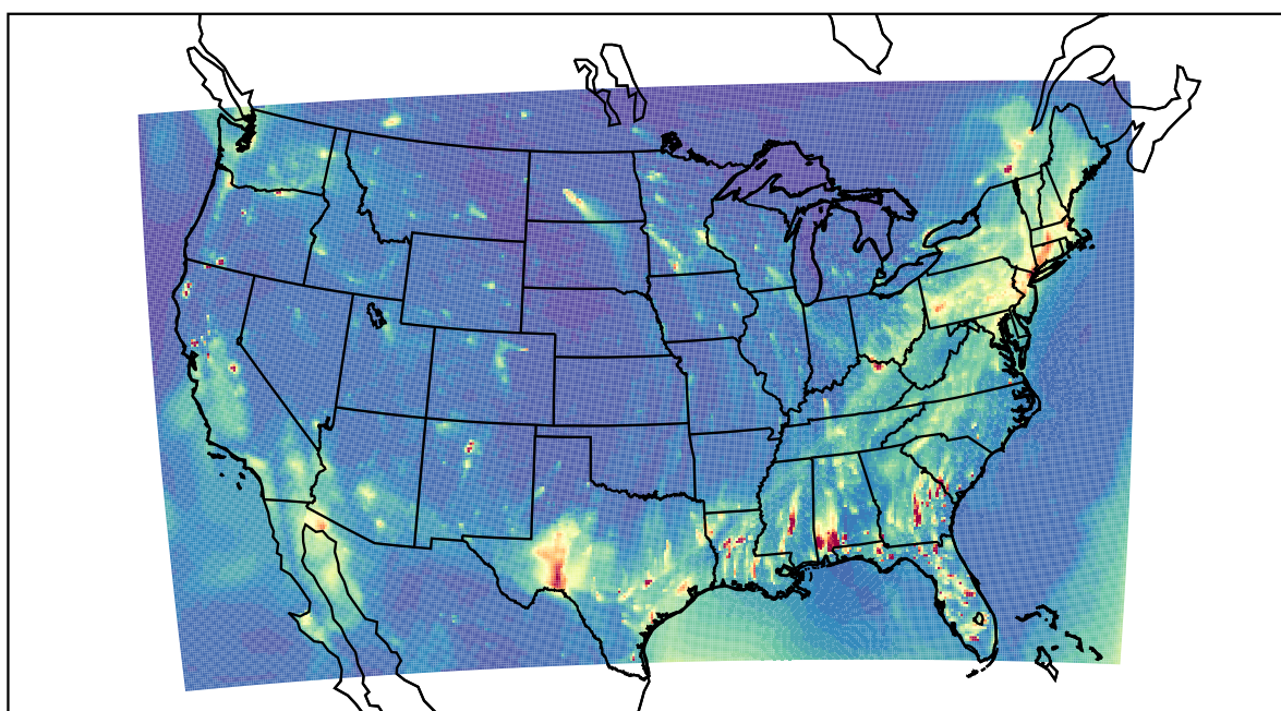
WRF 2022-01-20_01:00:00
