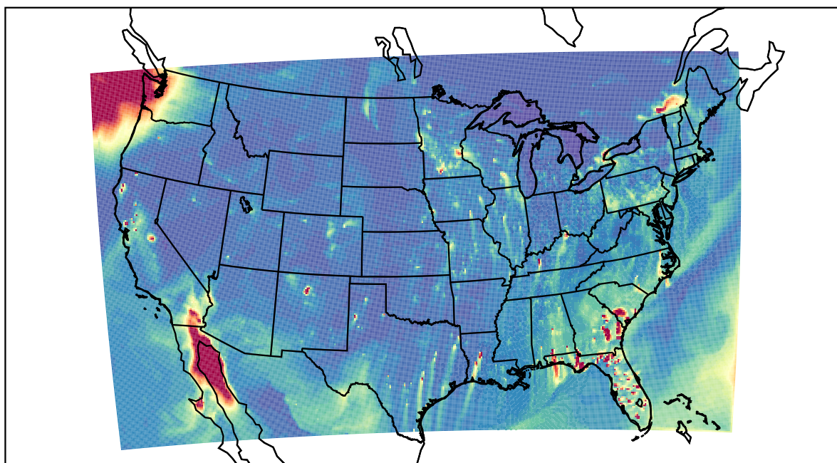
WRF 2022-01-21_00:00:00
