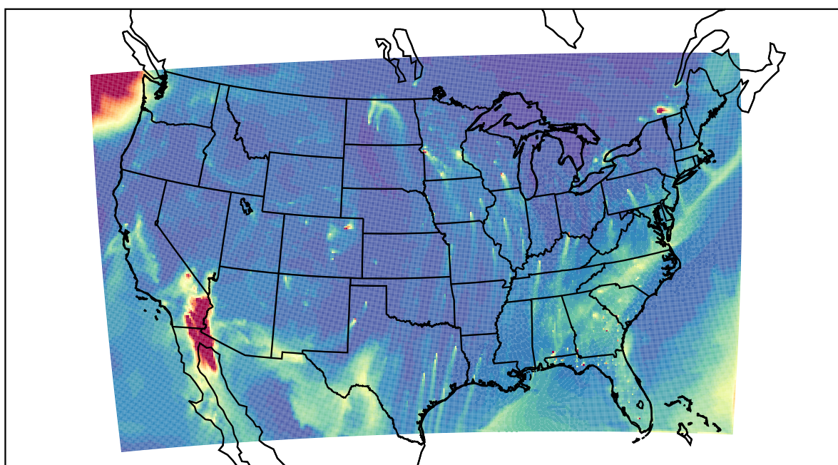
WRF 2022-01-20_17:00:00
