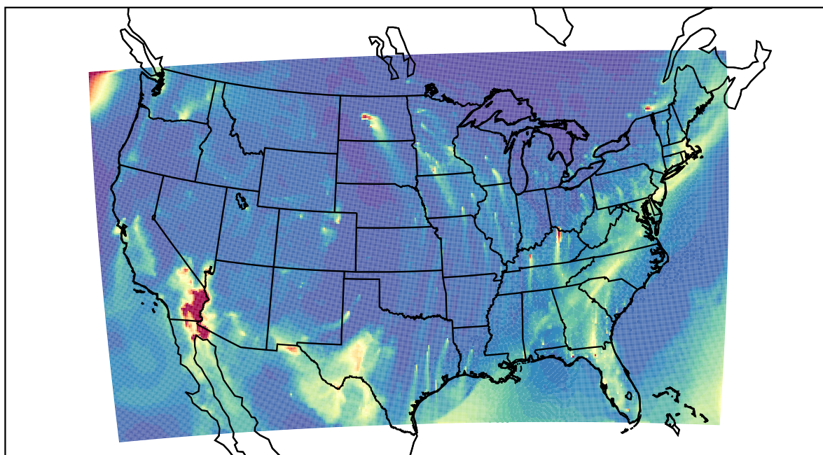
WRF 2022-01-20_11:00:00
