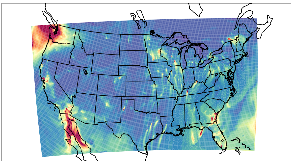
WRF 2022-01-21_05:00:00
