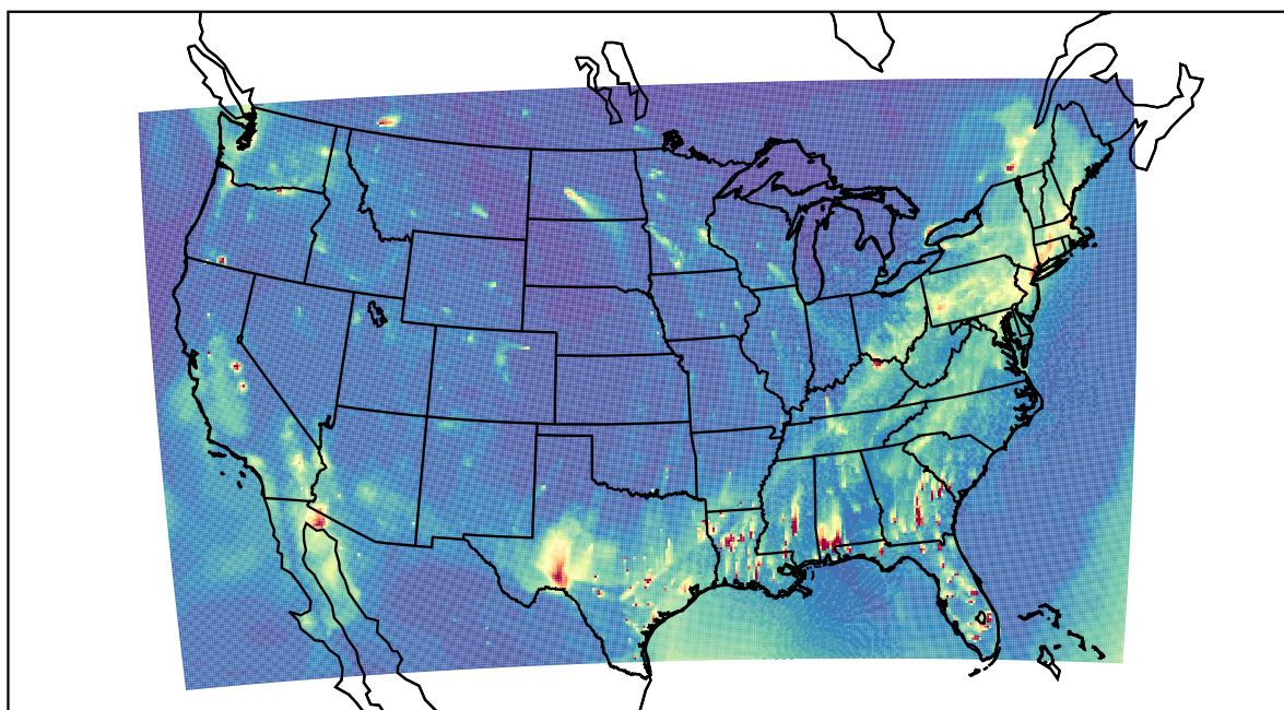
WRF 2022-01-20_00:00:00
