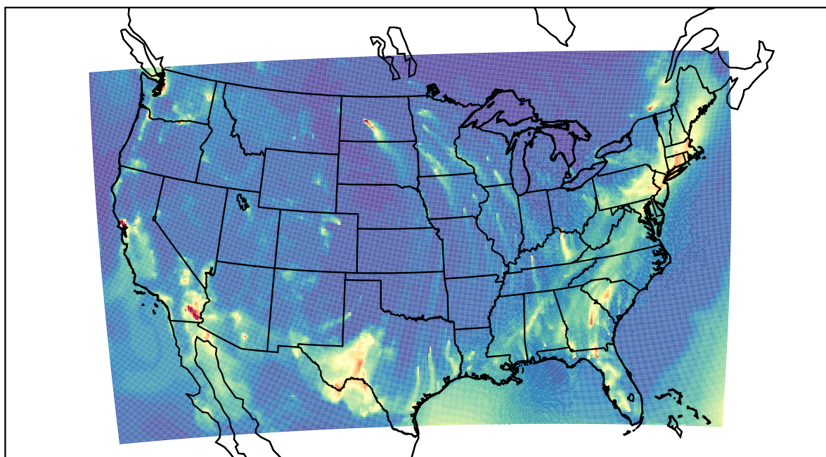
WRF 2022-01-20_06:00:00
