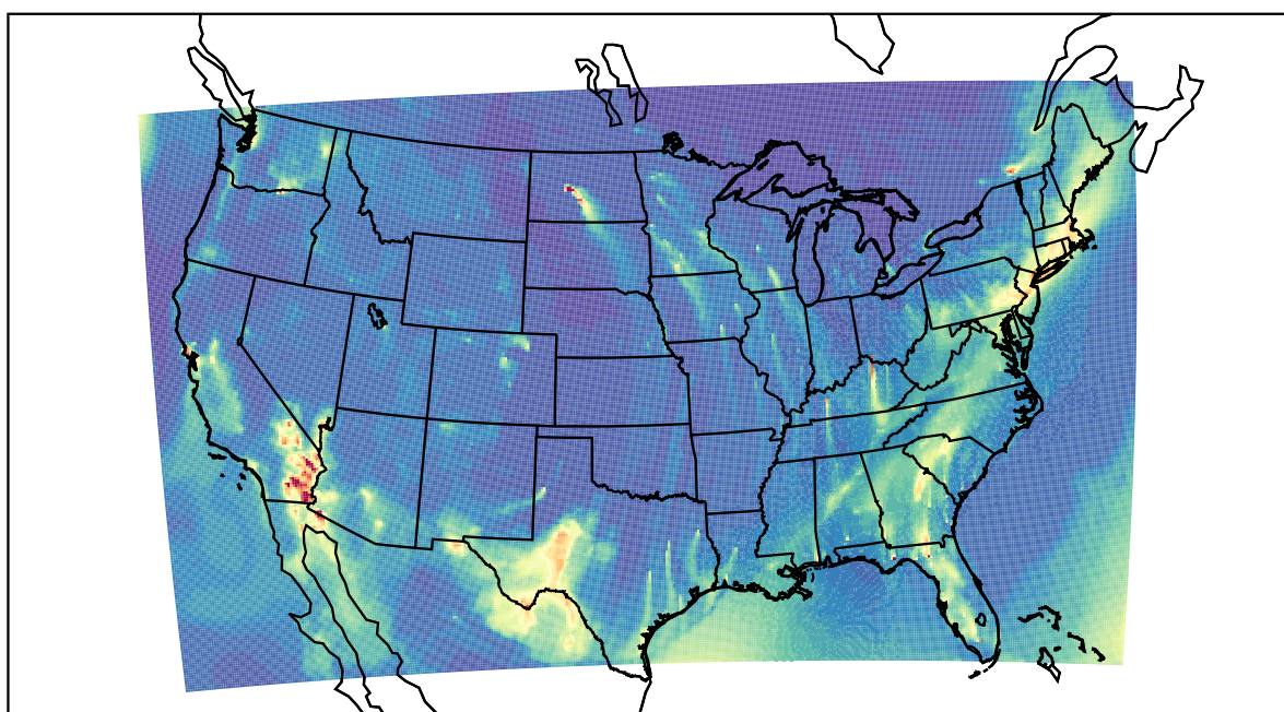
WRF 2022-01-20_08:00:00
