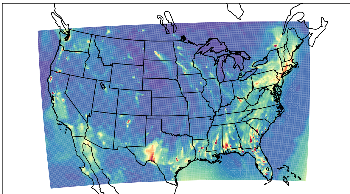
WRF 2022-01-20_02:00:00
