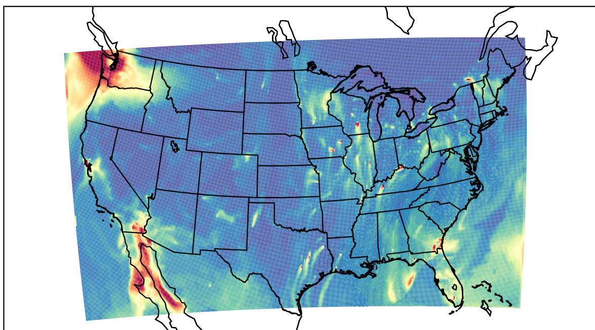
WRF 2022-01-21_08:00:00
