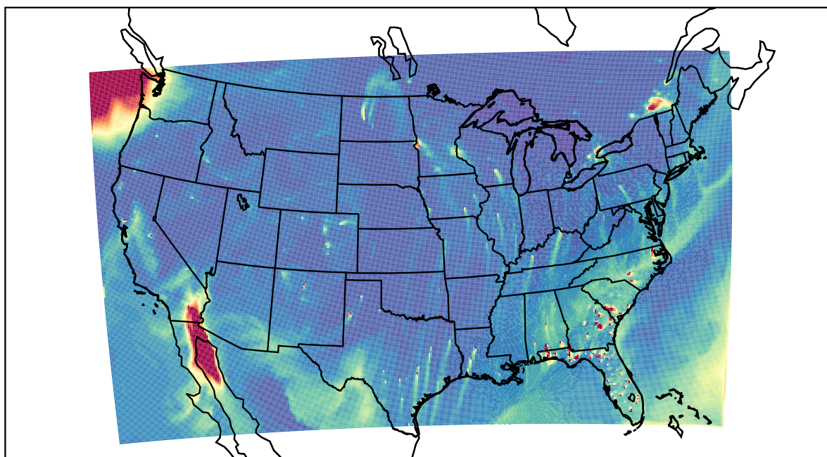
WRF 2022-01-20_21:00:00
