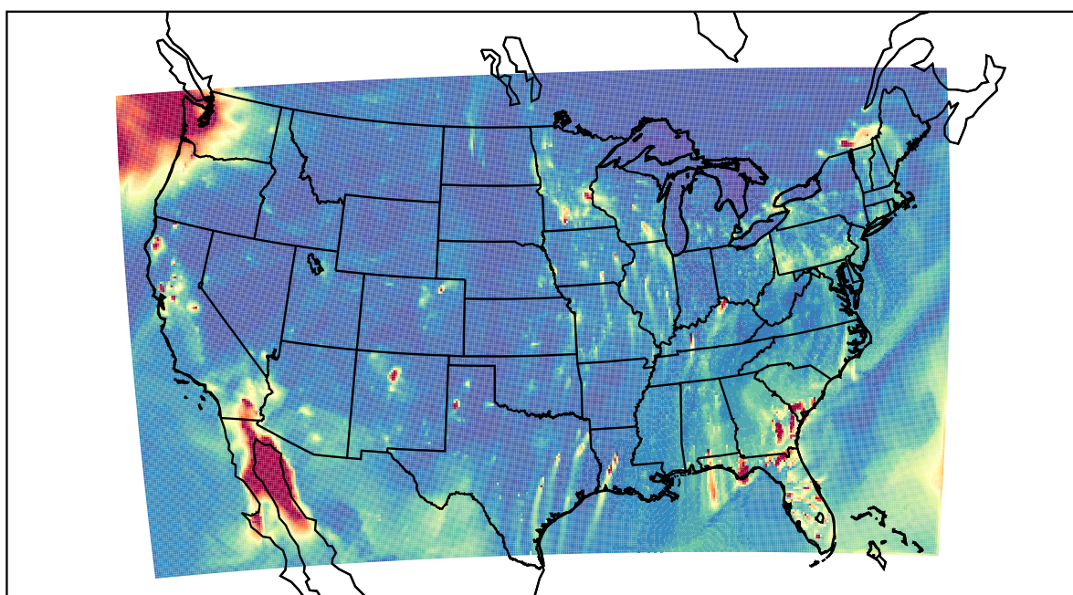
WRF 2022-01-21_02:00:00
