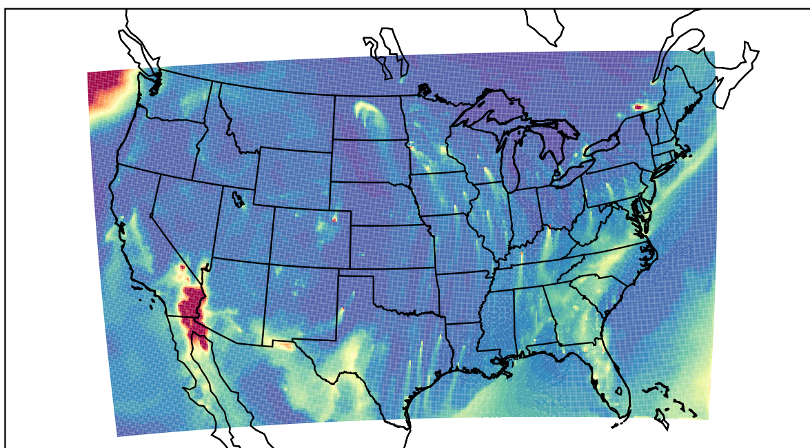
WRF 2022-01-20_15:00:00
