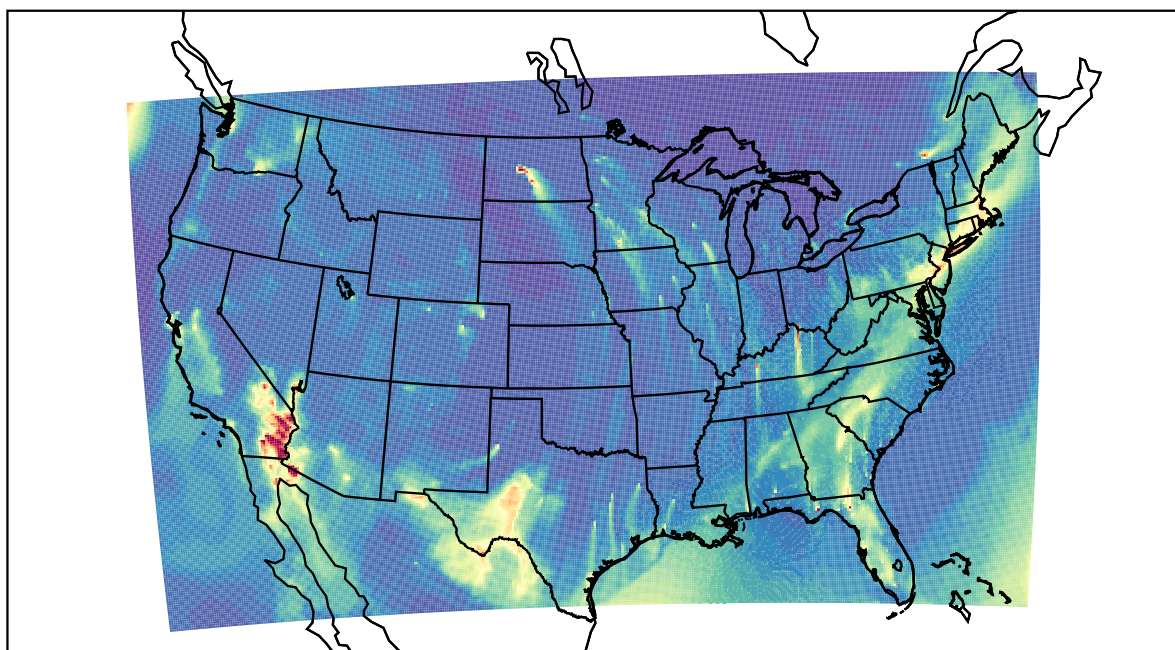
WRF 2022-01-20_09:00:00
