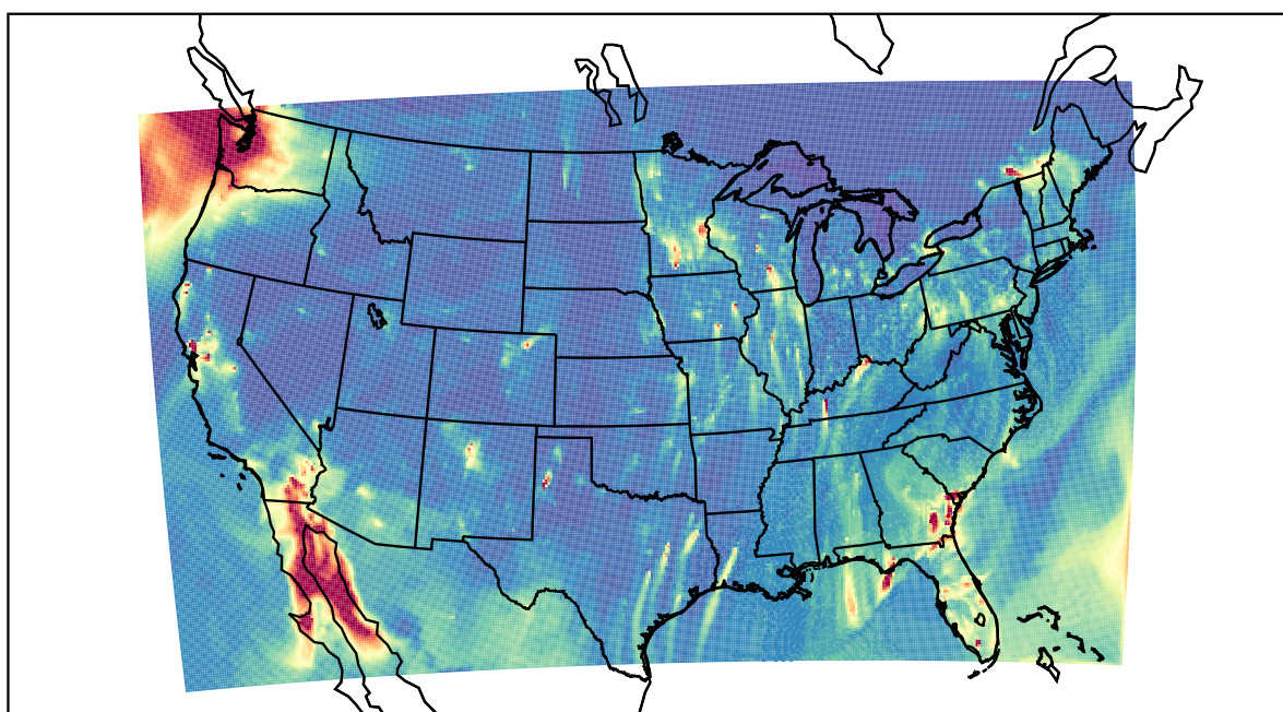
WRF 2022-01-21_04:00:00
