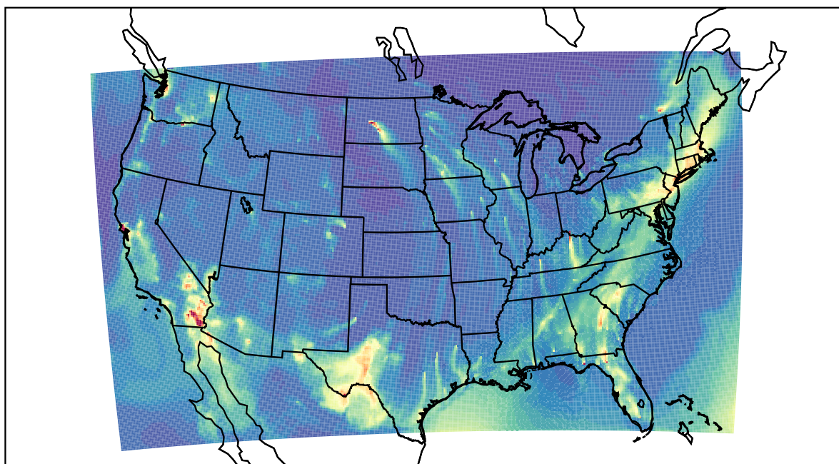
WRF 2022-01-20_07:00:00
