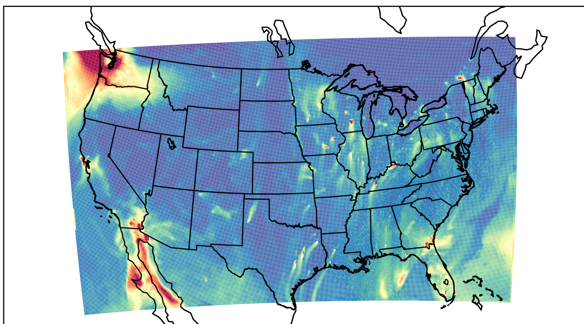
WRF 2022-01-21_09:00:00
