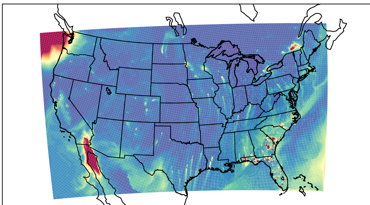
WRF 2022-01-20_22:00:00
