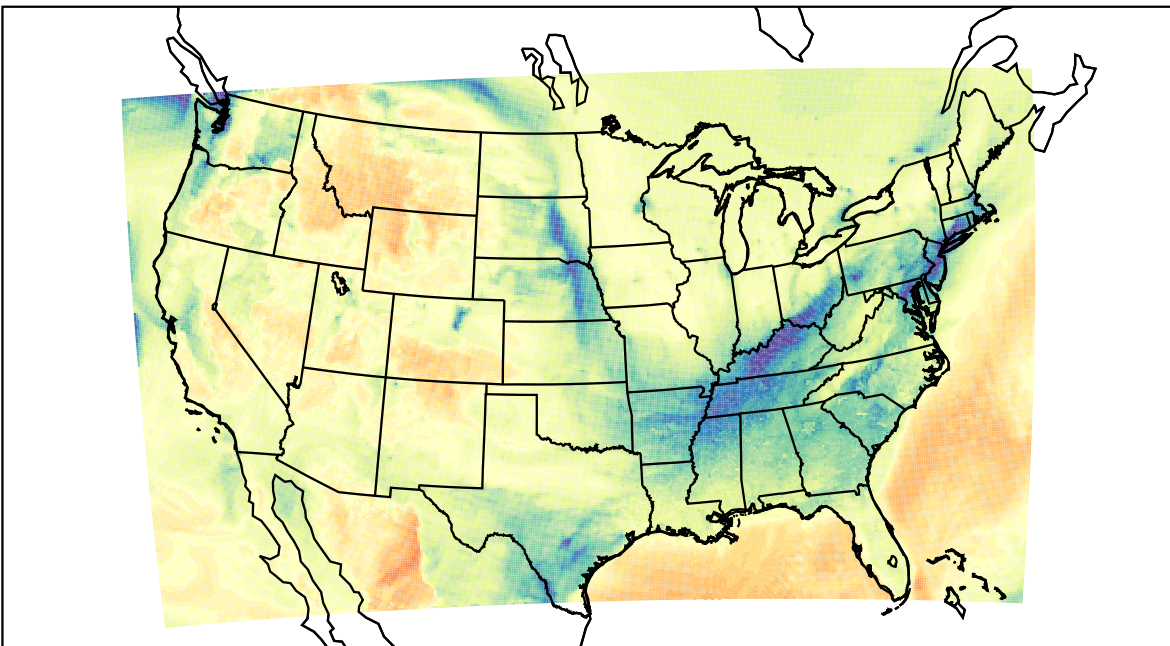
WRF (2022-01-23_22:00:00)
