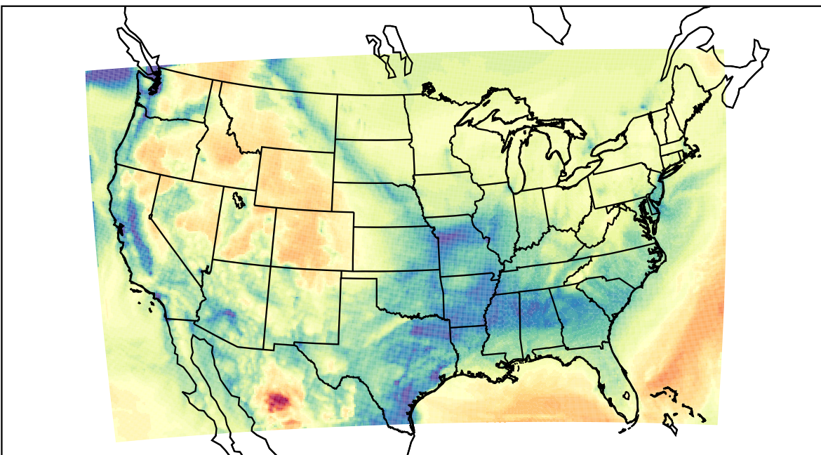
WRF (2022-01-24_17:00:00)
