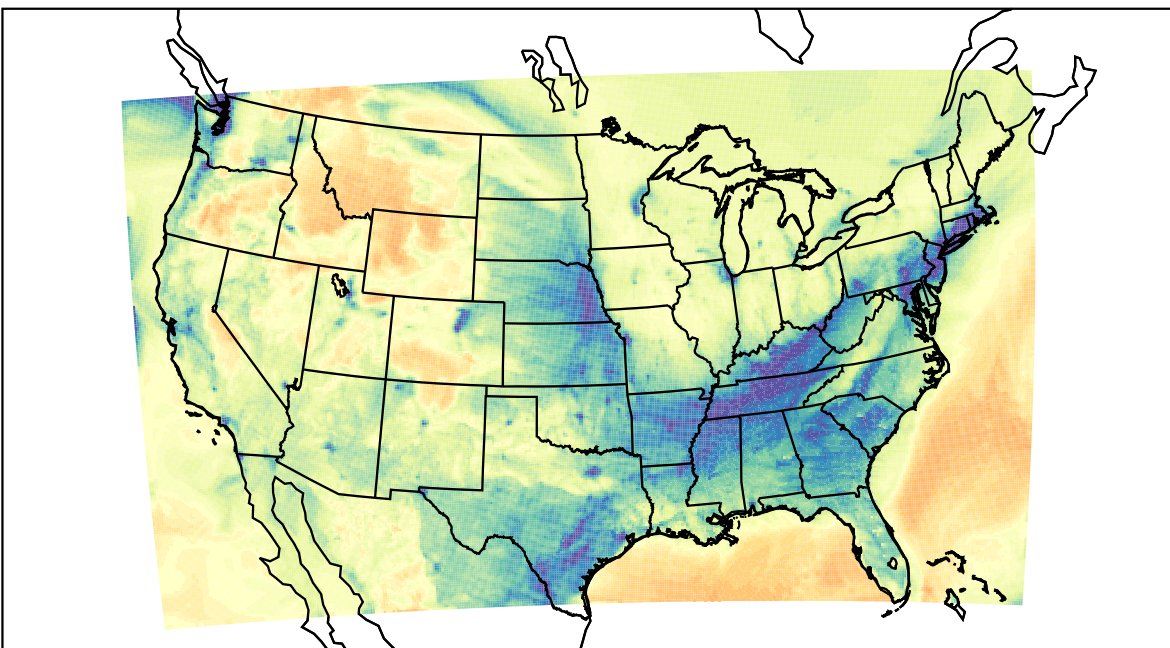
WRF (2022-01-24_01:00:00)
