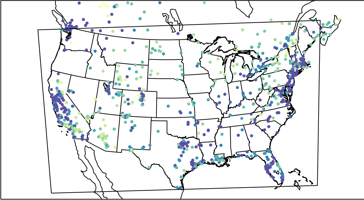
AirNOW (2022-01-23_03:00:00)
