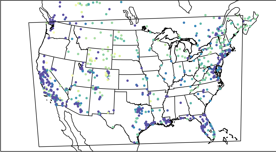
AirNOW (2022-01-24_08:00:00)
