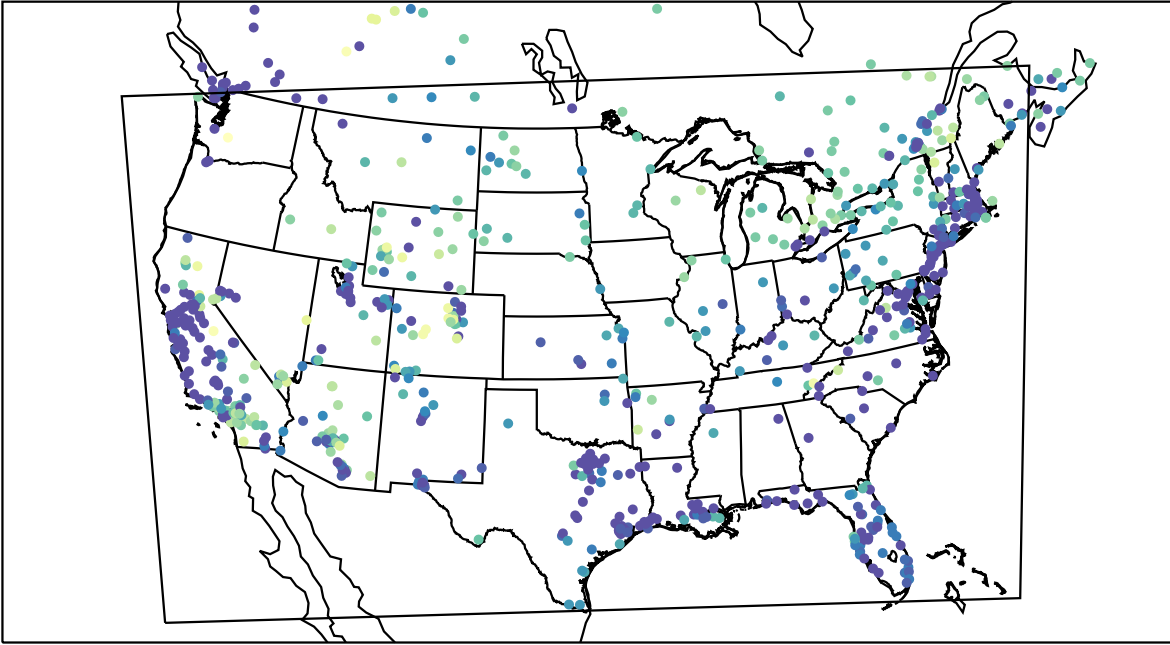
AirNOW (2022-01-23_10:00:00)
