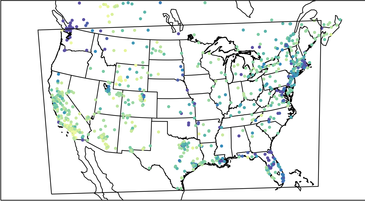
AirNOW (2022-01-24_00:00:00)
