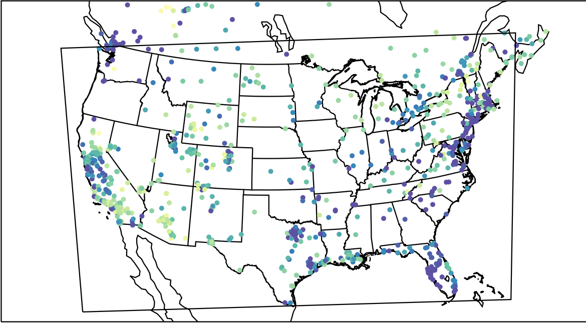
AirNOW (2022-01-23_01:00:00)
