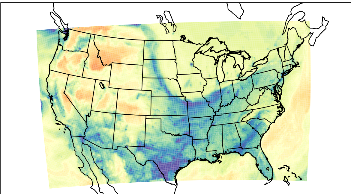
WRF (2022-01-23_14:00:00)
