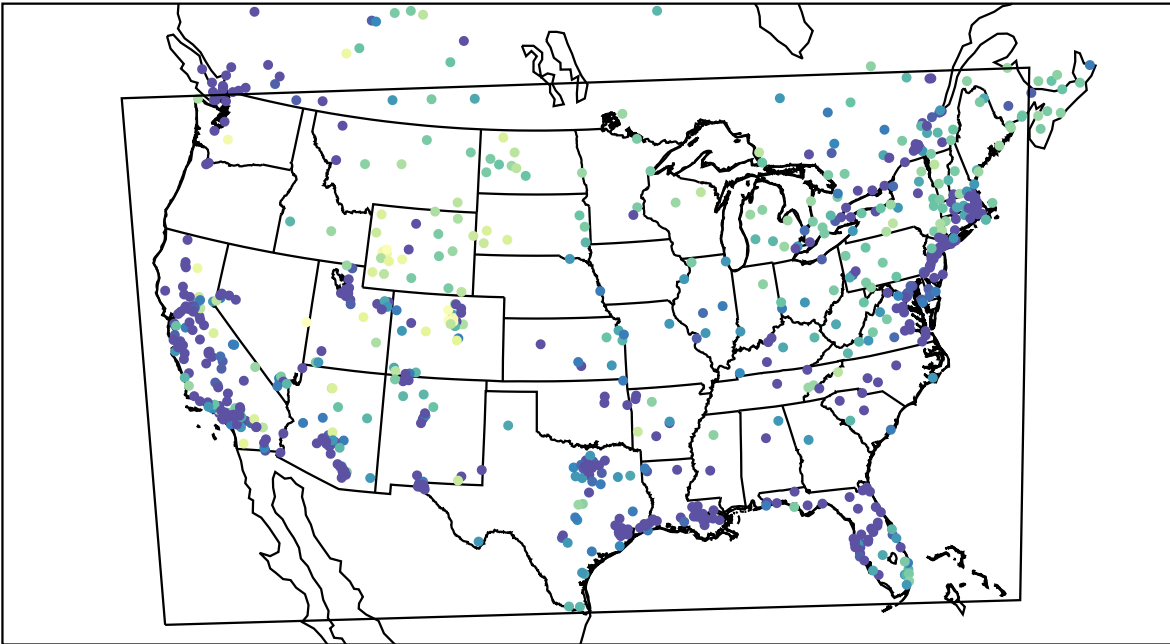
AirNOW (2022-01-24_10:00:00)
