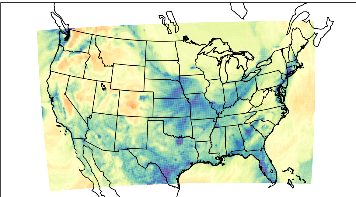
WRF (2022-01-23_05:00:00)
