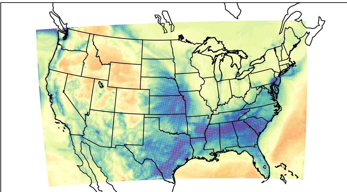
WRF (2022-01-24_08:00:00)
