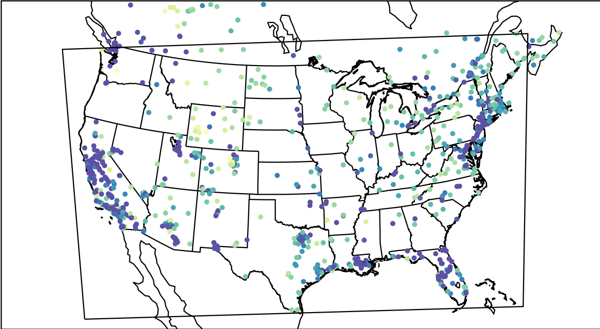
AirNOW (2022-01-24_04:00:00)
