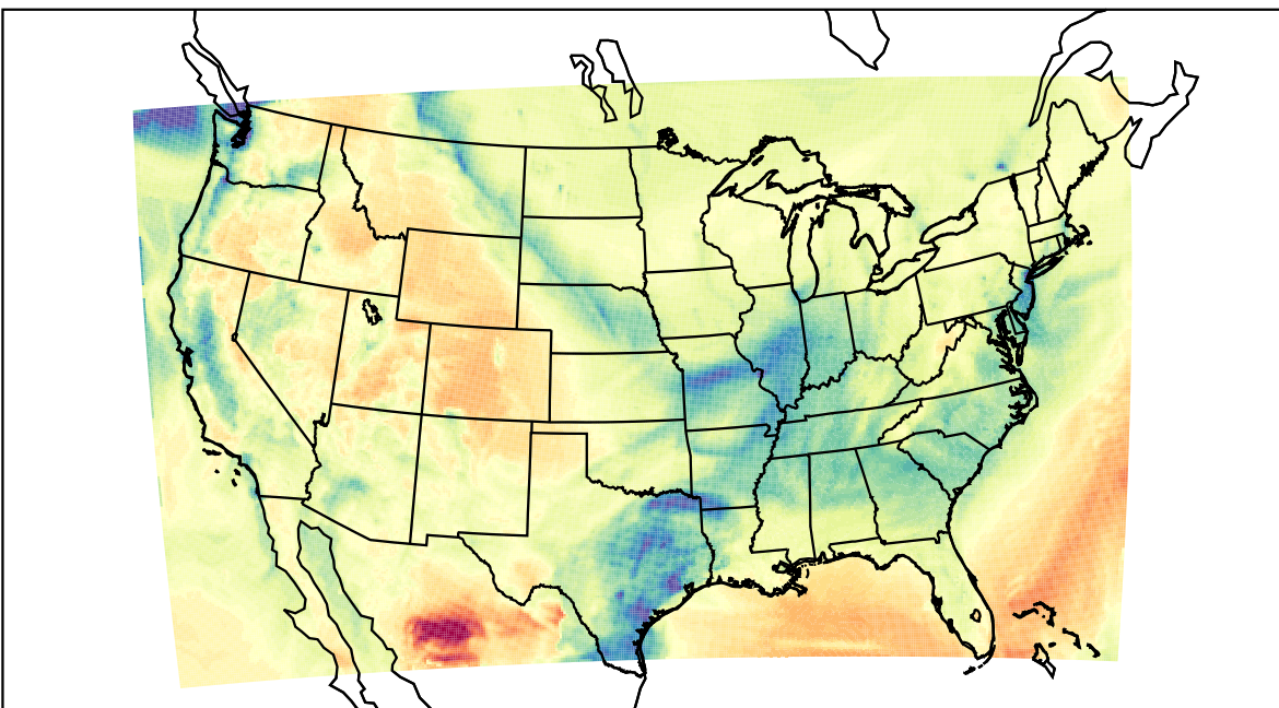
WRF (2022-01-24_20:00:00)
