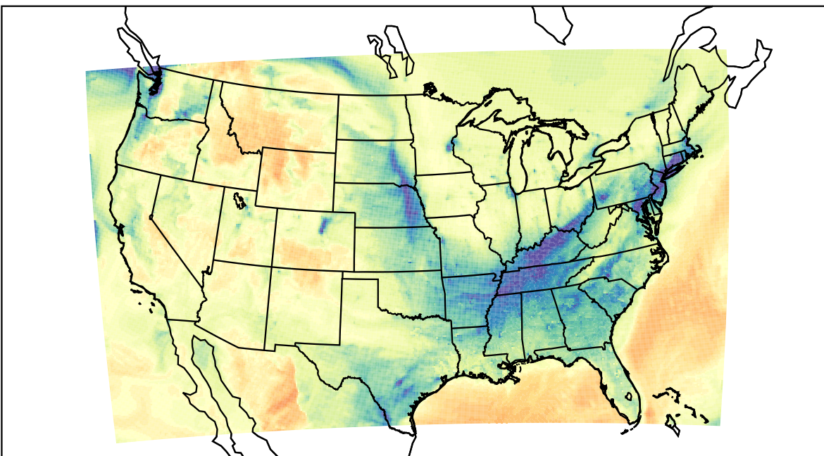
WRF (2022-01-23_23:00:00)
