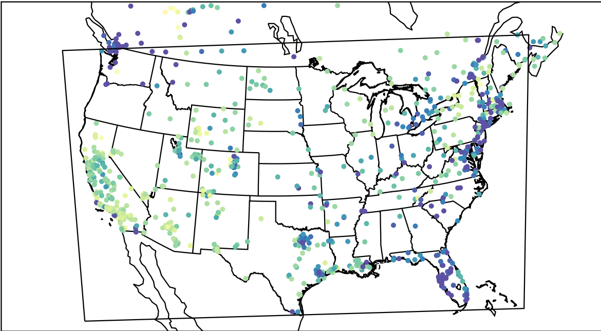
AirNOW (2022-01-23_00:00:00)
