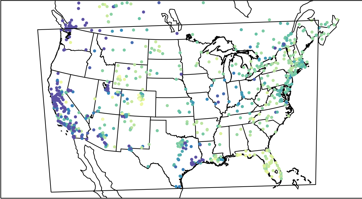
AirNOW (2022-01-24_17:00:00)
