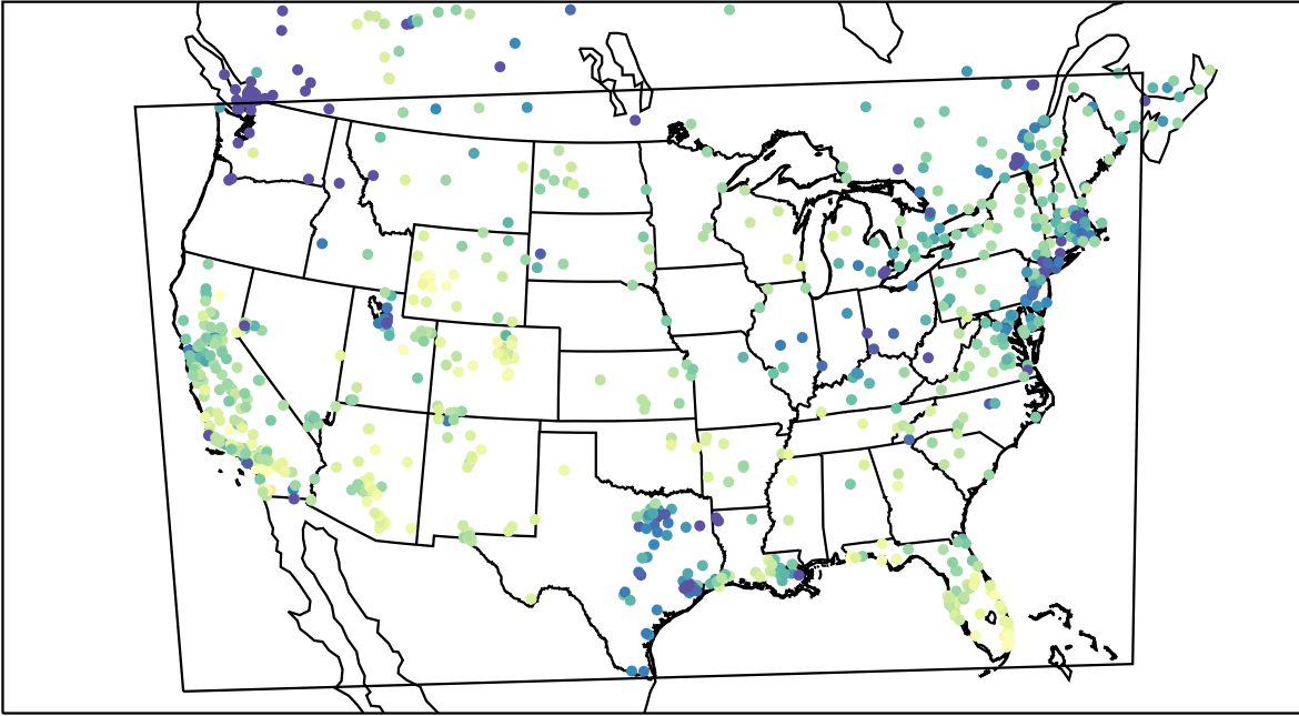
AirNOW (2022-01-24_22:00:00)
