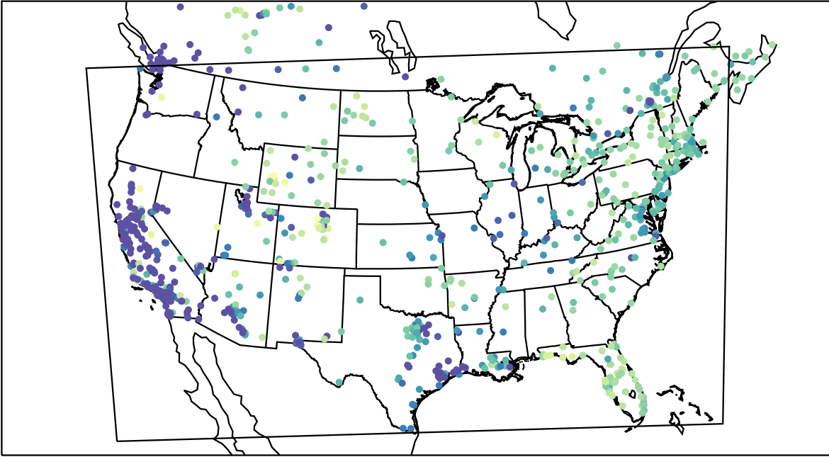
AirNOW (2022-01-24_16:00:00)
