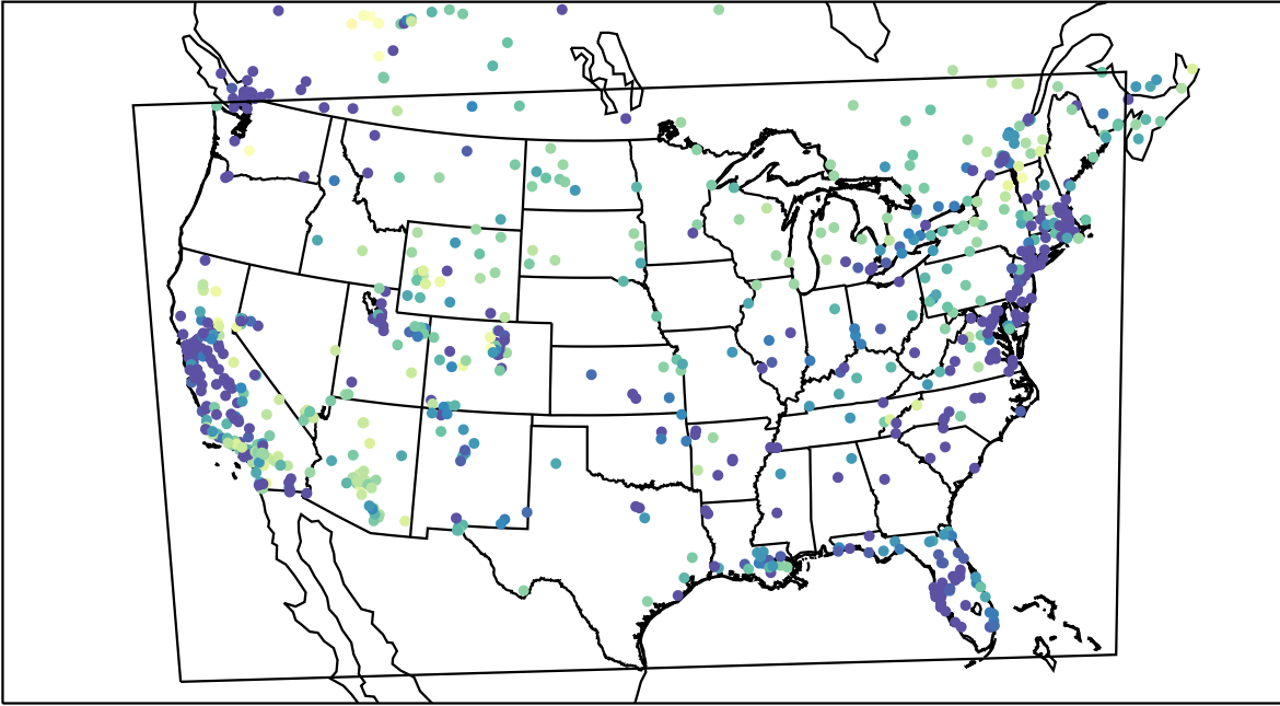
AirNOW (2022-01-23_04:00:00)
