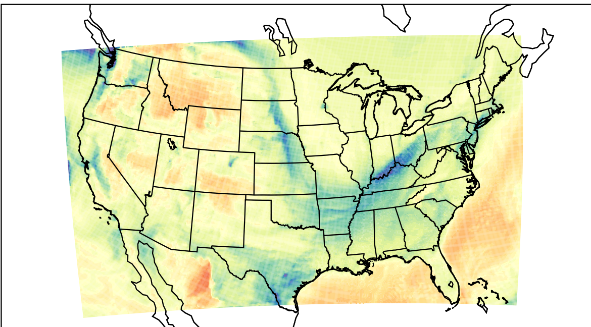
WRF (2022-01-23_20:00:00)
