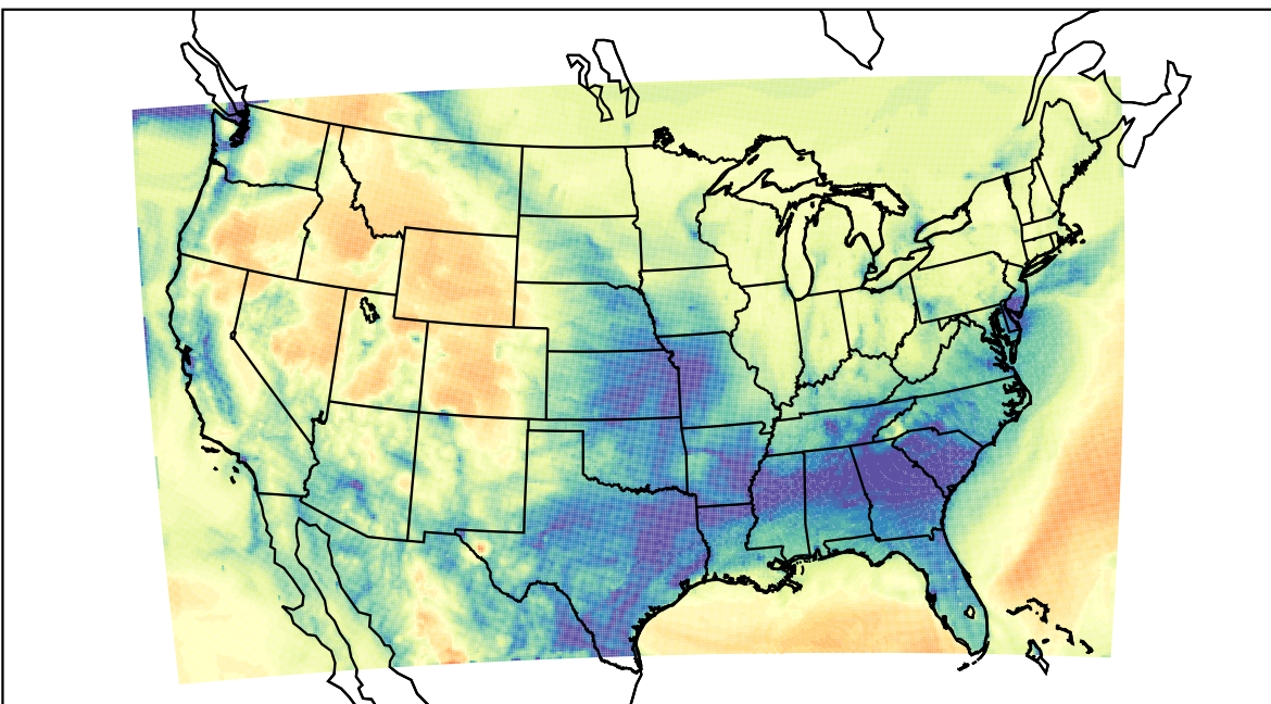
WRF (2022-01-24_12:00:00)
