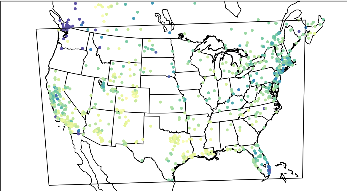
AirNOW (2022-01-23_21:00:00)
