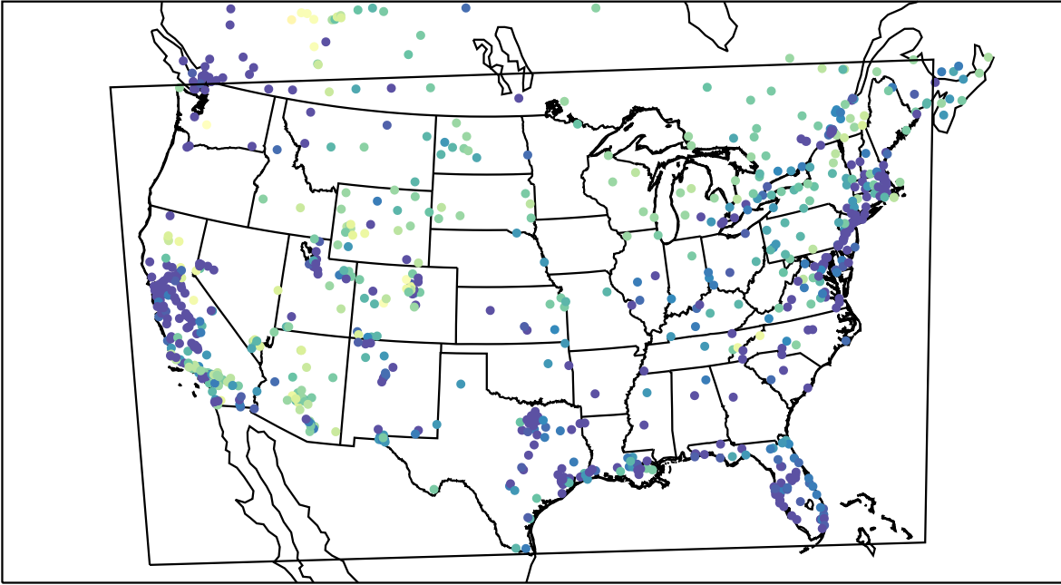
AirNOW (2022-01-23_06:00:00)
