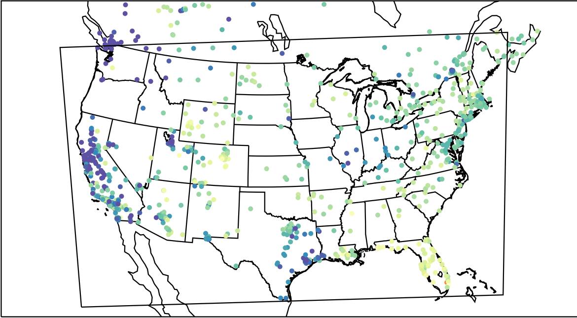
AirNOW (2022-01-24_18:00:00)
