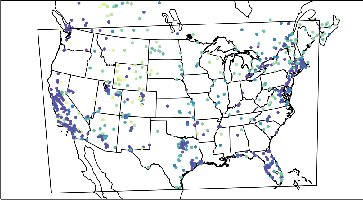
AirNOW (2022-01-24_07:00:00)
