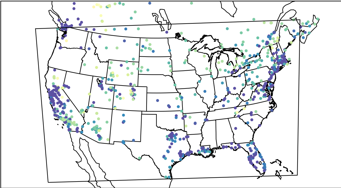
AirNOW (2022-01-23_08:00:00)
