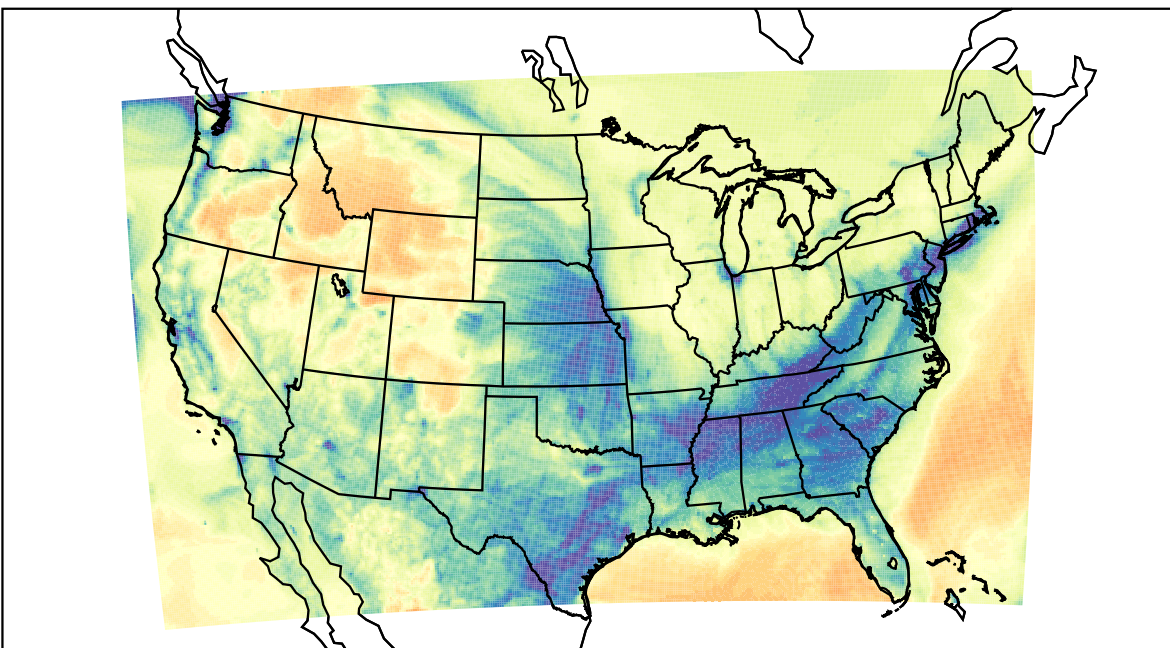
WRF (2022-01-24_04:00:00)
