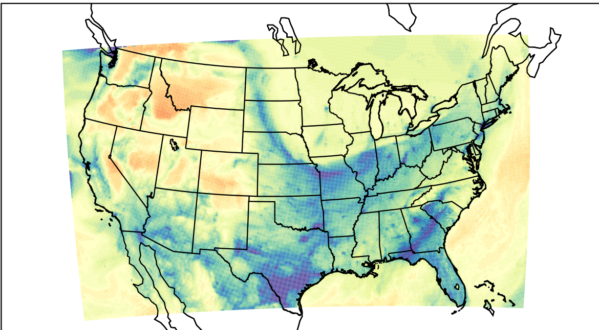
WRF (2022-01-23_13:00:00)
