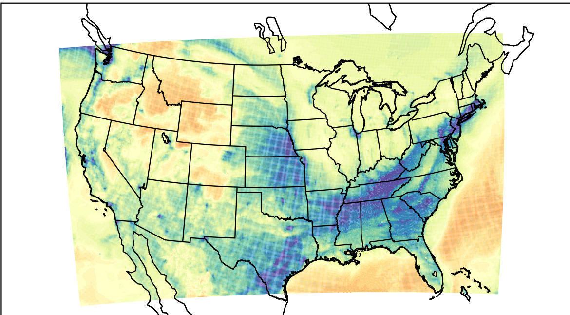
WRF (2022-01-24_03:00:00)
