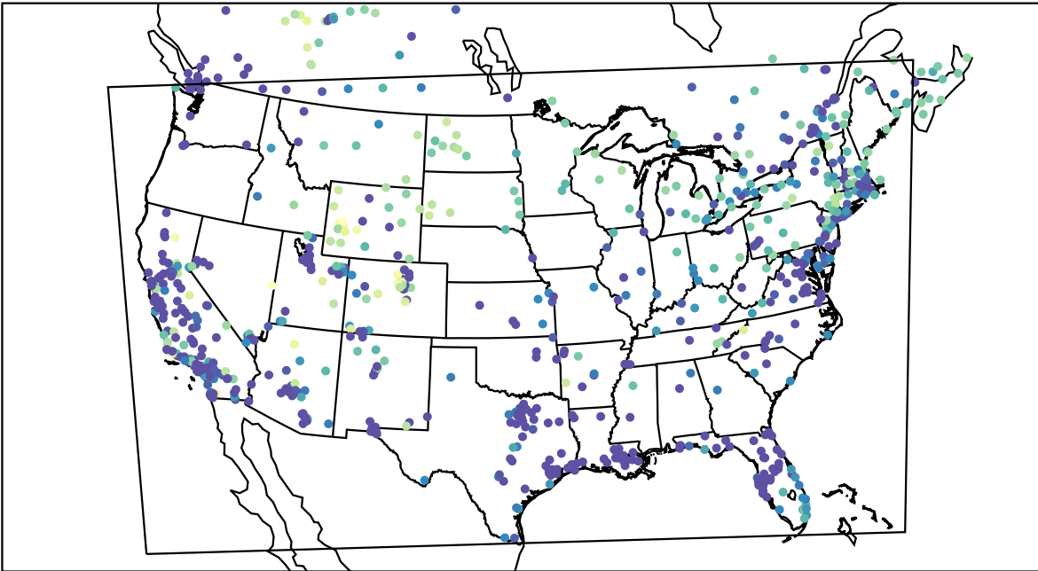
AirNOW (2022-01-24_13:00:00)
