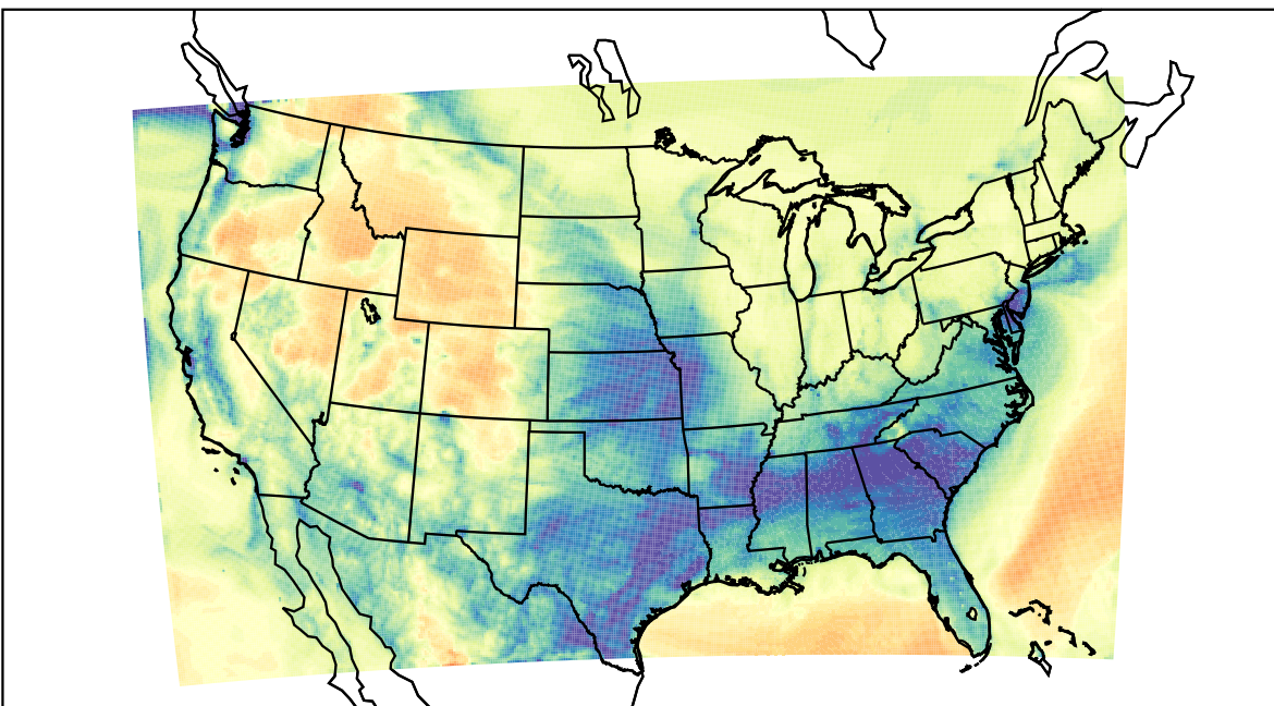
WRF (2022-01-24_10:00:00)
