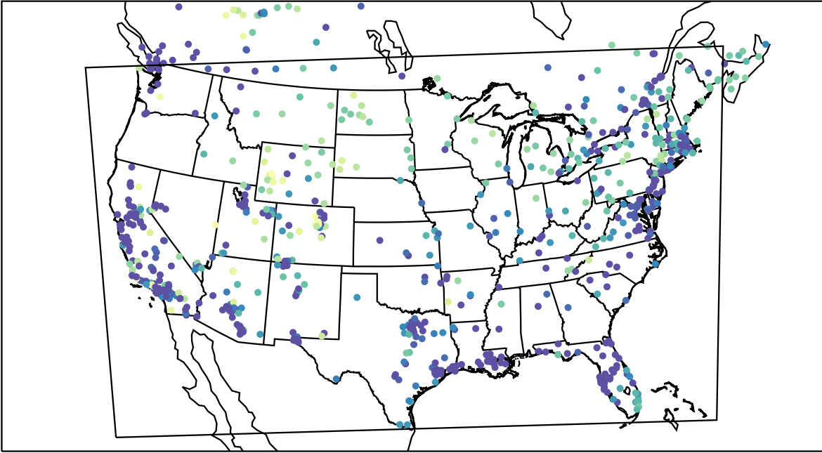
AirNOW (2022-01-24_11:00:00)
