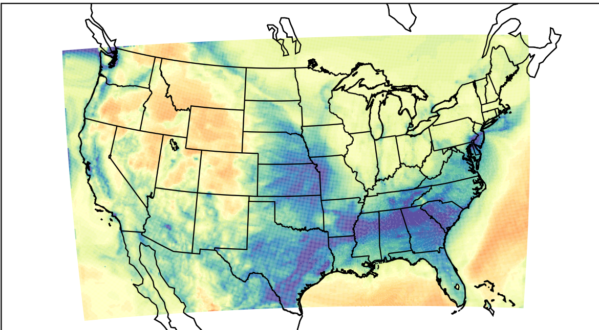
WRF (2022-01-24_09:00:00)
