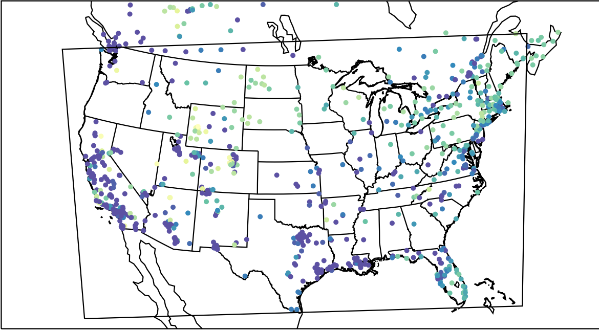
AirNOW (2022-01-24_14:00:00)
