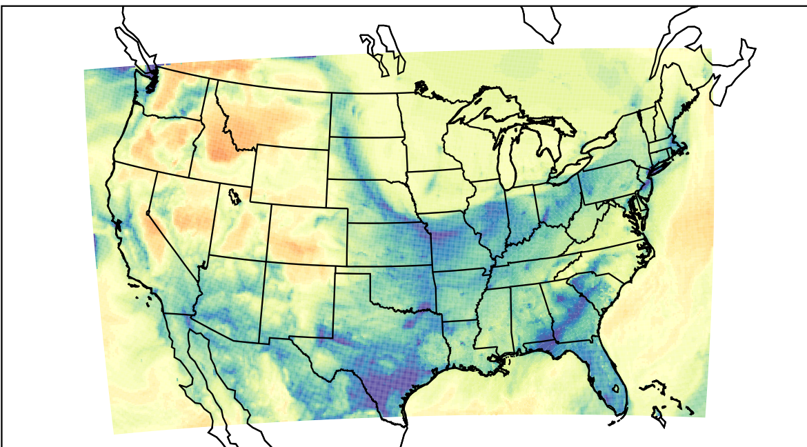
WRF (2022-01-23_12:00:00)
