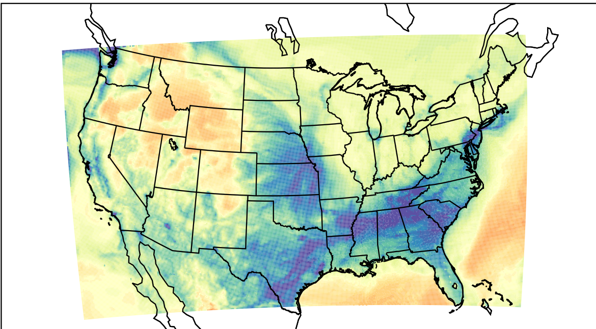
WRF (2022-01-24_07:00:00)
