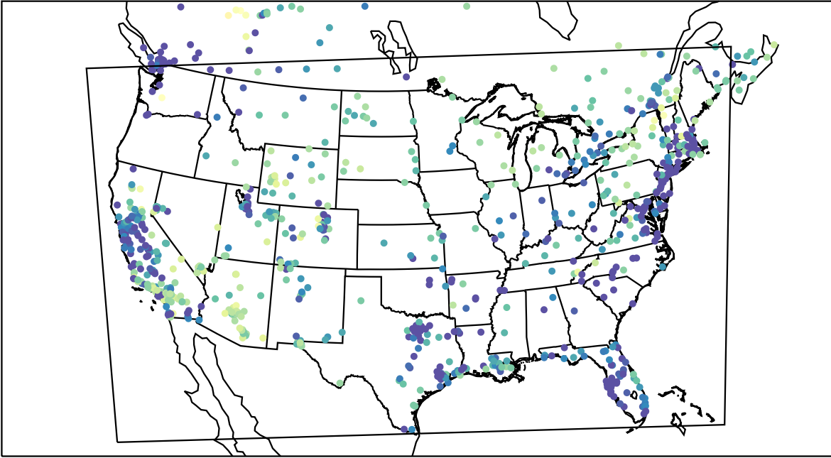
AirNOW (2022-01-23_02:00:00)
