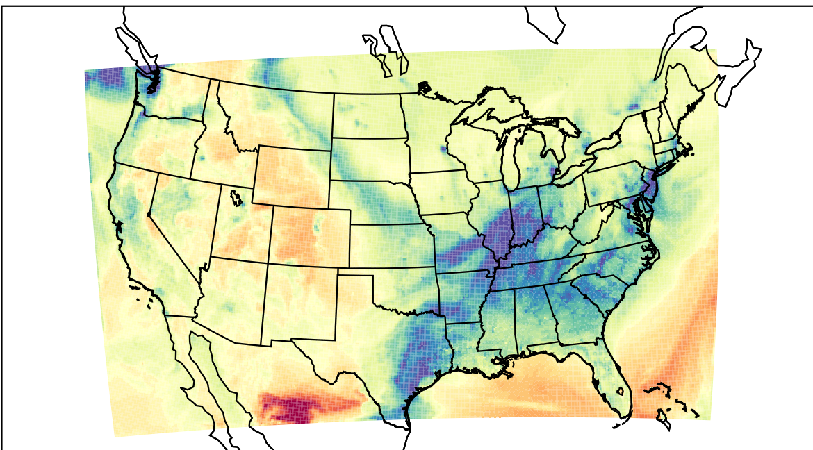
WRF (2022-01-24_23:00:00)
