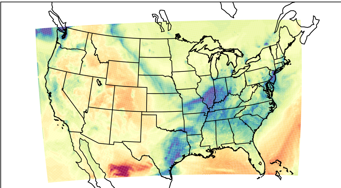
WRF (2022-01-24_22:00:00)
