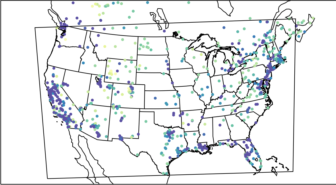
AirNOW (2022-01-24_05:00:00)
