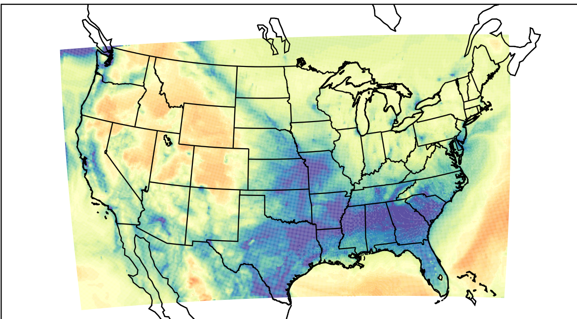
WRF (2022-01-24_14:00:00)
