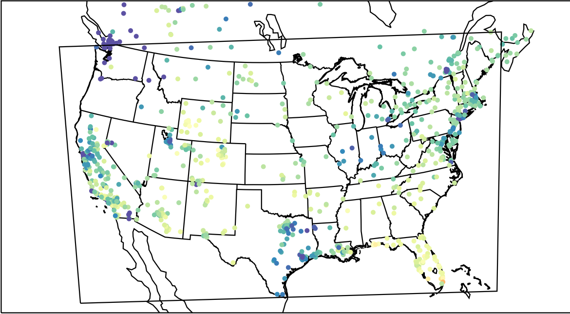
AirNOW (2022-01-24_20:00:00)
