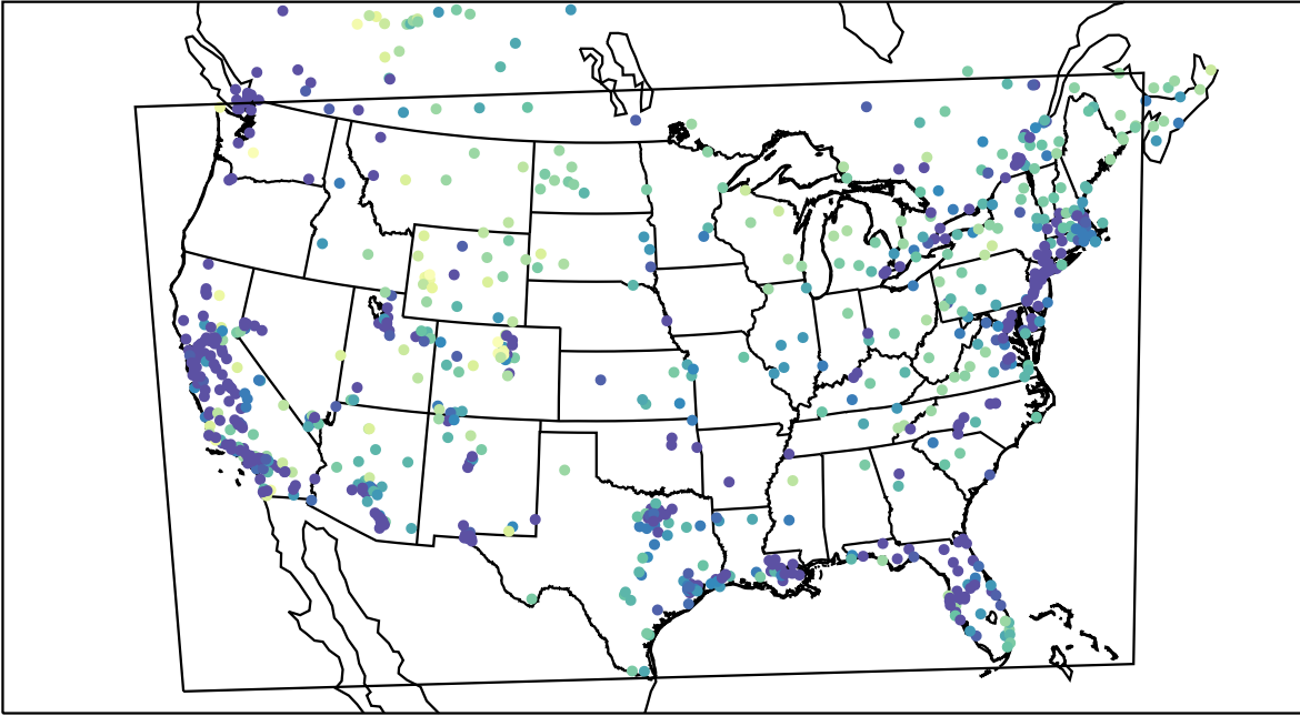
AirNOW (2022-01-24_06:00:00)
