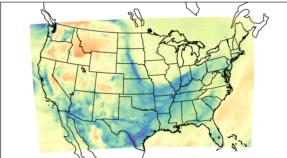
WRF (2022-01-23_16:00:00)
