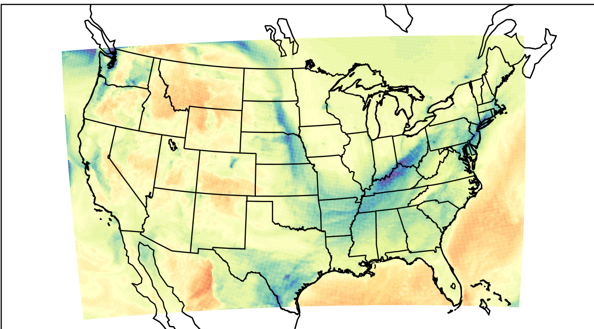
WRF (2022-01-23_21:00:00)
