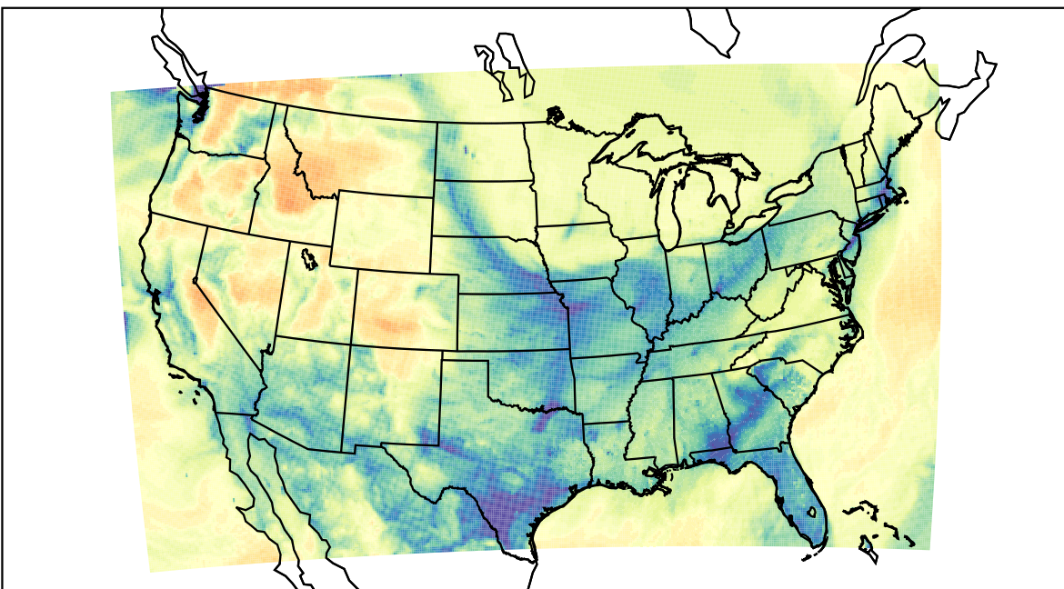
WRF (2022-01-23_10:00:00)
