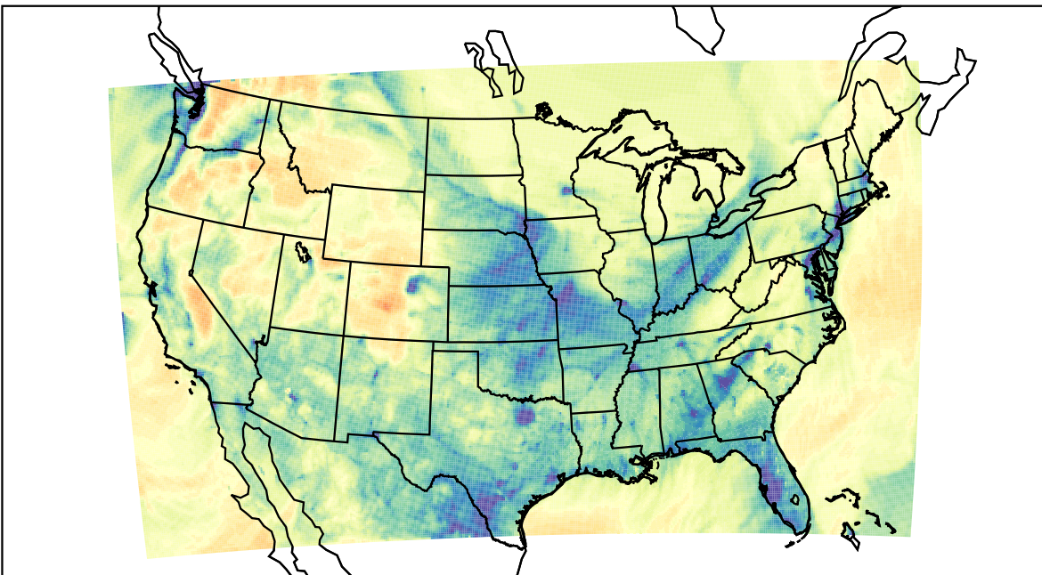
WRF (2022-01-23_03:00:00)
