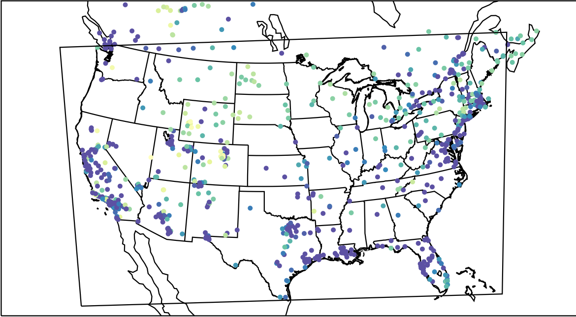
AirNOW (2022-01-24_12:00:00)
