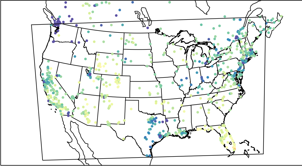
AirNOW (2022-01-24_21:00:00)
