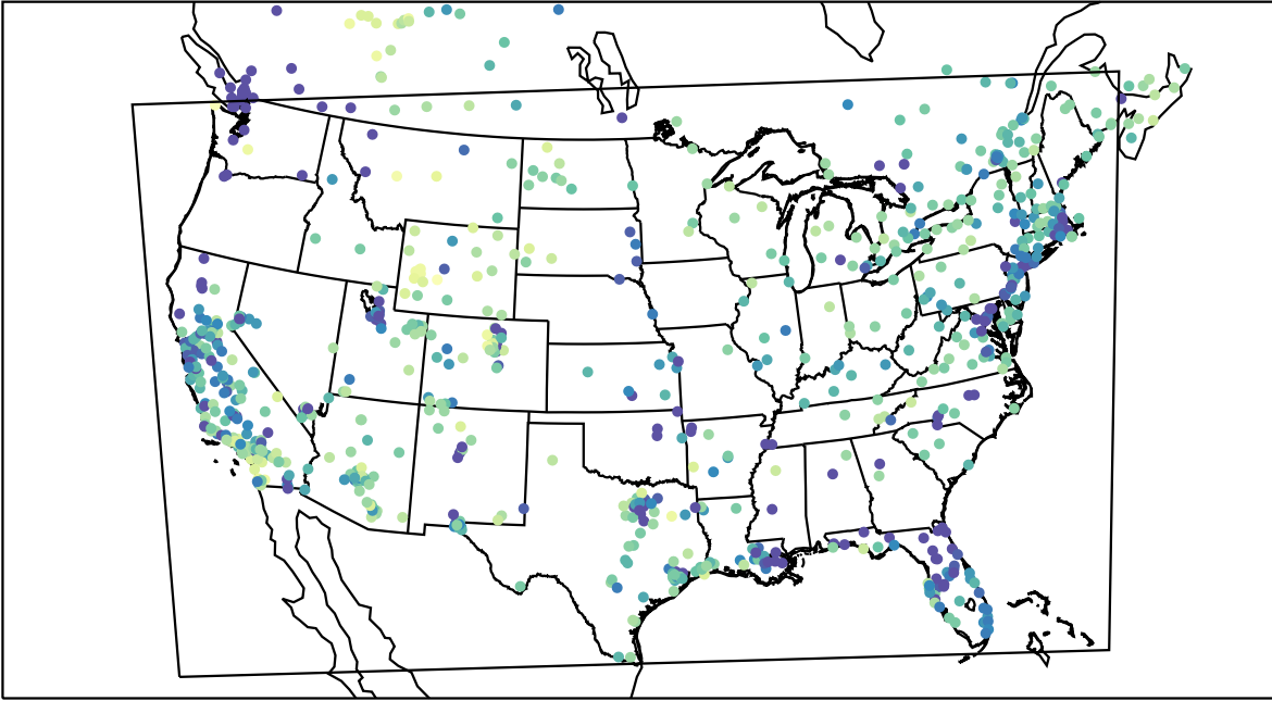
AirNOW (2022-01-24_01:00:00)
