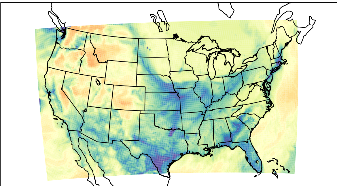
WRF (2022-01-23_09:00:00)
