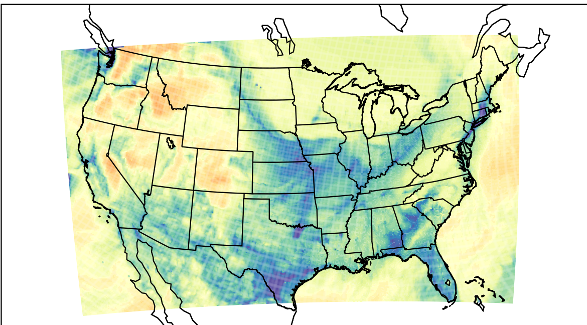
WRF (2022-01-23_08:00:00)
