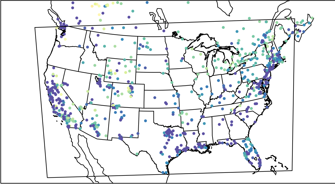
AirNOW (2022-01-23_13:00:00)
