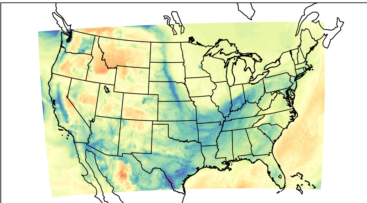
WRF (2022-01-23_17:00:00)
