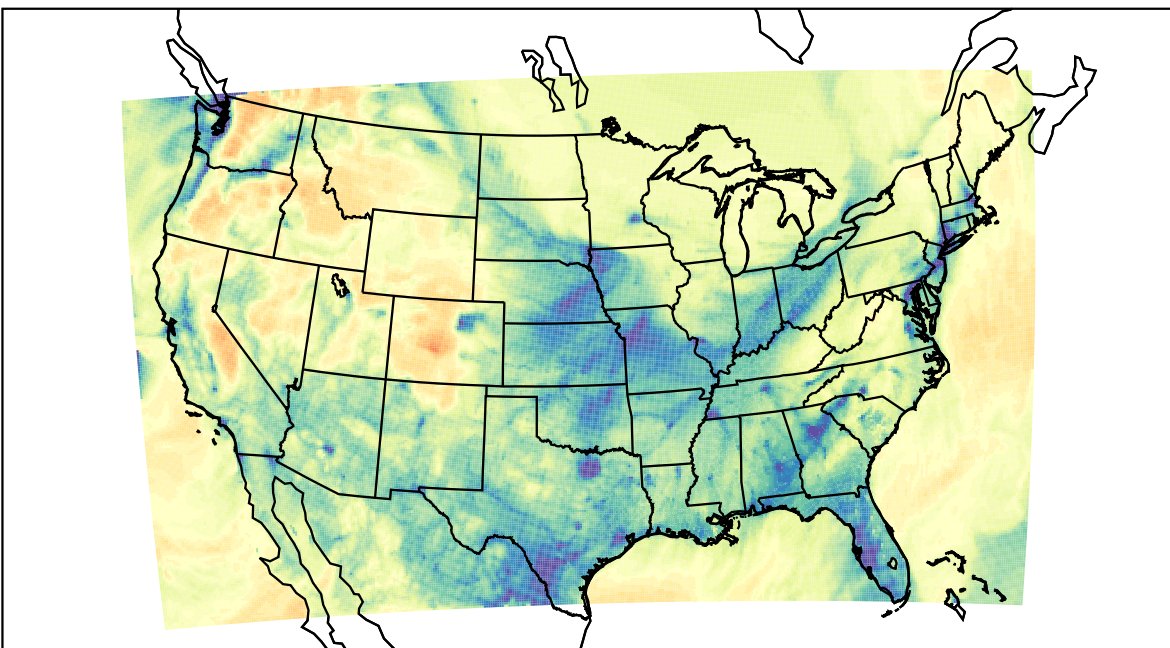
WRF (2022-01-23_04:00:00)
