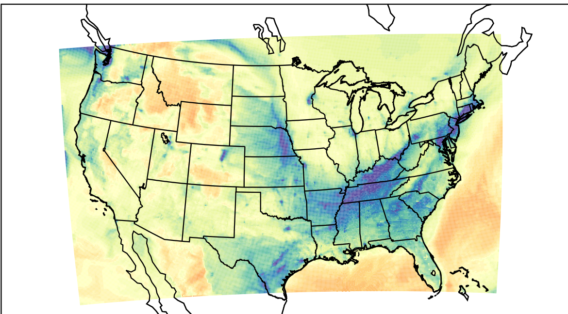
WRF (2022-01-24_00:00:00)
