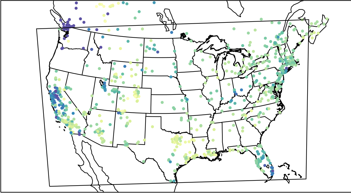
AirNOW (2022-01-23_19:00:00)
