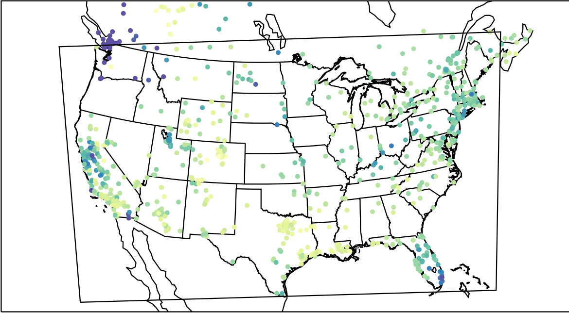
AirNOW (2022-01-23_20:00:00)
