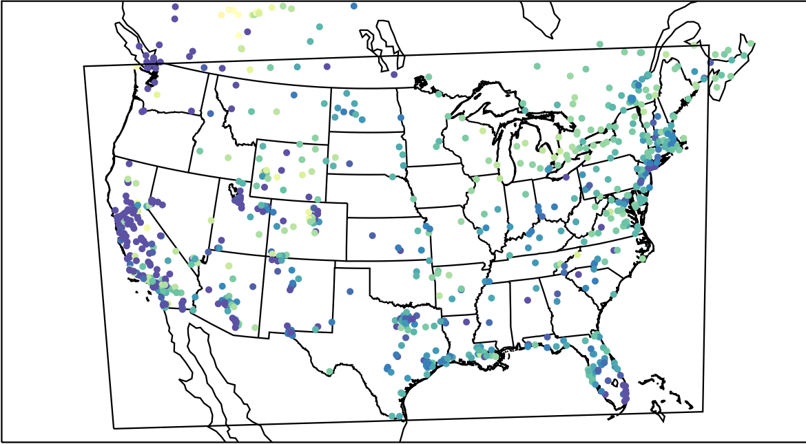
AirNOW (2022-01-23_15:00:00)
