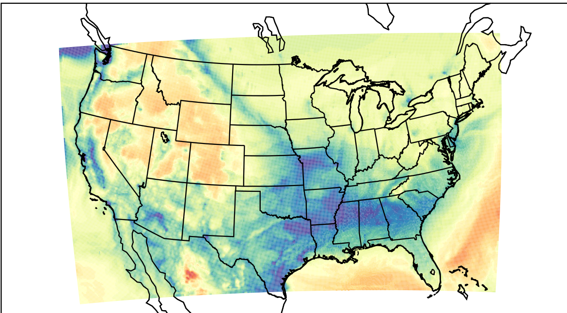
WRF (2022-01-24_16:00:00)
