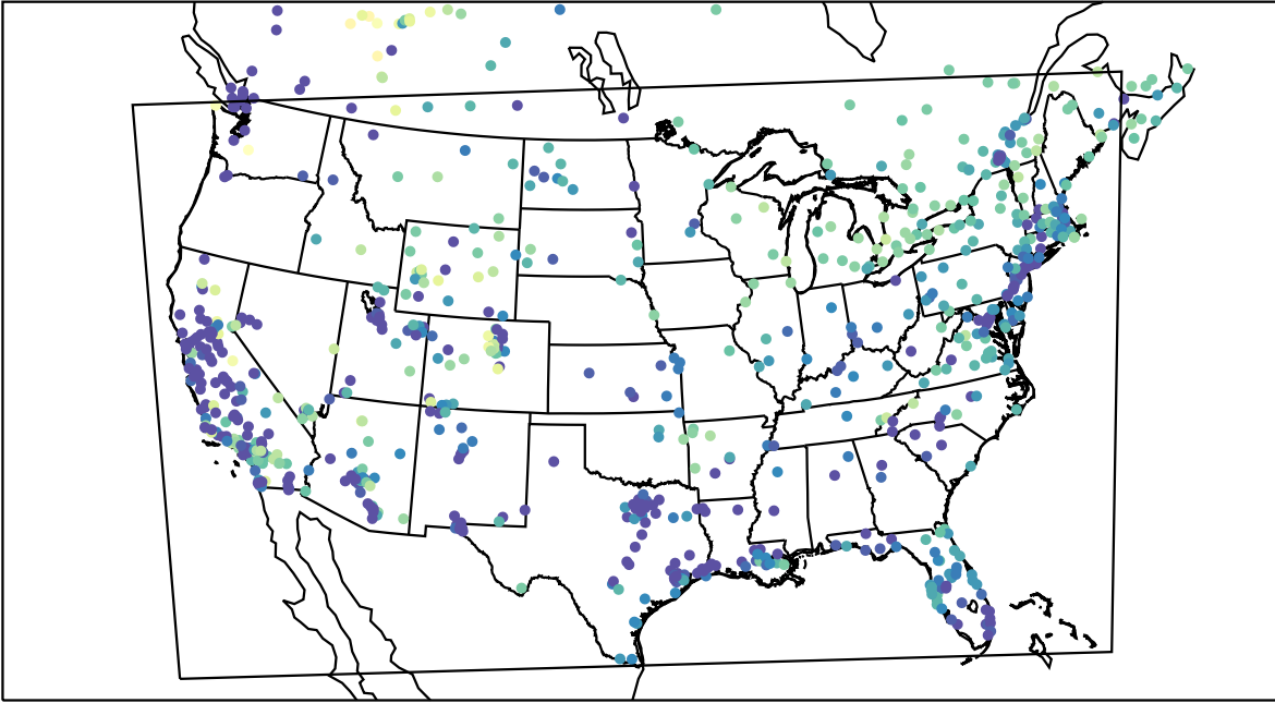
AirNOW (2022-01-23_14:00:00)
