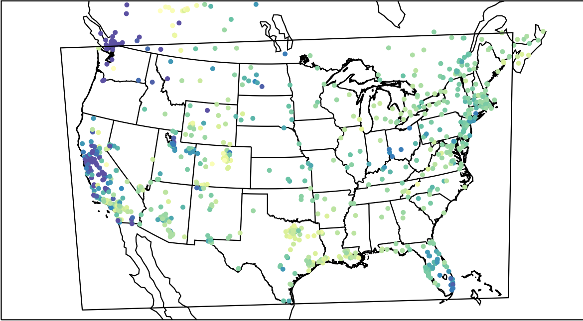
AirNOW (2022-01-23_18:00:00)
