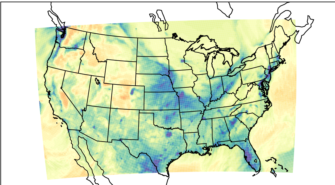
WRF (2022-01-23_02:00:00)
