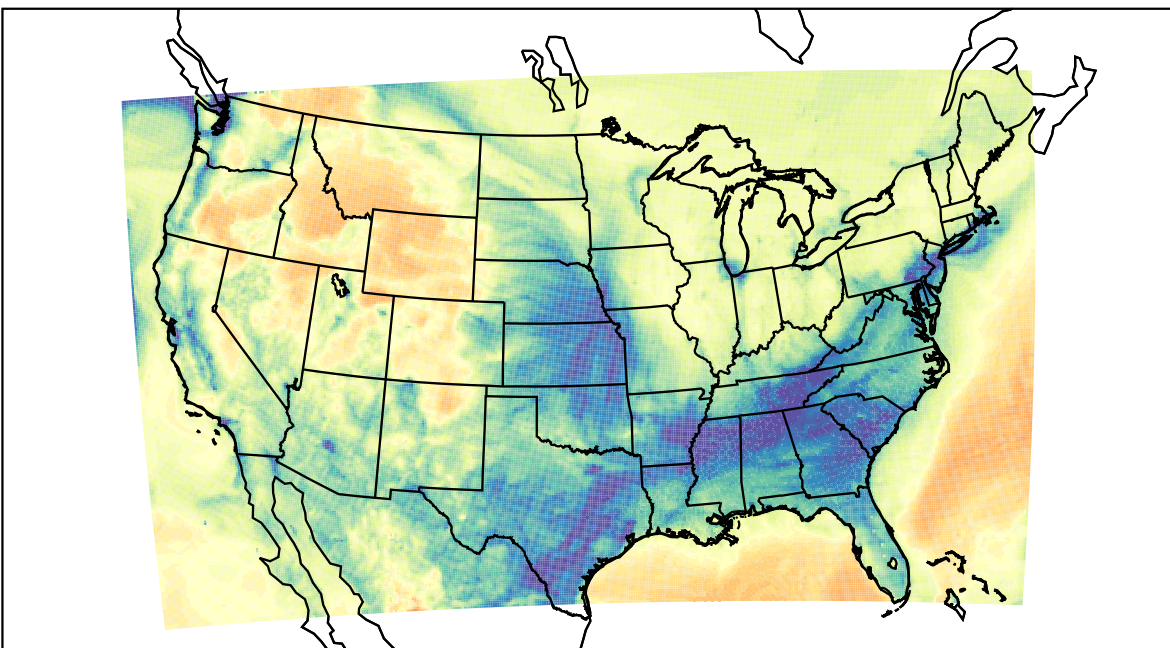
WRF (2022-01-24_06:00:00)
