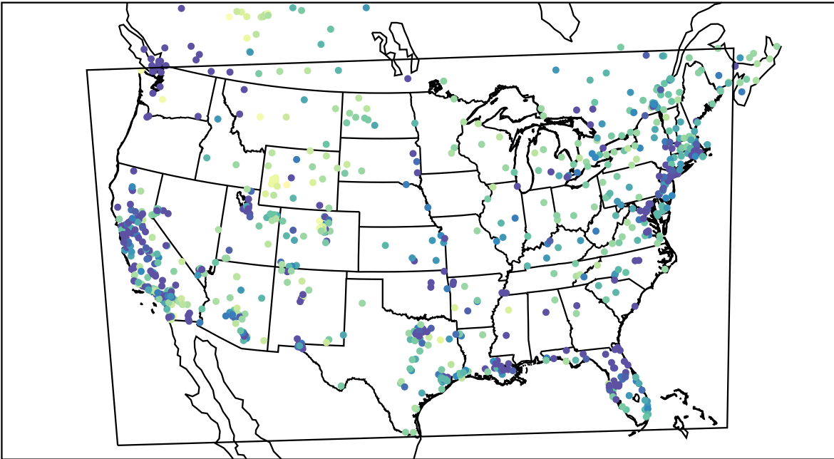
AirNOW (2022-01-24_02:00:00)
