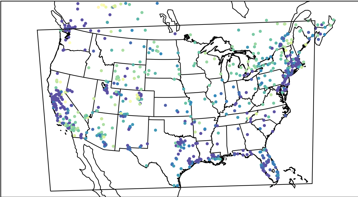
AirNOW (2022-01-23_09:00:00)
