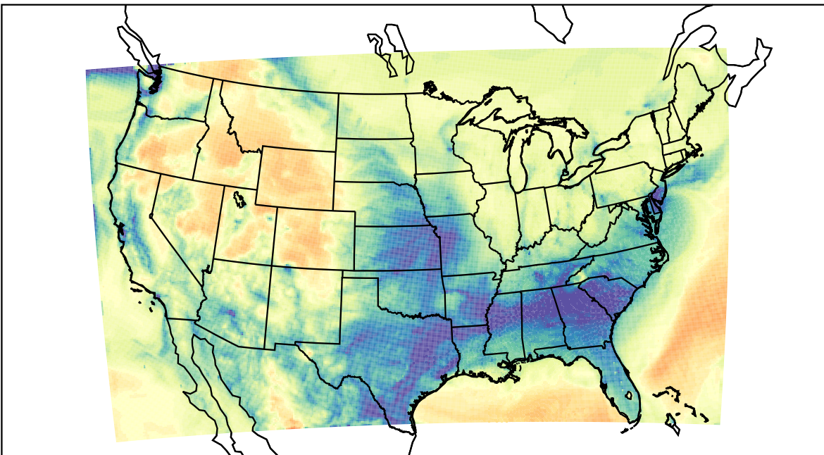
WRF (2022-01-24_11:00:00)
