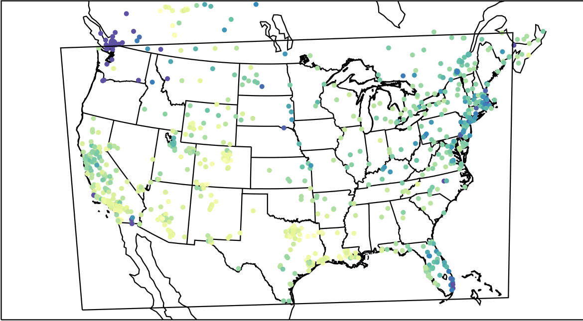
AirNOW (2022-01-23_22:00:00)
