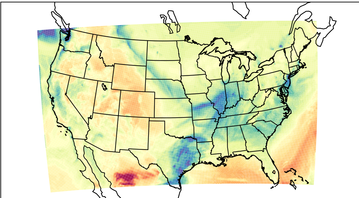
WRF (2022-01-24_21:00:00)
