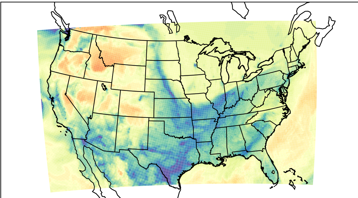
WRF (2022-01-23_15:00:00)
