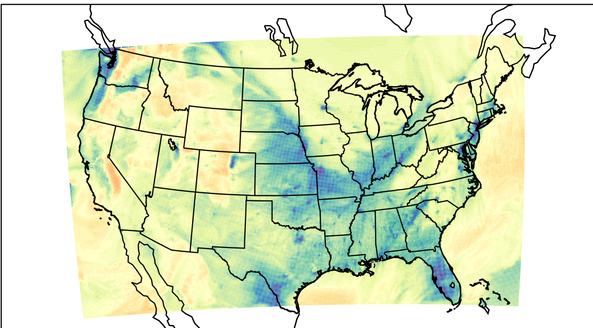
WRF (2022-01-23_00:00:00)
