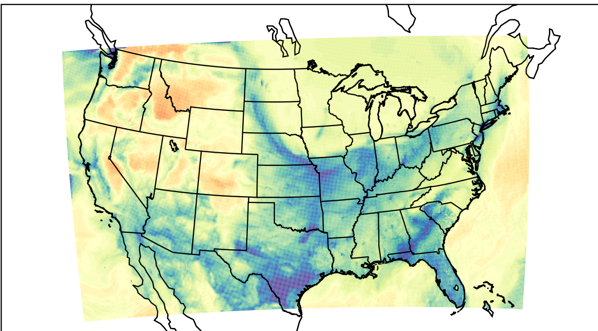
WRF (2022-01-23_11:00:00)
