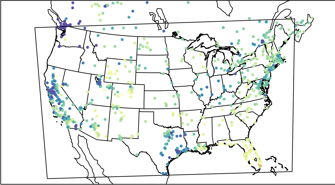
AirNOW (2022-01-24_19:00:00)
