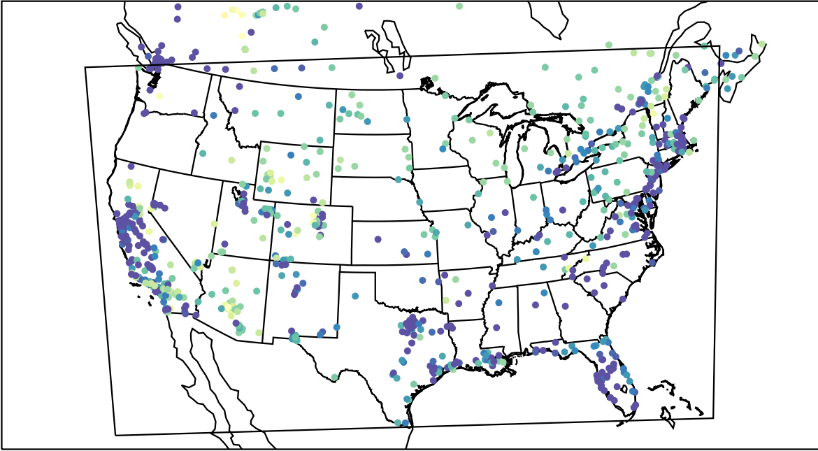
AirNOW (2022-01-23_05:00:00)
