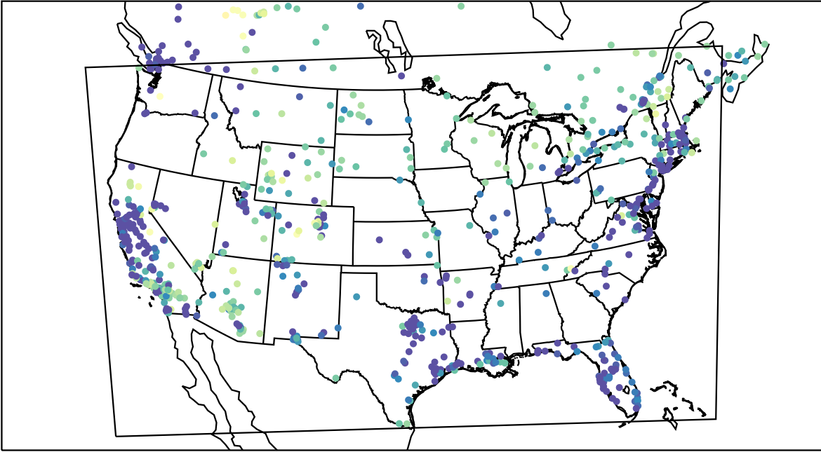
AirNOW (2022-01-23_07:00:00)
