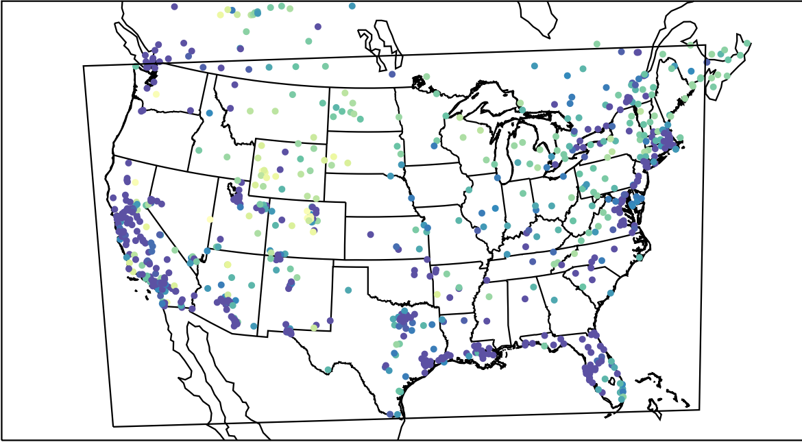
AirNOW (2022-01-24_09:00:00)
