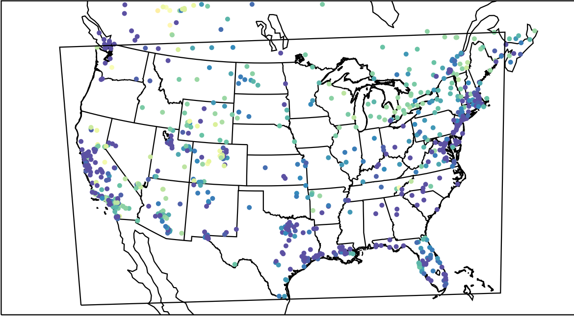
AirNOW (2022-01-23_12:00:00)
