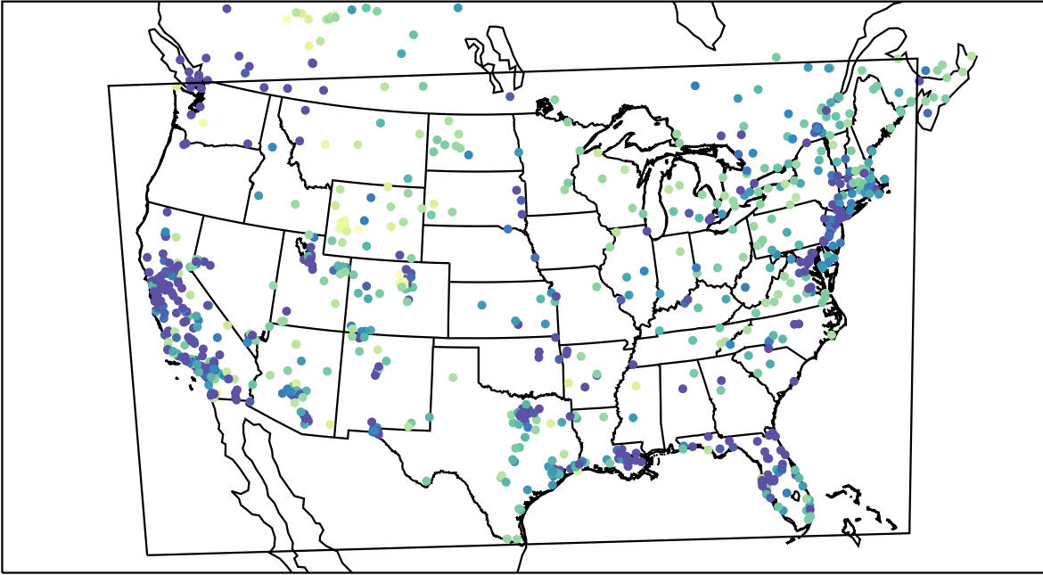
AirNOW (2022-01-24_03:00:00)
