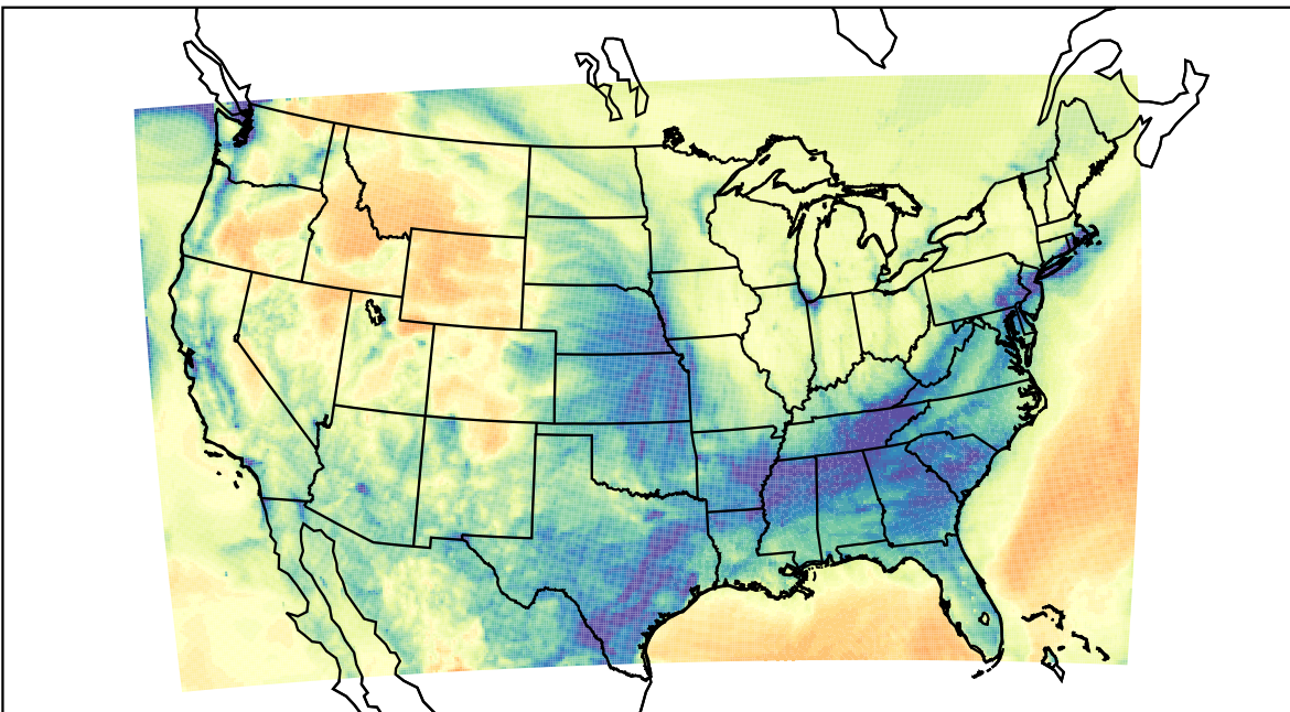
WRF (2022-01-24_05:00:00)
