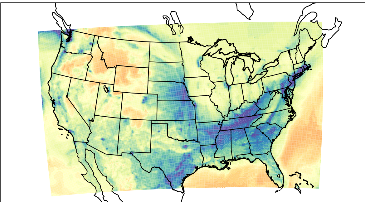
WRF (2022-01-24_02:00:00)
