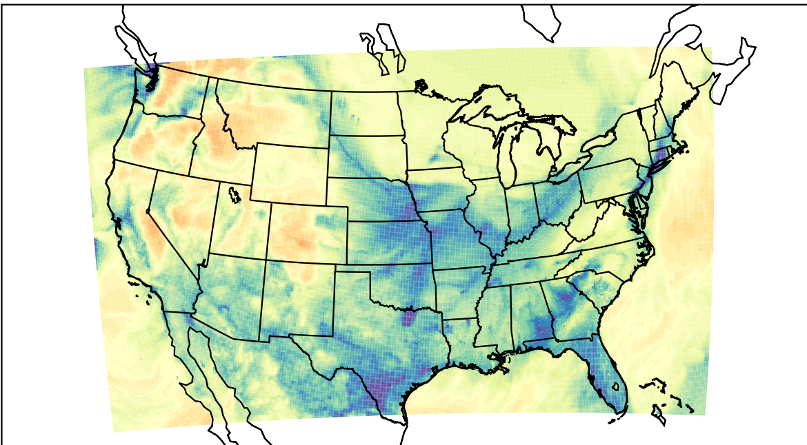
WRF (2022-01-23_07:00:00)
