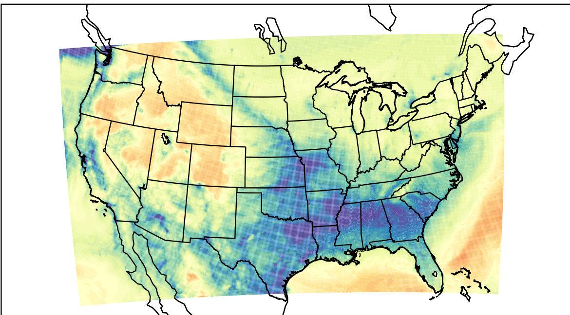
WRF (2022-01-24_15:00:00)
