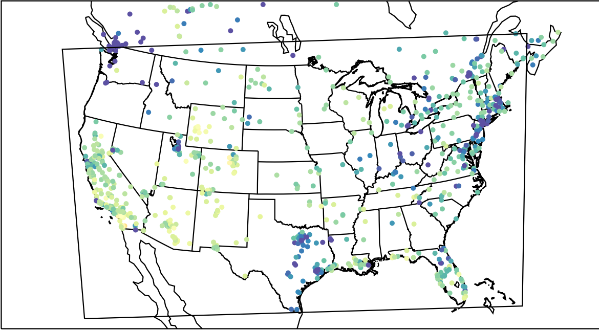
AirNOW (2022-01-24_23:00:00)
