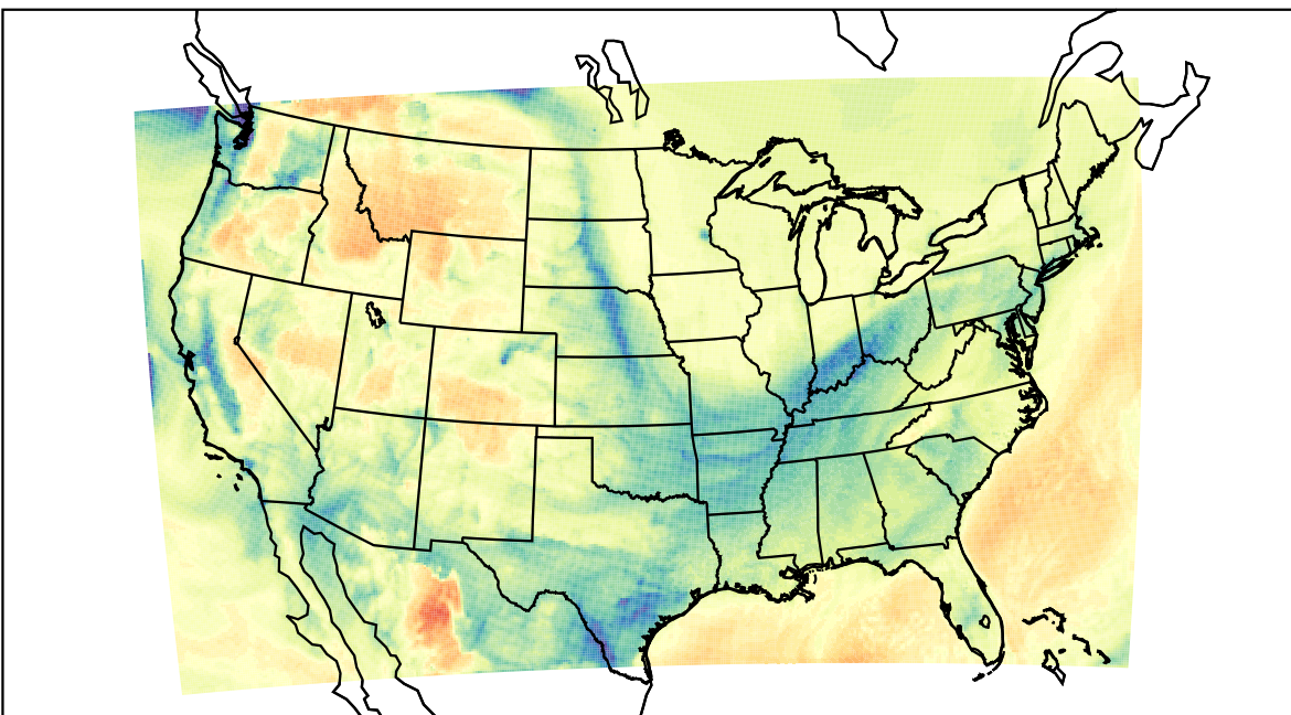
WRF (2022-01-23_18:00:00)
