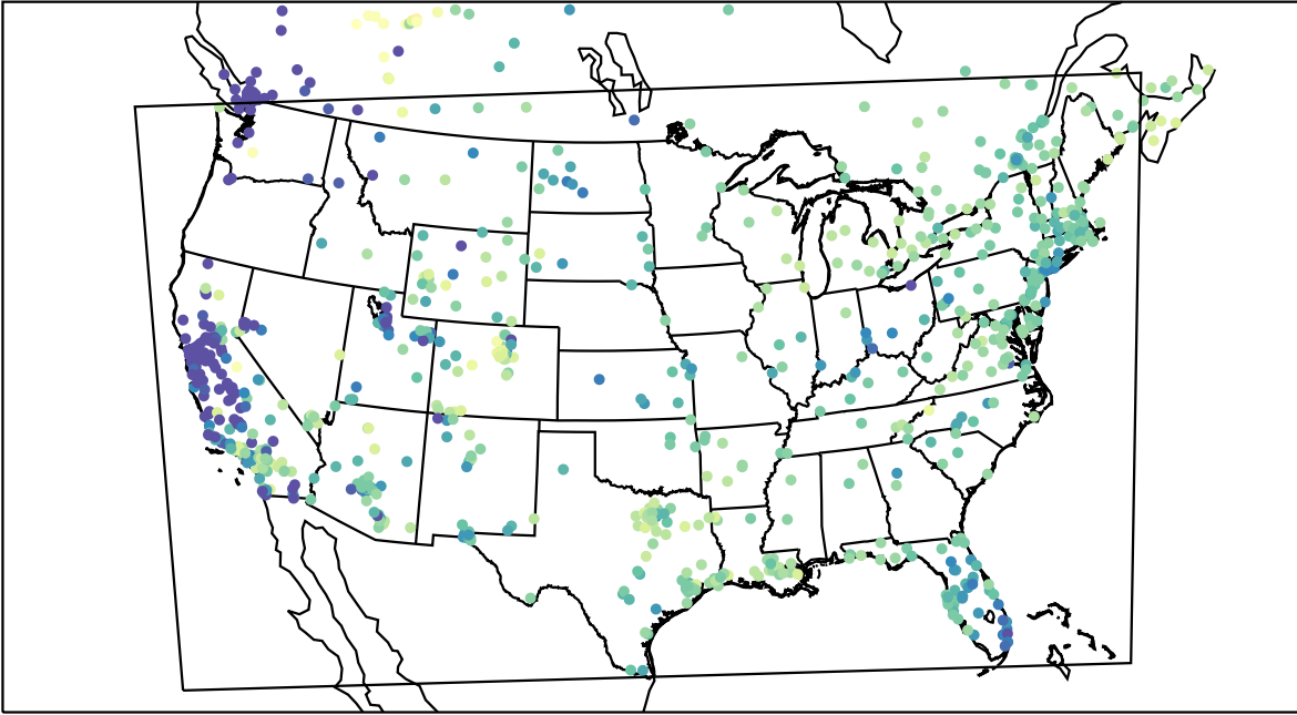
AirNOW (2022-01-23_17:00:00)
