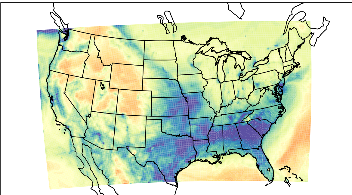
WRF (2022-01-24_13:00:00)
