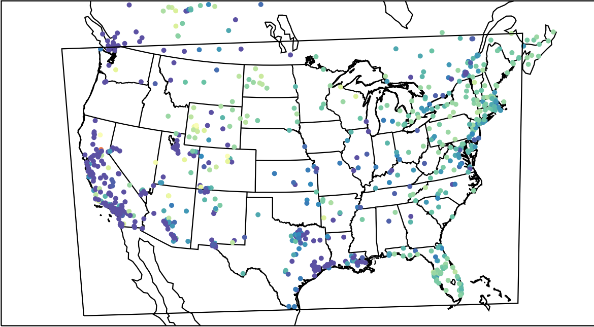
AirNOW (2022-01-24_15:00:00)
