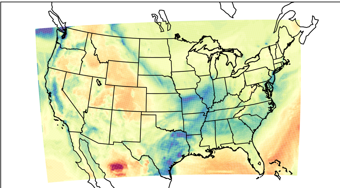
WRF (2022-01-24_19:00:00)
