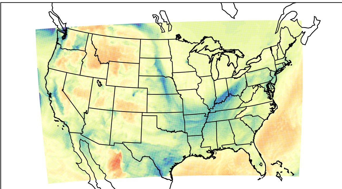
WRF (2022-01-23_19:00:00)
