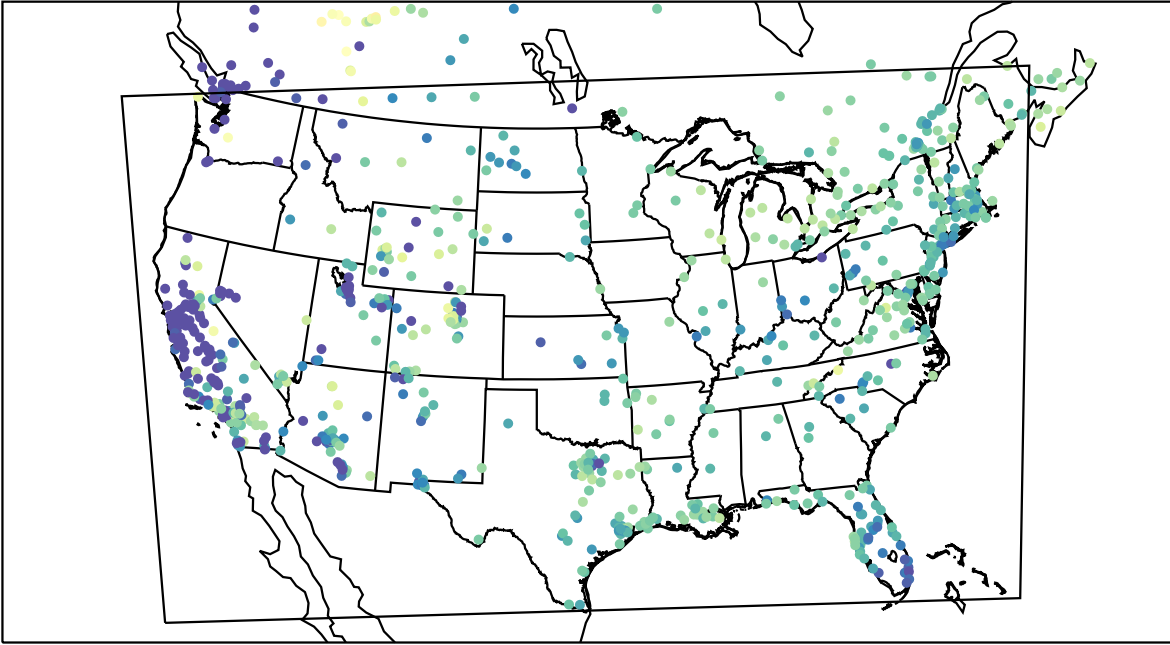
AirNOW (2022-01-23_16:00:00)
