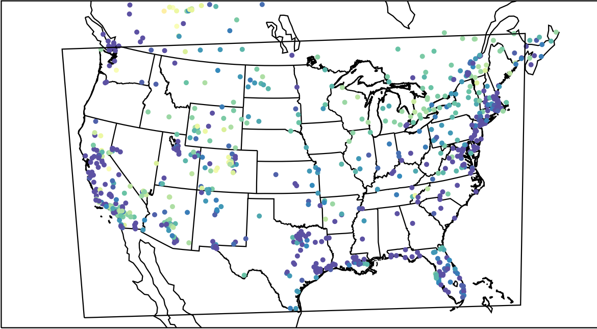
AirNOW (2022-01-23_11:00:00)
