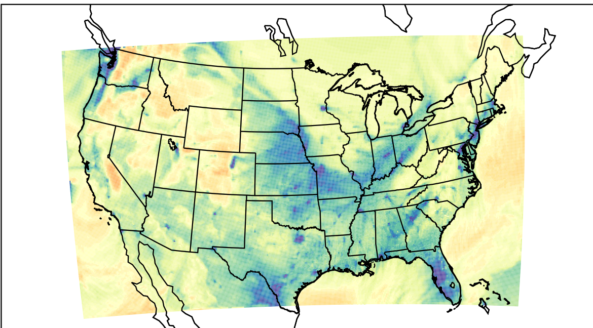
WRF (2022-01-23_01:00:00)
