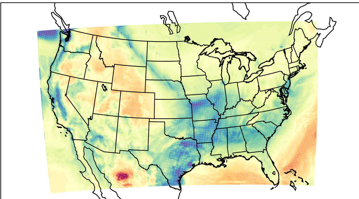
WRF (2022-01-24_18:00:00)
