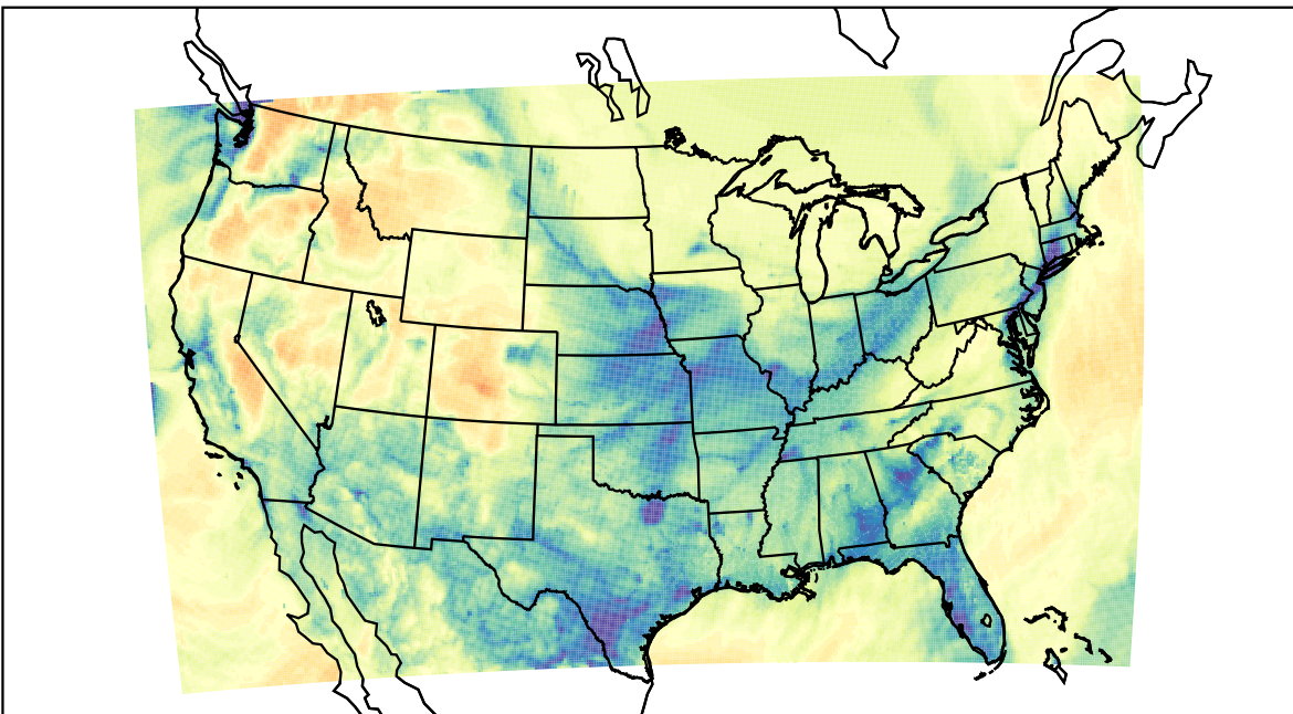
WRF (2022-01-23_06:00:00)
