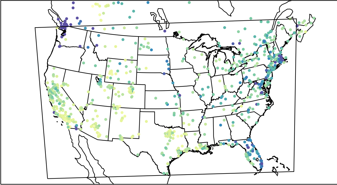
AirNOW (2022-01-23_23:00:00)
