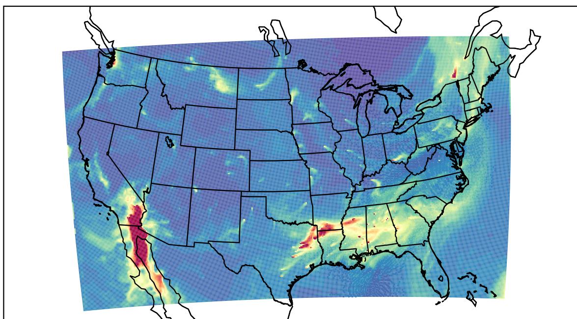
WRF 2022-02-10_17:00:00
