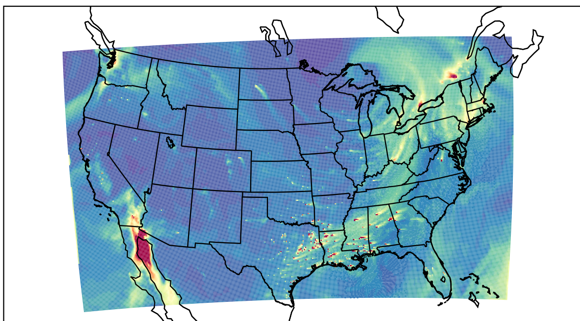
WRF 2022-02-09_21:00:00
