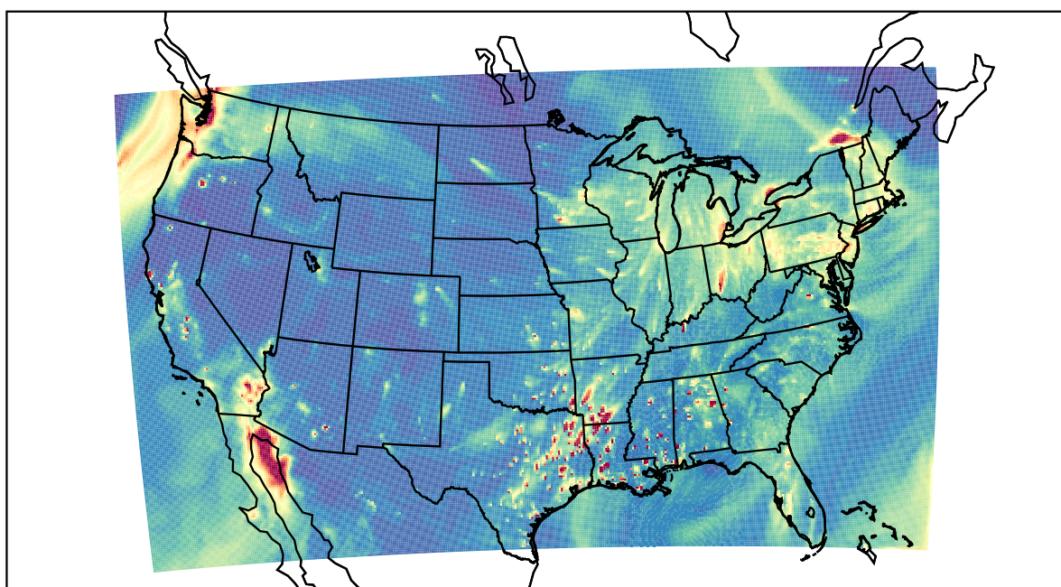
WRF 2022-02-09_02:00:00
