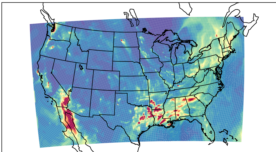
WRF 2022-02-10_05:00:00
