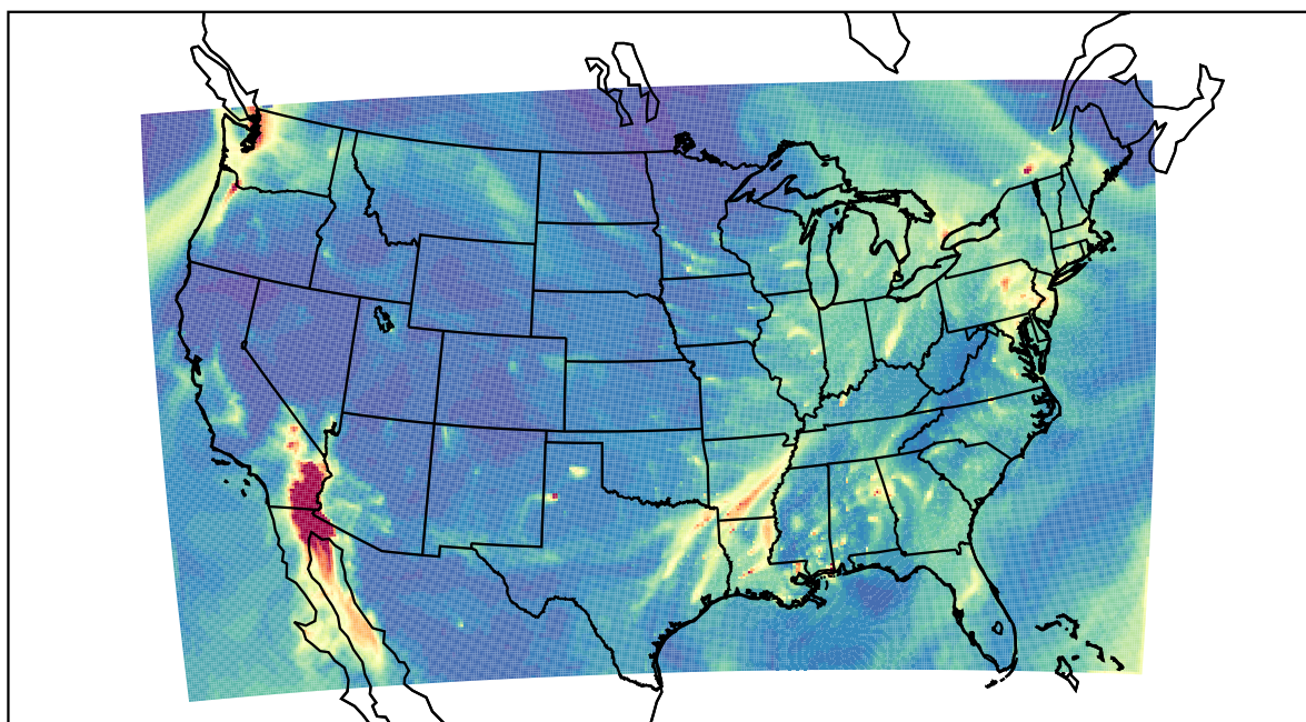
WRF 2022-02-09_11:00:00
