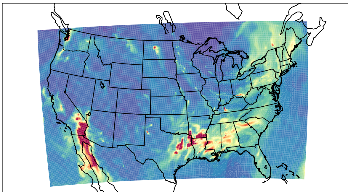
WRF 2022-02-10_09:00:00
