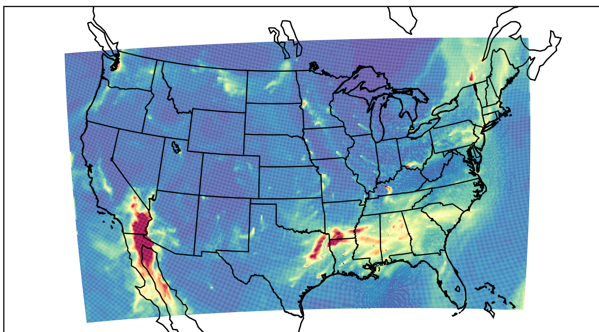
WRF 2022-02-10_15:00:00
