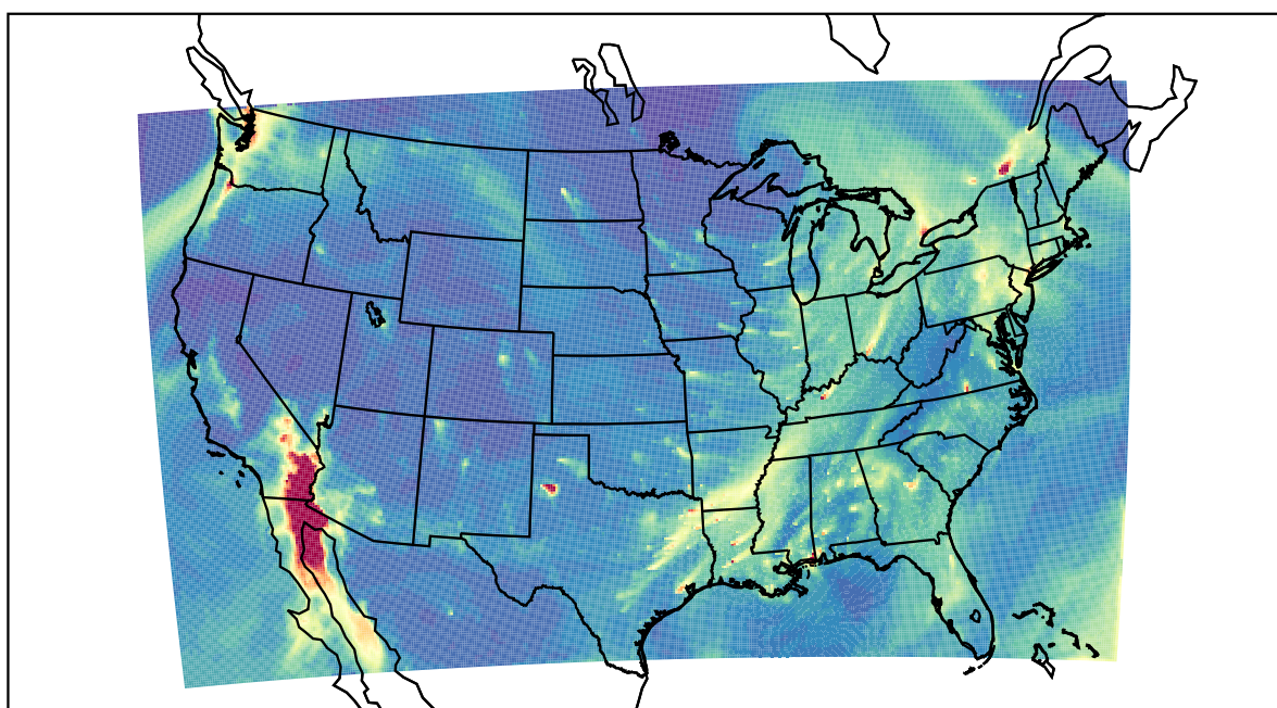
WRF 2022-02-09_15:00:00
