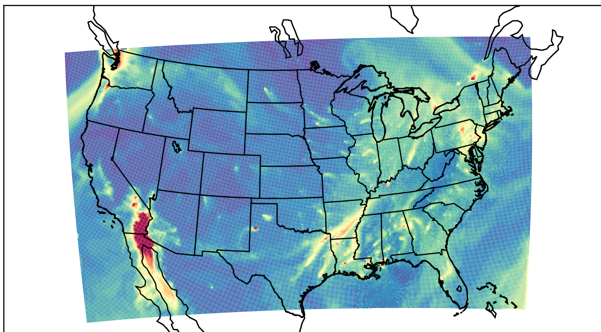
WRF 2022-02-09_12:00:00
