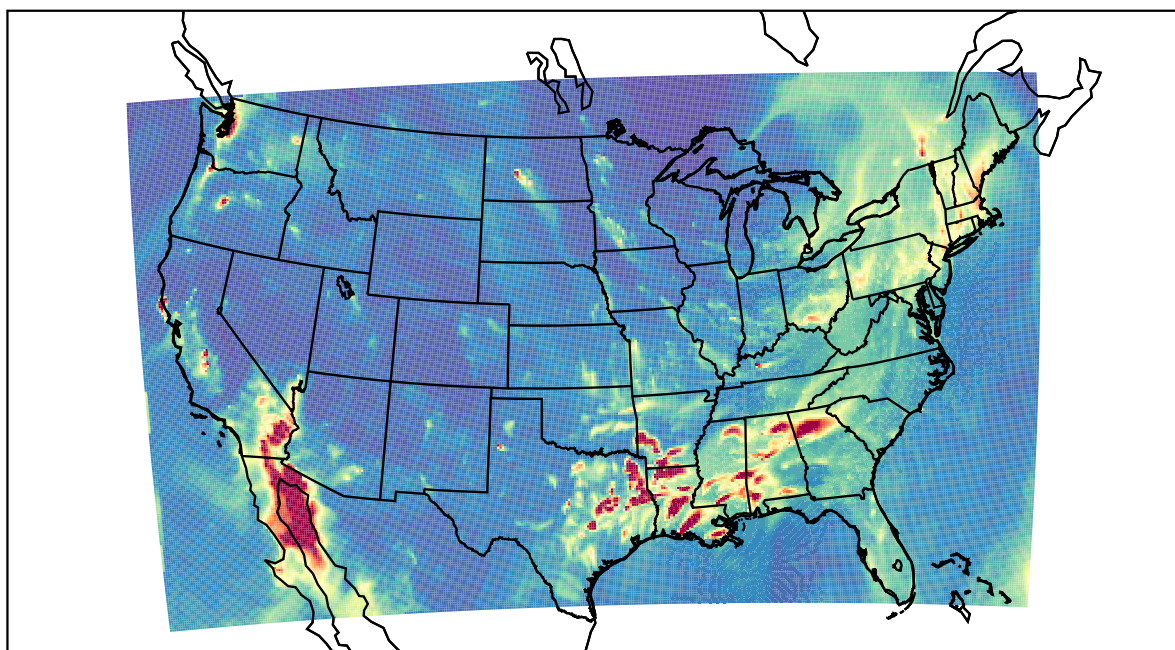
WRF 2022-02-10_04:00:00
