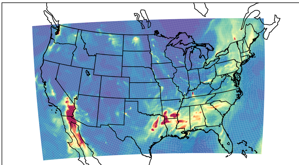
WRF 2022-02-10_11:00:00
