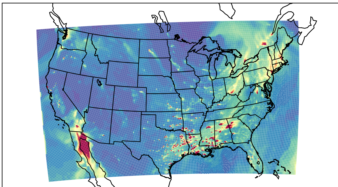
WRF 2022-02-10_00:00:00
