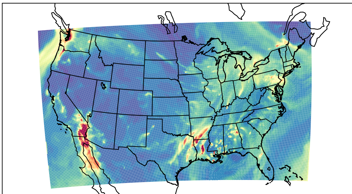
WRF 2022-02-09_07:00:00
