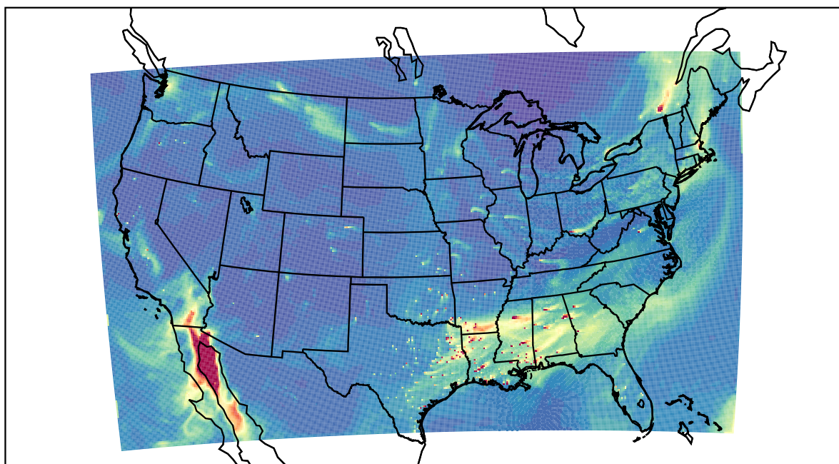
WRF 2022-02-10_21:00:00
