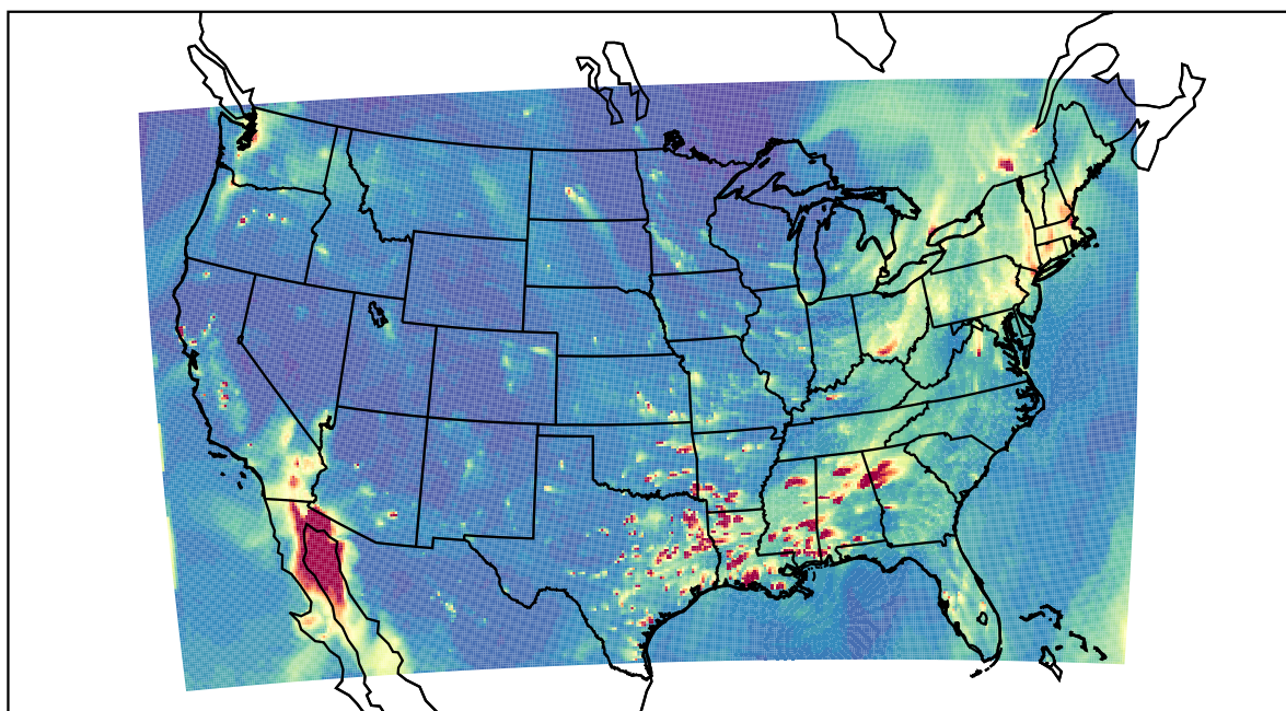
WRF 2022-02-10_01:00:00
