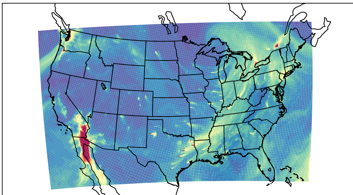
WRF 2022-02-09_17:00:00
