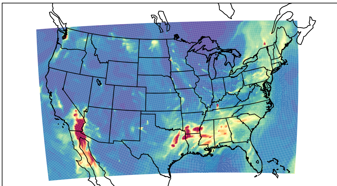
WRF 2022-02-10_12:00:00
