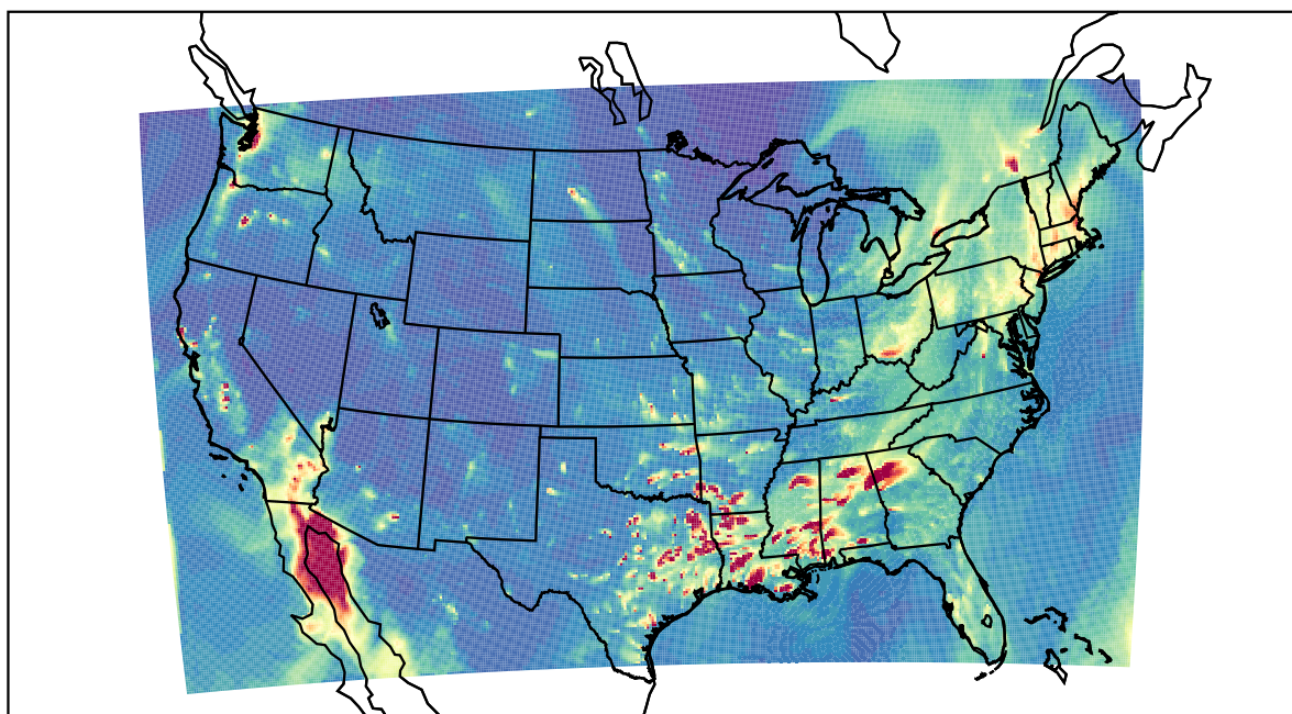
WRF 2022-02-10_02:00:00
