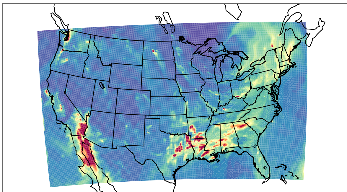
WRF 2022-02-10_06:00:00
