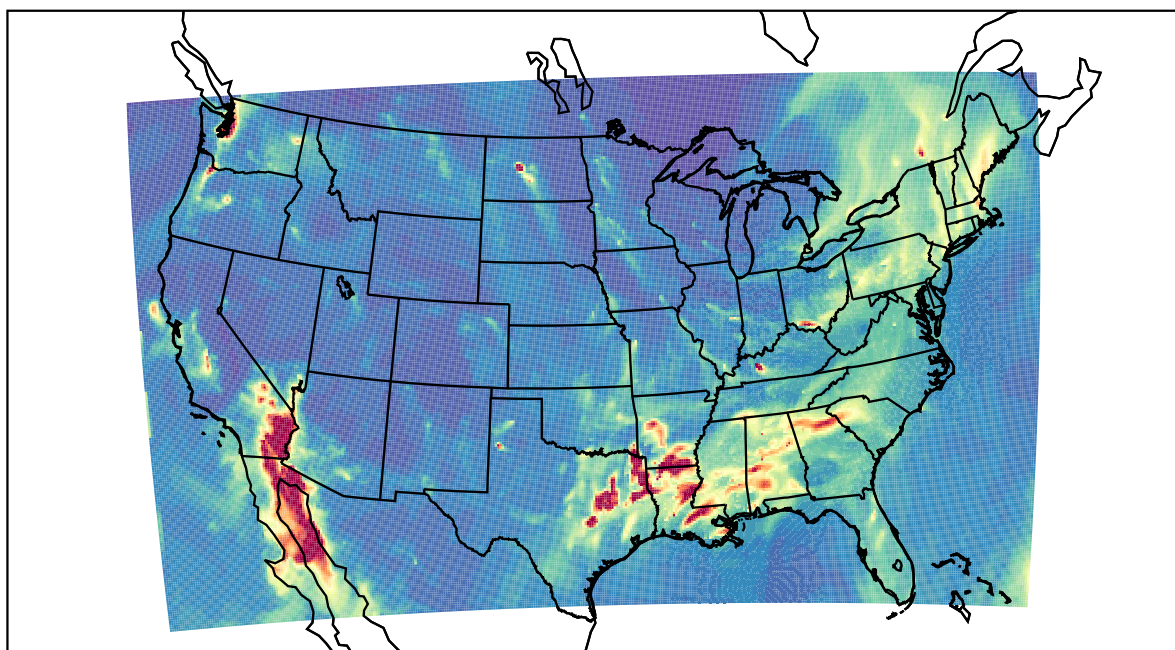
WRF 2022-02-10_07:00:00
