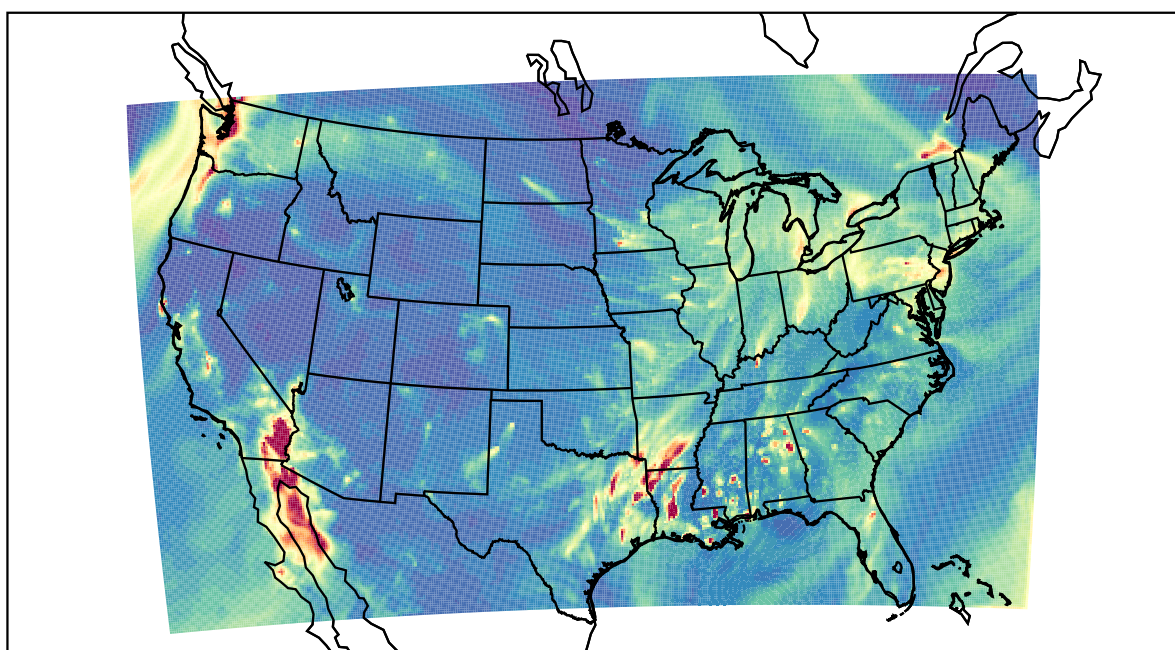
WRF 2022-02-09_05:00:00
