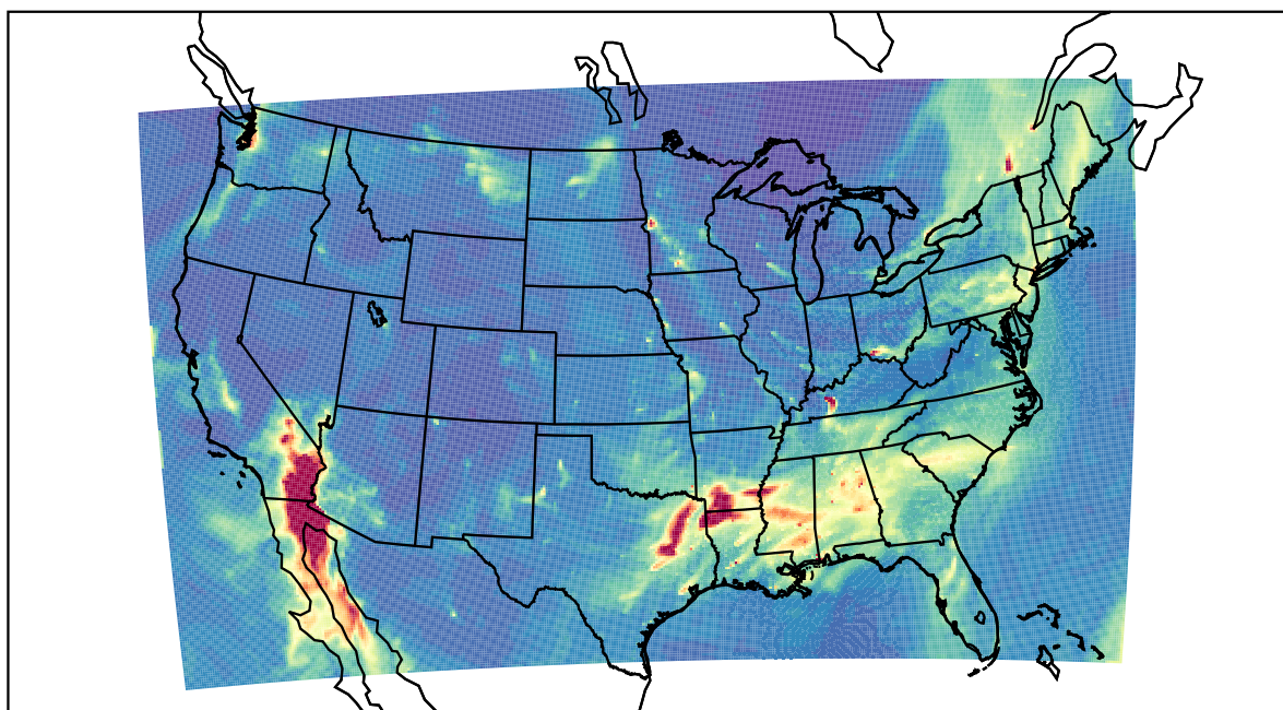
WRF 2022-02-10_14:00:00
