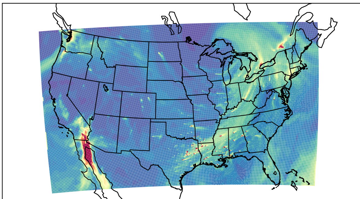
WRF 2022-02-09_19:00:00
