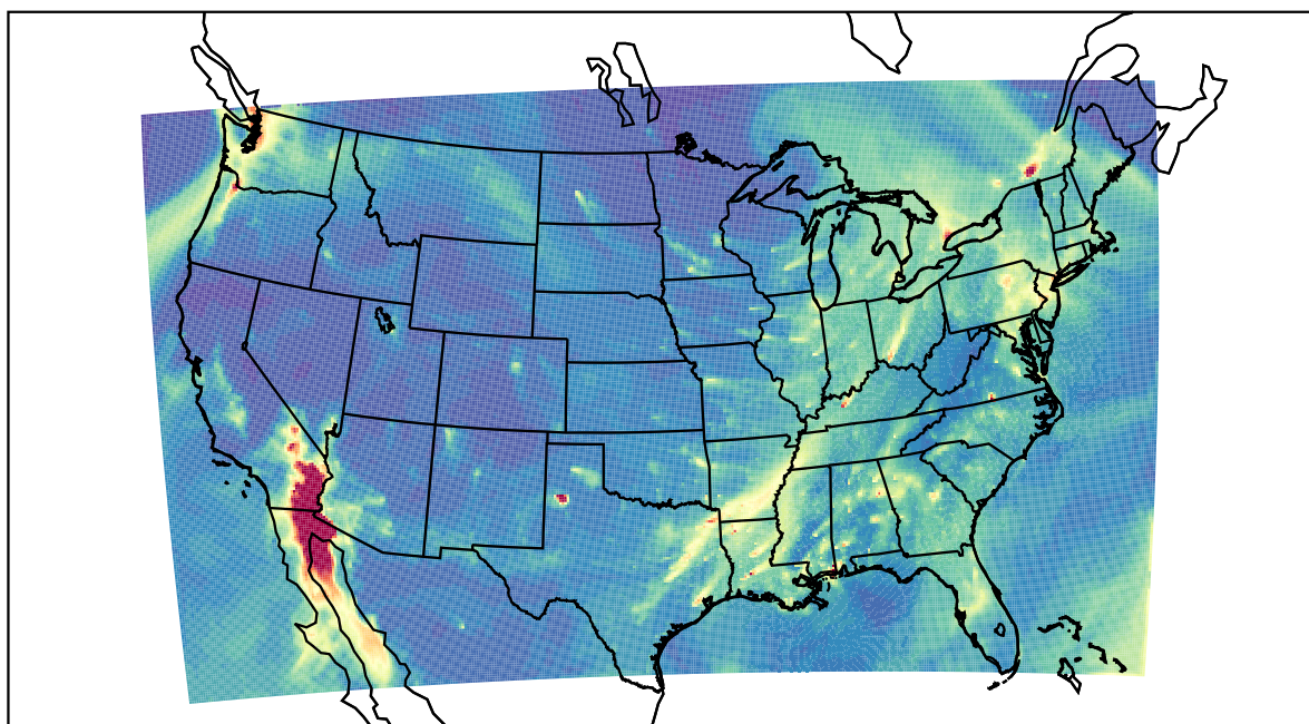
WRF 2022-02-09_14:00:00
