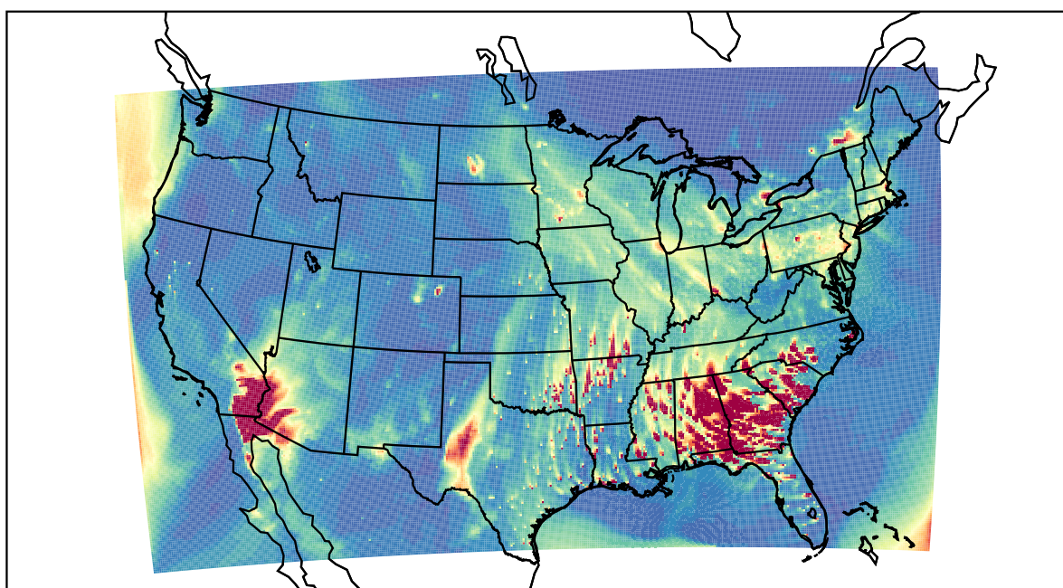
WRF 2022-02-16_00:00:00
