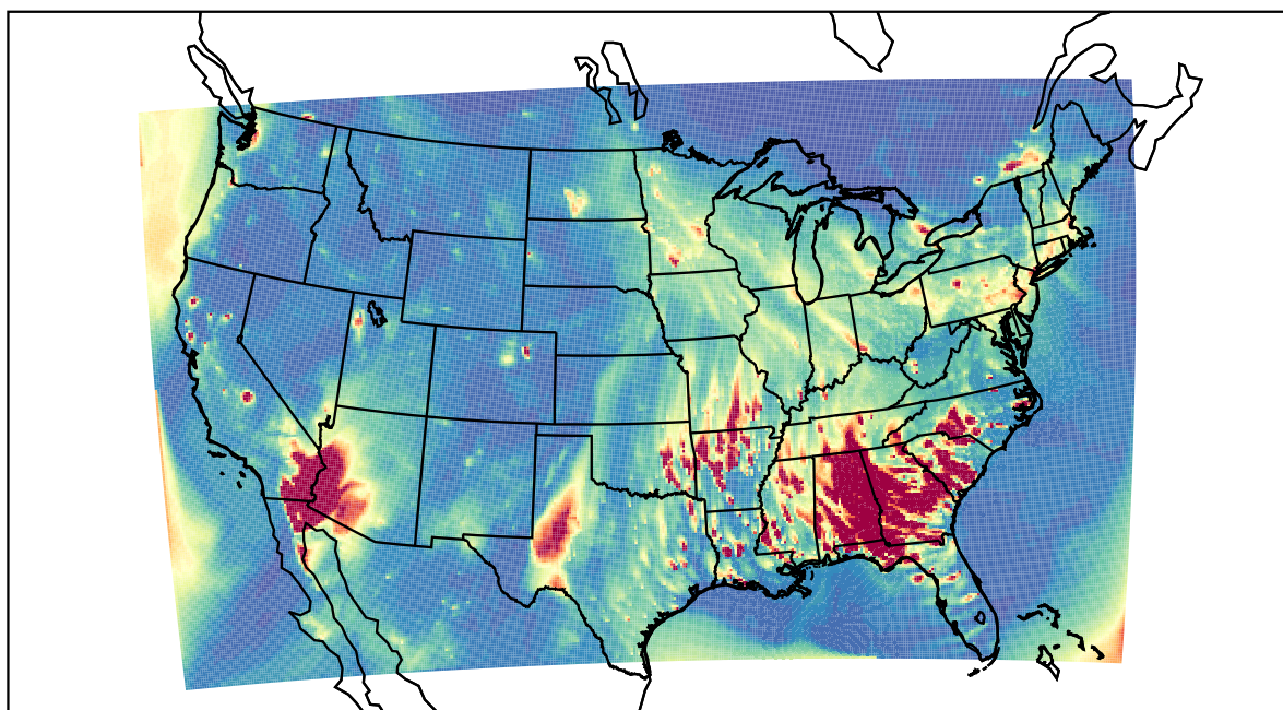
WRF 2022-02-16_02:00:00
