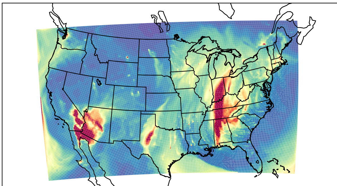
WRF 2022-02-16_12:00:00
