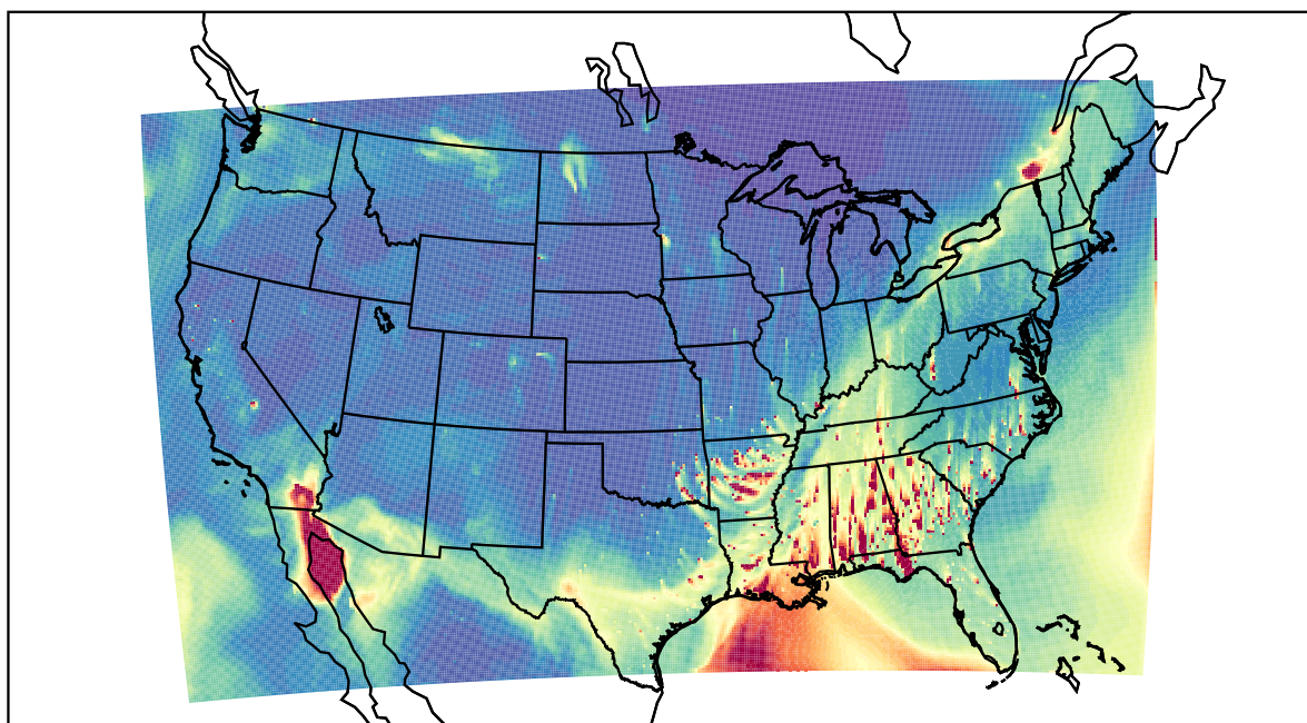
WRF 2022-02-17_21:00:00
