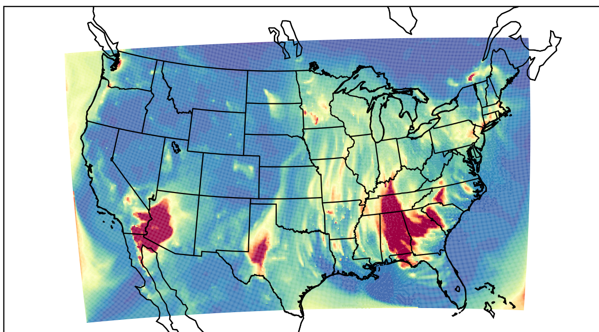
WRF 2022-02-16_06:00:00
