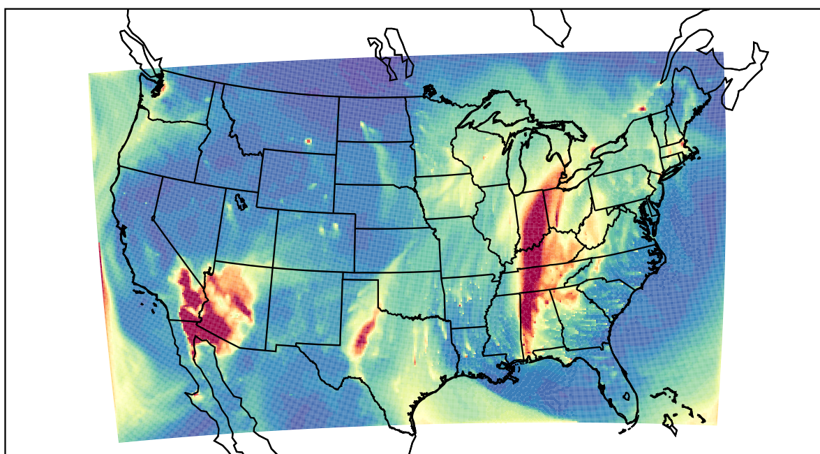
WRF 2022-02-16_13:00:00
