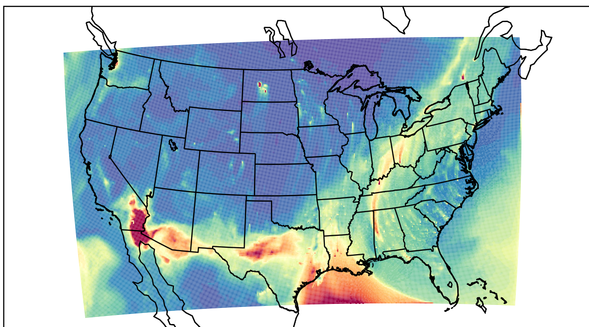
WRF 2022-02-17_13:00:00
