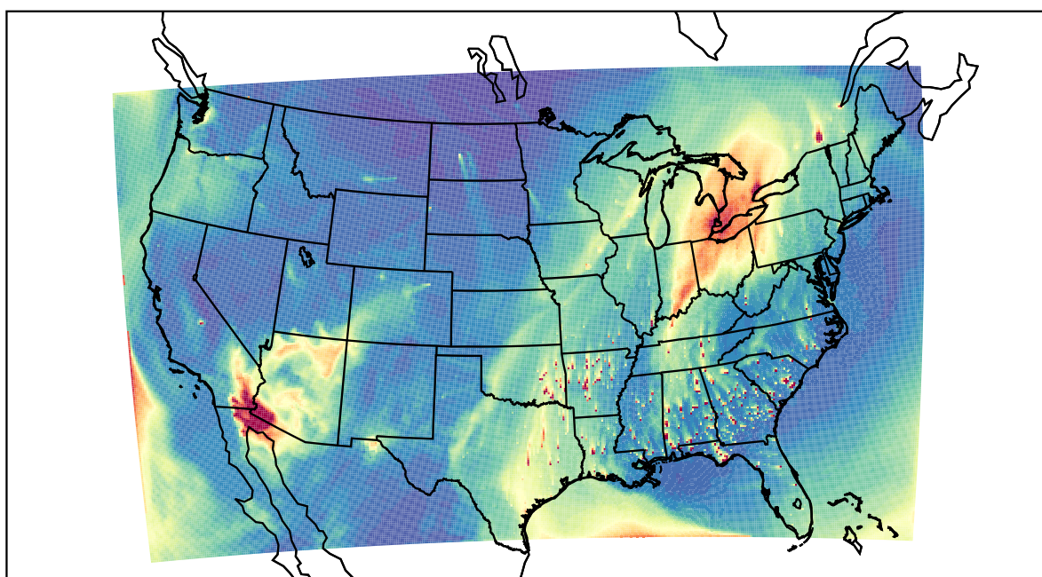
WRF 2022-02-16_19:00:00
