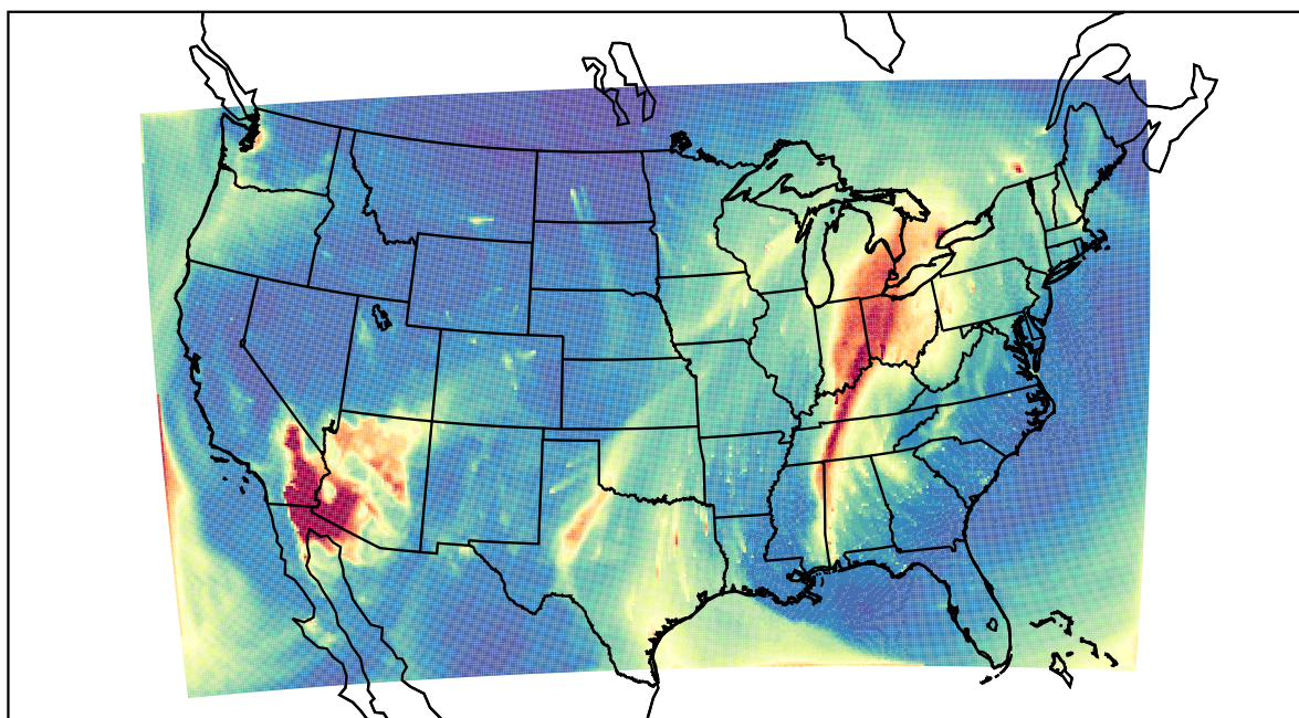
WRF 2022-02-16_16:00:00
