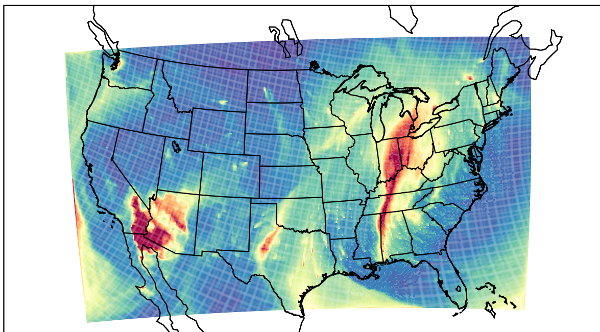
WRF 2022-02-16_15:00:00
