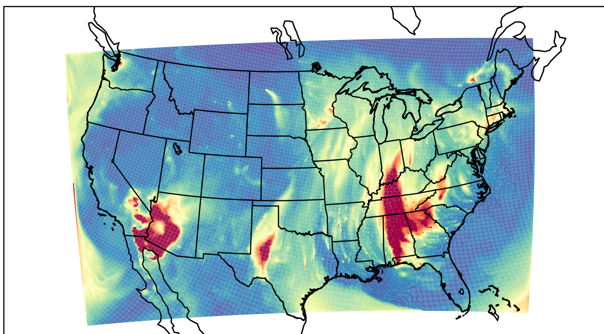
WRF 2022-02-16_09:00:00
