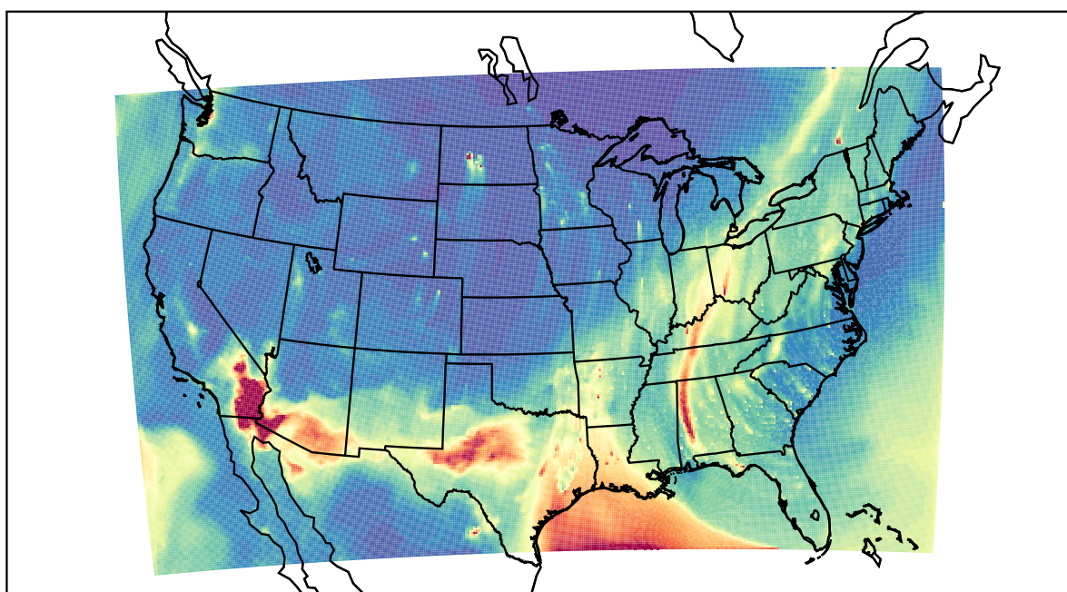
WRF 2022-02-17_11:00:00
