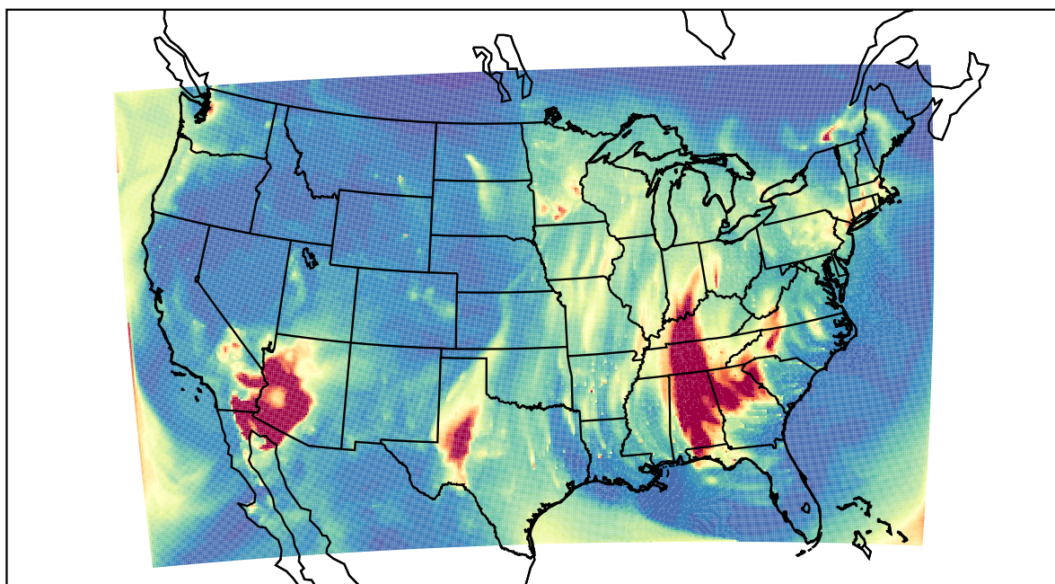
WRF 2022-02-16_08:00:00
