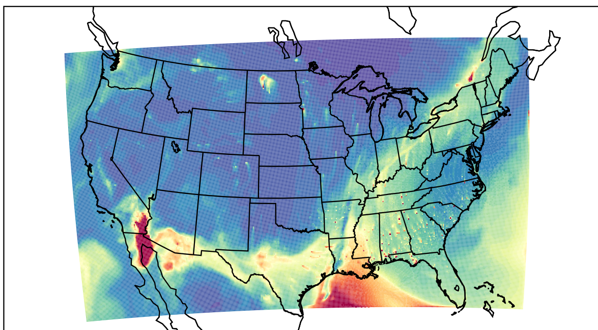
WRF 2022-02-17_17:00:00
