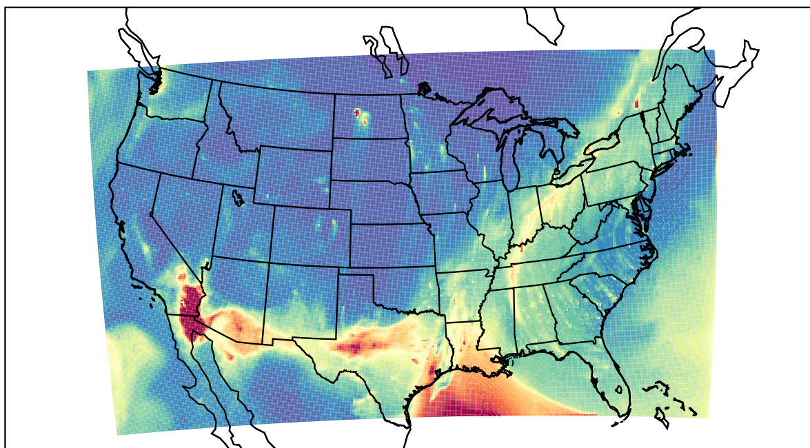
WRF 2022-02-17_14:00:00
