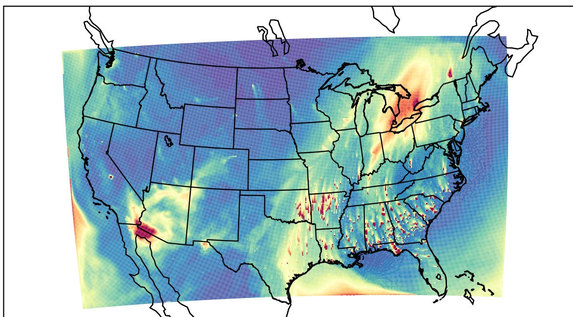
WRF 2022-02-16_21:00:00
