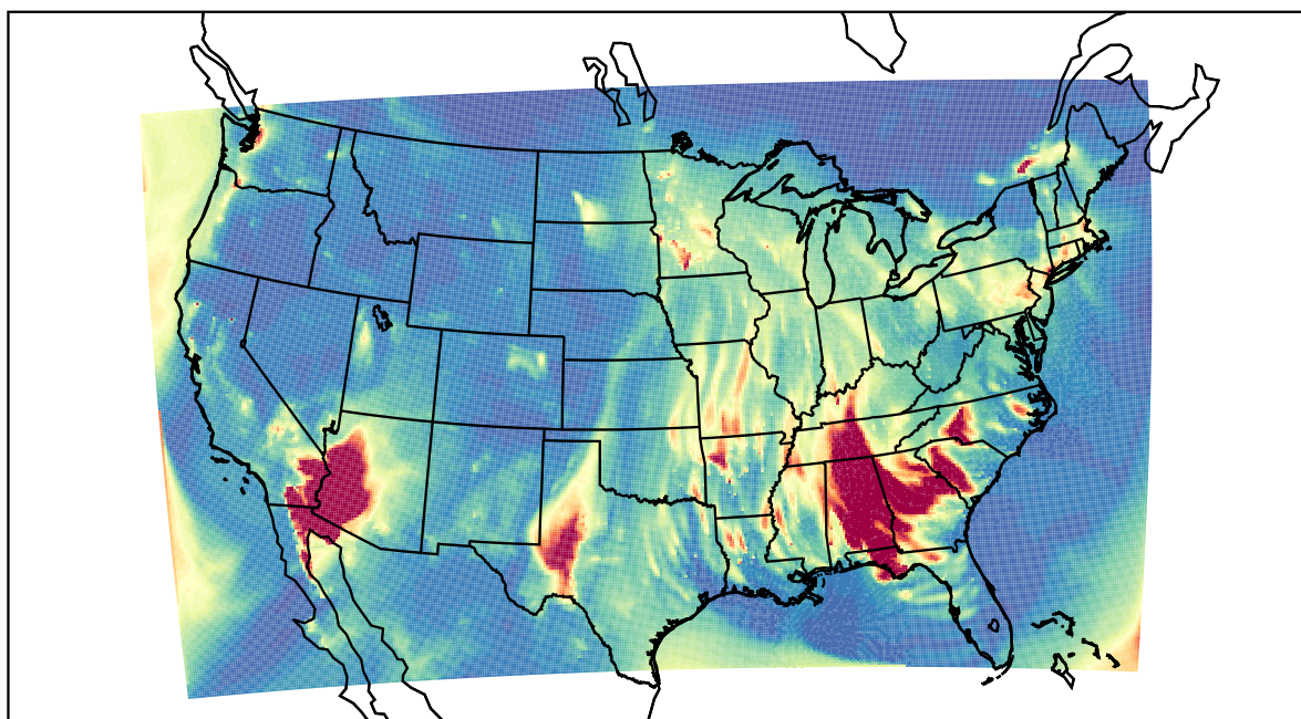
WRF 2022-02-16_05:00:00
