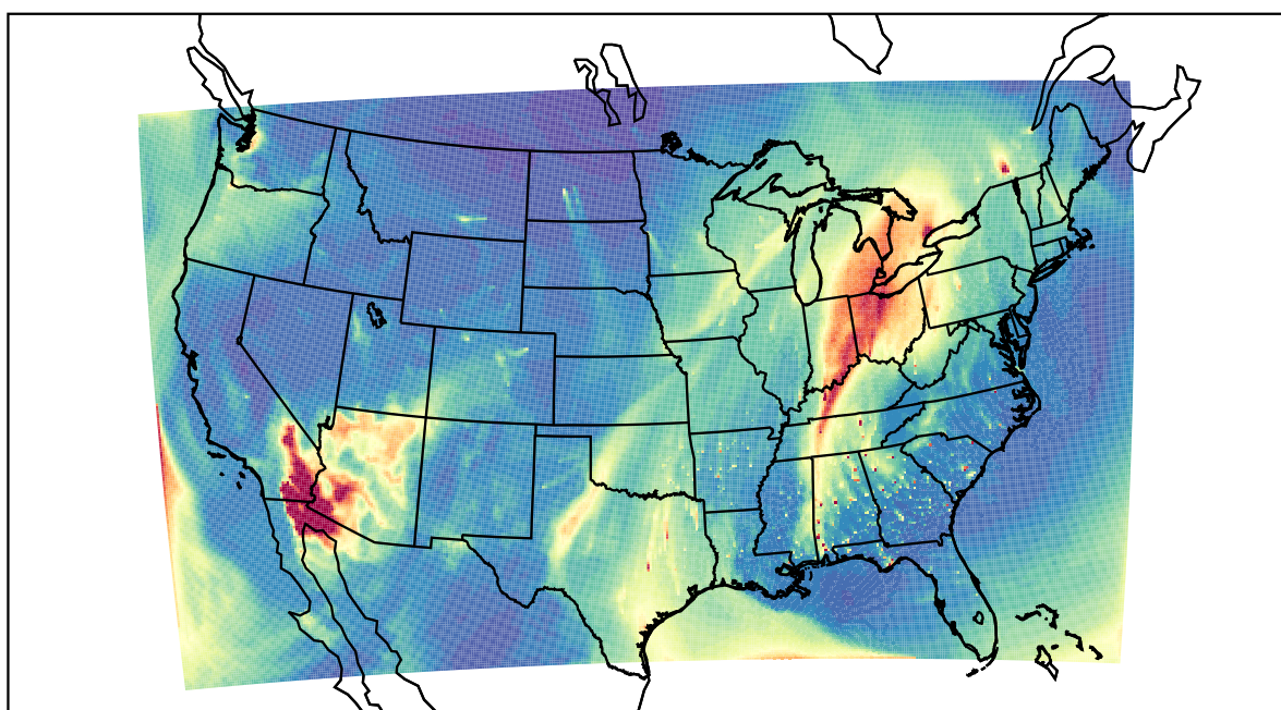
WRF 2022-02-16_17:00:00
