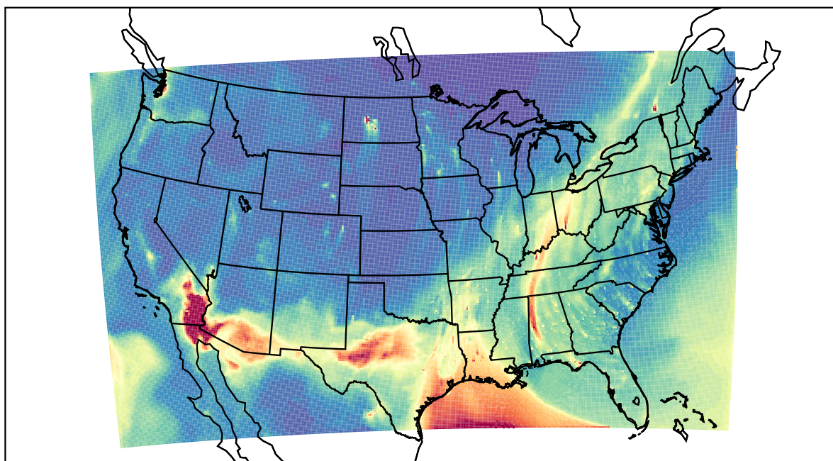
WRF 2022-02-17_12:00:00
