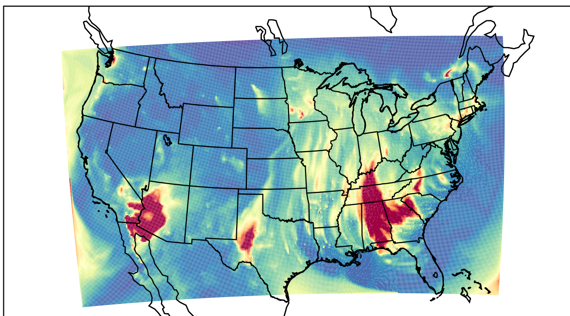
WRF 2022-02-16_07:00:00
