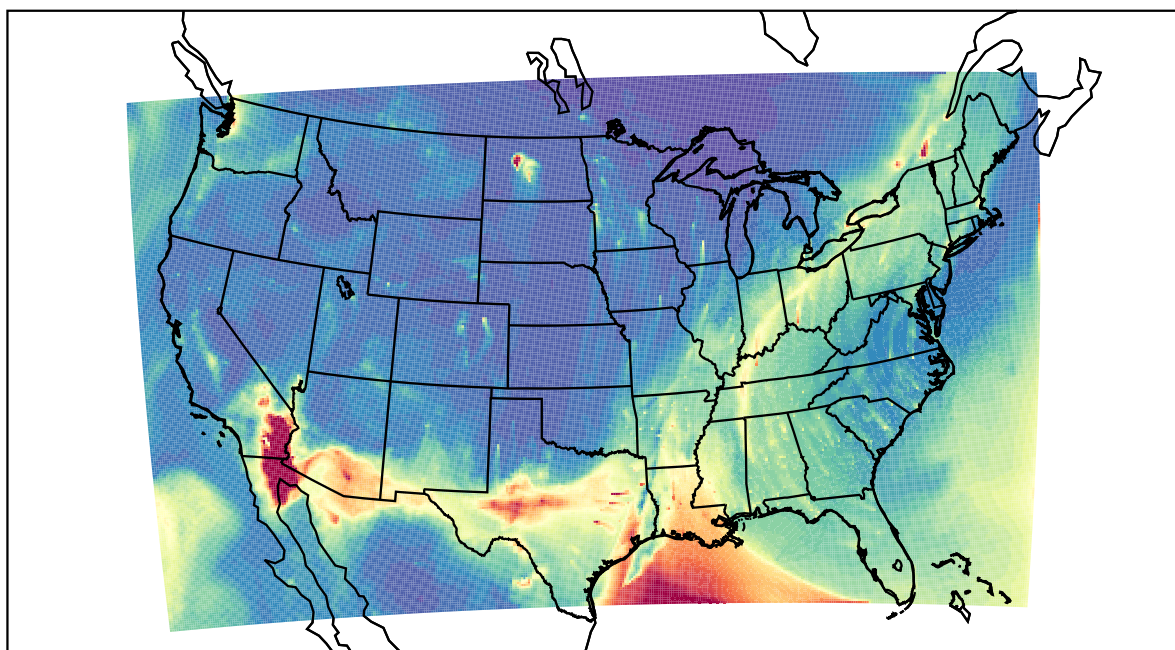
WRF 2022-02-17_15:00:00
