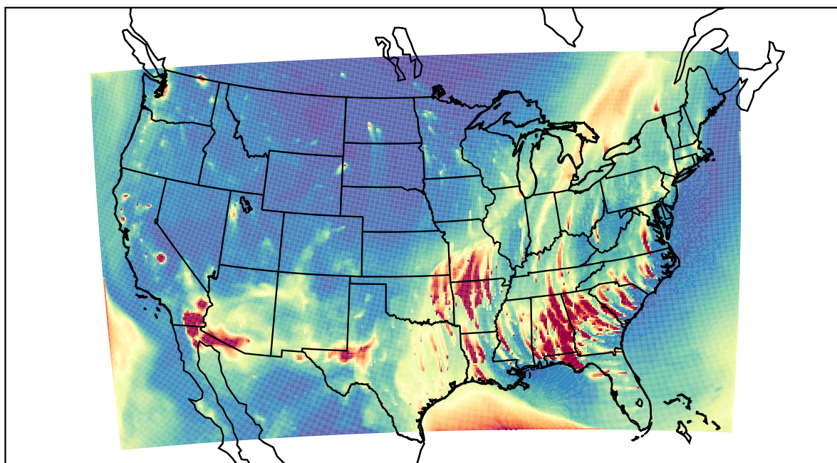
WRF 2022-02-17_02:00:00
