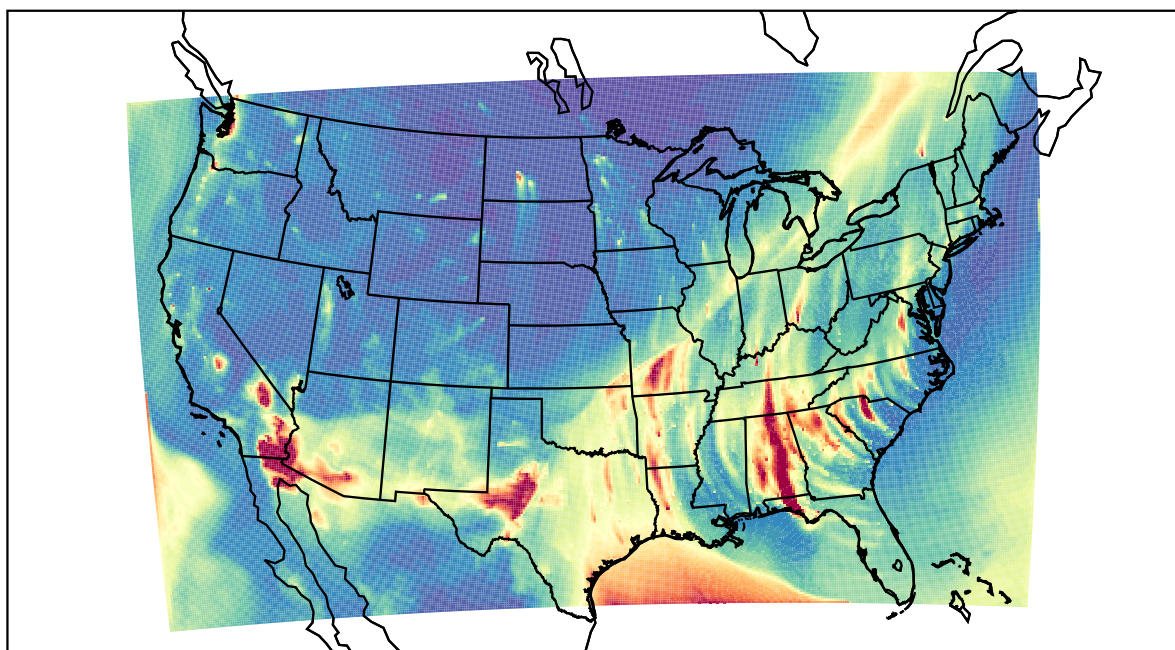
WRF 2022-02-17_05:00:00
