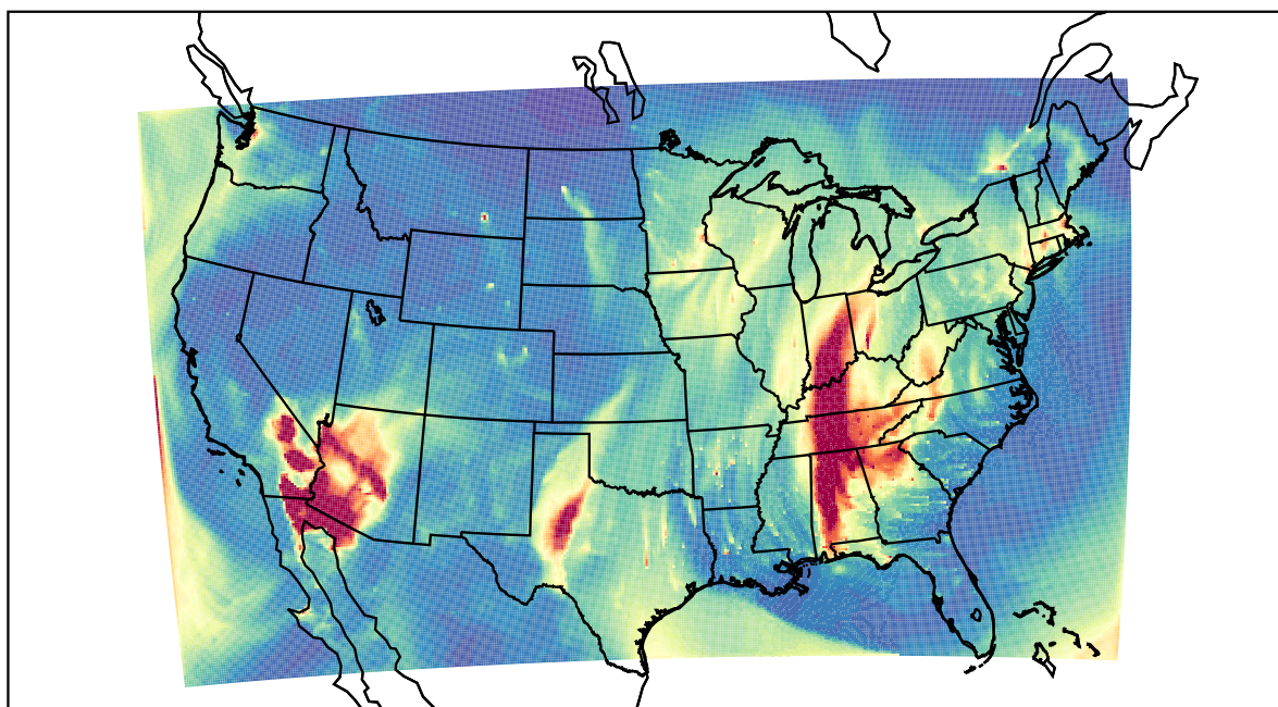
WRF 2022-02-16_11:00:00
