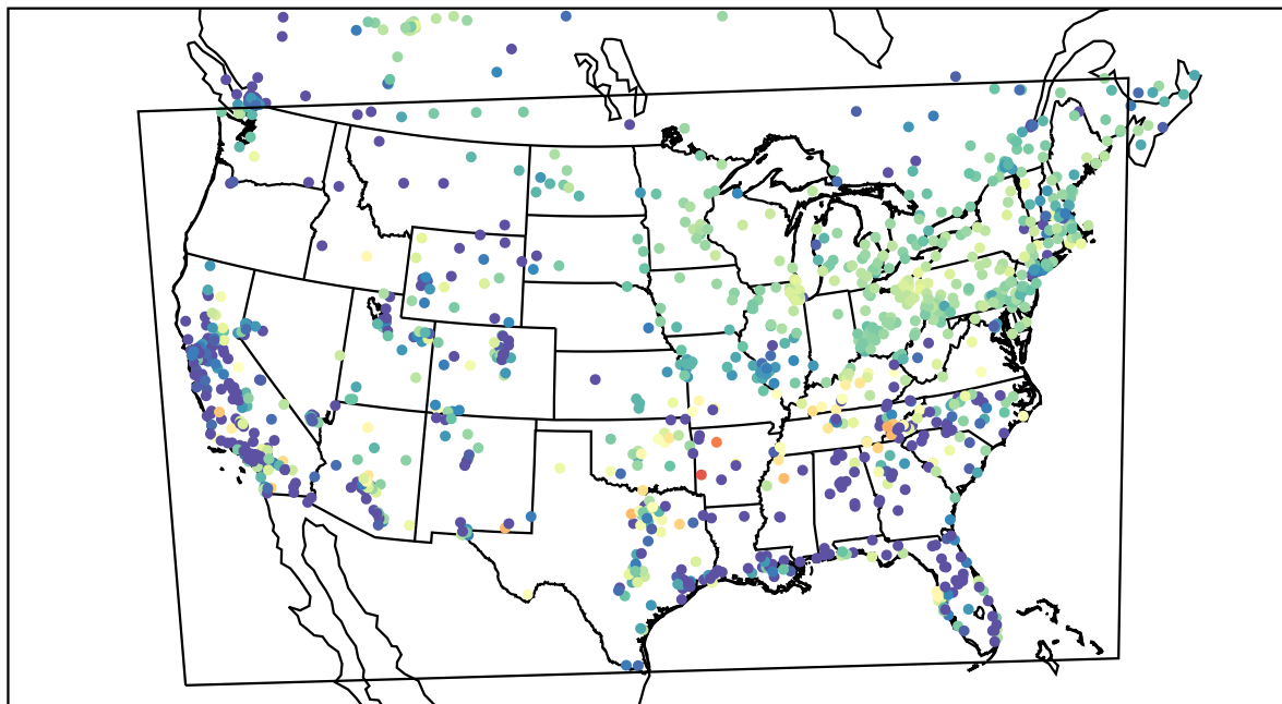
AirNOW (2022-03-03_09:00:00)
