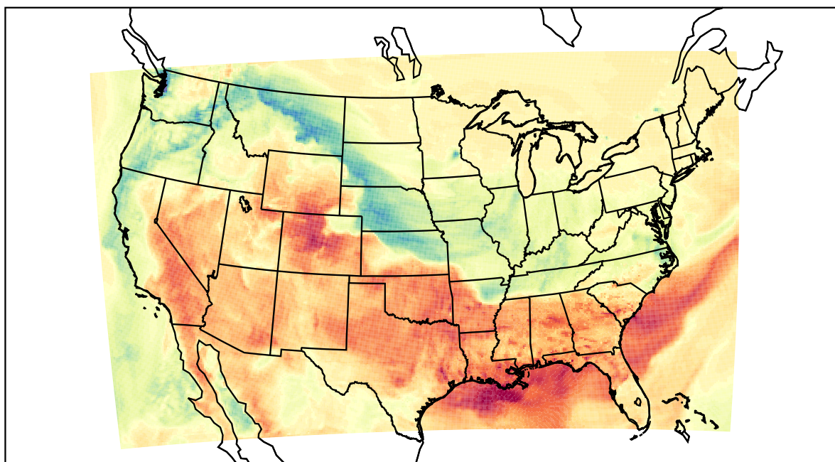
WRF (2022-03-03_22:00:00)
