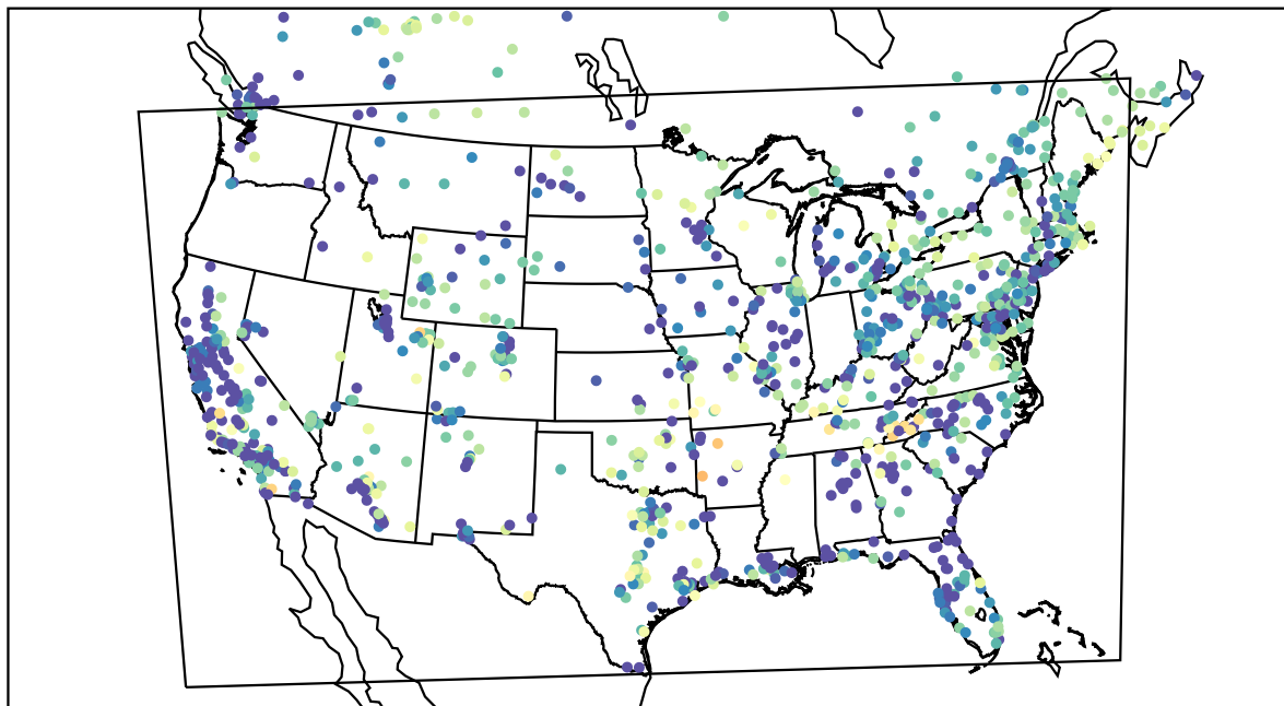
AirNOW (2022-03-02_07:00:00)
