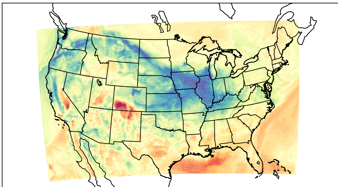
WRF (2022-03-02_17:00:00)
