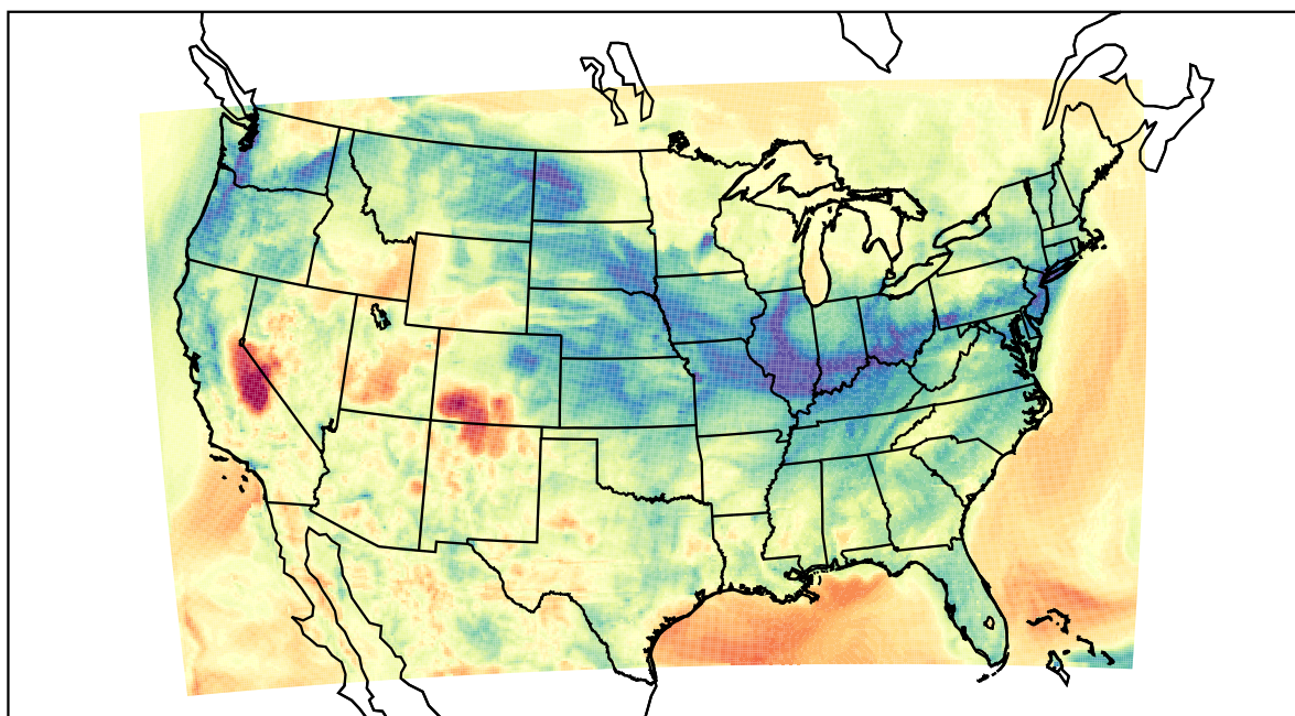
WRF (2022-03-02_07:00:00)
