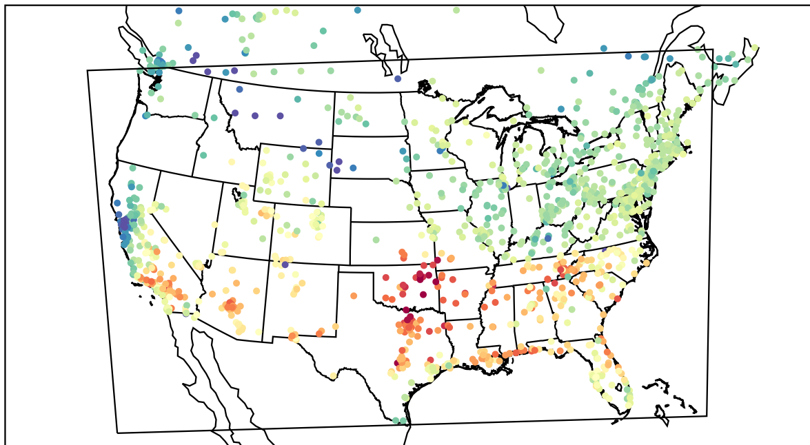
AirNOW (2022-03-03_23:00:00)
