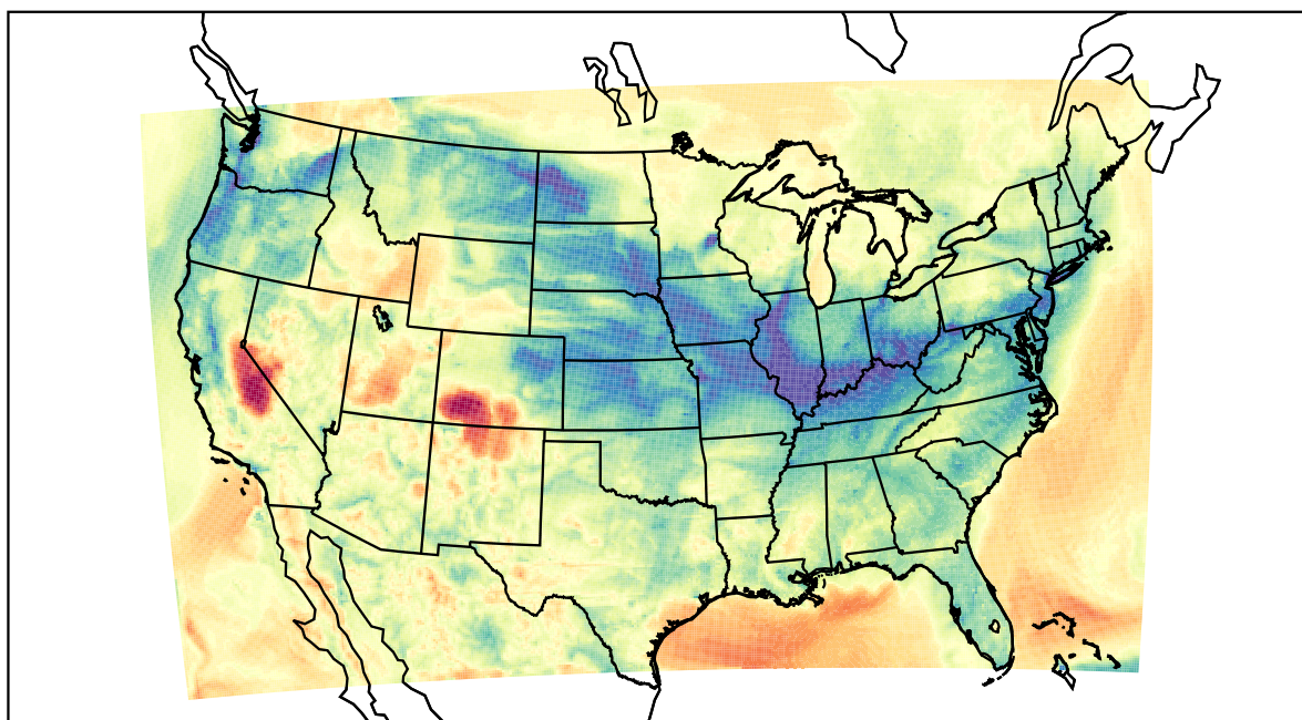
WRF (2022-03-02_09:00:00)
