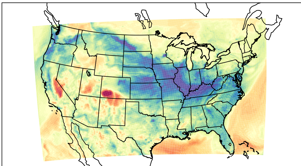
WRF (2022-03-02_13:00:00)
