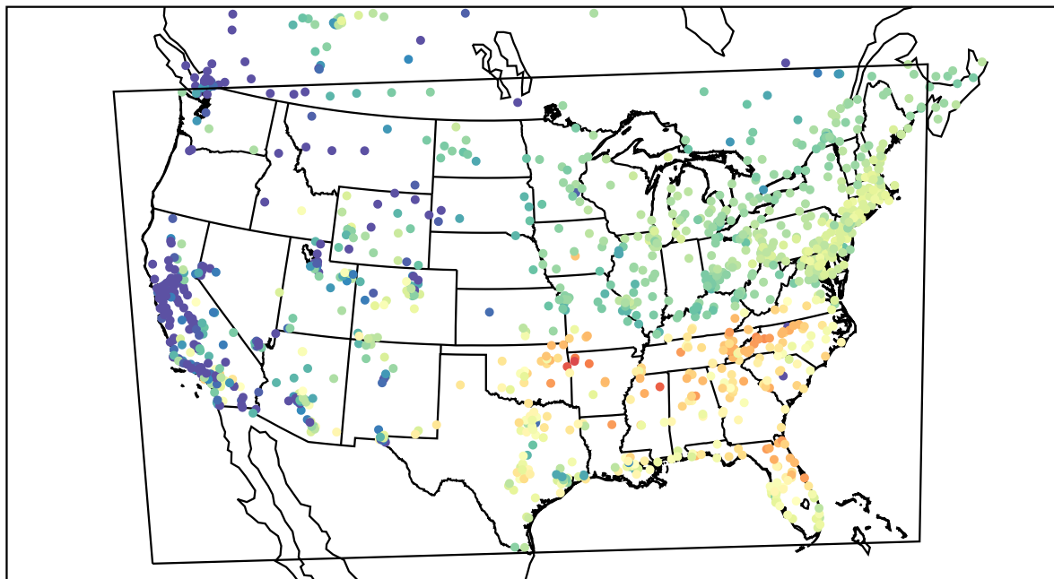
AirNOW (2022-03-03_16:00:00)
