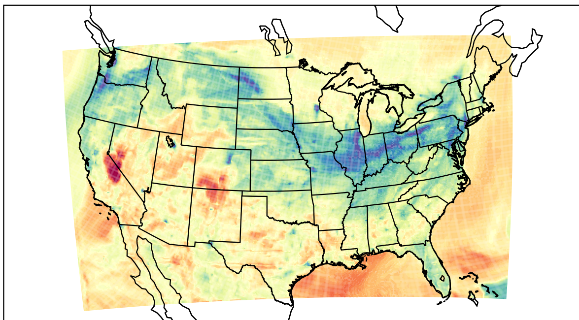
WRF (2022-03-02_02:00:00)
