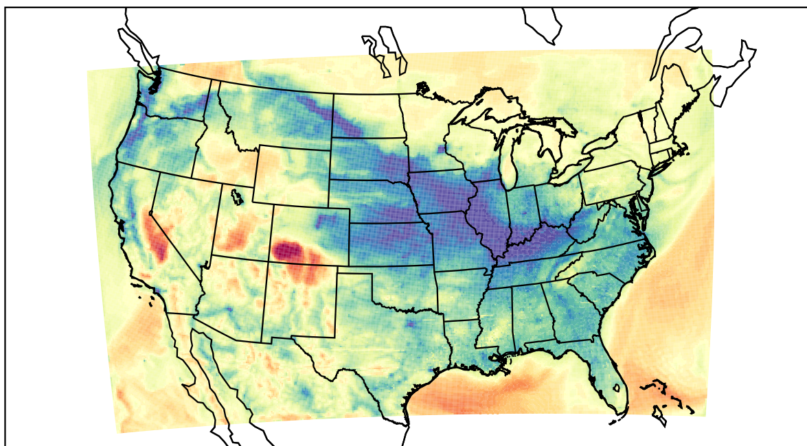
WRF (2022-03-02_14:00:00)
