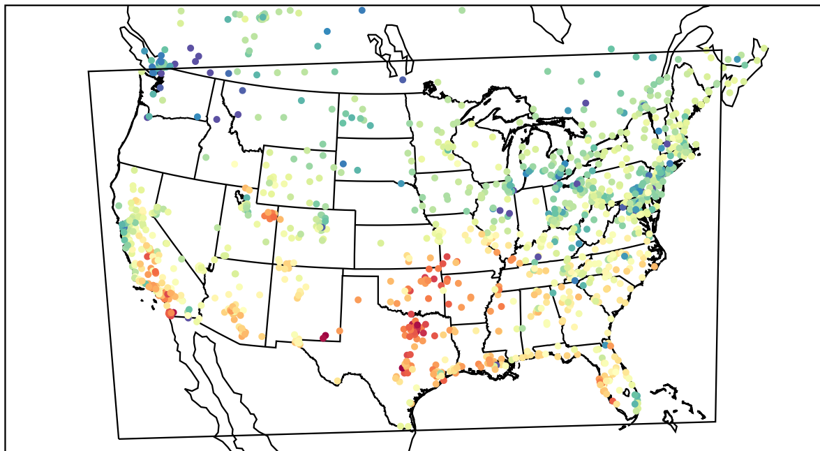
AirNOW (2022-03-02_23:00:00)
