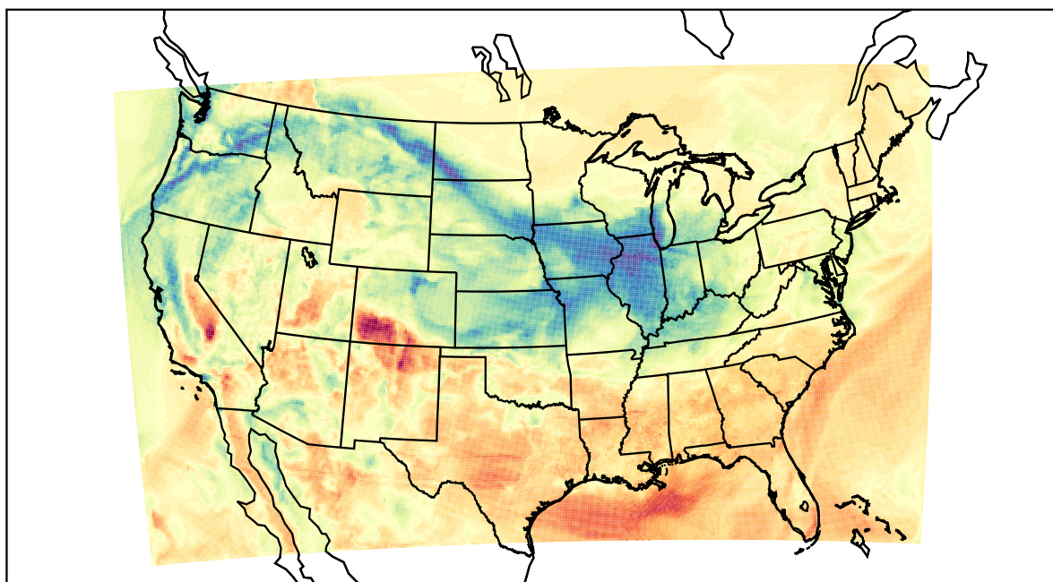
WRF (2022-03-02_18:00:00)
