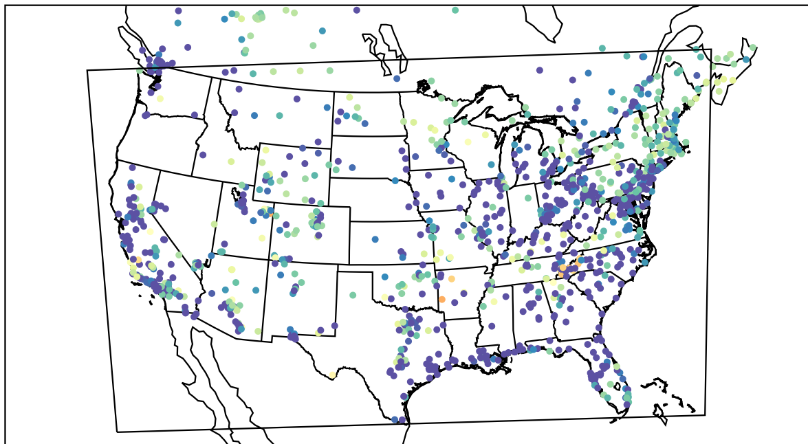
AirNOW (2022-03-02_11:00:00)
