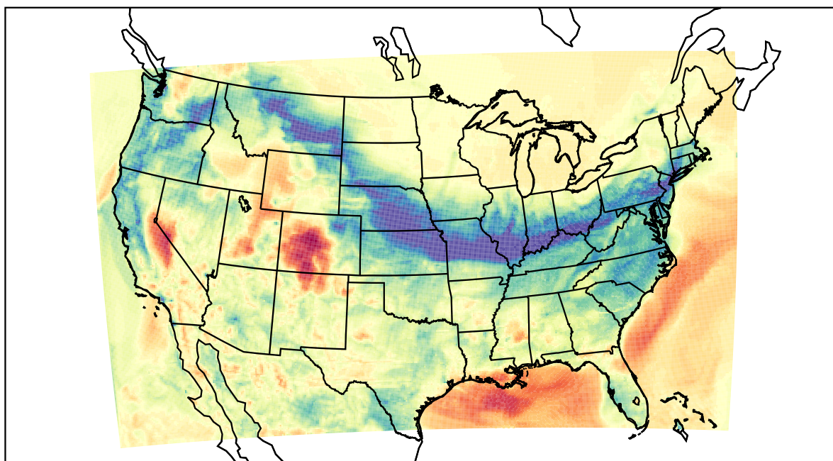
WRF (2022-03-03_08:00:00)
