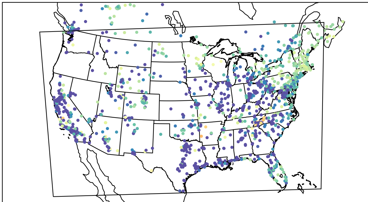
AirNOW (2022-03-02_13:00:00)
