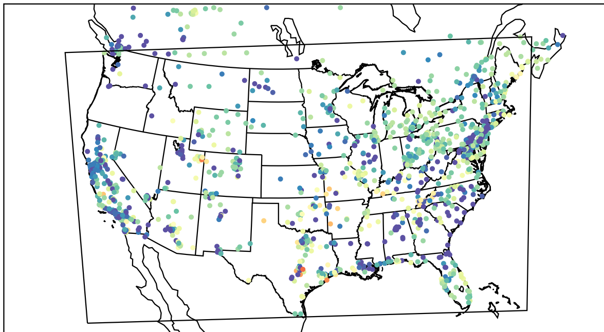
AirNOW (2022-03-02_03:00:00)
