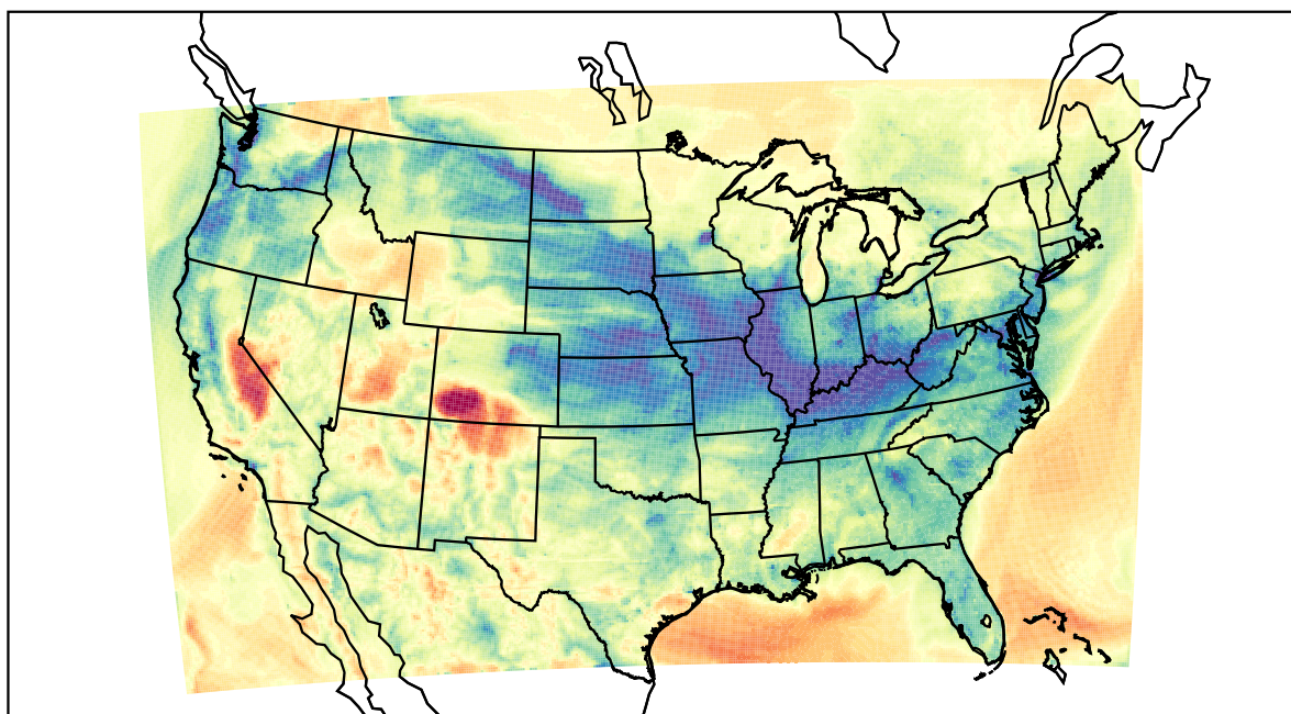
WRF (2022-03-02_12:00:00)
