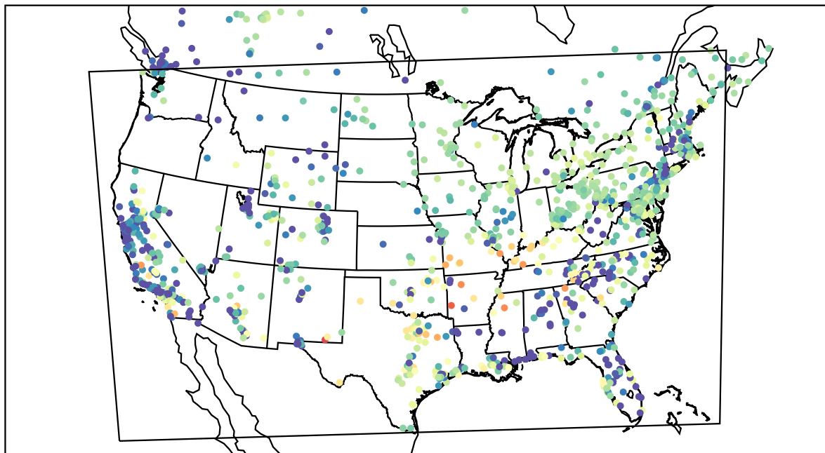
AirNOW (2022-03-03_05:00:00)
