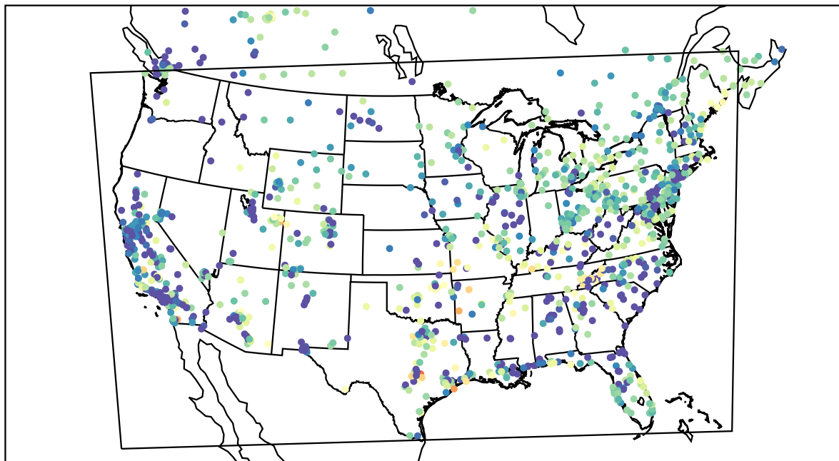
AirNOW (2022-03-02_04:00:00)
