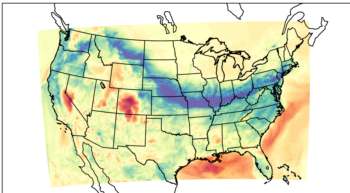
WRF (2022-03-03_07:00:00)
