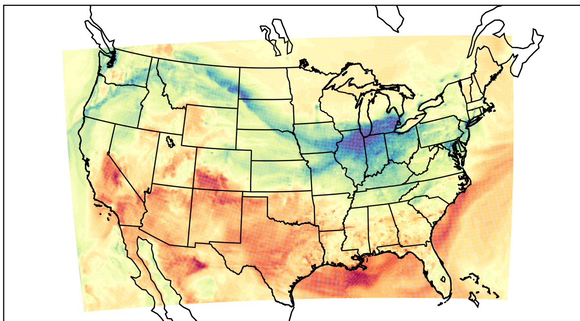
WRF (2022-03-02_23:00:00)
