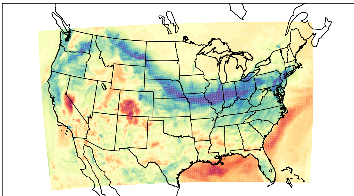
WRF (2022-03-03_04:00:00)
