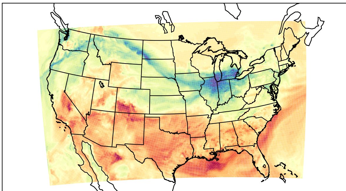
WRF (2022-03-02_22:00:00)
