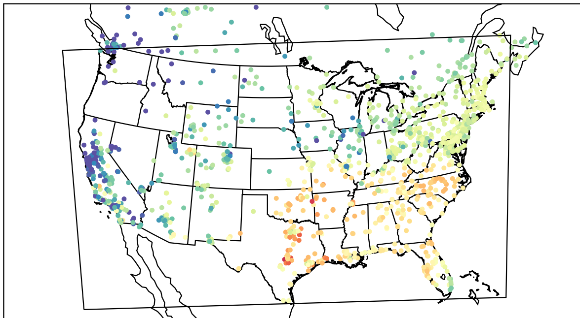
AirNOW (2022-03-02_17:00:00)
