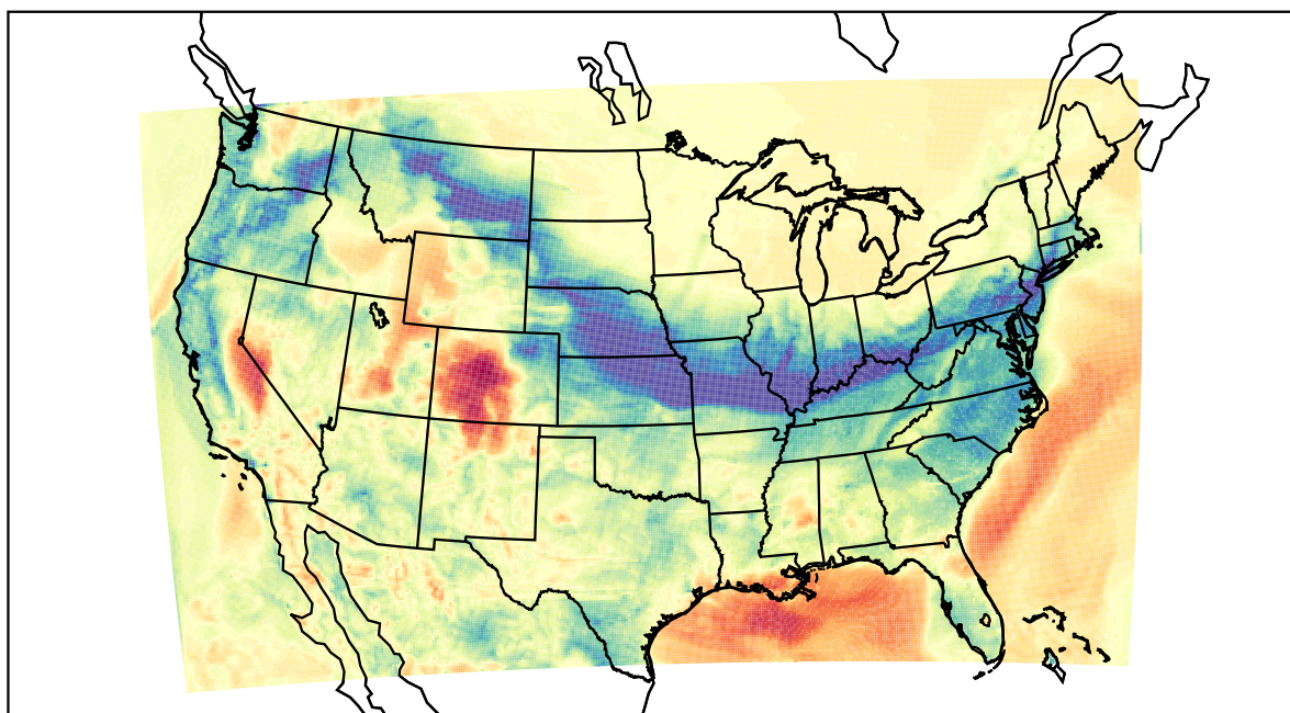
WRF (2022-03-03_09:00:00)
