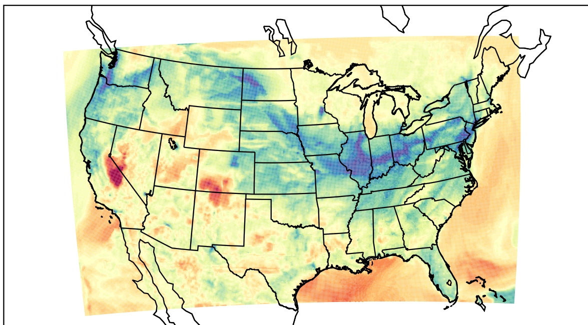
WRF (2022-03-02_04:00:00)
