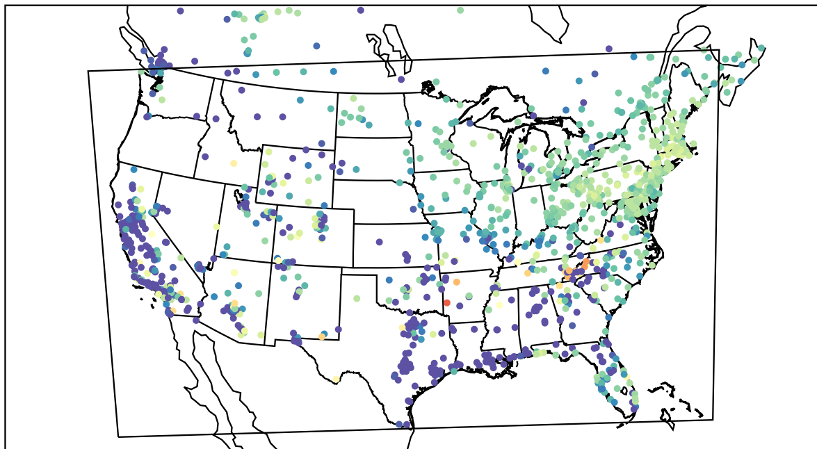
AirNOW (2022-03-03_13:00:00)
