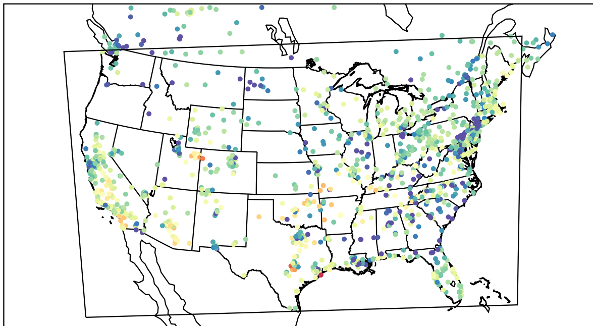
AirNOW (2022-03-02_01:00:00)
