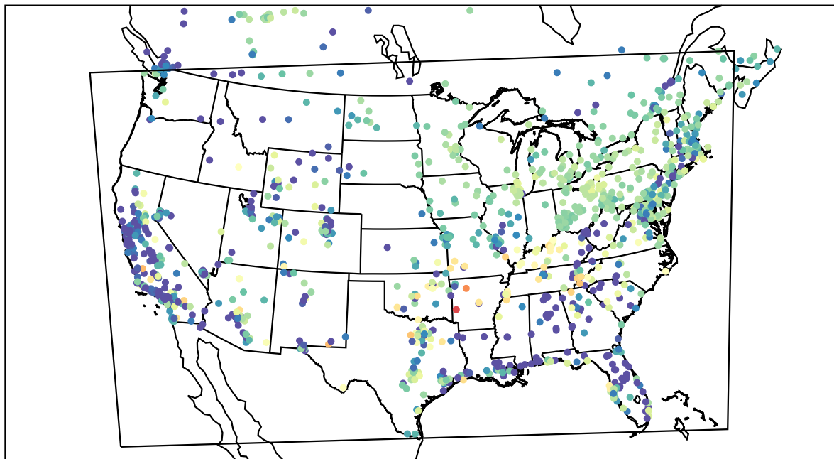
AirNOW (2022-03-03_08:00:00)
