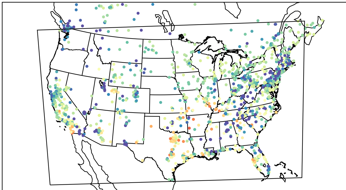
AirNOW (2022-03-03_02:00:00)
