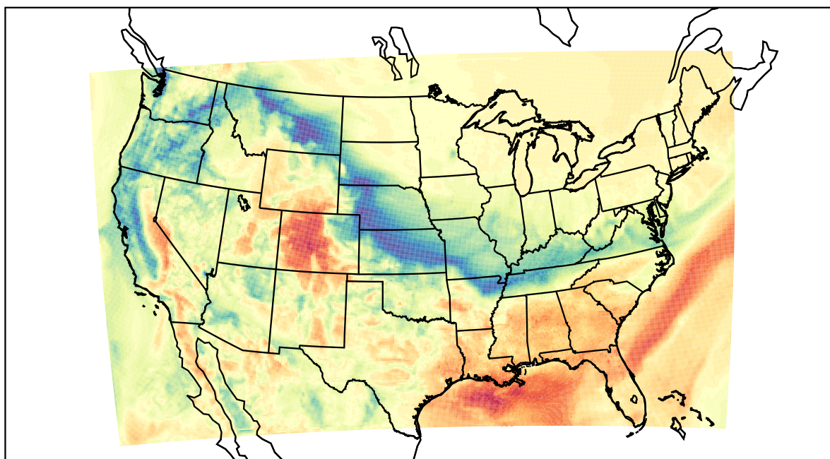
WRF (2022-03-03_17:00:00)
