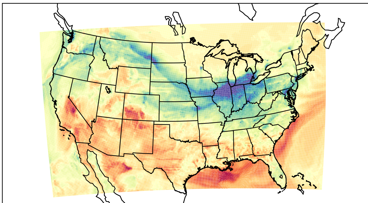
WRF (2022-03-03_00:00:00)
