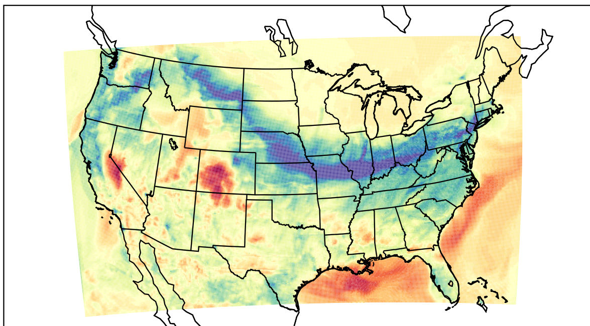
WRF (2022-03-03_06:00:00)
