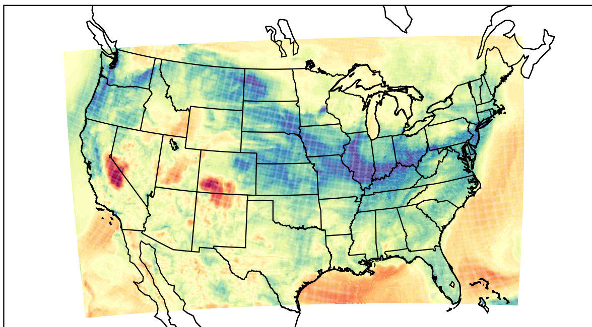
WRF (2022-03-02_08:00:00)
