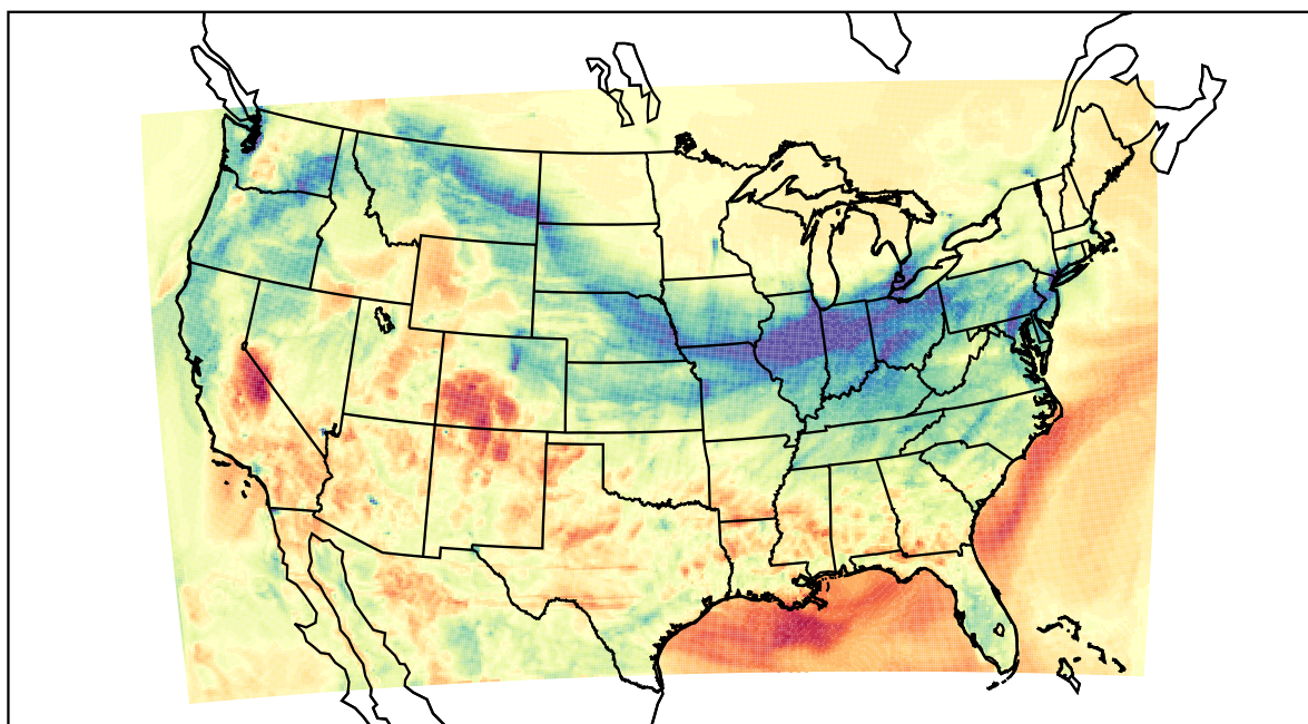
WRF (2022-03-03_02:00:00)
