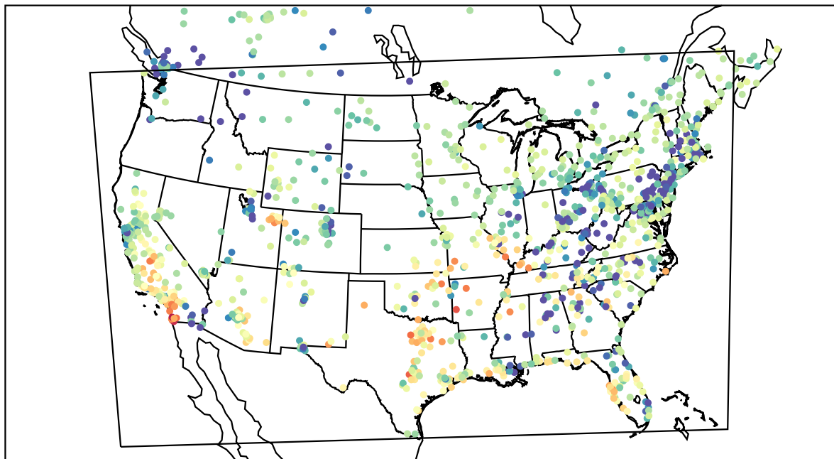
AirNOW (2022-03-03_01:00:00)
