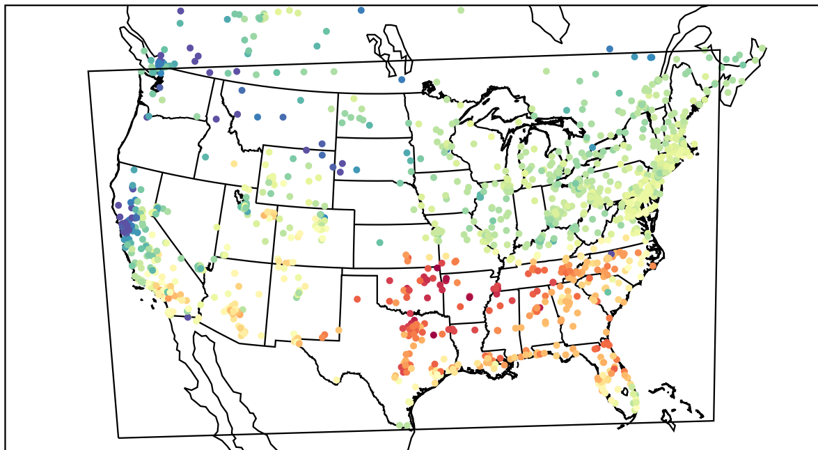
AirNOW (2022-03-03_19:00:00)
