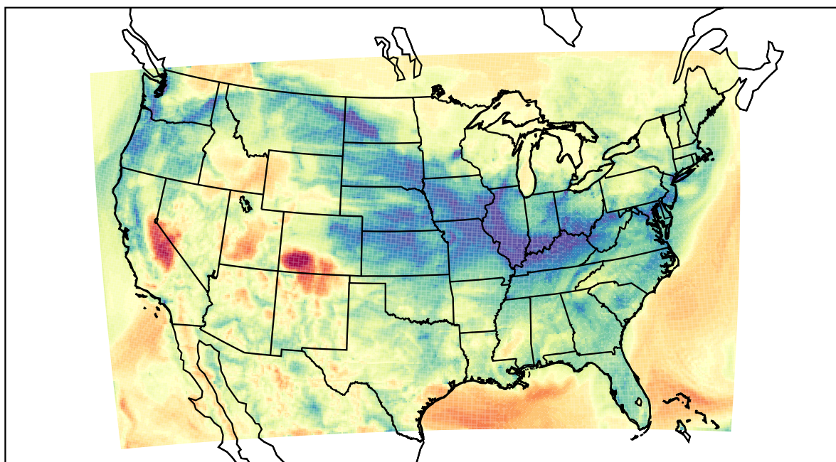
WRF (2022-03-02_11:00:00)
