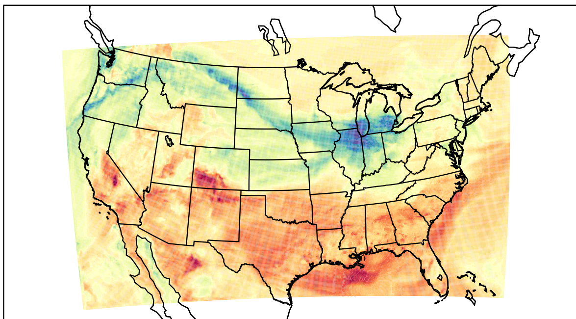
WRF (2022-03-02_21:00:00)
