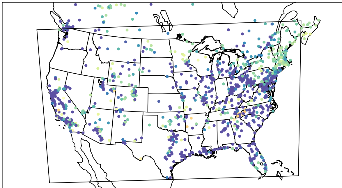
AirNOW (2022-03-02_12:00:00)
