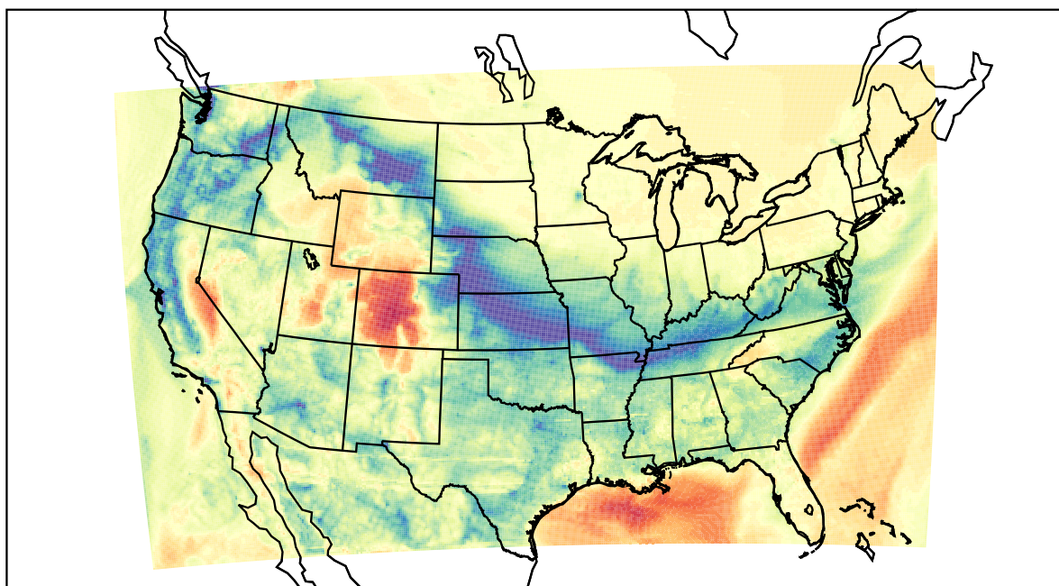
WRF (2022-03-03_15:00:00)
