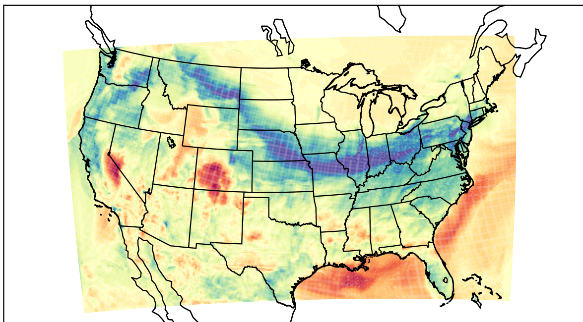
WRF (2022-03-03_05:00:00)
