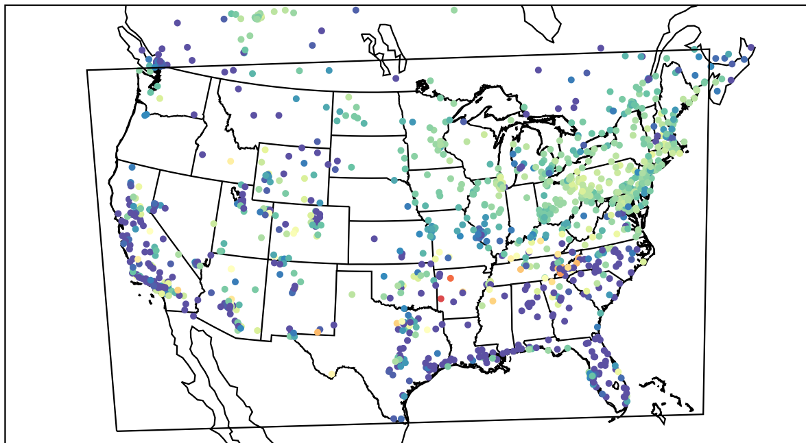
AirNOW (2022-03-03_11:00:00)
