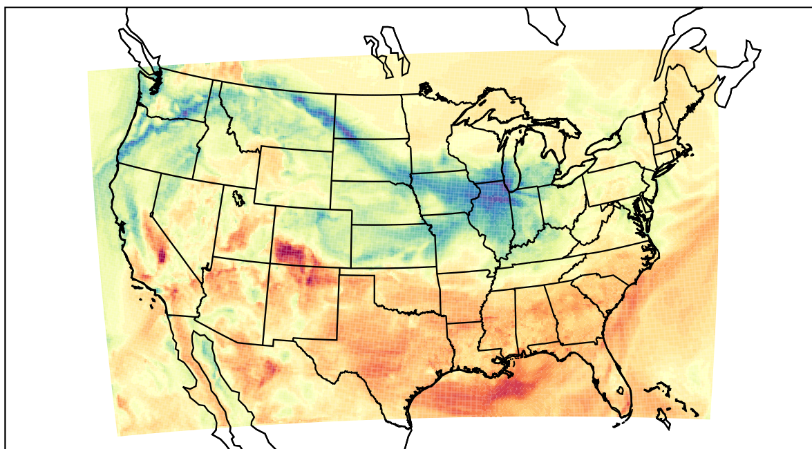
WRF (2022-03-02_19:00:00)
