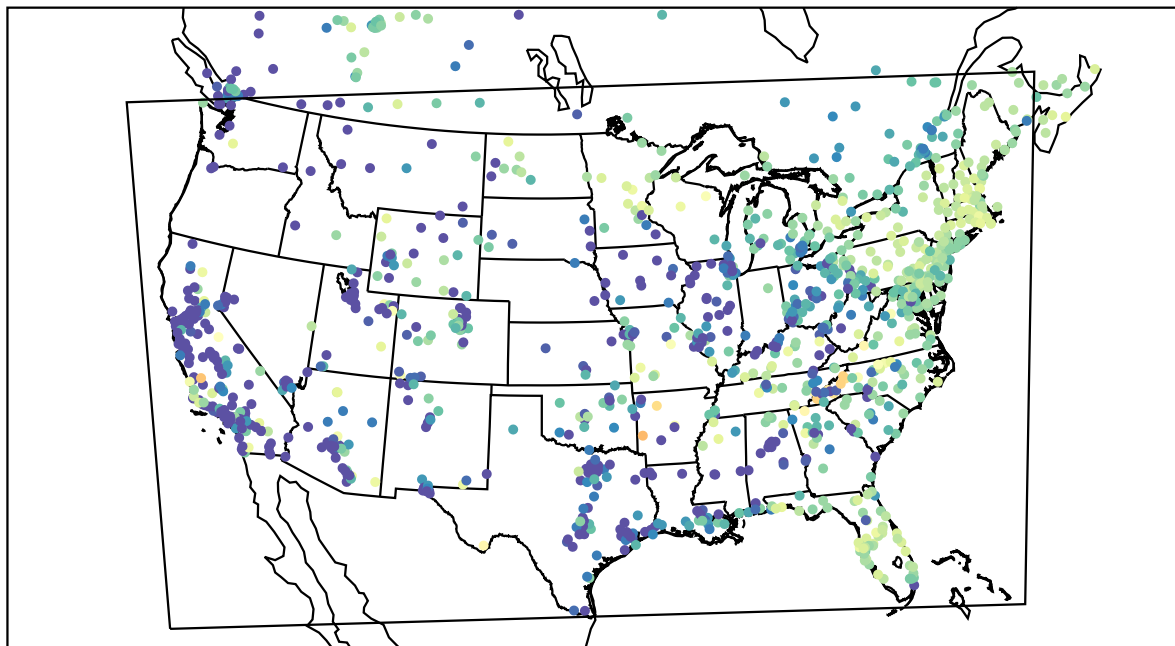
AirNOW (2022-03-02_14:00:00)
