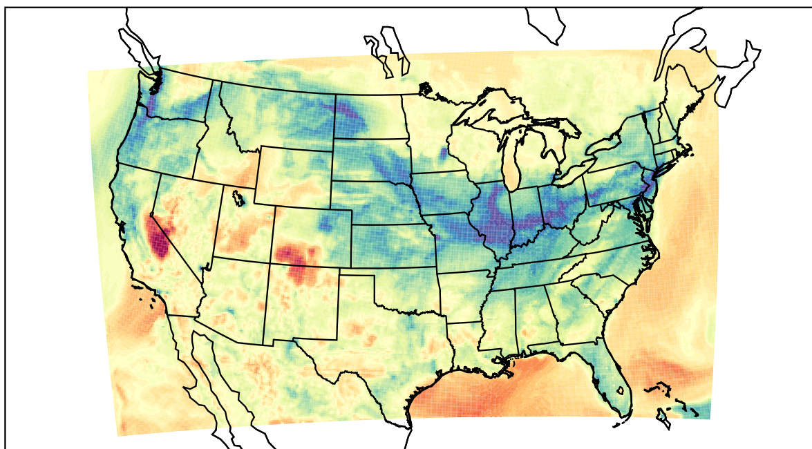
WRF (2022-03-02_05:00:00)
