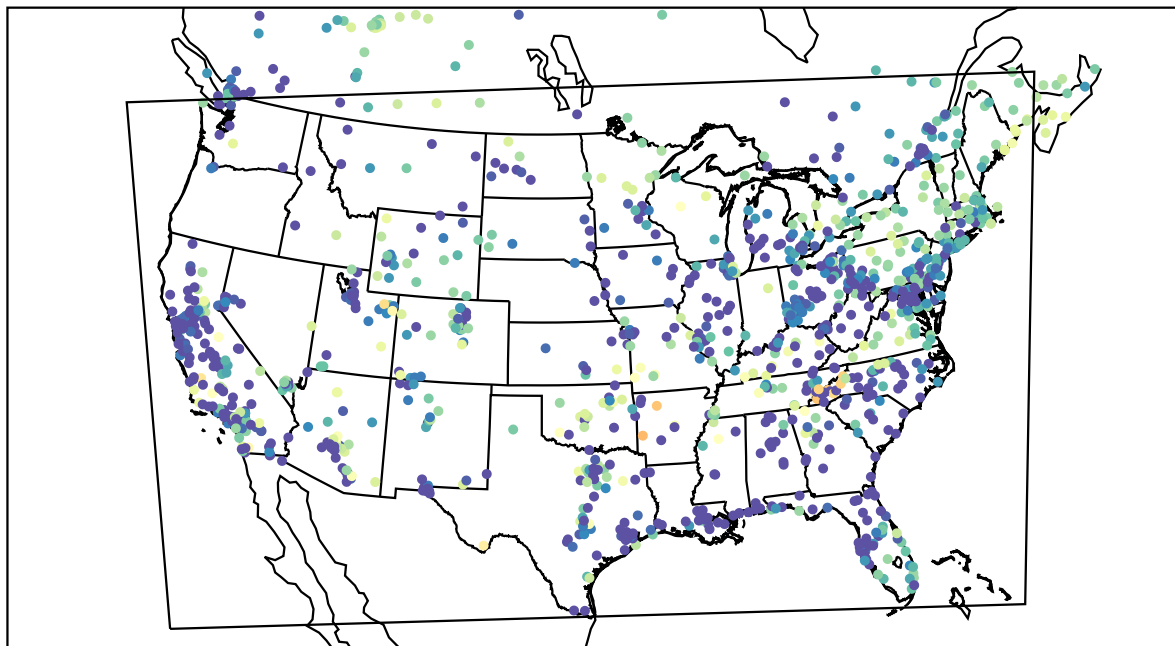
AirNOW (2022-03-02_09:00:00)
