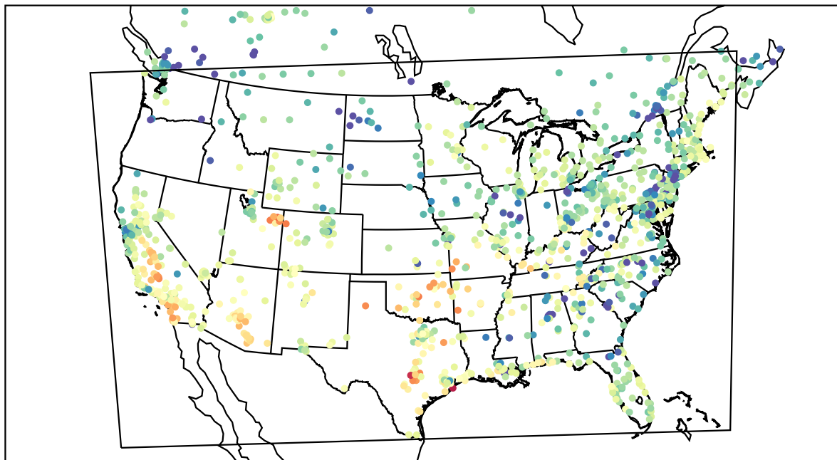
AirNOW (2022-03-02_00:00:00)
