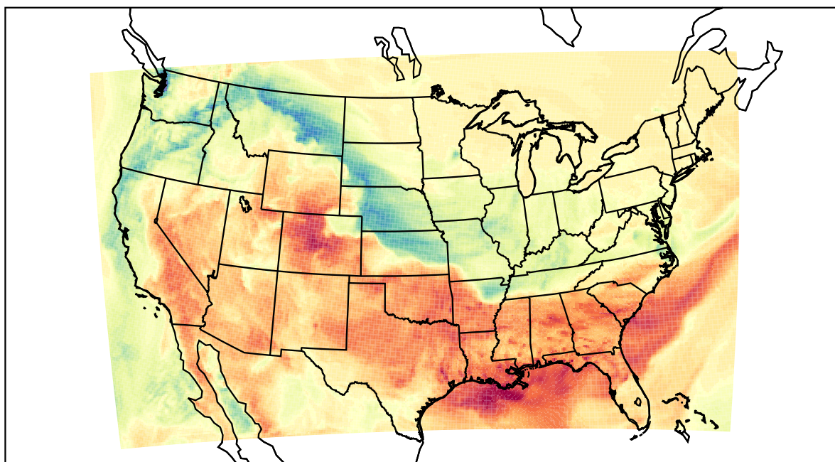
WRF (2022-03-03_21:00:00)
