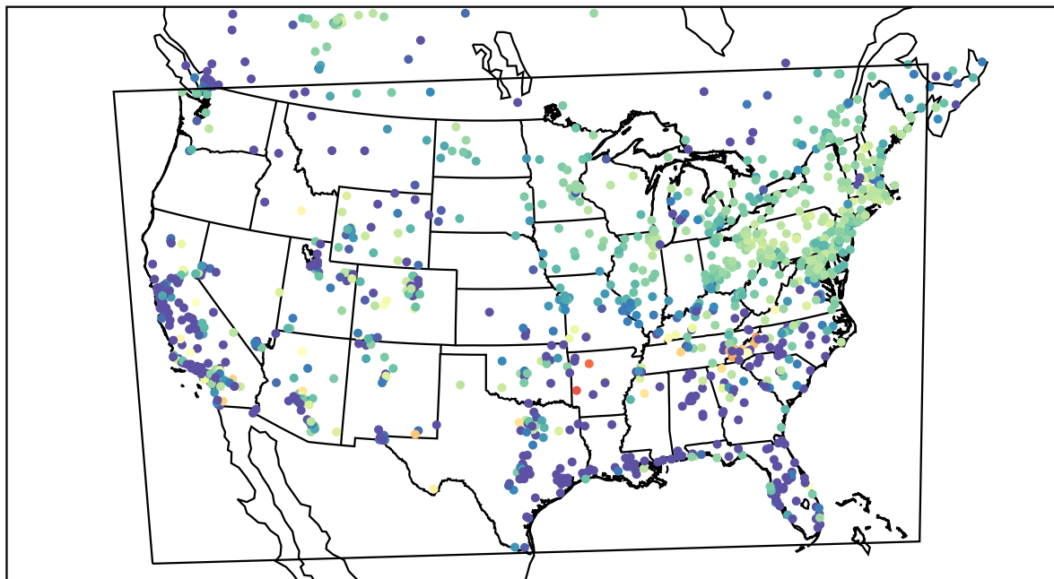
AirNOW (2022-03-03_12:00:00)
