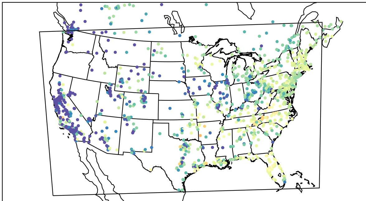
AirNOW (2022-03-02_15:00:00)
