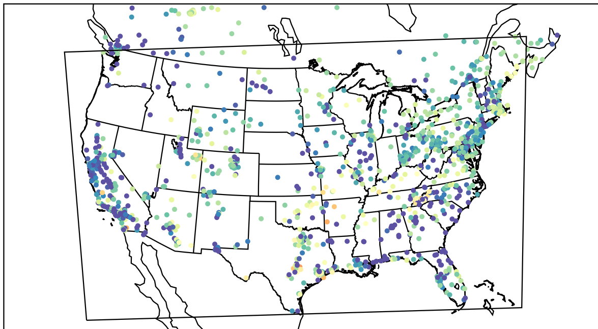
AirNOW (2022-03-02_05:00:00)
