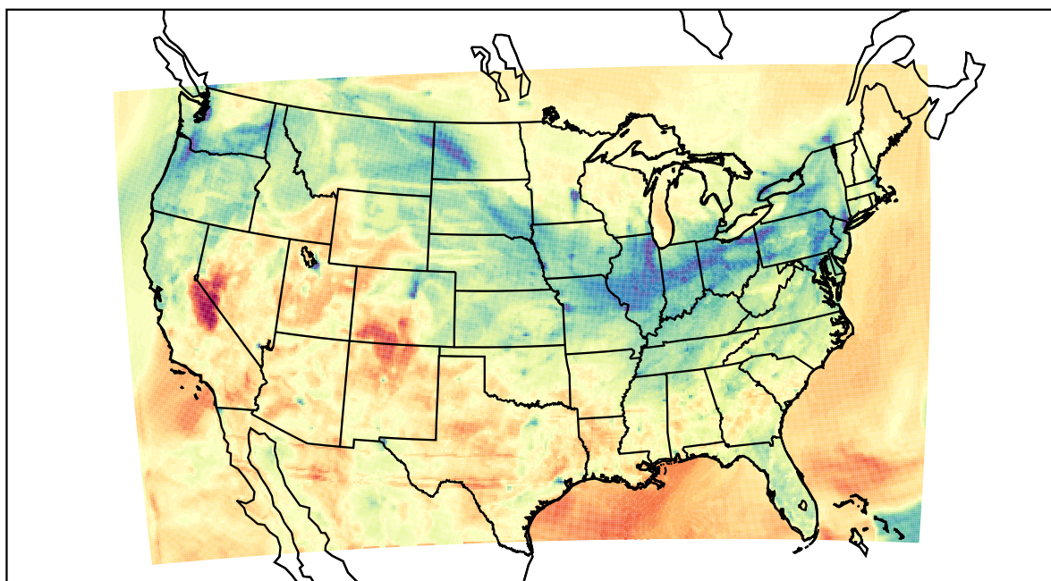
WRF (2022-03-02_01:00:00)
