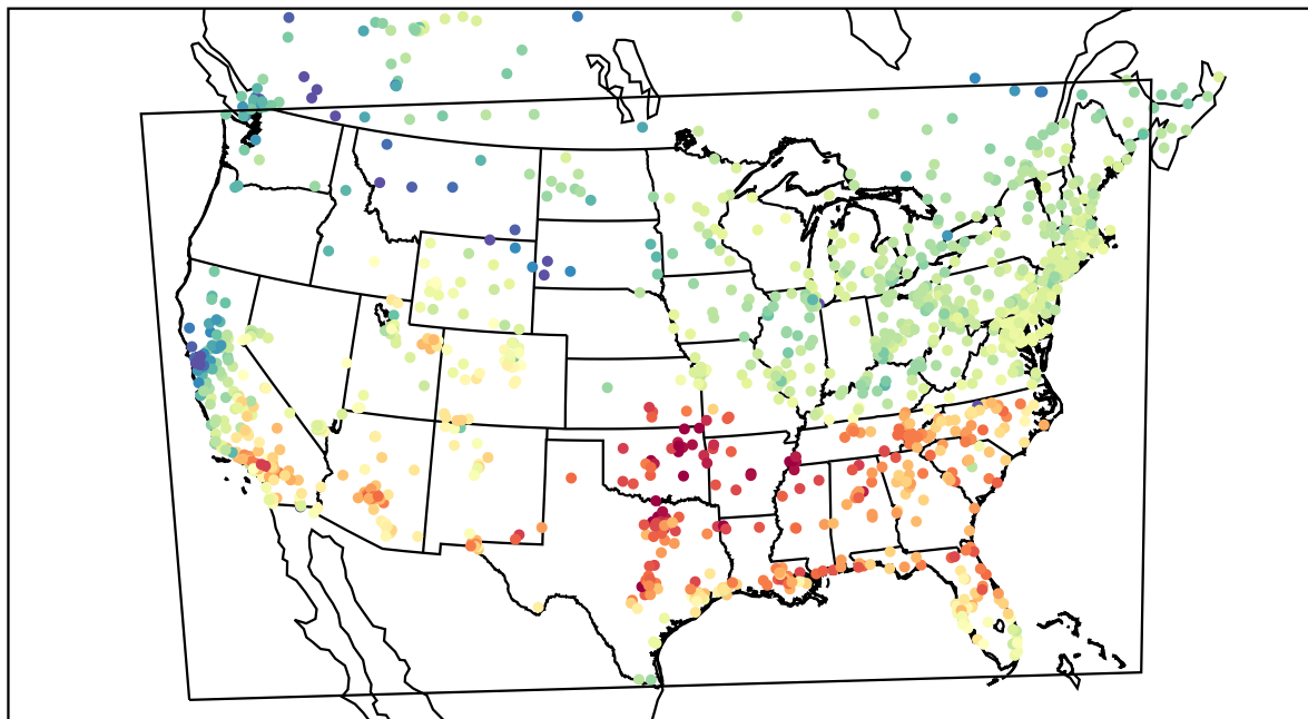
AirNOW (2022-03-03_21:00:00)
