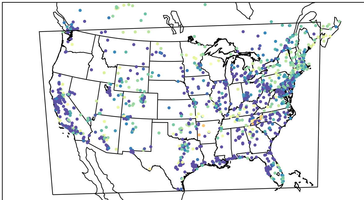
AirNOW (2022-03-02_10:00:00)
