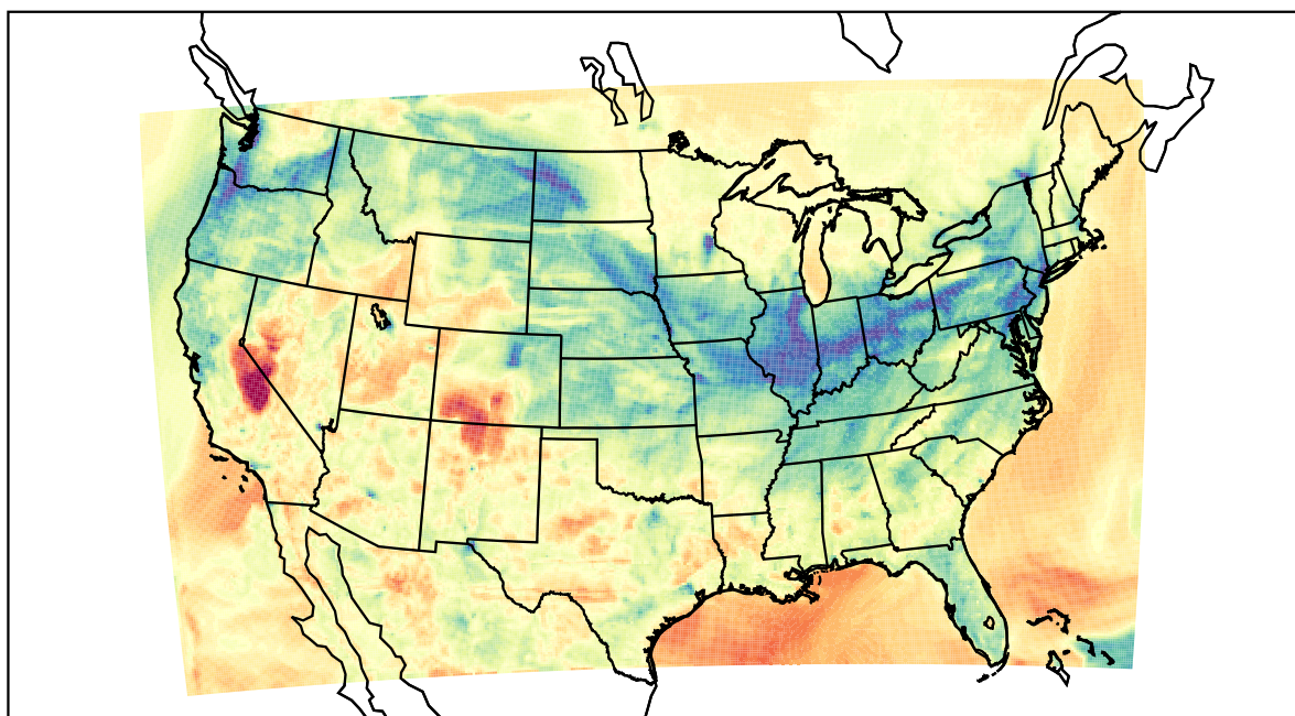
WRF (2022-03-02_03:00:00)
