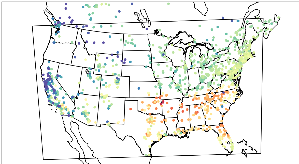
AirNOW (2022-03-03_17:00:00)
