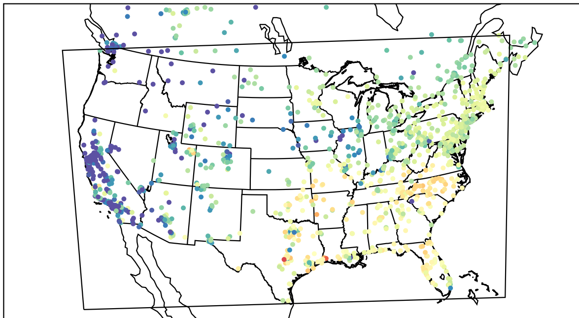
AirNOW (2022-03-02_16:00:00)
