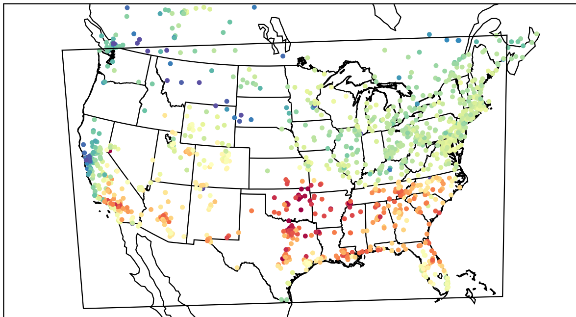
AirNOW (2022-03-03_22:00:00)
