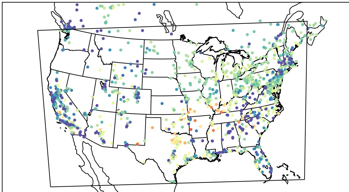
AirNOW (2022-03-03_04:00:00)
