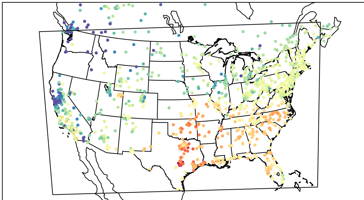
AirNOW (2022-03-02_18:00:00)
