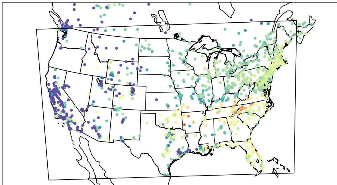
AirNOW (2022-03-03_15:00:00)
