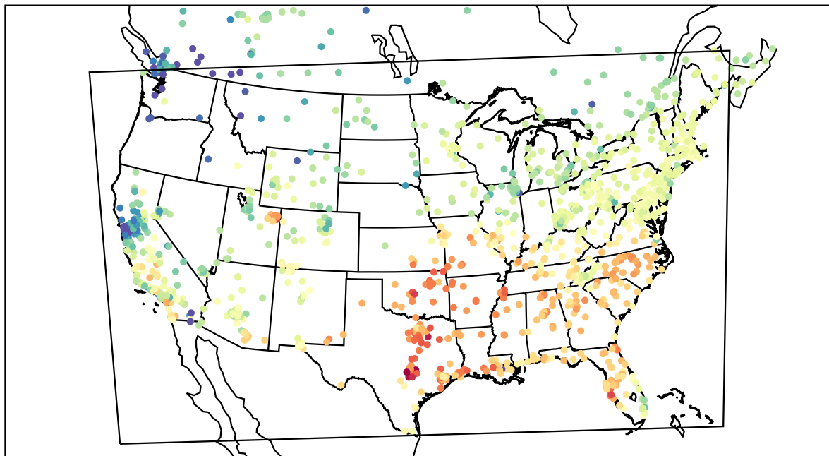
AirNOW (2022-03-02_19:00:00)
