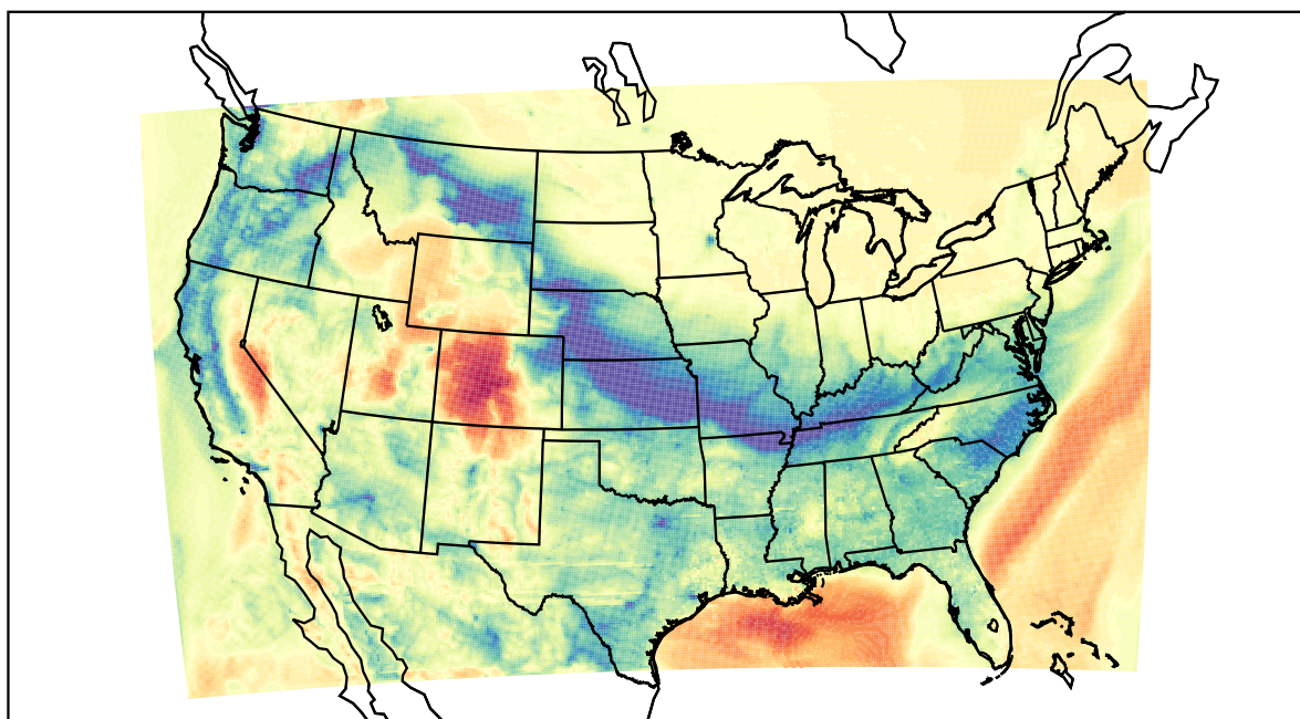
WRF (2022-03-03_14:00:00)
