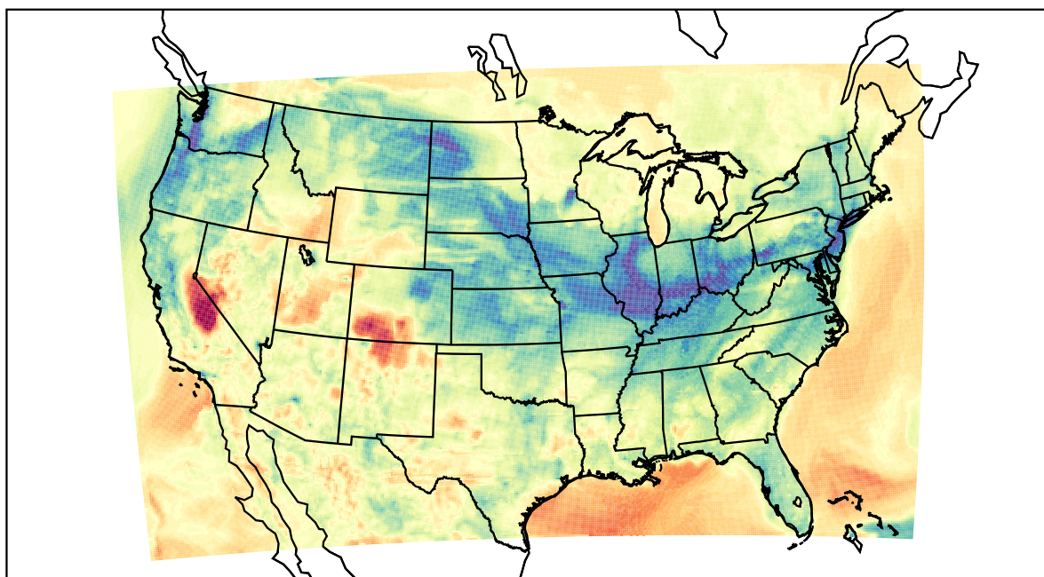
WRF (2022-03-02_06:00:00)
