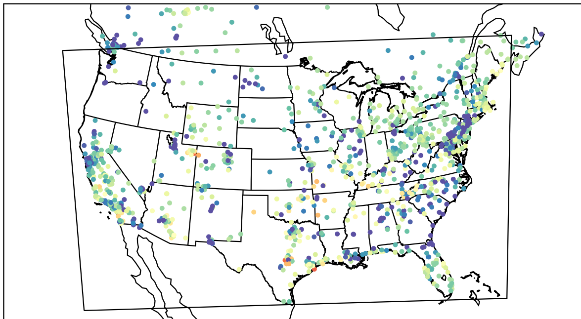
AirNOW (2022-03-02_02:00:00)
