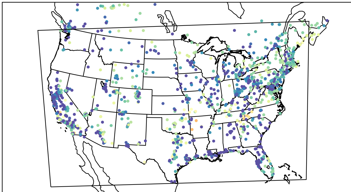
AirNOW (2022-03-02_08:00:00)
