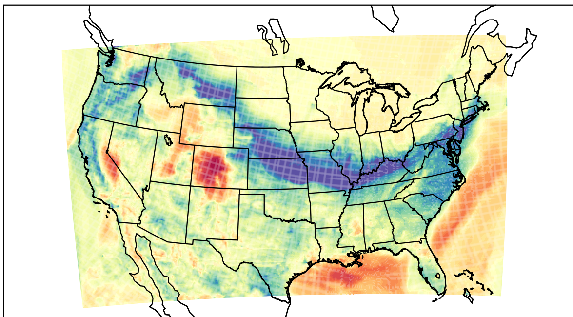
WRF (2022-03-03_11:00:00)
