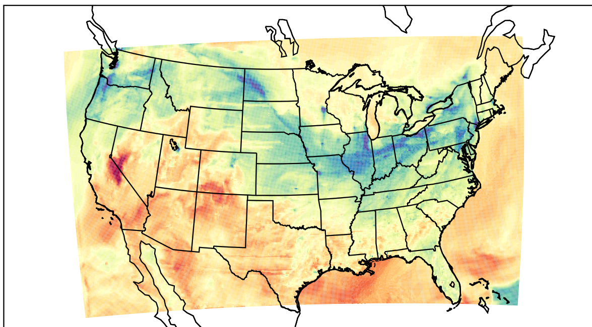
WRF (2022-03-02_00:00:00)
