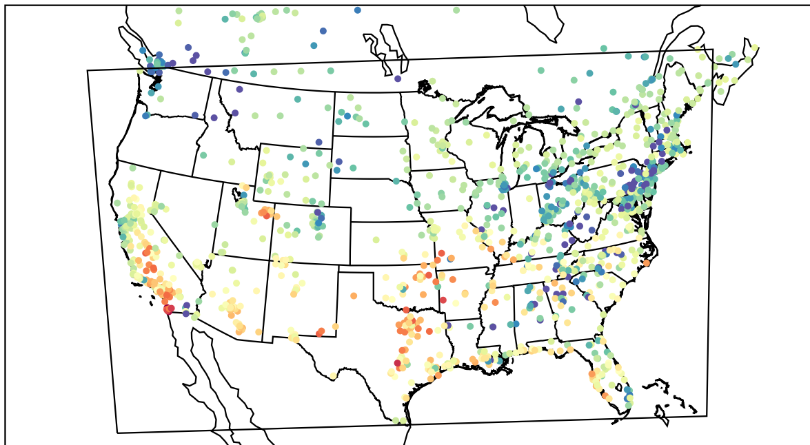
AirNOW (2022-03-03_00:00:00)
