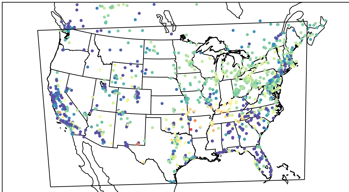
AirNOW (2022-03-03_07:00:00)
