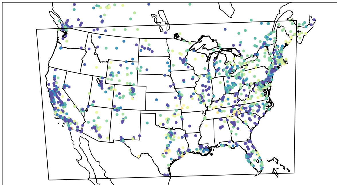
AirNOW (2022-03-02_06:00:00)
