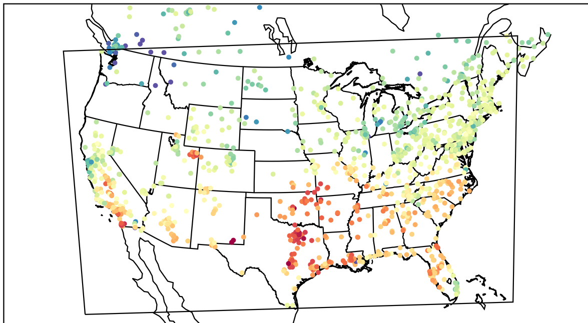
AirNOW (2022-03-02_22:00:00)
