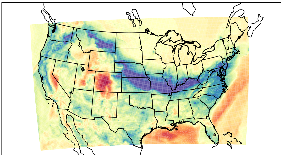
WRF (2022-03-03_12:00:00)
