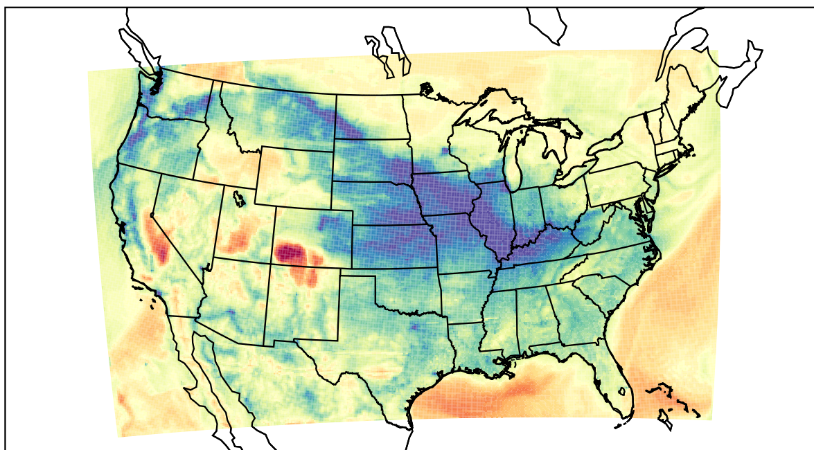
WRF (2022-03-02_15:00:00)
