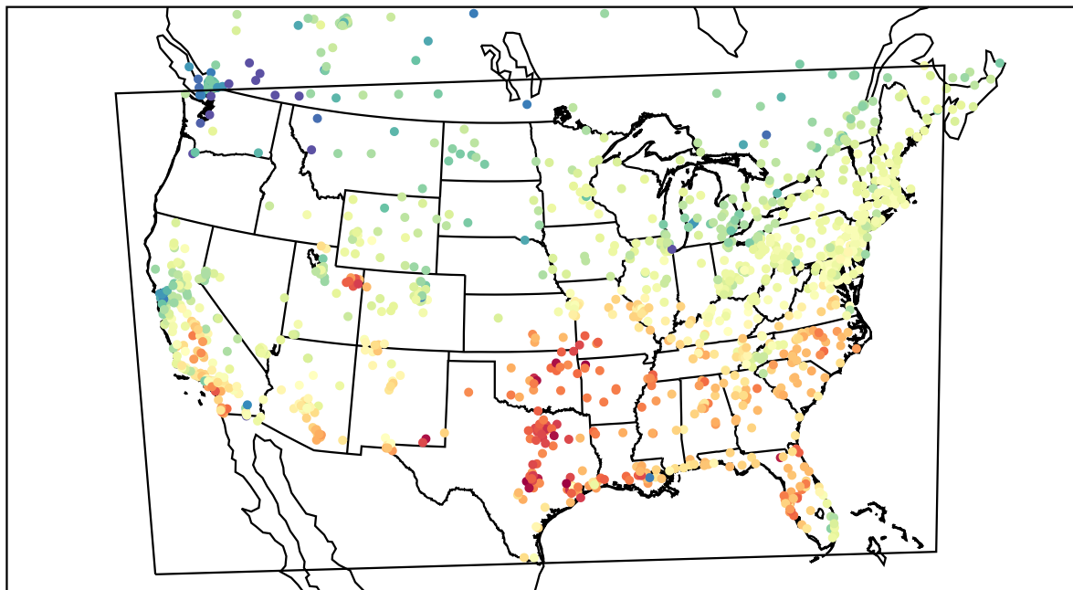
AirNOW (2022-03-02_21:00:00)
