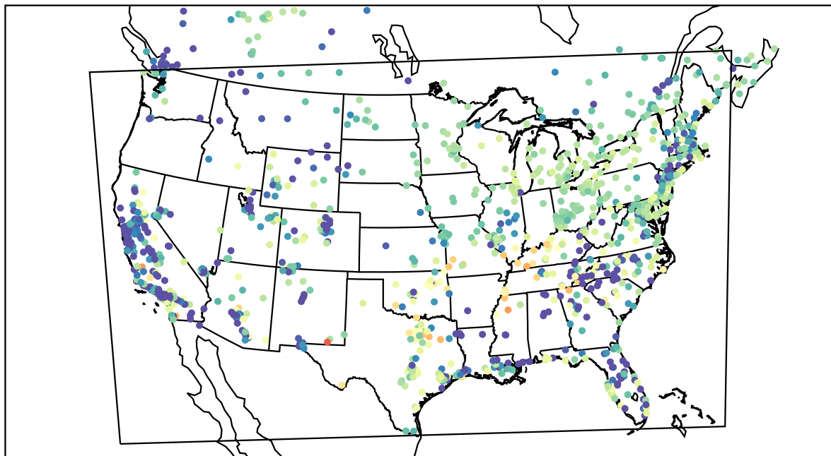
AirNOW (2022-03-03_06:00:00)
