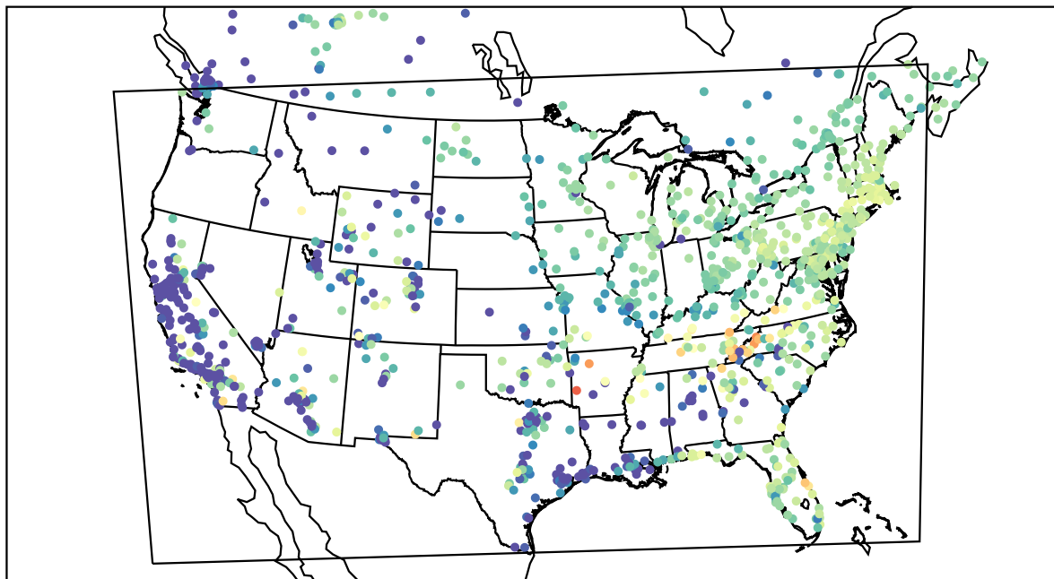
AirNOW (2022-03-03_14:00:00)
