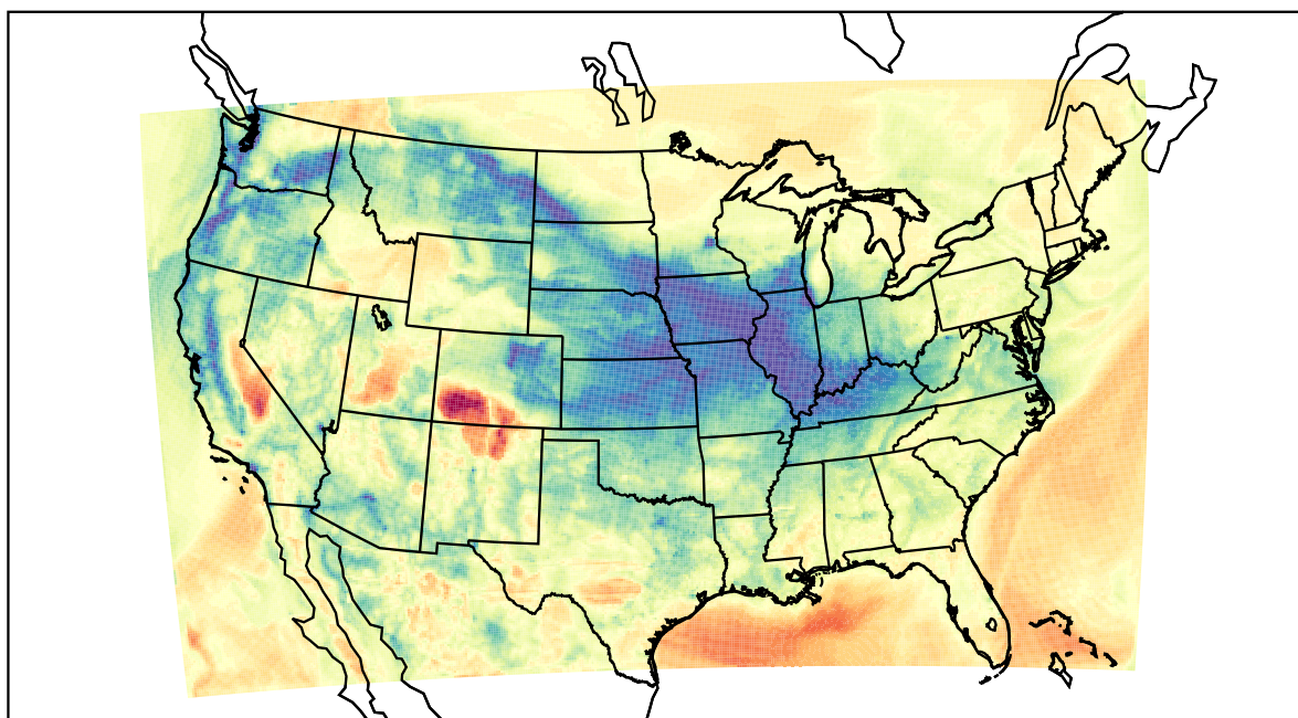
WRF (2022-03-02_16:00:00)
