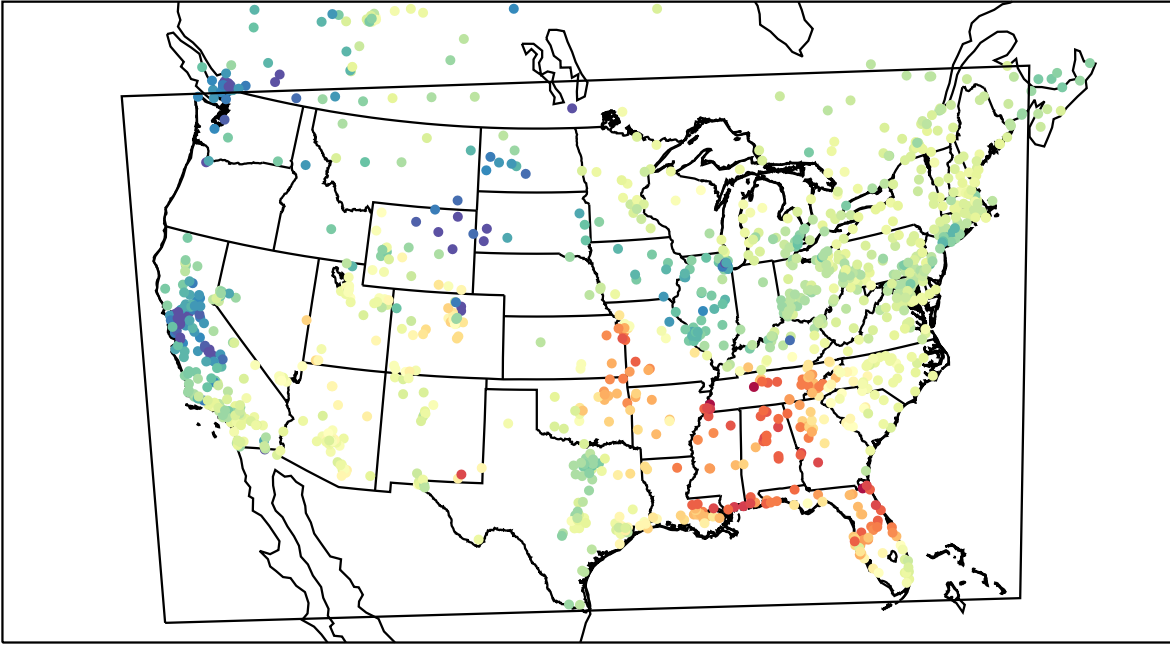
AirNOW (2022-03-04_19:00:00)
