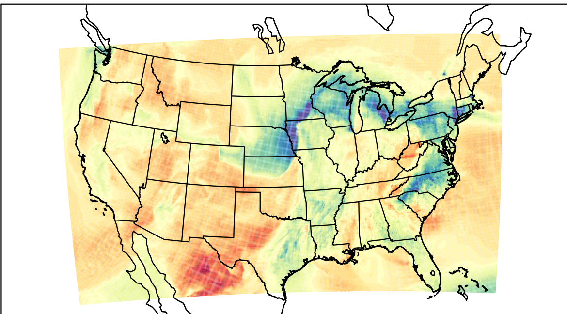
WRF (2022-03-05_23:00:00)
