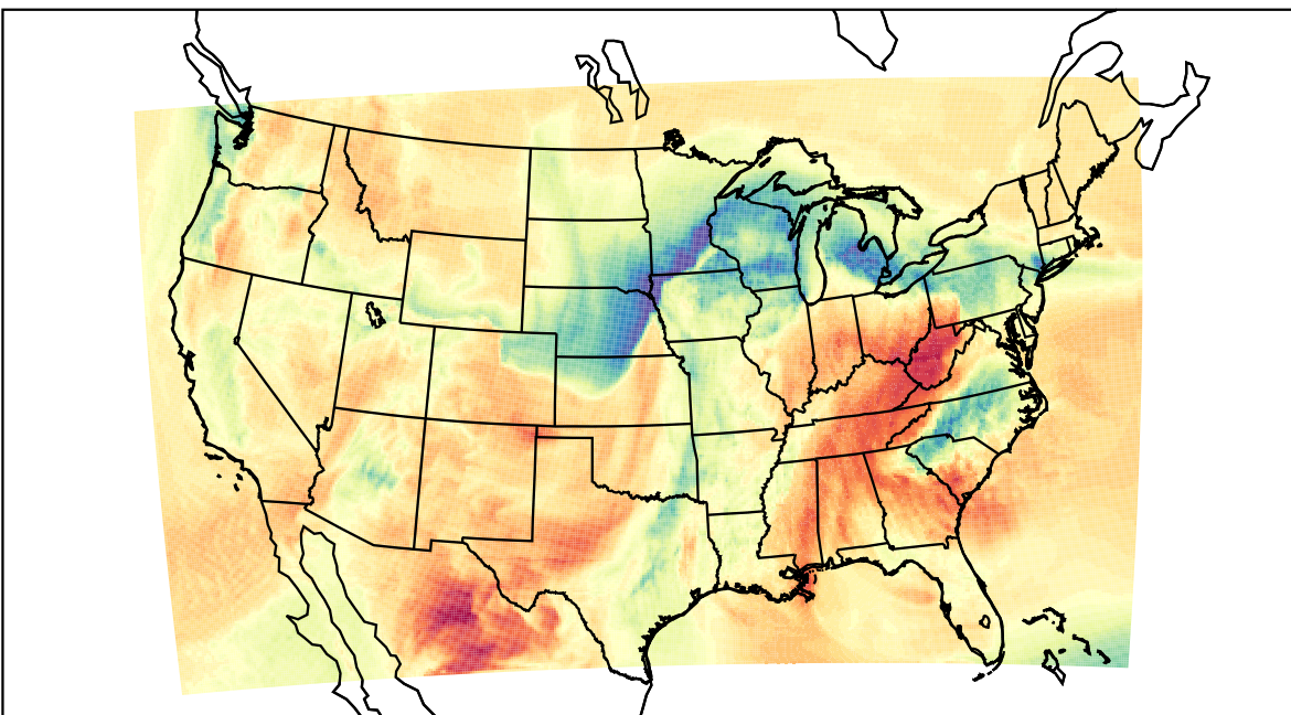
WRF (2022-03-05_20:00:00)
