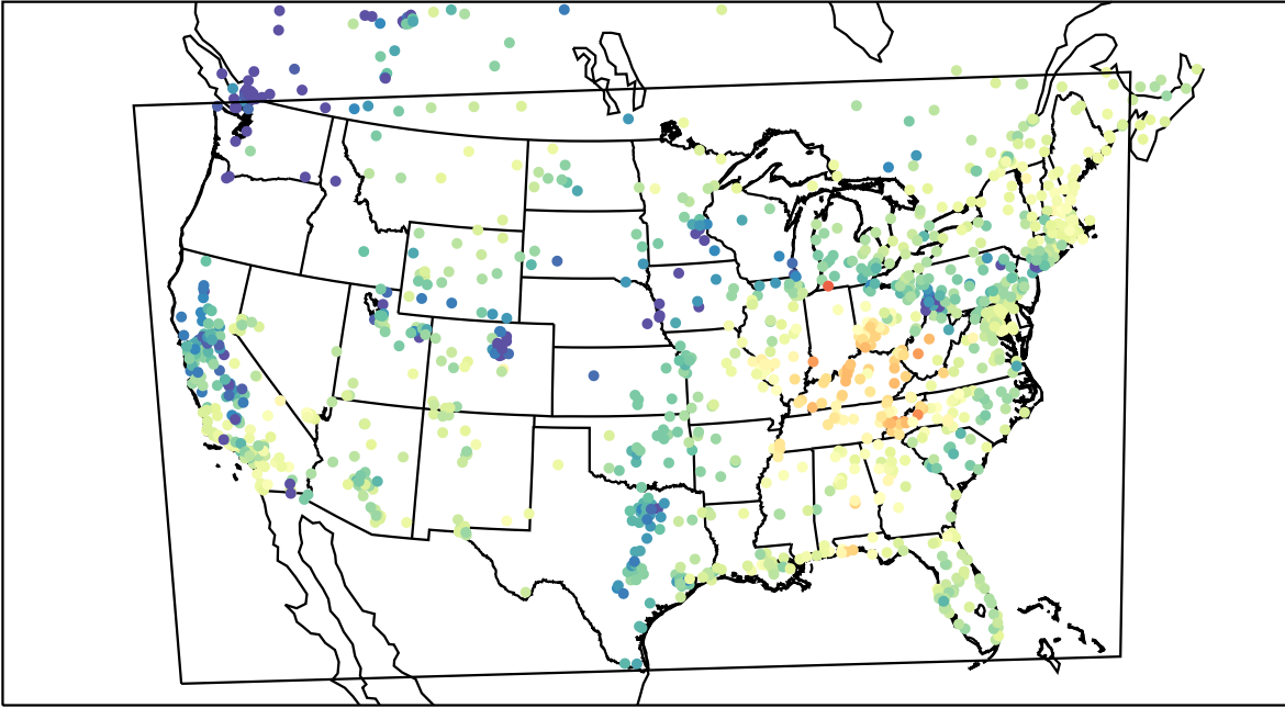
AirNOW (2022-03-05_16:00:00)
