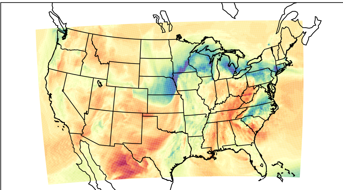
WRF (2022-03-05_22:00:00)
