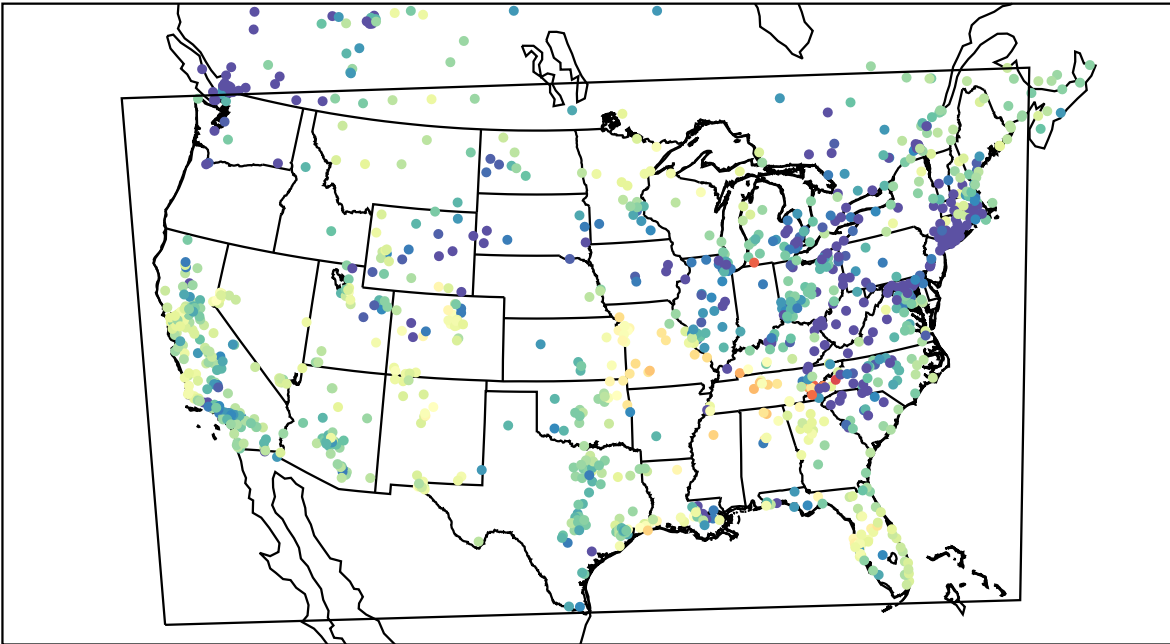
AirNOW (2022-03-05_06:00:00)
