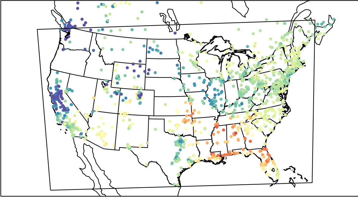
AirNOW (2022-03-04_17:00:00)
