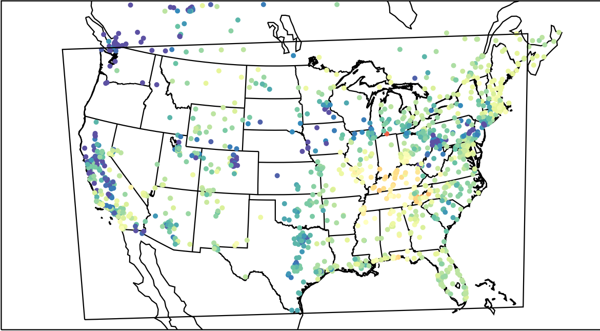
AirNOW (2022-03-05_15:00:00)
