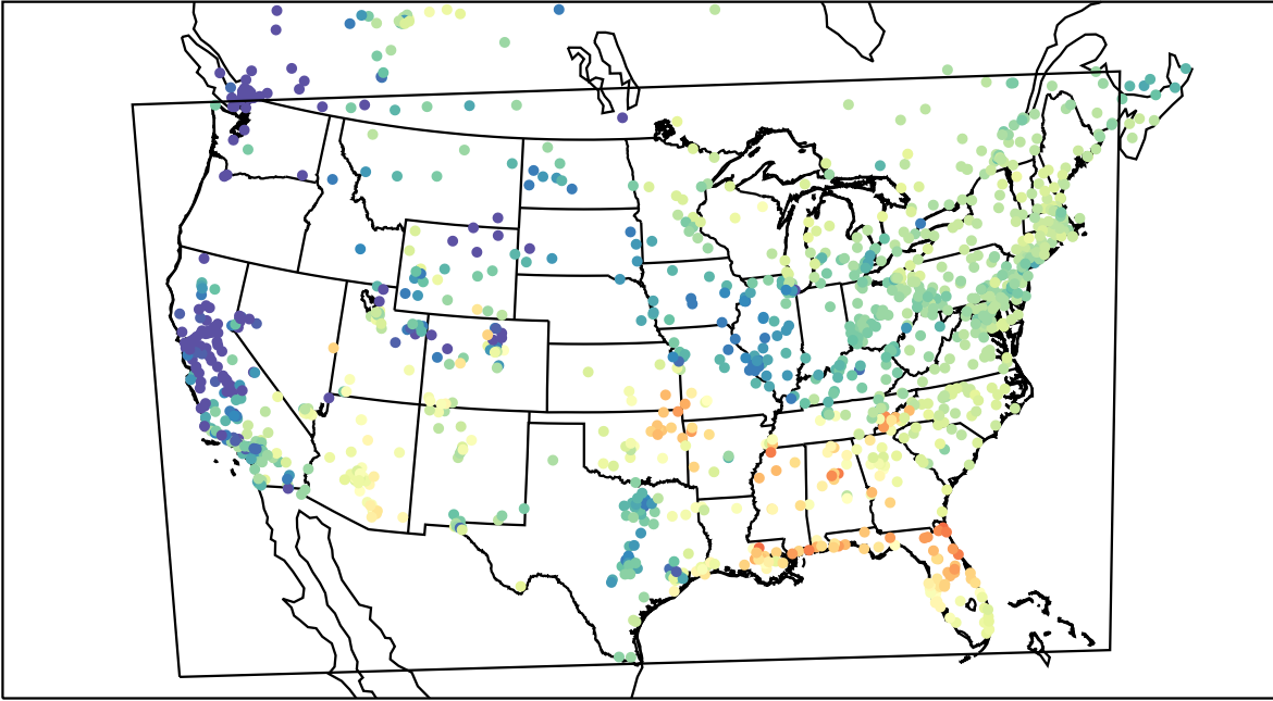
AirNOW (2022-03-04_16:00:00)
