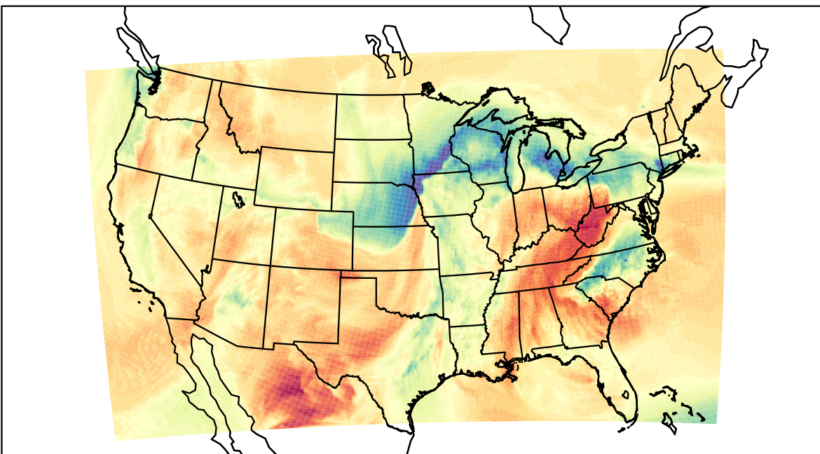
WRF (2022-03-05_21:00:00)
