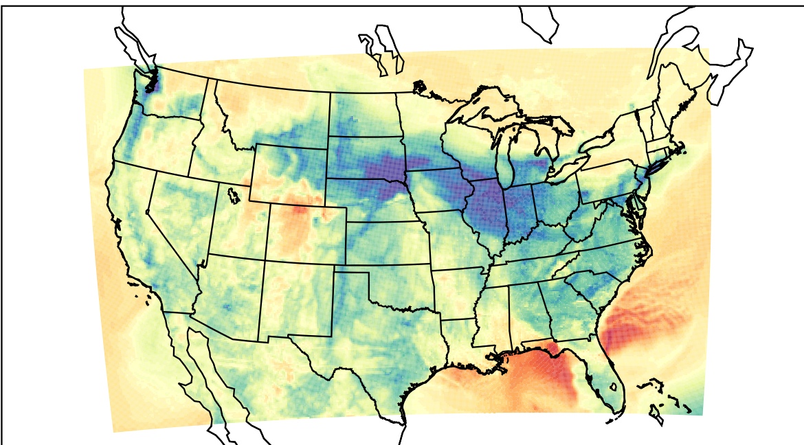
WRF (2022-03-05_05:00:00)
