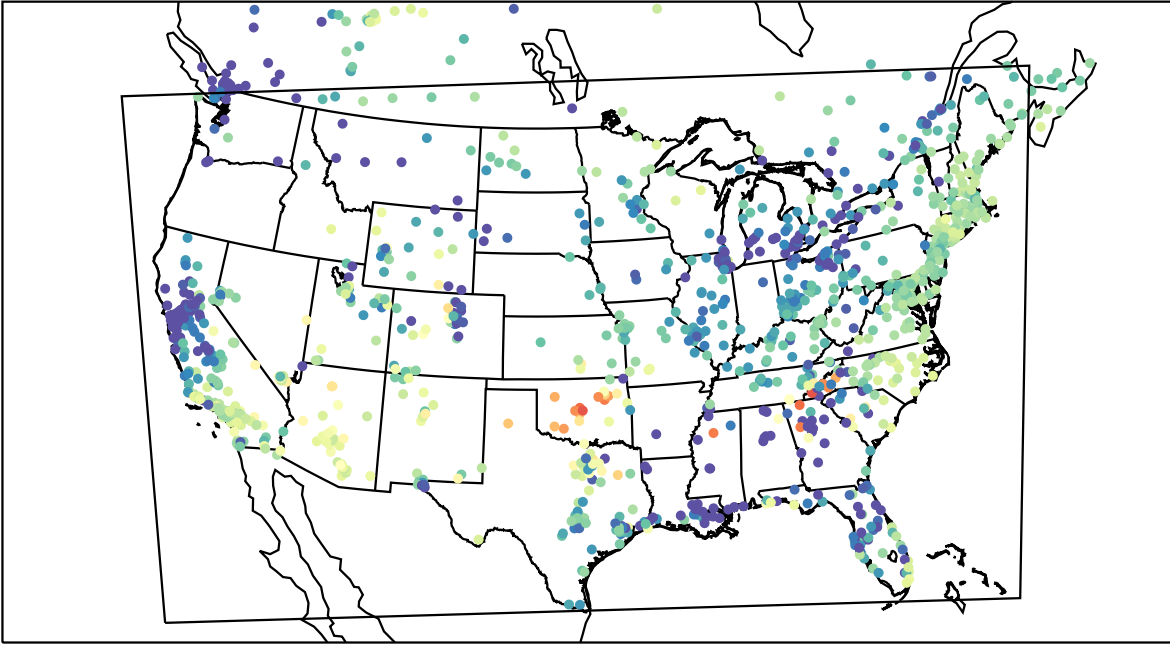
AirNOW (2022-03-04_06:00:00)
