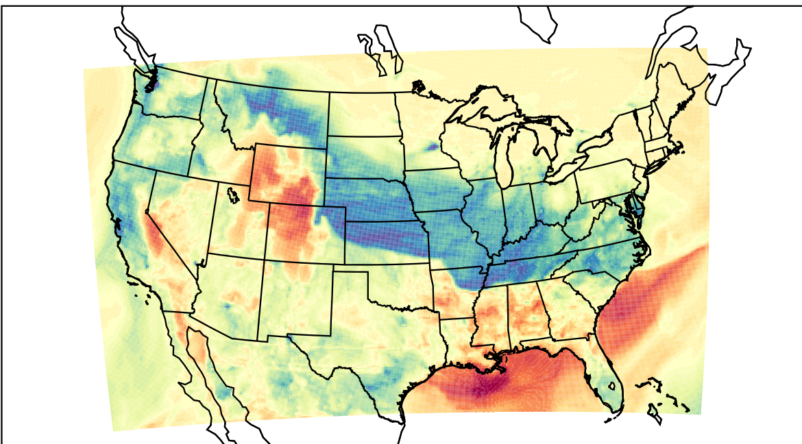
WRF (2022-03-04_03:00:00)
