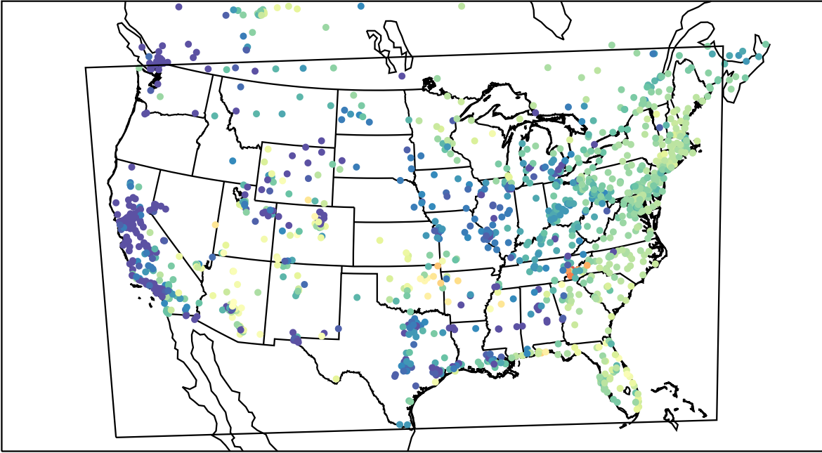
AirNOW (2022-03-04_14:00:00)
