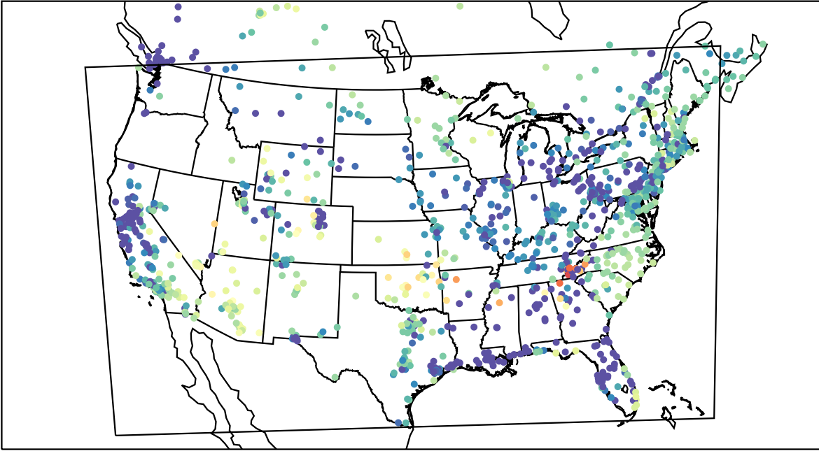
AirNOW (2022-03-04_10:00:00)
