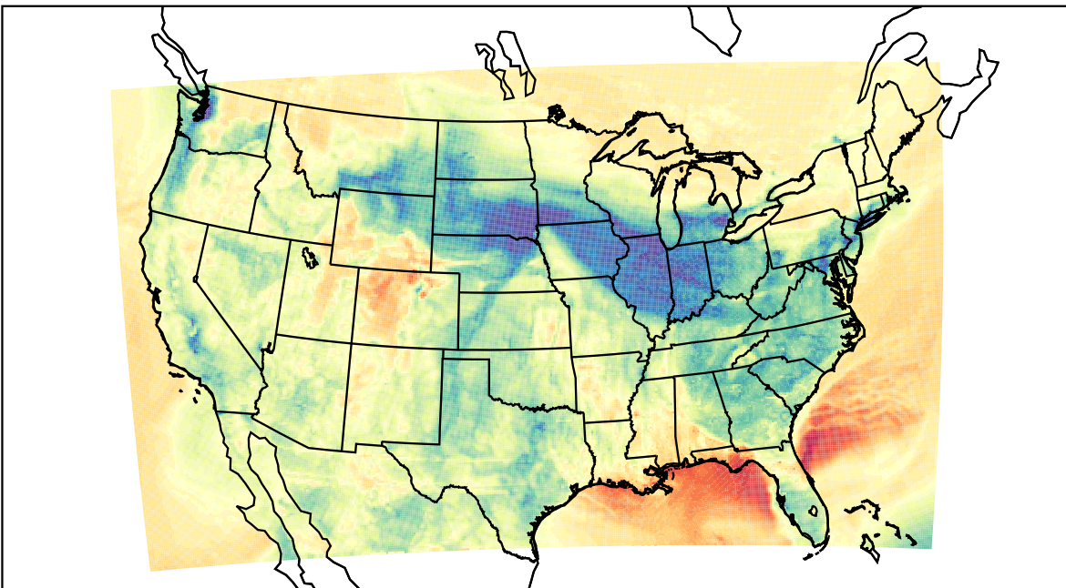
WRF (2022-03-05_03:00:00)
