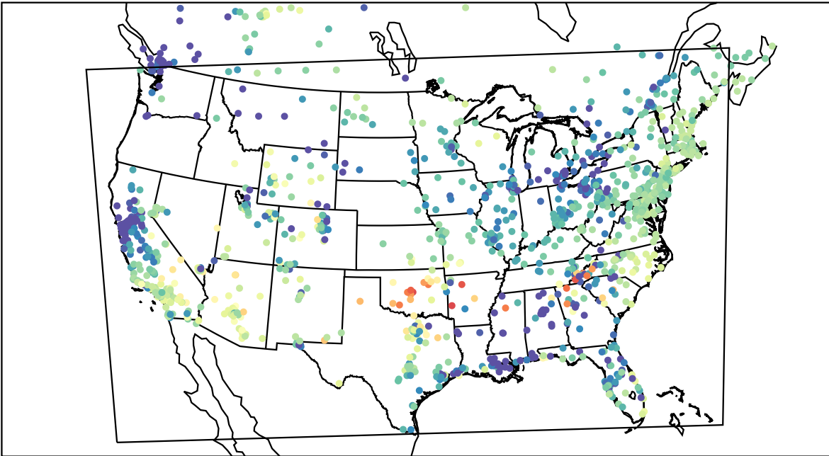
AirNOW (2022-03-04_05:00:00)
