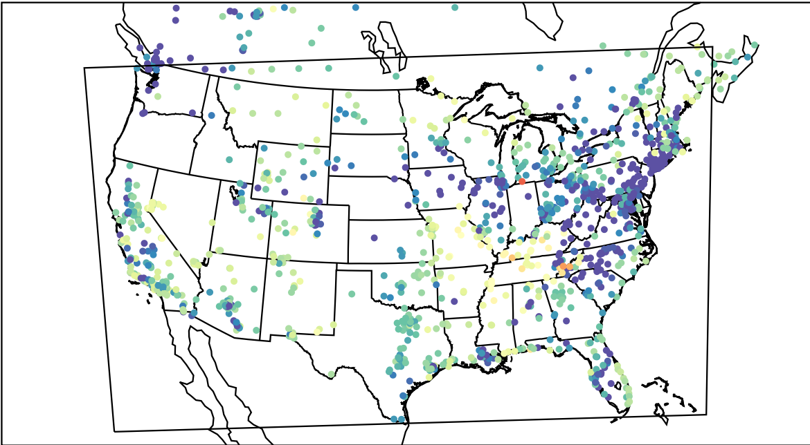
AirNOW (2022-03-05_11:00:00)
