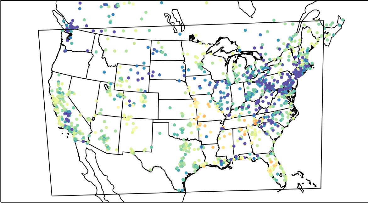
AirNOW (2022-03-05_04:00:00)
