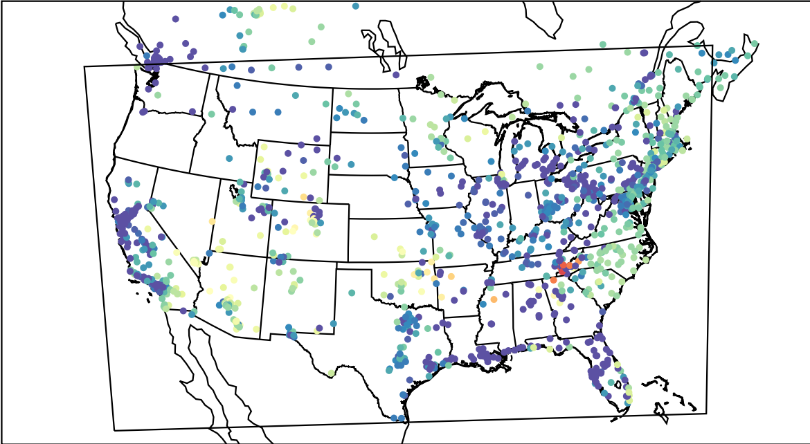
AirNOW (2022-03-04_12:00:00)
