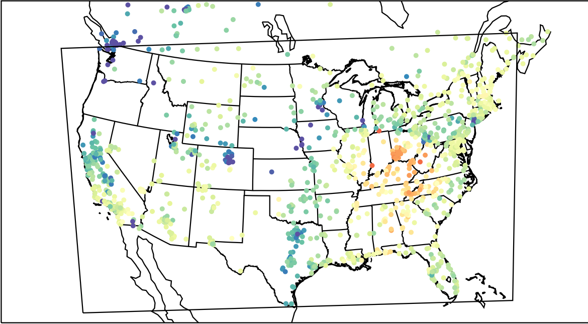
AirNOW (2022-03-05_17:00:00)
