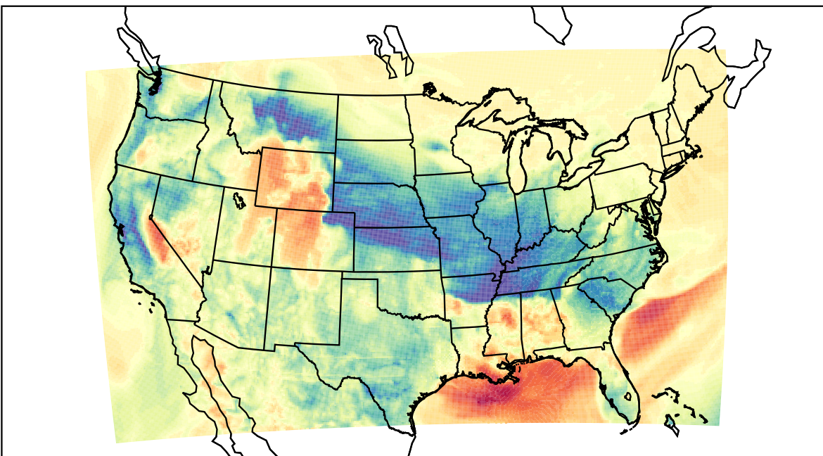
WRF (2022-03-04_08:00:00)
