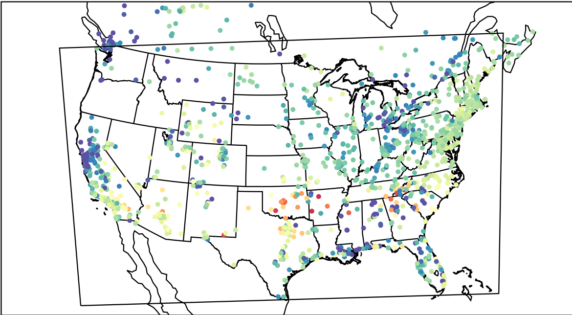
AirNOW (2022-03-04_03:00:00)
