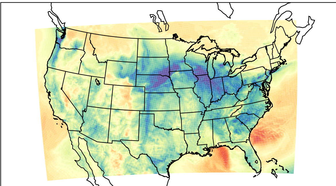
WRF (2022-03-05_10:00:00)
