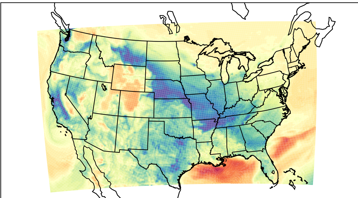
WRF (2022-03-04_14:00:00)
