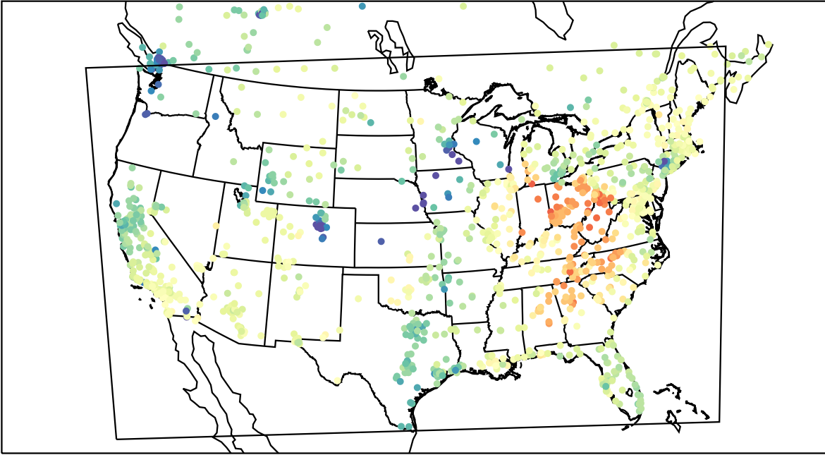
AirNOW (2022-03-05_20:00:00)
