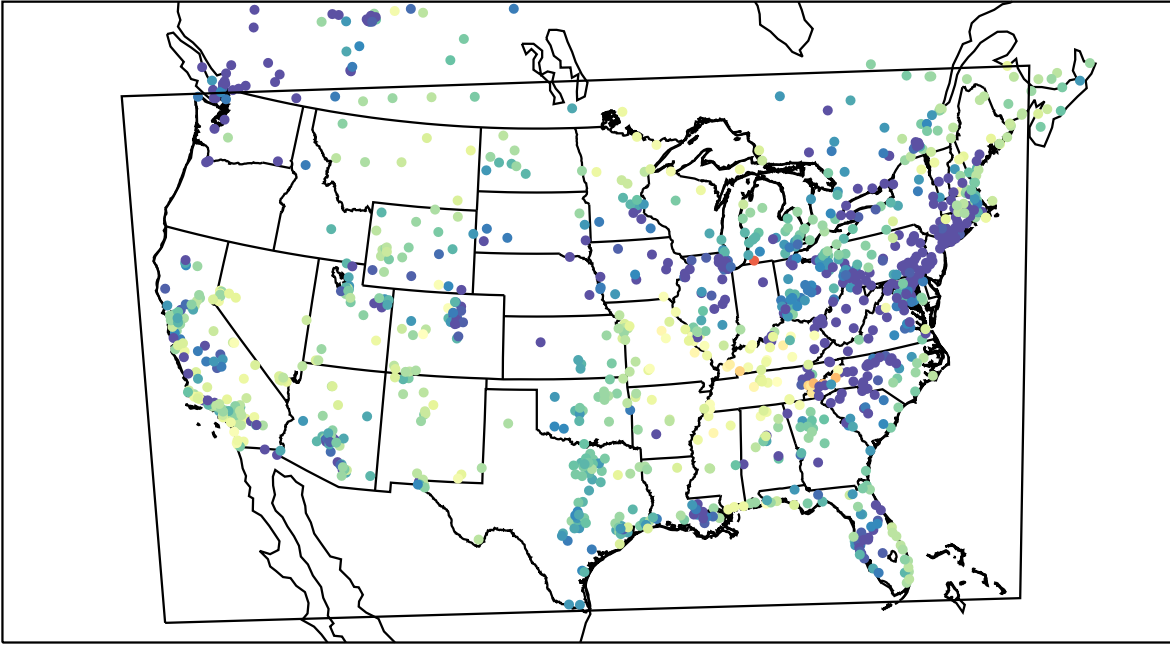
AirNOW (2022-03-05_12:00:00)
