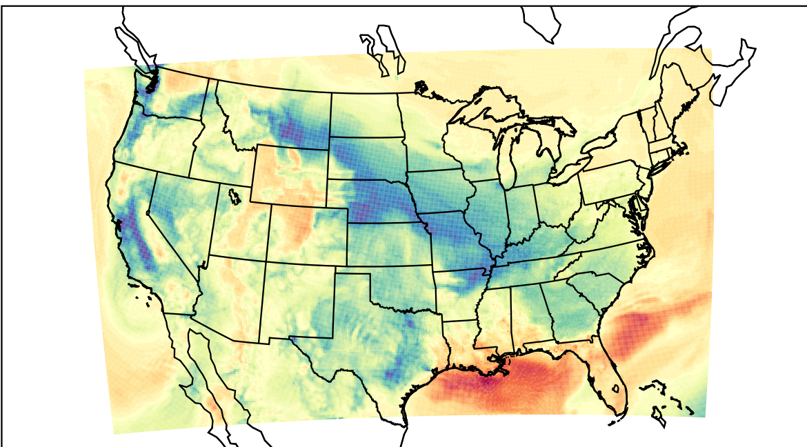
WRF (2022-03-04_16:00:00)
