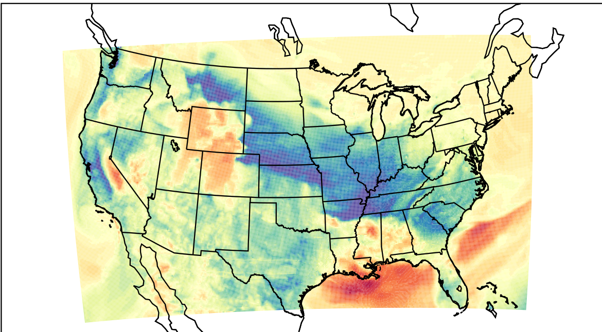
WRF (2022-03-04_10:00:00)
