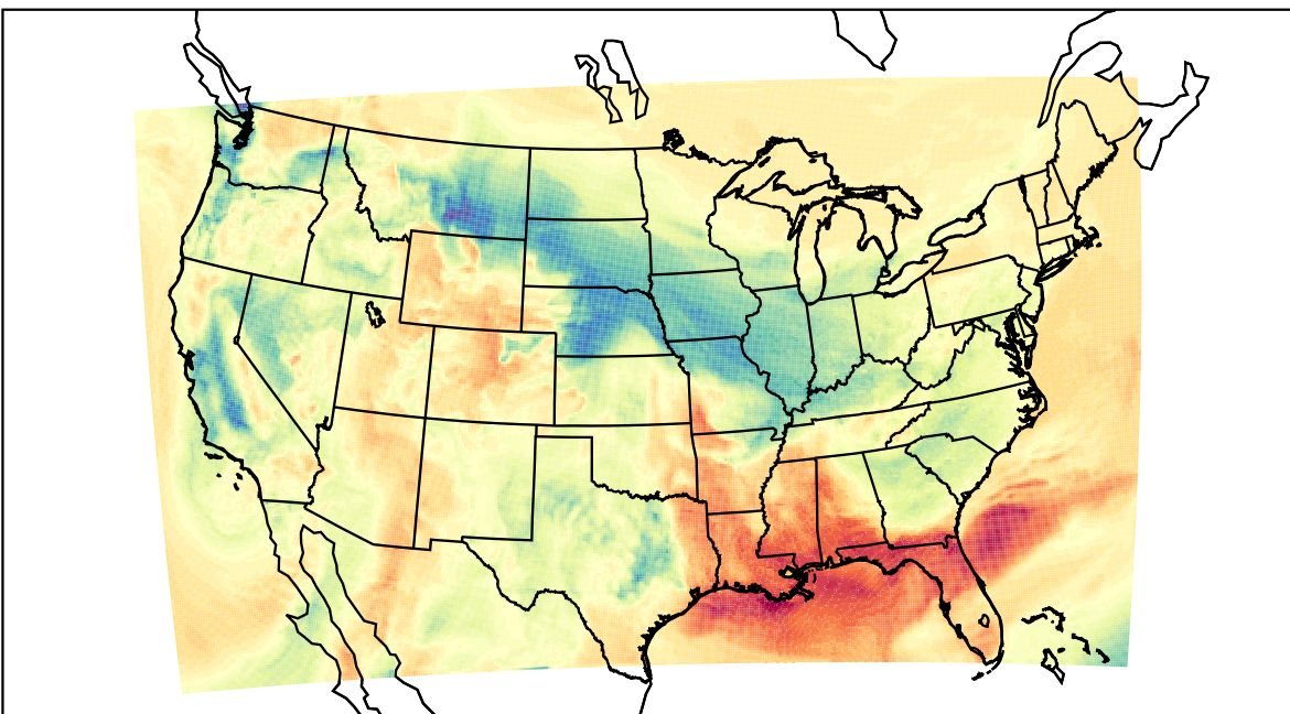
WRF (2022-03-04_18:00:00)
