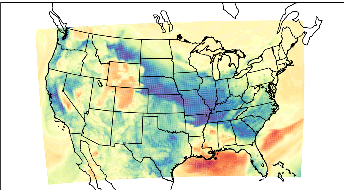
WRF (2022-03-04_12:00:00)
