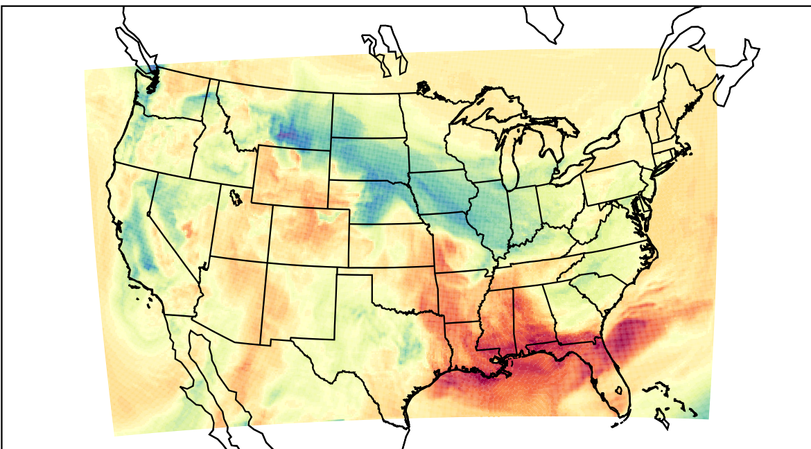
WRF (2022-03-04_19:00:00)
