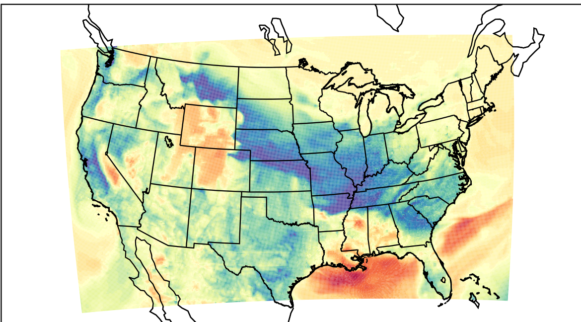
WRF (2022-03-04_11:00:00)
