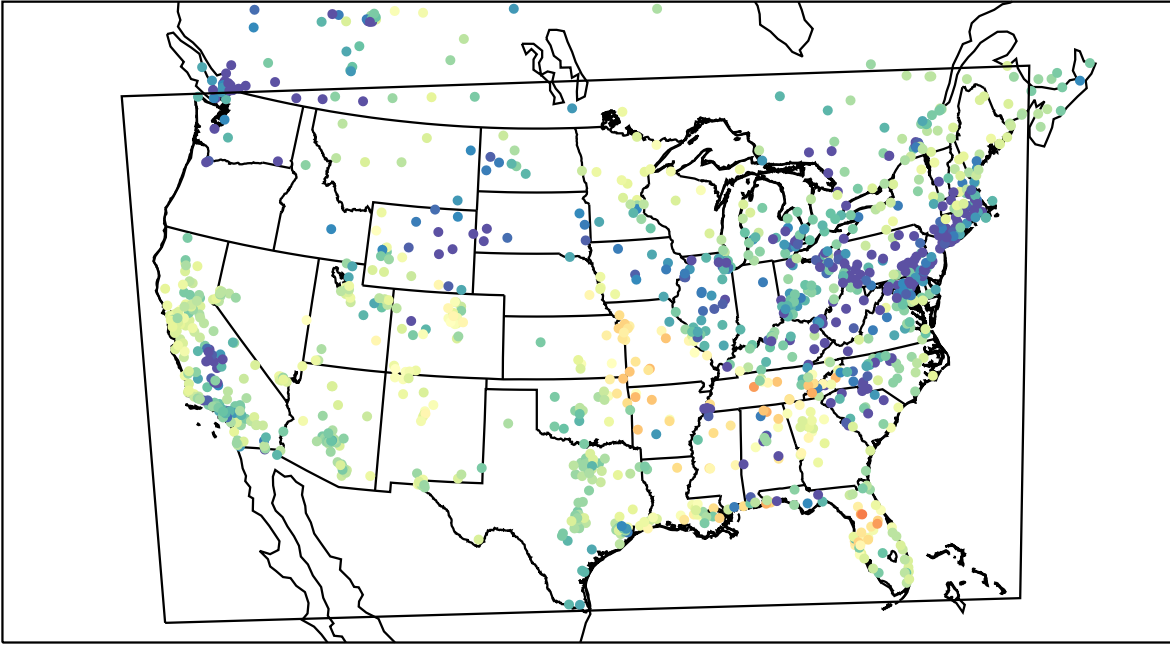
AirNOW (2022-03-05_03:00:00)
