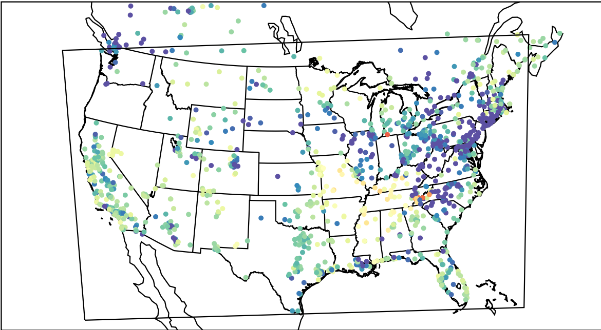
AirNOW (2022-03-05_09:00:00)
