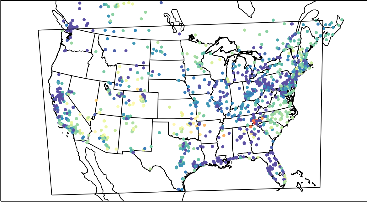
AirNOW (2022-03-04_11:00:00)
