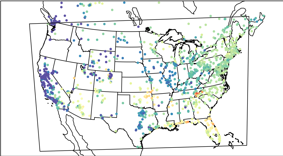
AirNOW (2022-03-04_15:00:00)
