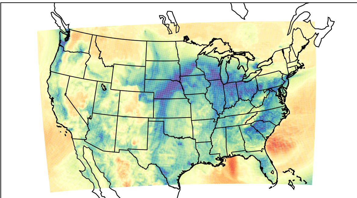
WRF (2022-03-05_13:00:00)
