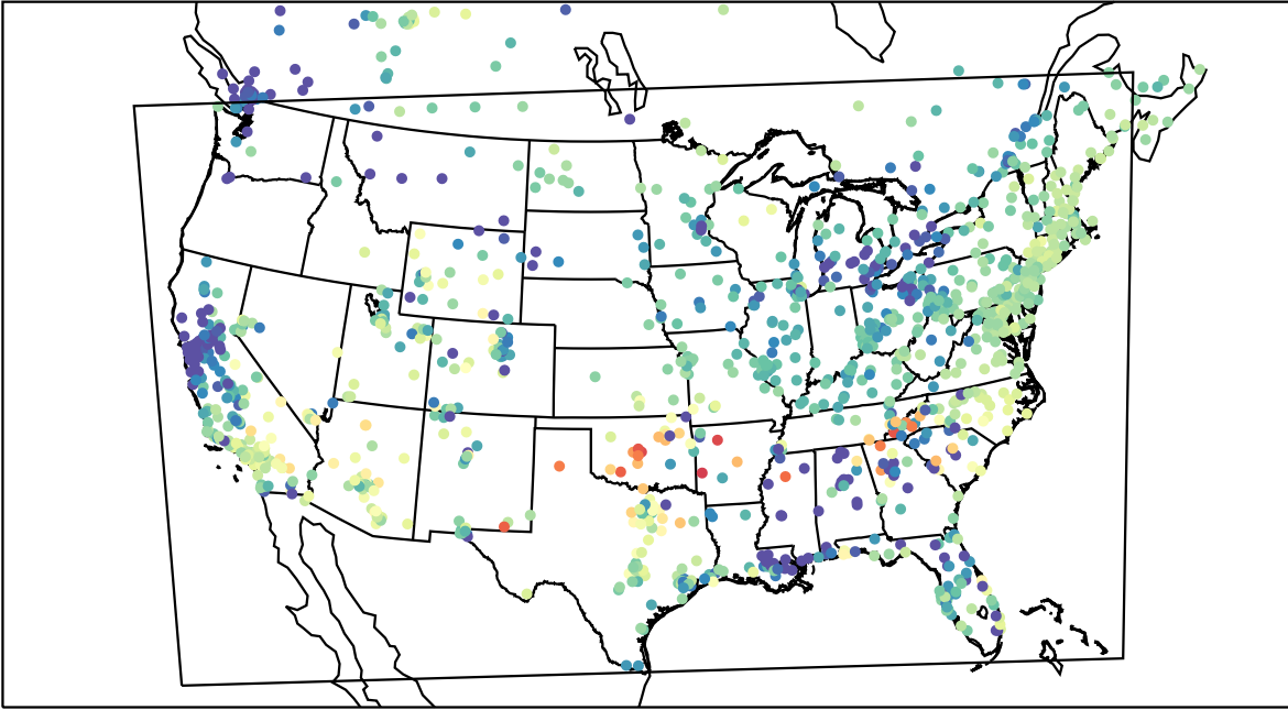
AirNOW (2022-03-04_04:00:00)
