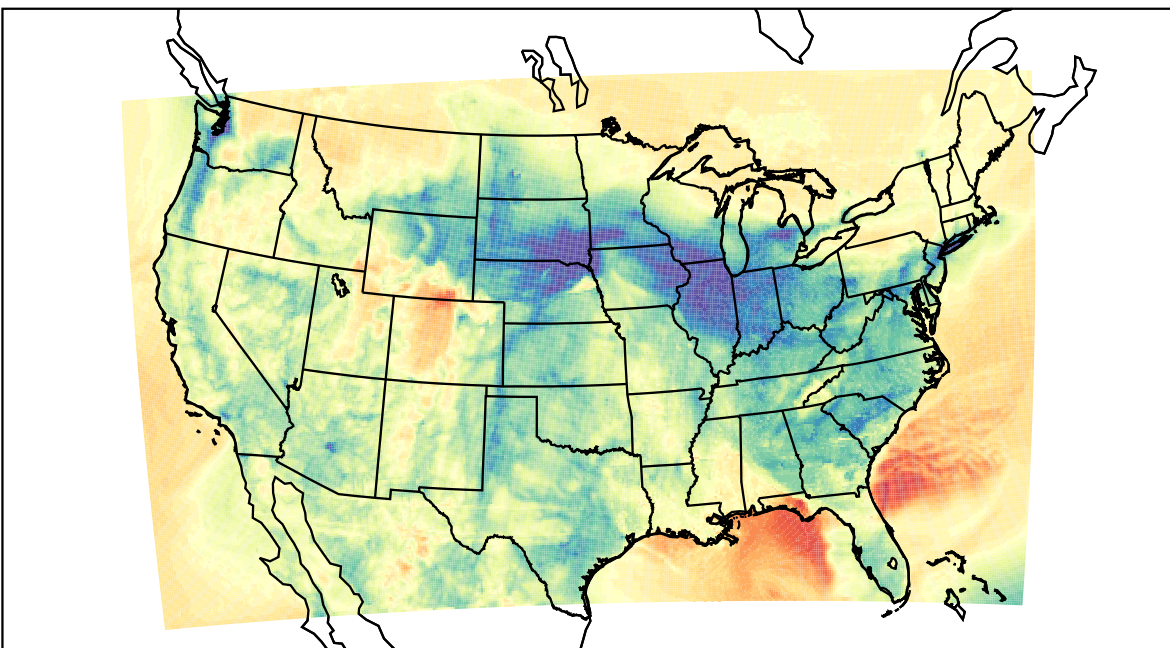
WRF (2022-03-05_06:00:00)
