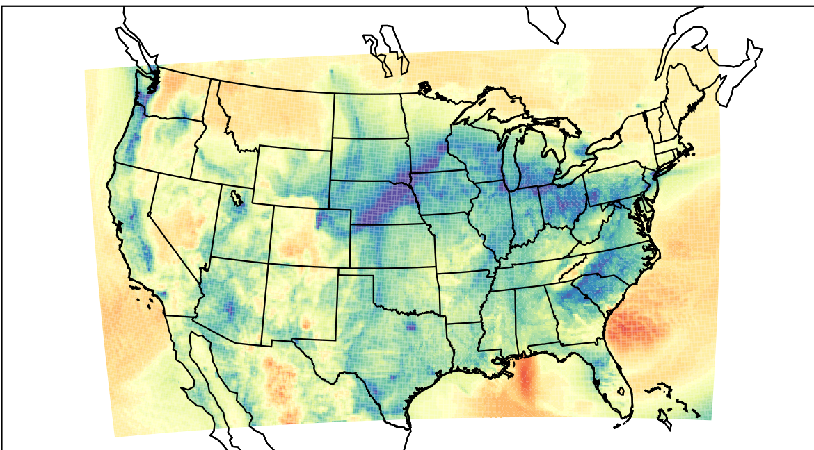
WRF (2022-03-05_14:00:00)
