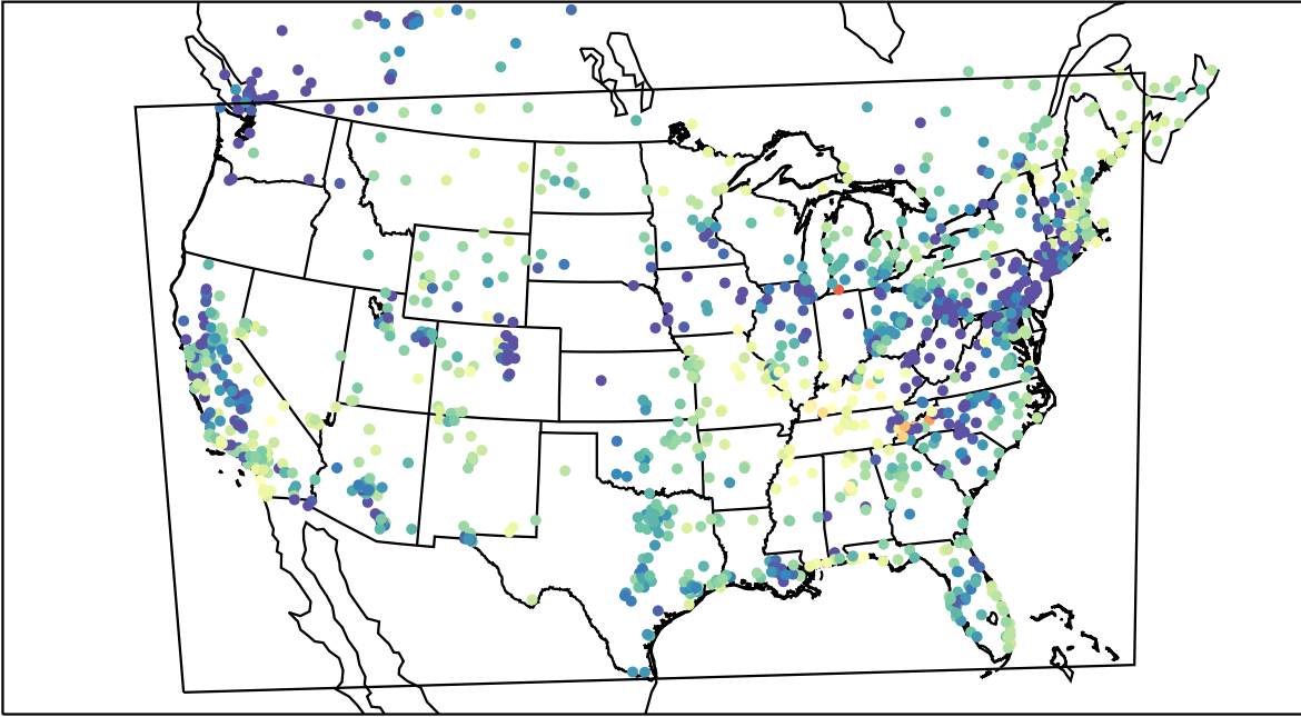
AirNOW (2022-03-05_13:00:00)
