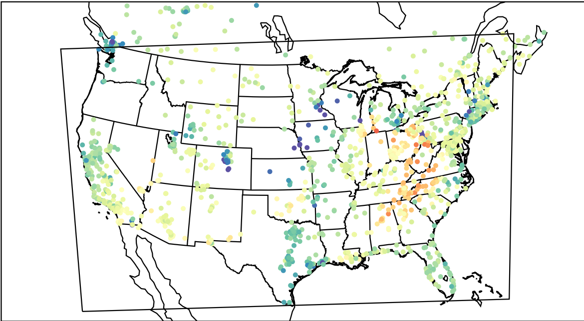
AirNOW (2022-03-05_23:00:00)
