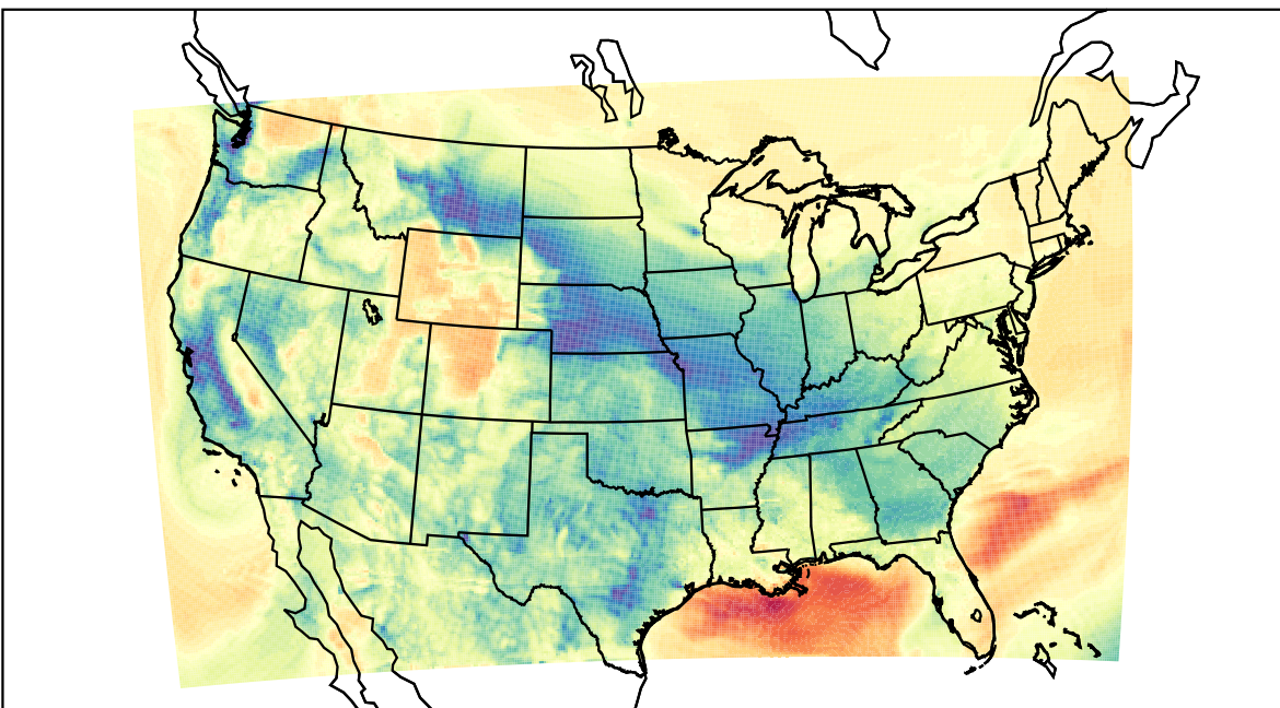
WRF (2022-03-04_15:00:00)
