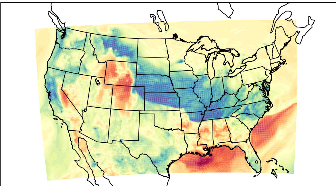
WRF (2022-03-04_04:00:00)
