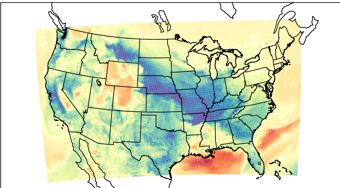
WRF (2022-03-04_13:00:00)
