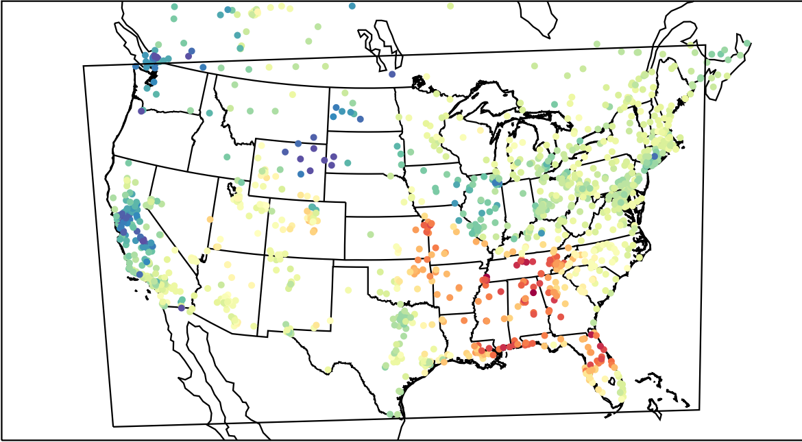
AirNOW (2022-03-04_20:00:00)
