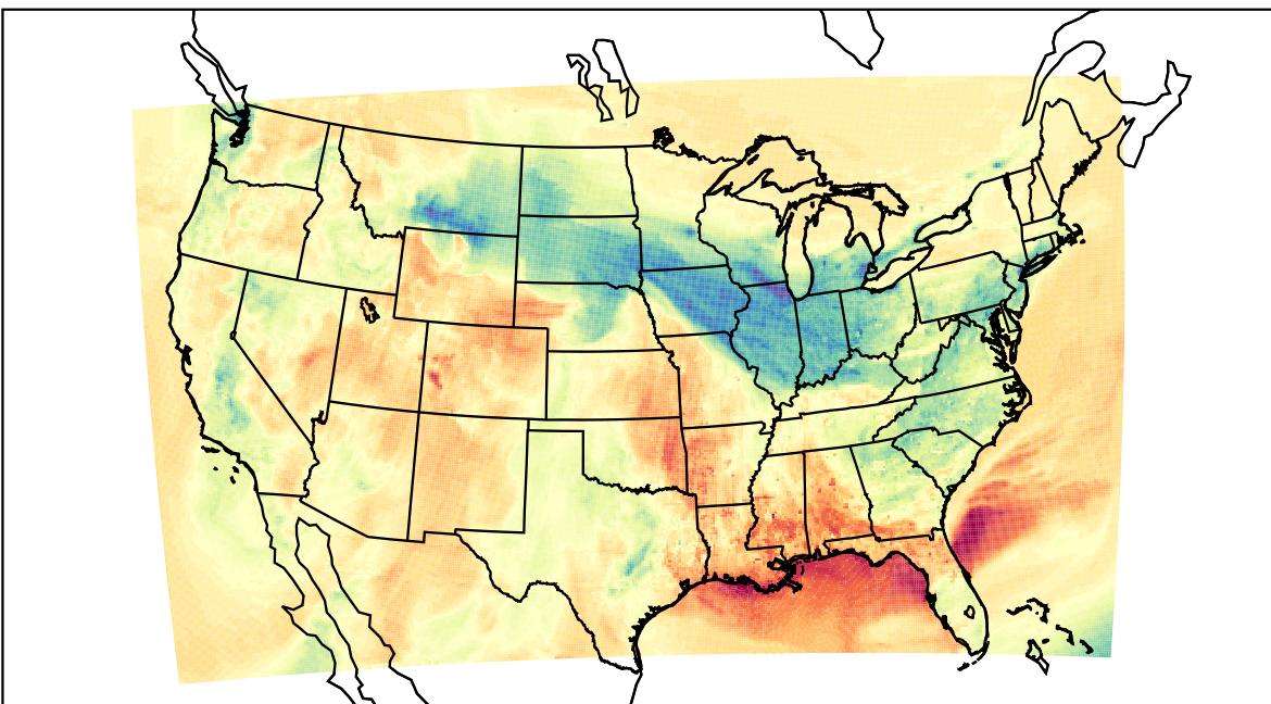
WRF (2022-03-04_23:00:00)
