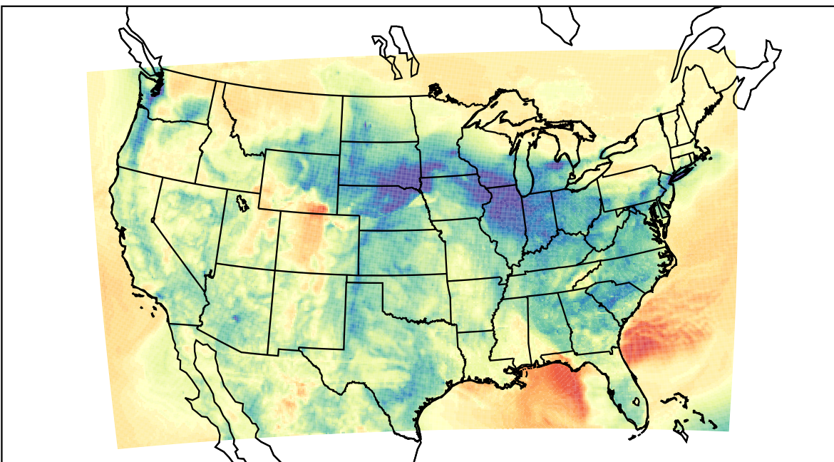
WRF (2022-03-05_07:00:00)
