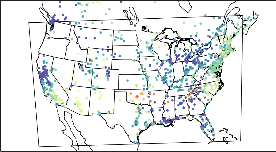
AirNOW (2022-03-04_07:00:00)
