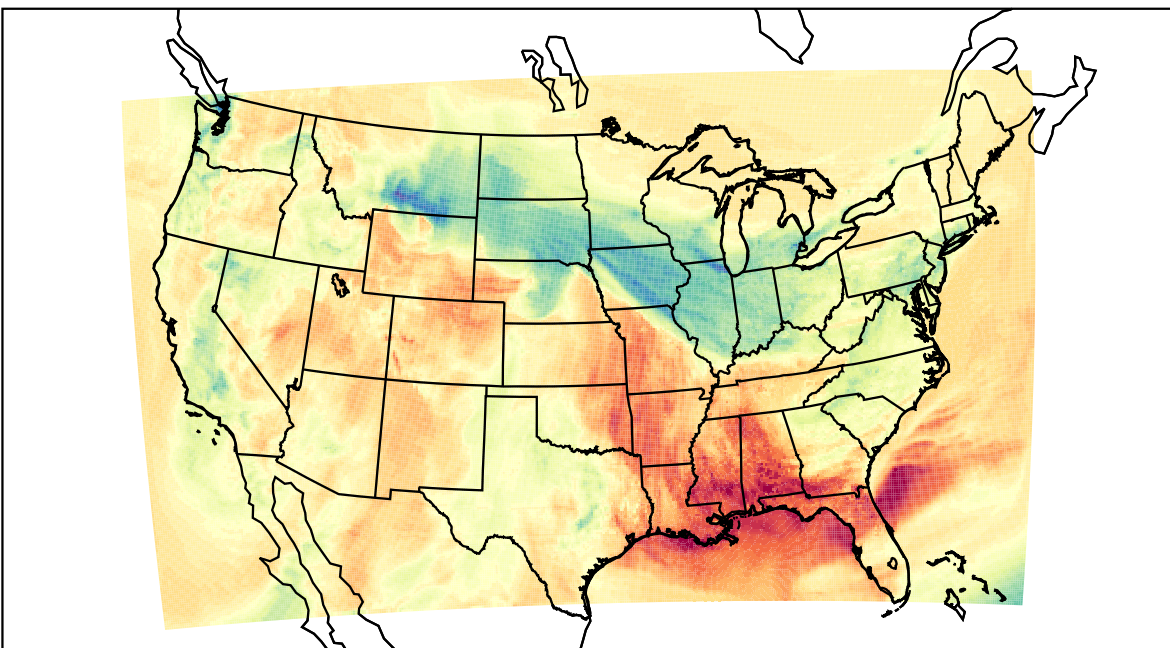
WRF (2022-03-04_22:00:00)
