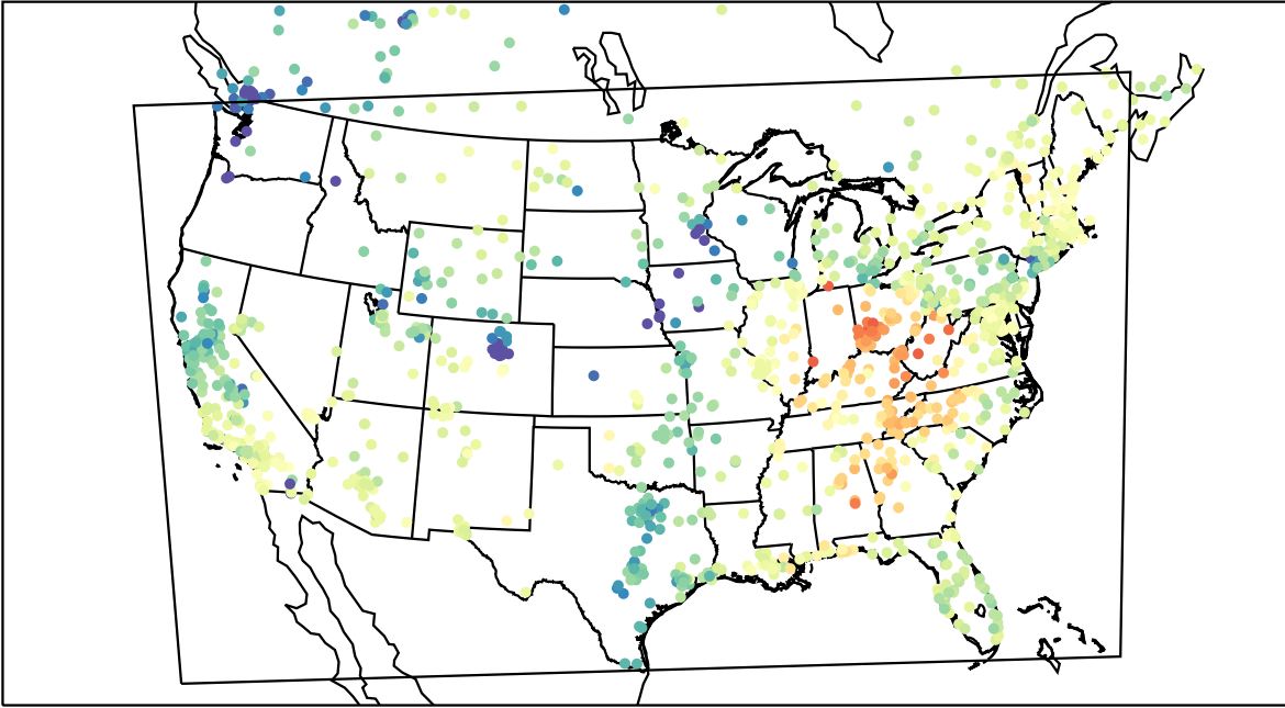
AirNOW (2022-03-05_18:00:00)
