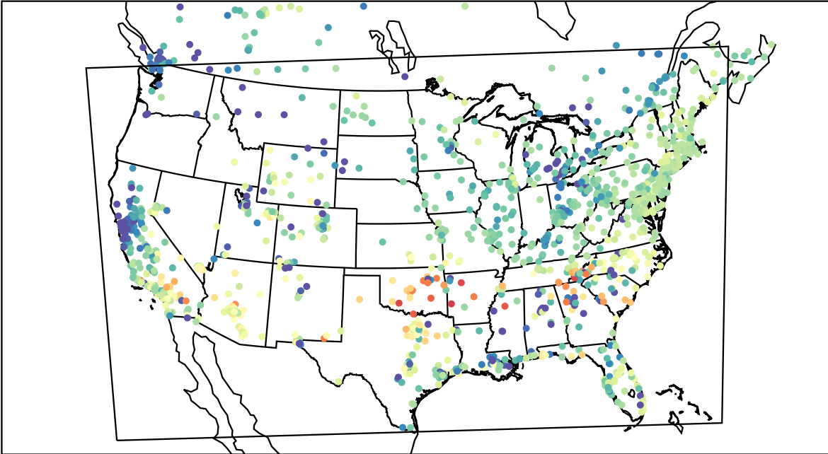
AirNOW (2022-03-04_02:00:00)
