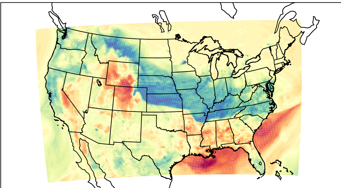
WRF (2022-03-04_02:00:00)
