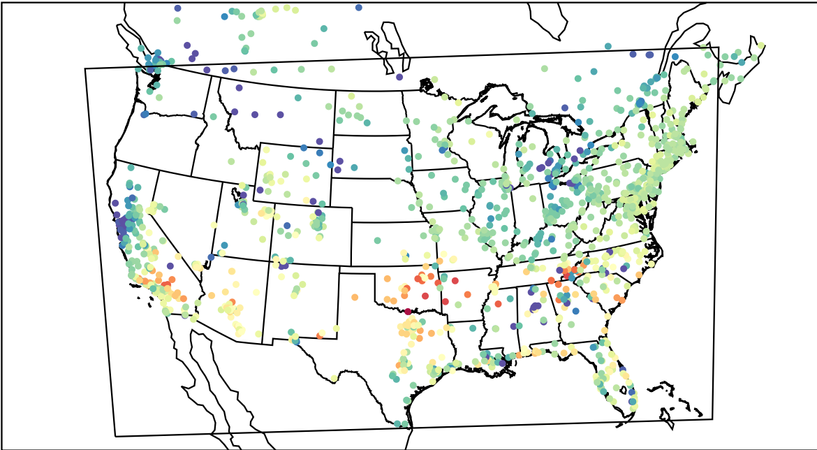
AirNOW (2022-03-04_01:00:00)
