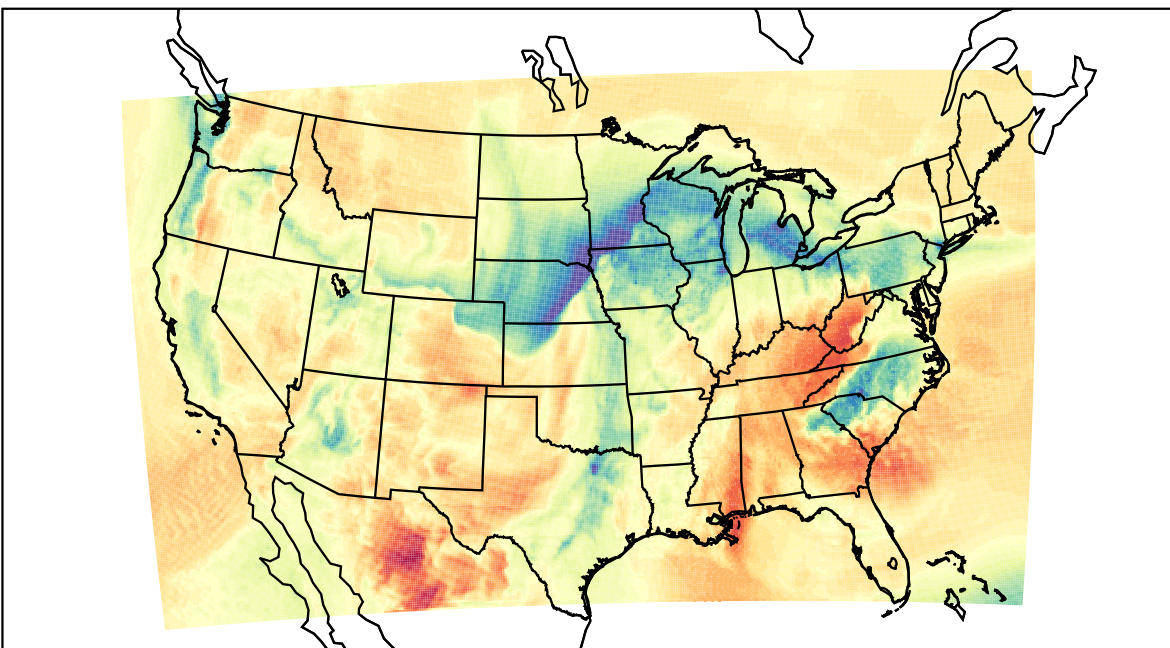
WRF (2022-03-05_18:00:00)
