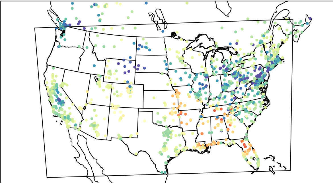
AirNOW (2022-03-05_00:00:00)
