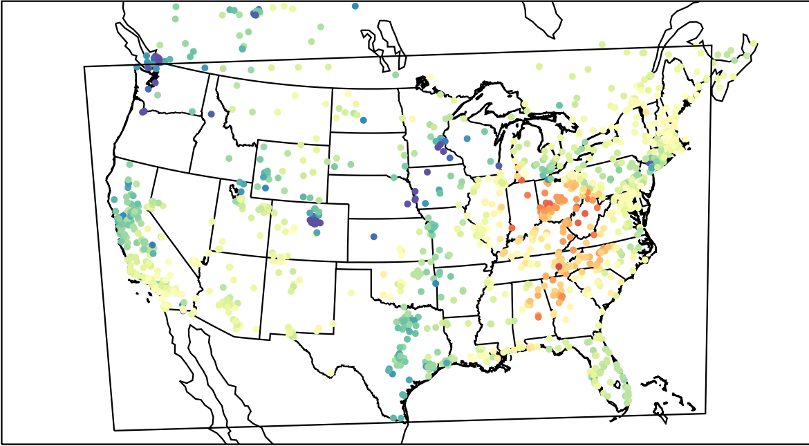
AirNOW (2022-03-05_19:00:00)
