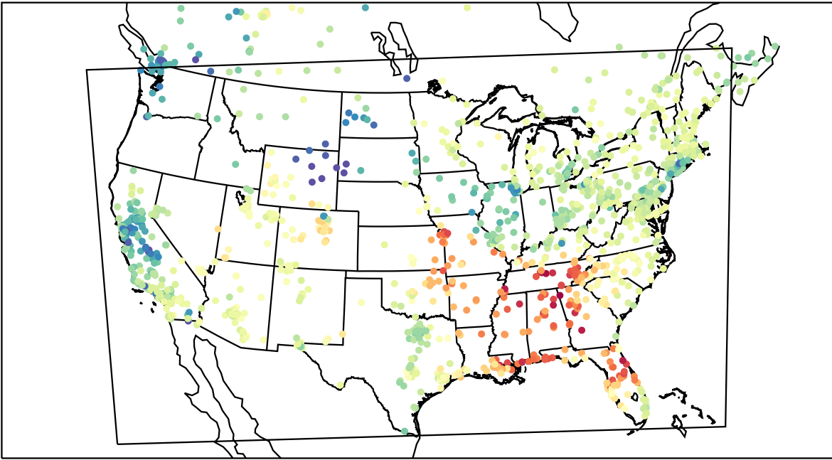
AirNOW (2022-03-04_21:00:00)
