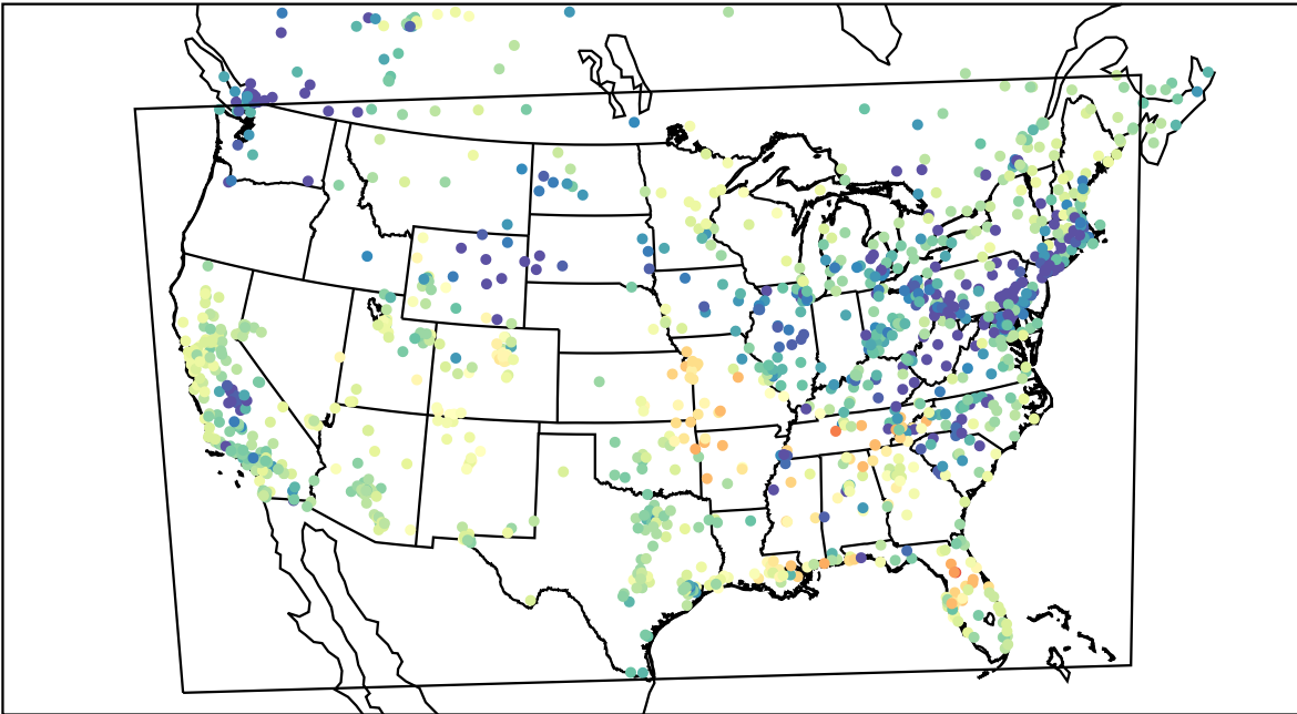
AirNOW (2022-03-05_02:00:00)
