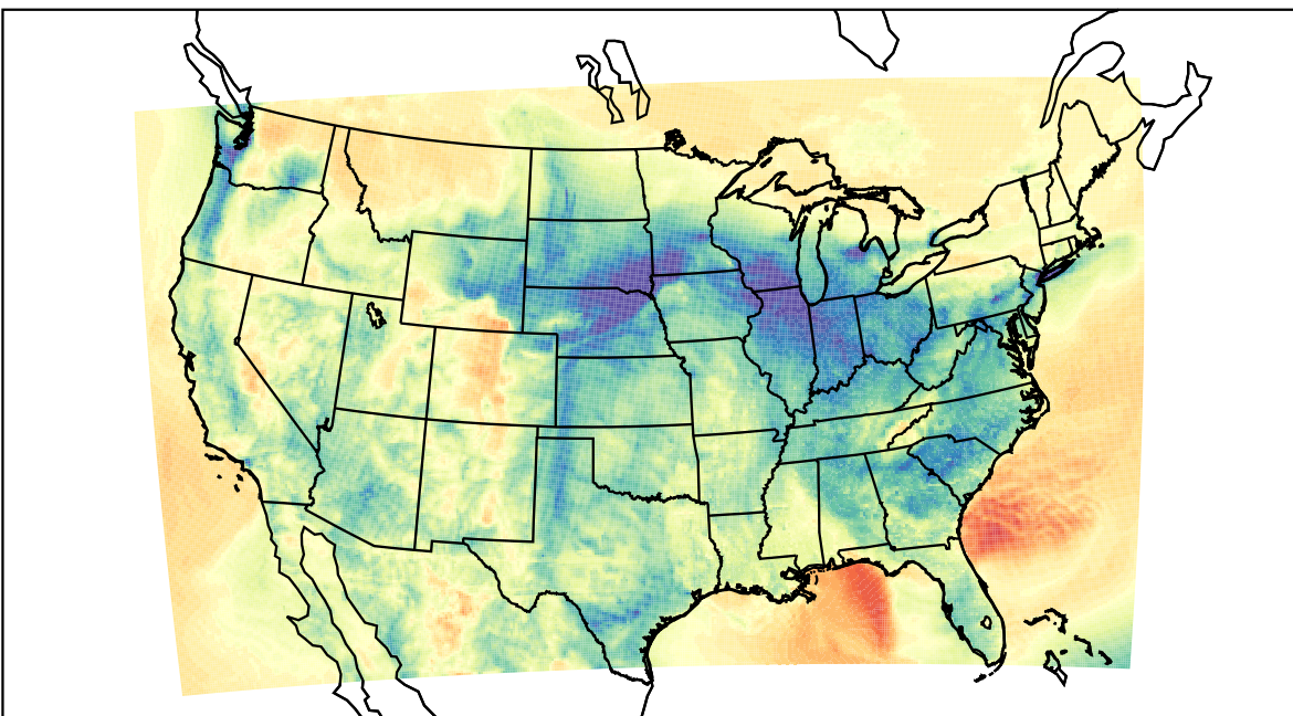
WRF (2022-03-05_09:00:00)
