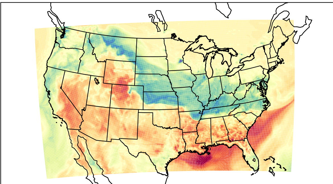
WRF (2022-03-04_00:00:00)
