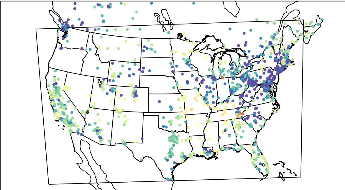
AirNOW (2022-03-05_08:00:00)
