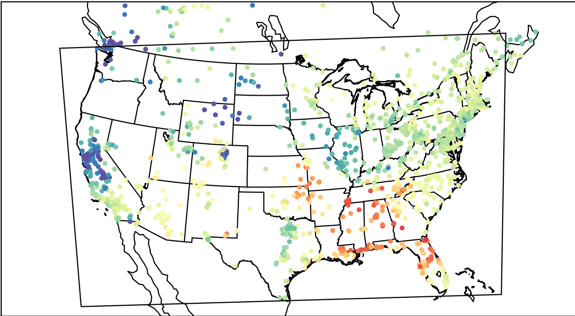
AirNOW (2022-03-04_18:00:00)
