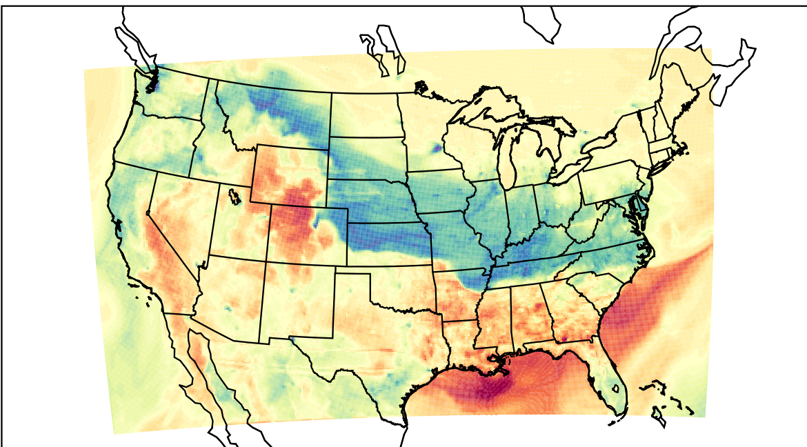
WRF (2022-03-04_01:00:00)
