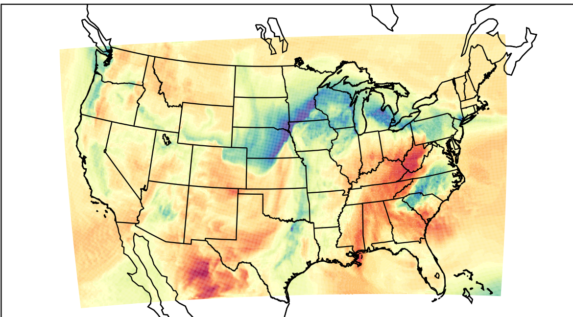
WRF (2022-03-05_19:00:00)
