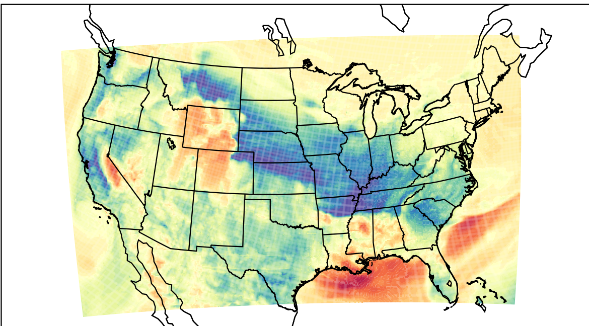
WRF (2022-03-04_09:00:00)
