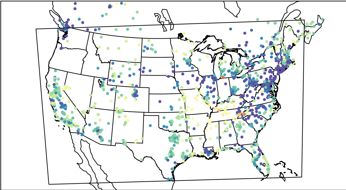
AirNOW (2022-03-05_10:00:00)
