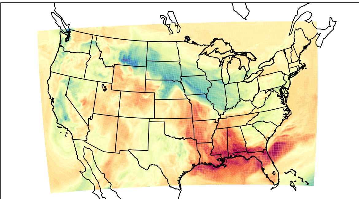
WRF (2022-03-04_20:00:00)
