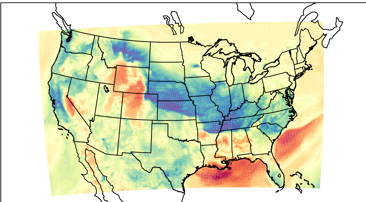
WRF (2022-03-04_06:00:00)
