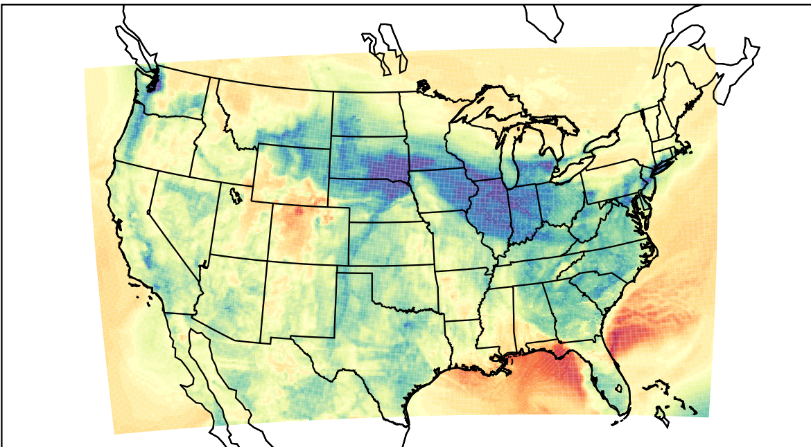
WRF (2022-03-05_04:00:00)
