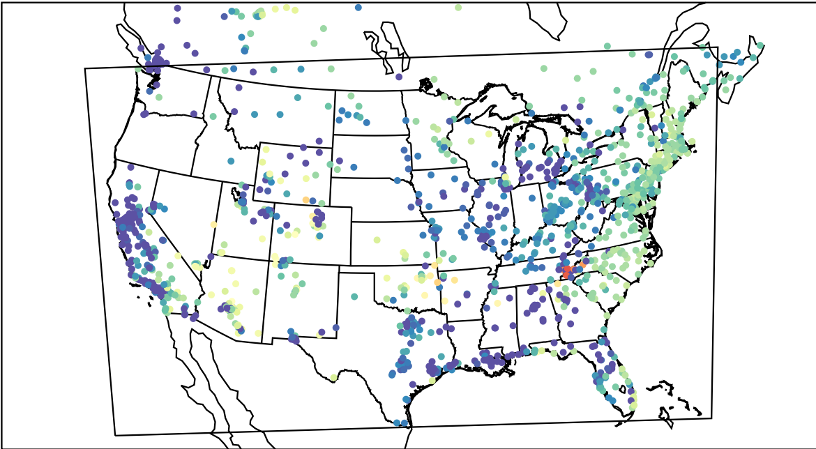
AirNOW (2022-03-04_13:00:00)
