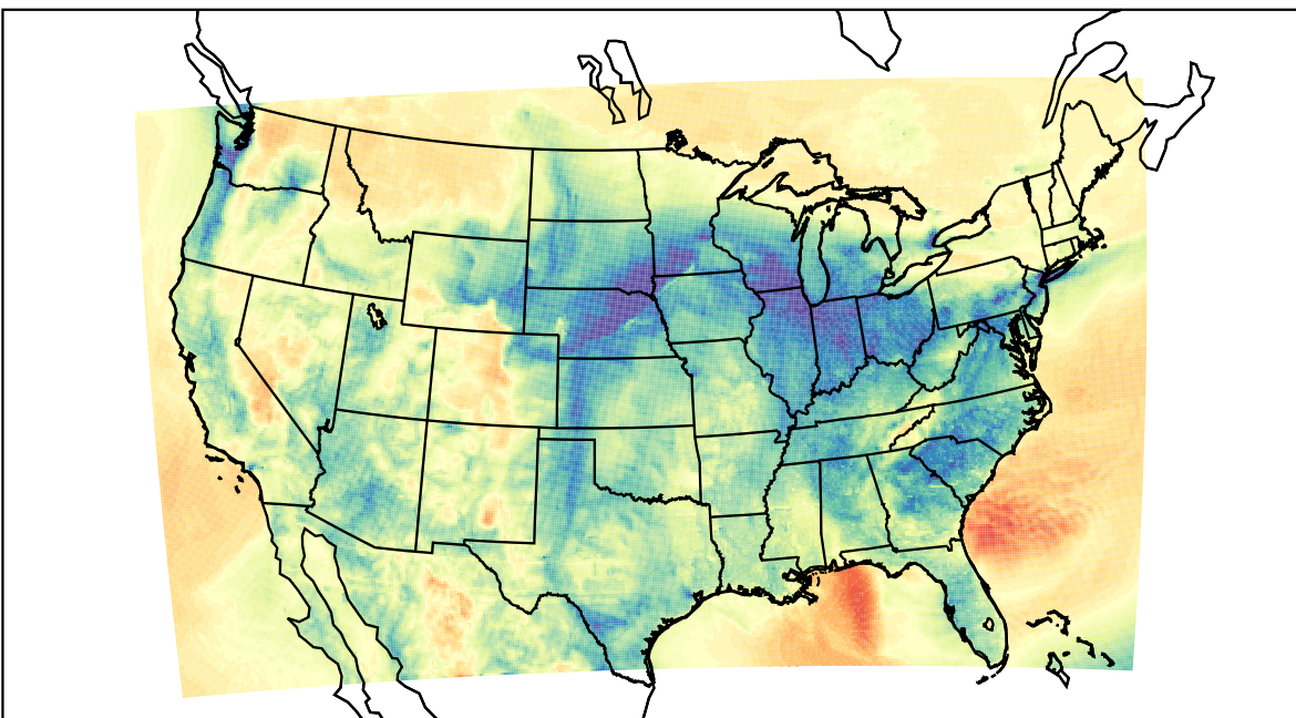
WRF (2022-03-05_11:00:00)
