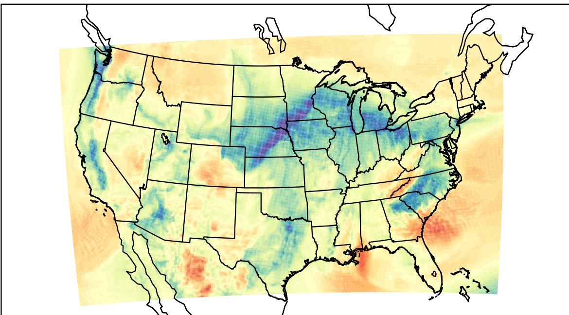
WRF (2022-03-05_16:00:00)
