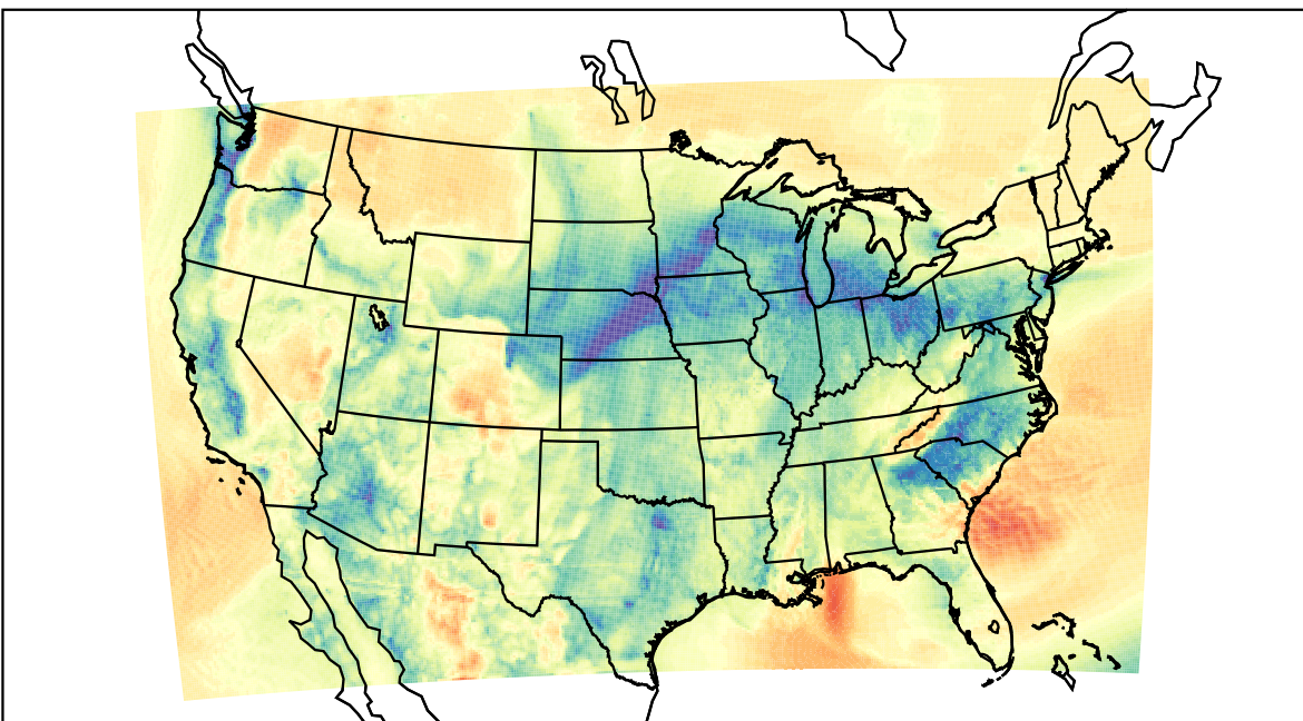
WRF (2022-03-05_15:00:00)
