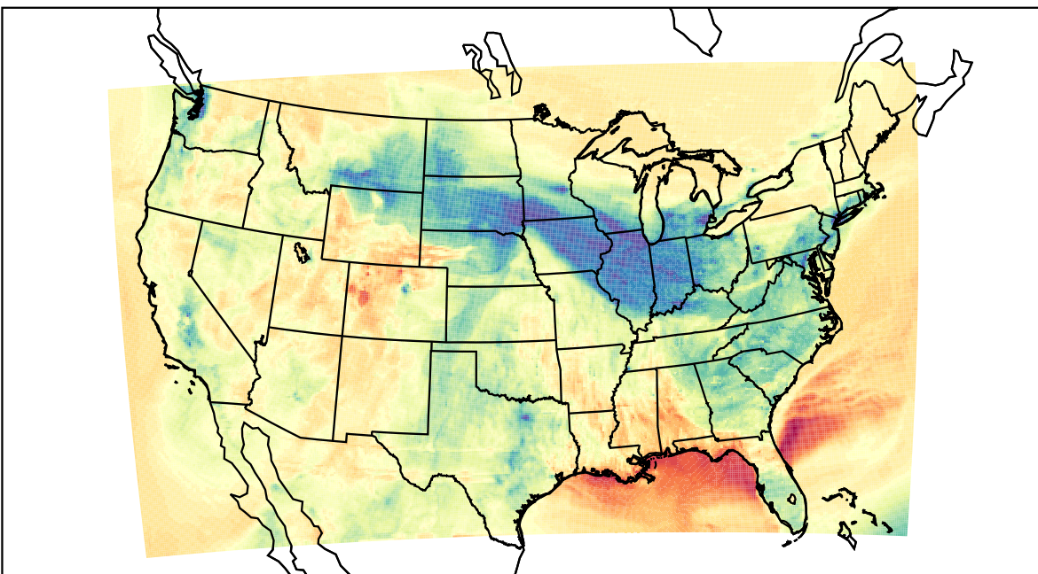
WRF (2022-03-05_01:00:00)
