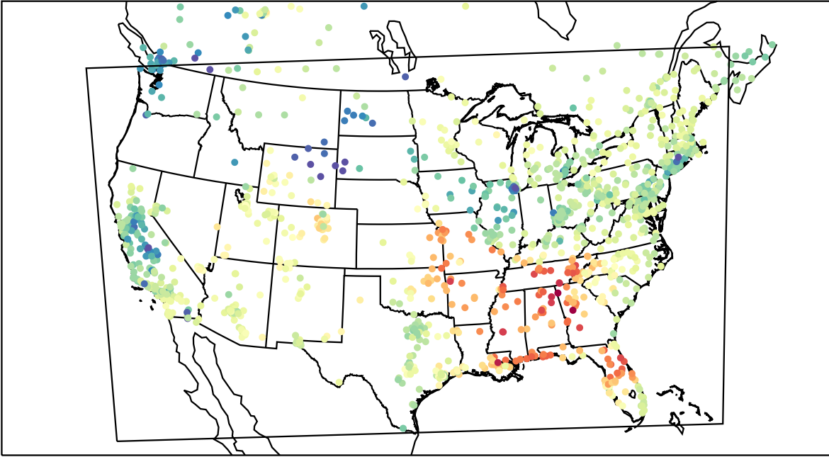
AirNOW (2022-03-04_22:00:00)
