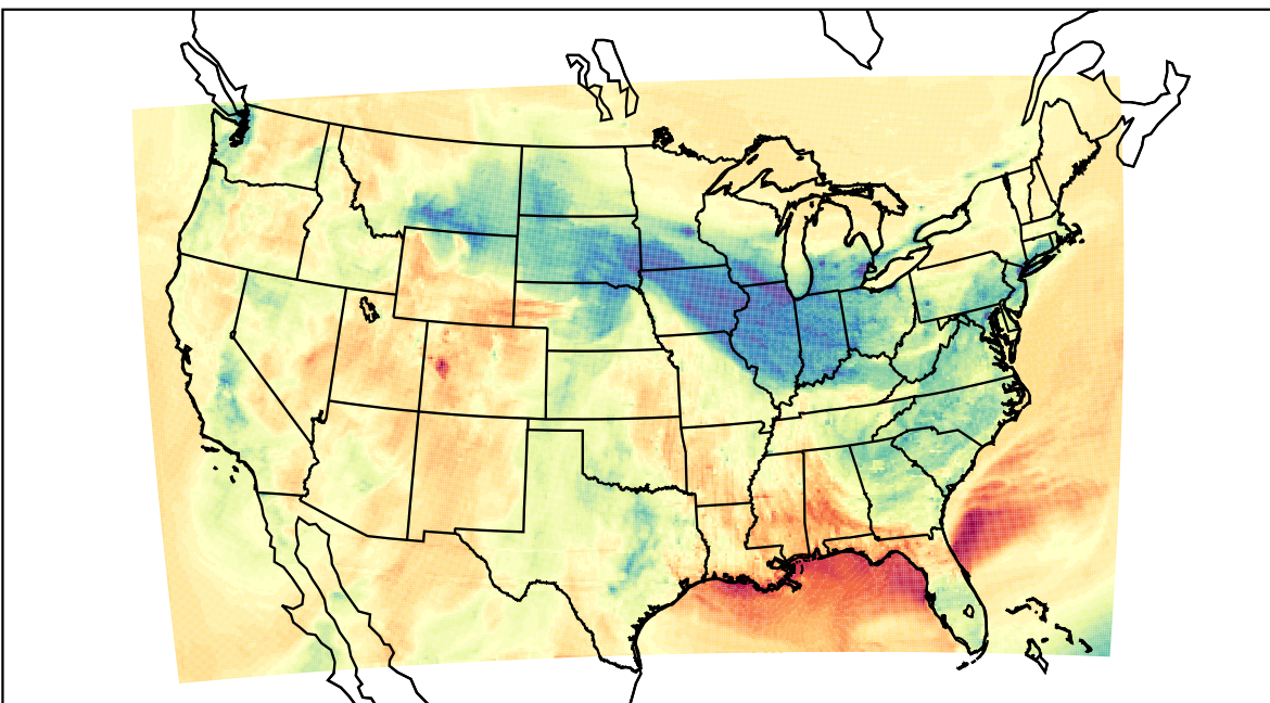
WRF (2022-03-05_00:00:00)
