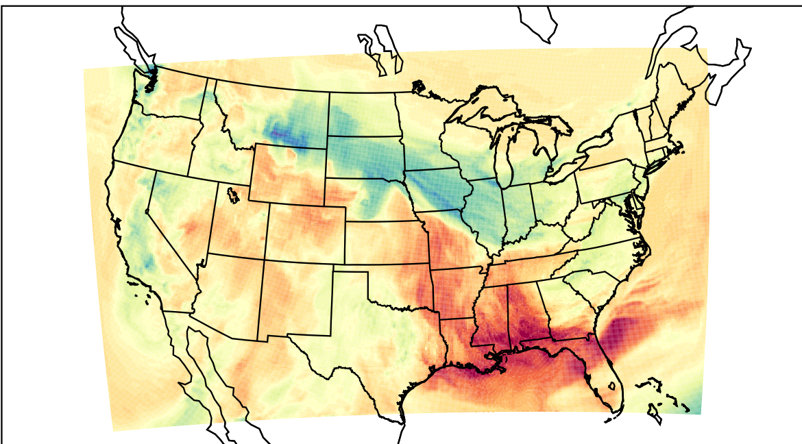
WRF (2022-03-04_21:00:00)
