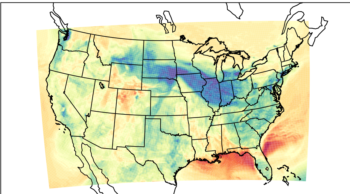
WRF (2022-03-05_02:00:00)
