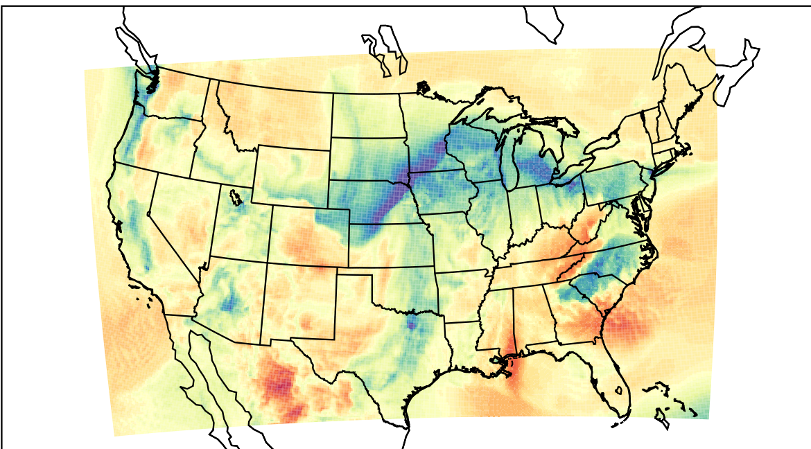
WRF (2022-03-05_17:00:00)
