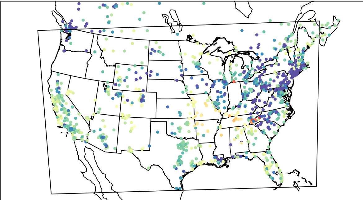
AirNOW (2022-03-05_07:00:00)
