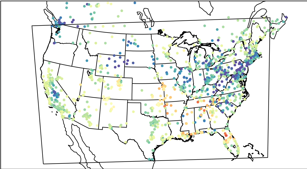
AirNOW (2022-03-05_01:00:00)
