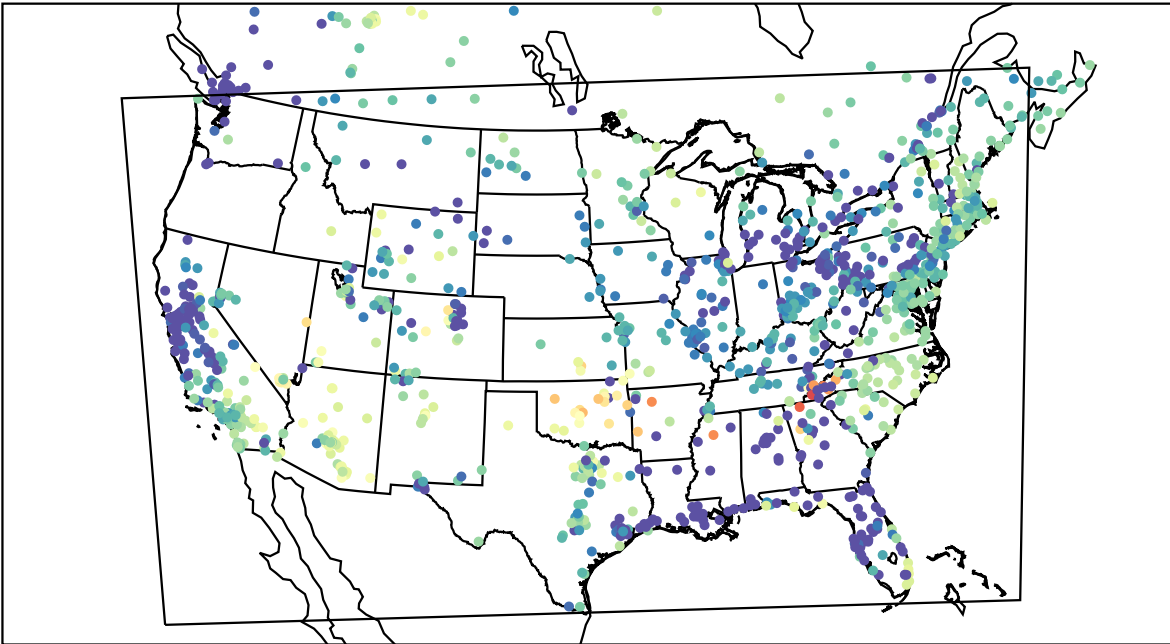
AirNOW (2022-03-04_09:00:00)
