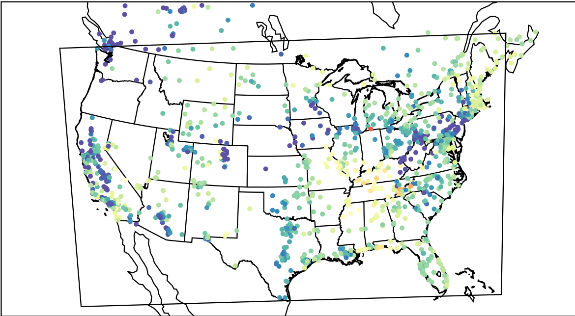
AirNOW (2022-03-05_14:00:00)
