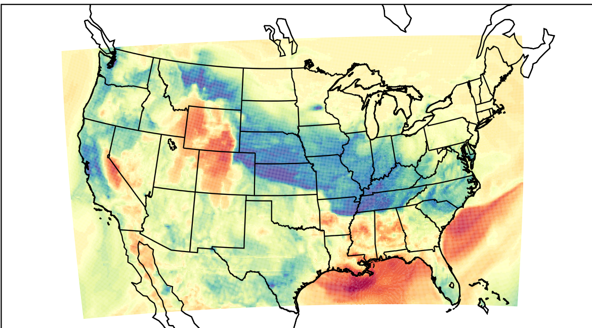
WRF (2022-03-04_05:00:00)
