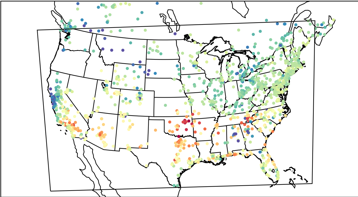
AirNOW (2022-03-04_00:00:00)
