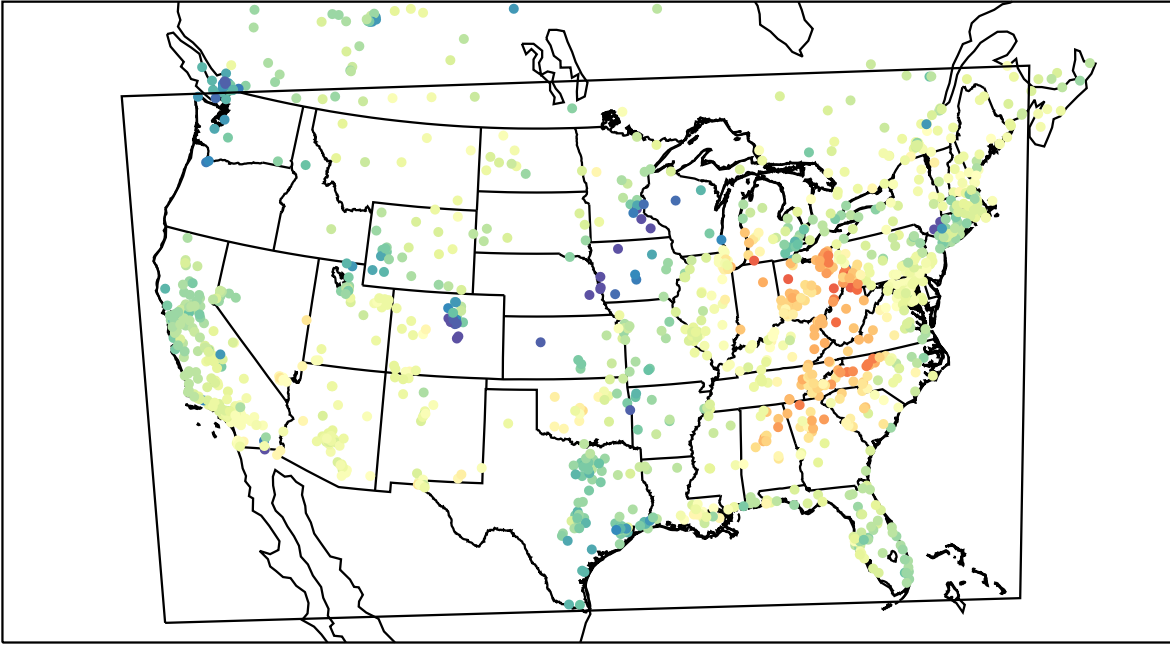
AirNOW (2022-03-05_22:00:00)
