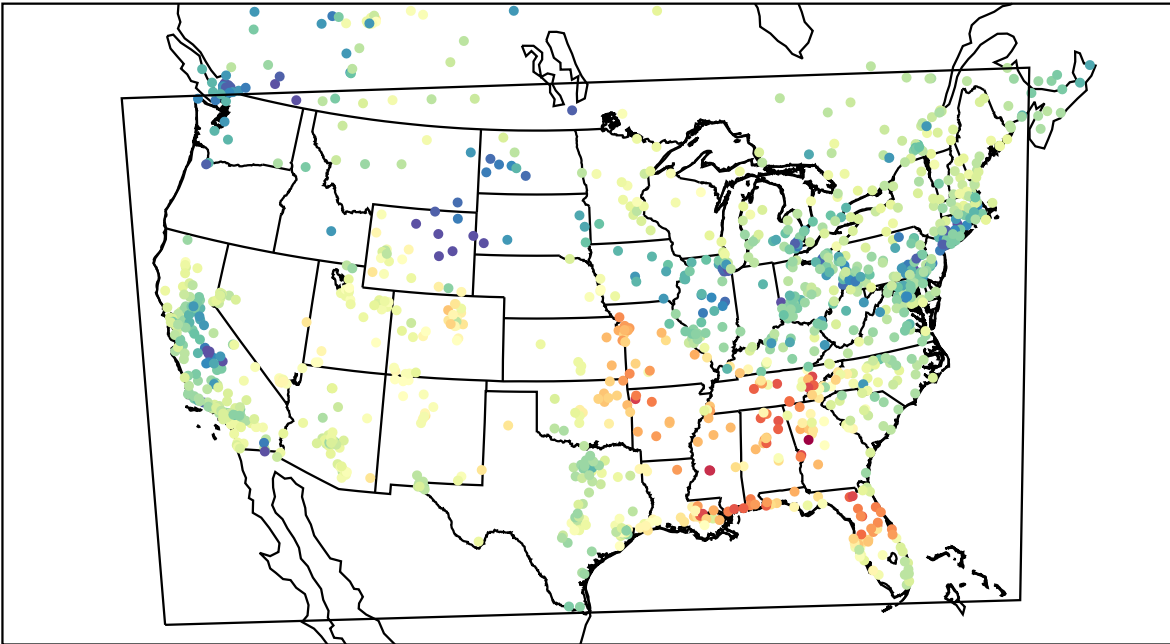
AirNOW (2022-03-04_23:00:00)
