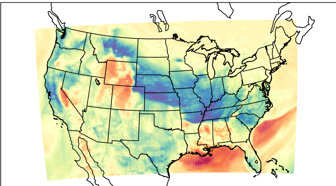
WRF (2022-03-04_07:00:00)
