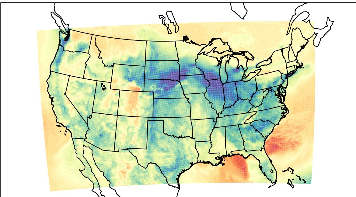
WRF (2022-03-05_08:00:00)
