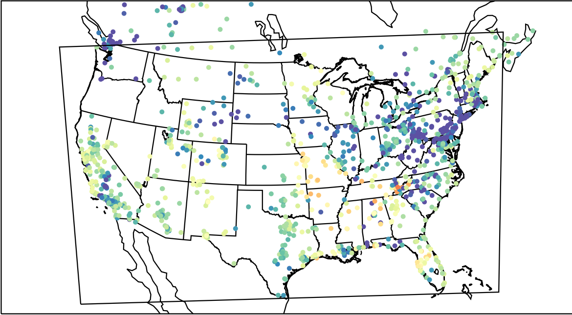
AirNOW (2022-03-05_05:00:00)
