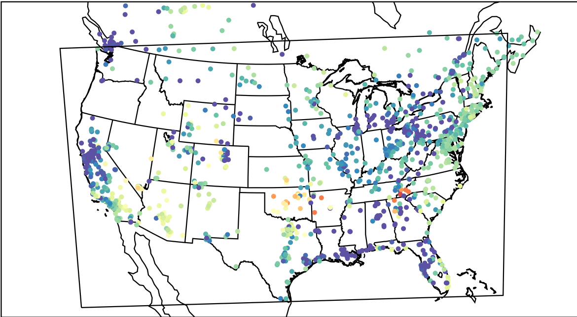
AirNOW (2022-03-04_08:00:00)
