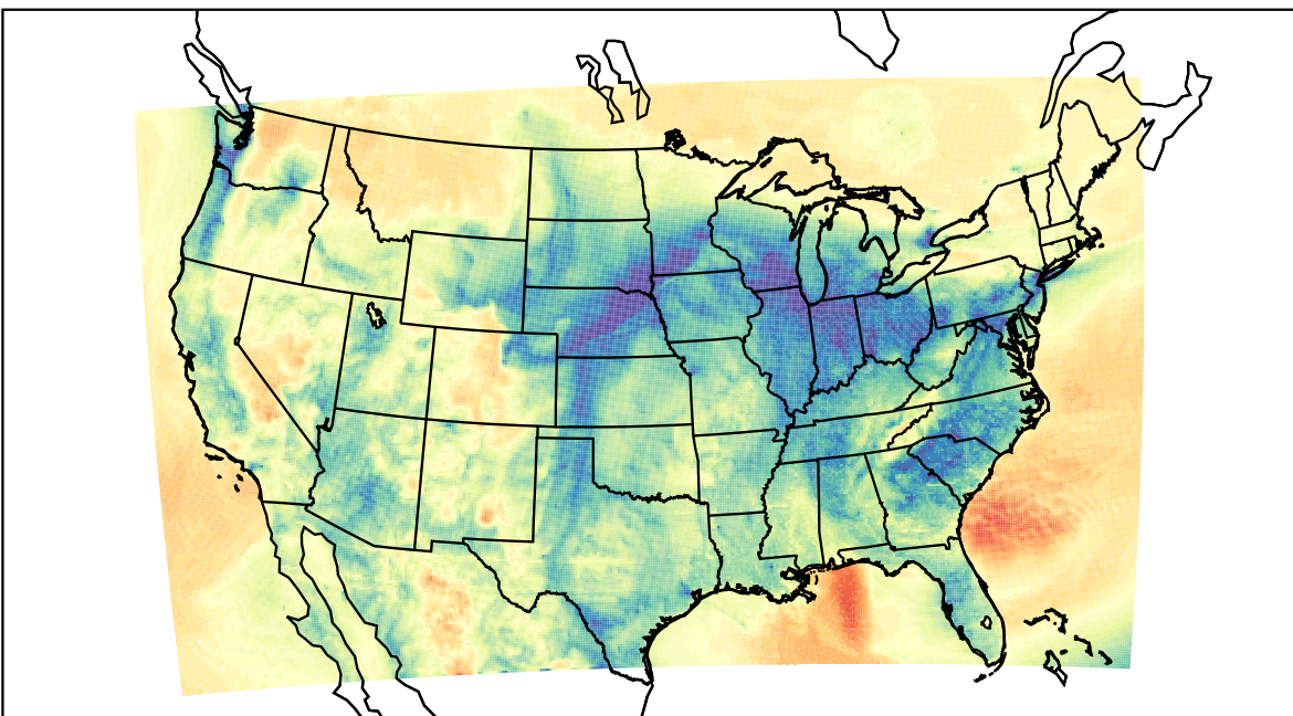
WRF (2022-03-05_12:00:00)
