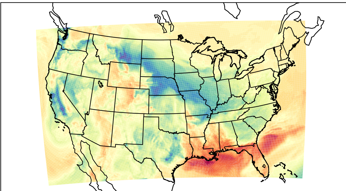
WRF (2022-03-04_17:00:00)
