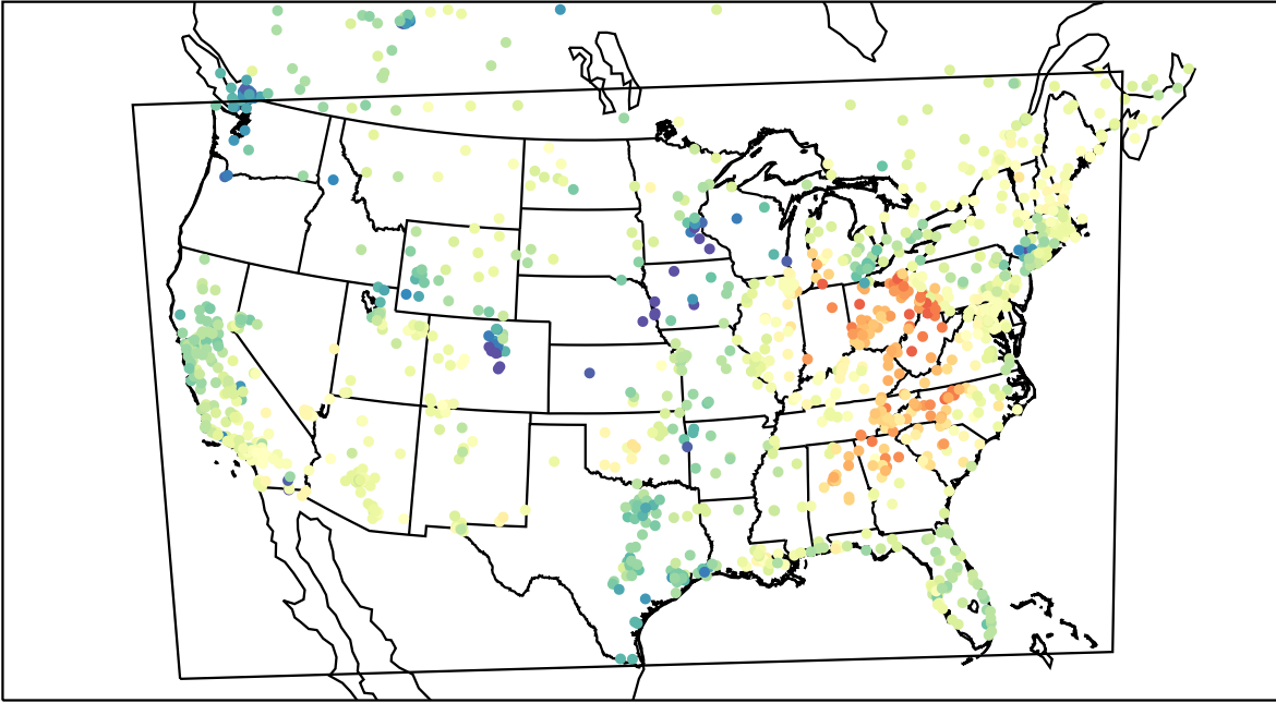
AirNOW (2022-03-05_21:00:00)
