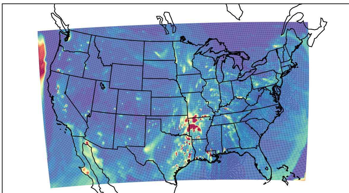
WRF 2022-03-13_02:00:00
