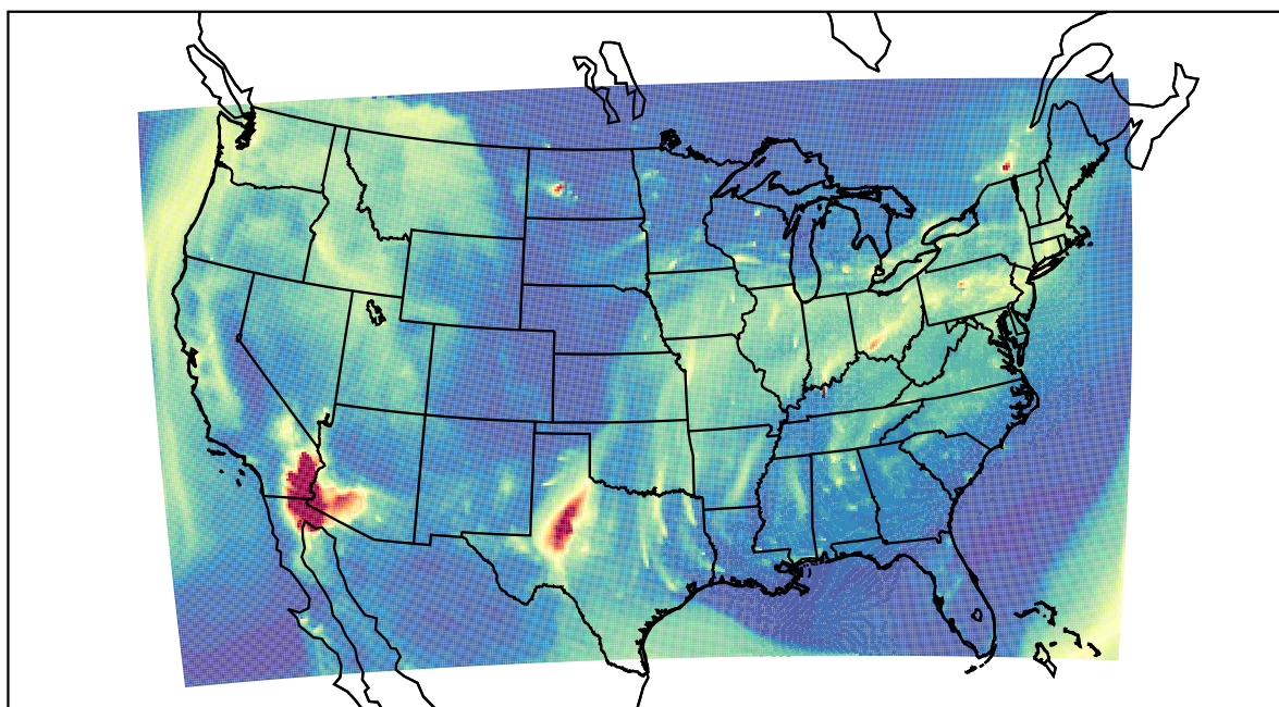
WRF 2022-03-14_12:00:00
