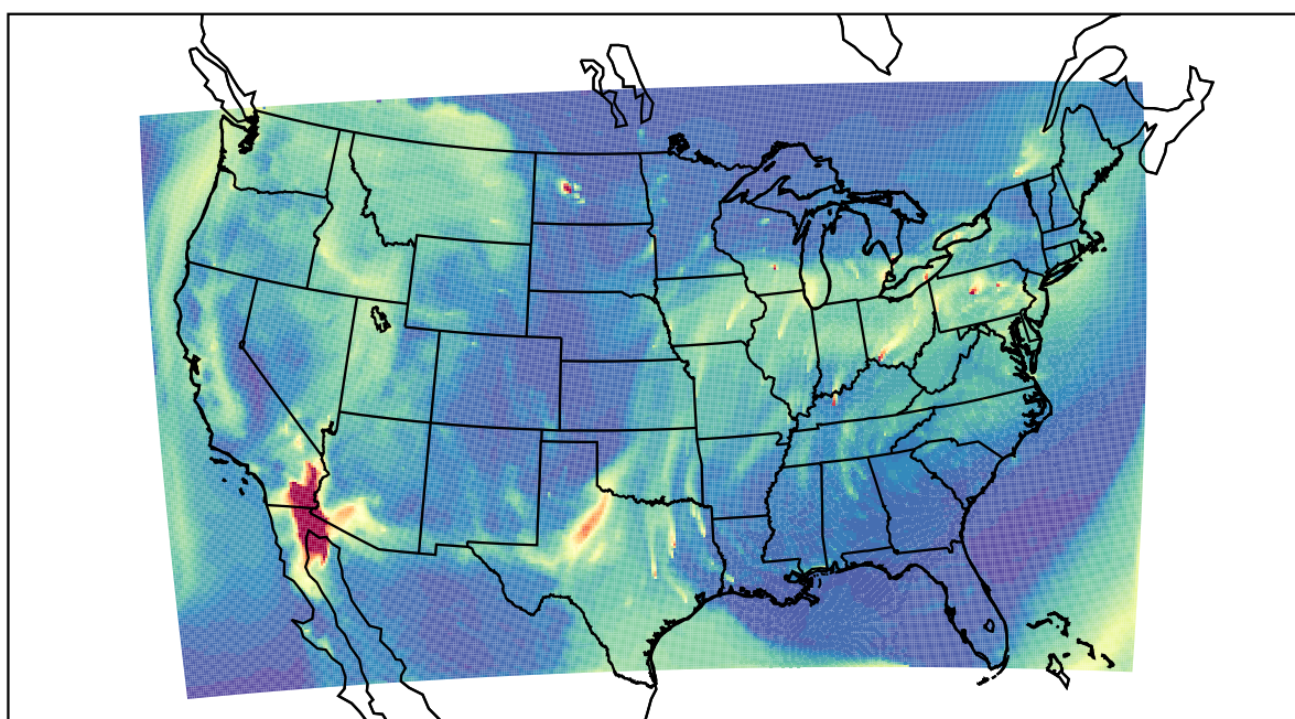
WRF 2022-03-14_16:00:00
