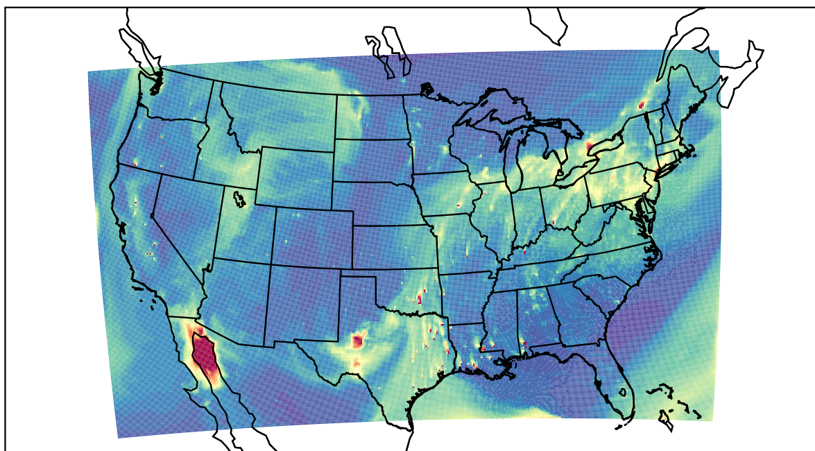
WRF 2022-03-14_23:00:00
