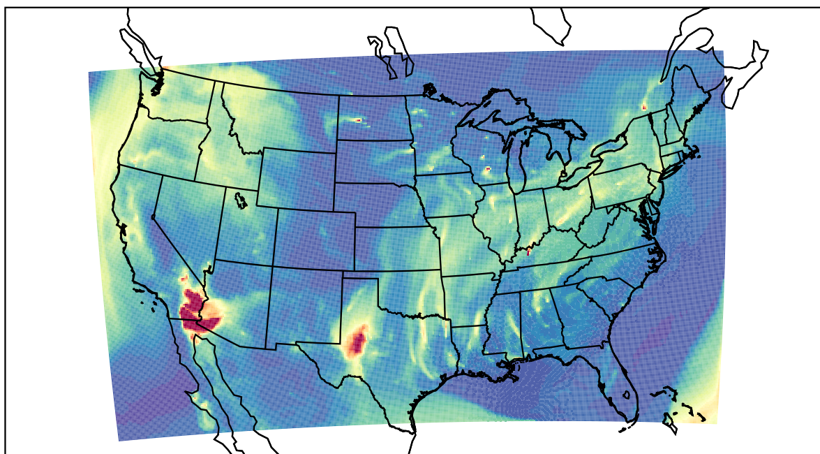
WRF 2022-03-14_08:00:00
