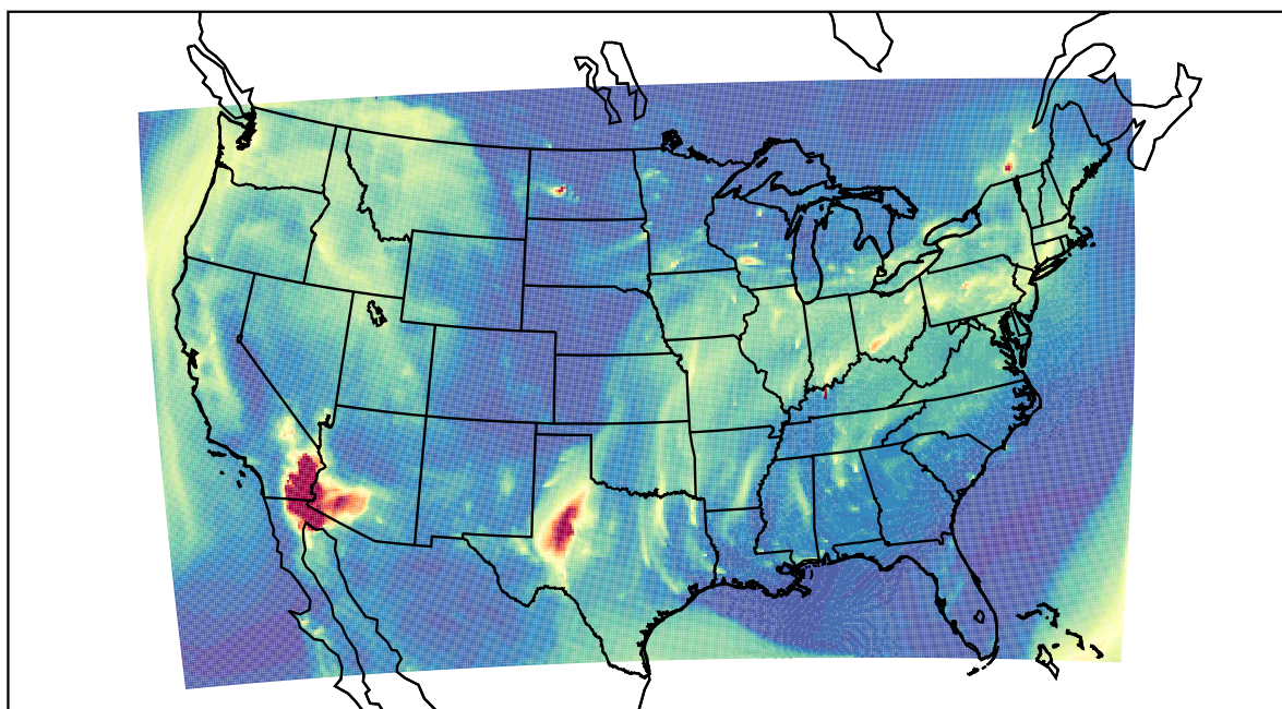
WRF 2022-03-14_11:00:00
