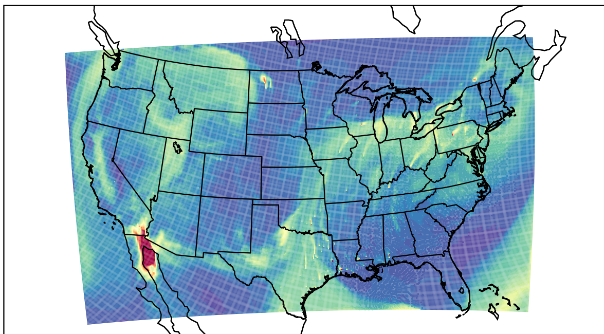
WRF 2022-03-14_19:00:00
