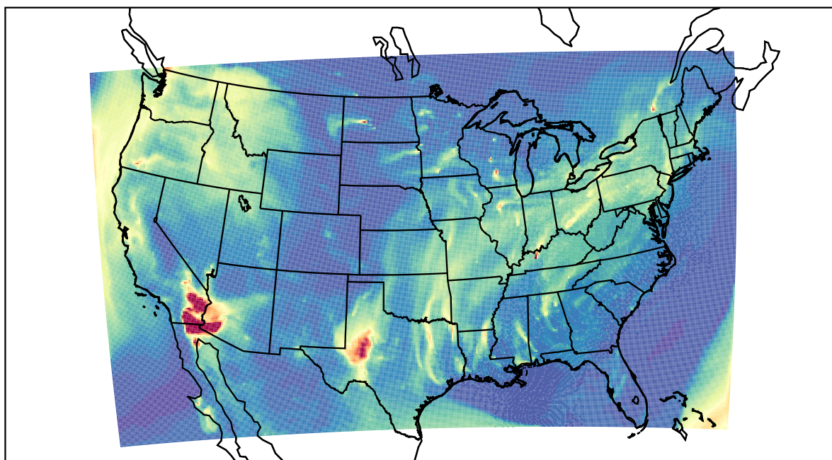
WRF 2022-03-14_07:00:00
