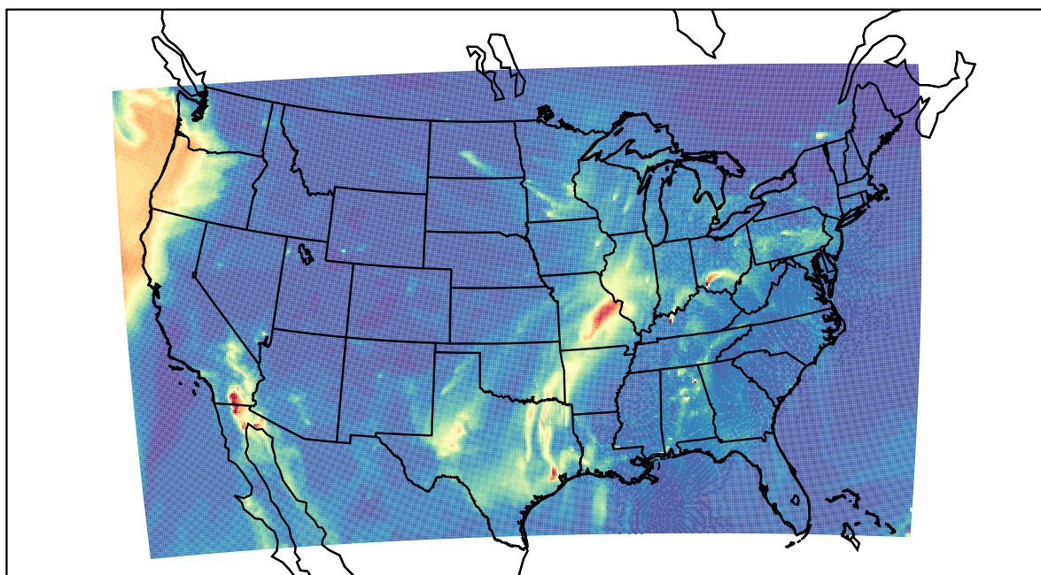
WRF 2022-03-13_11:00:00
