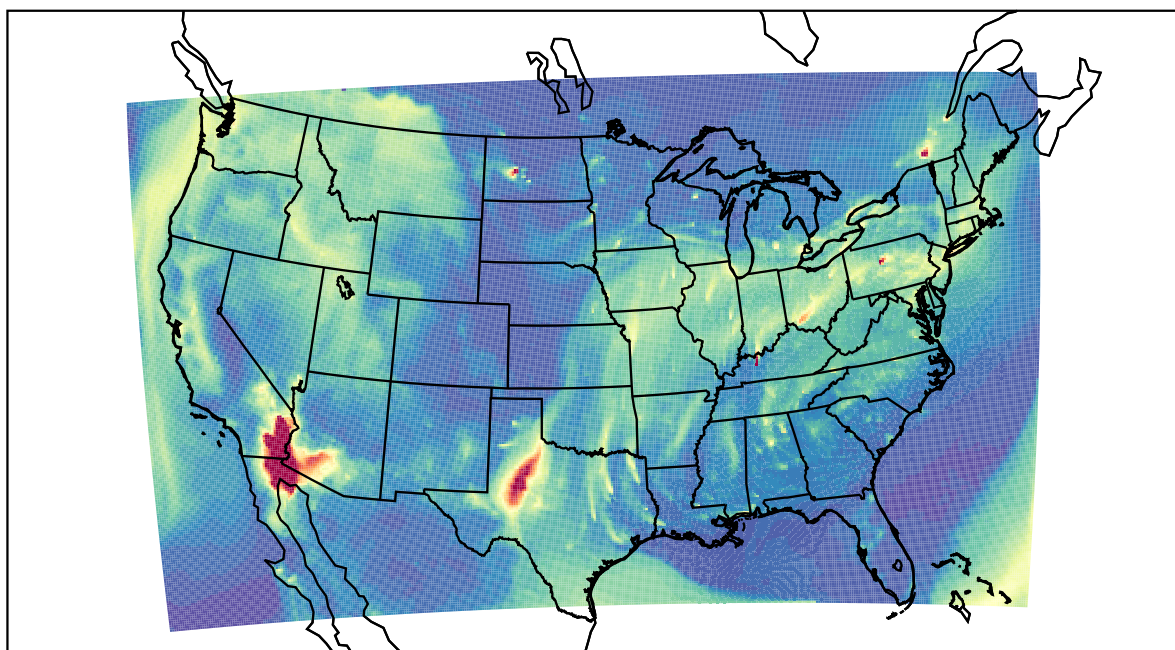
WRF 2022-03-14_13:00:00
