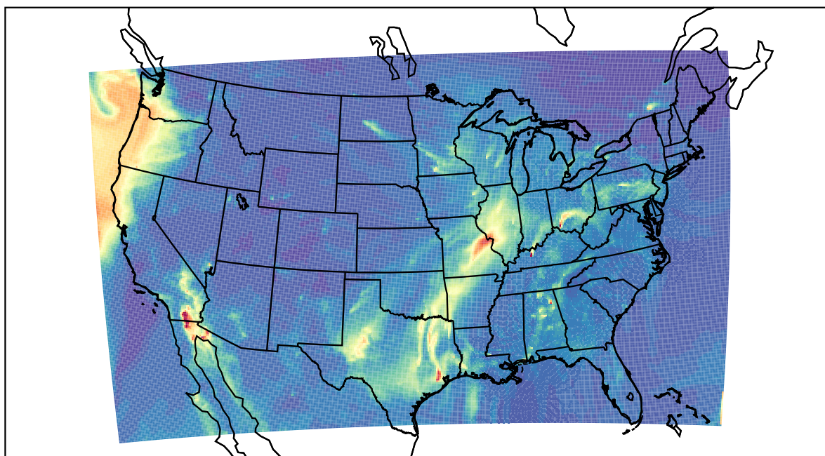
WRF 2022-03-13_12:00:00
