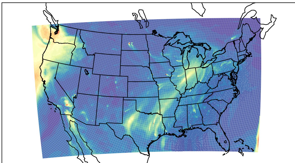
WRF 2022-03-13_17:00:00
