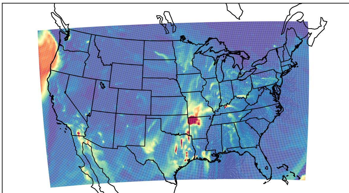
WRF 2022-03-13_06:00:00
