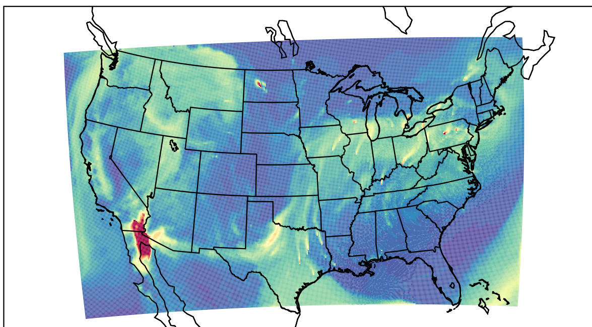
WRF 2022-03-14_17:00:00
