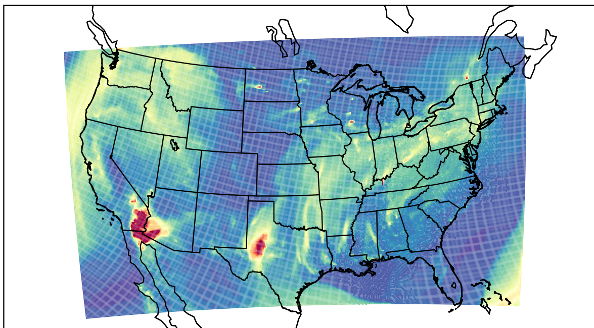
WRF 2022-03-14_09:00:00
