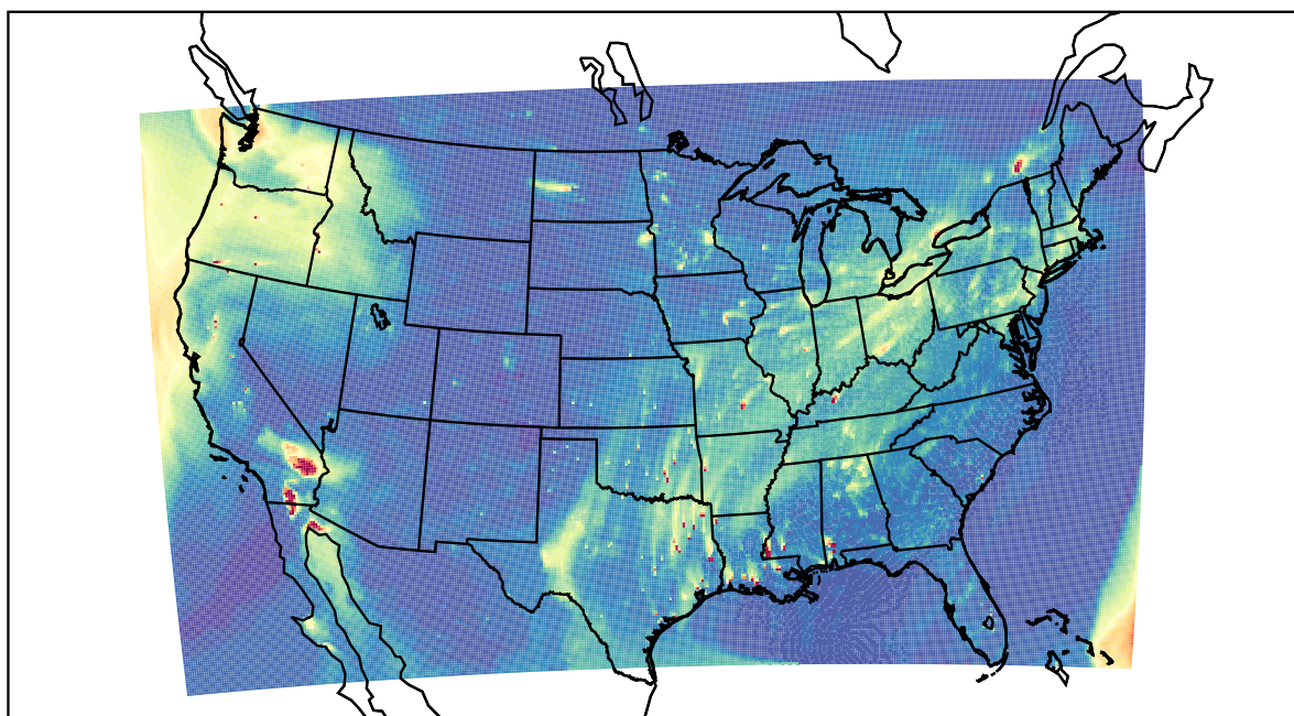
WRF 2022-03-14_00:00:00
