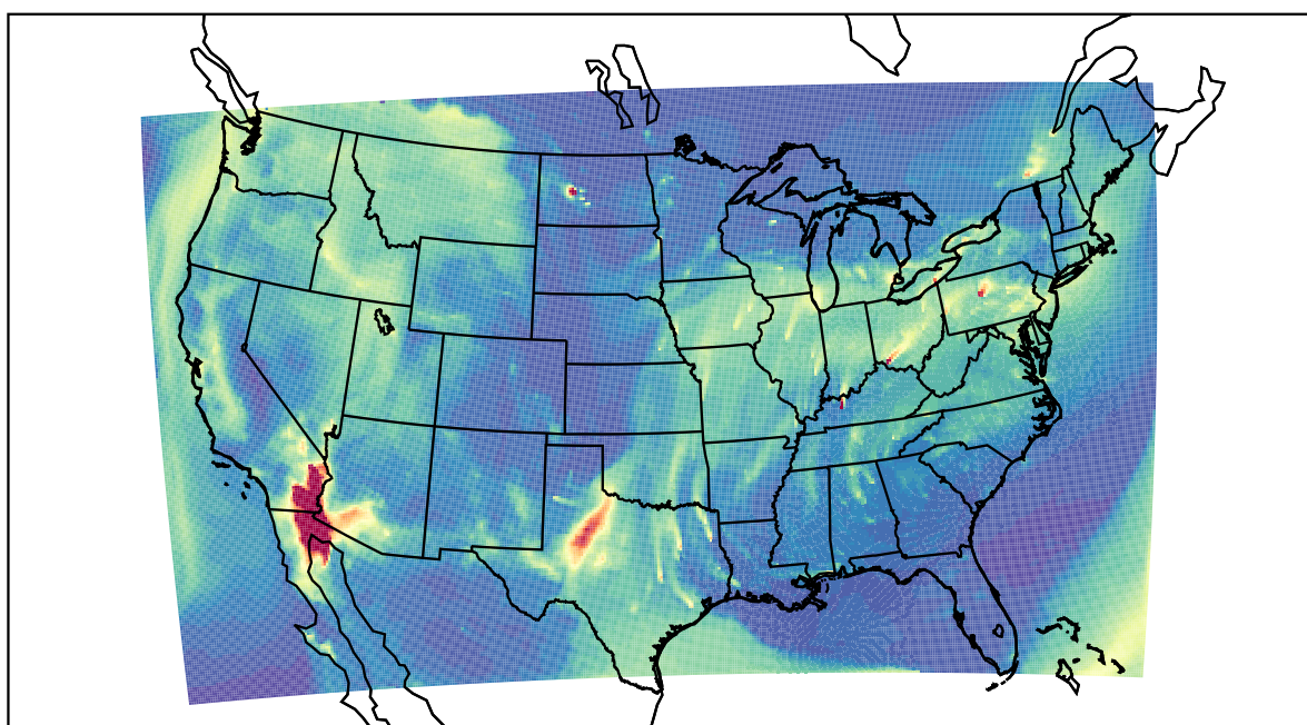
WRF 2022-03-14_15:00:00
