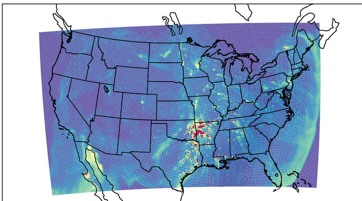
WRF 2022-03-13_00:00:00
