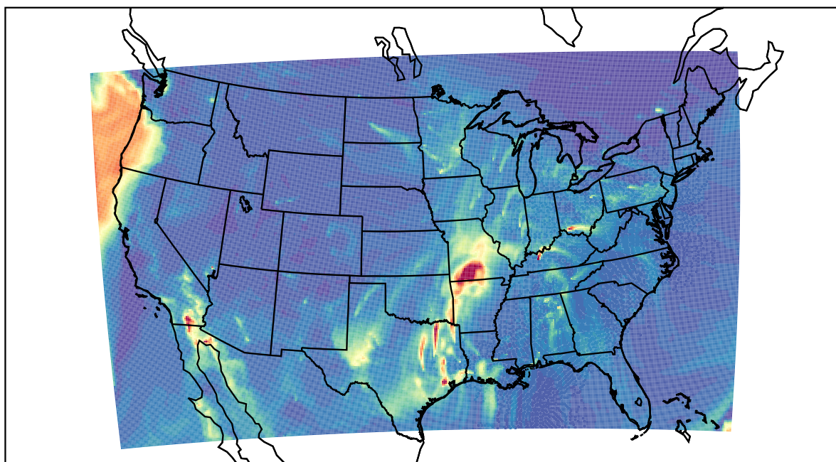
WRF 2022-03-13_08:00:00
