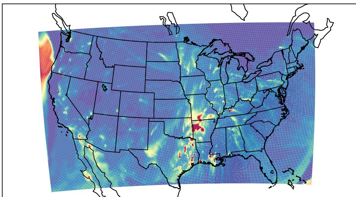
WRF 2022-03-13_04:00:00
