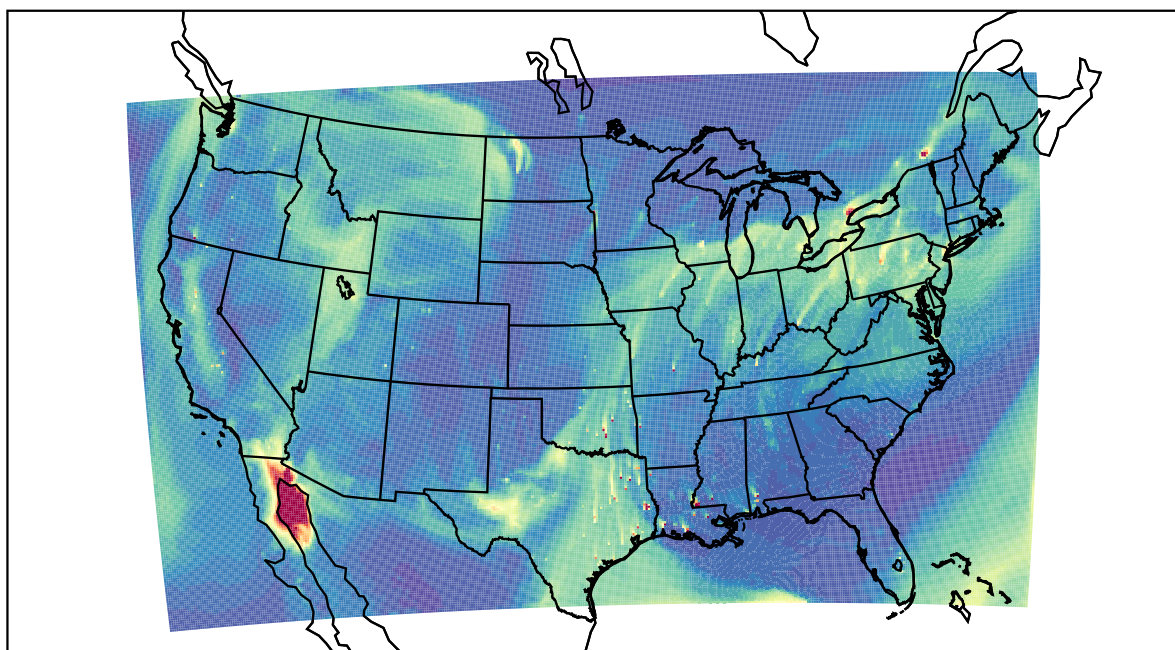
WRF 2022-03-14_21:00:00
