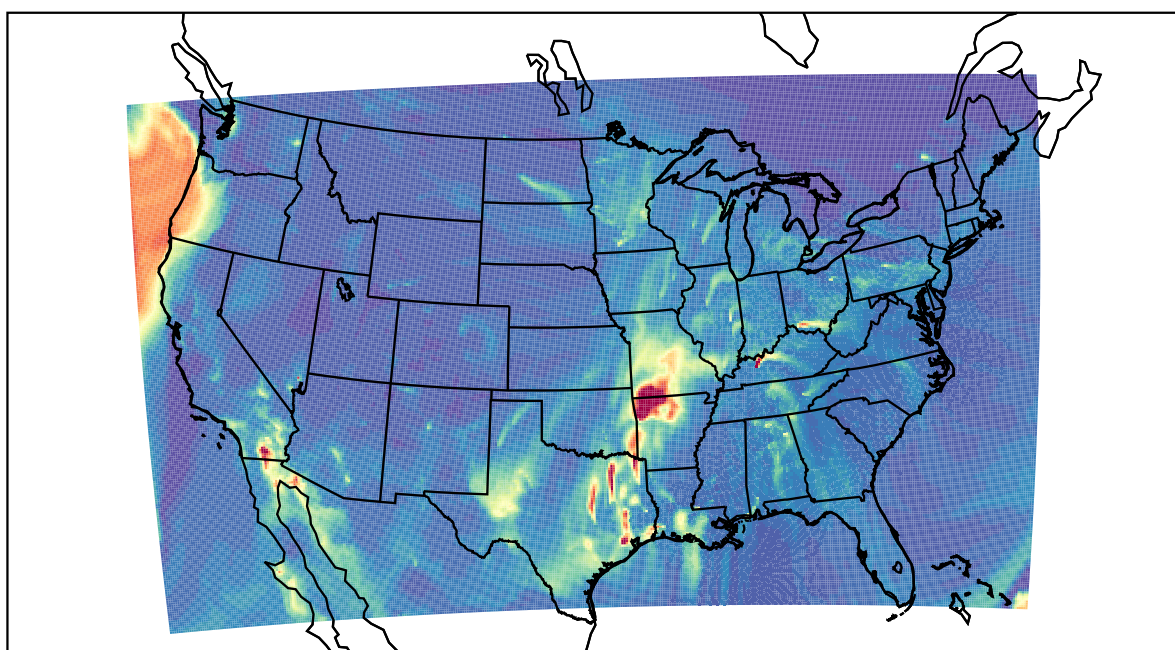
WRF 2022-03-13_07:00:00
