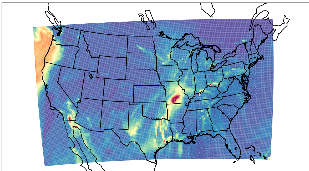
WRF 2022-03-13_09:00:00
