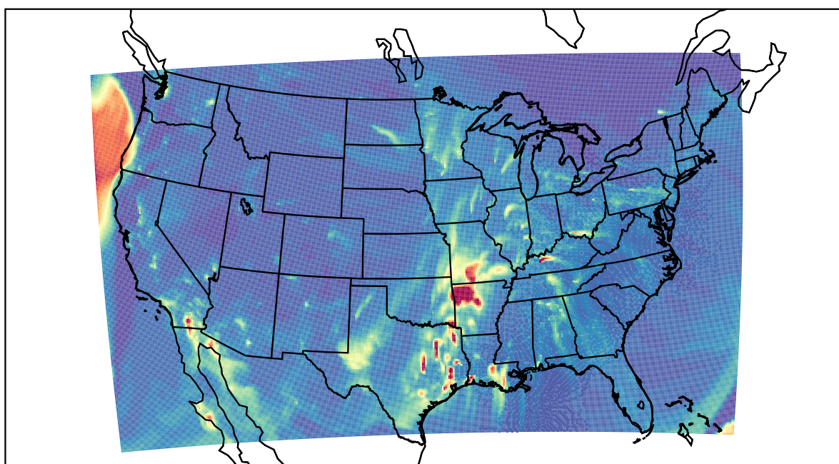
WRF 2022-03-13_05:00:00
