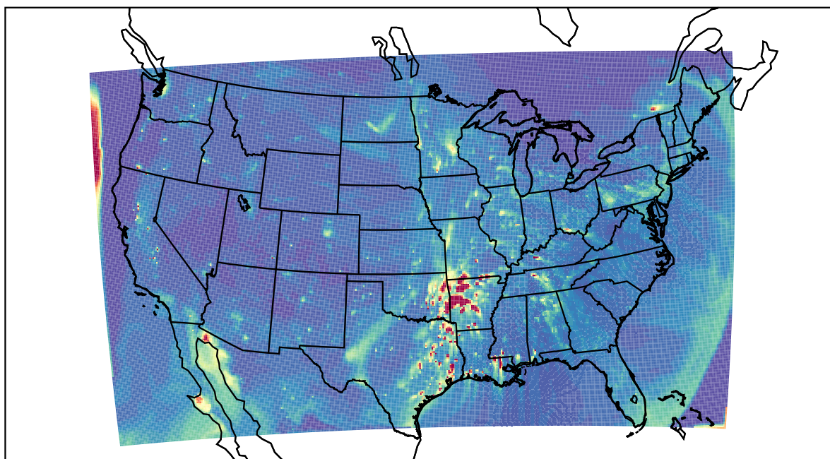
WRF 2022-03-13_01:00:00
