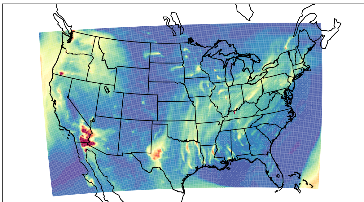
WRF 2022-03-14_05:00:00
