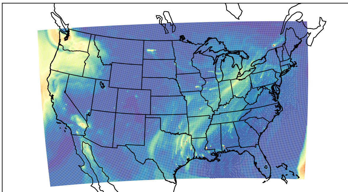
WRF 2022-03-13_21:00:00
