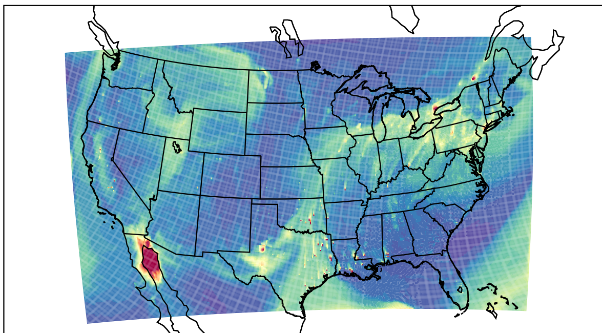
WRF 2022-03-14_22:00:00
