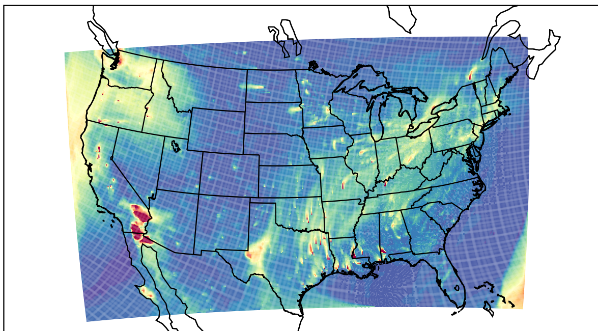
WRF 2022-03-14_02:00:00
