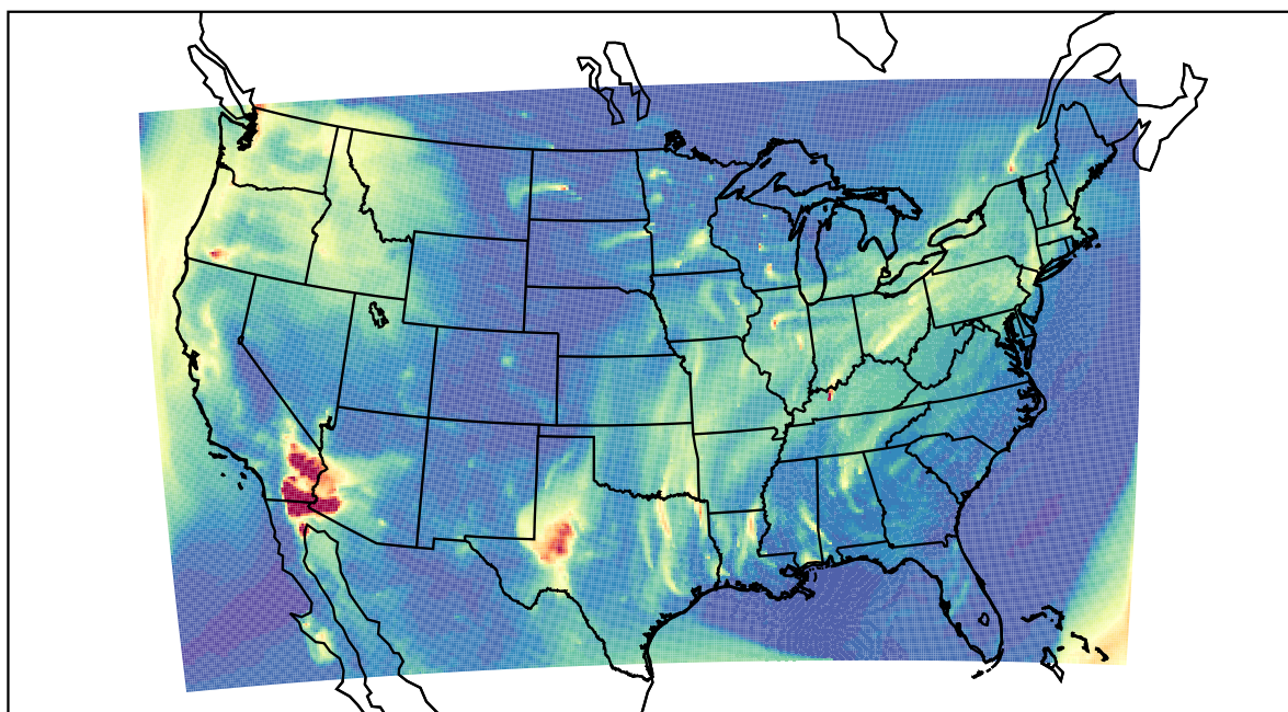
WRF 2022-03-14_06:00:00
