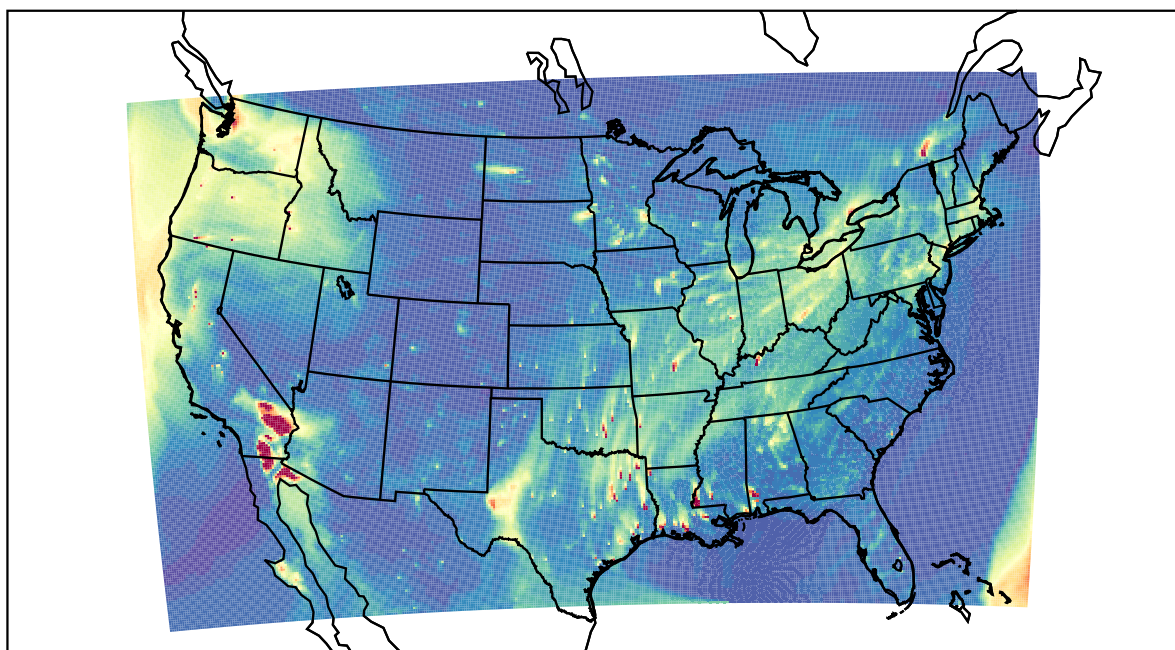
WRF 2022-03-14_01:00:00
