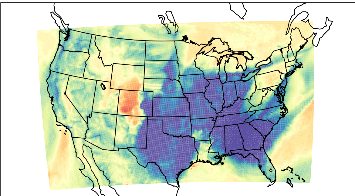
WRF (2022-03-15_12:00:00)
