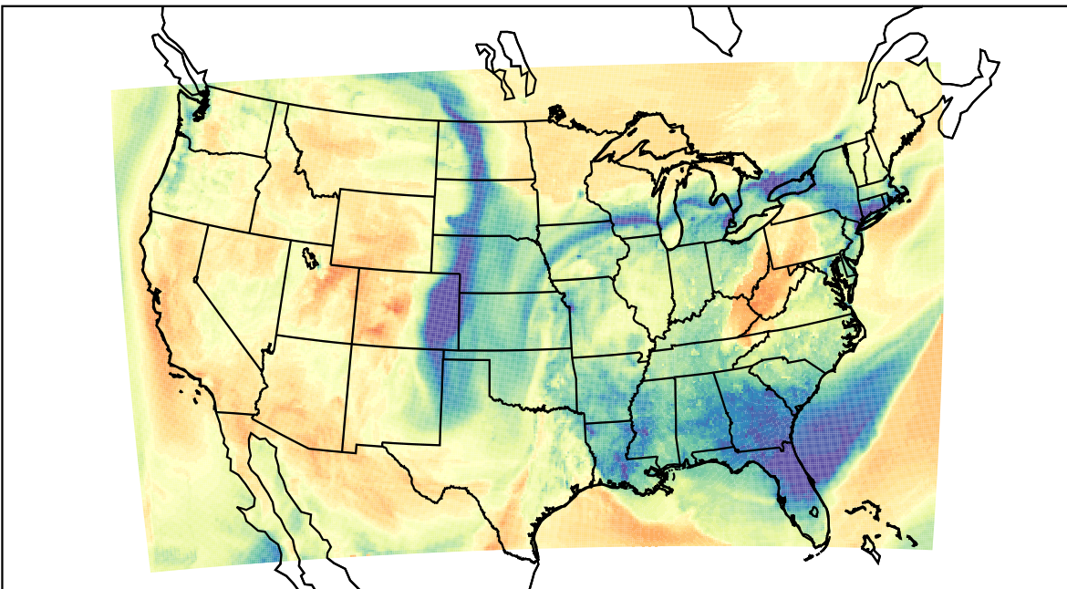
WRF (2022-03-14_23:00:00)
