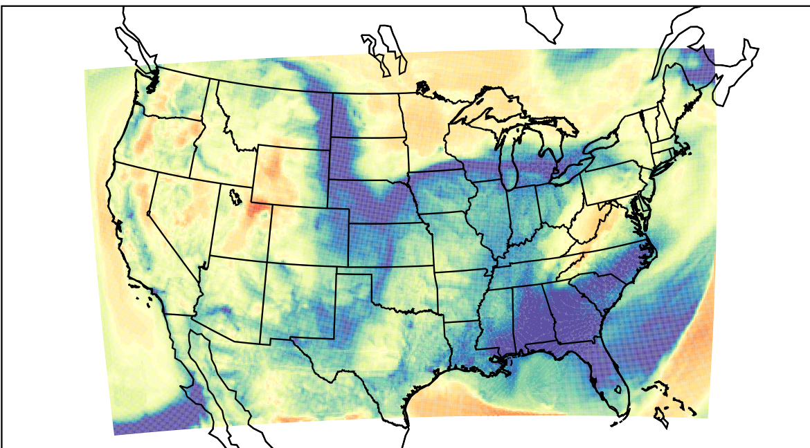
WRF (2022-03-14_14:00:00)
