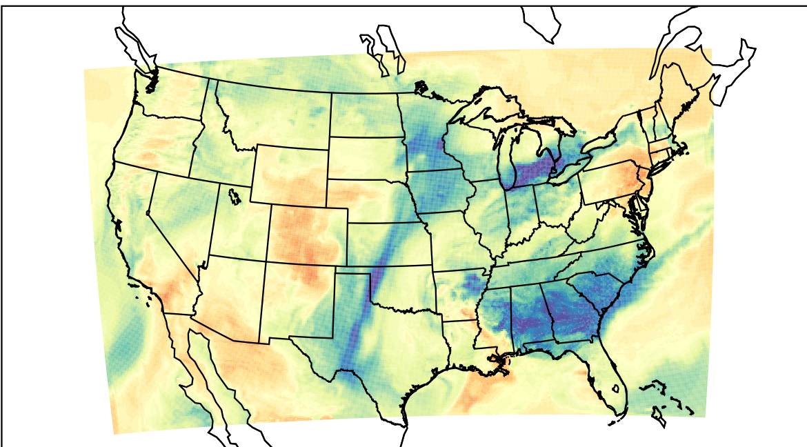
WRF (2022-03-15_21:00:00)
