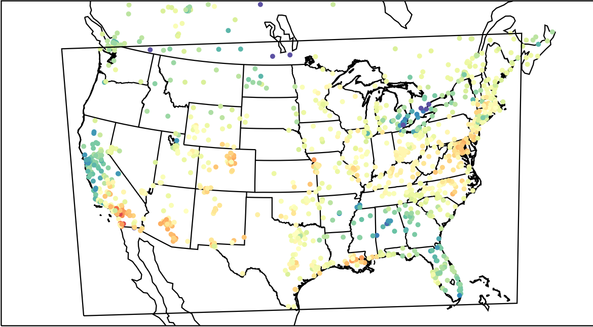
AirNOW (2022-03-15_21:00:00)
