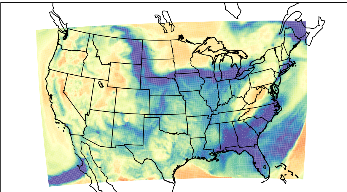
WRF (2022-03-14_11:00:00)
