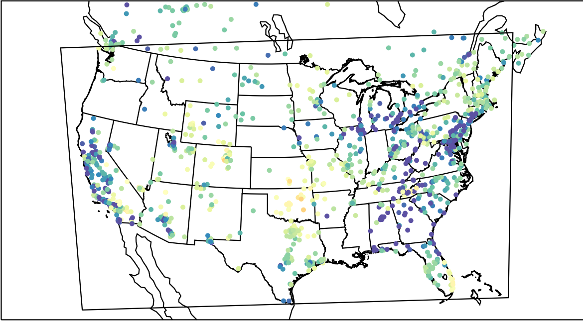
AirNOW (2022-03-14_07:00:00)
