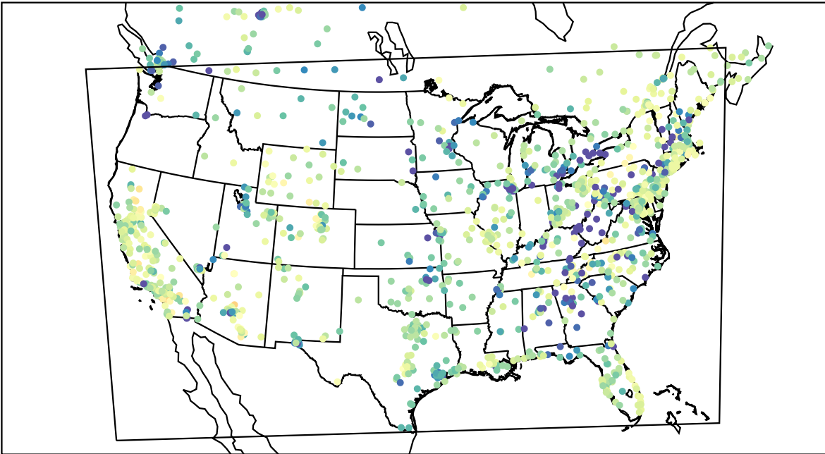
AirNOW (2022-03-15_02:00:00)
