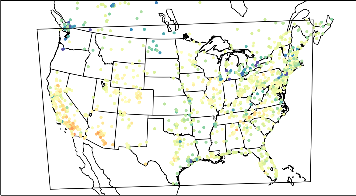
AirNOW (2022-03-14_23:00:00)
