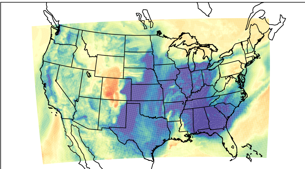
WRF (2022-03-15_15:00:00)
