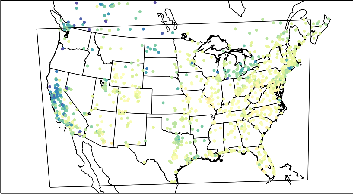
AirNOW (2022-03-14_17:00:00)
