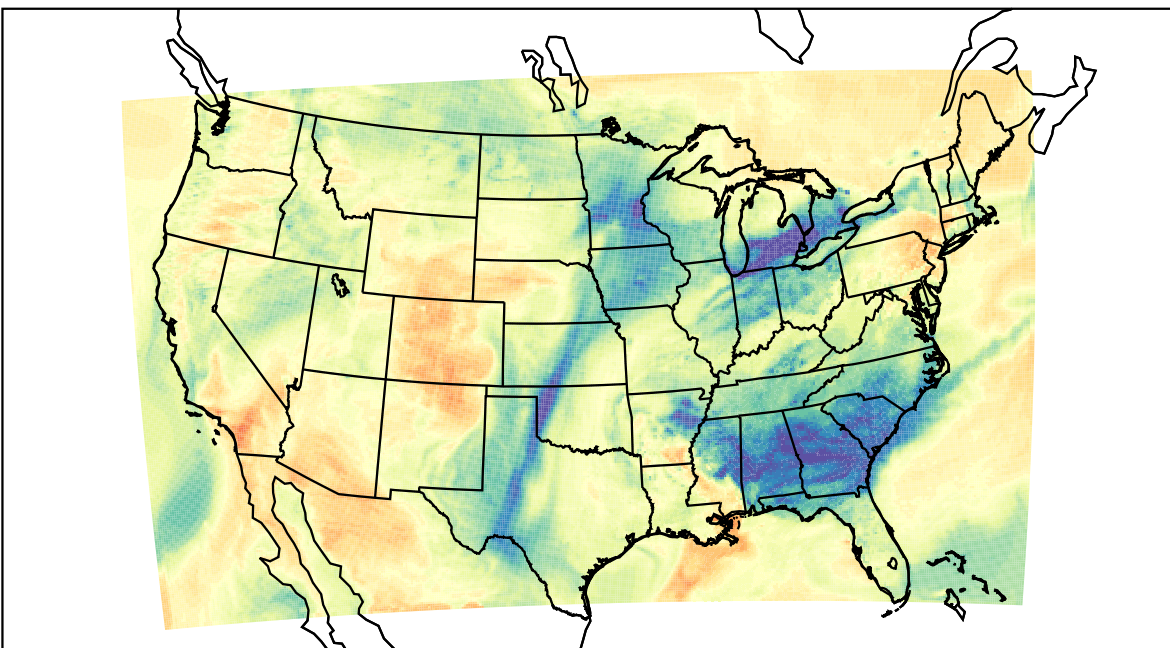
WRF (2022-03-15_22:00:00)
