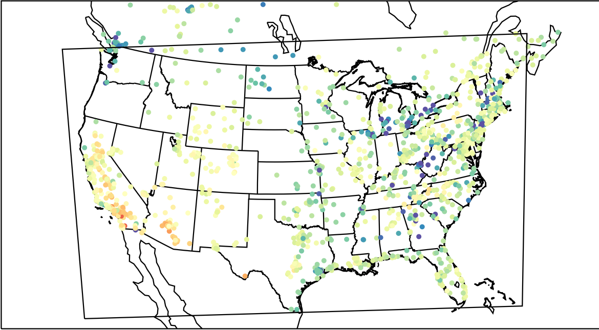
AirNOW (2022-03-15_00:00:00)
