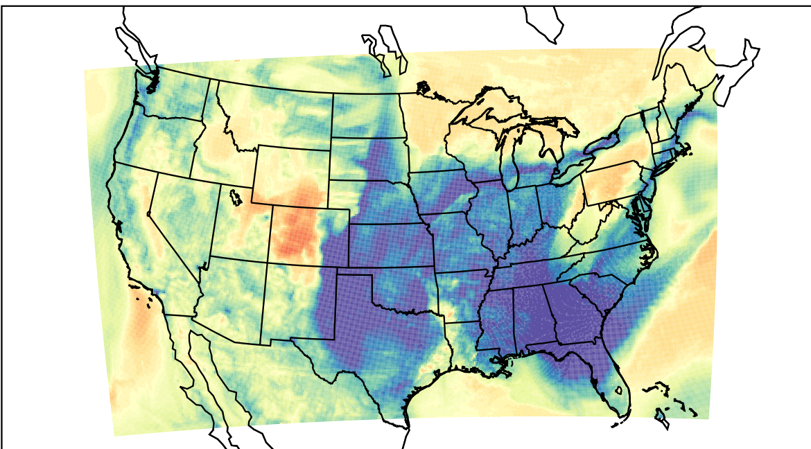
WRF (2022-03-15_08:00:00)
