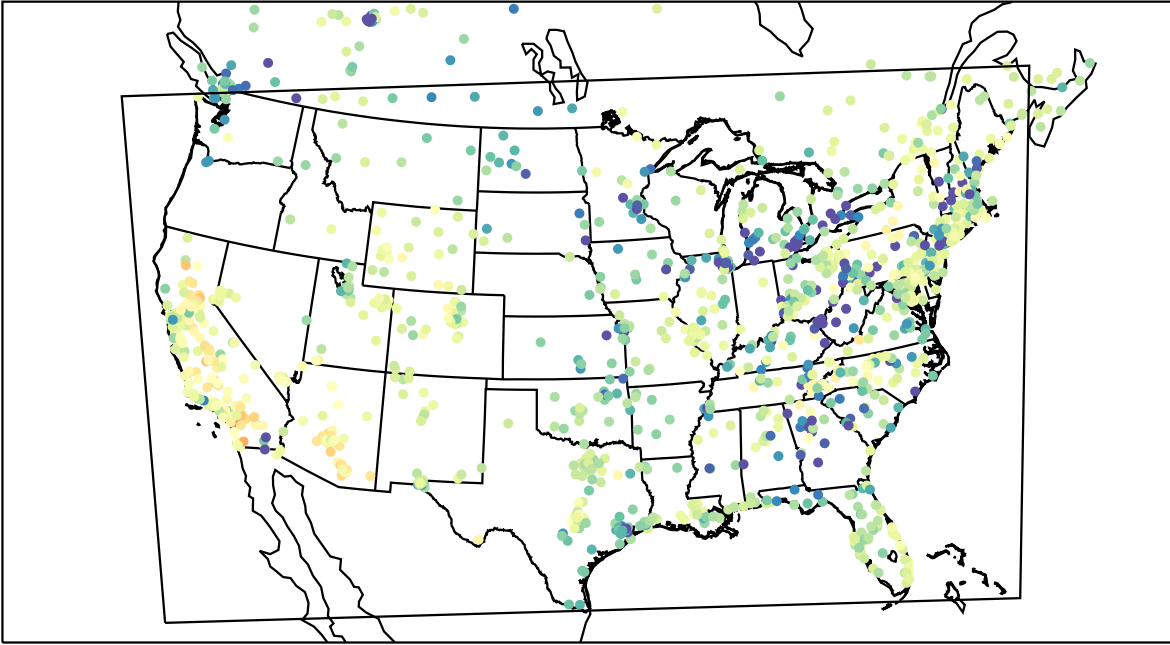
AirNOW (2022-03-15_01:00:00)
