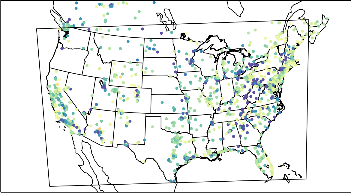
AirNOW (2022-03-15_03:00:00)
