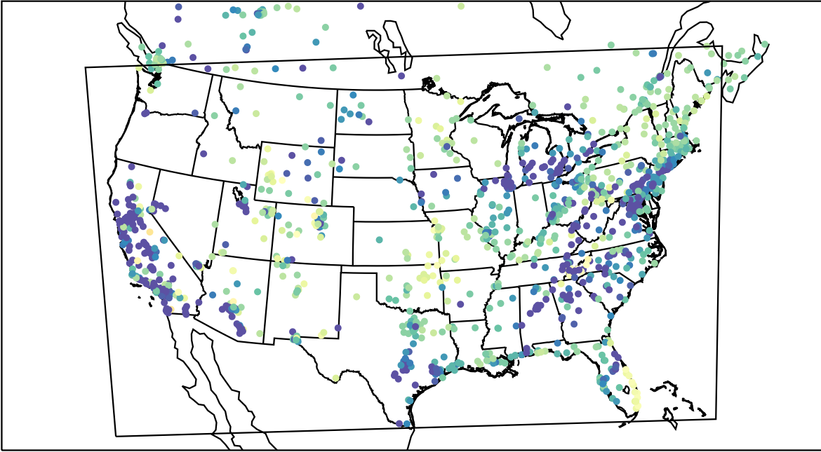
AirNOW (2022-03-14_13:00:00)
