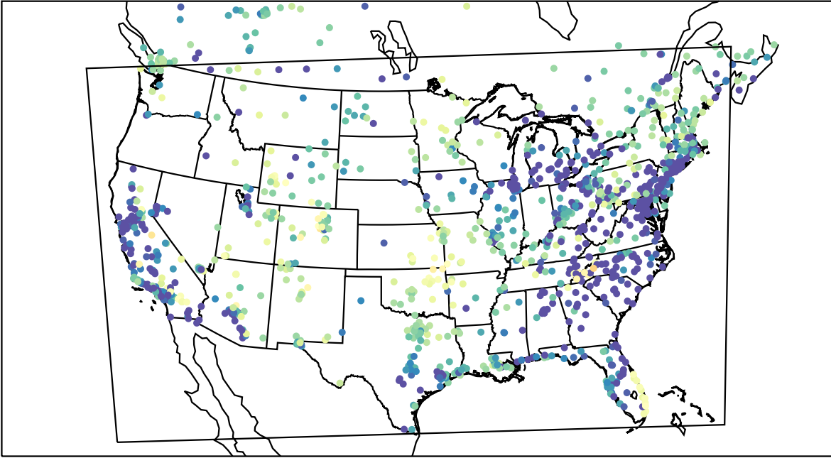
AirNOW (2022-03-14_11:00:00)
