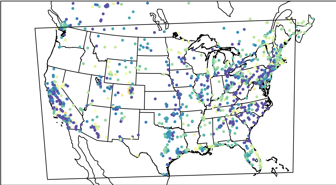
AirNOW (2022-03-15_09:00:00)
