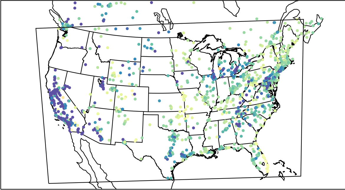
AirNOW (2022-03-14_14:00:00)
