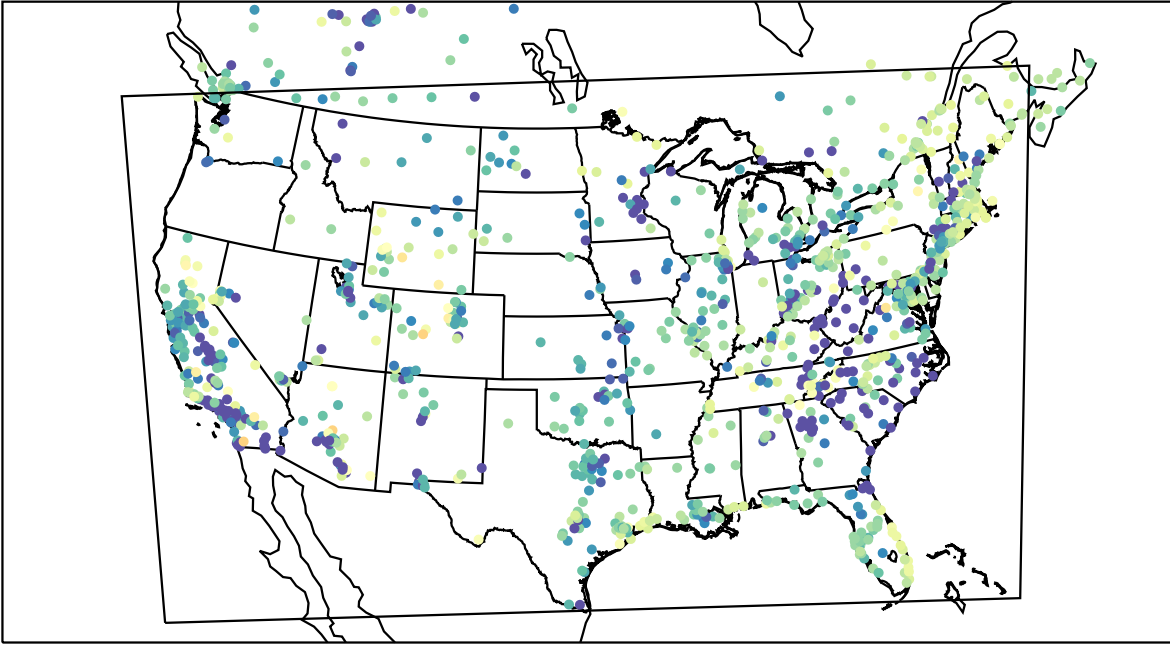
AirNOW (2022-03-15_06:00:00)
