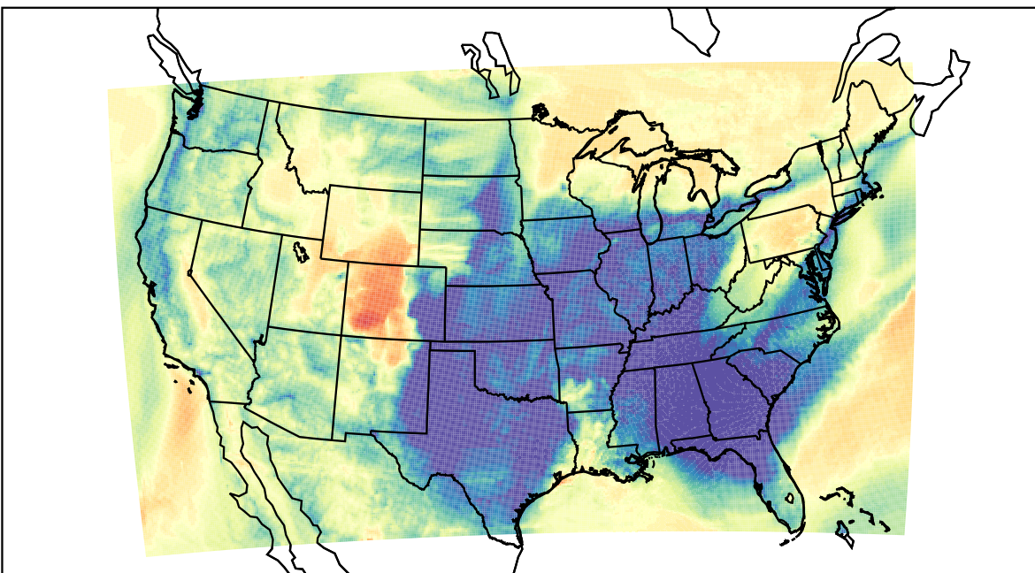
WRF (2022-03-15_11:00:00)
