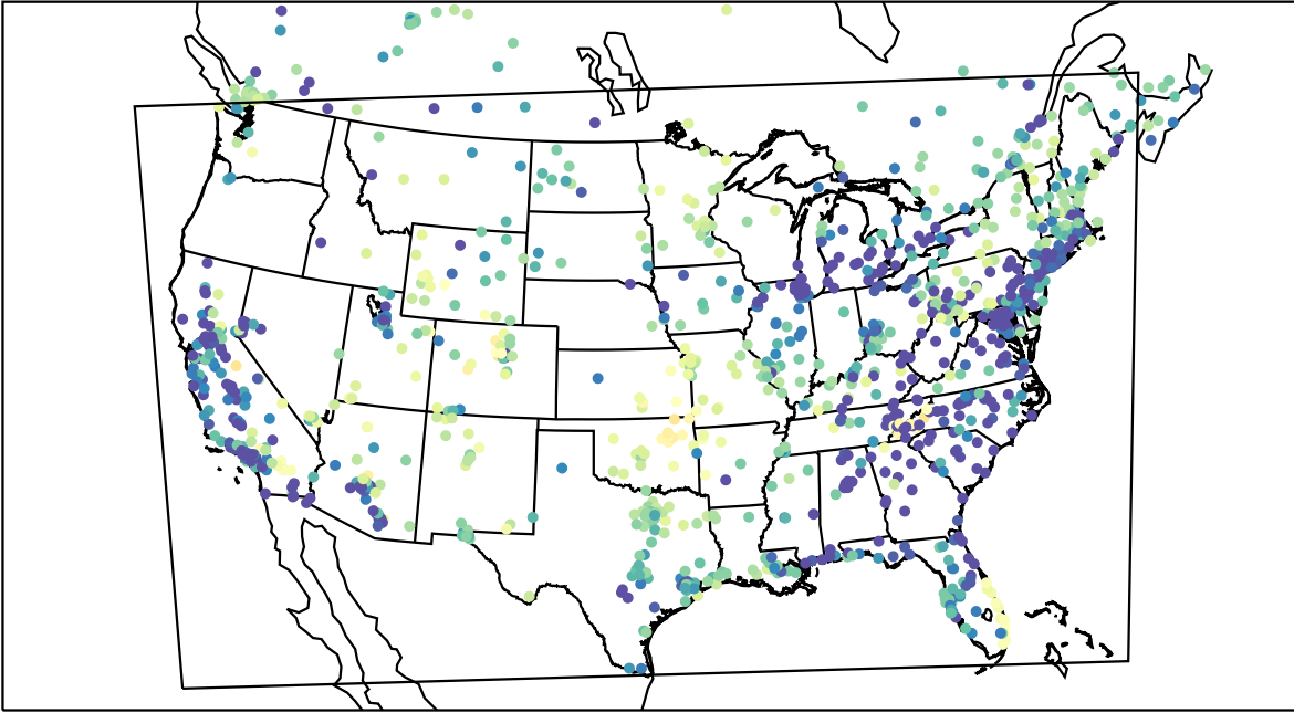
AirNOW (2022-03-14_10:00:00)
