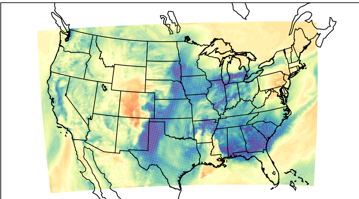
WRF (2022-03-15_17:00:00)
