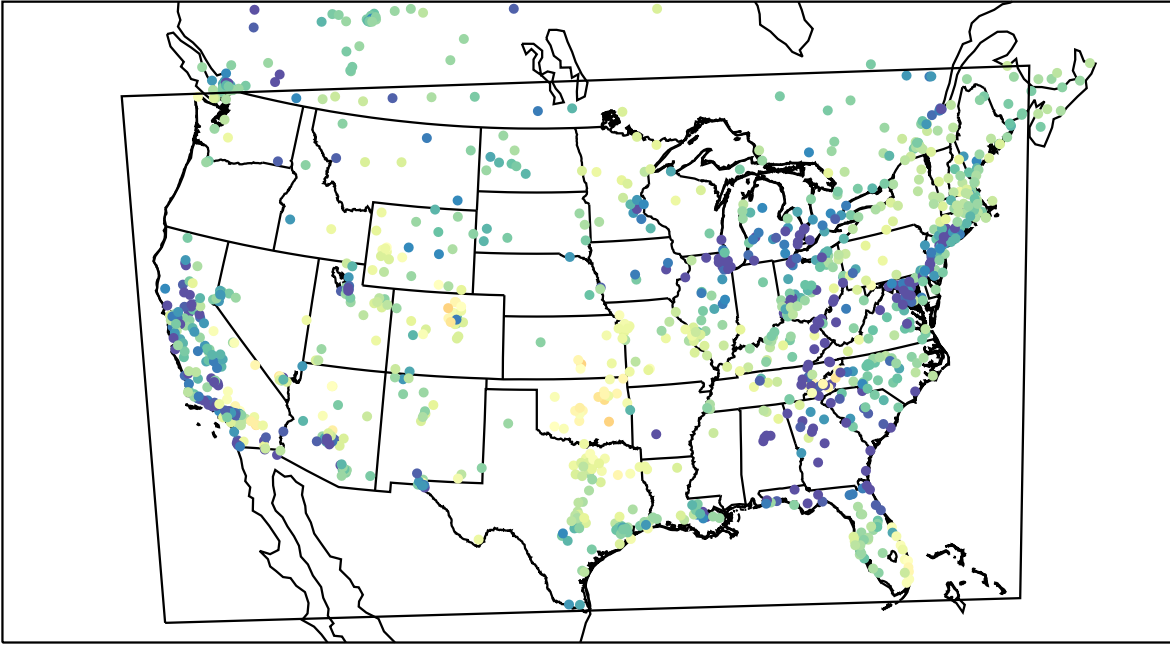
AirNOW (2022-03-14_06:00:00)
