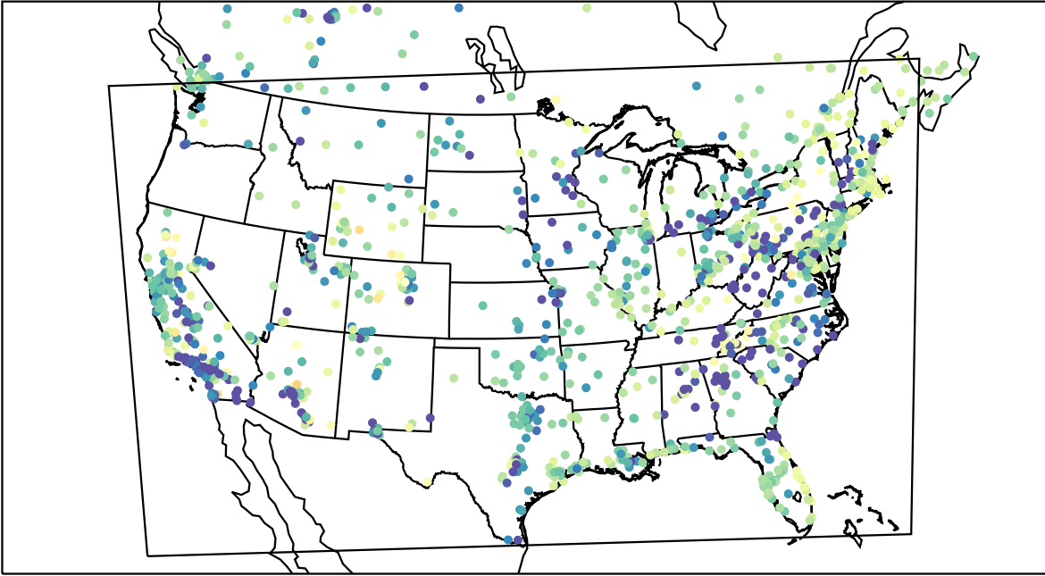
AirNOW (2022-03-15_05:00:00)
