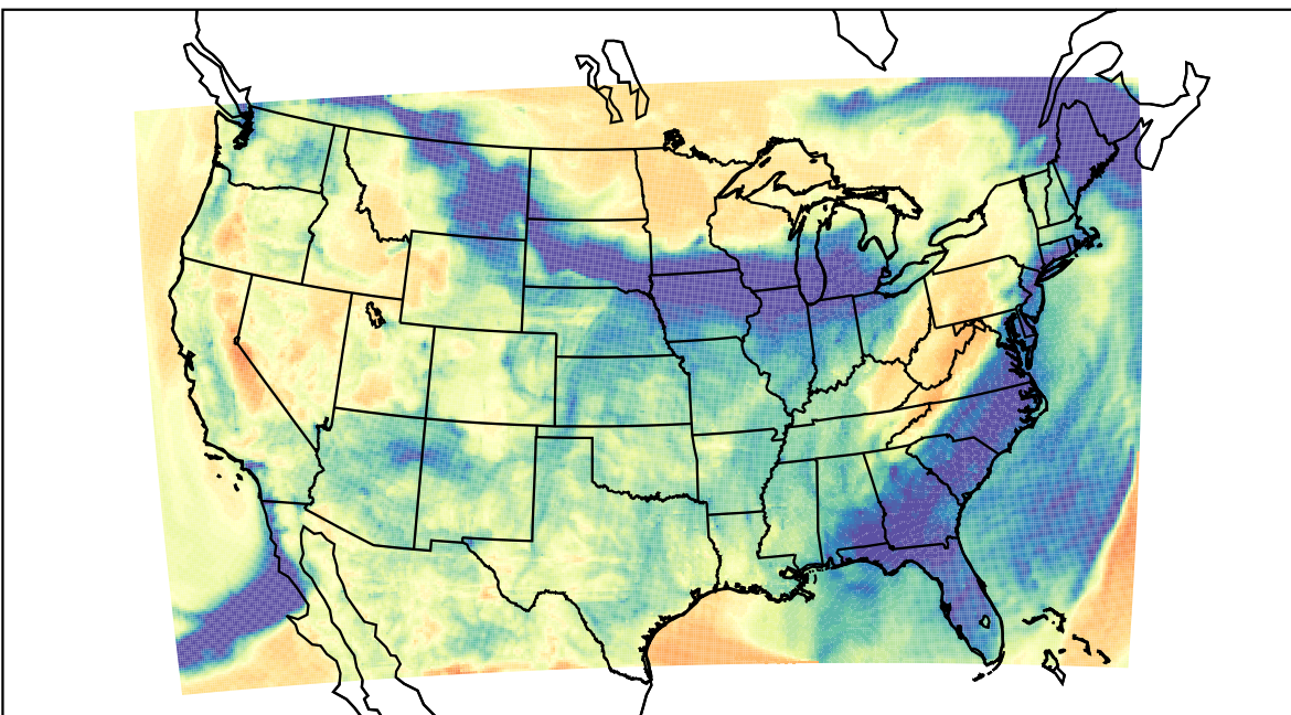
WRF (2022-03-14_05:00:00)
