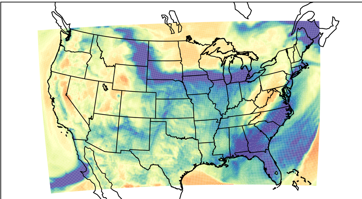
WRF (2022-03-14_09:00:00)
