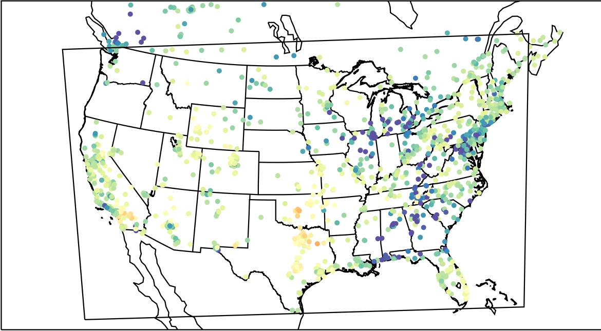
AirNOW (2022-03-14_02:00:00)
