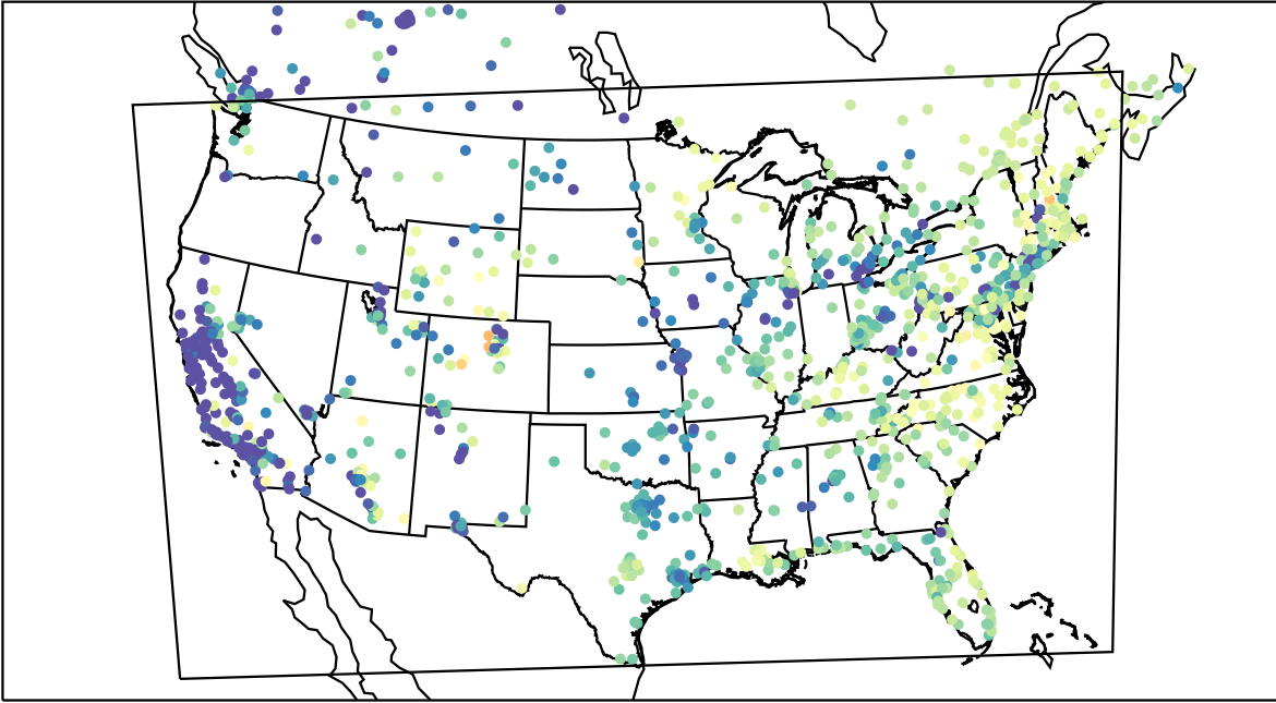
AirNOW (2022-03-15_15:00:00)
