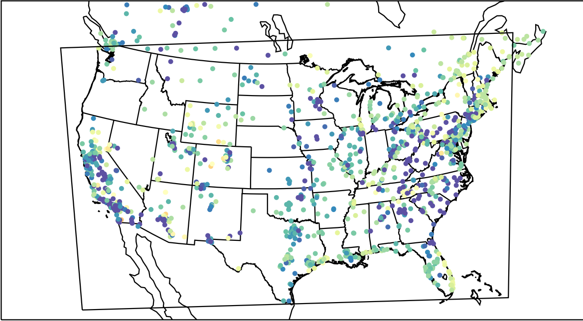
AirNOW (2022-03-15_07:00:00)
