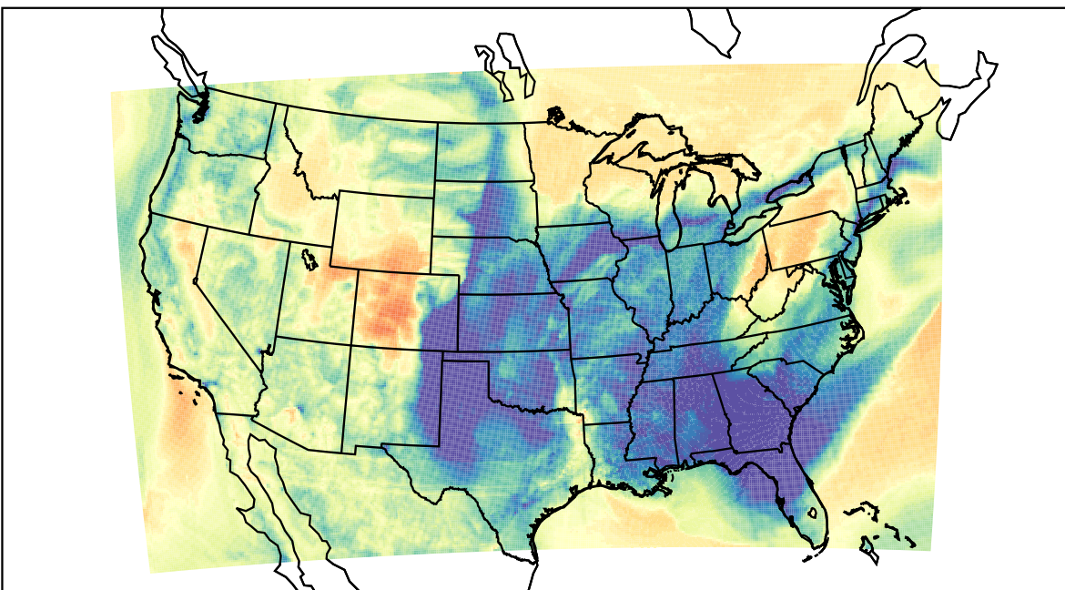
WRF (2022-03-15_06:00:00)
