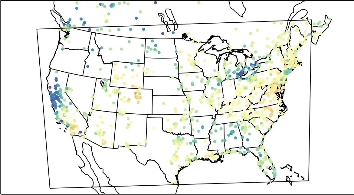
AirNOW (2022-03-15_18:00:00)
