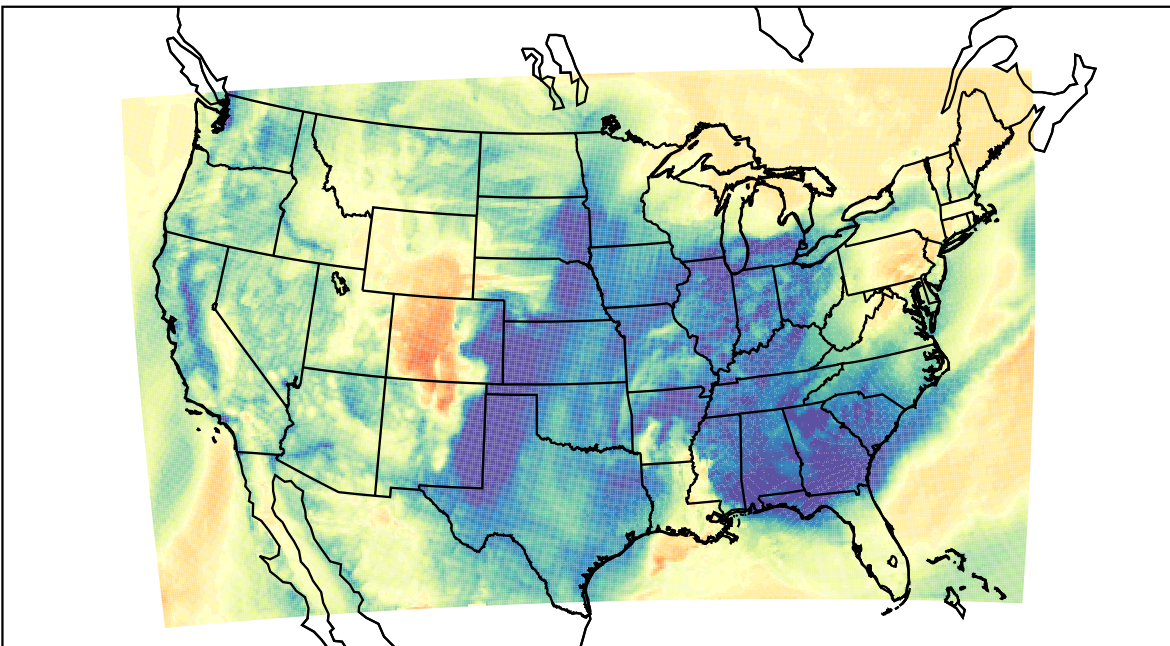
WRF (2022-03-15_16:00:00)
