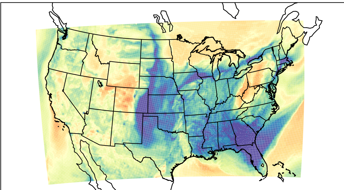
WRF (2022-03-15_03:00:00)
