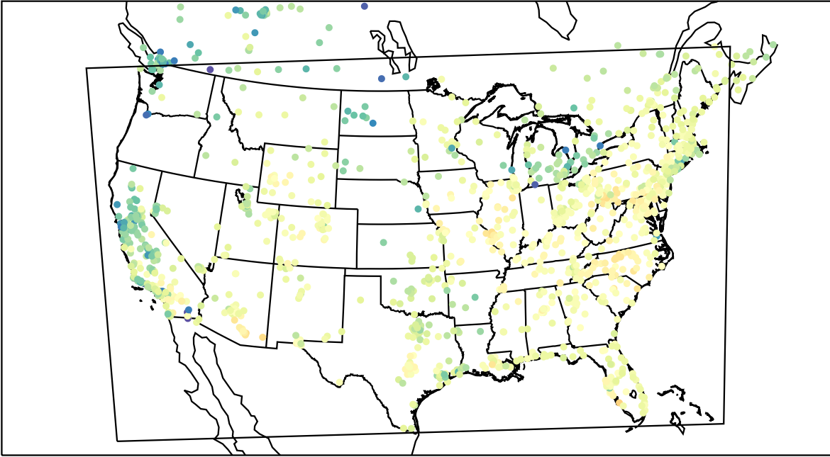
AirNOW (2022-03-14_18:00:00)
