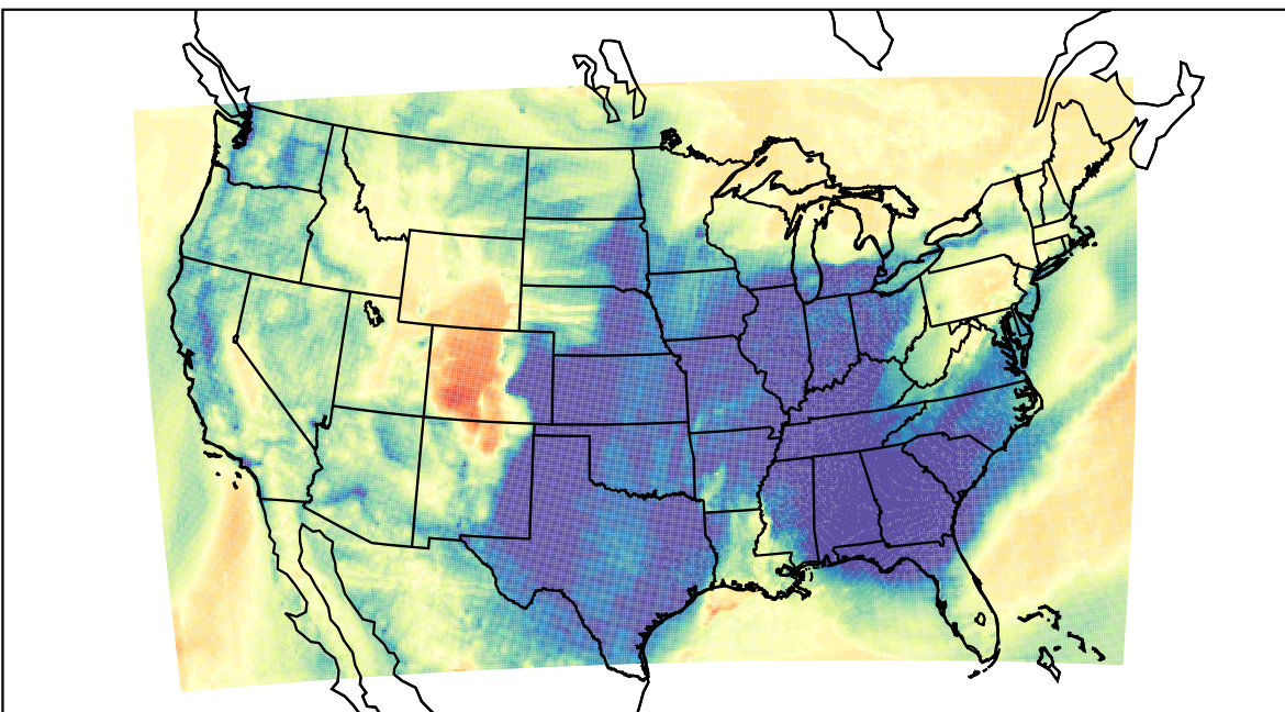
WRF (2022-03-15_14:00:00)
