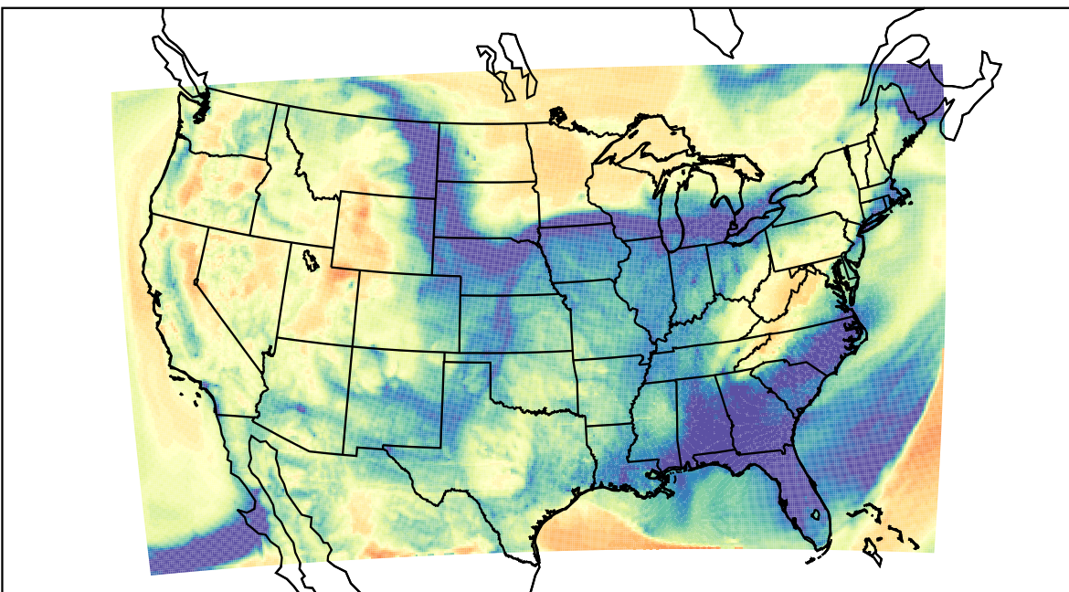
WRF (2022-03-14_12:00:00)
