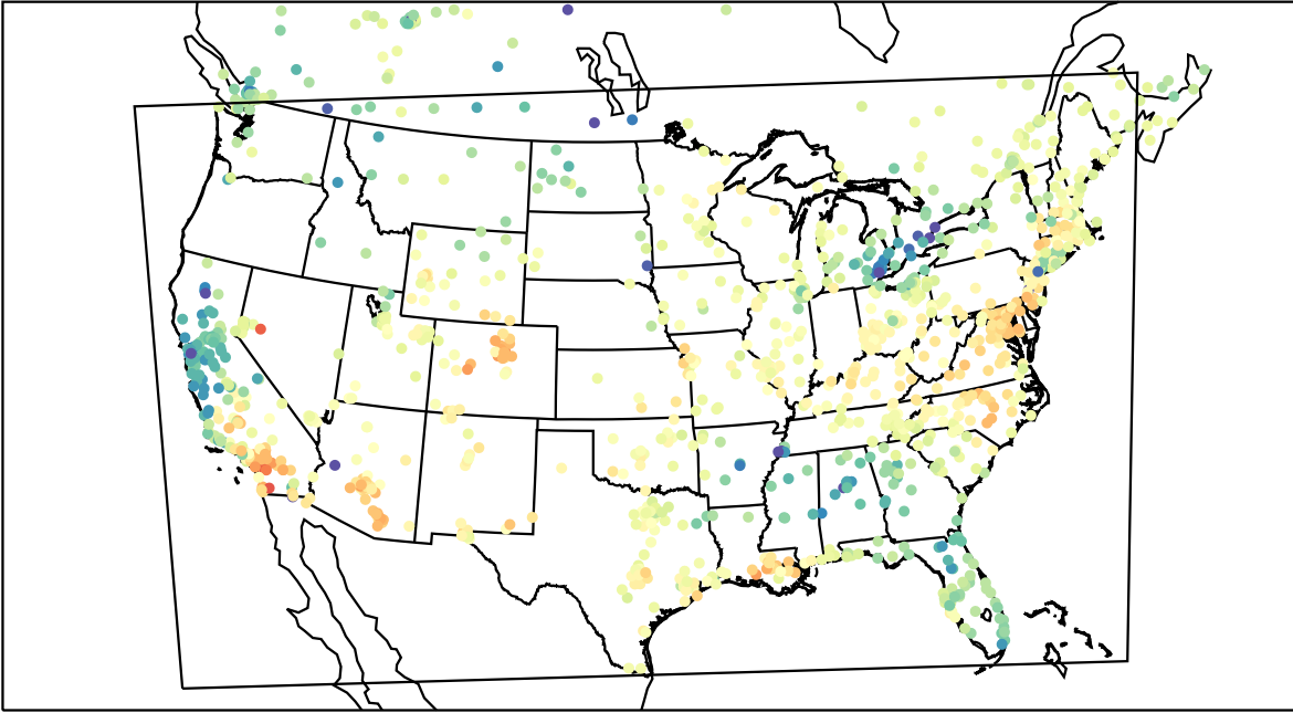
AirNOW (2022-03-15_20:00:00)
