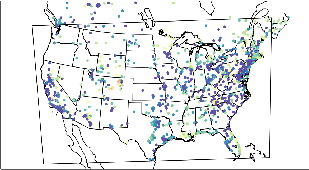
AirNOW (2022-03-15_11:00:00)
