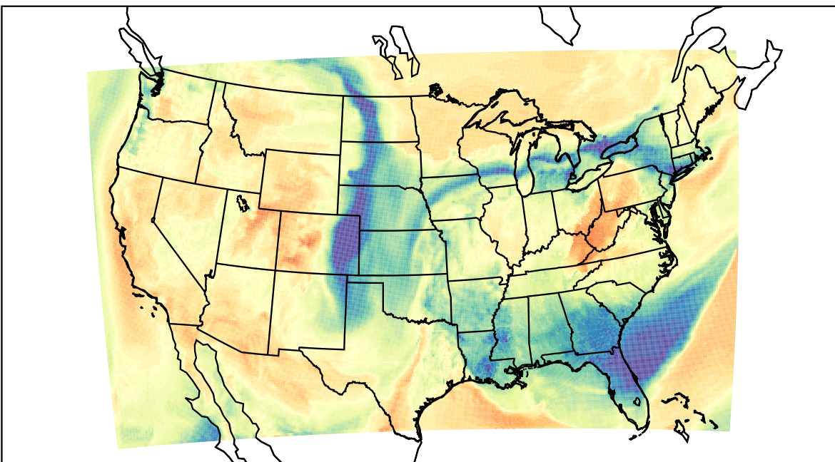
WRF (2022-03-14_22:00:00)
