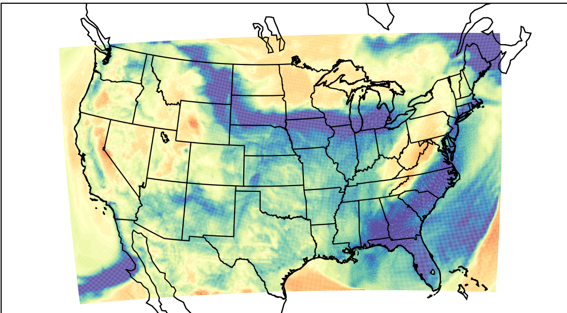
WRF (2022-03-14_08:00:00)
