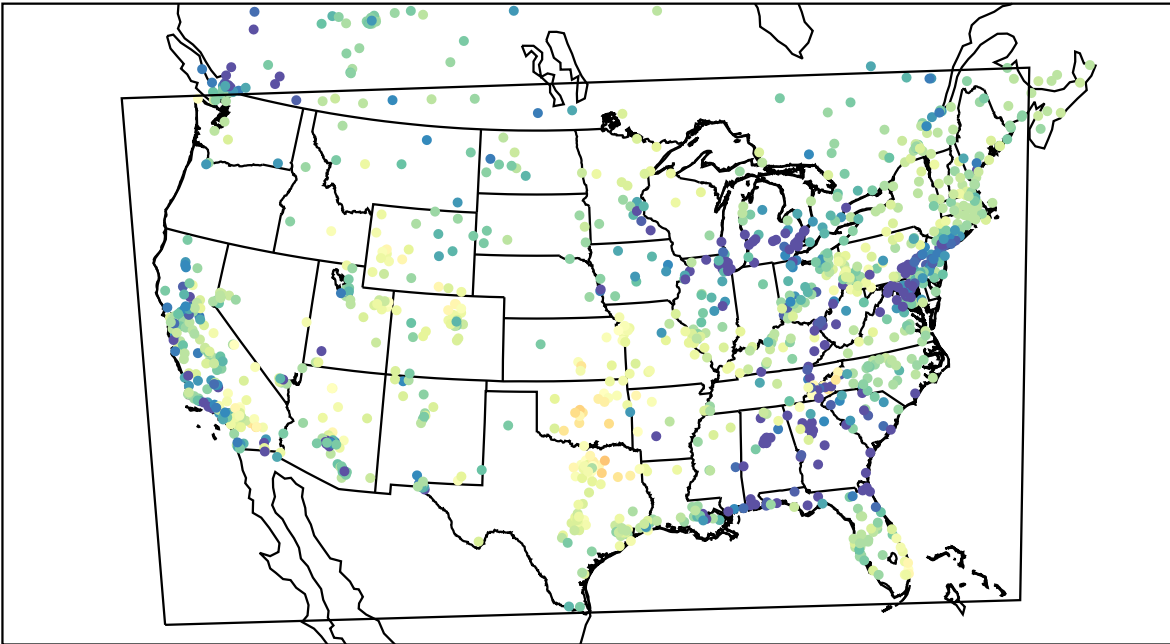
AirNOW (2022-03-14_04:00:00)
