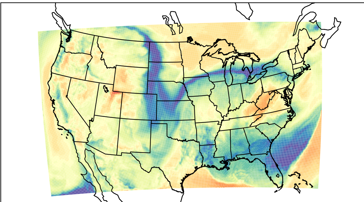
WRF (2022-03-14_17:00:00)
