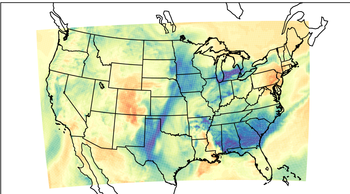
WRF (2022-03-15_19:00:00)
