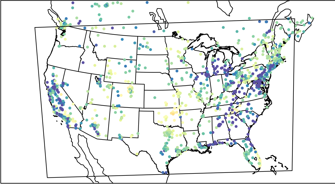
AirNOW (2022-03-14_08:00:00)
