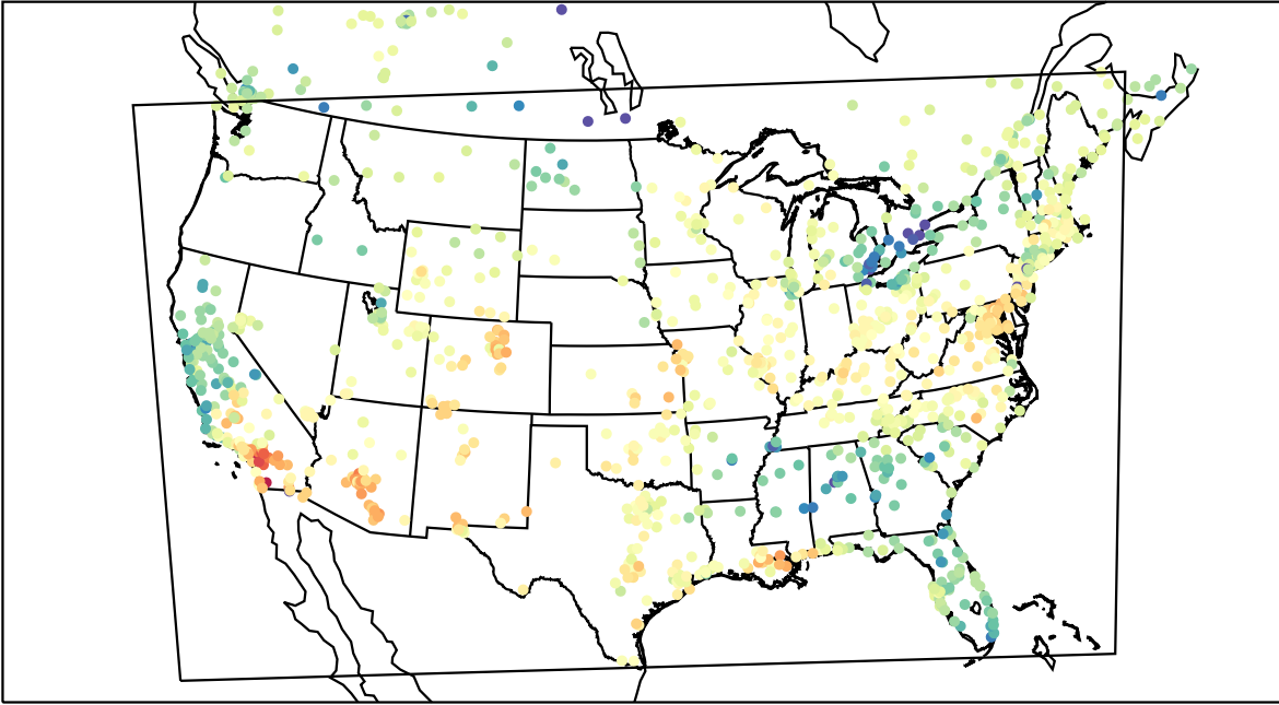
AirNOW (2022-03-15_22:00:00)
