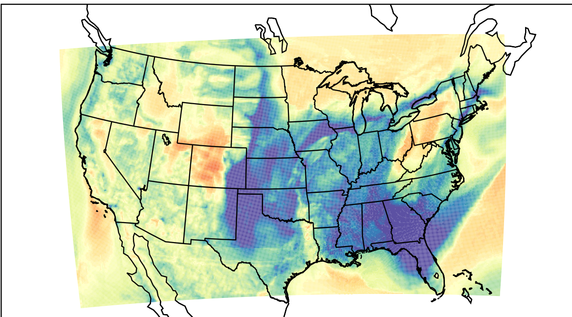
WRF (2022-03-15_05:00:00)
