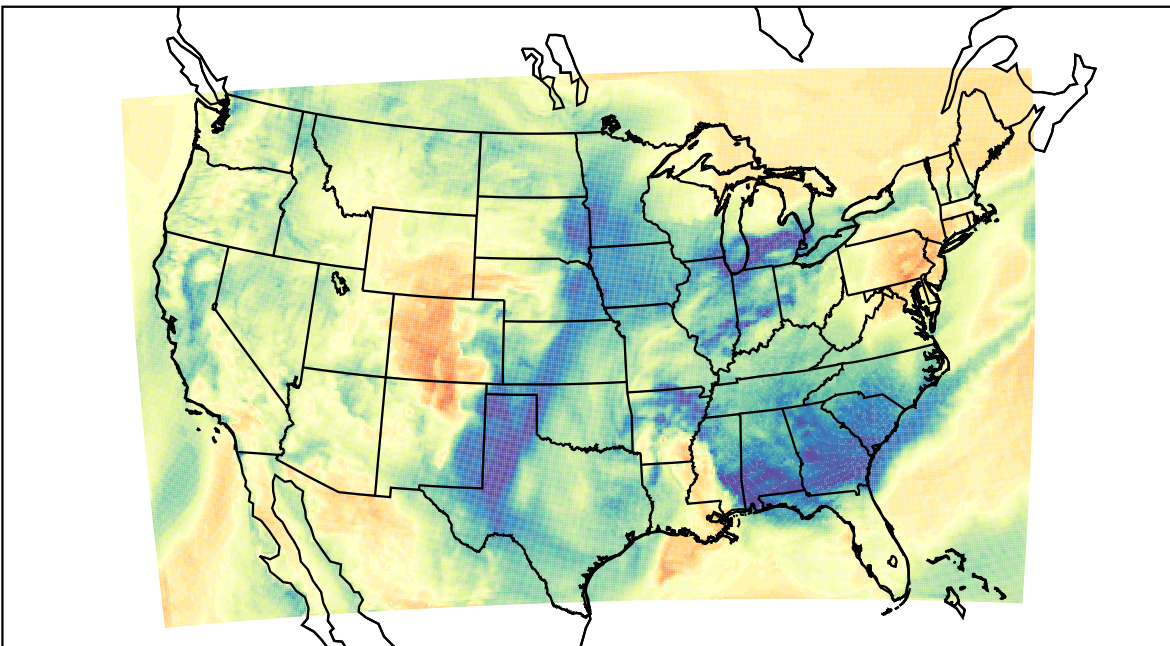
WRF (2022-03-15_18:00:00)
