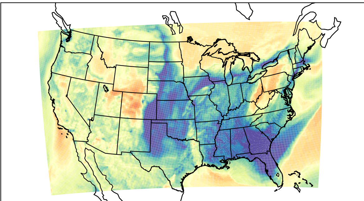
WRF (2022-03-15_04:00:00)
