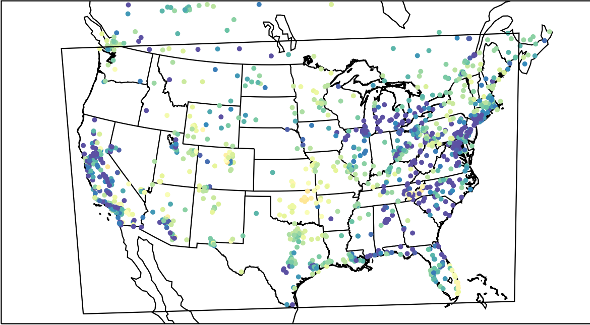
AirNOW (2022-03-14_09:00:00)
