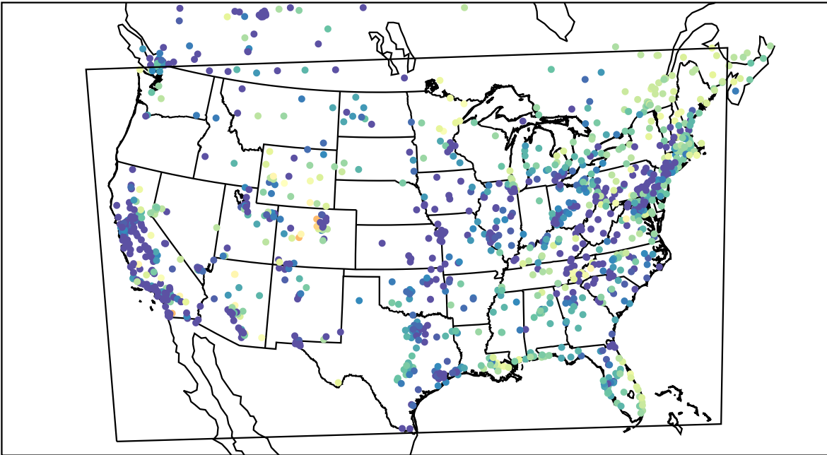
AirNOW (2022-03-15_13:00:00)
