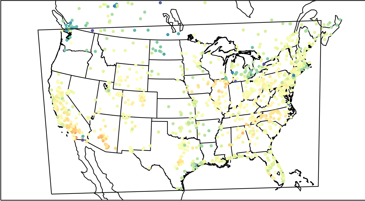
AirNOW (2022-03-14_22:00:00)
