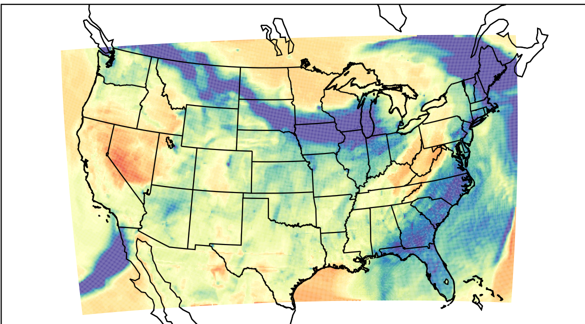
WRF (2022-03-14_01:00:00)
