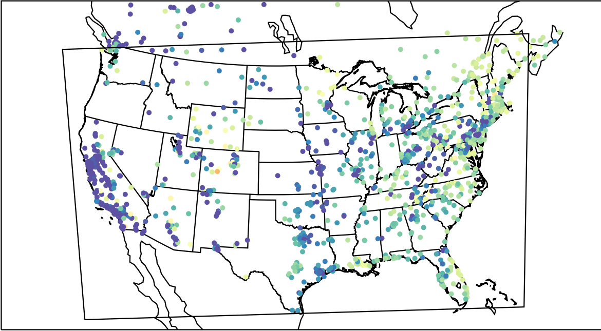
AirNOW (2022-03-15_14:00:00)
