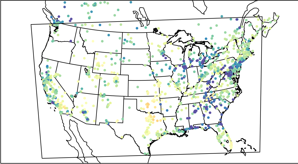
AirNOW (2022-03-14_03:00:00)
