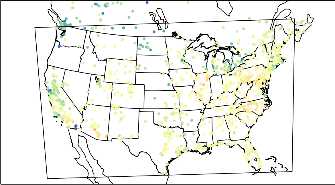
AirNOW (2022-03-14_19:00:00)
