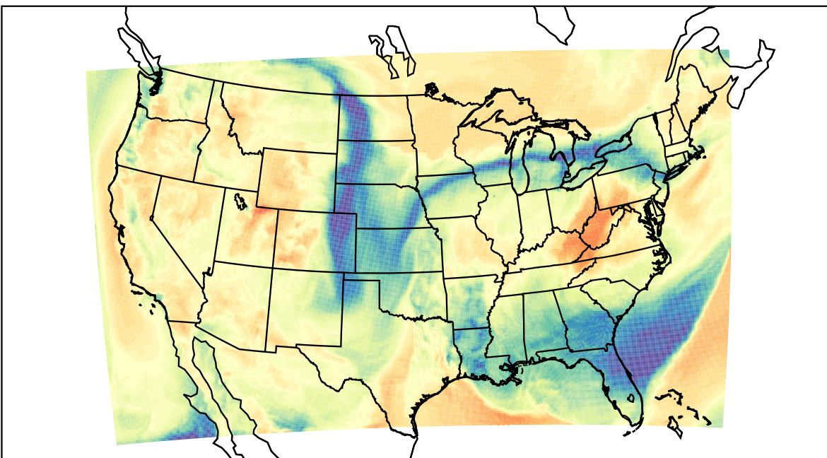
WRF (2022-03-14_19:00:00)
