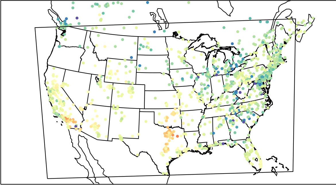
AirNOW (2022-03-14_00:00:00)
