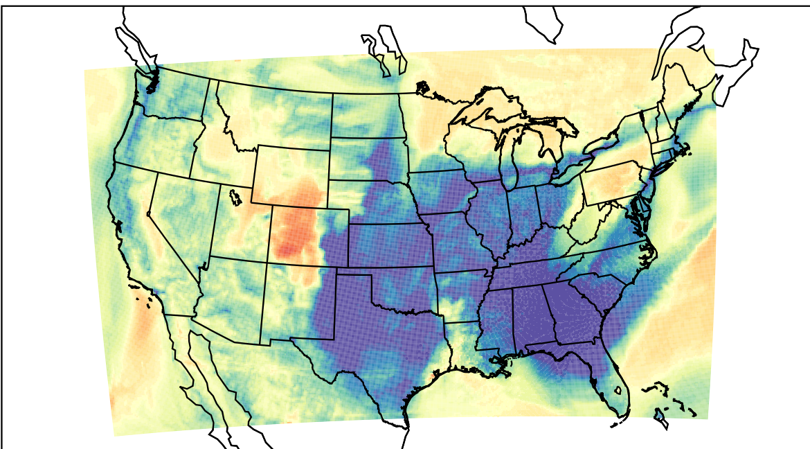
WRF (2022-03-15_10:00:00)
