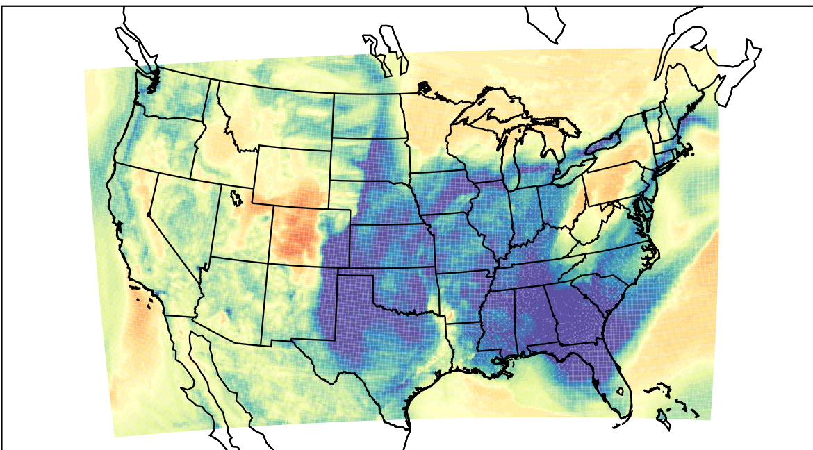
WRF (2022-03-15_07:00:00)
