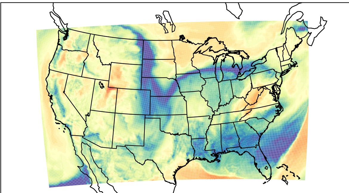
WRF (2022-03-14_16:00:00)
