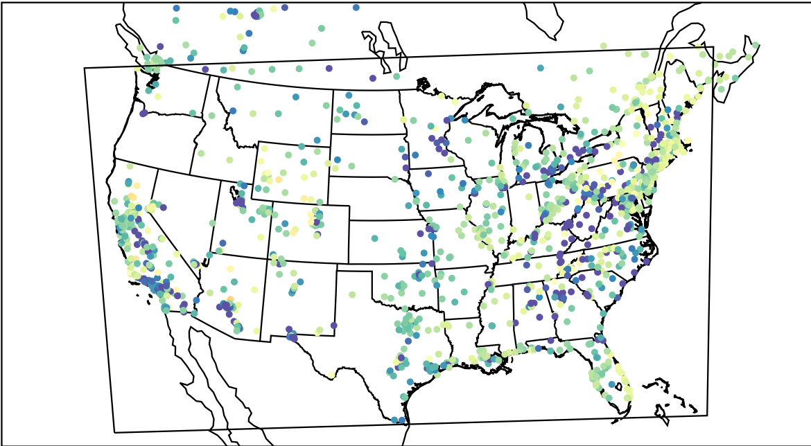
AirNOW (2022-03-15_04:00:00)
