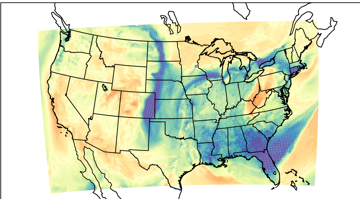
WRF (2022-03-15_00:00:00)
