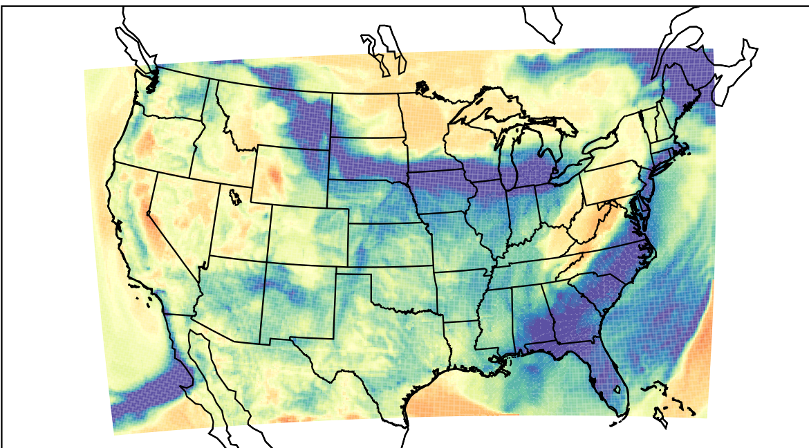
WRF (2022-03-14_07:00:00)
