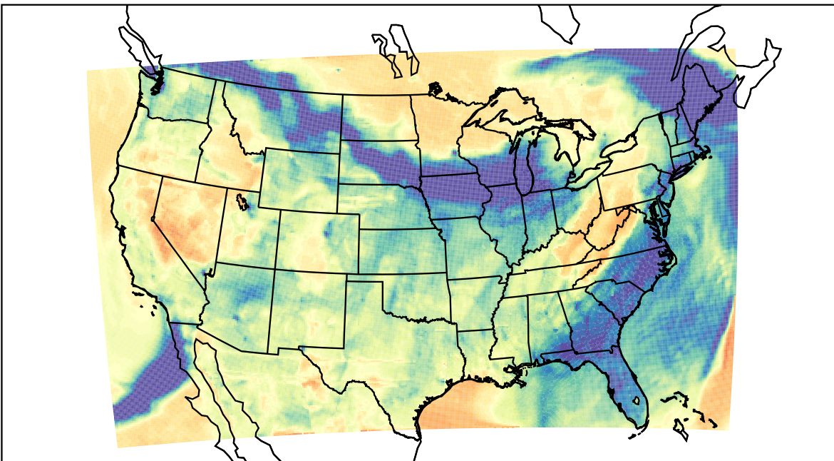
WRF (2022-03-14_02:00:00)
