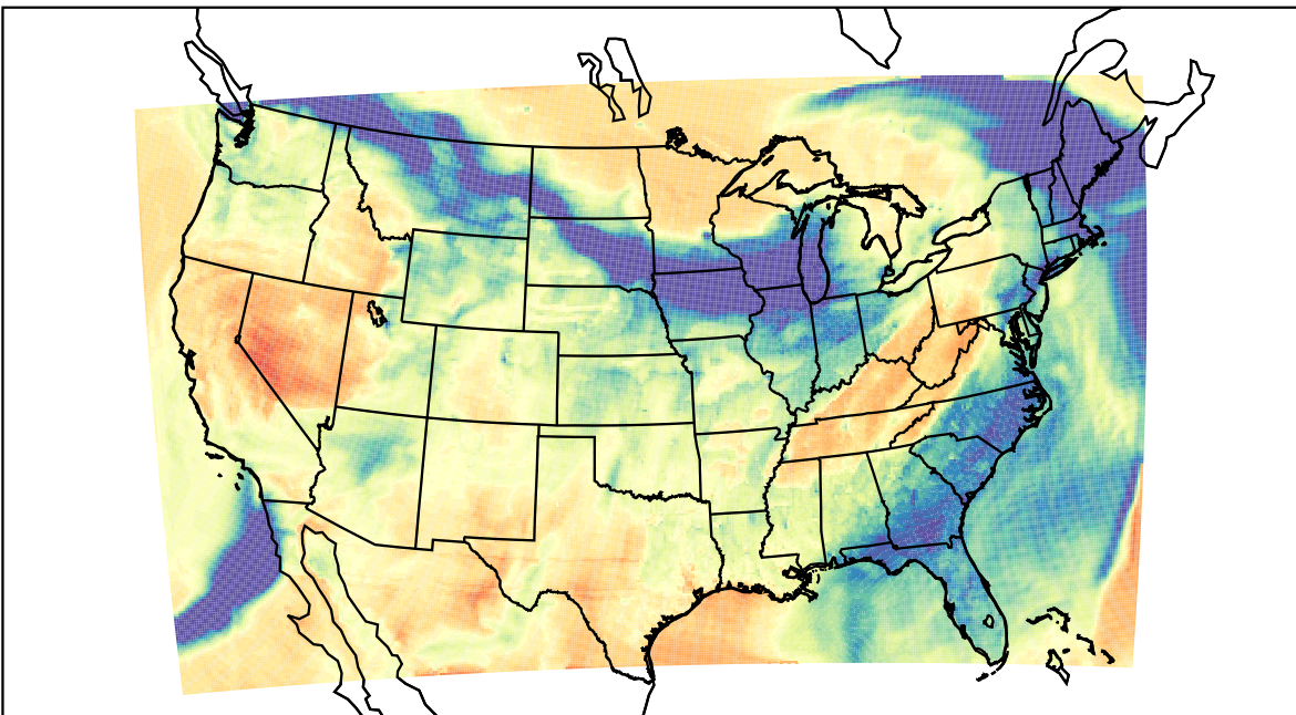
WRF (2022-03-14_00:00:00)
