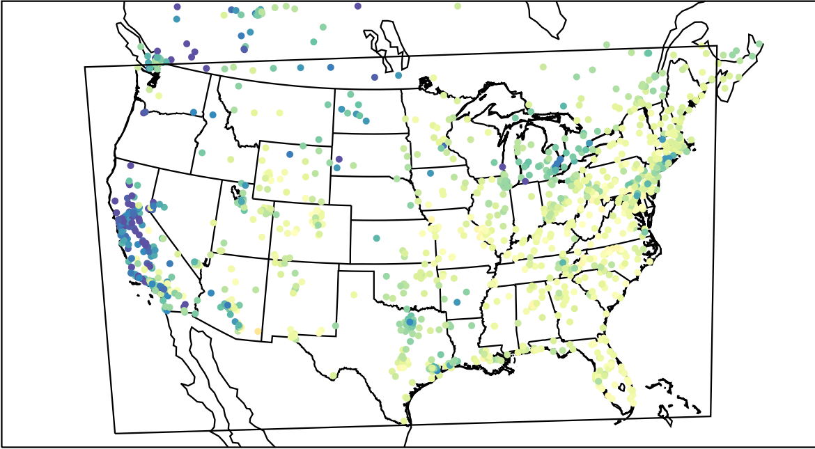
AirNOW (2022-03-14_16:00:00)
