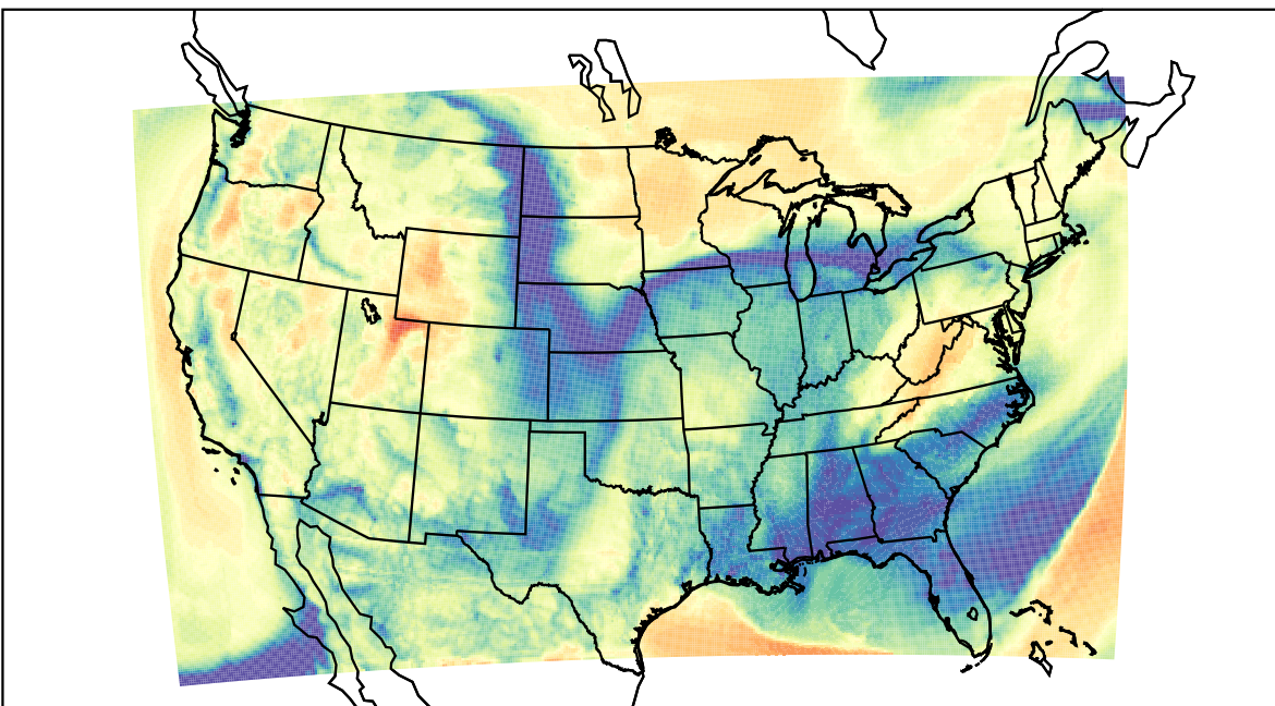
WRF (2022-03-14_15:00:00)
