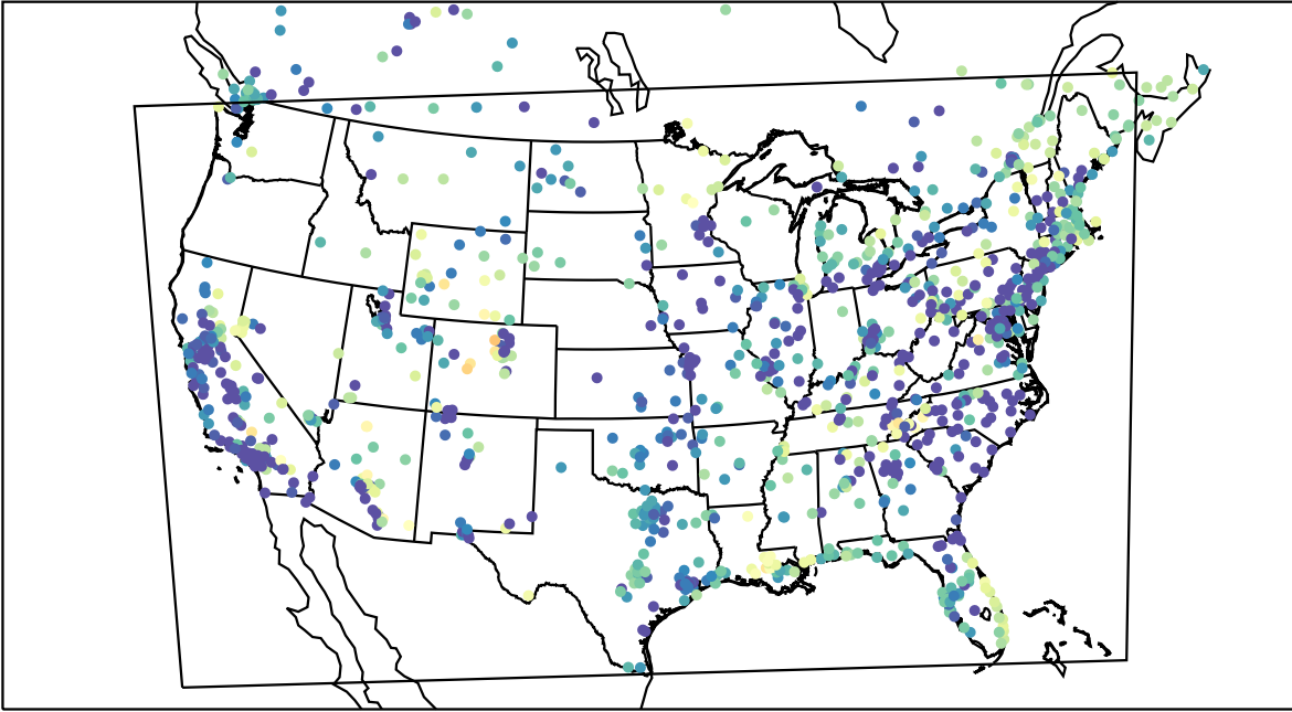
AirNOW (2022-03-15_10:00:00)
