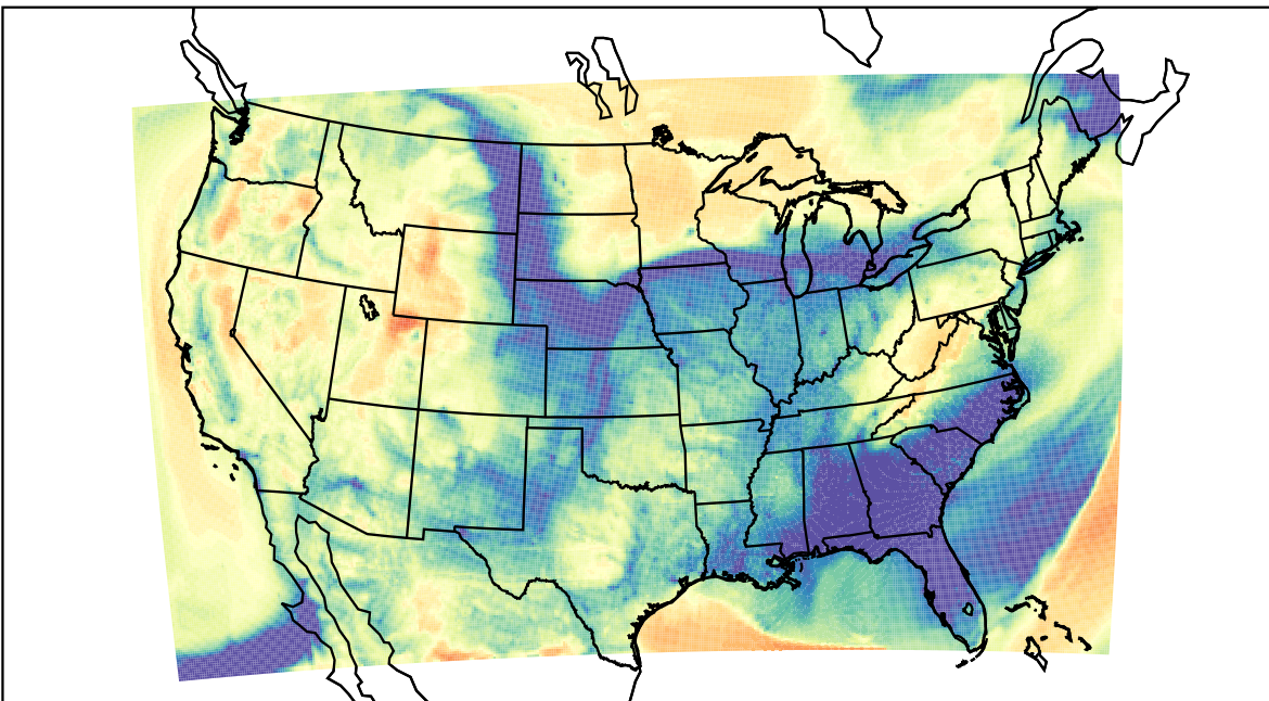
WRF (2022-03-14_13:00:00)
