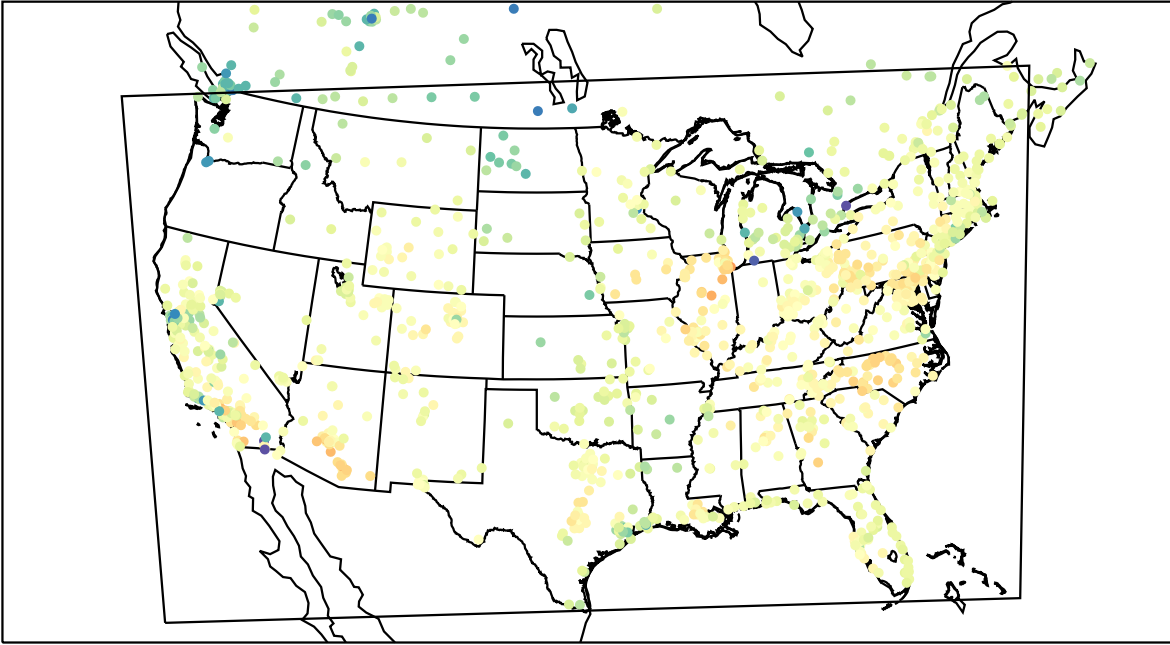
AirNOW (2022-03-14_20:00:00)
