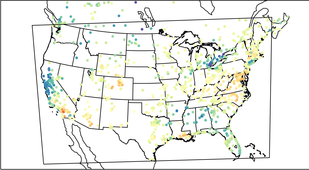
AirNOW (2022-03-15_19:00:00)
