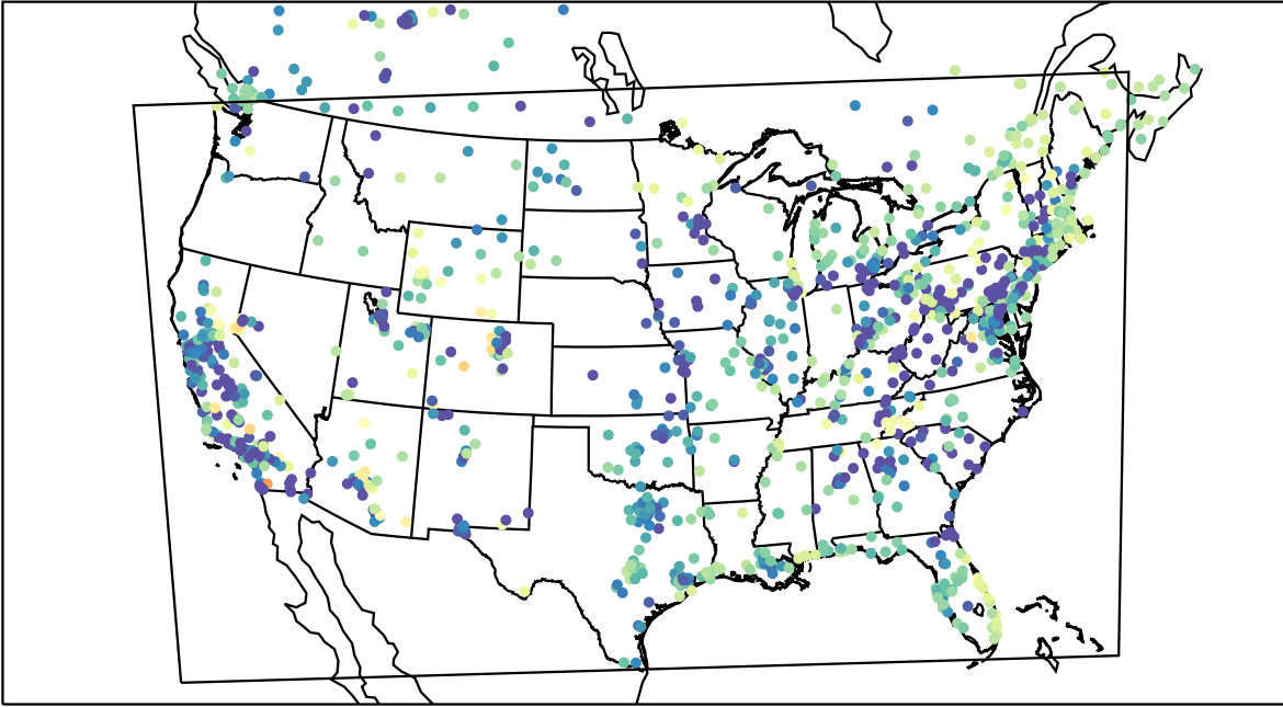
AirNOW (2022-03-15_08:00:00)
