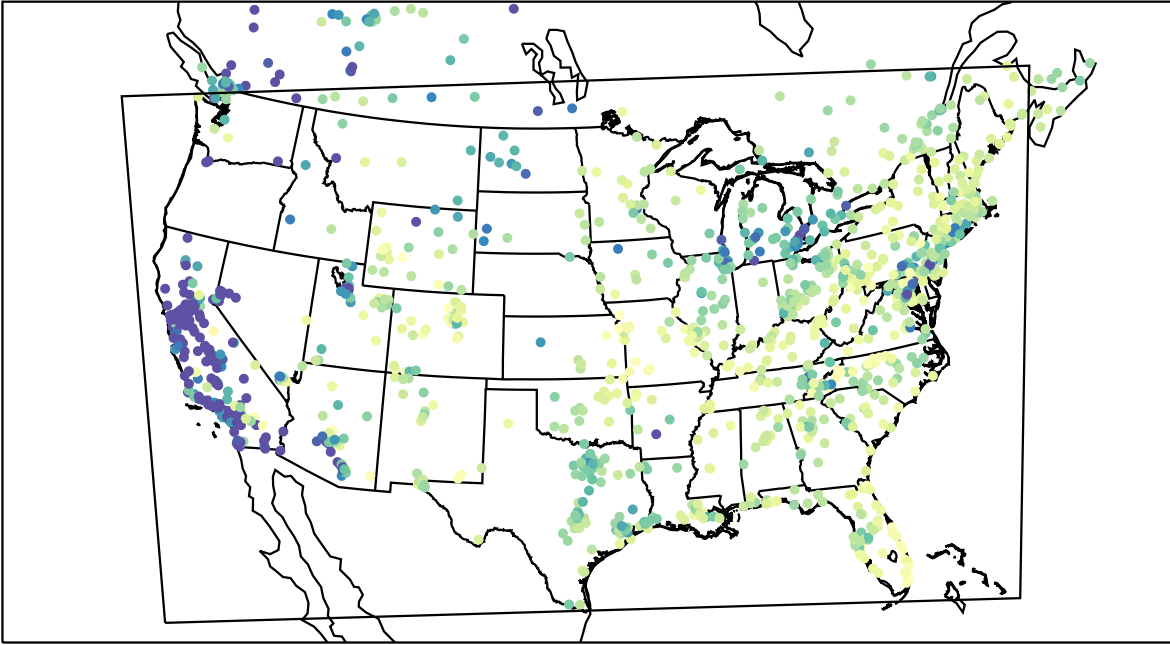
AirNOW (2022-03-14_15:00:00)
