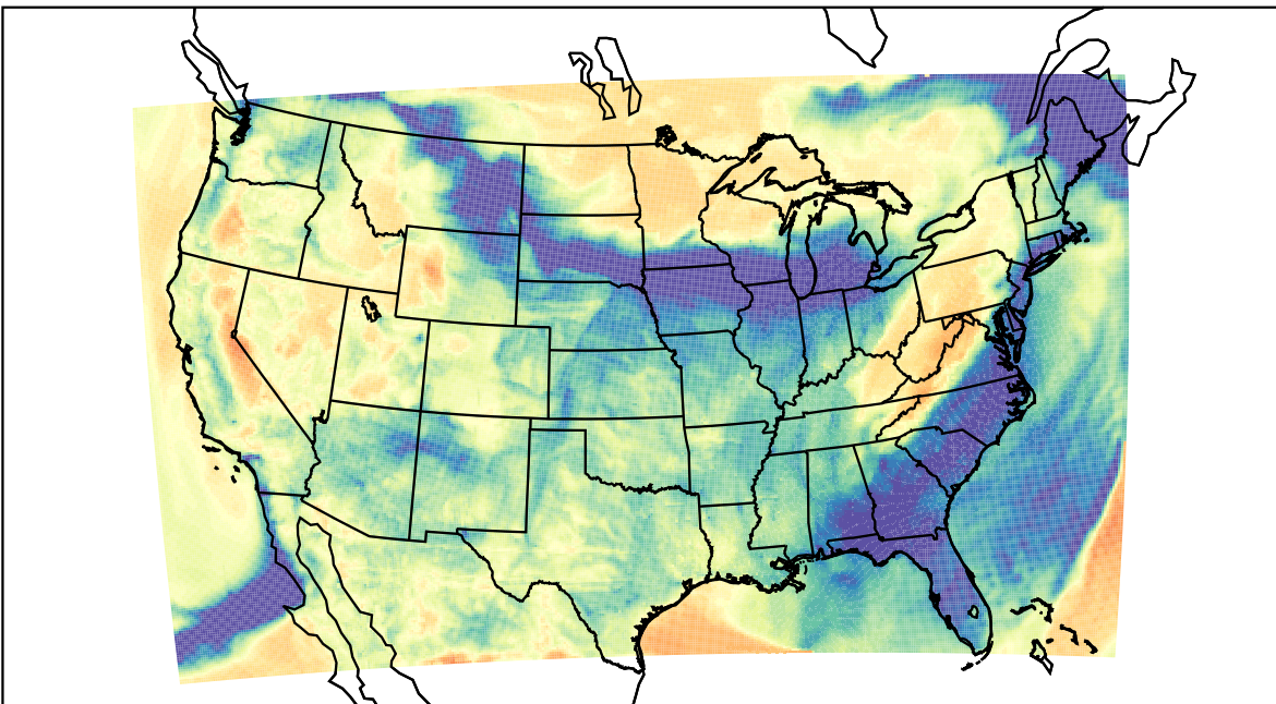
WRF (2022-03-14_06:00:00)
