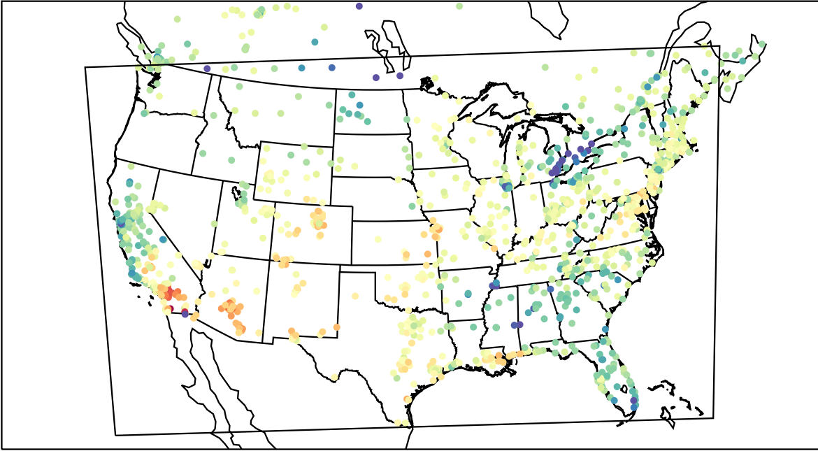
AirNOW (2022-03-15_23:00:00)
