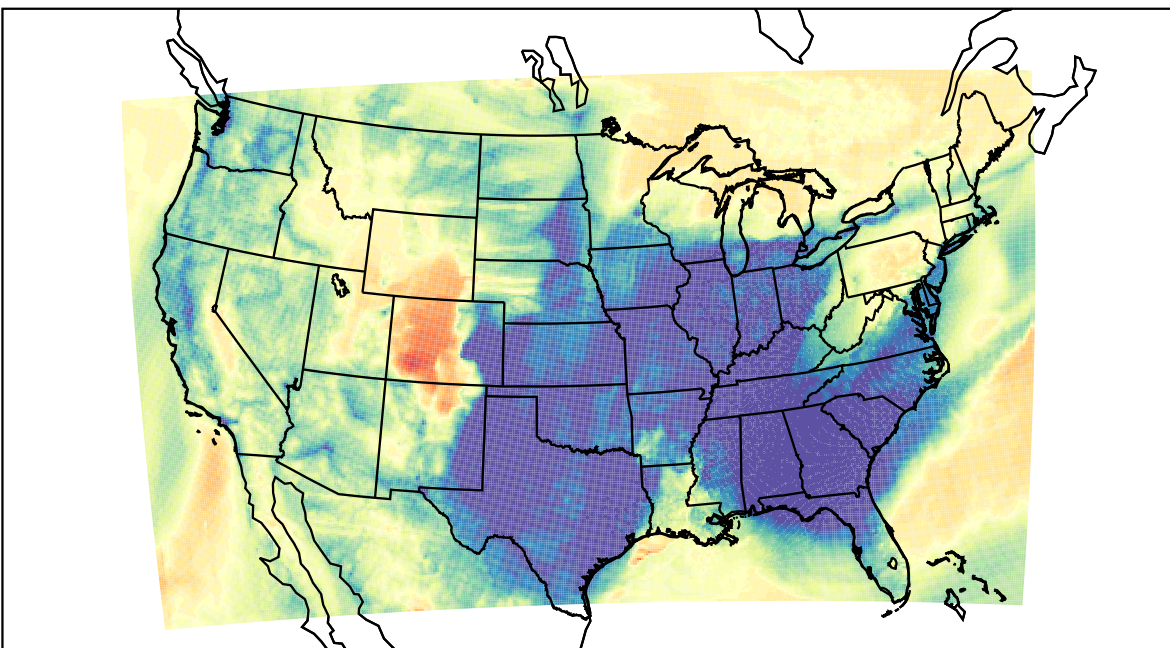
WRF (2022-03-15_13:00:00)
