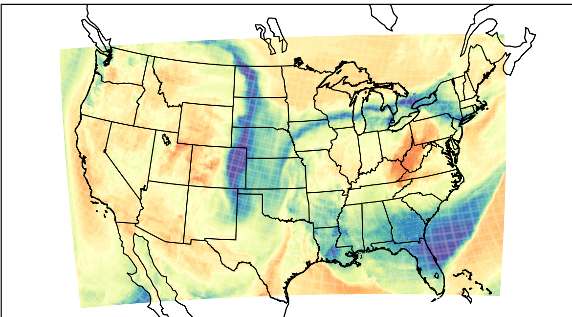
WRF (2022-03-14_21:00:00)
