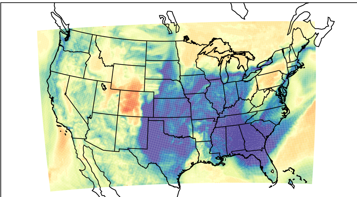
WRF (2022-03-15_09:00:00)
