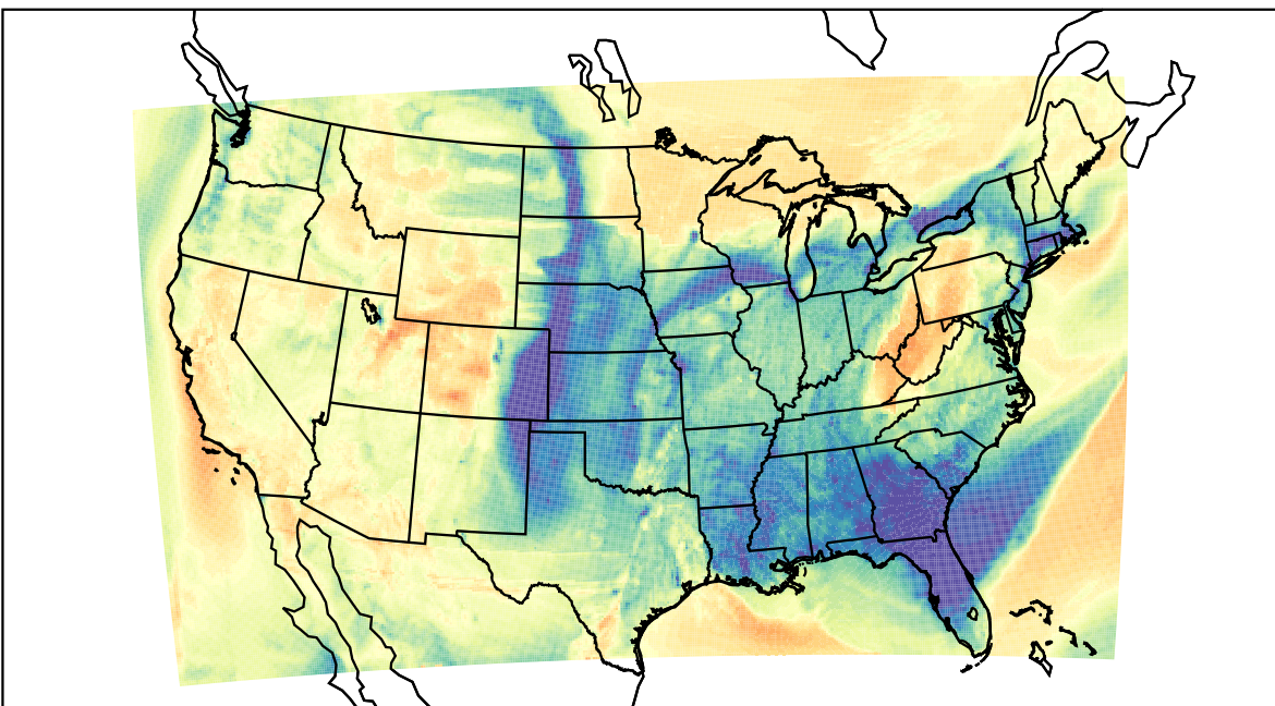
WRF (2022-03-15_01:00:00)
