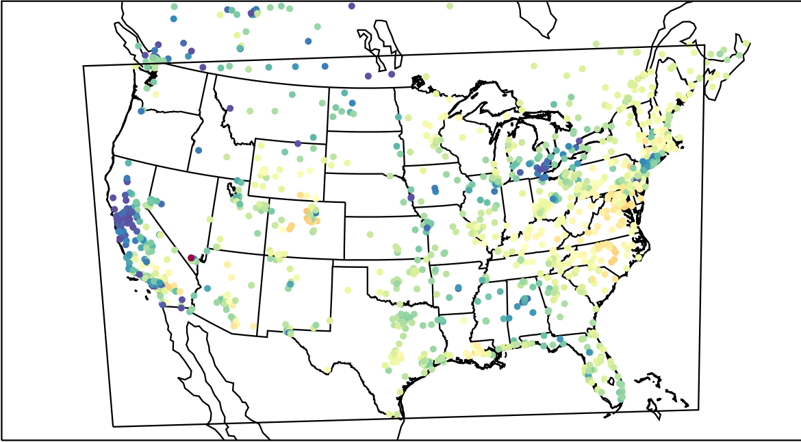
AirNOW (2022-03-15_17:00:00)
