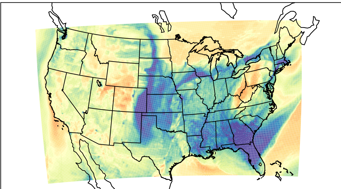
WRF (2022-03-15_02:00:00)
