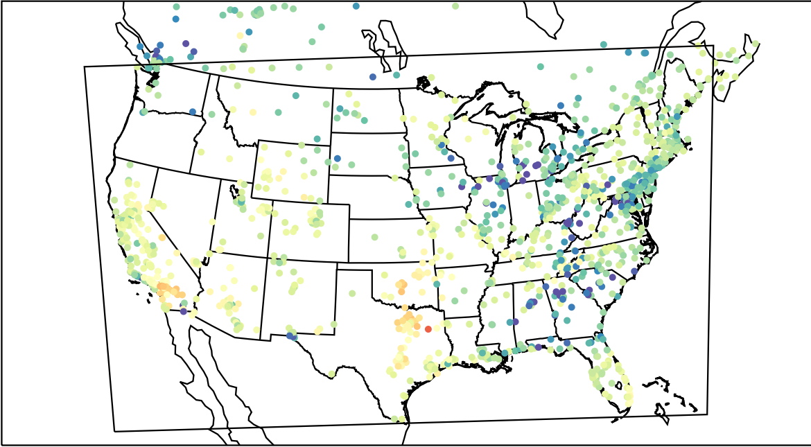
AirNOW (2022-03-14_01:00:00)
