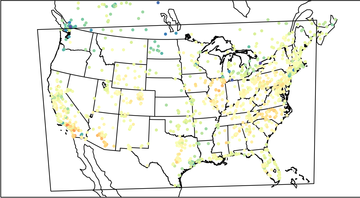
AirNOW (2022-03-14_21:00:00)
