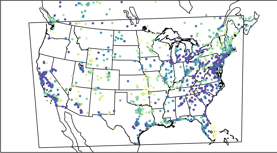
AirNOW (2022-03-14_12:00:00)
