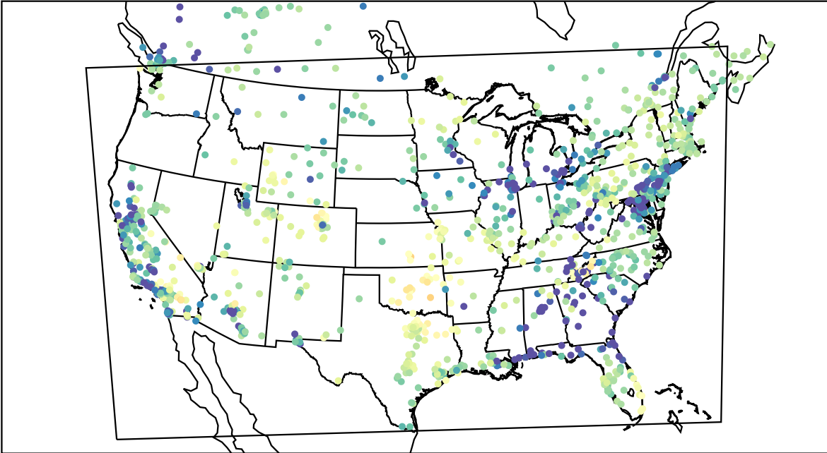
AirNOW (2022-03-14_05:00:00)
