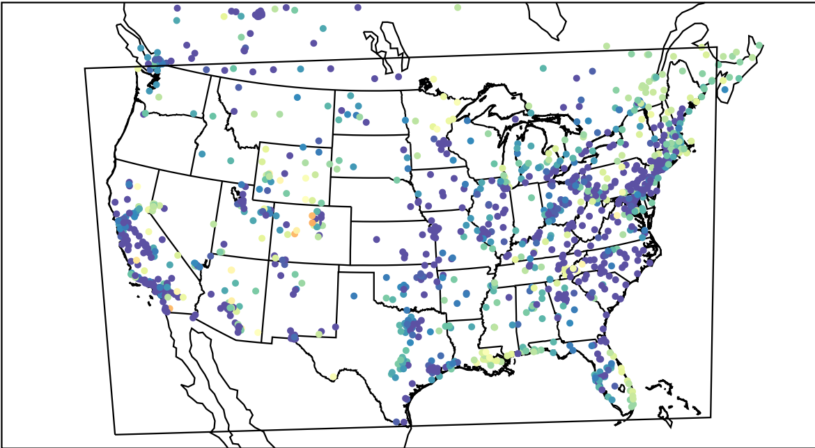
AirNOW (2022-03-15_12:00:00)
