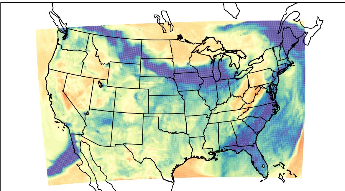
WRF (2022-03-14_03:00:00)
