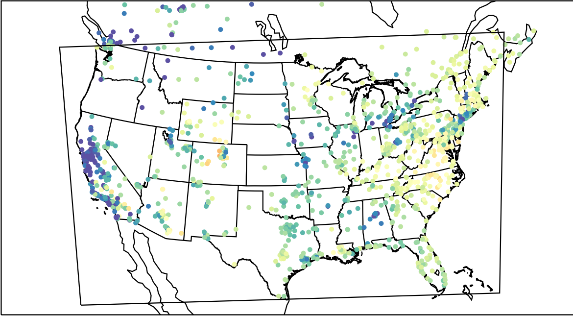
AirNOW (2022-03-15_16:00:00)
