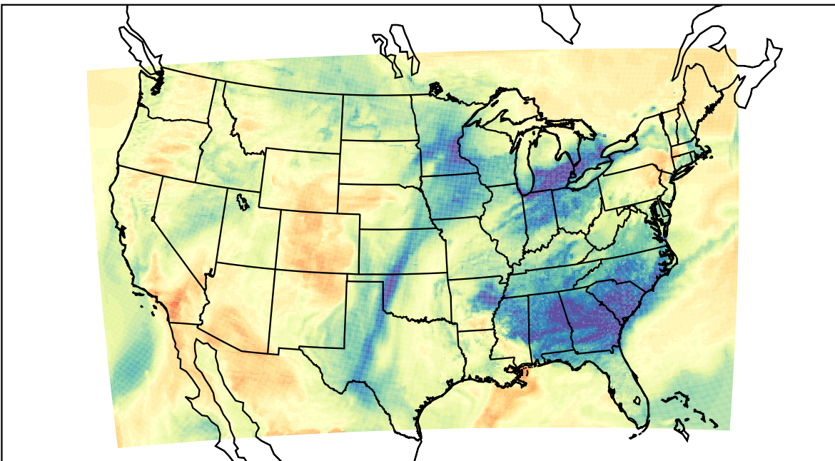
WRF (2022-03-15_23:00:00)
