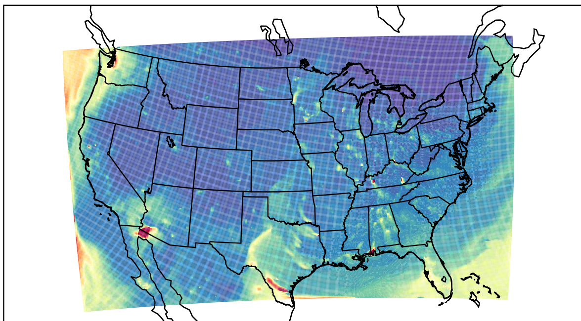
WRF 2022-04-02_03:00:00
