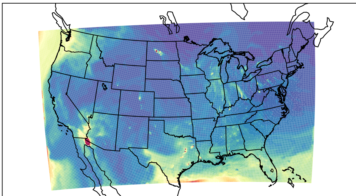
WRF 2022-04-02_17:00:00
