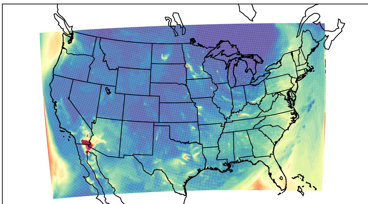
WRF 2022-04-01_09:00:00
