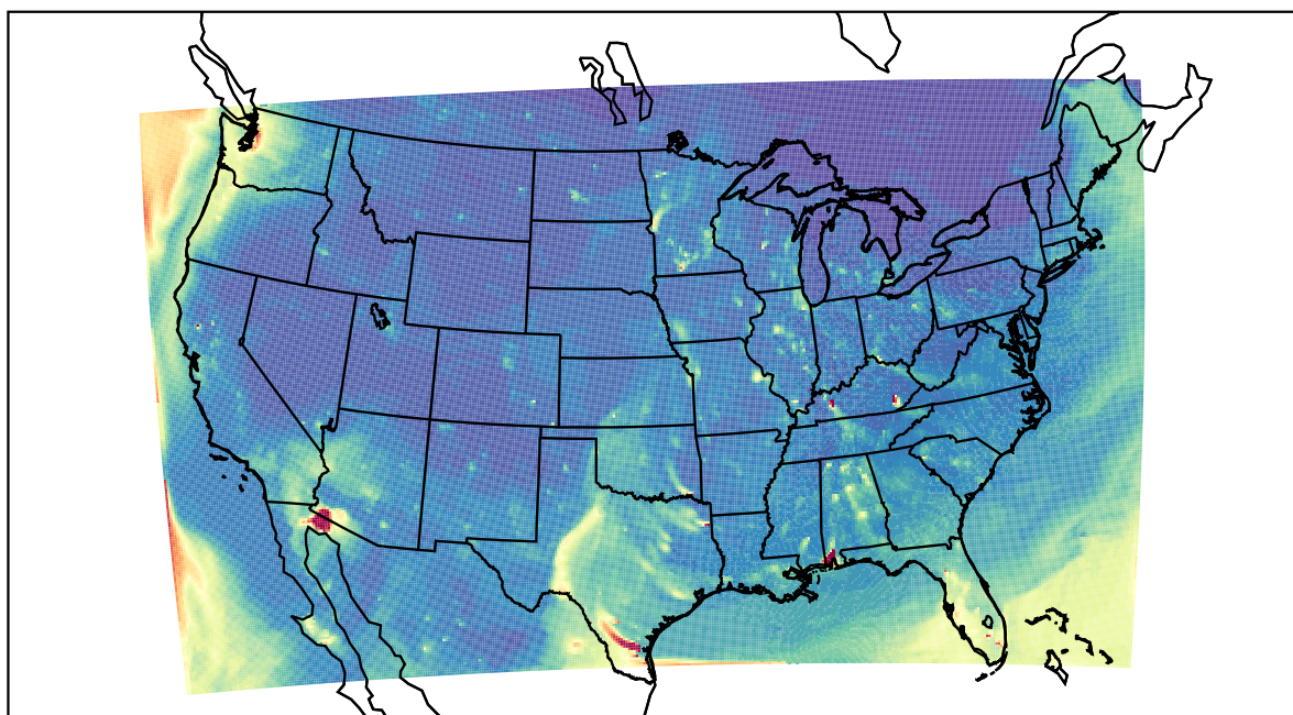
WRF 2022-04-02_02:00:00
