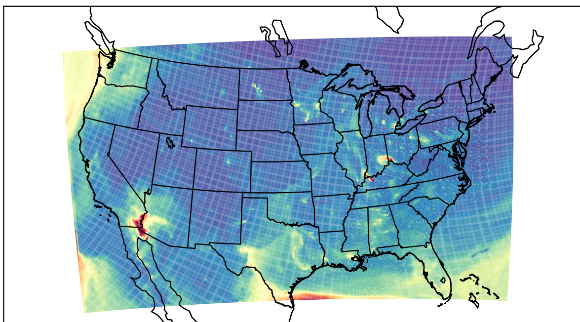
WRF 2022-04-02_11:00:00
