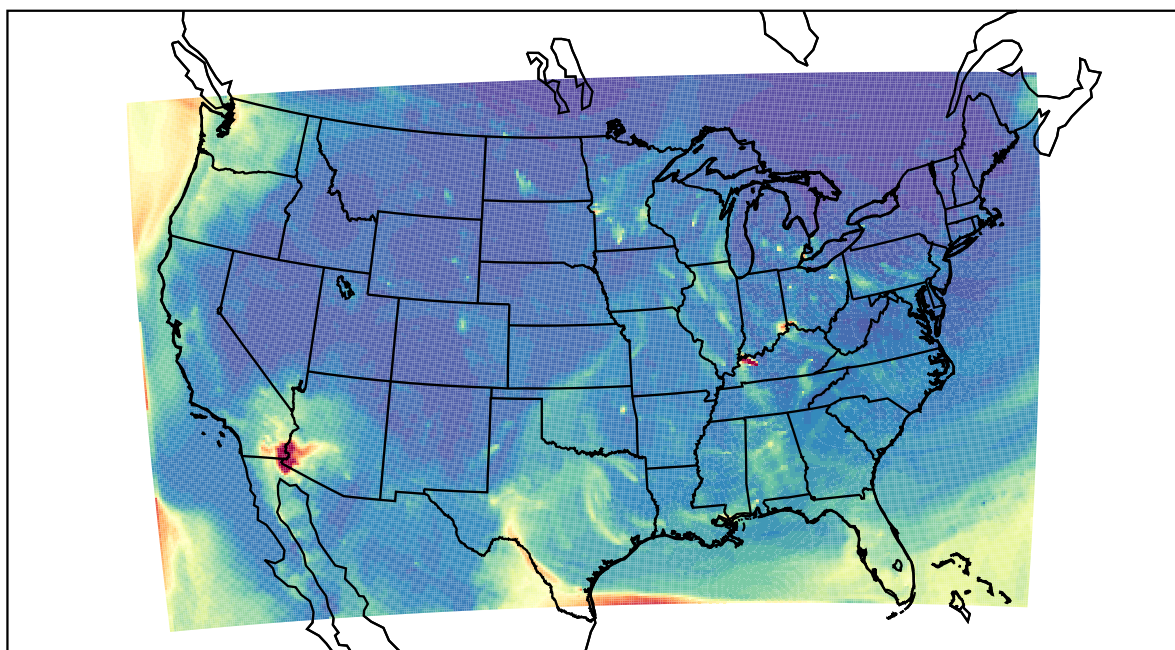
WRF 2022-04-02_08:00:00
