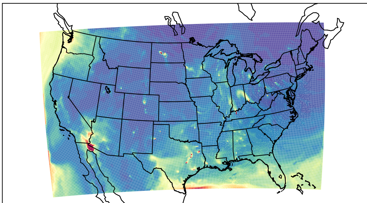
WRF 2022-04-02_15:00:00
