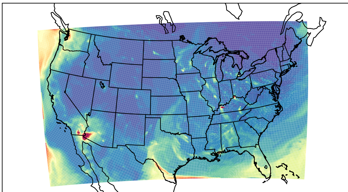
WRF 2022-04-02_06:00:00
