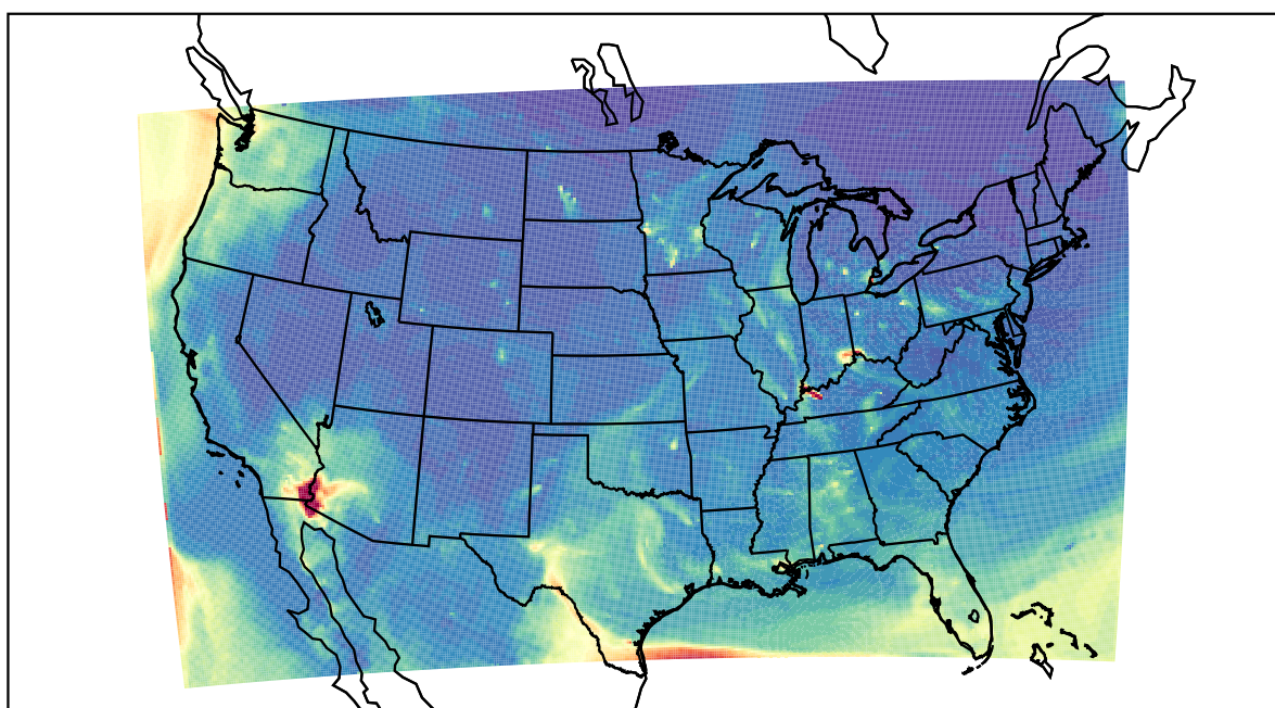
WRF 2022-04-02_09:00:00
