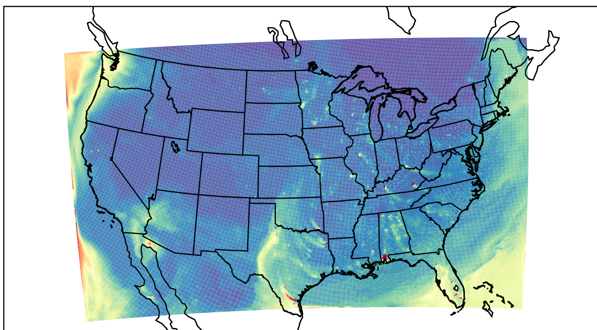
WRF 2022-04-02_00:00:00
