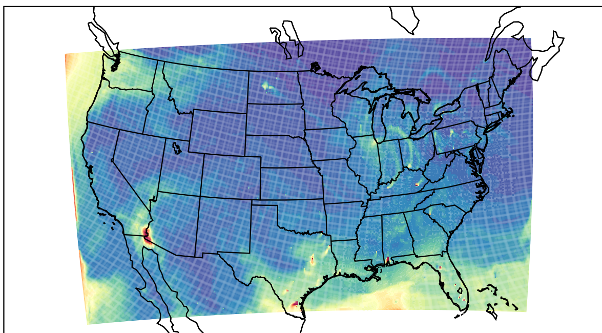
WRF 2022-04-02_22:00:00
