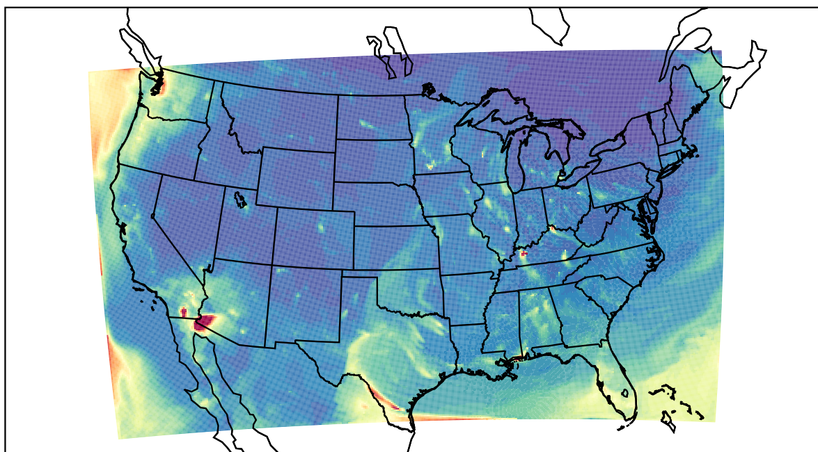
WRF 2022-04-02_05:00:00
