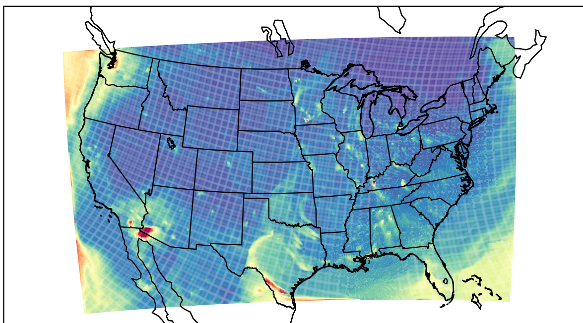
WRF 2022-04-02_04:00:00
