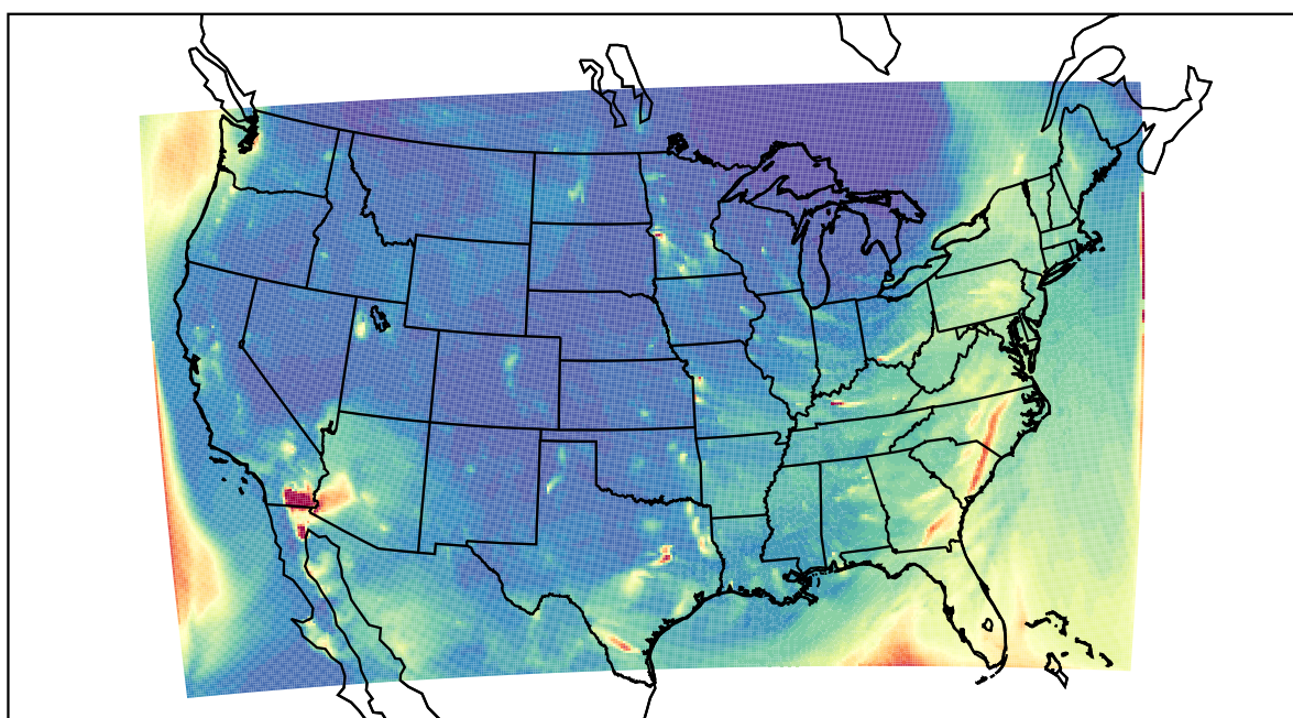
WRF 2022-04-01_05:00:00
