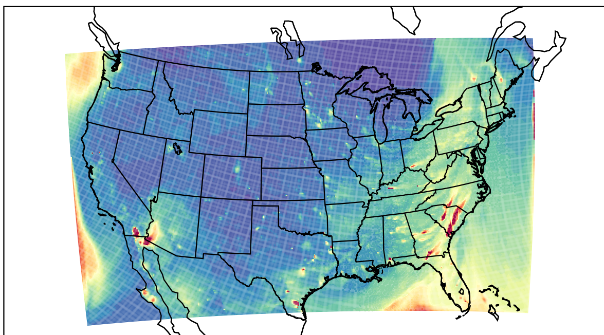
WRF 2022-04-01_02:00:00
