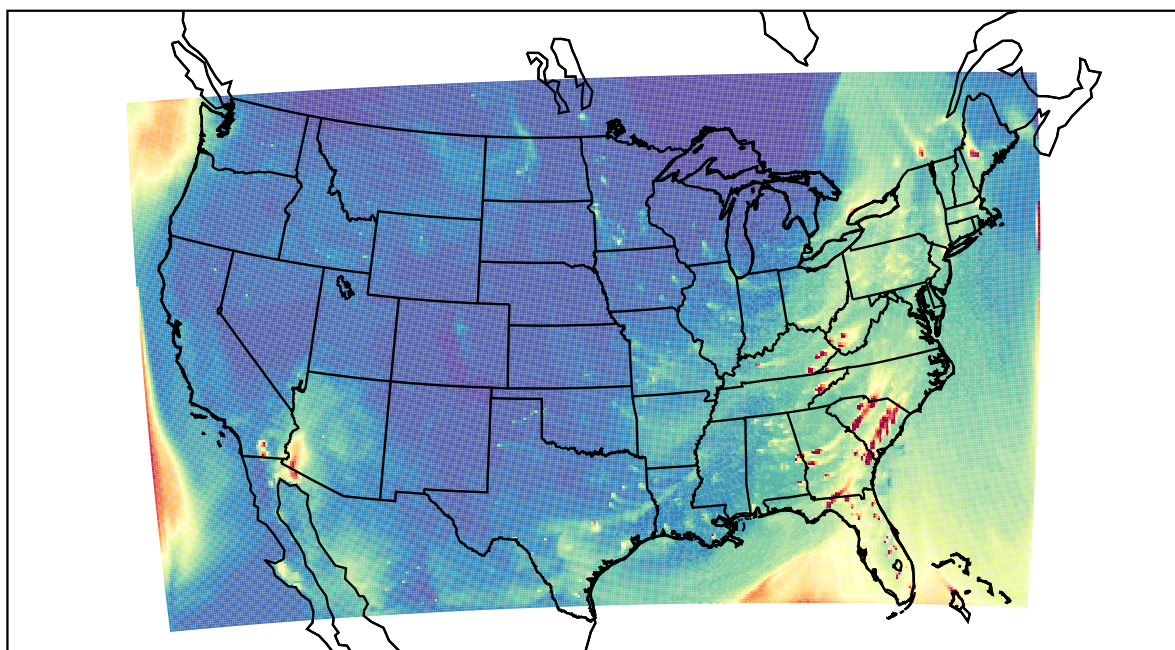
WRF 2022-04-01_00:00:00
