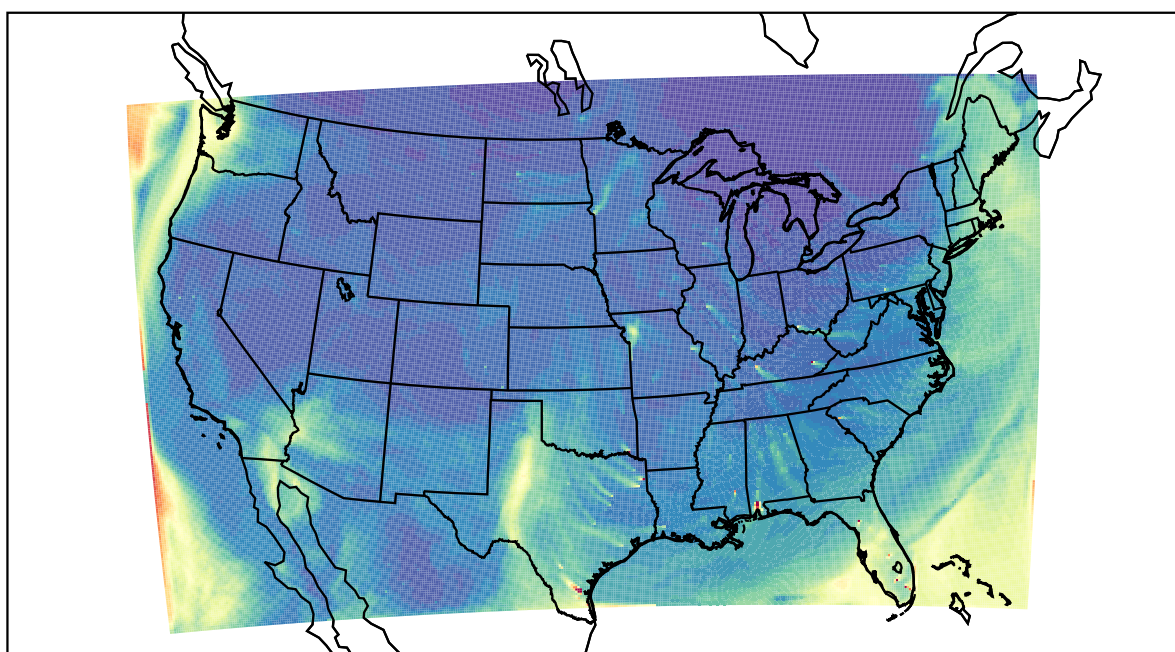
WRF 2022-04-01_21:00:00
