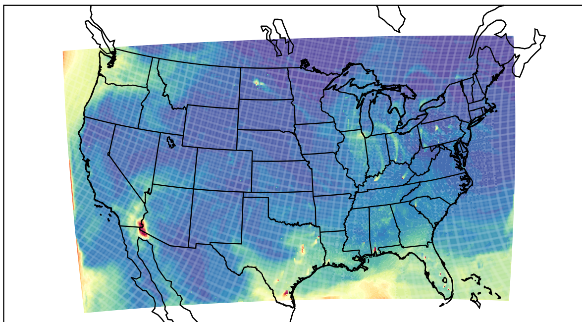
WRF 2022-04-02_21:00:00
