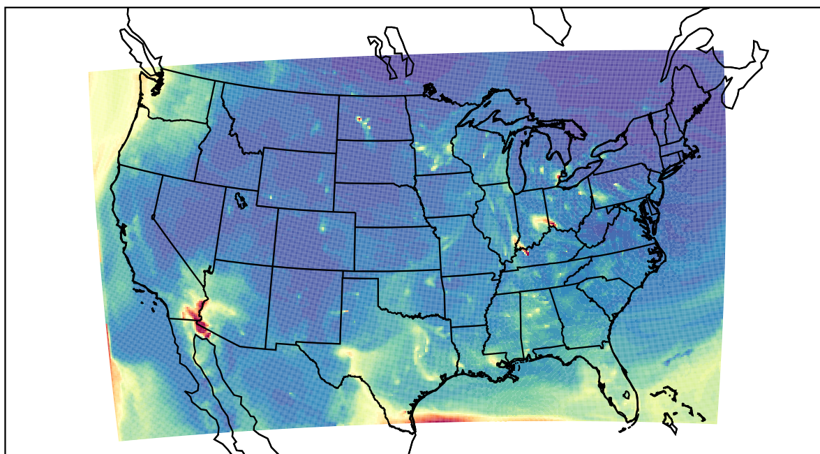
WRF 2022-04-02_12:00:00
