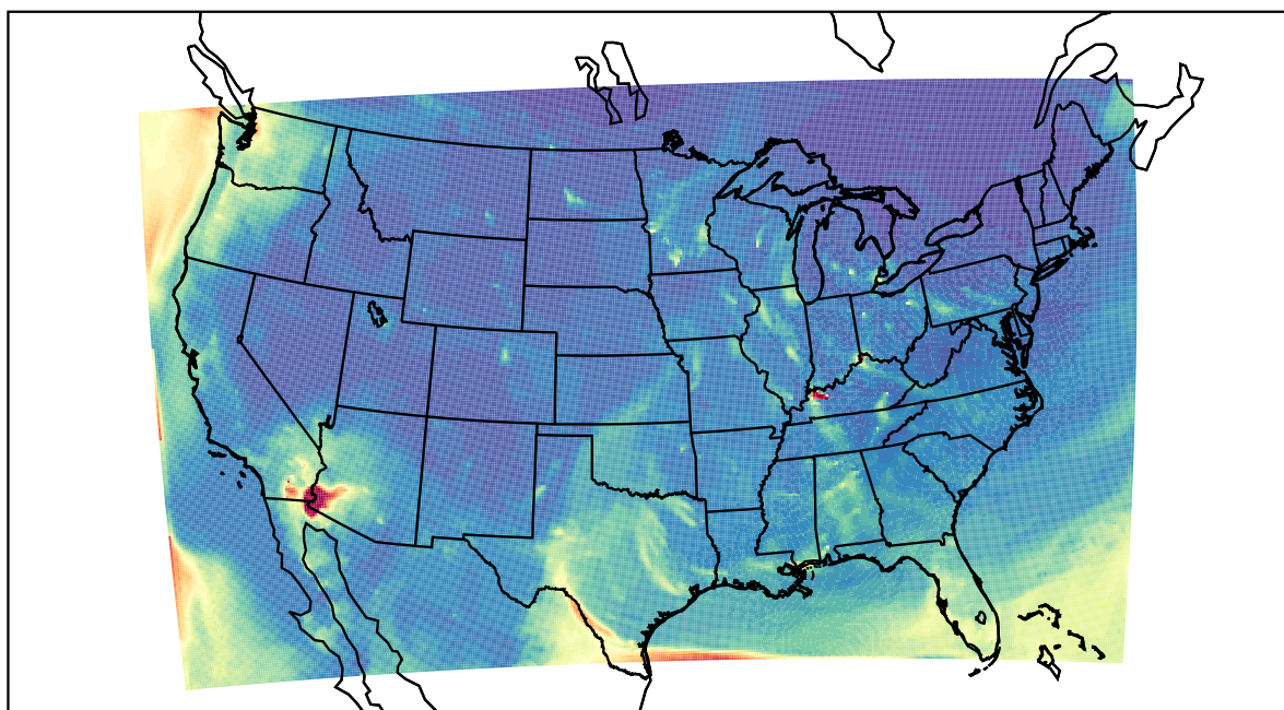
WRF 2022-04-02_07:00:00
