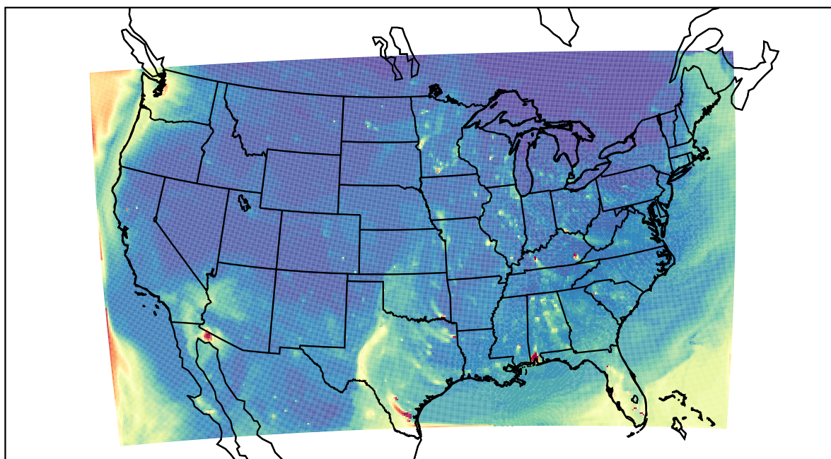
WRF 2022-04-02_01:00:00
