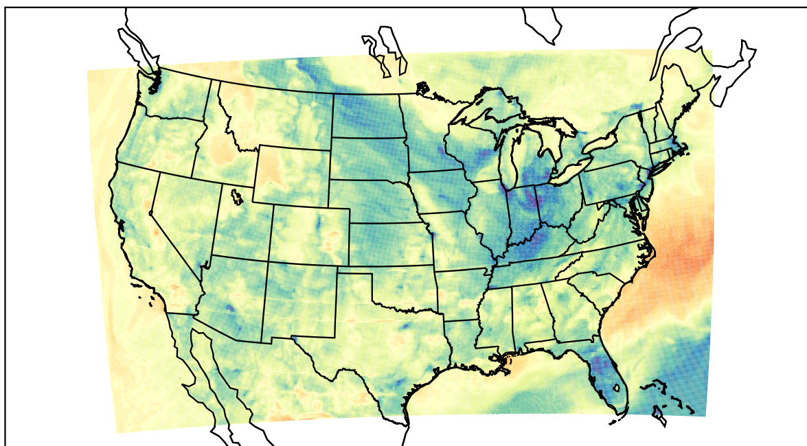
WRF (2022-04-03_04:00:00)
