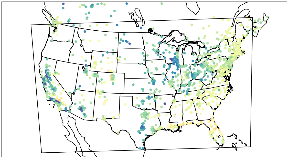
AirNOW (2022-04-04_16:00:00)
