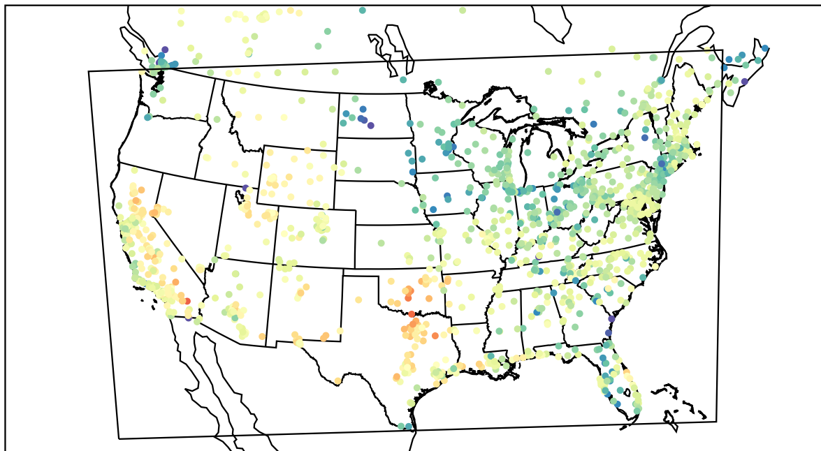
AirNOW (2022-04-04_00:00:00)
