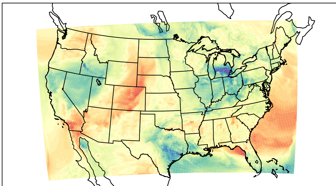
WRF (2022-04-04_23:00:00)
