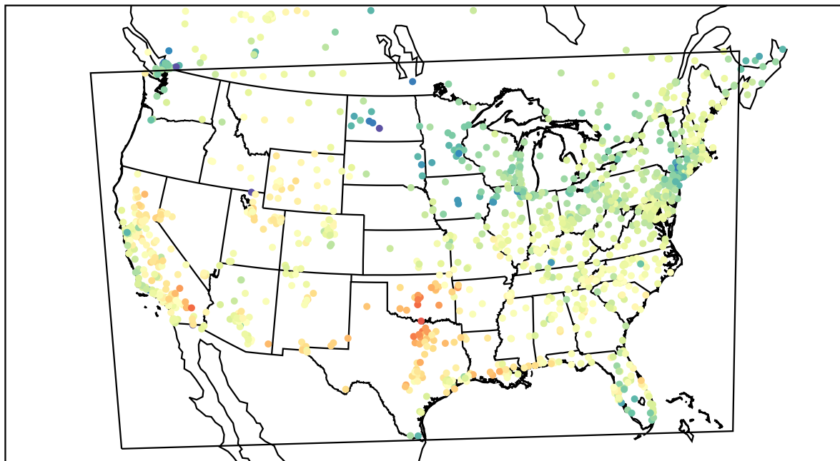
AirNOW (2022-04-03_23:00:00)
