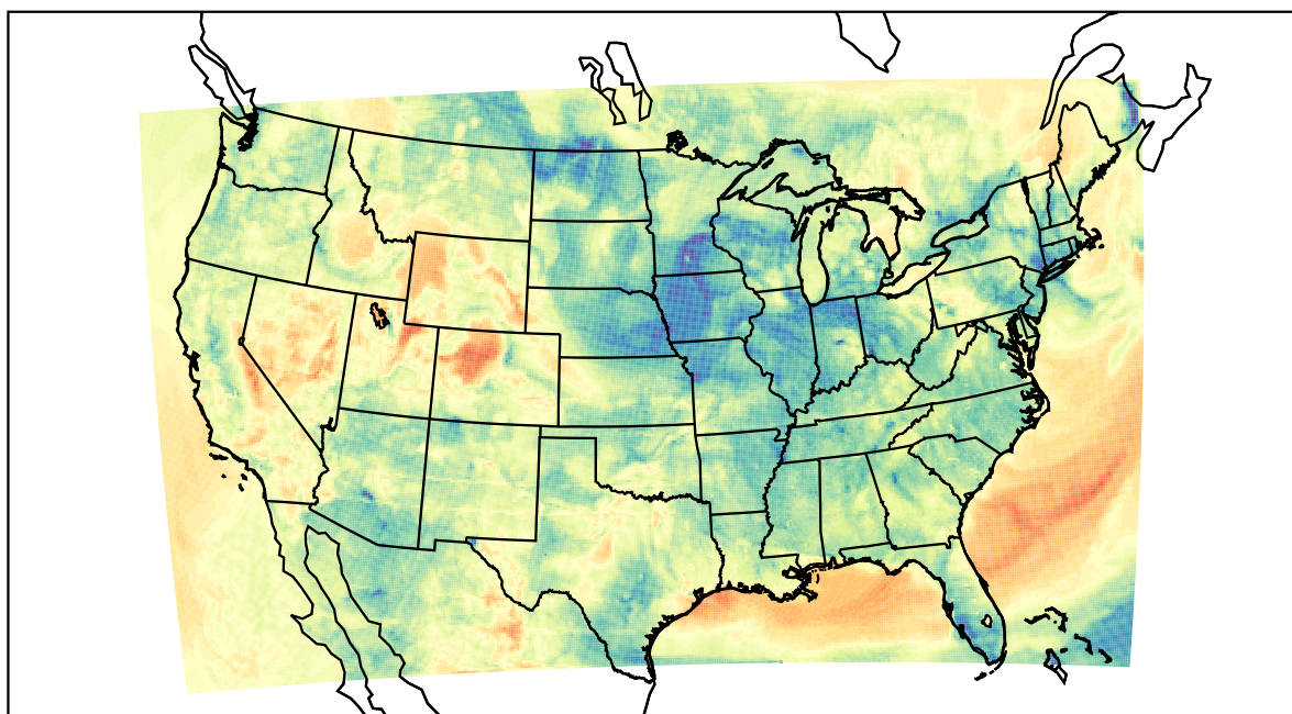
WRF (2022-04-04_04:00:00)
