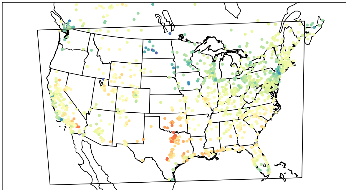
AirNOW (2022-04-03_21:00:00)
