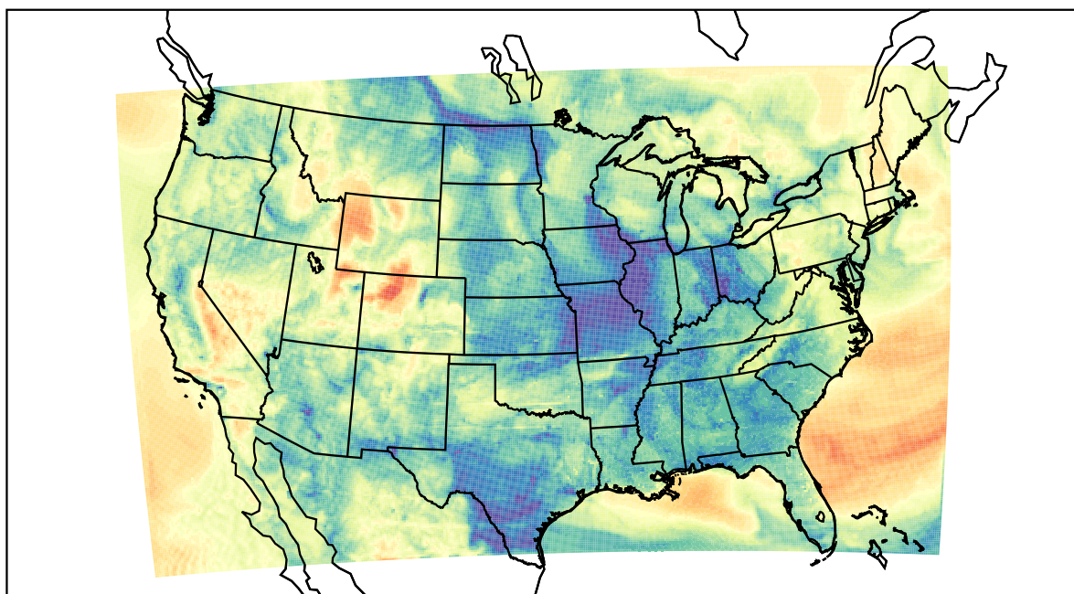
WRF (2022-04-04_13:00:00)
