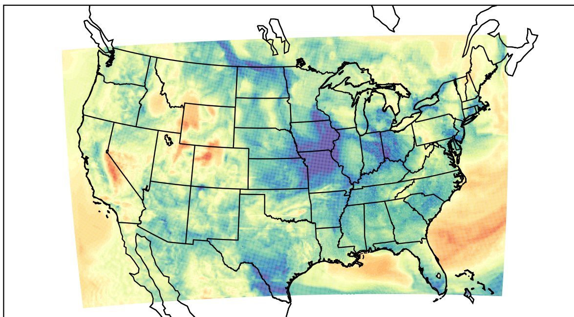
WRF (2022-04-04_10:00:00)
