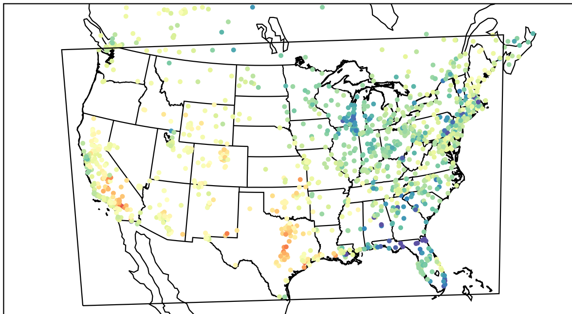
AirNOW (2022-04-03_00:00:00)
