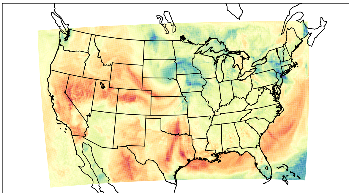
WRF (2022-04-03_23:00:00)
