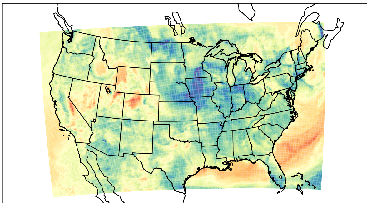
WRF (2022-04-04_05:00:00)
