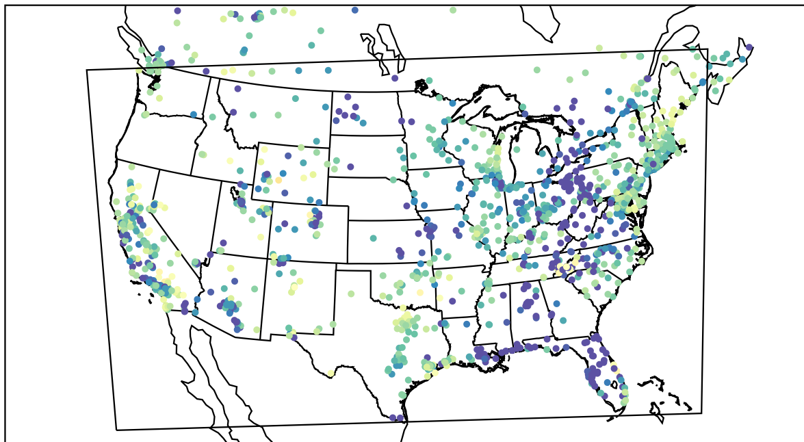
AirNOW (2022-04-04_09:00:00)
