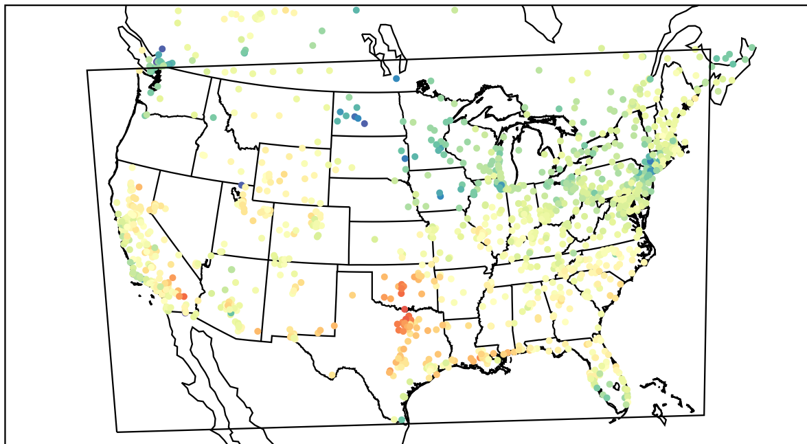
AirNOW (2022-04-03_22:00:00)
