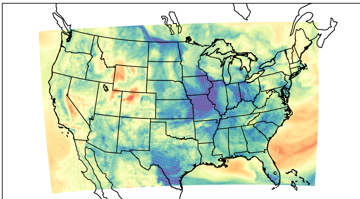
WRF (2022-04-04_12:00:00)
