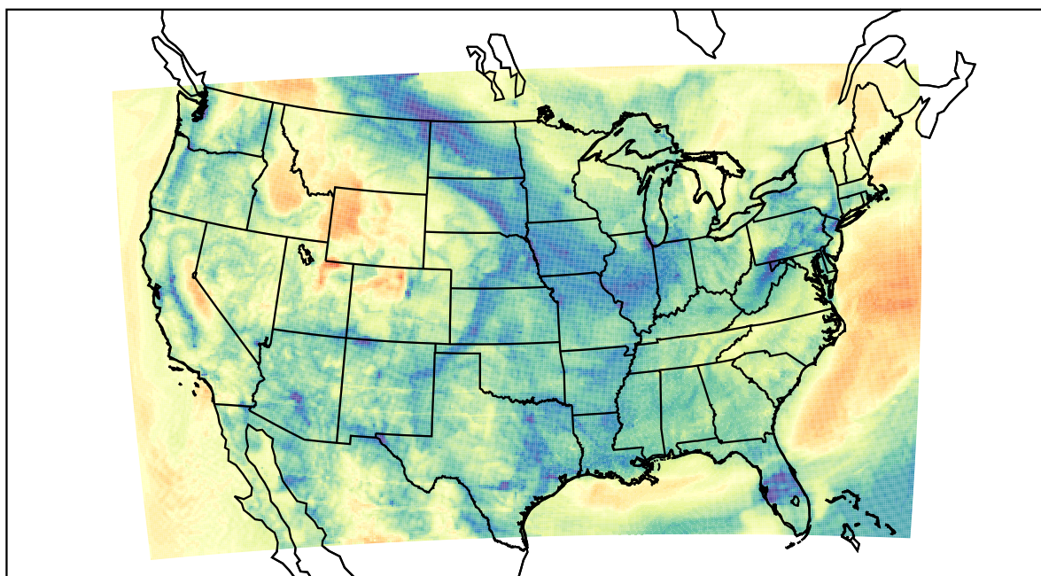
WRF (2022-04-03_14:00:00)
