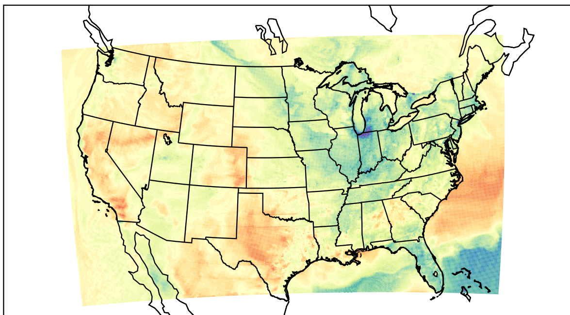
WRF (2022-04-03_00:00:00)
