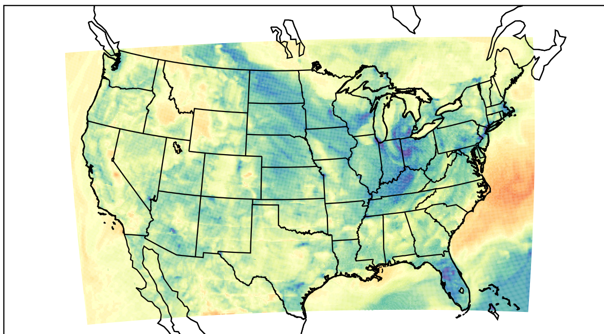
WRF (2022-04-03_05:00:00)
