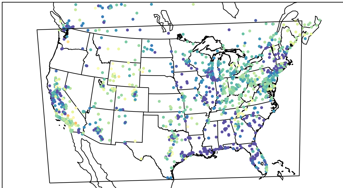
AirNOW (2022-04-03_08:00:00)
