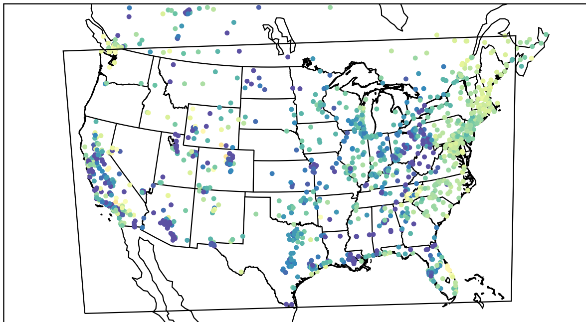
AirNOW (2022-04-04_13:00:00)
