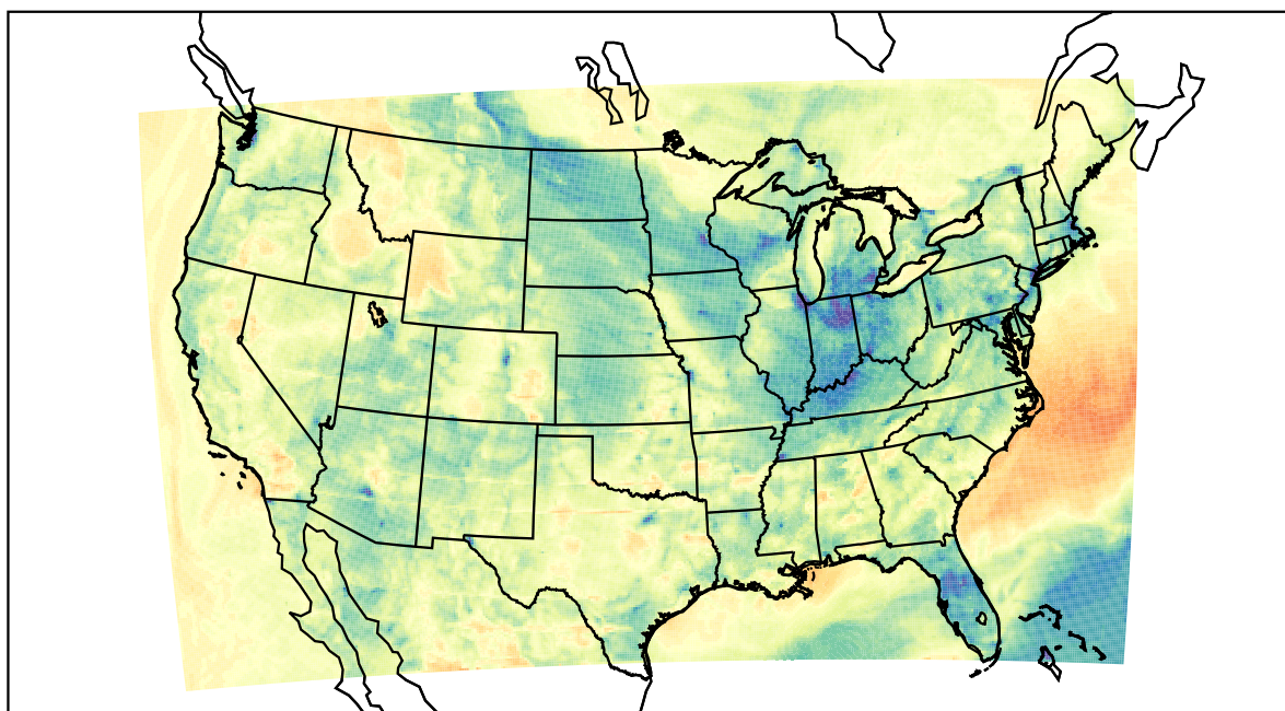
WRF (2022-04-03_03:00:00)
