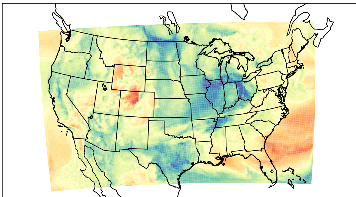
WRF (2022-04-04_16:00:00)
