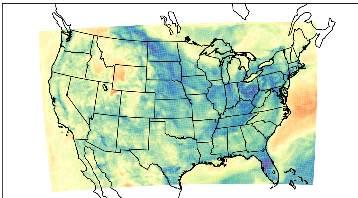
WRF (2022-04-03_09:00:00)
