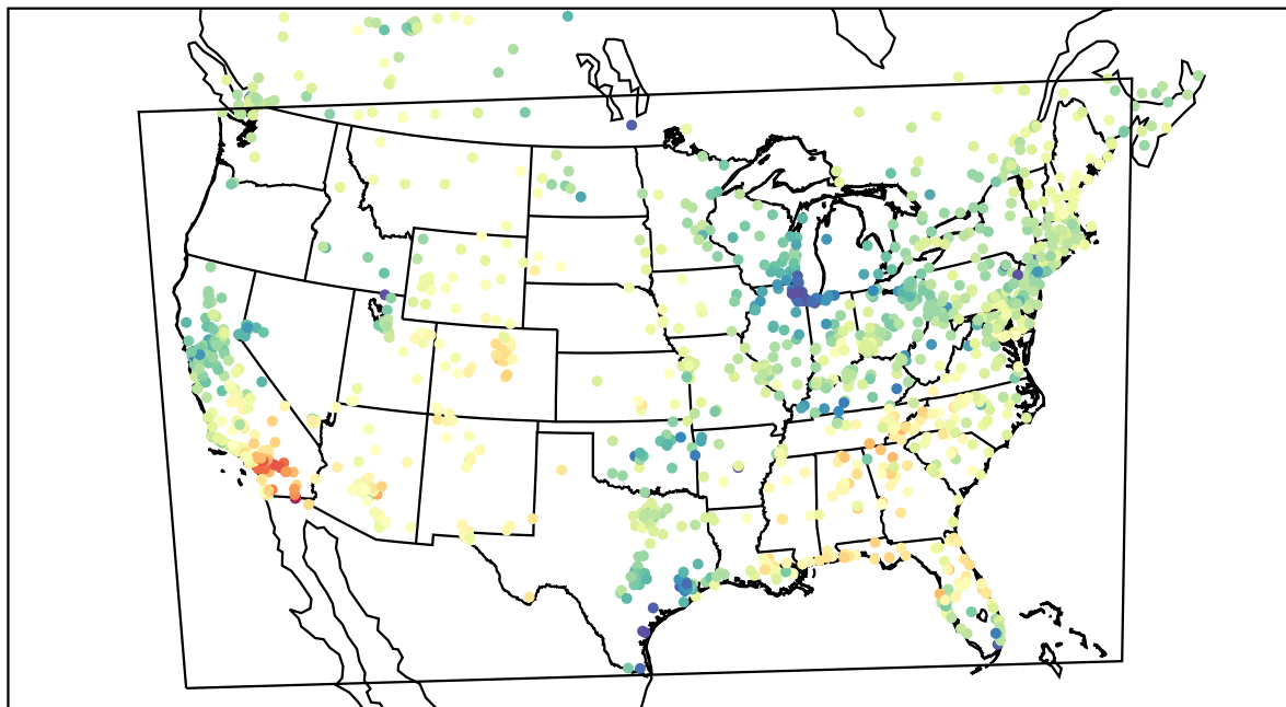
AirNOW (2022-04-04_23:00:00)
