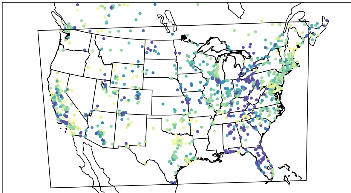
AirNOW (2022-04-04_07:00:00)
