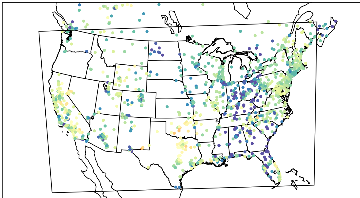
AirNOW (2022-04-04_03:00:00)
