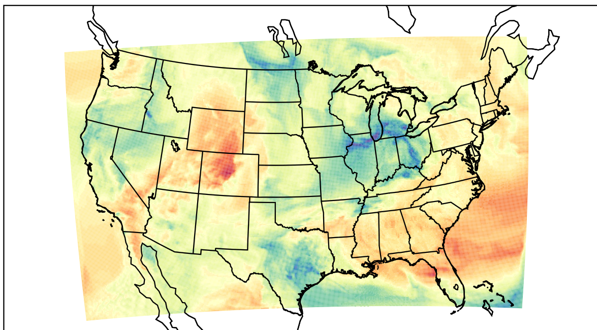
WRF (2022-04-04_18:00:00)
