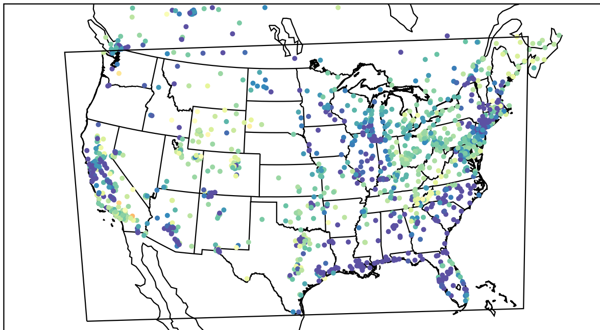
AirNOW (2022-04-03_09:00:00)
