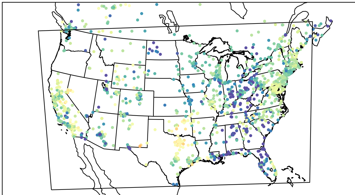
AirNOW (2022-04-04_04:00:00)
