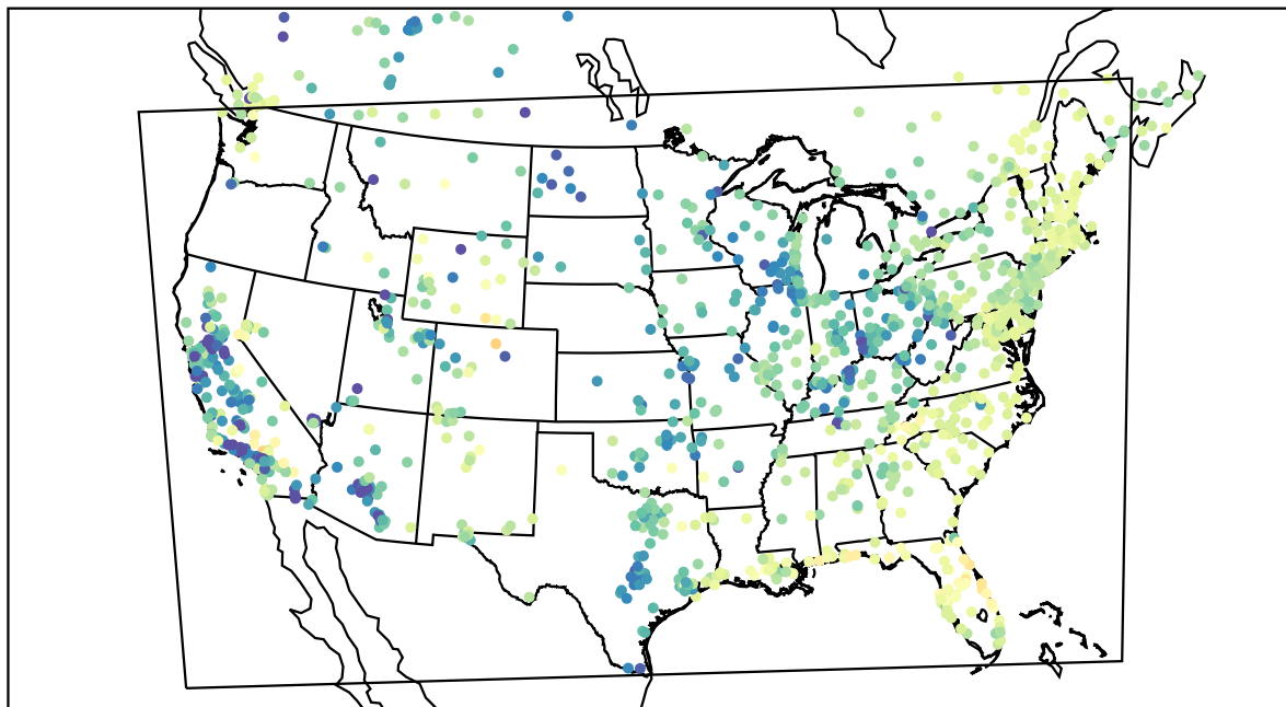
AirNOW (2022-04-04_15:00:00)
