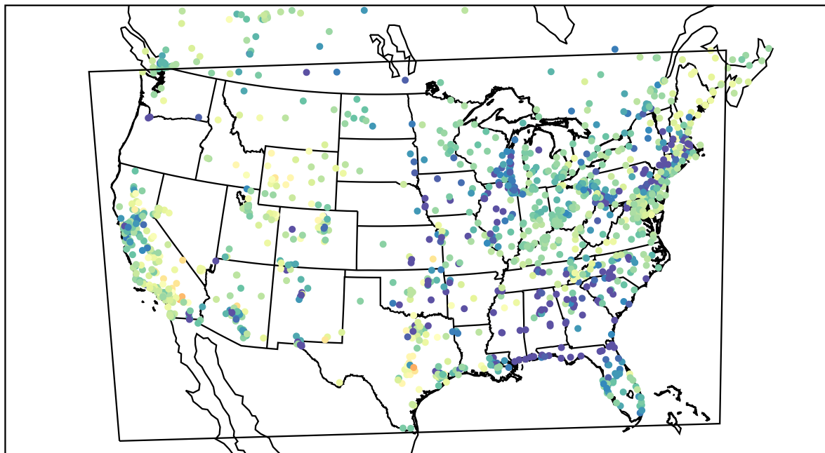
AirNOW (2022-04-03_03:00:00)
