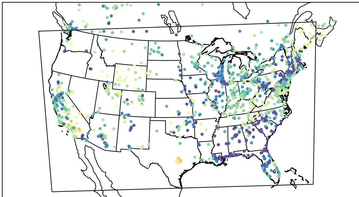
AirNOW (2022-04-03_04:00:00)
