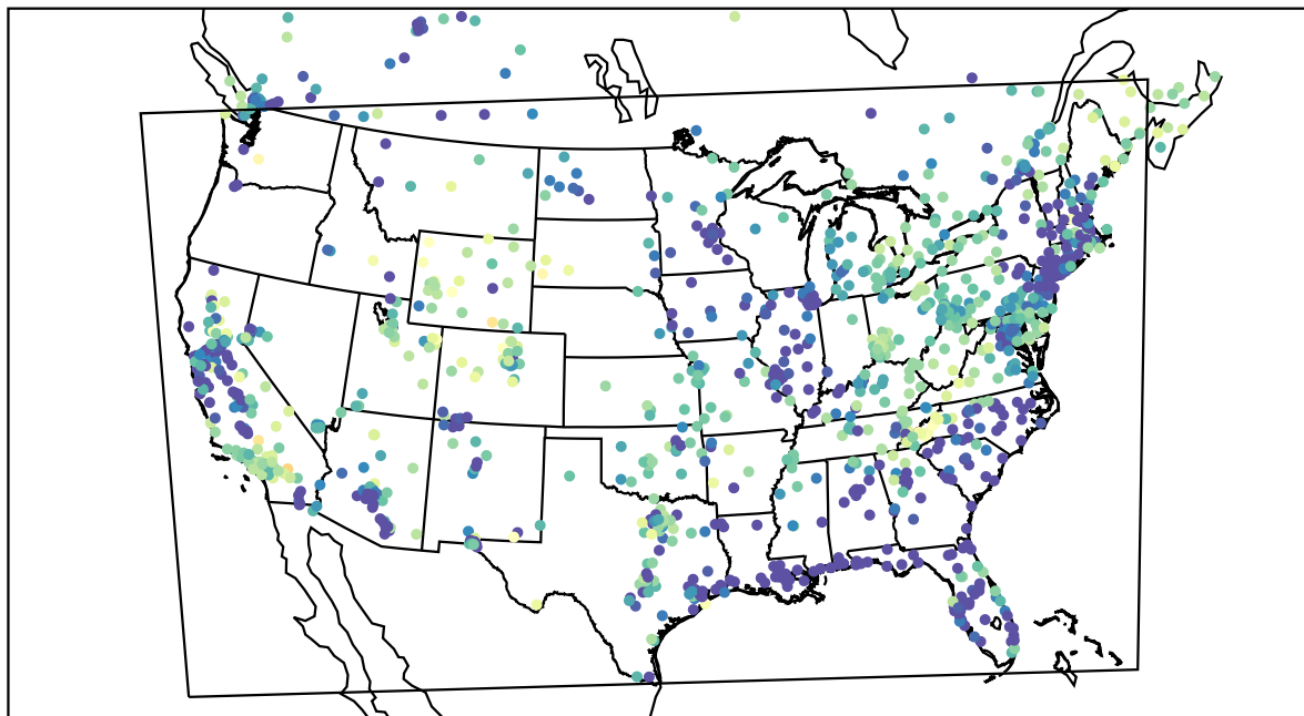
AirNOW (2022-04-03_10:00:00)
