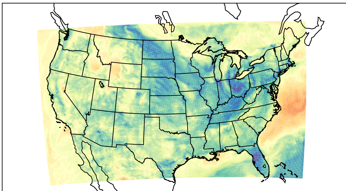
WRF (2022-04-03_07:00:00)
