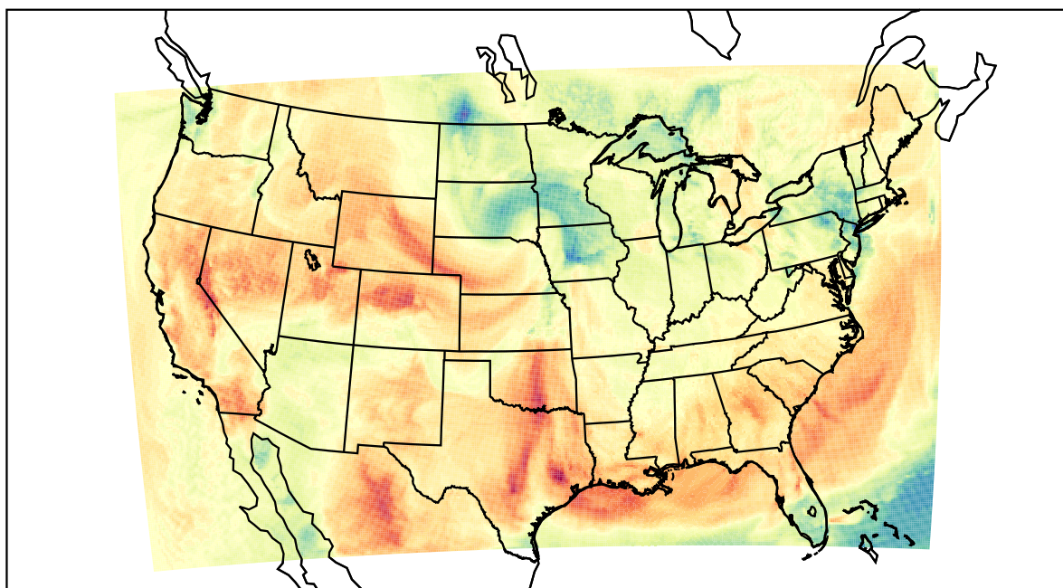
WRF (2022-04-03_21:00:00)
