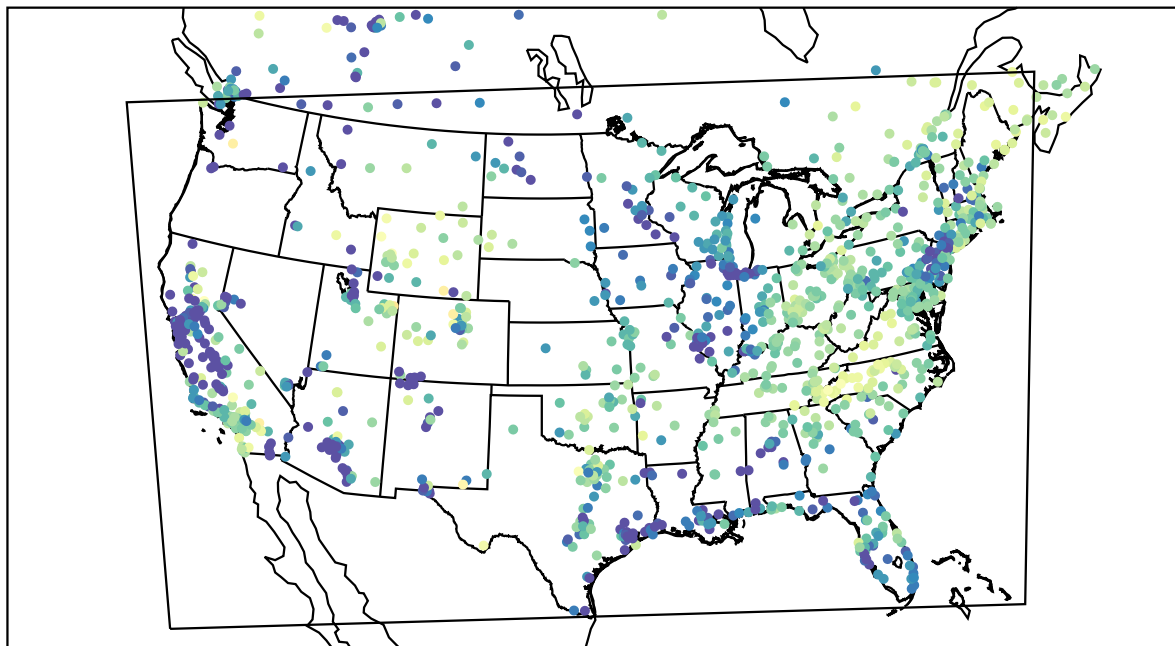
AirNOW (2022-04-03_13:00:00)
