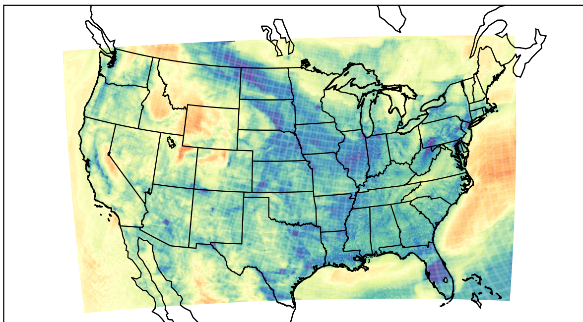
WRF (2022-04-03_13:00:00)
