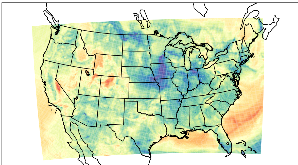
WRF (2022-04-04_06:00:00)
