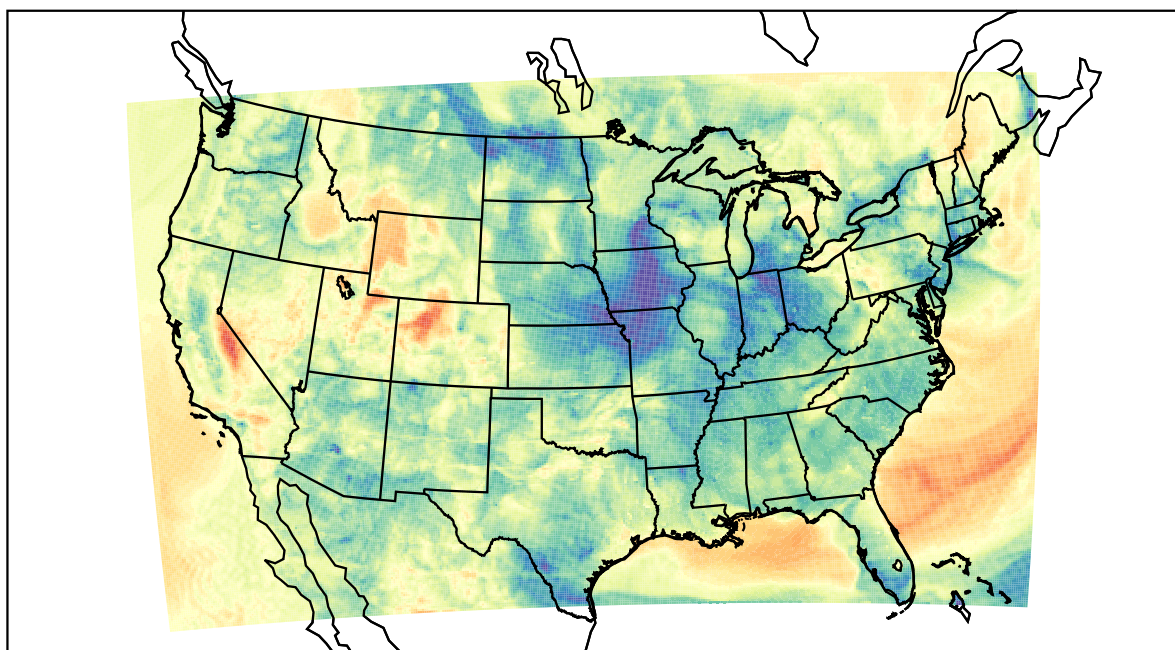
WRF (2022-04-04_07:00:00)
