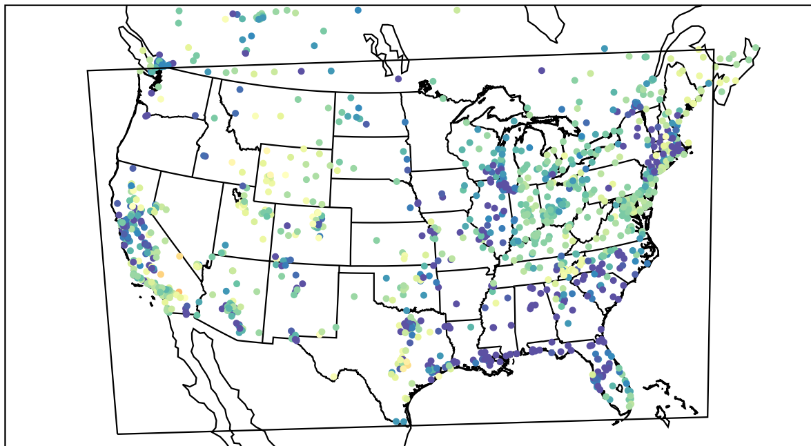
AirNOW (2022-04-03_06:00:00)
