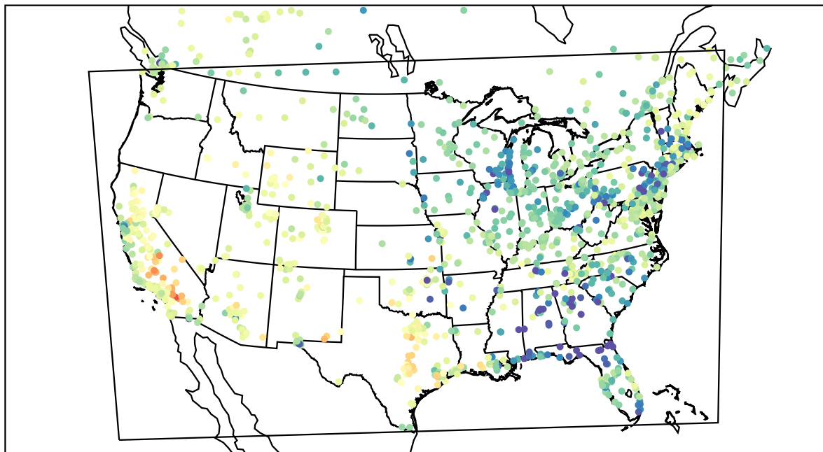
AirNOW (2022-04-03_01:00:00)
