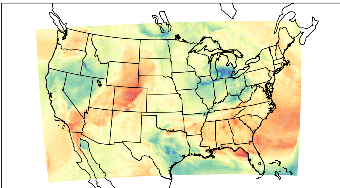
WRF (2022-04-04_21:00:00)
