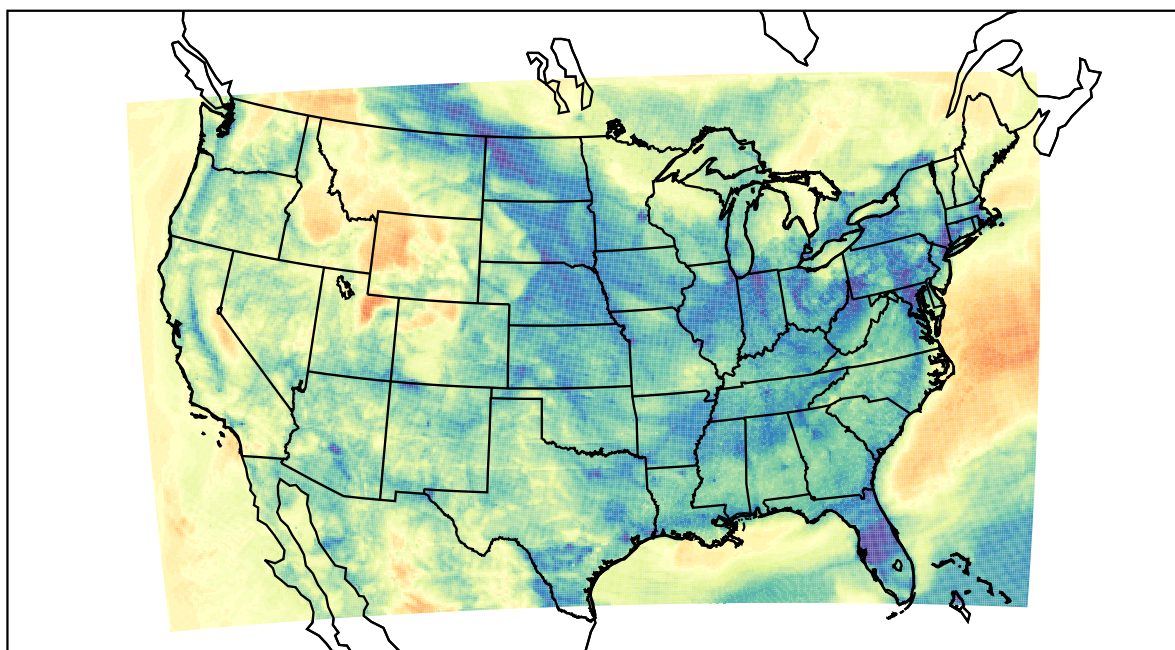
WRF (2022-04-03_11:00:00)
