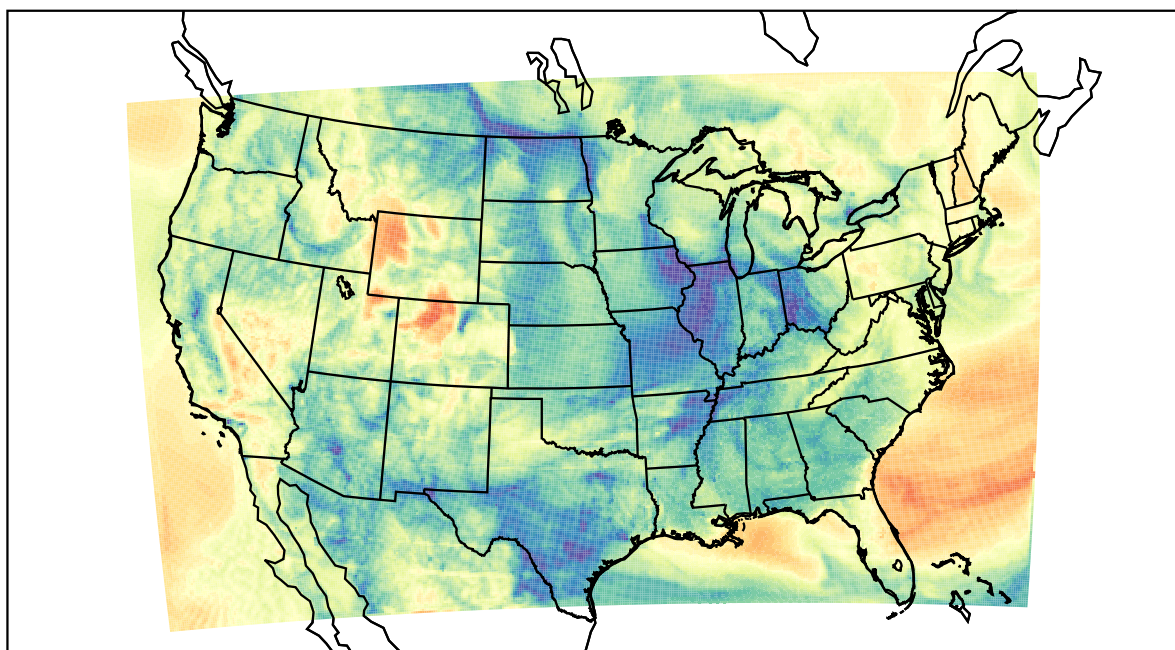
WRF (2022-04-04_14:00:00)
