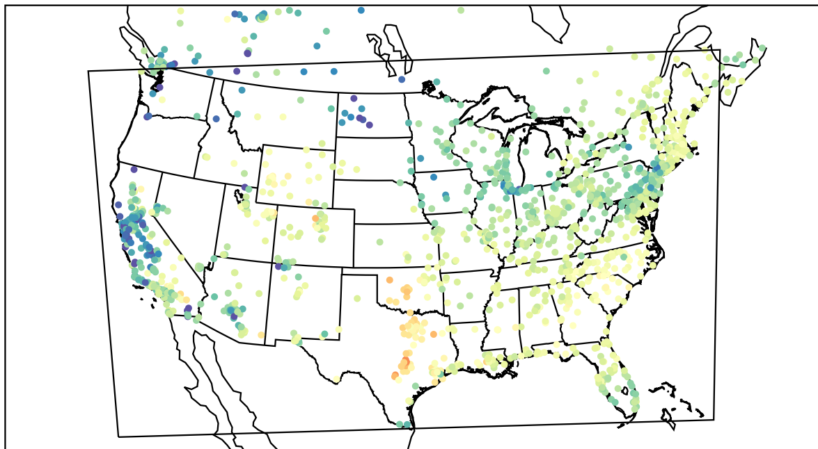
AirNOW (2022-04-03_16:00:00)
