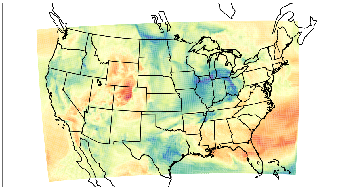
WRF (2022-04-04_17:00:00)
