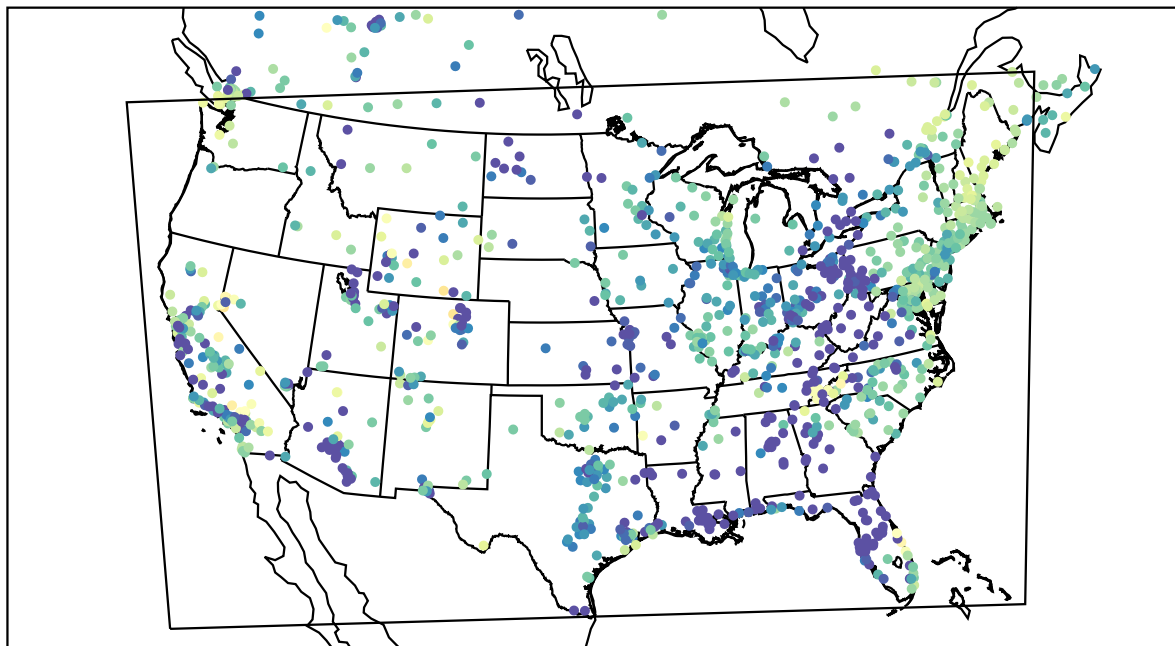
AirNOW (2022-04-04_12:00:00)
