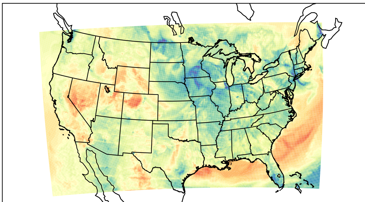
WRF (2022-04-04_02:00:00)
