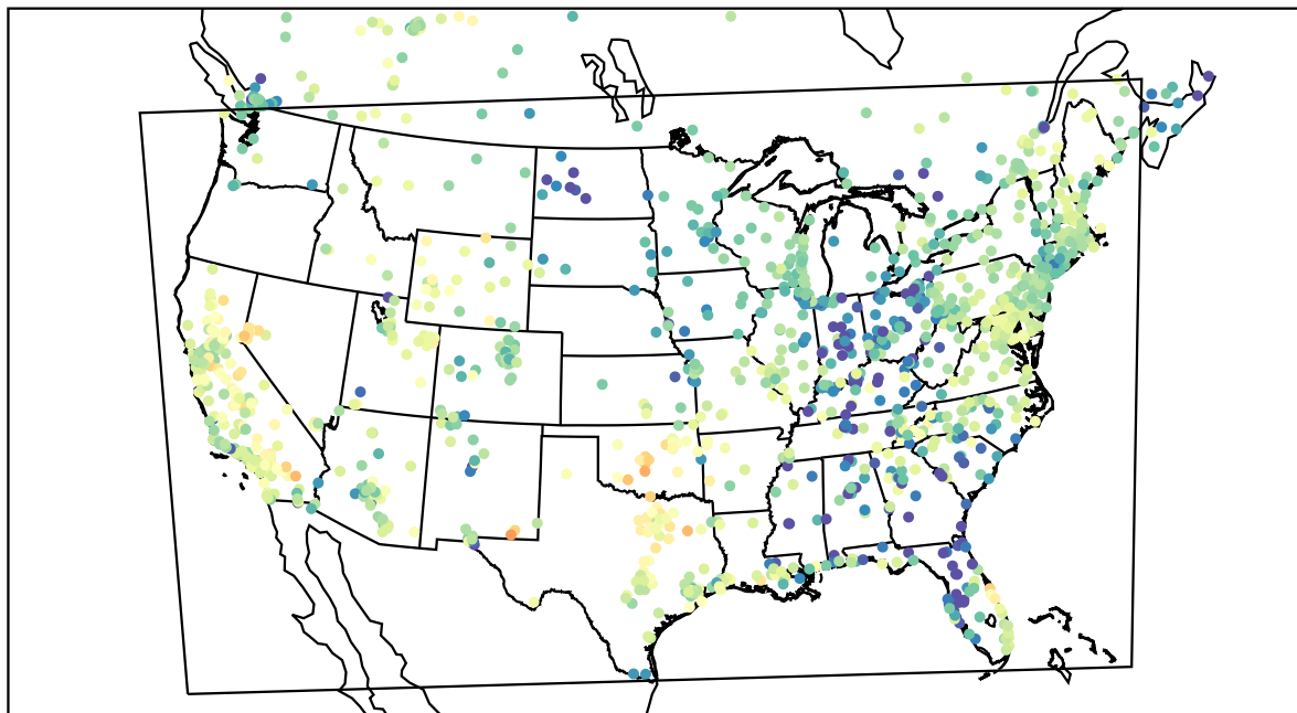
AirNOW (2022-04-04_02:00:00)
