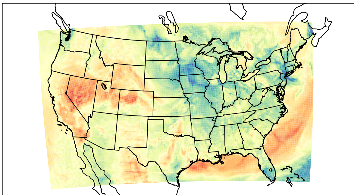
WRF (2022-04-04_01:00:00)
