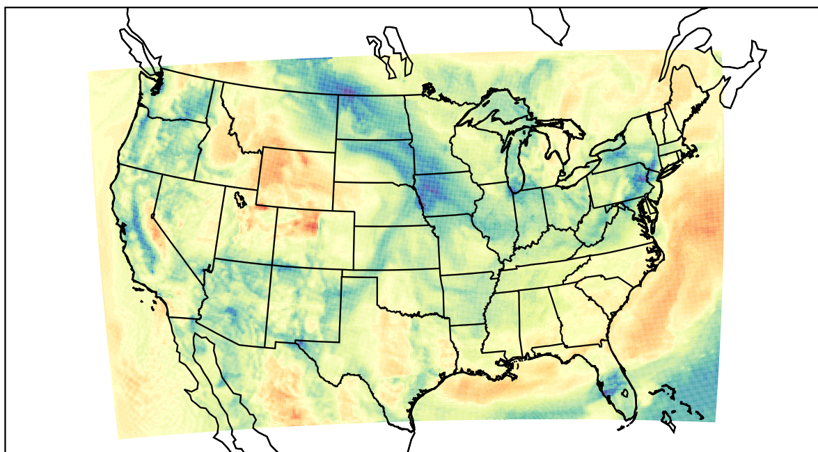
WRF (2022-04-03_16:00:00)
