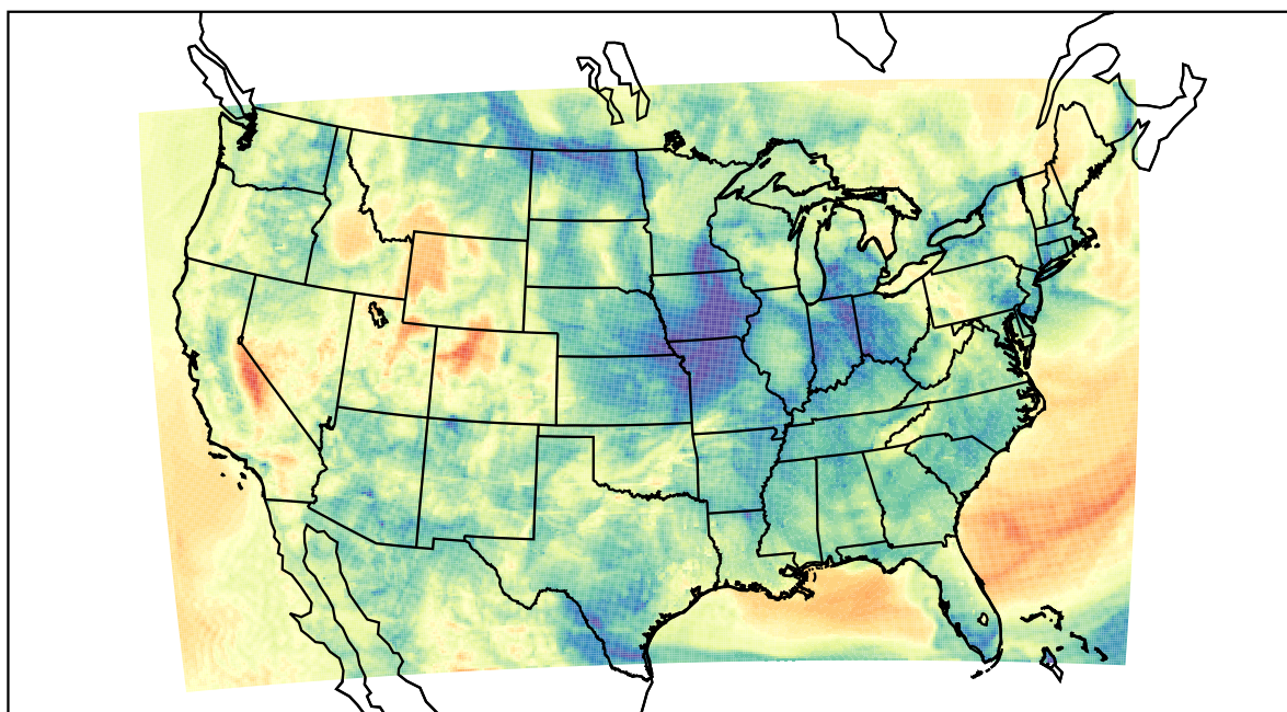
WRF (2022-04-04_08:00:00)
