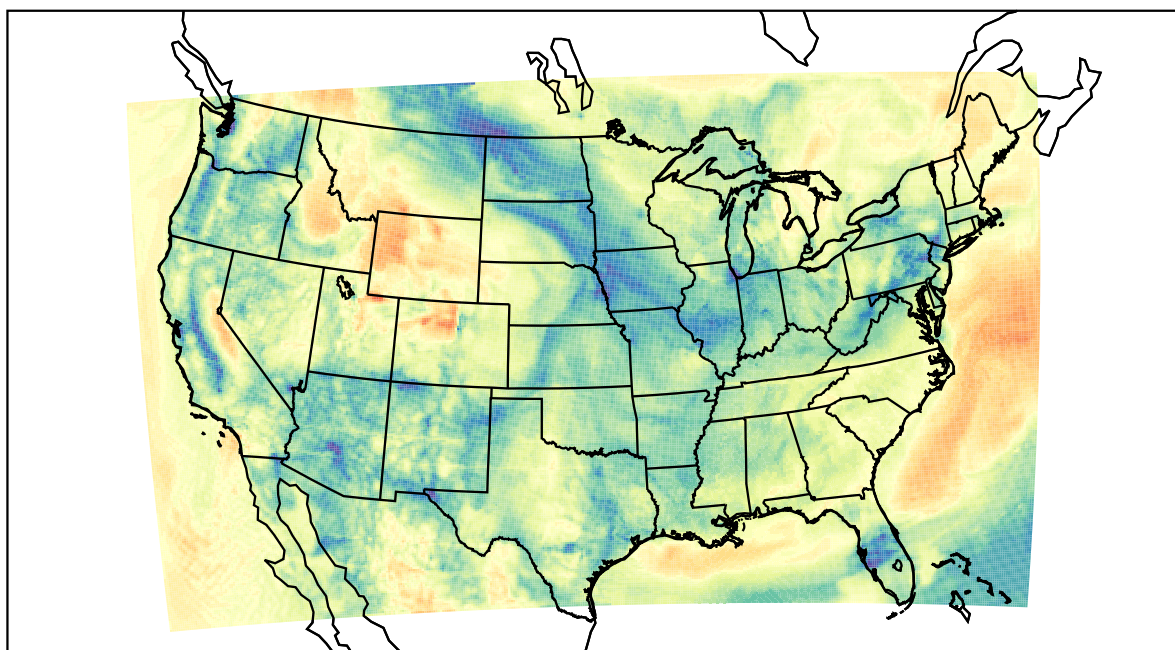
WRF (2022-04-03_15:00:00)
