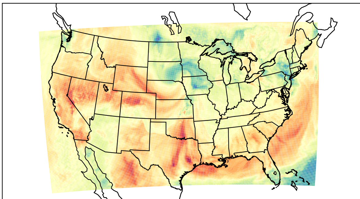
WRF (2022-04-03_22:00:00)
