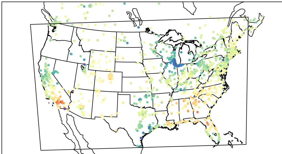
AirNOW (2022-04-04_22:00:00)
