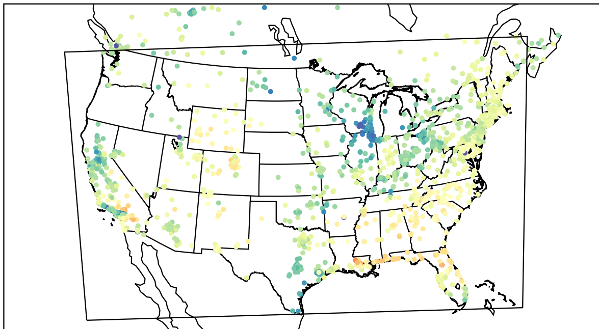
AirNOW (2022-04-04_18:00:00)
