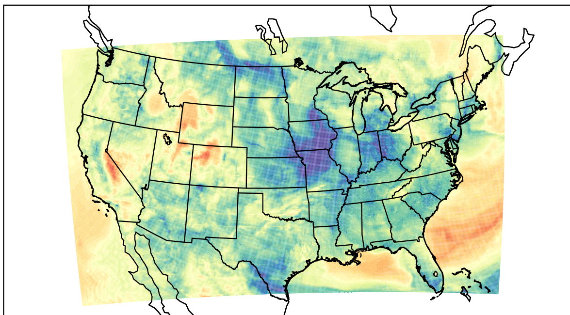
WRF (2022-04-04_09:00:00)
