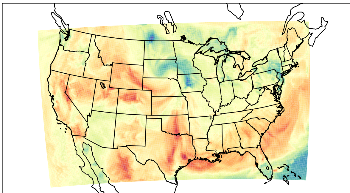
WRF (2022-04-03_20:00:00)
