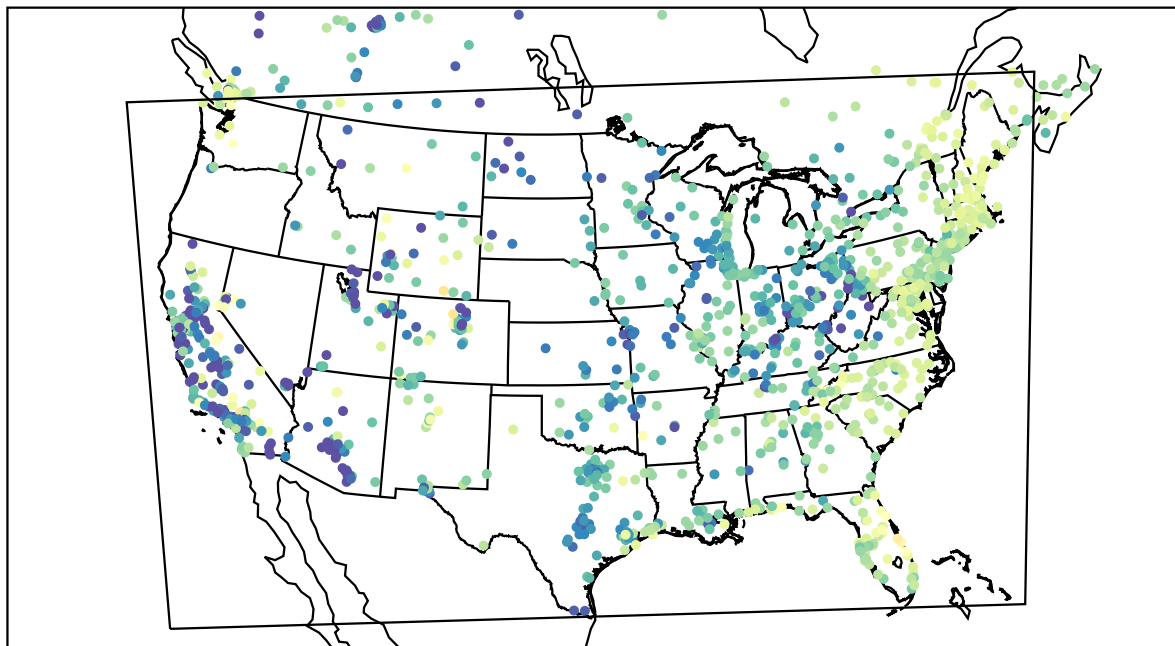
AirNOW (2022-04-04_14:00:00)
