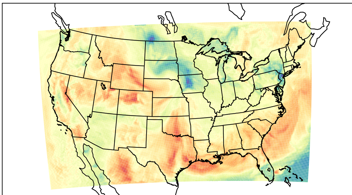
WRF (2022-04-03_19:00:00)
