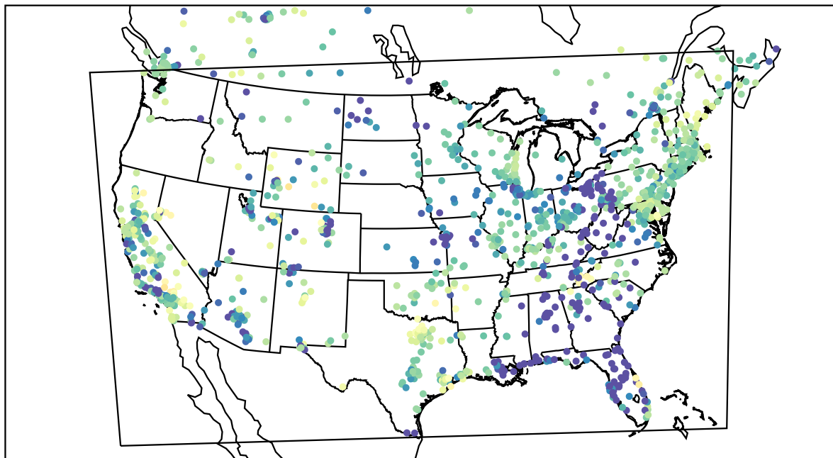
AirNOW (2022-04-04_08:00:00)
