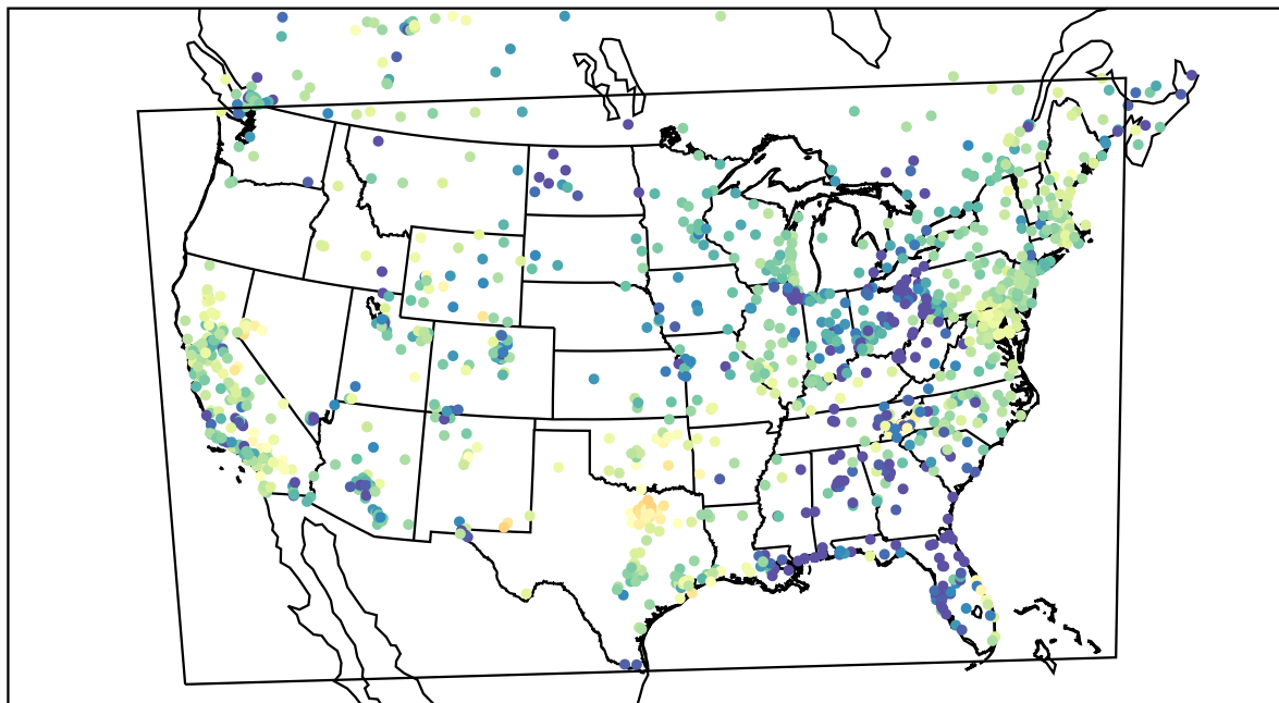
AirNOW (2022-04-04_05:00:00)
