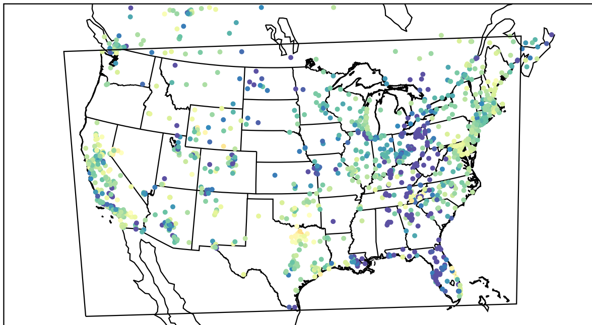
AirNOW (2022-04-04_06:00:00)
