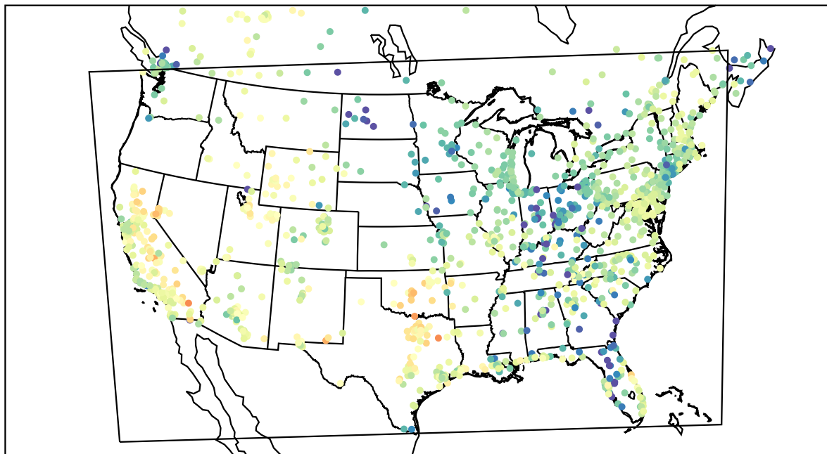
AirNOW (2022-04-04_01:00:00)
