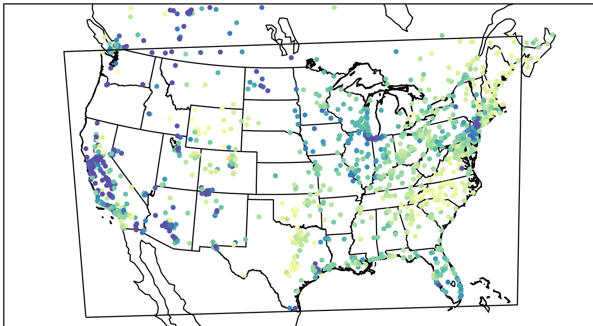
AirNOW (2022-04-03_14:00:00)
