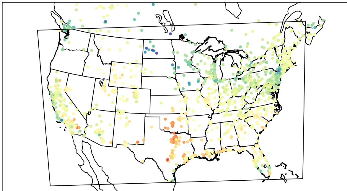
AirNOW (2022-04-03_20:00:00)
