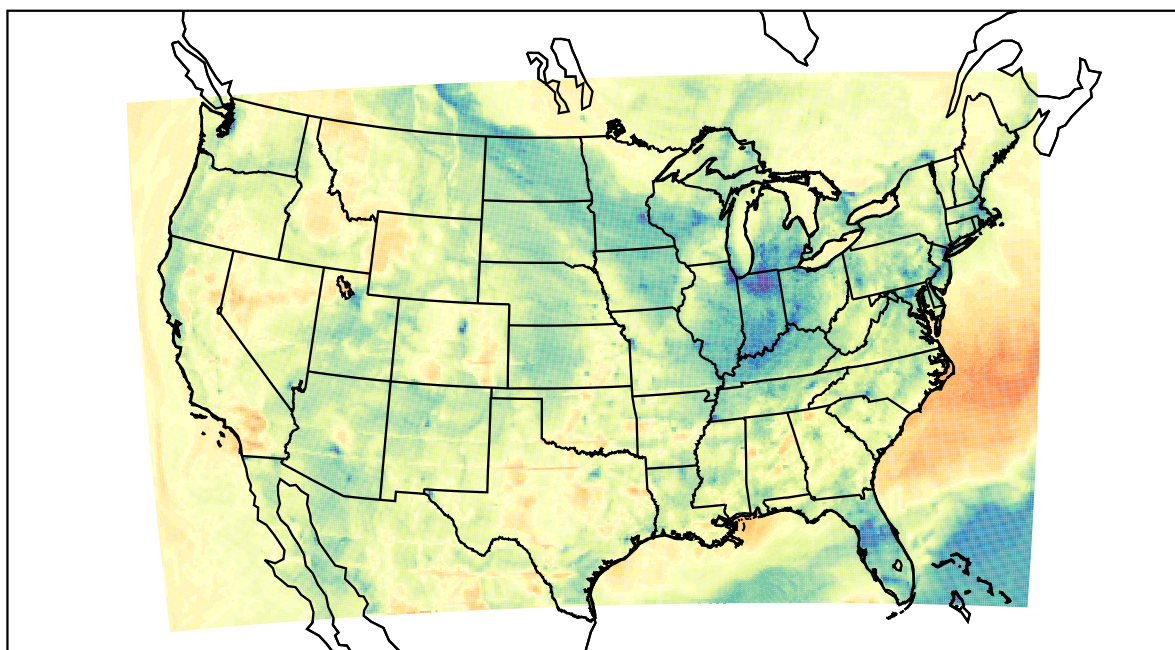
WRF (2022-04-03_02:00:00)
