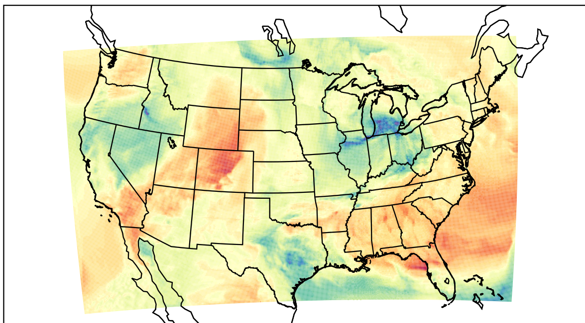
WRF (2022-04-04_20:00:00)
