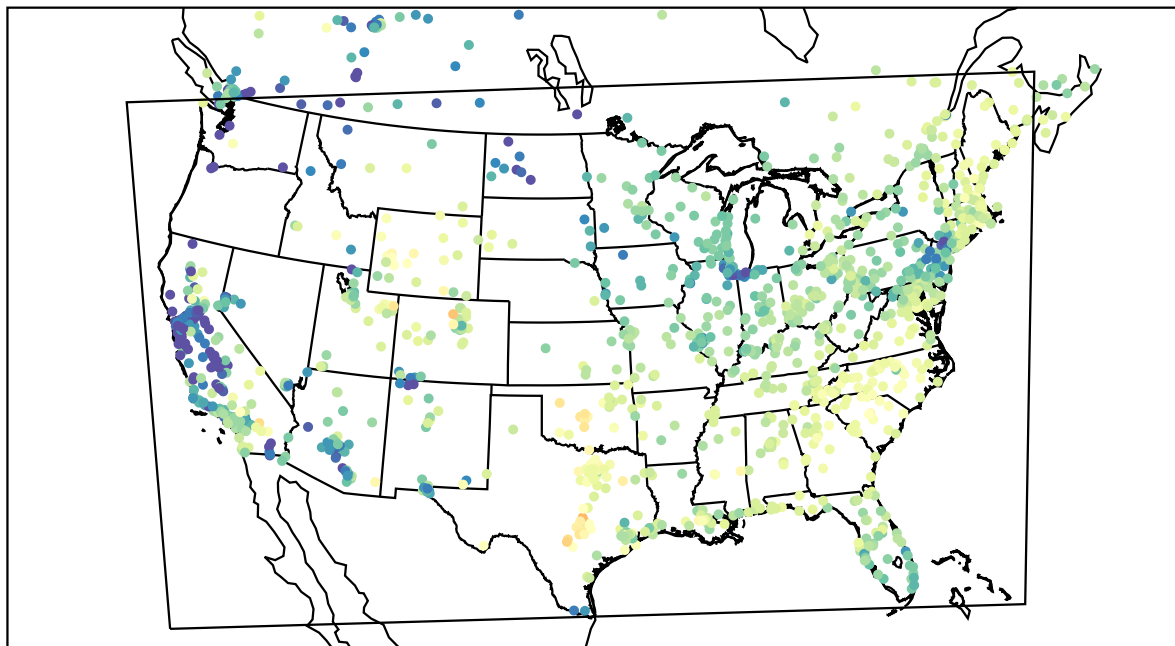
AirNOW (2022-04-03_15:00:00)
