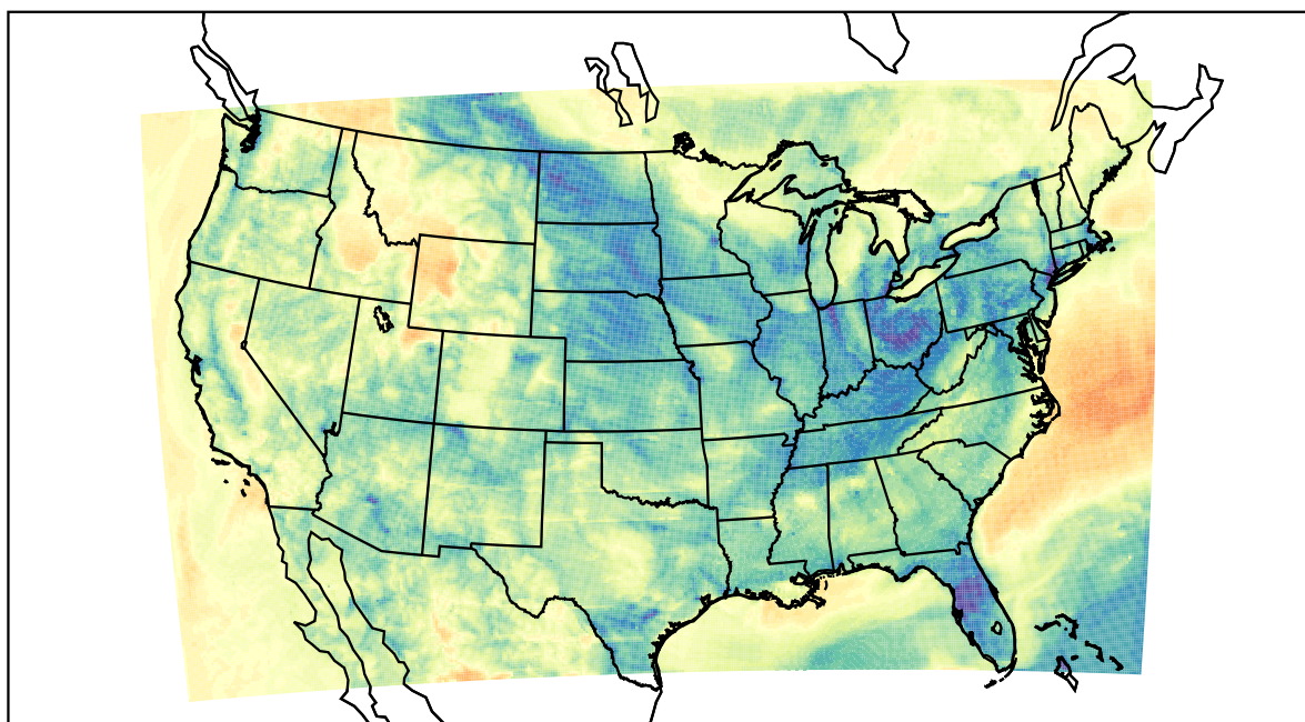
WRF (2022-04-03_08:00:00)
