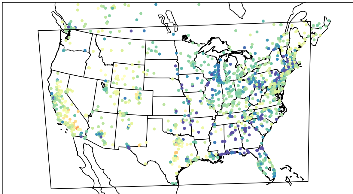
AirNOW (2022-04-03_02:00:00)
