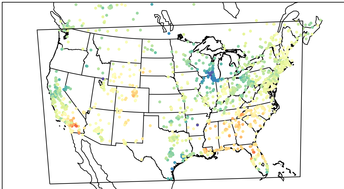
AirNOW (2022-04-04_20:00:00)
