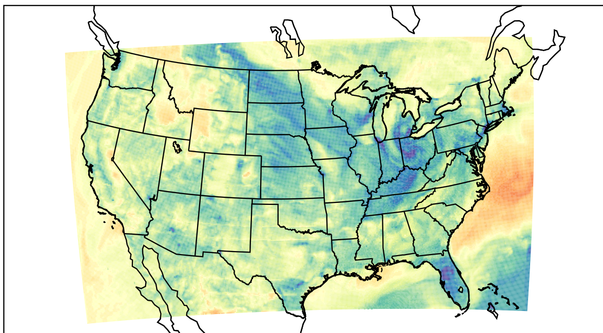
WRF (2022-04-03_06:00:00)
