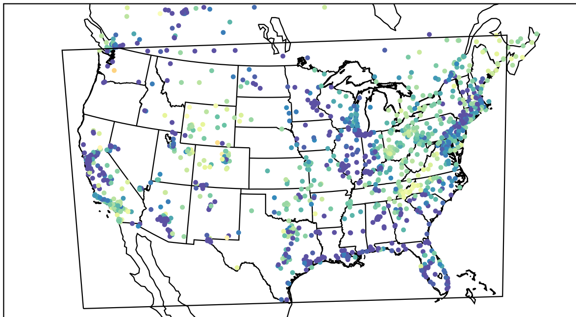
AirNOW (2022-04-03_12:00:00)
