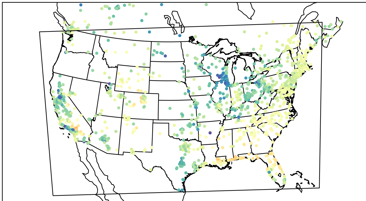
AirNOW (2022-04-04_17:00:00)
