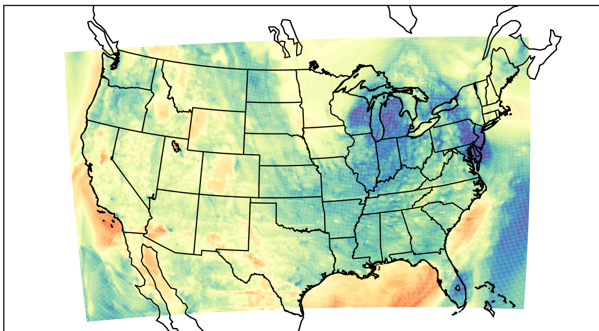
WRF (2022-04-08_03:00:00)
