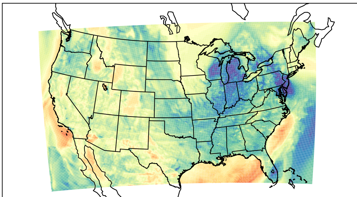
WRF (2022-04-08_04:00:00)
