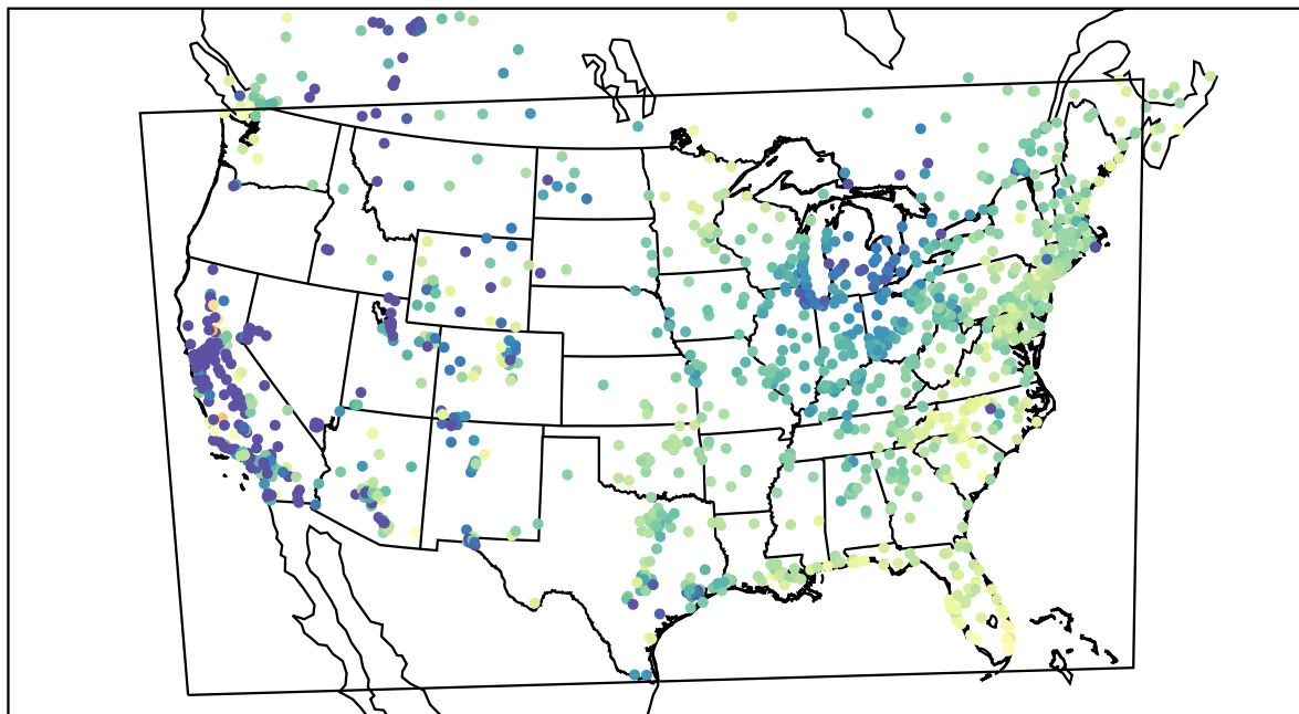
AirNOW (2022-04-08_14:00:00)
