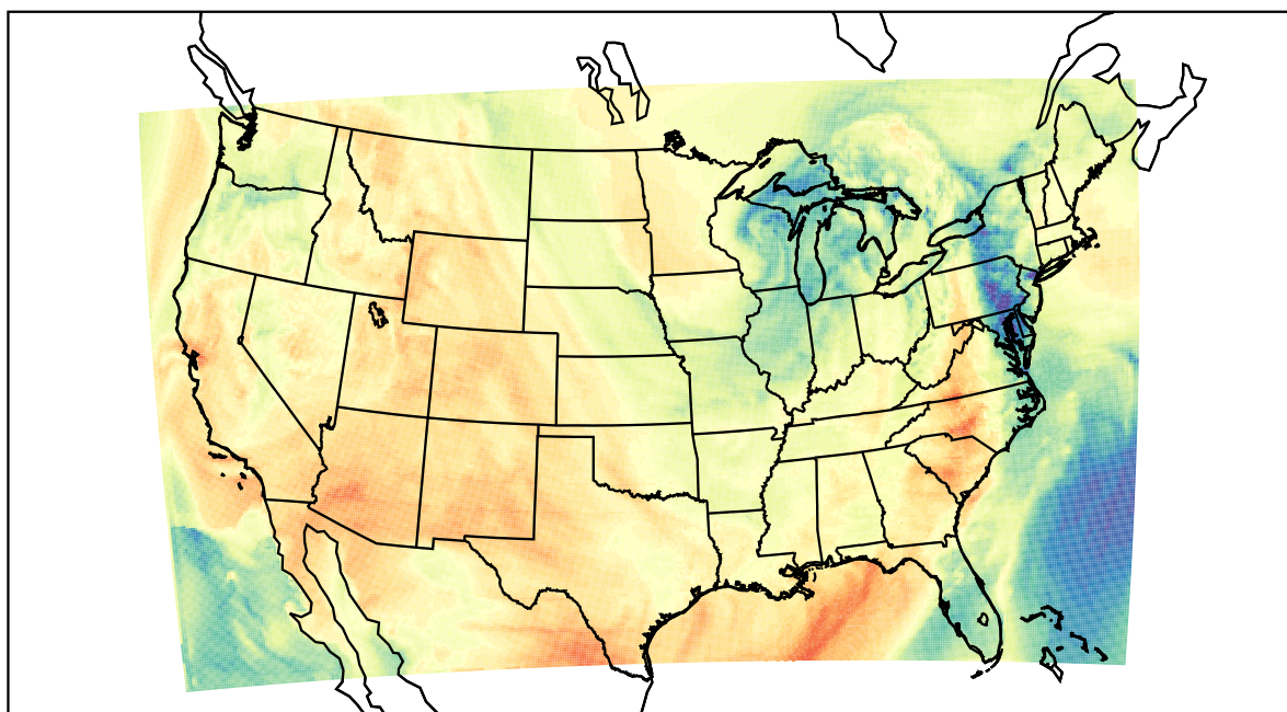
WRF (2022-04-07_21:00:00)
