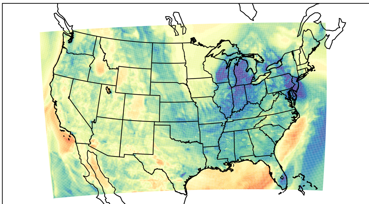
WRF (2022-04-08_05:00:00)
