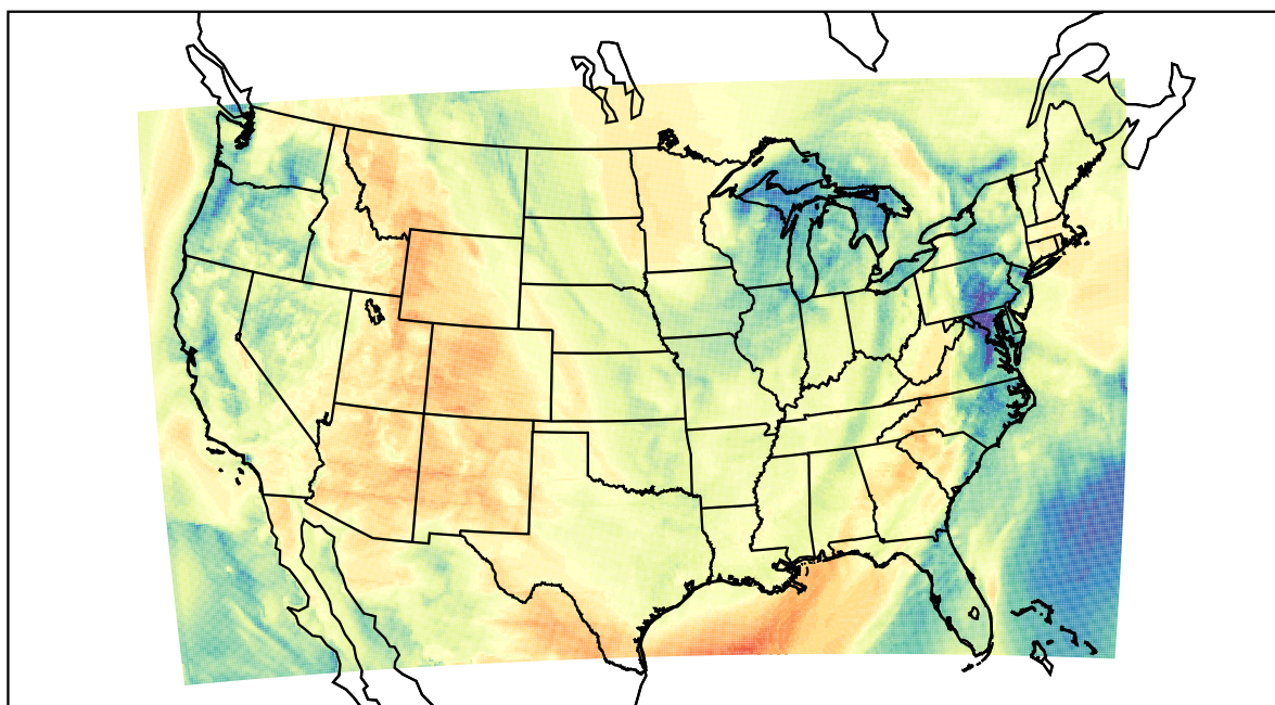
WRF (2022-04-07_17:00:00)
