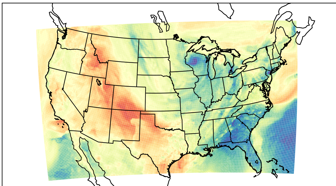
WRF (2022-04-07_00:00:00)
