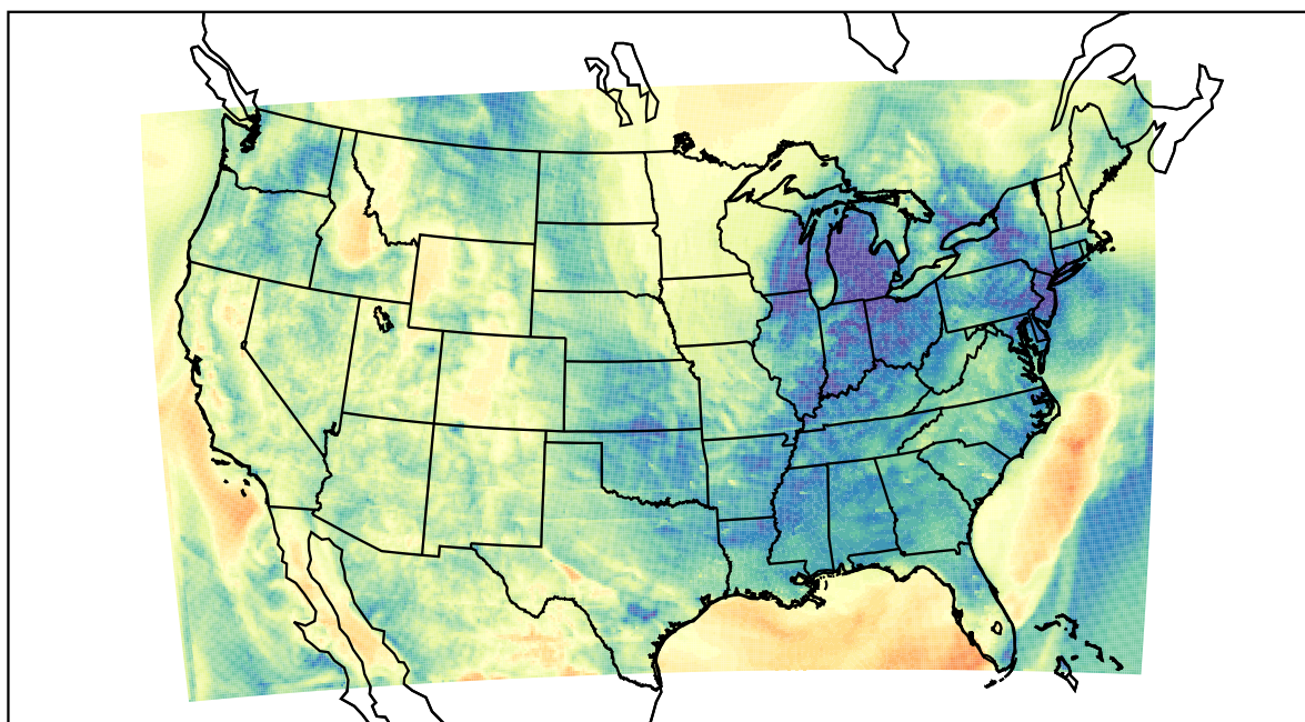
WRF (2022-04-08_09:00:00)
