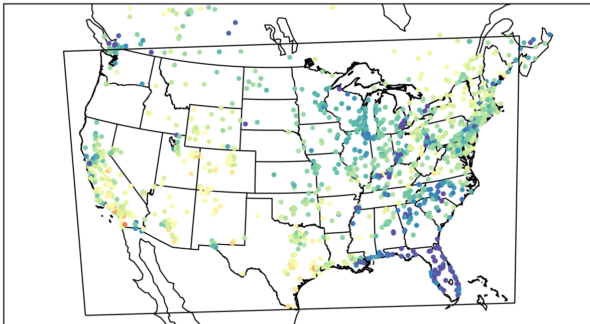
AirNOW (2022-04-07_02:00:00)
