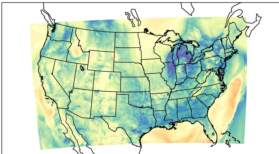
WRF (2022-04-08_13:00:00)
