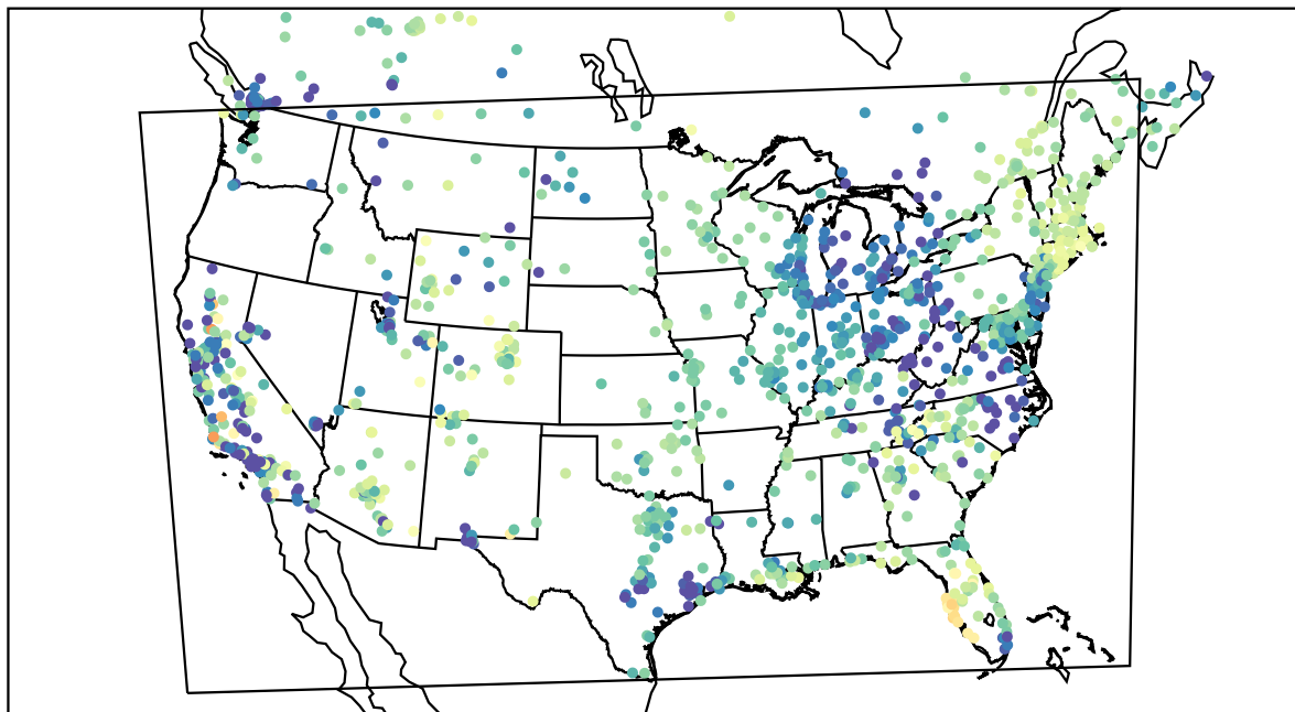
AirNOW (2022-04-08_06:00:00)
