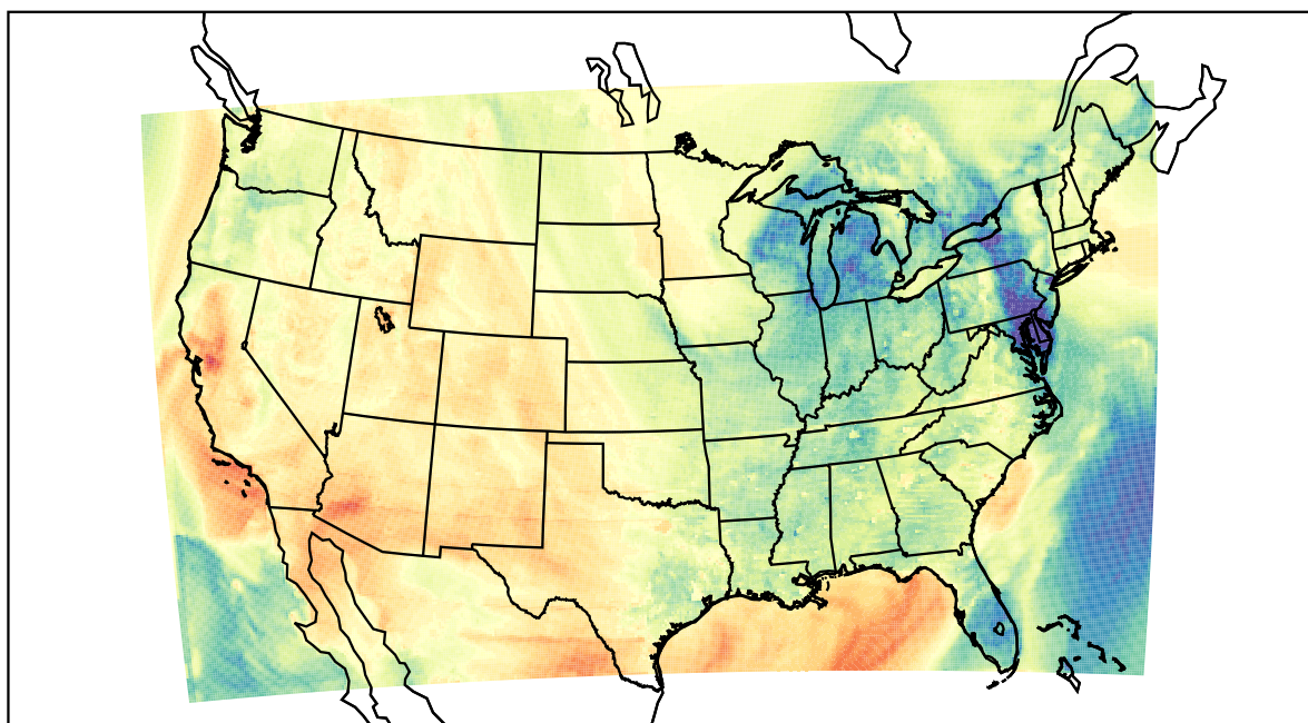
WRF (2022-04-08_00:00:00)
