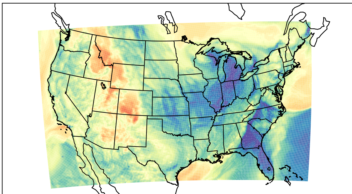
WRF (2022-04-07_07:00:00)
