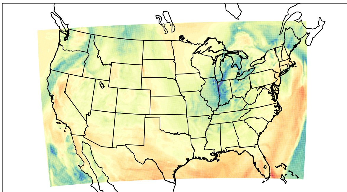
WRF (2022-04-08_19:00:00)
