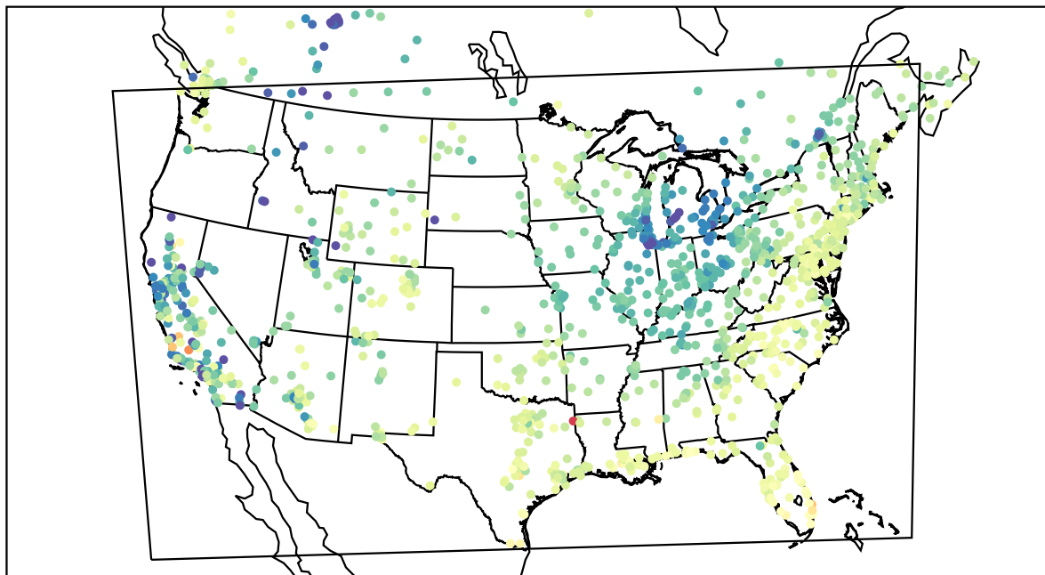
AirNOW (2022-04-08_16:00:00)
