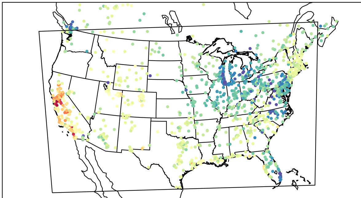
AirNOW (2022-04-08_01:00:00)
