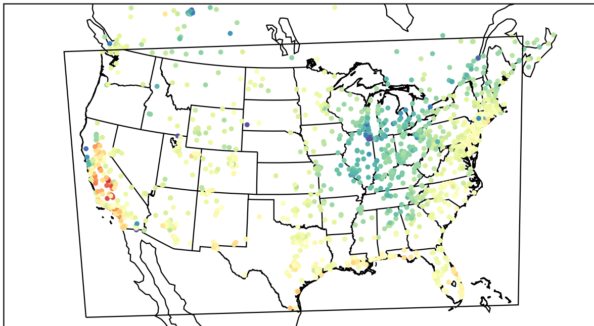
AirNOW (2022-04-08_20:00:00)
