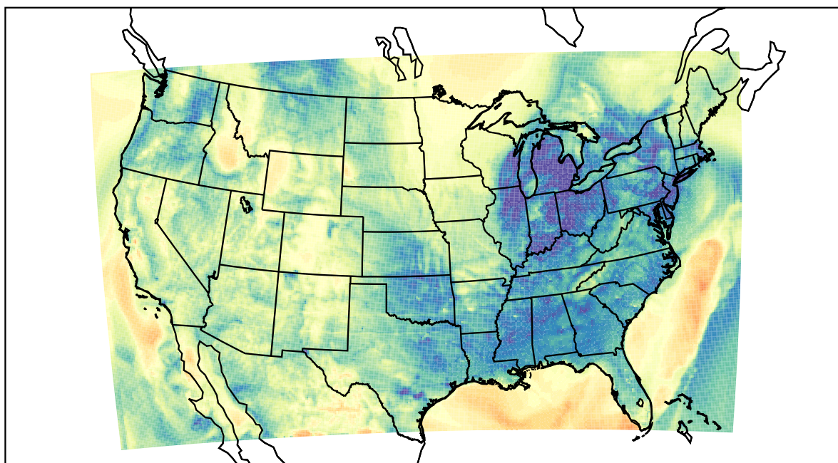
WRF (2022-04-08_12:00:00)
