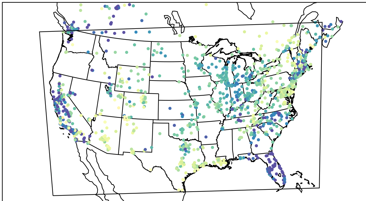
AirNOW (2022-04-07_06:00:00)
