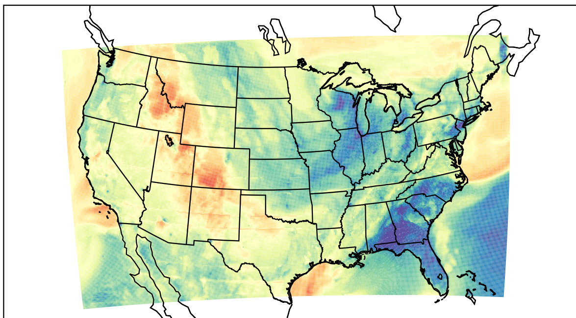
WRF (2022-04-07_02:00:00)
