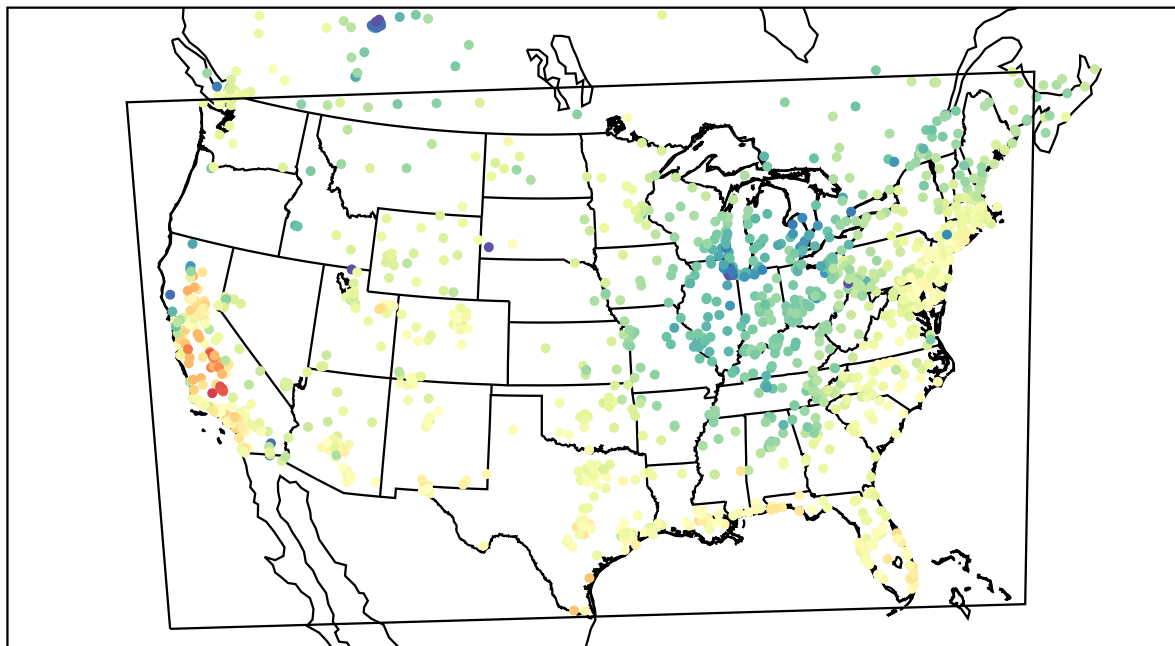
AirNOW (2022-04-08_19:00:00)
