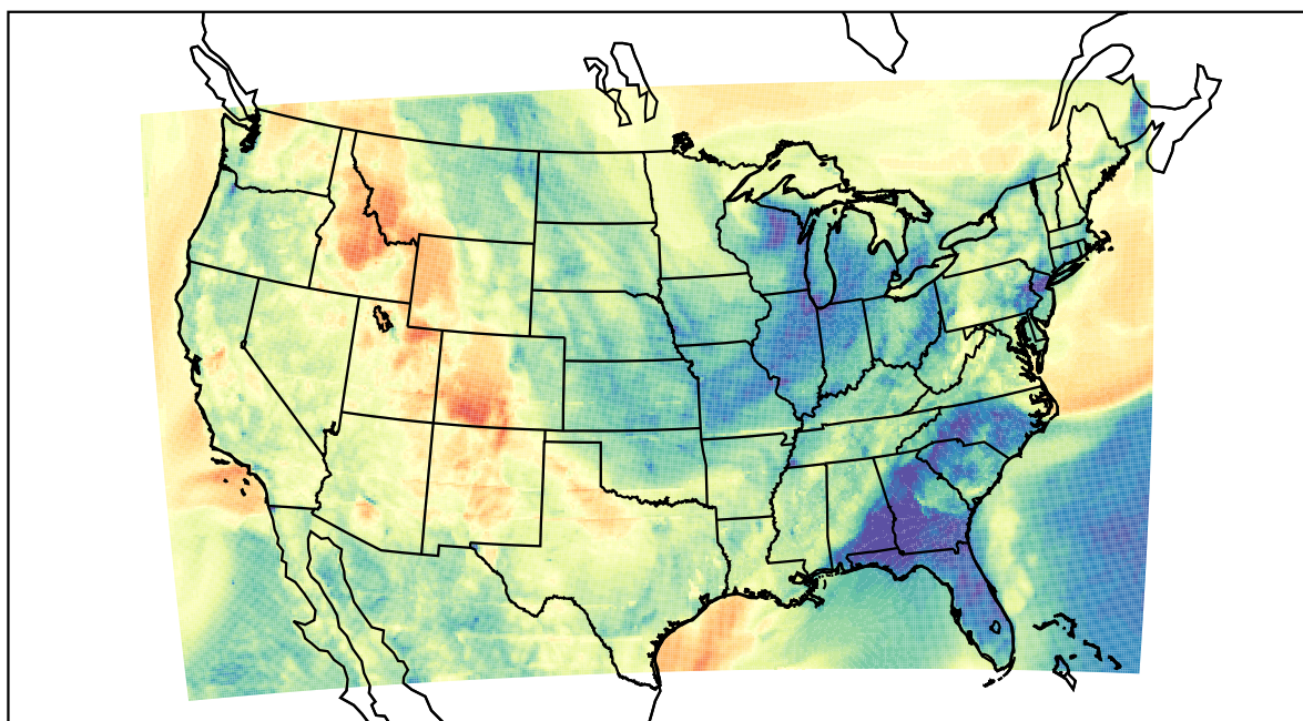
WRF (2022-04-07_03:00:00)
