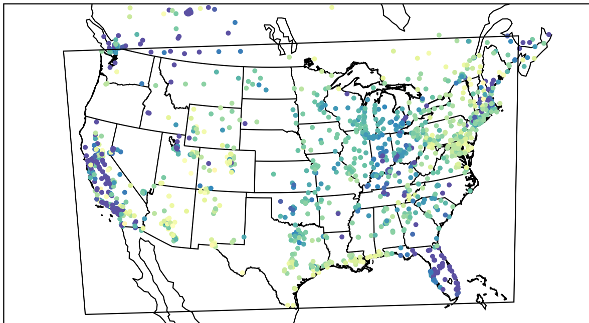
AirNOW (2022-04-07_08:00:00)
