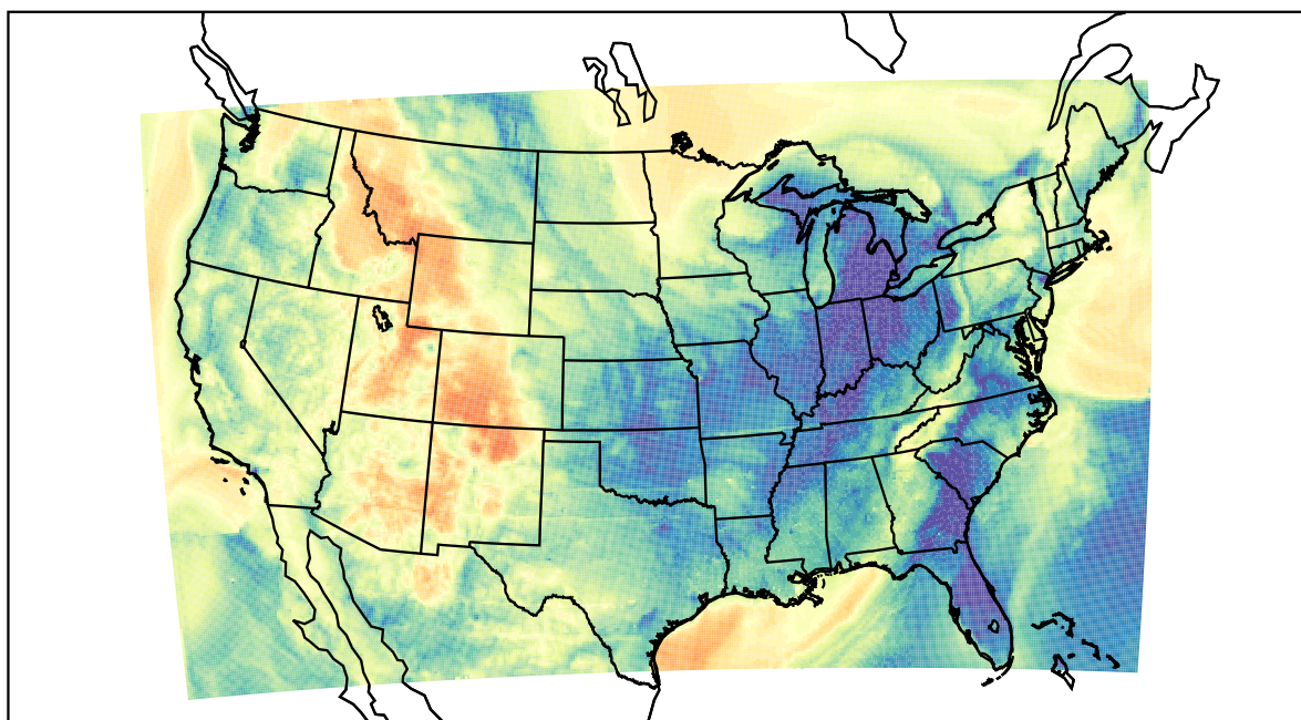
WRF (2022-04-07_11:00:00)
