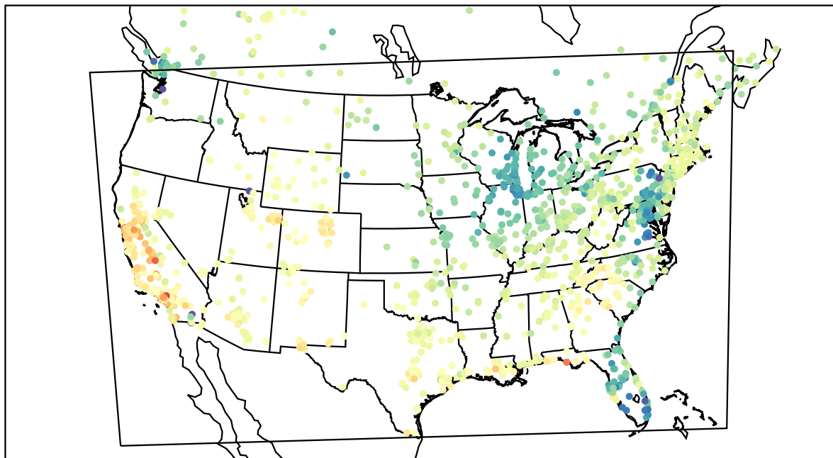
AirNOW (2022-04-07_20:00:00)
