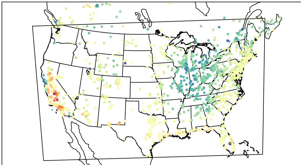
AirNOW (2022-04-08_22:00:00)
