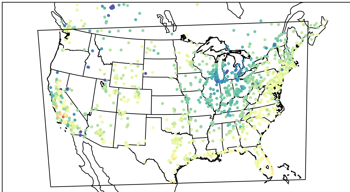
AirNOW (2022-04-08_17:00:00)
