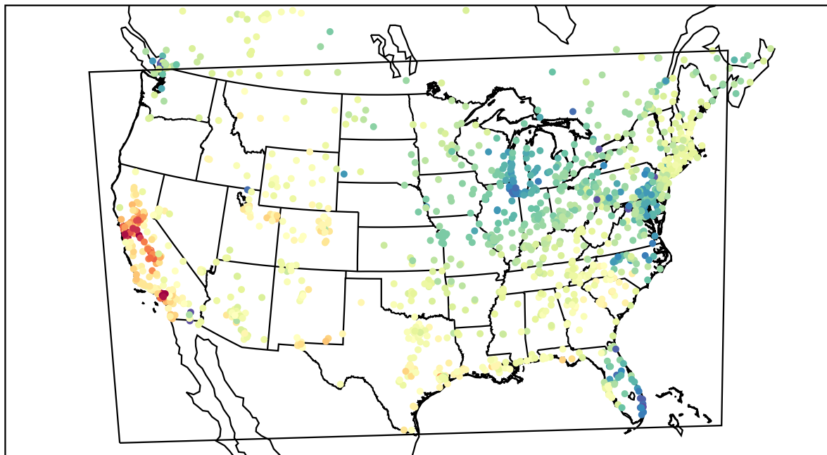
AirNOW (2022-04-07_23:00:00)
