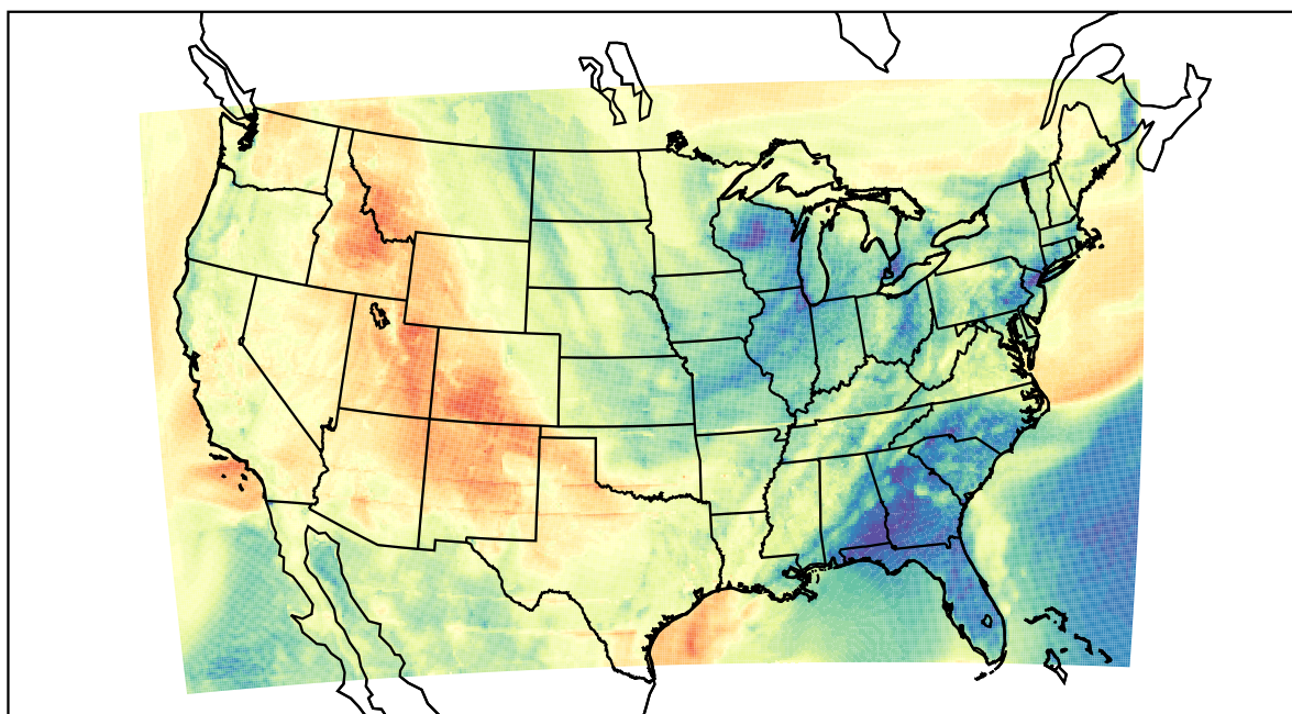
WRF (2022-04-07_01:00:00)
