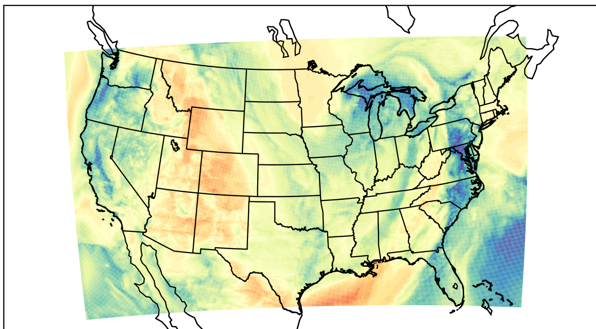
WRF (2022-04-07_16:00:00)
