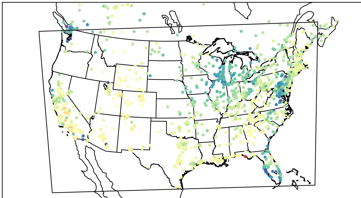
AirNOW (2022-04-07_18:00:00)
