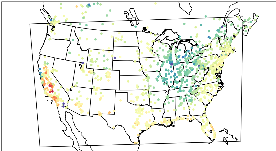
AirNOW (2022-04-08_21:00:00)
