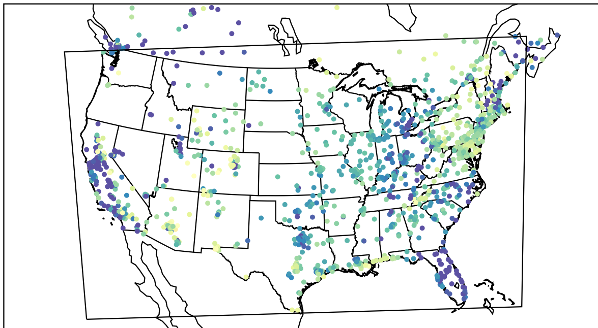
AirNOW (2022-04-07_10:00:00)
