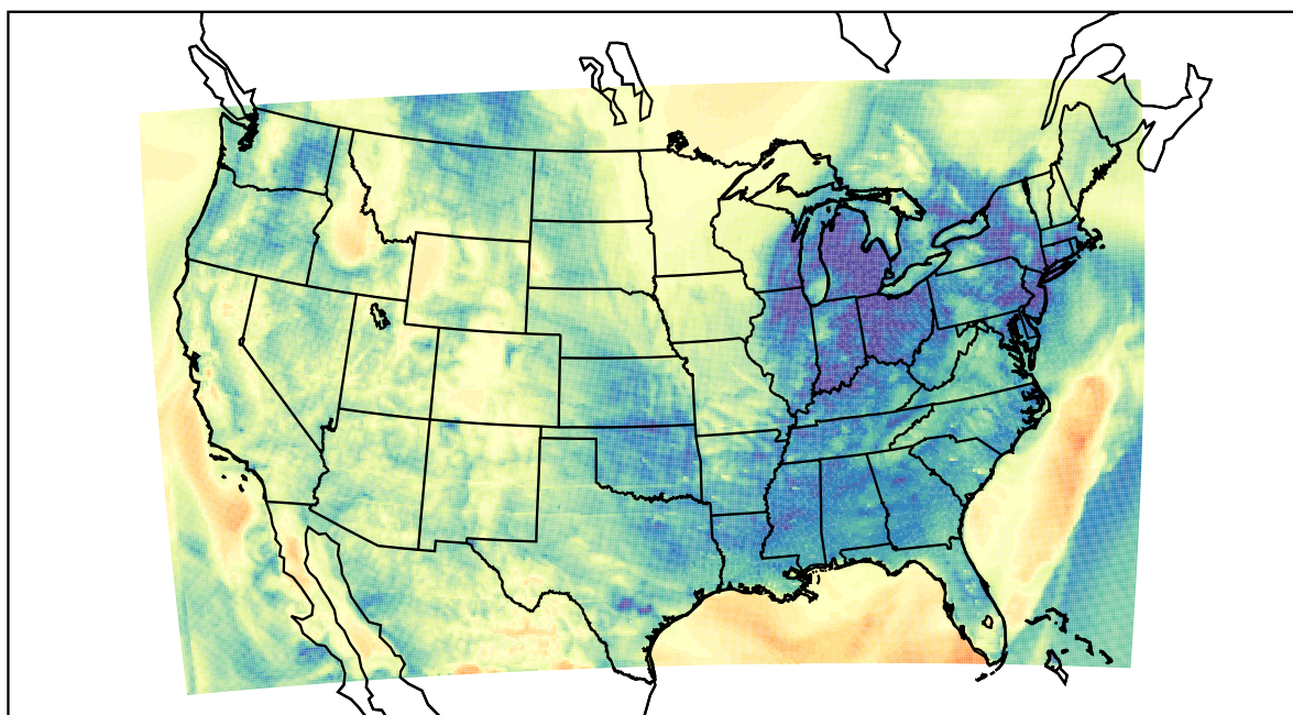
WRF (2022-04-08_11:00:00)
