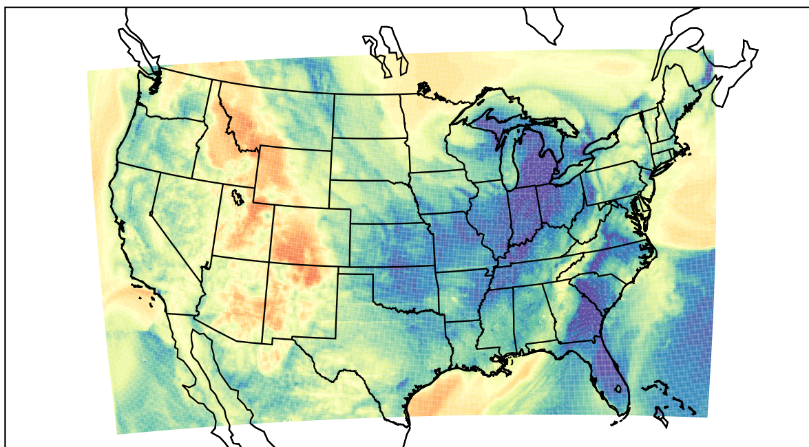
WRF (2022-04-07_10:00:00)
