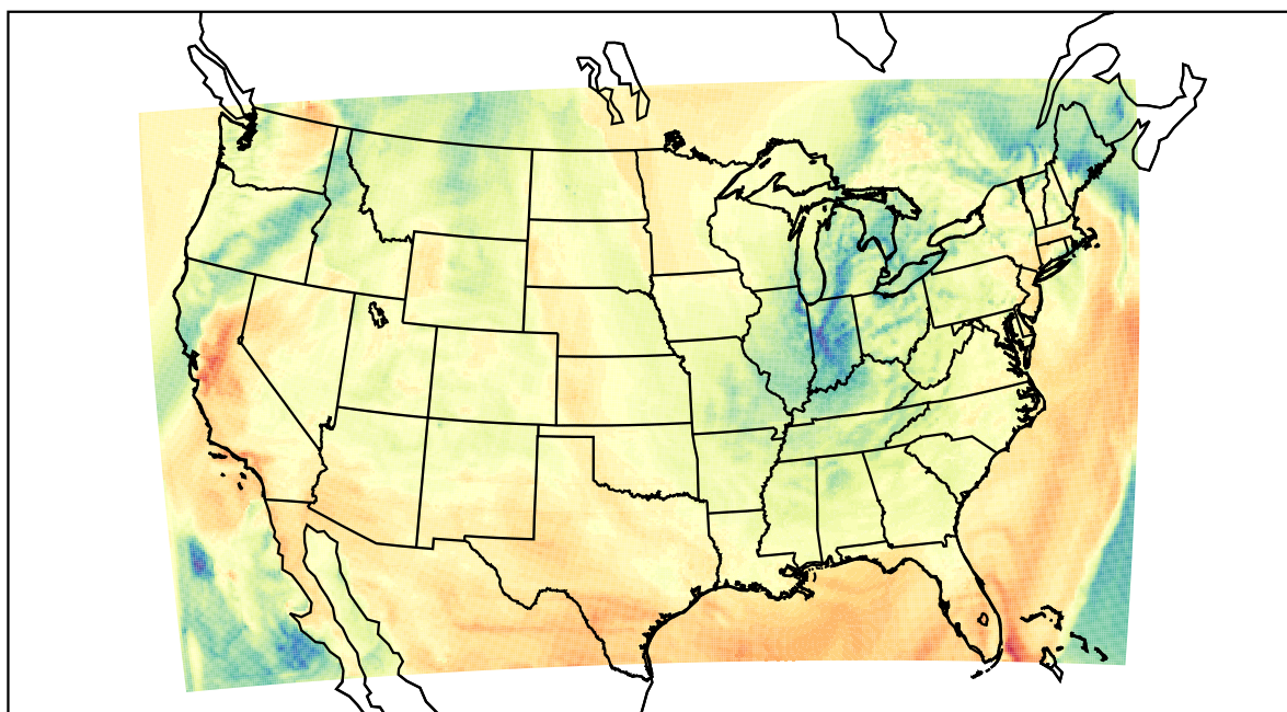
WRF (2022-04-08_21:00:00)
