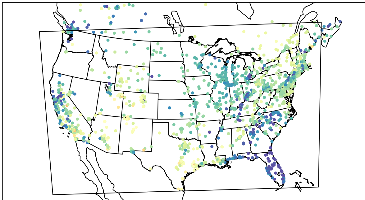
AirNOW (2022-04-07_03:00:00)
