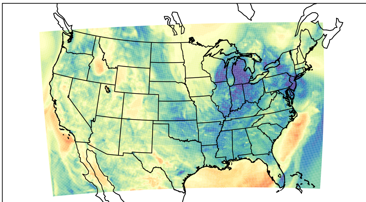
WRF (2022-04-08_07:00:00)
