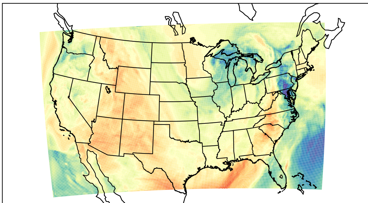
WRF (2022-04-07_19:00:00)
