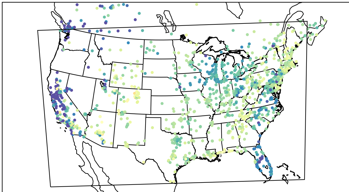
AirNOW (2022-04-07_15:00:00)
