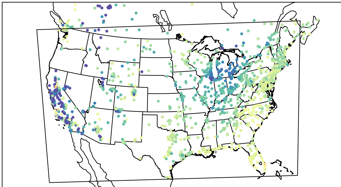
AirNOW (2022-04-08_15:00:00)
