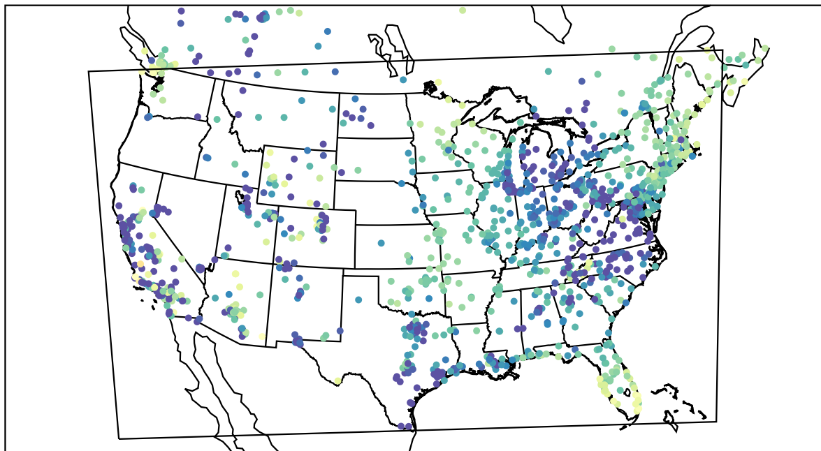
AirNOW (2022-04-08_12:00:00)
