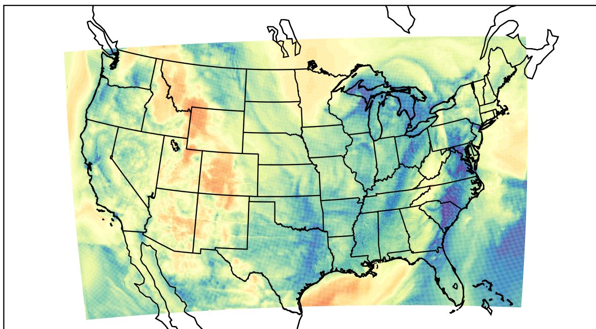
WRF (2022-04-07_14:00:00)
