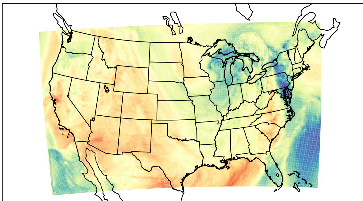
WRF (2022-04-07_22:00:00)
