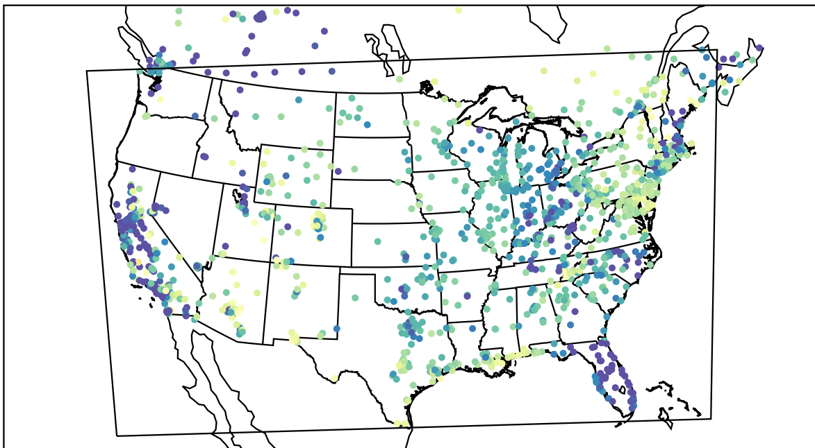
AirNOW (2022-04-07_09:00:00)
