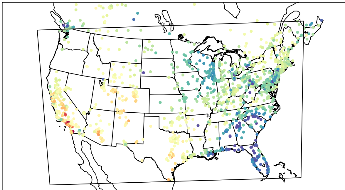
AirNOW (2022-04-07_00:00:00)
