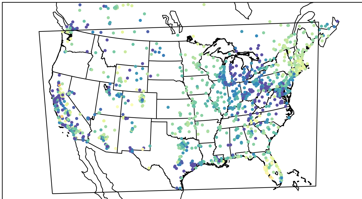
AirNOW (2022-04-08_08:00:00)
