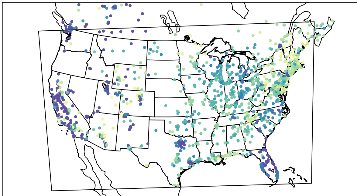
AirNOW (2022-04-07_13:00:00)
