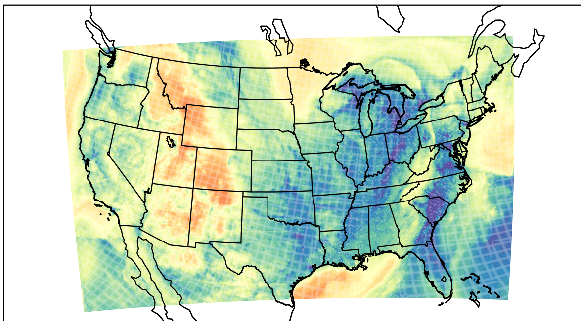
WRF (2022-04-07_13:00:00)
