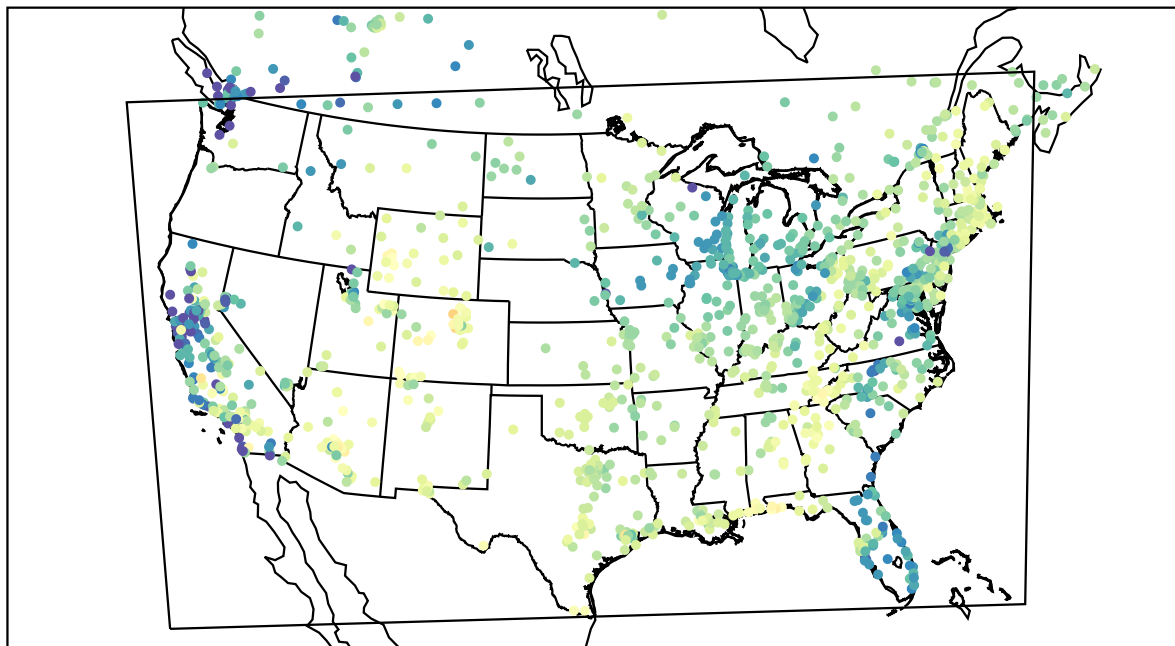
AirNOW (2022-04-07_16:00:00)
