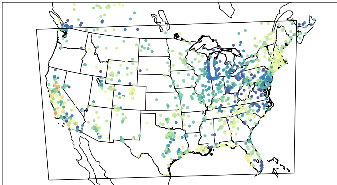
AirNOW (2022-04-08_03:00:00)
