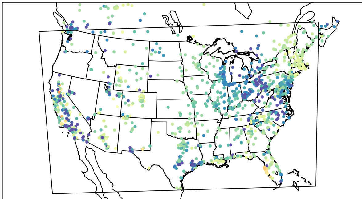
AirNOW (2022-04-08_05:00:00)
