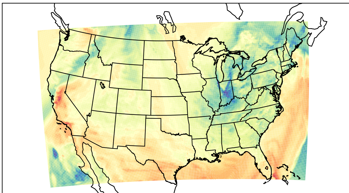
WRF (2022-04-08_23:00:00)
