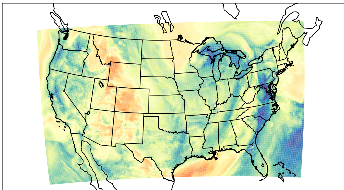
WRF (2022-04-07_15:00:00)
