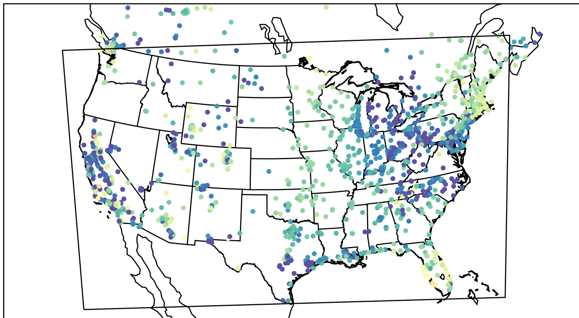
AirNOW (2022-04-08_09:00:00)
