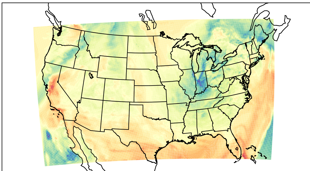
WRF (2022-04-08_22:00:00)
