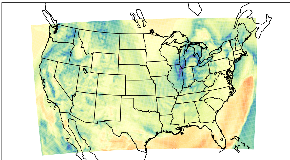
WRF (2022-04-08_16:00:00)
