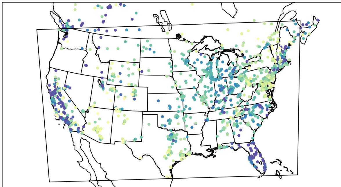
AirNOW (2022-04-07_07:00:00)
