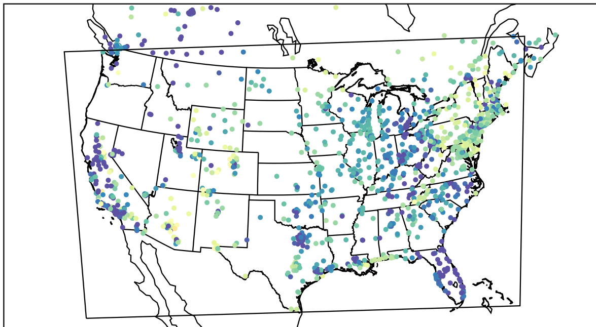
AirNOW (2022-04-07_11:00:00)
