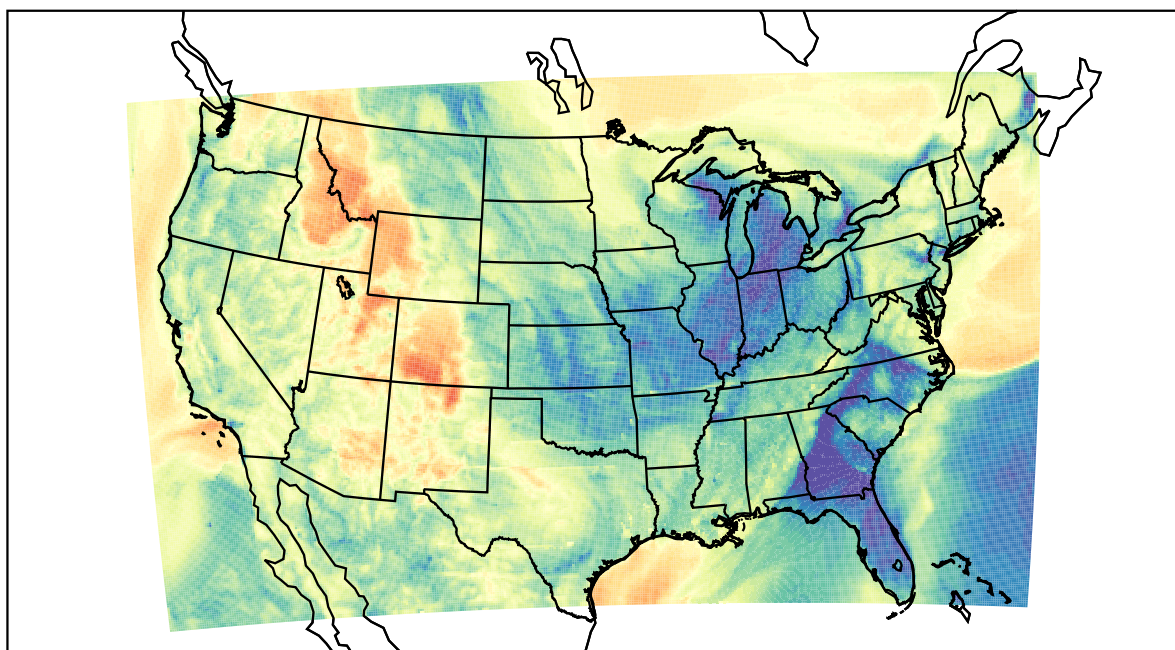
WRF (2022-04-07_06:00:00)
