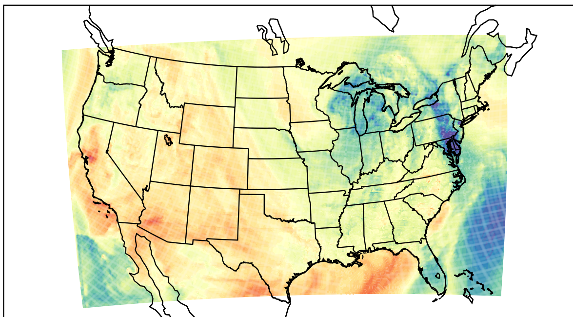
WRF (2022-04-07_23:00:00)
