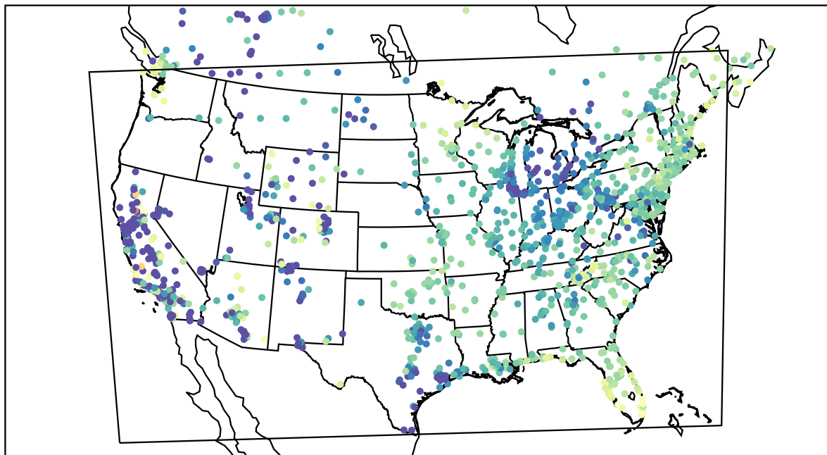
AirNOW (2022-04-08_13:00:00)
