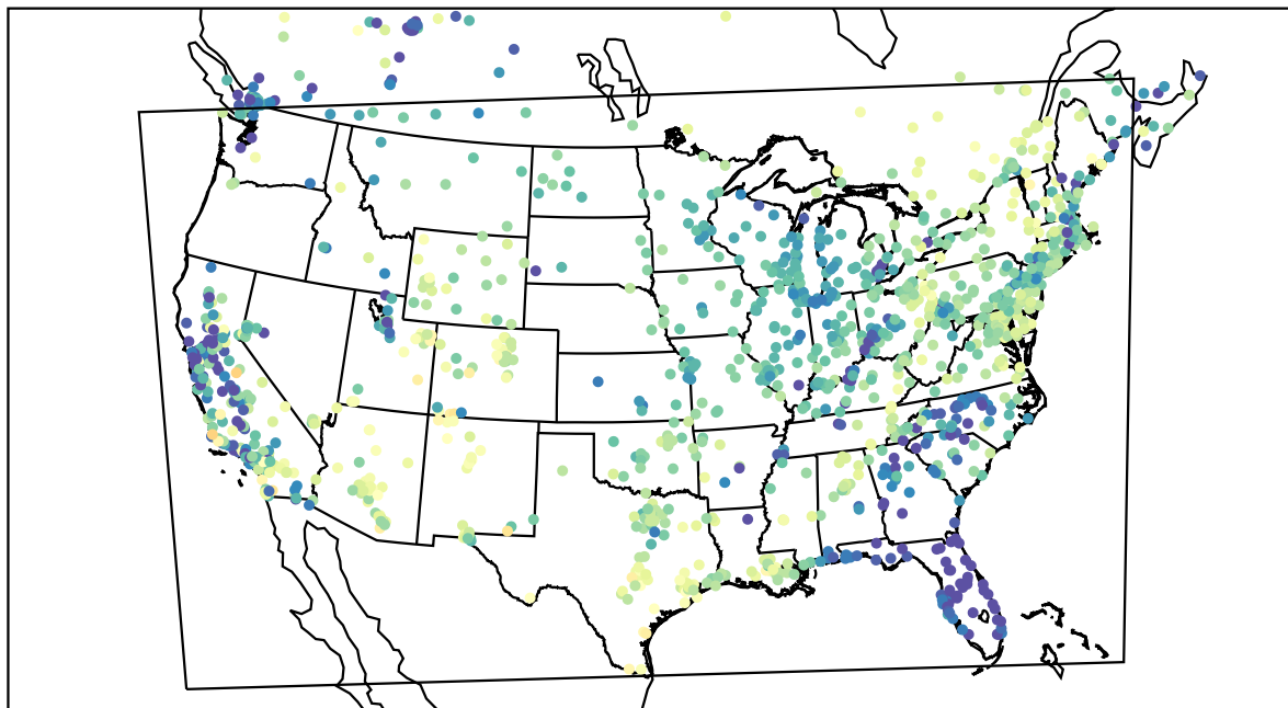
AirNOW (2022-04-07_04:00:00)
