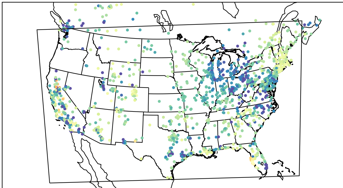
AirNOW (2022-04-08_04:00:00)
