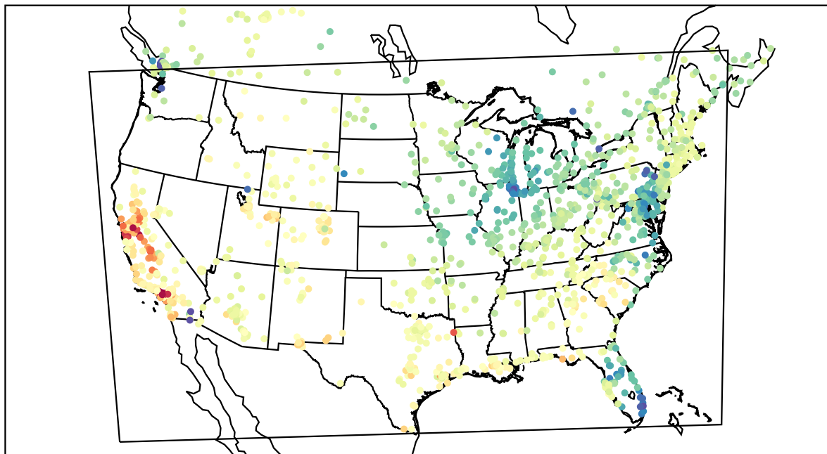
AirNOW (2022-04-07_22:00:00)
