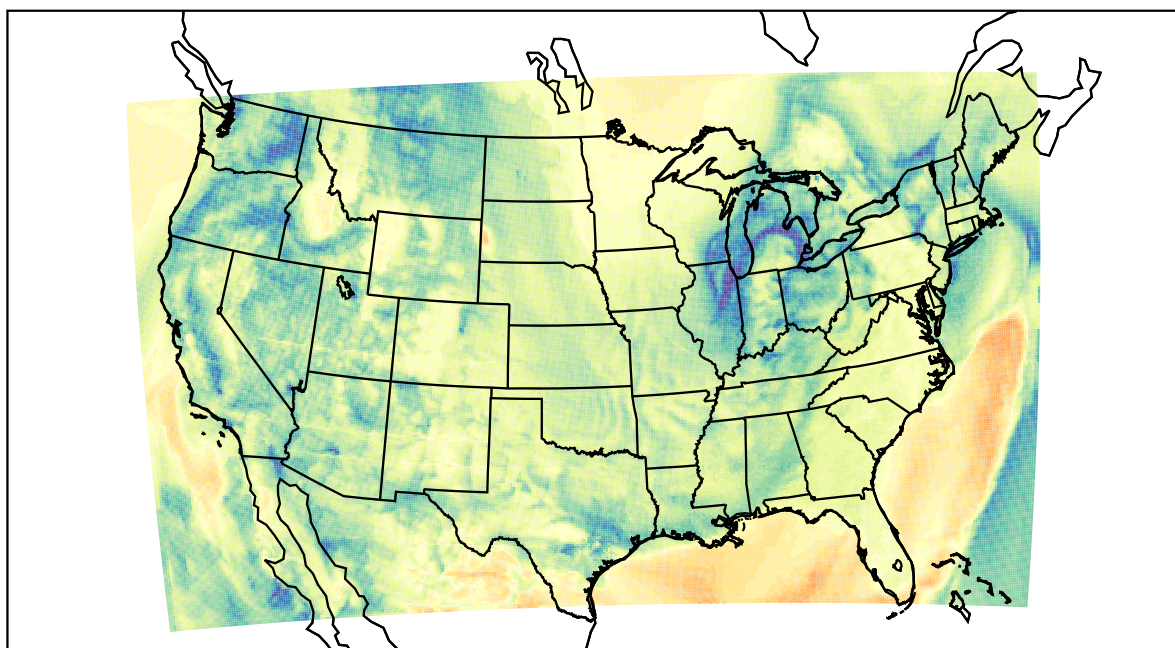
WRF (2022-04-08_15:00:00)
