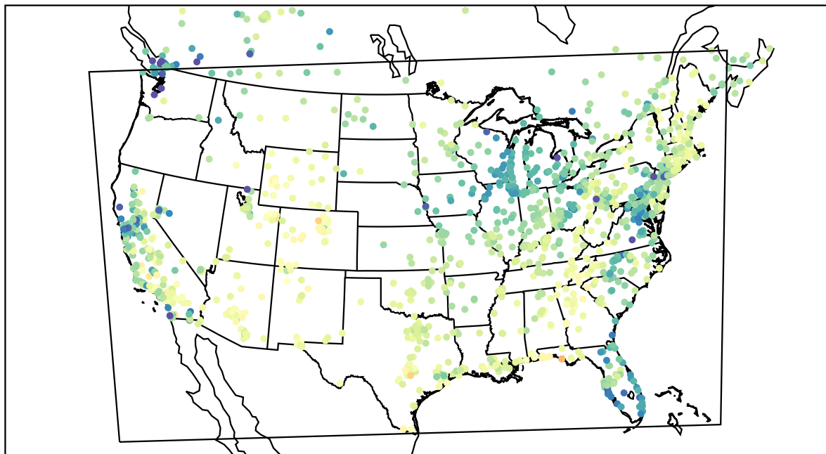
AirNOW (2022-04-07_17:00:00)
