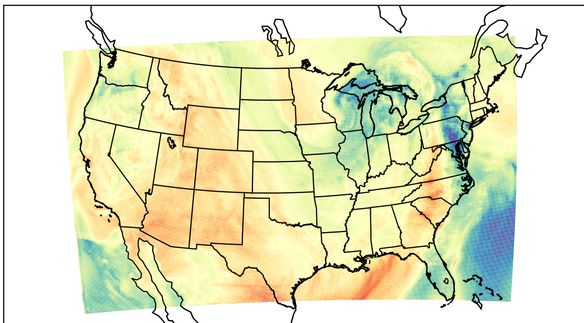
WRF (2022-04-07_20:00:00)
