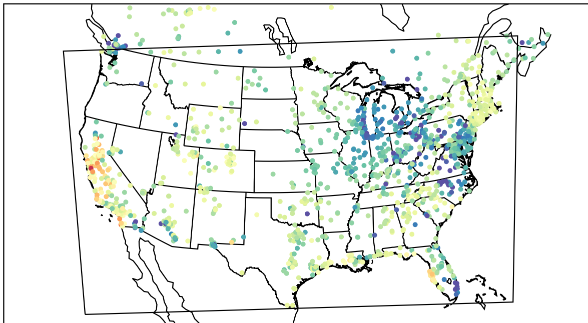
AirNOW (2022-04-08_02:00:00)
