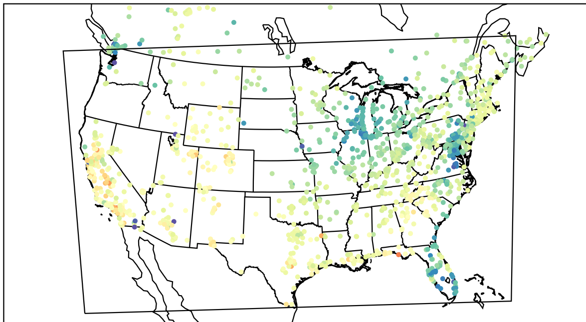
AirNOW (2022-04-07_19:00:00)
