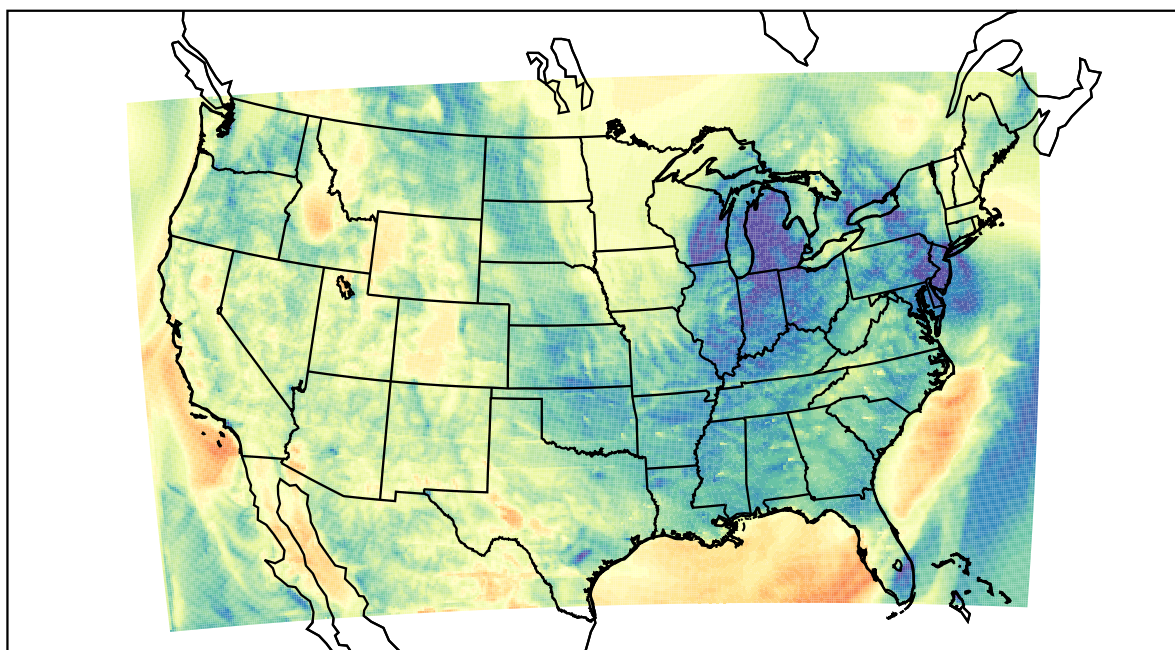
WRF (2022-04-08_06:00:00)
