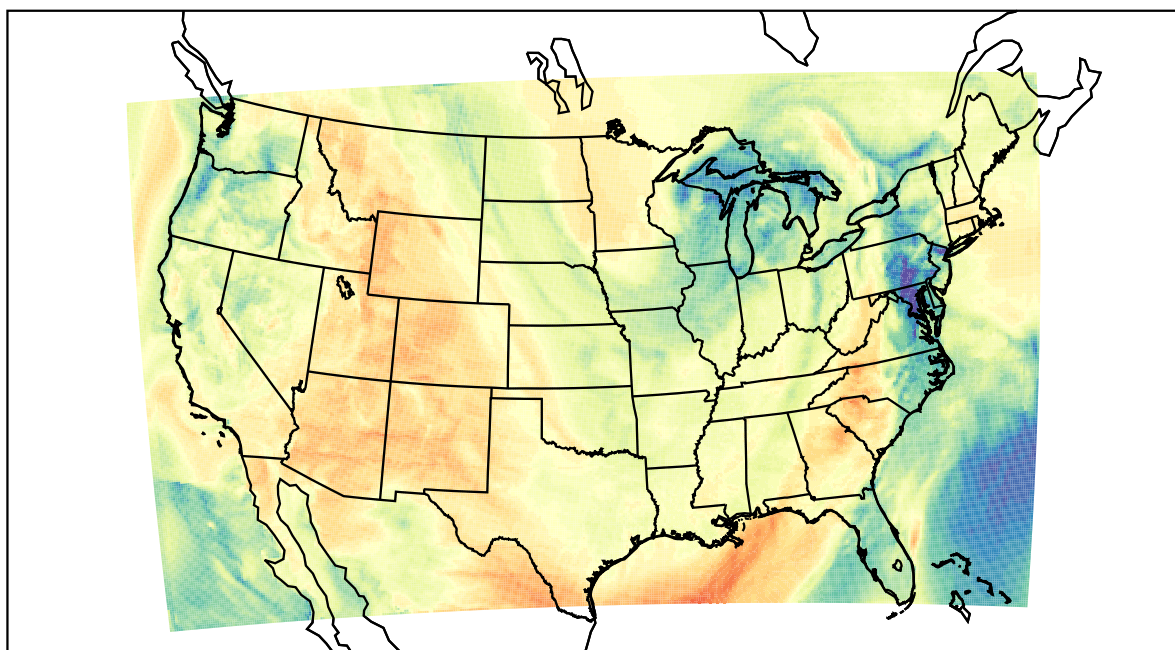
WRF (2022-04-07_18:00:00)
