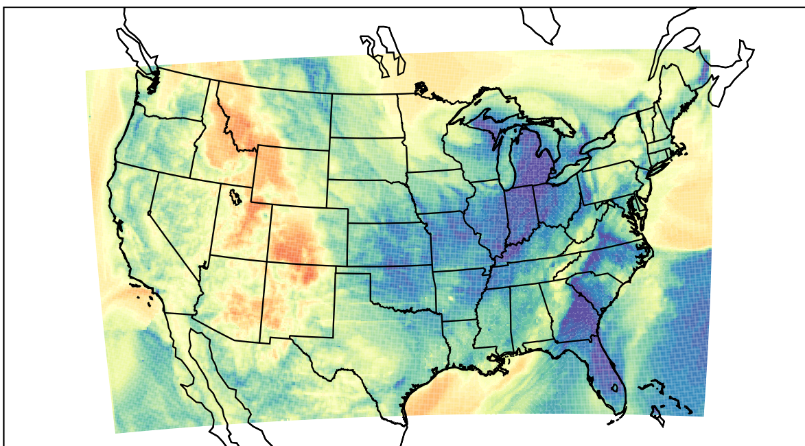
WRF (2022-04-07_09:00:00)
