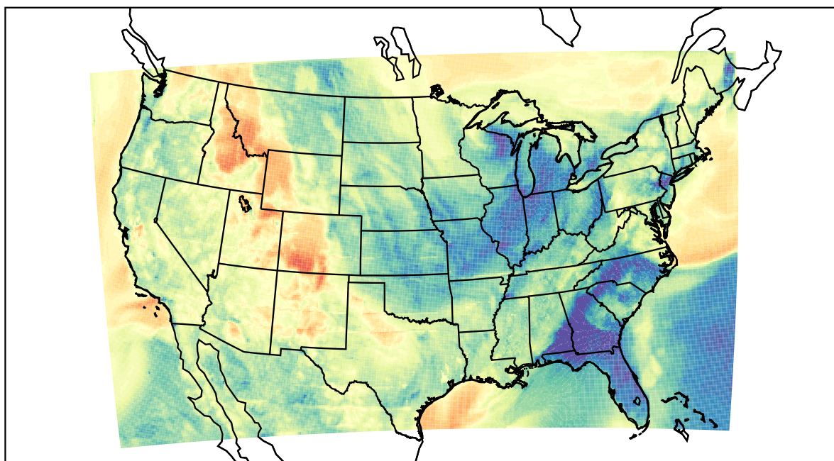
WRF (2022-04-07_04:00:00)
