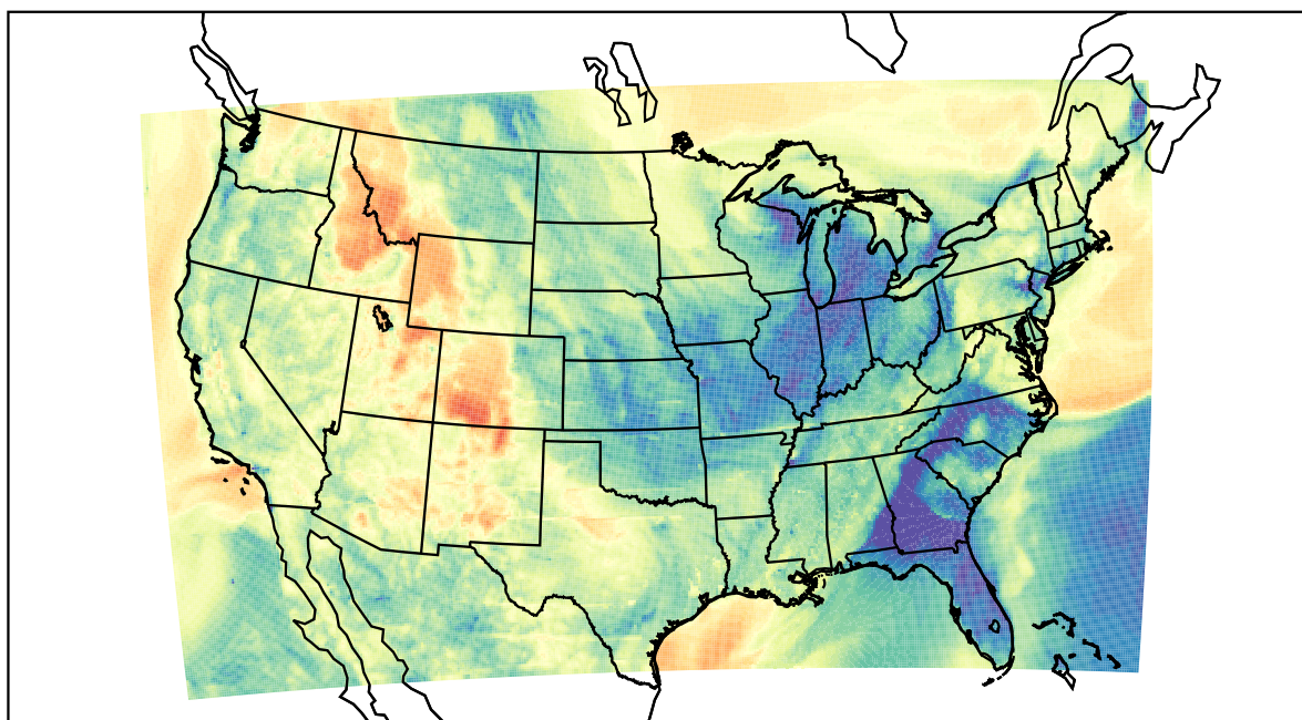
WRF (2022-04-07_05:00:00)
