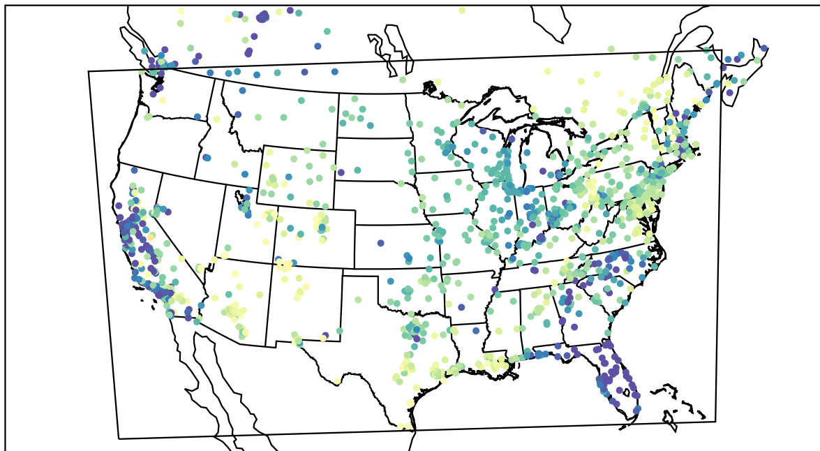
AirNOW (2022-04-07_05:00:00)
