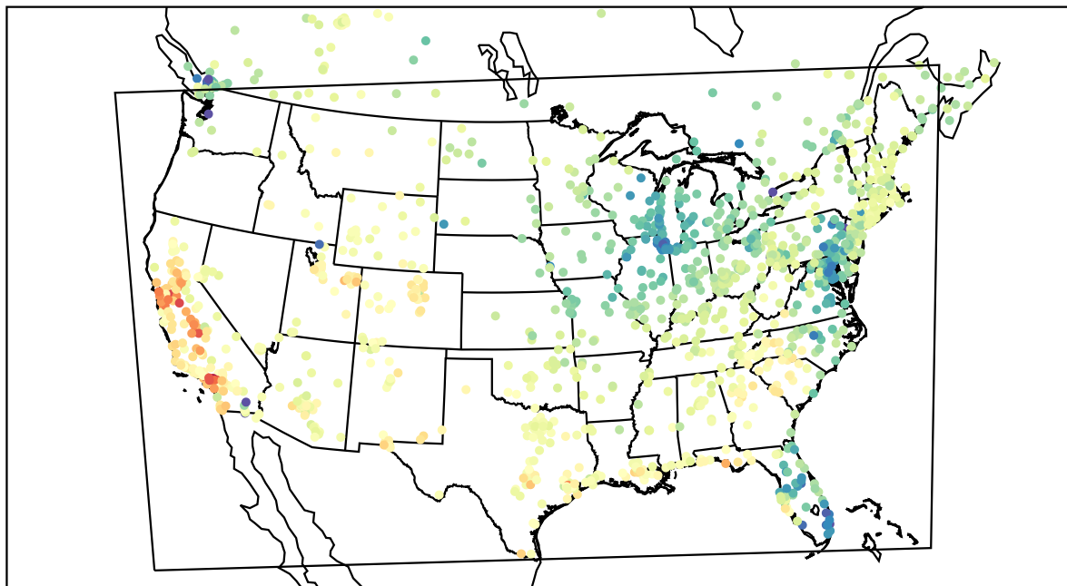
AirNOW (2022-04-07_21:00:00)
