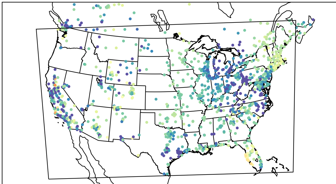
AirNOW (2022-04-08_07:00:00)
