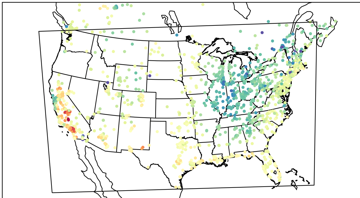
AirNOW (2022-04-08_23:00:00)
