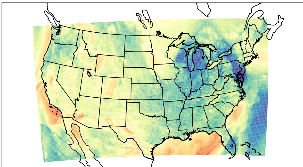
WRF (2022-04-08_02:00:00)
