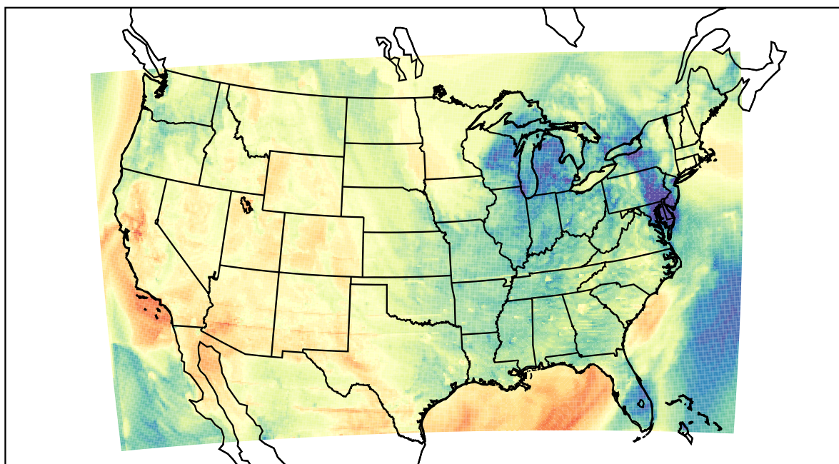
WRF (2022-04-08_01:00:00)
