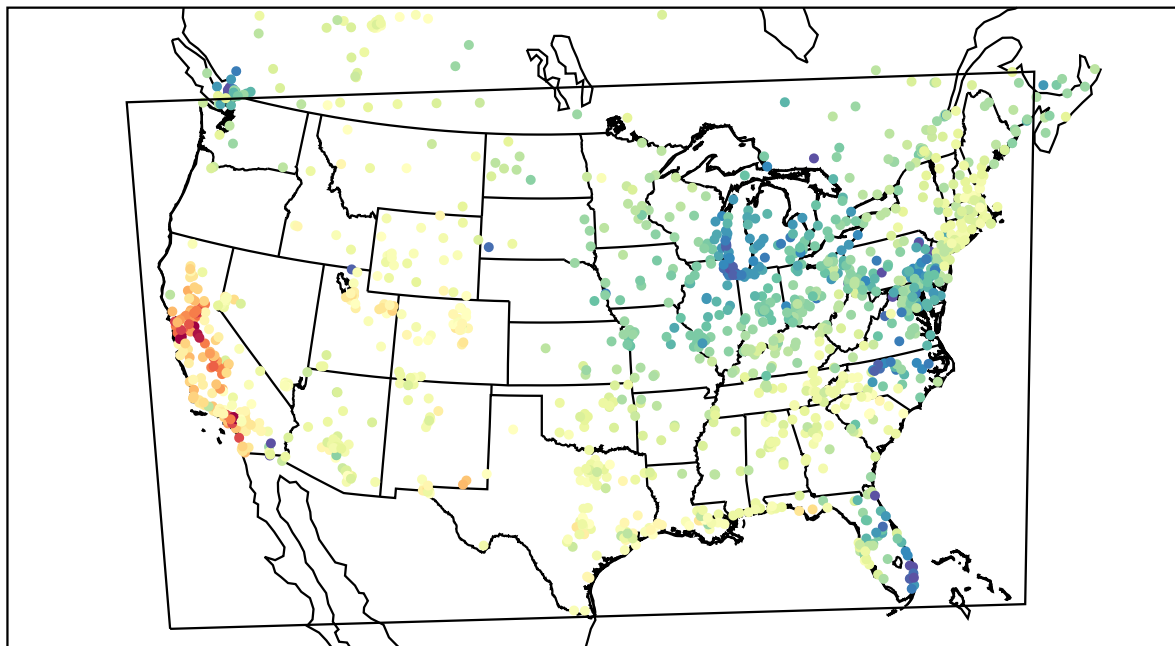
AirNOW (2022-04-08_00:00:00)
