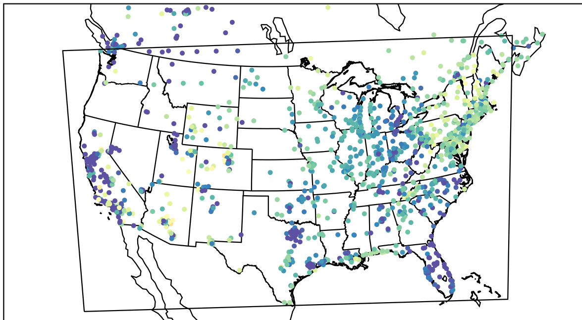
AirNOW (2022-04-07_12:00:00)
