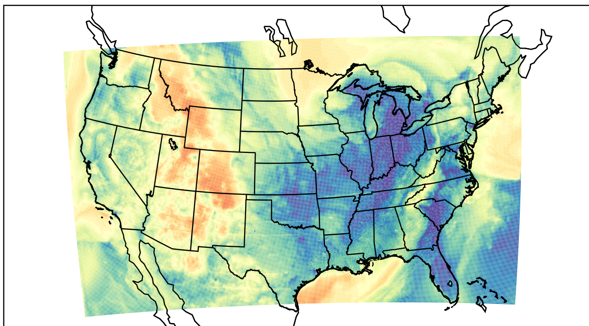
WRF (2022-04-07_12:00:00)
