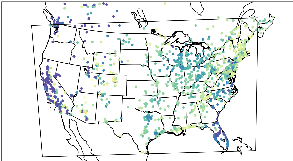
AirNOW (2022-04-07_14:00:00)
