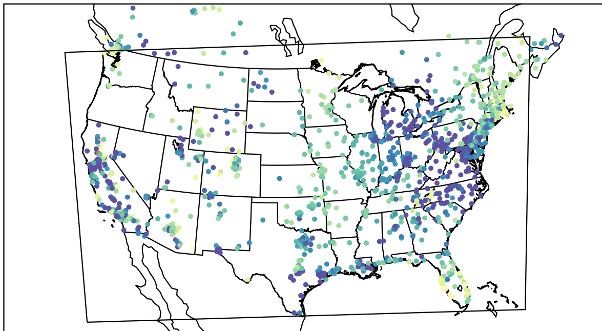
AirNOW (2022-04-08_10:00:00)
