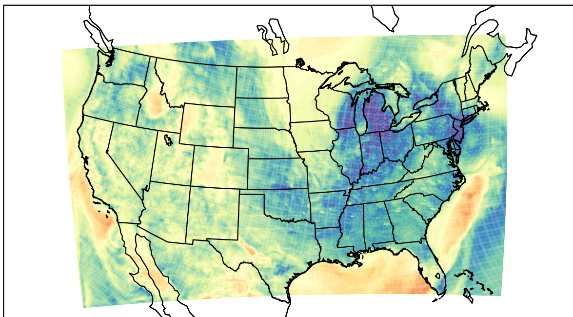
WRF (2022-04-08_08:00:00)
