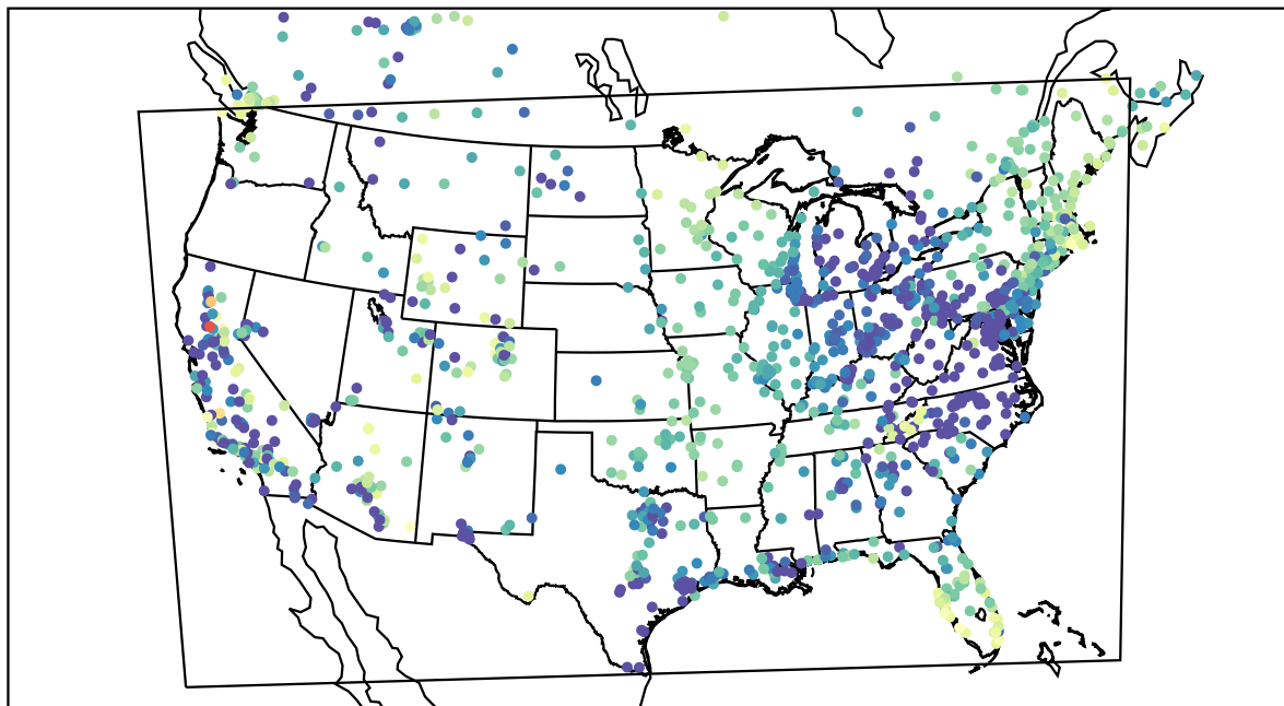
AirNOW (2022-04-08_11:00:00)
