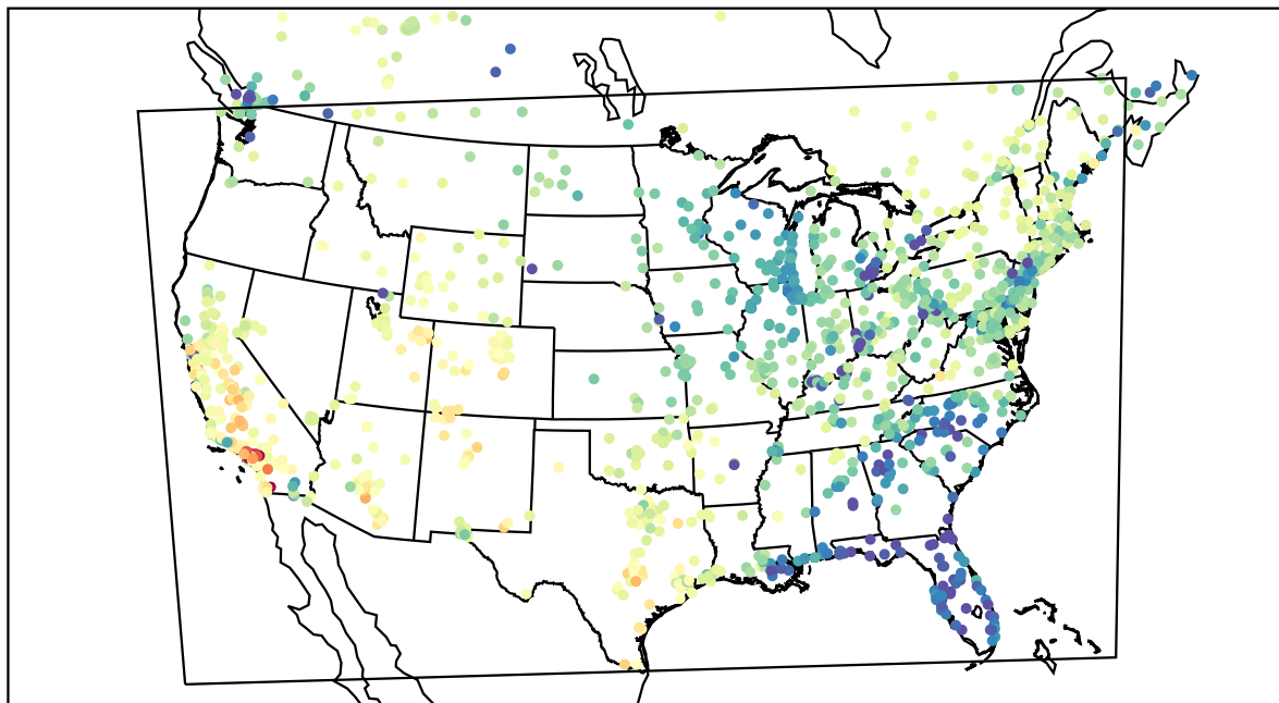
AirNOW (2022-04-07_01:00:00)
