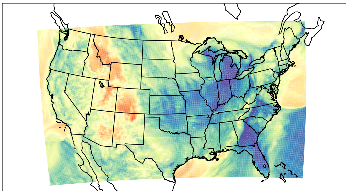
WRF (2022-04-07_08:00:00)
