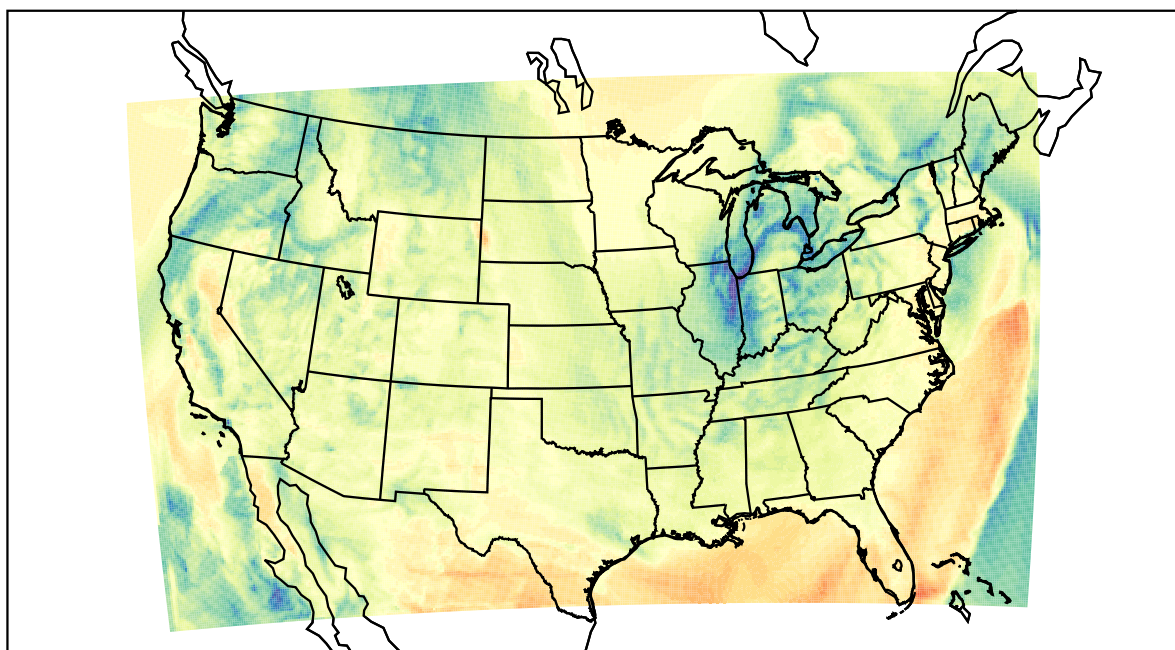
WRF (2022-04-08_17:00:00)
