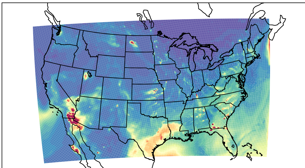
WRF 2022-04-17_02:00:00
