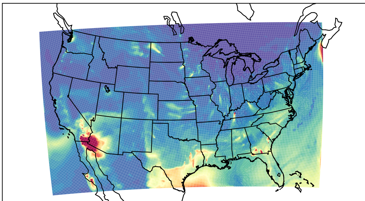
WRF 2022-04-17_06:00:00
