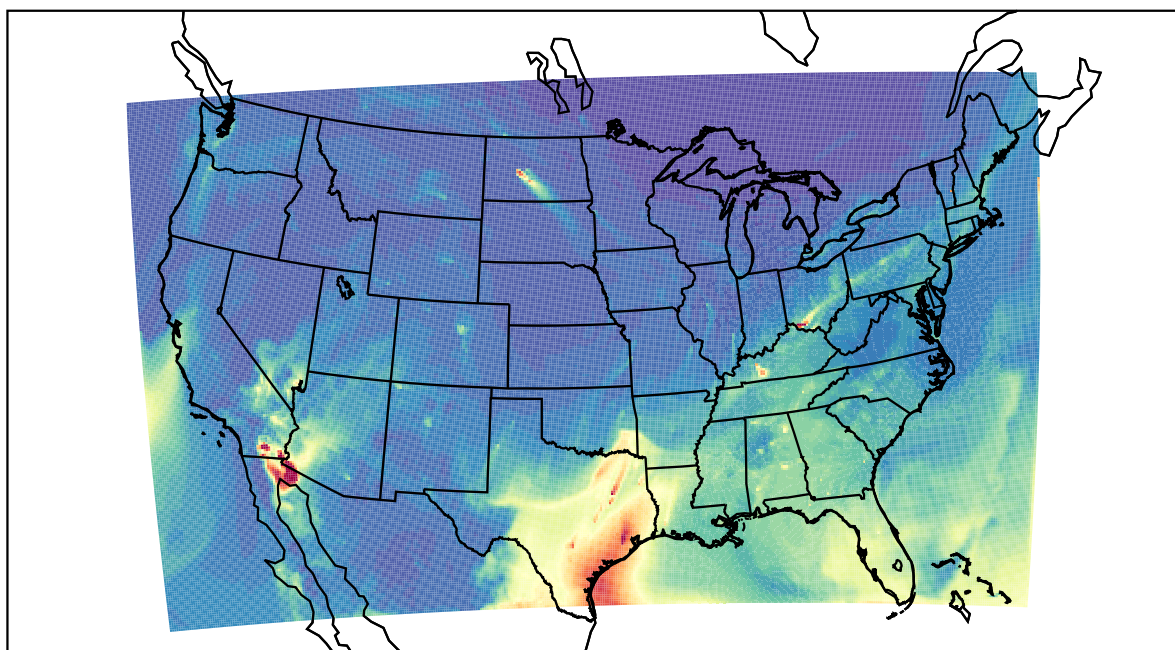
WRF 2022-04-16_16:00:00
