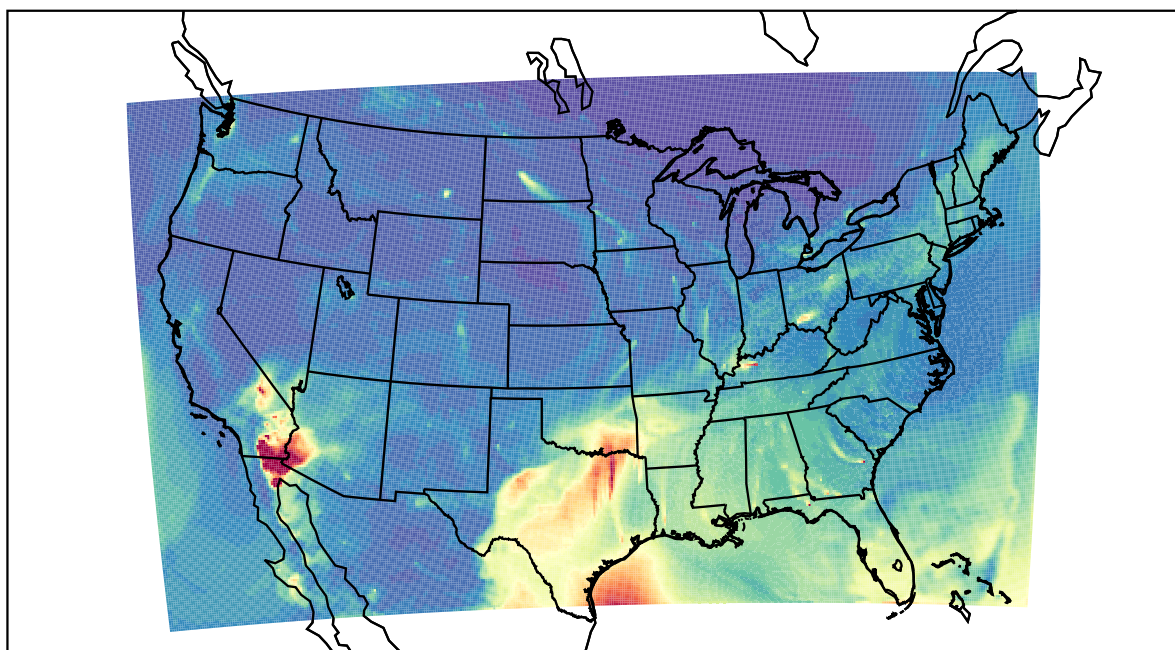
WRF 2022-04-16_08:00:00
