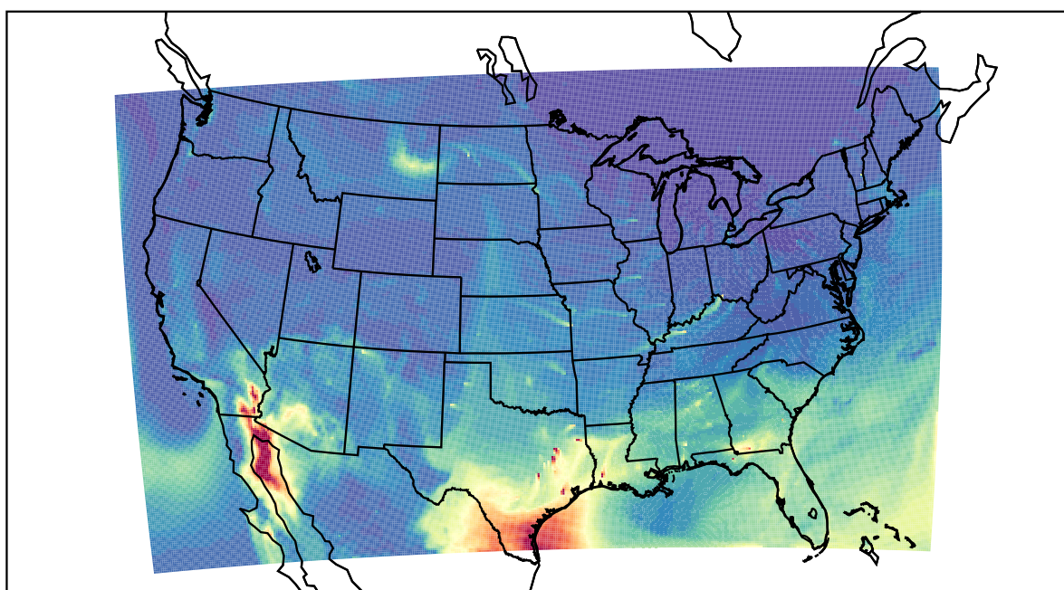
WRF 2022-04-17_16:00:00
