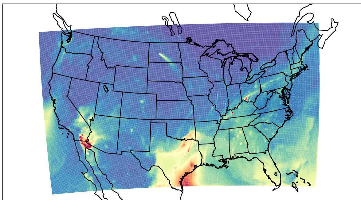
WRF 2022-04-16_14:00:00
