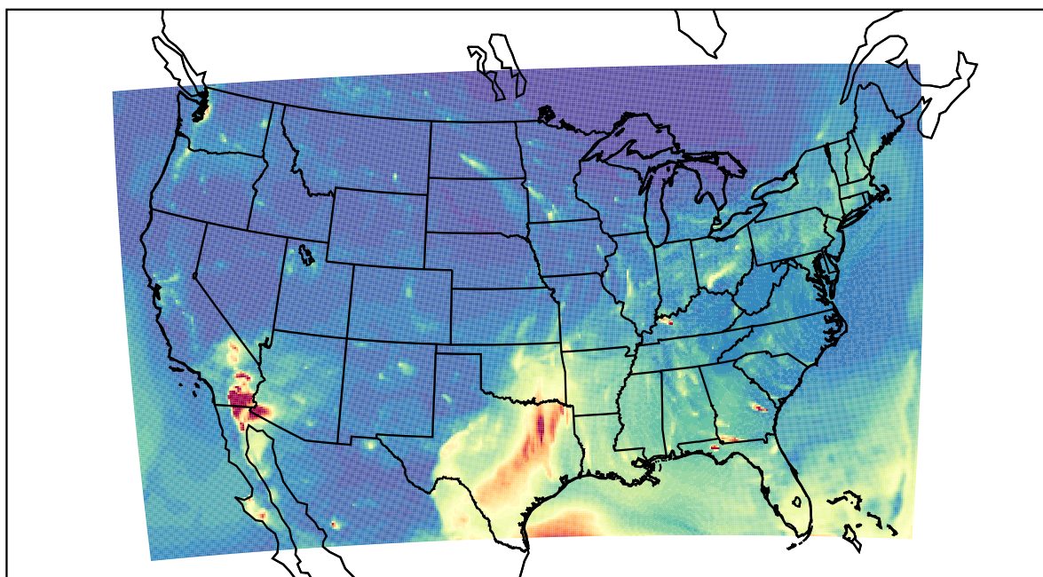
WRF 2022-04-16_04:00:00
