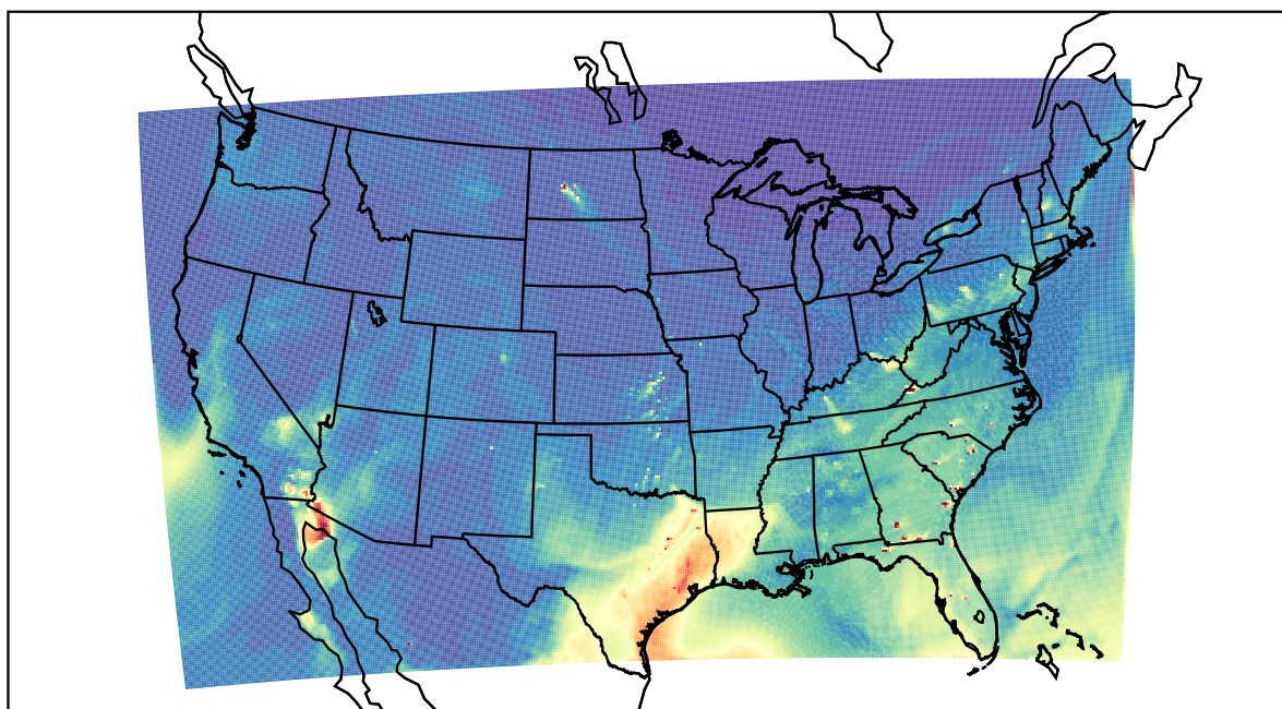
WRF 2022-04-16_21:00:00
