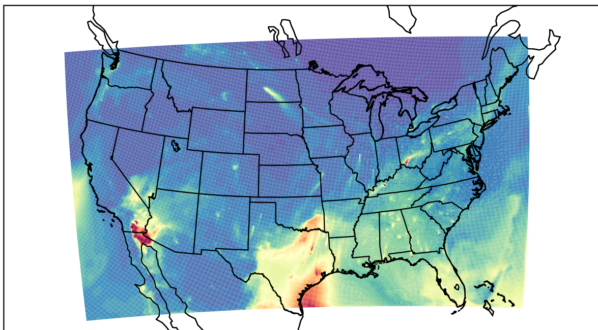
WRF 2022-04-16_13:00:00
