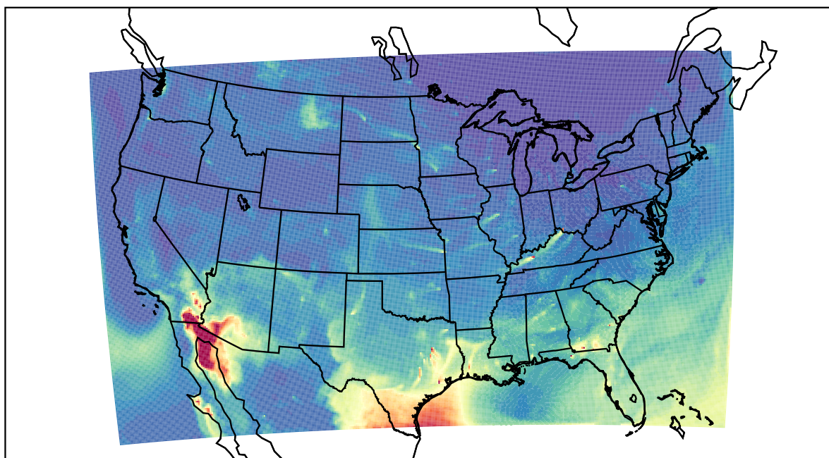
WRF 2022-04-17_13:00:00
