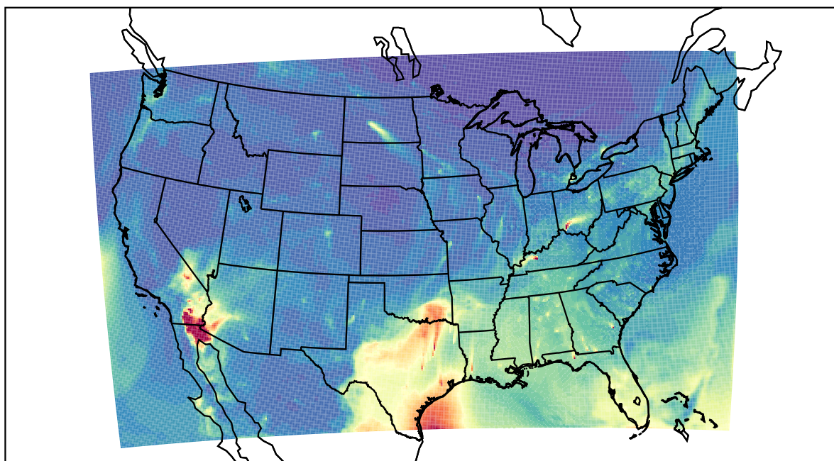
WRF 2022-04-16_11:00:00
