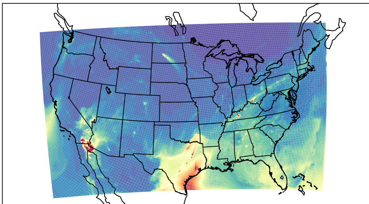
WRF 2022-04-16_15:00:00
