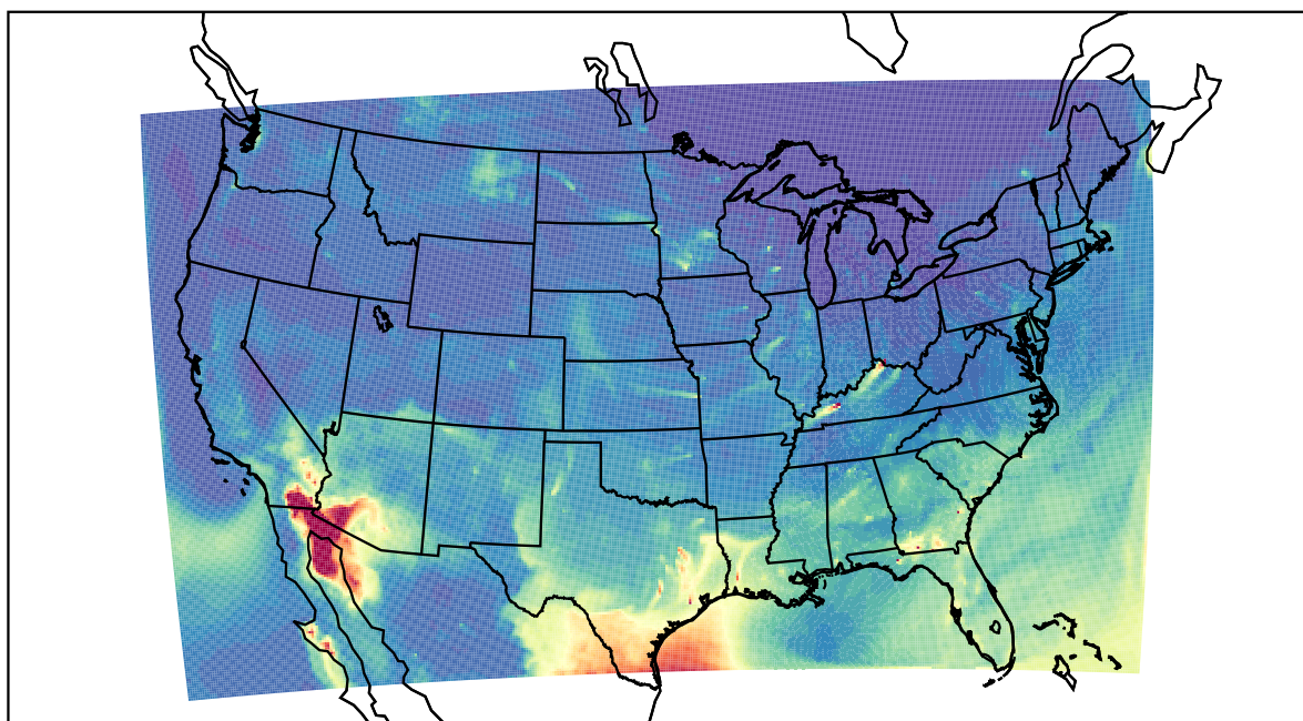
WRF 2022-04-17_12:00:00
