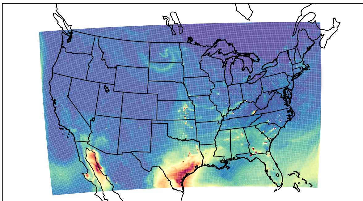
WRF 2022-04-17_23:00:00
