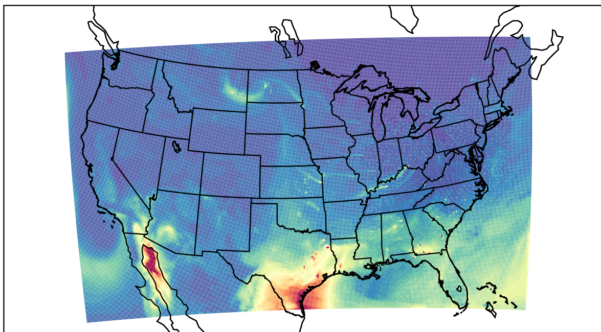
WRF 2022-04-17_18:00:00
