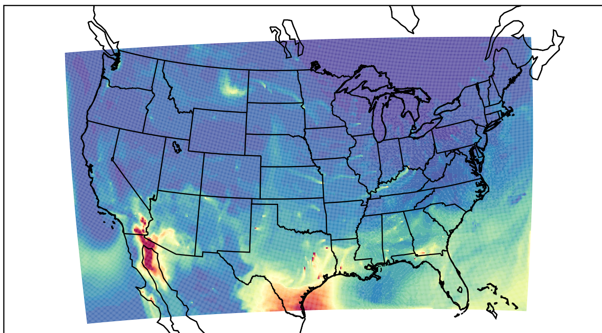
WRF 2022-04-17_15:00:00
