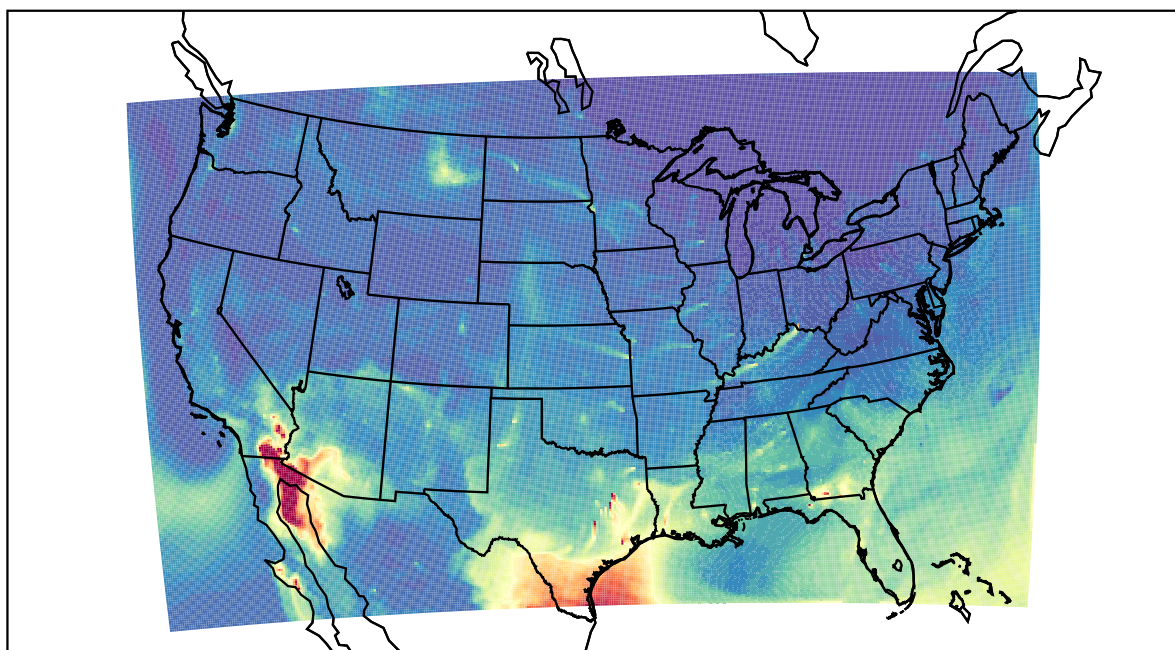
WRF 2022-04-17_14:00:00
