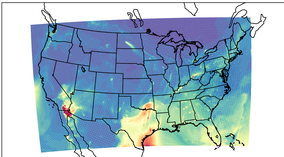
WRF 2022-04-16_12:00:00
