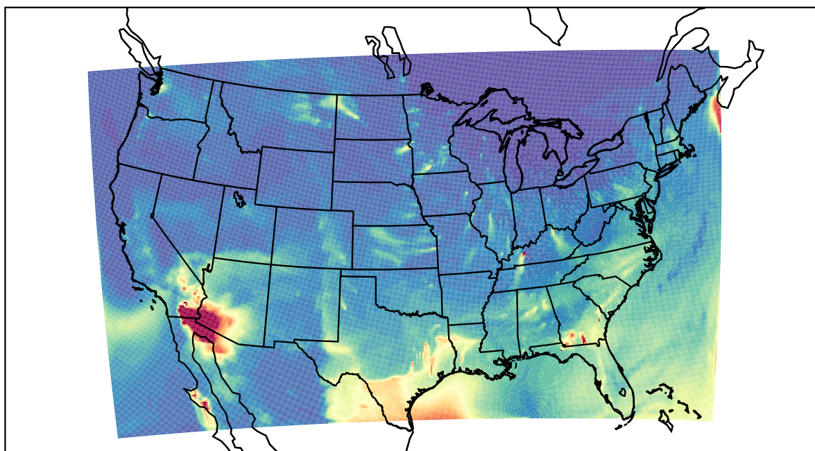
WRF 2022-04-17_07:00:00
