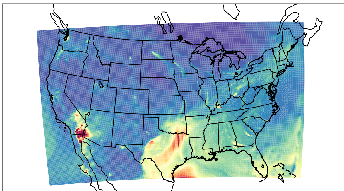
WRF 2022-04-16_06:00:00
