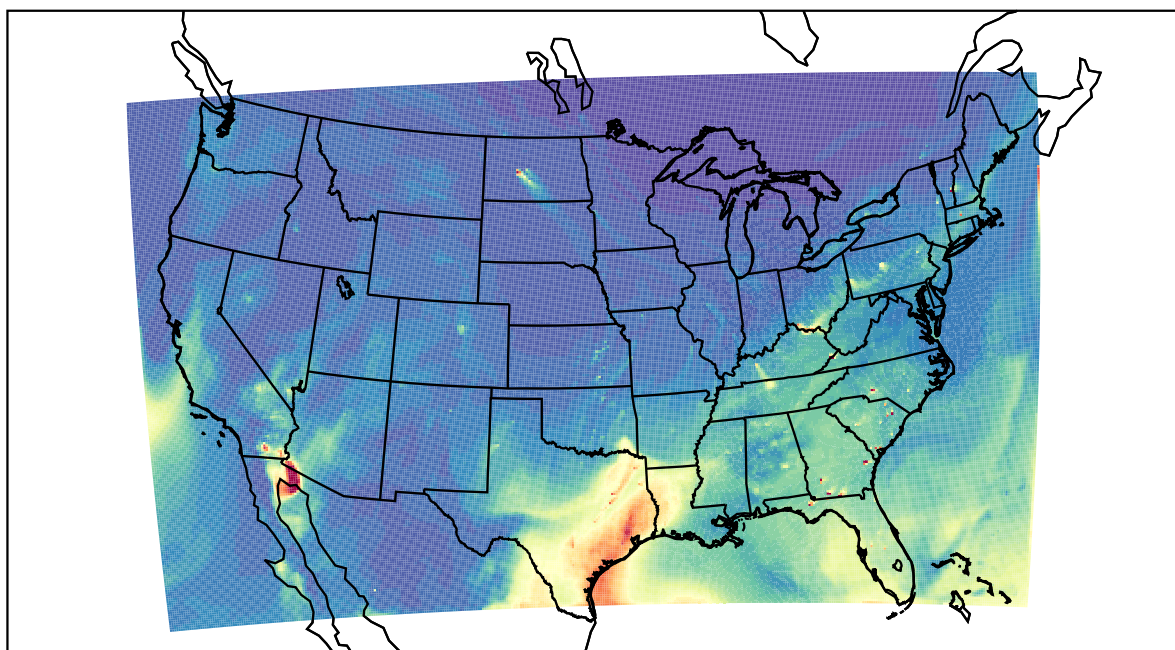
WRF 2022-04-16_19:00:00
