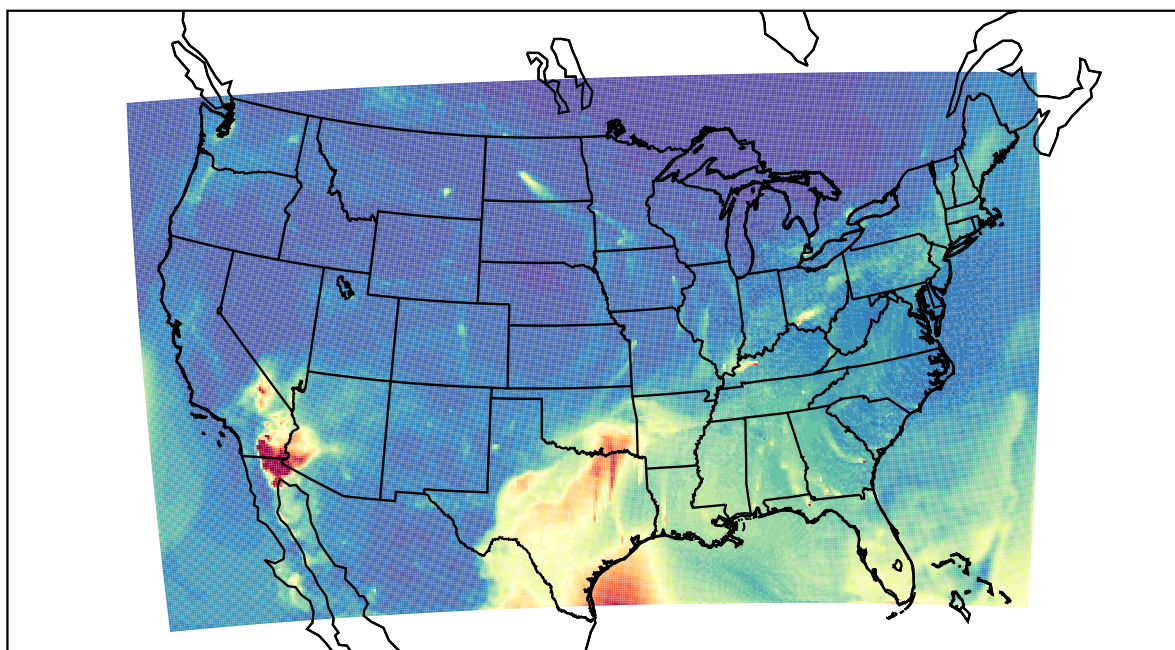
WRF 2022-04-16_09:00:00
