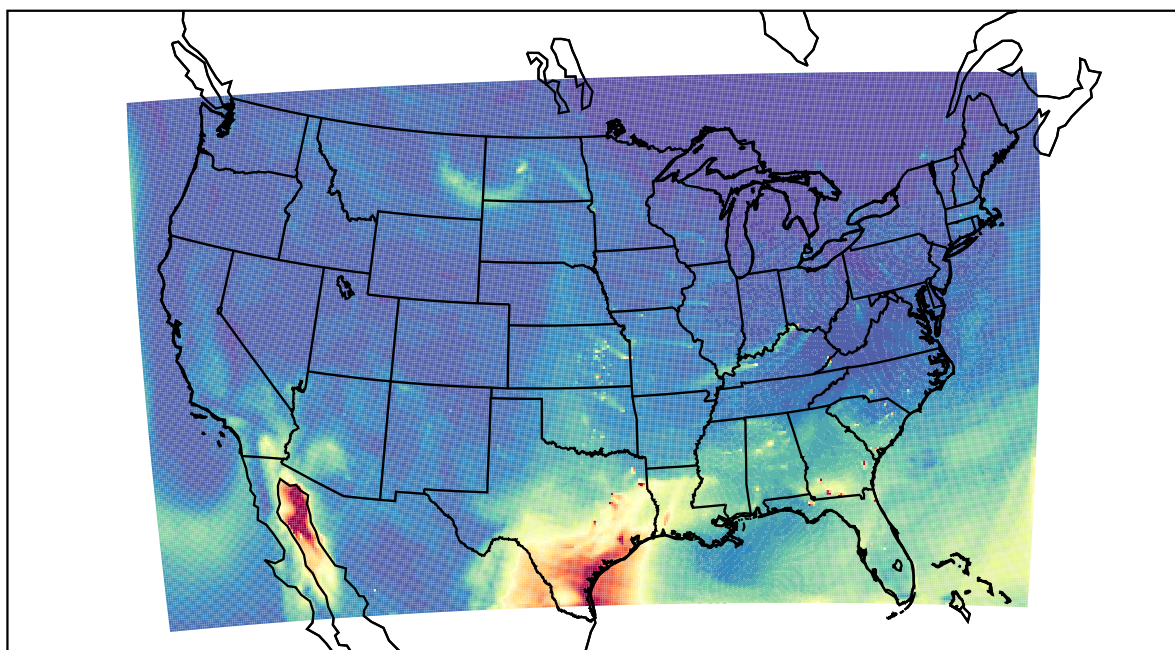
WRF 2022-04-17_19:00:00
