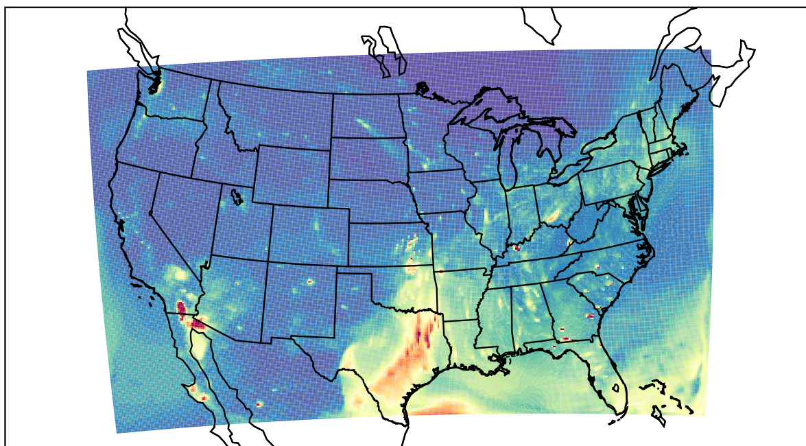
WRF 2022-04-16_02:00:00
