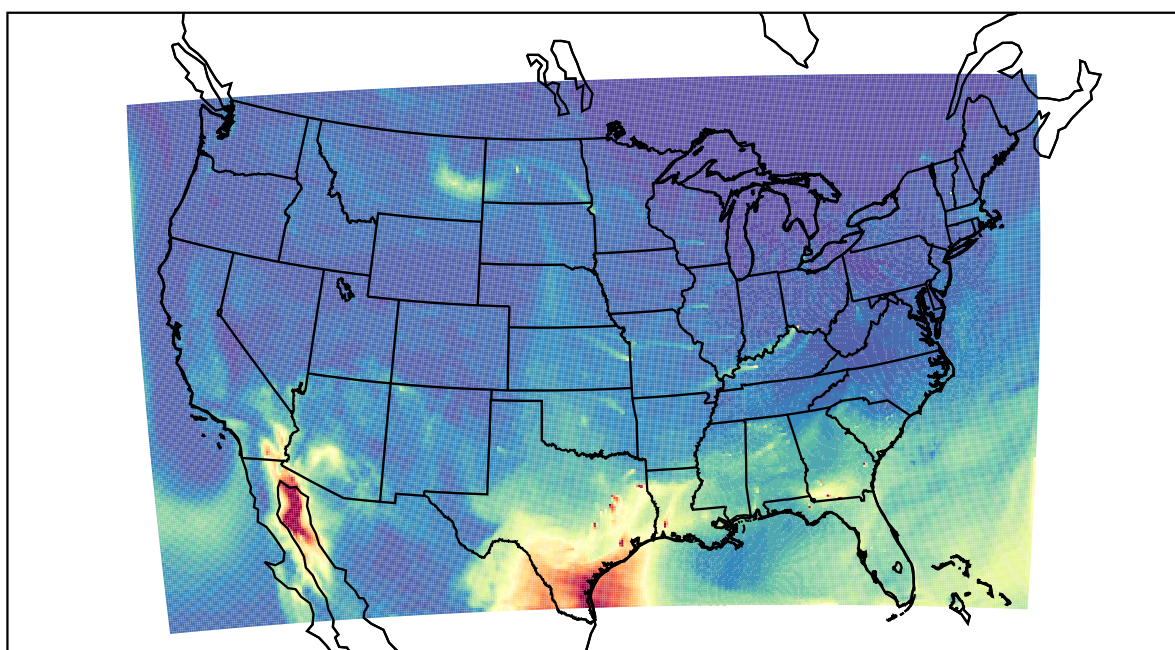
WRF 2022-04-17_17:00:00
