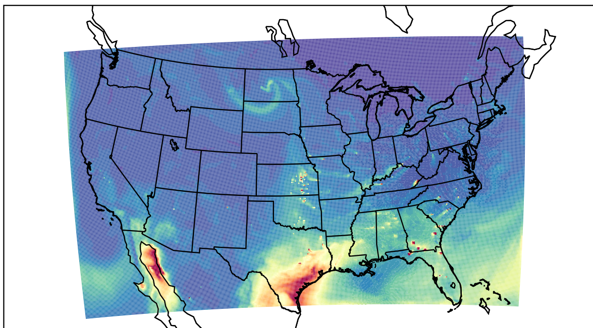
WRF 2022-04-17_22:00:00
