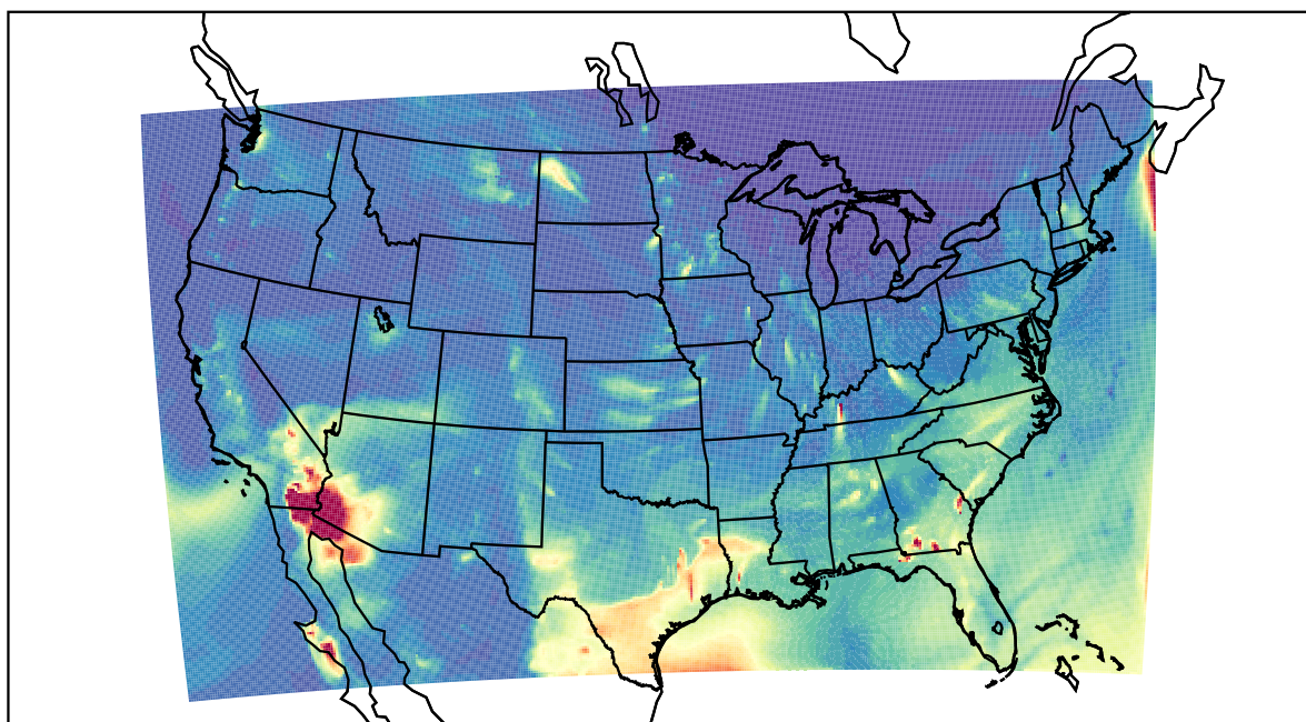
WRF 2022-04-17_05:00:00
