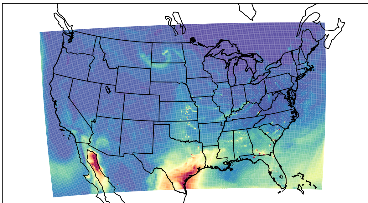
WRF 2022-04-17_21:00:00
