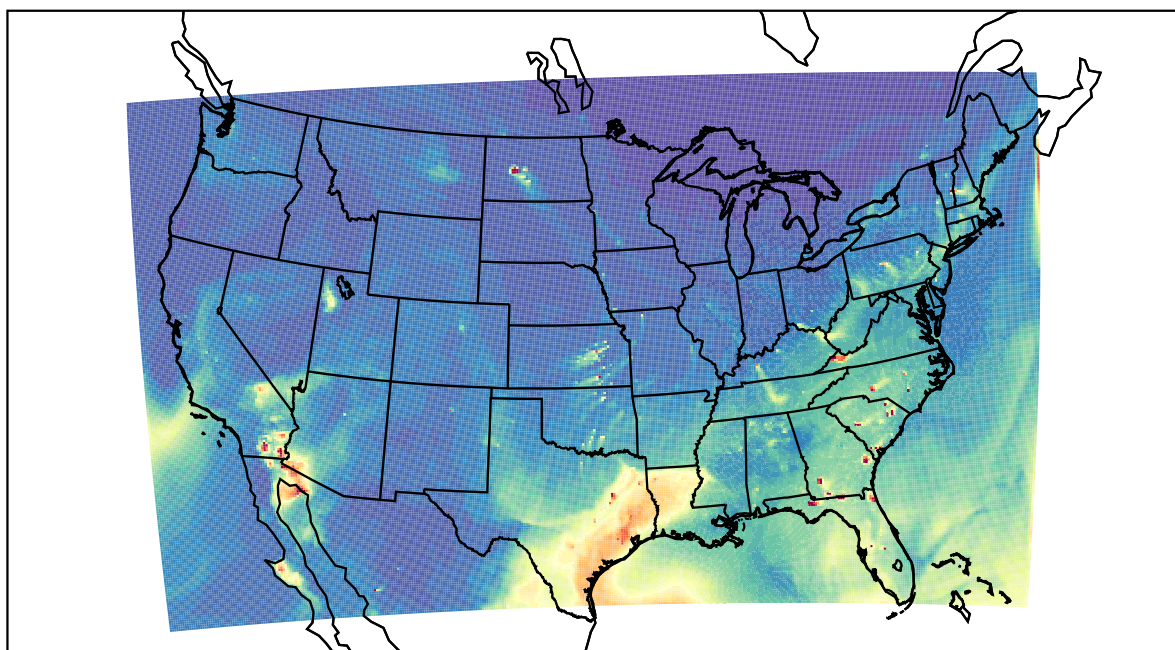
WRF 2022-04-16_23:00:00
