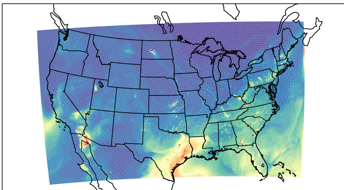
WRF 2022-04-16_22:00:00
