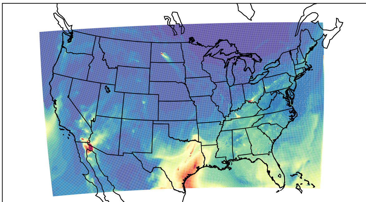
WRF 2022-04-16_17:00:00
