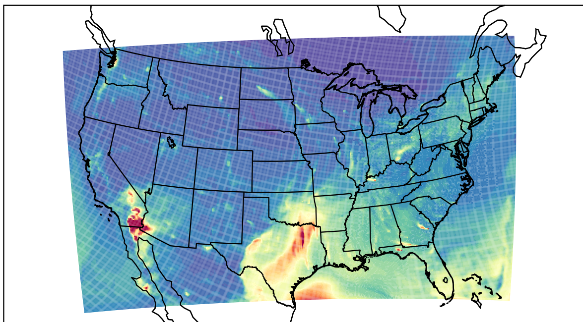
WRF 2022-04-16_05:00:00
