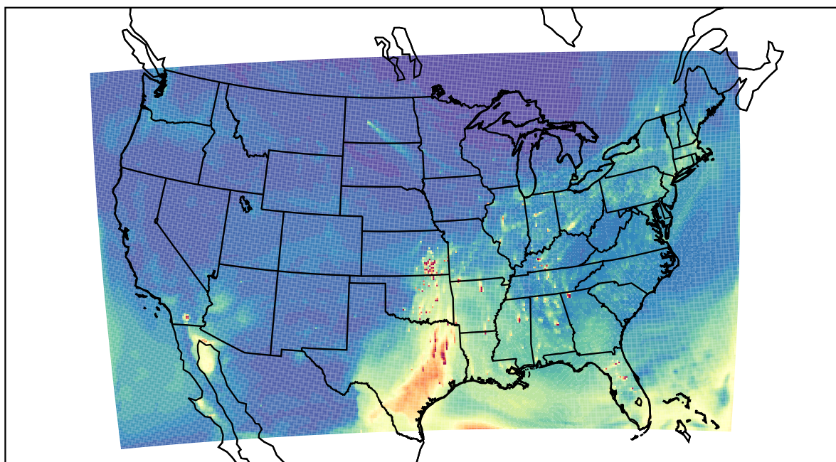
WRF 2022-04-16_00:00:00
