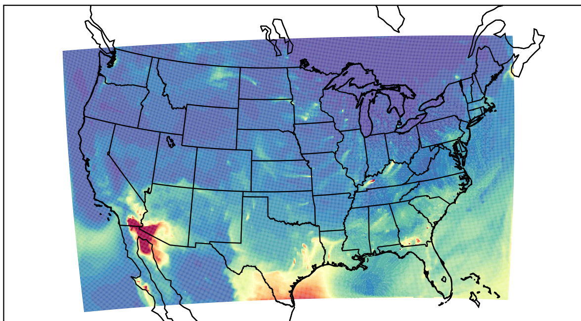
WRF 2022-04-17_11:00:00
