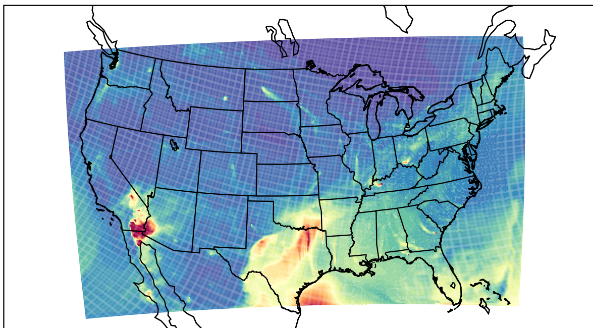
WRF 2022-04-16_07:00:00
