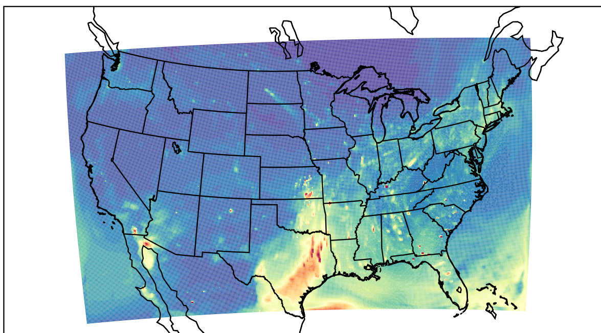
WRF 2022-04-16_01:00:00
