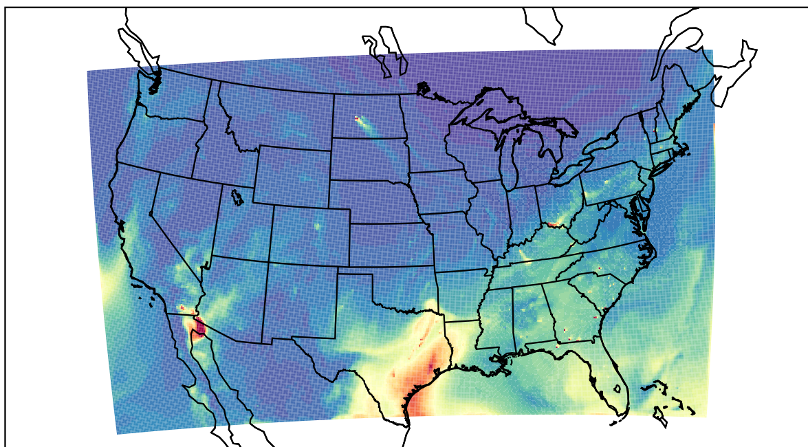
WRF 2022-04-16_18:00:00
