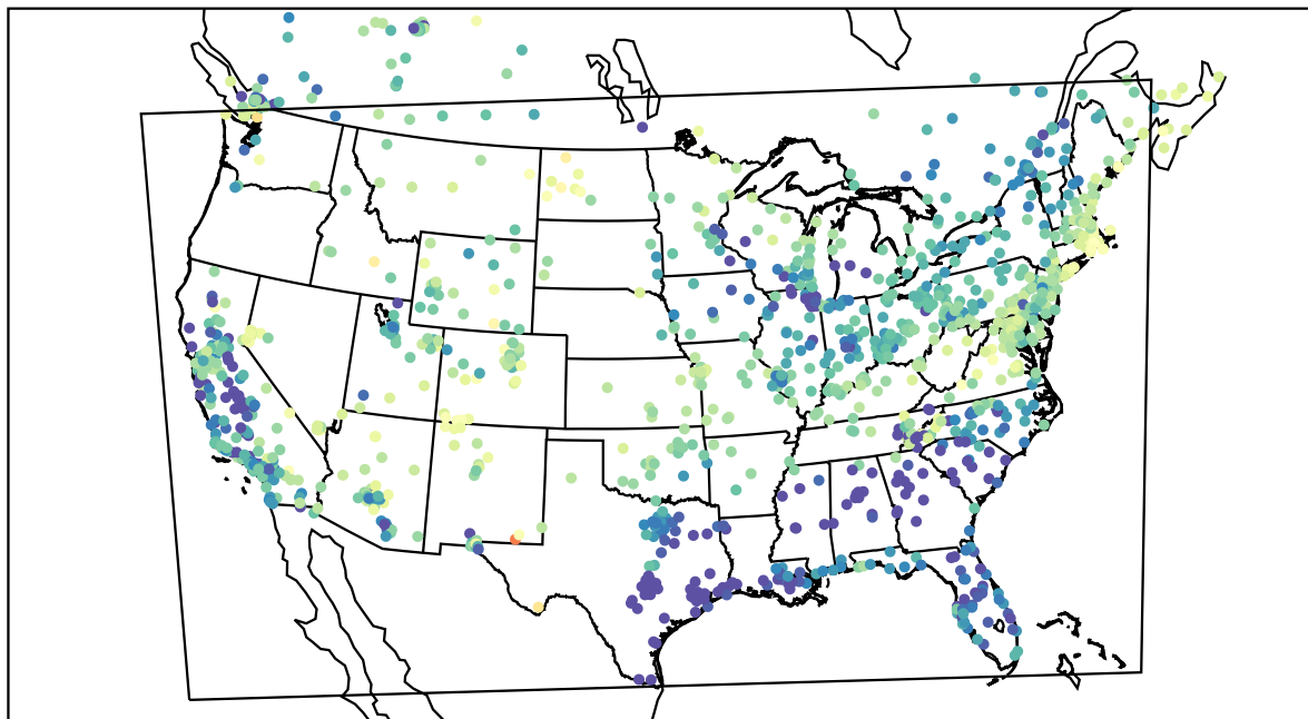
AirNOW (2022-04-17_05:00:00)
