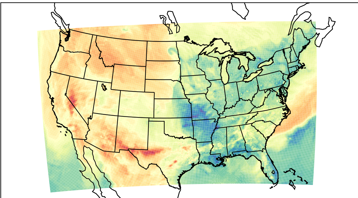
WRF (2022-04-18_00:00:00)
