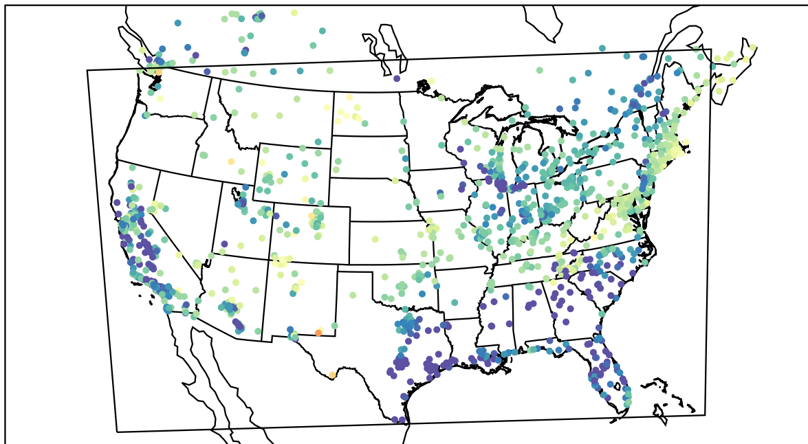
AirNOW (2022-04-17_06:00:00)
