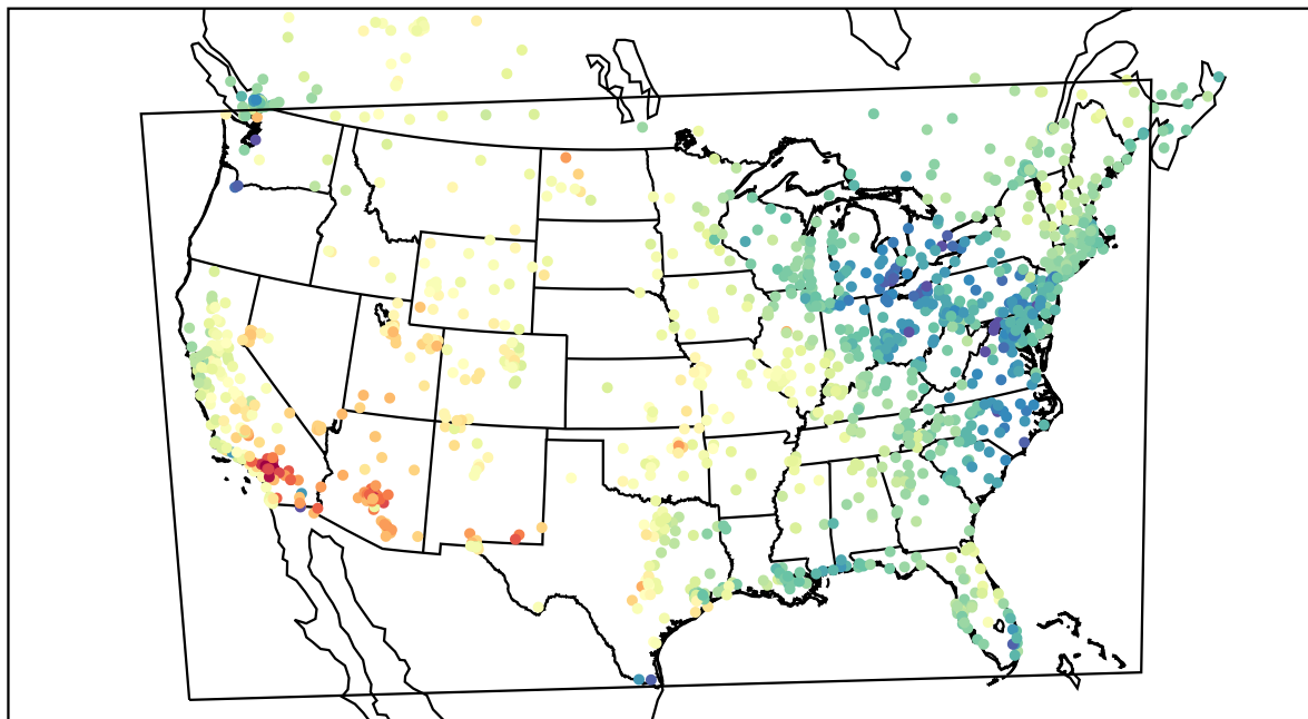
AirNOW (2022-04-18_22:00:00)
