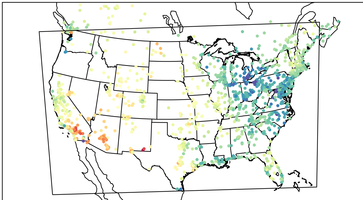
AirNOW (2022-04-18_20:00:00)
