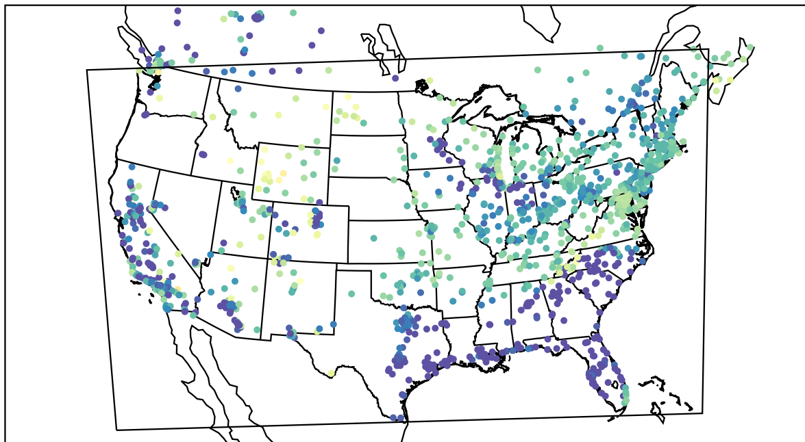
AirNOW (2022-04-17_11:00:00)
