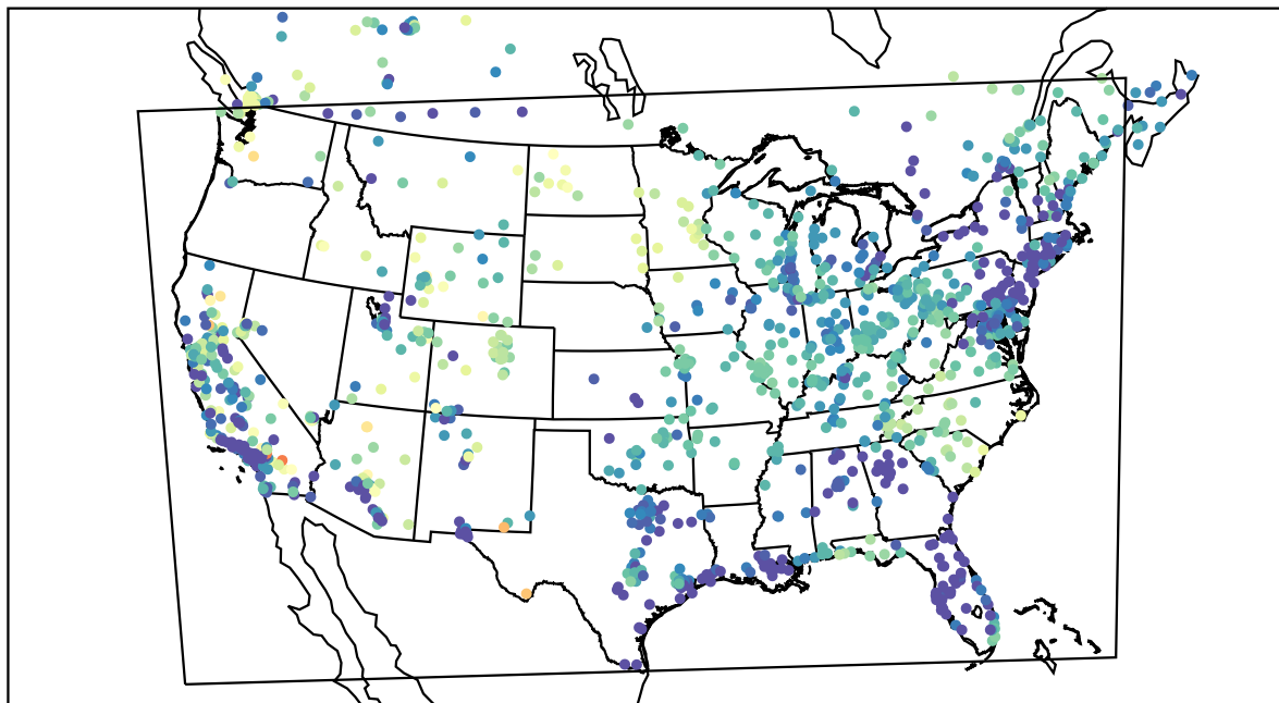
AirNOW (2022-04-18_08:00:00)
