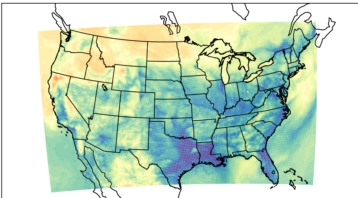
WRF (2022-04-17_07:00:00)
