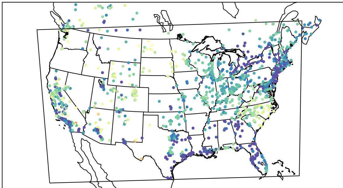
AirNOW (2022-04-18_06:00:00)
