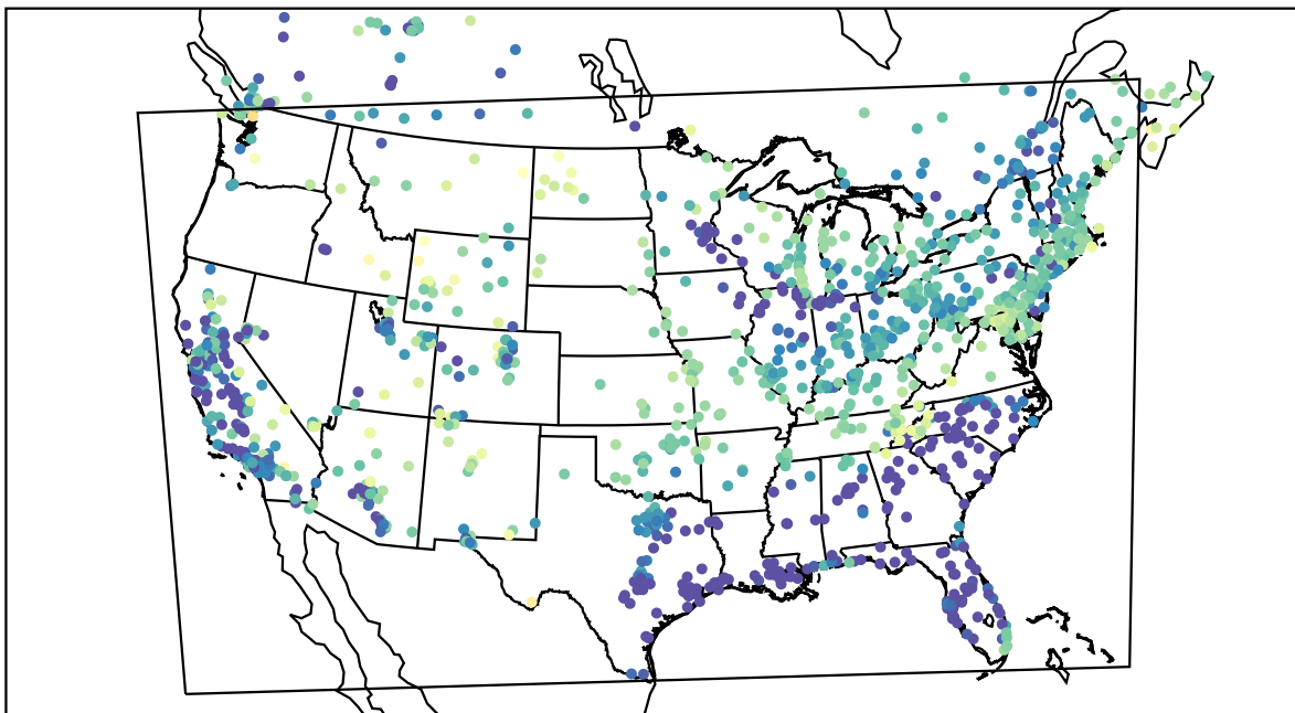
AirNOW (2022-04-17_09:00:00)
