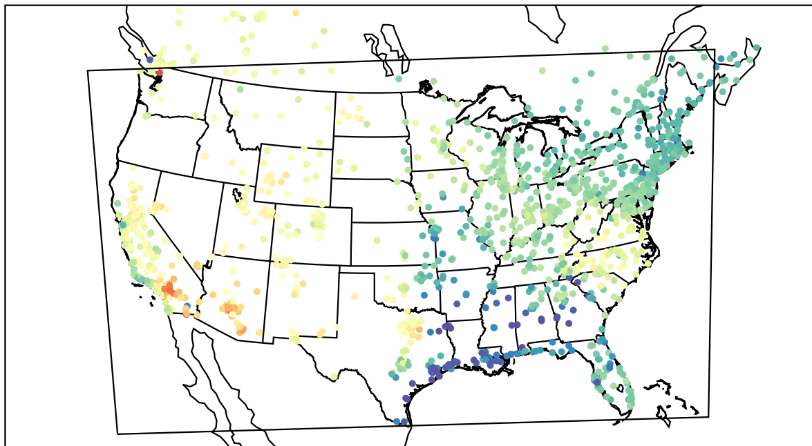
AirNOW (2022-04-17_23:00:00)
