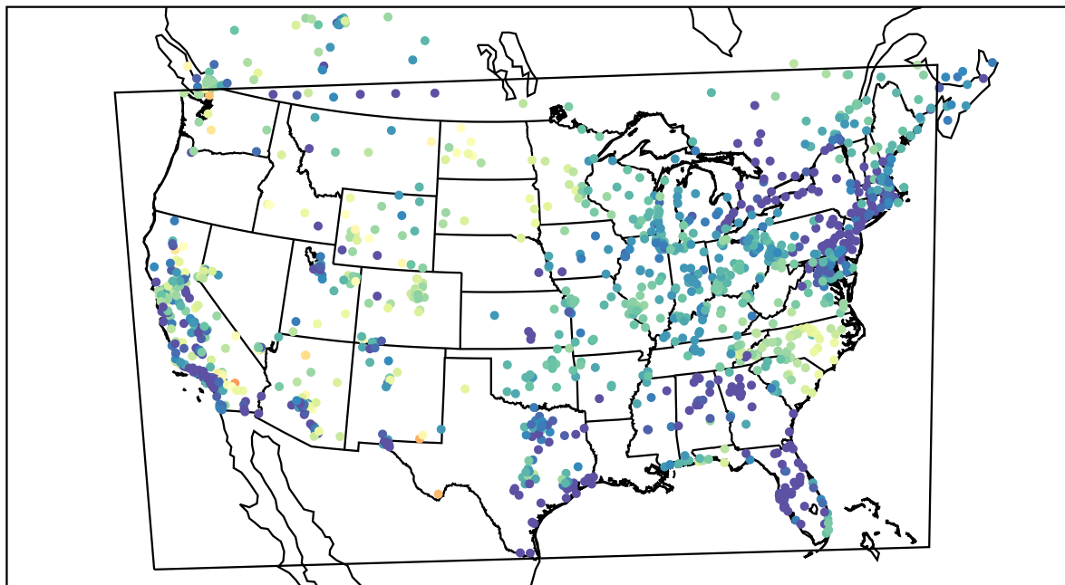
AirNOW (2022-04-18_07:00:00)
