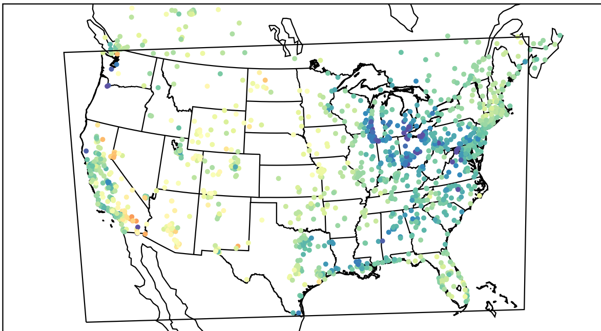
AirNOW (2022-04-18_17:00:00)
