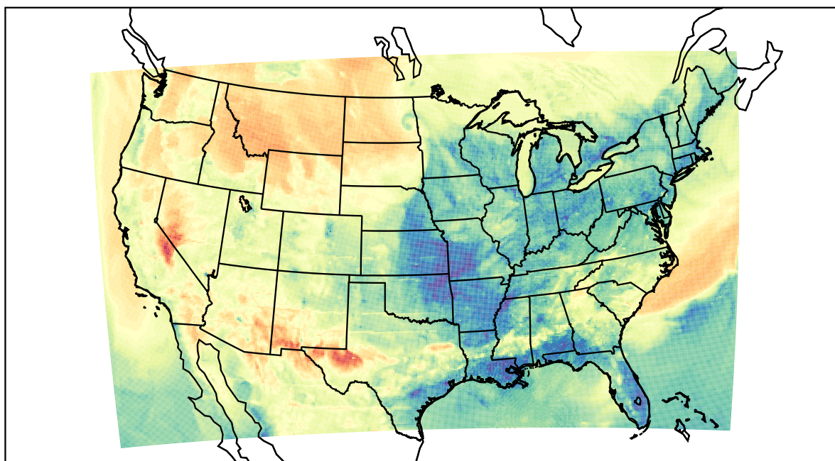
WRF (2022-04-18_02:00:00)
