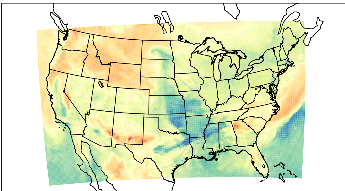
WRF (2022-04-17_18:00:00)
