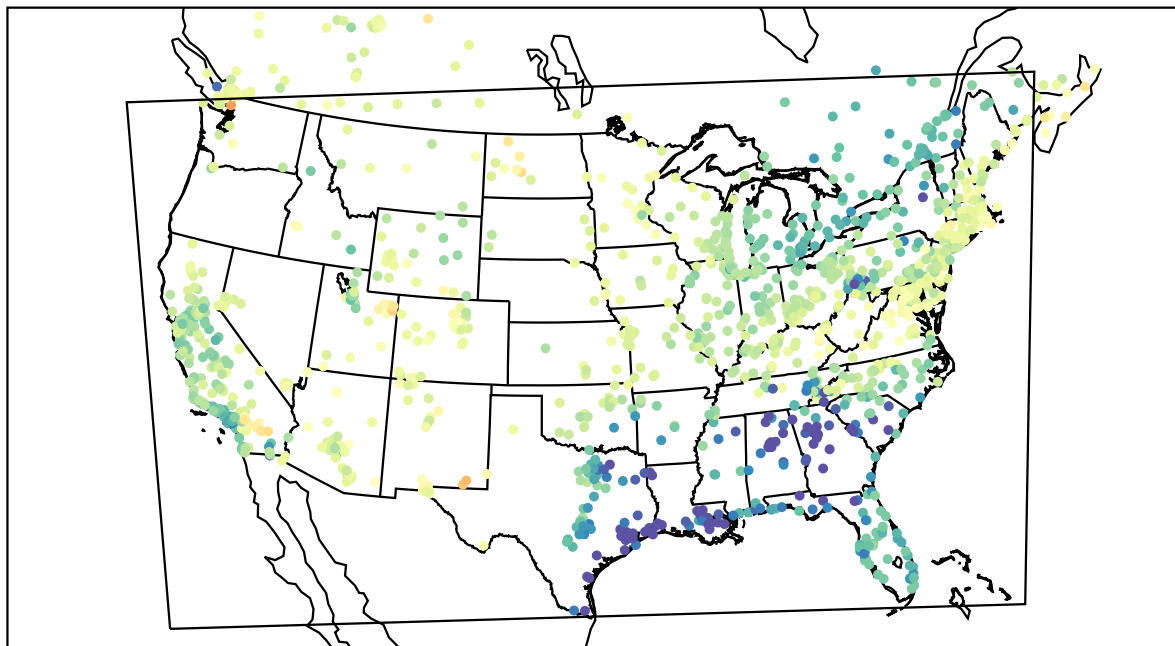
AirNOW (2022-04-17_00:00:00)
