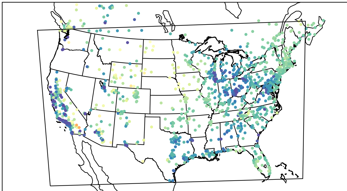
AirNOW (2022-04-18_15:00:00)
