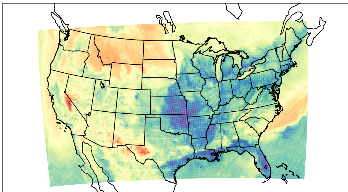
WRF (2022-04-18_04:00:00)
