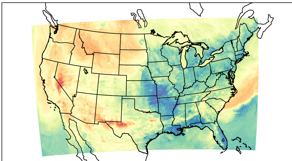
WRF (2022-04-18_01:00:00)
