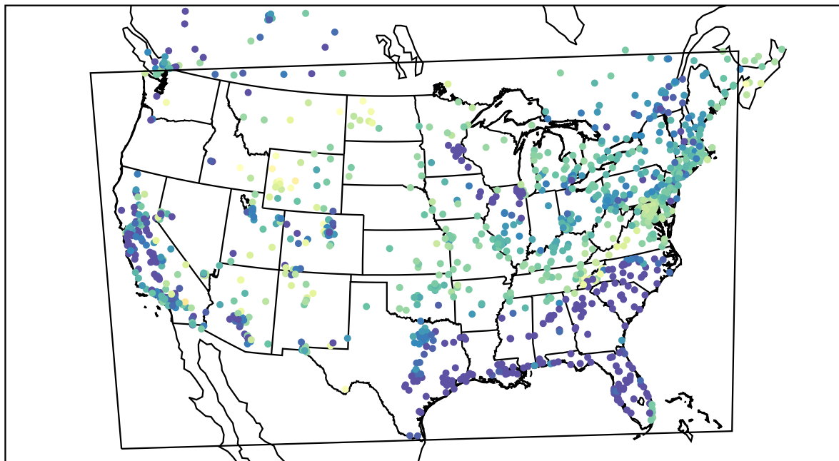
AirNOW (2022-04-17_10:00:00)
