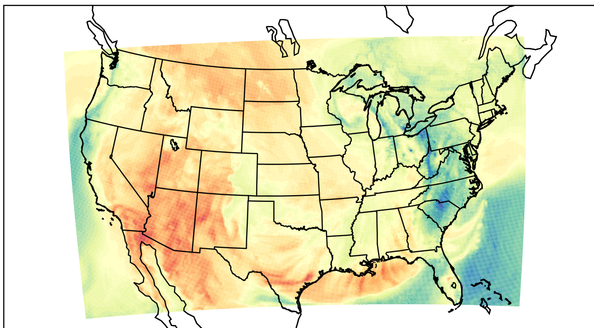
WRF (2022-04-18_22:00:00)
