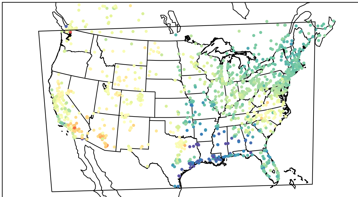
AirNOW (2022-04-17_22:00:00)
