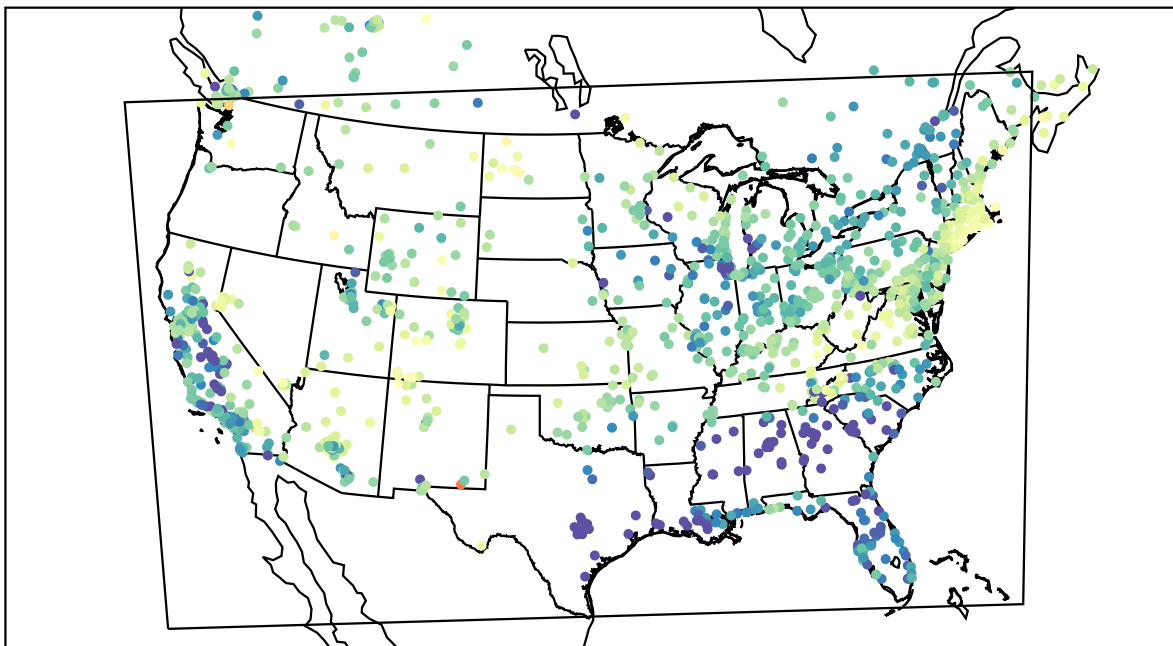
AirNOW (2022-04-17_04:00:00)
