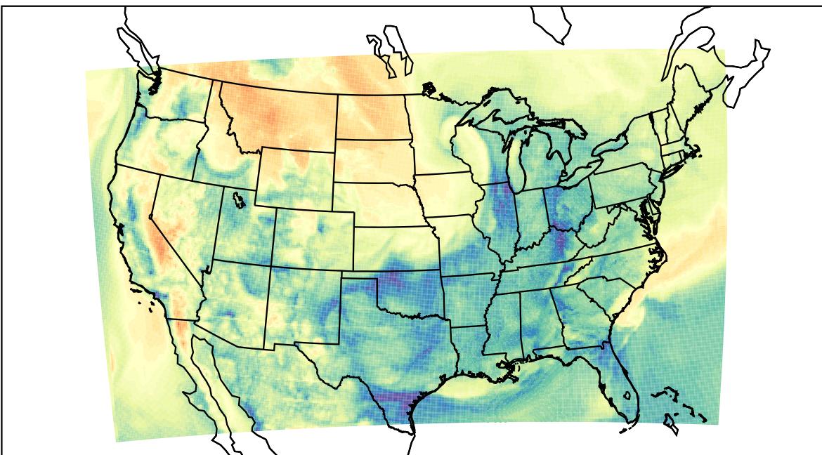
WRF (2022-04-18_14:00:00)
