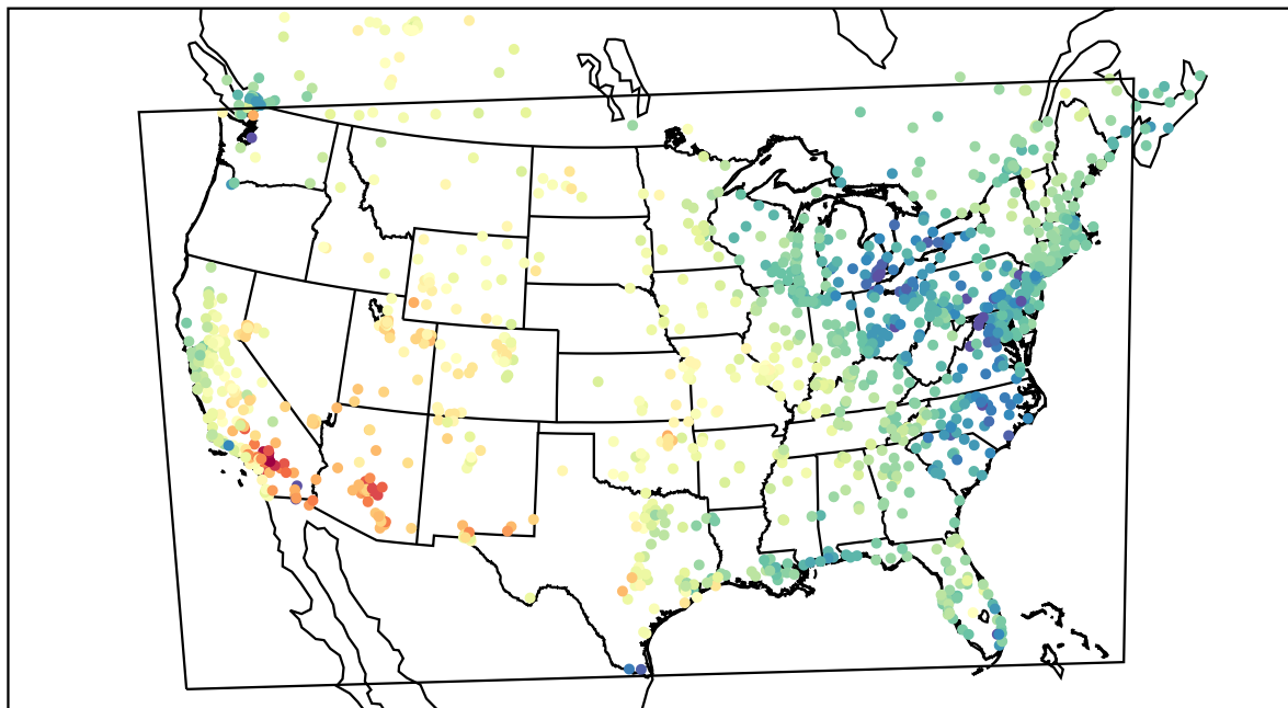
AirNOW (2022-04-18_23:00:00)
