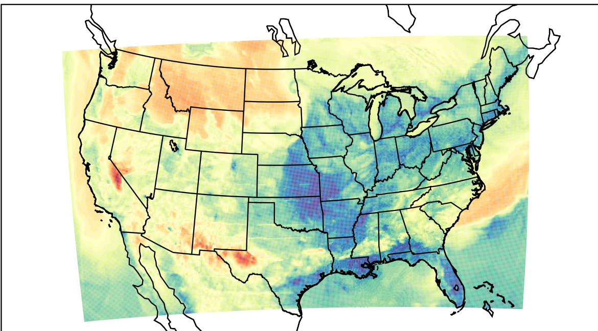
WRF (2022-04-18_03:00:00)
