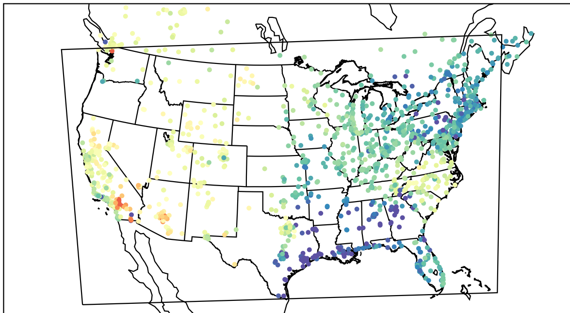
AirNOW (2022-04-18_01:00:00)
