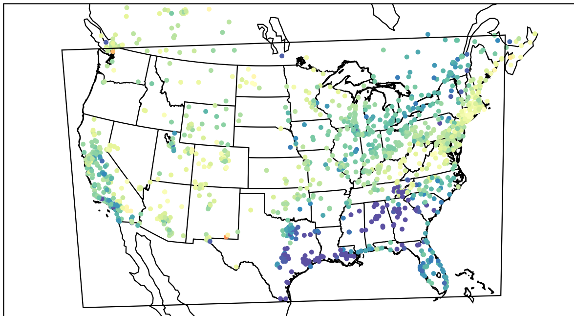
AirNOW (2022-04-17_02:00:00)
