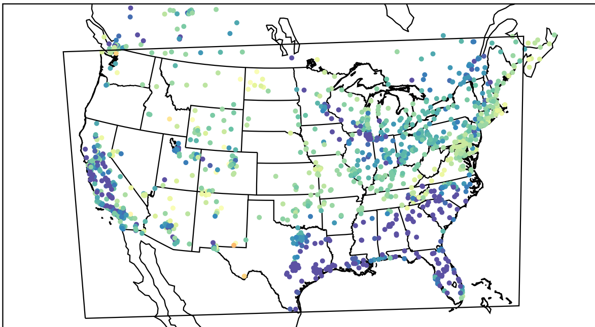
AirNOW (2022-04-17_07:00:00)
