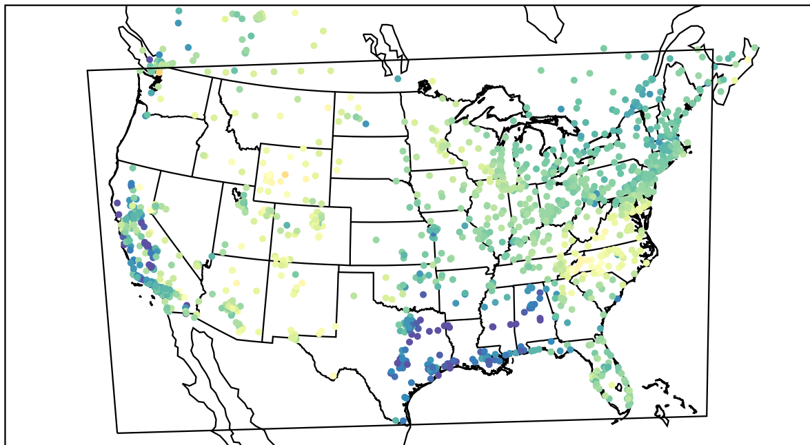
AirNOW (2022-04-17_16:00:00)
