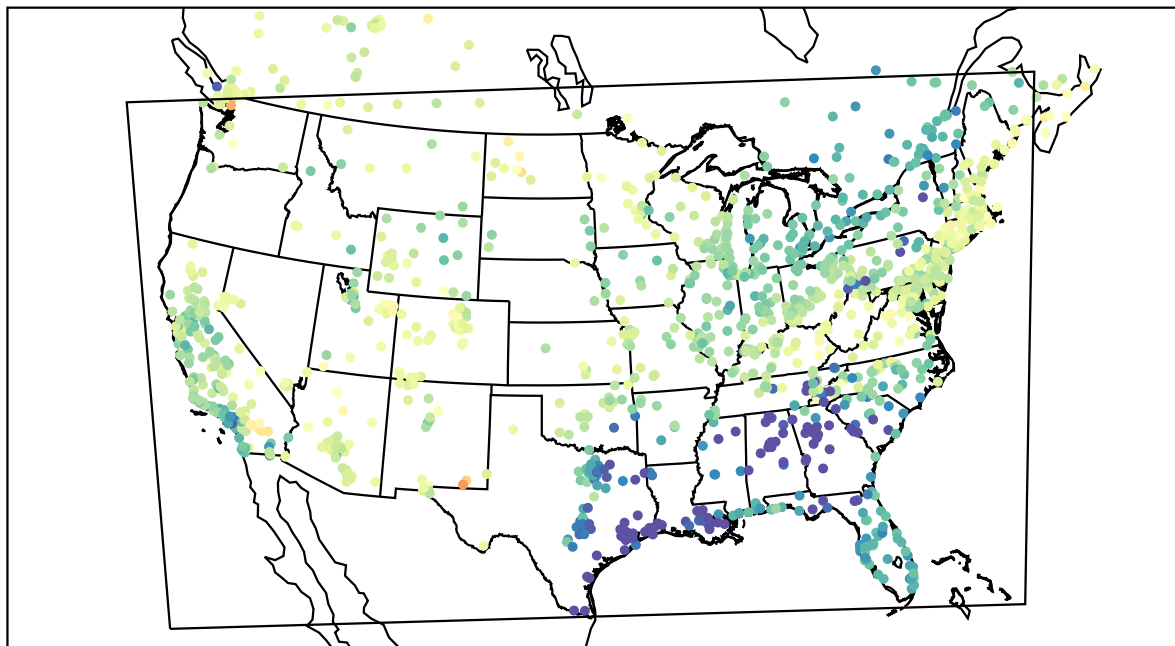
AirNOW (2022-04-17_01:00:00)
