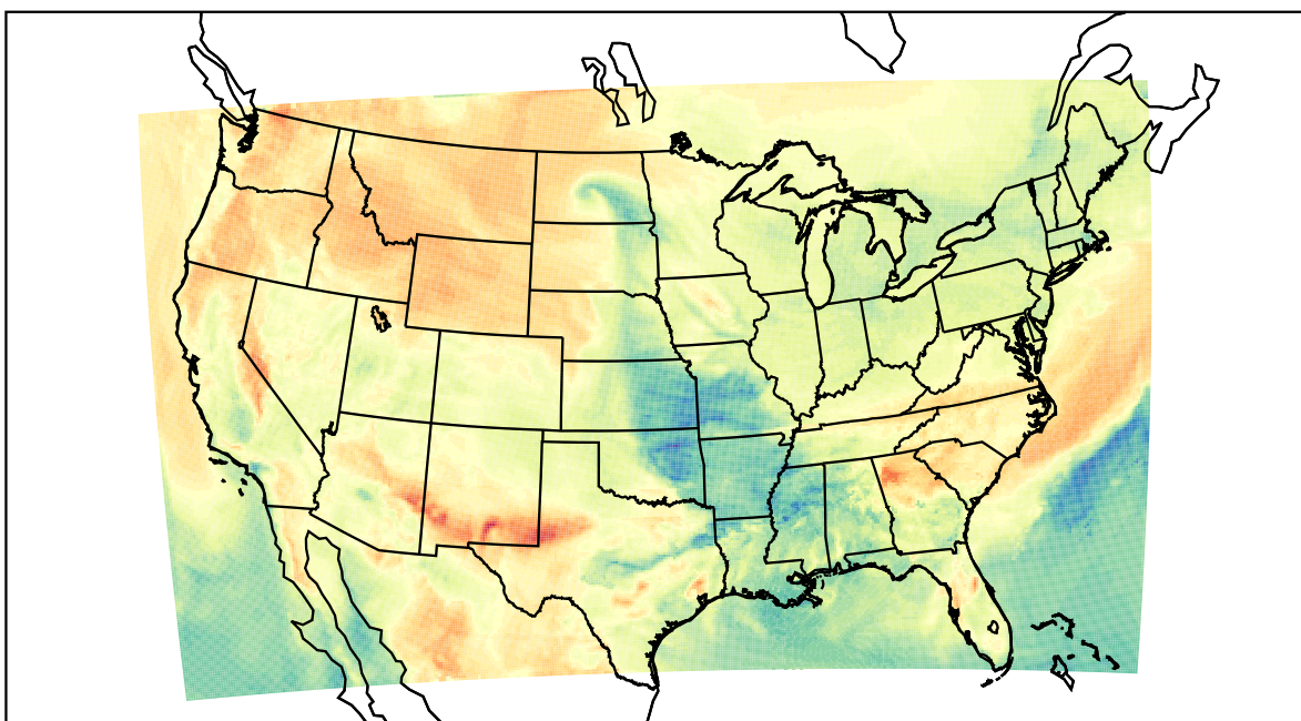
WRF (2022-04-17_19:00:00)
