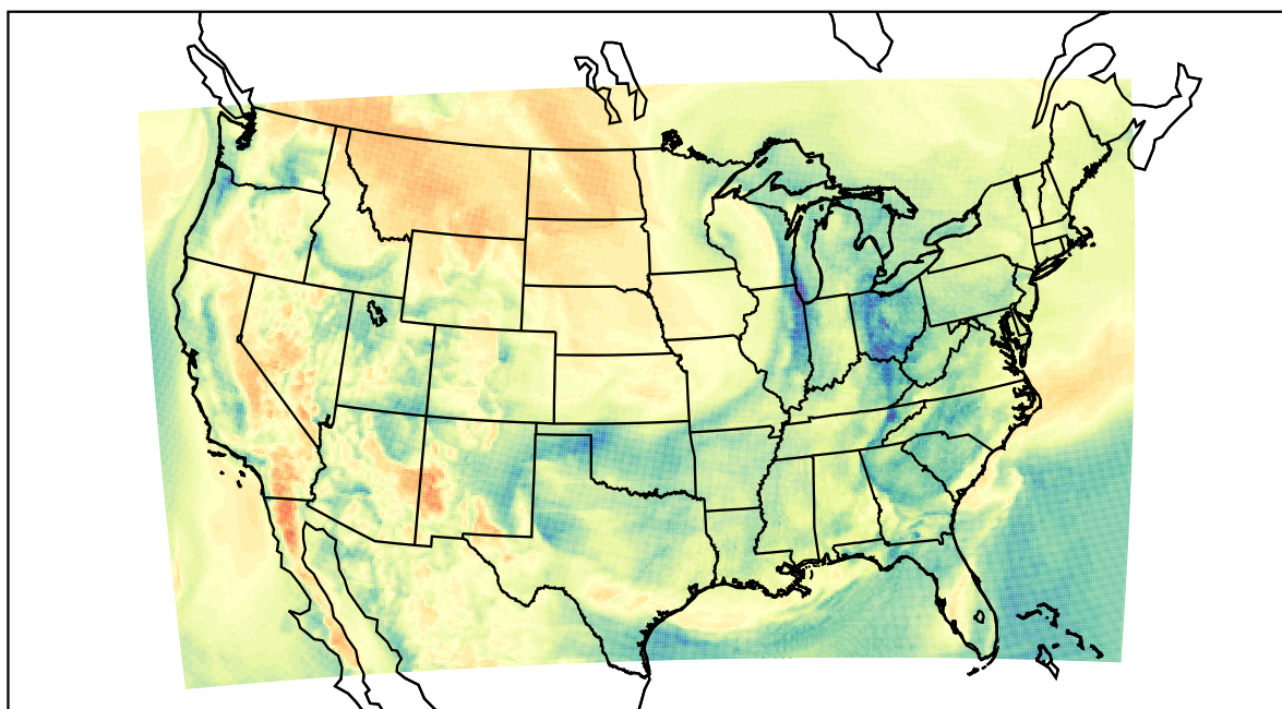
WRF (2022-04-18_16:00:00)
