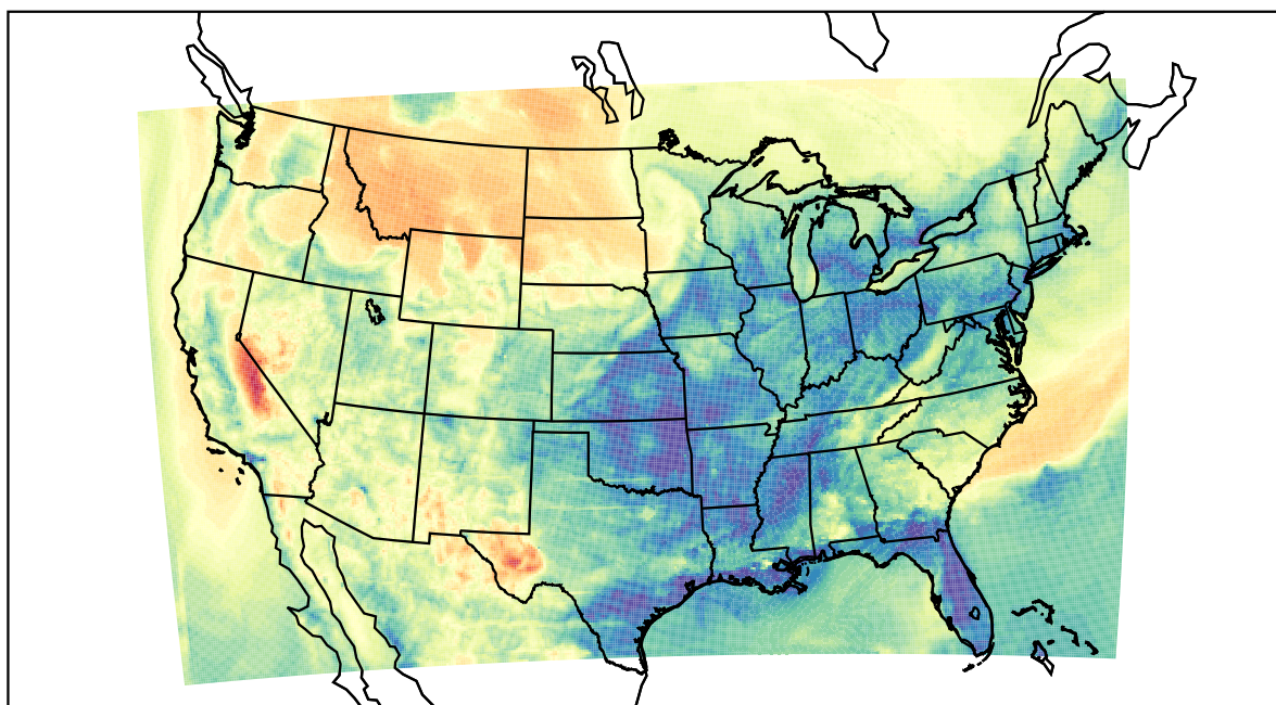
WRF (2022-04-18_07:00:00)
