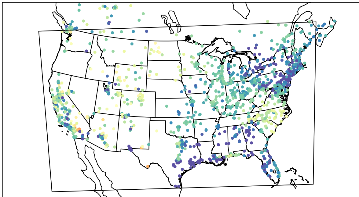
AirNOW (2022-04-18_04:00:00)
