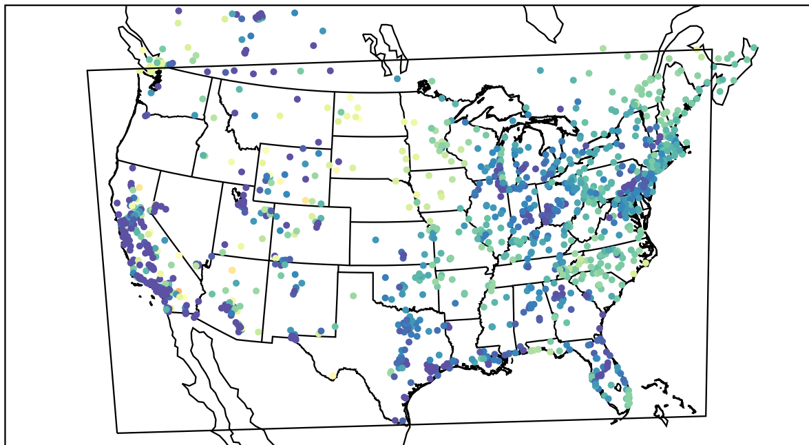
AirNOW (2022-04-18_13:00:00)
