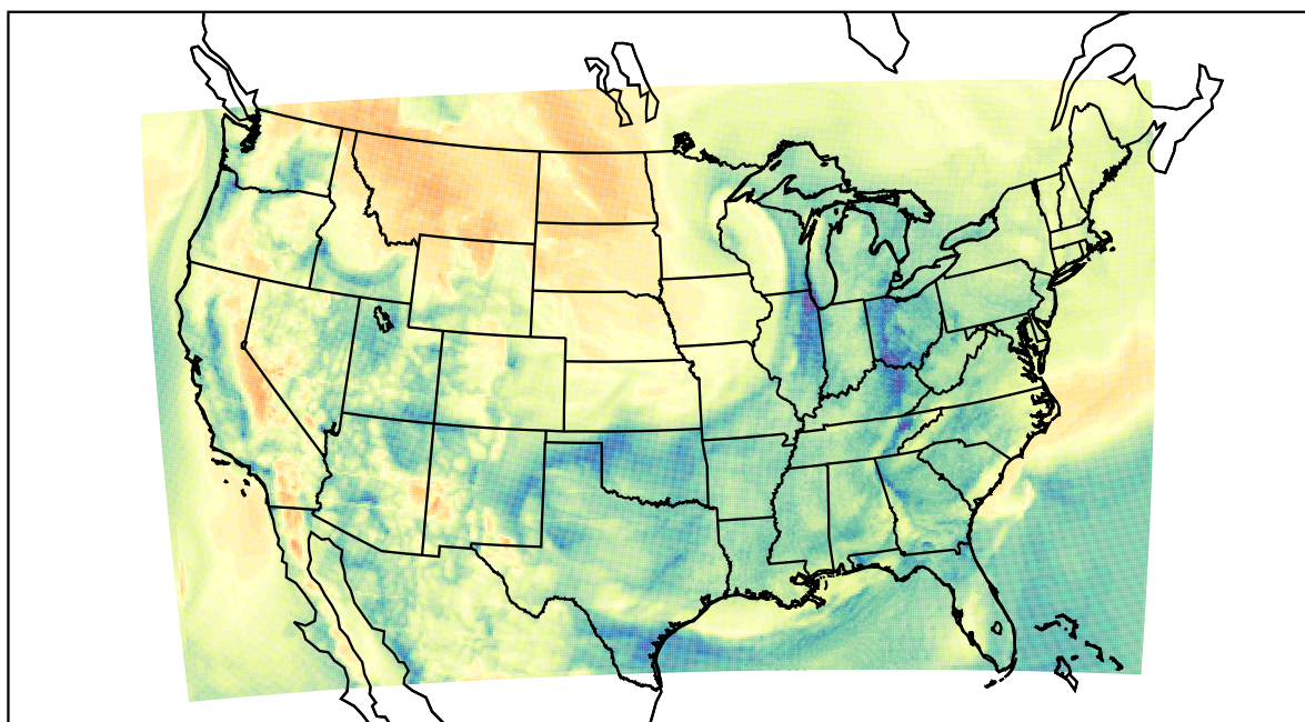
WRF (2022-04-18_15:00:00)
