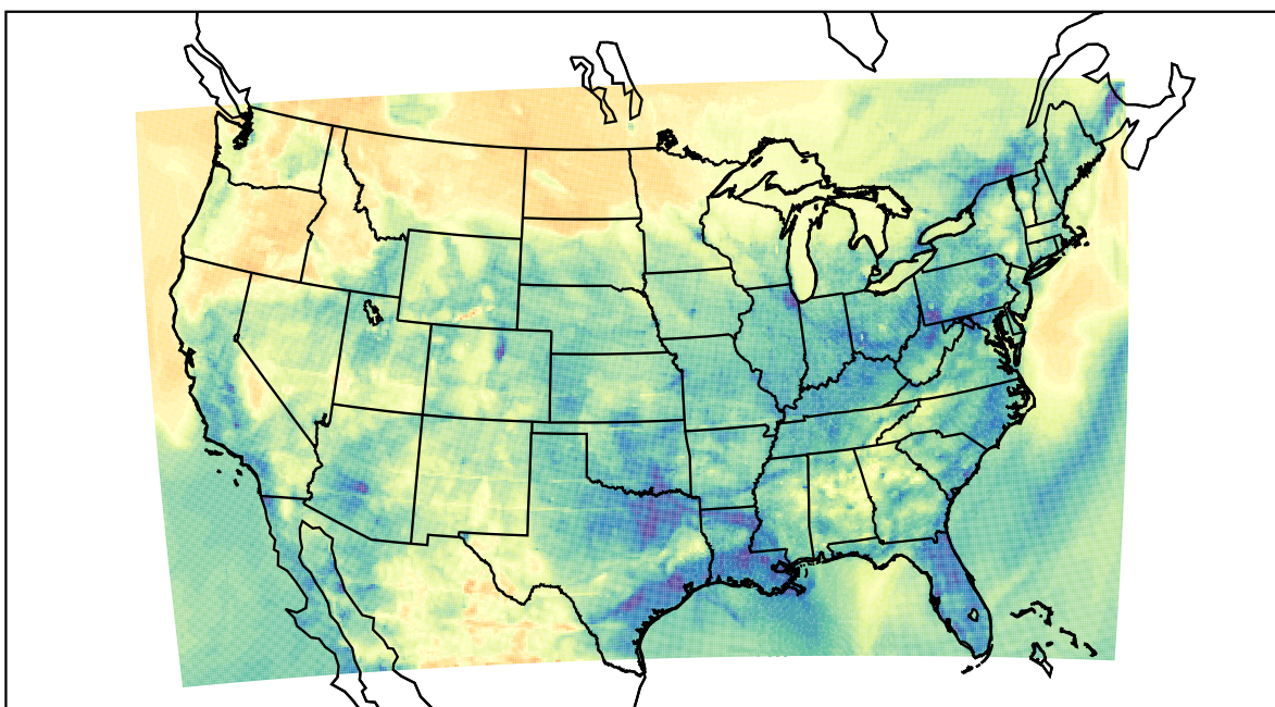
WRF (2022-04-17_03:00:00)
