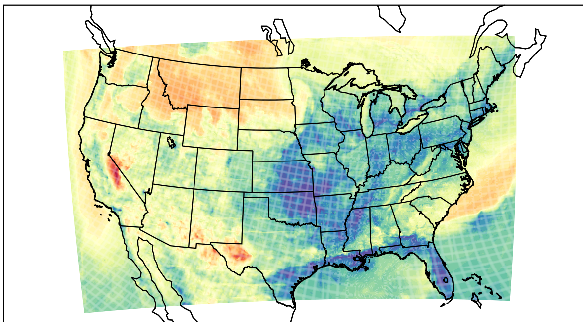
WRF (2022-04-18_05:00:00)
