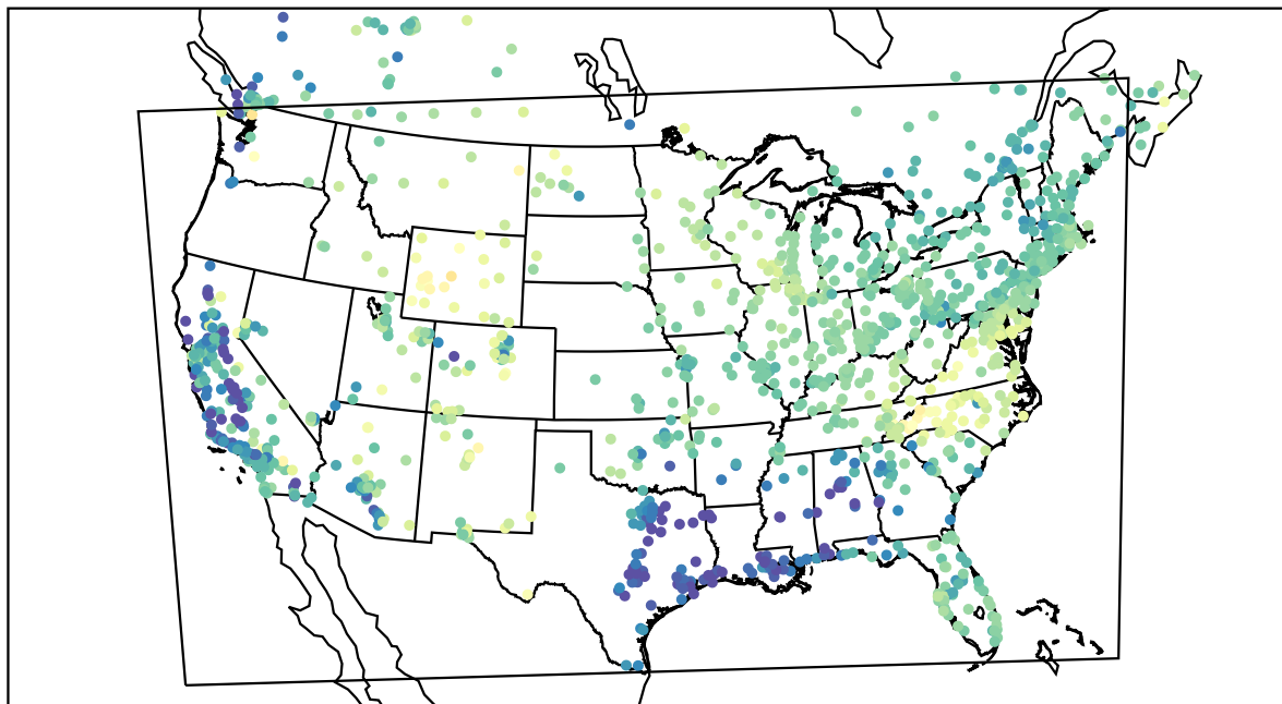
AirNOW (2022-04-17_15:00:00)
