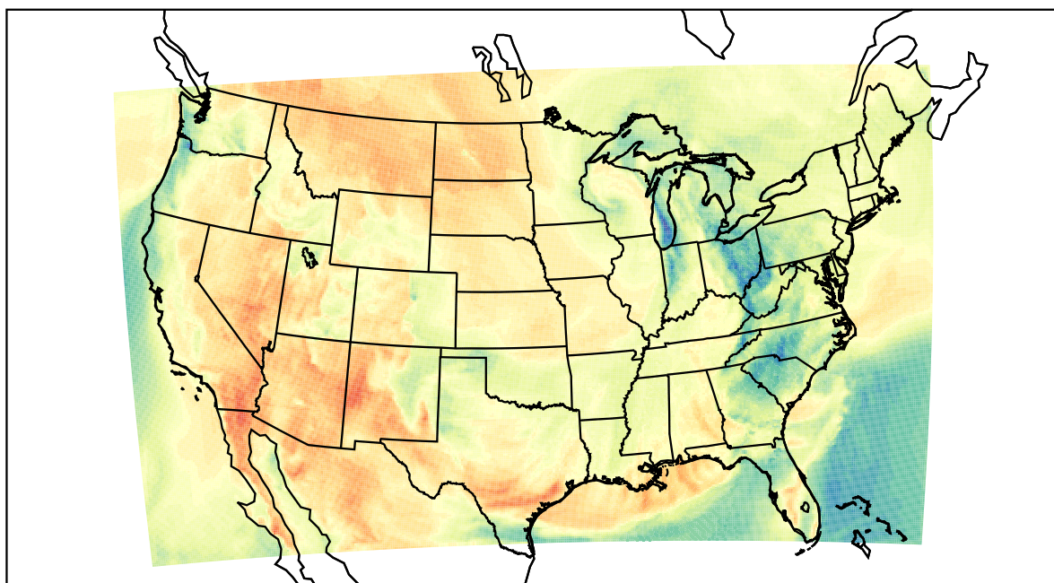
WRF (2022-04-18_19:00:00)
