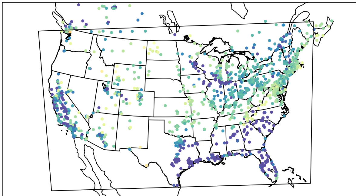
AirNOW (2022-04-17_08:00:00)
