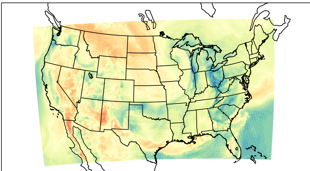
WRF (2022-04-18_17:00:00)
