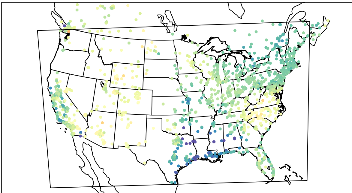
AirNOW (2022-04-17_18:00:00)
