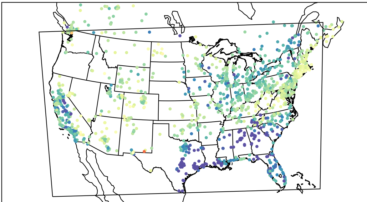
AirNOW (2022-04-17_03:00:00)
