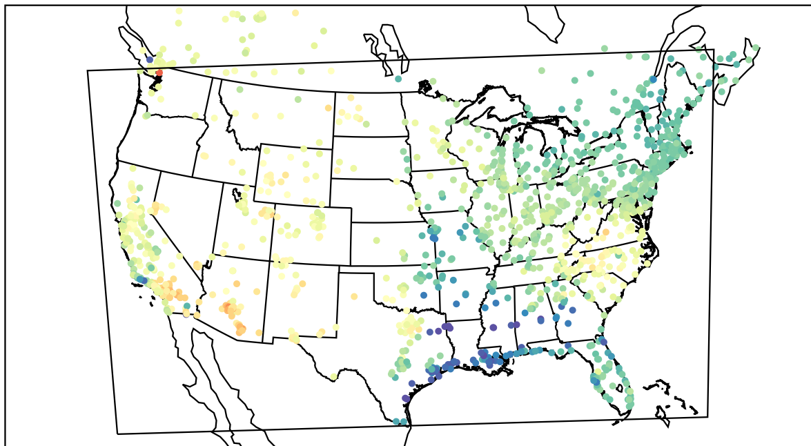
AirNOW (2022-04-17_21:00:00)
