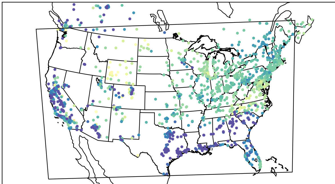
AirNOW (2022-04-17_13:00:00)
