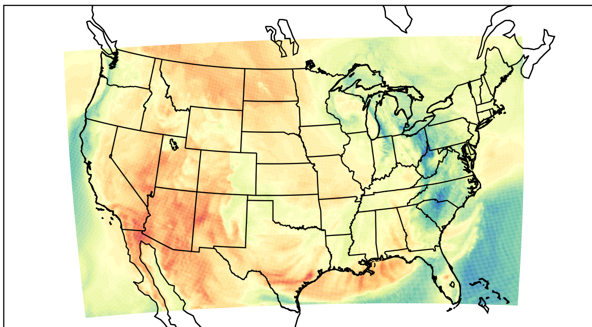
WRF (2022-04-18_21:00:00)
