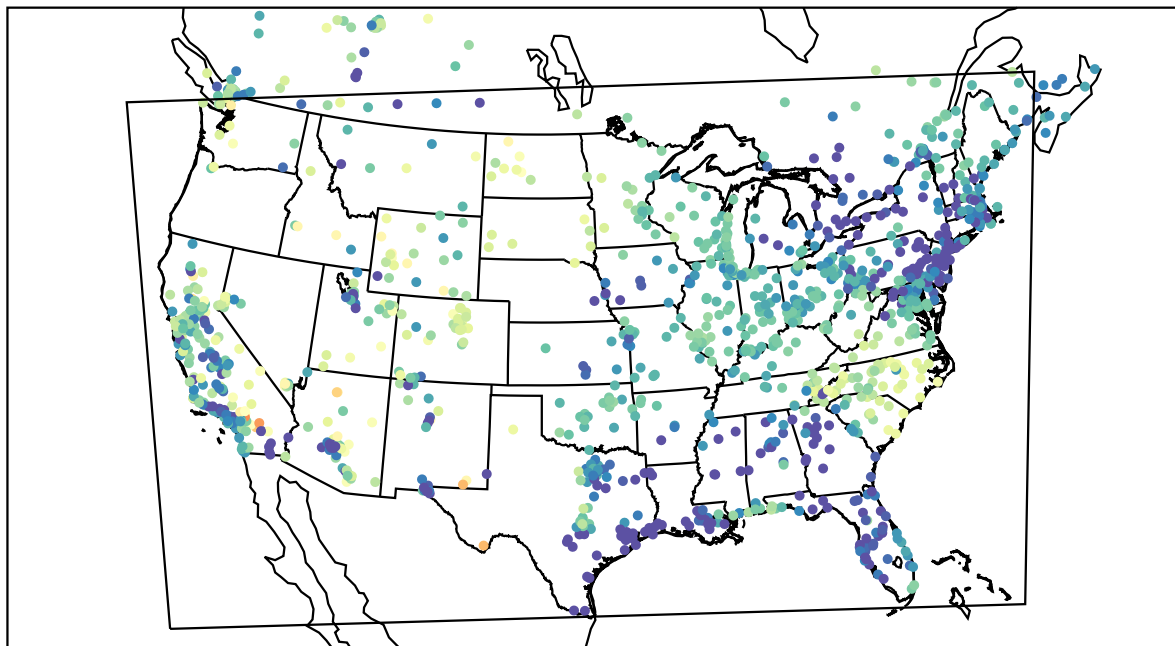
AirNOW (2022-04-18_05:00:00)
