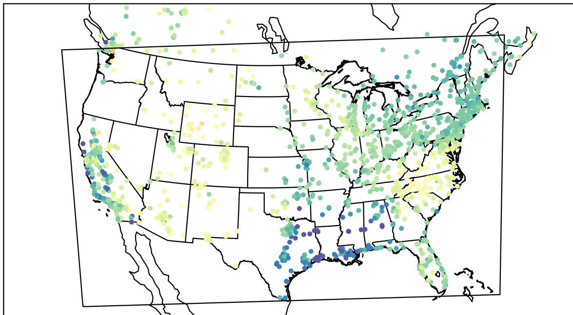
AirNOW (2022-04-17_17:00:00)
