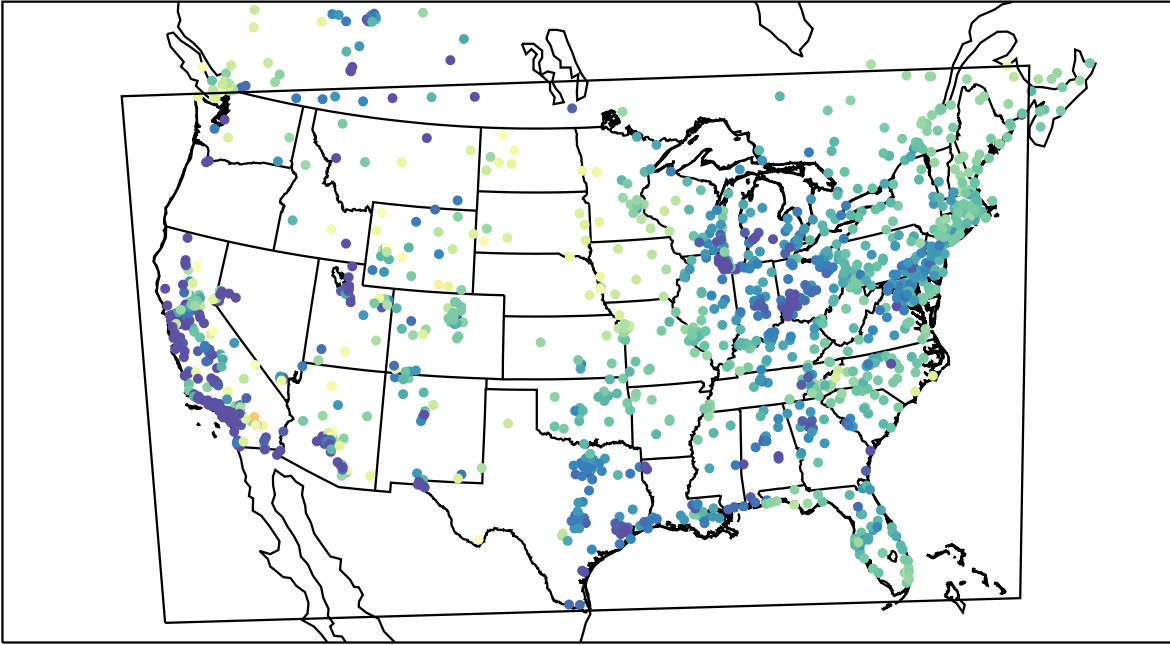
AirNOW (2022-04-18_14:00:00)
