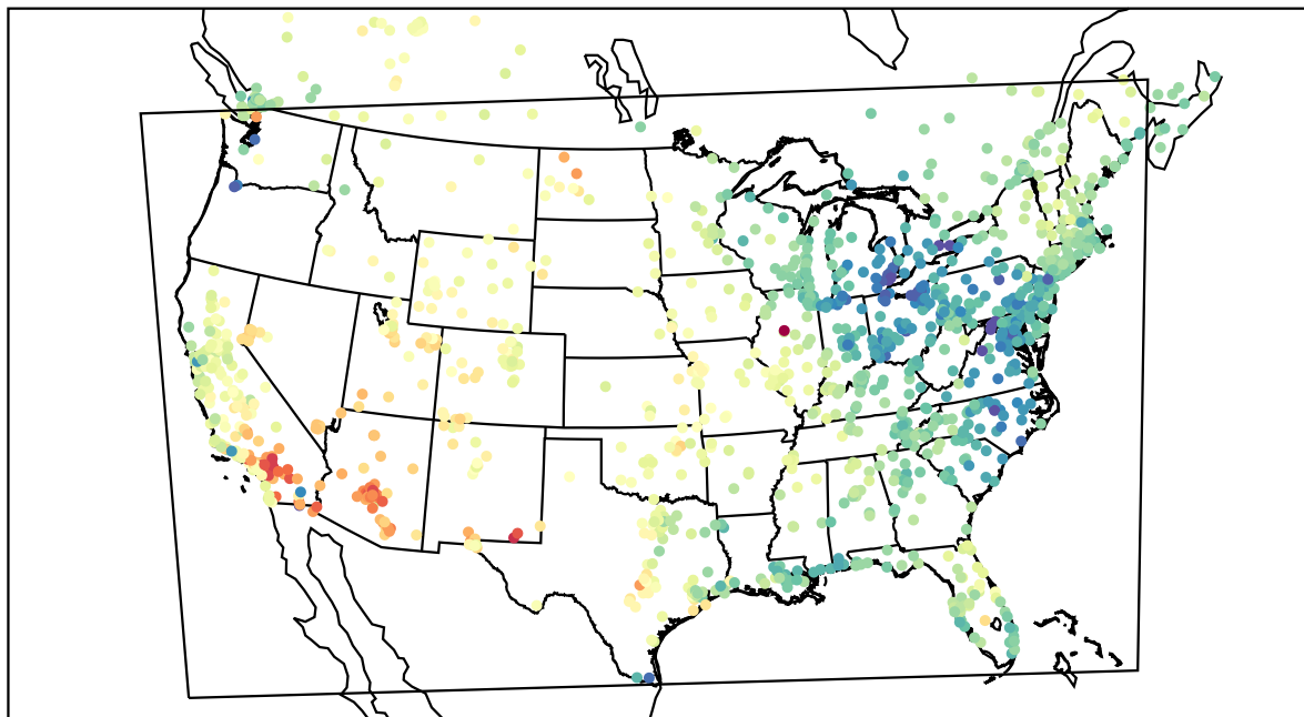
AirNOW (2022-04-18_21:00:00)
