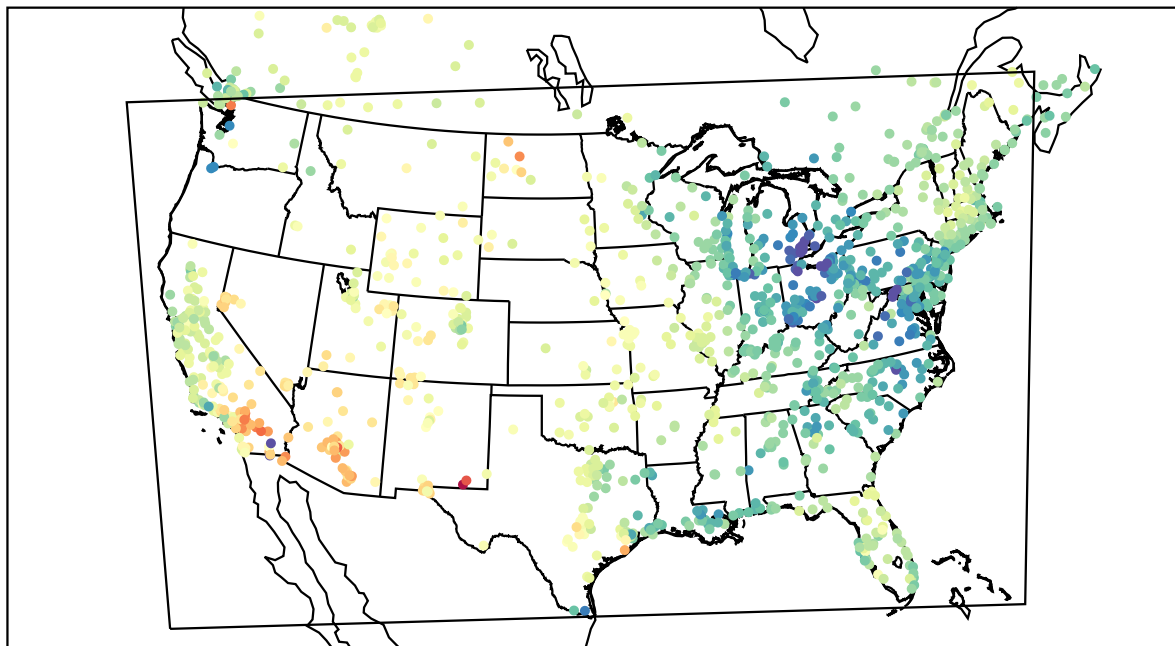
AirNOW (2022-04-18_19:00:00)
