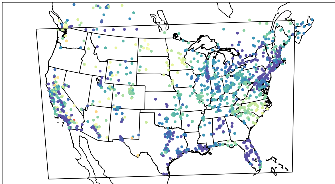
AirNOW (2022-04-18_09:00:00)
