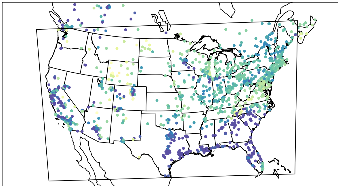
AirNOW (2022-04-17_12:00:00)
