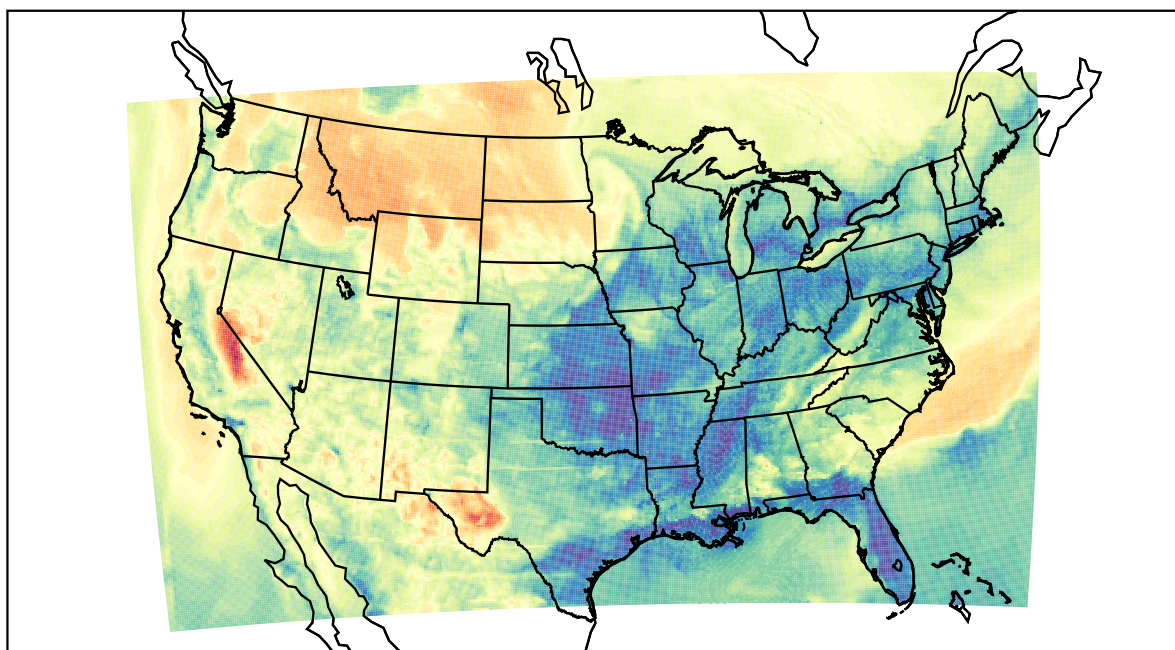
WRF (2022-04-18_06:00:00)
