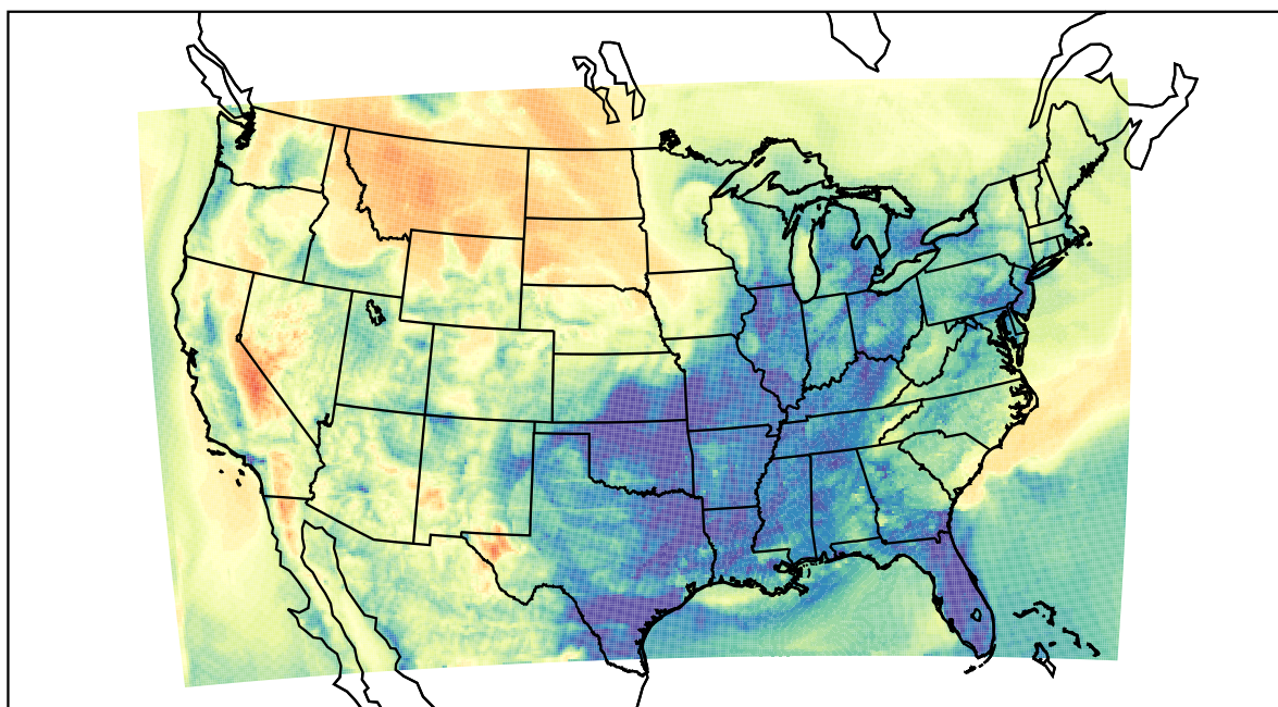
WRF (2022-04-18_12:00:00)
