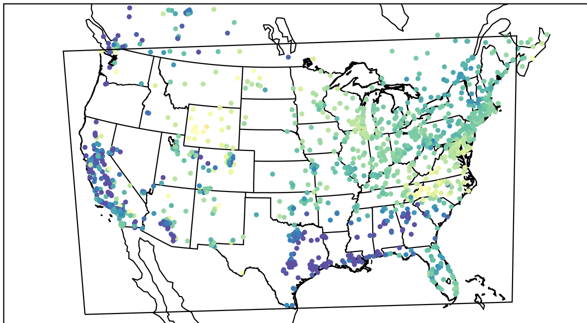
AirNOW (2022-04-17_14:00:00)
