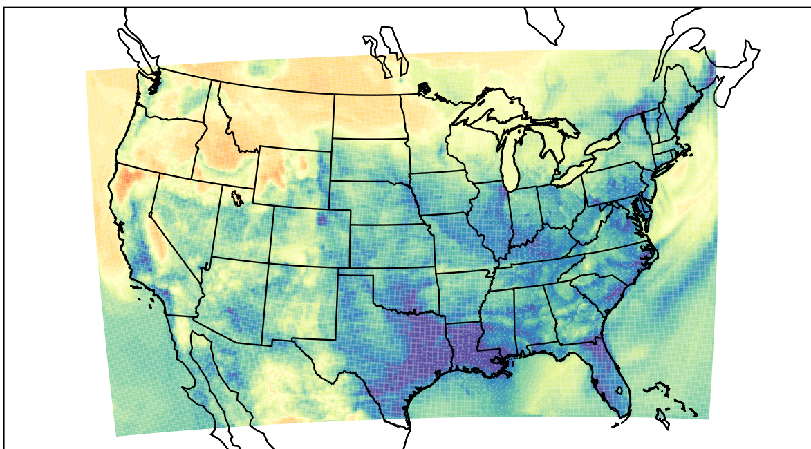
WRF (2022-04-17_09:00:00)
