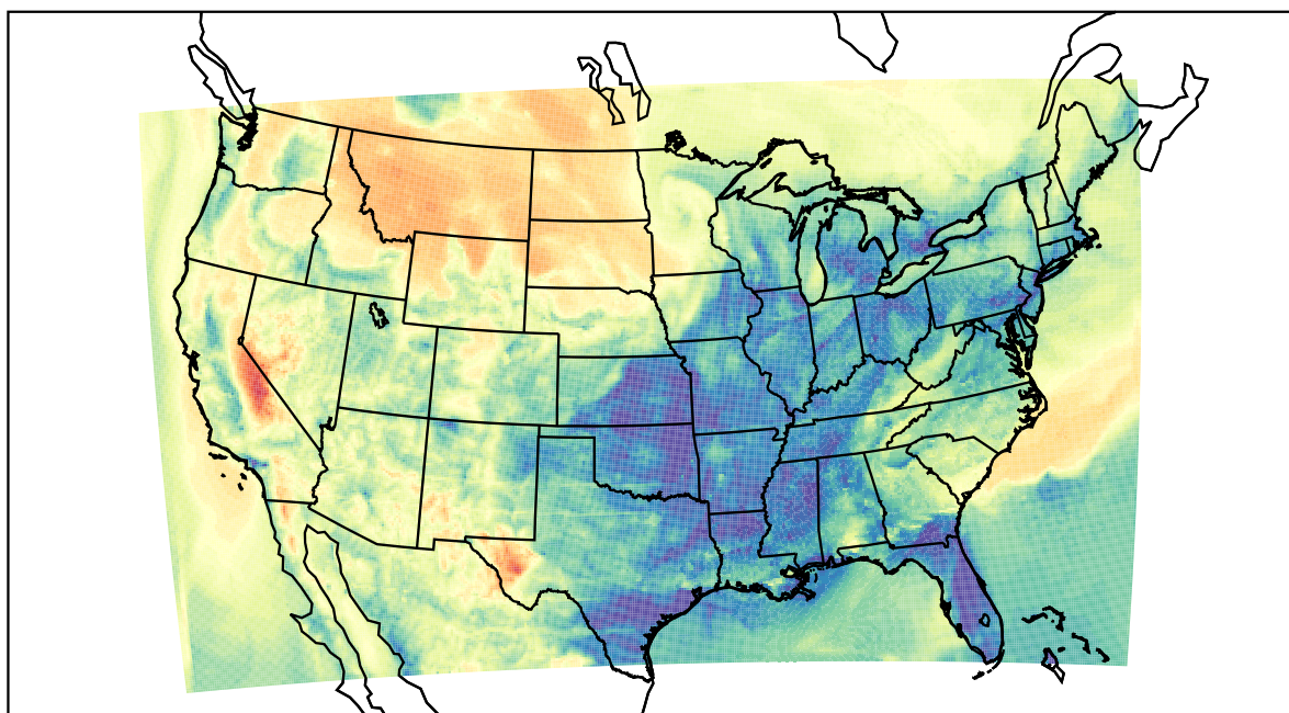
WRF (2022-04-18_09:00:00)
