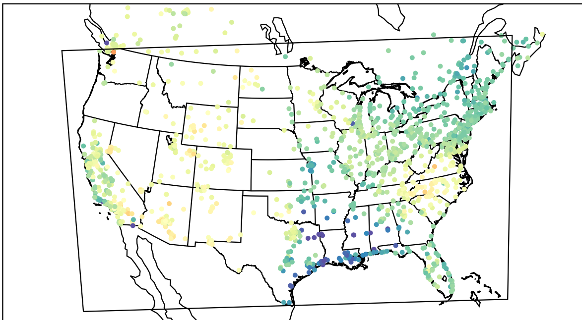
AirNOW (2022-04-17_19:00:00)
