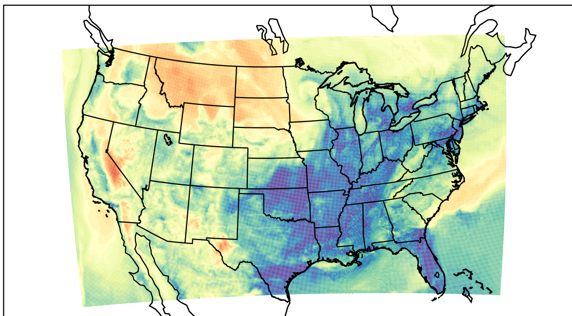
WRF (2022-04-18_11:00:00)
