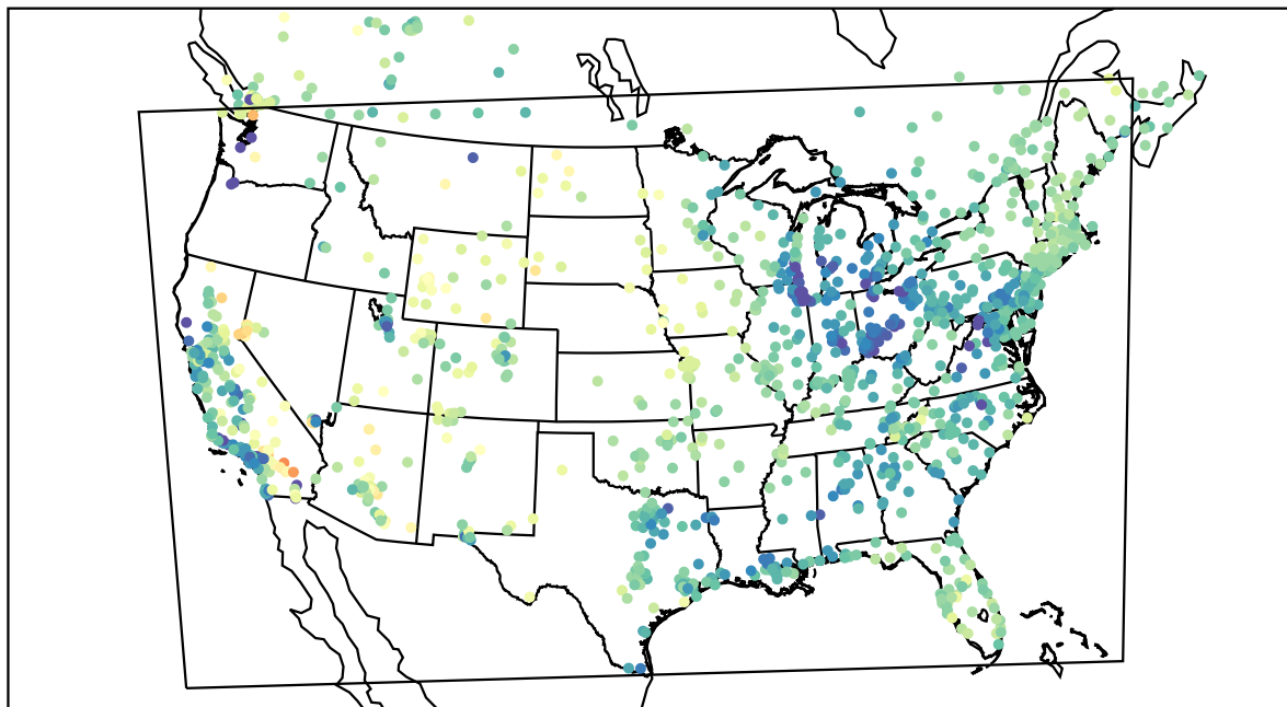
AirNOW (2022-04-18_16:00:00)
