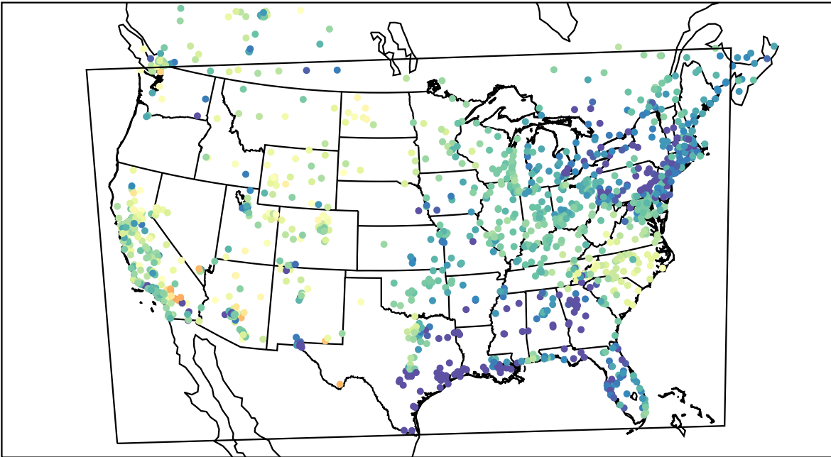
AirNOW (2022-04-18_03:00:00)
