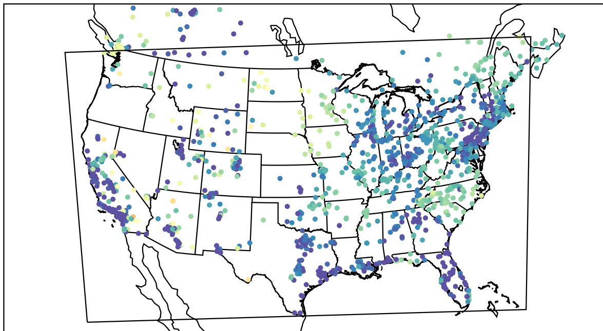
AirNOW (2022-04-18_12:00:00)
