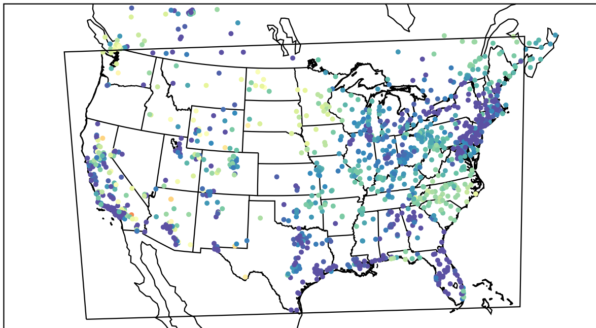
AirNOW (2022-04-18_11:00:00)
