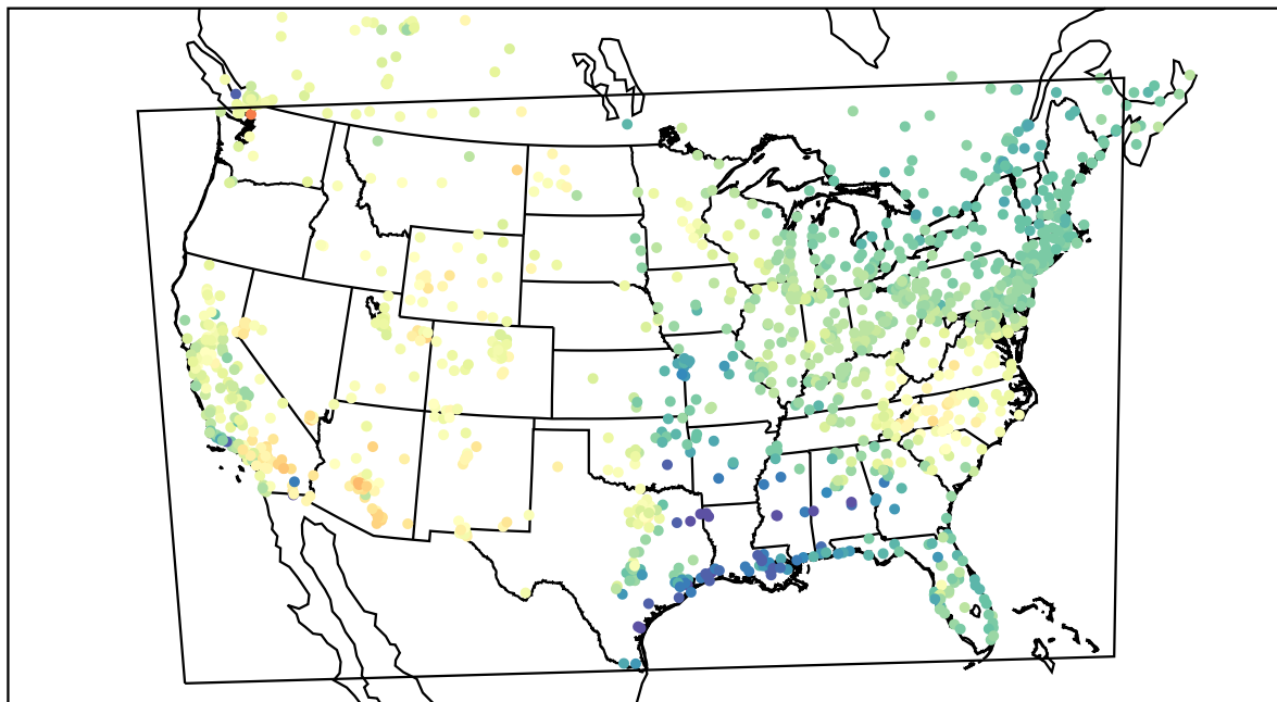
AirNOW (2022-04-17_20:00:00)
