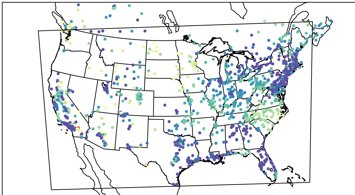
AirNOW (2022-04-18_10:00:00)
