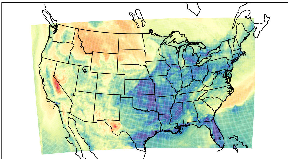
WRF (2022-04-18_08:00:00)
