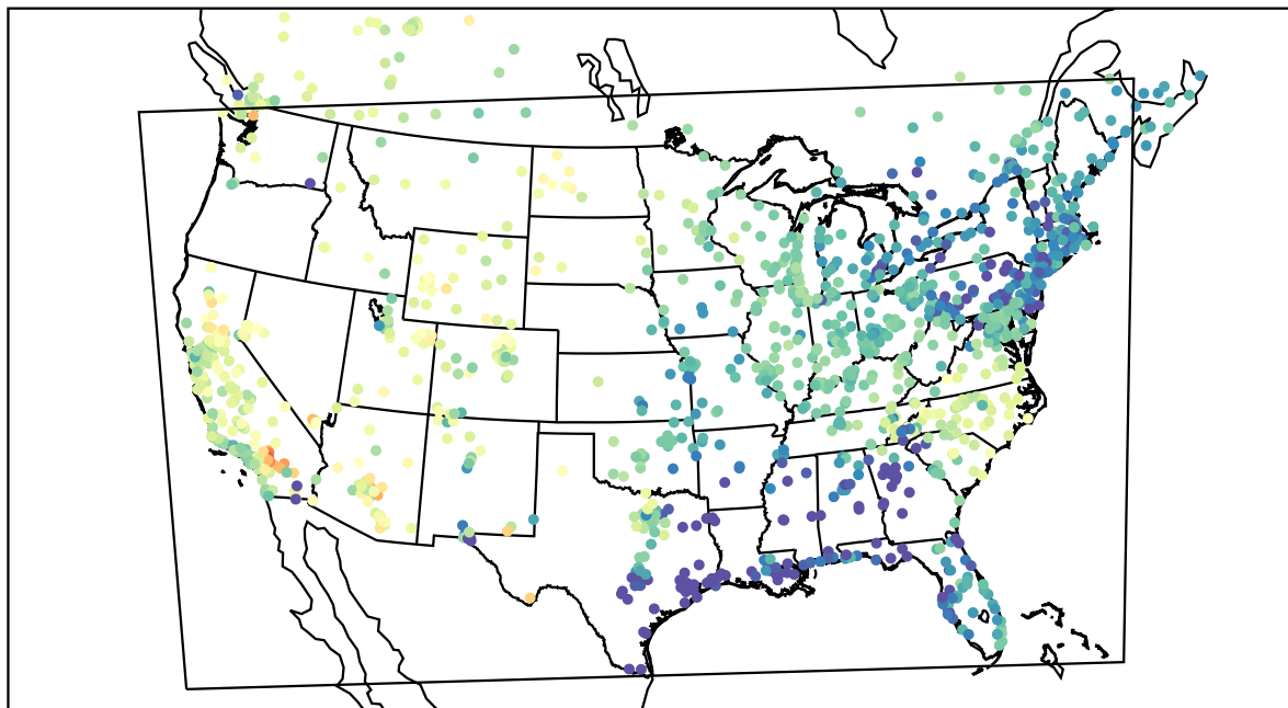
AirNOW (2022-04-18_02:00:00)
