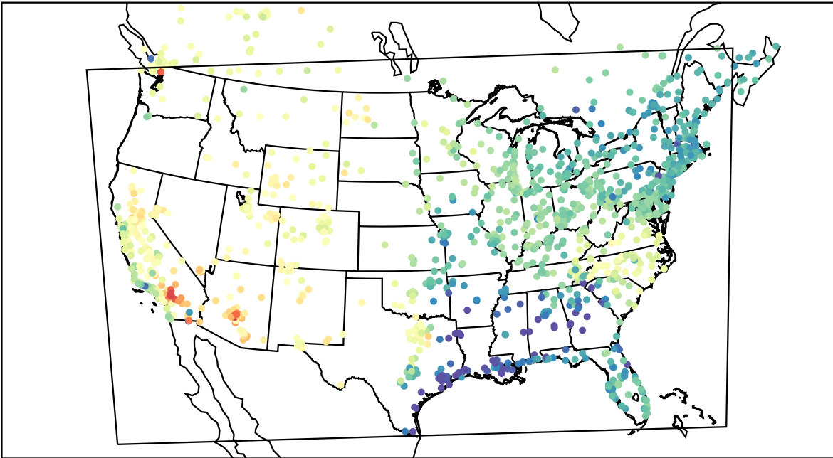
AirNOW (2022-04-18_00:00:00)
