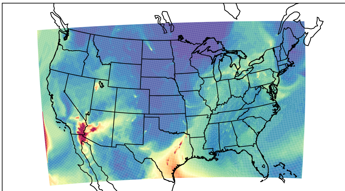
WRF 2022-05-03_15:00:00
