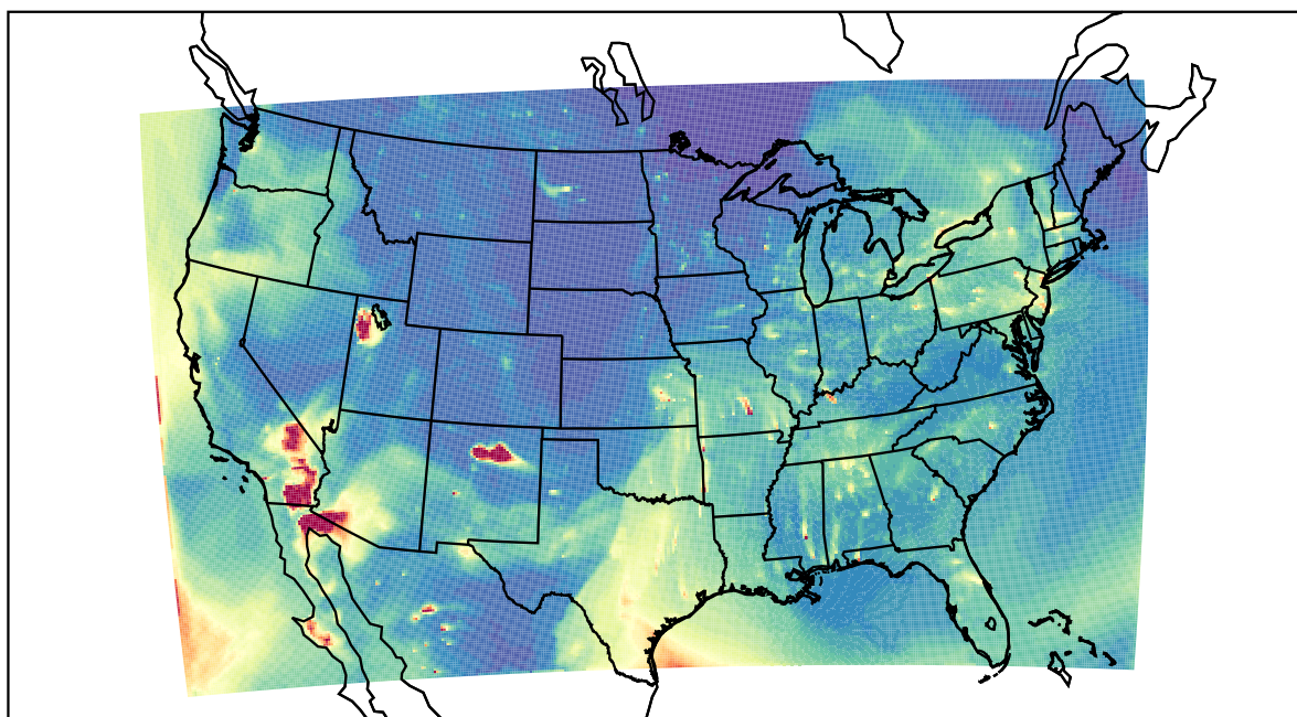
WRF 2022-05-03_02:00:00
