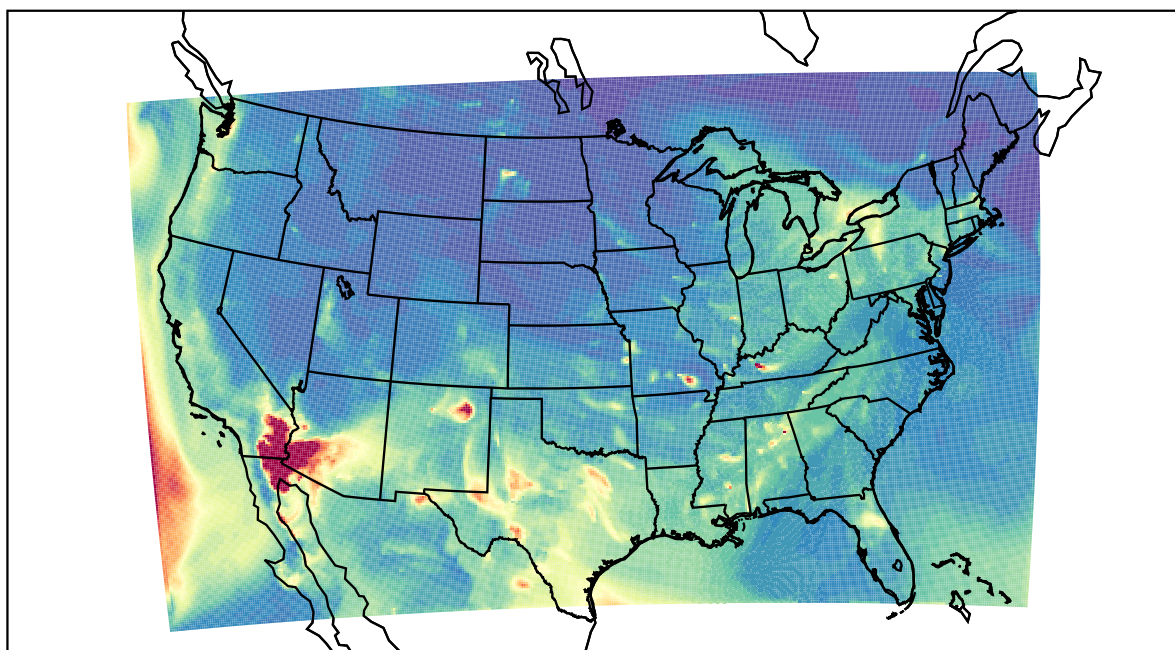
WRF 2022-05-02_06:00:00
