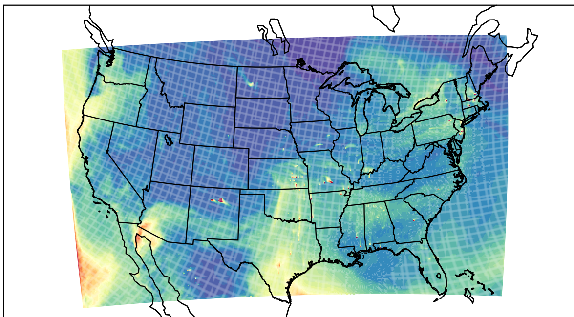
WRF 2022-05-02_21:00:00
