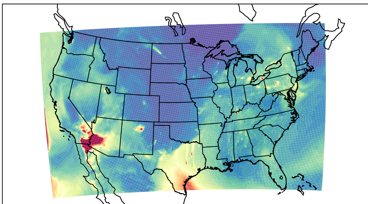
WRF 2022-05-03_09:00:00
