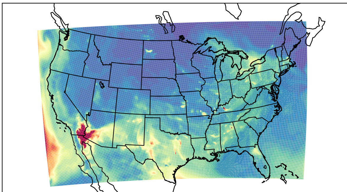
WRF 2022-05-02_08:00:00
