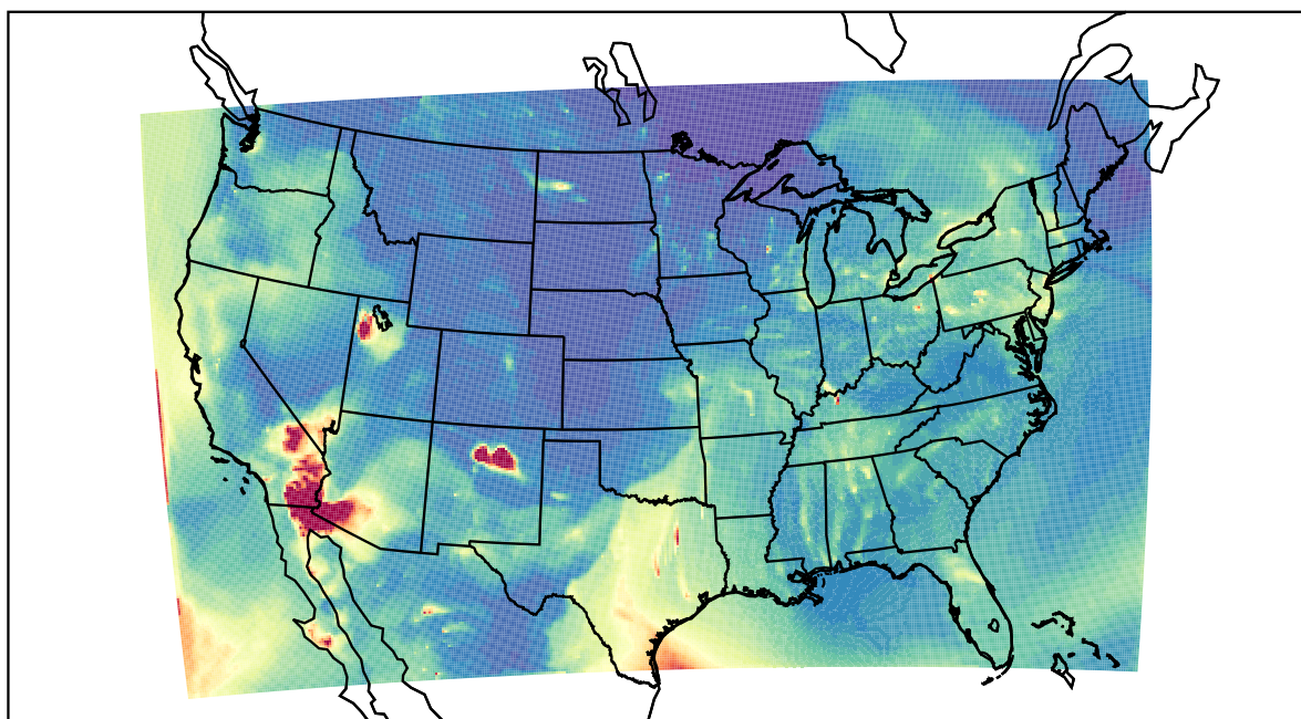
WRF 2022-05-03_04:00:00
