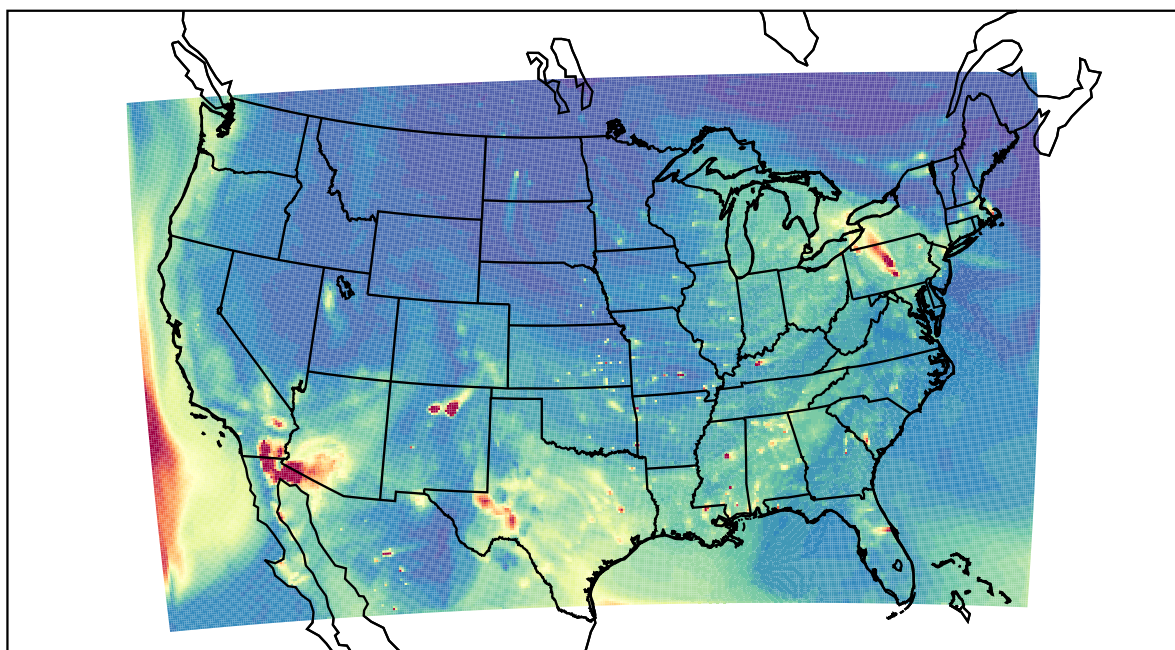
WRF 2022-05-02_01:00:00
