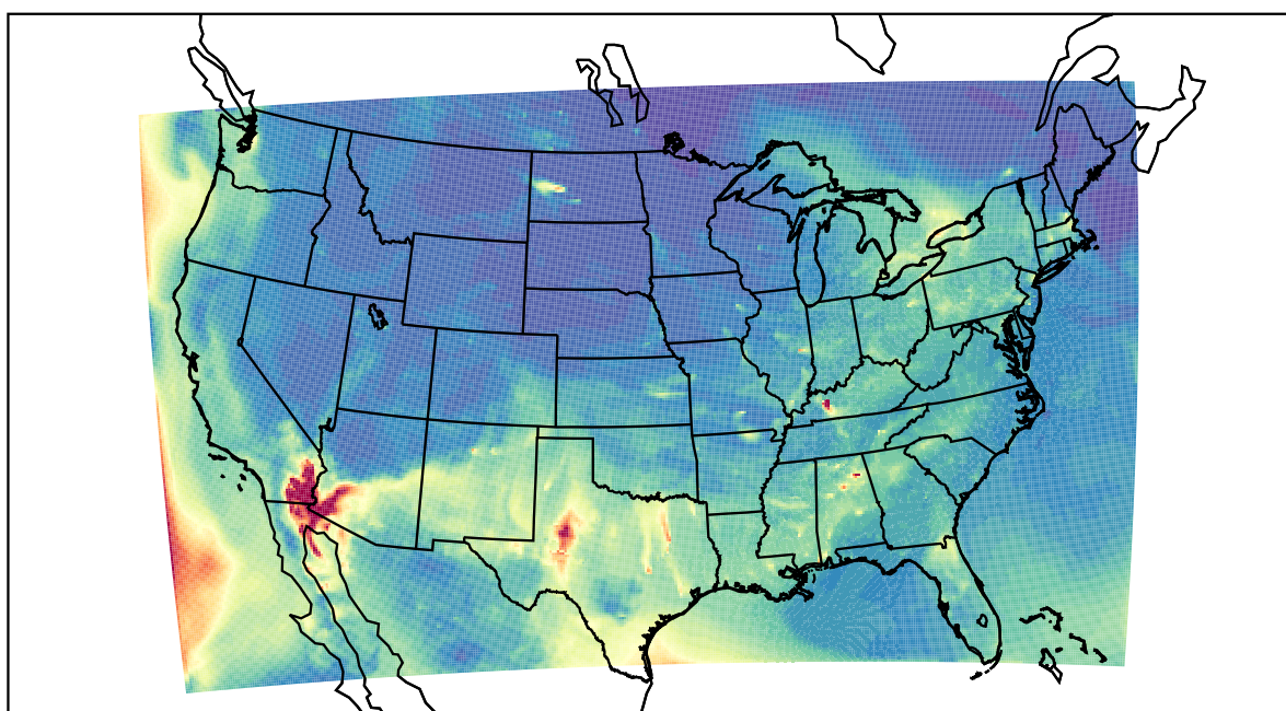
WRF 2022-05-02_11:00:00
