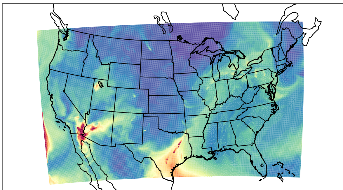
WRF 2022-05-03_16:00:00
