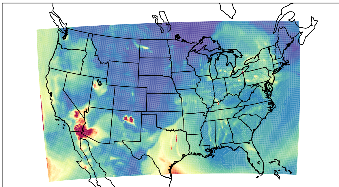
WRF 2022-05-03_05:00:00
