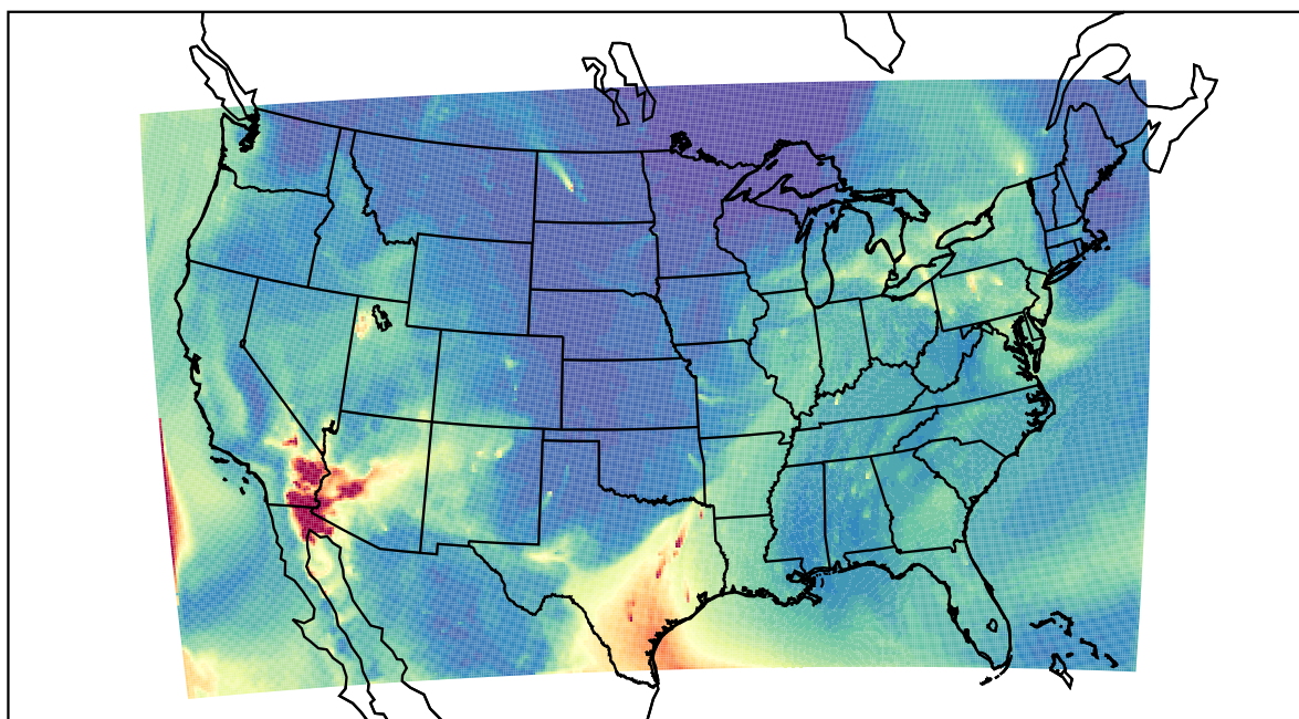
WRF 2022-05-03_14:00:00
