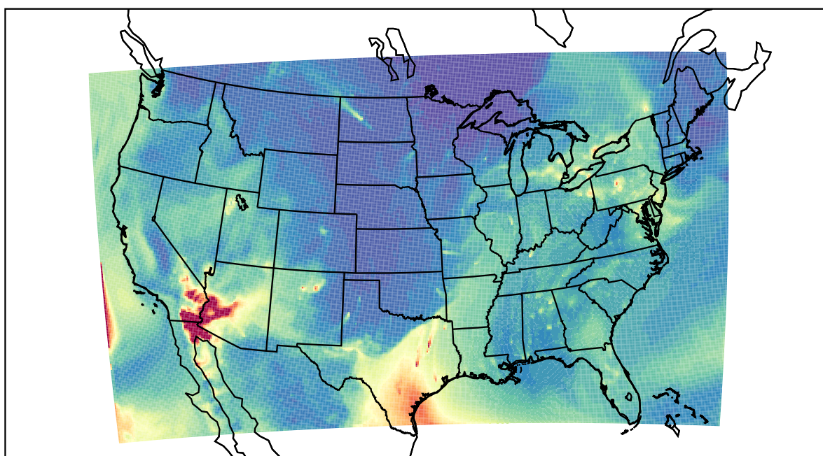
WRF 2022-05-03_12:00:00
