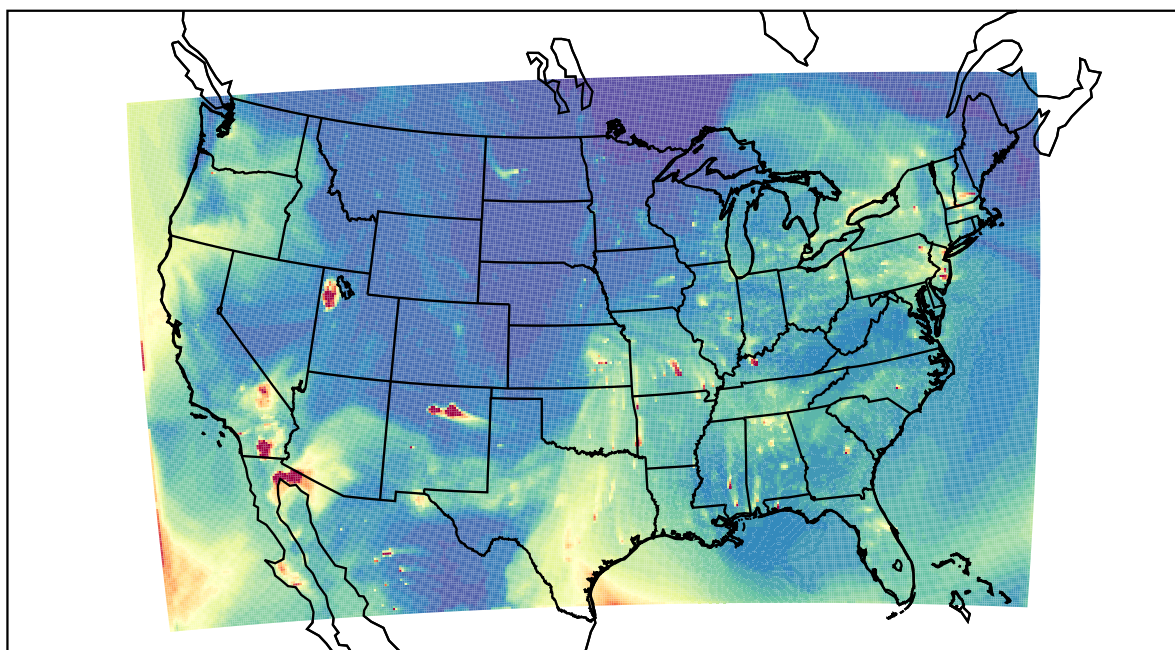
WRF 2022-05-03_01:00:00
