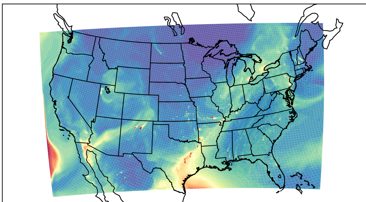
WRF 2022-05-03_22:00:00
