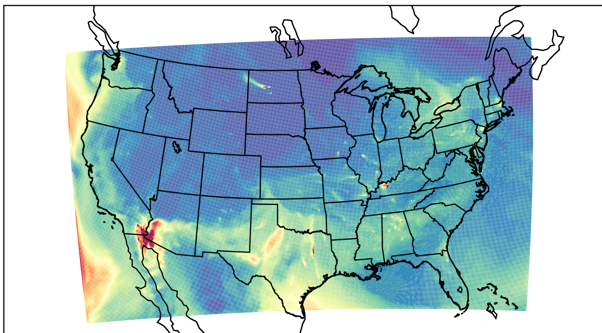
WRF 2022-05-02_15:00:00
