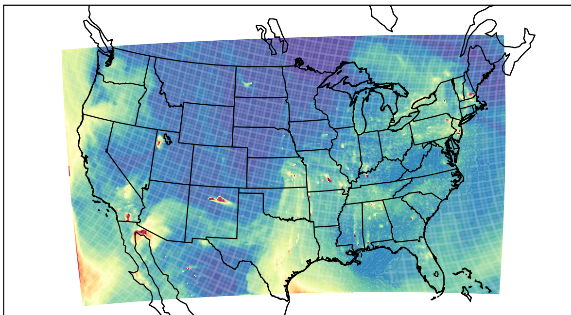
WRF 2022-05-03_00:00:00
