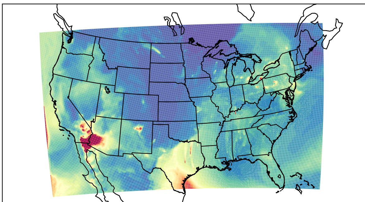
WRF 2022-05-03_08:00:00
