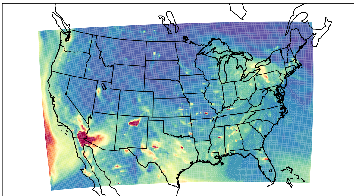
WRF 2022-05-02_03:00:00
