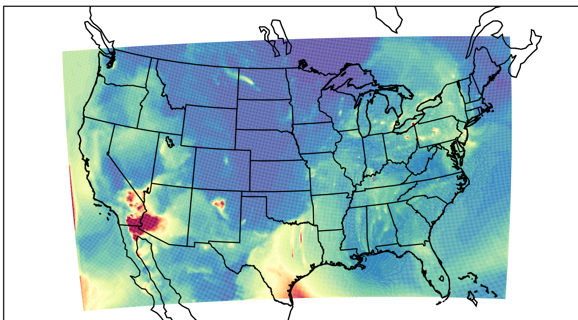
WRF 2022-05-03_07:00:00
