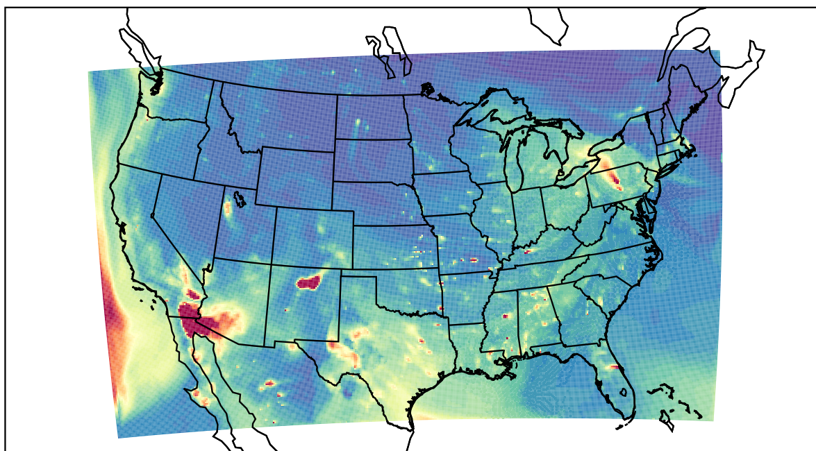
WRF 2022-05-02_02:00:00
