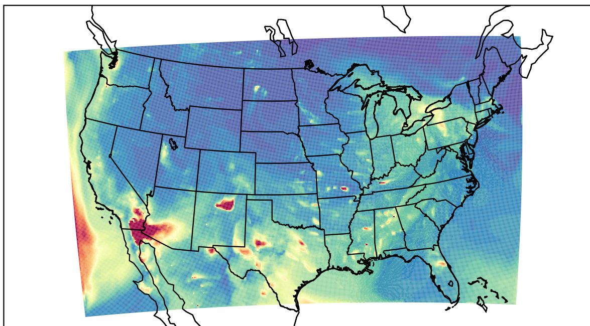
WRF 2022-05-02_04:00:00
