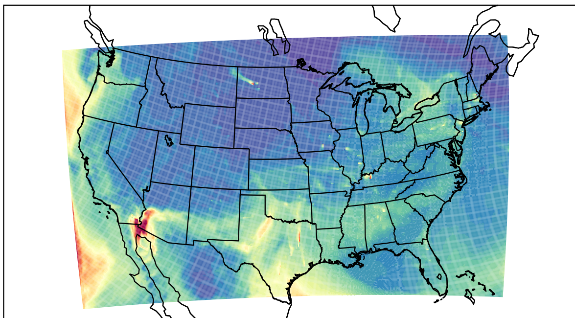
WRF 2022-05-02_16:00:00
