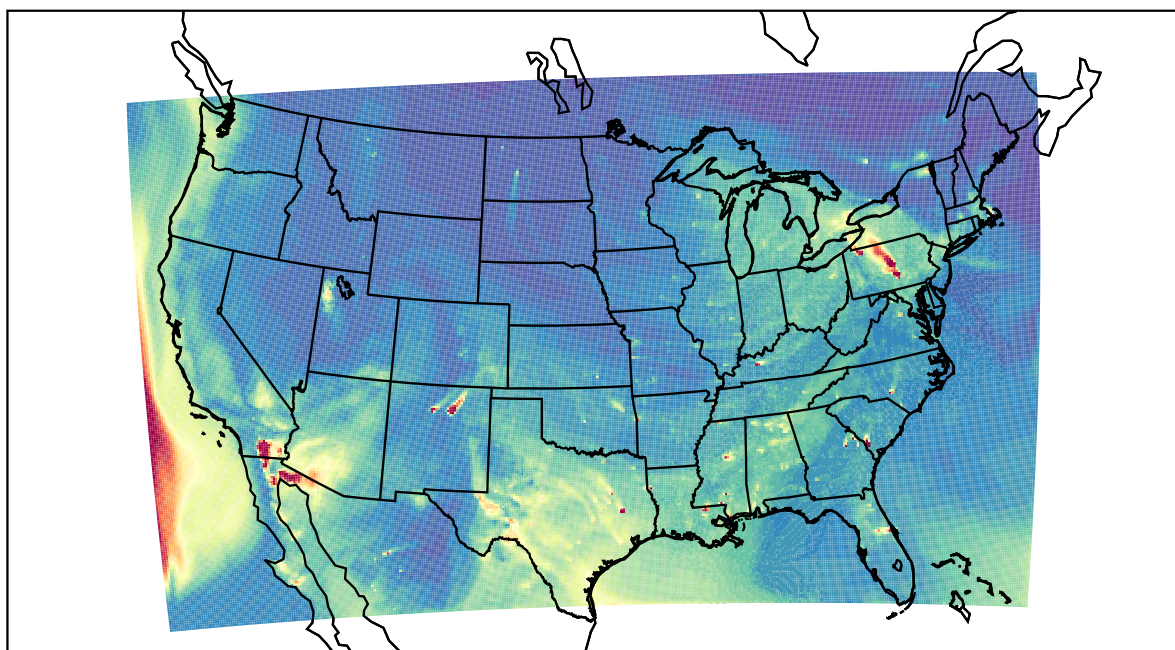
WRF 2022-05-02_00:00:00
