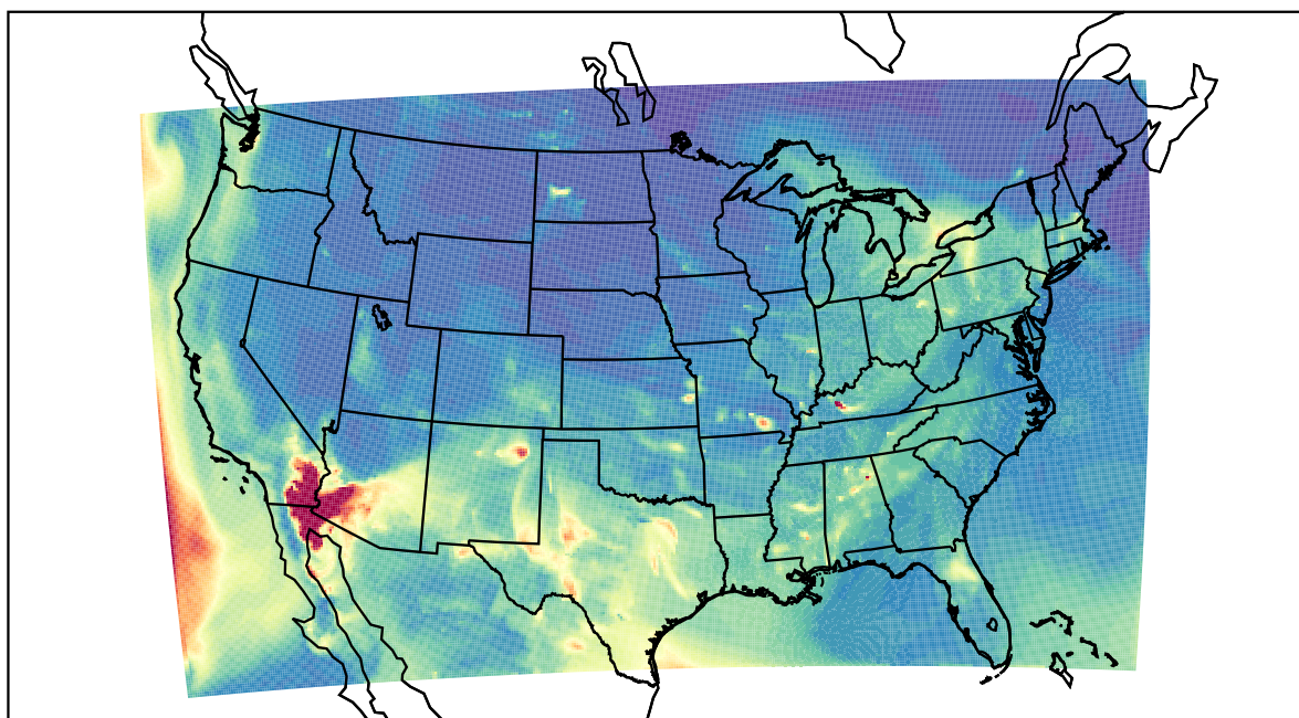
WRF 2022-05-02_07:00:00
