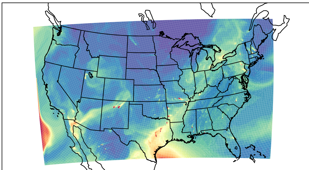
WRF 2022-05-03_23:00:00
