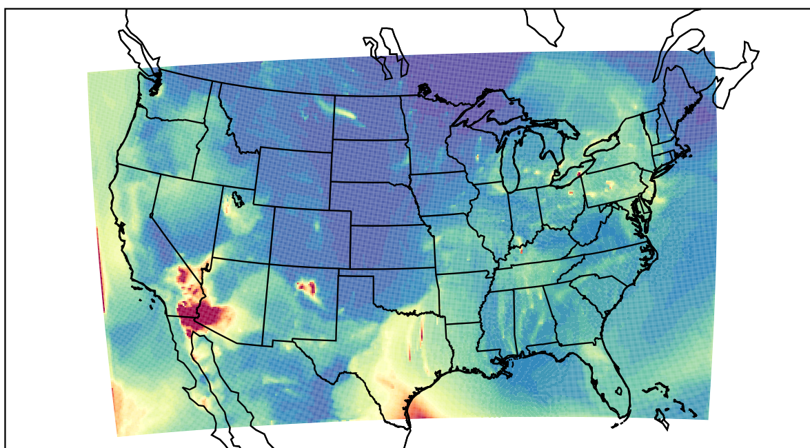
WRF 2022-05-03_06:00:00
