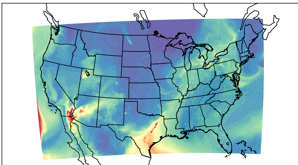
WRF 2022-05-03_17:00:00
