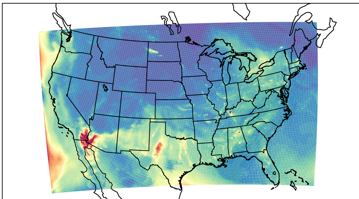
WRF 2022-05-02_12:00:00
