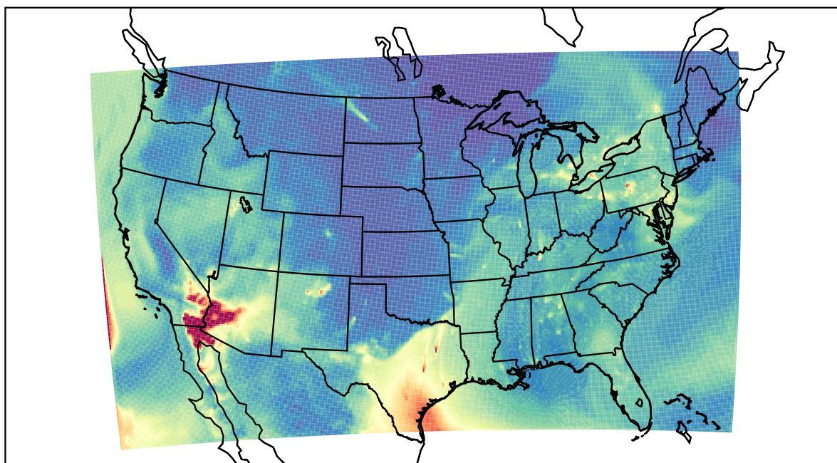
WRF 2022-05-03_11:00:00
