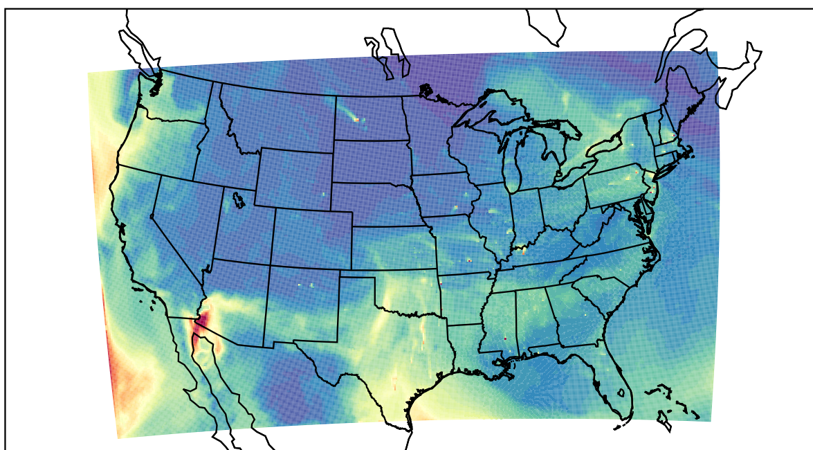
WRF 2022-05-02_18:00:00
