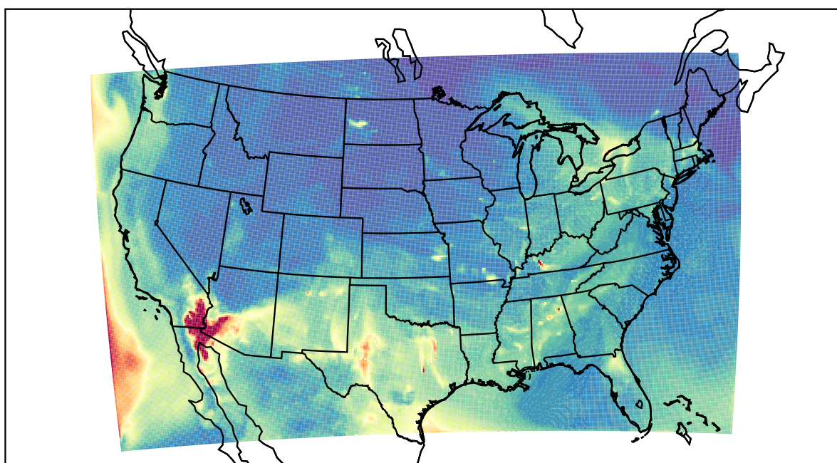
WRF 2022-05-02_09:00:00
