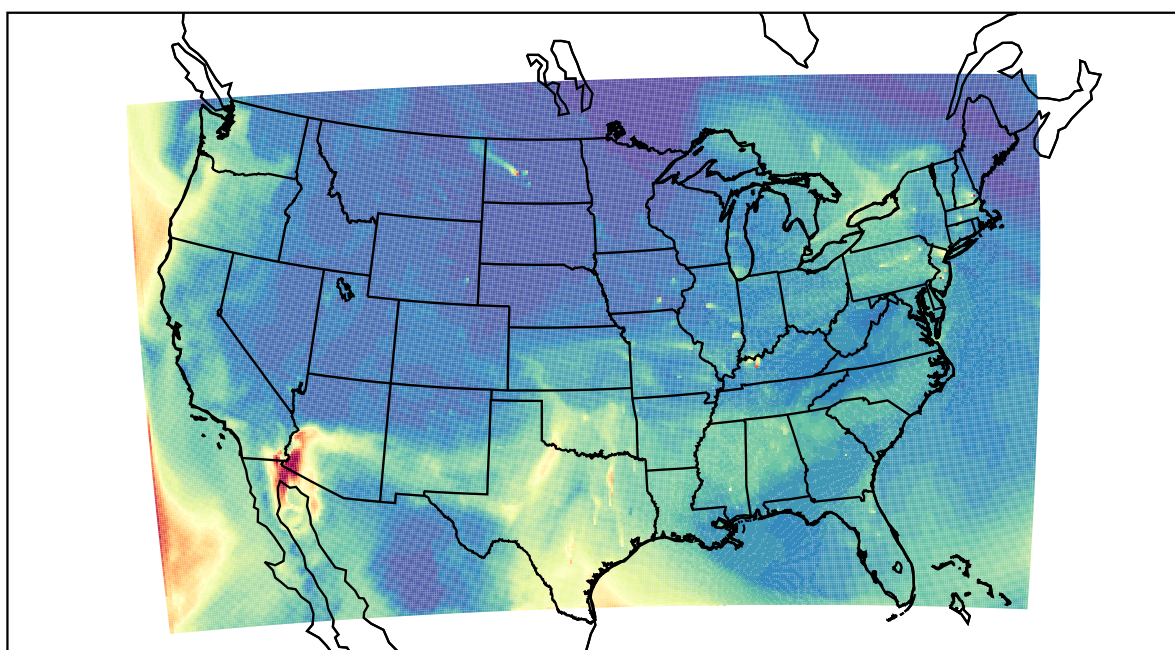
WRF 2022-05-02_17:00:00
