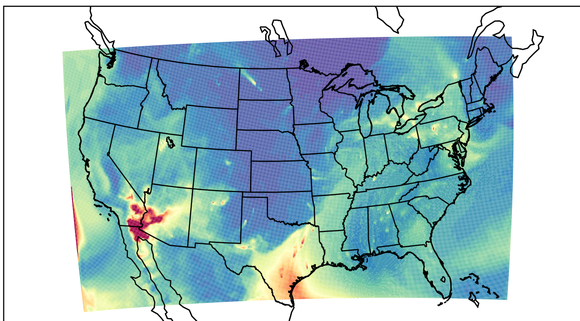
WRF 2022-05-03_13:00:00
