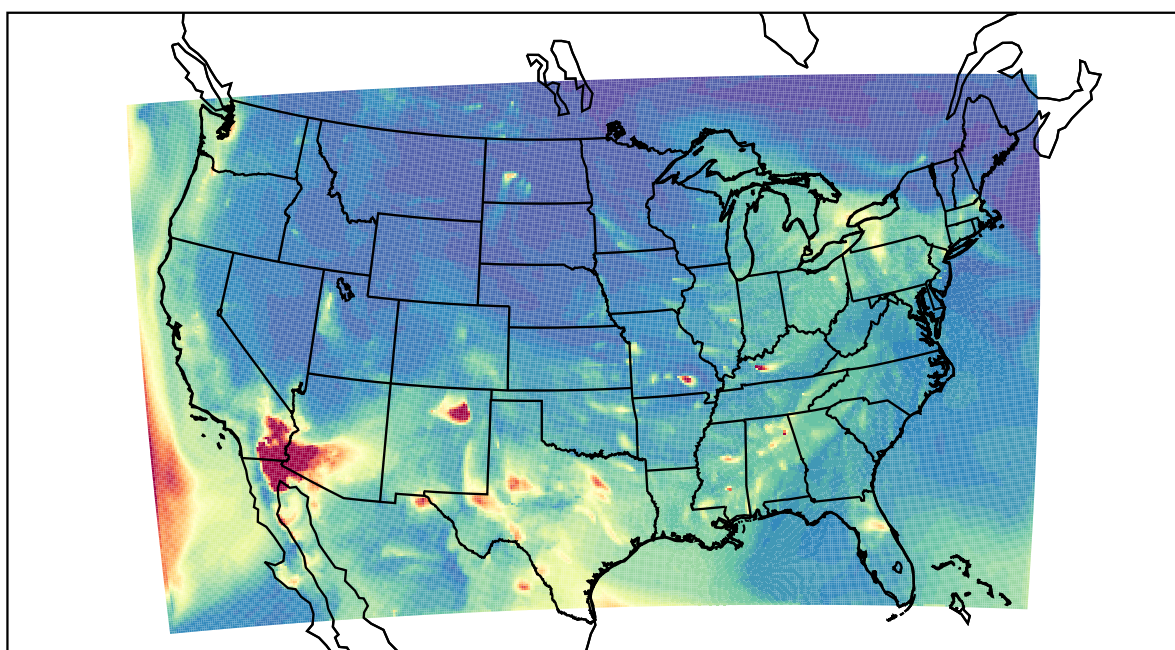
WRF 2022-05-02_05:00:00
