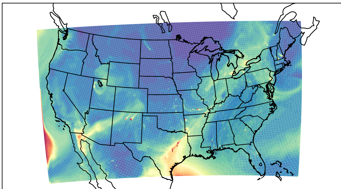
WRF 2022-05-03_21:00:00
