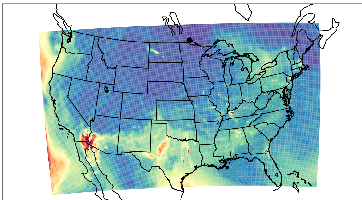
WRF 2022-05-02_14:00:00
