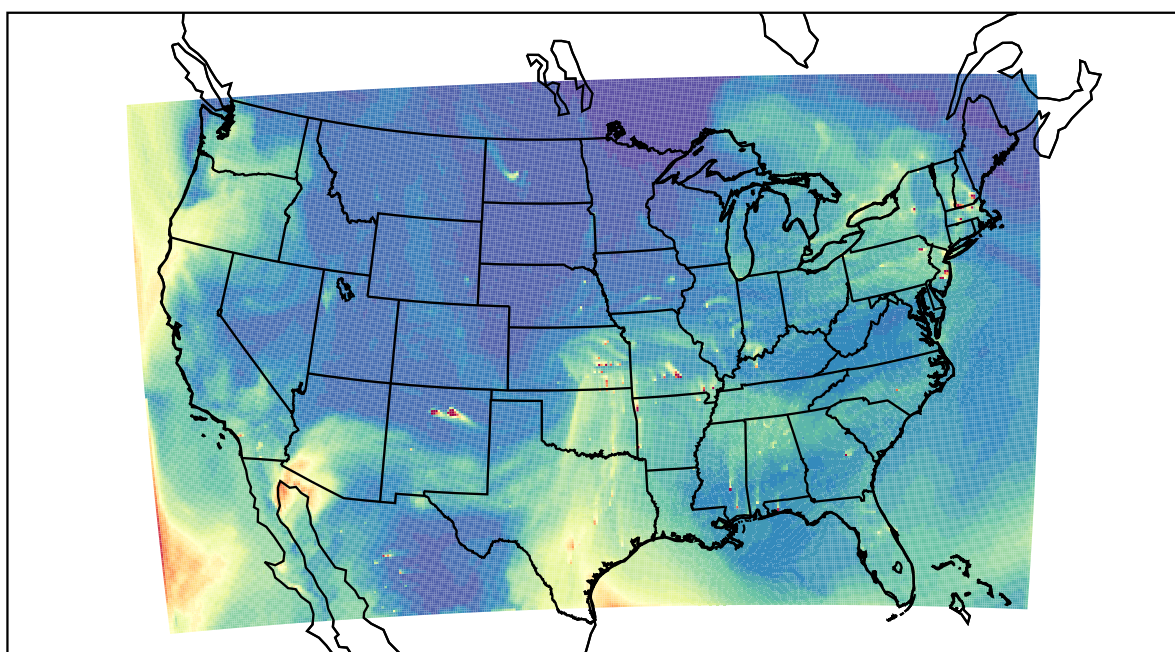
WRF 2022-05-02_22:00:00
