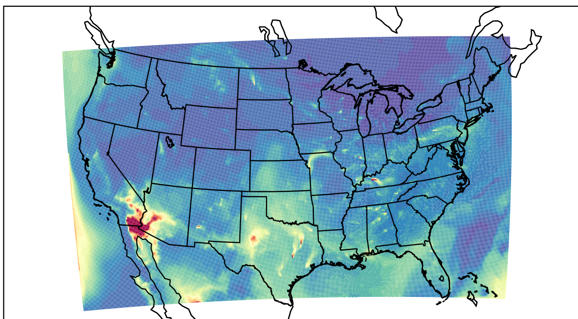
WRF 2022-05-17_13:00:00
