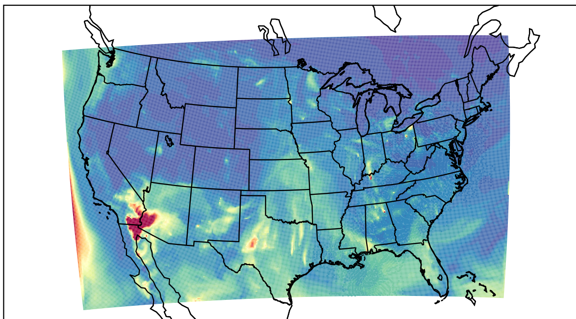
WRF 2022-05-18_08:00:00
