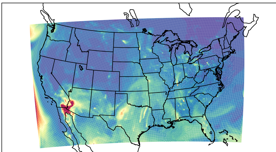
WRF 2022-05-18_12:00:00
