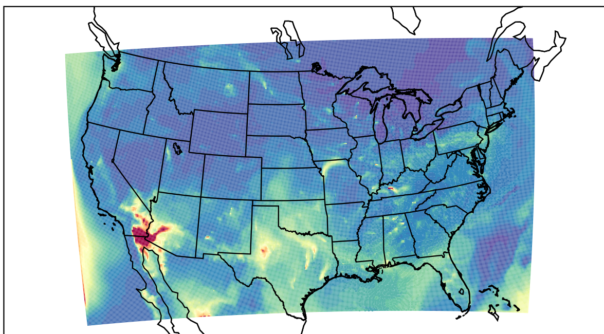
WRF 2022-05-17_12:00:00
