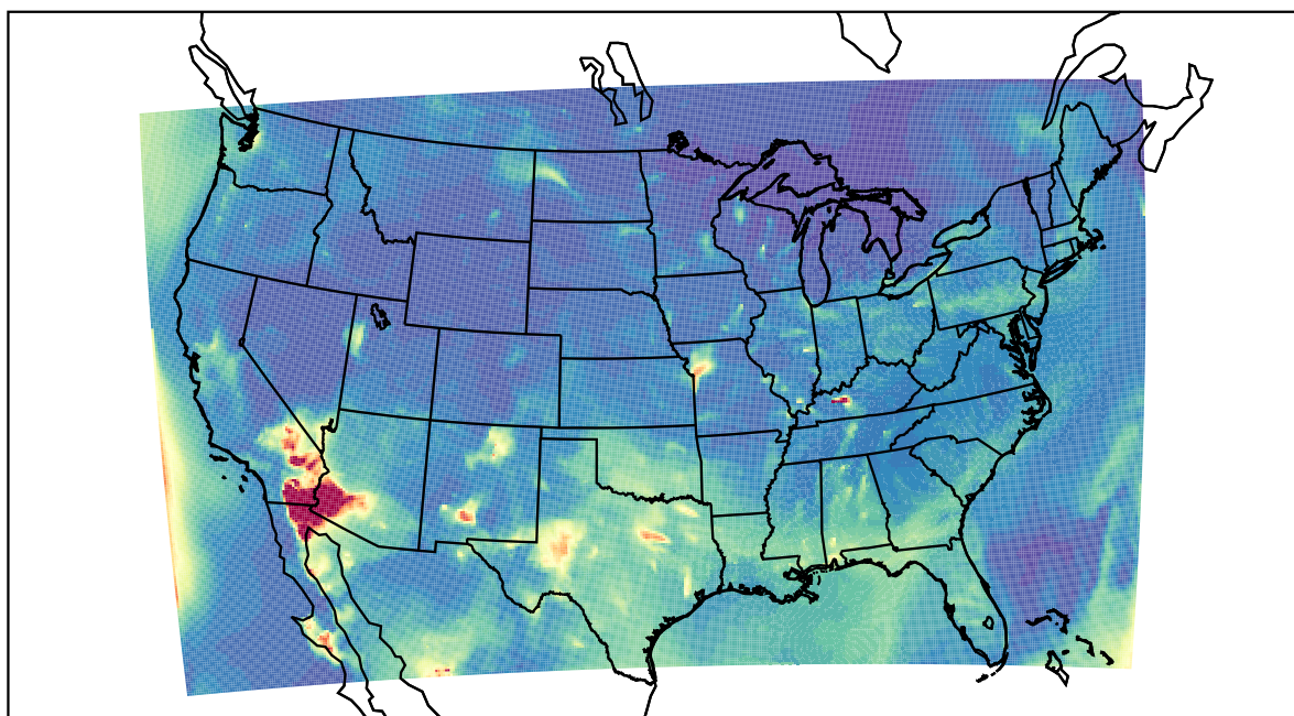
WRF 2022-05-17_06:00:00
