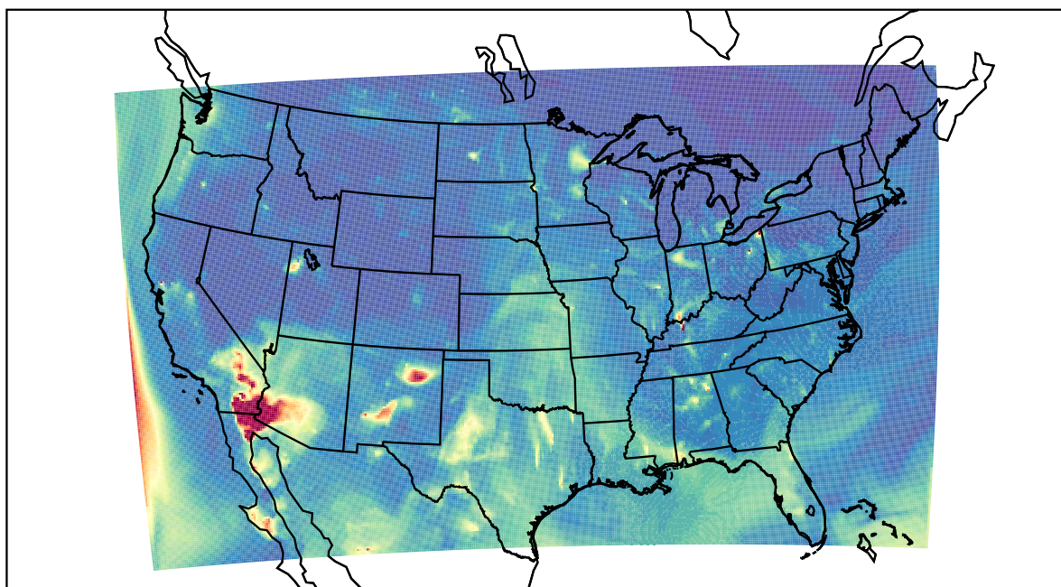
WRF 2022-05-18_05:00:00
