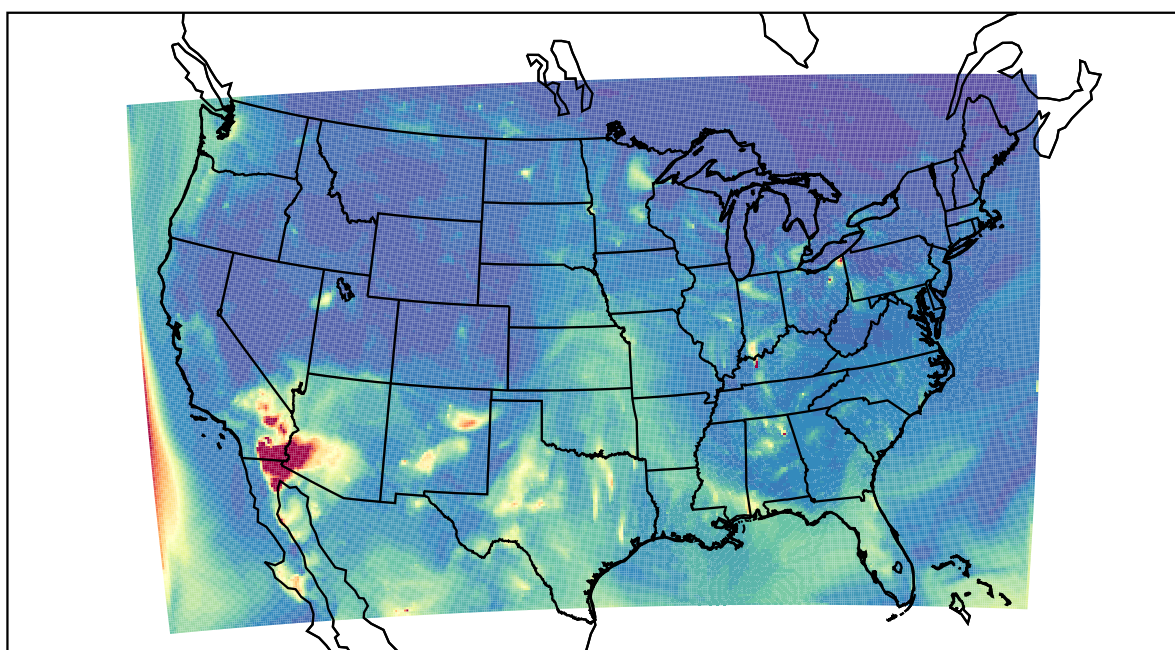
WRF 2022-05-18_06:00:00
