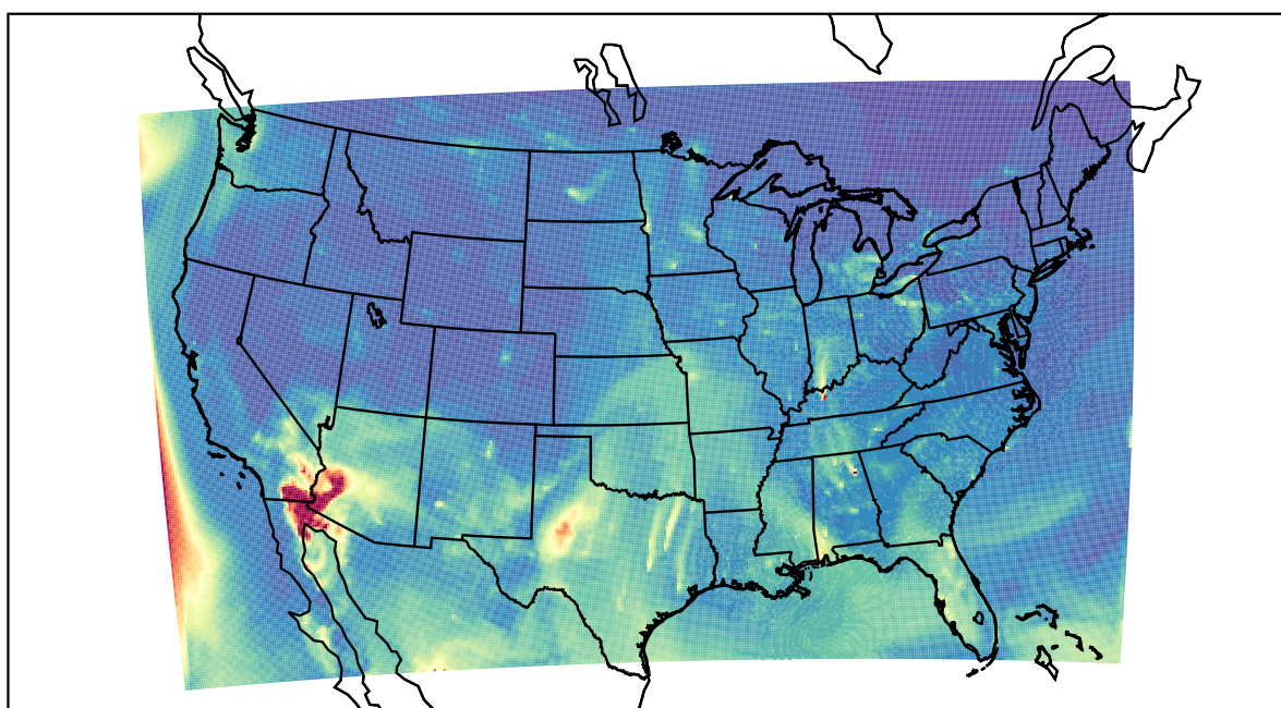
WRF 2022-05-18_11:00:00
