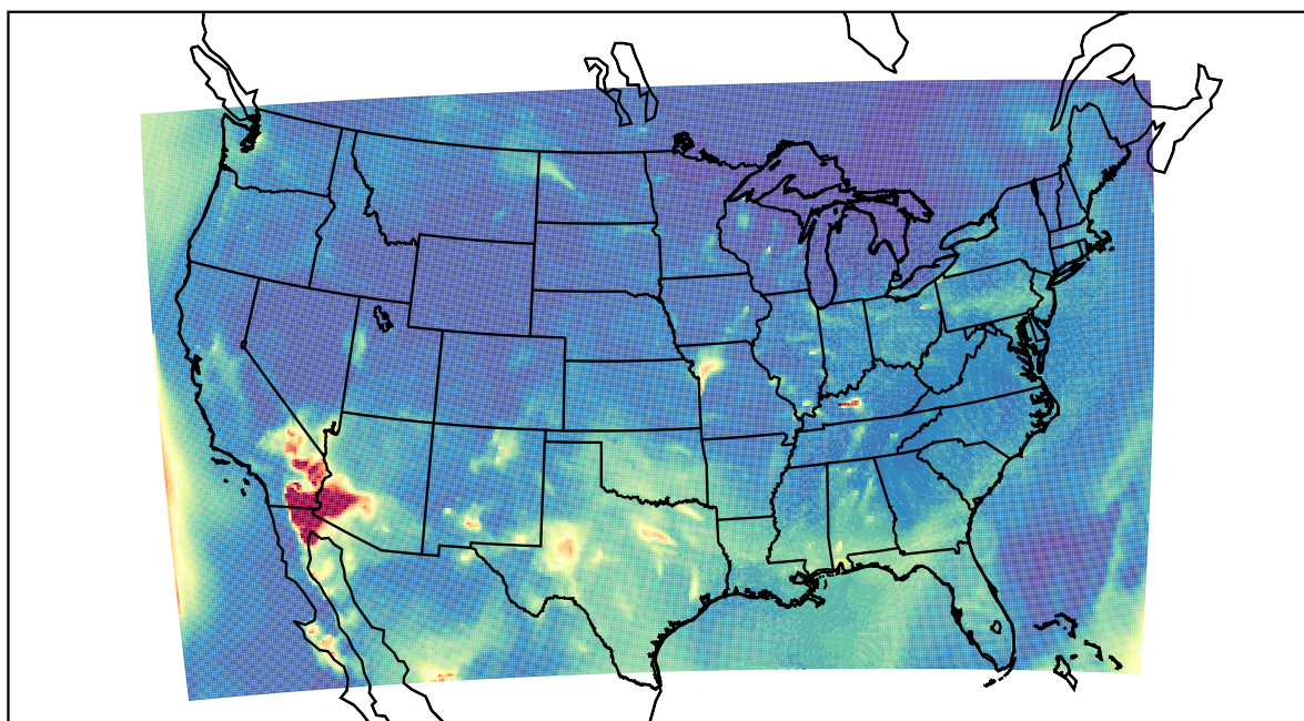
WRF 2022-05-17_07:00:00
