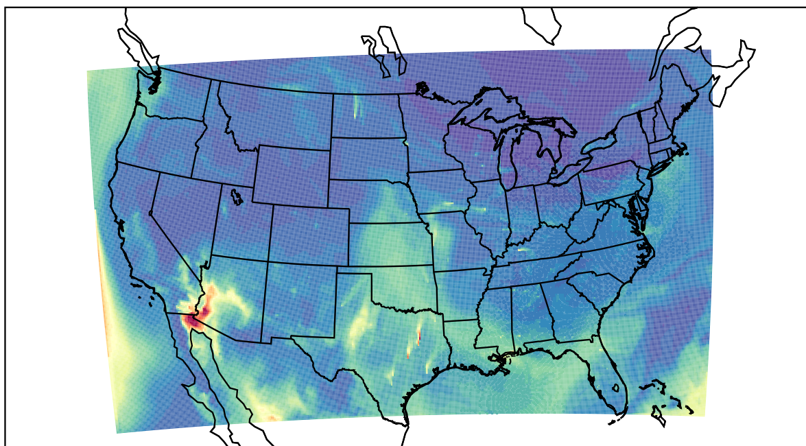
WRF 2022-05-17_17:00:00
