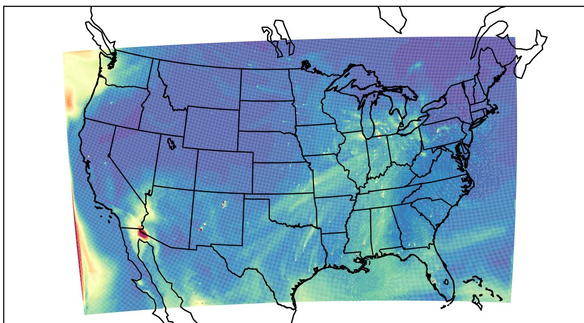
WRF 2022-05-18_21:00:00
