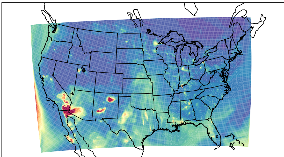
WRF 2022-05-18_04:00:00
