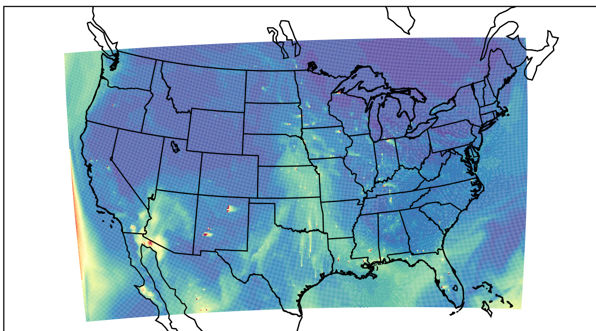
WRF 2022-05-17_23:00:00
