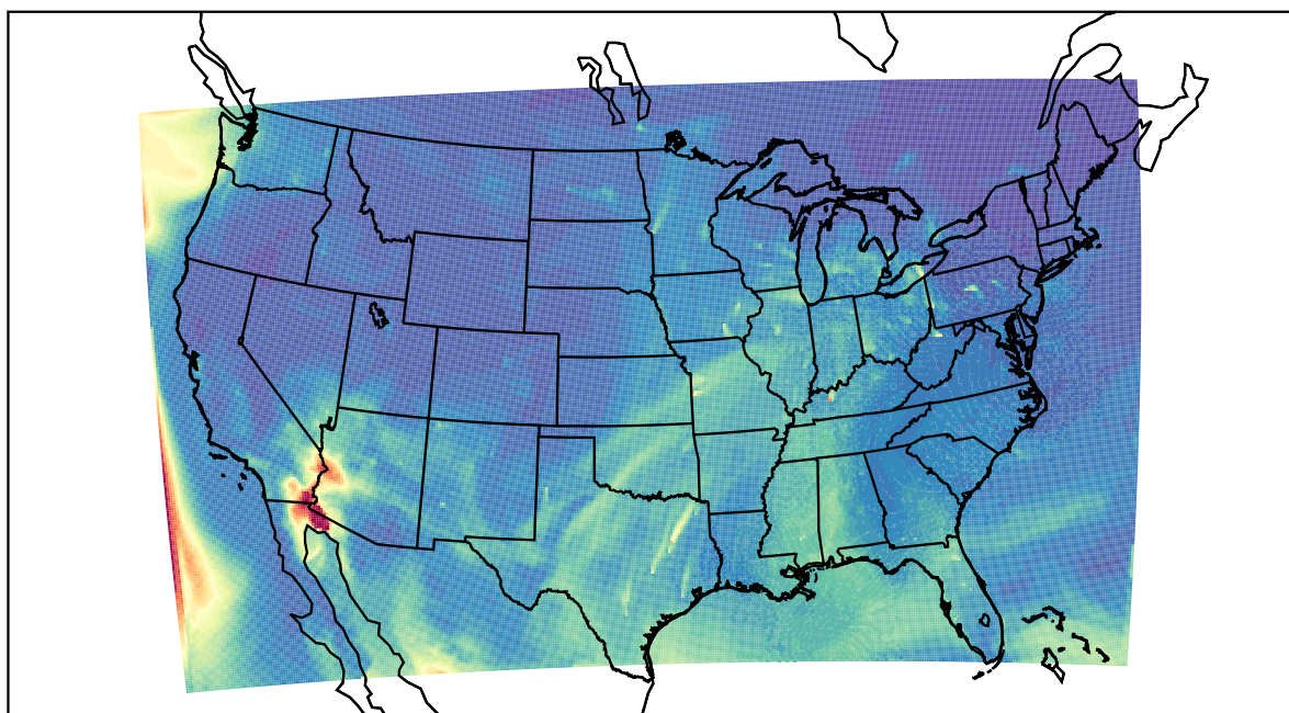
WRF 2022-05-18_17:00:00
