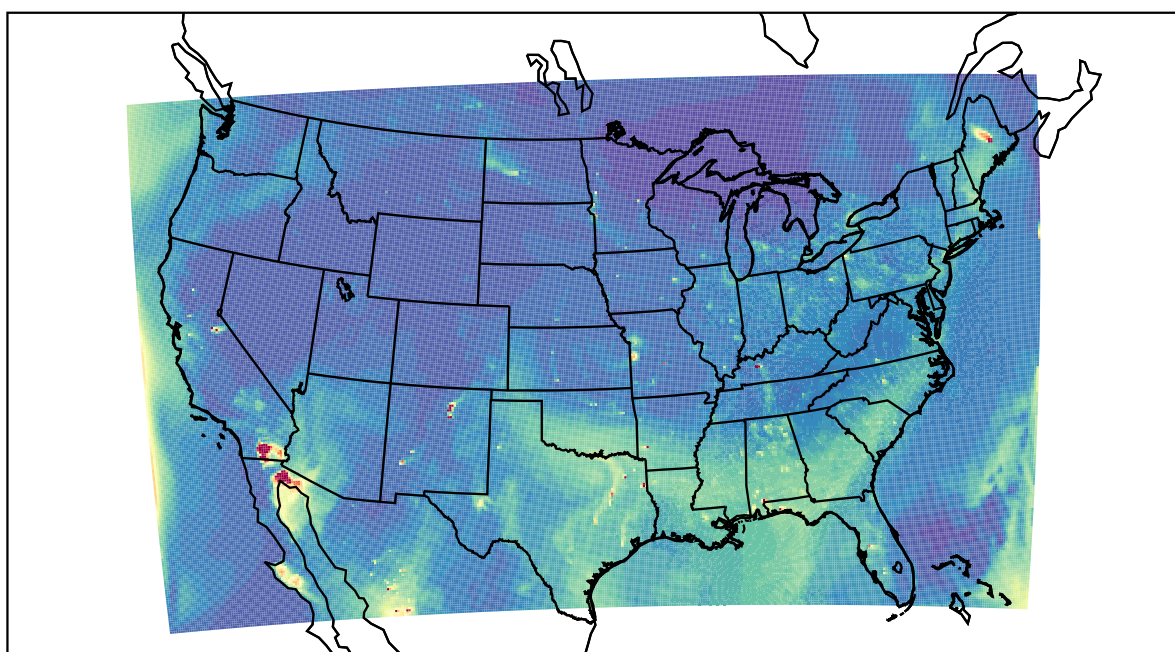
WRF 2022-05-17_00:00:00
