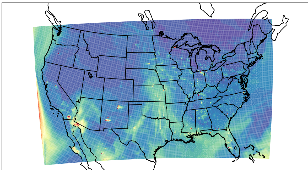
WRF 2022-05-18_00:00:00
