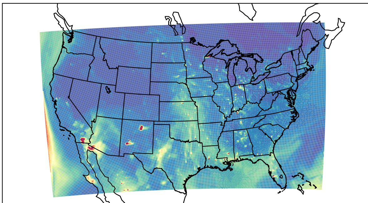
WRF 2022-05-18_01:00:00
