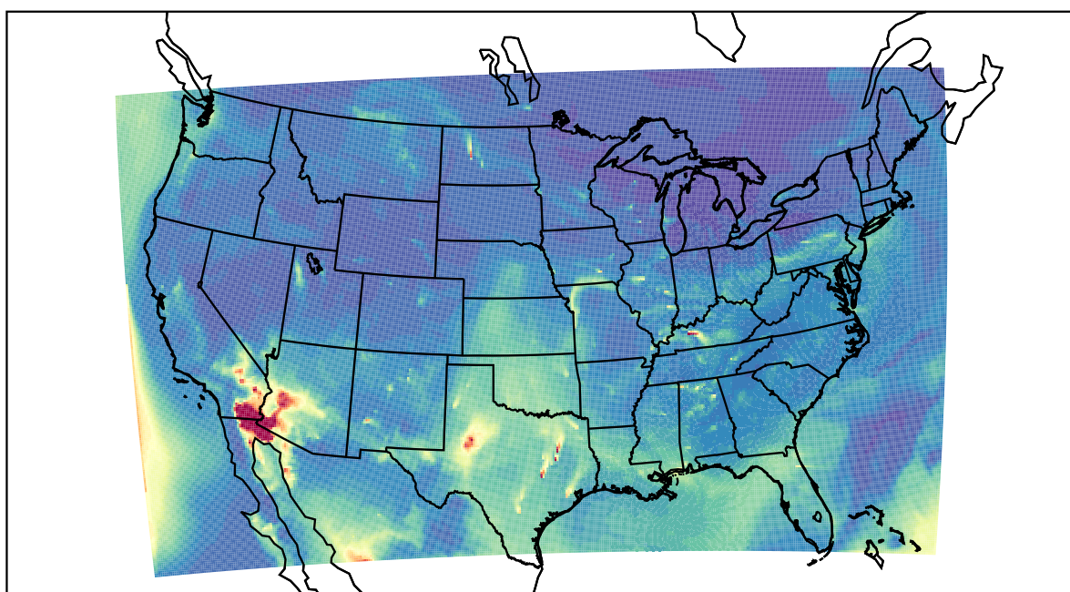
WRF 2022-05-17_14:00:00
