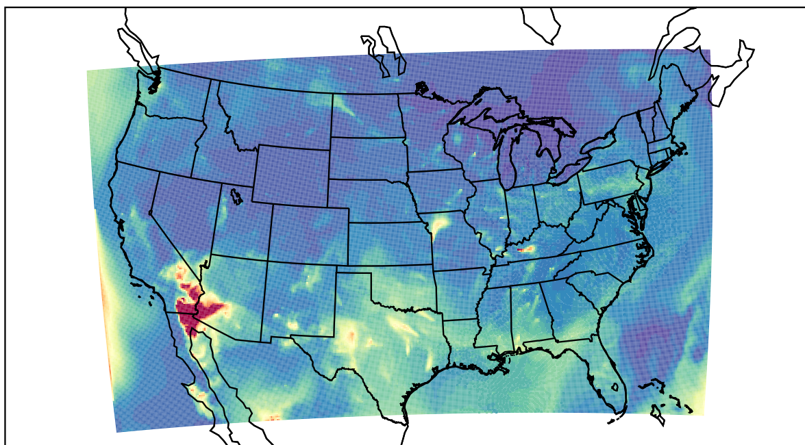
WRF 2022-05-17_08:00:00
