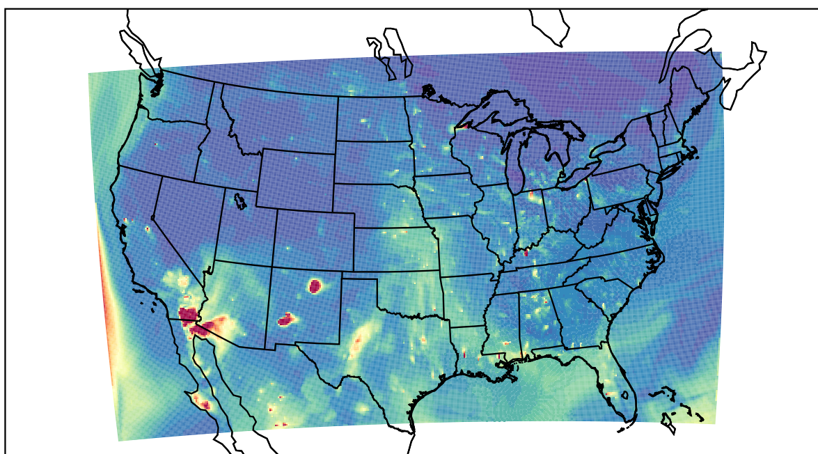
WRF 2022-05-18_02:00:00
