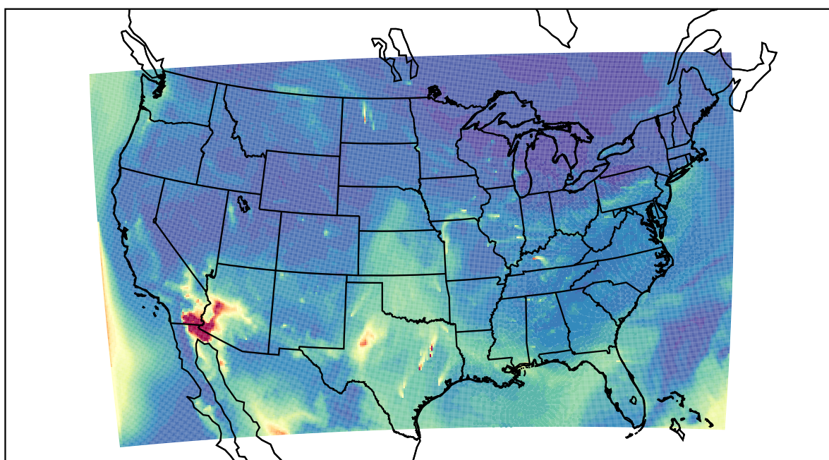
WRF 2022-05-17_15:00:00
