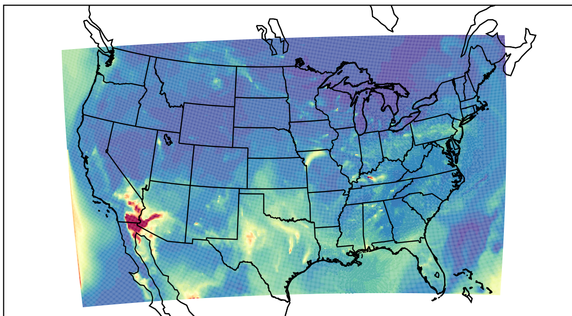
WRF 2022-05-17_11:00:00
