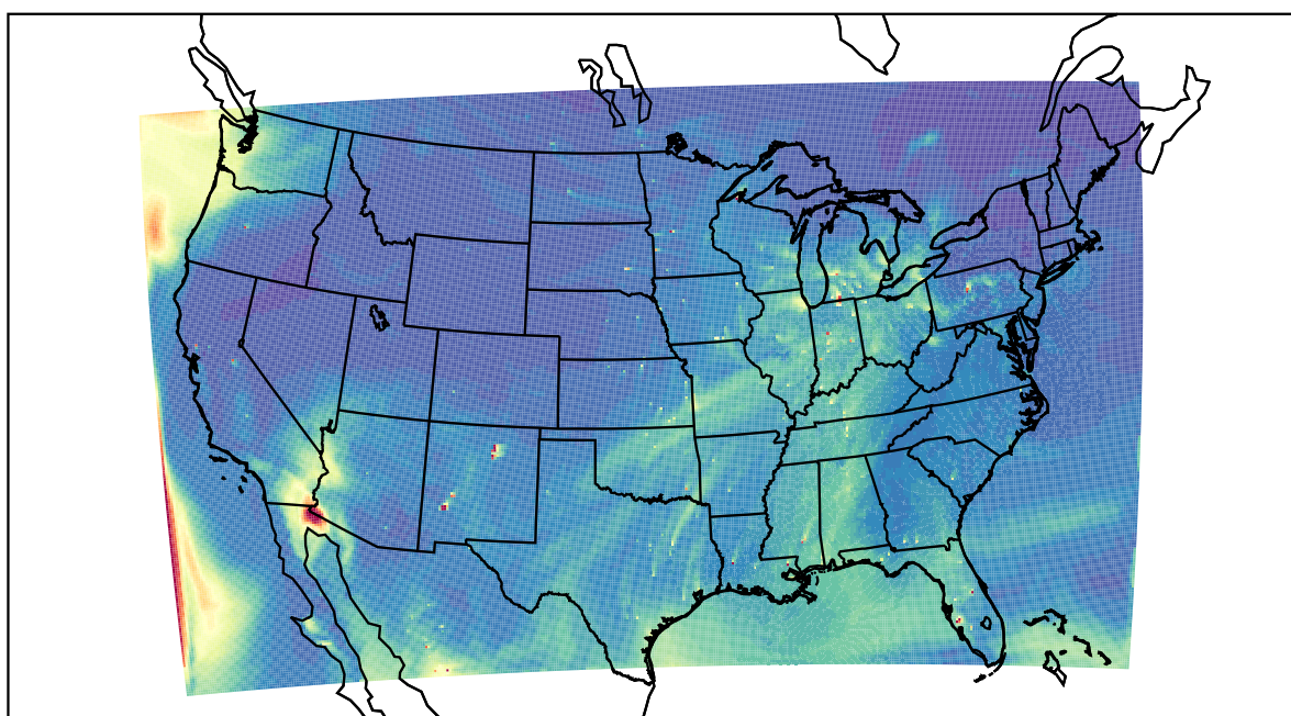
WRF 2022-05-18_22:00:00
