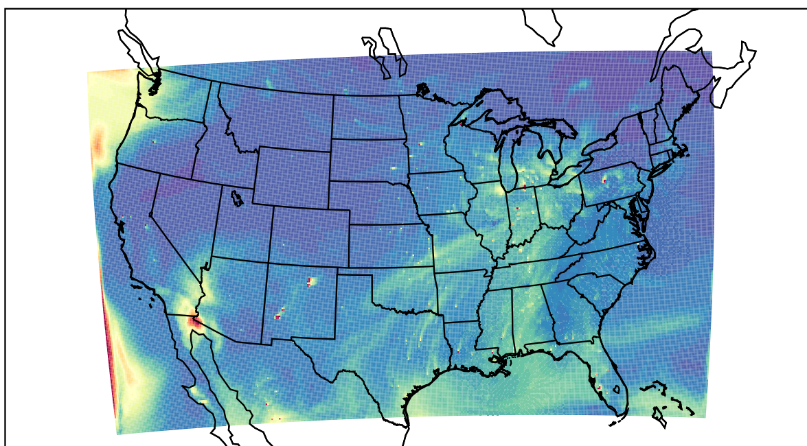
WRF 2022-05-18_23:00:00
