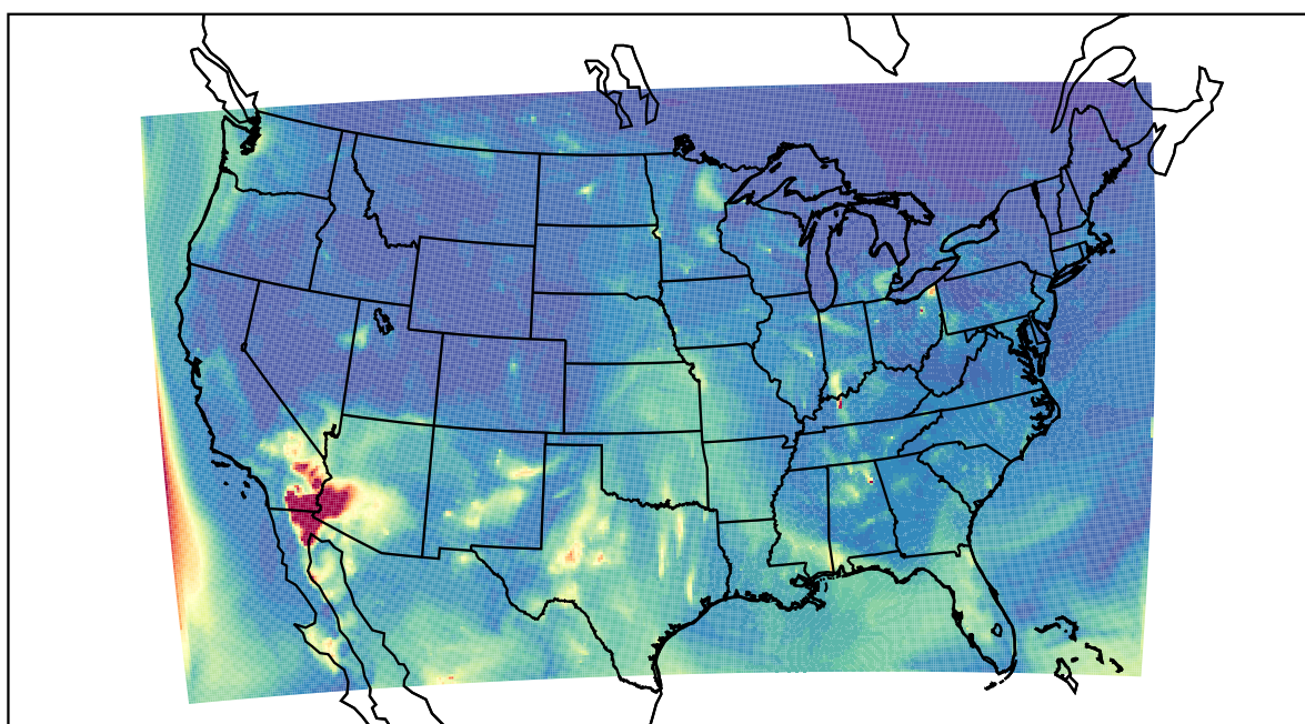
WRF 2022-05-18_07:00:00
