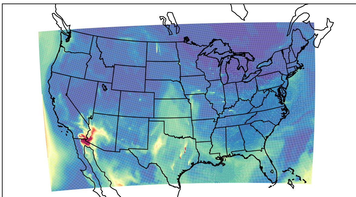
WRF 2022-05-17_16:00:00
