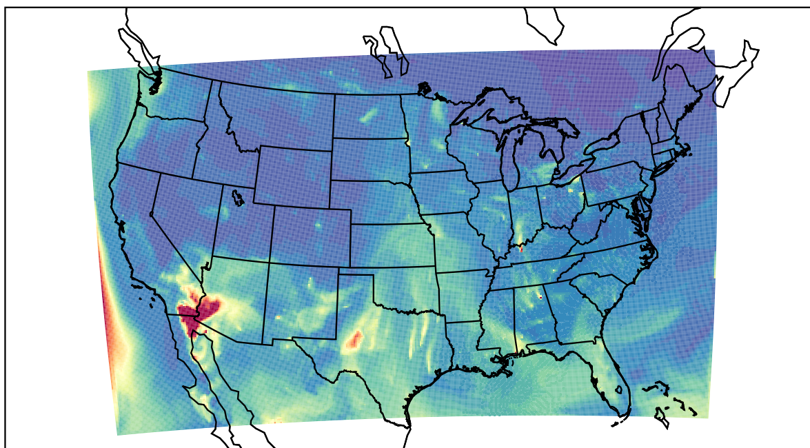
WRF 2022-05-18_09:00:00
