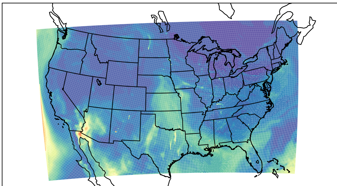
WRF 2022-05-17_19:00:00
