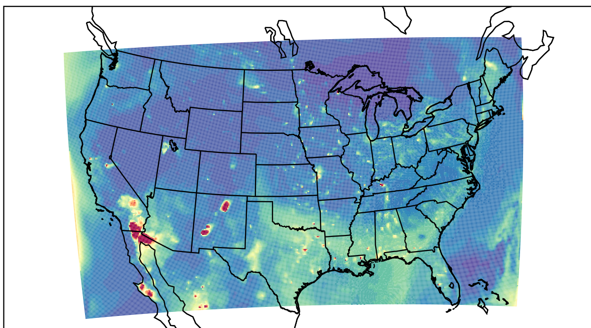
WRF 2022-05-17_02:00:00
