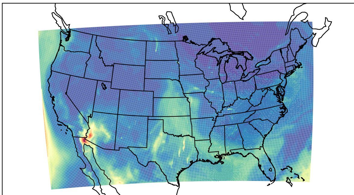
WRF 2022-05-17_18:00:00
