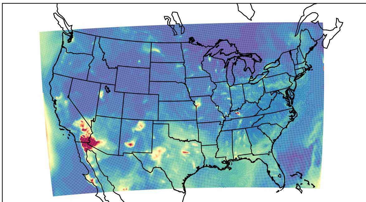
WRF 2022-05-17_05:00:00
