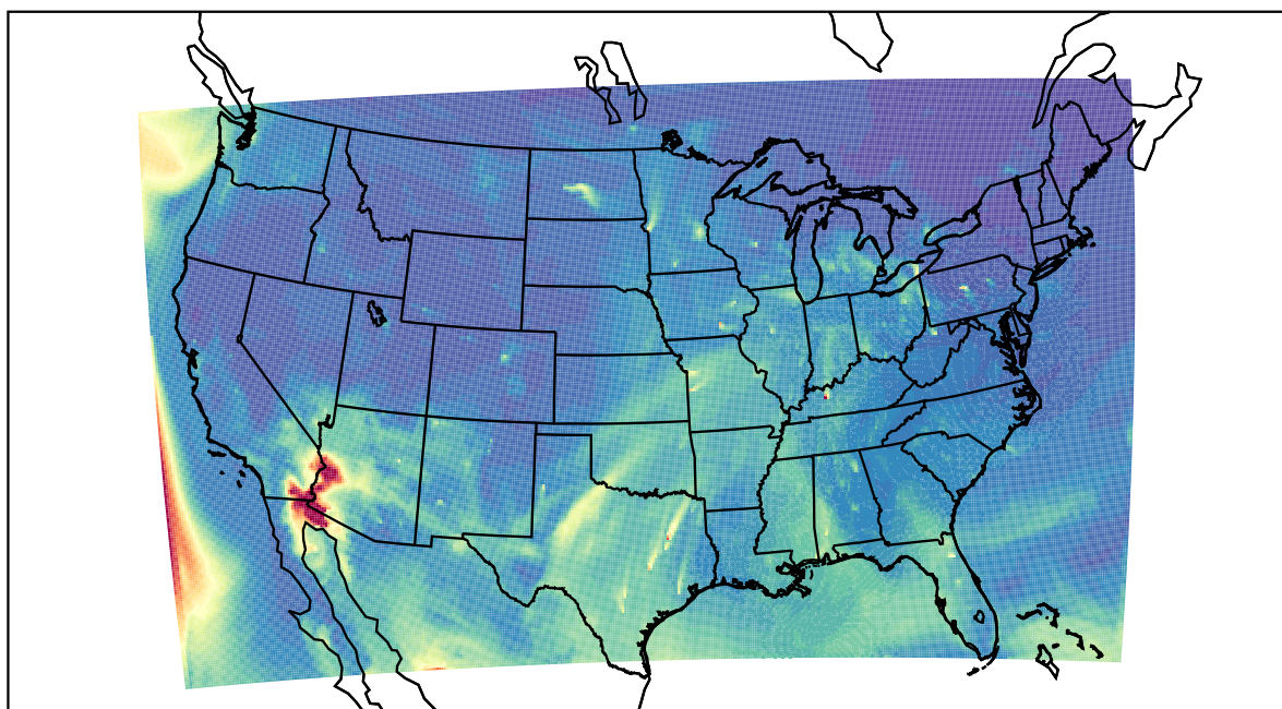
WRF 2022-05-18_15:00:00
