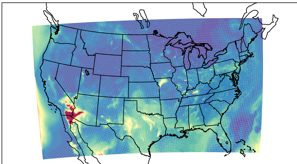
WRF 2022-05-17_09:00:00
