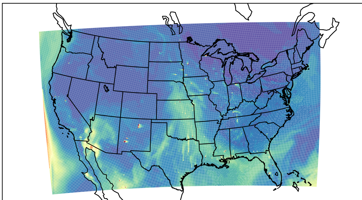
WRF 2022-05-17_22:00:00
