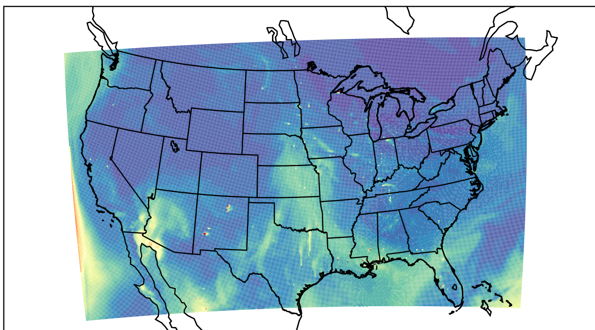
WRF 2022-05-17_21:00:00
