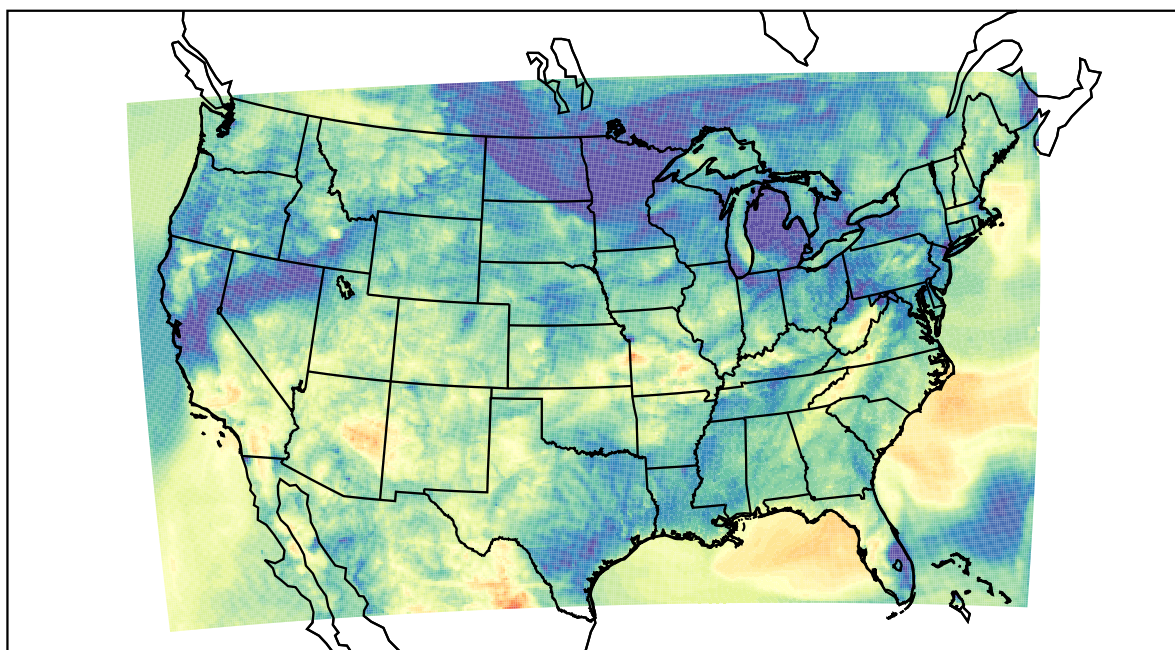
WRF (2022-05-19_07:00:00)
