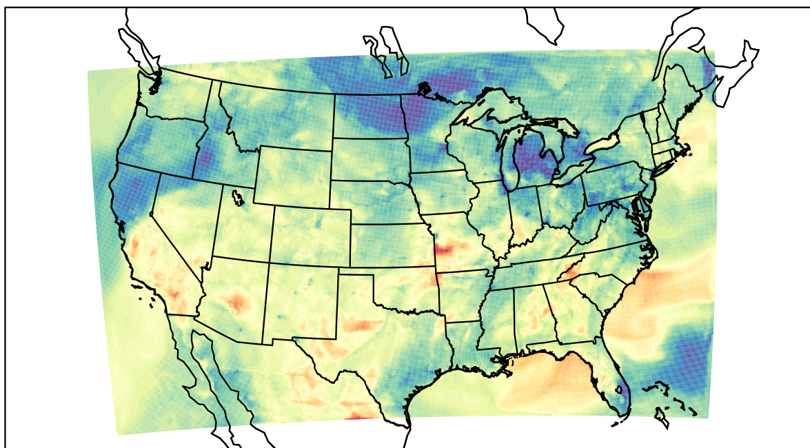
WRF (2022-05-19_02:00:00)
