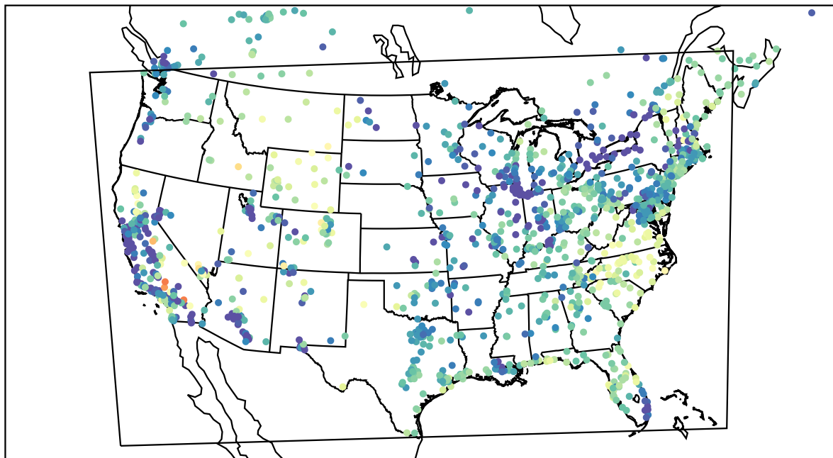
AirNOW (2022-05-19_13:00:00)
