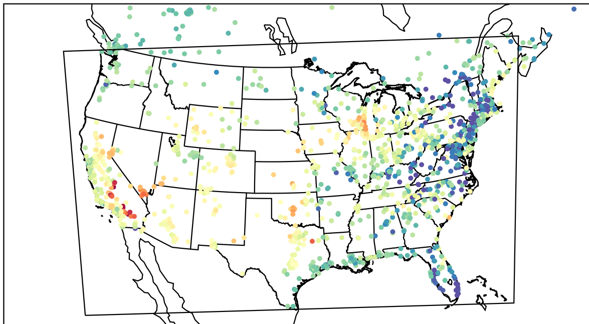
AirNOW (2022-05-20_01:00:00)
