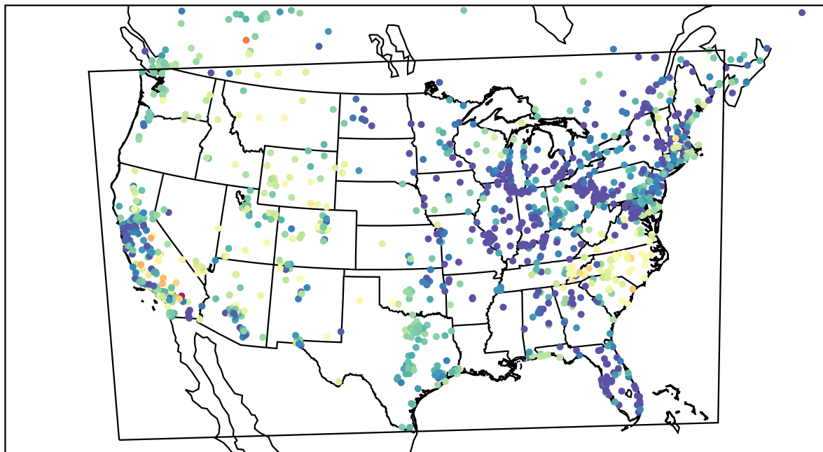
AirNOW (2022-05-19_07:00:00)
