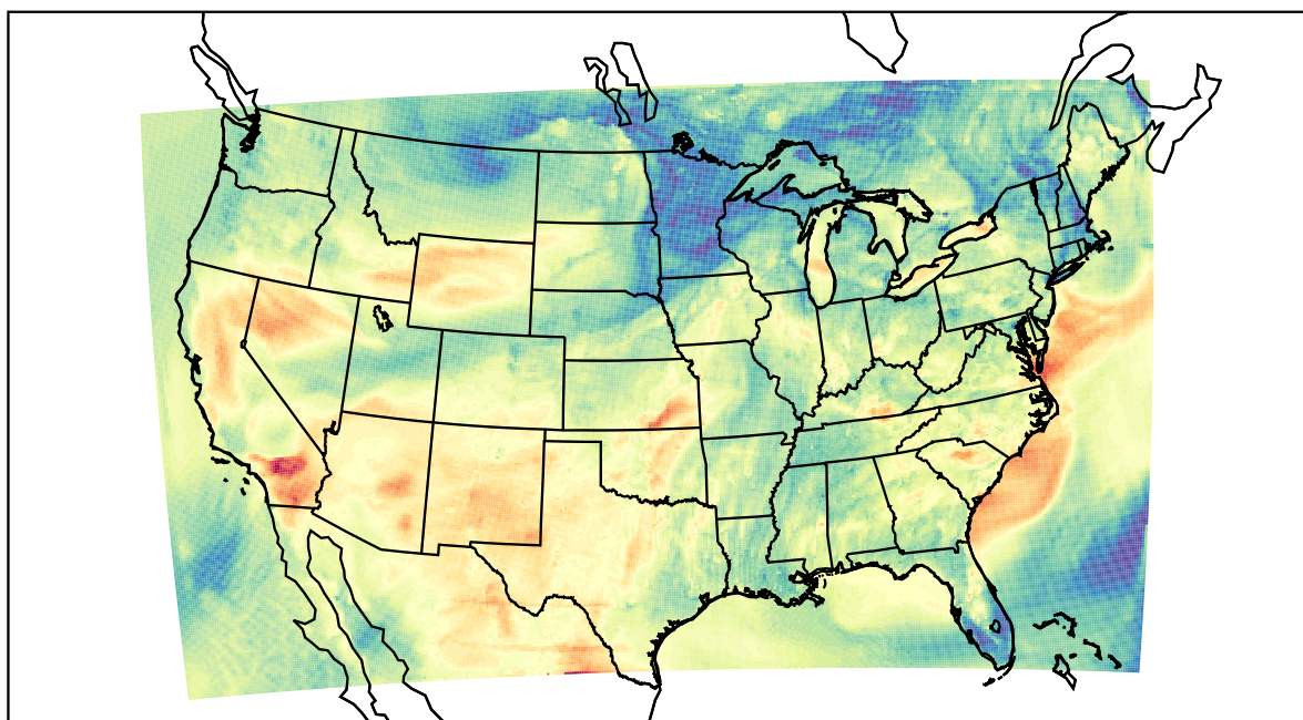
WRF (2022-05-20_01:00:00)
