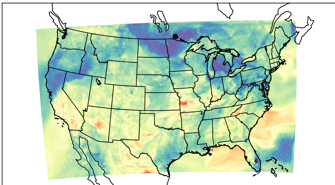
WRF (2022-05-19_03:00:00)
