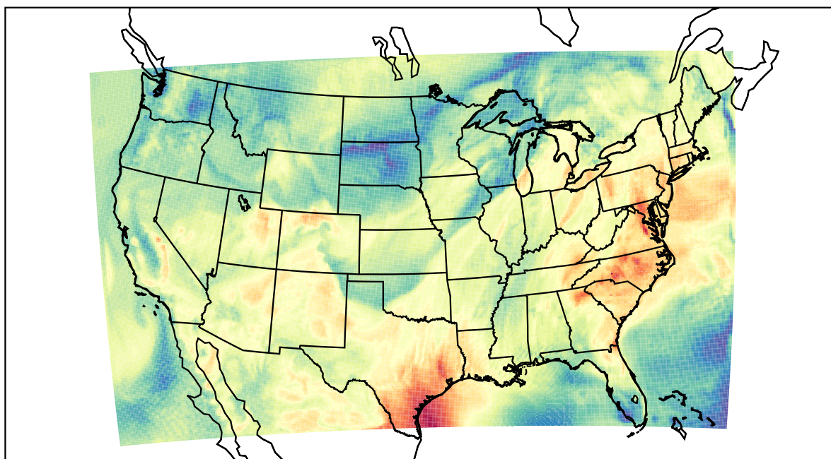
WRF (2022-05-20_16:00:00)
