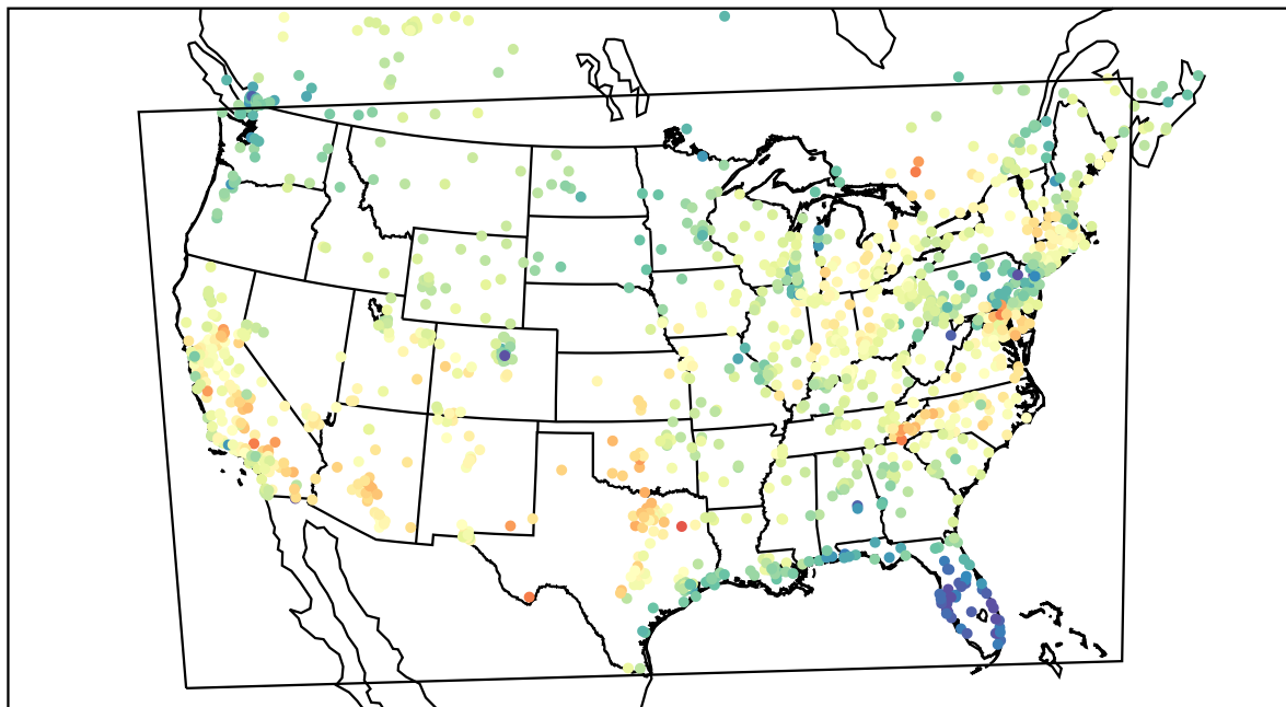
AirNOW (2022-05-20_22:00:00)
