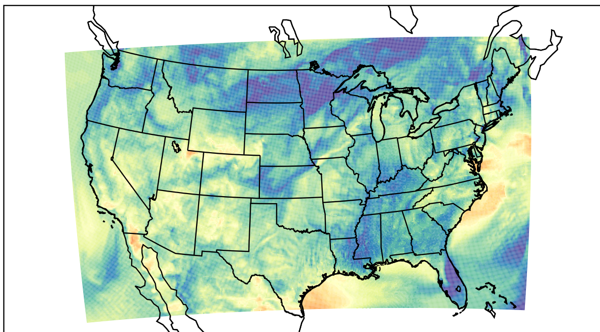
WRF (2022-05-20_09:00:00)
