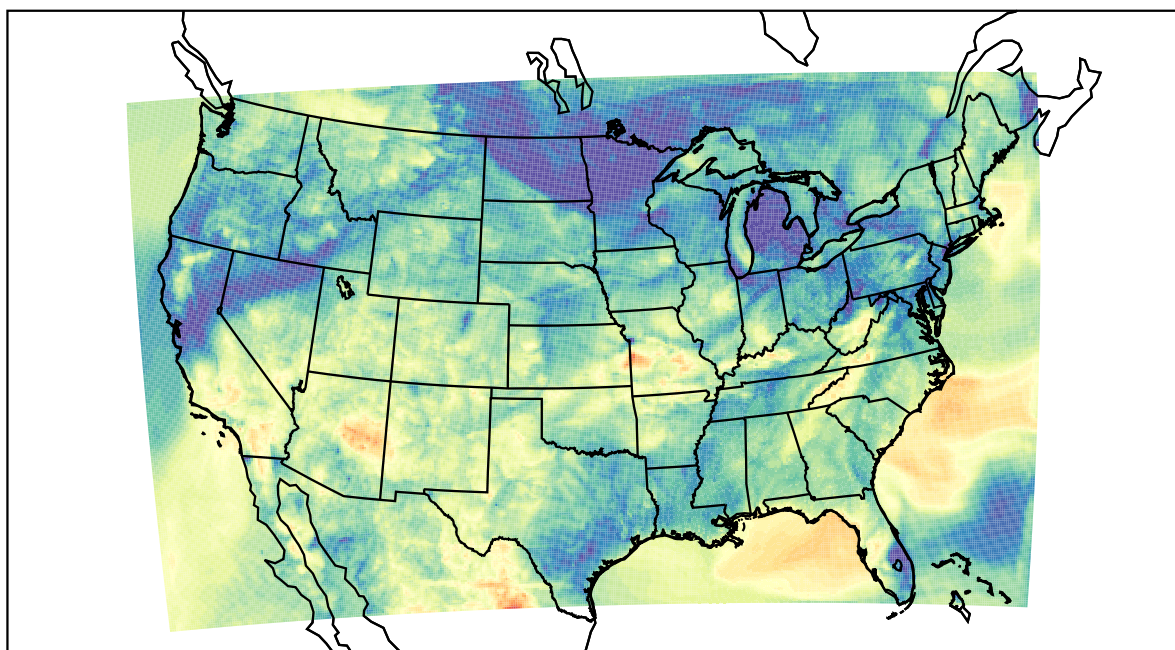
WRF (2022-05-19_06:00:00)
