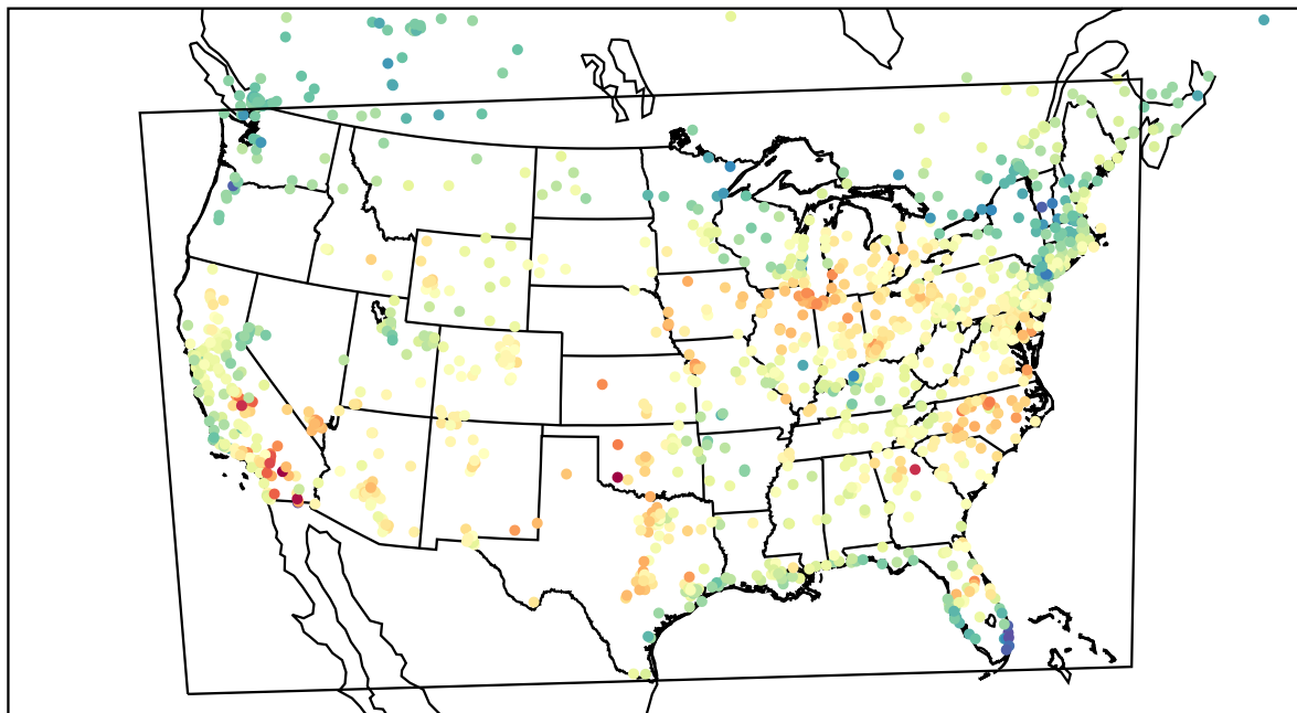
AirNOW (2022-05-19_20:00:00)
