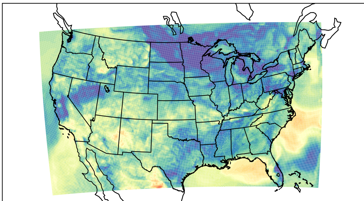
WRF (2022-05-19_10:00:00)
