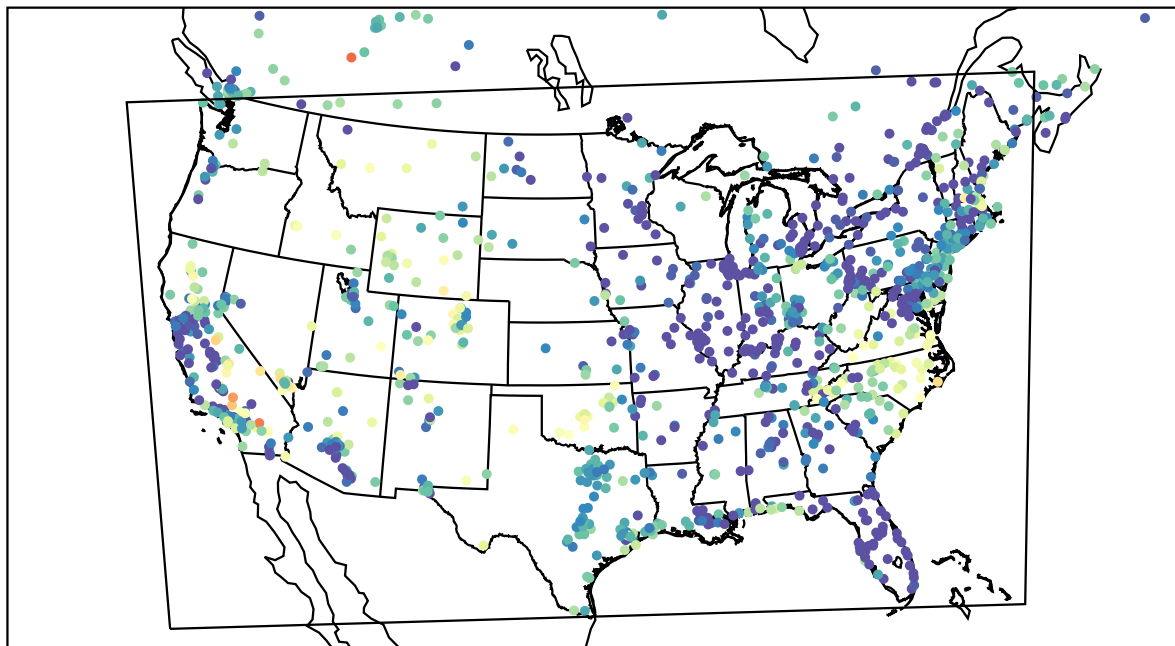
AirNOW (2022-05-19_10:00:00)
