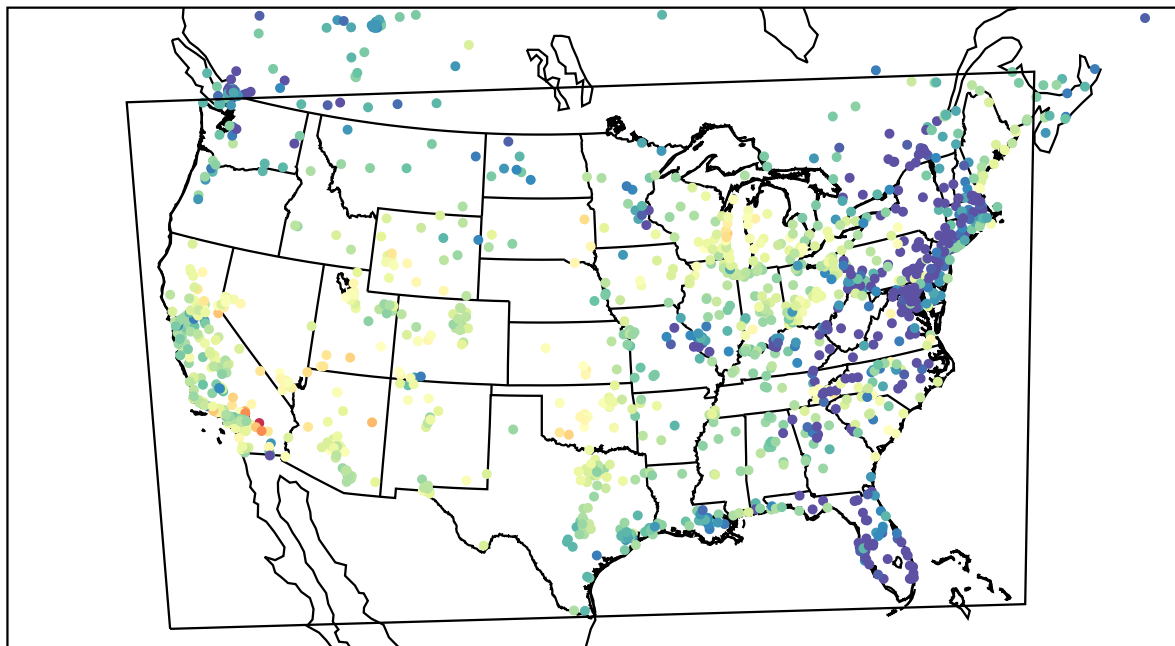
AirNOW (2022-05-20_04:00:00)
