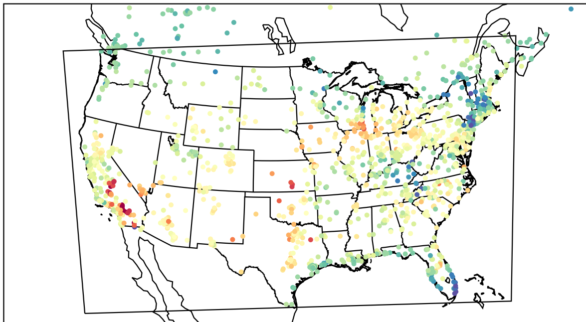
AirNOW (2022-05-19_23:00:00)
