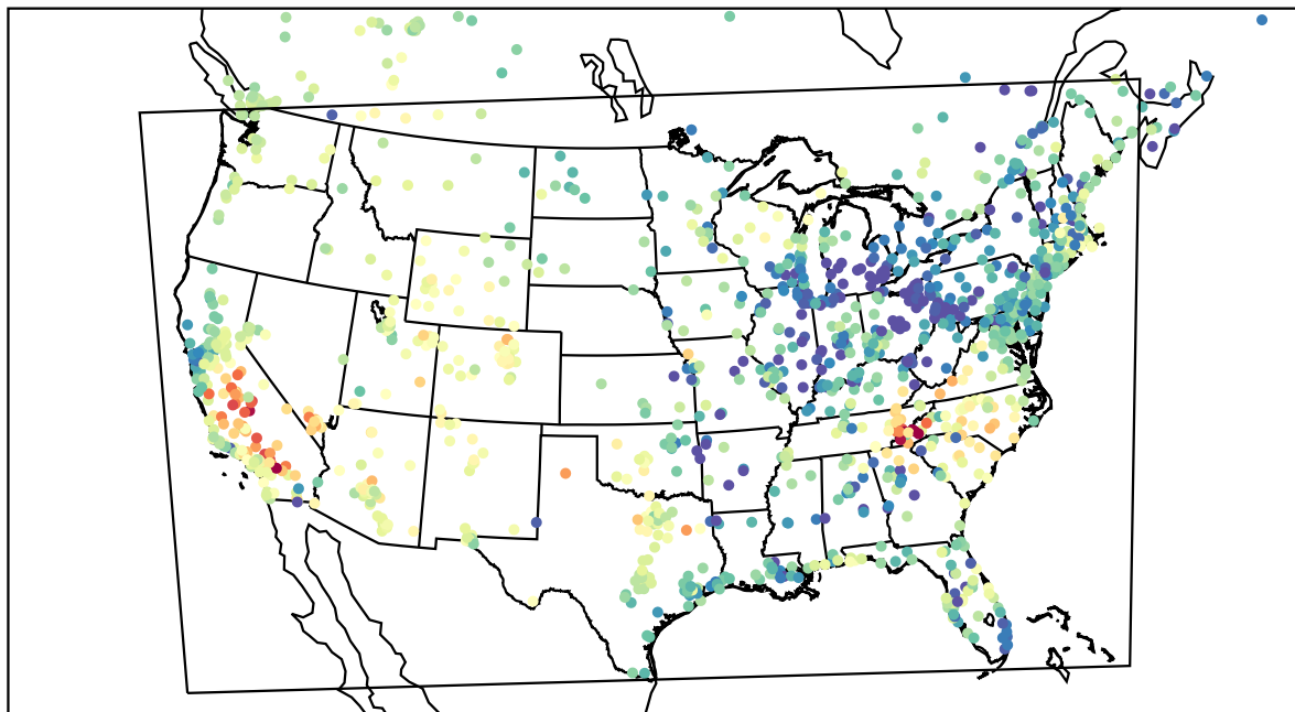
AirNOW (2022-05-19_02:00:00)
