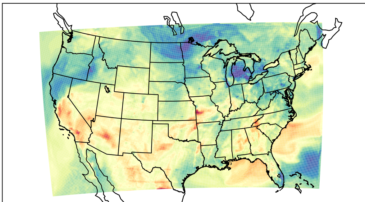
WRF (2022-05-19_01:00:00)
