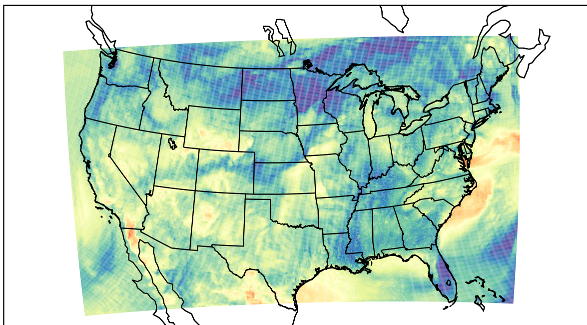
WRF (2022-05-20_07:00:00)
