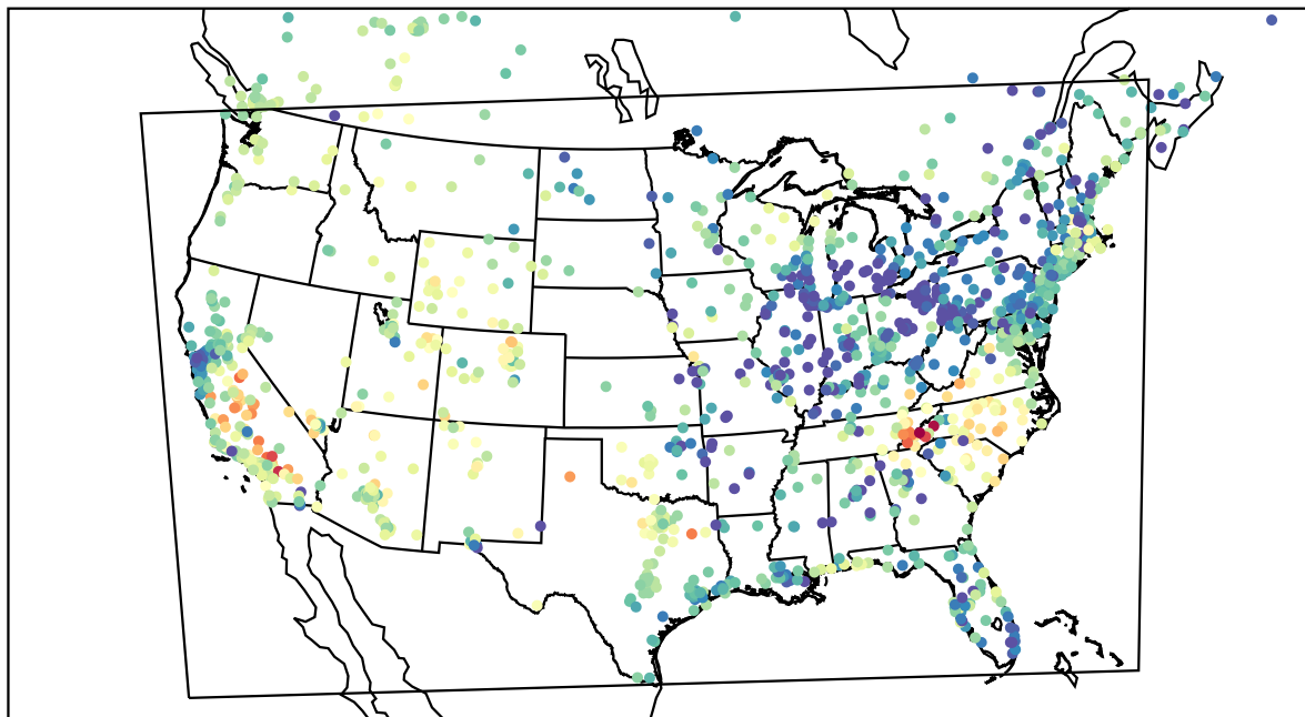
AirNOW (2022-05-19_03:00:00)
