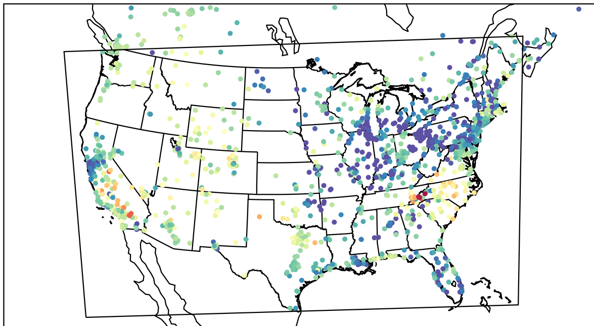
AirNOW (2022-05-19_04:00:00)
