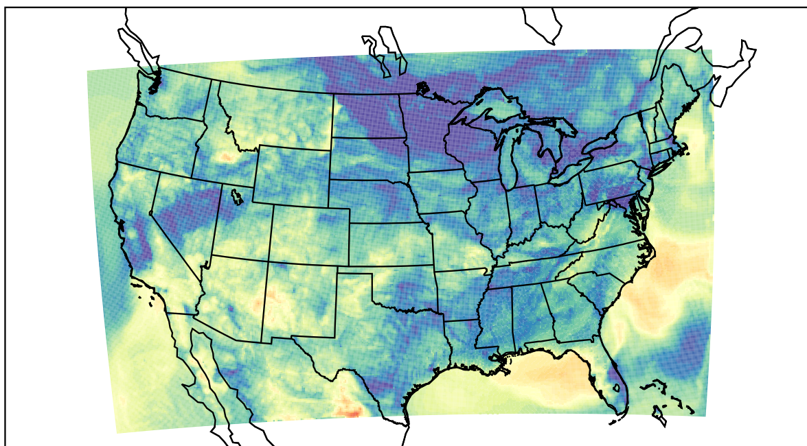
WRF (2022-05-19_11:00:00)
