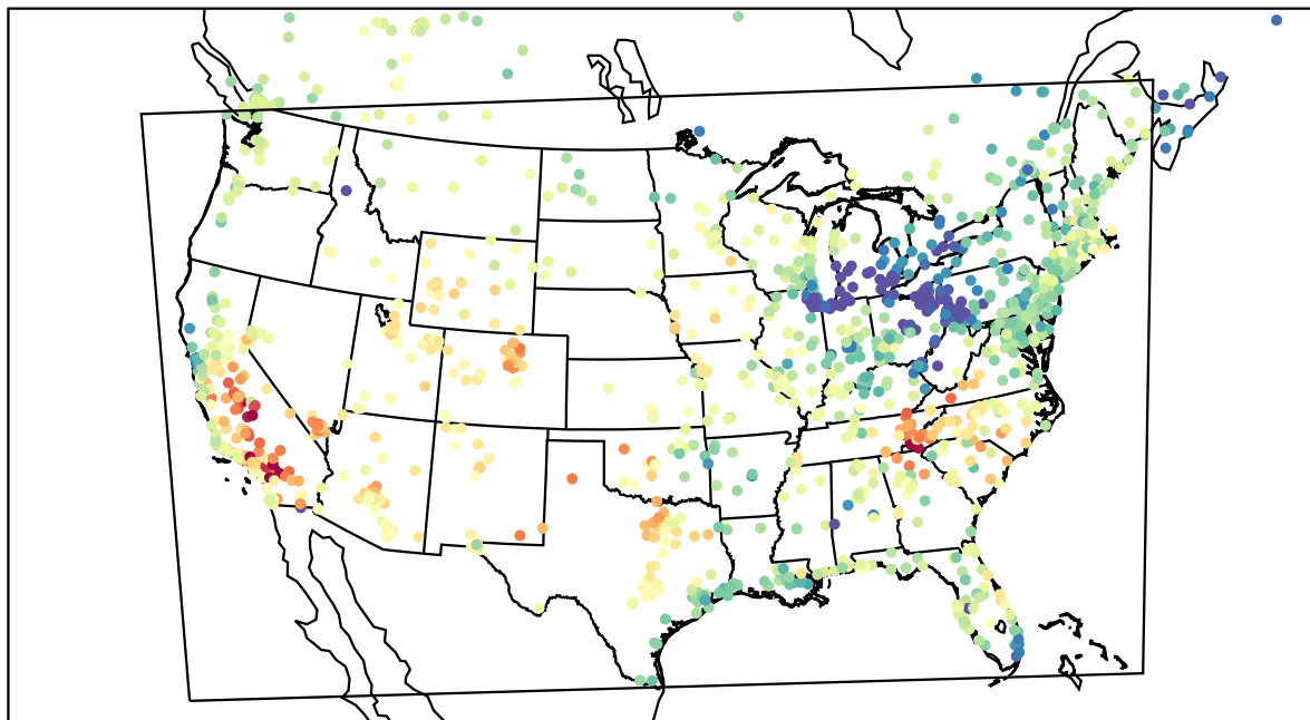
AirNOW (2022-05-19_00:00:00)
