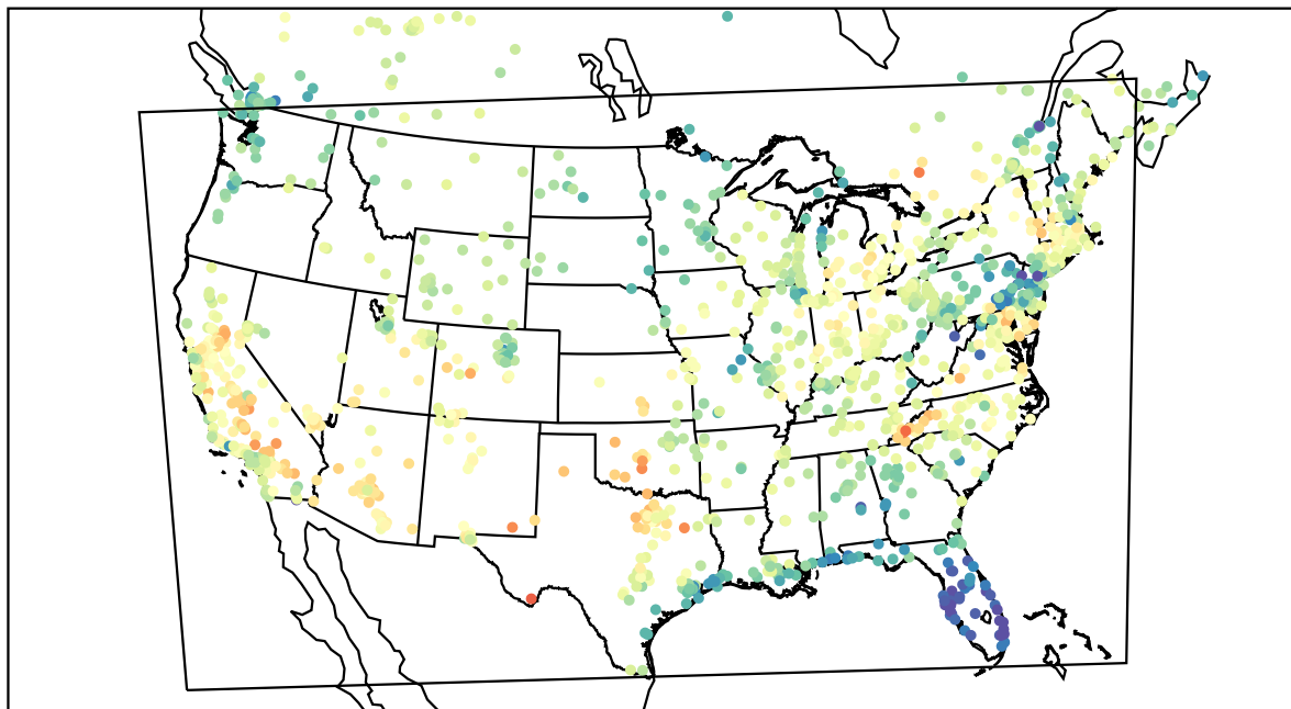
AirNOW (2022-05-20_23:00:00)
