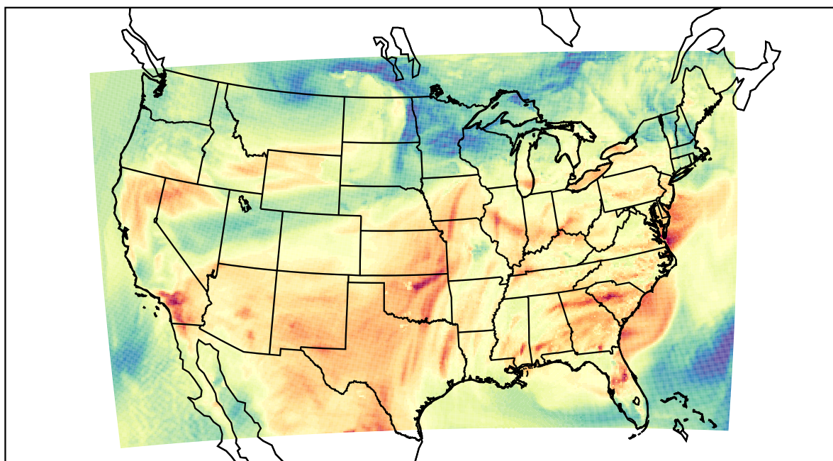
WRF (2022-05-19_22:00:00)
