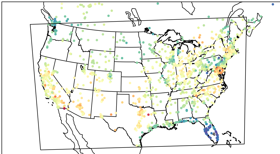
AirNOW (2022-05-20_21:00:00)
