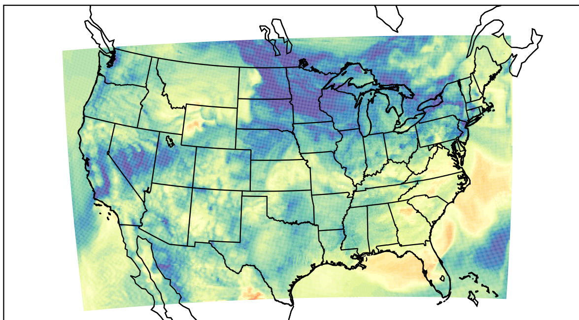
WRF (2022-05-19_14:00:00)
