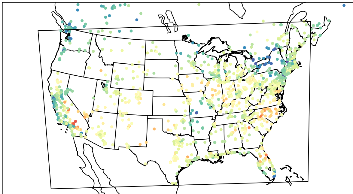
AirNOW (2022-05-19_17:00:00)
