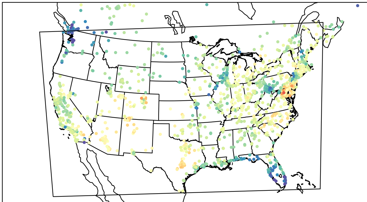
AirNOW (2022-05-20_17:00:00)
