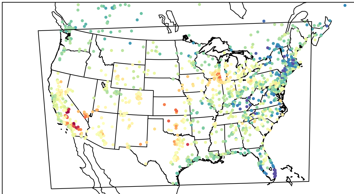
AirNOW (2022-05-20_00:00:00)
