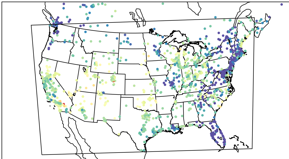
AirNOW (2022-05-20_06:00:00)
