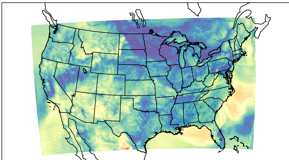
WRF (2022-05-19_12:00:00)
