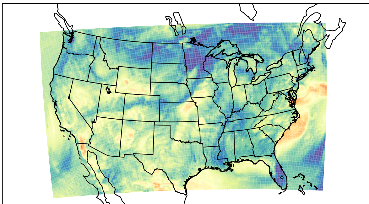
WRF (2022-05-20_06:00:00)
