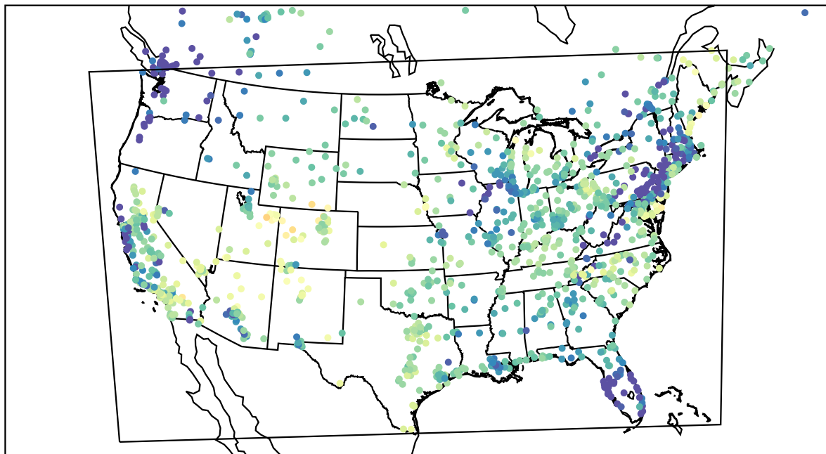
AirNOW (2022-05-20_13:00:00)
