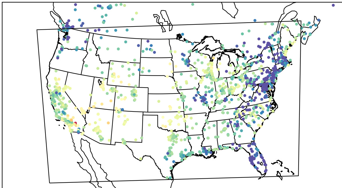
AirNOW (2022-05-20_05:00:00)
