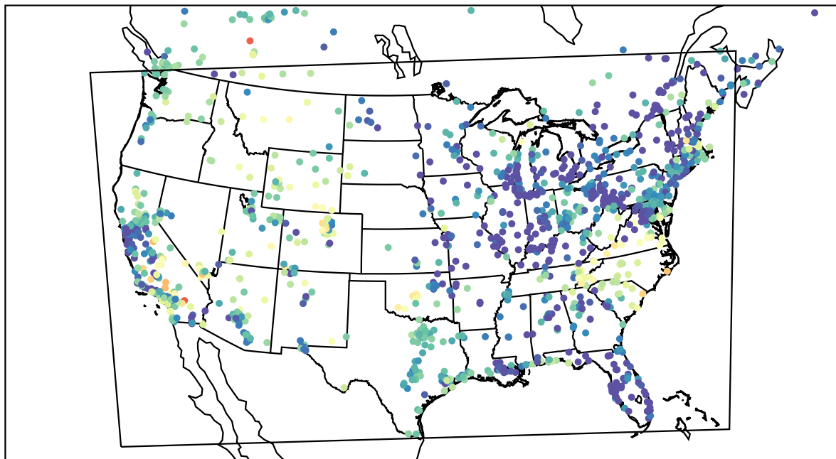
AirNOW (2022-05-19_08:00:00)
