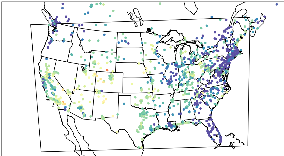
AirNOW (2022-05-20_10:00:00)
