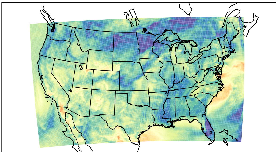
WRF (2022-05-20_08:00:00)
