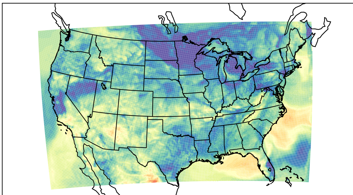
WRF (2022-05-19_09:00:00)
