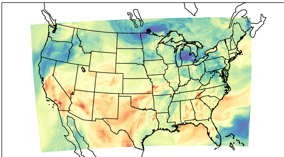
WRF (2022-05-19_00:00:00)
