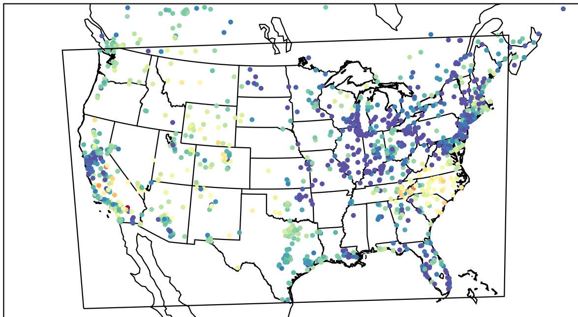
AirNOW (2022-05-19_06:00:00)
