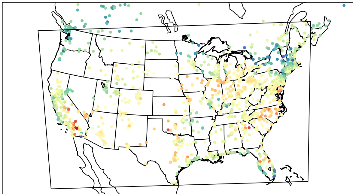
AirNOW (2022-05-19_19:00:00)
