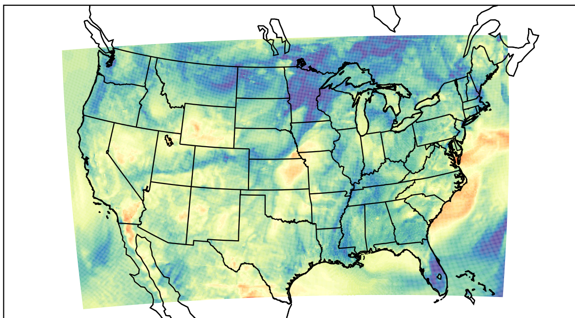
WRF (2022-05-20_05:00:00)
