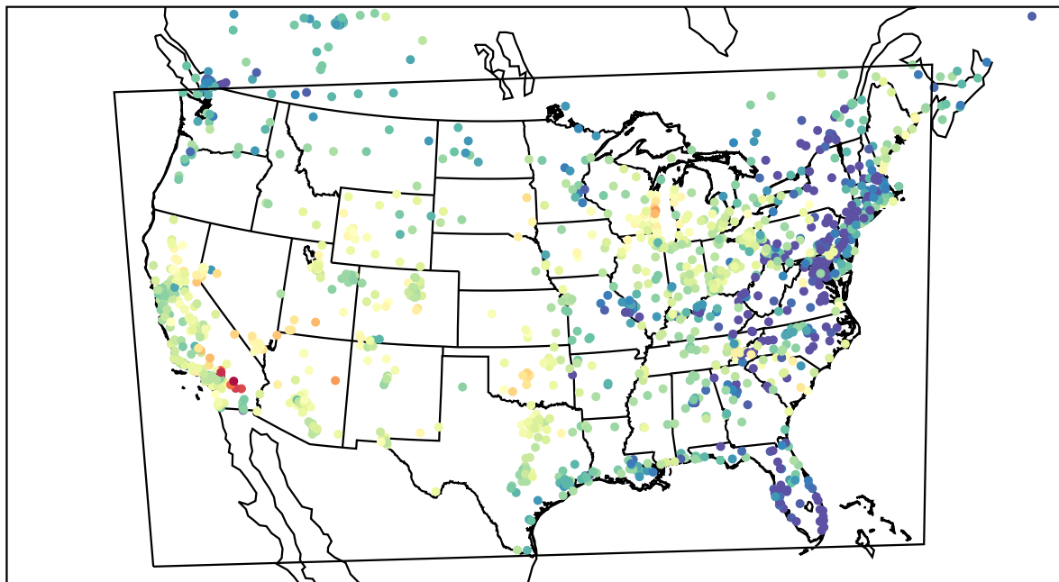
AirNOW (2022-05-20_03:00:00)
