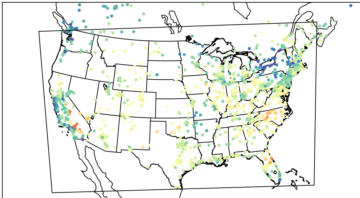
AirNOW (2022-05-19_16:00:00)
