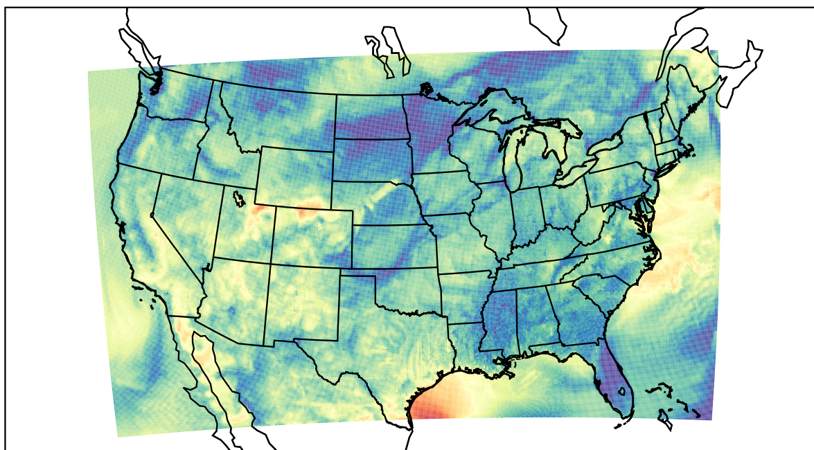
WRF (2022-05-20_12:00:00)
