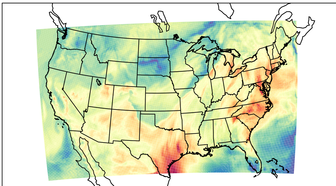
WRF (2022-05-20_17:00:00)
