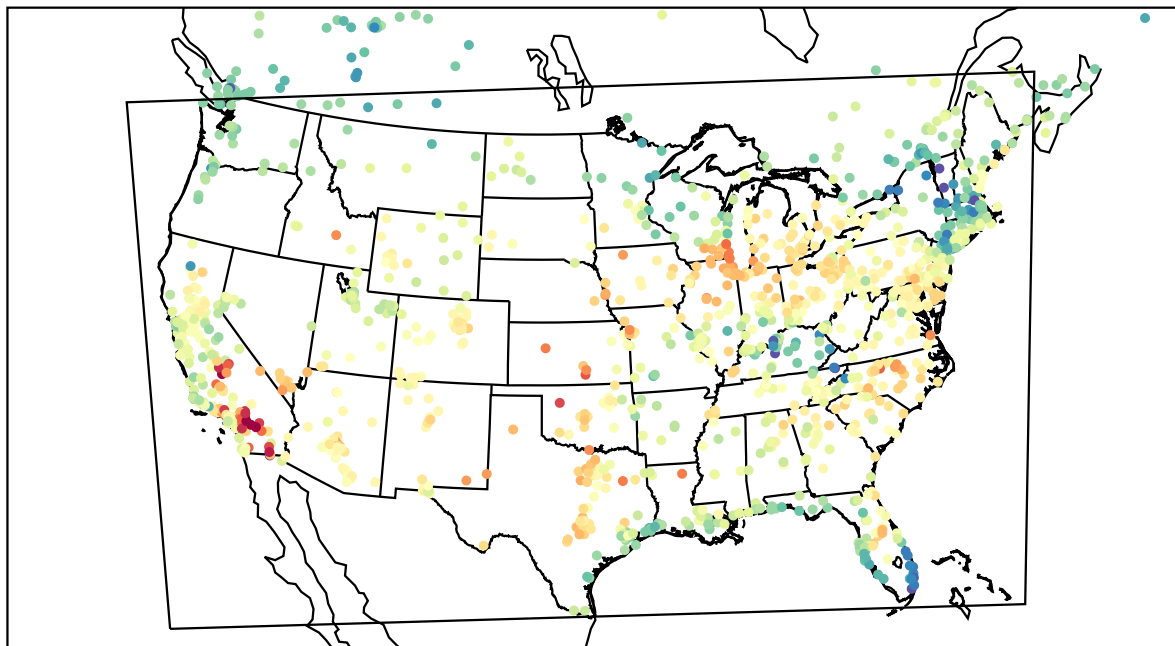
AirNOW (2022-05-19_22:00:00)
