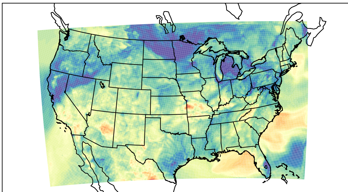
WRF (2022-05-19_05:00:00)
