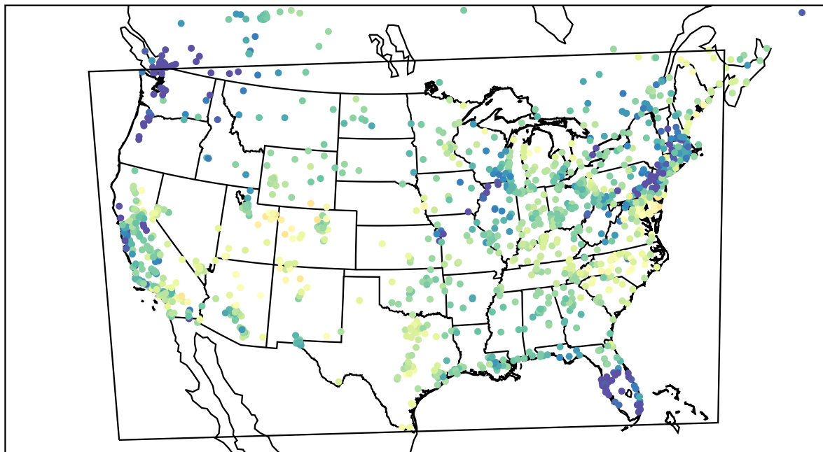
AirNOW (2022-05-20_14:00:00)
