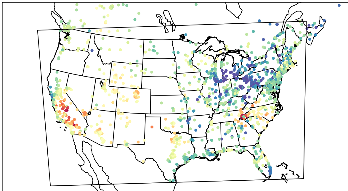
AirNOW (2022-05-19_01:00:00)
