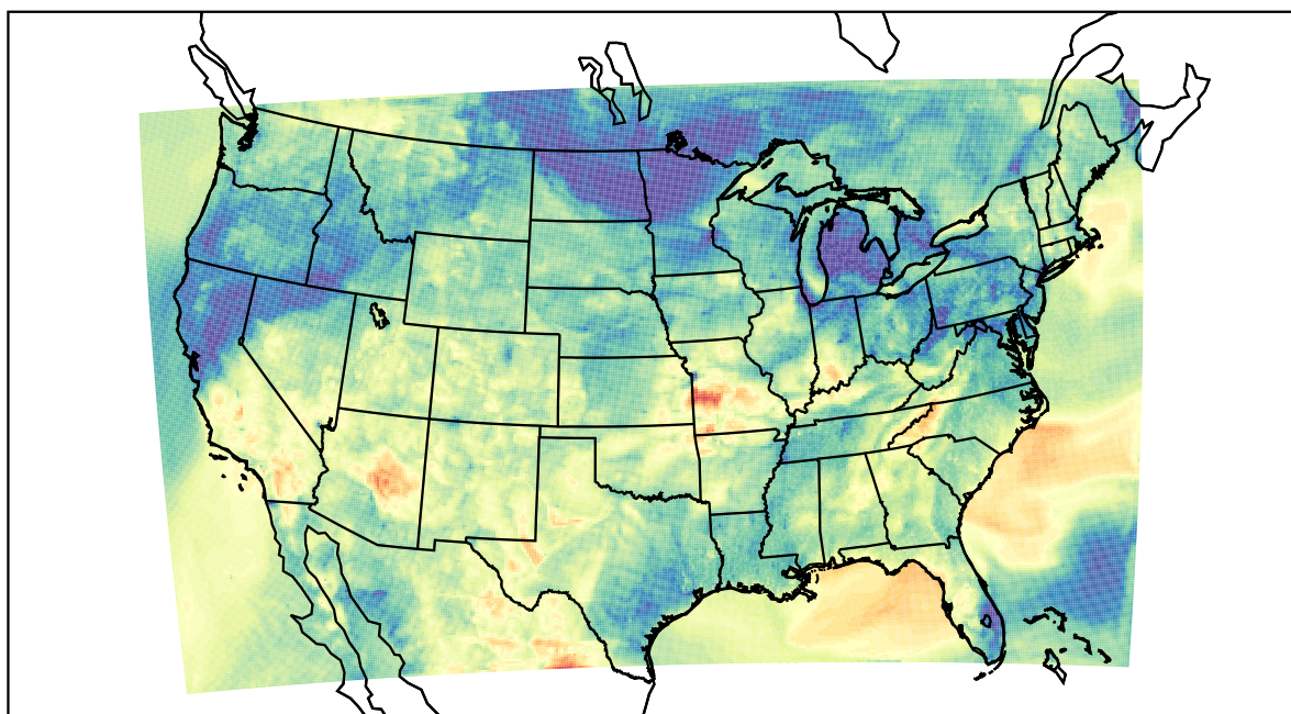
WRF (2022-05-19_04:00:00)
