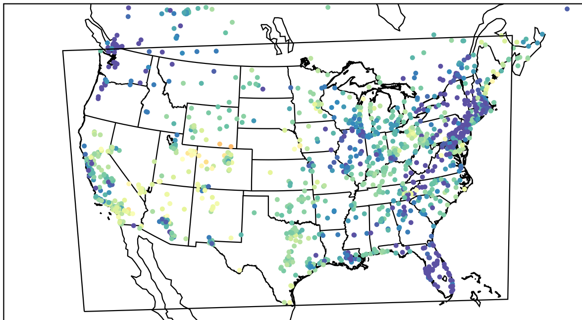
AirNOW (2022-05-20_12:00:00)
