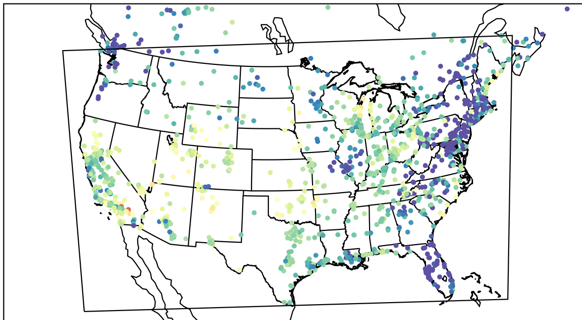
AirNOW (2022-05-20_07:00:00)
