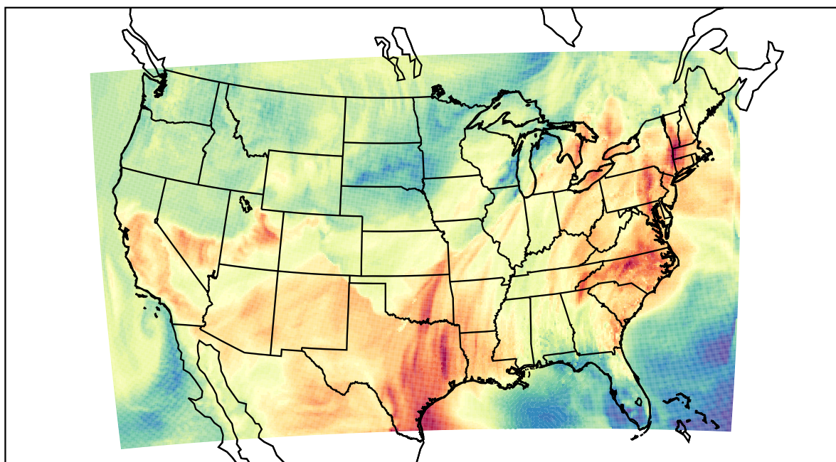
WRF (2022-05-20_21:00:00)
