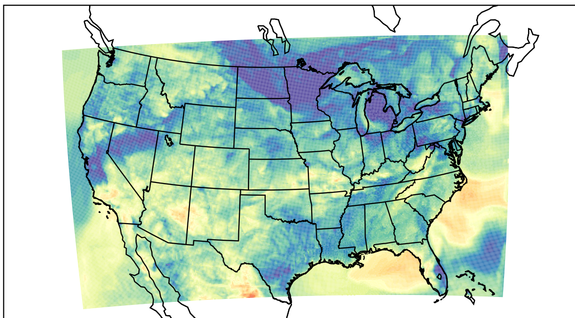
WRF (2022-05-19_08:00:00)
