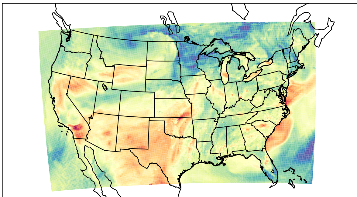
WRF (2022-05-20_00:00:00)
