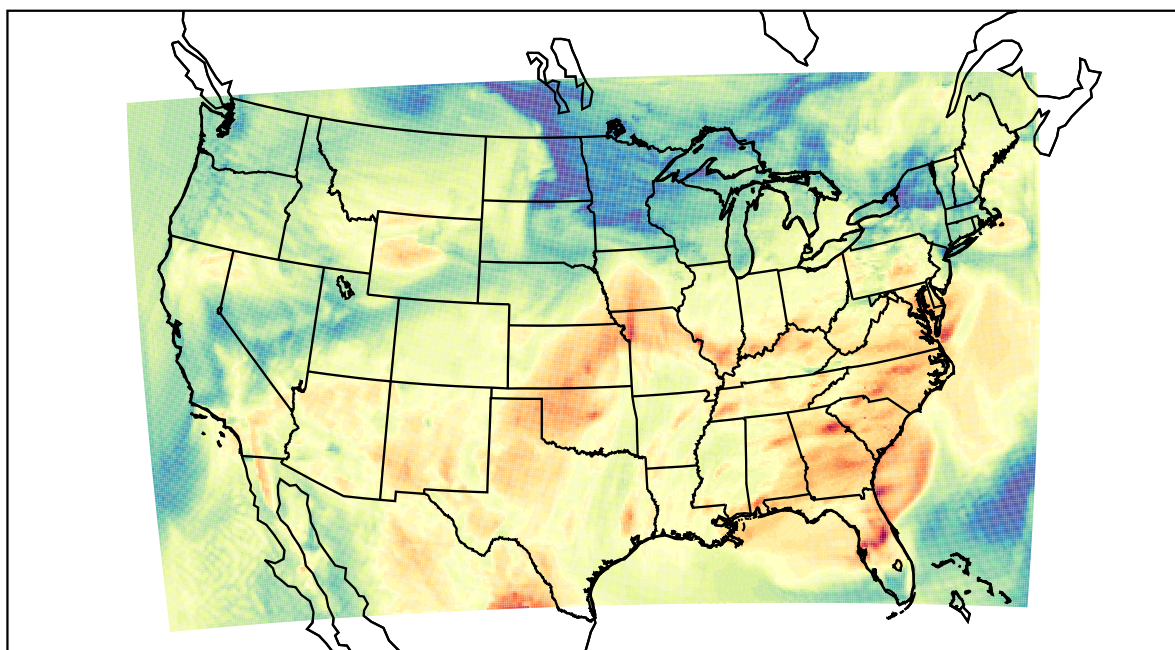
WRF (2022-05-19_17:00:00)
