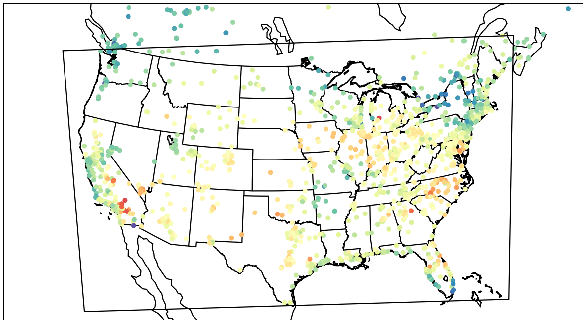
AirNOW (2022-05-19_18:00:00)
