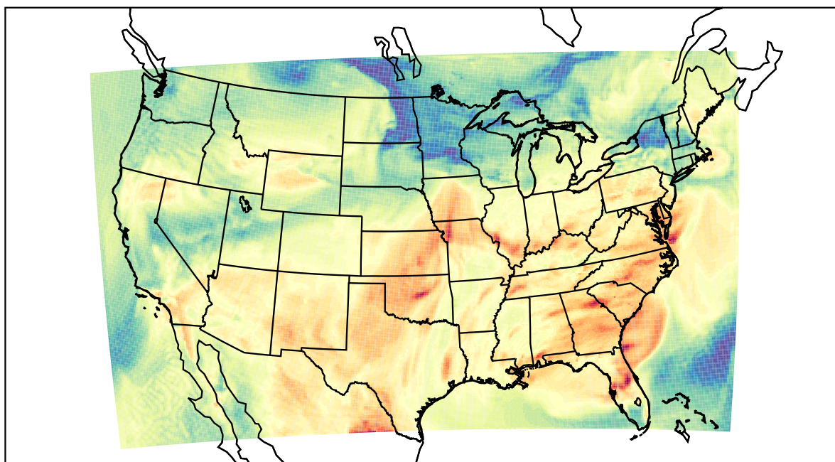
WRF (2022-05-19_18:00:00)
