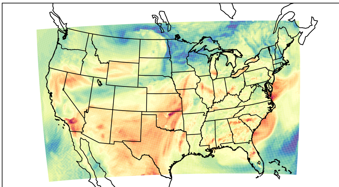
WRF (2022-05-19_23:00:00)
