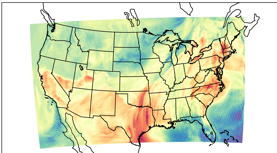
WRF (2022-05-20_22:00:00)
