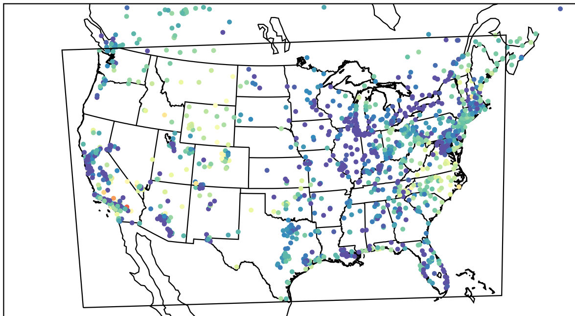
AirNOW (2022-05-19_12:00:00)
