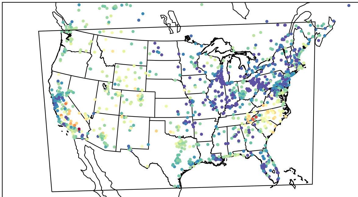
AirNOW (2022-05-19_05:00:00)
