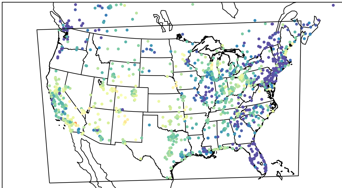
AirNOW (2022-05-20_09:00:00)
