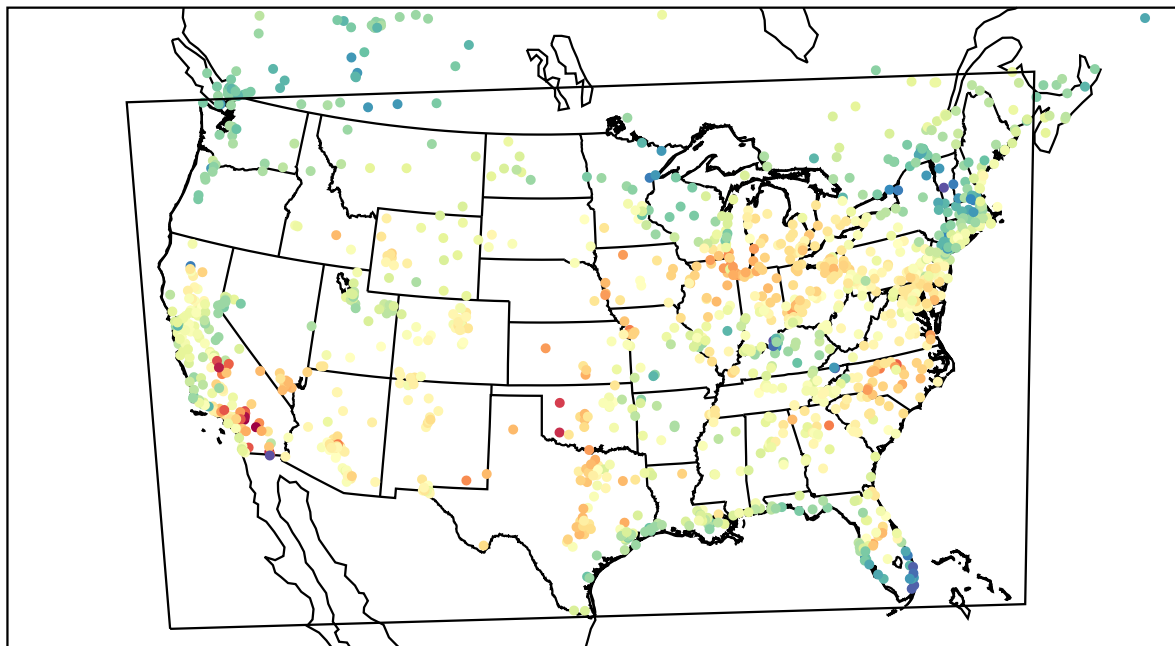
AirNOW (2022-05-19_21:00:00)
