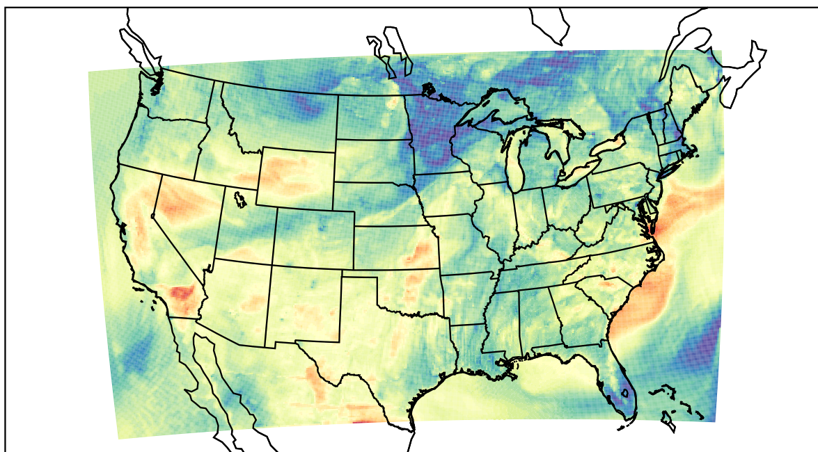
WRF (2022-05-20_02:00:00)
