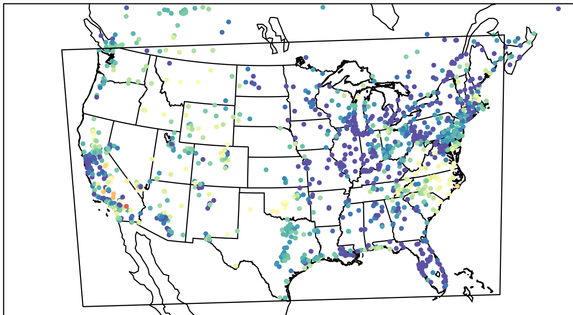
AirNOW (2022-05-19_09:00:00)
