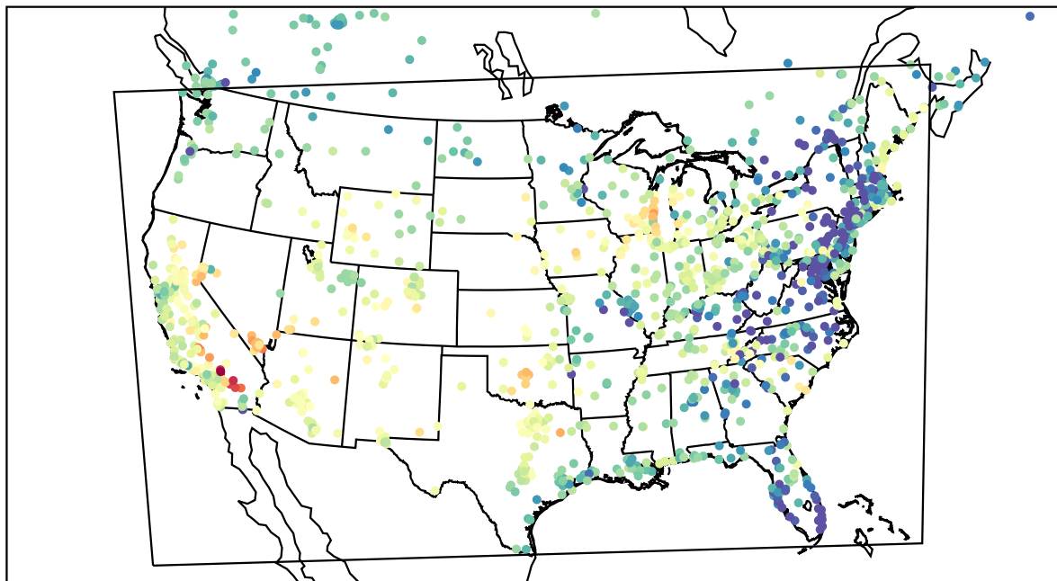
AirNOW (2022-05-20_02:00:00)
