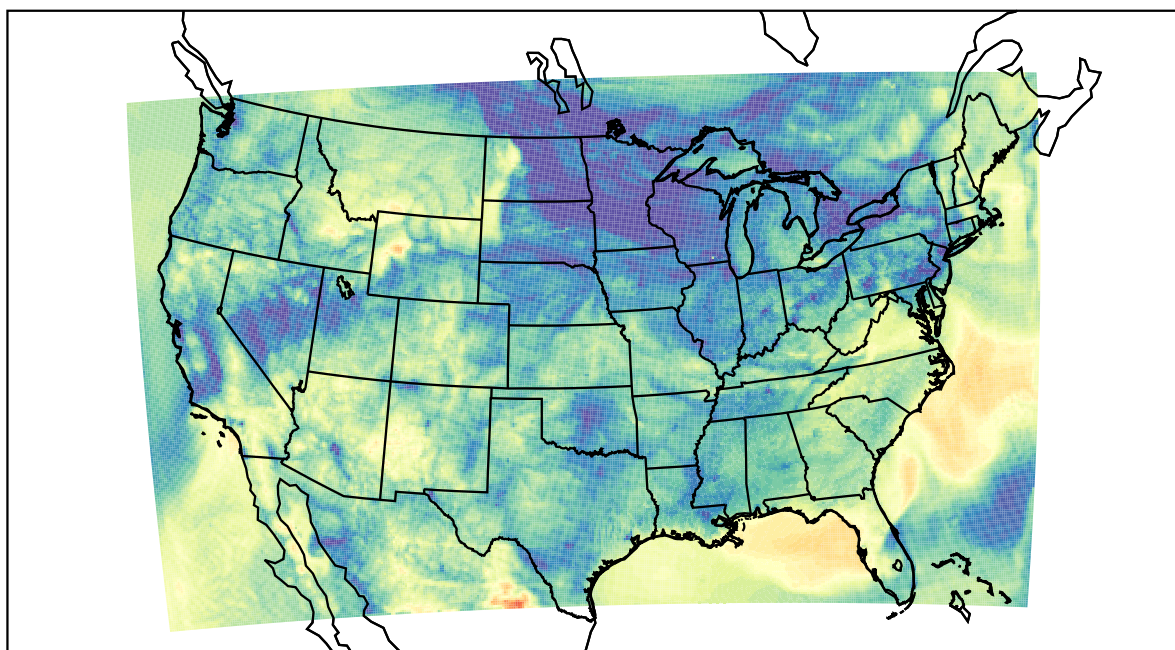
WRF (2022-05-19_13:00:00)
