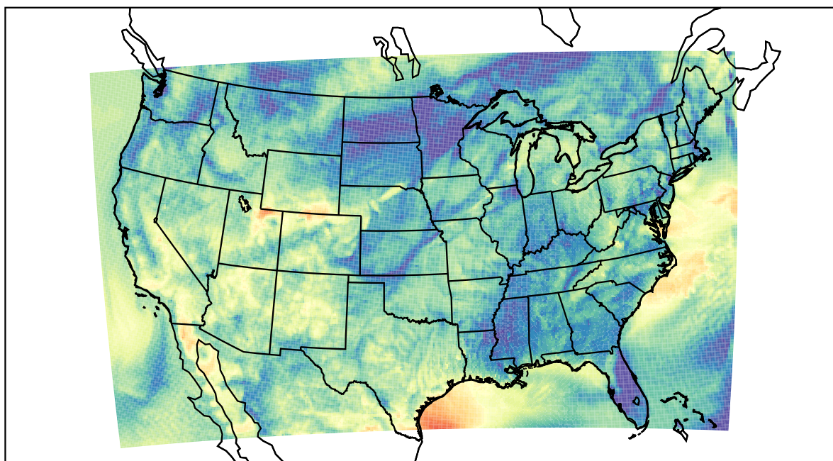
WRF (2022-05-20_11:00:00)
