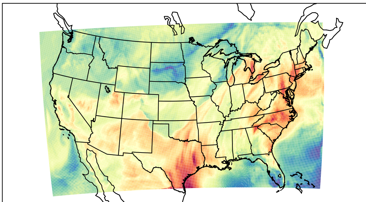
WRF (2022-05-20_18:00:00)
