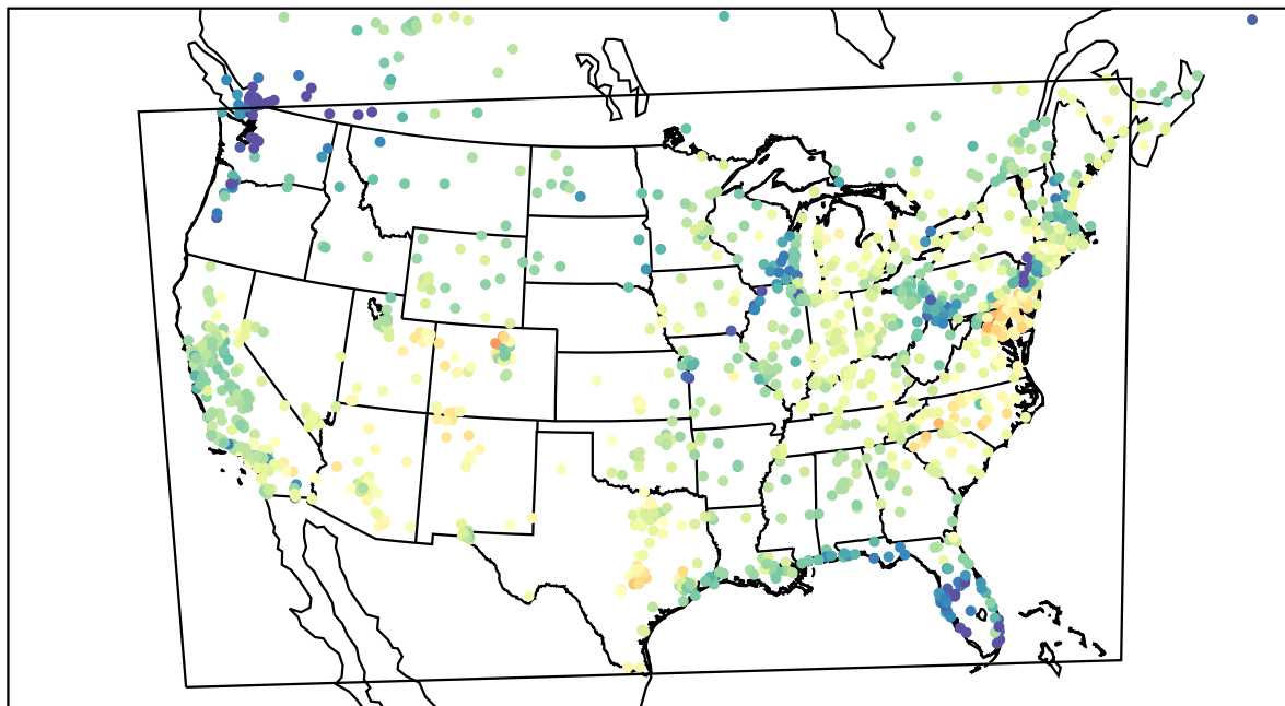
AirNOW (2022-05-20_16:00:00)
