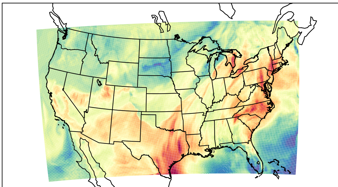
WRF (2022-05-20_19:00:00)
