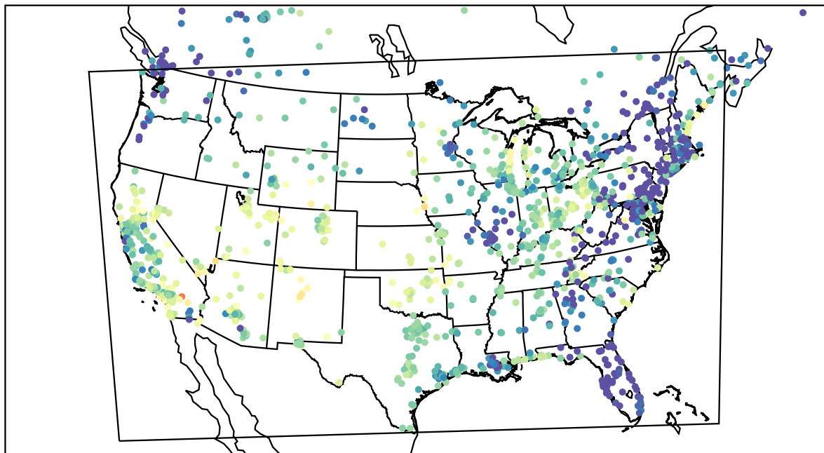
AirNOW (2022-05-20_08:00:00)
