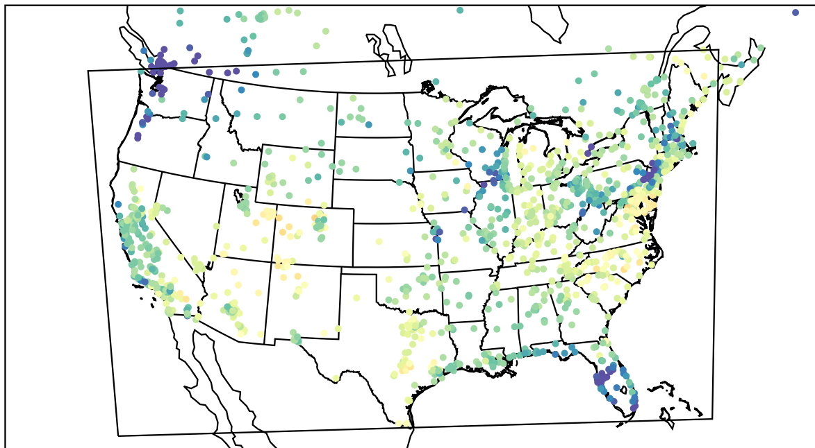
AirNOW (2022-05-20_15:00:00)
