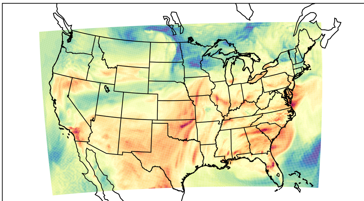
WRF (2022-05-19_21:00:00)
