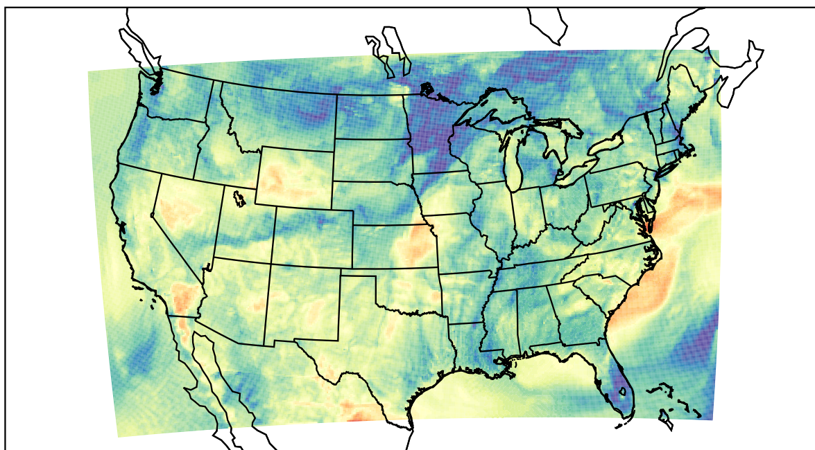
WRF (2022-05-20_04:00:00)
