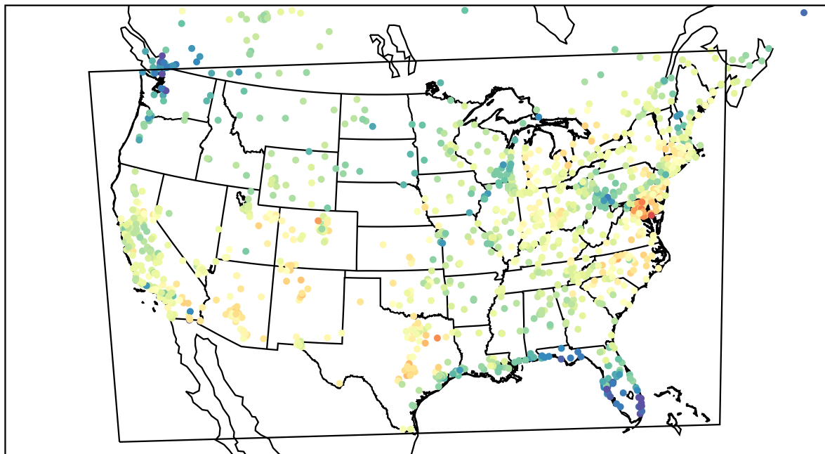
AirNOW (2022-05-20_18:00:00)
