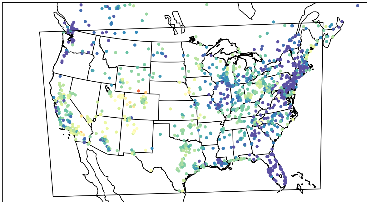
AirNOW (2022-05-20_11:00:00)
