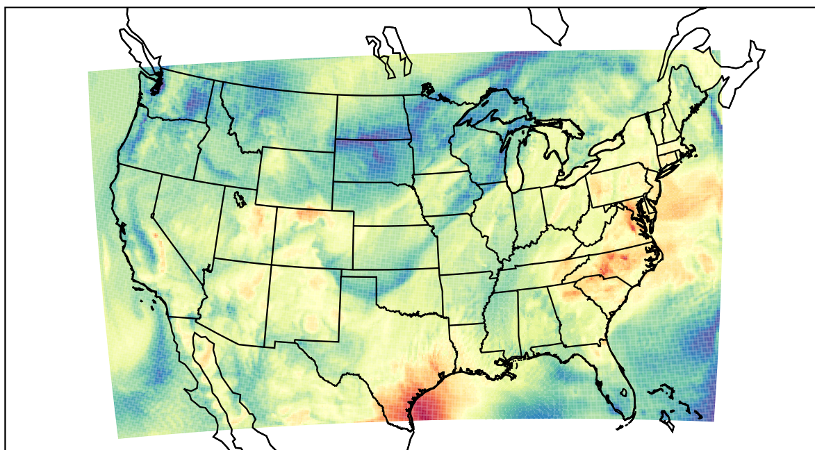
WRF (2022-05-20_15:00:00)
