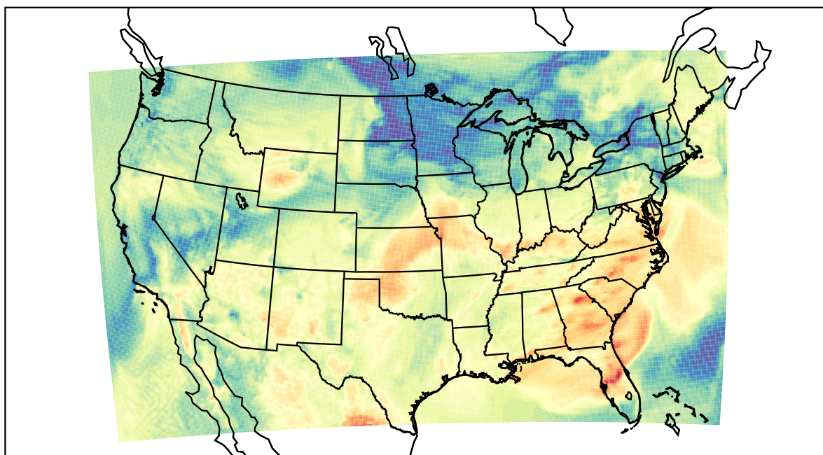
WRF (2022-05-19_16:00:00)
