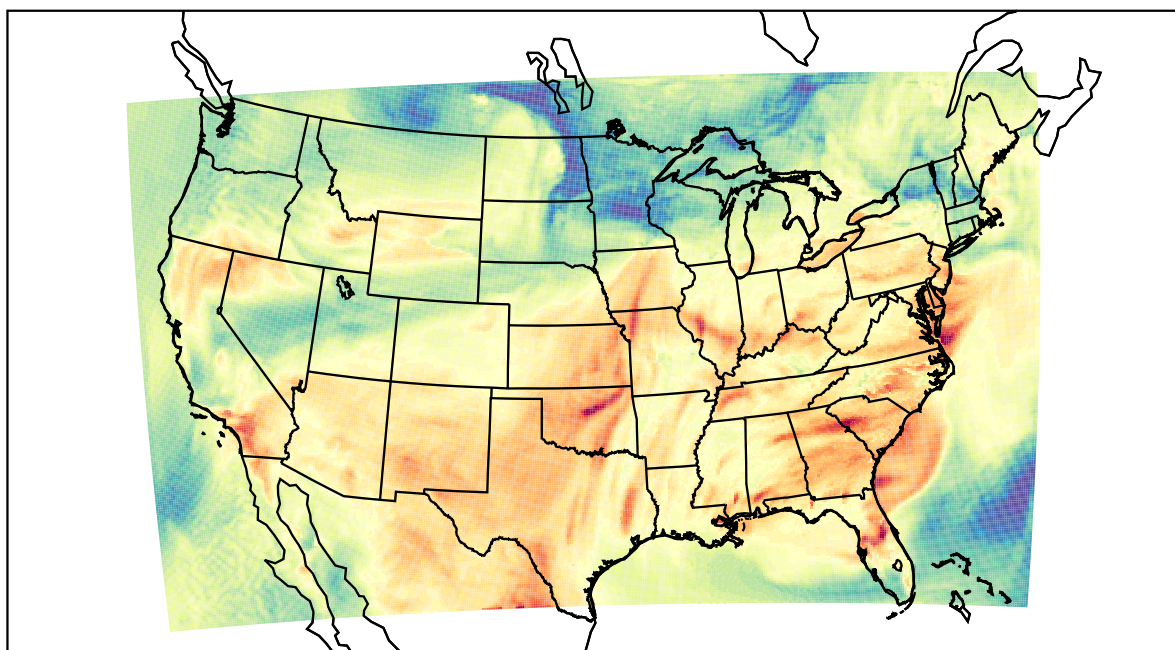
WRF (2022-05-19_20:00:00)
