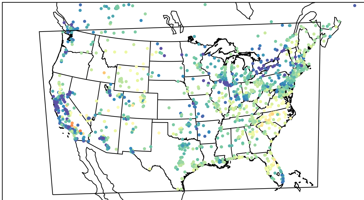
AirNOW (2022-05-19_14:00:00)
