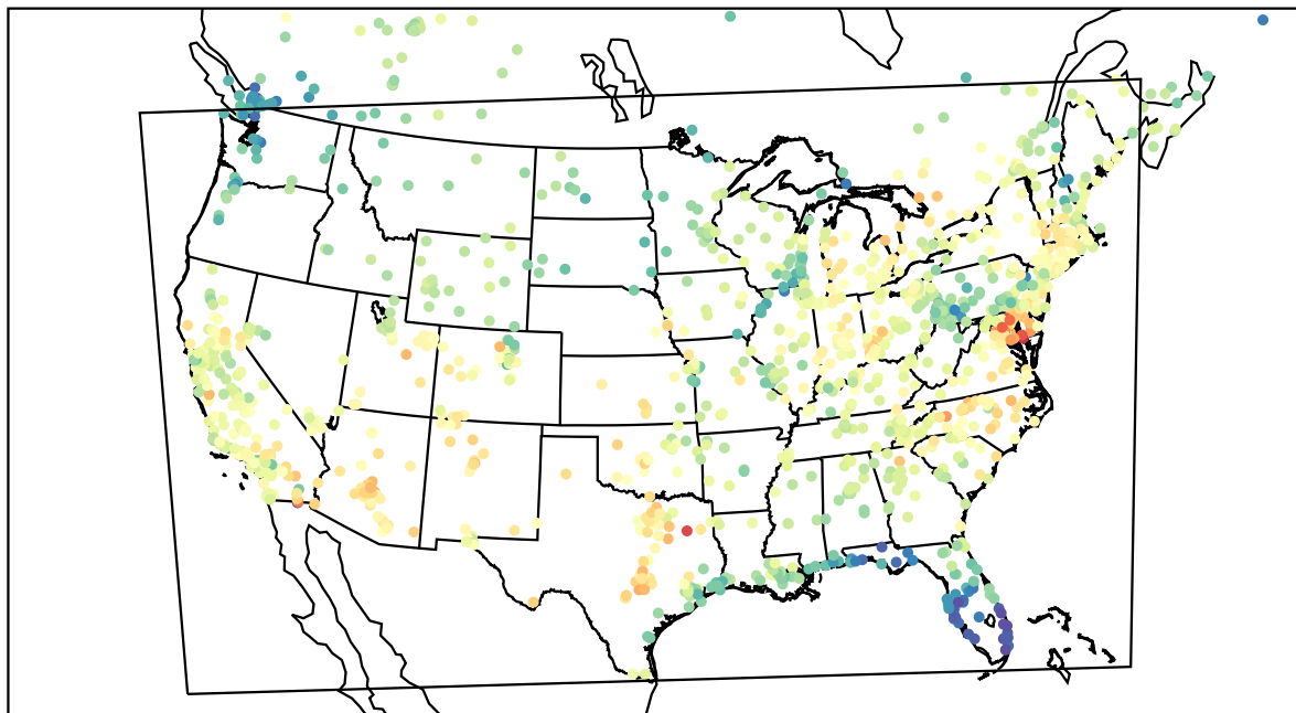
AirNOW (2022-05-20_19:00:00)
