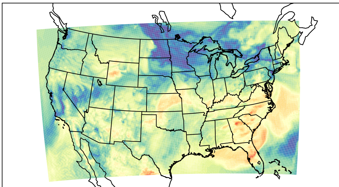
WRF (2022-05-19_15:00:00)
