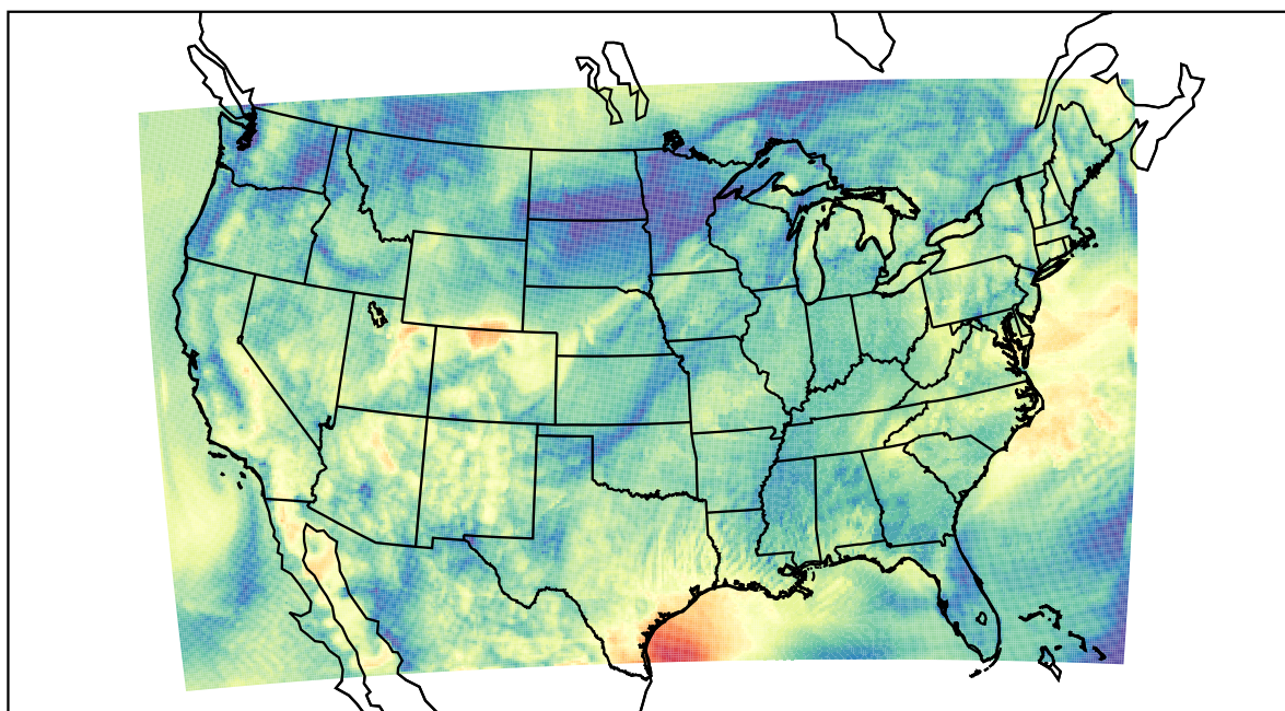
WRF (2022-05-20_13:00:00)
