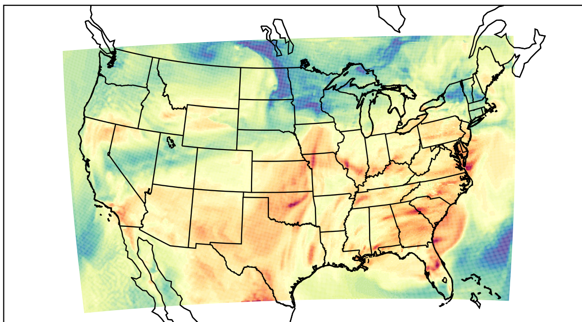
WRF (2022-05-19_19:00:00)
