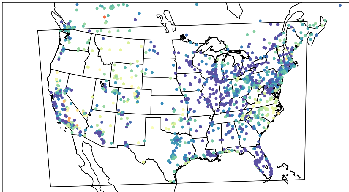
AirNOW (2022-05-19_11:00:00)
