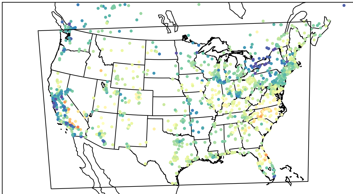
AirNOW (2022-05-19_15:00:00)
