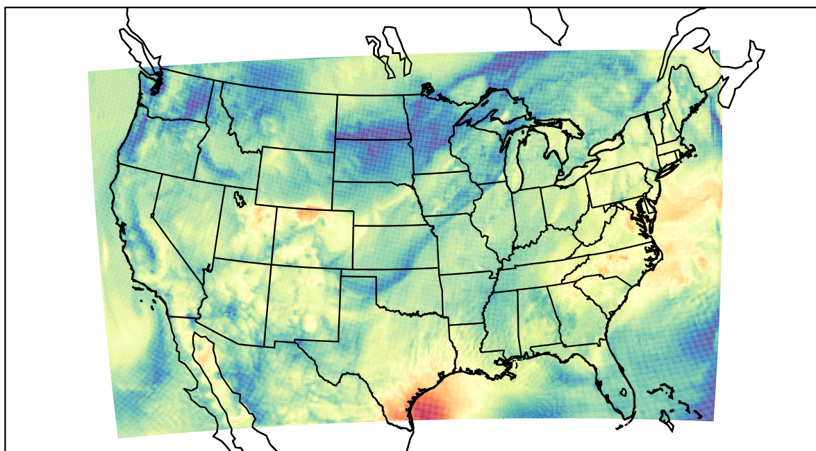
WRF (2022-05-20_14:00:00)
