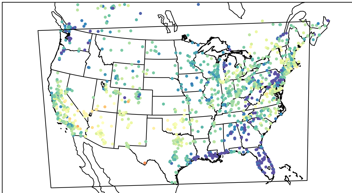
AirNOW (2022-05-21_04:00:00)
