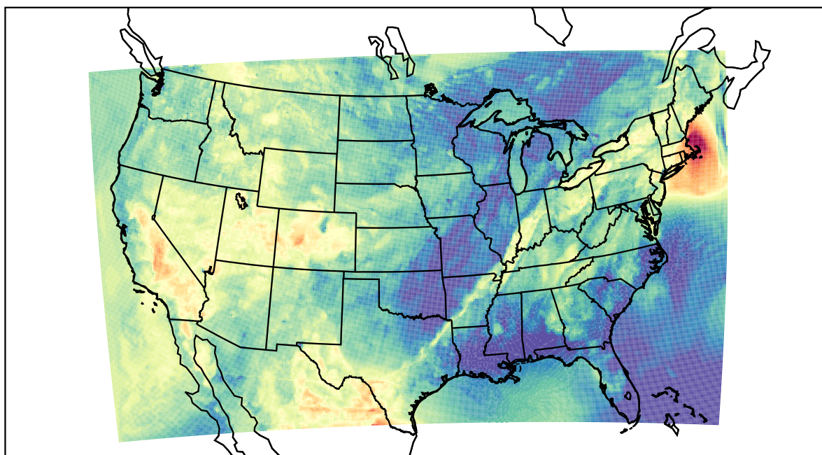
WRF (2022-05-22_03:00:00)
