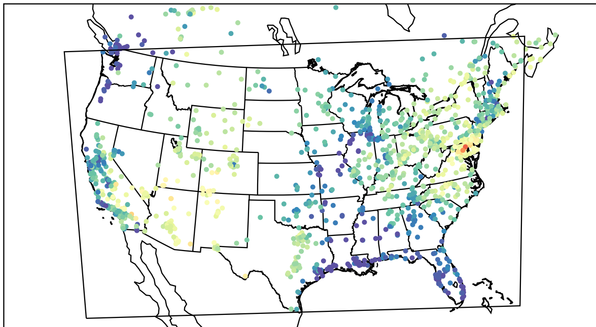
AirNOW (2022-05-21_15:00:00)
