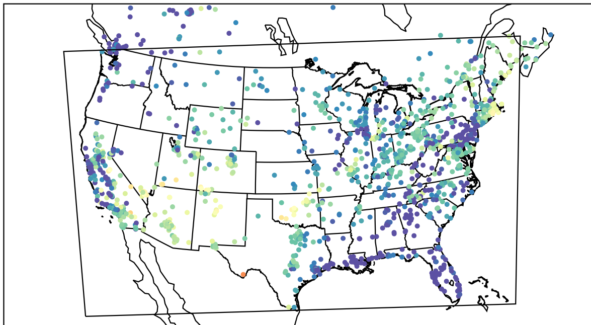
AirNOW (2022-05-21_09:00:00)
