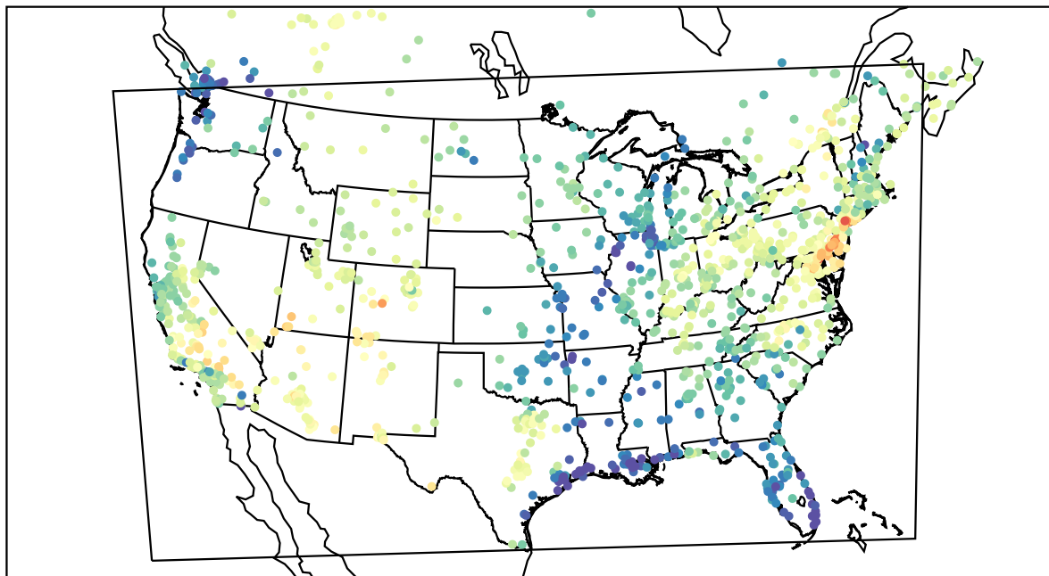
AirNOW (2022-05-21_17:00:00)
