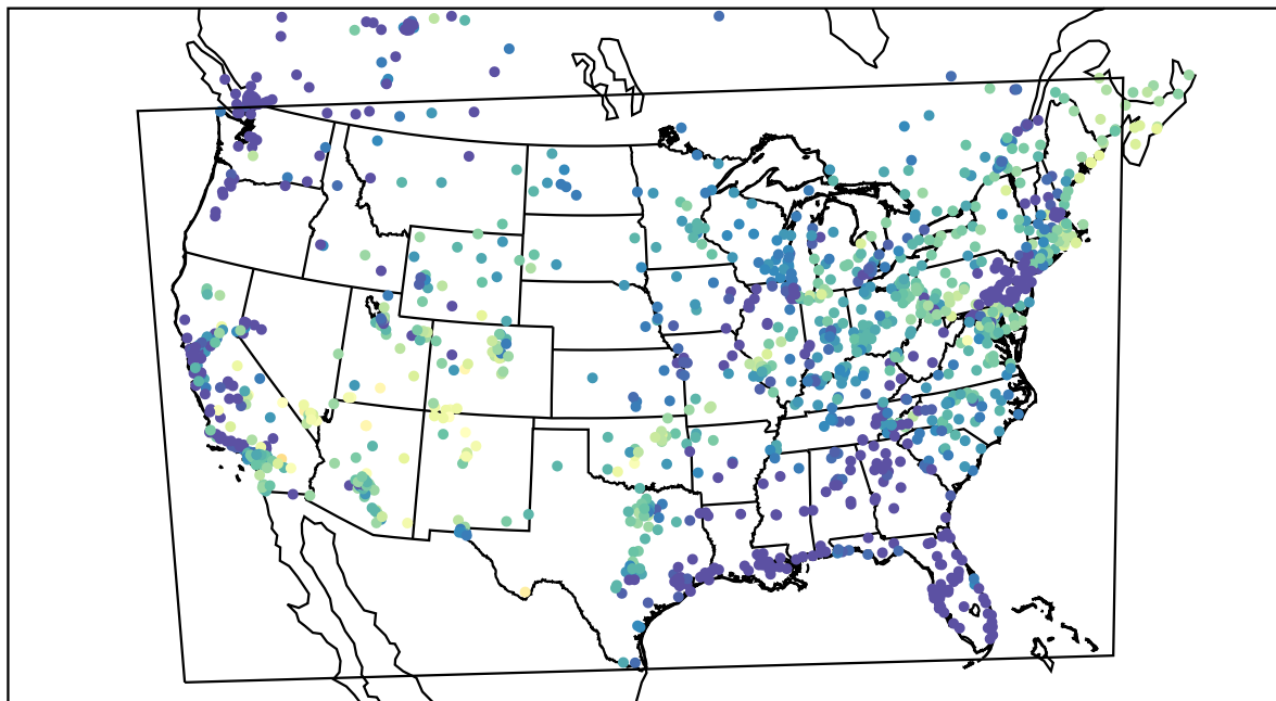
AirNOW (2022-05-21_12:00:00)
