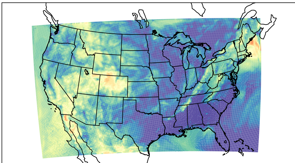
WRF (2022-05-22_12:00:00)
