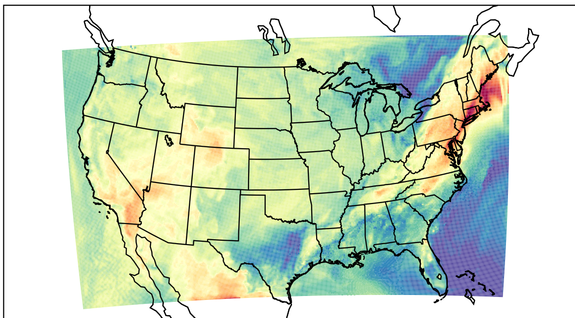
WRF (2022-05-22_18:00:00)
