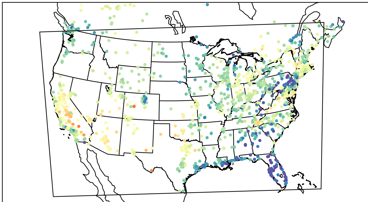
AirNOW (2022-05-21_01:00:00)
