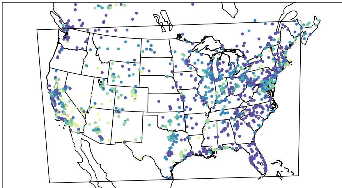
AirNOW (2022-05-22_09:00:00)
