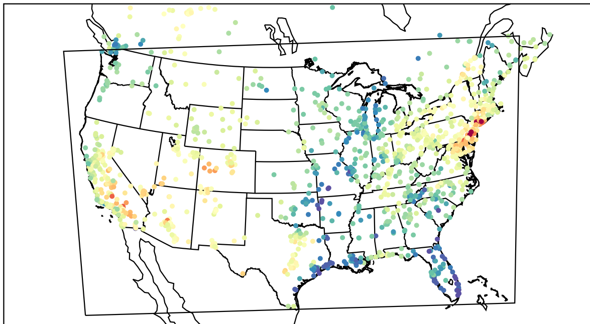
AirNOW (2022-05-21_20:00:00)
