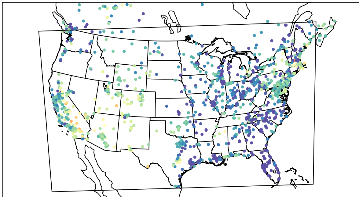
AirNOW (2022-05-22_05:00:00)
