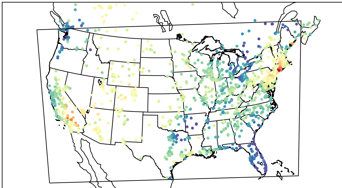
AirNOW (2022-05-22_17:00:00)
