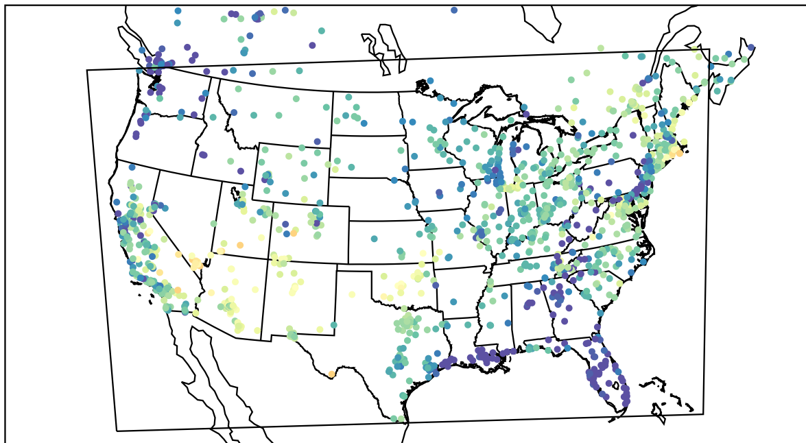
AirNOW (2022-05-21_06:00:00)
