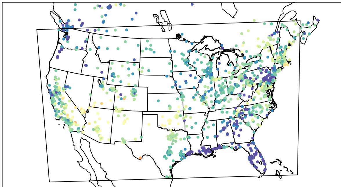
AirNOW (2022-05-21_05:00:00)
