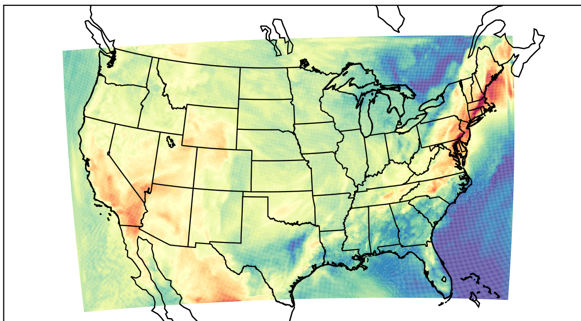
WRF (2022-05-22_21:00:00)
