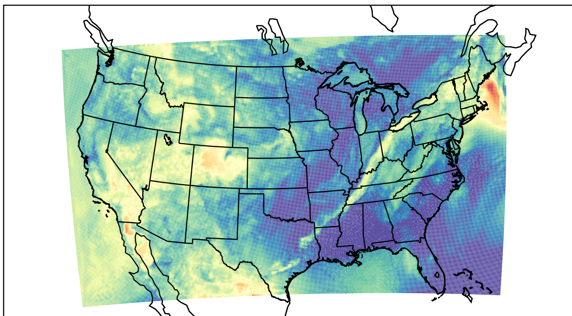
WRF (2022-05-22_07:00:00)
