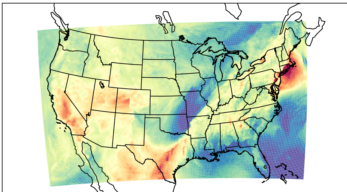
WRF (2022-05-21_23:00:00)
