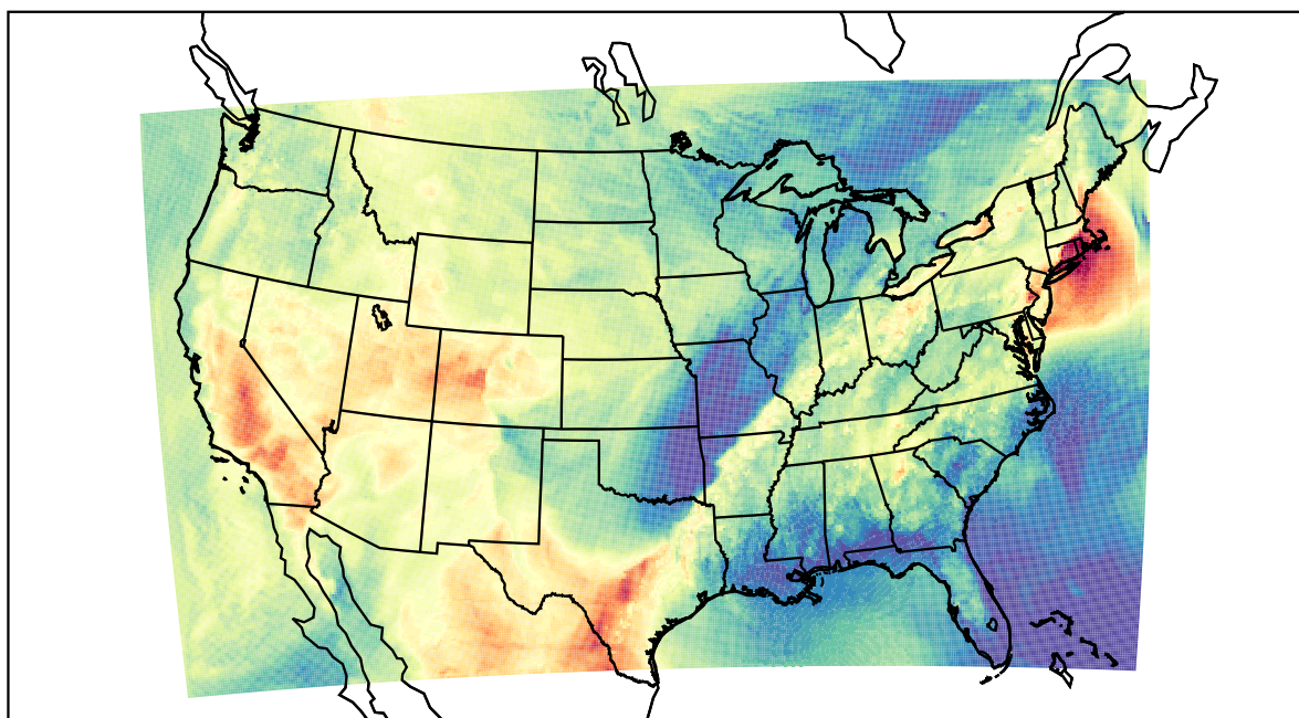
WRF (2022-05-22_00:00:00)
