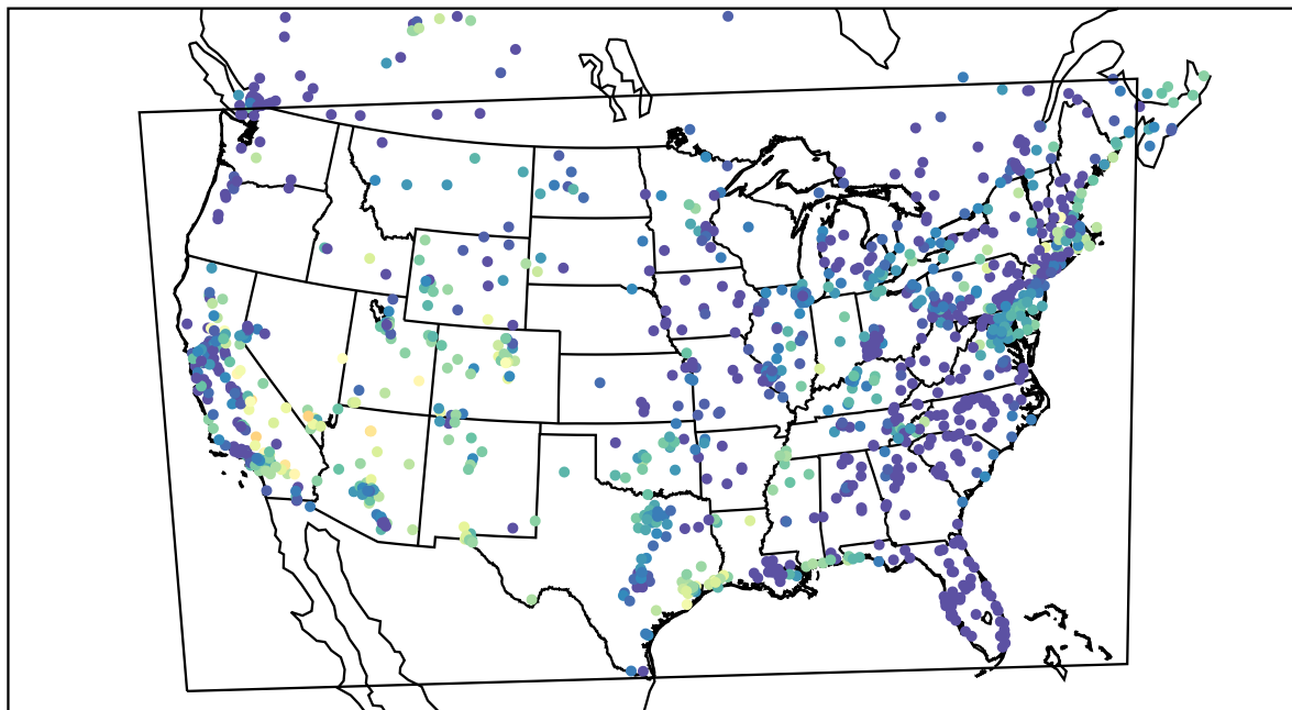
AirNOW (2022-05-22_10:00:00)
