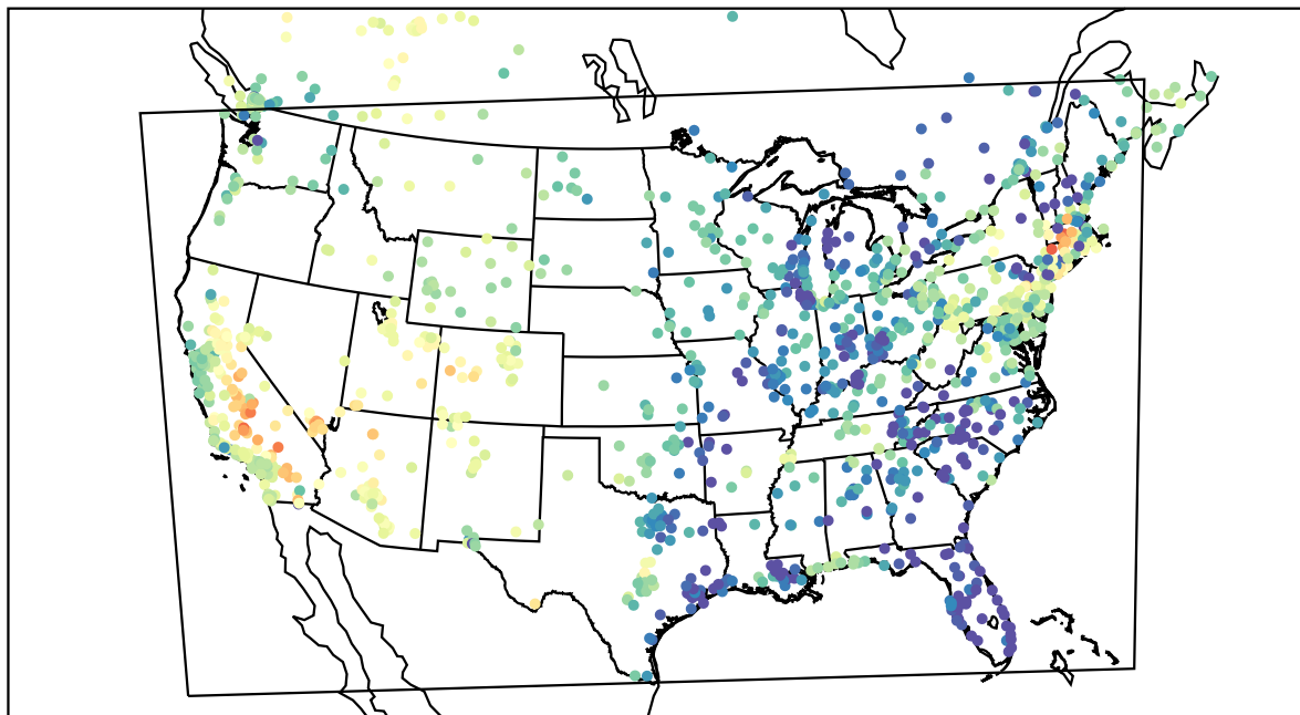
AirNOW (2022-05-22_02:00:00)
