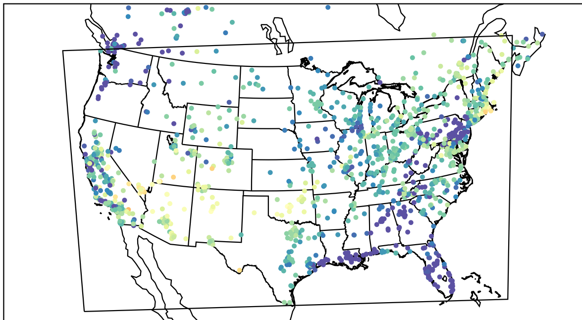
AirNOW (2022-05-21_07:00:00)
