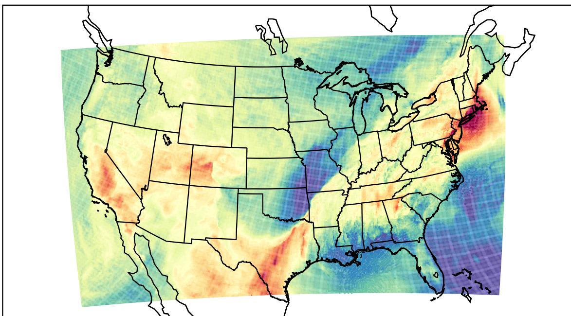
WRF (2022-05-21_22:00:00)
