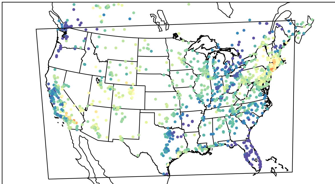
AirNOW (2022-05-22_15:00:00)
