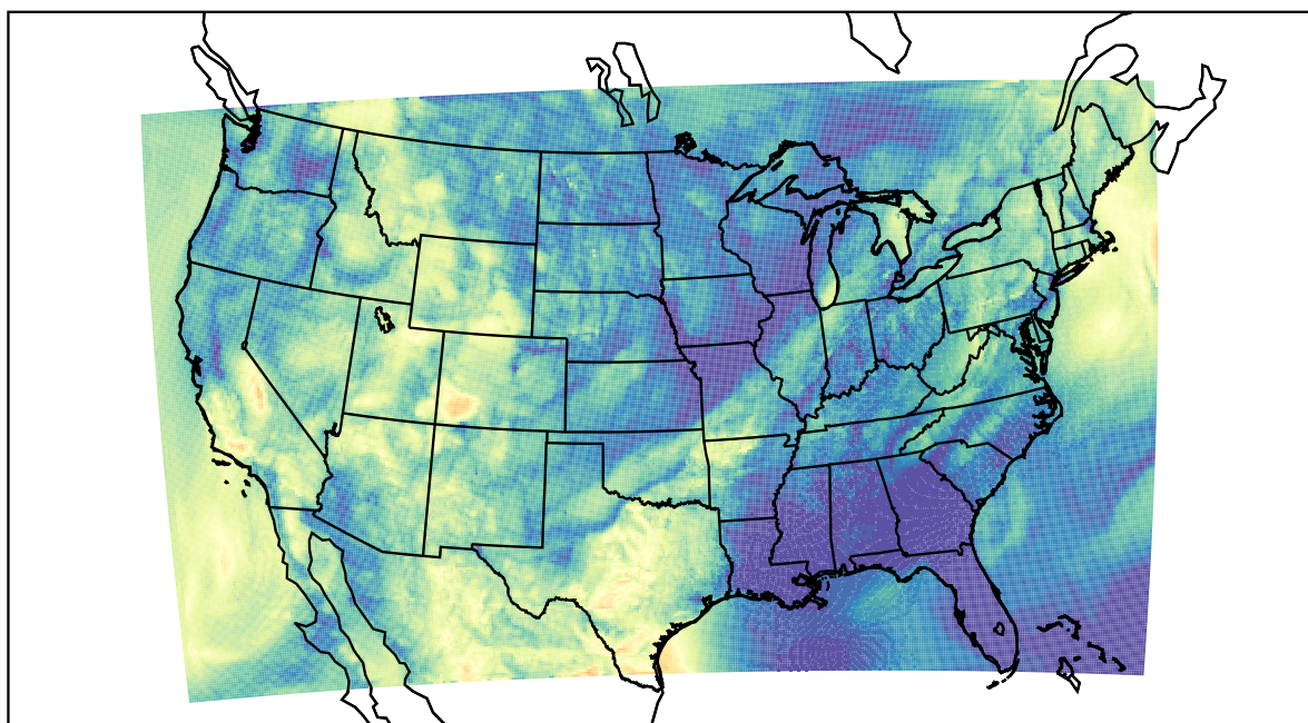
WRF (2022-05-21_12:00:00)
