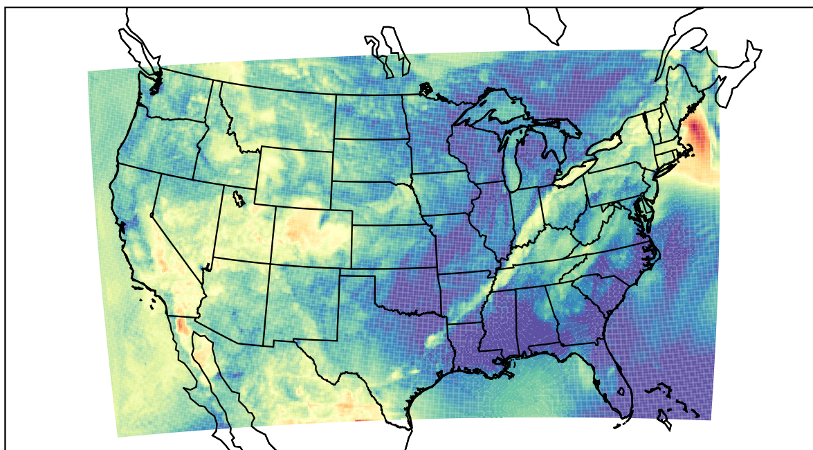
WRF (2022-05-22_06:00:00)
