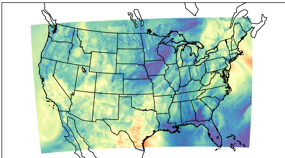
WRF (2022-05-21_05:00:00)
