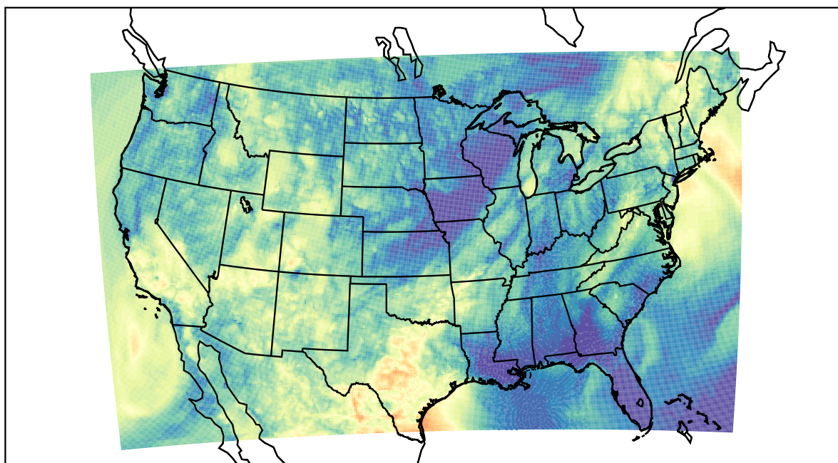
WRF (2022-05-21_07:00:00)
