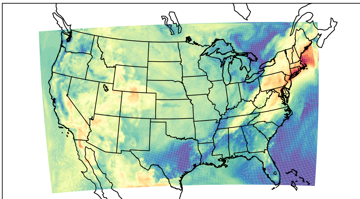
WRF (2022-05-22_16:00:00)
