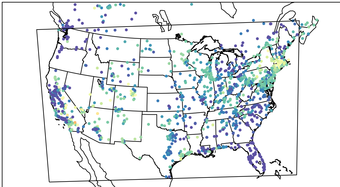
AirNOW (2022-05-22_13:00:00)
