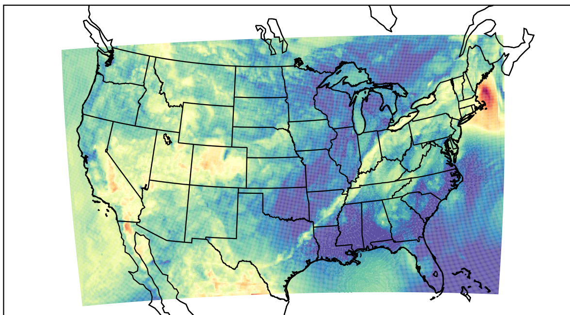
WRF (2022-05-22_05:00:00)
