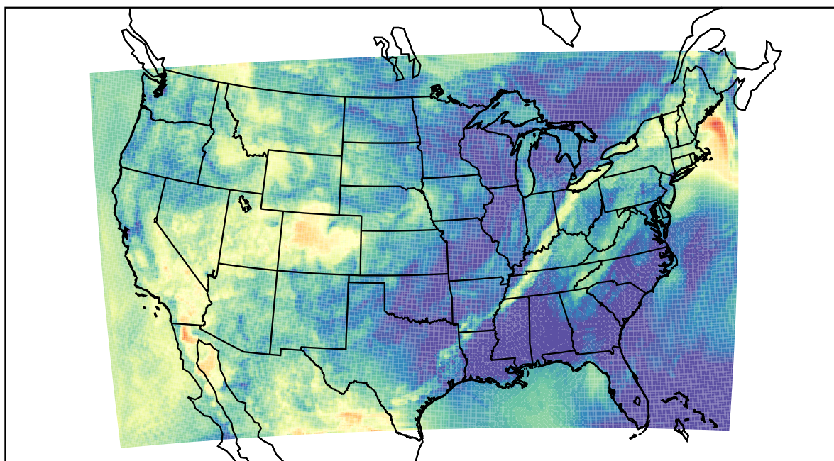
WRF (2022-05-22_08:00:00)
