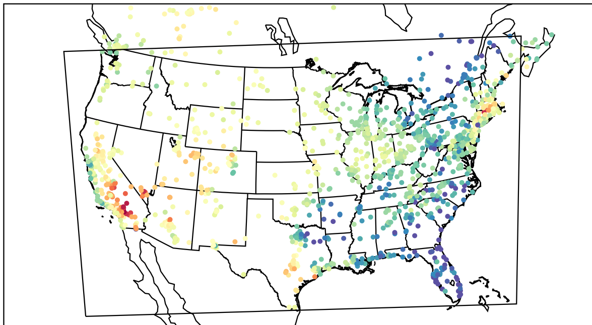
AirNOW (2022-05-22_23:00:00)
