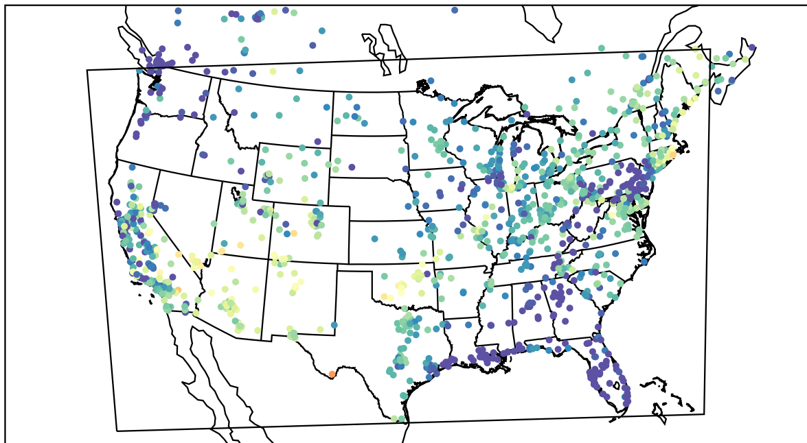
AirNOW (2022-05-21_08:00:00)
