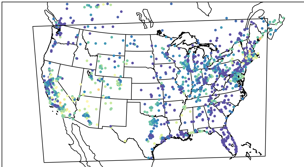
AirNOW (2022-05-22_08:00:00)
