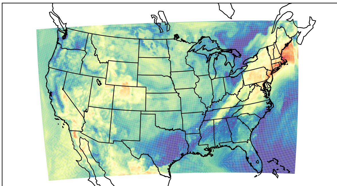
WRF (2022-05-22_15:00:00)
