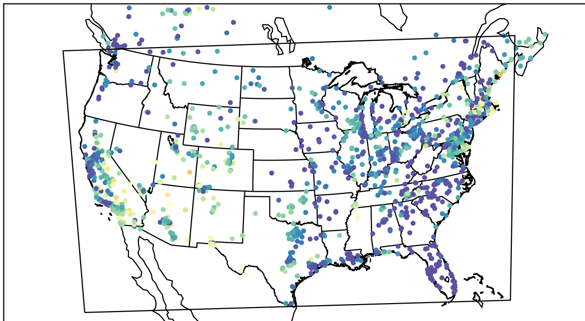
AirNOW (2022-05-22_07:00:00)
