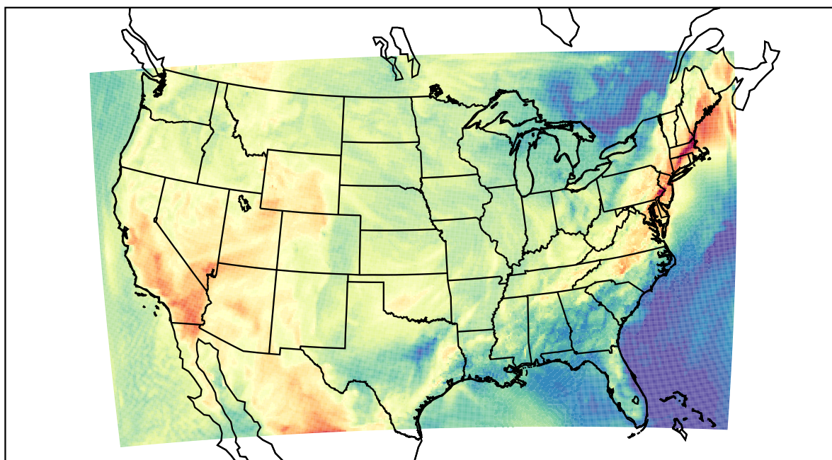
WRF (2022-05-22_22:00:00)
