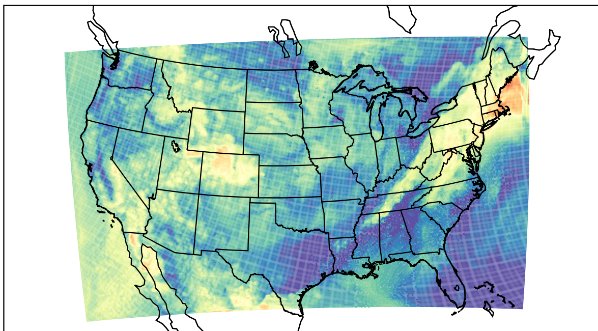
WRF (2022-05-22_14:00:00)
