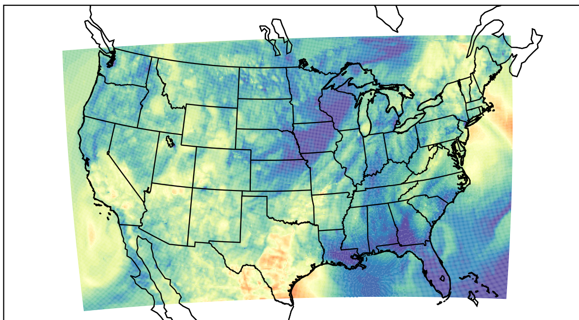
WRF (2022-05-21_06:00:00)
