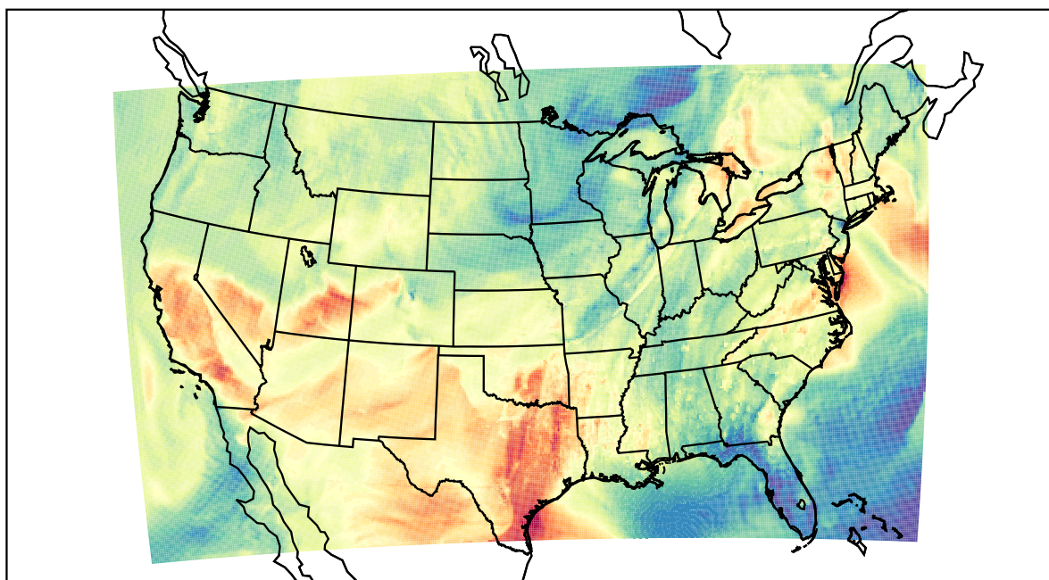
WRF (2022-05-21_00:00:00)
