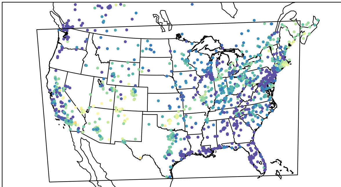
AirNOW (2022-05-21_11:00:00)
