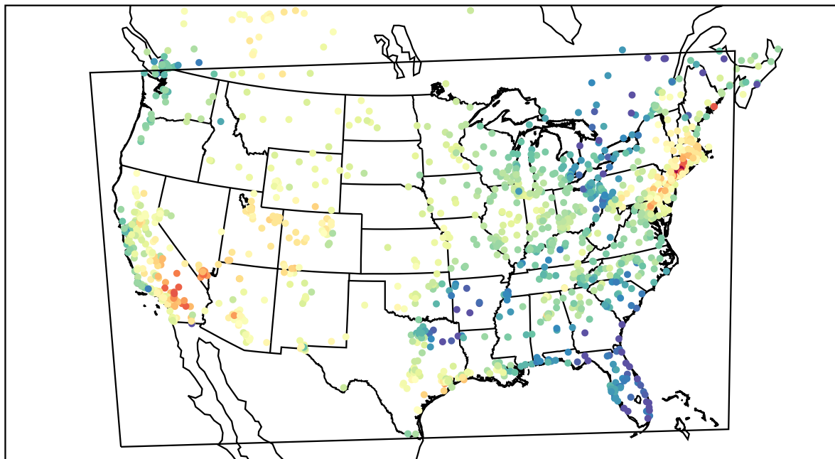
AirNOW (2022-05-22_19:00:00)
