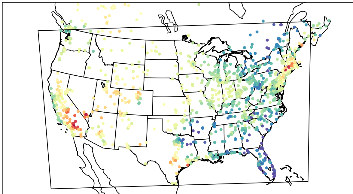
AirNOW (2022-05-22_22:00:00)
