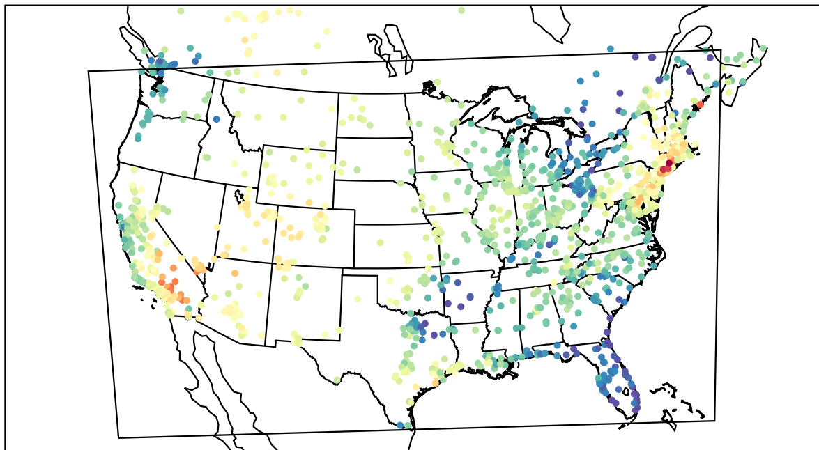
AirNOW (2022-05-22_18:00:00)
