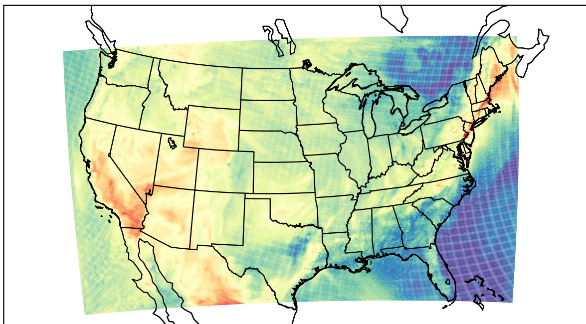
WRF (2022-05-22_23:00:00)
