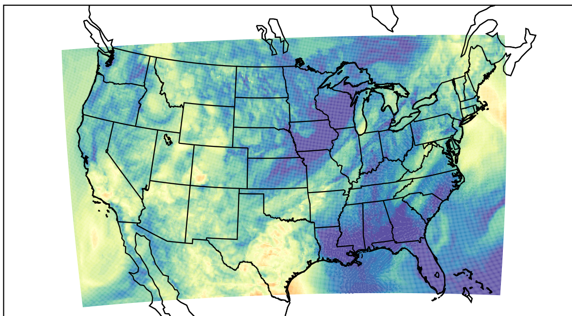
WRF (2022-05-21_09:00:00)
