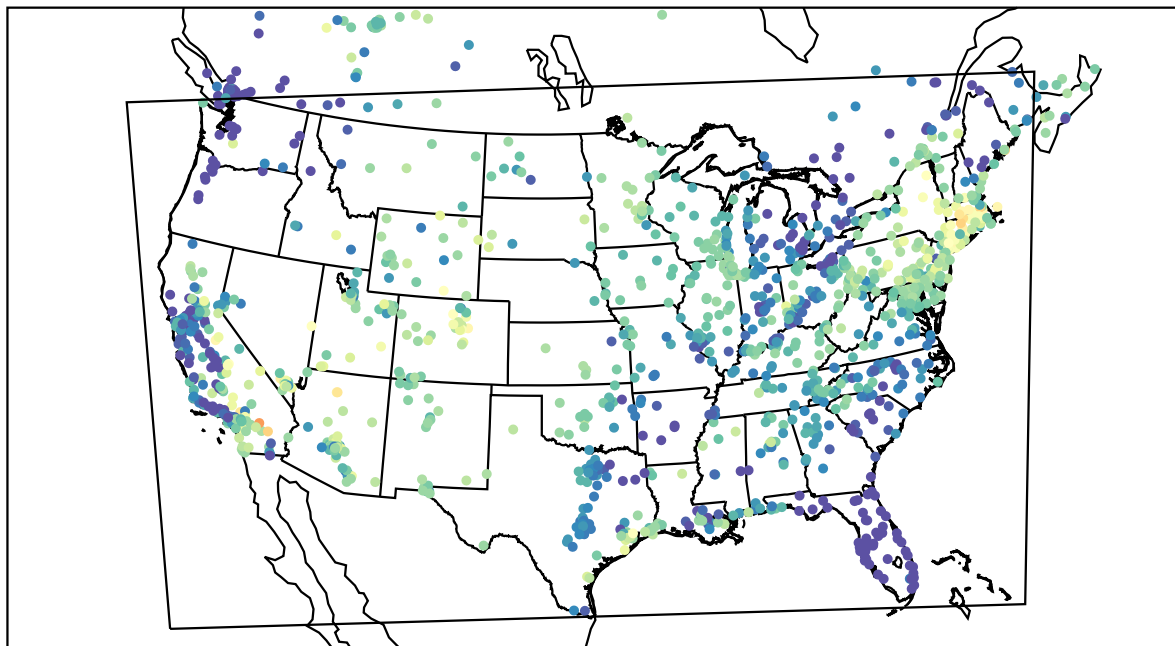
AirNOW (2022-05-22_14:00:00)
