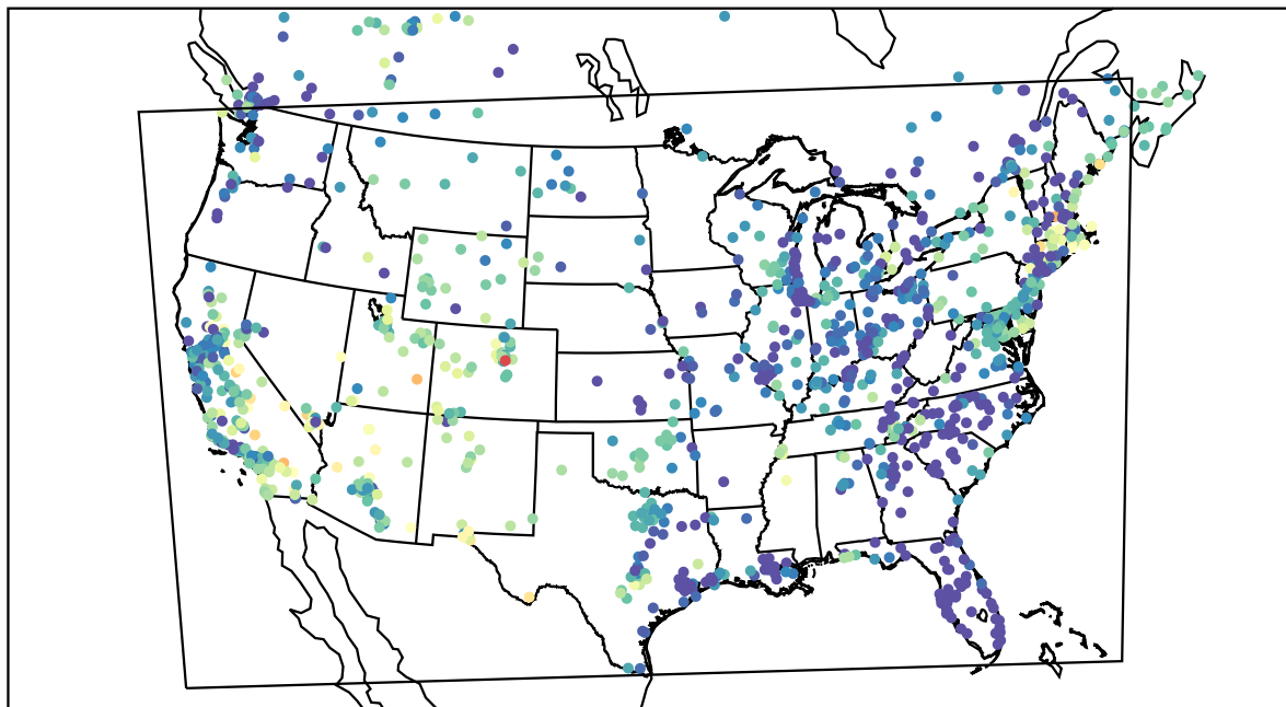
AirNOW (2022-05-22_06:00:00)
