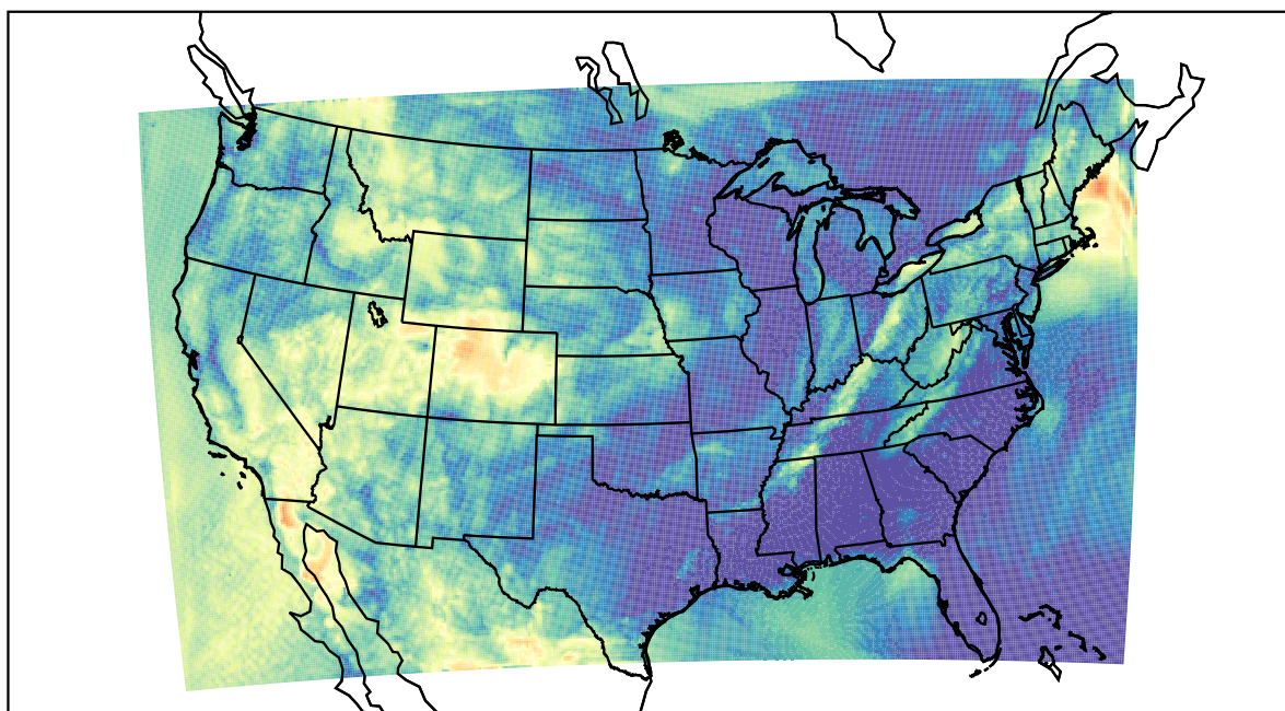
WRF (2022-05-22_11:00:00)
