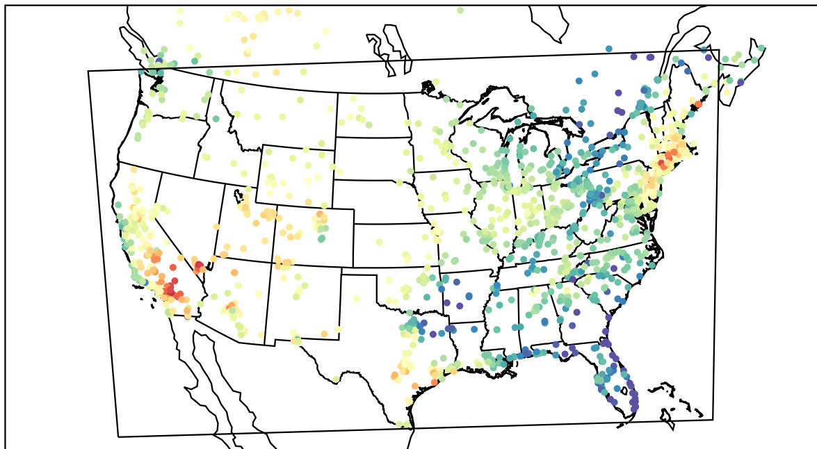
AirNOW (2022-05-22_21:00:00)
