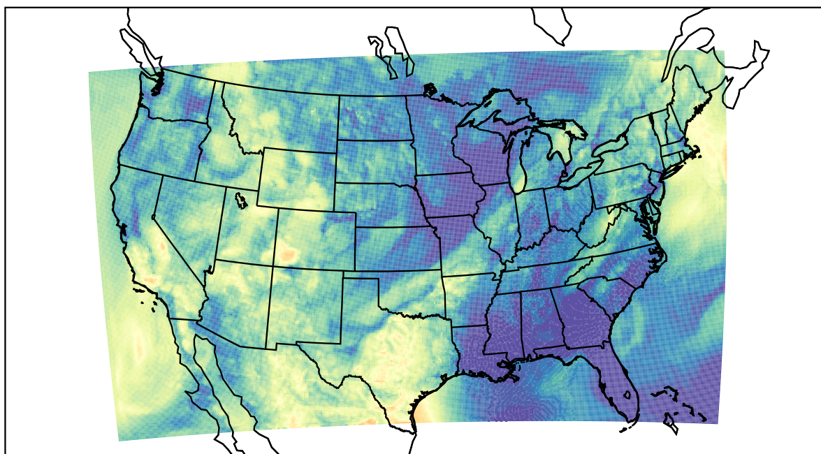
WRF (2022-05-21_11:00:00)
