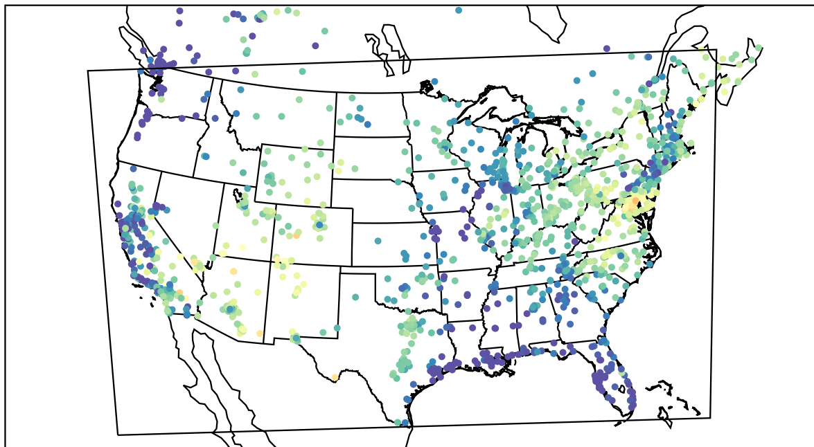
AirNOW (2022-05-21_14:00:00)
