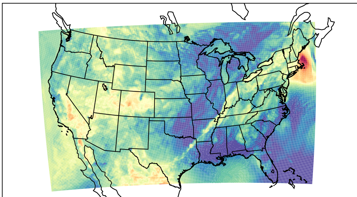
WRF (2022-05-22_04:00:00)
