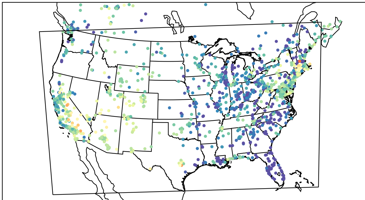
AirNOW (2022-05-22_04:00:00)
