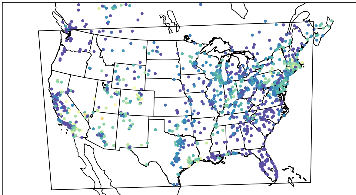
AirNOW (2022-05-22_12:00:00)
