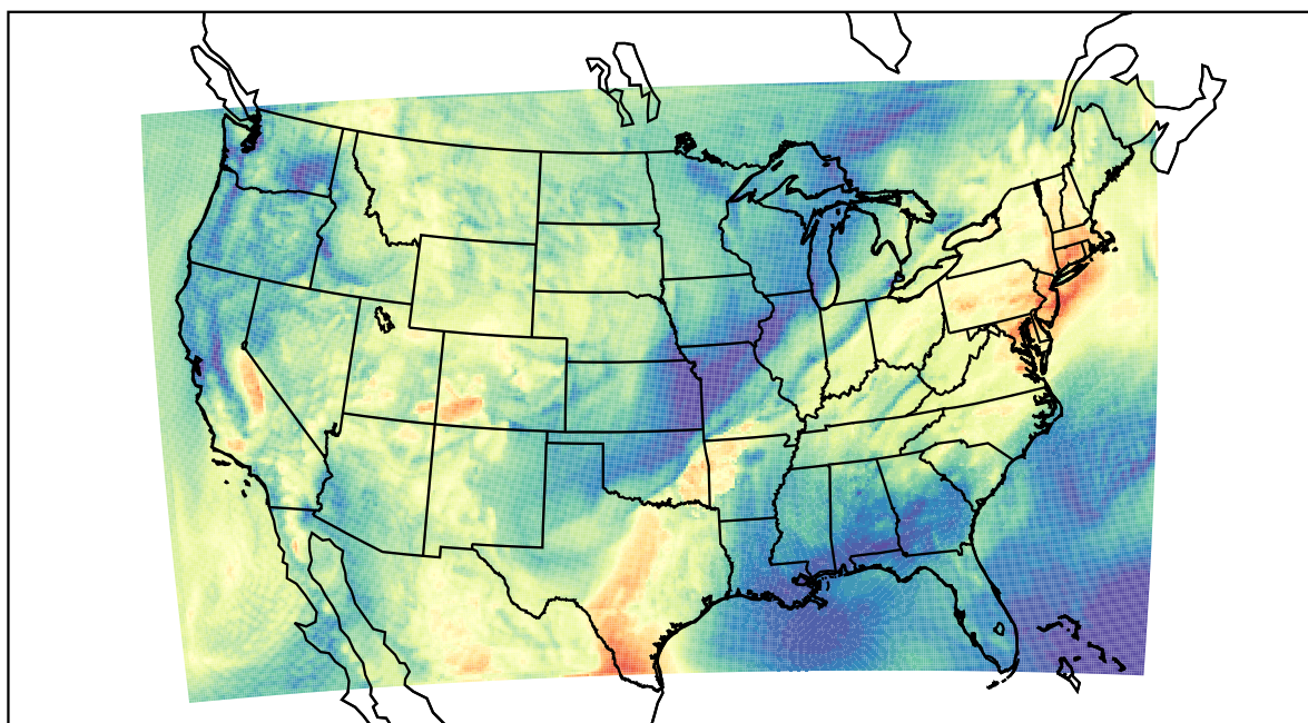
WRF (2022-05-21_15:00:00)
