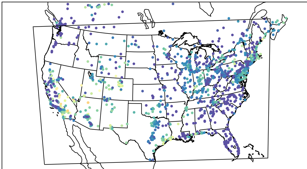
AirNOW (2022-05-22_11:00:00)
