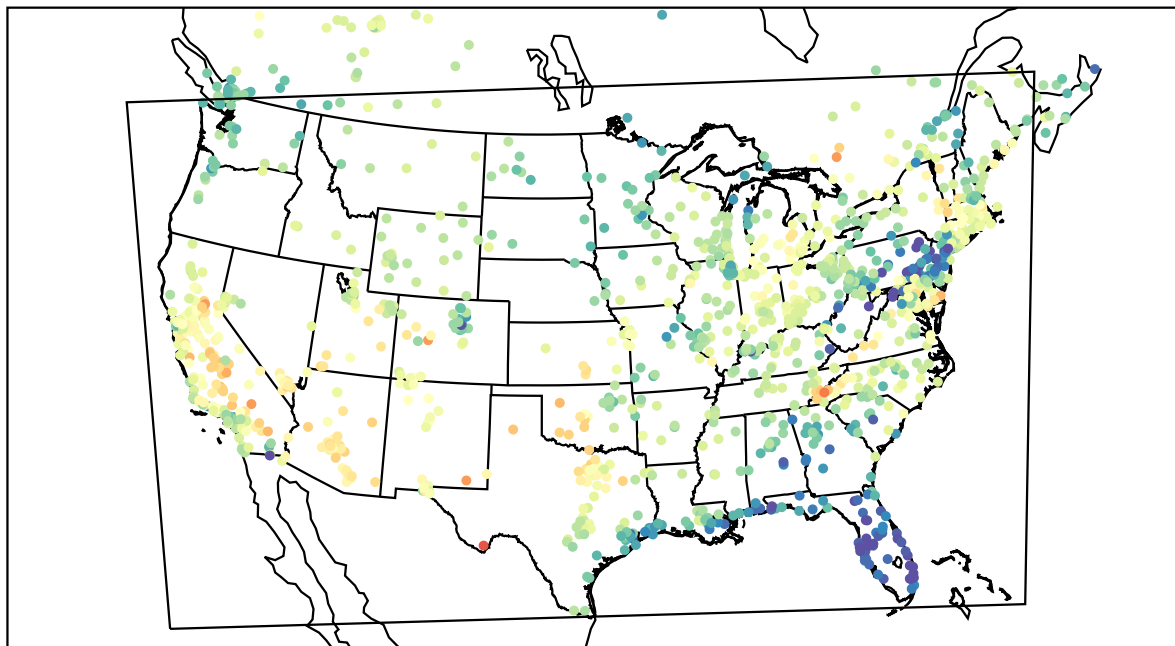
AirNOW (2022-05-21_00:00:00)
