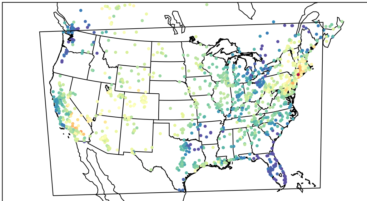
AirNOW (2022-05-22_16:00:00)
