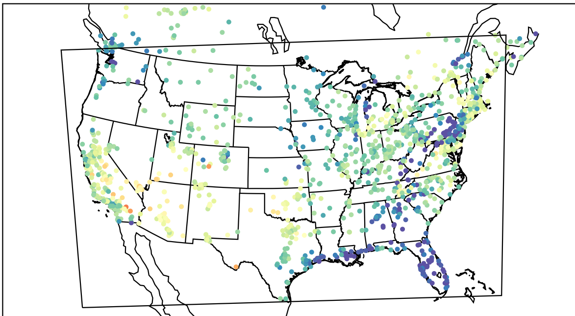
AirNOW (2022-05-21_03:00:00)
