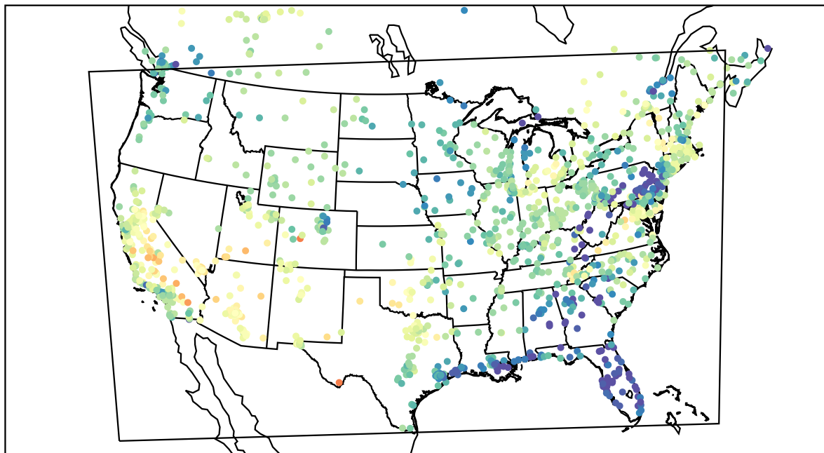
AirNOW (2022-05-21_02:00:00)
