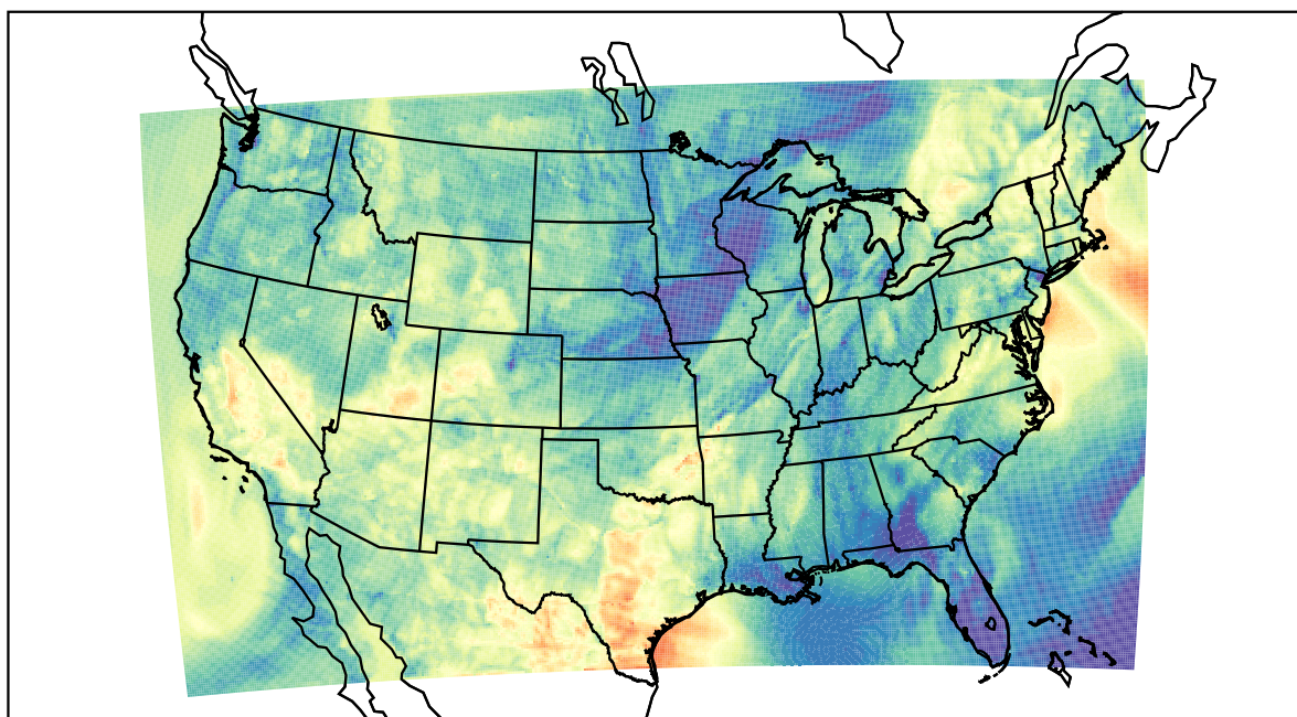
WRF (2022-05-21_04:00:00)
