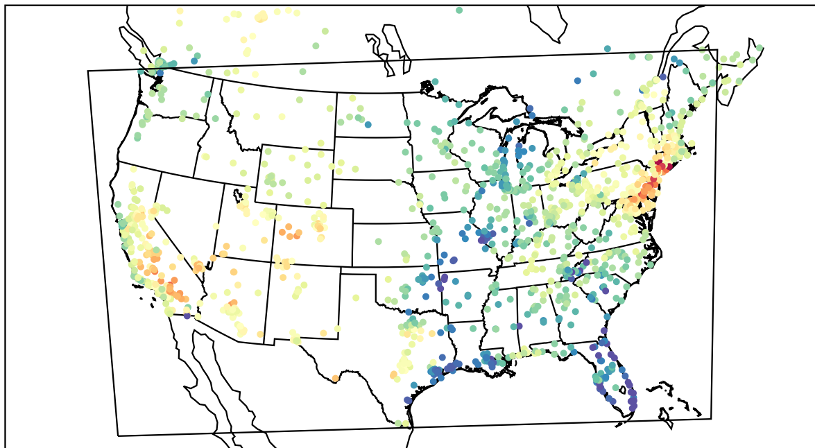
AirNOW (2022-05-21_21:00:00)
