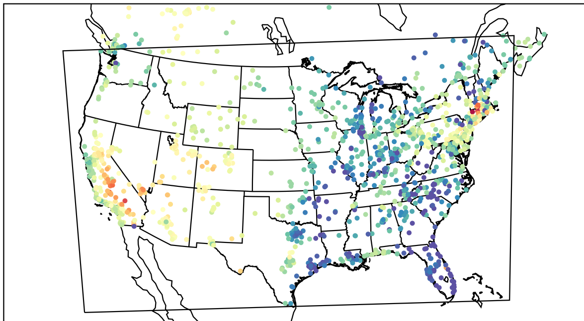
AirNOW (2022-05-22_01:00:00)
