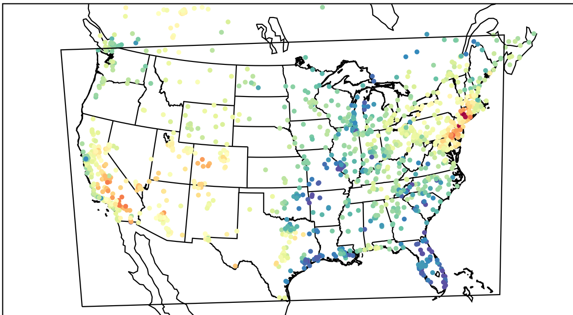
AirNOW (2022-05-21_22:00:00)
