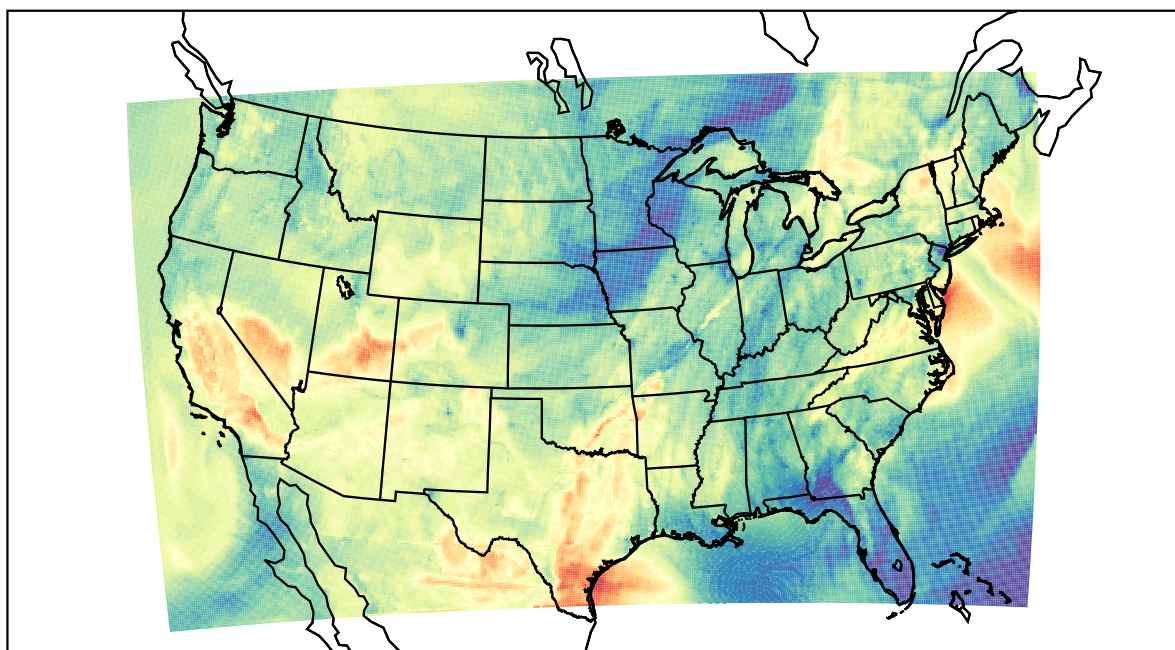
WRF (2022-05-21_02:00:00)
