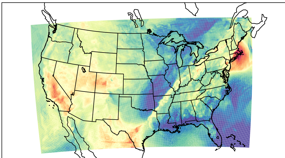
WRF (2022-05-22_01:00:00)
