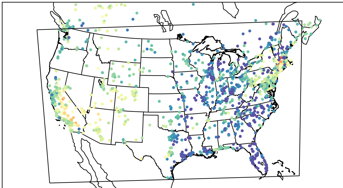
AirNOW (2022-05-22_03:00:00)
