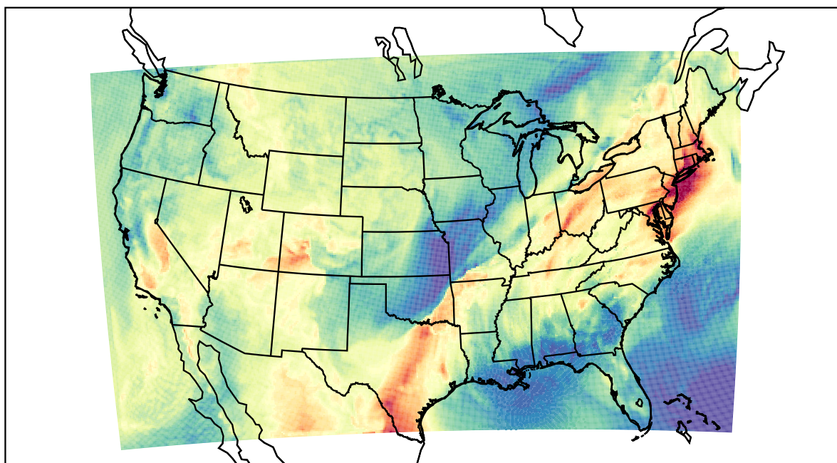
WRF (2022-05-21_17:00:00)
