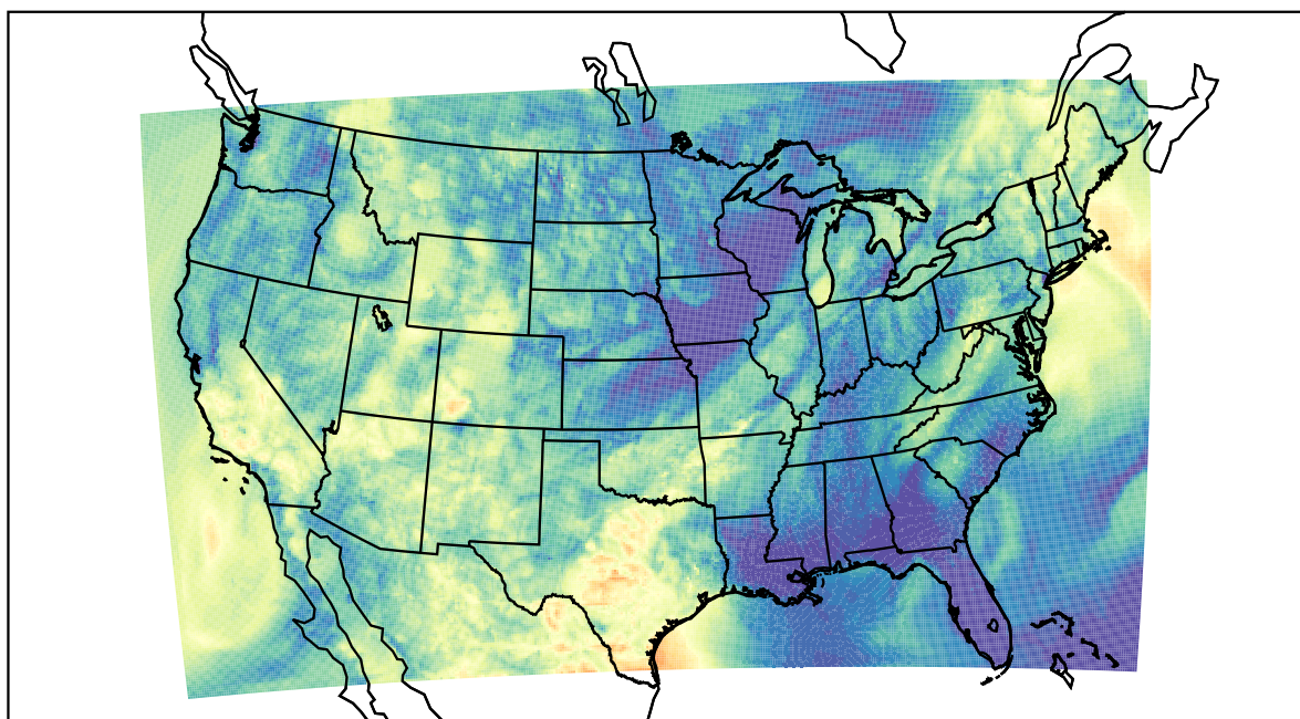
WRF (2022-05-21_08:00:00)
