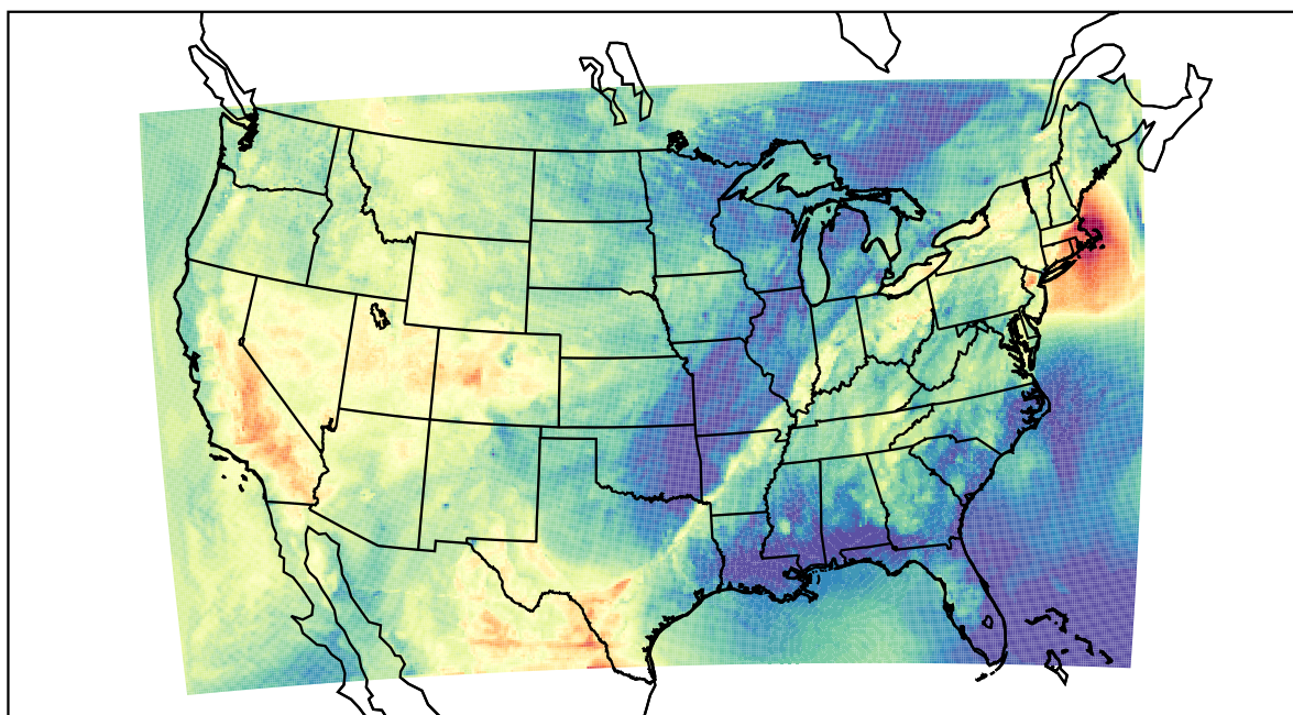
WRF (2022-05-22_02:00:00)
