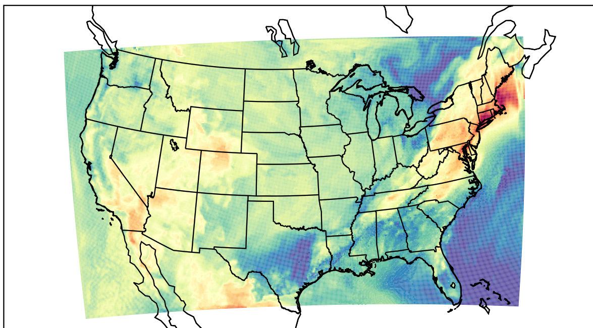
WRF (2022-05-22_17:00:00)
