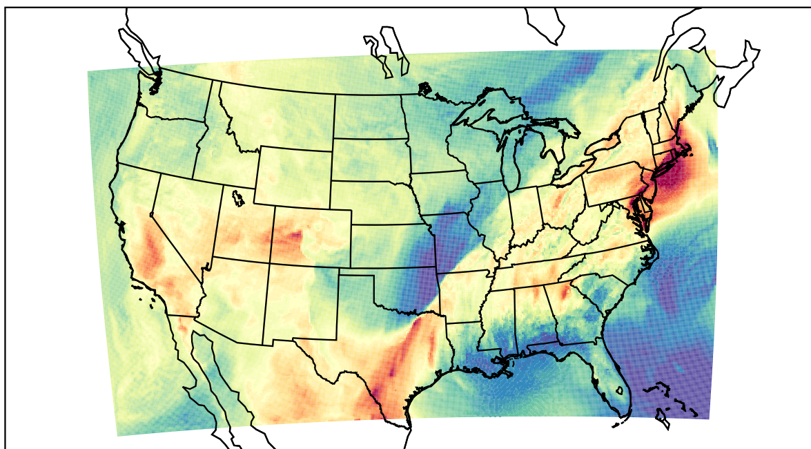
WRF (2022-05-21_21:00:00)
