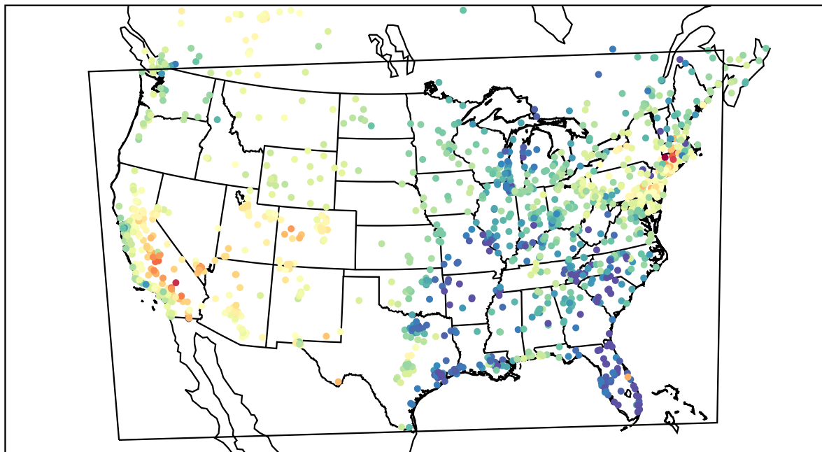
AirNOW (2022-05-22_00:00:00)
