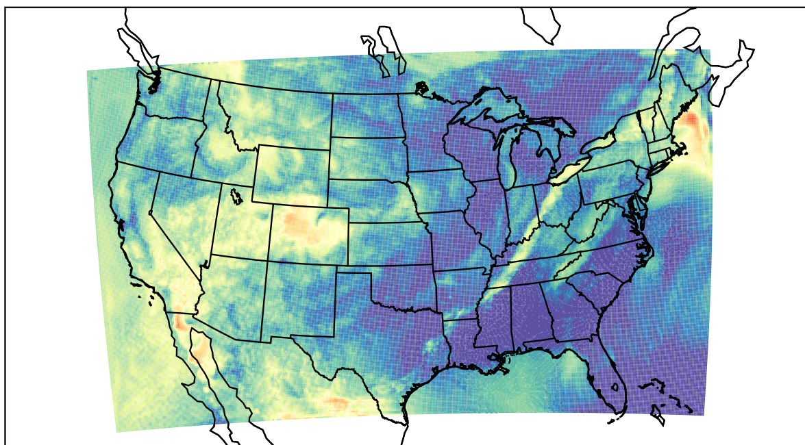
WRF (2022-05-22_09:00:00)
