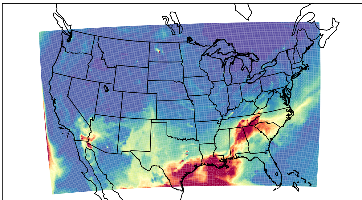
WRF 2022-05-23_15:00:00
