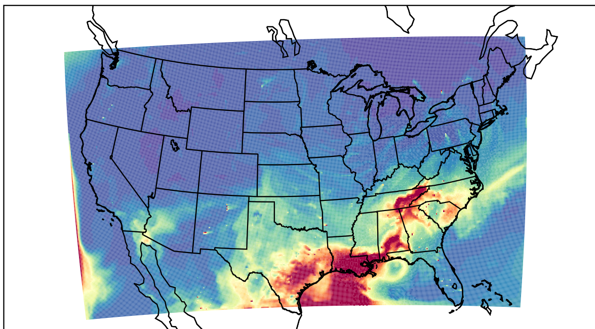
WRF 2022-05-23_21:00:00
