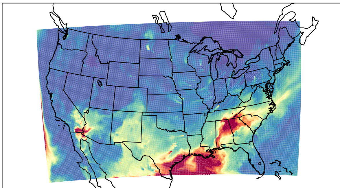
WRF 2022-05-23_13:00:00
