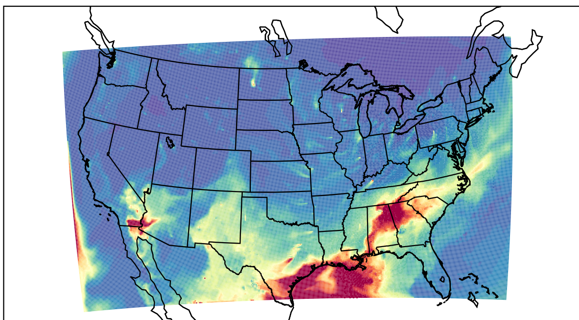
WRF 2022-05-23_12:00:00
