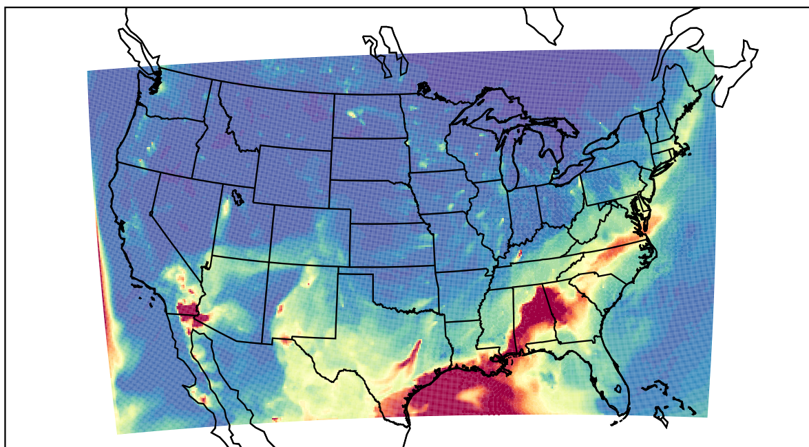
WRF 2022-05-23_05:00:00
