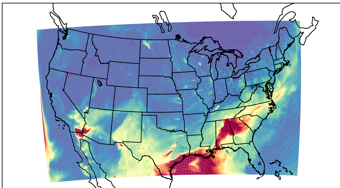
WRF 2022-05-23_09:00:00
