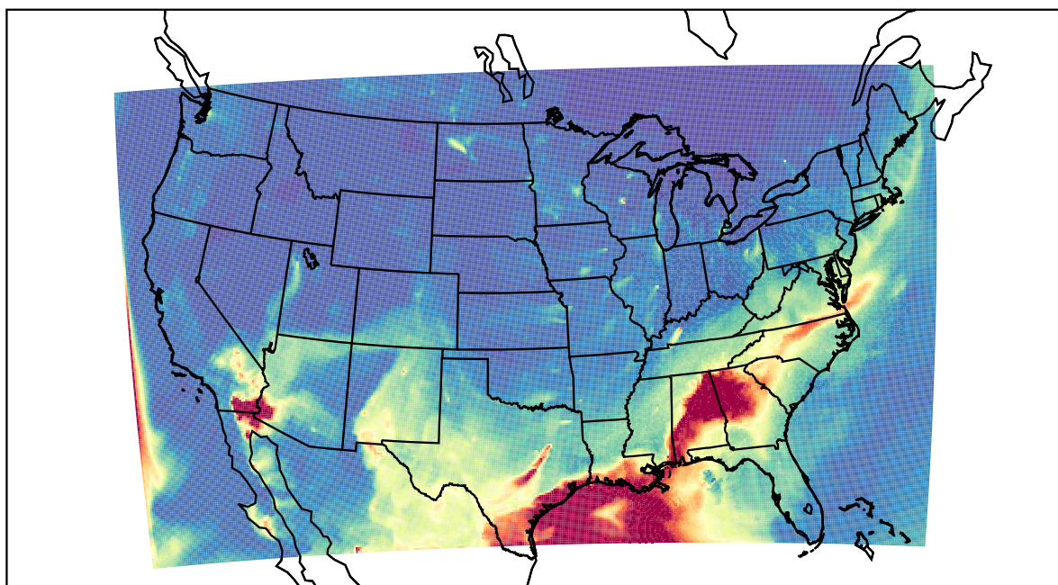
WRF 2022-05-23_07:00:00
