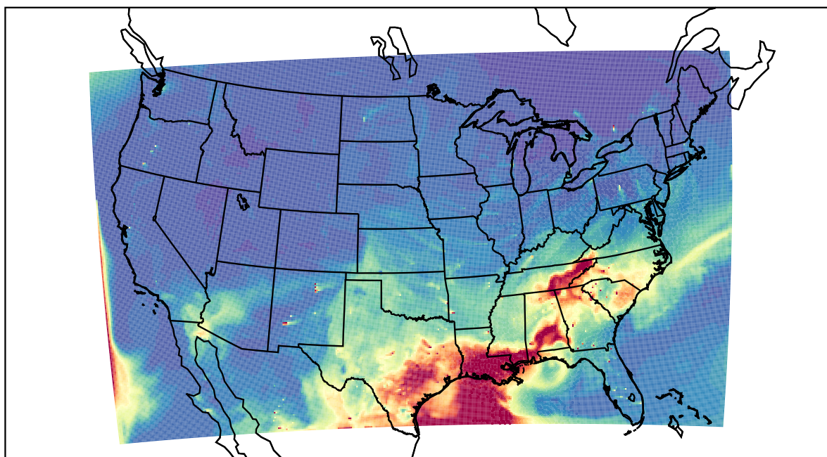
WRF 2022-05-23_22:00:00
