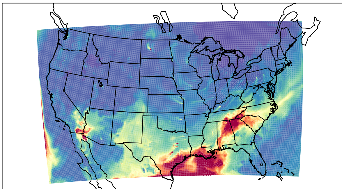
WRF 2022-05-23_14:00:00
