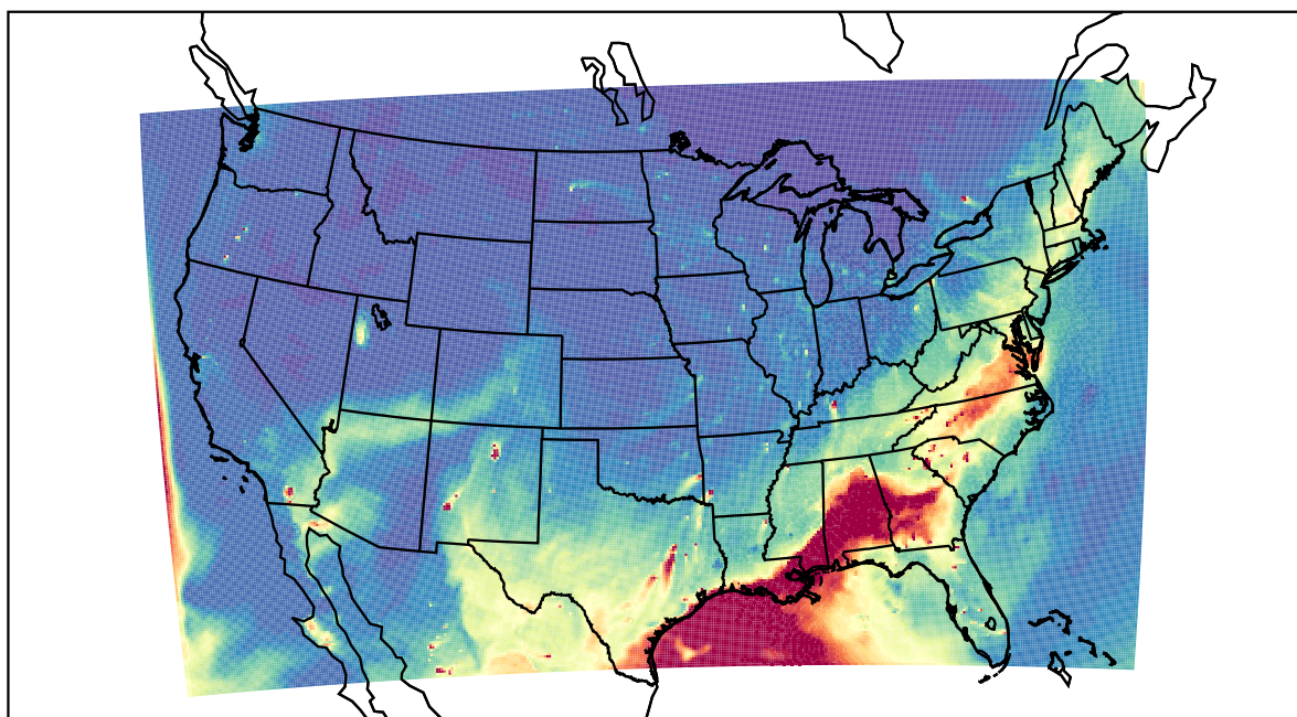
WRF 2022-05-23_01:00:00
