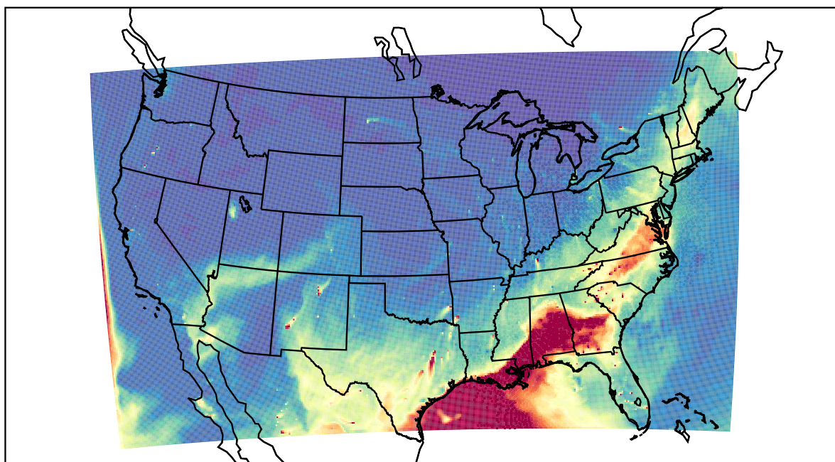
WRF 2022-05-23_00:00:00
