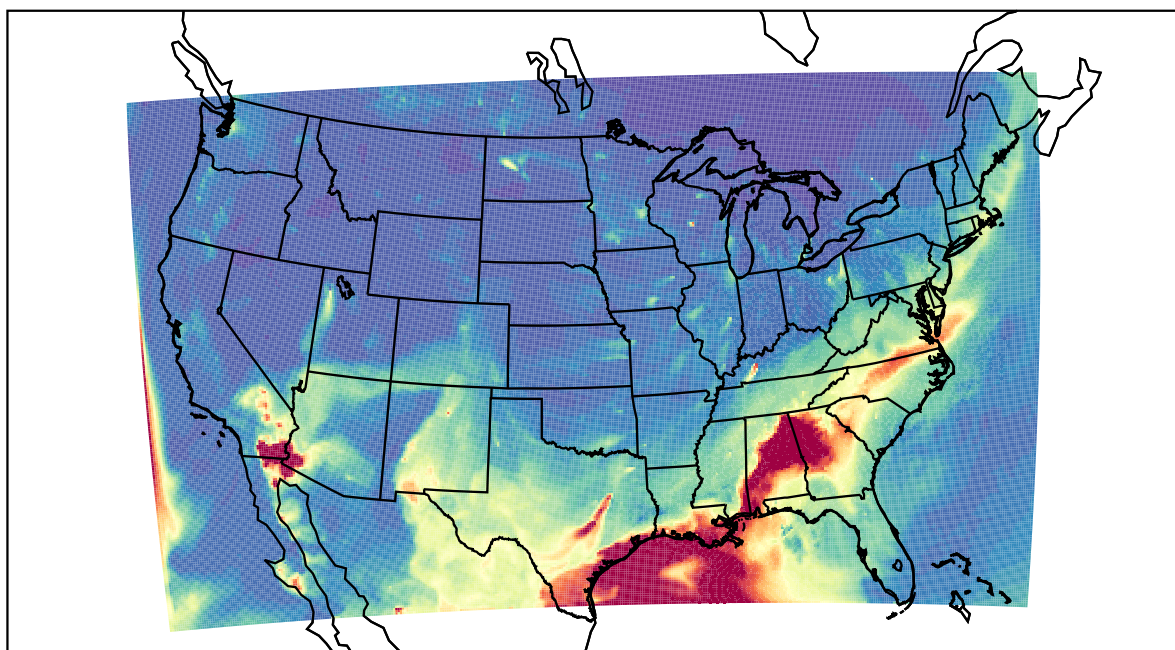
WRF 2022-05-23_06:00:00
