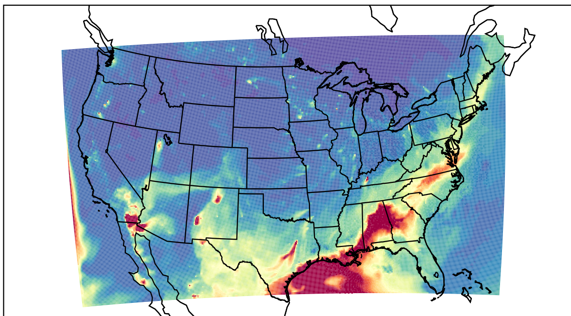
WRF 2022-05-23_04:00:00
