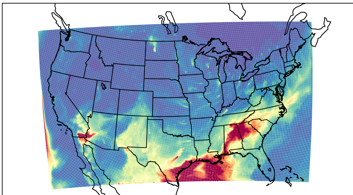
WRF 2022-05-23_11:00:00
