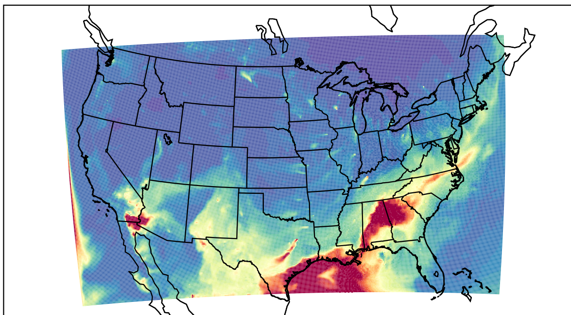
WRF 2022-05-23_08:00:00
