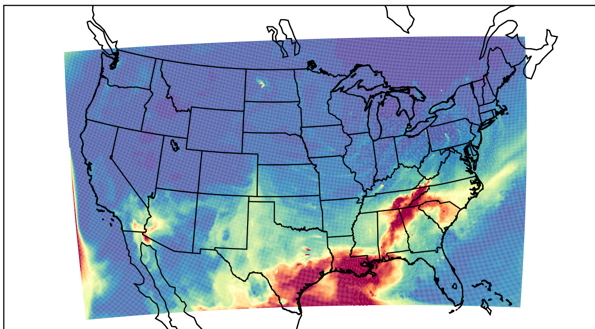
WRF 2022-05-23_17:00:00
