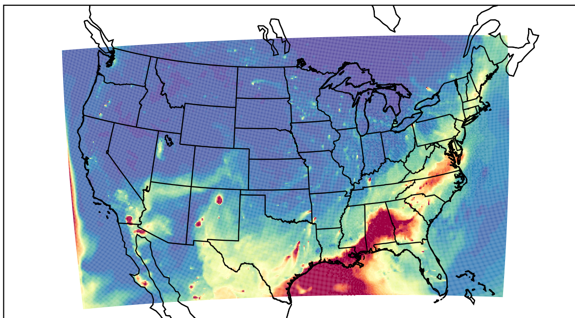
WRF 2022-05-23_02:00:00
