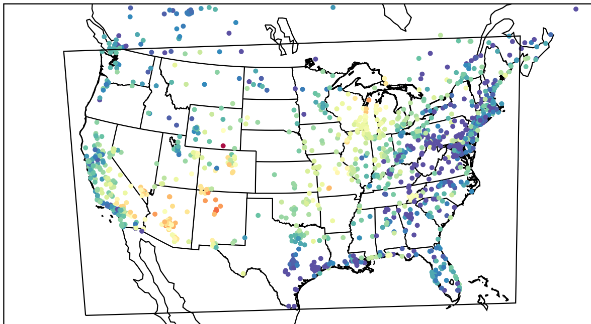
AirNOW (2022-05-30_04:00:00)
