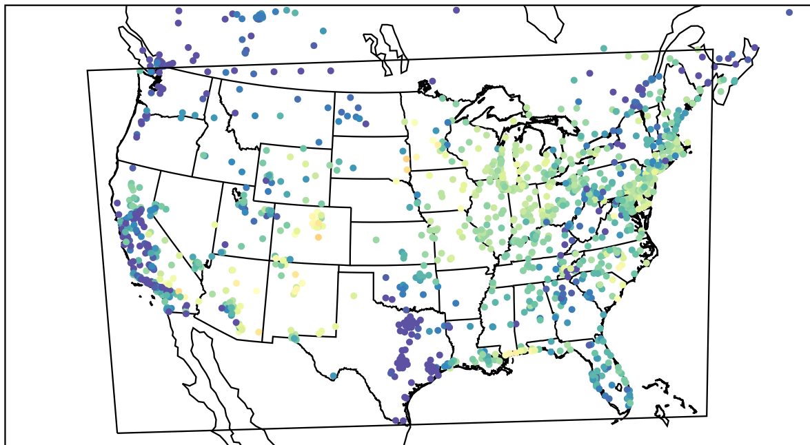
AirNOW (2022-05-30_13:00:00)
