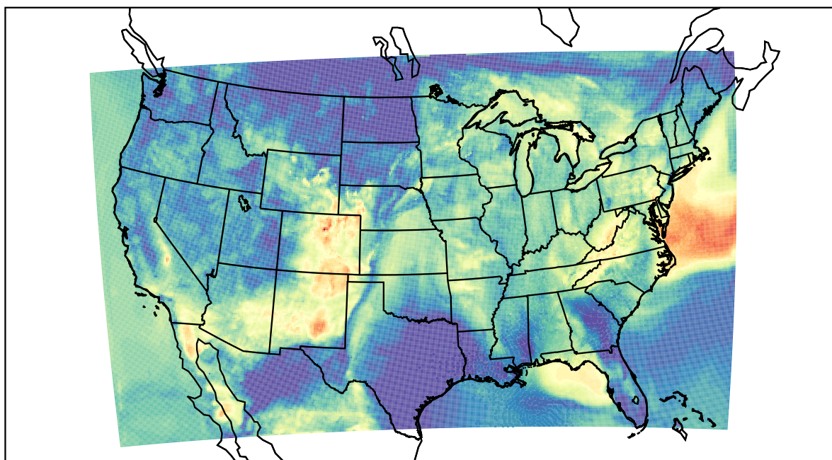
WRF (2022-05-30_08:00:00)
