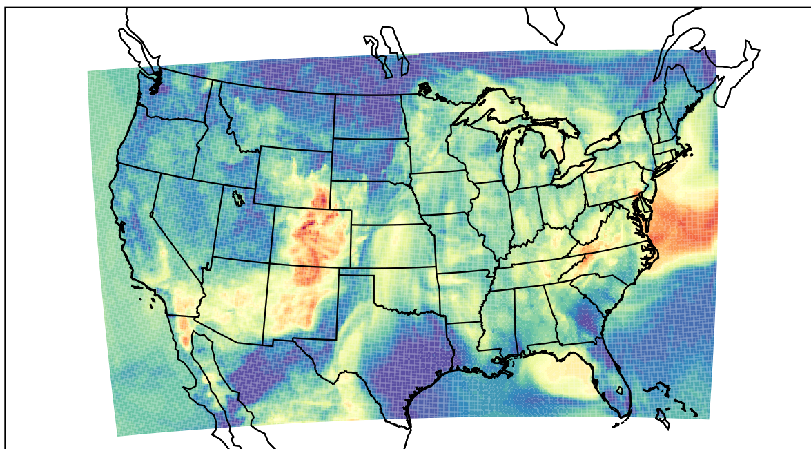
WRF (2022-05-30_05:00:00)
