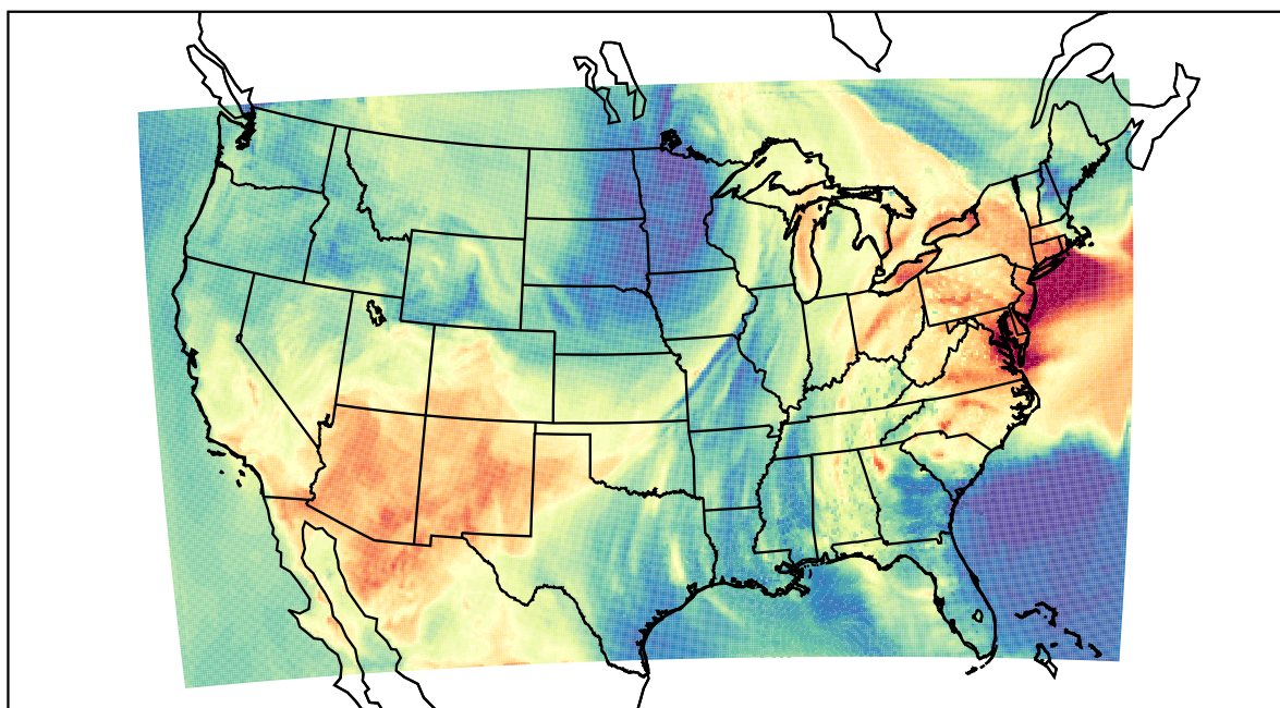
WRF (2022-05-31_20:00:00)
