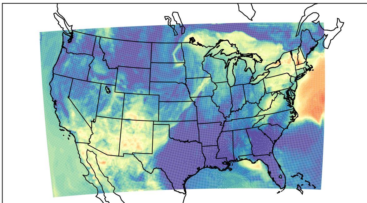
WRF (2022-05-31_09:00:00)
