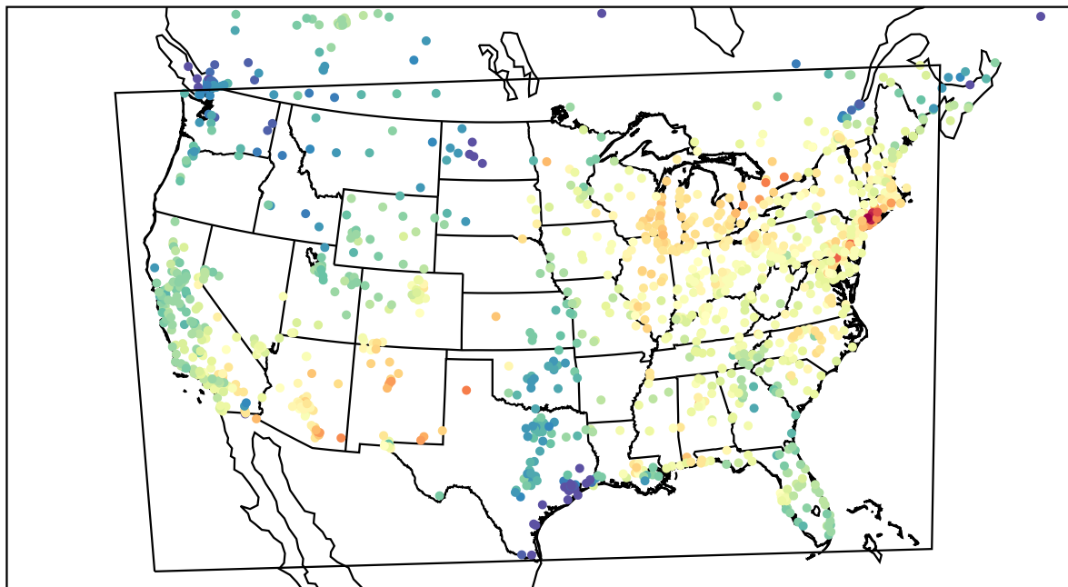
AirNOW (2022-05-30_18:00:00)
