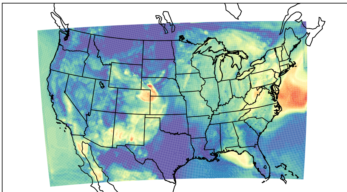
WRF (2022-05-30_13:00:00)
