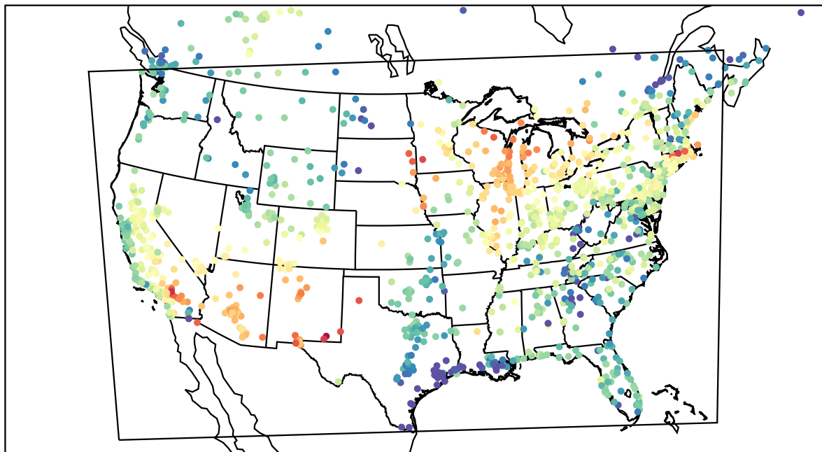
AirNOW (2022-05-31_00:00:00)
