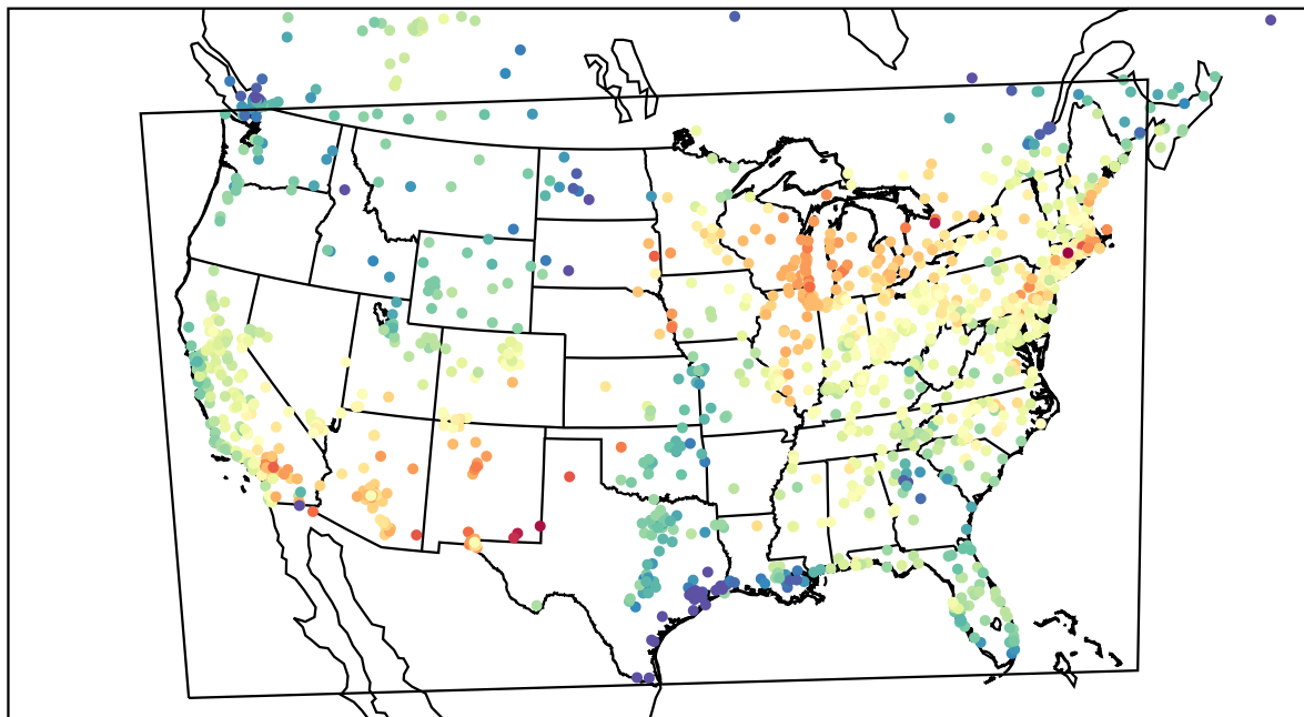
AirNOW (2022-05-30_22:00:00)
