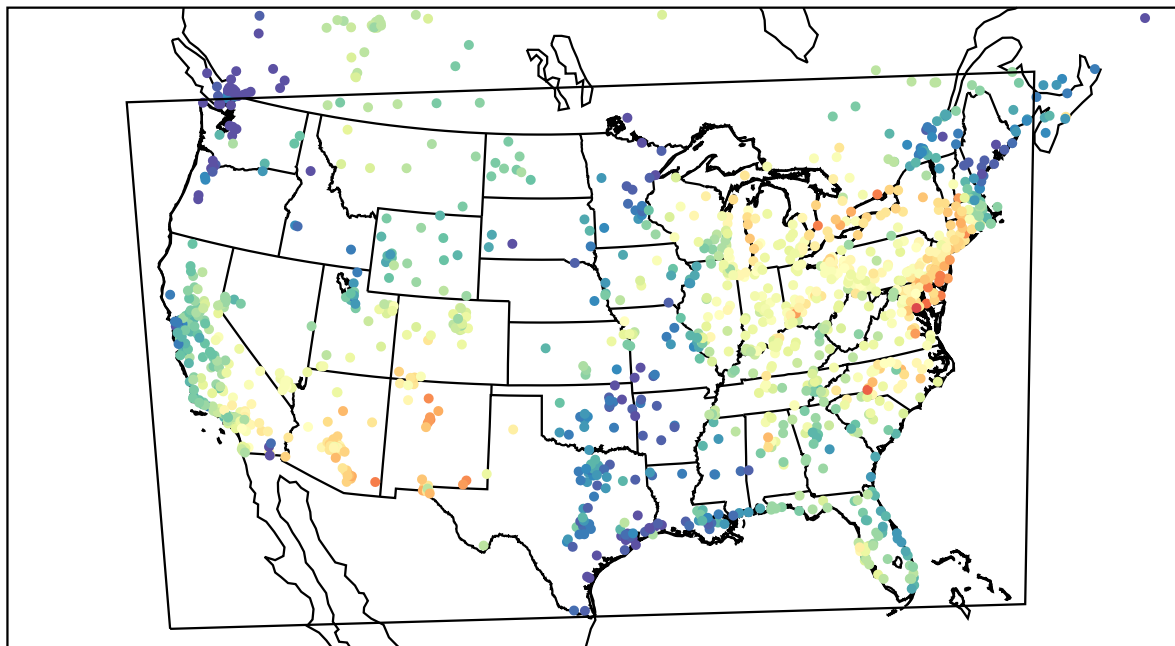
AirNOW (2022-05-31_17:00:00)
