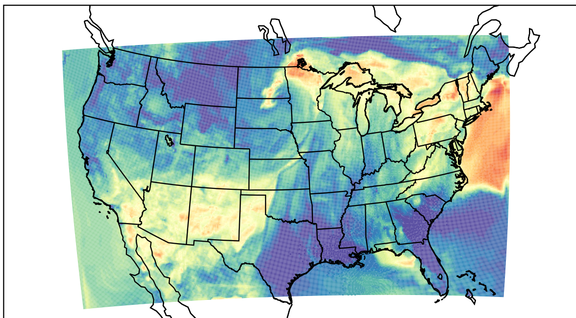
WRF (2022-05-31_05:00:00)
