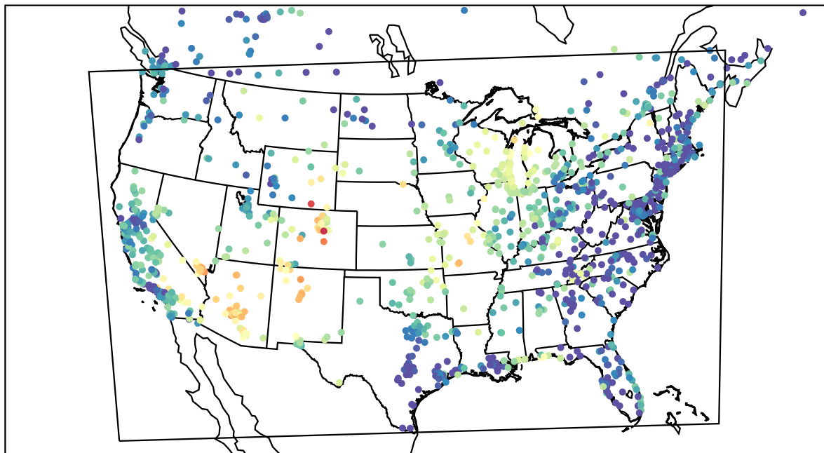
AirNOW (2022-05-30_06:00:00)
