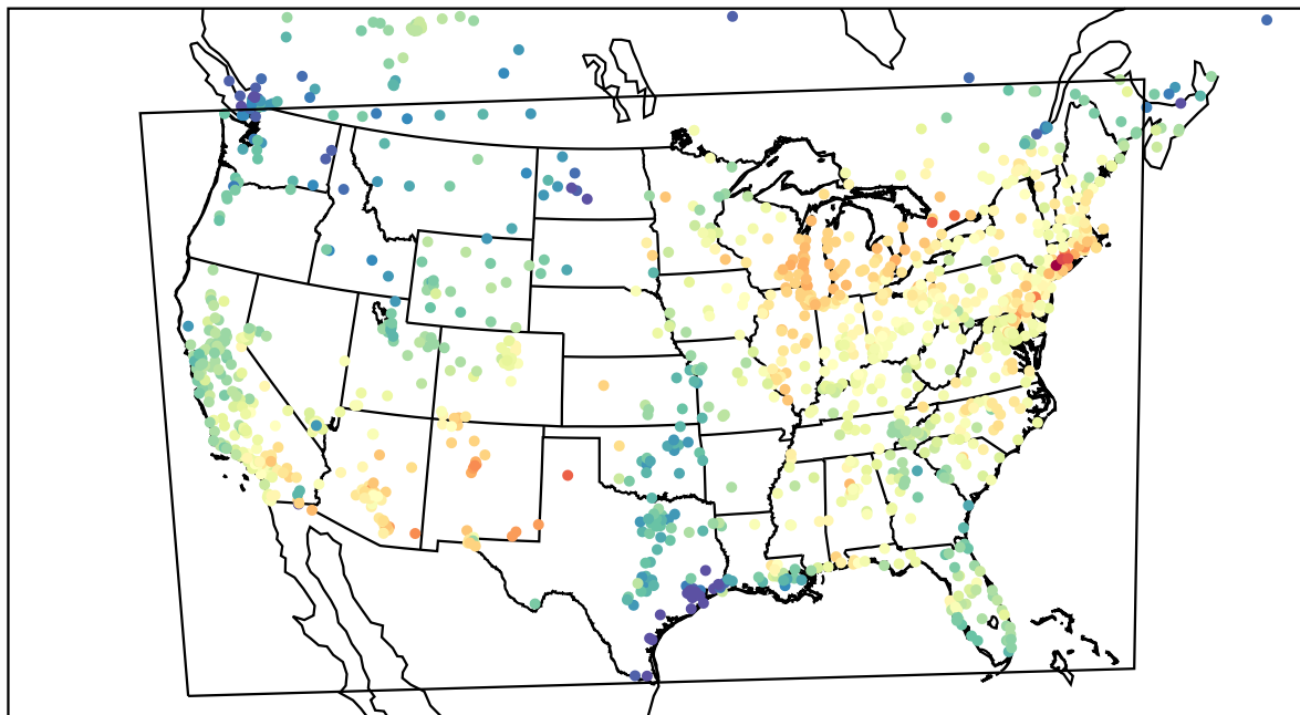
AirNOW (2022-05-30_19:00:00)
