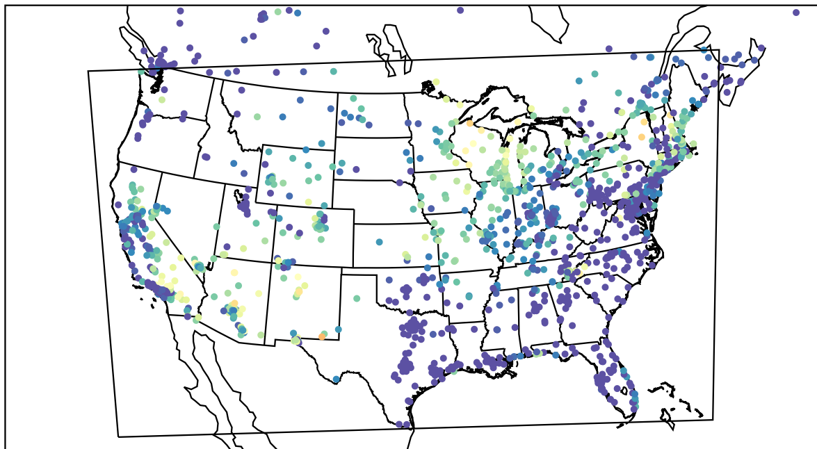
AirNOW (2022-05-31_10:00:00)
