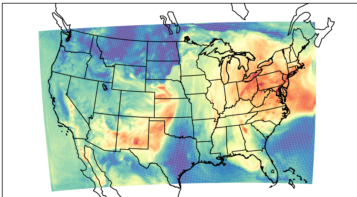
WRF (2022-05-30_16:00:00)
