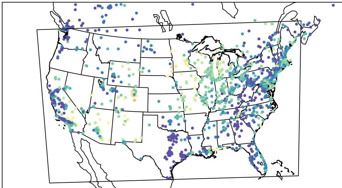
AirNOW (2022-05-30_12:00:00)
