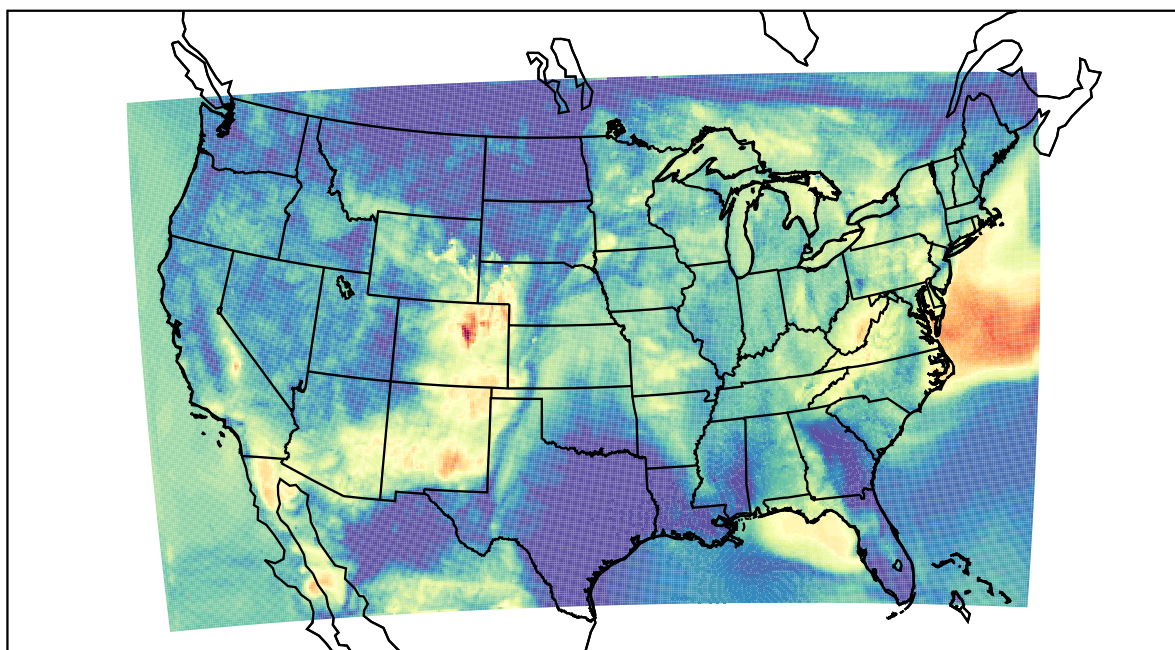
WRF (2022-05-30_09:00:00)
