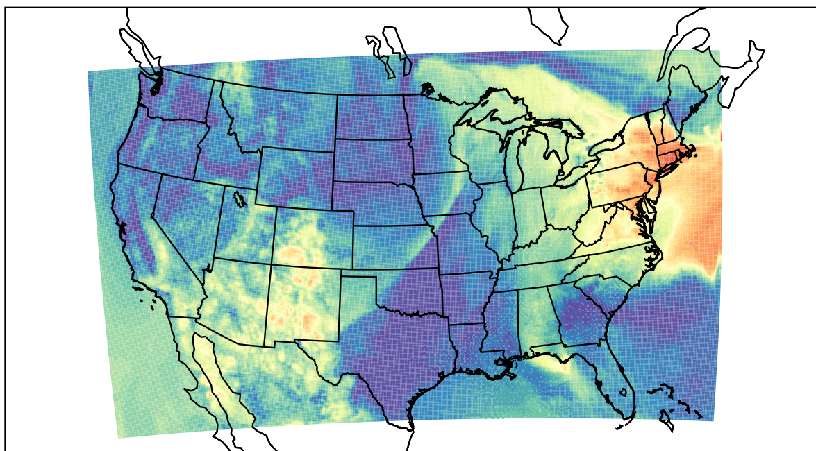
WRF (2022-05-31_14:00:00)
