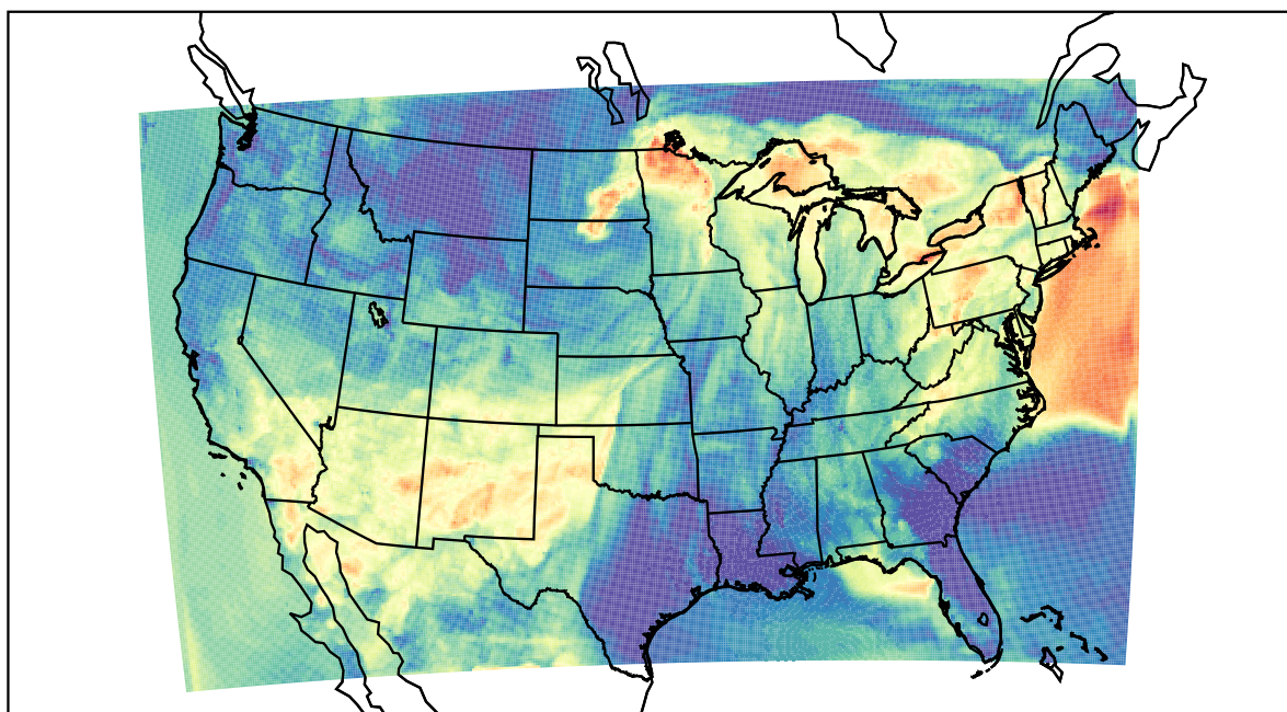
WRF (2022-05-31_04:00:00)
