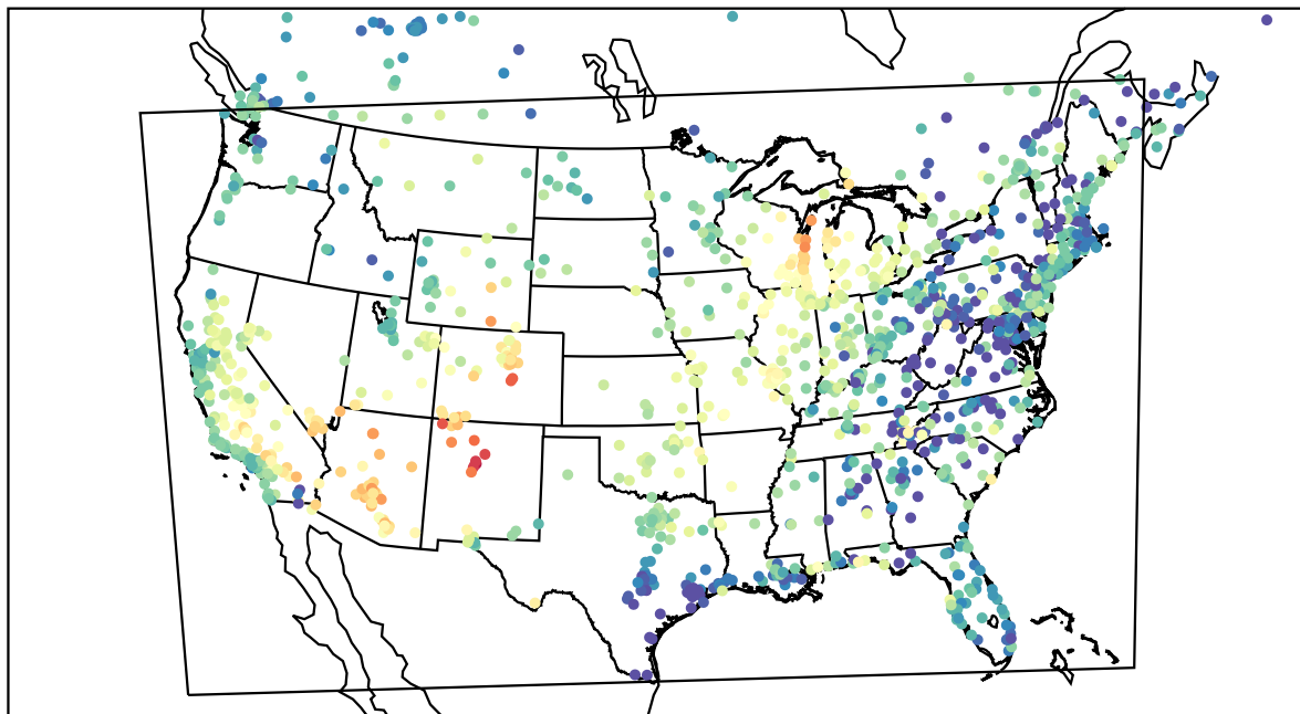
AirNOW (2022-05-30_02:00:00)
