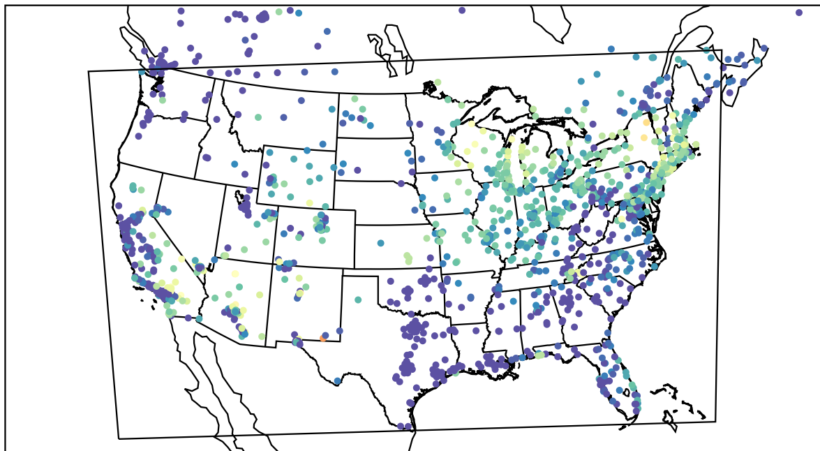
AirNOW (2022-05-31_12:00:00)
