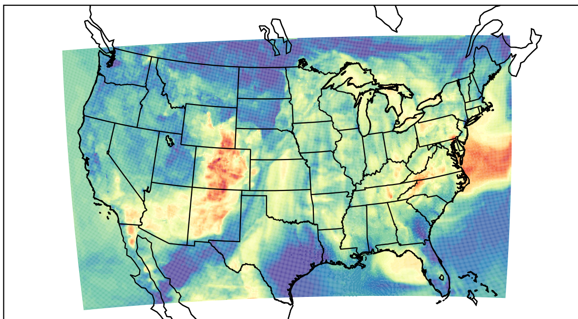
WRF (2022-05-30_04:00:00)
