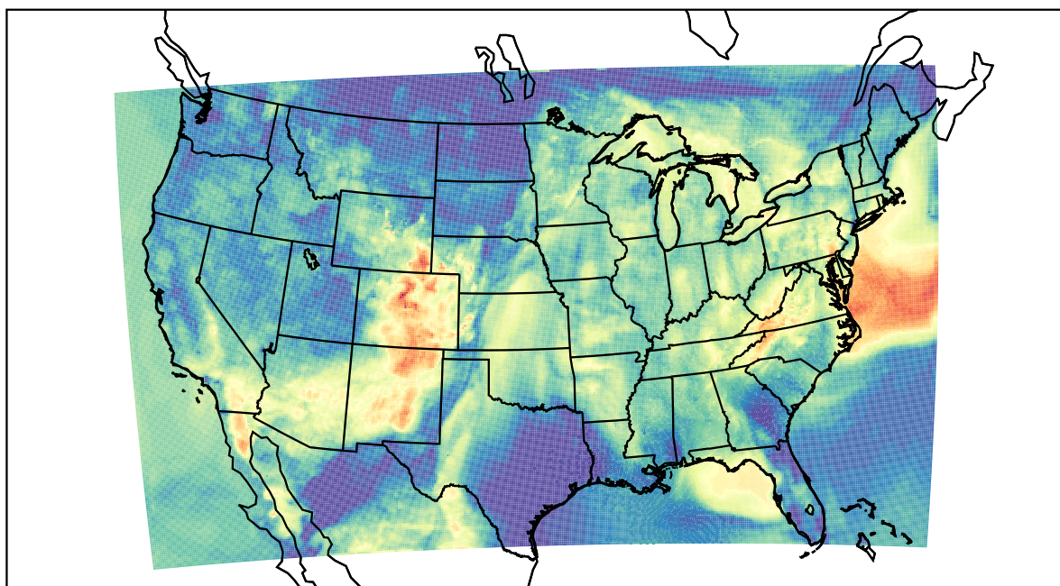
WRF (2022-05-30_06:00:00)
