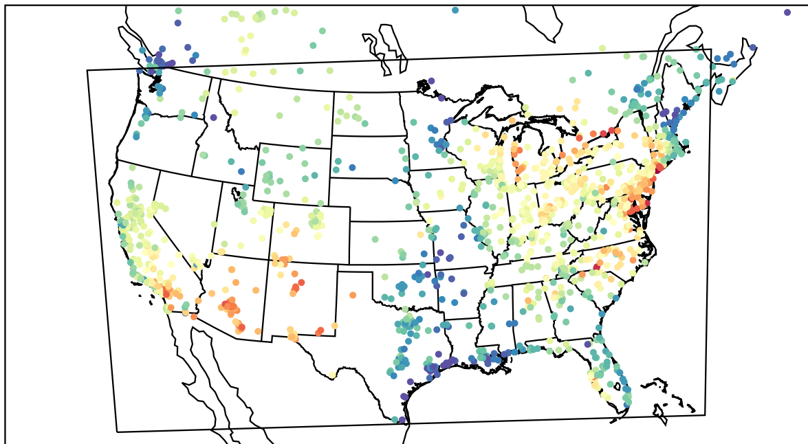
AirNOW (2022-05-31_20:00:00)
