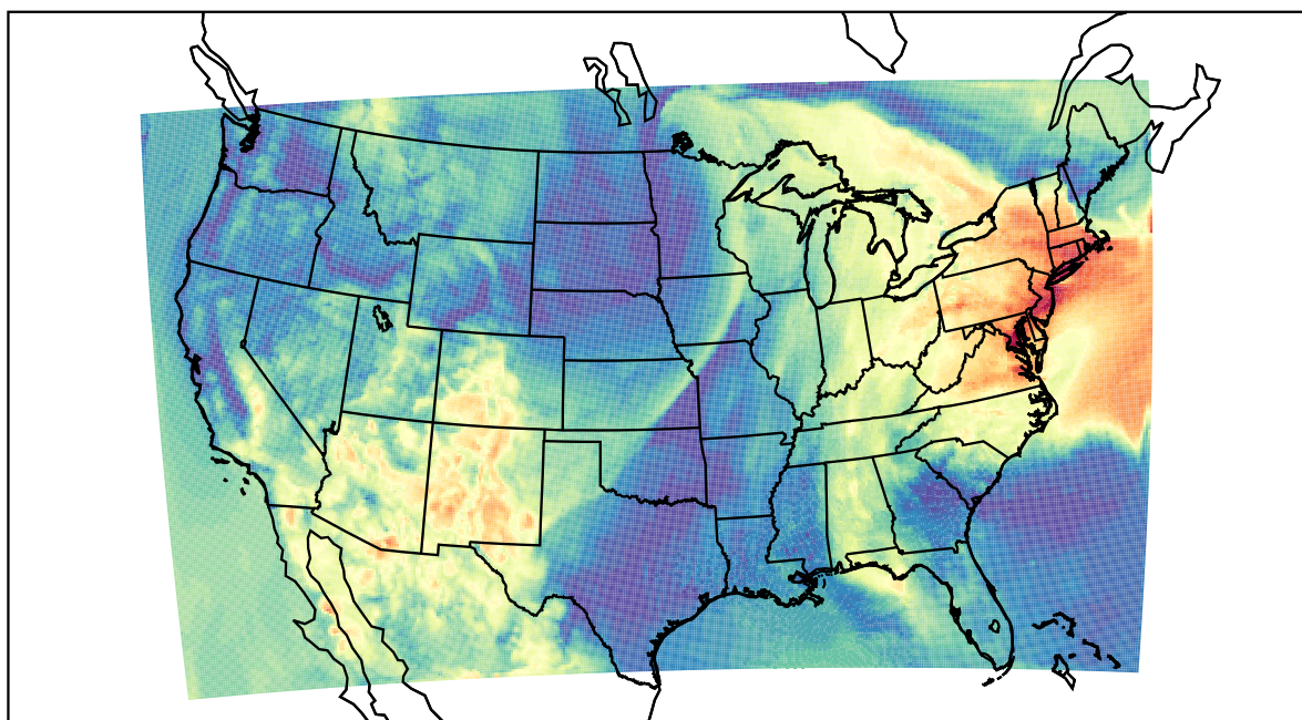
WRF (2022-05-31_15:00:00)
