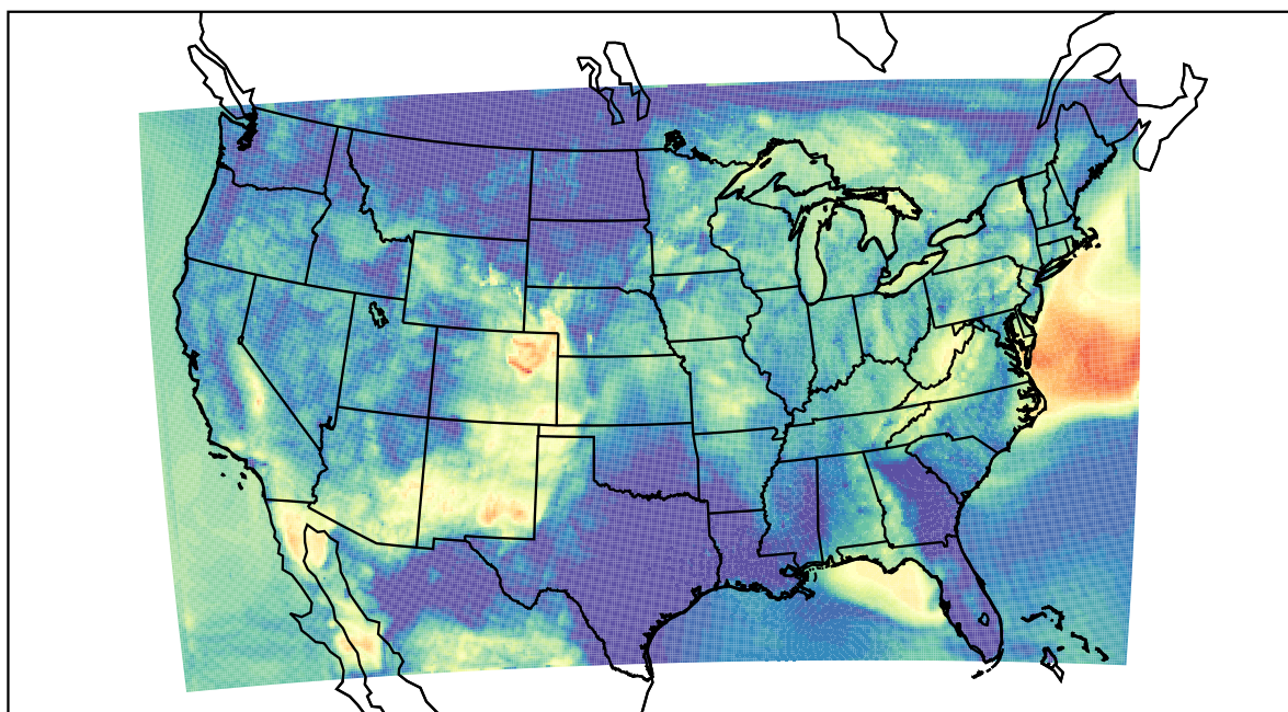
WRF (2022-05-30_11:00:00)
