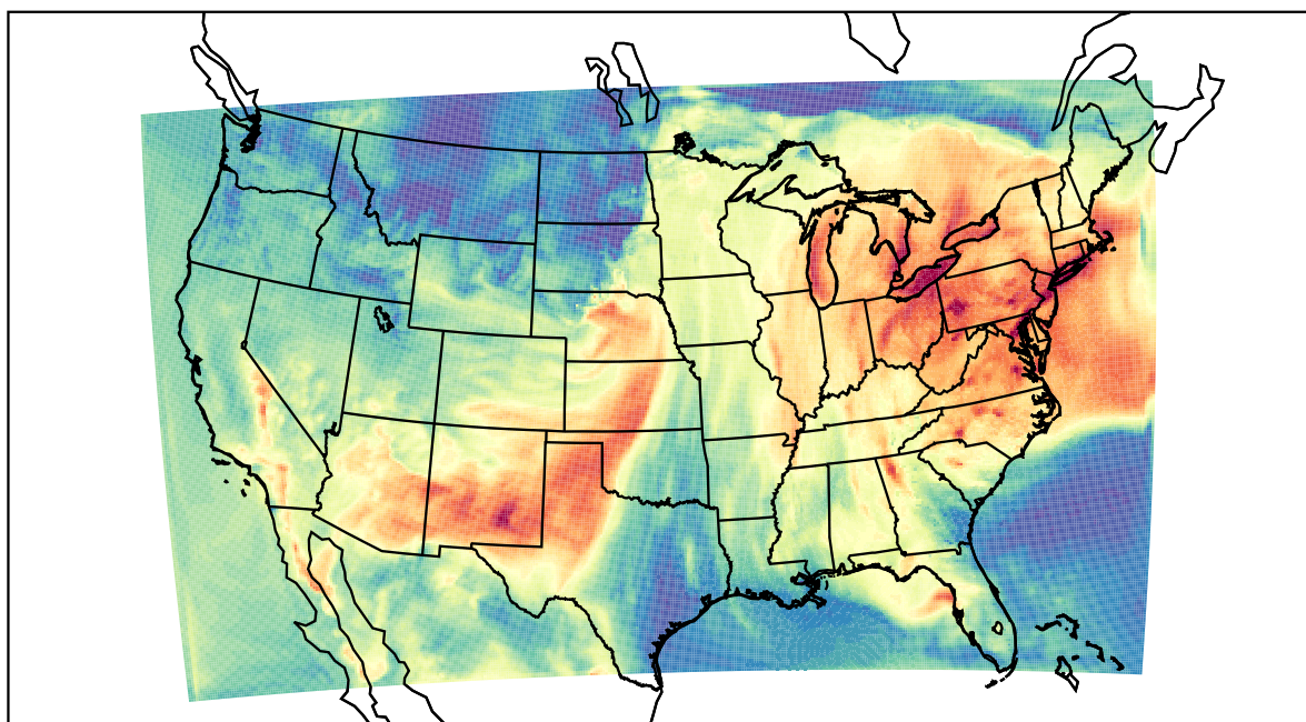
WRF (2022-05-30_18:00:00)
