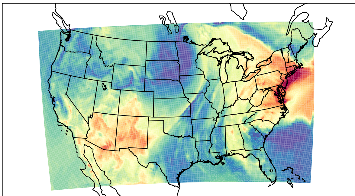
WRF (2022-05-31_17:00:00)
