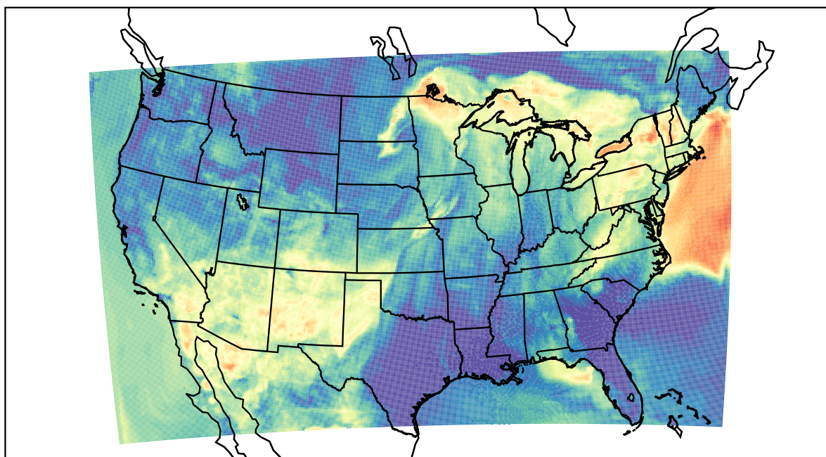
WRF (2022-05-31_06:00:00)
