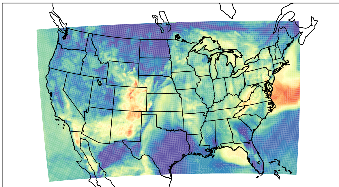
WRF (2022-05-30_07:00:00)
