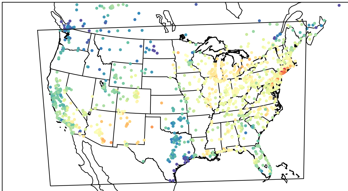
AirNOW (2022-05-30_17:00:00)
