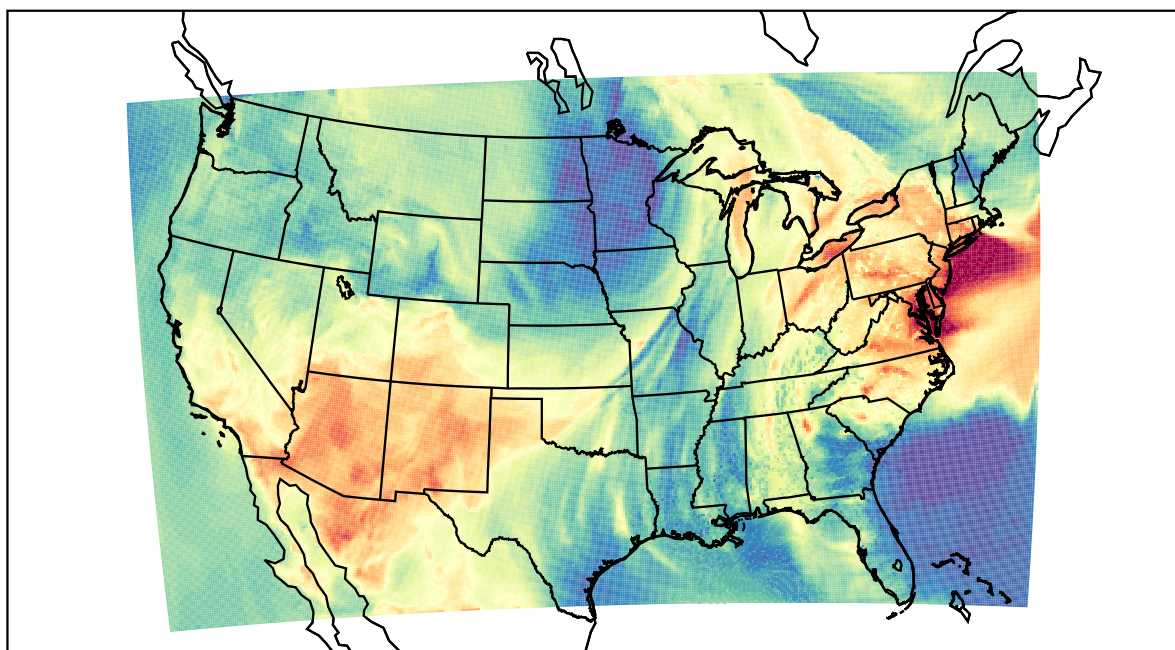
WRF (2022-05-31_21:00:00)
