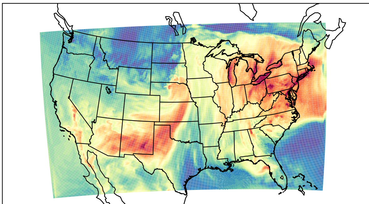
WRF (2022-05-30_19:00:00)
