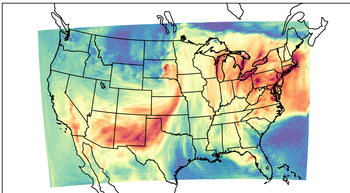
WRF (2022-05-30_21:00:00)
