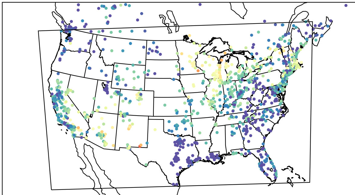
AirNOW (2022-05-31_06:00:00)
