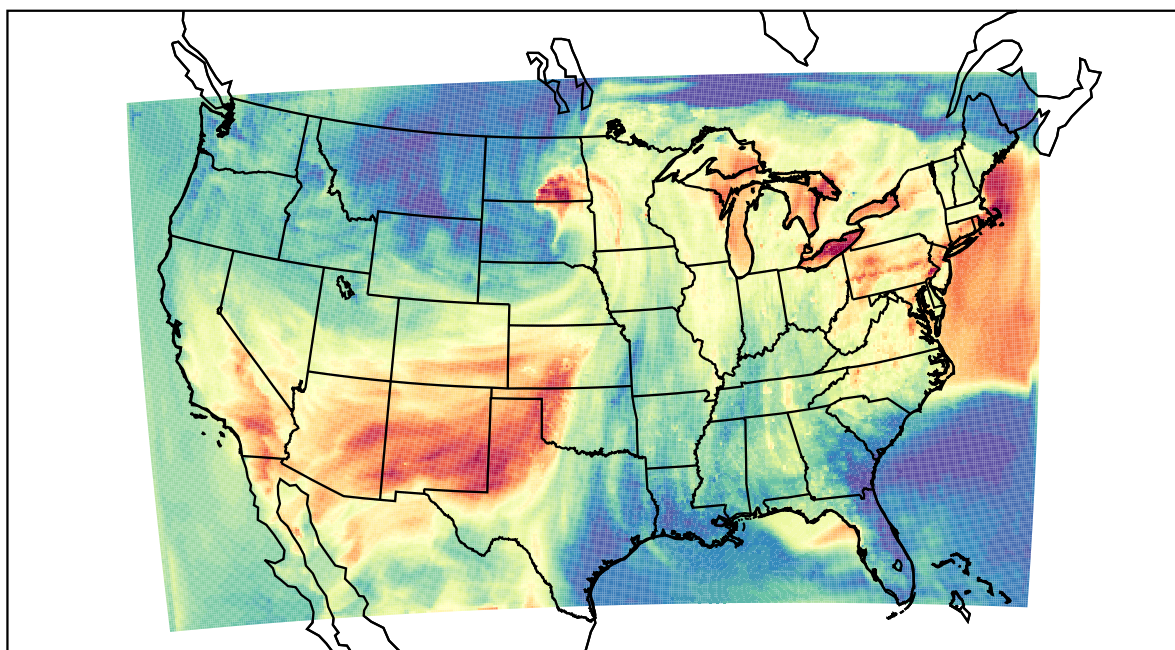
WRF (2022-05-31_00:00:00)
