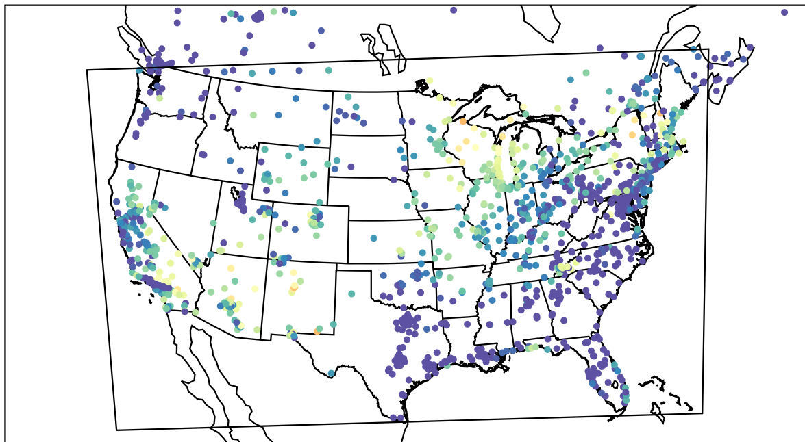
AirNOW (2022-05-31_09:00:00)
