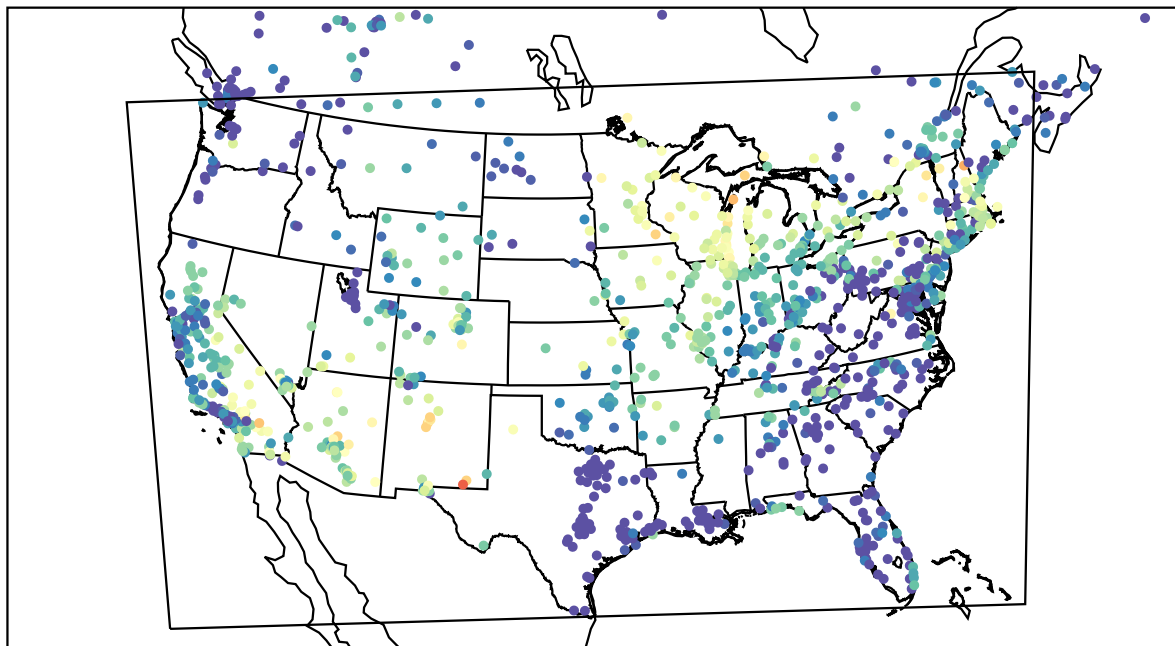
AirNOW (2022-05-31_07:00:00)
