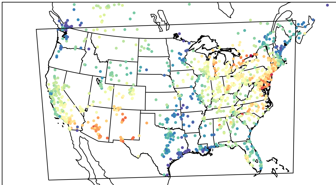
AirNOW (2022-05-31_19:00:00)
