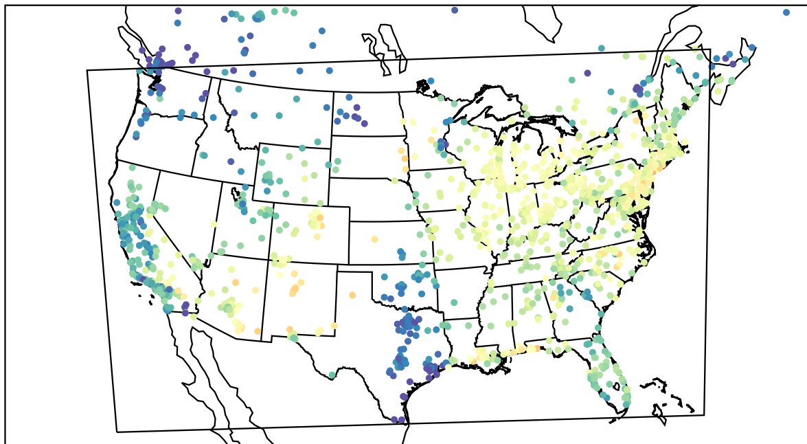
AirNOW (2022-05-30_15:00:00)
