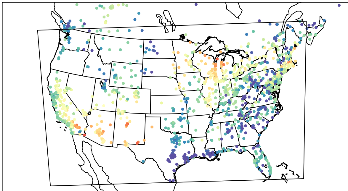
AirNOW (2022-05-31_02:00:00)
