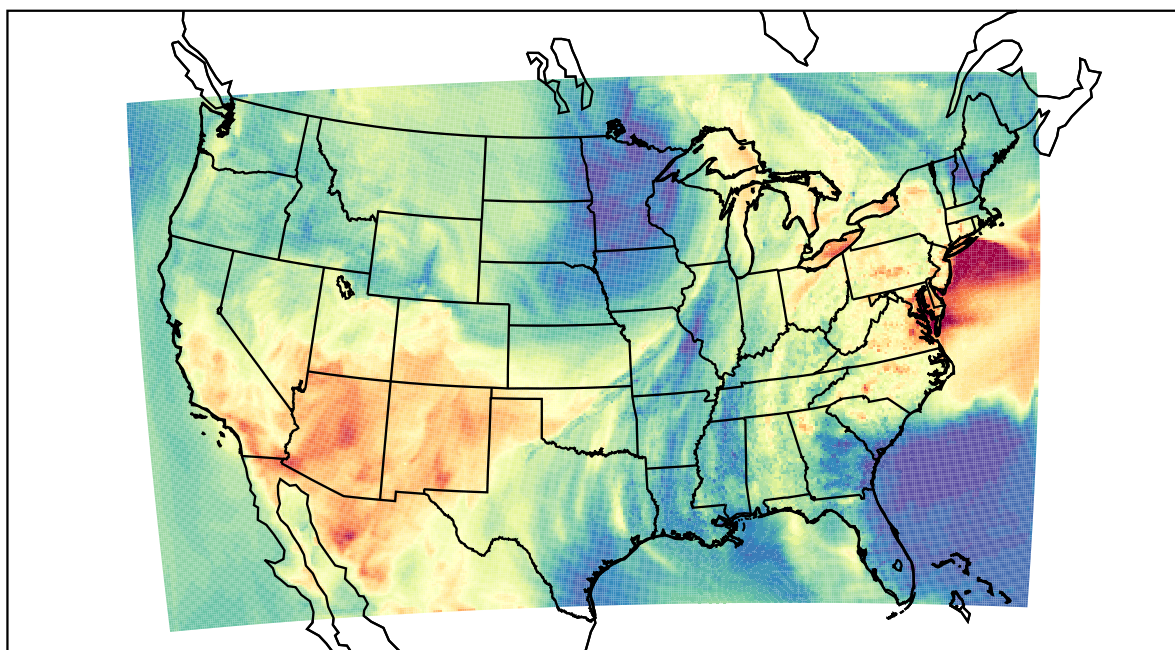
WRF (2022-05-31_23:00:00)
