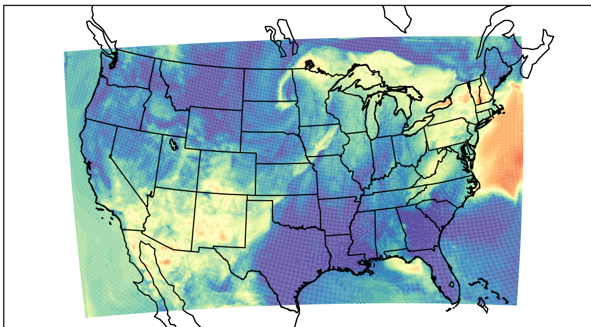
WRF (2022-05-31_08:00:00)
