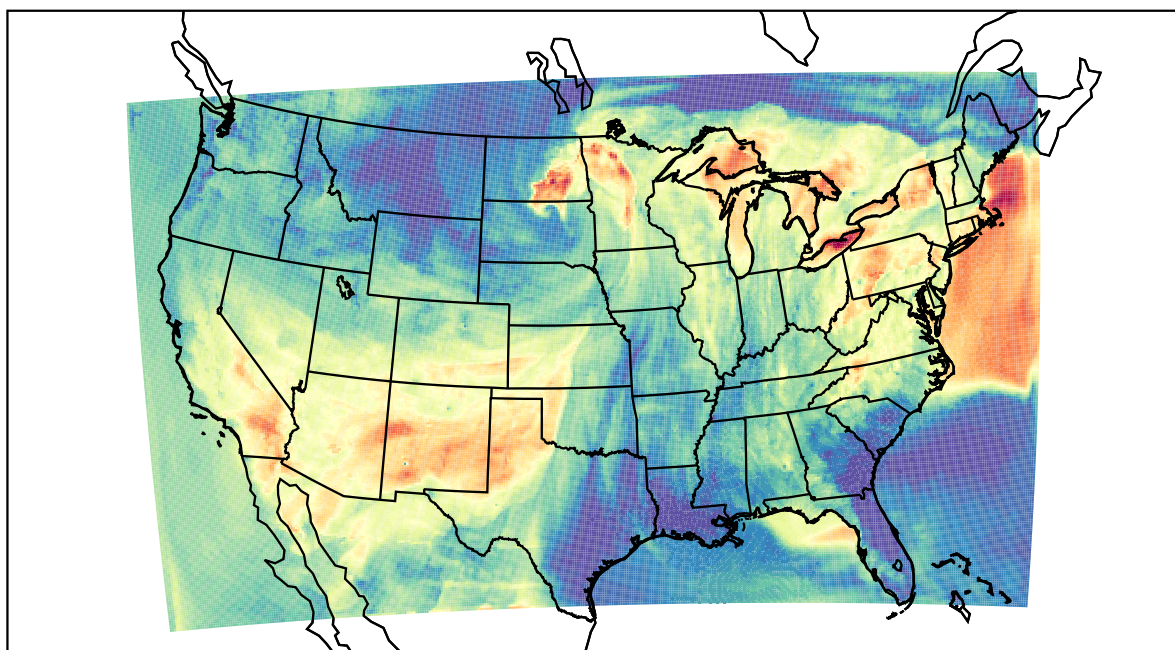
WRF (2022-05-31_02:00:00)
