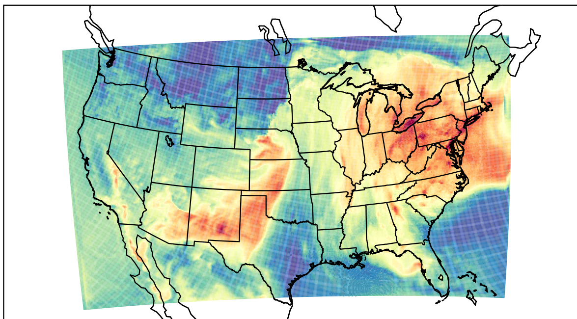
WRF (2022-05-30_17:00:00)
