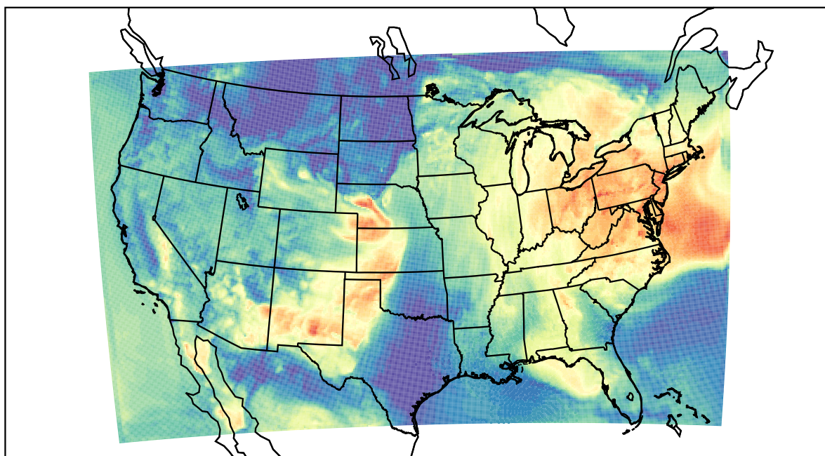
WRF (2022-05-30_15:00:00)
