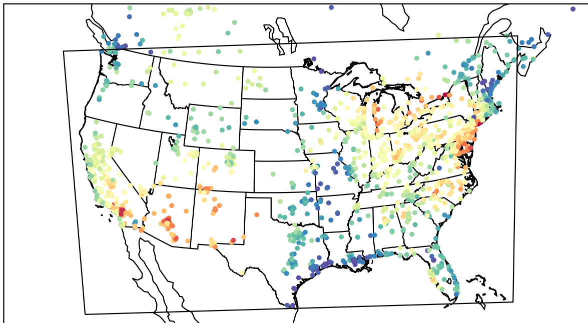
AirNOW (2022-05-31_21:00:00)
