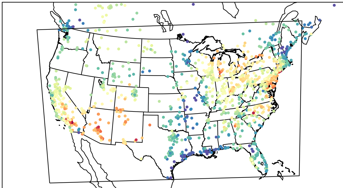
AirNOW (2022-05-31_22:00:00)
