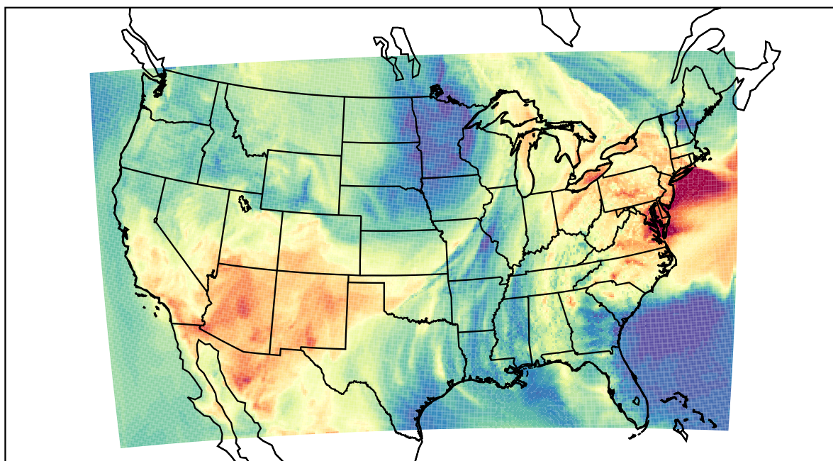
WRF (2022-05-31_22:00:00)
