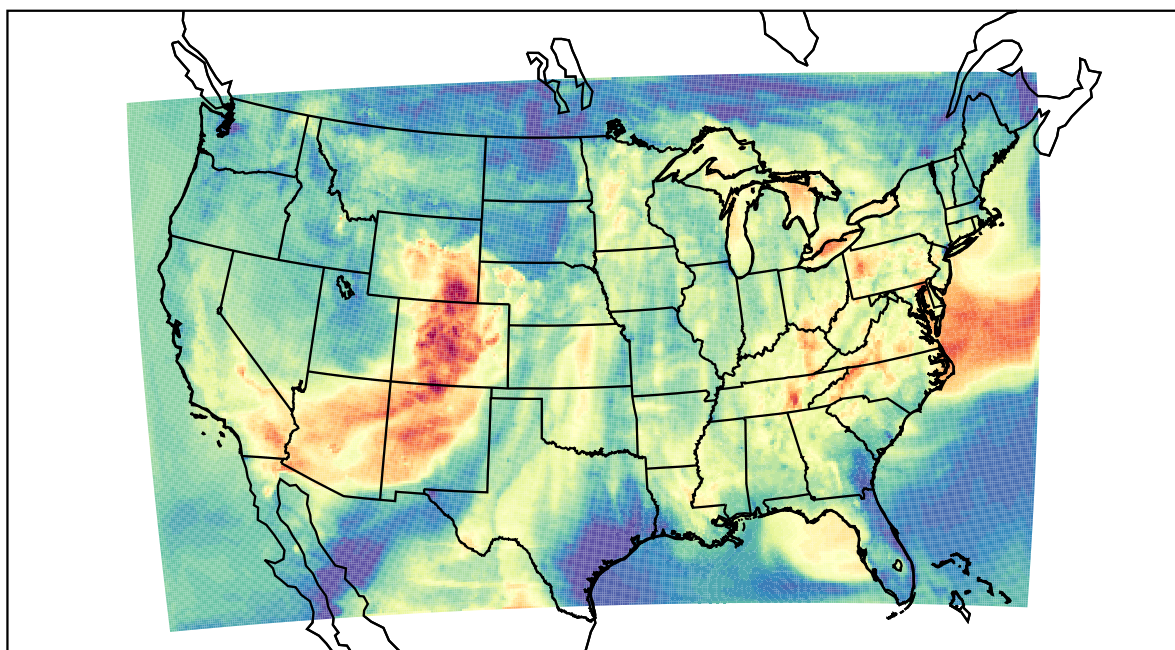
WRF (2022-05-30_02:00:00)
