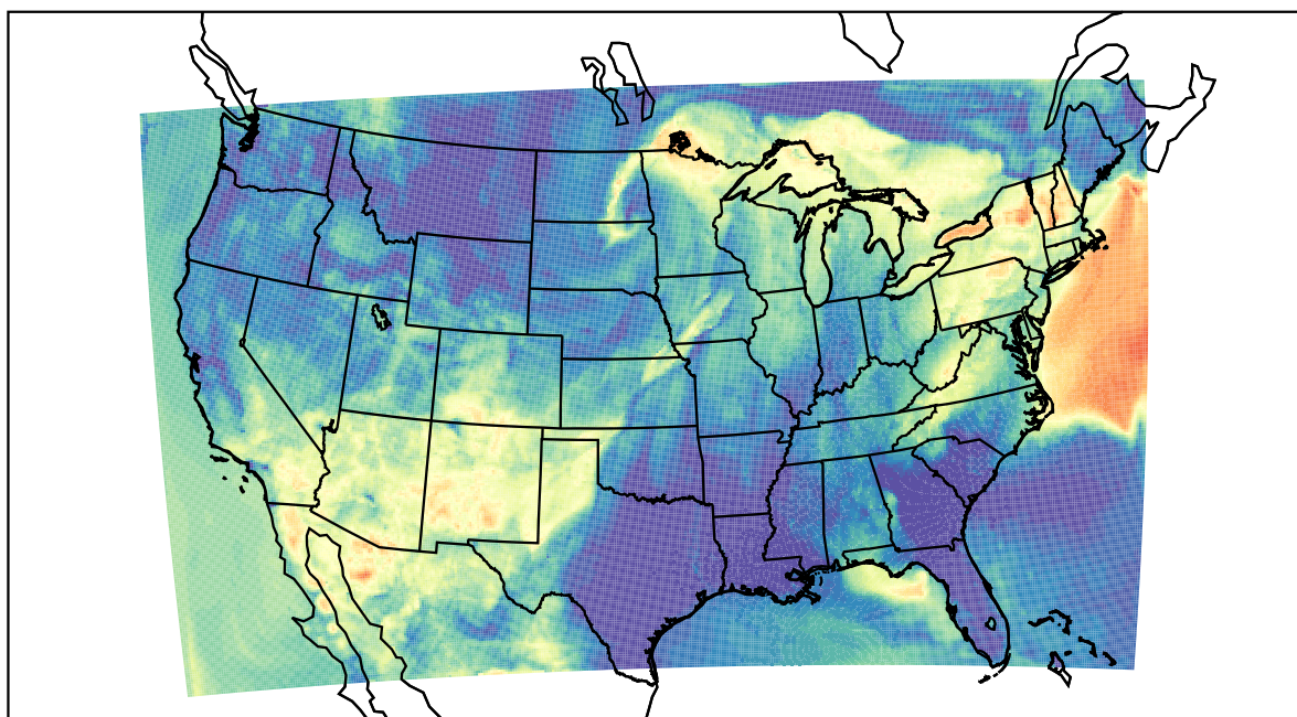
WRF (2022-05-31_07:00:00)
