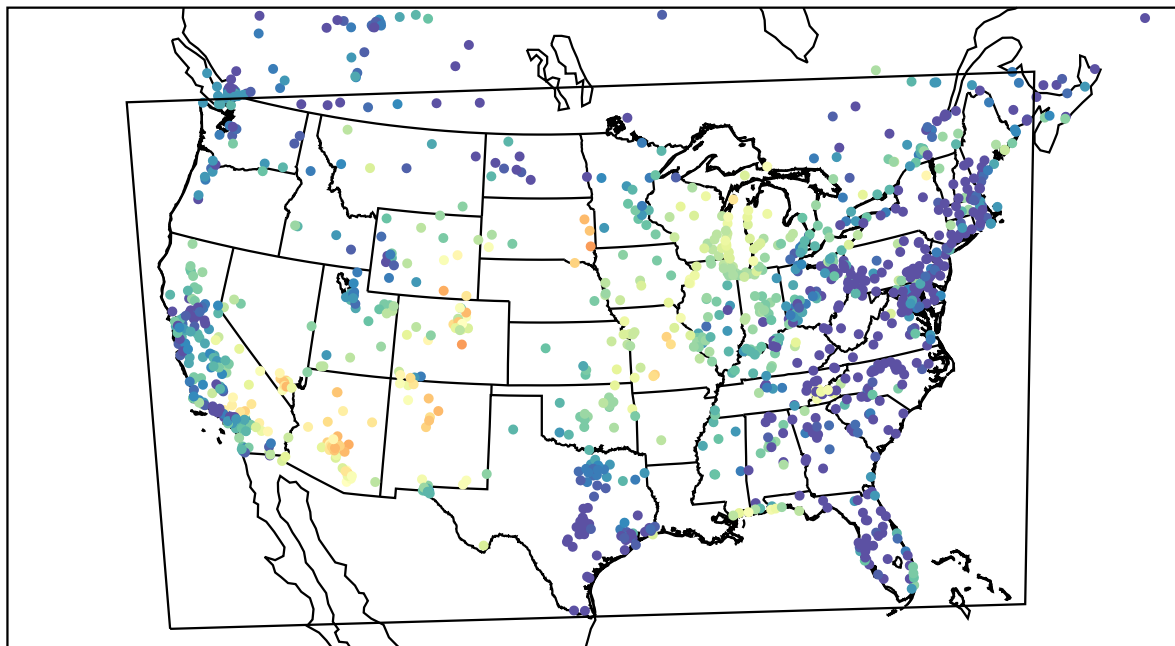
AirNOW (2022-05-30_07:00:00)
