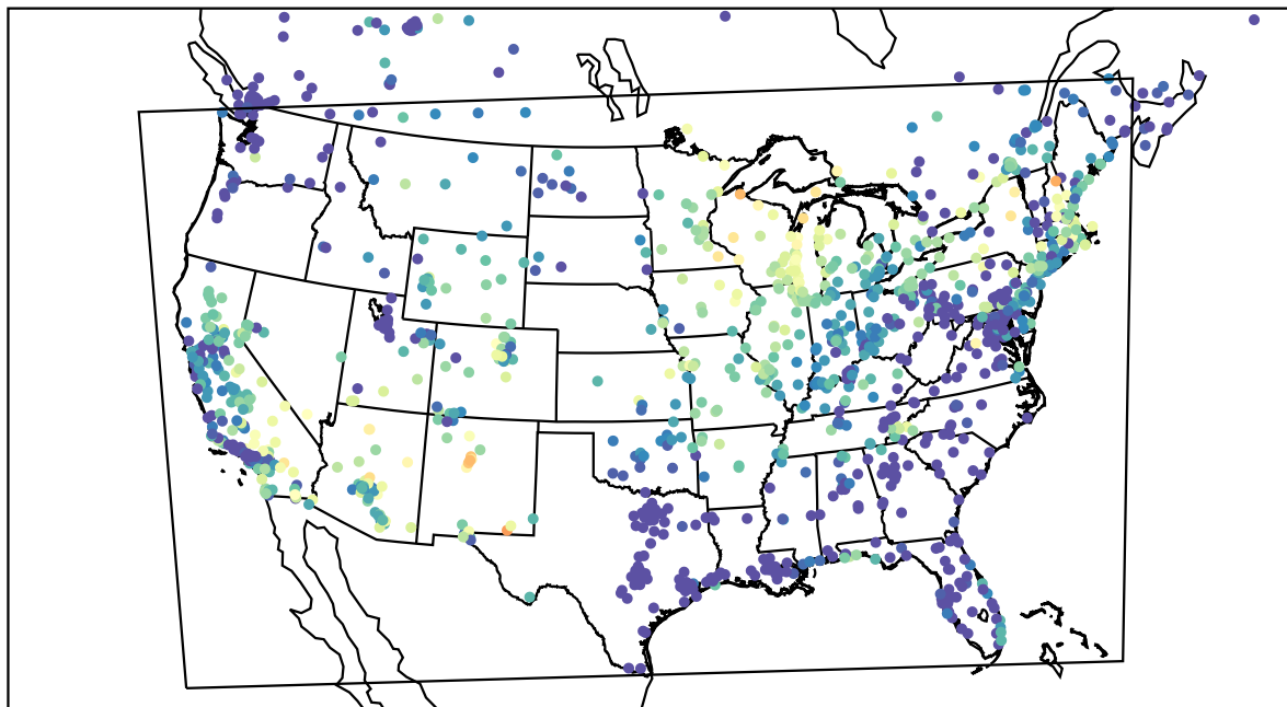
AirNOW (2022-05-31_08:00:00)
