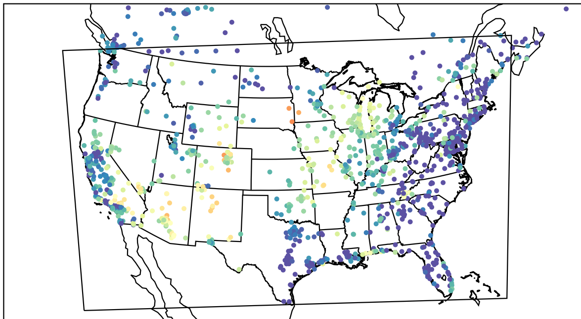
AirNOW (2022-05-30_08:00:00)
