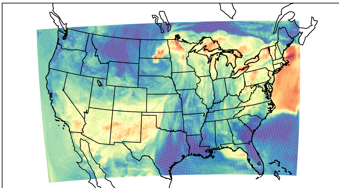
WRF (2022-05-31_03:00:00)
