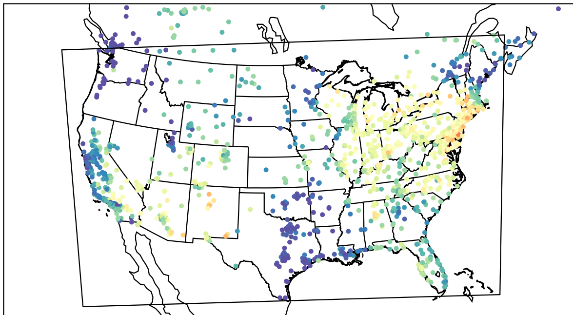
AirNOW (2022-05-31_15:00:00)
