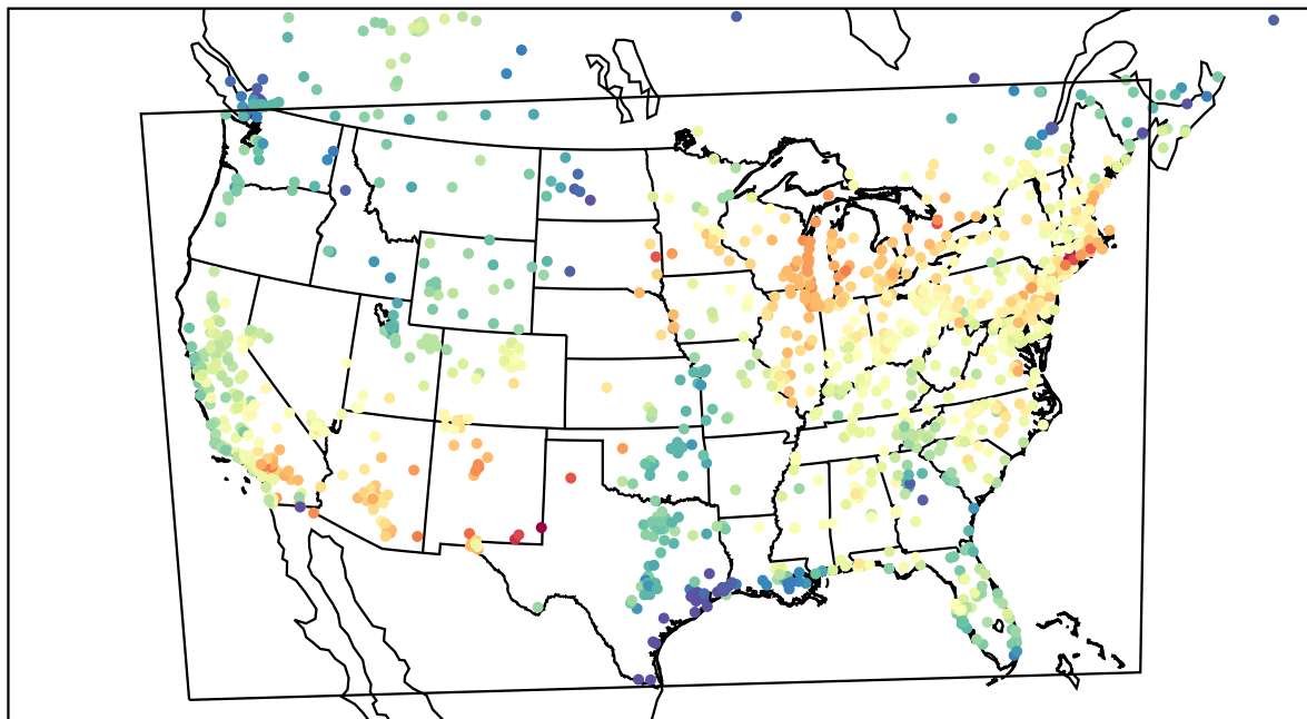
AirNOW (2022-05-30_21:00:00)
