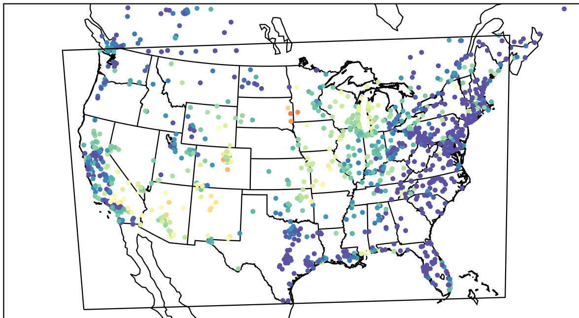
AirNOW (2022-05-30_09:00:00)
