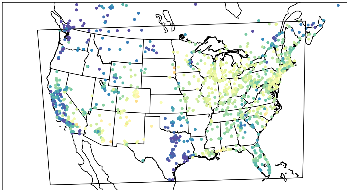
AirNOW (2022-05-30_14:00:00)
