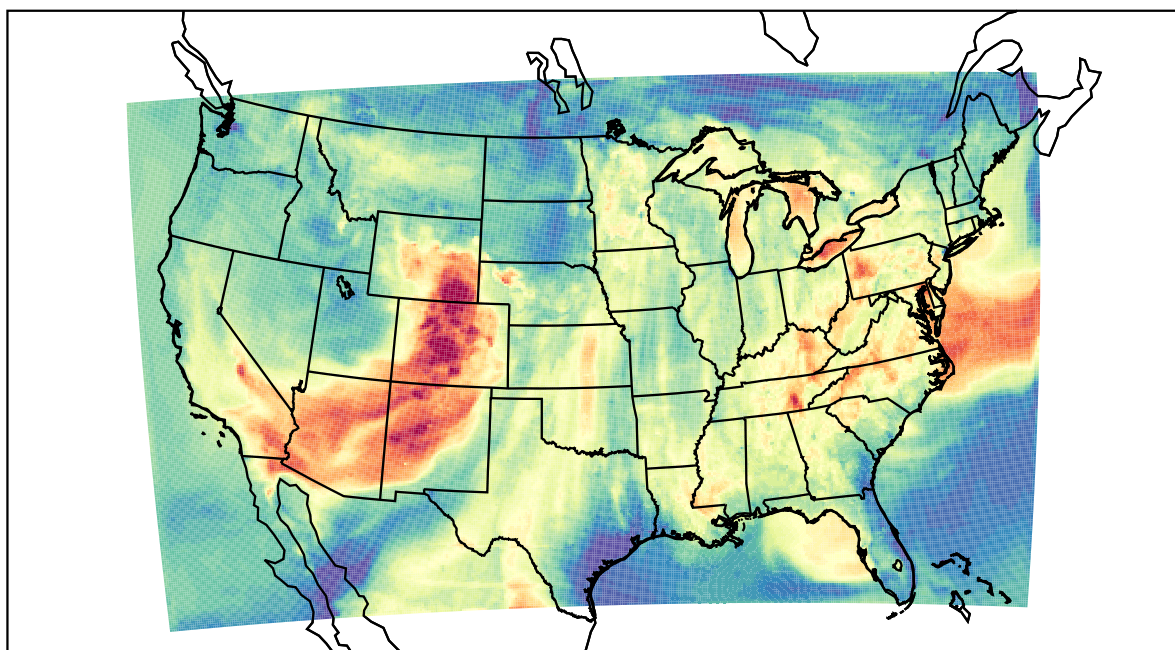
WRF (2022-05-30_01:00:00)
