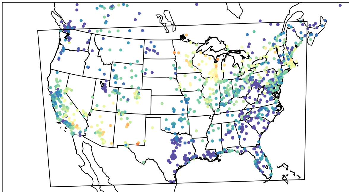
AirNOW (2022-05-31_05:00:00)
