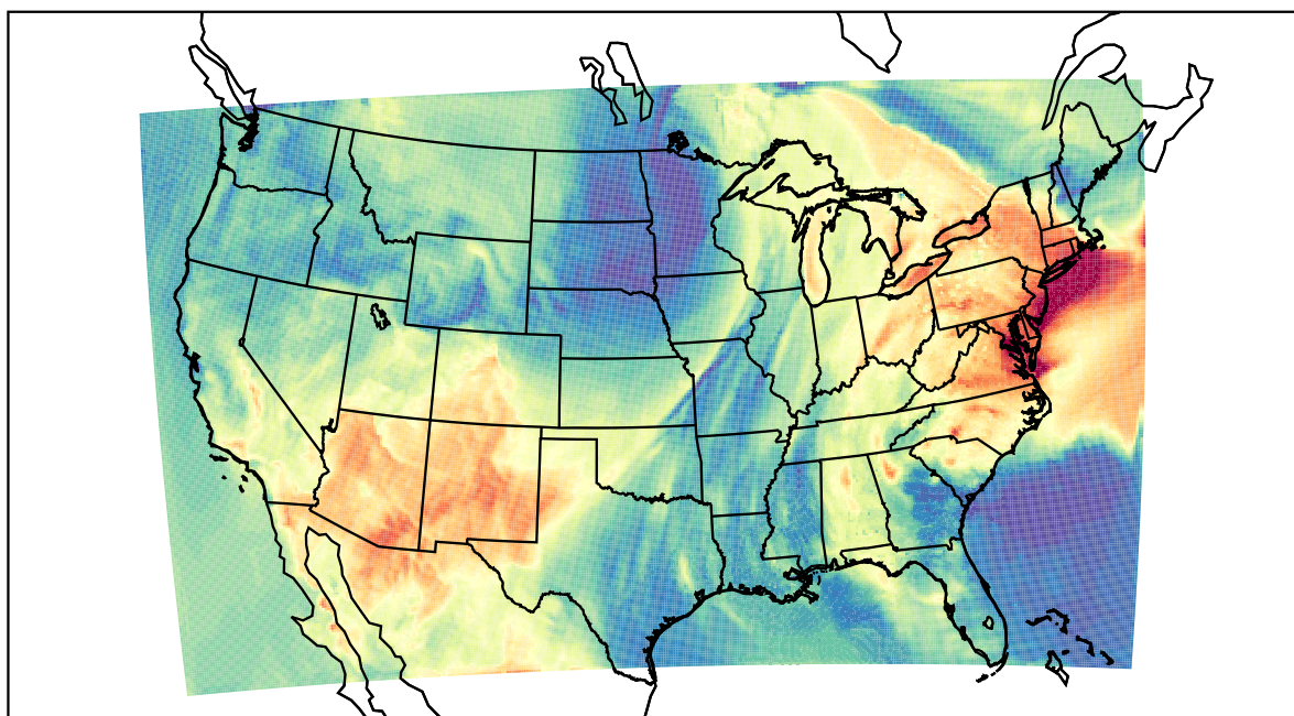
WRF (2022-05-31_18:00:00)
