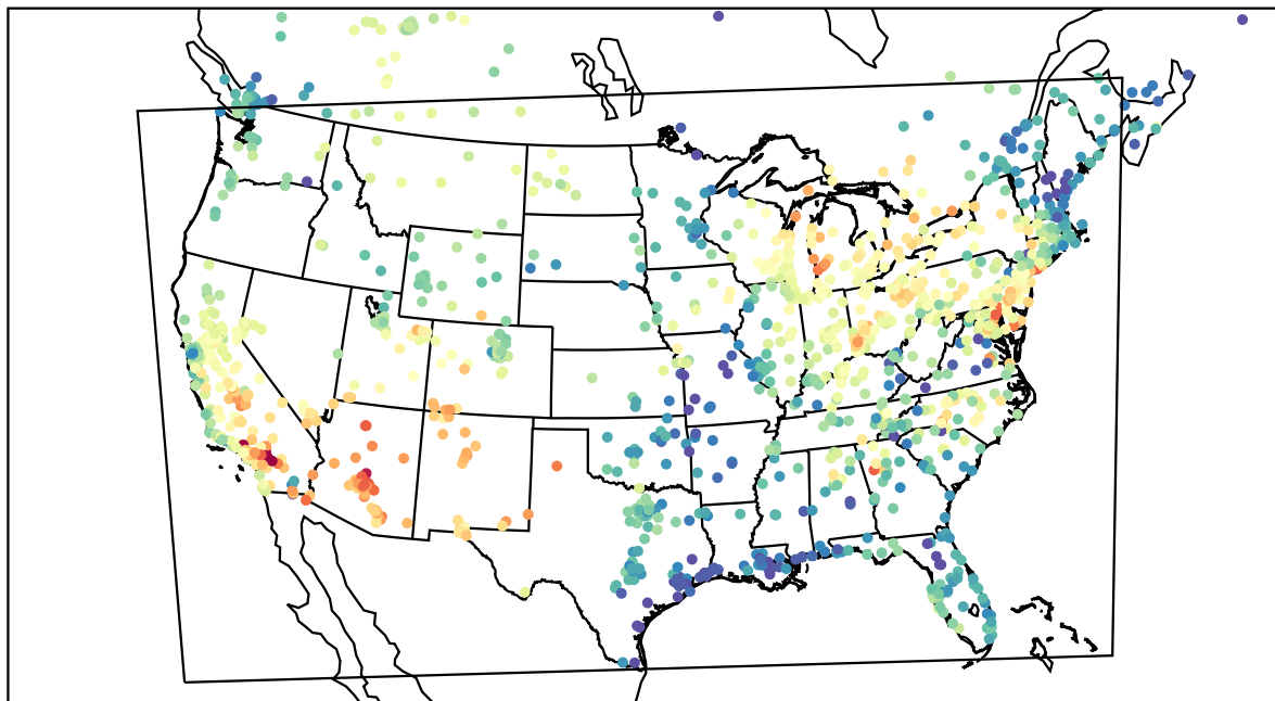
AirNOW (2022-05-31_23:00:00)
