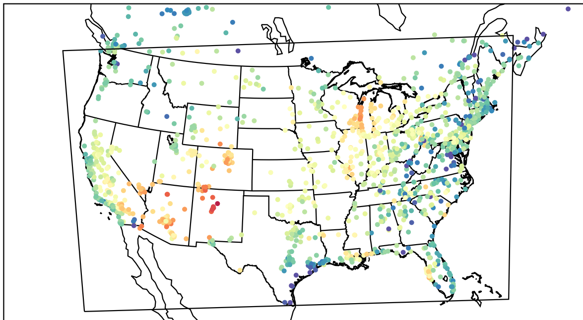
AirNOW (2022-05-30_00:00:00)
