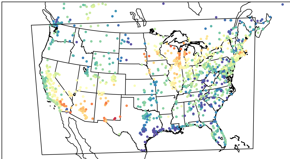
AirNOW (2022-05-31_01:00:00)
