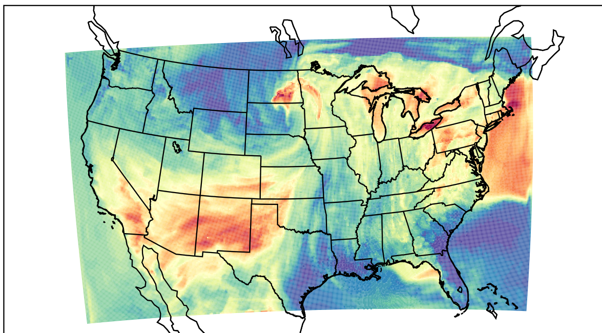
WRF (2022-05-31_01:00:00)
