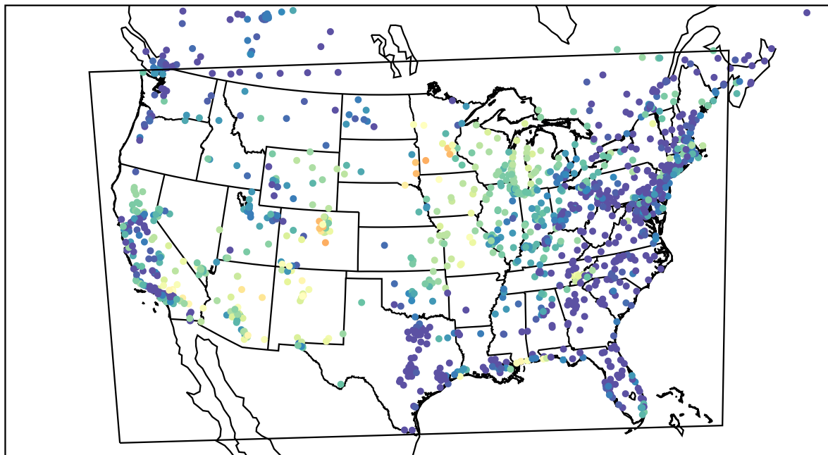
AirNOW (2022-05-30_11:00:00)
