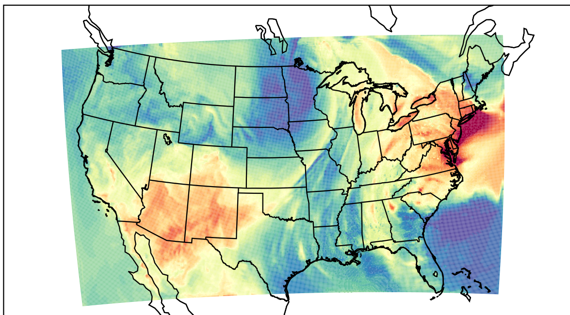
WRF (2022-05-31_19:00:00)
