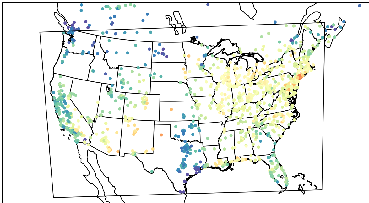
AirNOW (2022-05-30_16:00:00)
