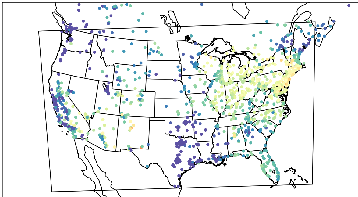
AirNOW (2022-05-31_14:00:00)
