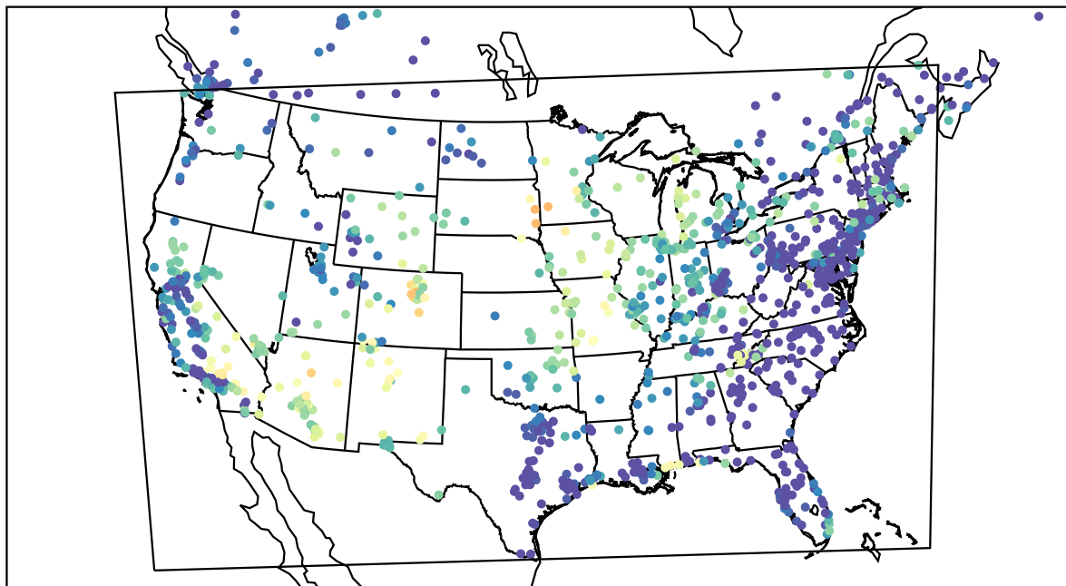
AirNOW (2022-05-30_10:00:00)
