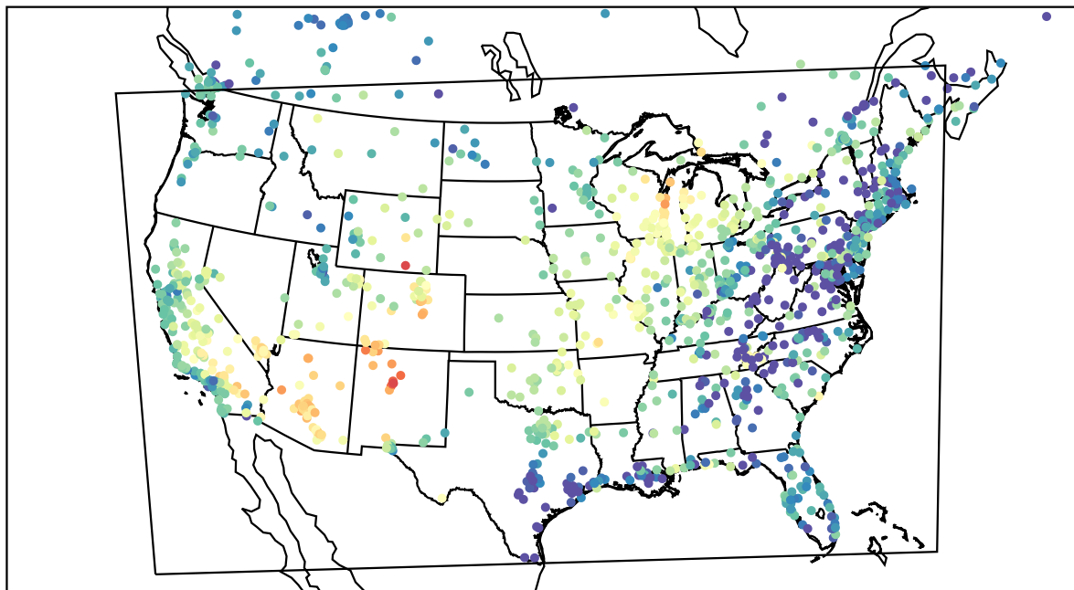
AirNOW (2022-05-30_03:00:00)
