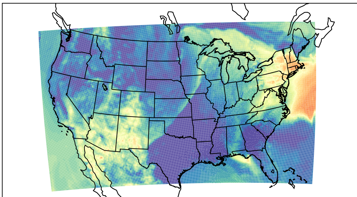
WRF (2022-05-31_13:00:00)
