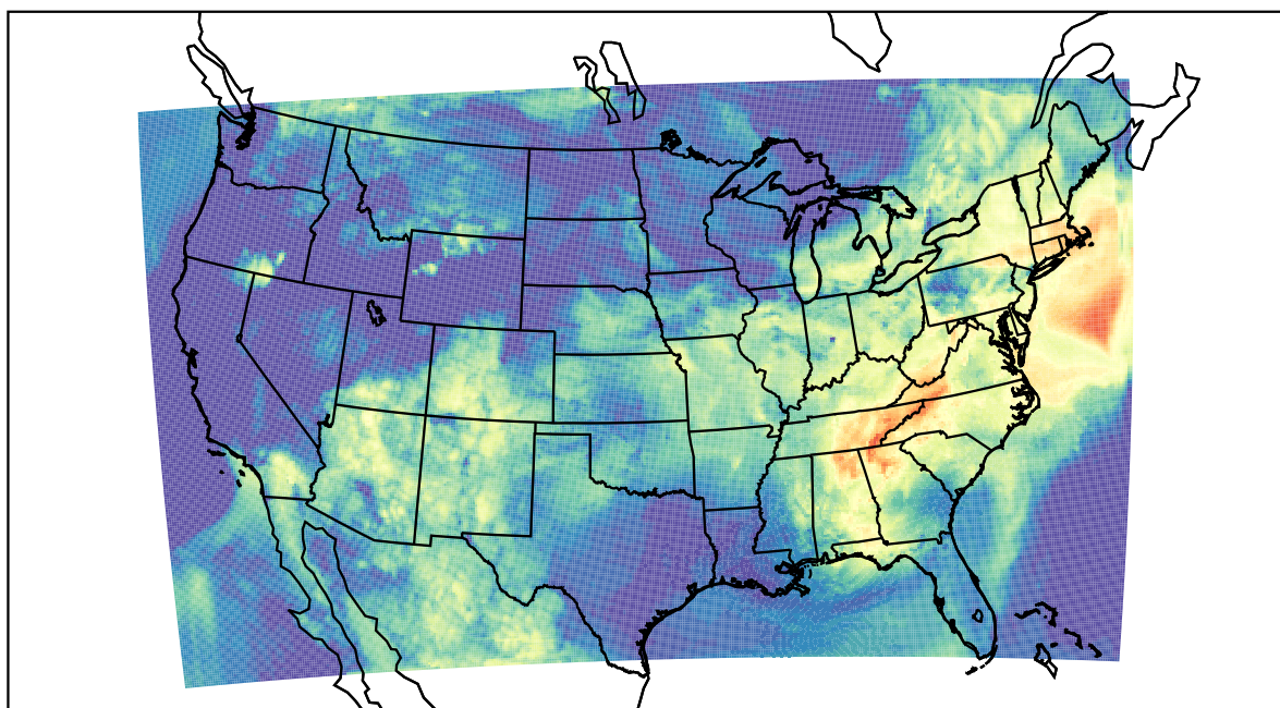
WRF (2022-06-12_14:00:00)
