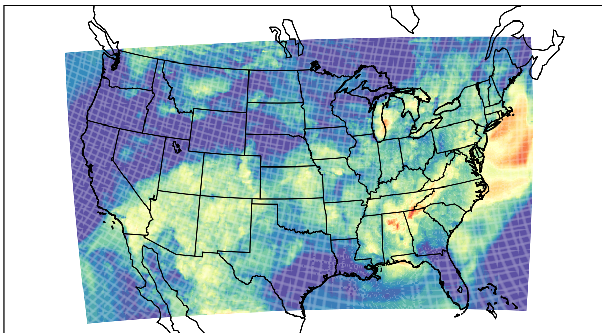
WRF (2022-06-12_06:00:00)
