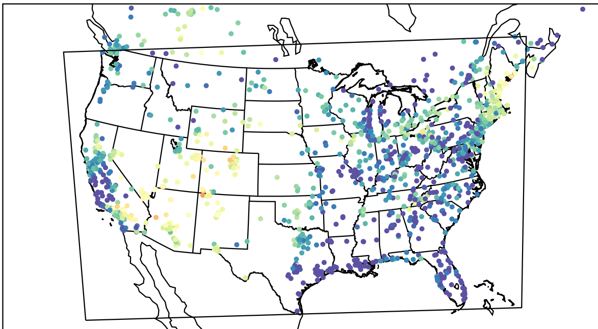
AirNOW (2022-06-13_03:00:00)
