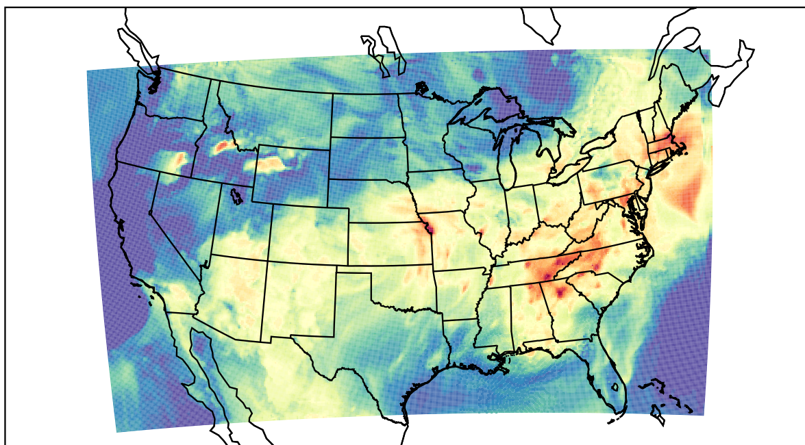
WRF (2022-06-12_16:00:00)
