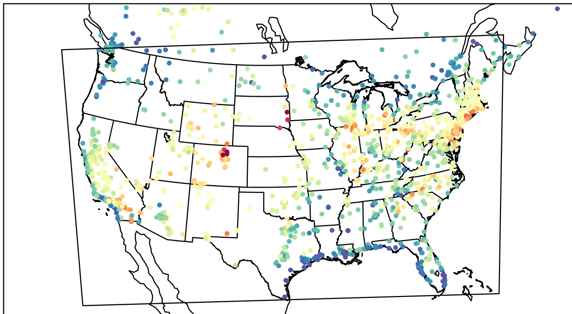
AirNOW (2022-06-13_21:00:00)
