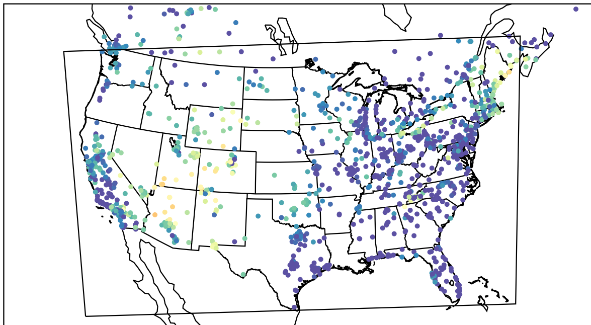
AirNOW (2022-06-13_07:00:00)
