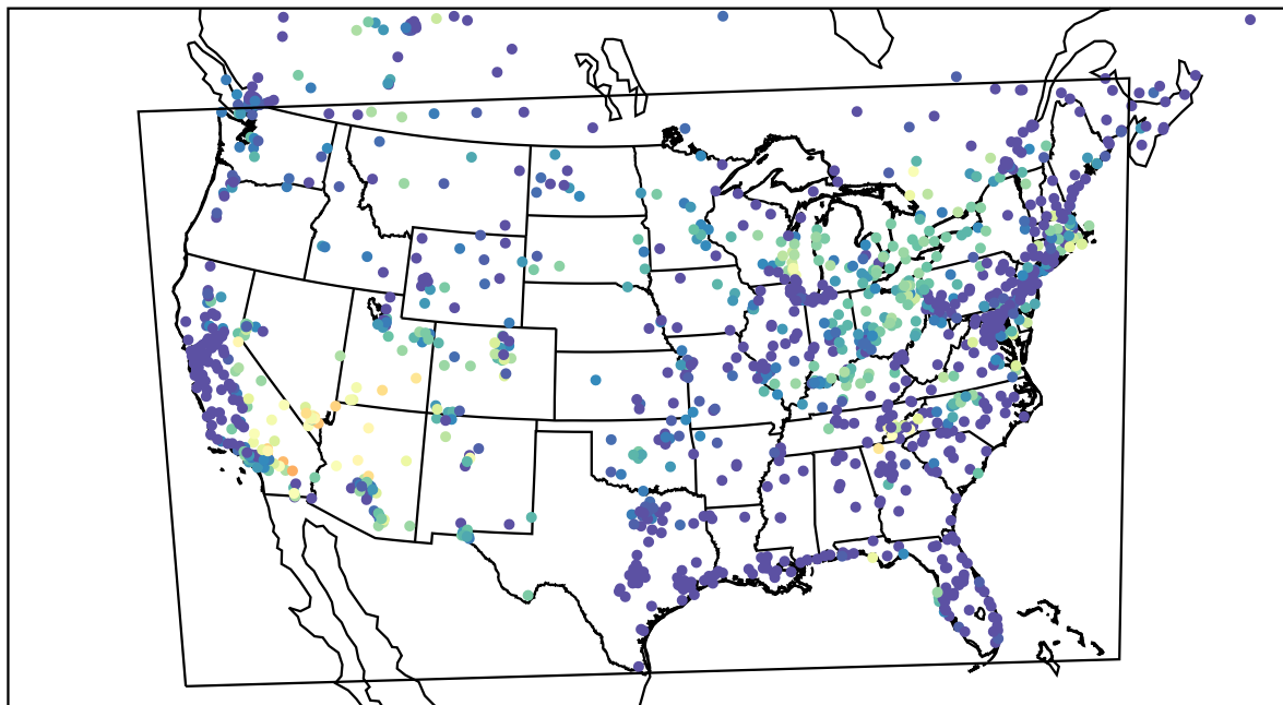
AirNOW (2022-06-12_09:00:00)
