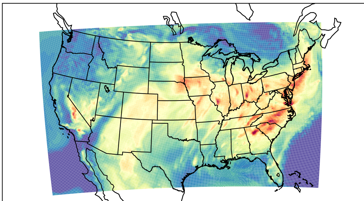
WRF (2022-06-13_17:00:00)
