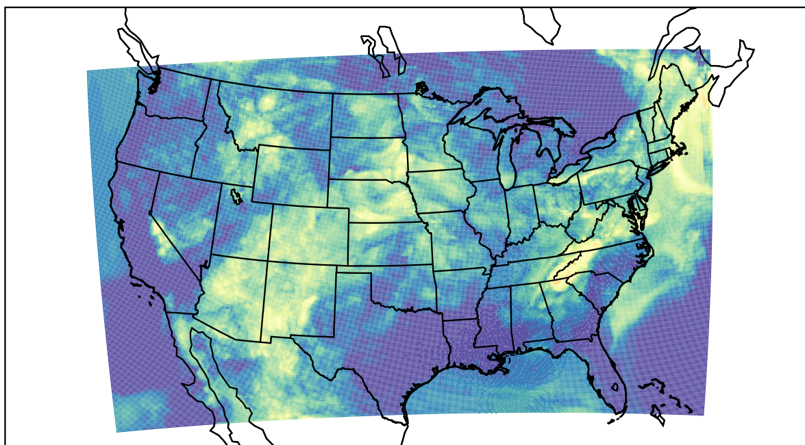
WRF (2022-06-13_08:00:00)
