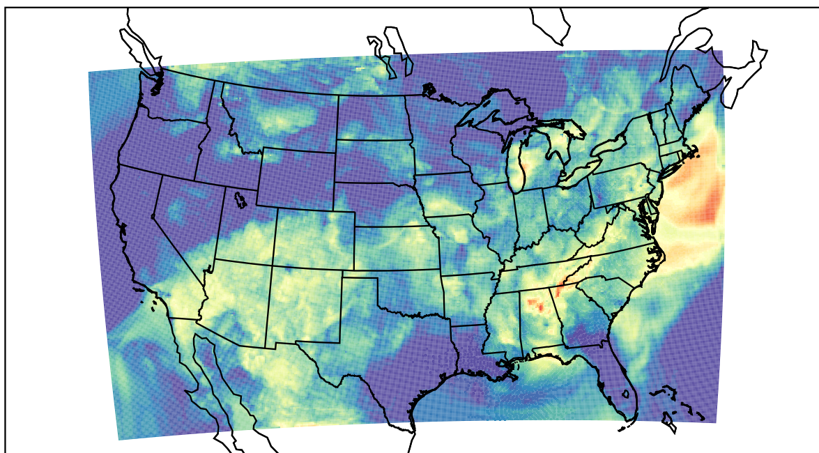
WRF (2022-06-12_07:00:00)
