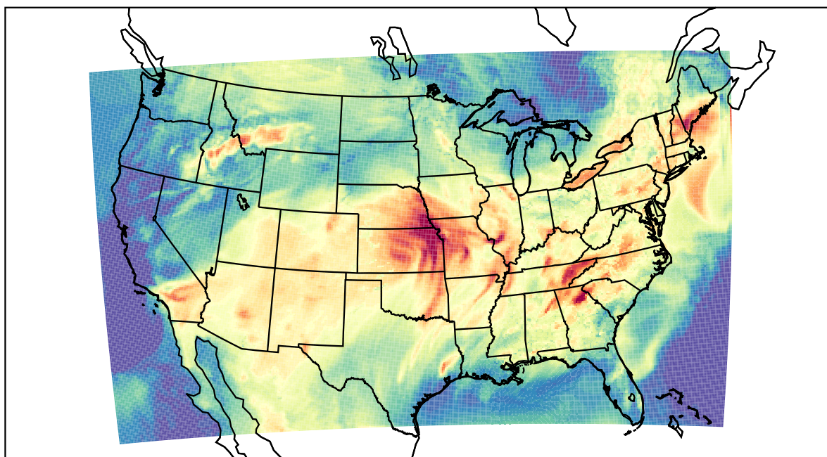
WRF (2022-06-12_22:00:00)
