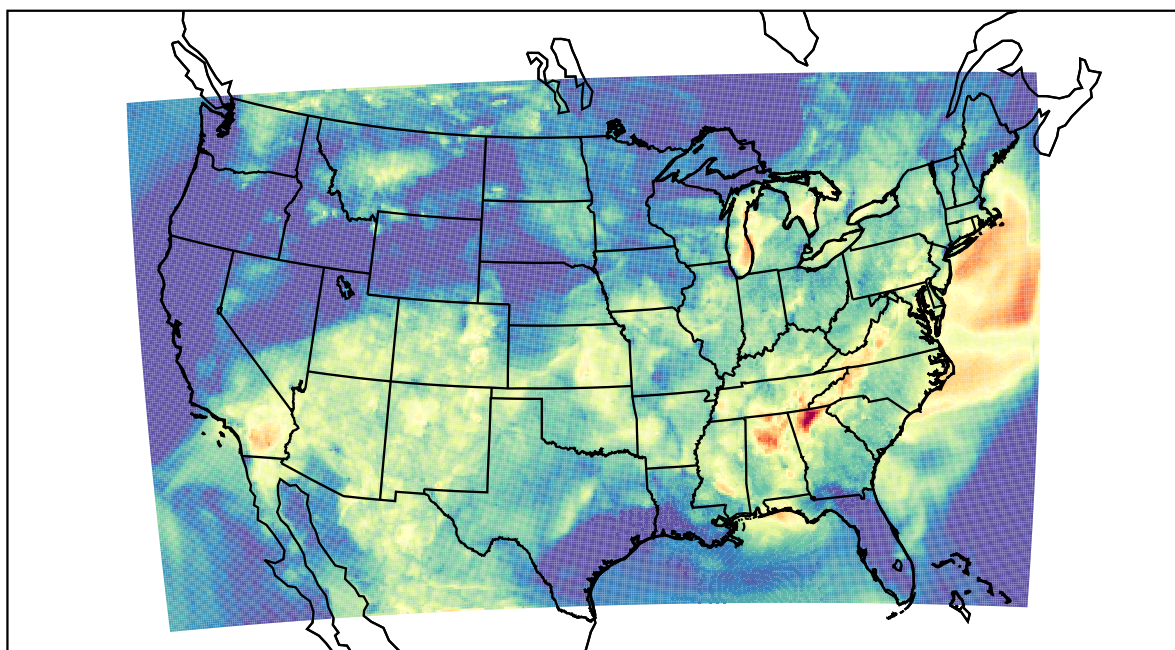
WRF (2022-06-12_04:00:00)
