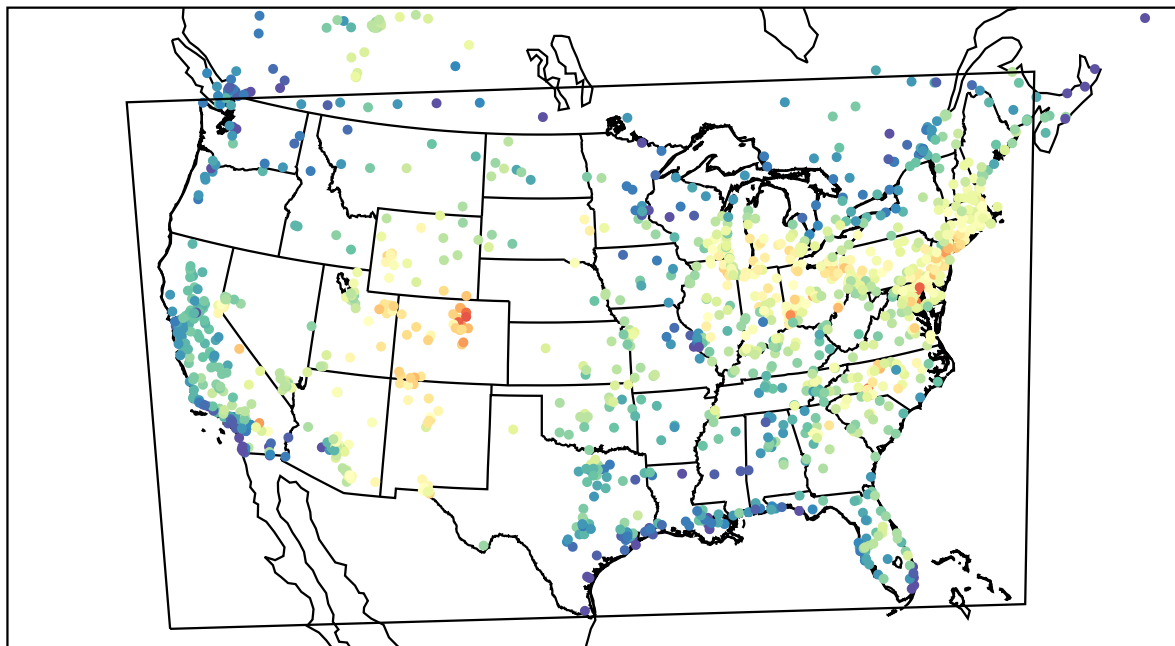
AirNOW (2022-06-13_17:00:00)
