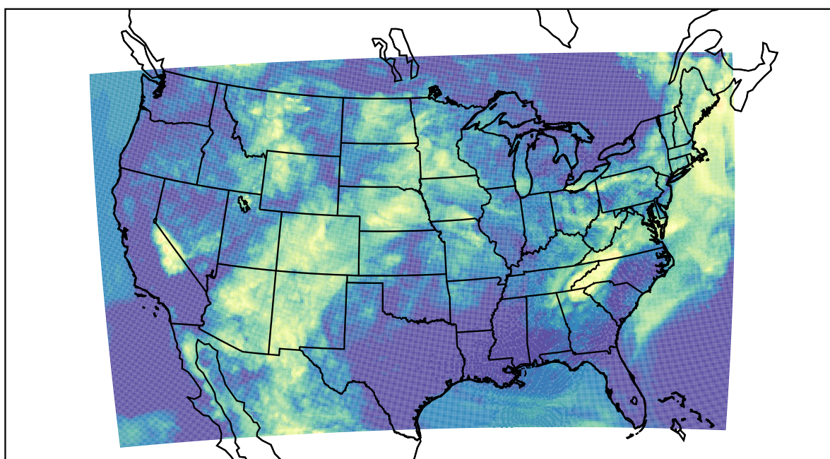
WRF (2022-06-13_10:00:00)
