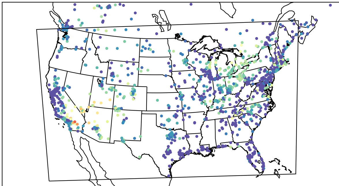
AirNOW (2022-06-12_07:00:00)
