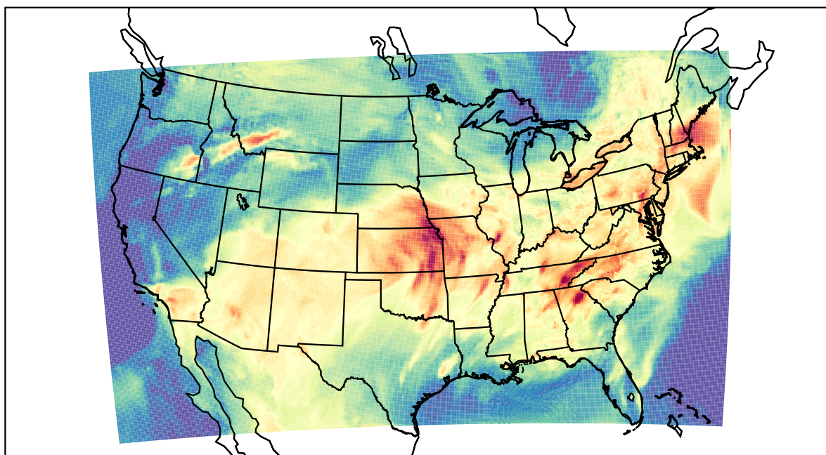
WRF (2022-06-12_19:00:00)
