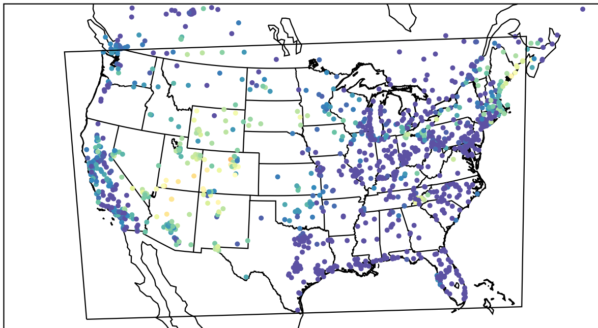
AirNOW (2022-06-13_09:00:00)
