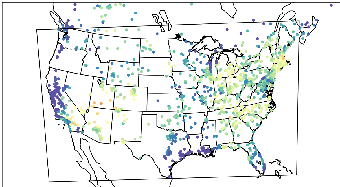
AirNOW (2022-06-12_15:00:00)
