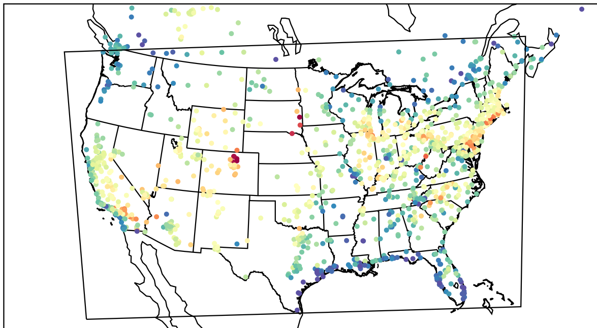
AirNOW (2022-06-13_22:00:00)
