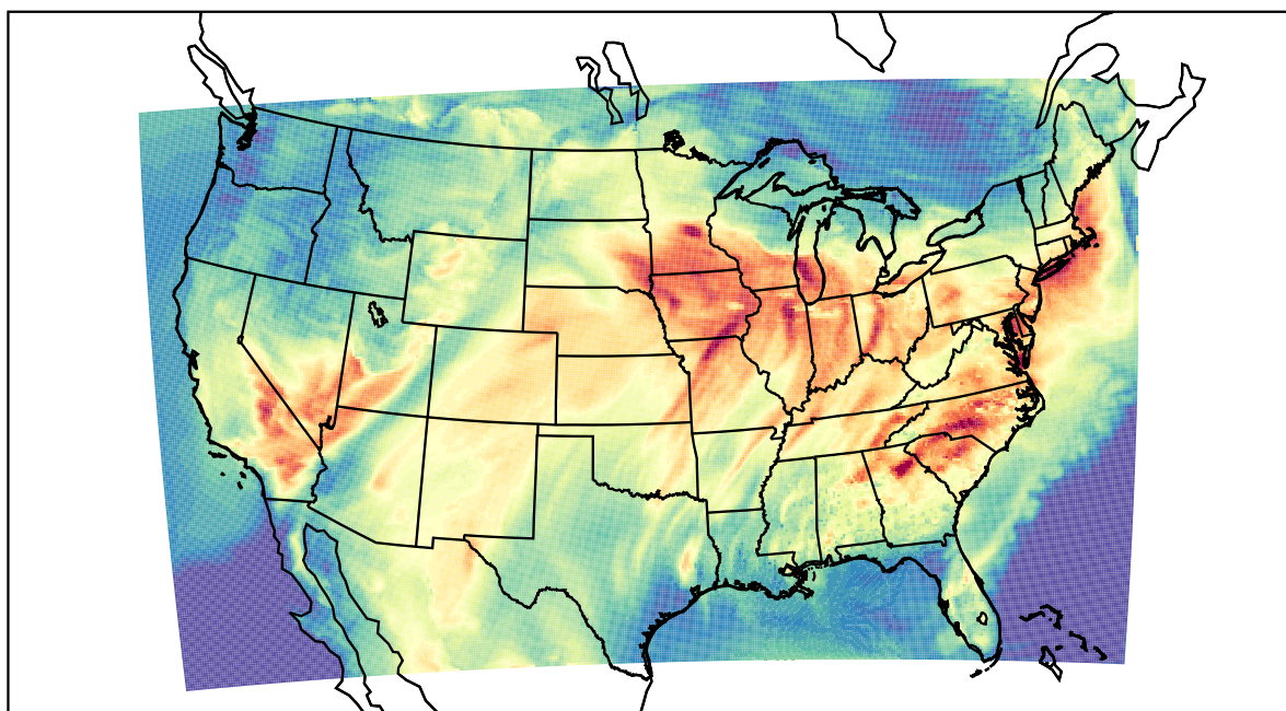
WRF (2022-06-13_21:00:00)
