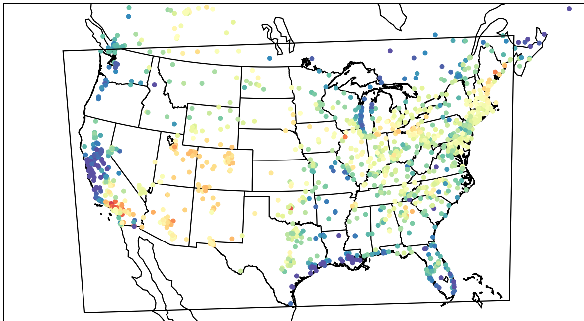
AirNOW (2022-06-12_22:00:00)
