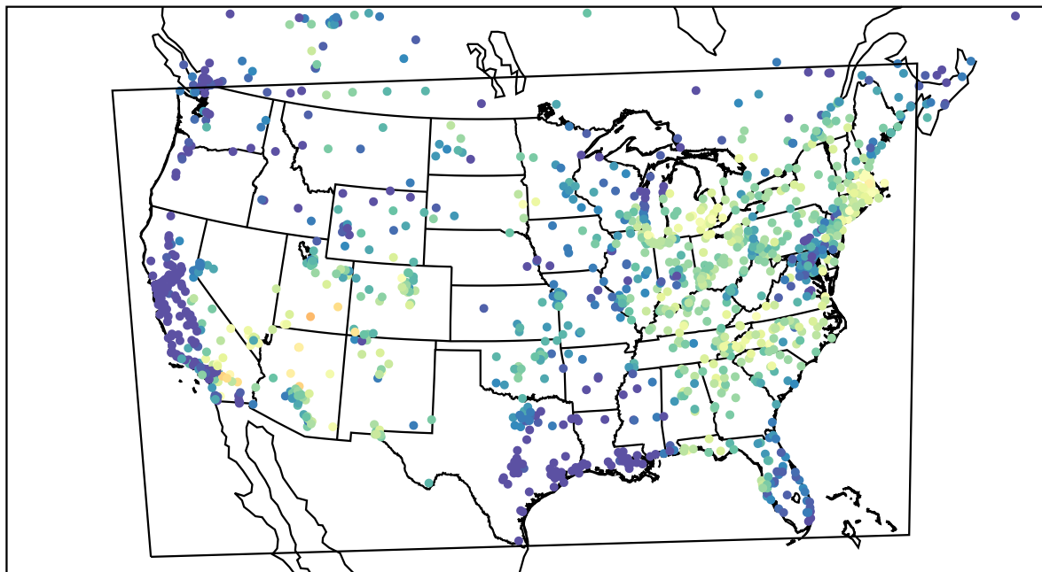
AirNOW (2022-06-12_14:00:00)
