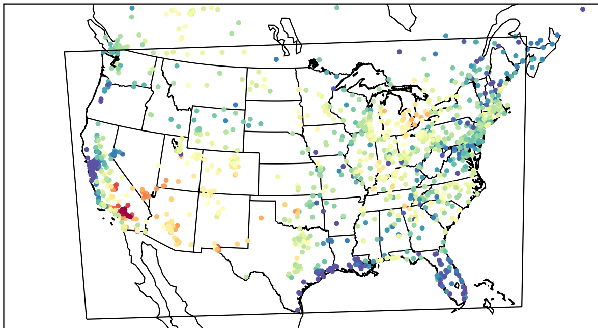
AirNOW (2022-06-12_00:00:00)
