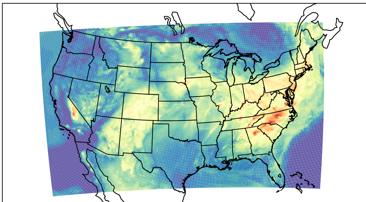
WRF (2022-06-13_15:00:00)
