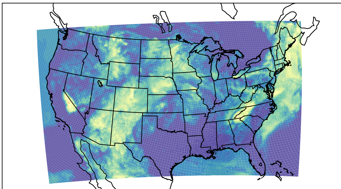
WRF (2022-06-13_11:00:00)
