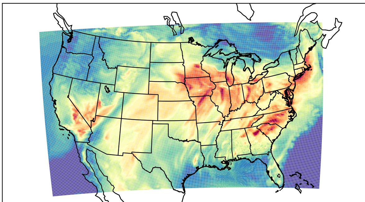
WRF (2022-06-13_20:00:00)
