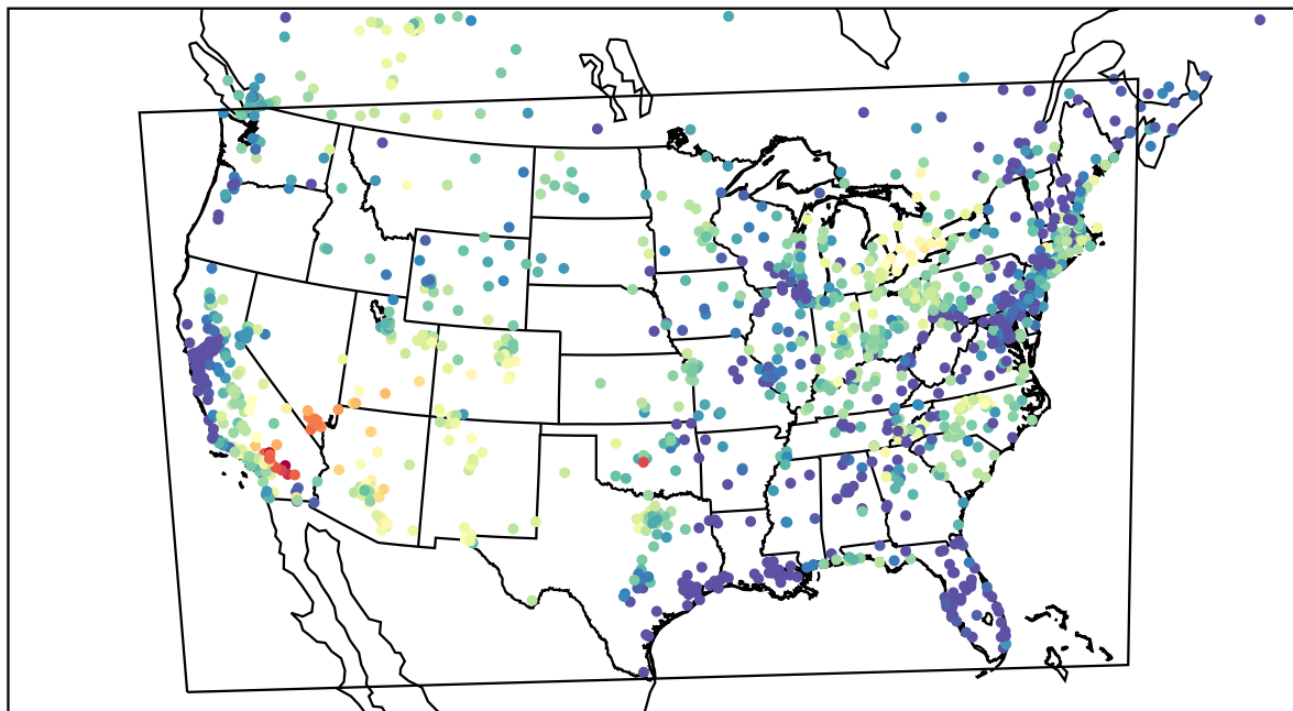
AirNOW (2022-06-12_03:00:00)
