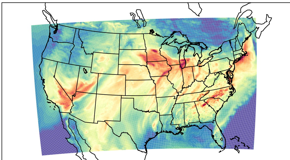
WRF (2022-06-13_23:00:00)
