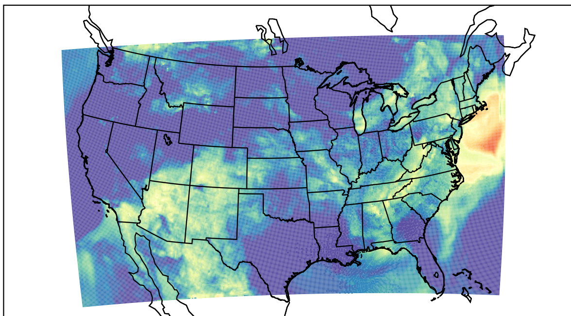
WRF (2022-06-12_12:00:00)
