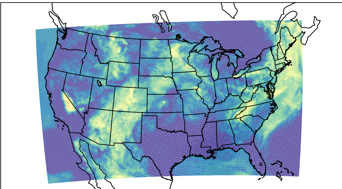
WRF (2022-06-13_12:00:00)
