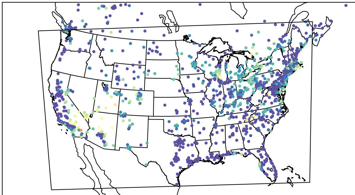
AirNOW (2022-06-12_11:00:00)
