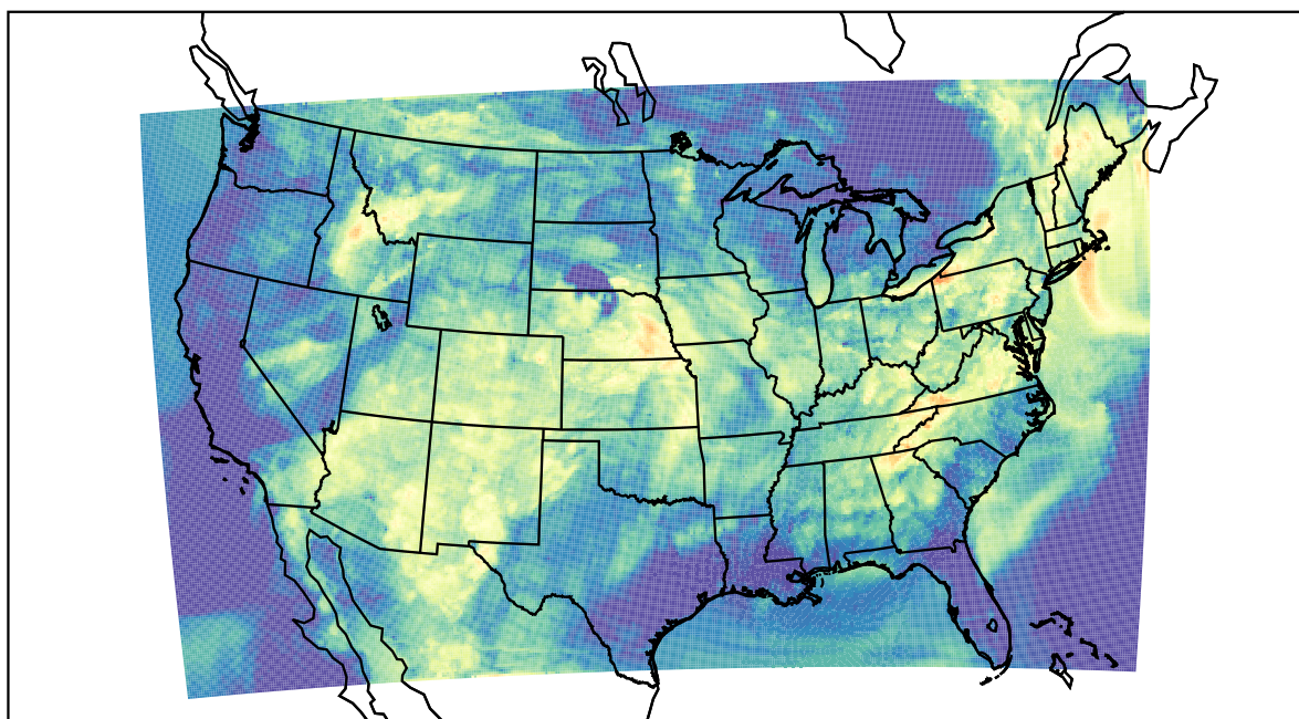
WRF (2022-06-13_04:00:00)
