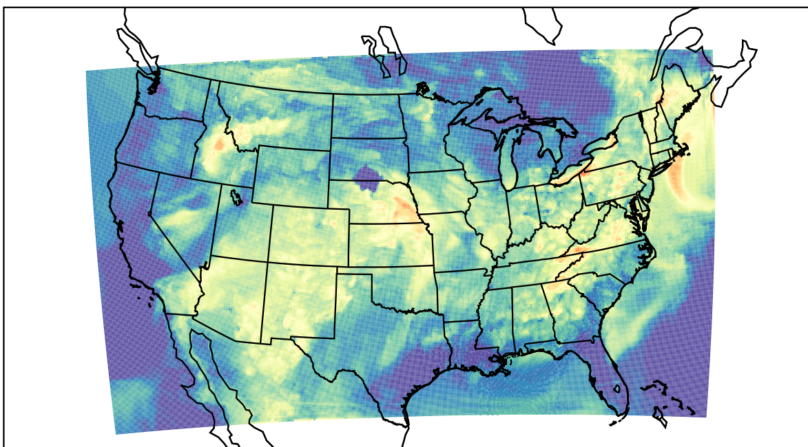
WRF (2022-06-13_03:00:00)
