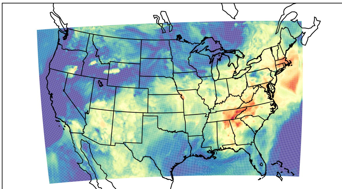
WRF (2022-06-12_15:00:00)
