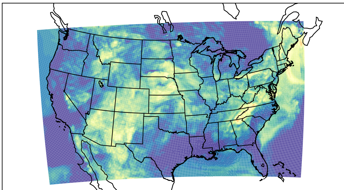
WRF (2022-06-13_07:00:00)
