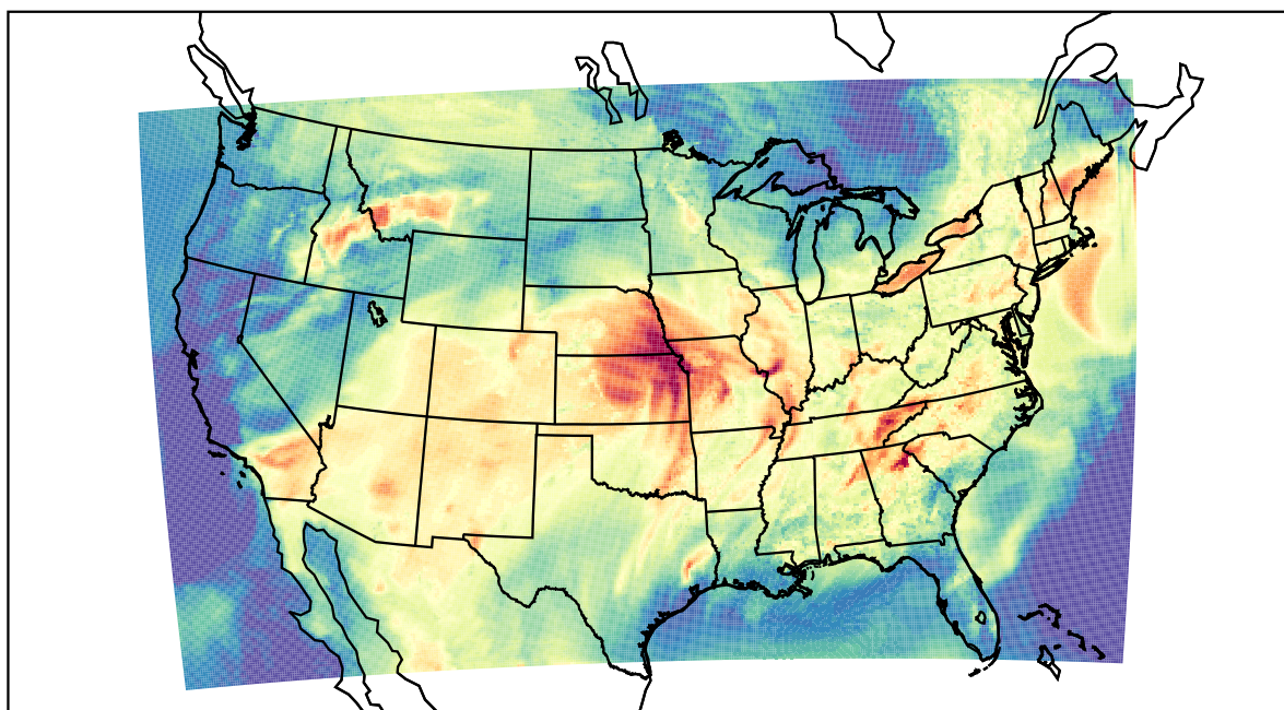
WRF (2022-06-12_23:00:00)
