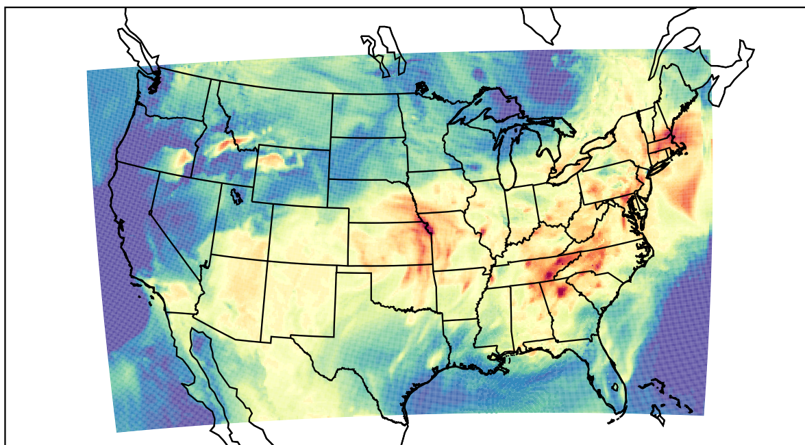
WRF (2022-06-12_17:00:00)
