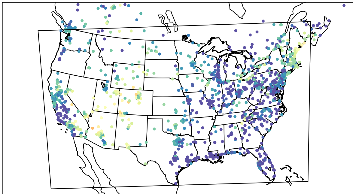
AirNOW (2022-06-13_05:00:00)
