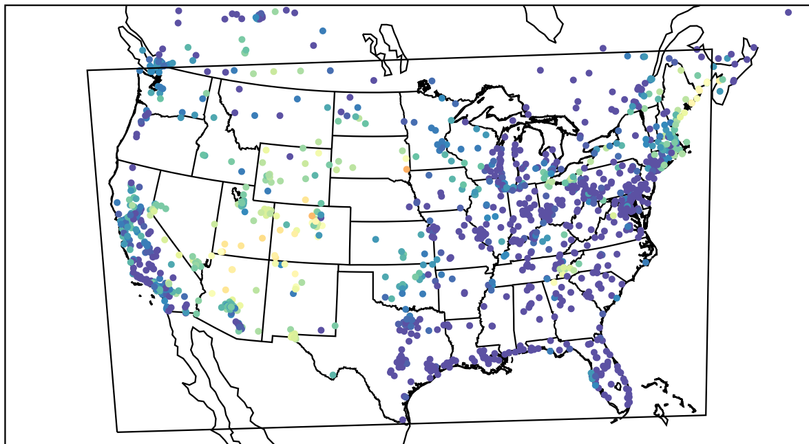
AirNOW (2022-06-13_08:00:00)
