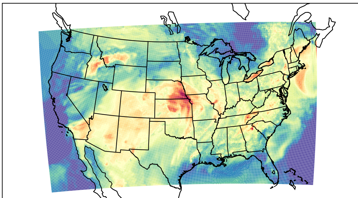
WRF (2022-06-13_00:00:00)
