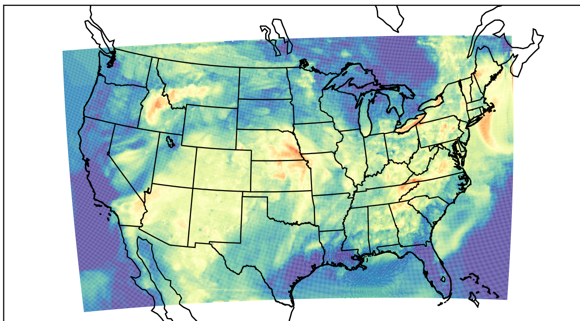
WRF (2022-06-13_02:00:00)
