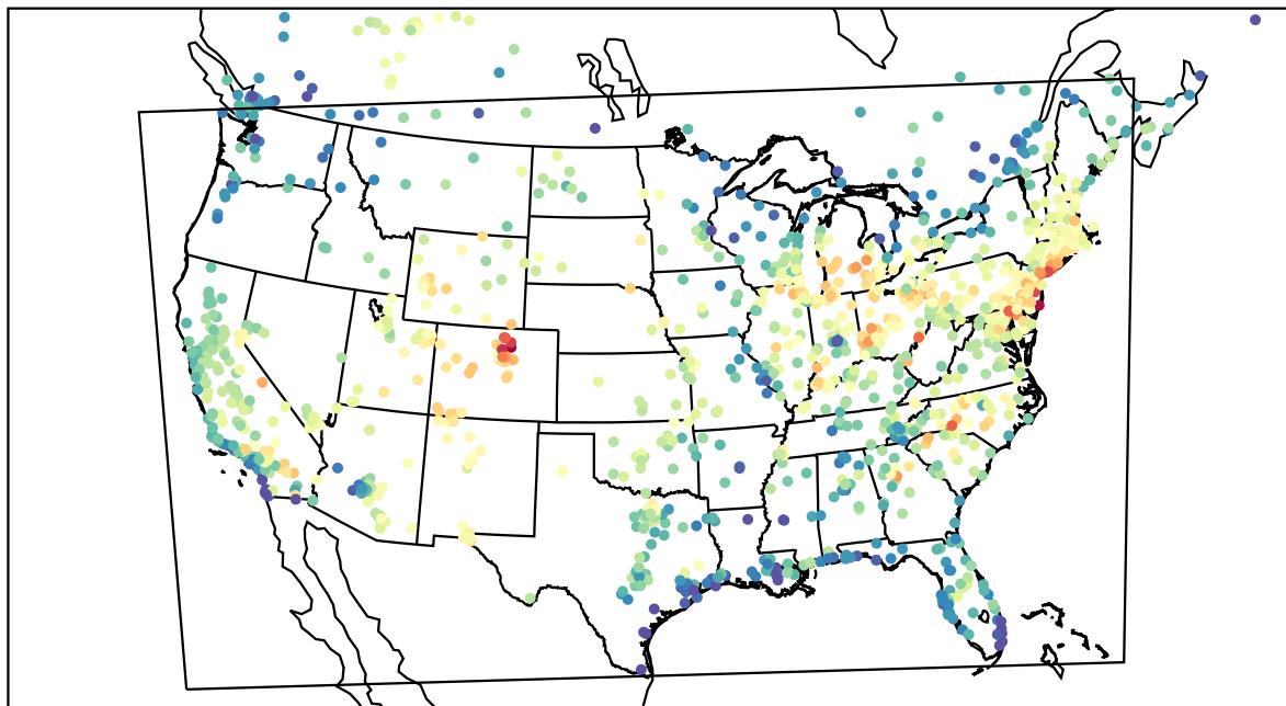
AirNOW (2022-06-13_19:00:00)
