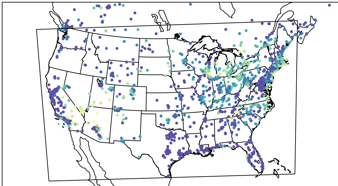
AirNOW (2022-06-12_12:00:00)
