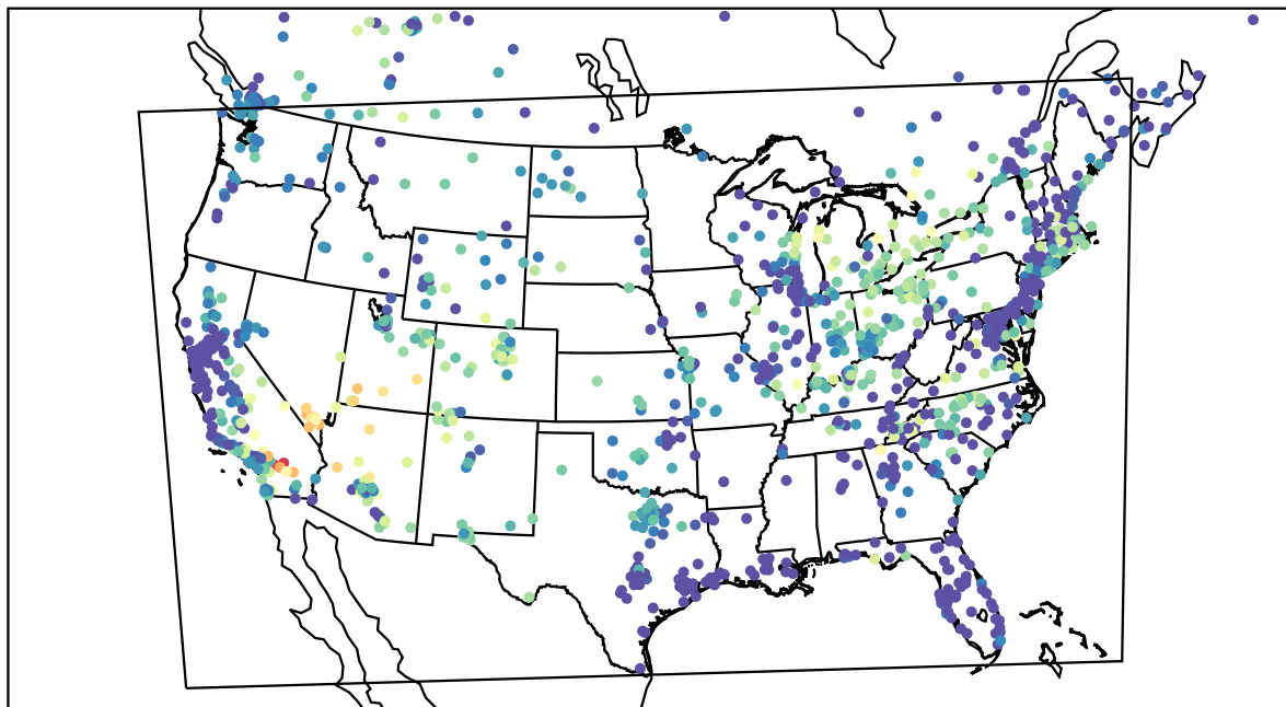
AirNOW (2022-06-12_06:00:00)
