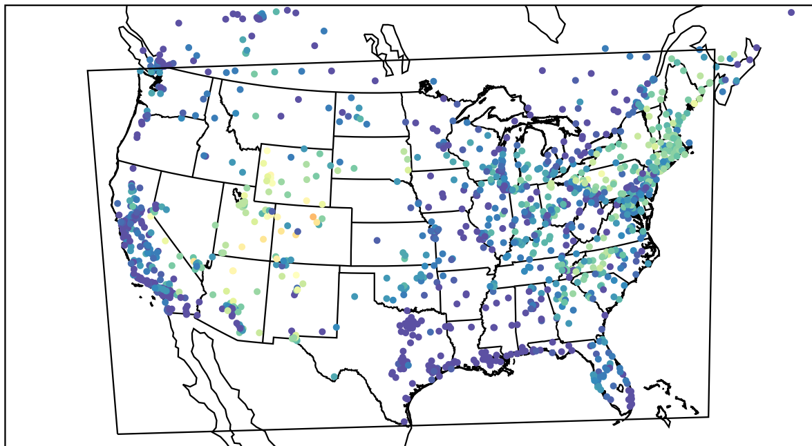
AirNOW (2022-06-13_13:00:00)
