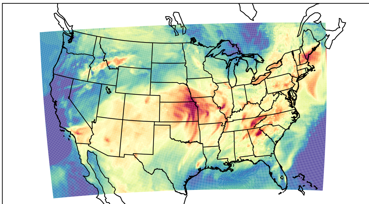
WRF (2022-06-12_21:00:00)
