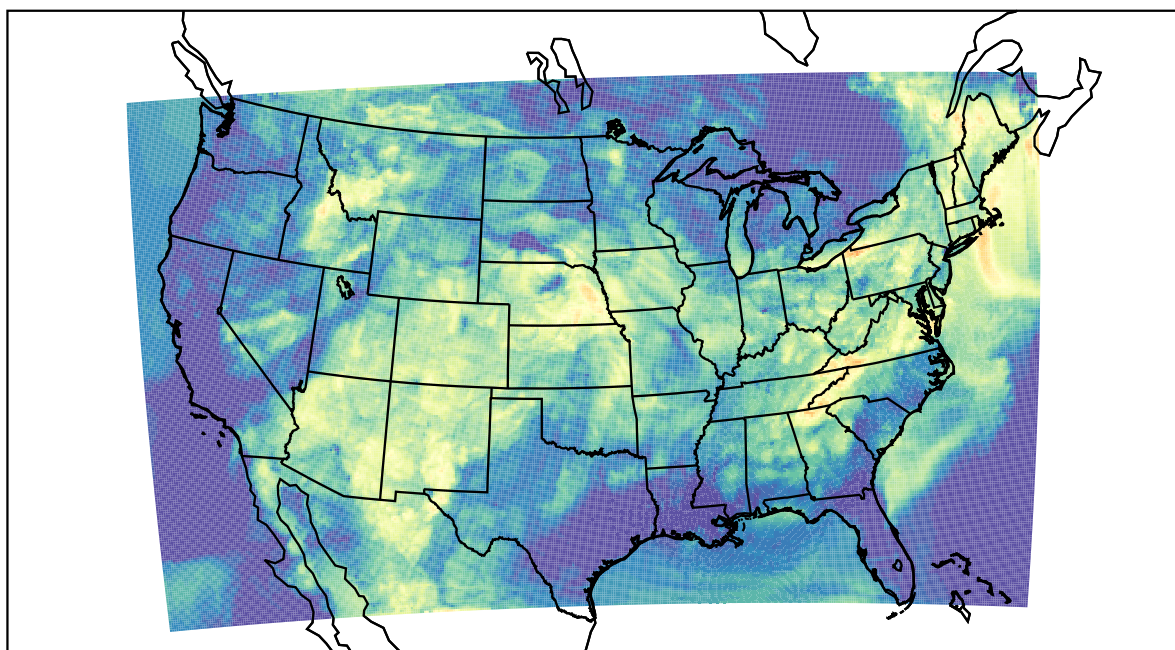
WRF (2022-06-13_05:00:00)
