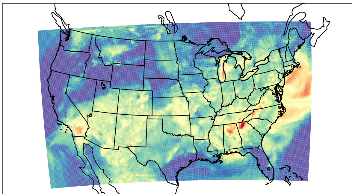
WRF (2022-06-12_03:00:00)
