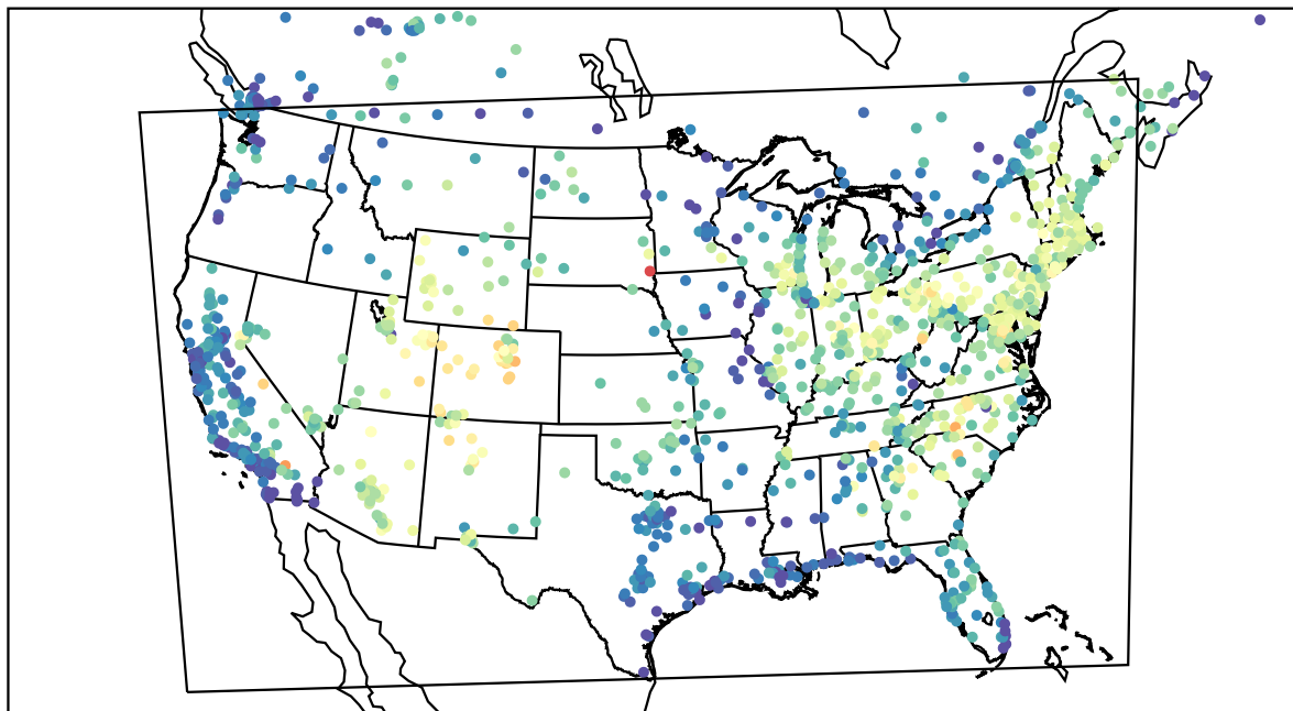
AirNOW (2022-06-13_15:00:00)
