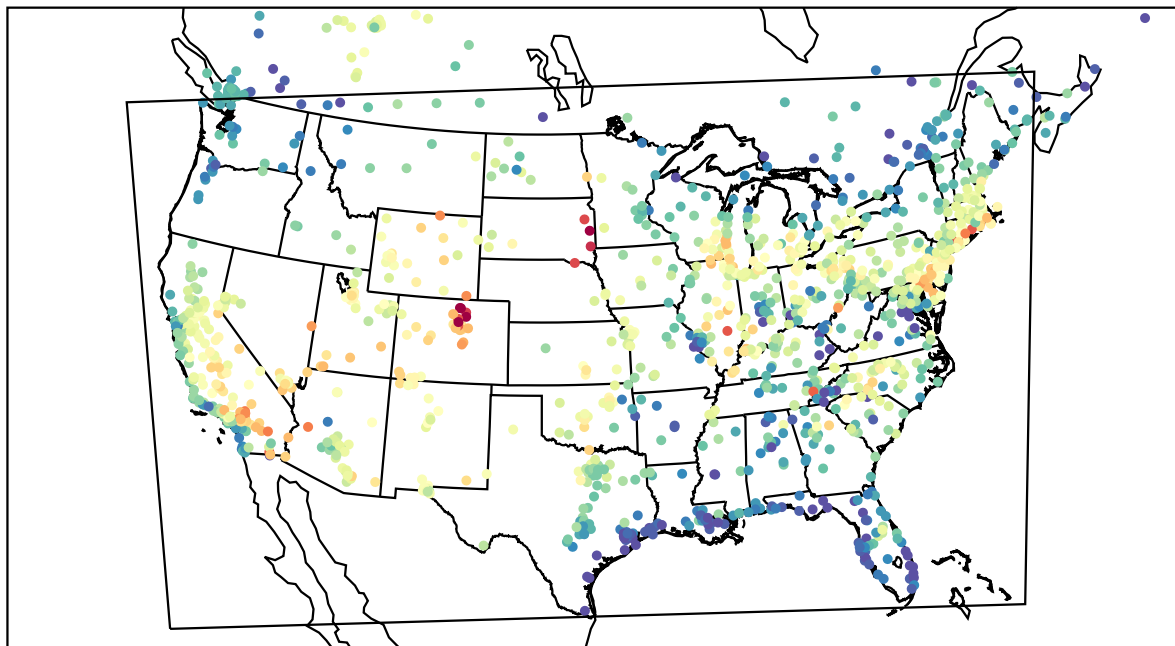
AirNOW (2022-06-13_23:00:00)
