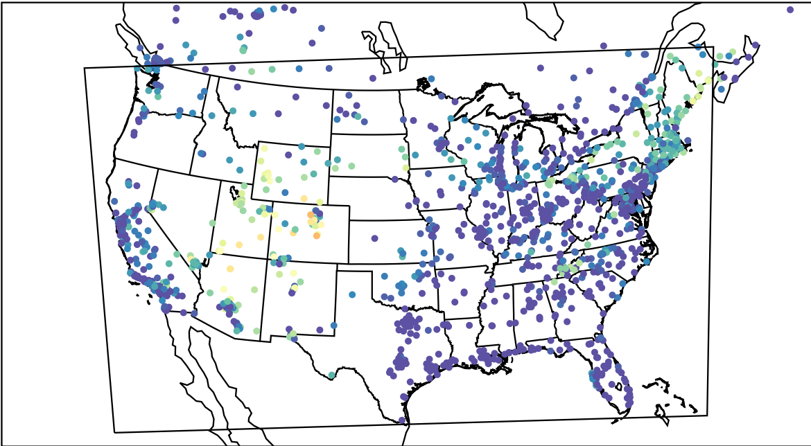
AirNOW (2022-06-13_12:00:00)
