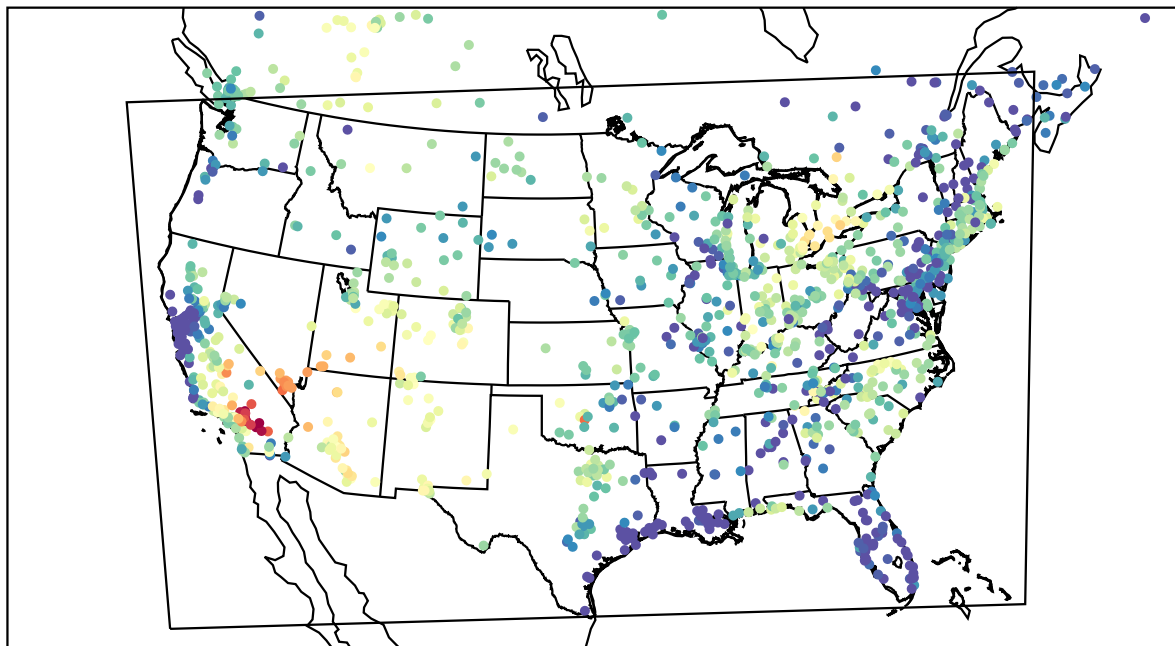
AirNOW (2022-06-12_02:00:00)
