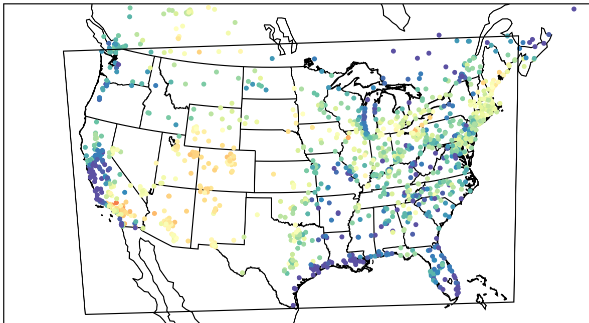
AirNOW (2022-06-13_00:00:00)
