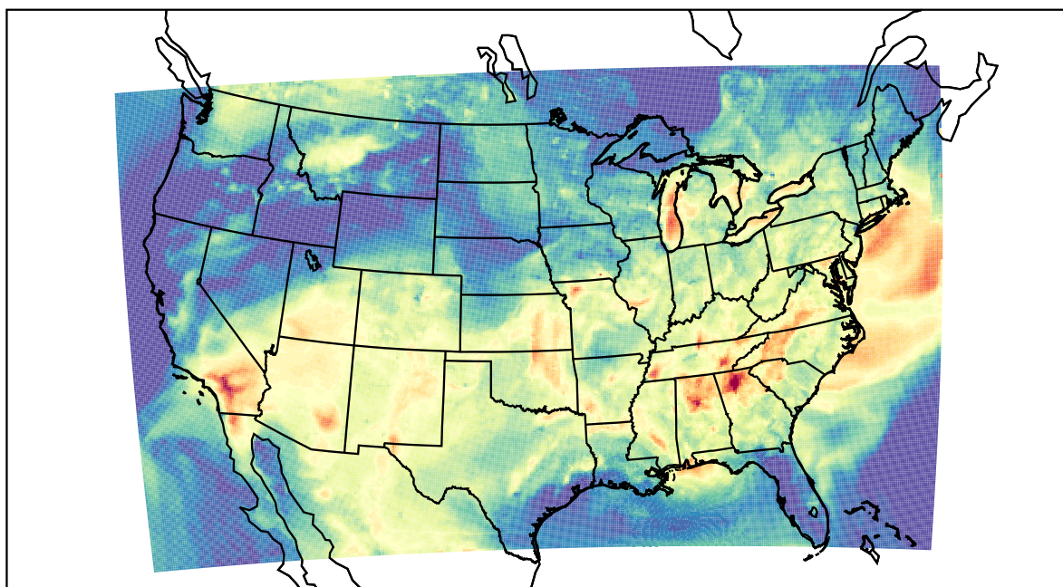
WRF (2022-06-12_01:00:00)
