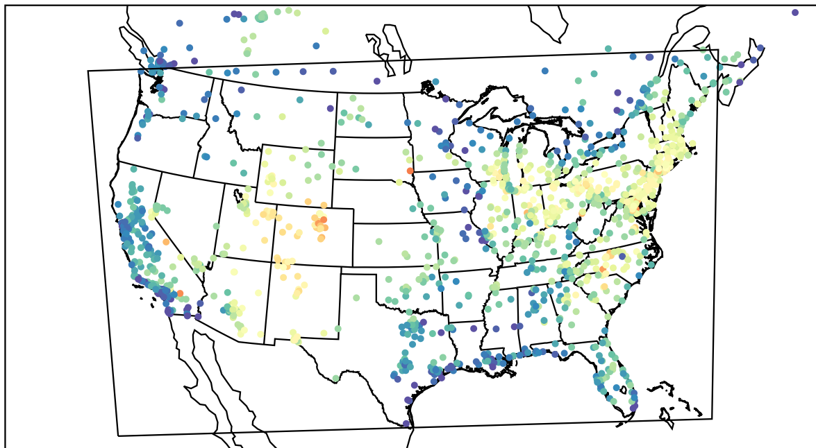
AirNOW (2022-06-13_16:00:00)
