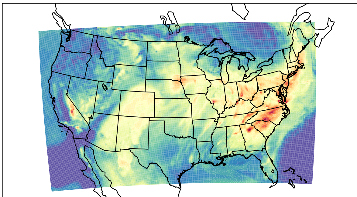
WRF (2022-06-13_16:00:00)
