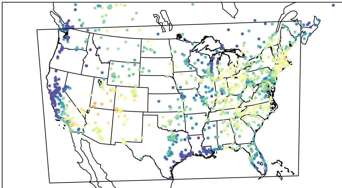
AirNOW (2022-06-12_16:00:00)
