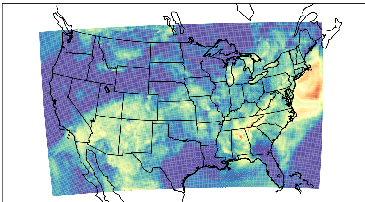
WRF (2022-06-12_08:00:00)
