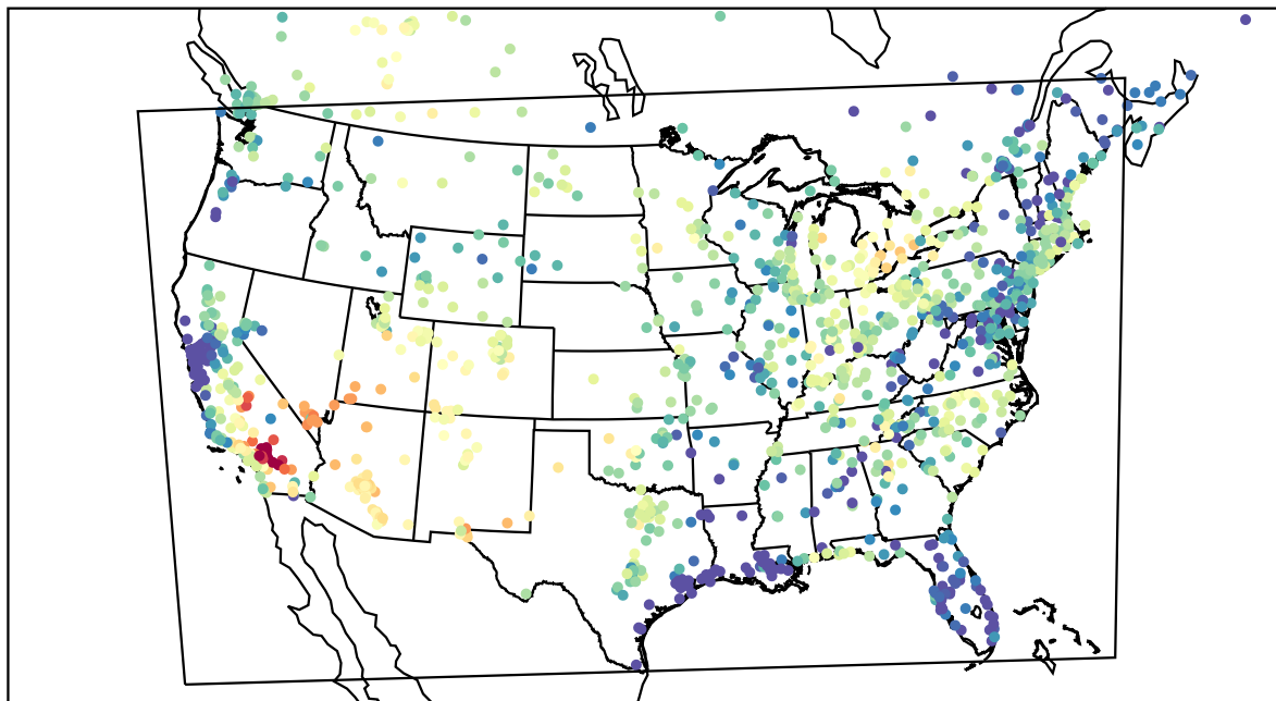
AirNOW (2022-06-12_01:00:00)
