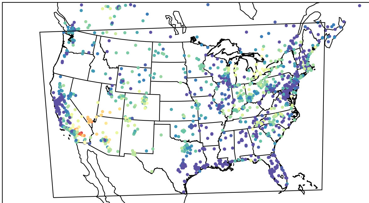
AirNOW (2022-06-12_05:00:00)
