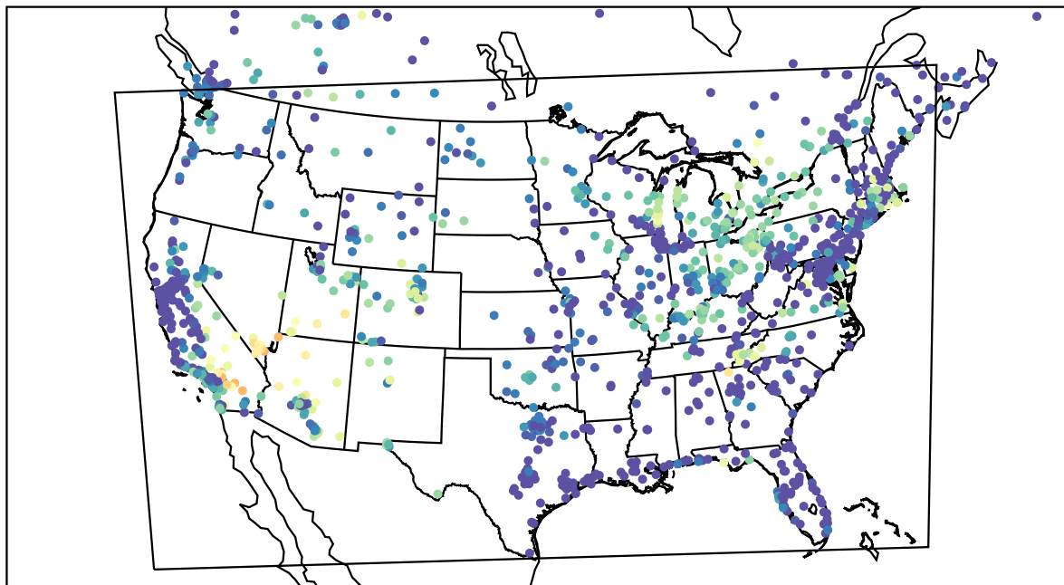
AirNOW (2022-06-12_08:00:00)
