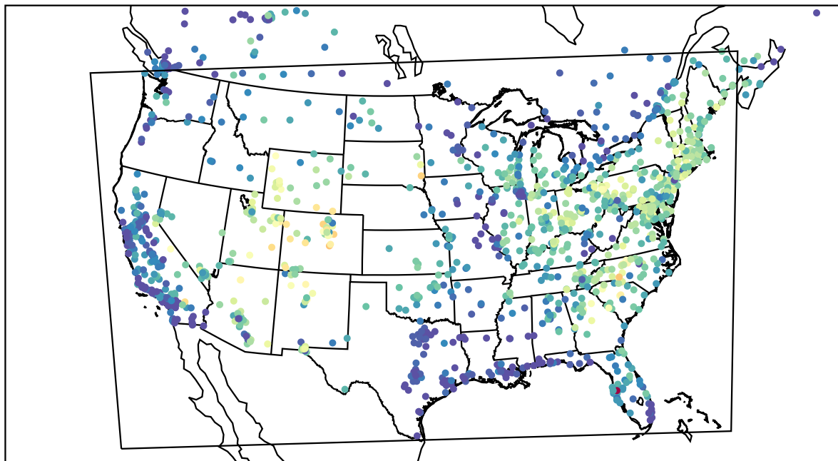
AirNOW (2022-06-13_14:00:00)
