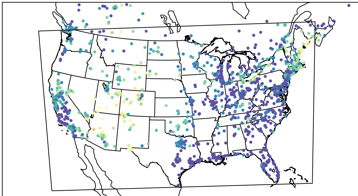
AirNOW (2022-06-13_06:00:00)
