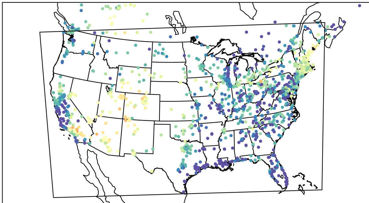
AirNOW (2022-06-13_02:00:00)
