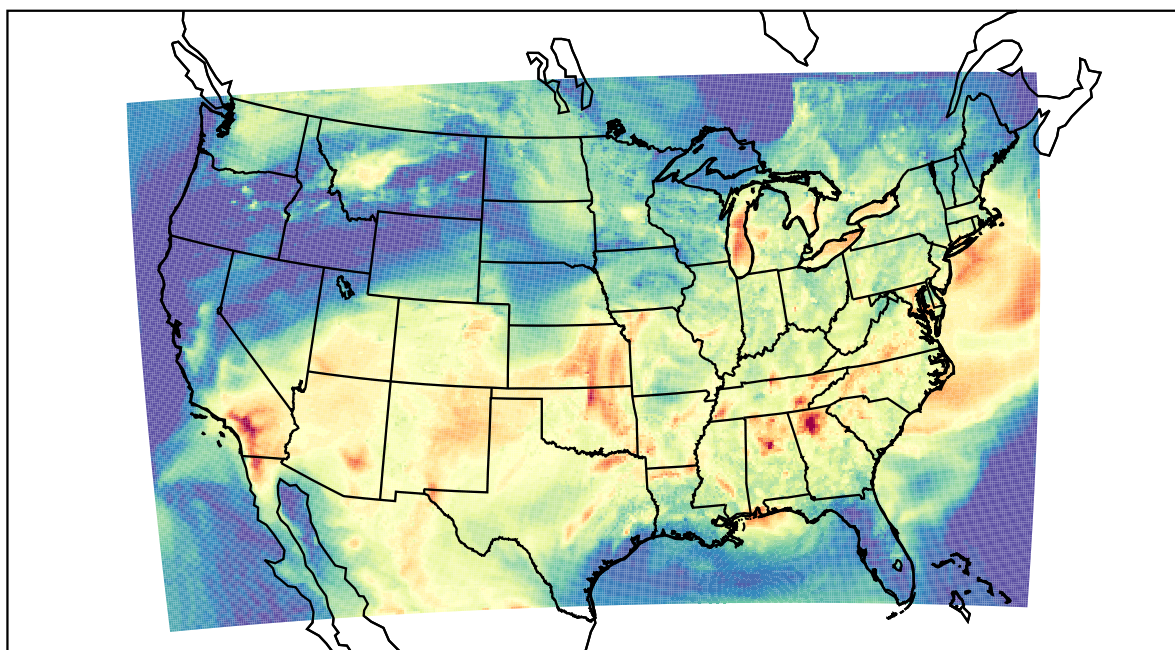
WRF (2022-06-12_00:00:00)
