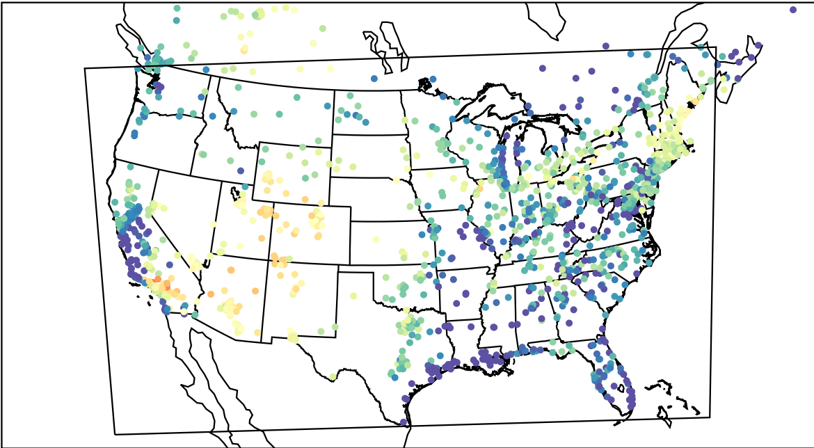
AirNOW (2022-06-13_01:00:00)
