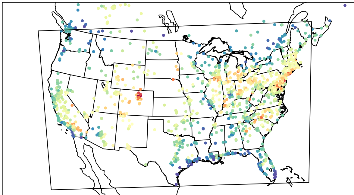
AirNOW (2022-06-13_20:00:00)
