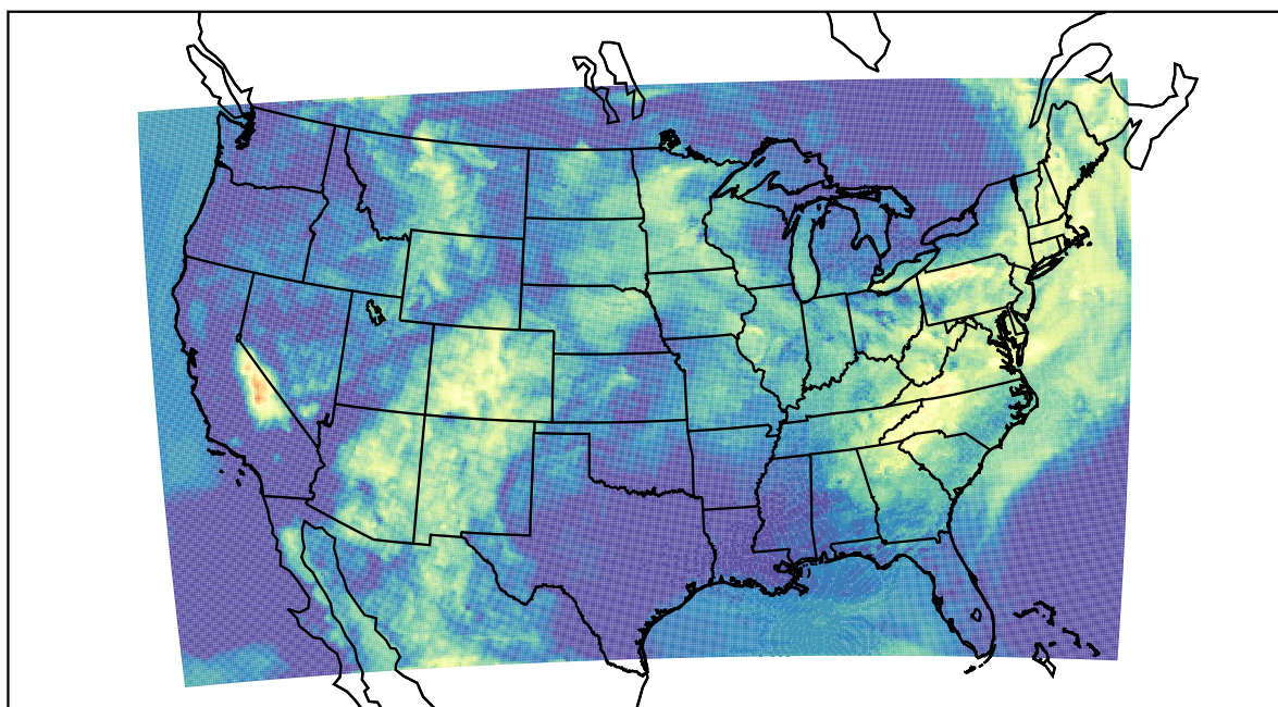
WRF (2022-06-13_13:00:00)
