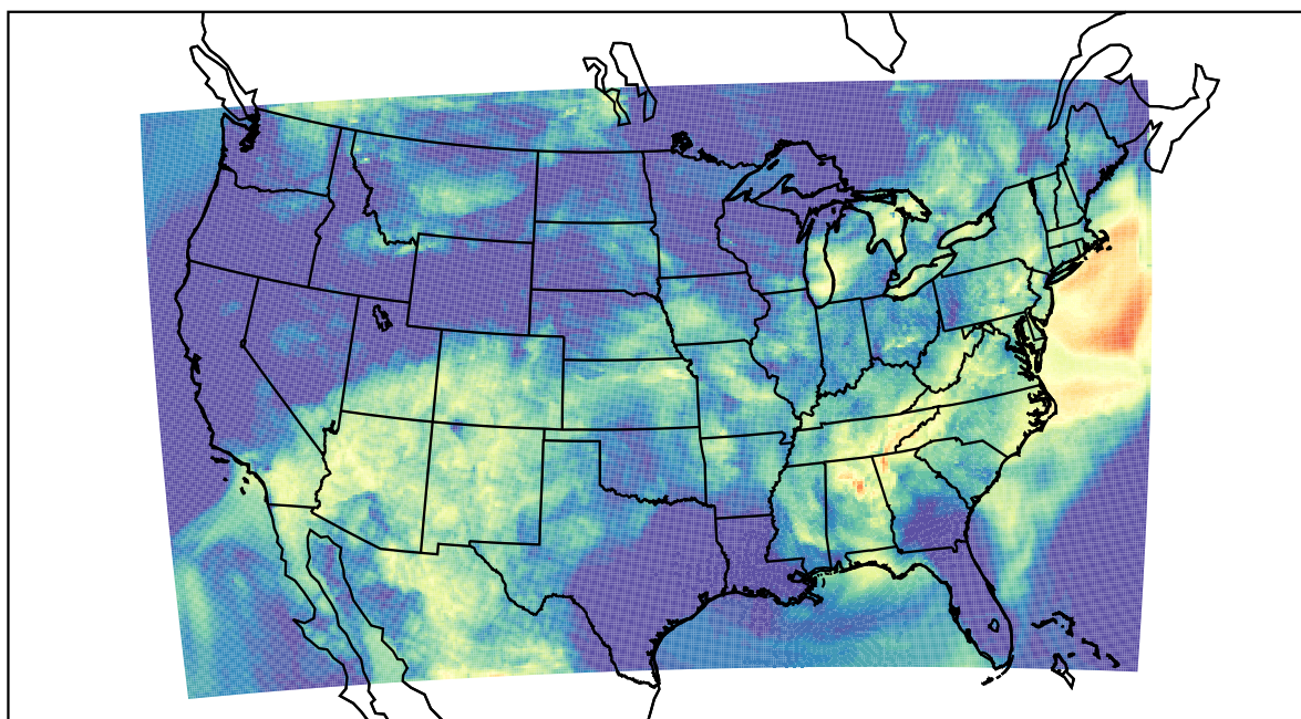
WRF (2022-06-12_09:00:00)
