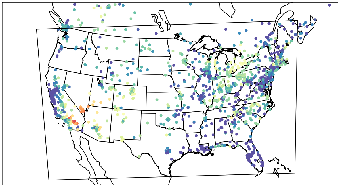
AirNOW (2022-06-12_04:00:00)
