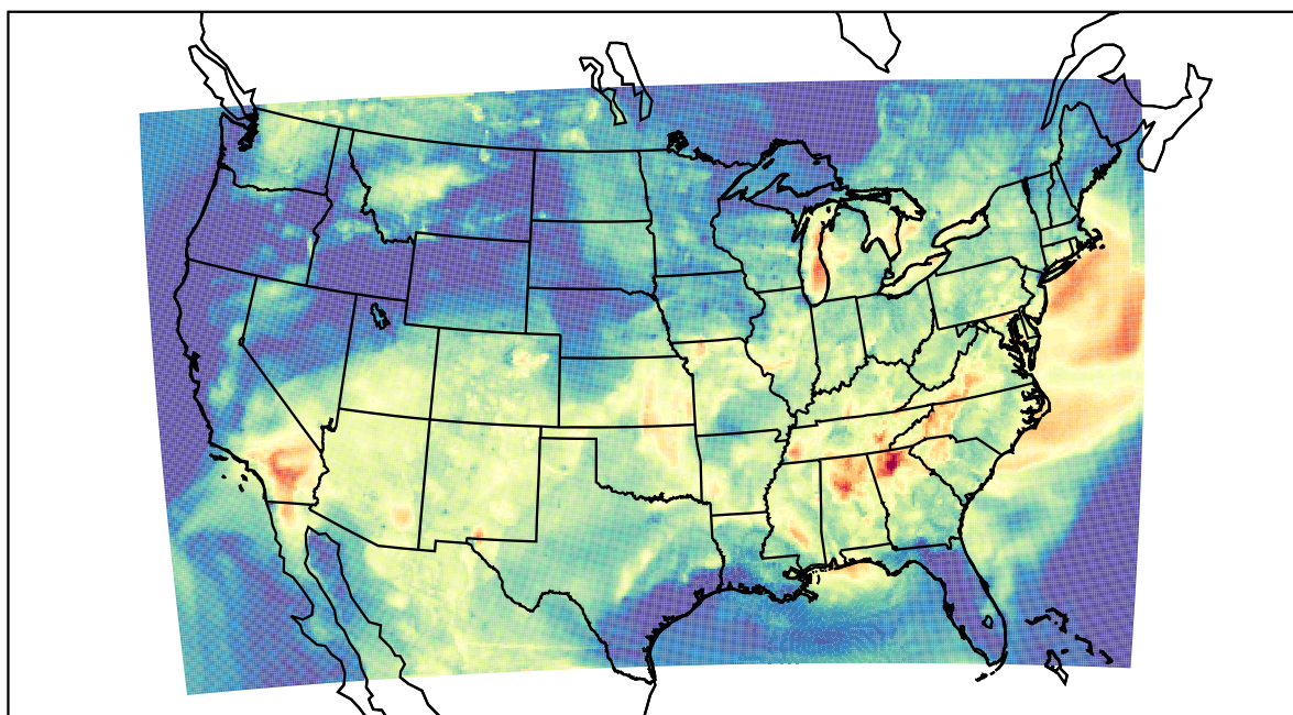
WRF (2022-06-12_02:00:00)
