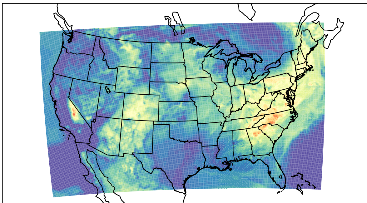
WRF (2022-06-13_14:00:00)
