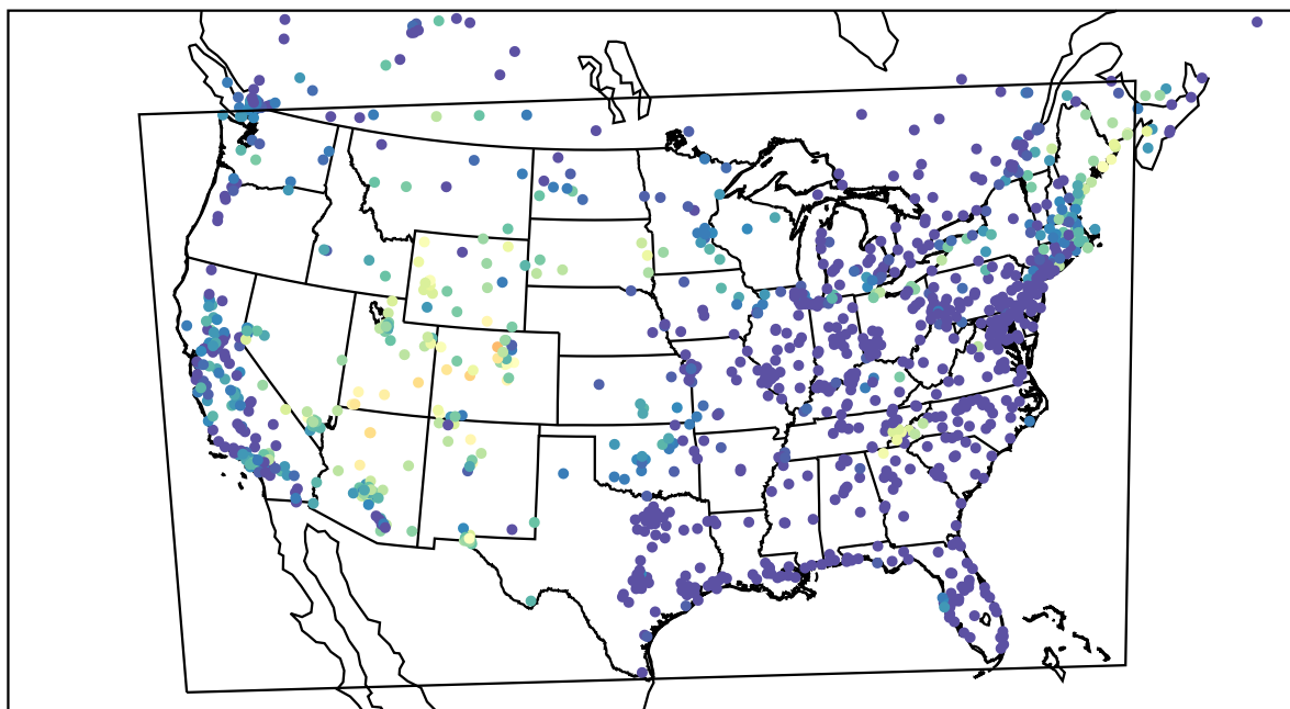
AirNOW (2022-06-13_10:00:00)
