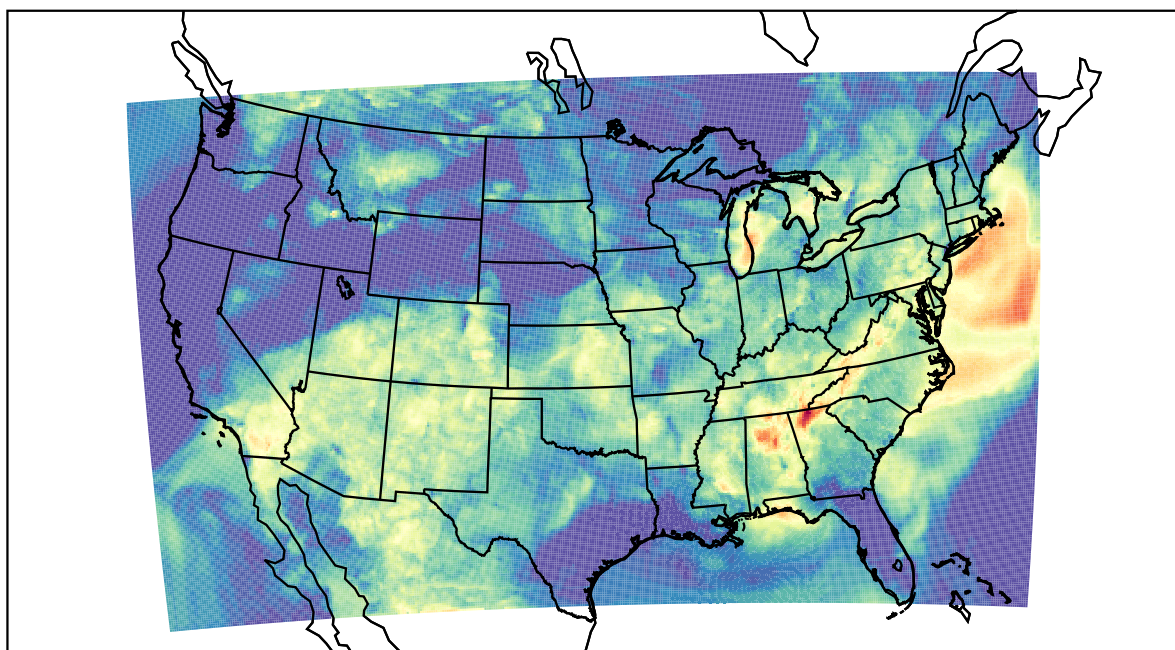
WRF (2022-06-12_05:00:00)
