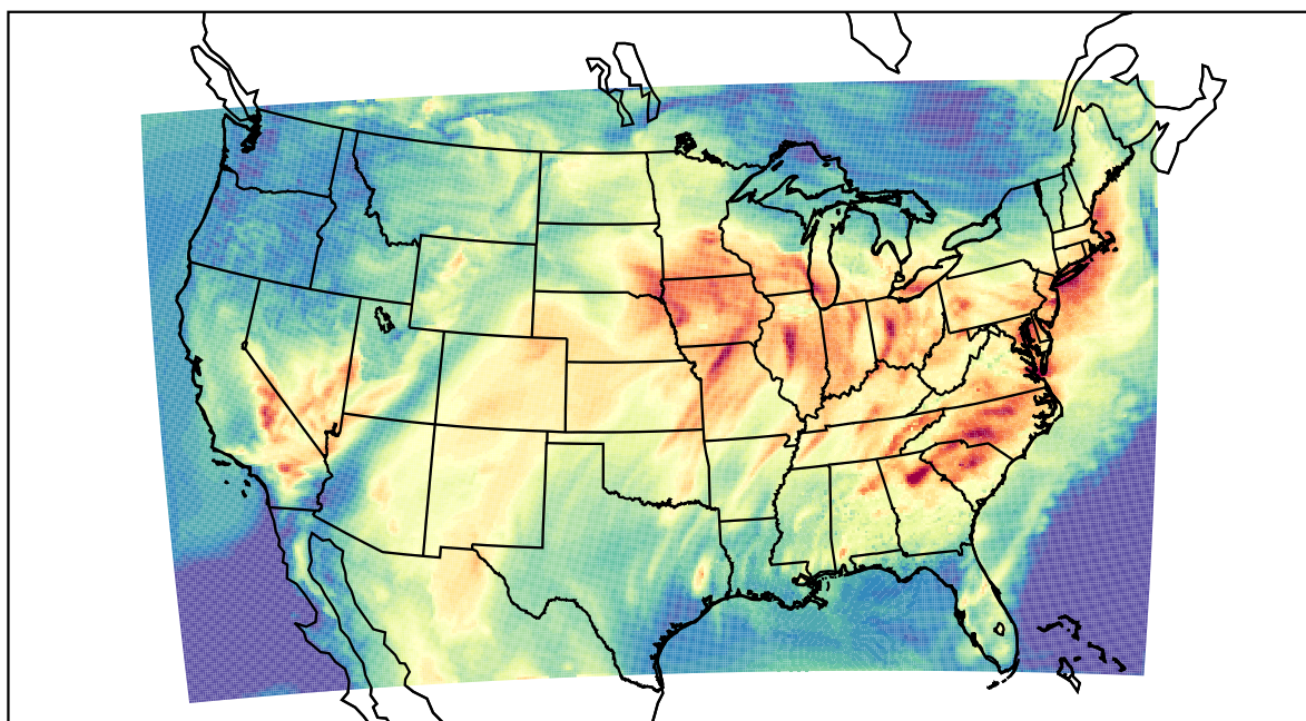
WRF (2022-06-13_19:00:00)
