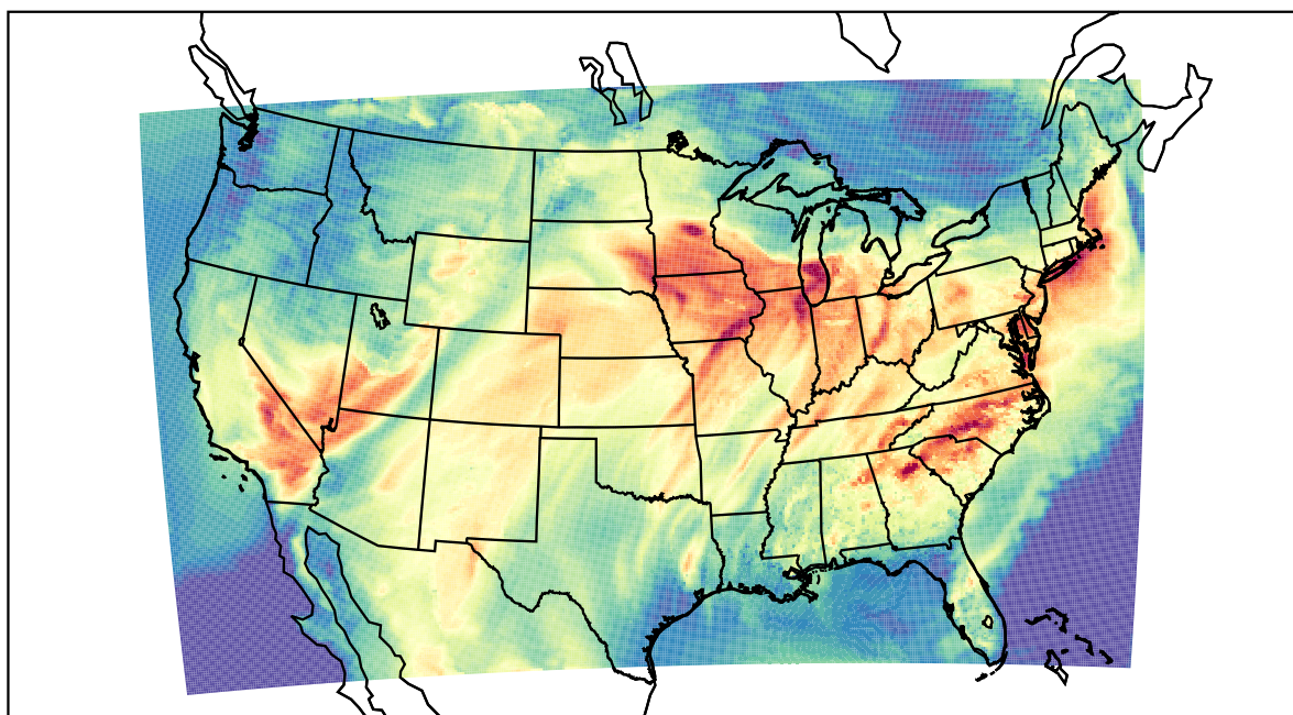
WRF (2022-06-13_22:00:00)
