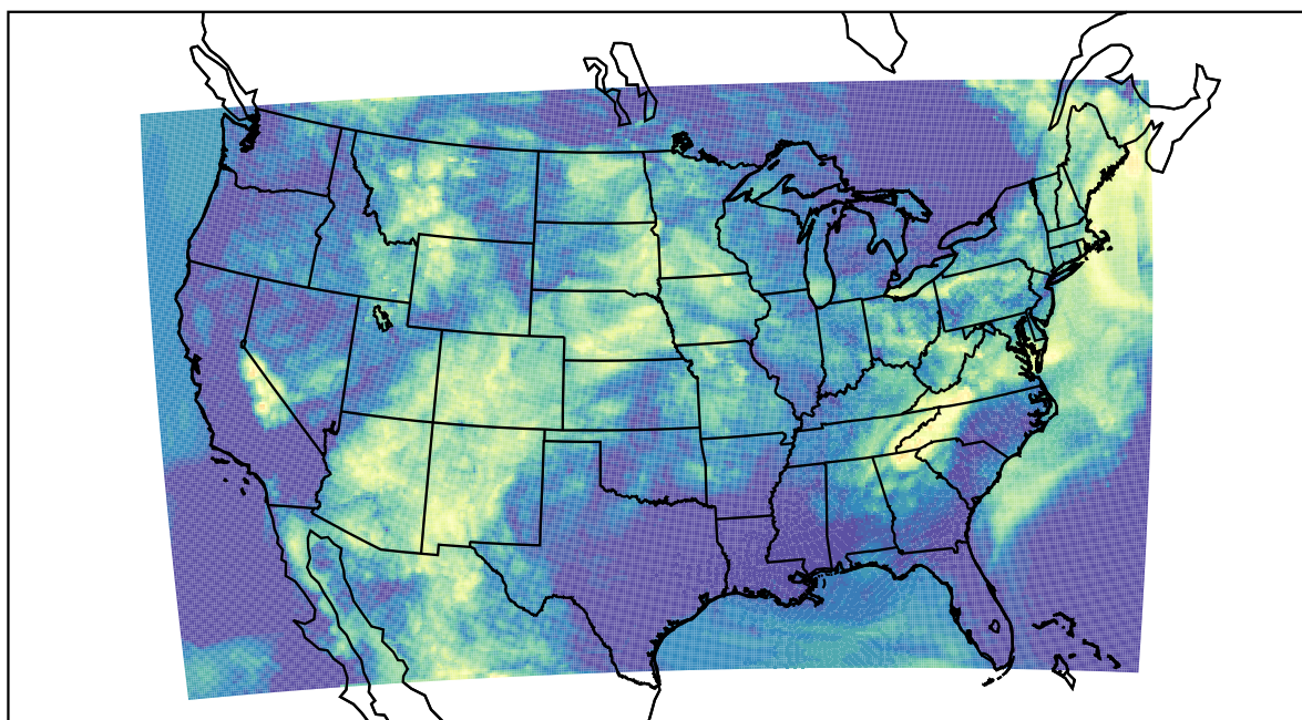
WRF (2022-06-13_09:00:00)
