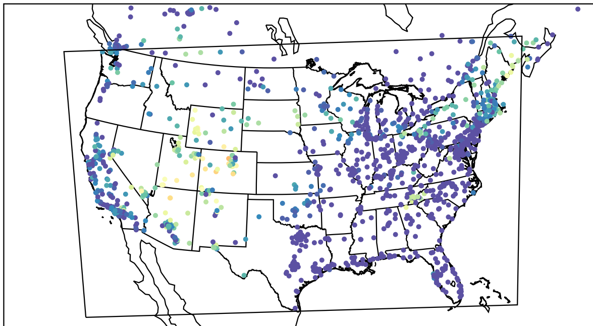
AirNOW (2022-06-13_11:00:00)
