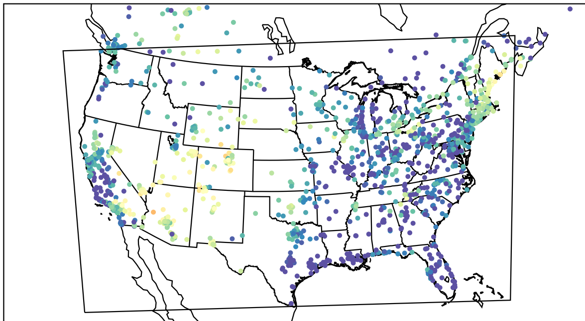
AirNOW (2022-06-13_04:00:00)
