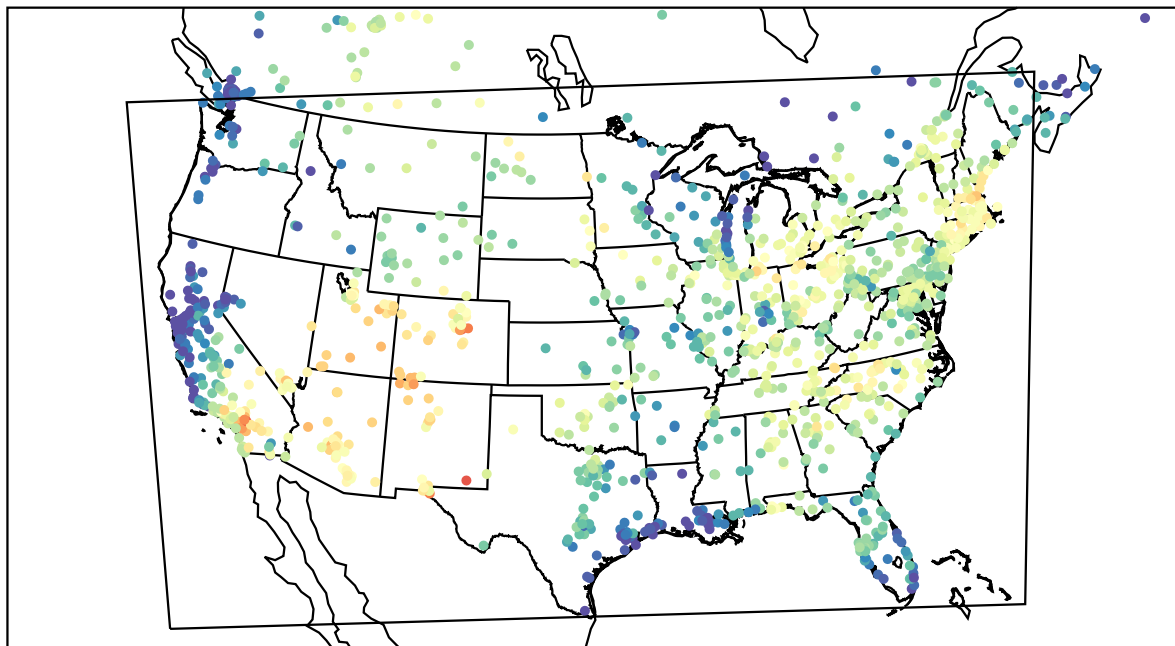
AirNOW (2022-06-12_17:00:00)
