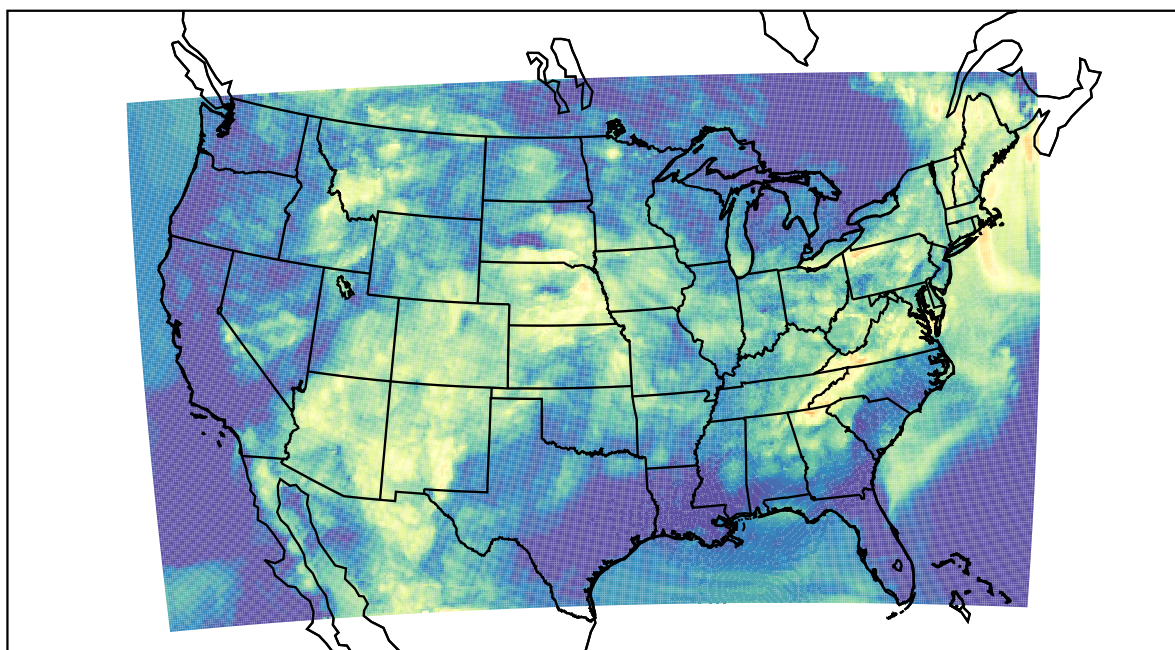
WRF (2022-06-13_06:00:00)
