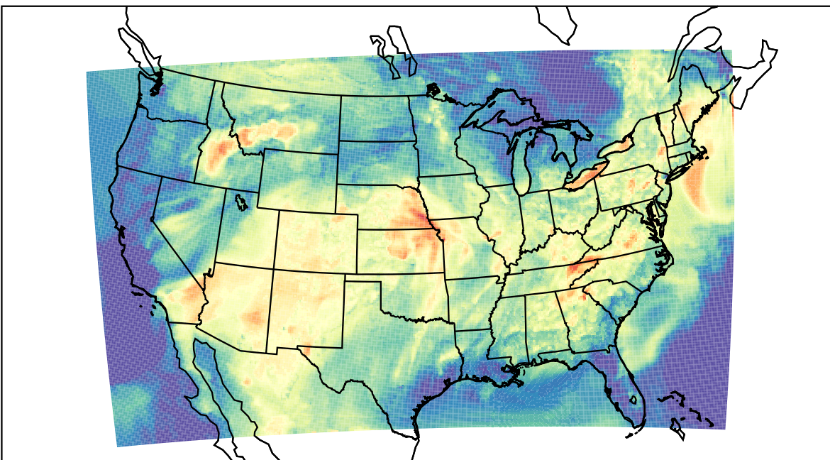
WRF (2022-06-13_01:00:00)
