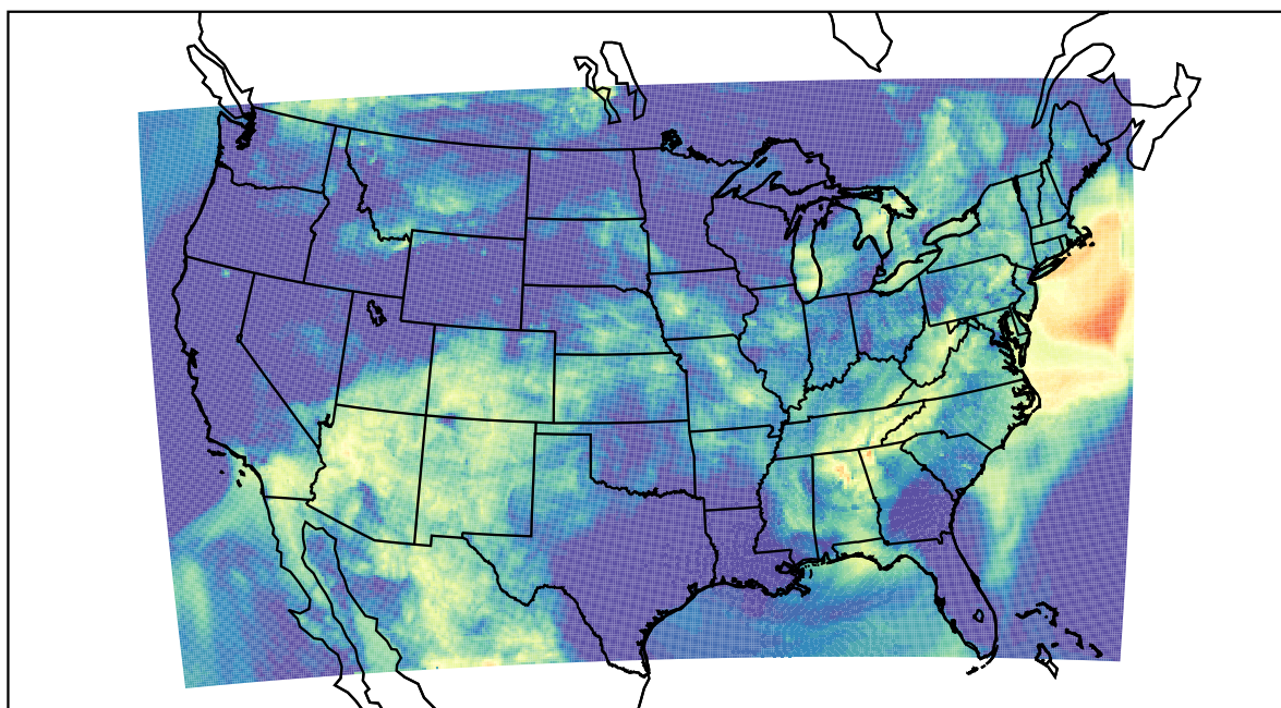
WRF (2022-06-12_11:00:00)
