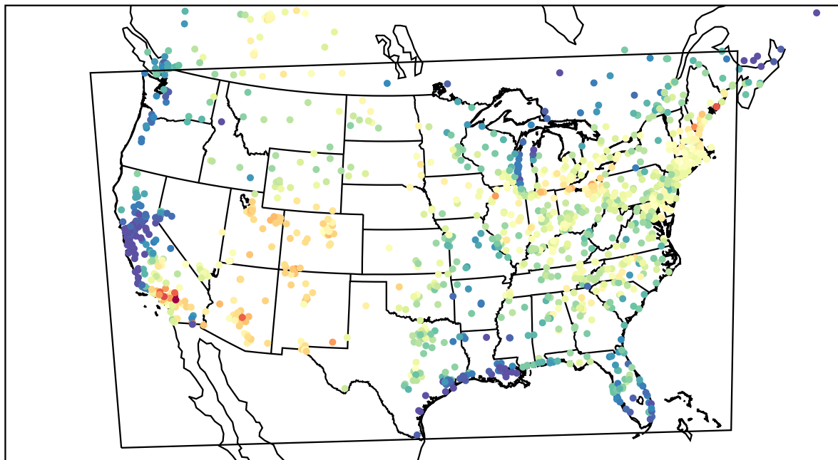
AirNOW (2022-06-12_21:00:00)
