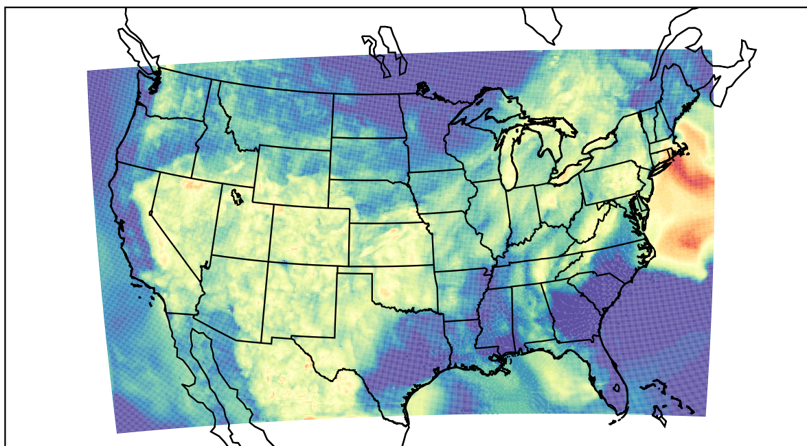
WRF (2022-07-01_06:00:00)
