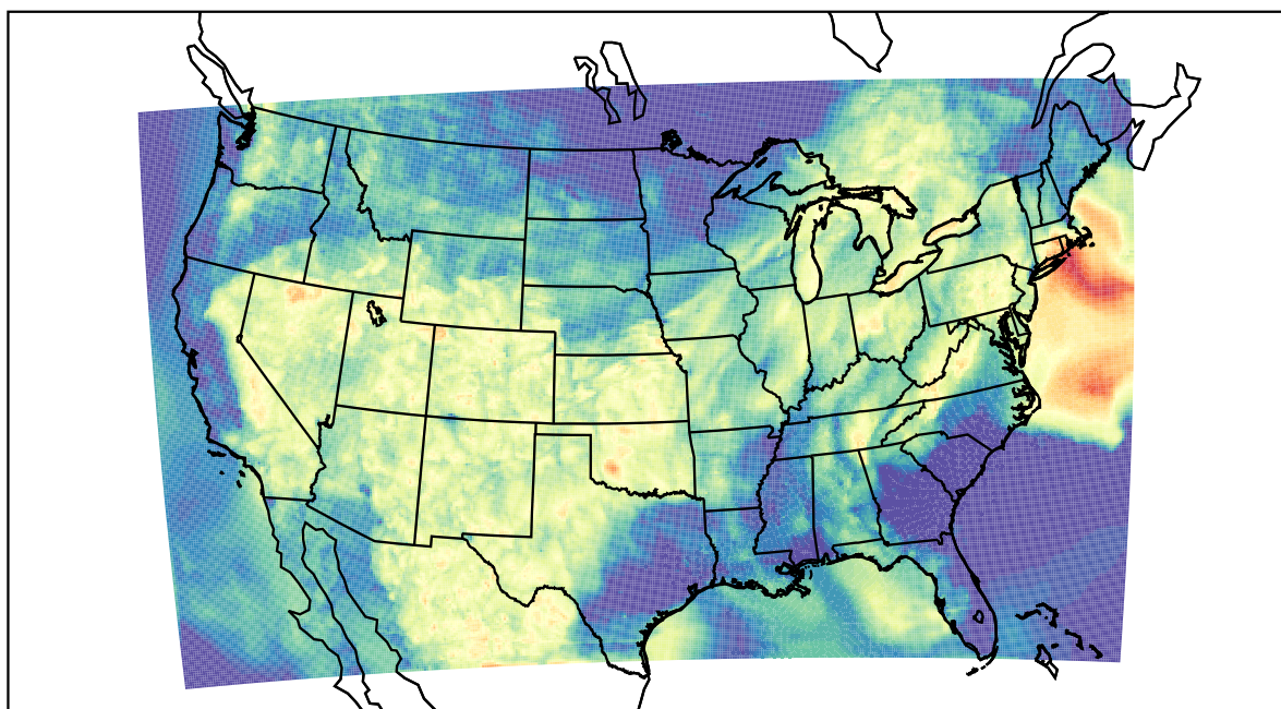
WRF (2022-07-01_05:00:00)
