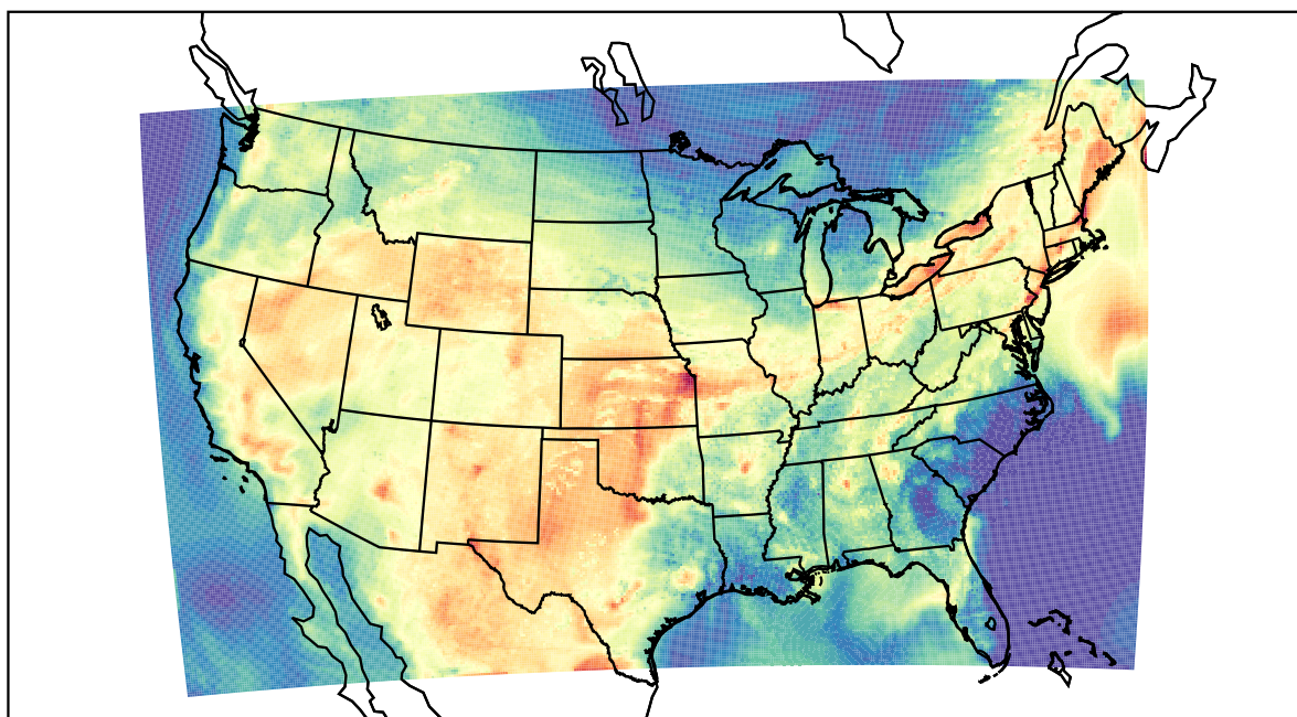
WRF (2022-07-02_00:00:00)
