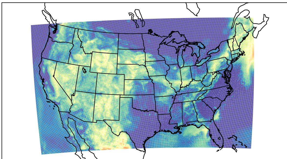
WRF (2022-07-02_11:00:00)
