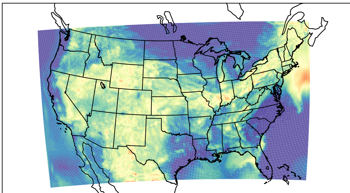
WRF (2022-07-02_05:00:00)
