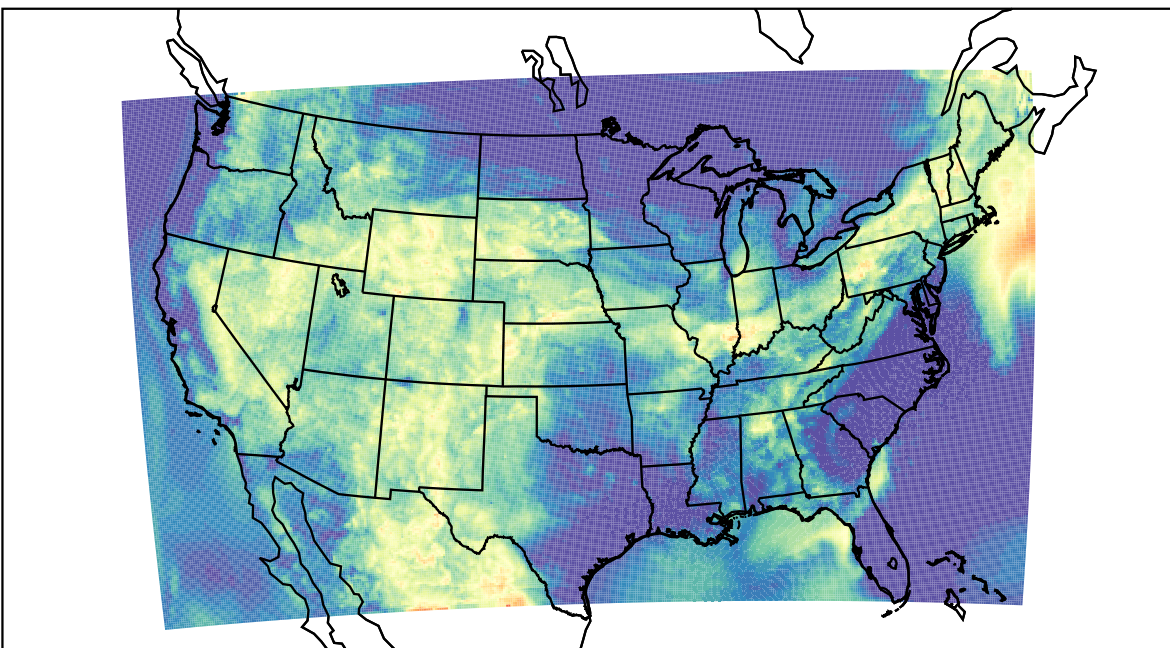
WRF (2022-07-02_08:00:00)
