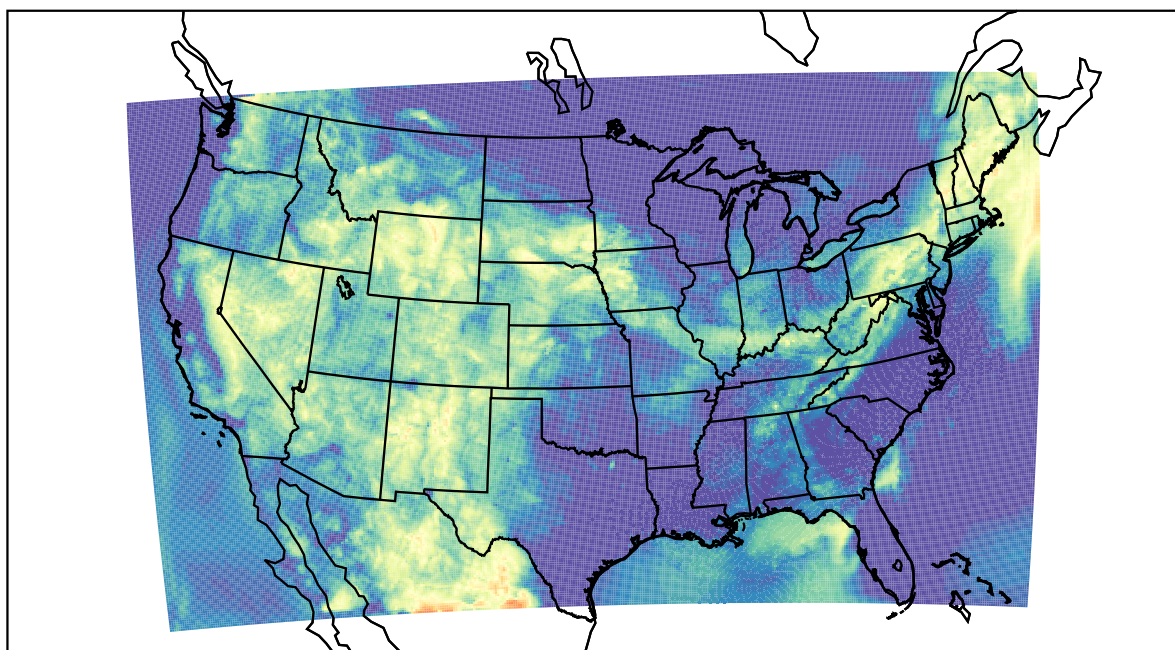
WRF (2022-07-02_12:00:00)
