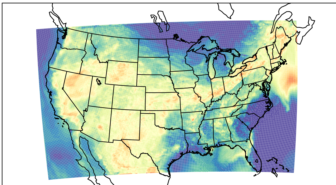
WRF (2022-07-02_02:00:00)
