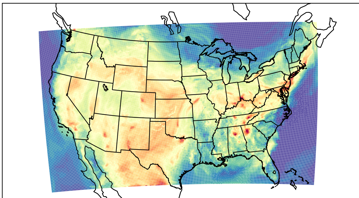
WRF (2022-07-02_22:00:00)
