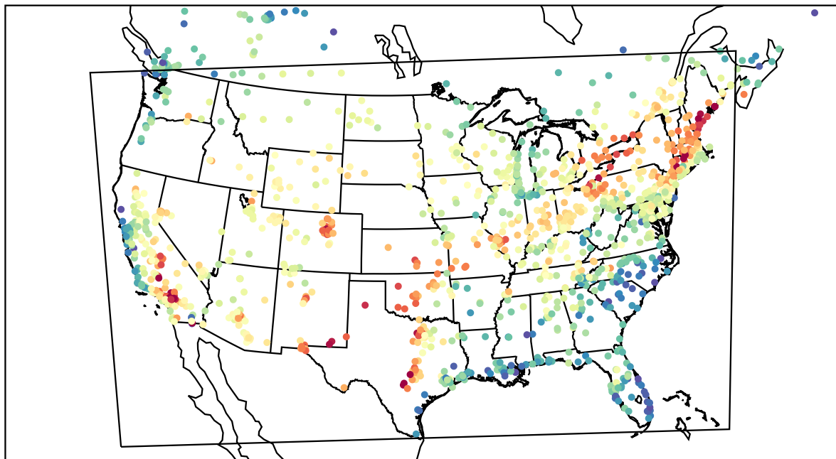
AirNOW (2022-07-01_21:00:00)
