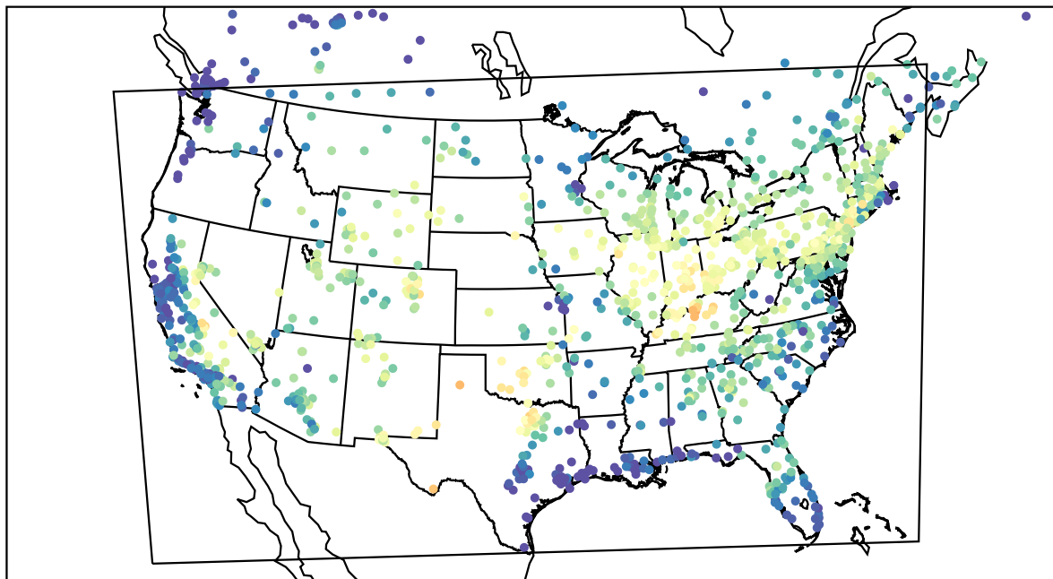
AirNOW (2022-07-02_15:00:00)
