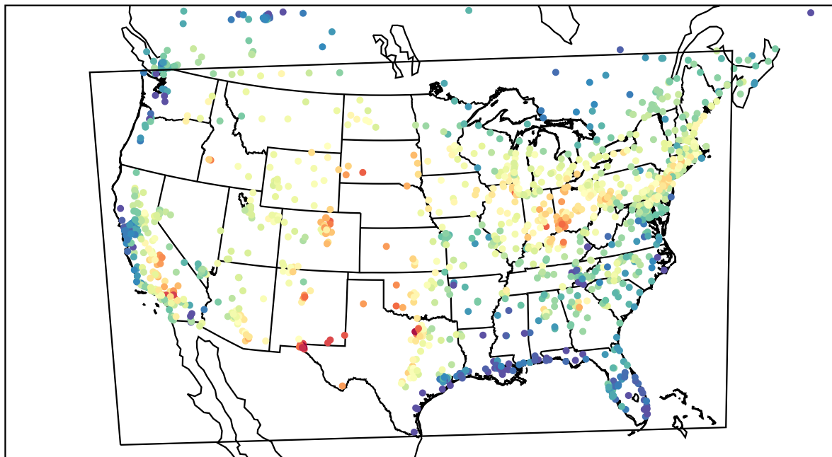
AirNOW (2022-07-02_22:00:00)
