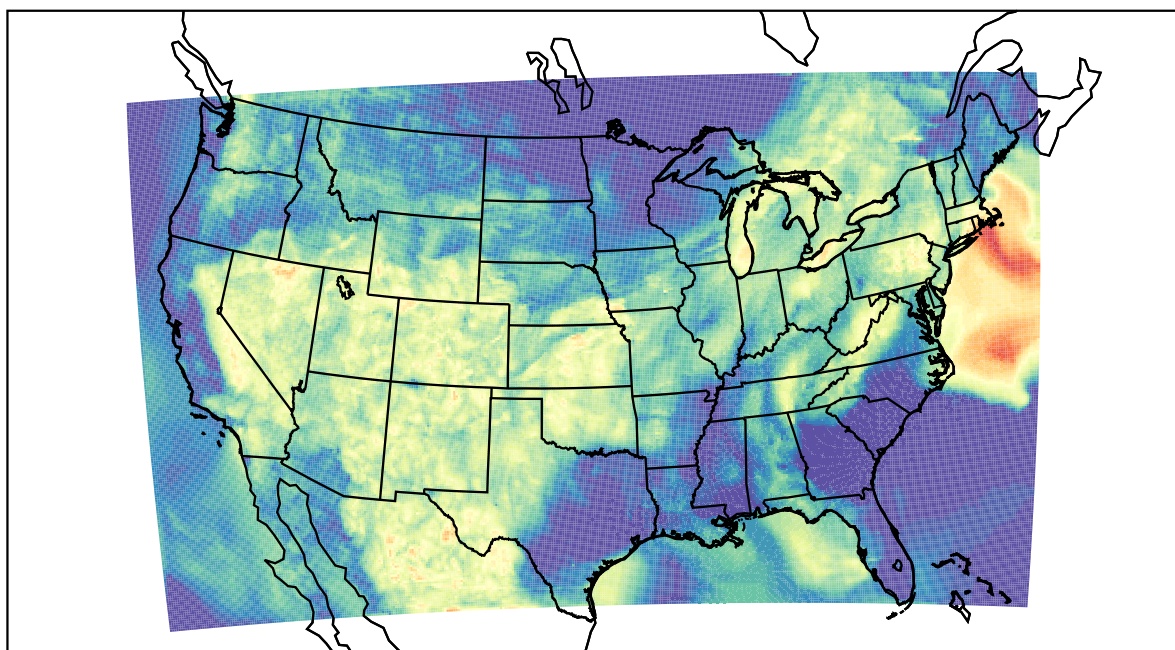
WRF (2022-07-01_07:00:00)
