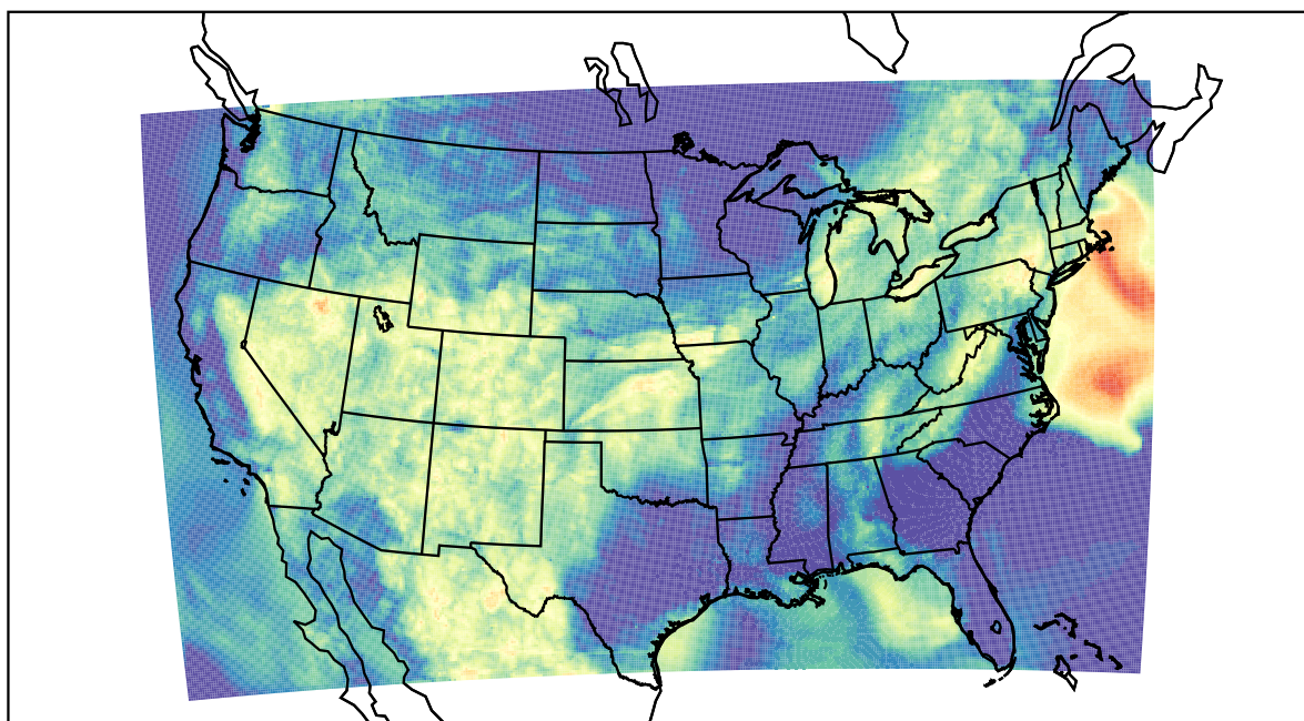
WRF (2022-07-01_09:00:00)
