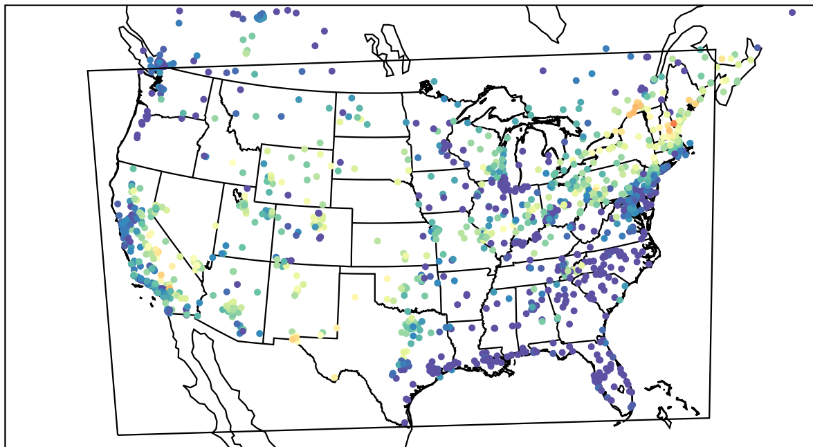
AirNOW (2022-07-02_05:00:00)
