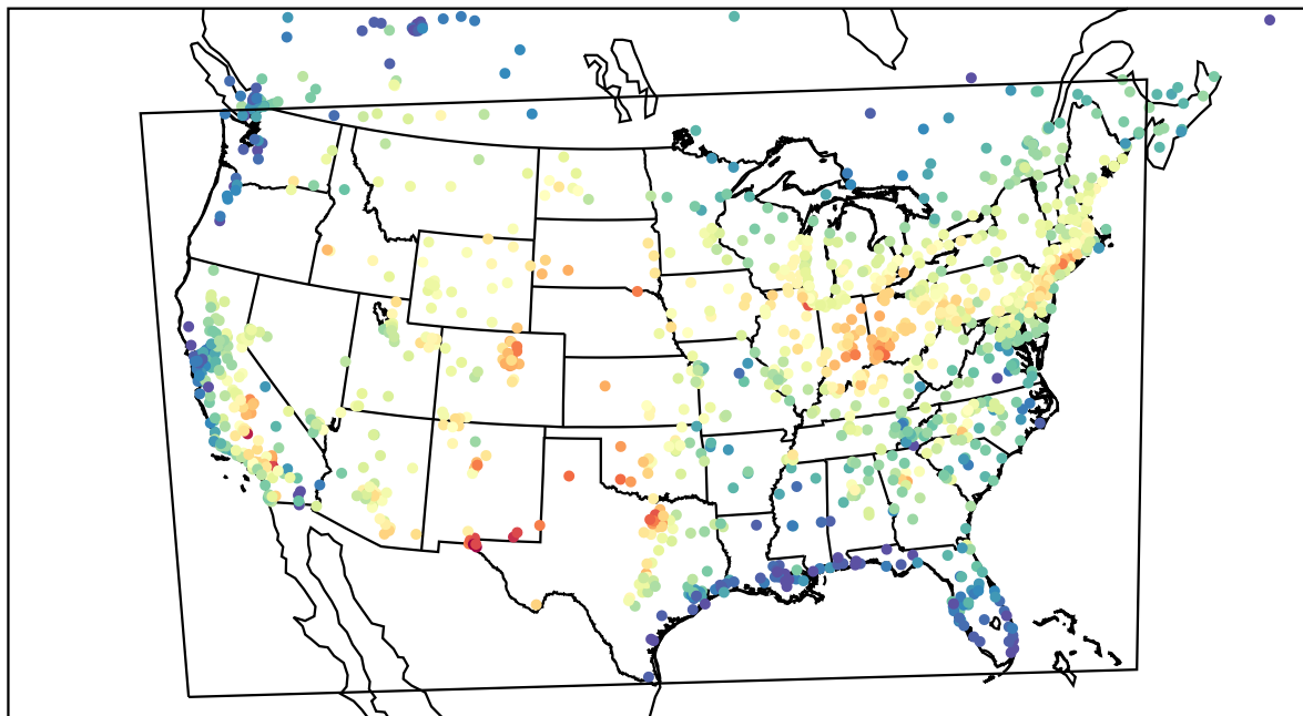
AirNOW (2022-07-02_20:00:00)
