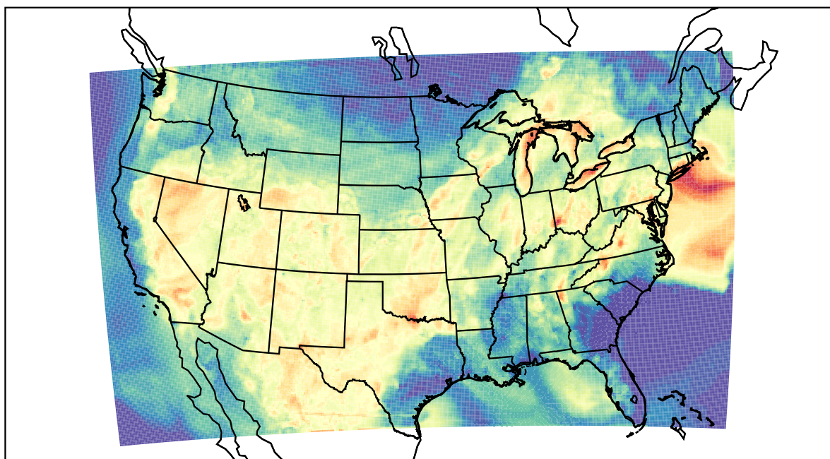
WRF (2022-07-01_02:00:00)
