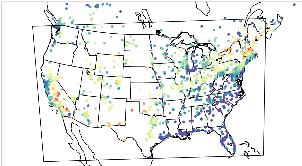
AirNOW (2022-07-02_02:00:00)
