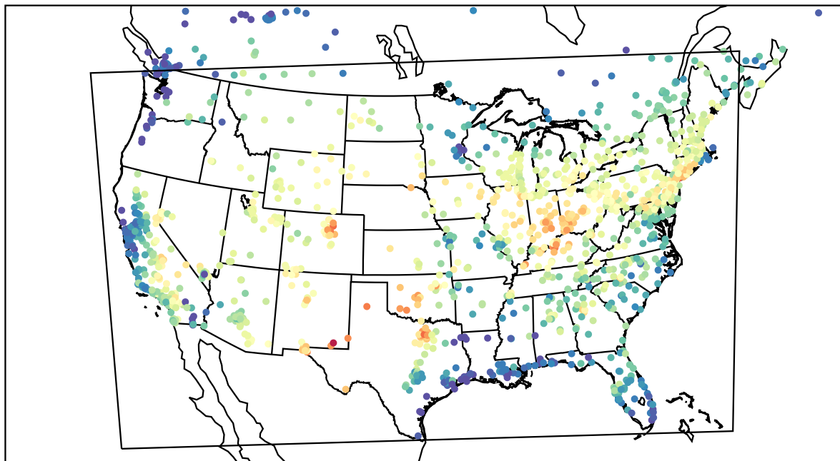
AirNOW (2022-07-02_17:00:00)
