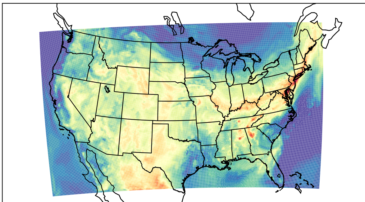
WRF (2022-07-02_16:00:00)
