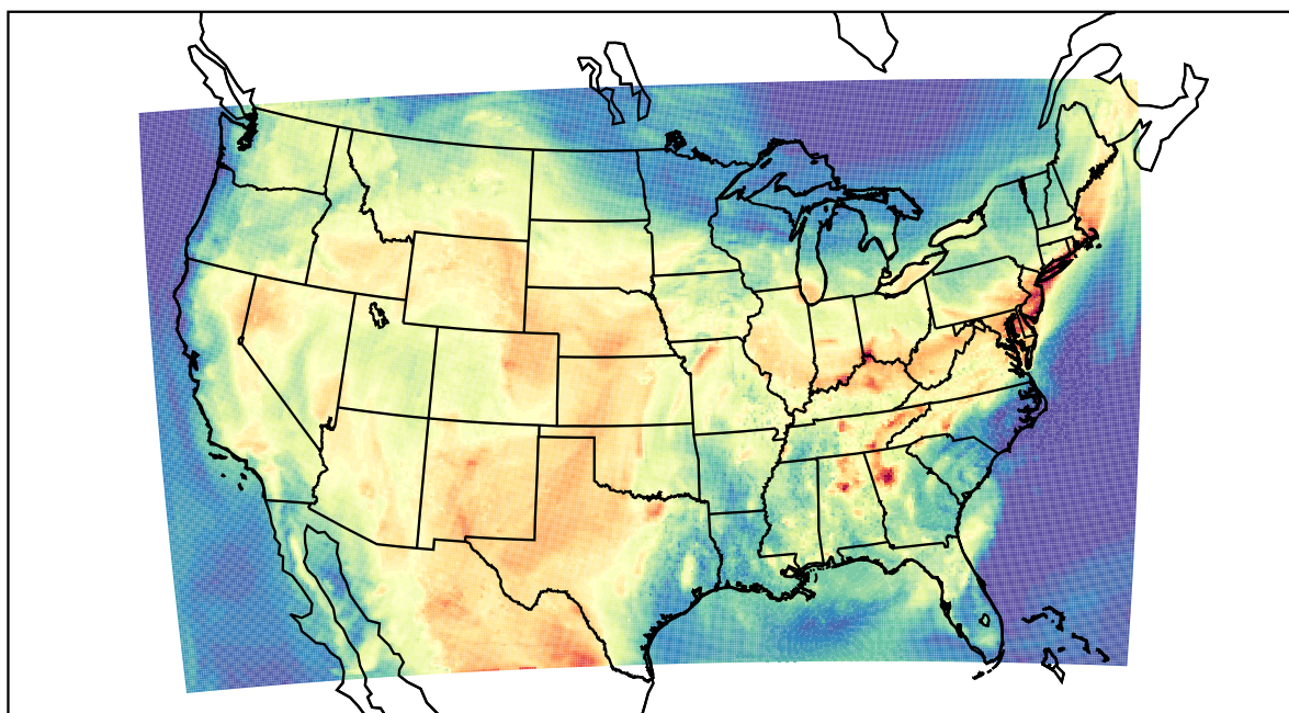
WRF (2022-07-02_19:00:00)
