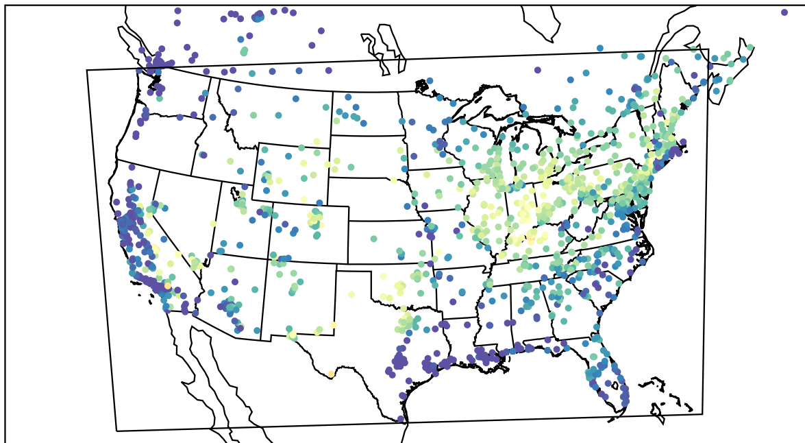
AirNOW (2022-07-02_14:00:00)
