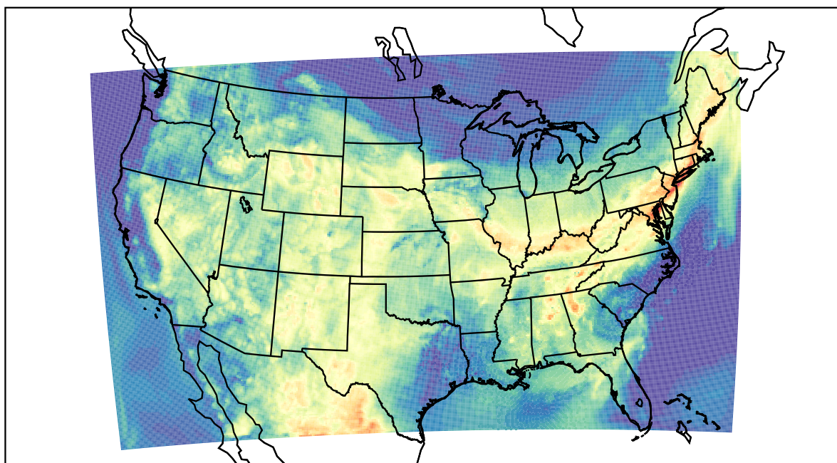
WRF (2022-07-02_15:00:00)
