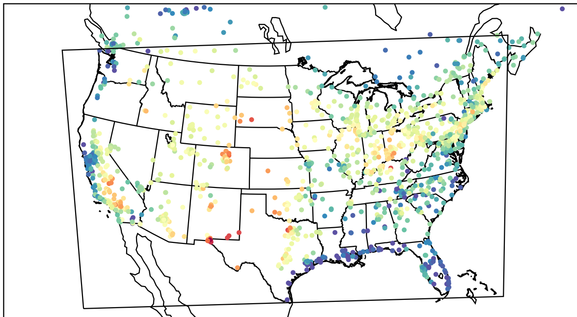
AirNOW (2022-07-02_23:00:00)
