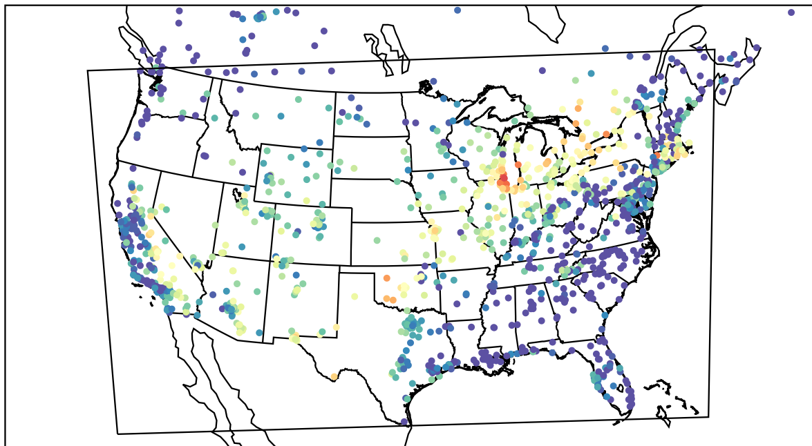
AirNOW (2022-07-01_07:00:00)
