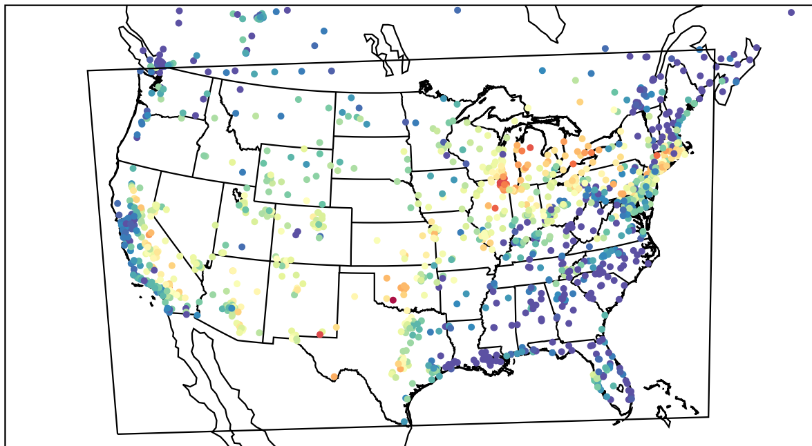
AirNOW (2022-07-01_04:00:00)
