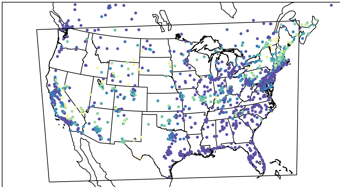
AirNOW (2022-07-02_10:00:00)
