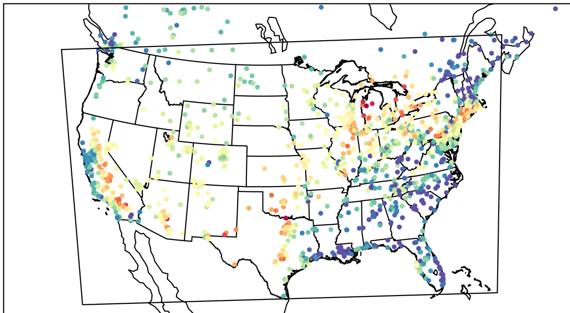
AirNOW (2022-07-01_02:00:00)
