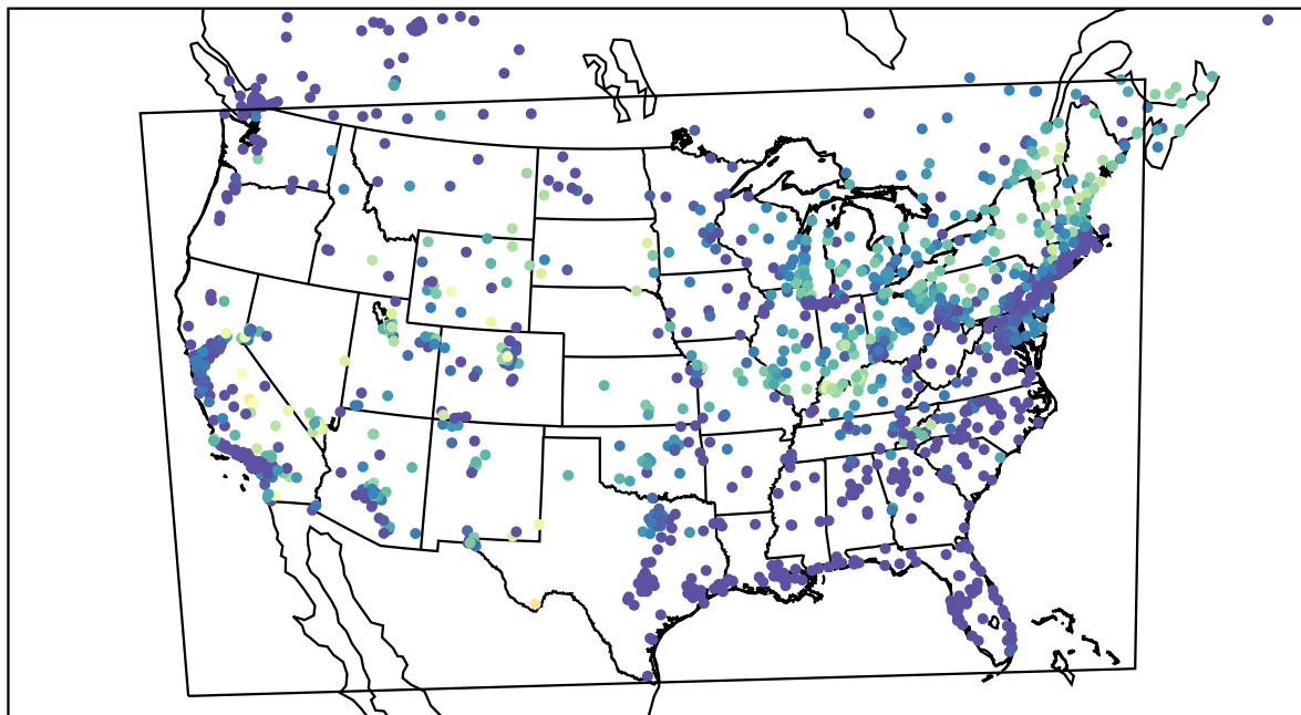
AirNOW (2022-07-02_12:00:00)
