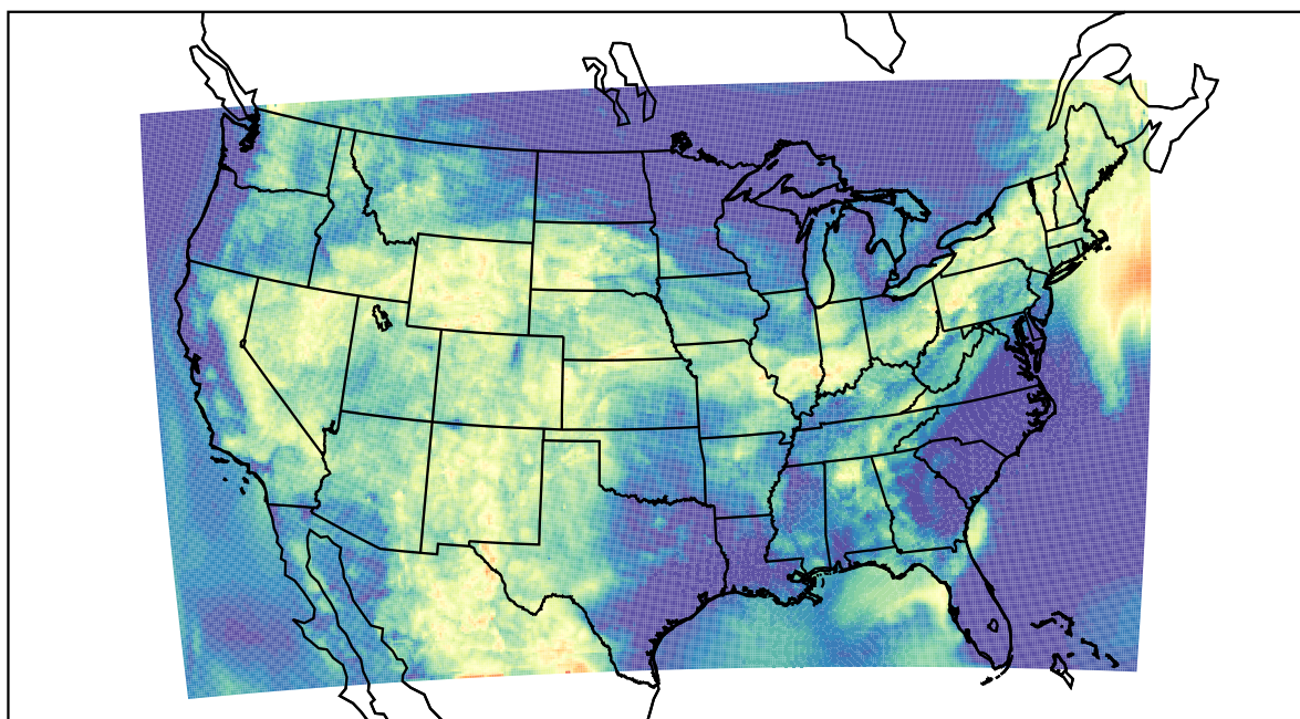
WRF (2022-07-02_07:00:00)
