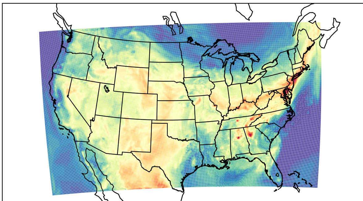
WRF (2022-07-02_17:00:00)
