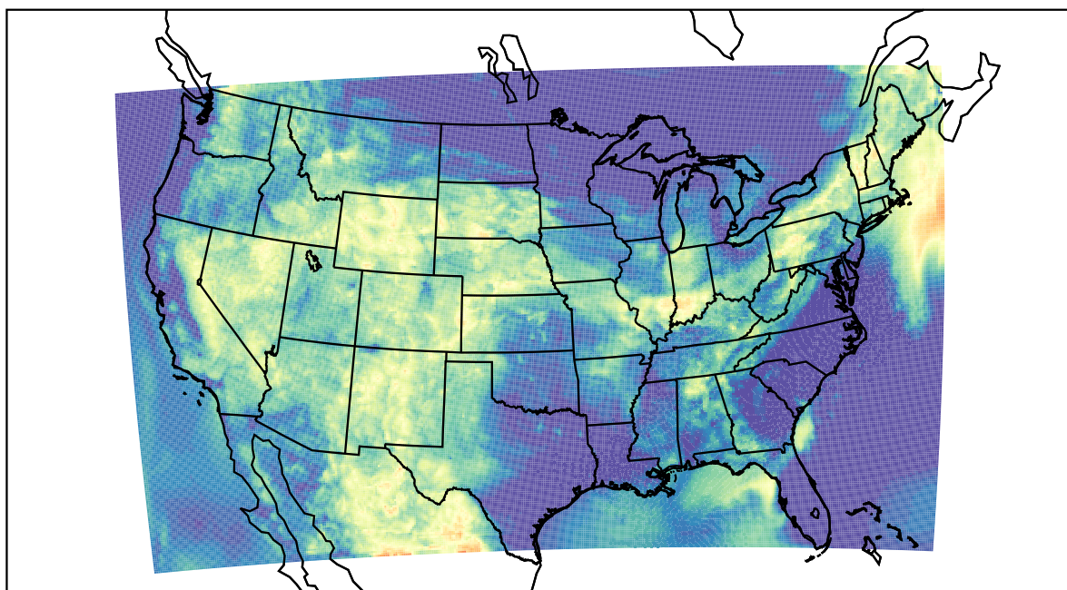
WRF (2022-07-02_09:00:00)
