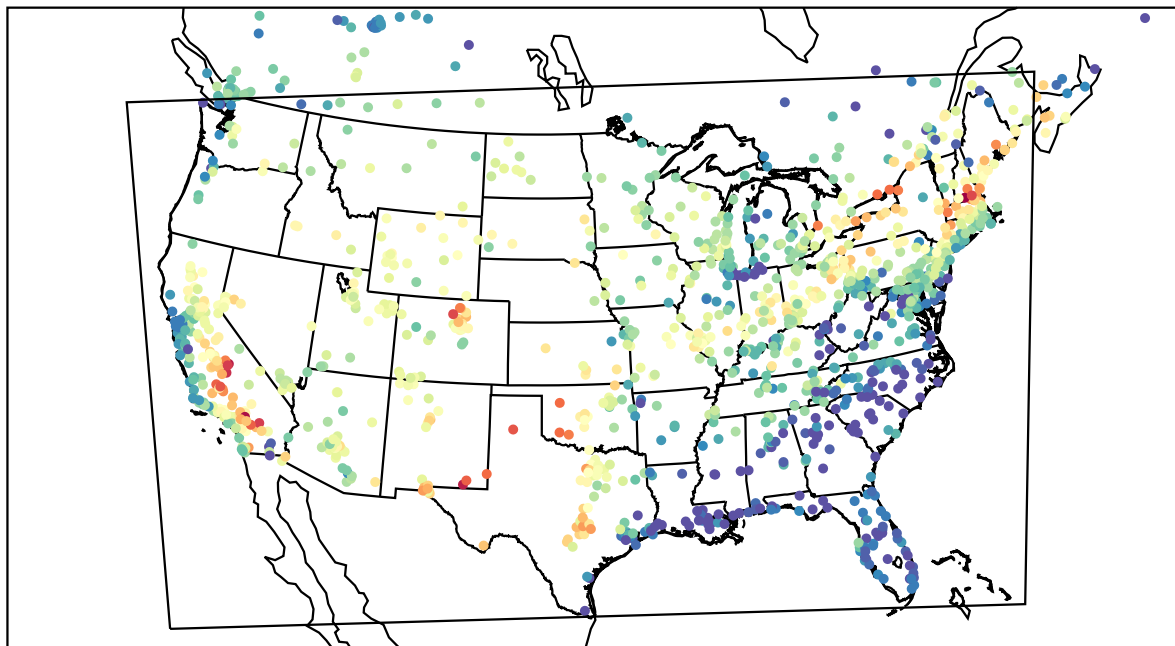
AirNOW (2022-07-02_01:00:00)
