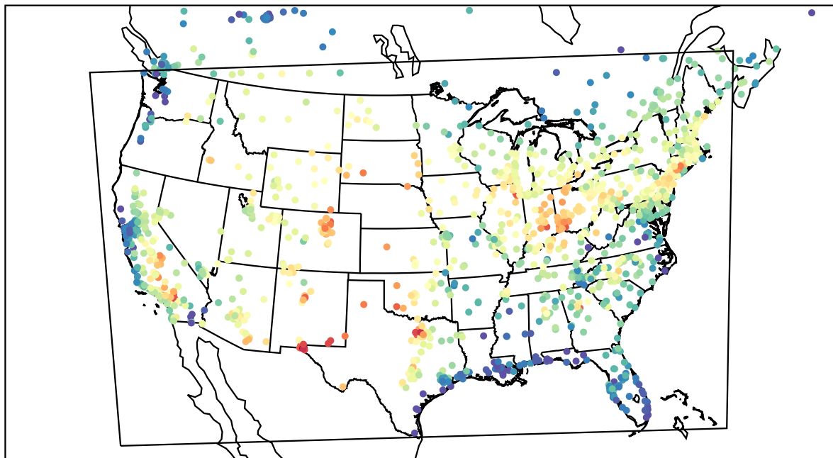
AirNOW (2022-07-02_21:00:00)
