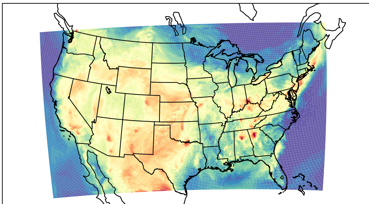
WRF (2022-07-02_23:00:00)
