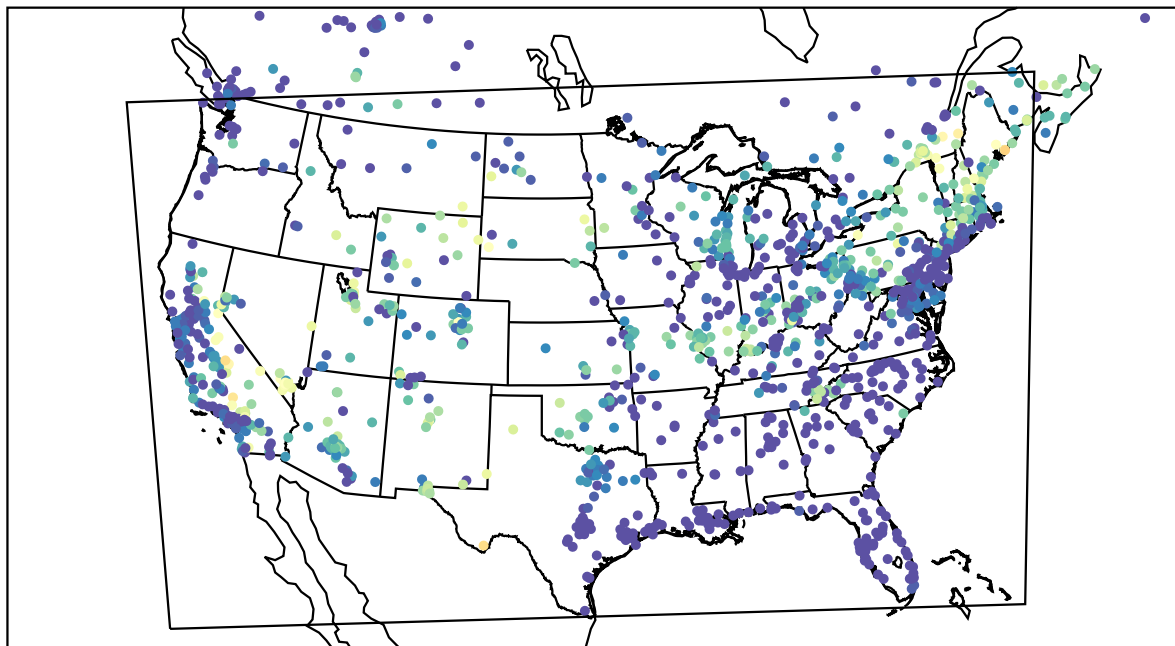
AirNOW (2022-07-02_09:00:00)
