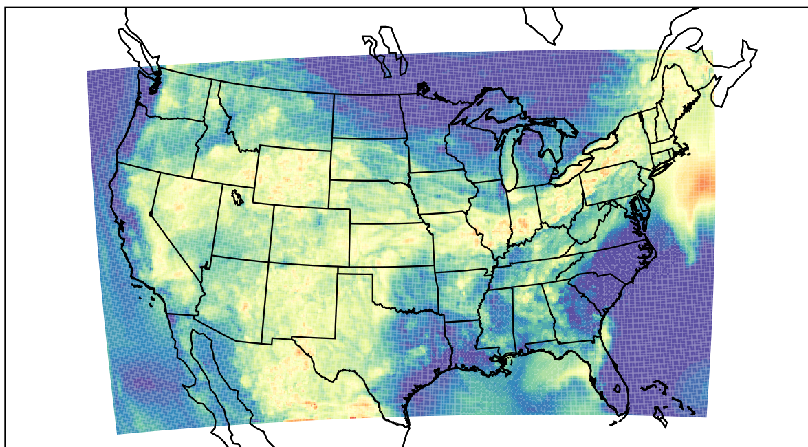
WRF (2022-07-02_04:00:00)
