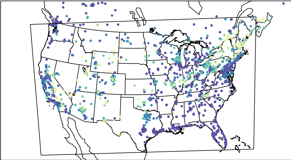
AirNOW (2022-07-02_08:00:00)
