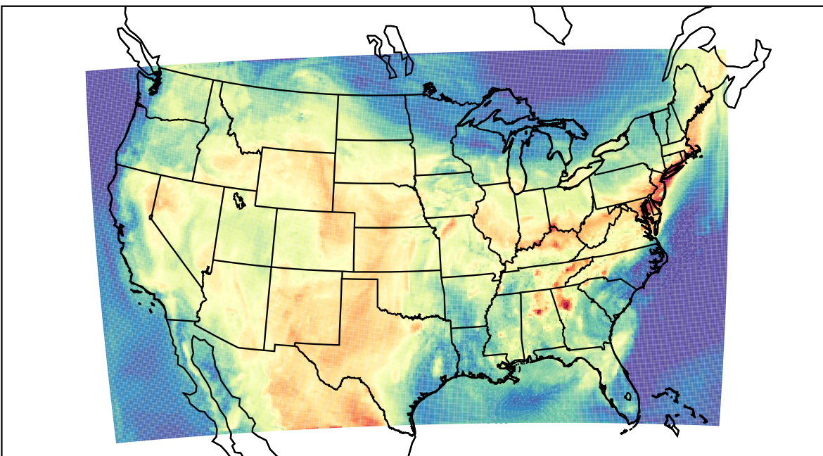
WRF (2022-07-02_18:00:00)
