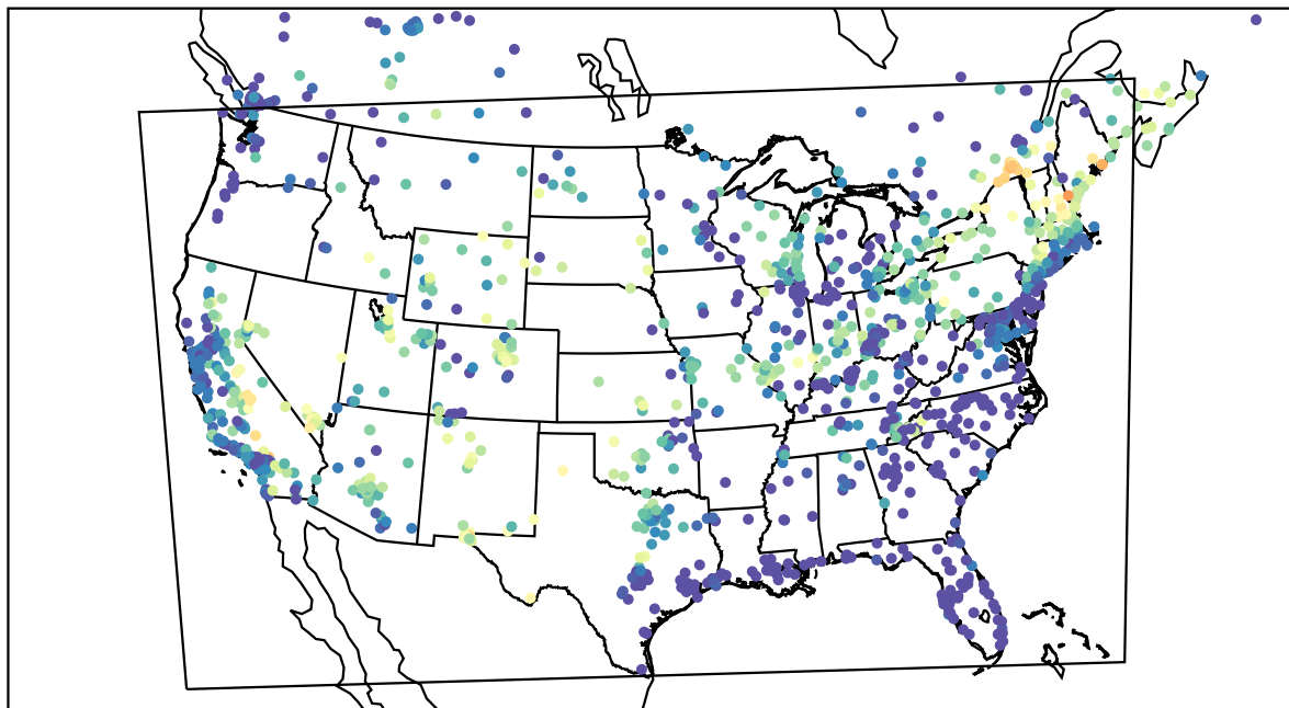
AirNOW (2022-07-02_06:00:00)
