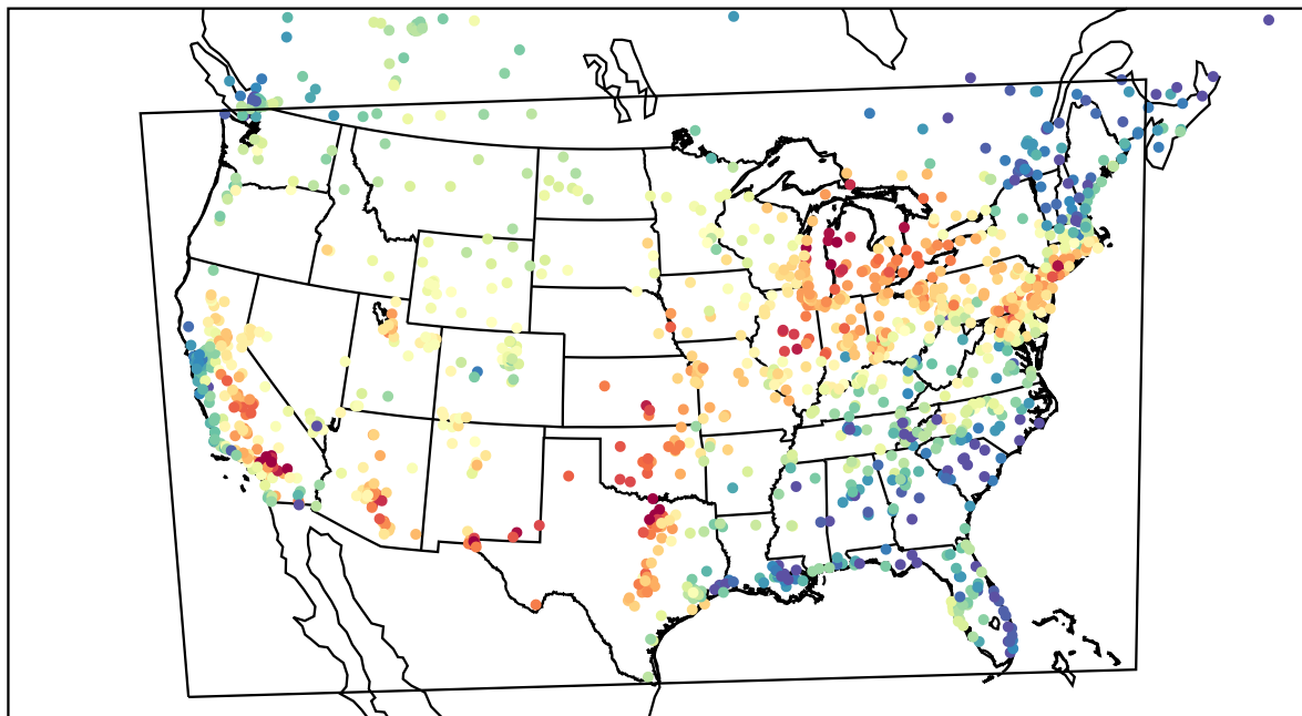
AirNOW (2022-07-01_00:00:00)
