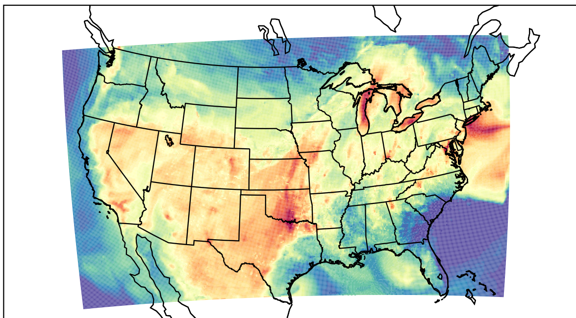
WRF (2022-07-01_00:00:00)
