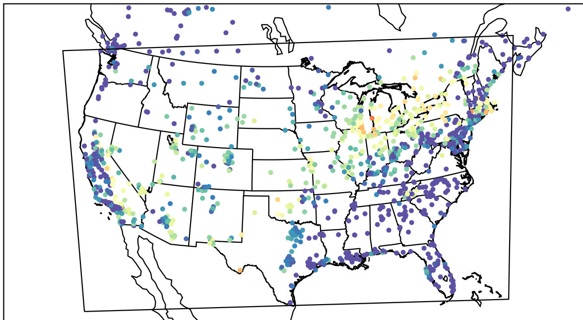
AirNOW (2022-07-01_09:00:00)
