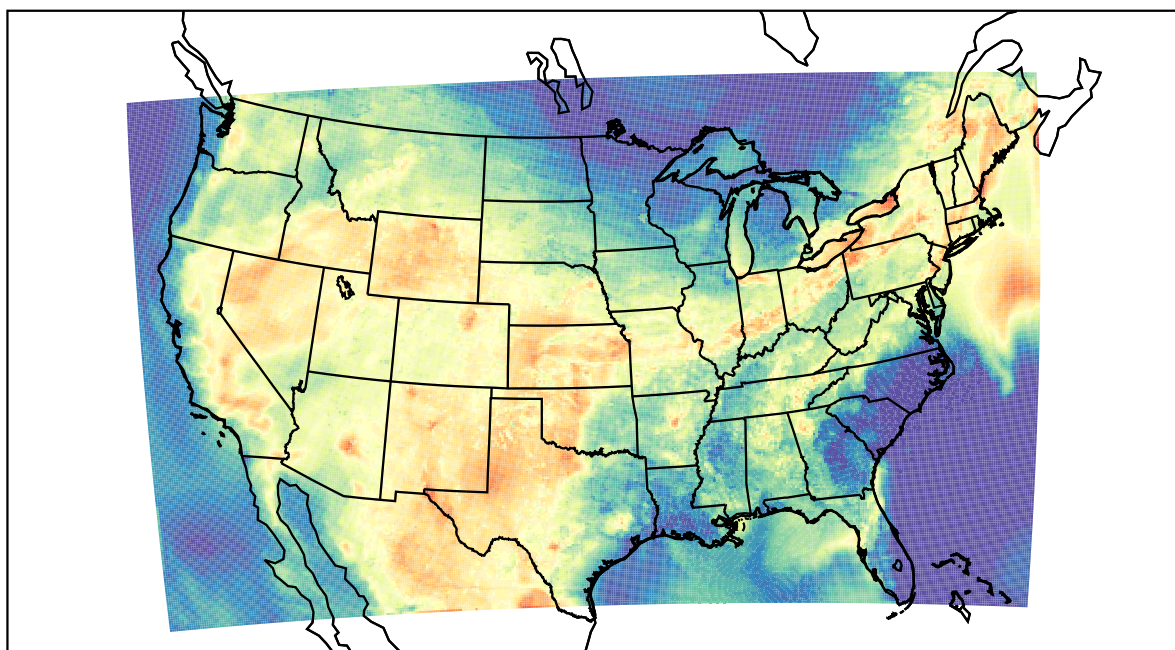
WRF (2022-07-02_01:00:00)
