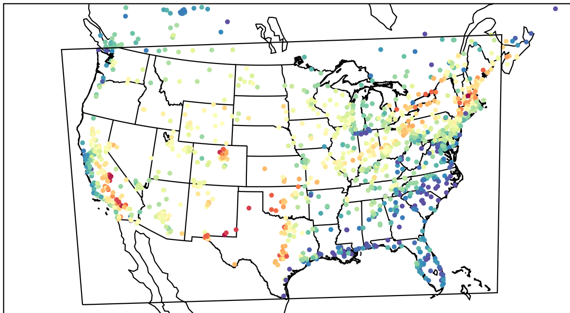
AirNOW (2022-07-02_00:00:00)
