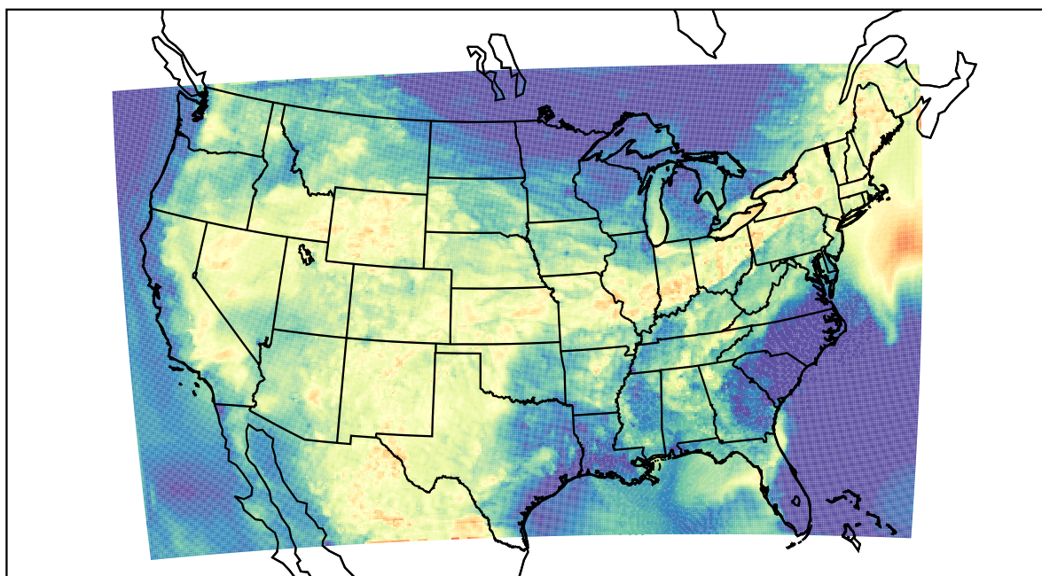
WRF (2022-07-02_03:00:00)
