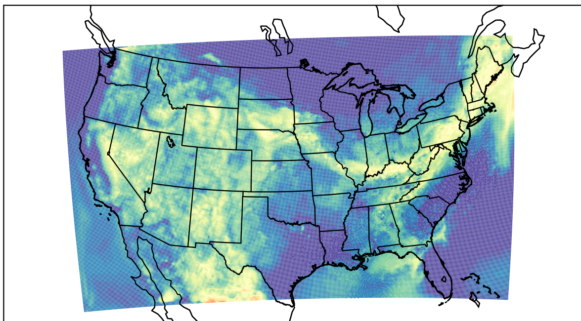
WRF (2022-07-02_13:00:00)
