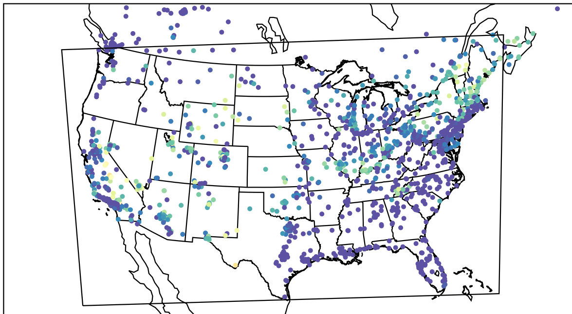
AirNOW (2022-07-02_11:00:00)
