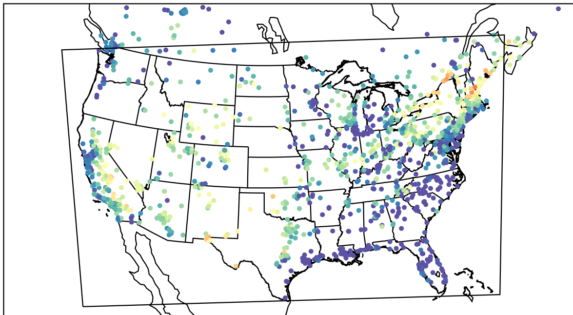
AirNOW (2022-07-02_04:00:00)
