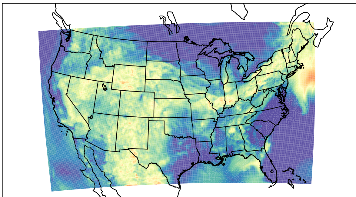
WRF (2022-07-02_06:00:00)
