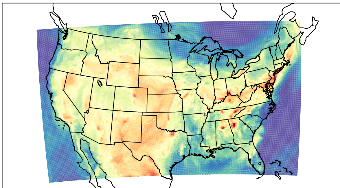
WRF (2022-07-02_21:00:00)
