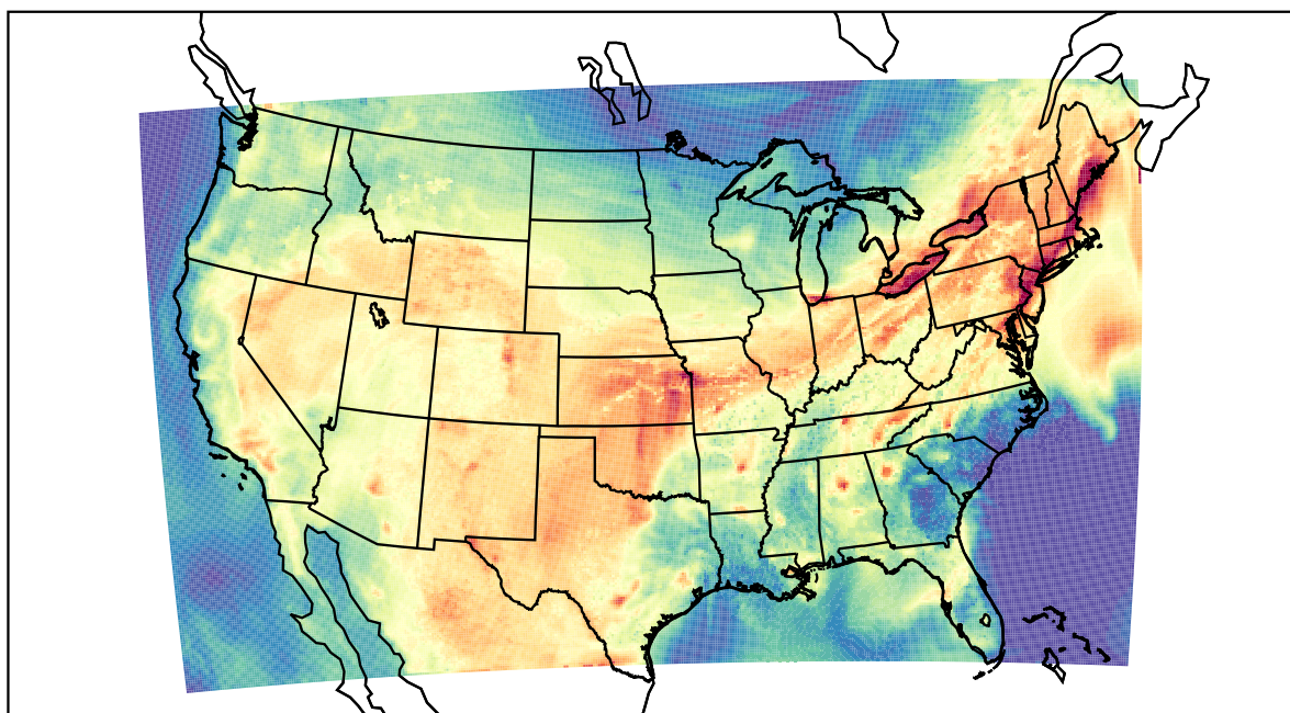
WRF (2022-07-01_21:00:00)
