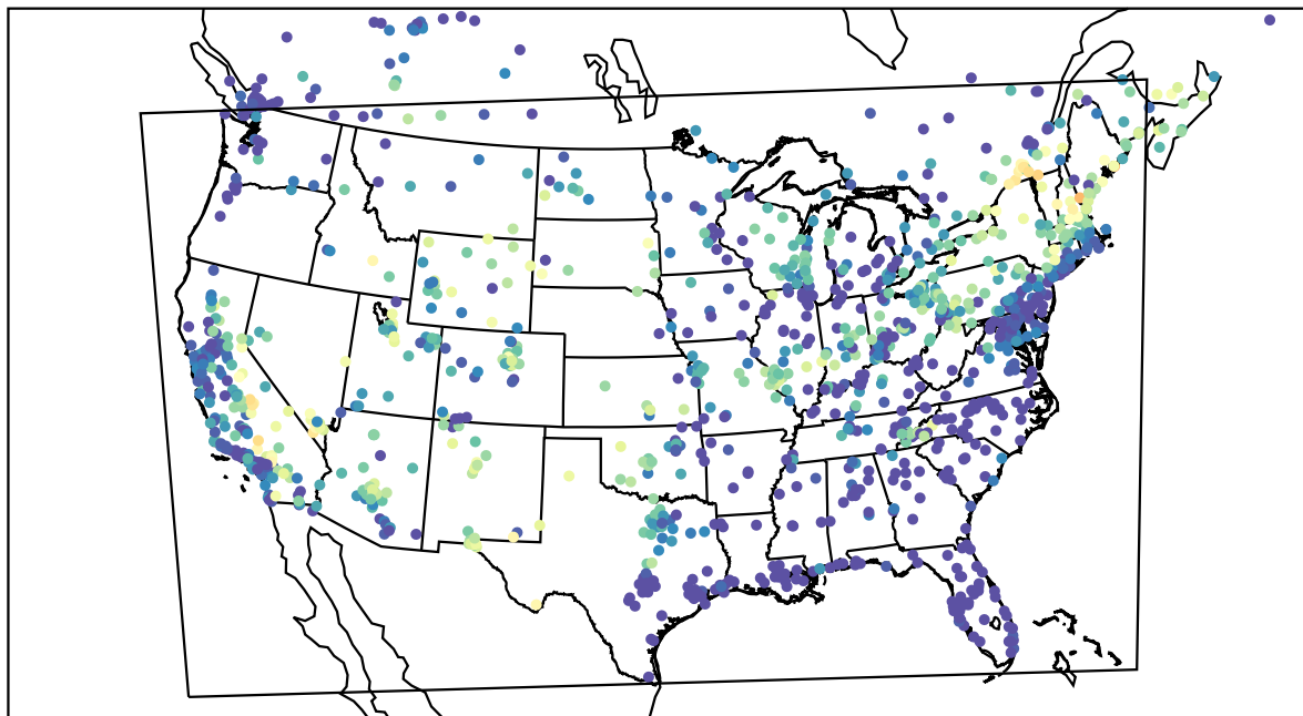
AirNOW (2022-07-02_07:00:00)
