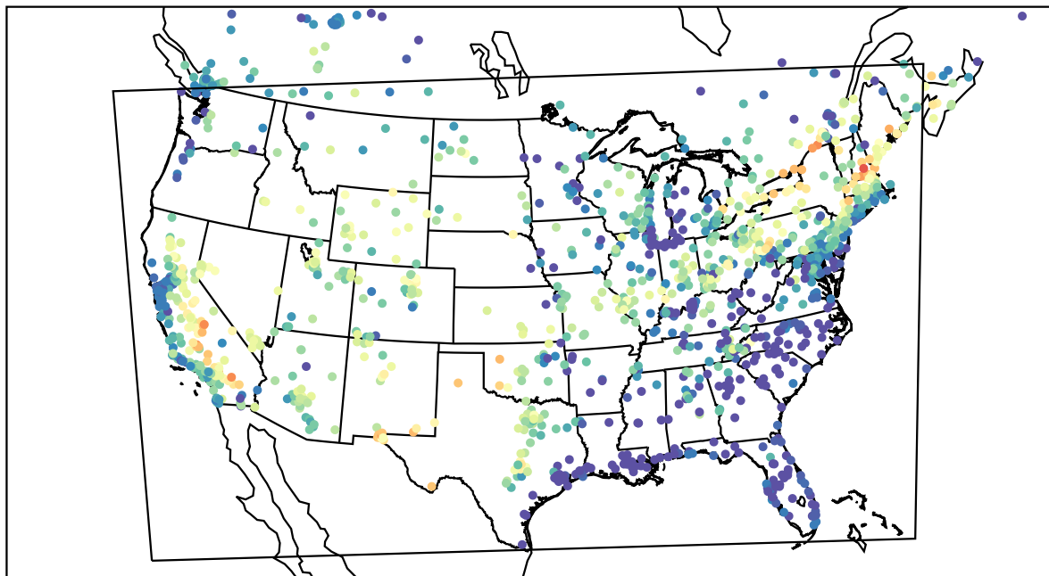
AirNOW (2022-07-02_03:00:00)
