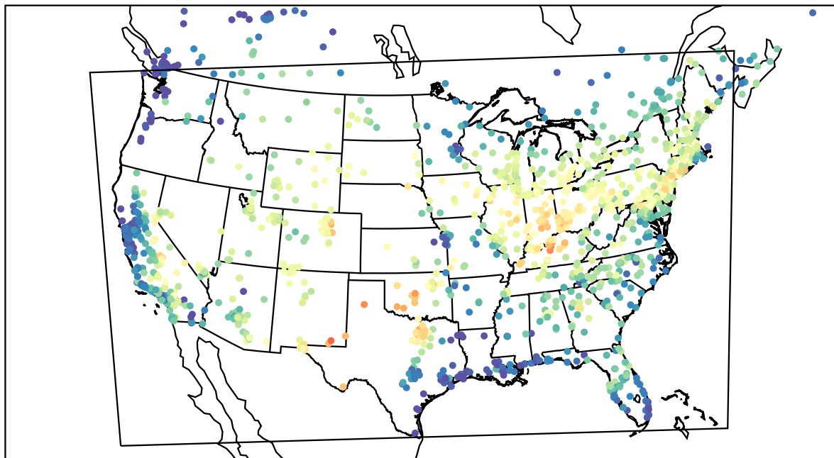
AirNOW (2022-07-02_16:00:00)
