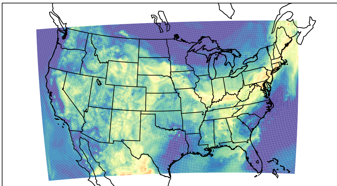
WRF (2022-07-02_14:00:00)
