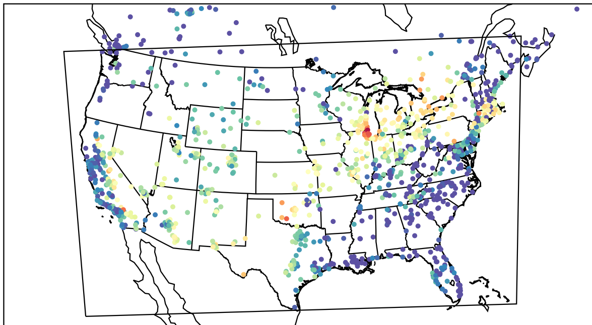
AirNOW (2022-07-01_06:00:00)
