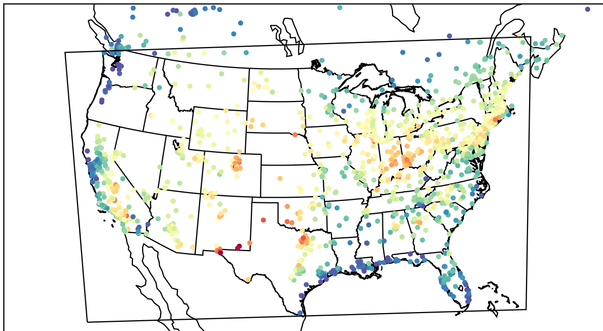
AirNOW (2022-07-02_19:00:00)
