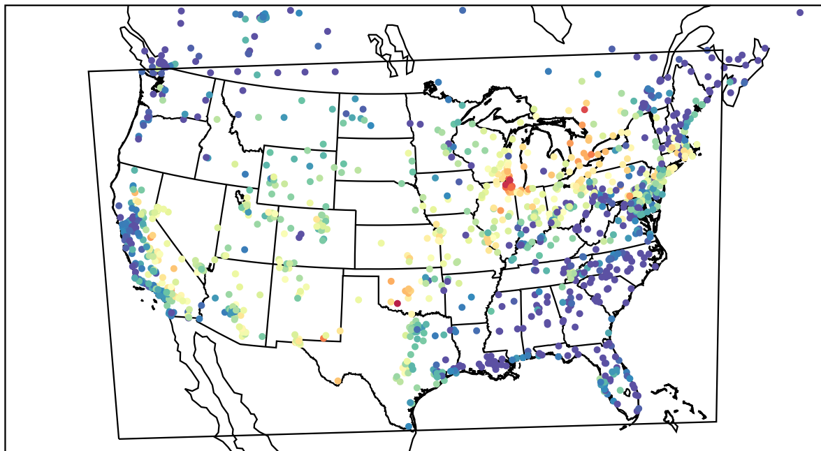
AirNOW (2022-07-01_05:00:00)
