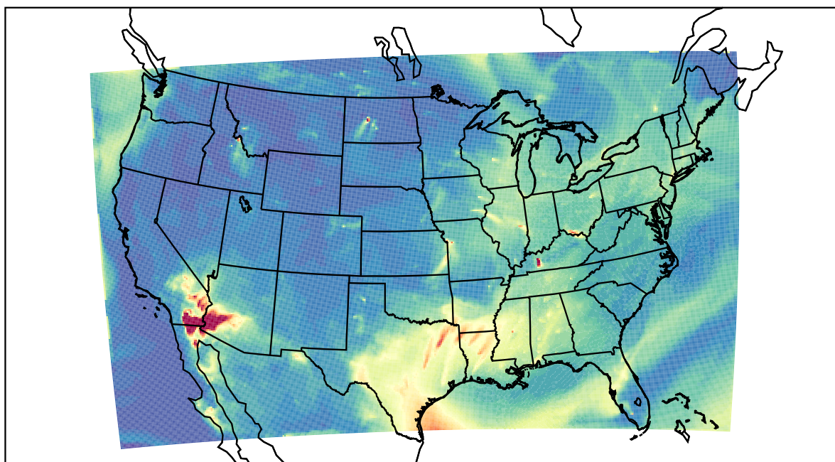
WRF 2022-07-21_09:00:00
