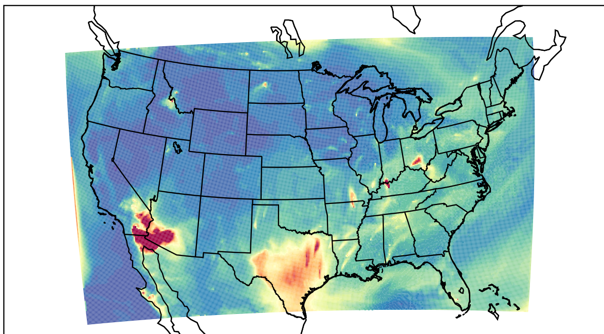
WRF 2022-07-22_09:00:00
