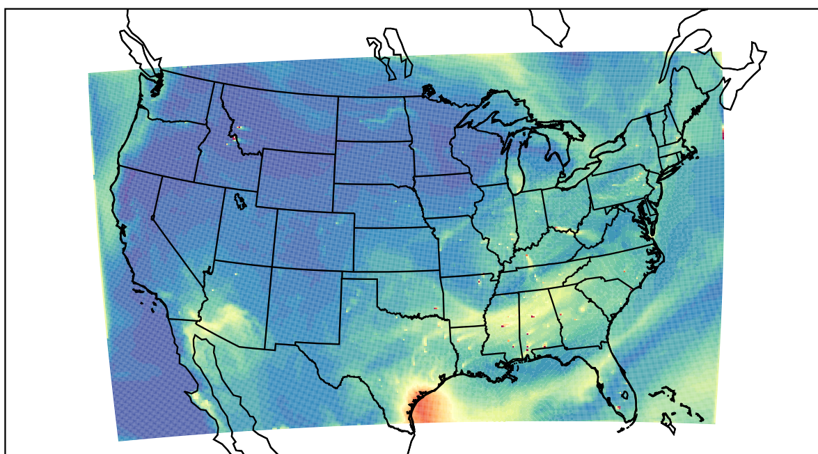
WRF 2022-07-21_21:00:00
