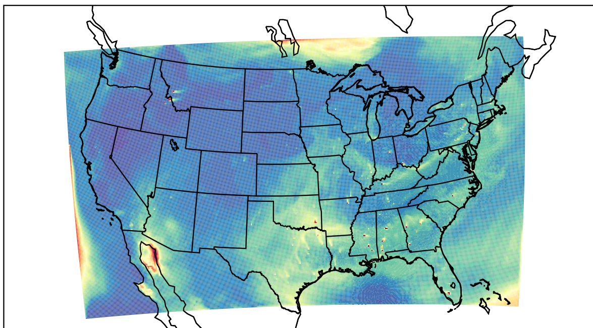
WRF 2022-07-22_22:00:00
