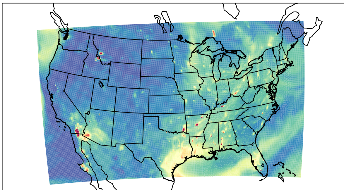
WRF 2022-07-21_02:00:00
