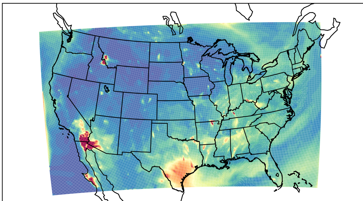
WRF 2022-07-22_04:00:00
