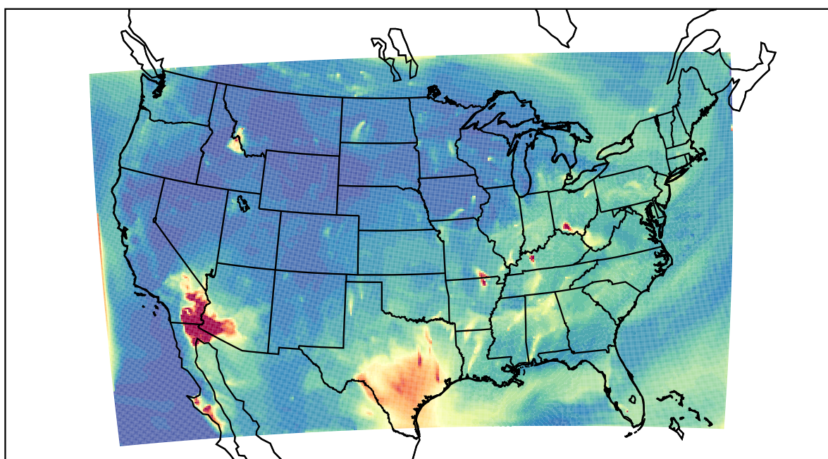
WRF 2022-07-22_06:00:00
