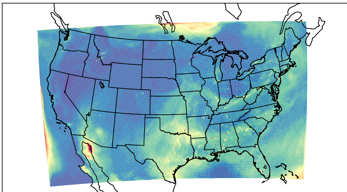
WRF 2022-07-22_21:00:00
