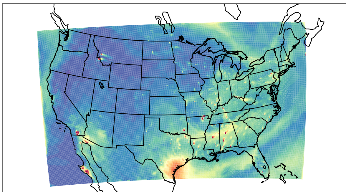
WRF 2022-07-22_01:00:00
