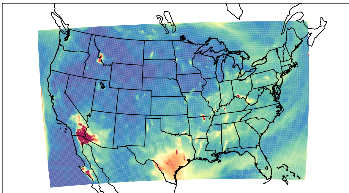
WRF 2022-07-22_05:00:00
