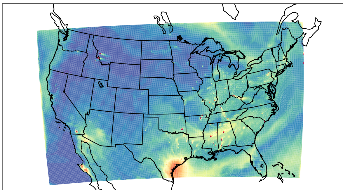
WRF 2022-07-22_00:00:00
