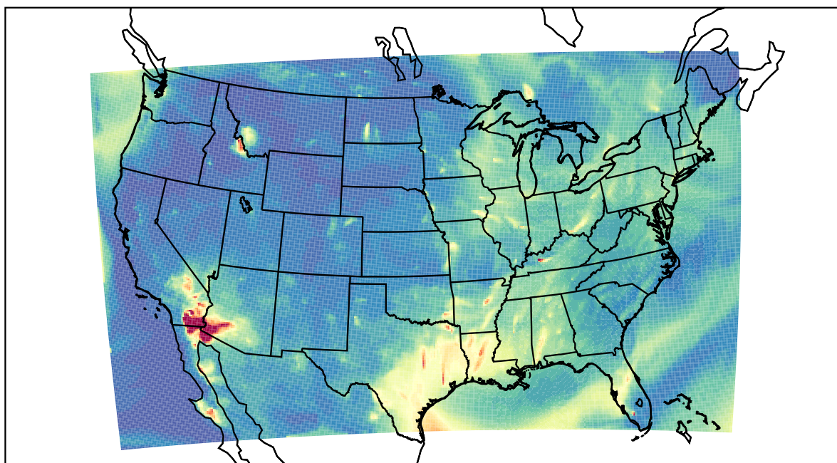
WRF 2022-07-21_05:00:00
