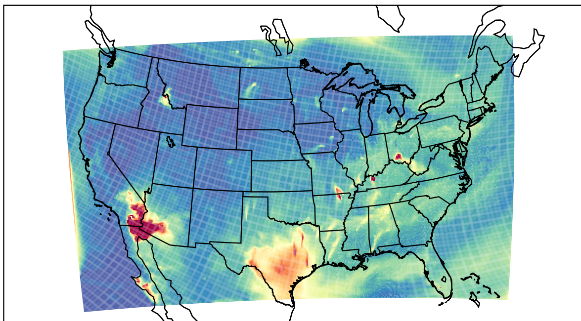
WRF 2022-07-22_07:00:00
