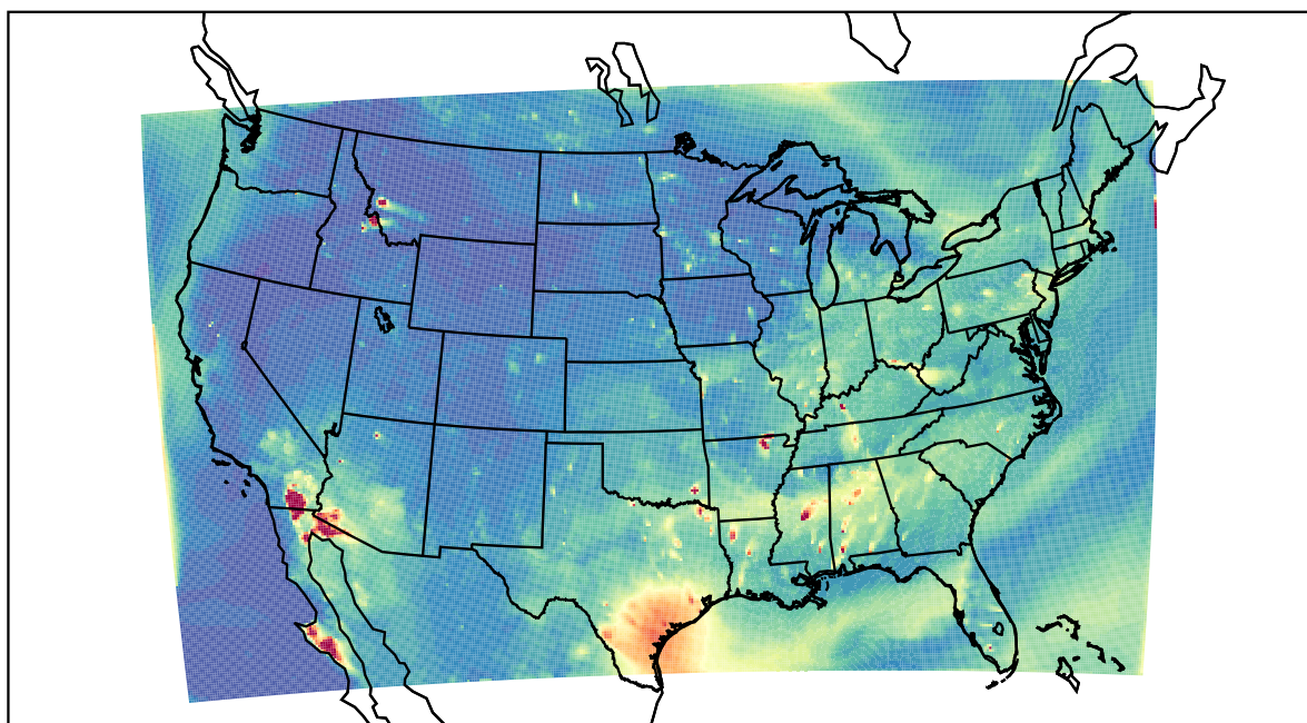
WRF 2022-07-22_02:00:00
