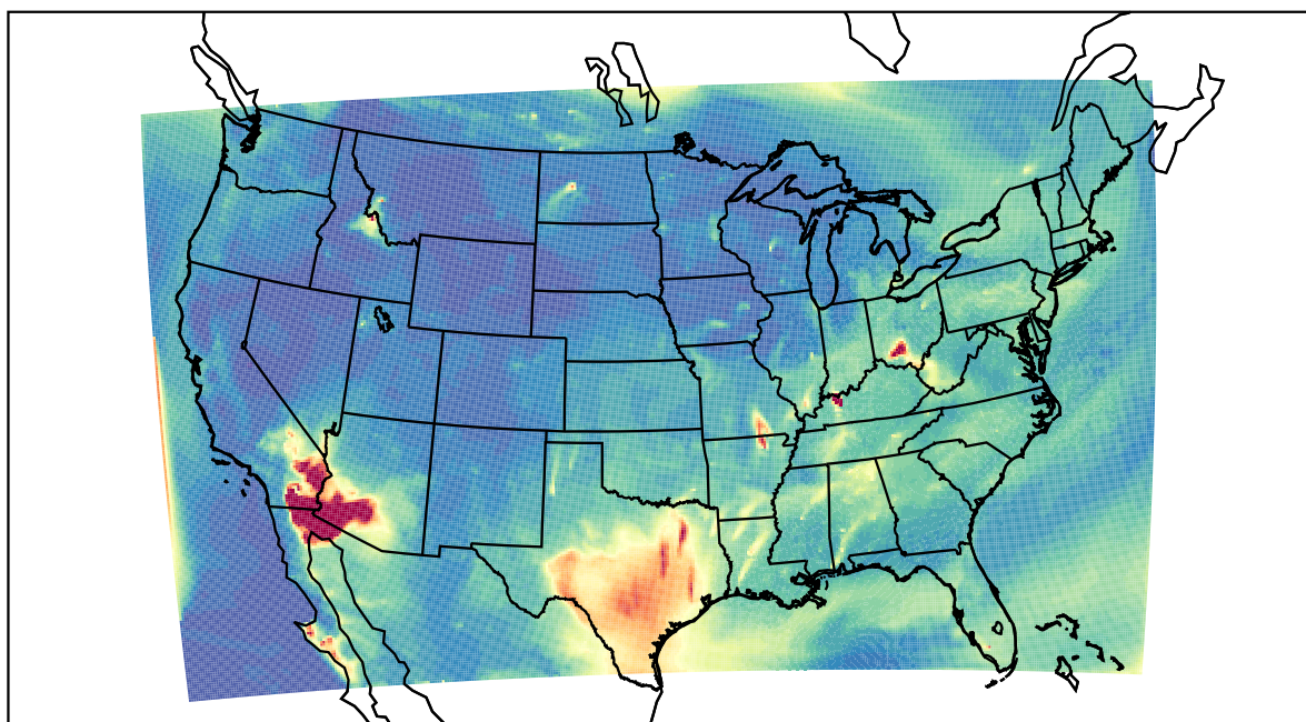
WRF 2022-07-22_08:00:00
