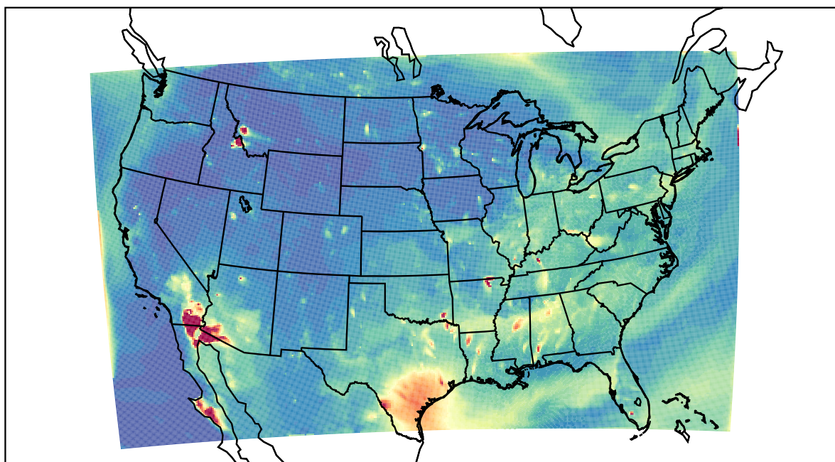
WRF 2022-07-22_03:00:00
