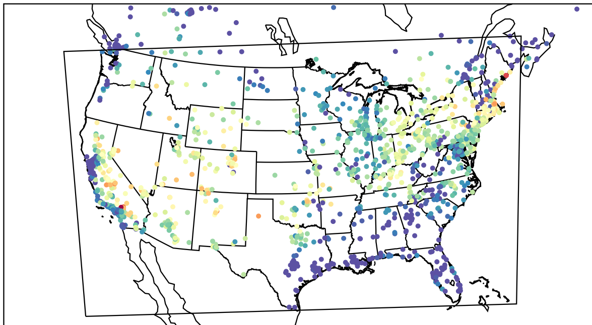
AirNOW (2022-07-21_04:00:00)
