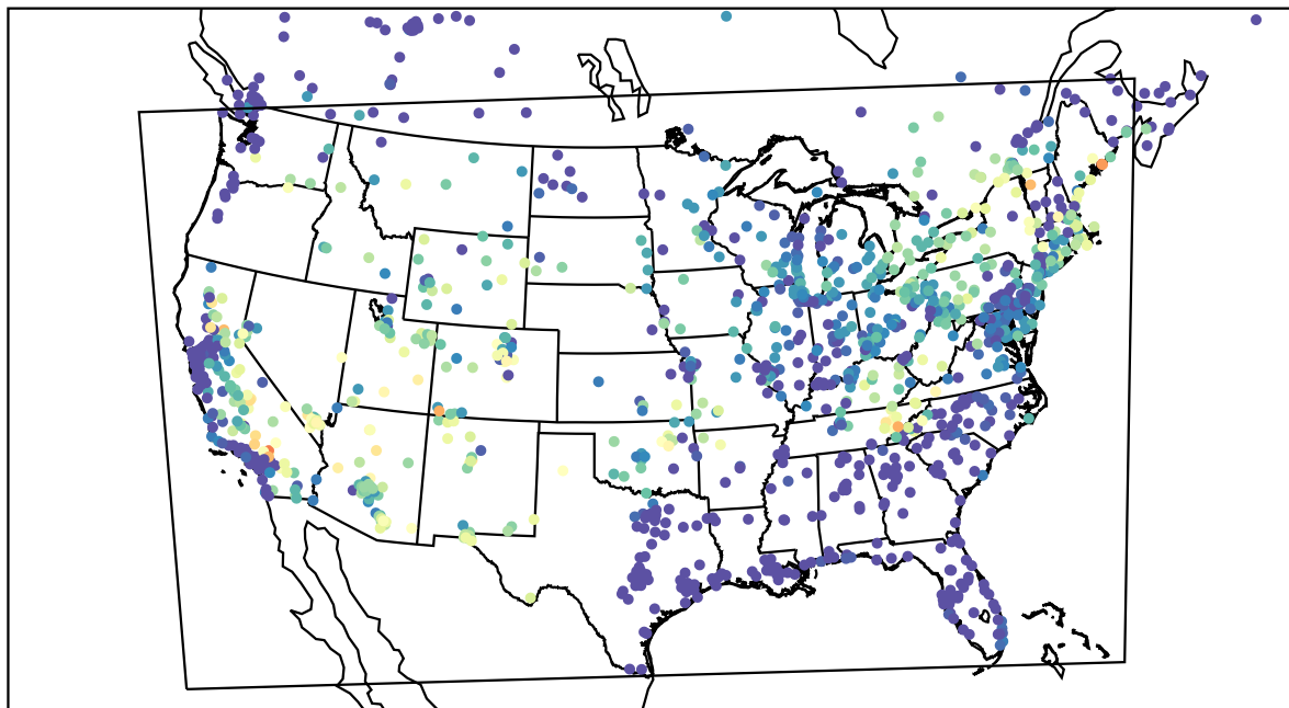
AirNOW (2022-07-21_09:00:00)
