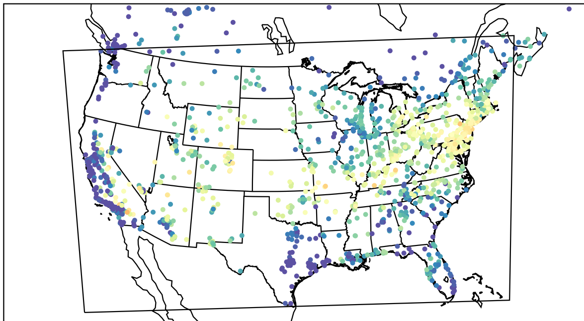
AirNOW (2022-07-22_14:00:00)
