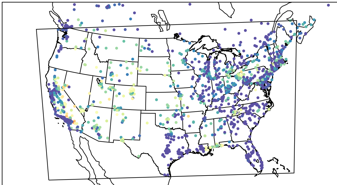
AirNOW (2022-07-22_09:00:00)
