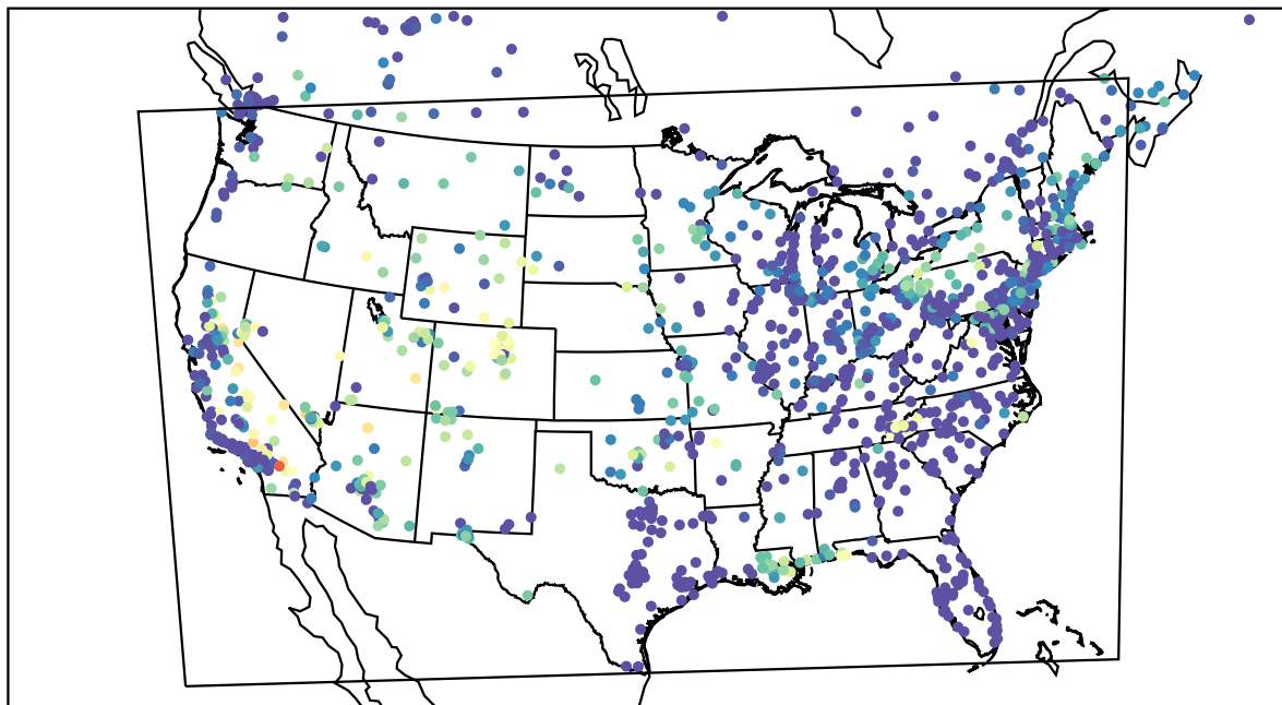
AirNOW (2022-07-22_11:00:00)
