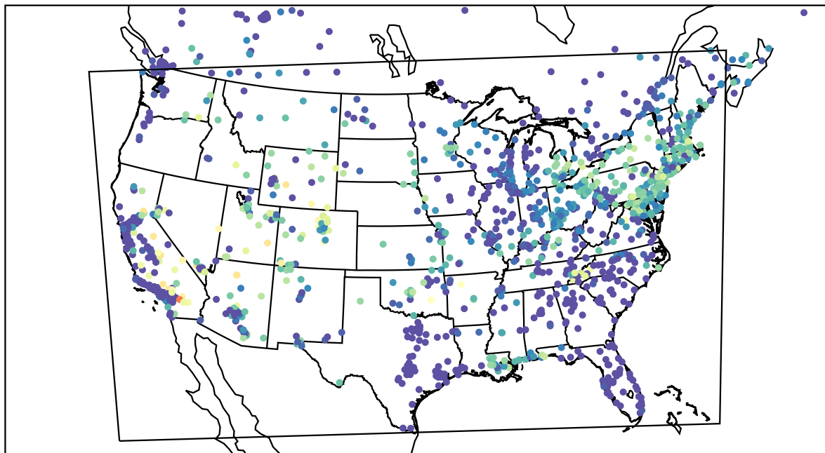
AirNOW (2022-07-22_12:00:00)
