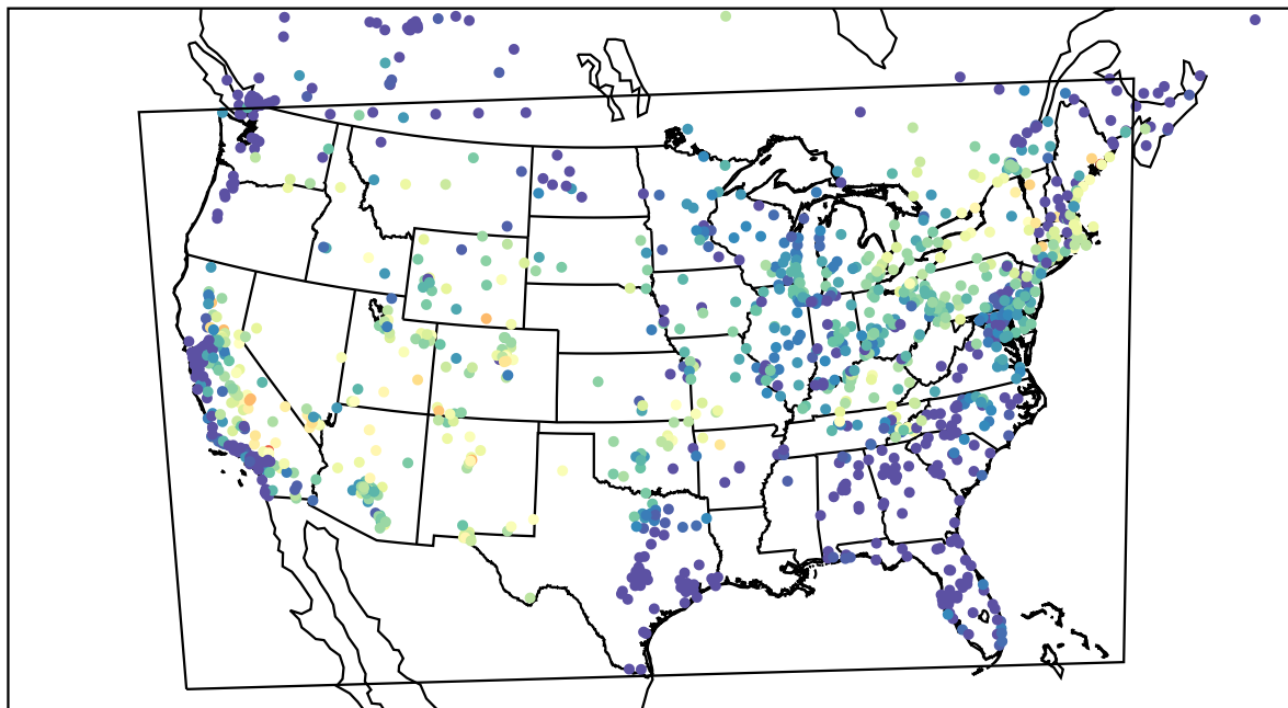
AirNOW (2022-07-21_07:00:00)
