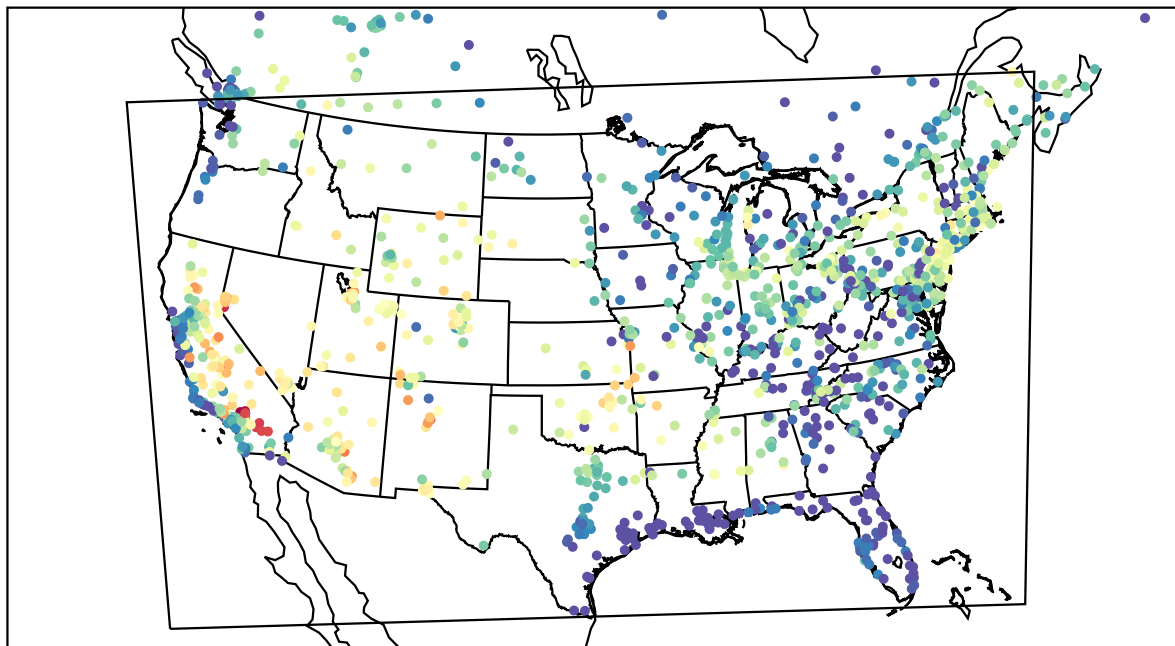
AirNOW (2022-07-22_03:00:00)
