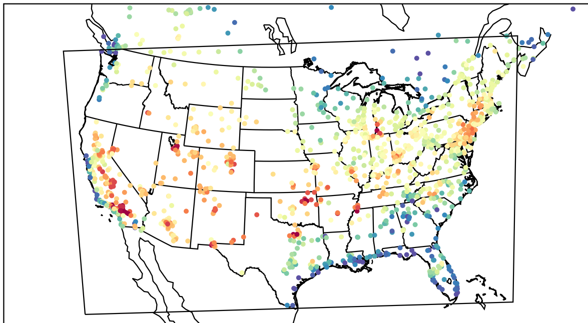
AirNOW (2022-07-21_21:00:00)
