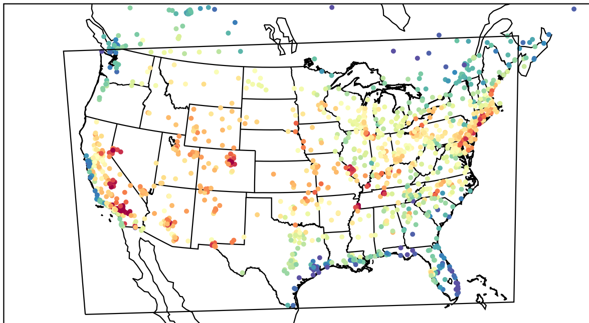
AirNOW (2022-07-22_22:00:00)
