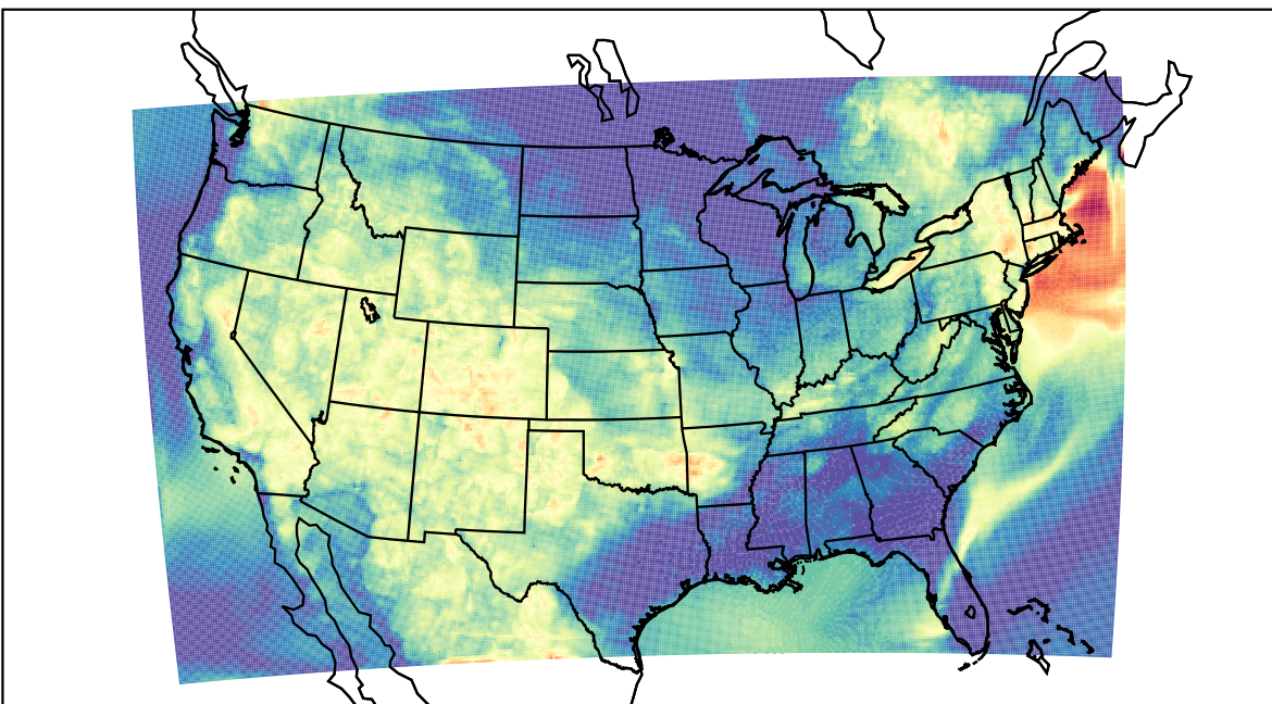
WRF (2022-07-21_06:00:00)
