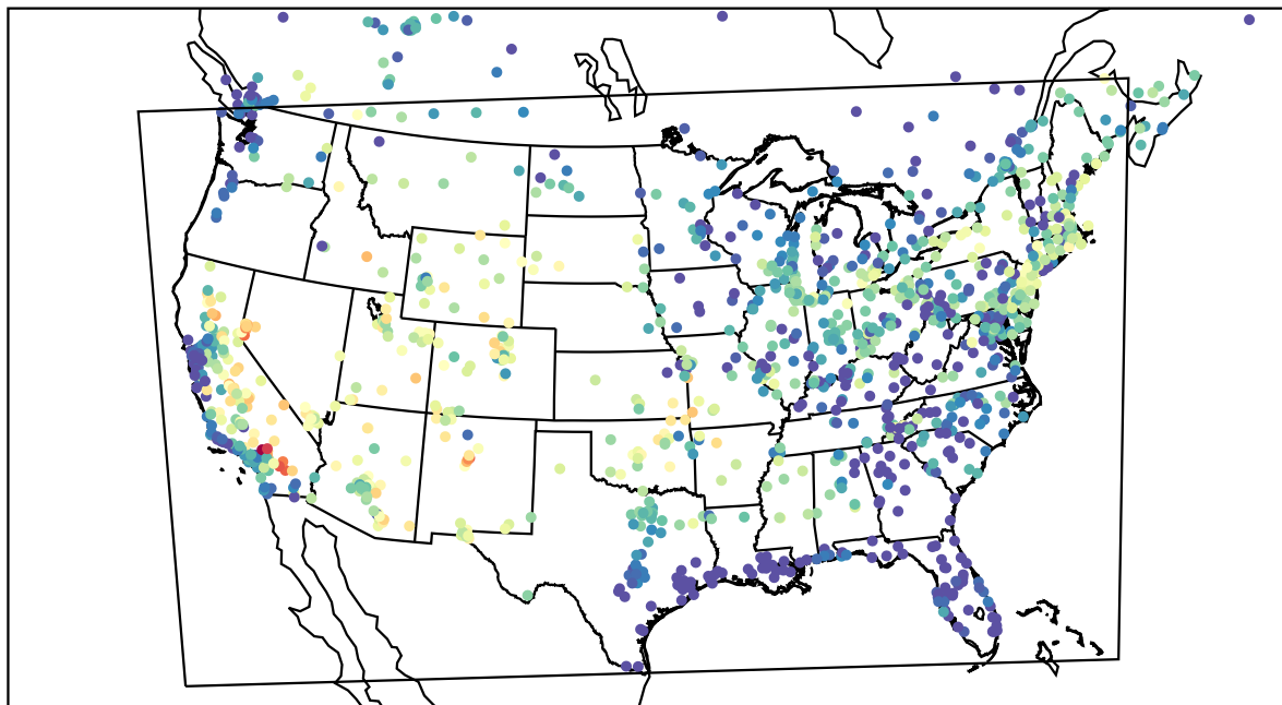
AirNOW (2022-07-22_04:00:00)
