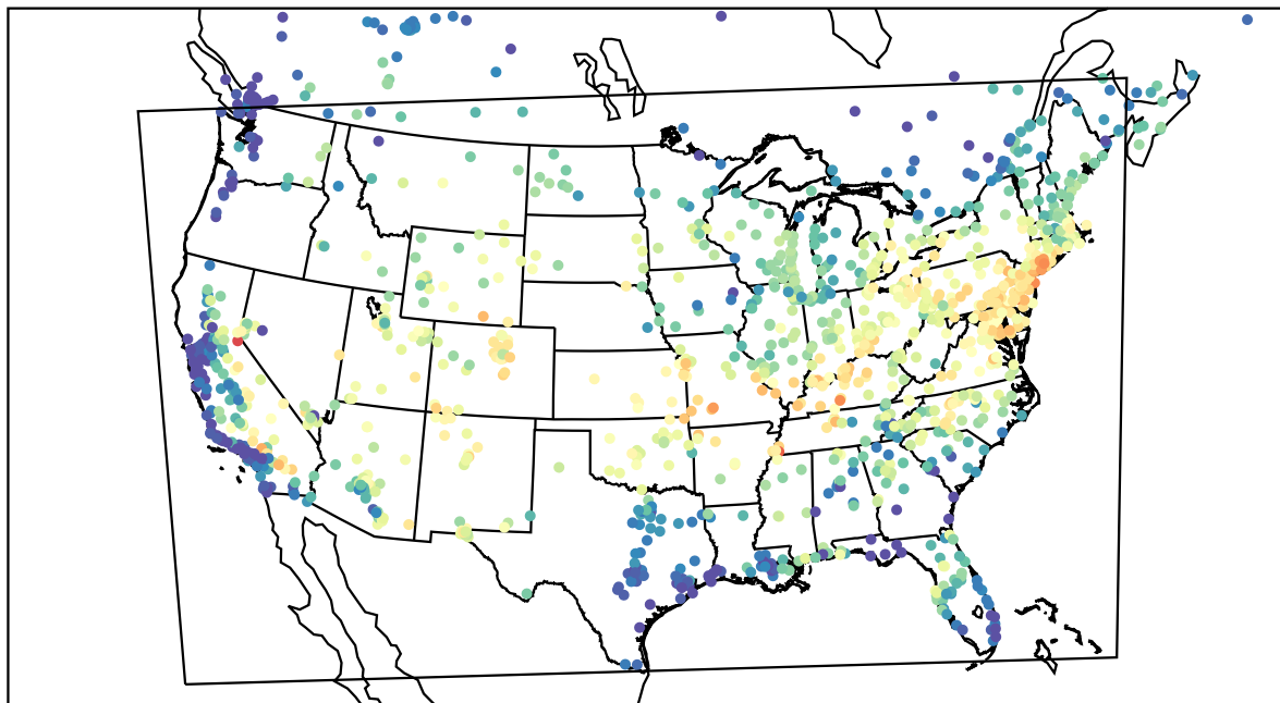
AirNOW (2022-07-22_15:00:00)
