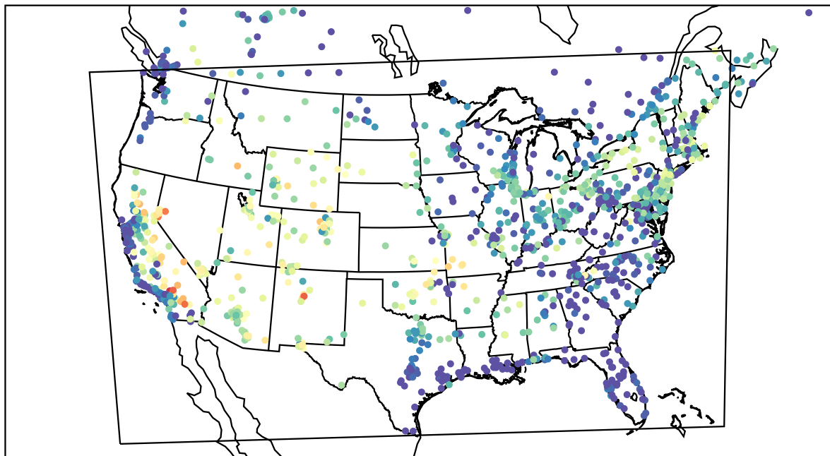
AirNOW (2022-07-22_05:00:00)
