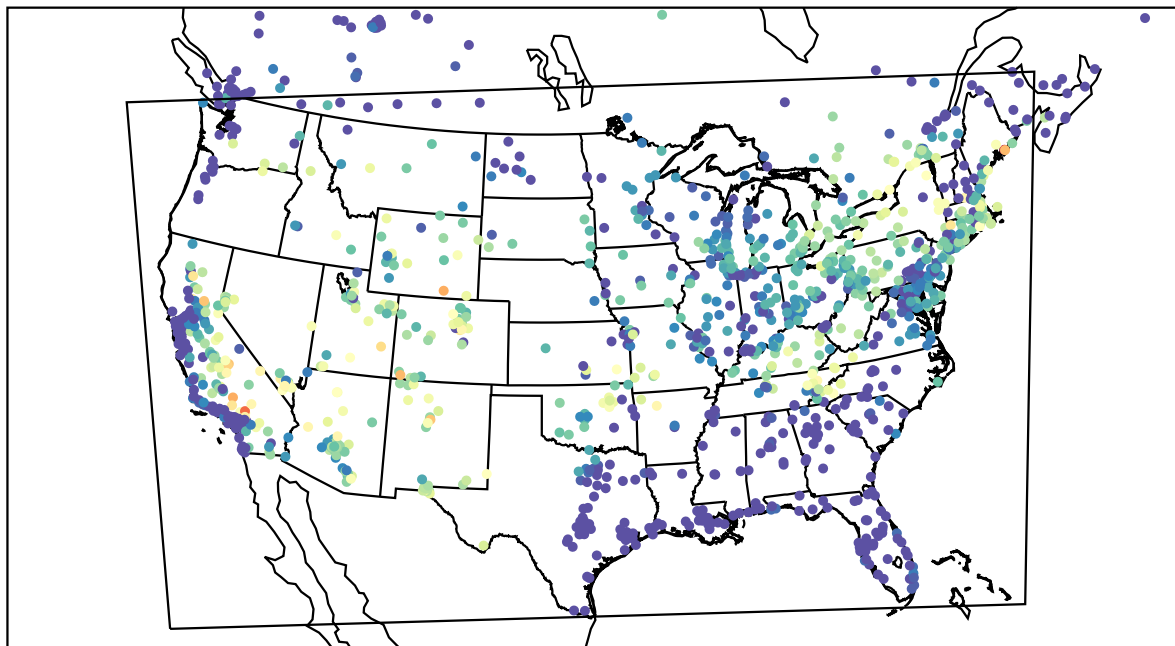
AirNOW (2022-07-21_08:00:00)
