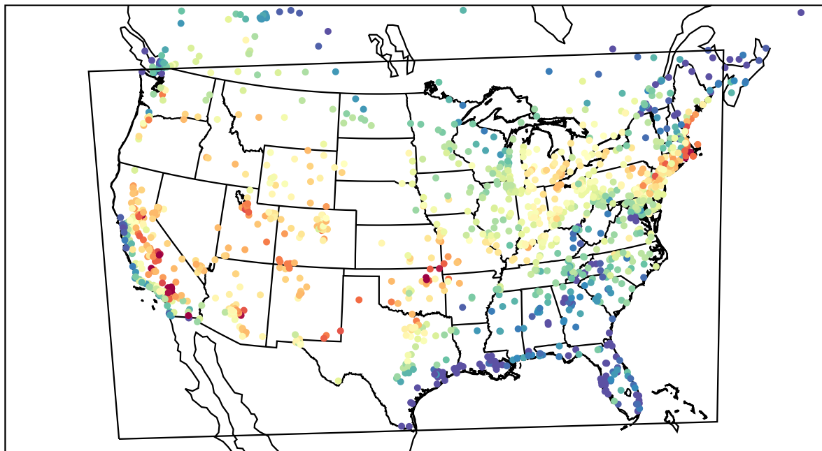
AirNOW (2022-07-21_00:00:00)
