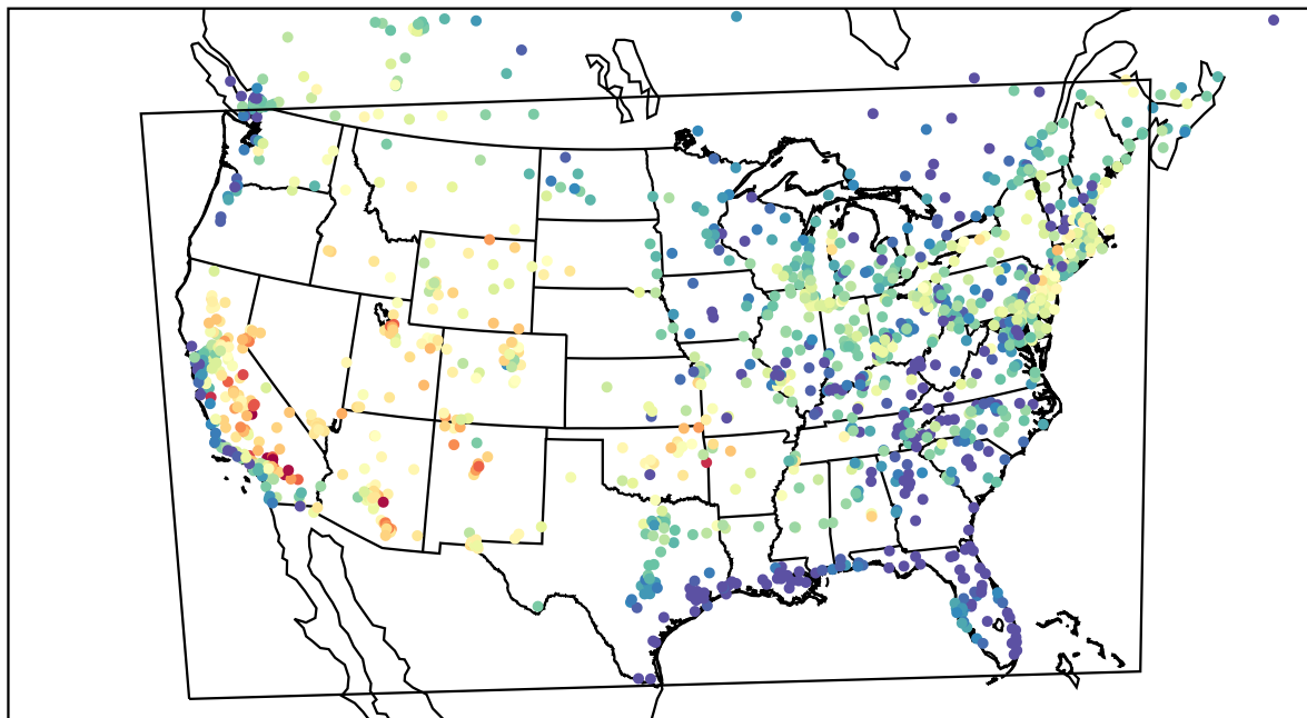
AirNOW (2022-07-22_02:00:00)
