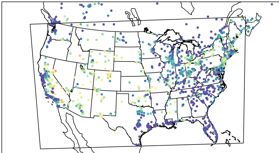
AirNOW (2022-07-22_06:00:00)
