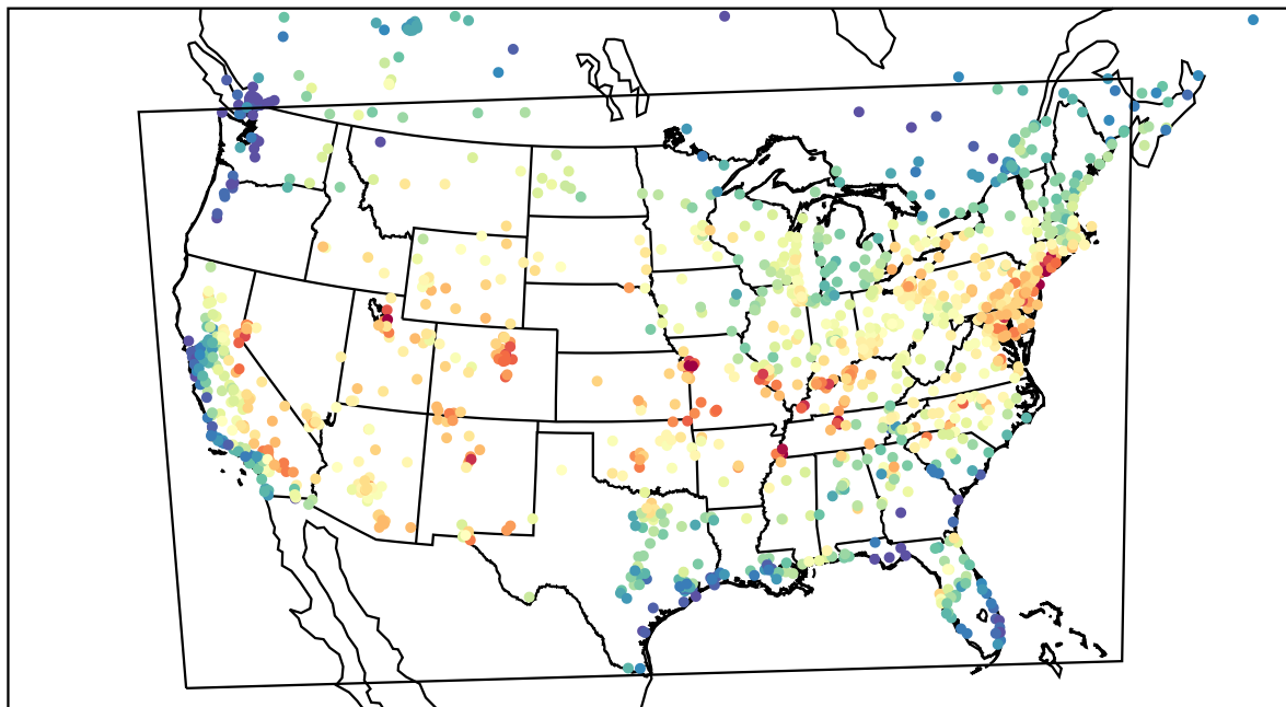
AirNOW (2022-07-22_17:00:00)
