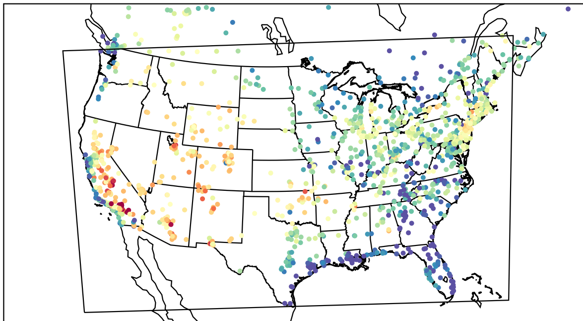
AirNOW (2022-07-22_01:00:00)
