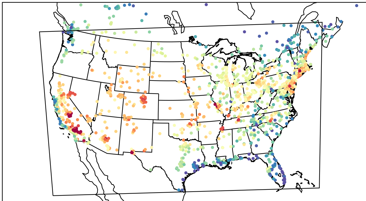
AirNOW (2022-07-22_23:00:00)
