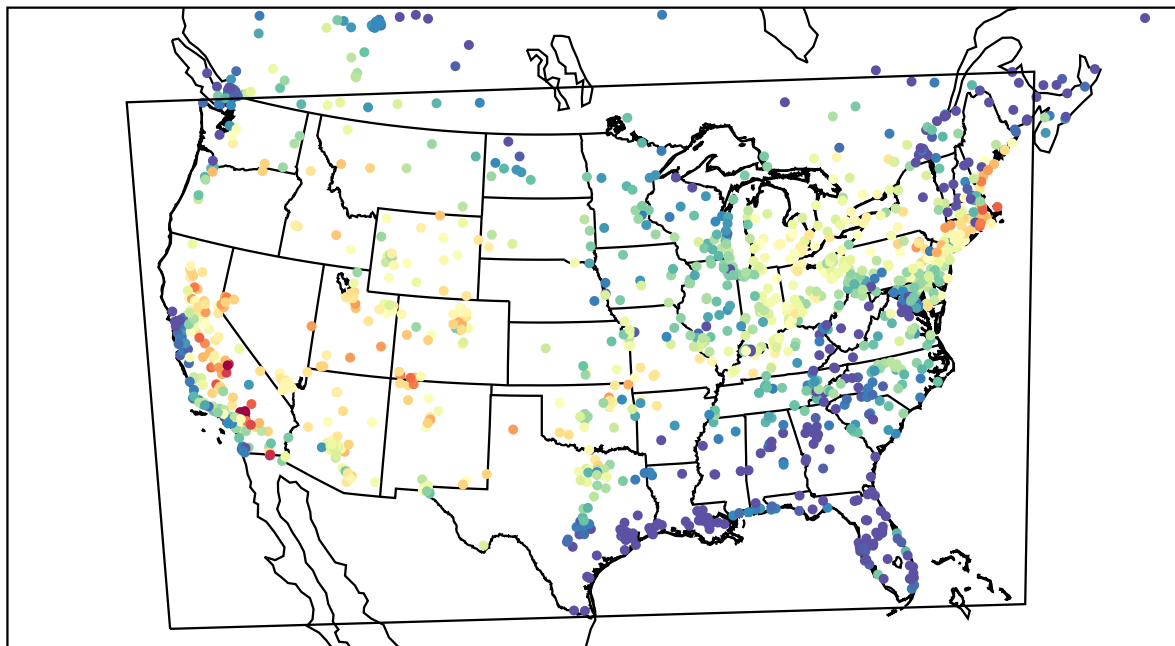
AirNOW (2022-07-21_02:00:00)
