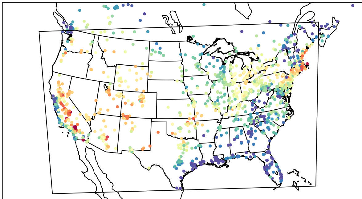
AirNOW (2022-07-21_01:00:00)
