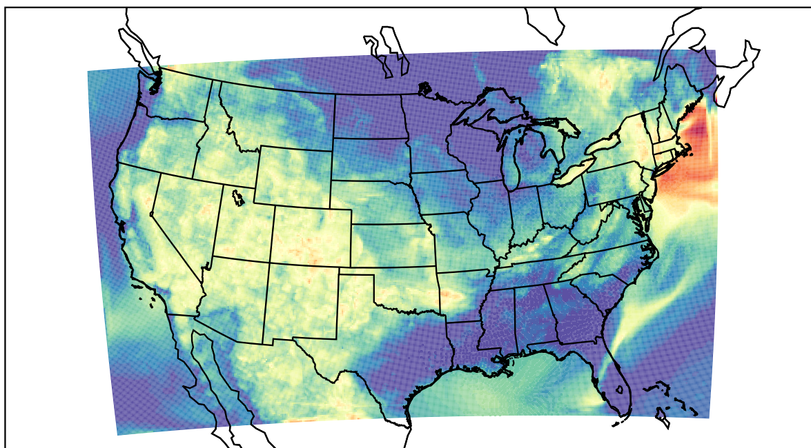
WRF (2022-07-21_07:00:00)
