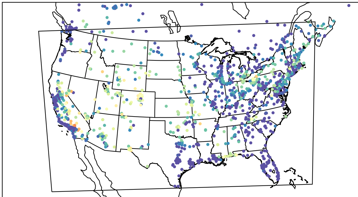
AirNOW (2022-07-22_08:00:00)
