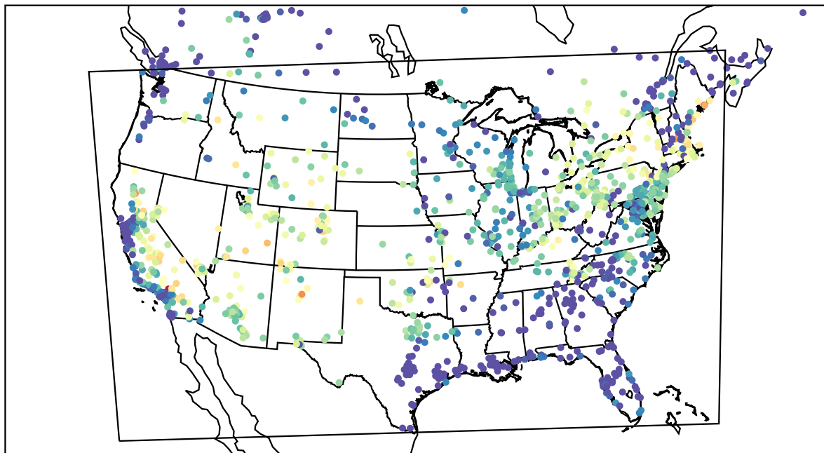
AirNOW (2022-07-21_05:00:00)
