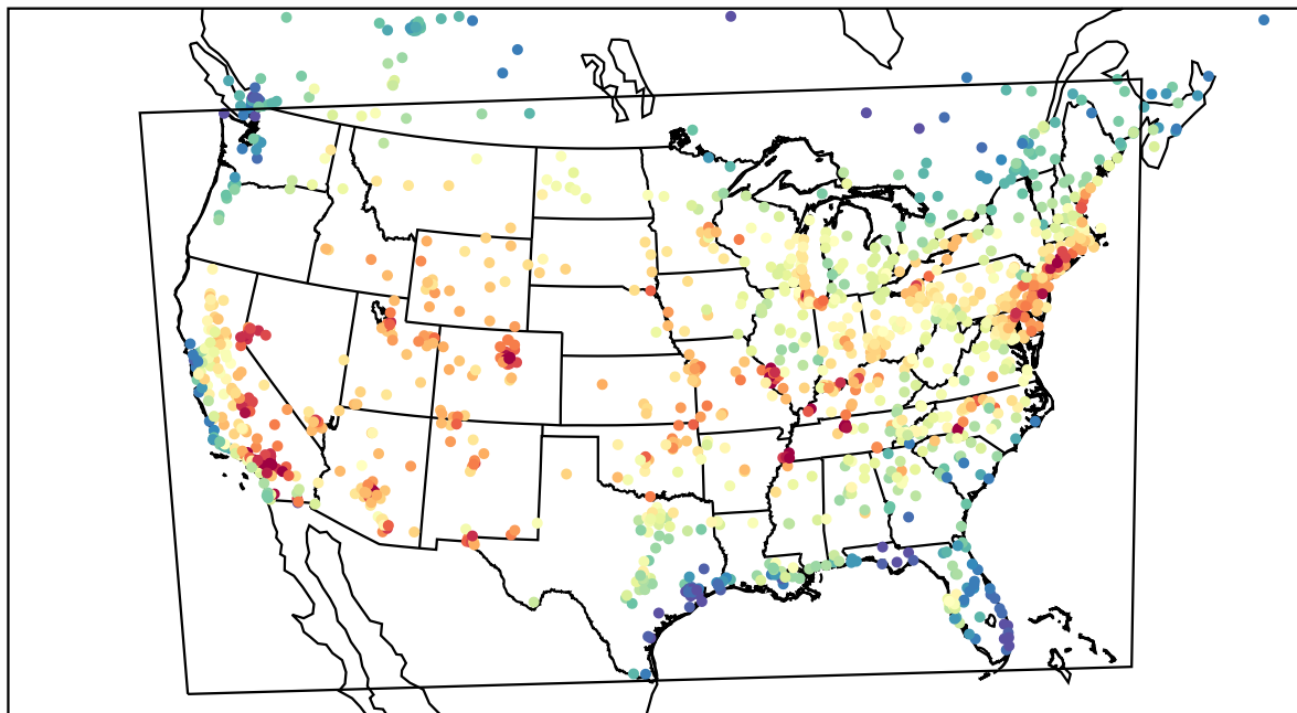
AirNOW (2022-07-22_21:00:00)
