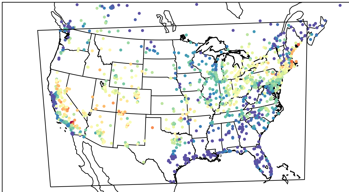
AirNOW (2022-07-21_03:00:00)
