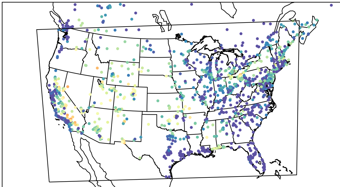
AirNOW (2022-07-22_07:00:00)
