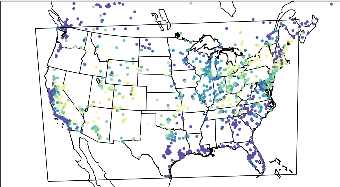
AirNOW (2022-07-21_06:00:00)
