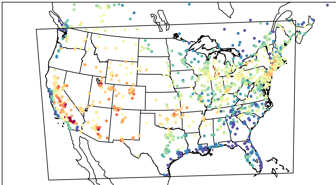
AirNOW (2022-07-22_00:00:00)
