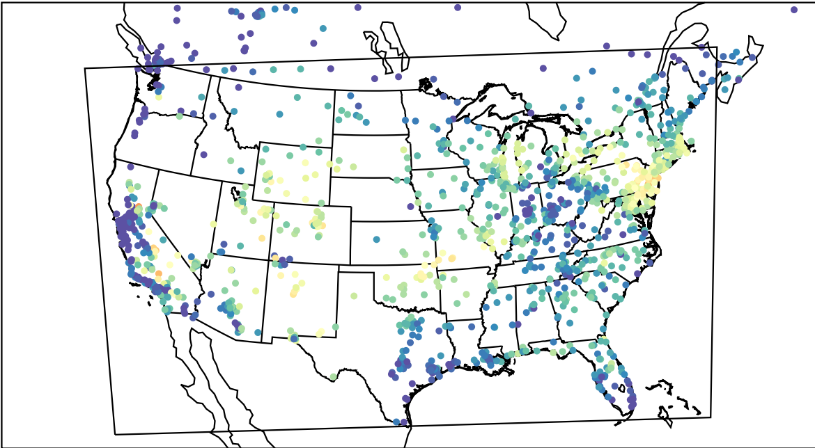
AirNOW (2022-07-27_15:00:00)
