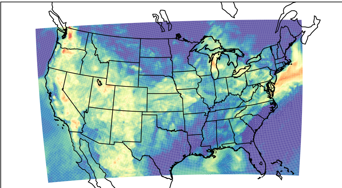
WRF (2022-07-27_07:00:00)
