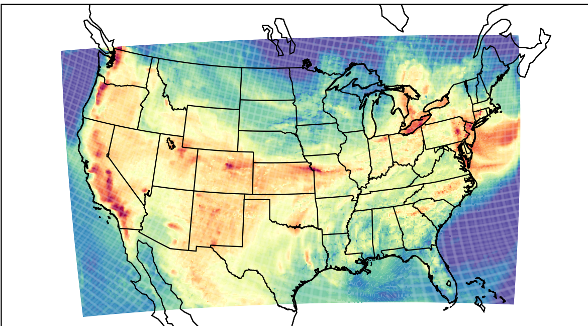
WRF (2022-07-27_23:00:00)
