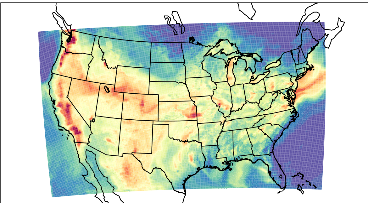
WRF (2022-07-27_00:00:00)
