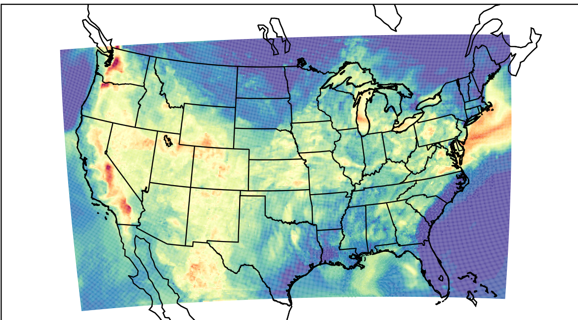
WRF (2022-07-27_03:00:00)
