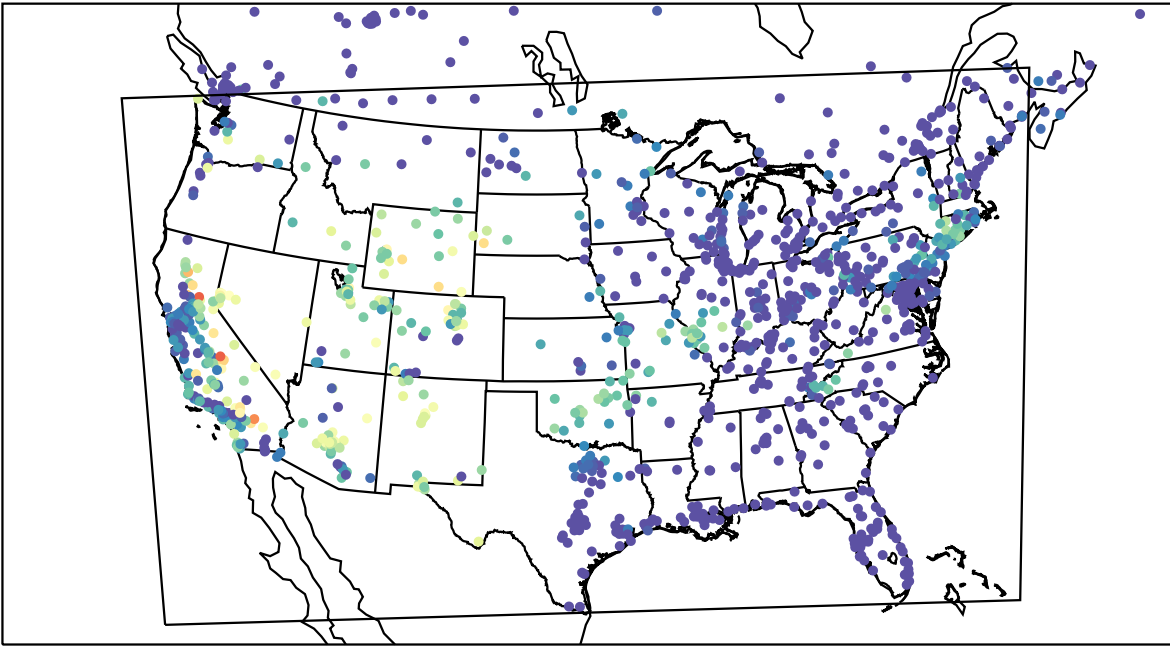
AirNOW (2022-07-26_08:00:00)
