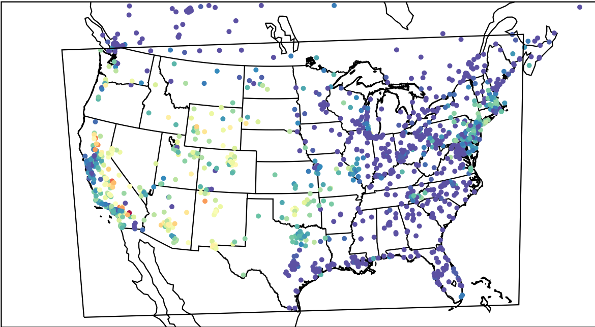
AirNOW (2022-07-26_05:00:00)
