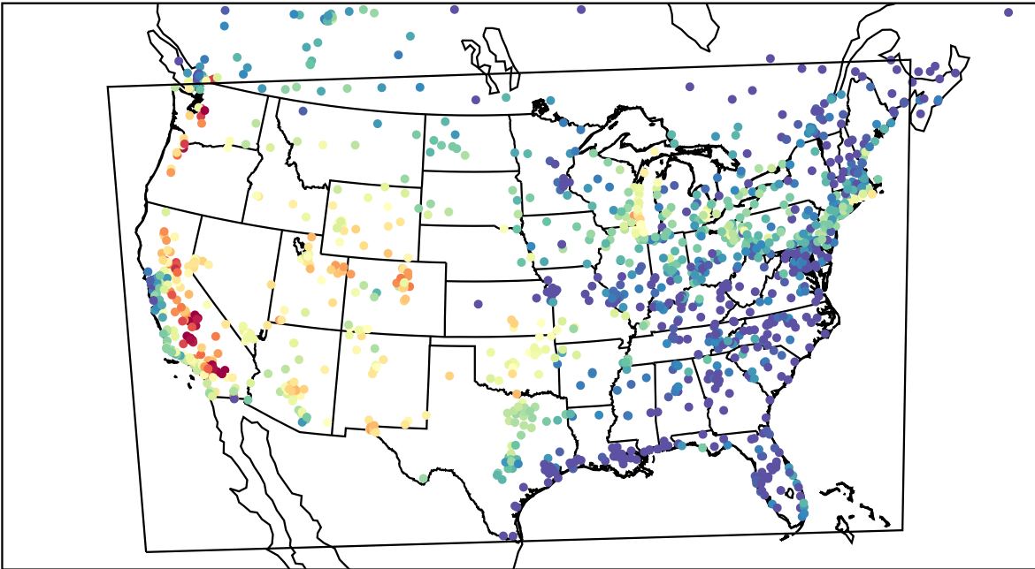
AirNOW (2022-07-27_01:00:00)
