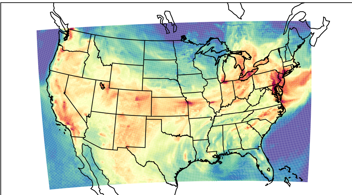
WRF (2022-07-27_20:00:00)
