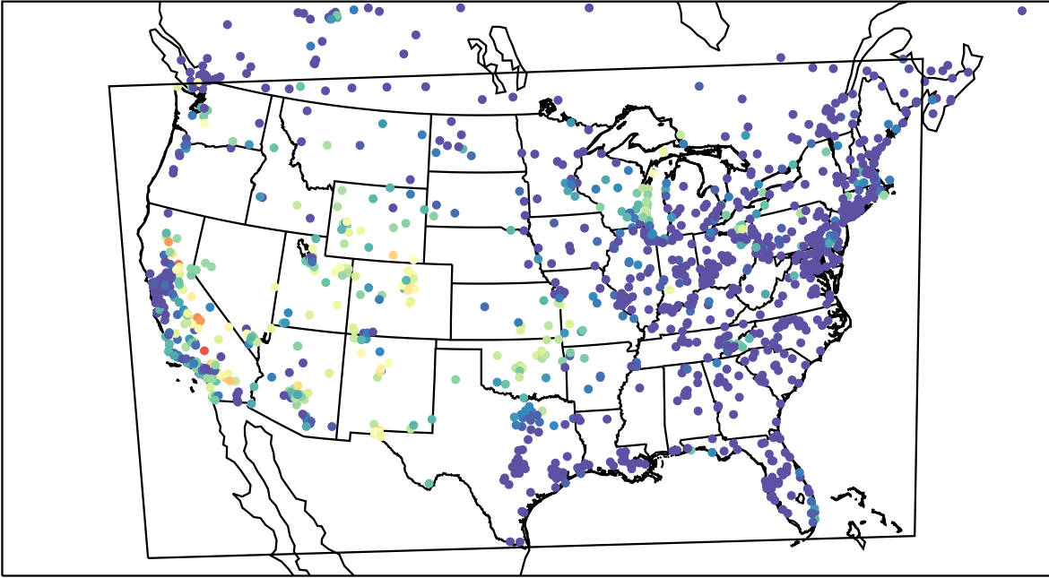
AirNOW (2022-07-27_07:00:00)
