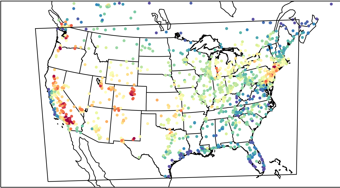
AirNOW (2022-07-27_22:00:00)
