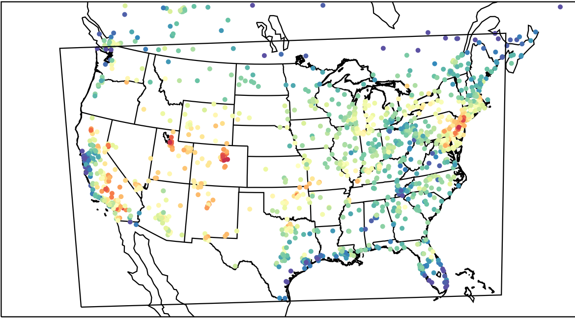
AirNOW (2022-07-27_18:00:00)
