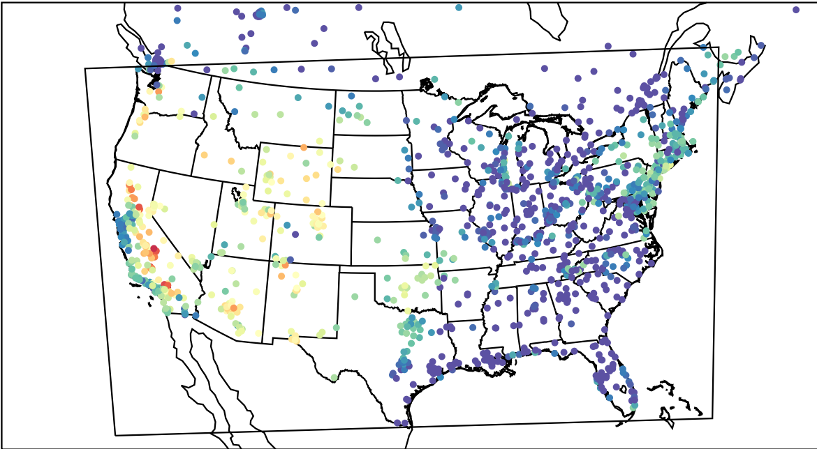
AirNOW (2022-07-26_03:00:00)
