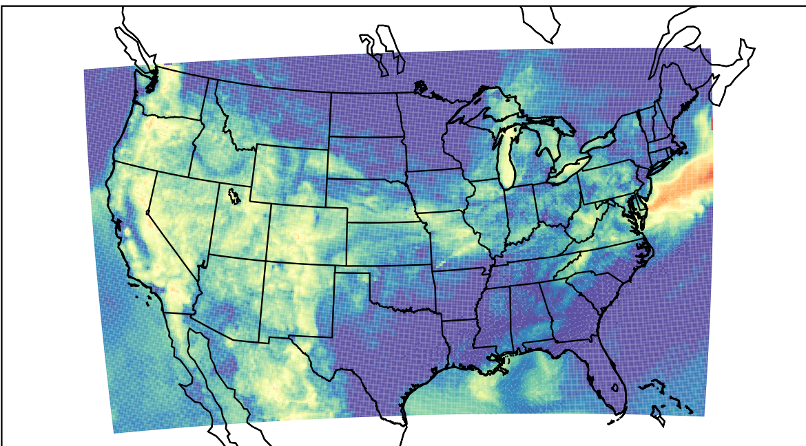
WRF (2022-07-27_12:00:00)
