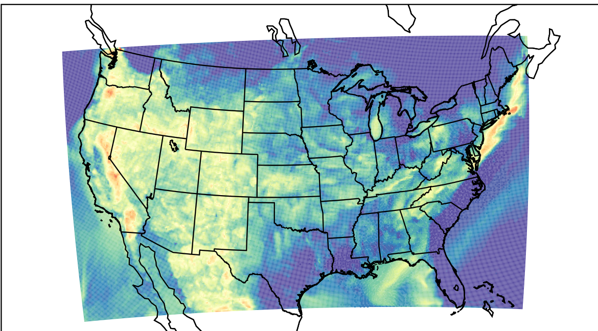
WRF (2022-07-26_06:00:00)
