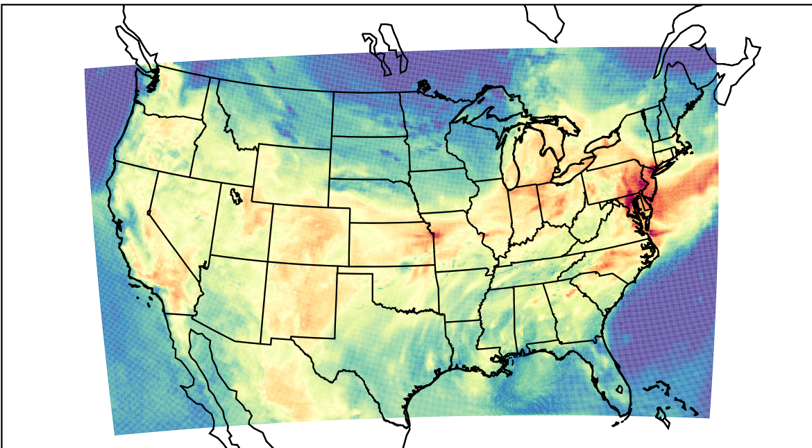
WRF (2022-07-27_17:00:00)
