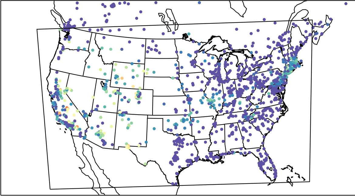
AirNOW (2022-07-26_11:00:00)
