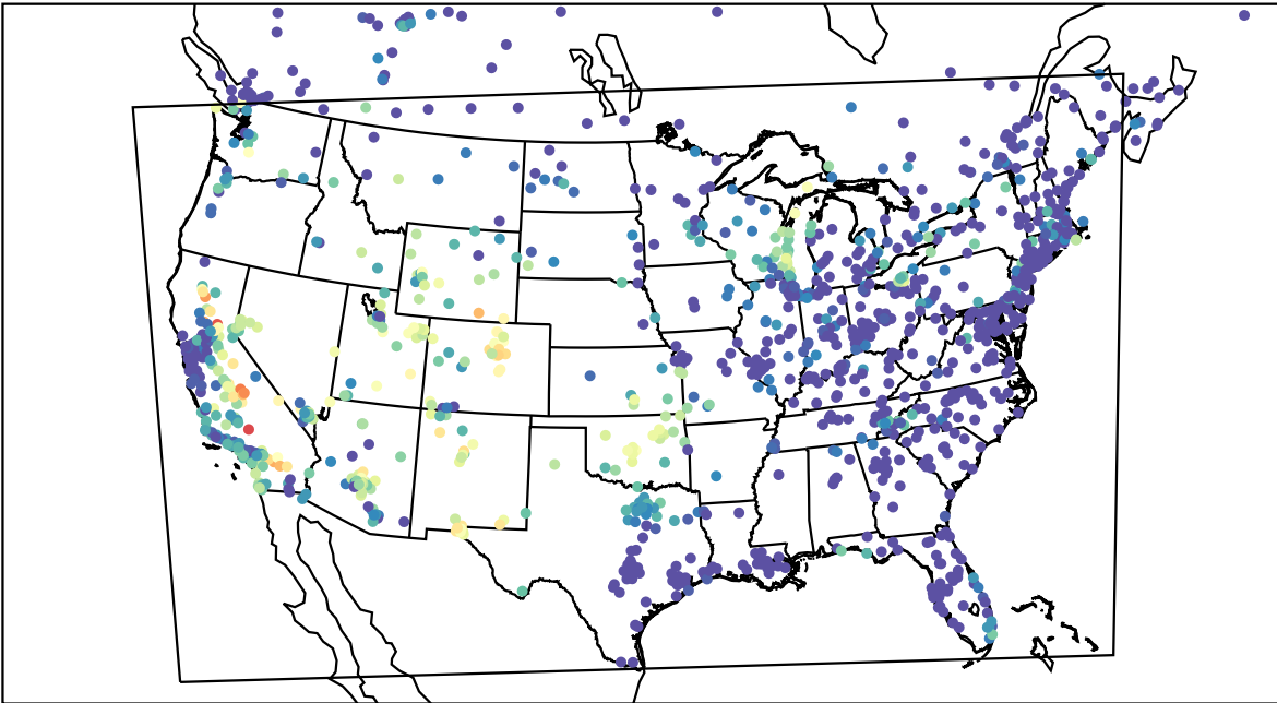
AirNOW (2022-07-27_06:00:00)
