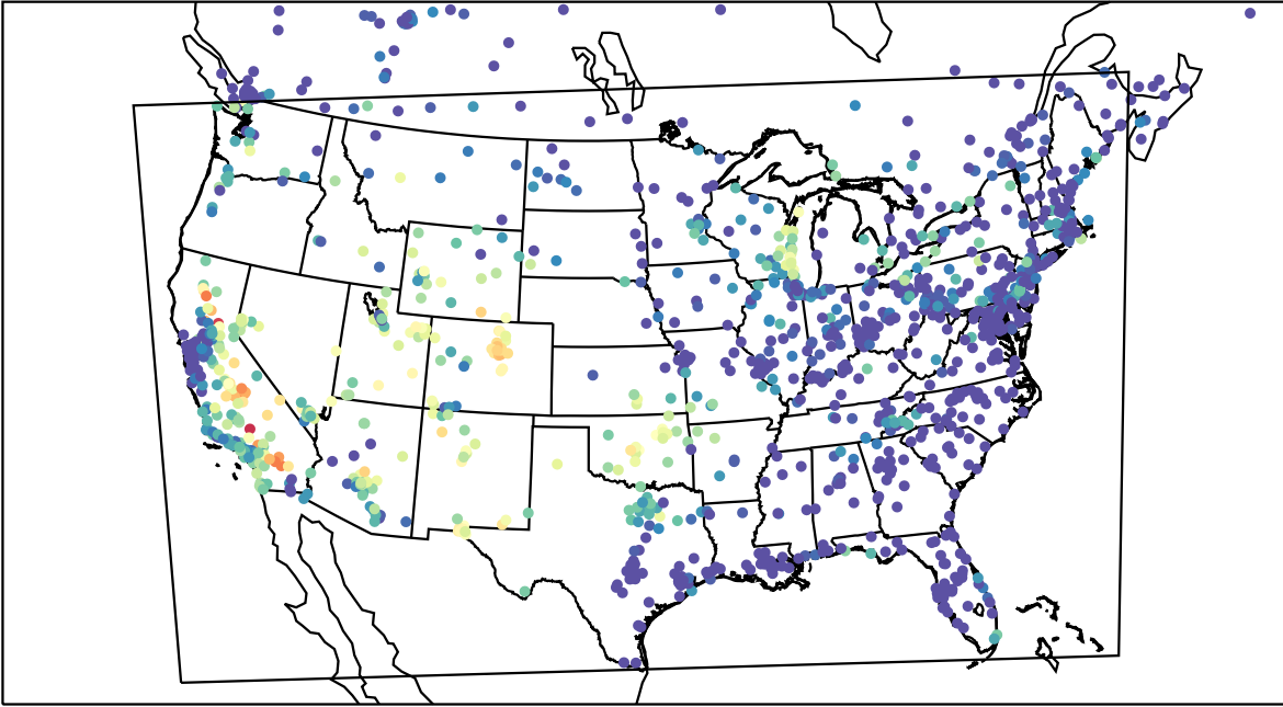
AirNOW (2022-07-27_05:00:00)
