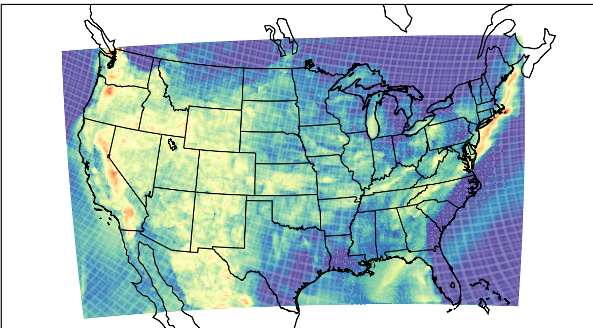
WRF (2022-07-26_05:00:00)
