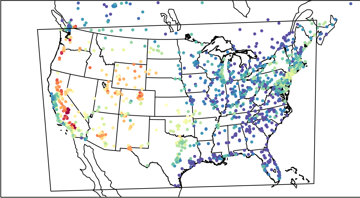
AirNOW (2022-07-26_01:00:00)
