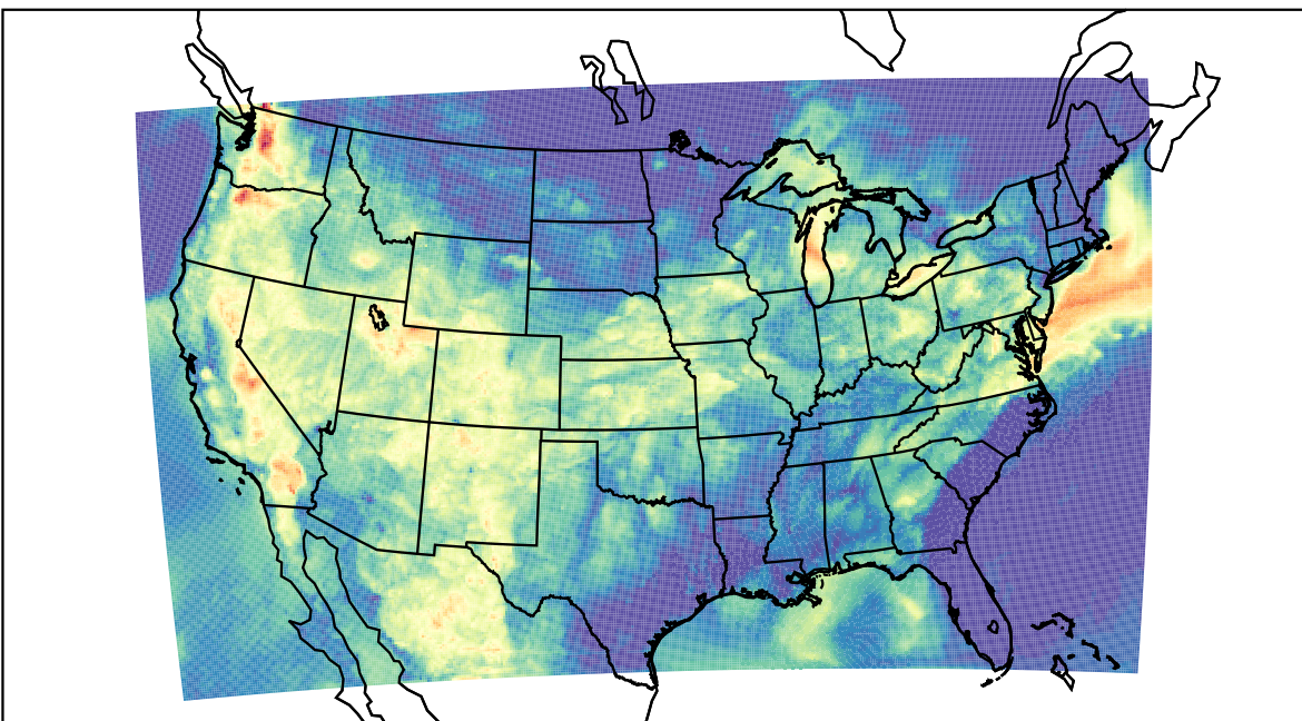
WRF (2022-07-27_06:00:00)
