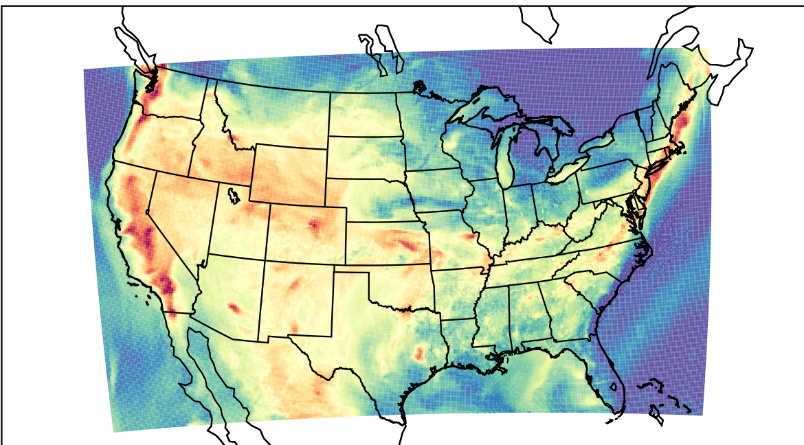
WRF (2022-07-26_00:00:00)
