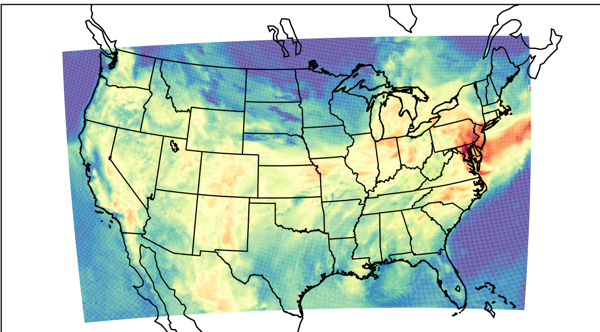
WRF (2022-07-27_16:00:00)
