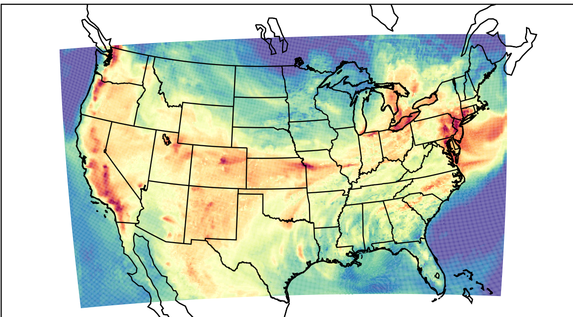
WRF (2022-07-27_22:00:00)
