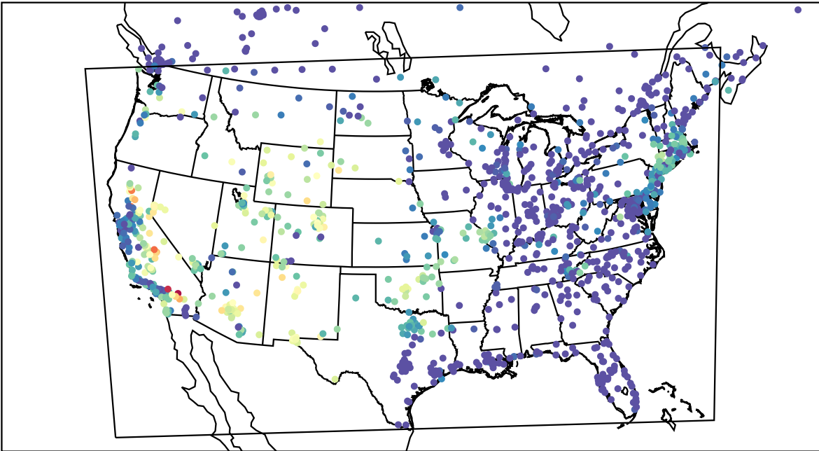
AirNOW (2022-07-26_06:00:00)
