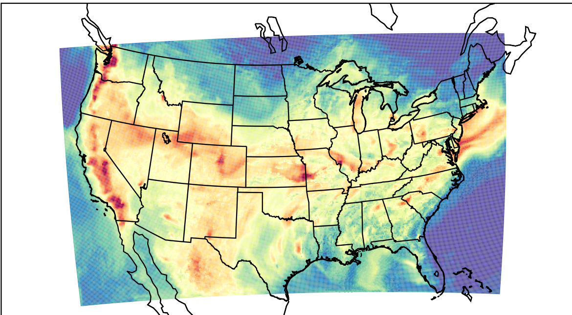
WRF (2022-07-26_23:00:00)
