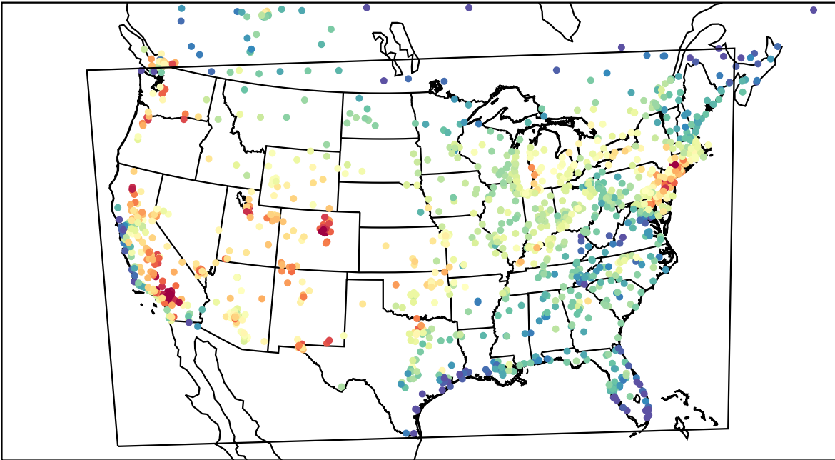
AirNOW (2022-07-27_21:00:00)
