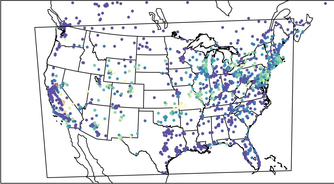
AirNOW (2022-07-27_13:00:00)
