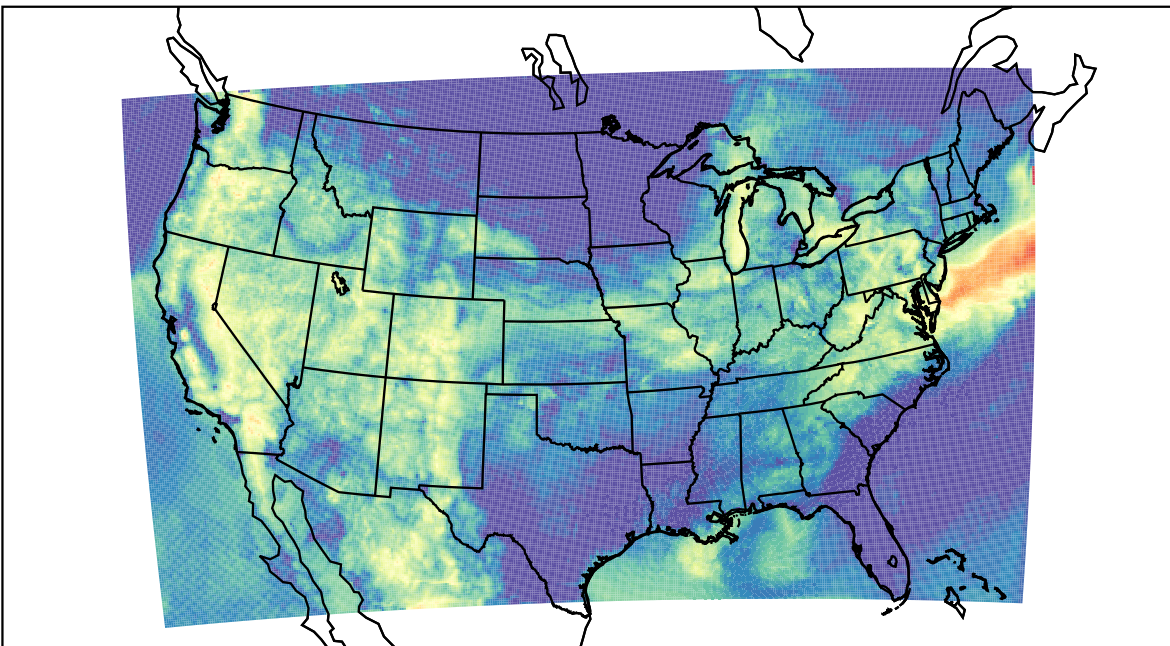
WRF (2022-07-27_13:00:00)
