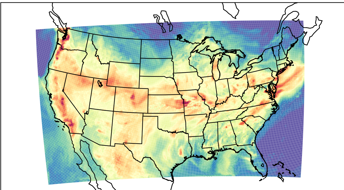
WRF (2022-07-26_21:00:00)
