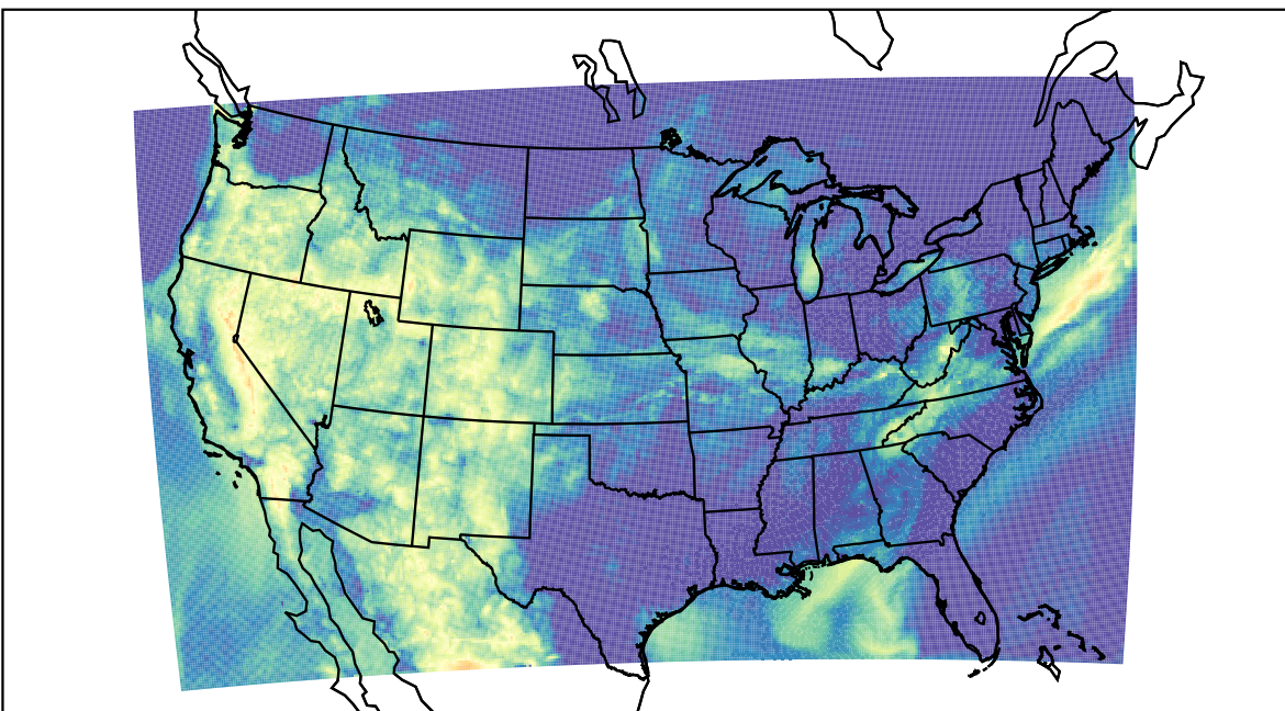
WRF (2022-07-26_12:00:00)
