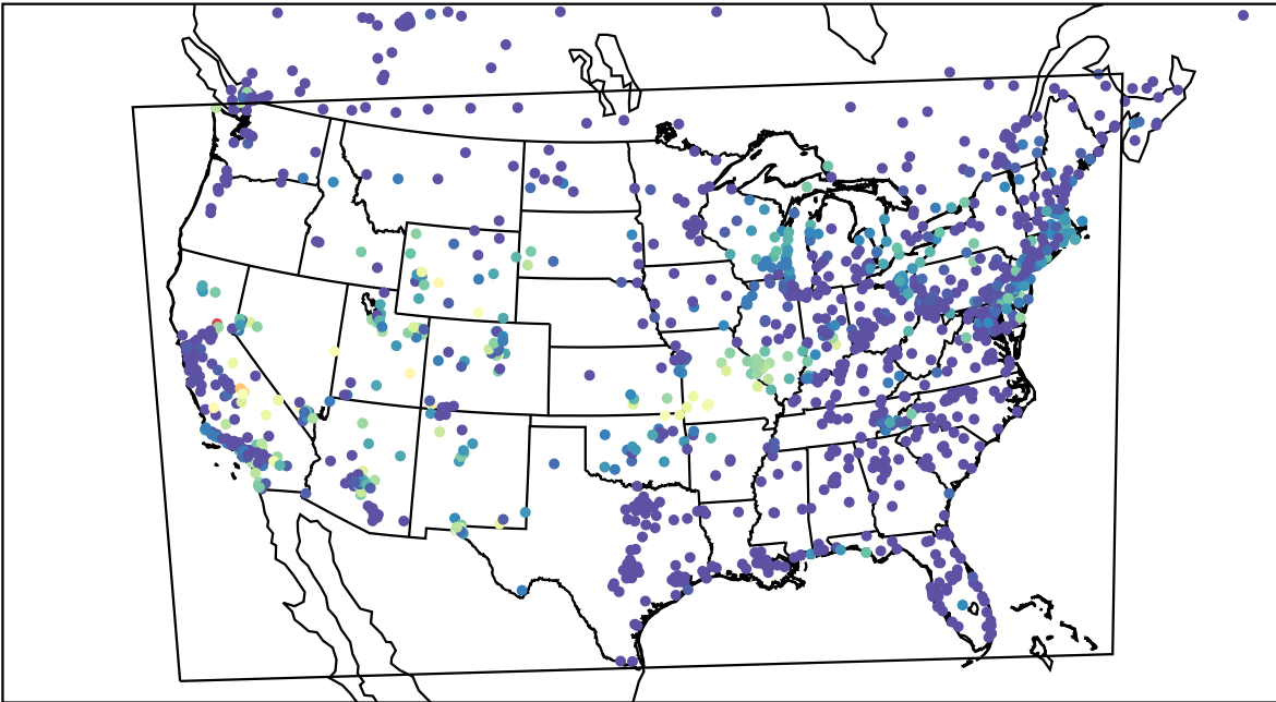
AirNOW (2022-07-27_12:00:00)
