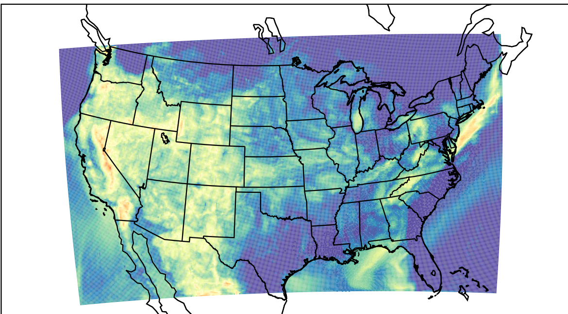
WRF (2022-07-26_08:00:00)
