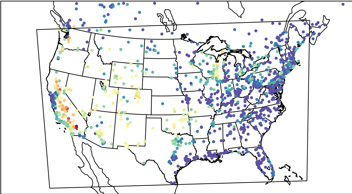
AirNOW (2022-07-27_03:00:00)
