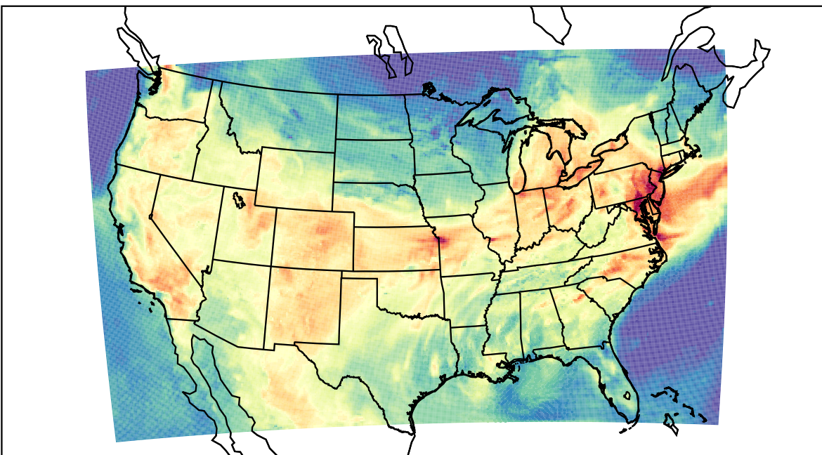
WRF (2022-07-27_18:00:00)
