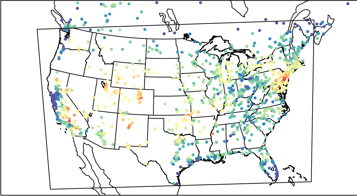
AirNOW (2022-07-27_17:00:00)
