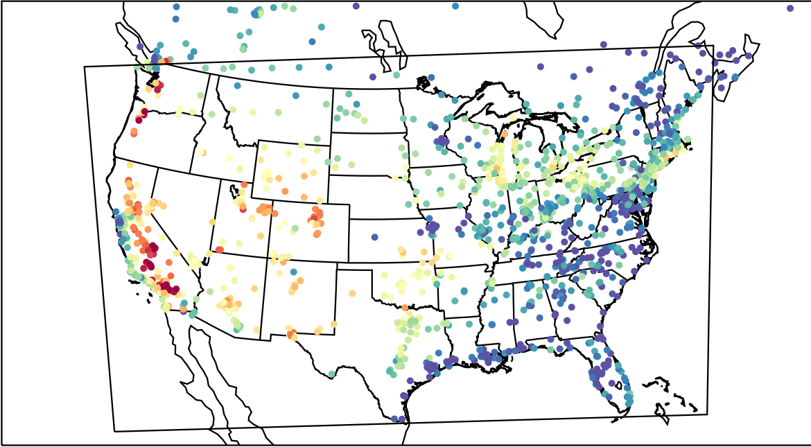
AirNOW (2022-07-27_00:00:00)
