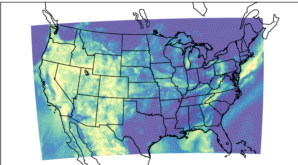
WRF (2022-07-26_11:00:00)
