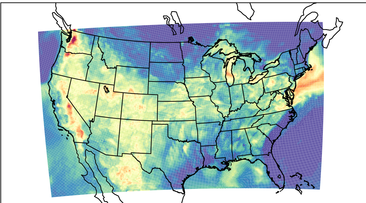
WRF (2022-07-27_04:00:00)
