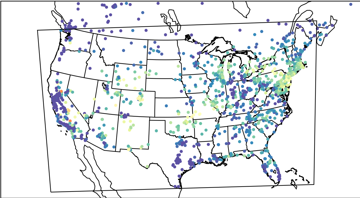
AirNOW (2022-07-27_14:00:00)
