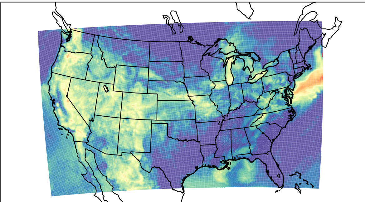
WRF (2022-07-27_11:00:00)
