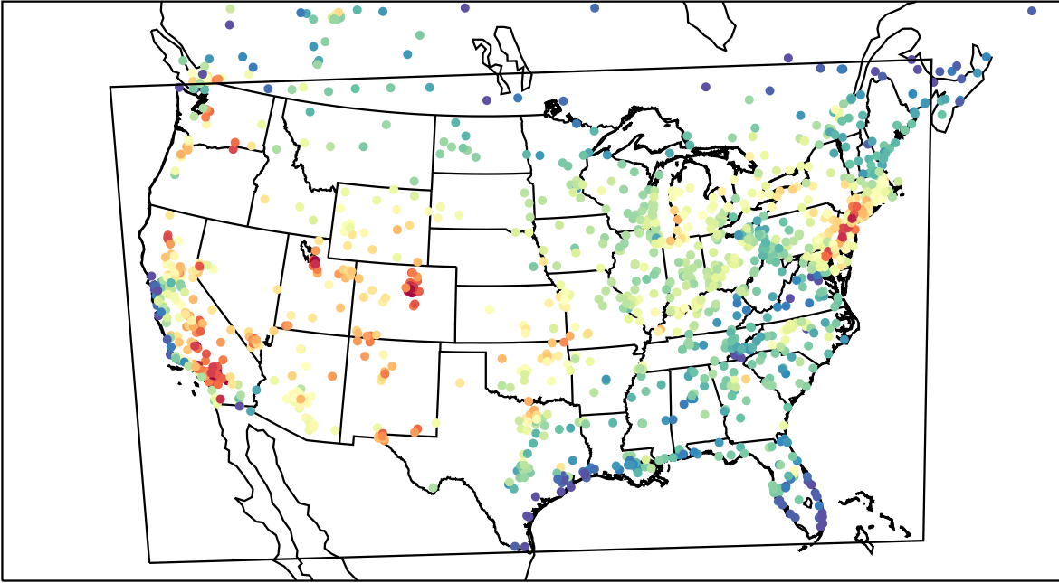
AirNOW (2022-07-27_20:00:00)
