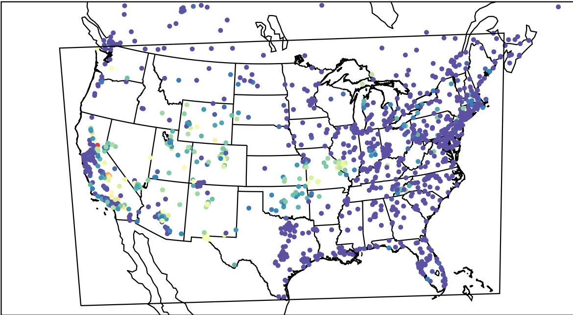
AirNOW (2022-07-27_10:00:00)
