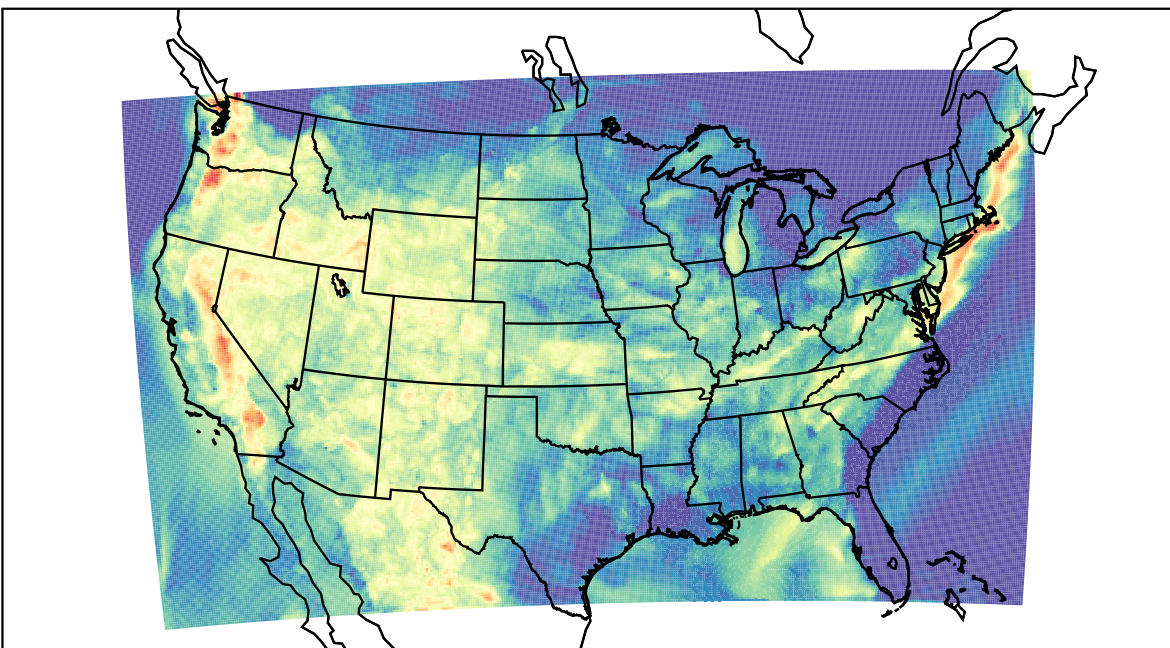
WRF (2022-07-26_04:00:00)
