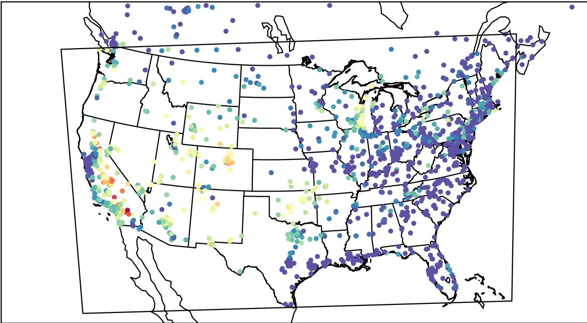
AirNOW (2022-07-27_04:00:00)
