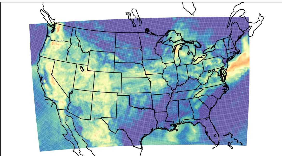
WRF (2022-07-27_09:00:00)
