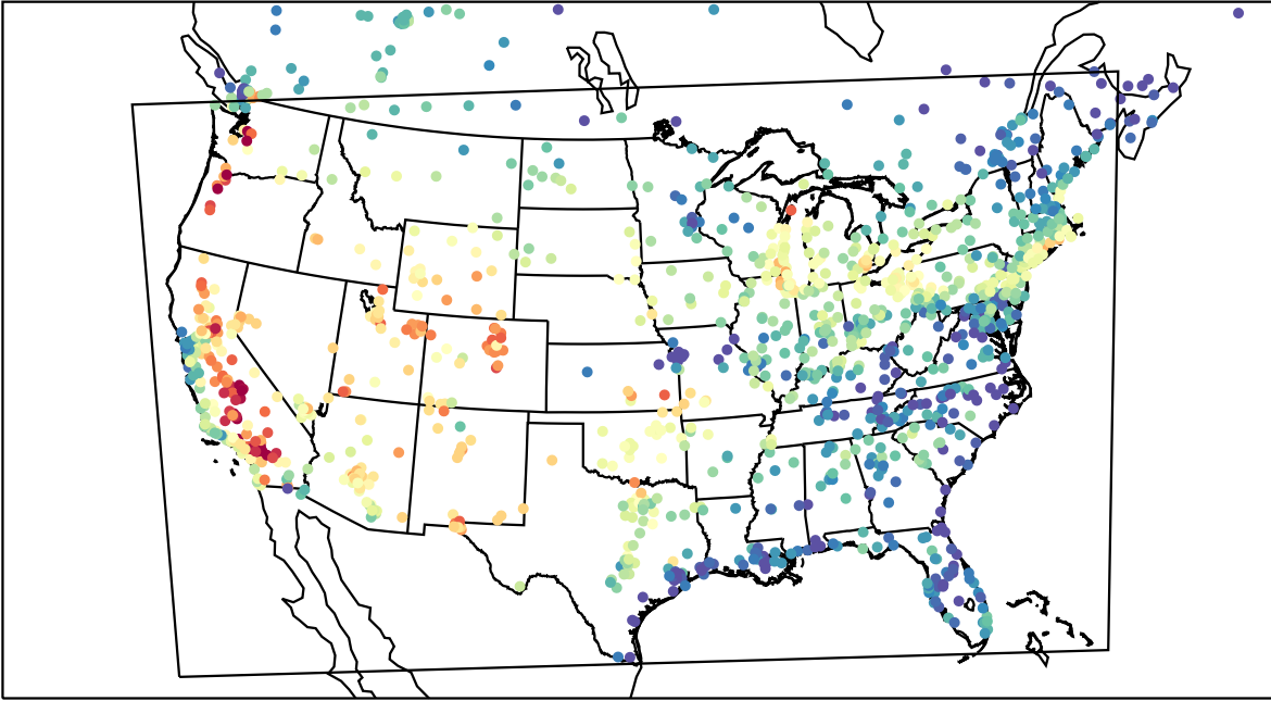
AirNOW (2022-07-26_23:00:00)
