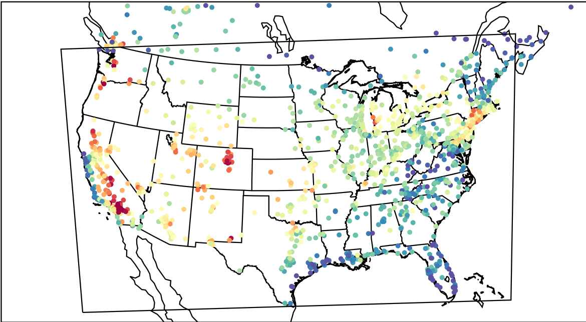
AirNOW (2022-07-27_23:00:00)
