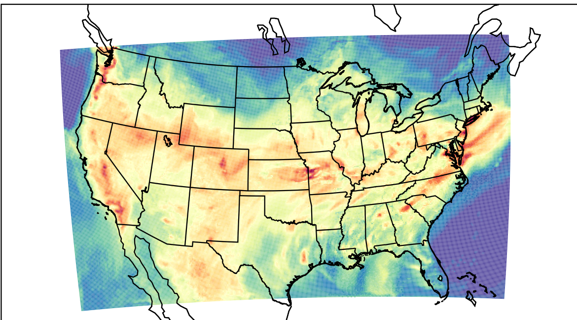
WRF (2022-07-26_20:00:00)
