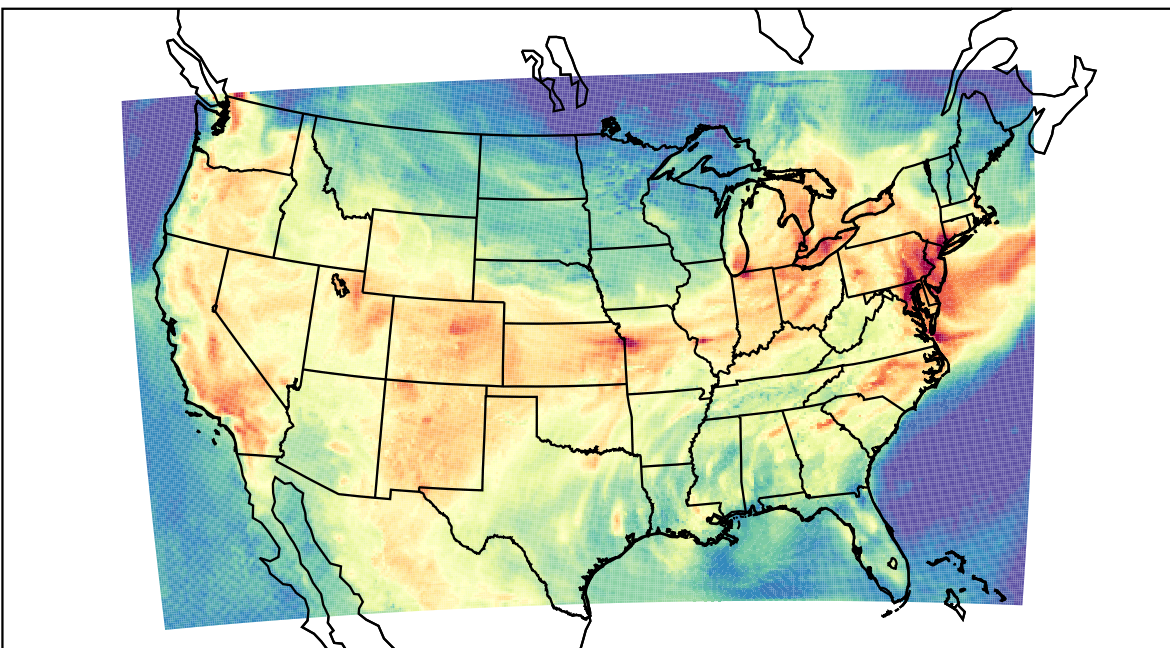
WRF (2022-07-27_19:00:00)
