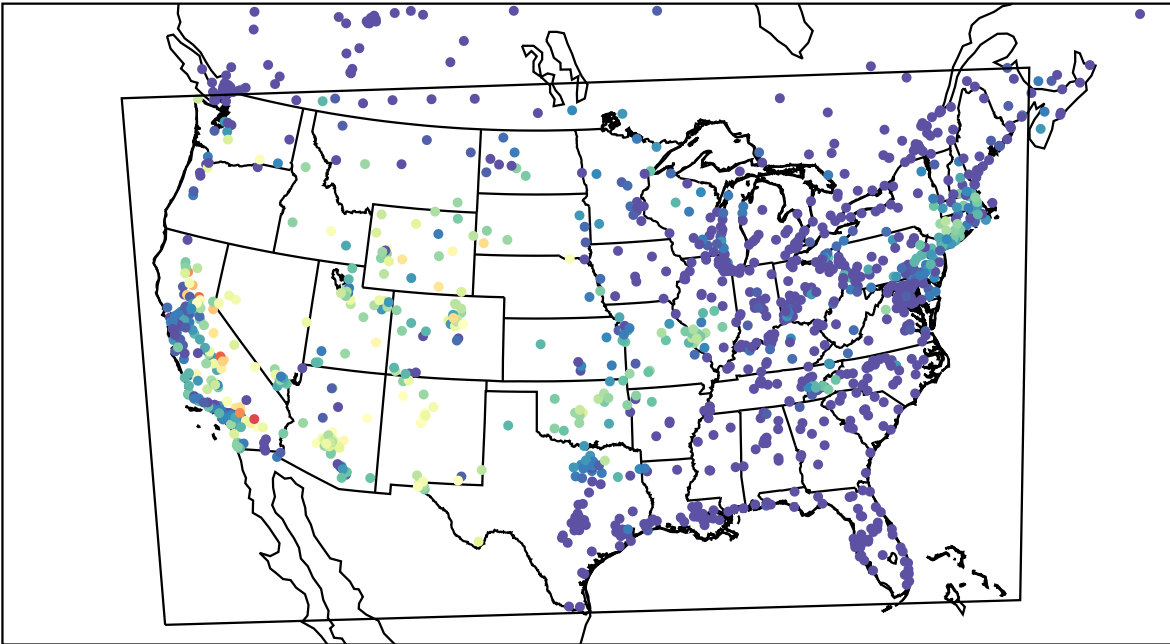
AirNOW (2022-07-26_07:00:00)
