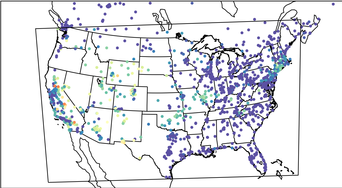
AirNOW (2022-07-26_09:00:00)
