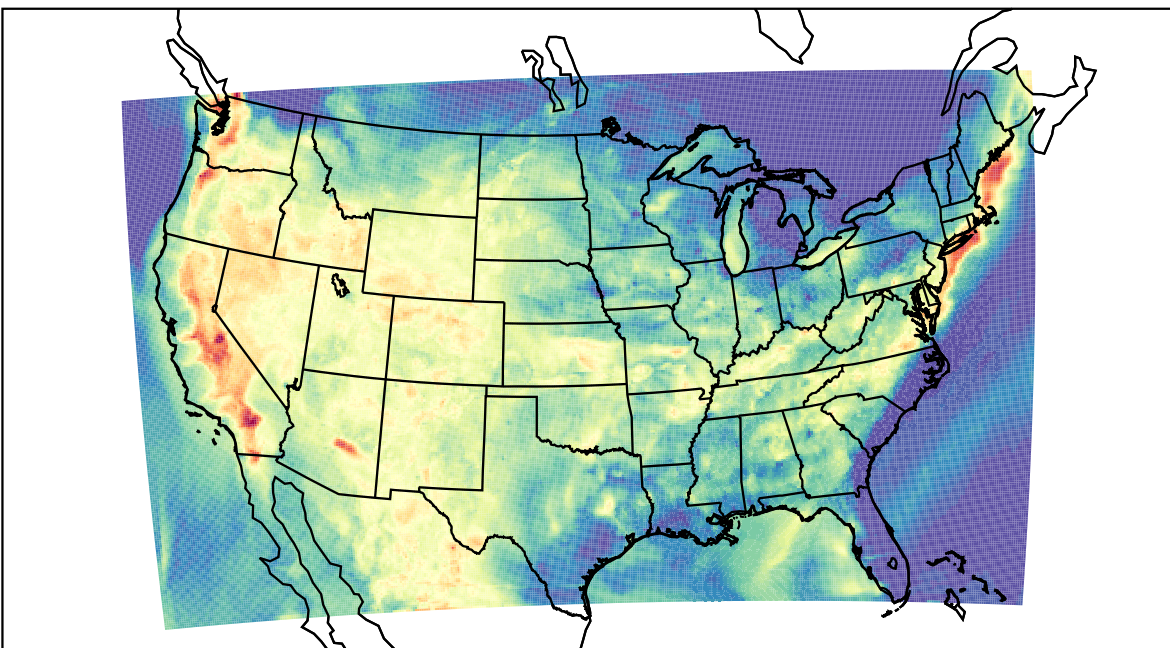
WRF (2022-07-26_02:00:00)
