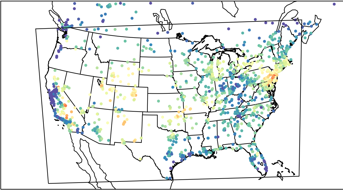
AirNOW (2022-07-27_16:00:00)
