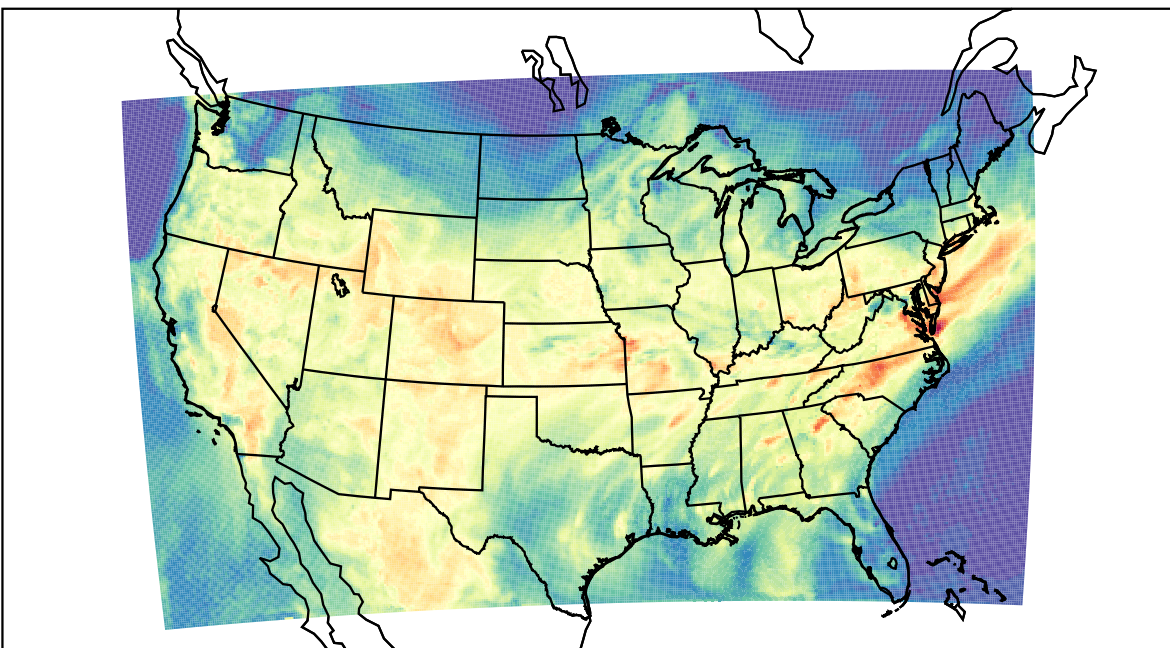
WRF (2022-07-26_17:00:00)
