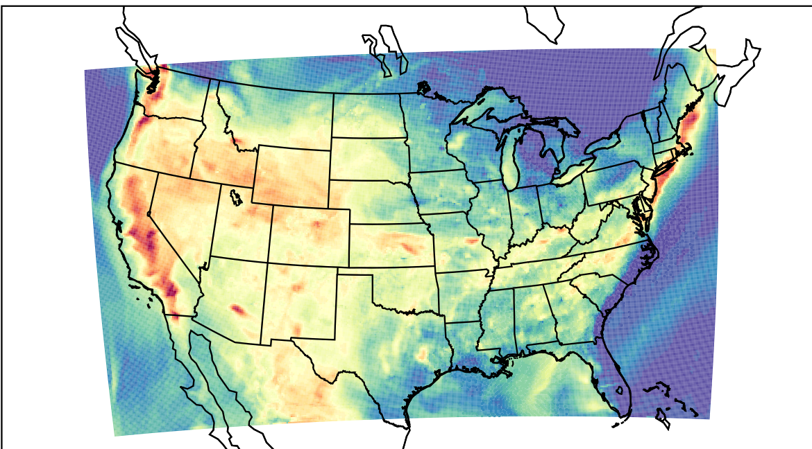
WRF (2022-07-26_01:00:00)
