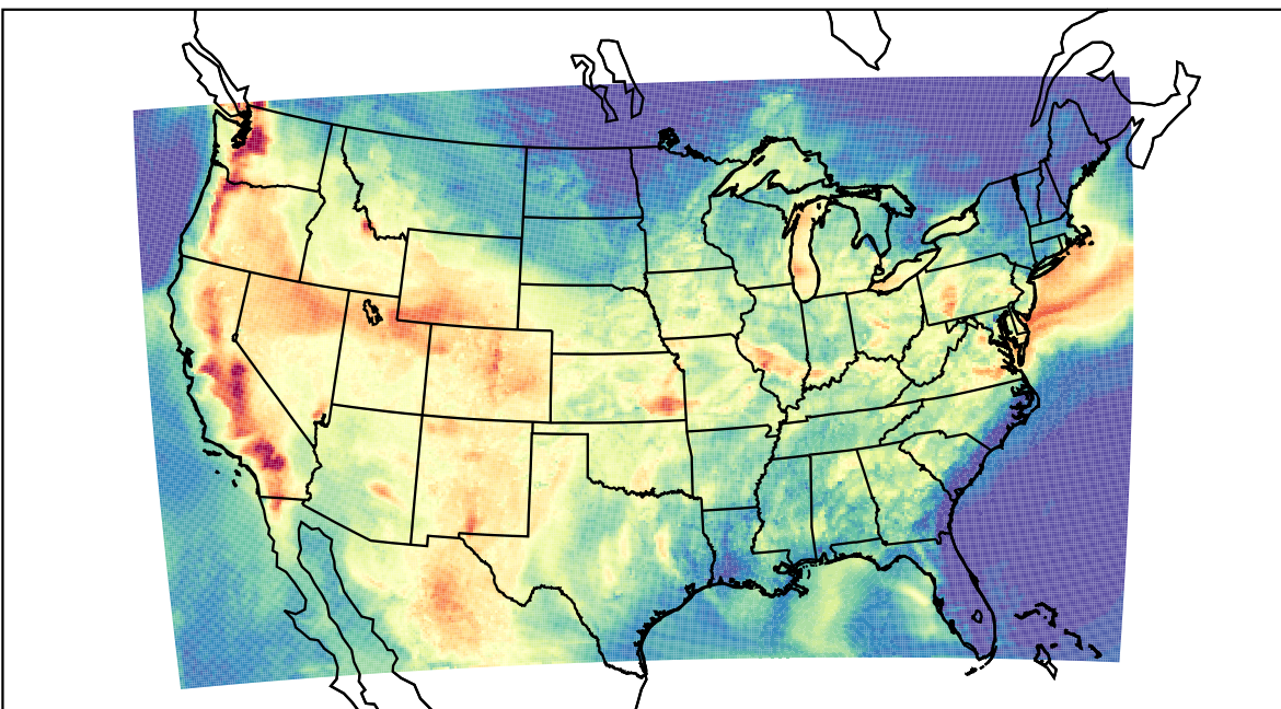
WRF (2022-07-27_01:00:00)
