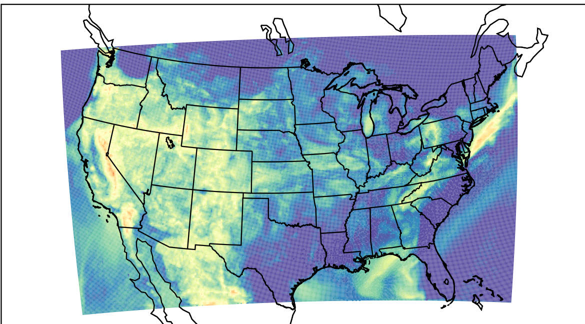
WRF (2022-07-26_09:00:00)
