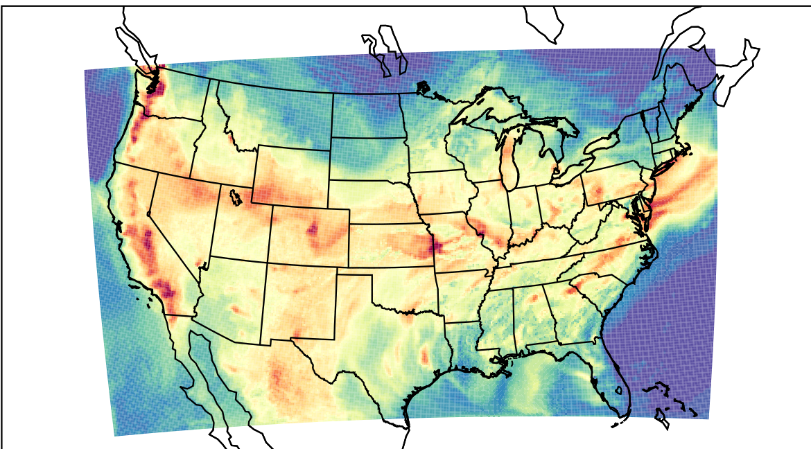
WRF (2022-07-26_22:00:00)
