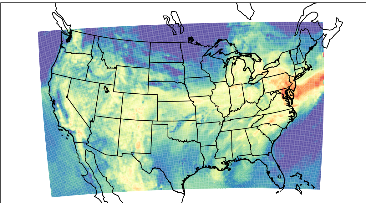
WRF (2022-07-27_15:00:00)
