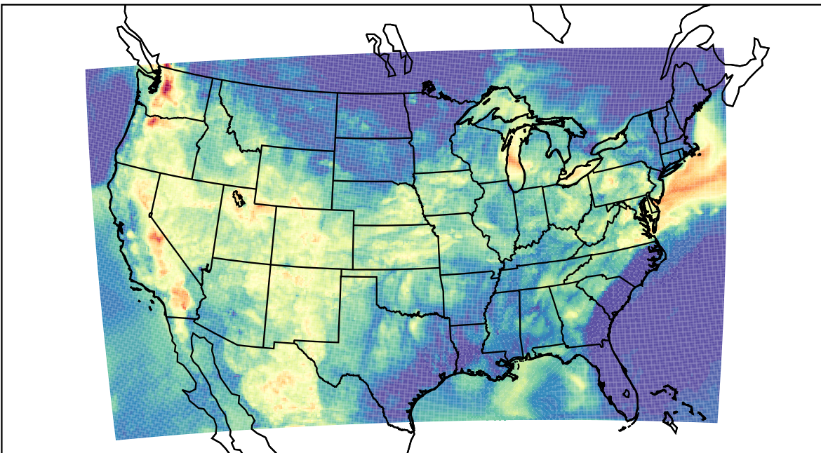
WRF (2022-07-27_05:00:00)
