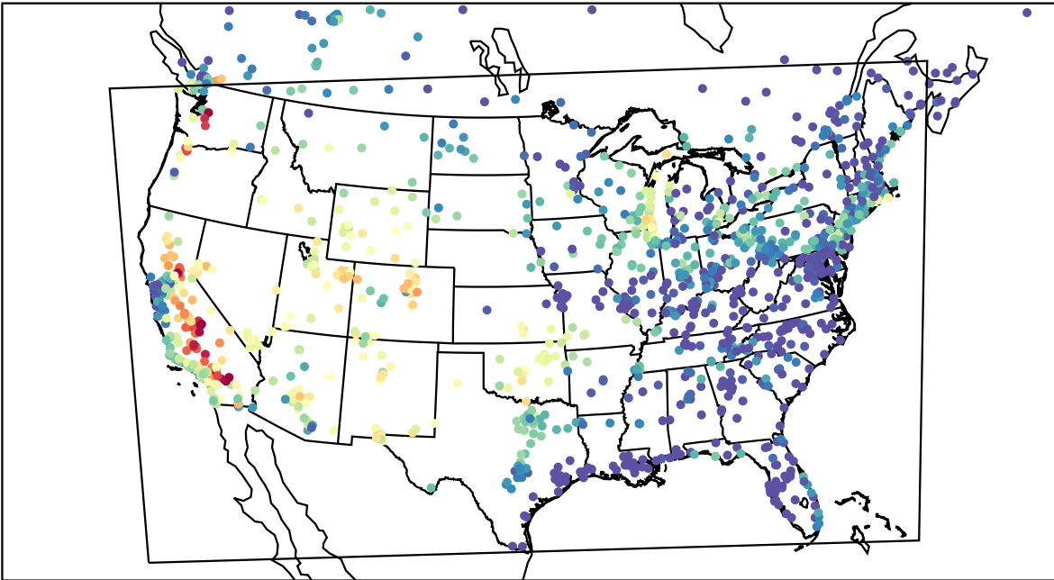
AirNOW (2022-07-27_02:00:00)
