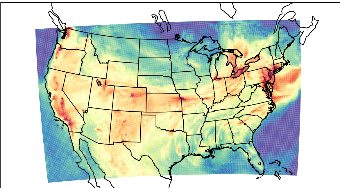
WRF (2022-07-27_21:00:00)
