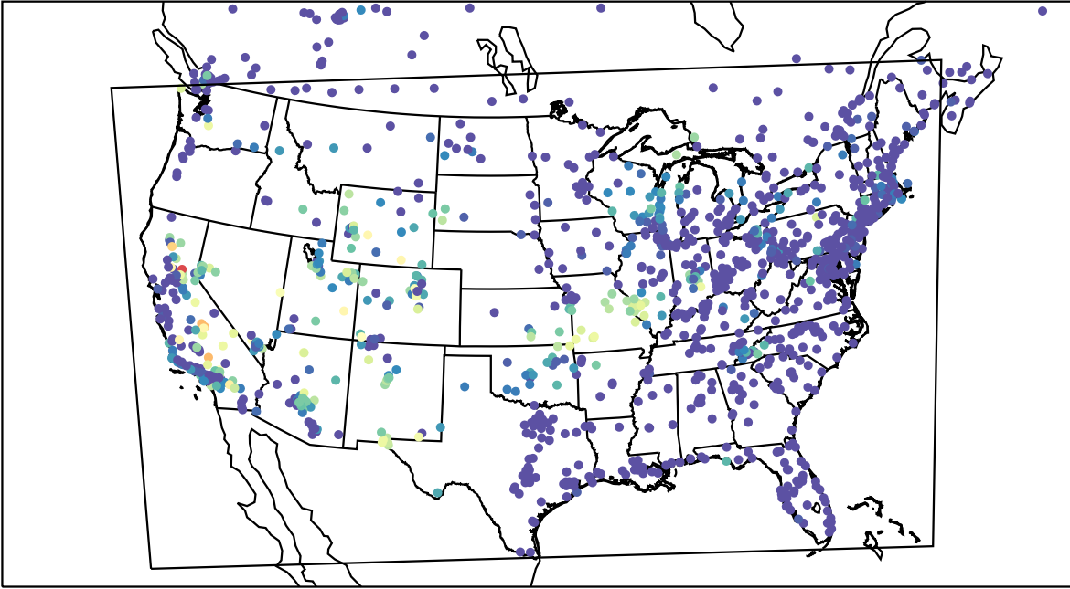
AirNOW (2022-07-27_11:00:00)
