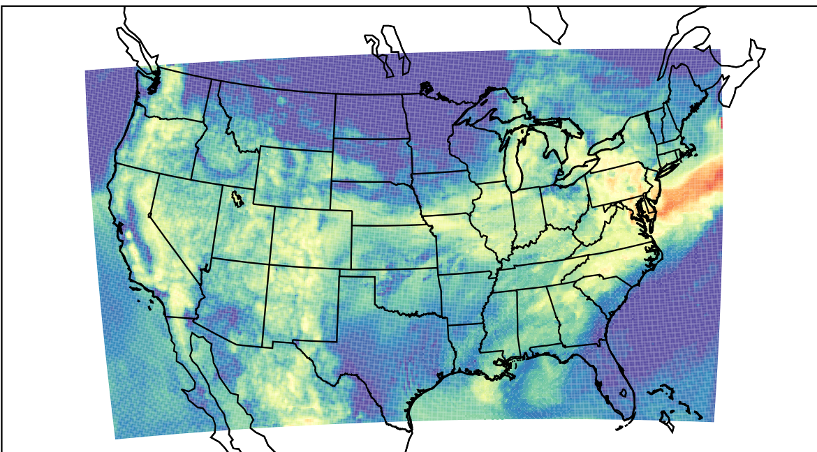
WRF (2022-07-27_14:00:00)
