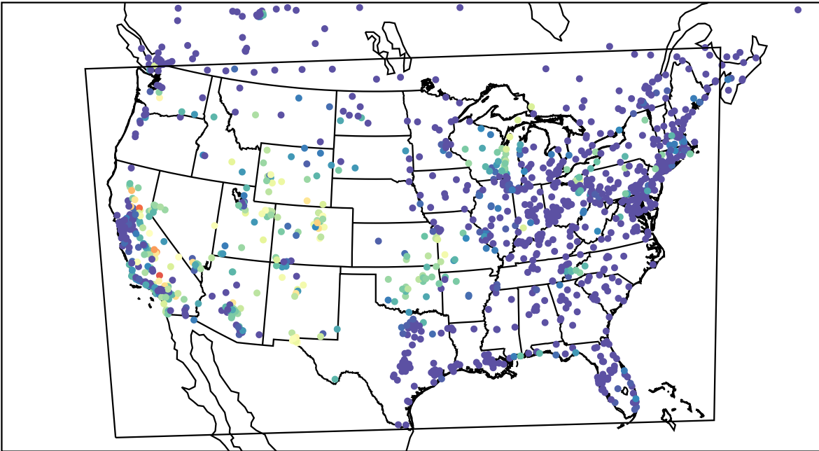
AirNOW (2022-07-27_08:00:00)
