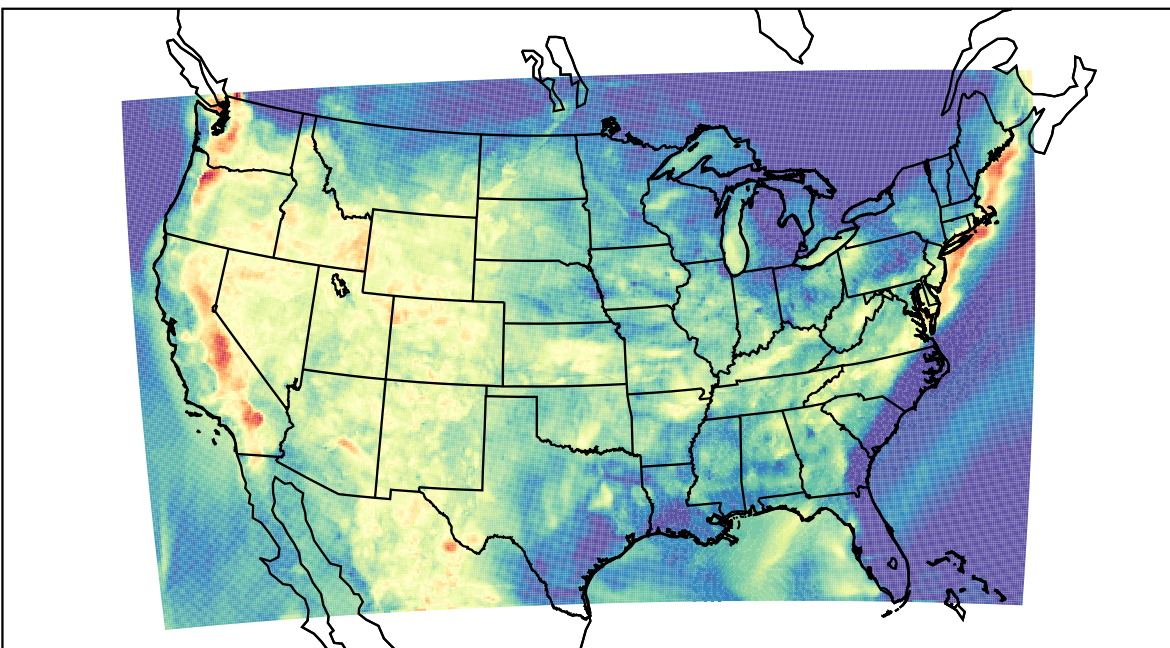
WRF (2022-07-26_03:00:00)
