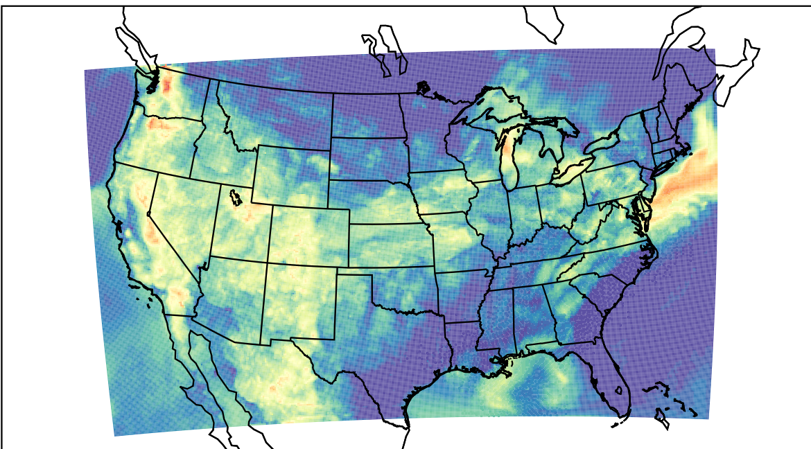
WRF (2022-07-27_08:00:00)
