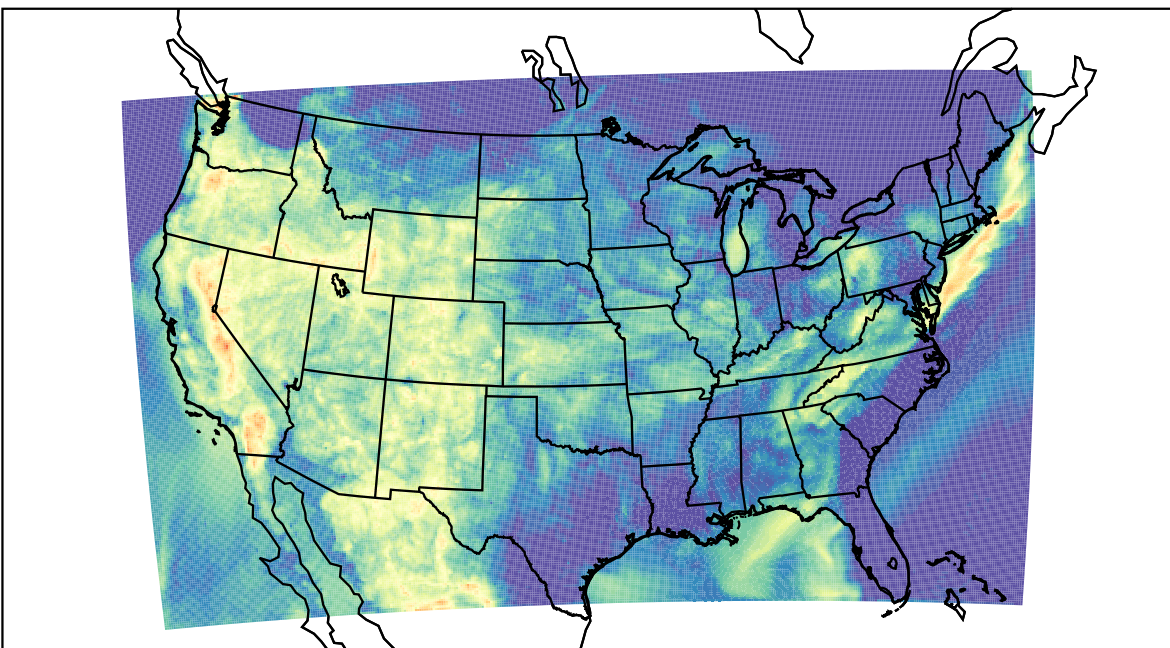
WRF (2022-07-26_07:00:00)
