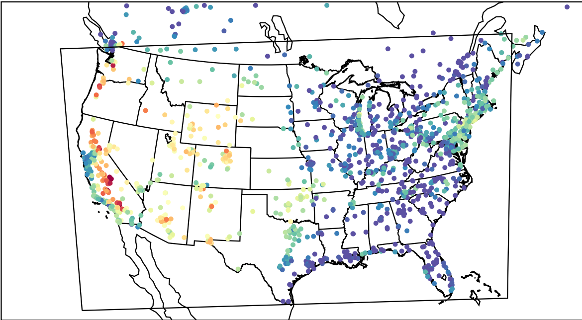
AirNOW (2022-07-26_02:00:00)
