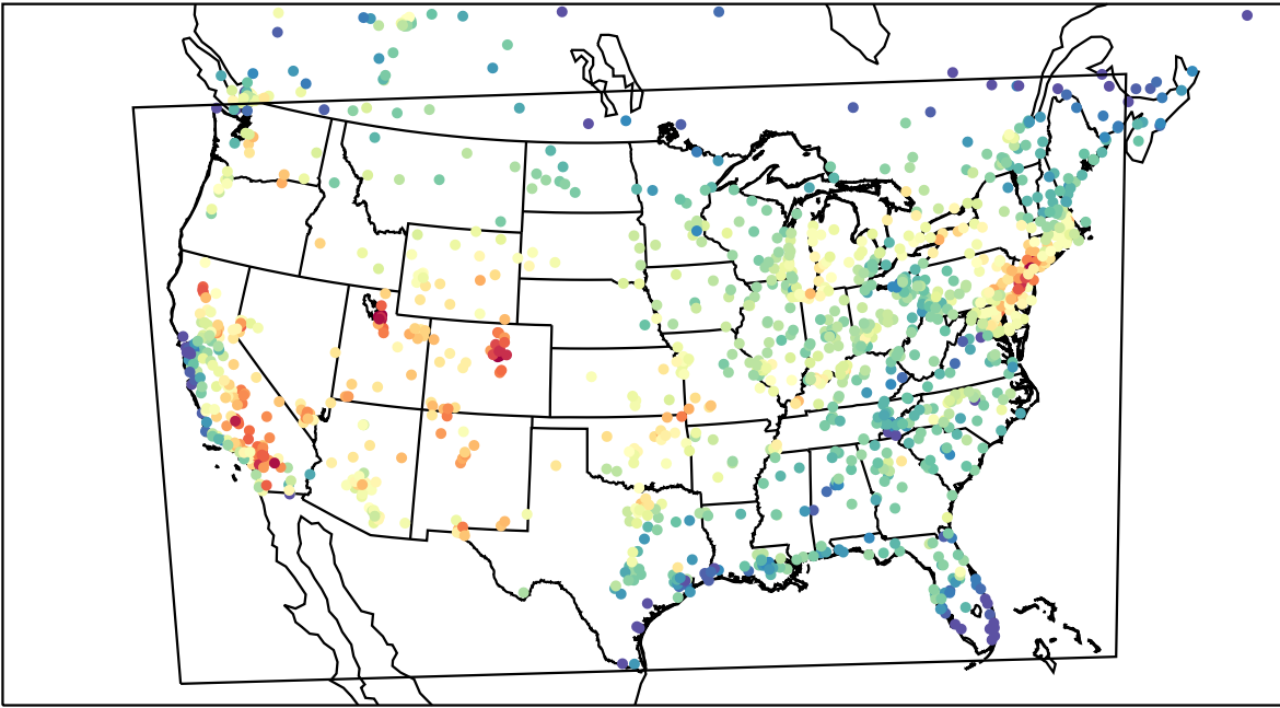
AirNOW (2022-07-27_19:00:00)
