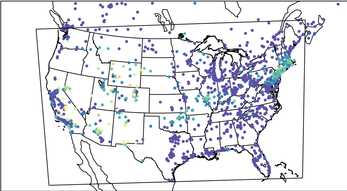
AirNOW (2022-07-26_12:00:00)
