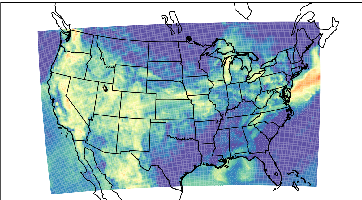
WRF (2022-07-27_10:00:00)
