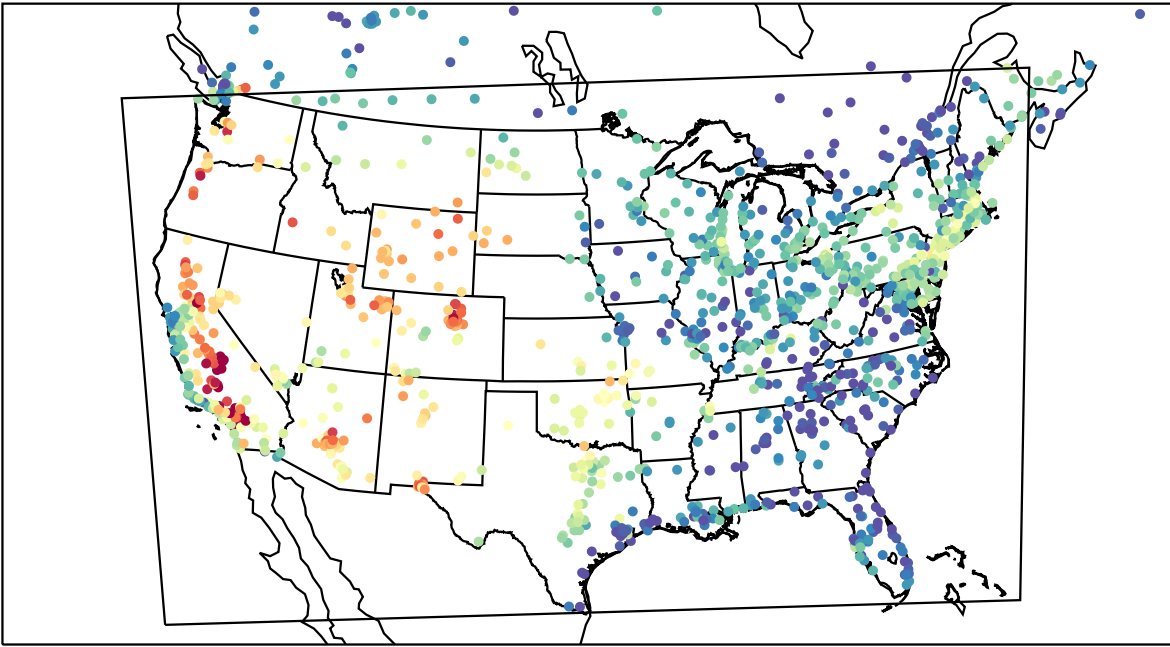
AirNOW (2022-07-26_00:00:00)
