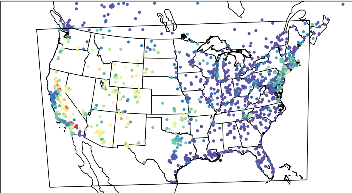
AirNOW (2022-07-26_04:00:00)
