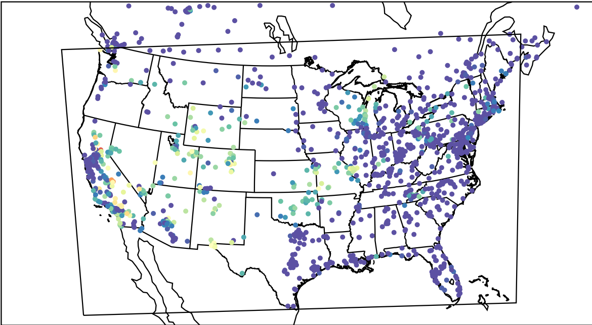
AirNOW (2022-07-27_09:00:00)
