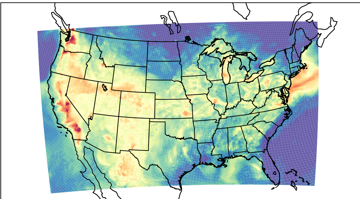
WRF (2022-07-27_02:00:00)
