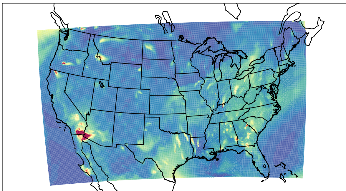
WRF 2022-08-04_05:00:00
