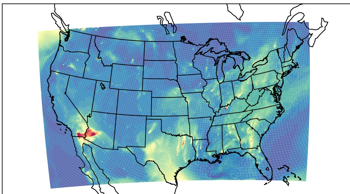
WRF 2022-08-04_11:00:00
