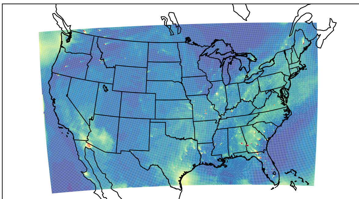
WRF 2022-08-04_22:00:00
