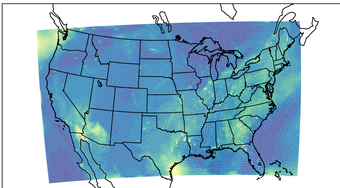
WRF 2022-08-04_20:00:00
