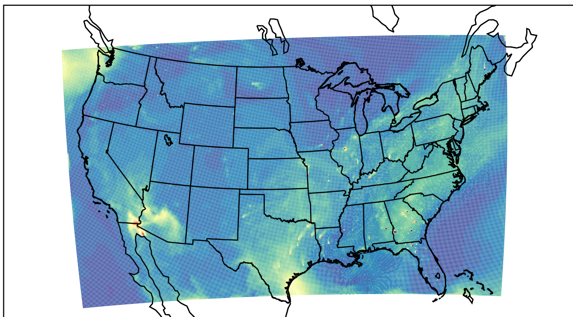
WRF 2022-08-04_18:00:00
