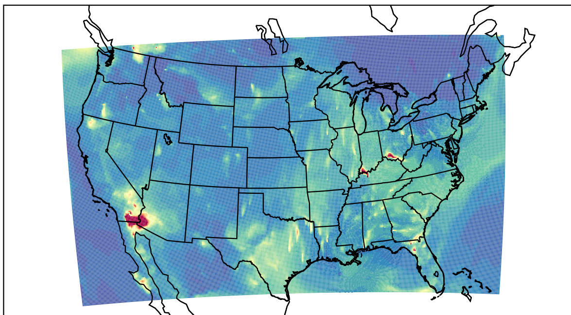
WRF 2022-08-03_07:00:00
