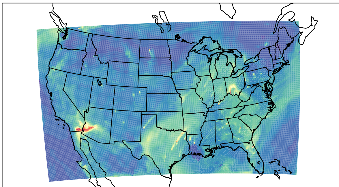
WRF 2022-08-03_15:00:00
