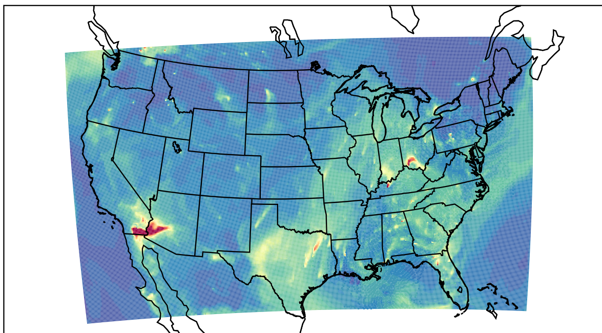
WRF 2022-08-03_12:00:00
