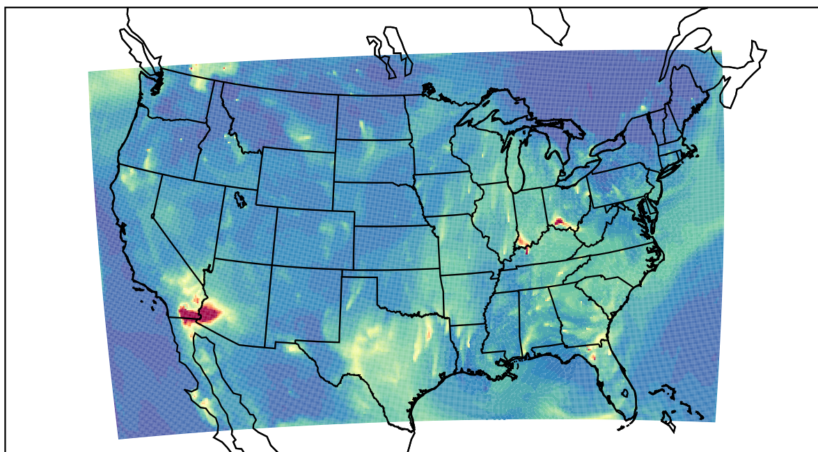
WRF 2022-08-03_09:00:00
