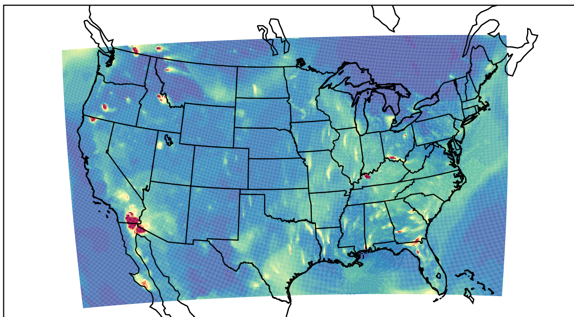
WRF 2022-08-03_04:00:00
