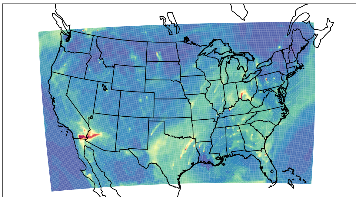
WRF 2022-08-03_14:00:00
