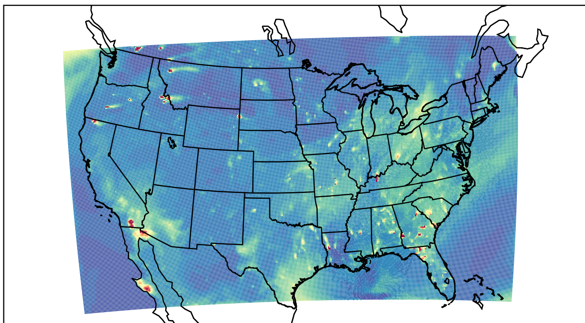
WRF 2022-08-04_02:00:00
