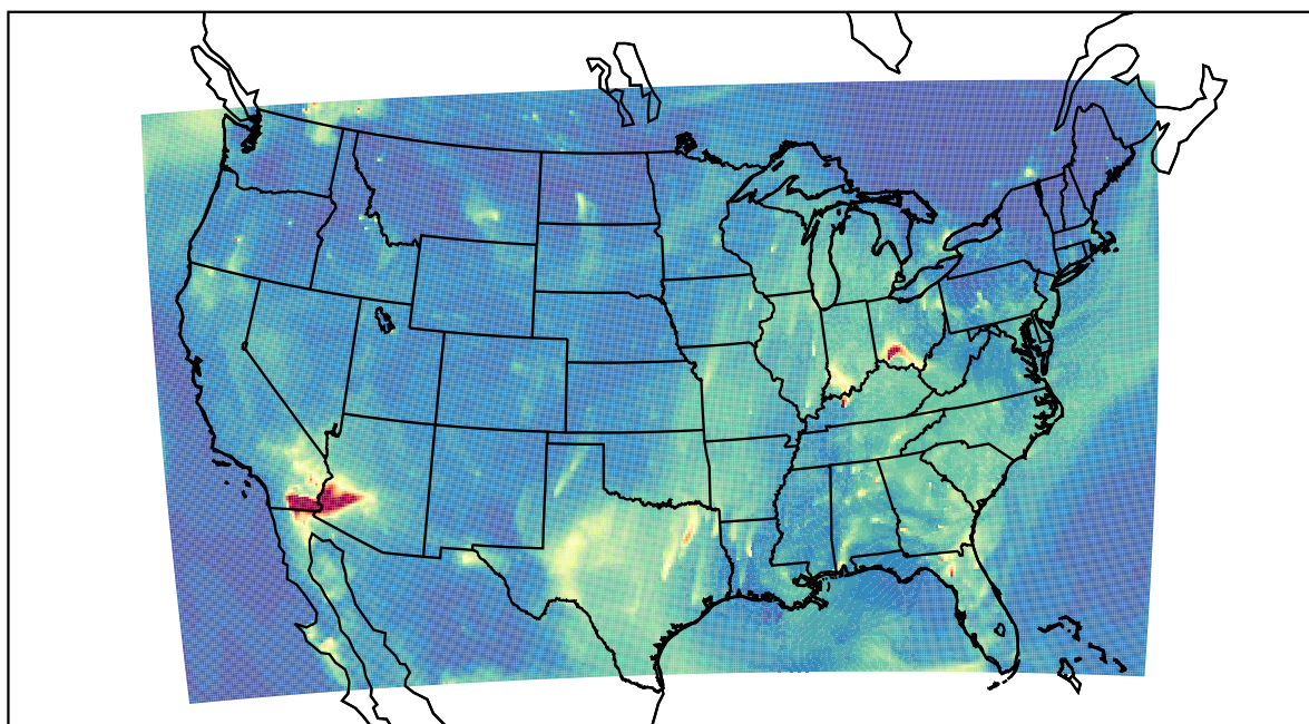
WRF 2022-08-03_11:00:00
