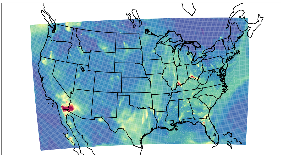
WRF 2022-08-03_08:00:00
