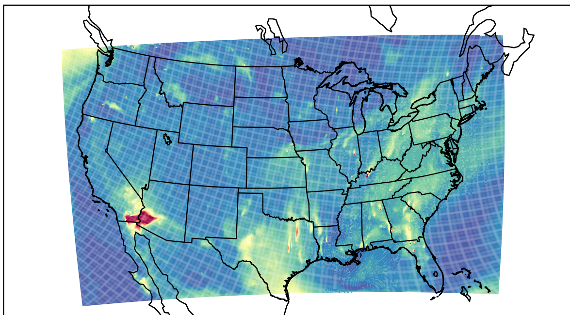
WRF 2022-08-04_09:00:00
