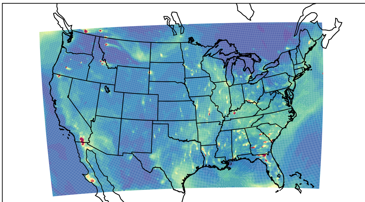
WRF 2022-08-03_02:00:00
