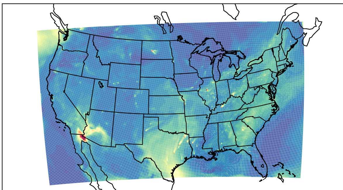
WRF 2022-08-04_16:00:00
