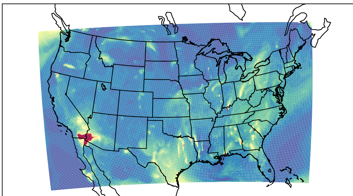
WRF 2022-08-04_07:00:00
