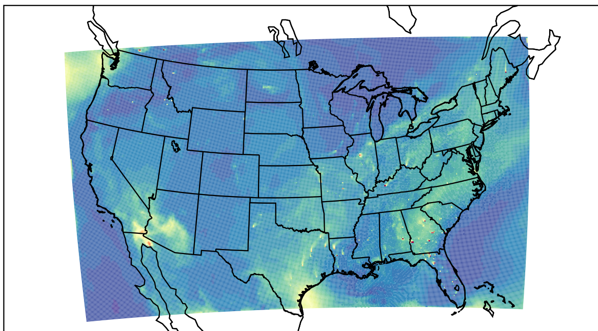
WRF 2022-08-04_19:00:00
