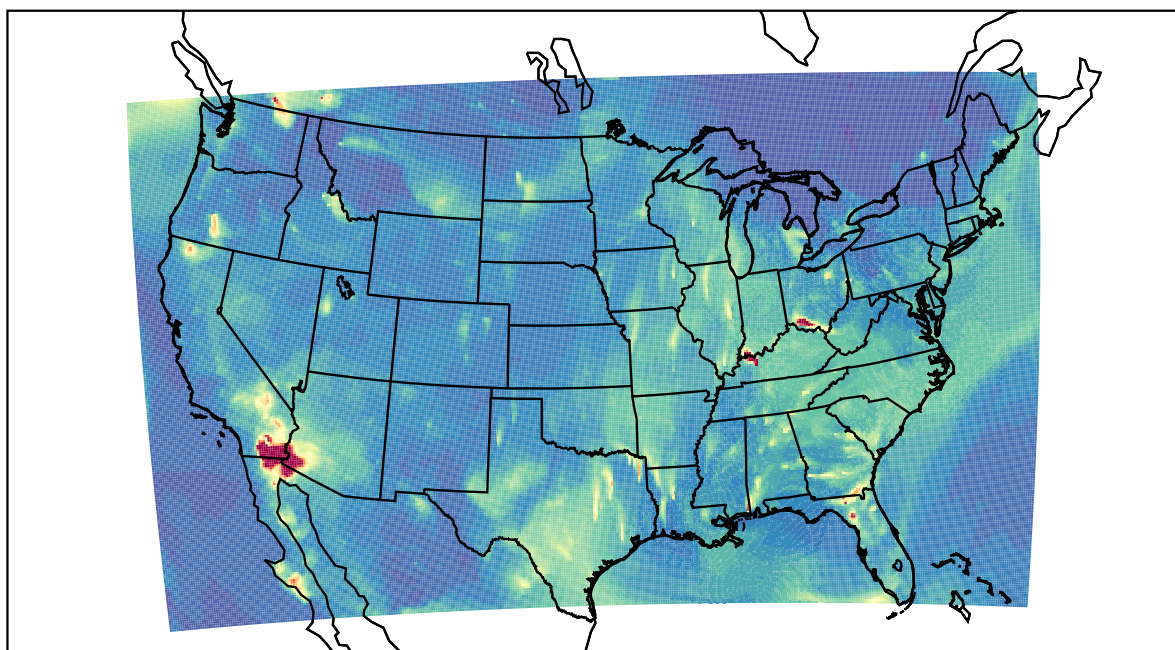
WRF 2022-08-03_06:00:00
