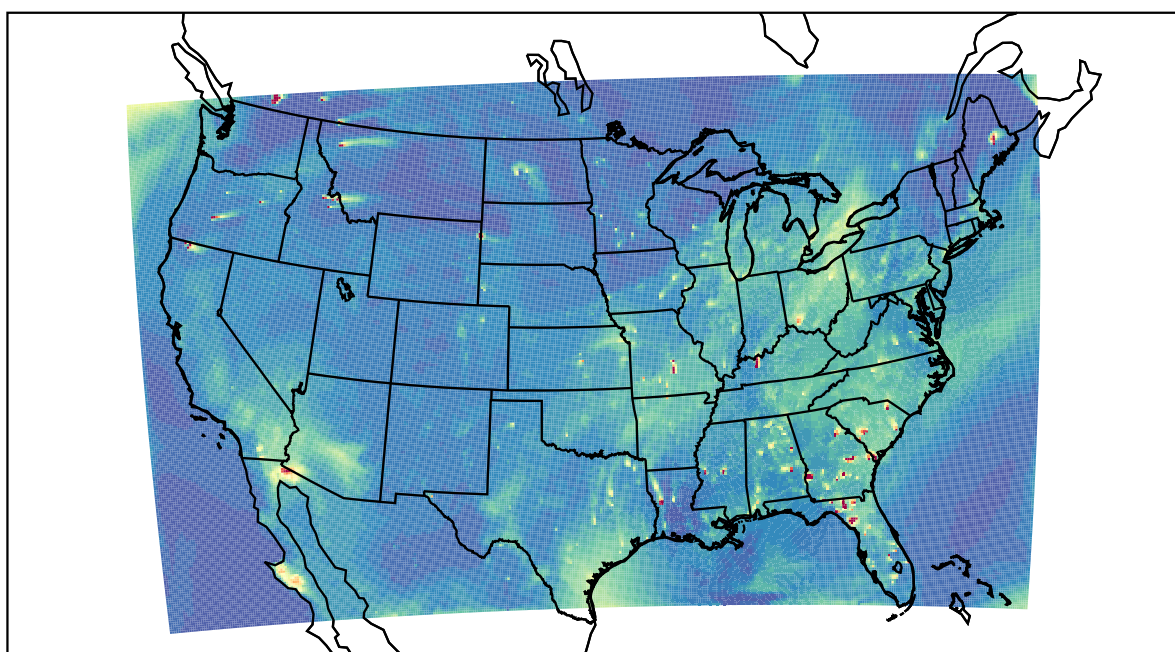
WRF 2022-08-04_01:00:00
