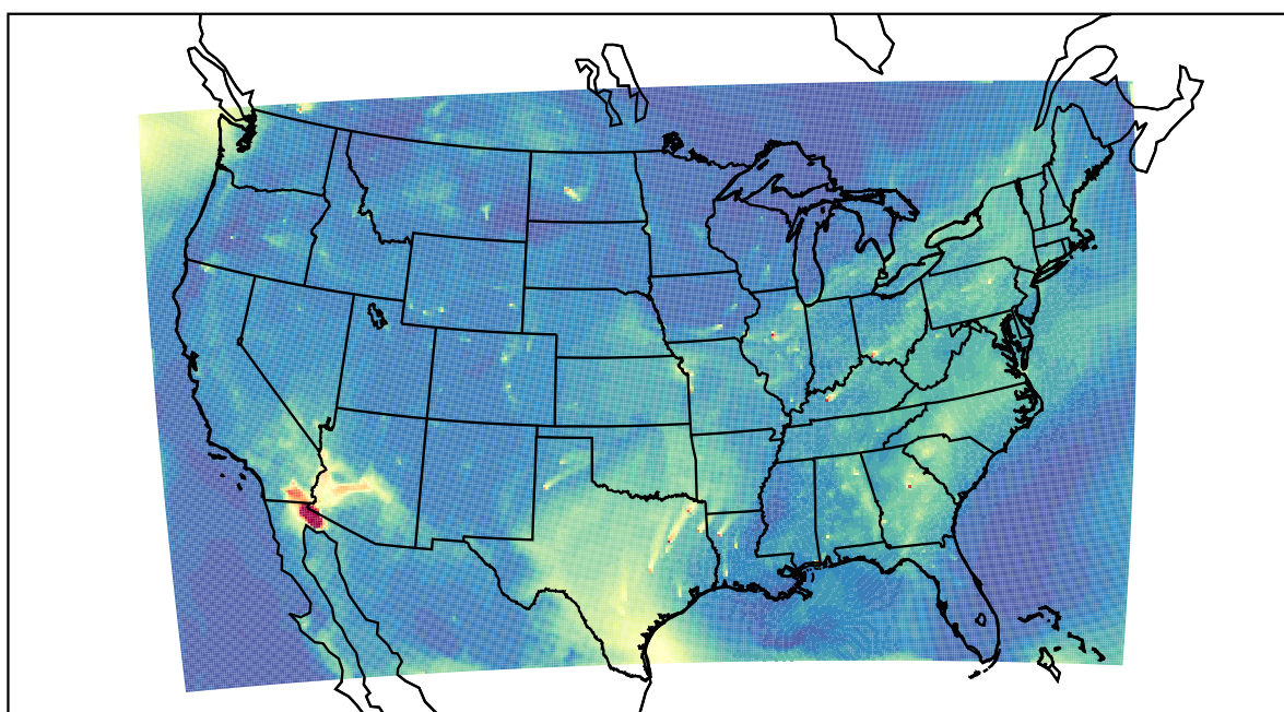
WRF 2022-08-04_15:00:00
