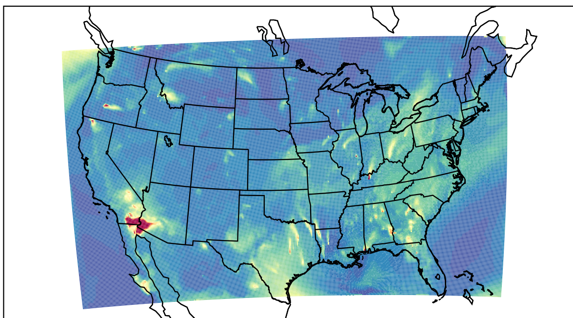
WRF 2022-08-04_06:00:00
