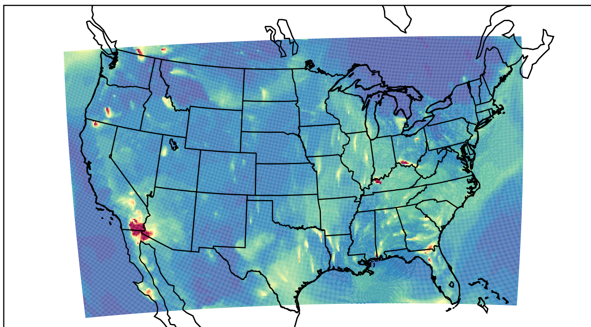
WRF 2022-08-03_05:00:00
