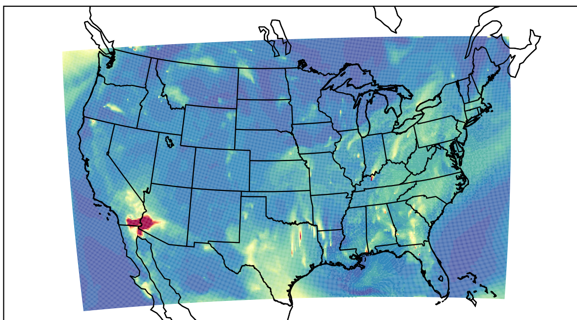
WRF 2022-08-04_08:00:00
