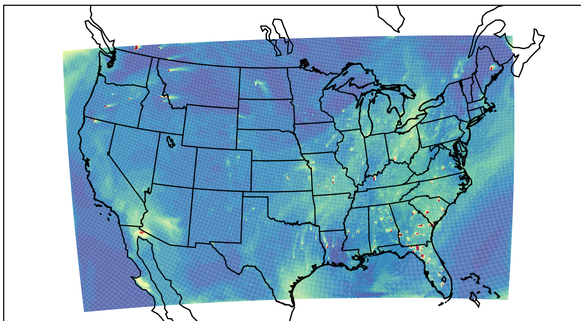
WRF 2022-08-04_00:00:00
