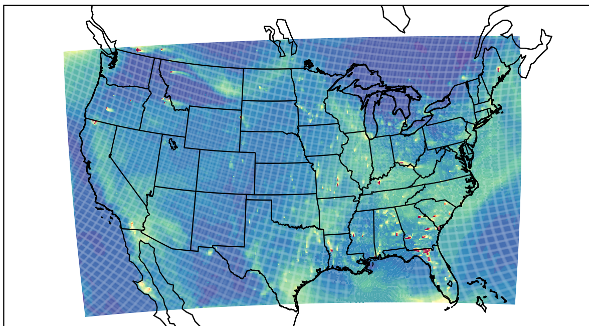
WRF 2022-08-03_01:00:00
