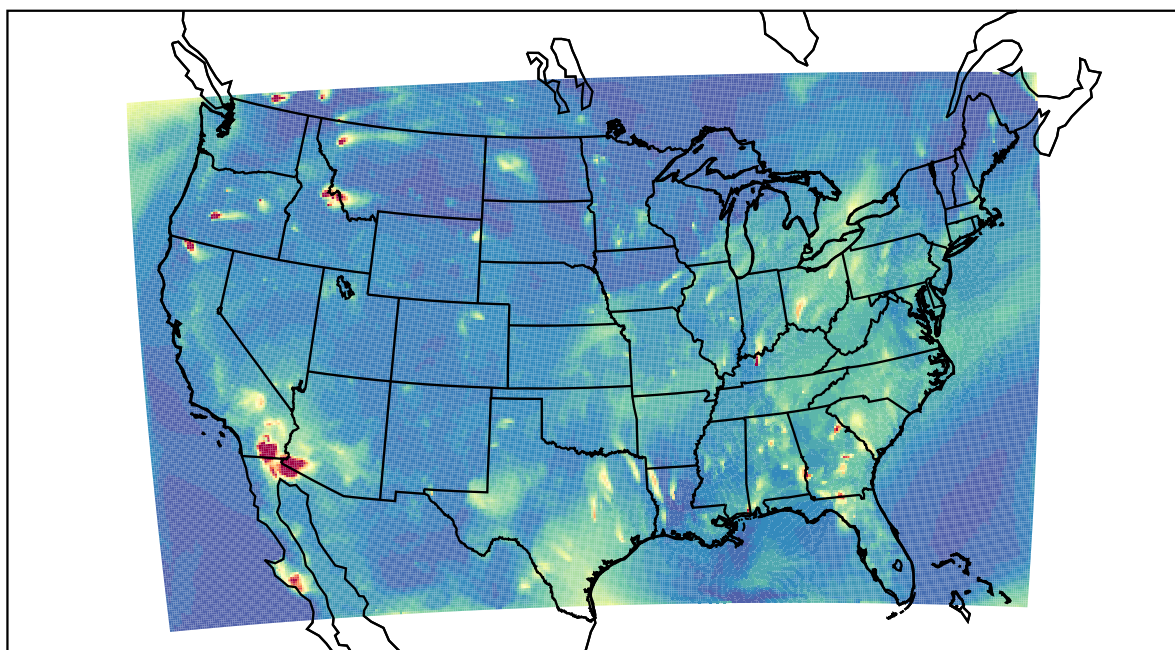
WRF 2022-08-04_04:00:00
