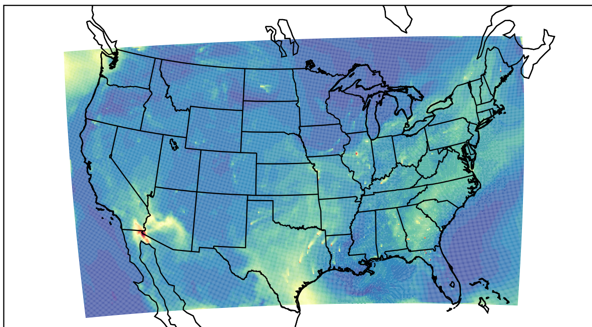
WRF 2022-08-04_17:00:00
