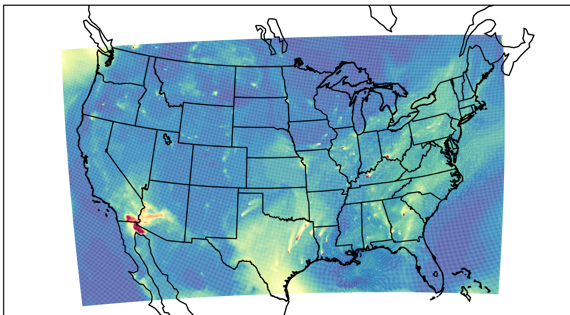
WRF 2022-08-04_14:00:00
