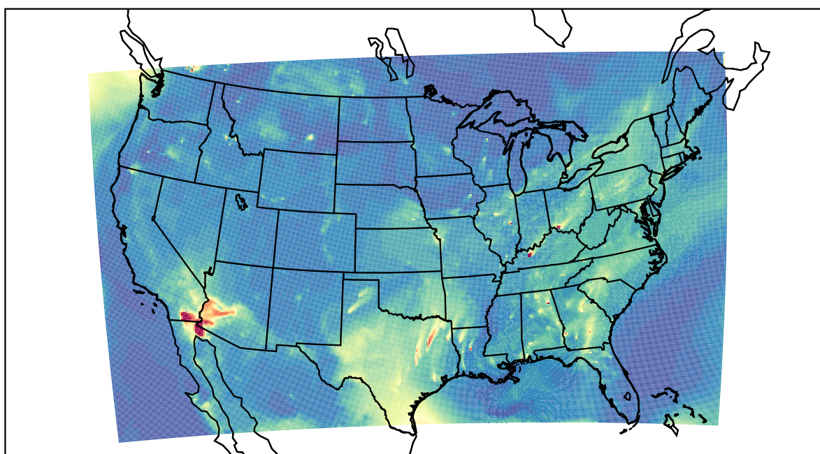
WRF 2022-08-04_13:00:00
