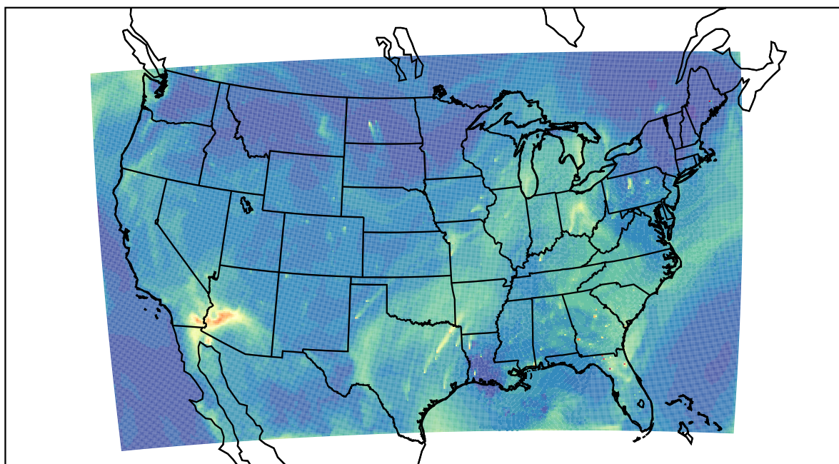
WRF 2022-08-03_17:00:00
