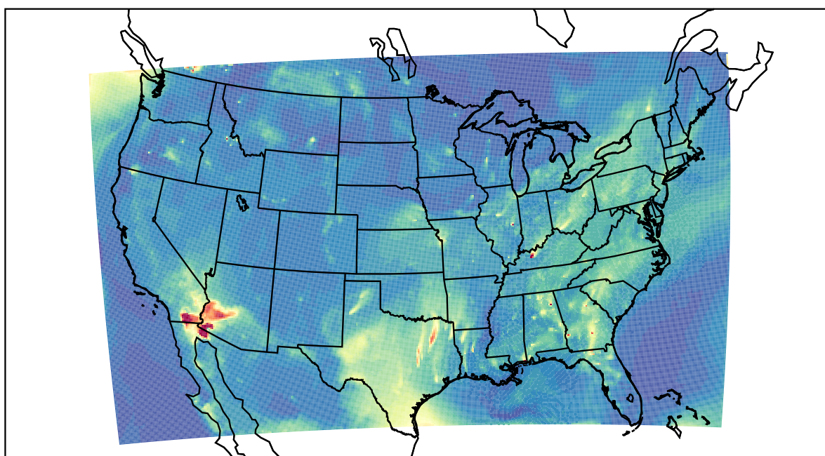
WRF 2022-08-04_12:00:00
