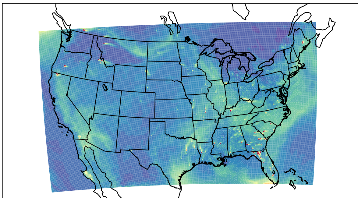
WRF 2022-08-03_00:00:00
