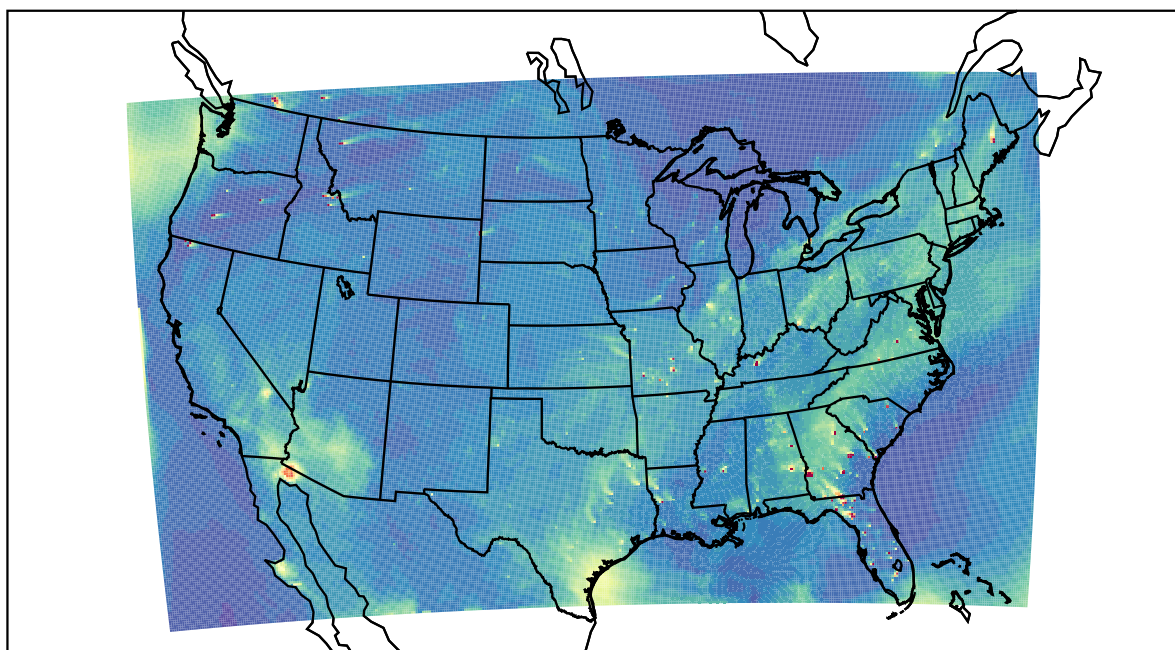
WRF 2022-08-04_23:00:00
