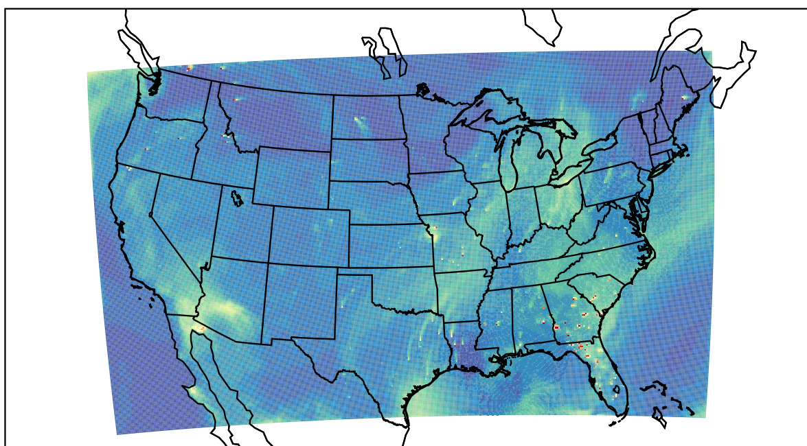
WRF 2022-08-03_21:00:00
