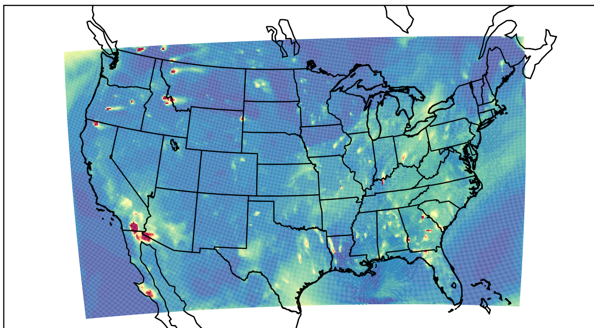
WRF 2022-08-04_03:00:00
