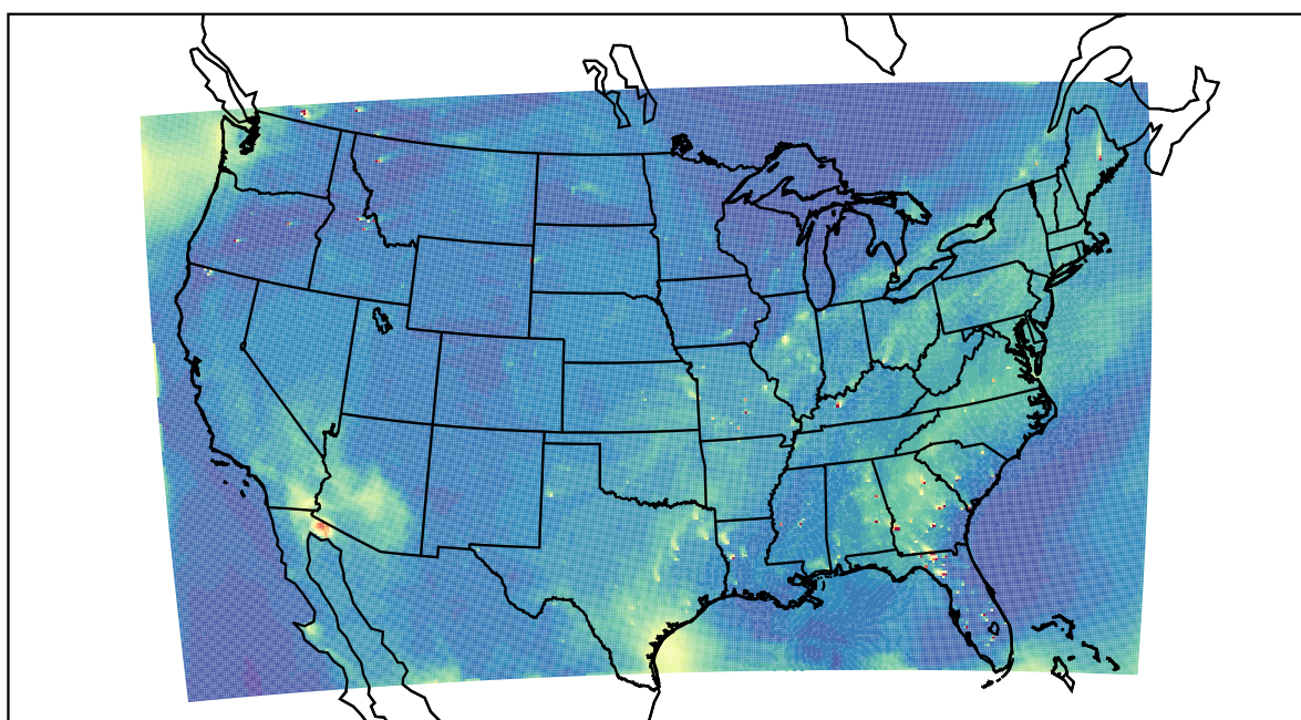
WRF 2022-08-04_21:00:00
