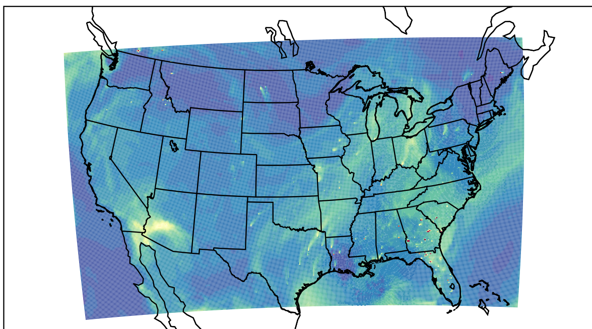
WRF 2022-08-03_19:00:00
