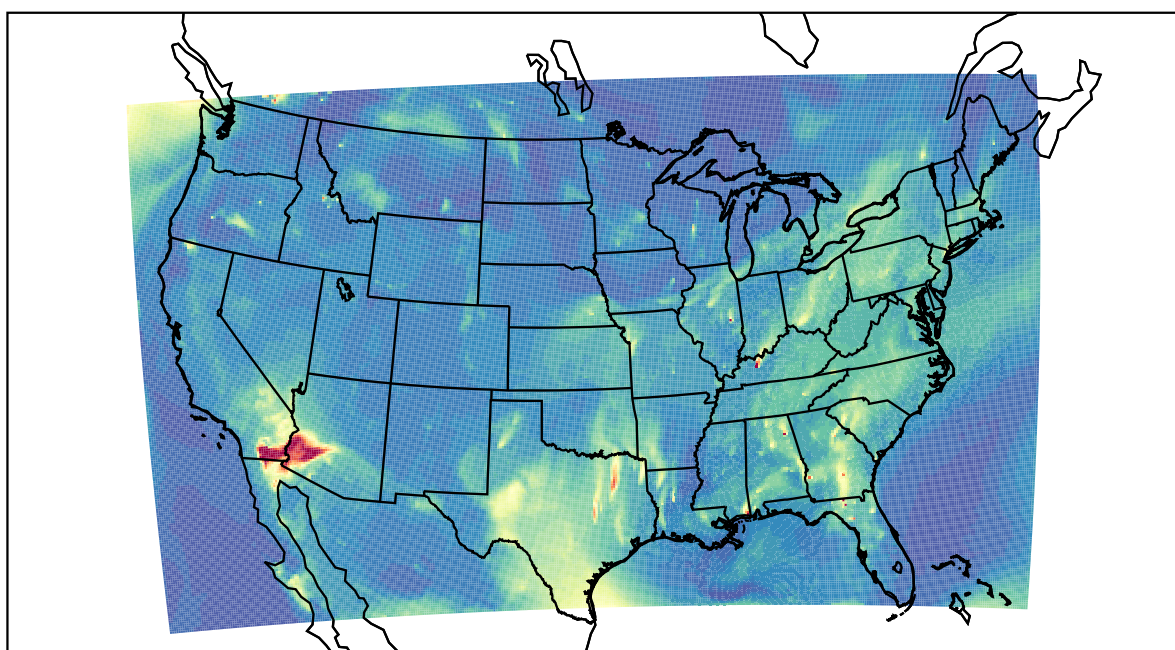
WRF 2022-08-04_10:00:00
