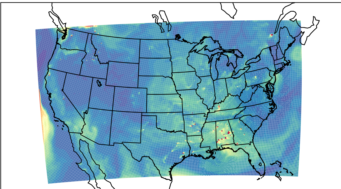
WRF 2022-08-17_21:00:00
