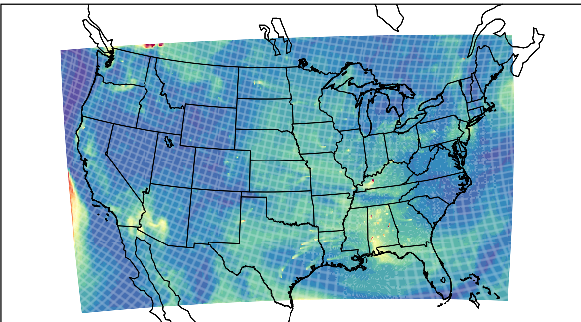
WRF 2022-08-17_17:00:00
