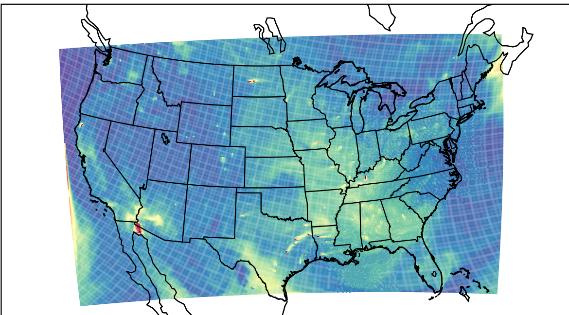
WRF 2022-08-16_16:00:00
