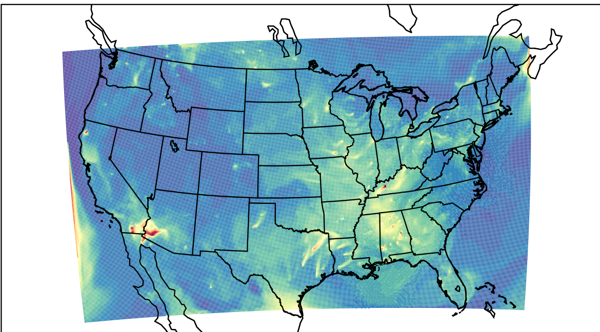
WRF 2022-08-16_11:00:00
