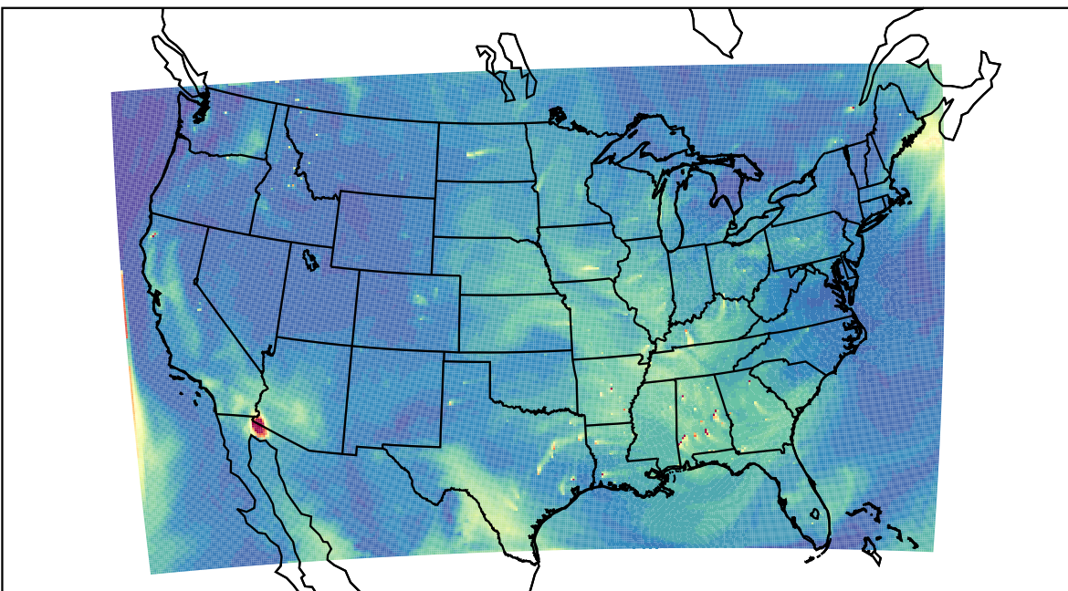
WRF 2022-08-16_19:00:00
