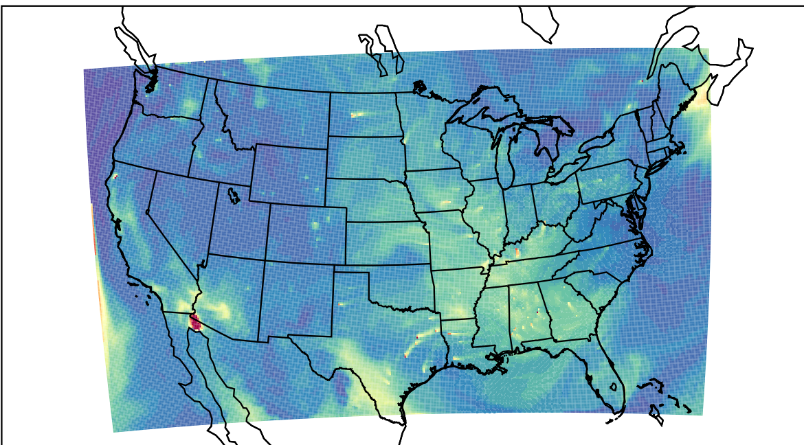
WRF 2022-08-16_17:00:00
