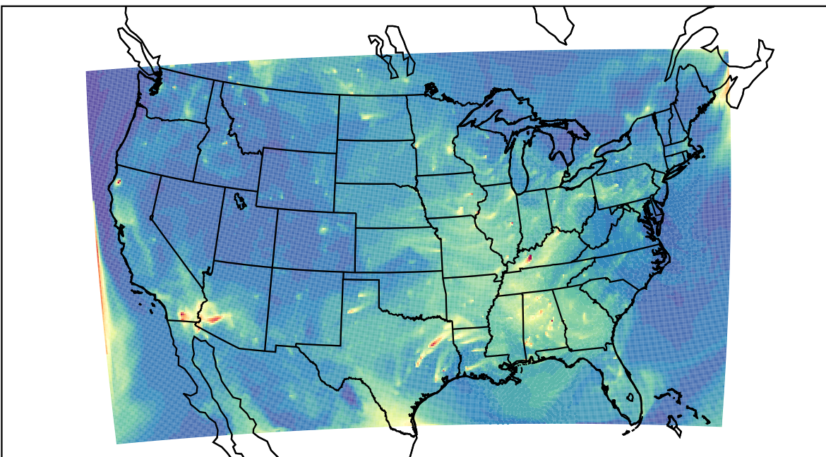
WRF 2022-08-16_13:00:00
