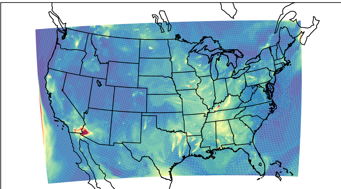
WRF 2022-08-16_09:00:00
