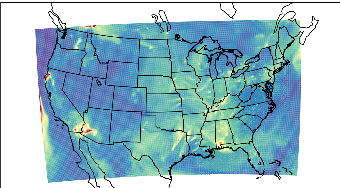
WRF 2022-08-17_11:00:00
