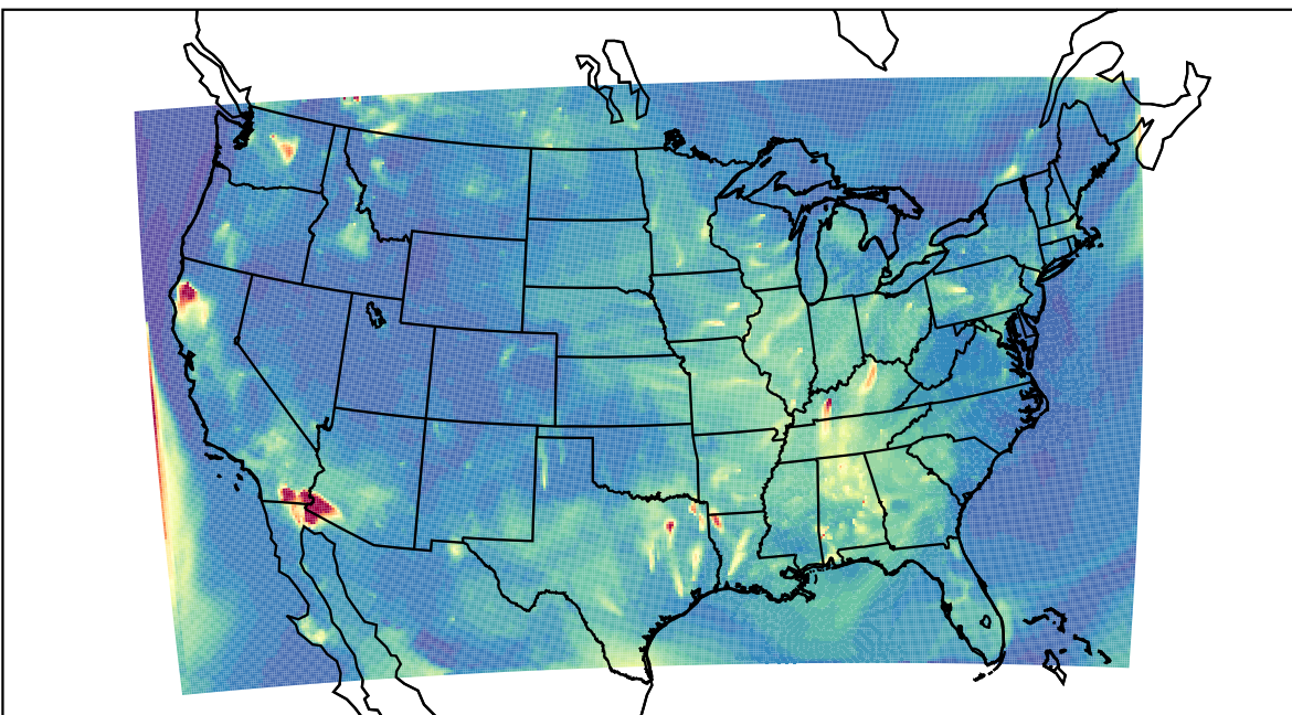
WRF 2022-08-16_06:00:00
