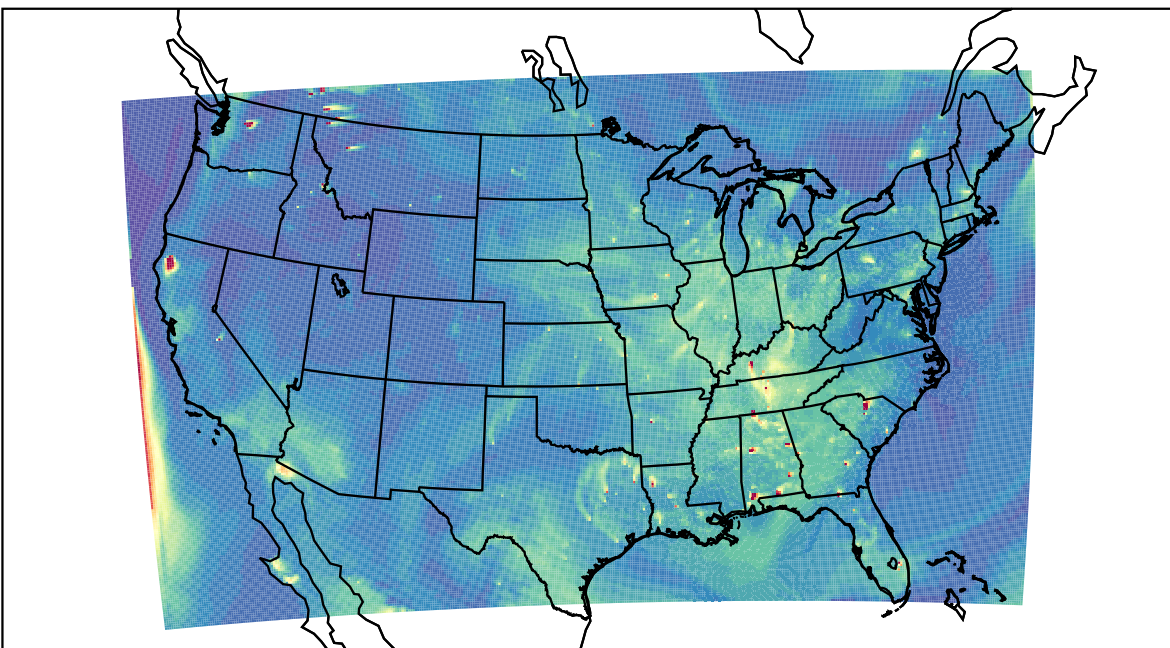
WRF 2022-08-16_00:00:00
