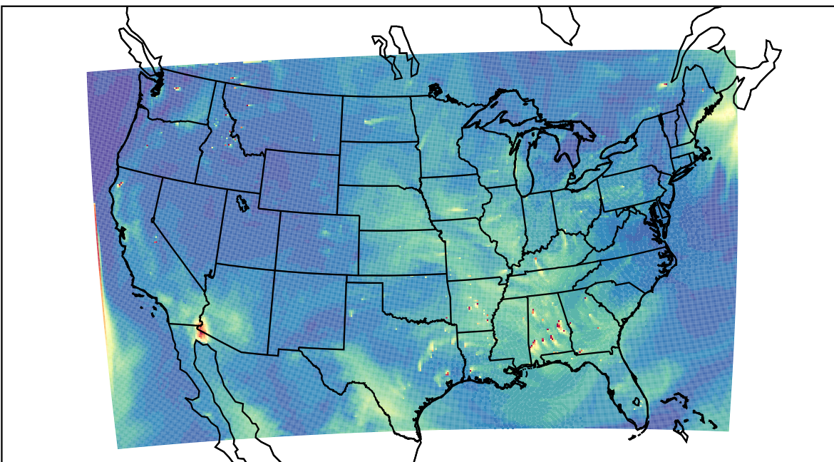
WRF 2022-08-16_21:00:00
