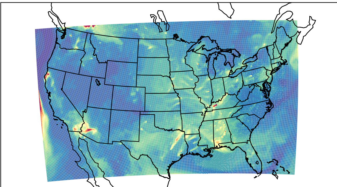
WRF 2022-08-17_12:00:00
