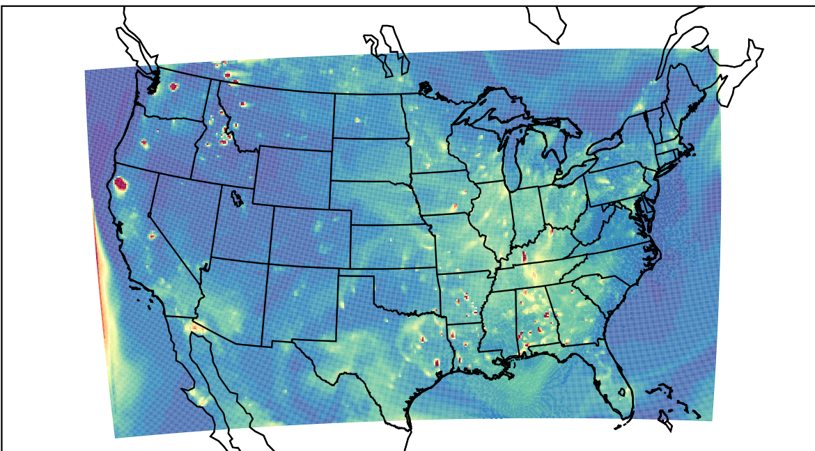
WRF 2022-08-16_02:00:00
