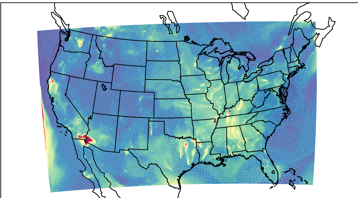
WRF 2022-08-16_07:00:00
