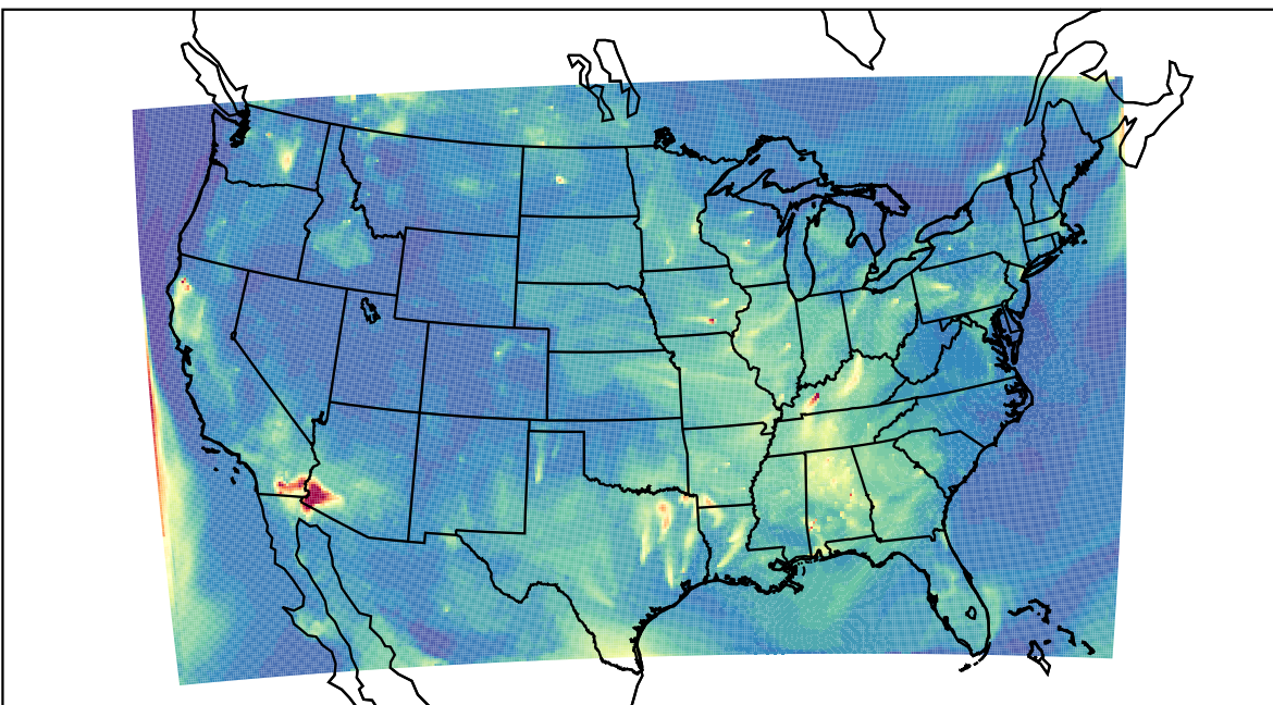
WRF 2022-08-16_08:00:00
