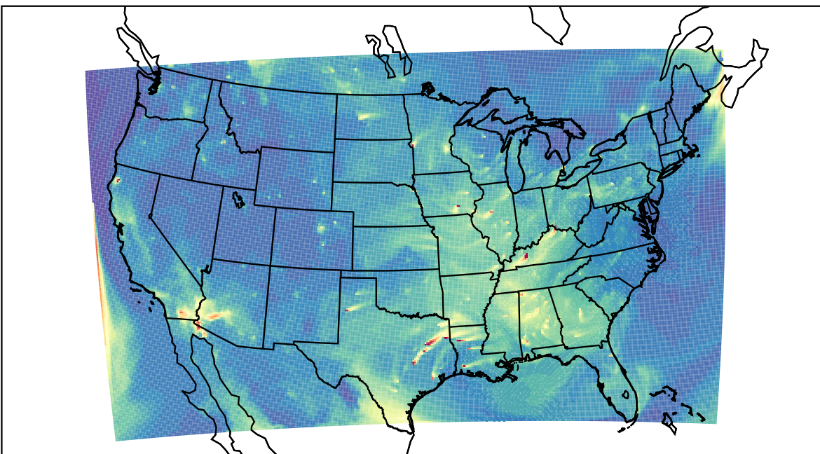
WRF 2022-08-16_14:00:00
