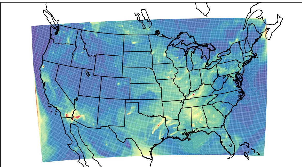
WRF 2022-08-16_12:00:00
