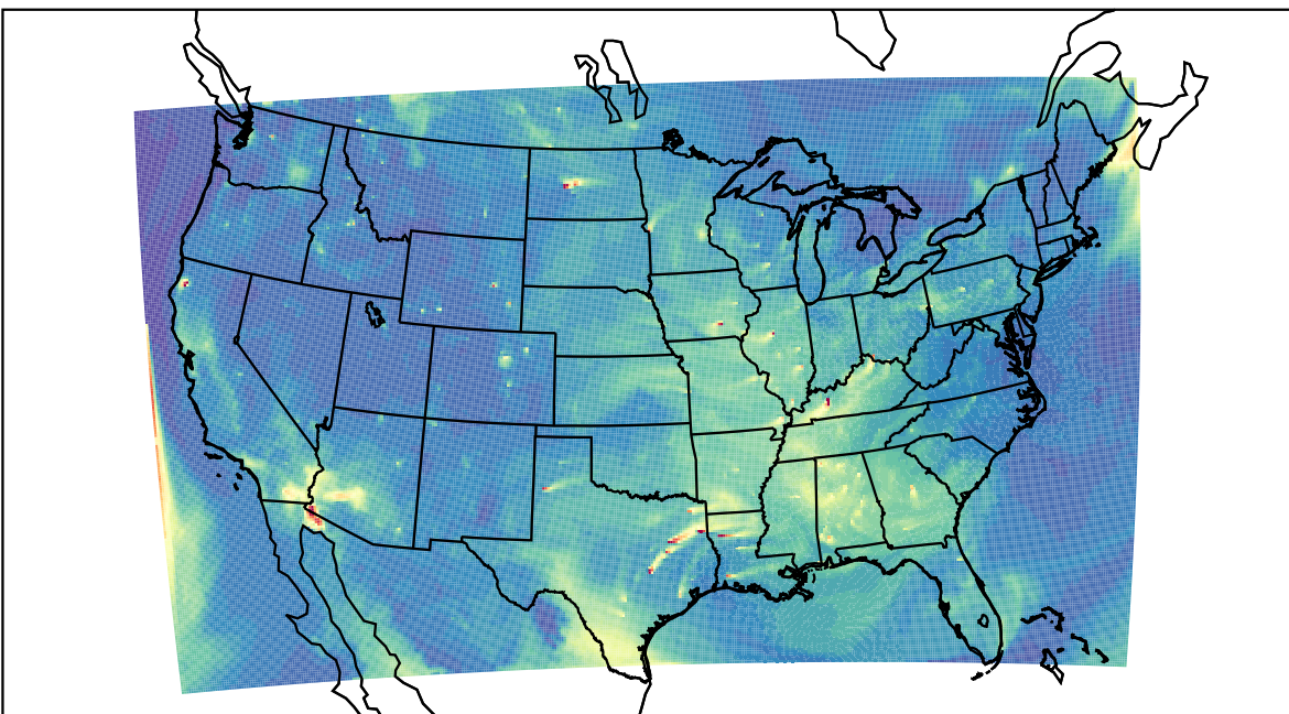
WRF 2022-08-16_15:00:00
