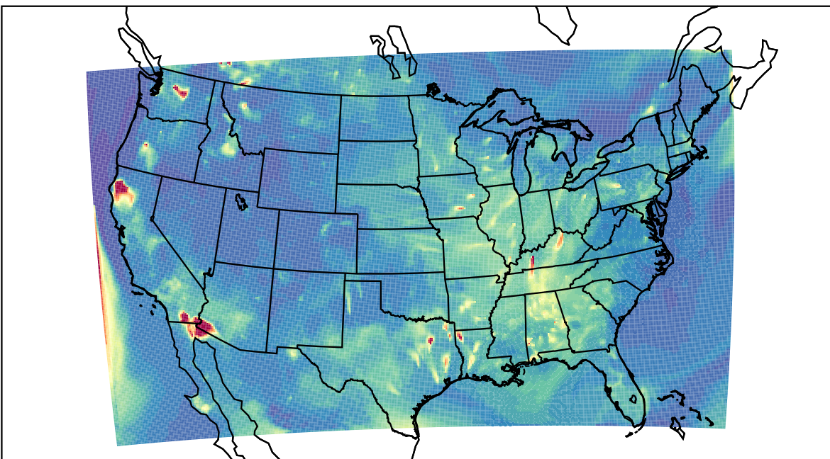
WRF 2022-08-16_05:00:00
