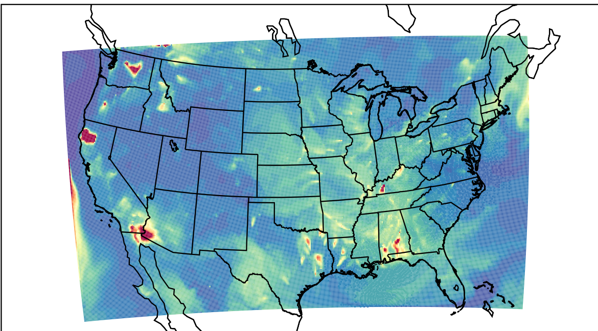
WRF 2022-08-17_05:00:00
