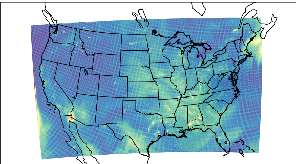
WRF 2022-08-16_22:00:00
