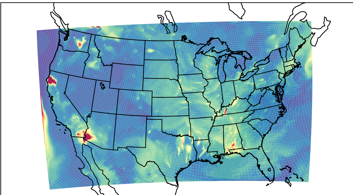
WRF 2022-08-17_07:00:00
