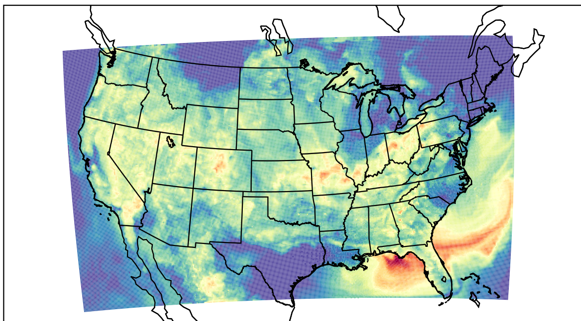
WRF (2022-08-18_08:00:00)
