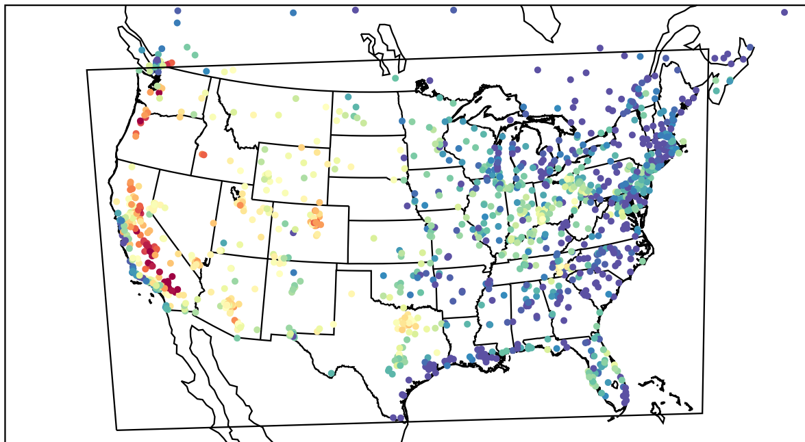
AirNOW (2022-08-18_01:00:00)
