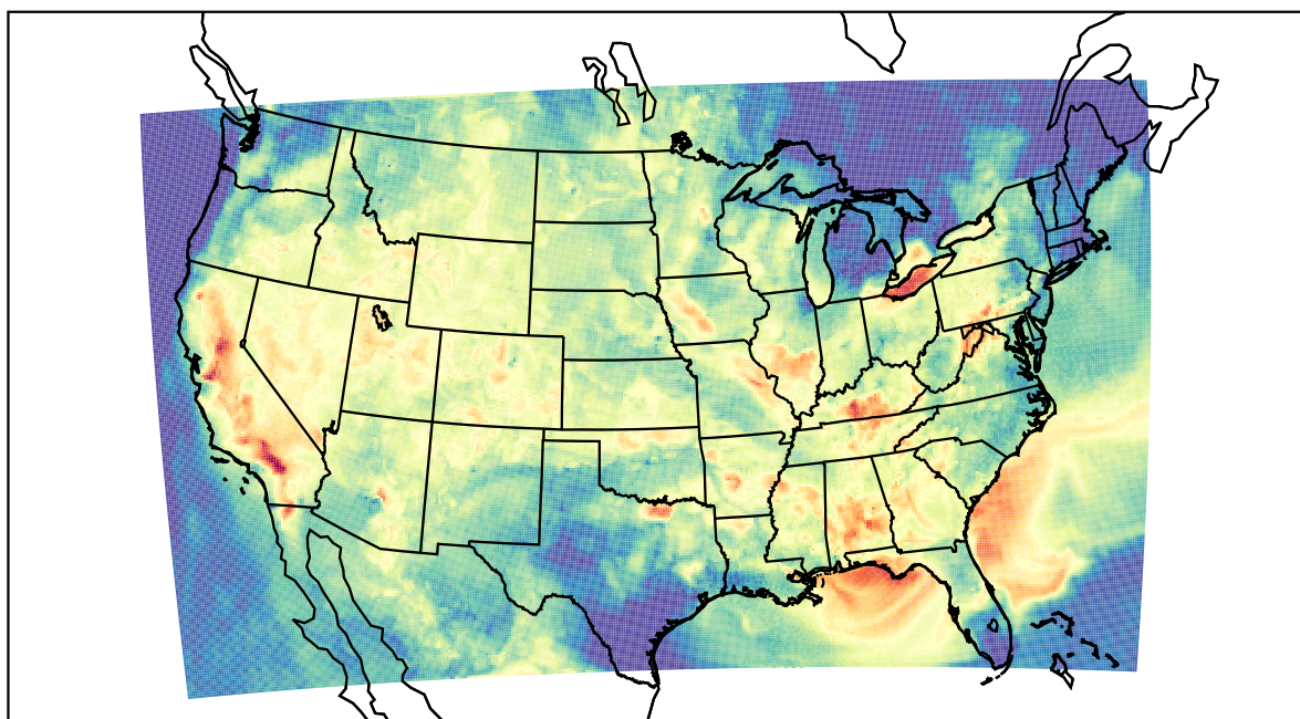
WRF (2022-08-17_02:00:00)
