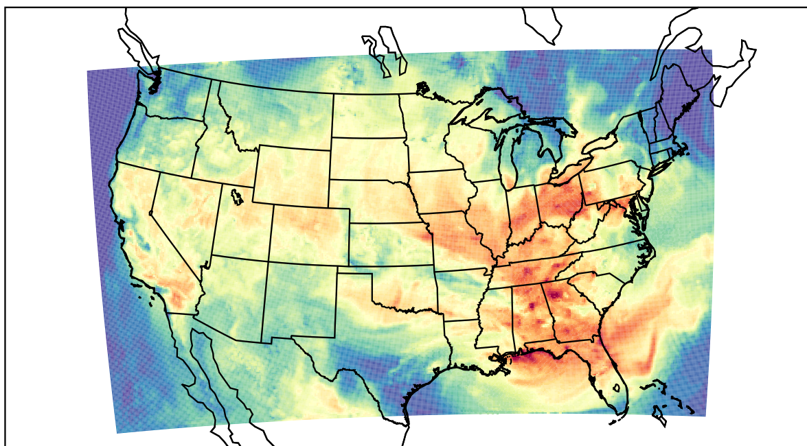
WRF (2022-08-17_17:00:00)
