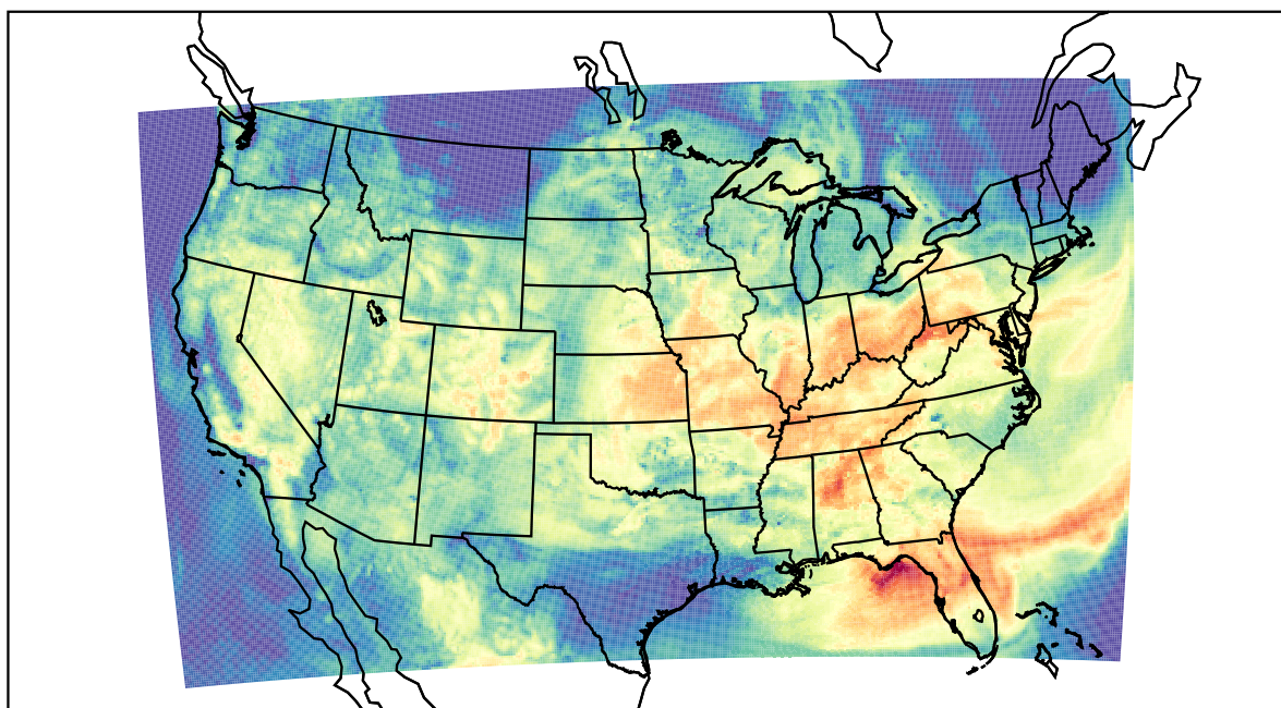
WRF (2022-08-18_15:00:00)
