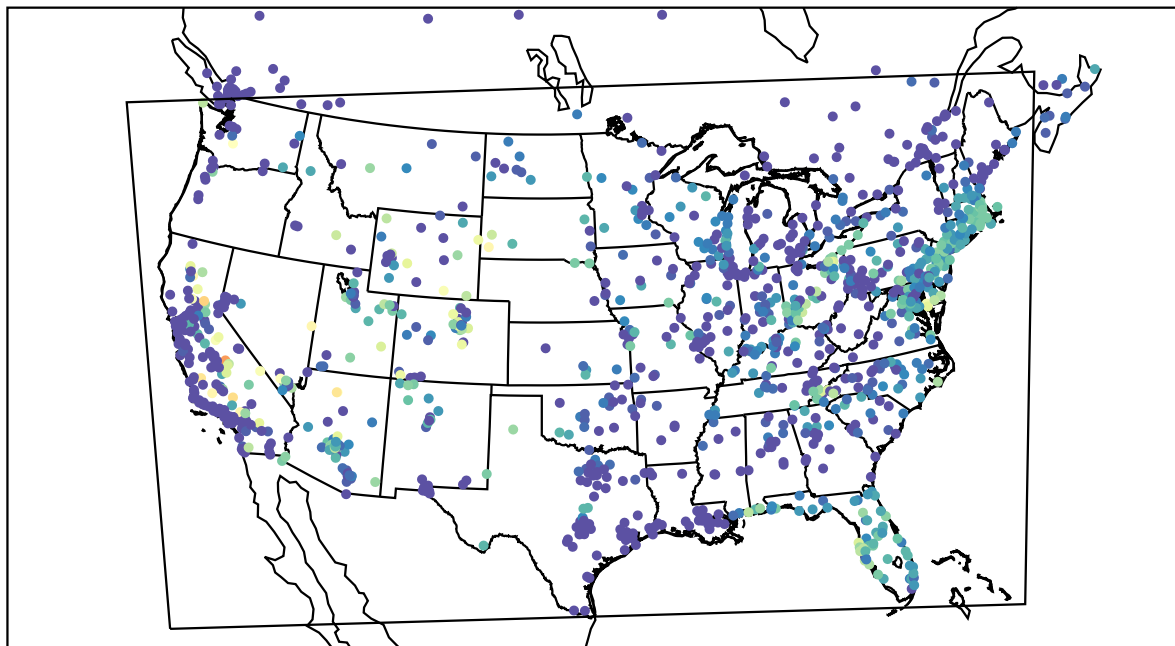
AirNOW (2022-08-18_13:00:00)
