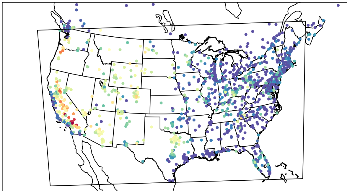
AirNOW (2022-08-18_03:00:00)
