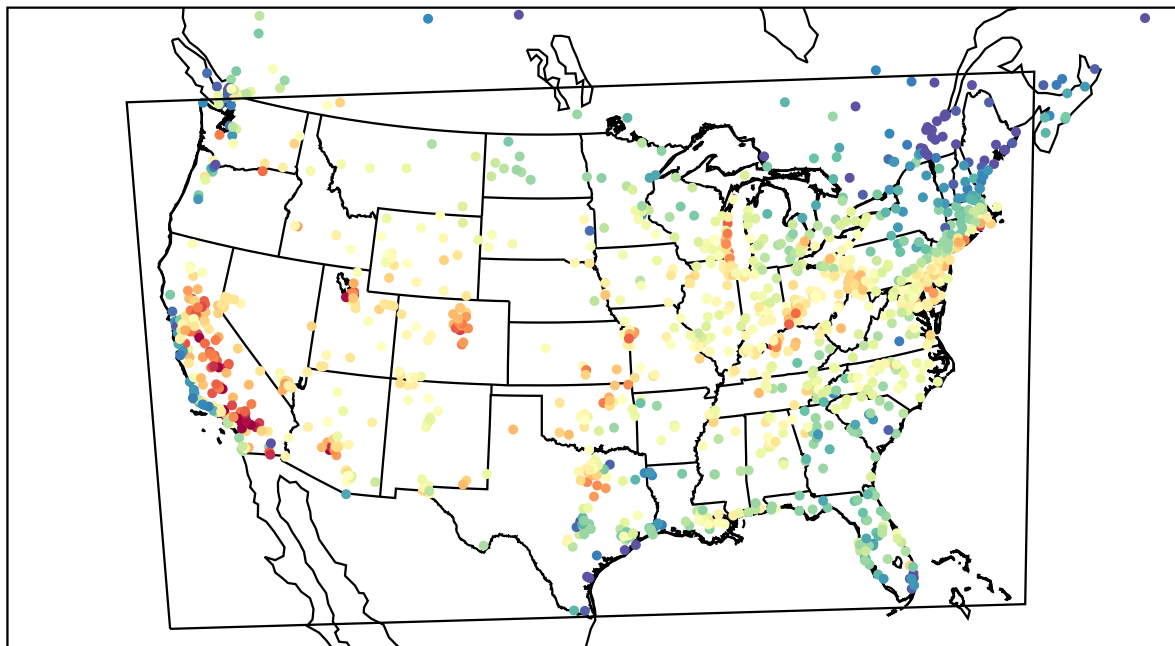
AirNOW (2022-08-18_21:00:00)
