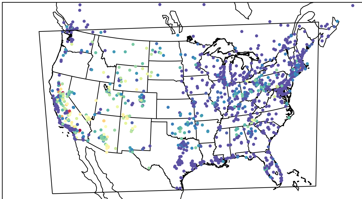
AirNOW (2022-08-17_08:00:00)
