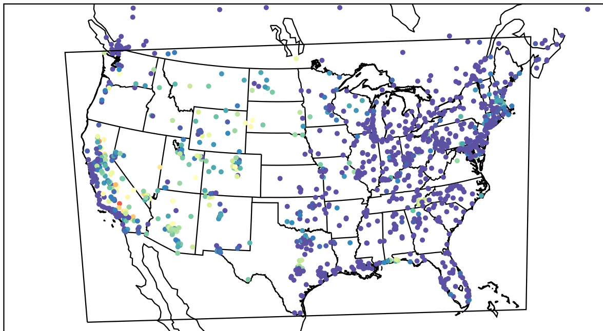
AirNOW (2022-08-18_09:00:00)
