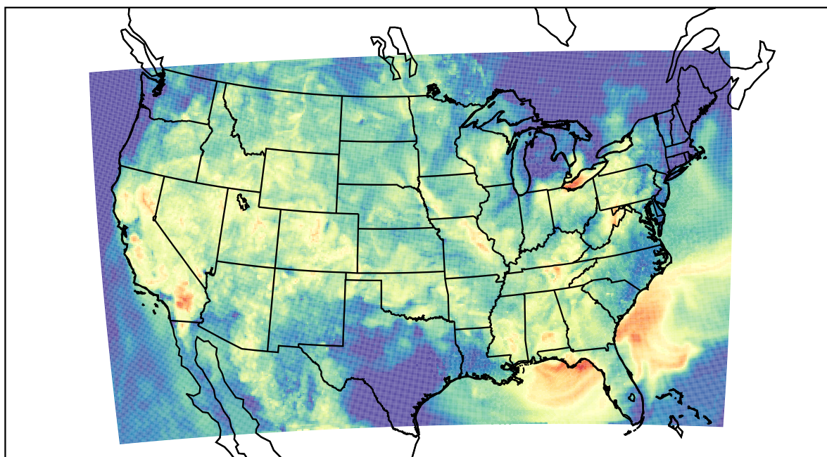
WRF (2022-08-17_06:00:00)
