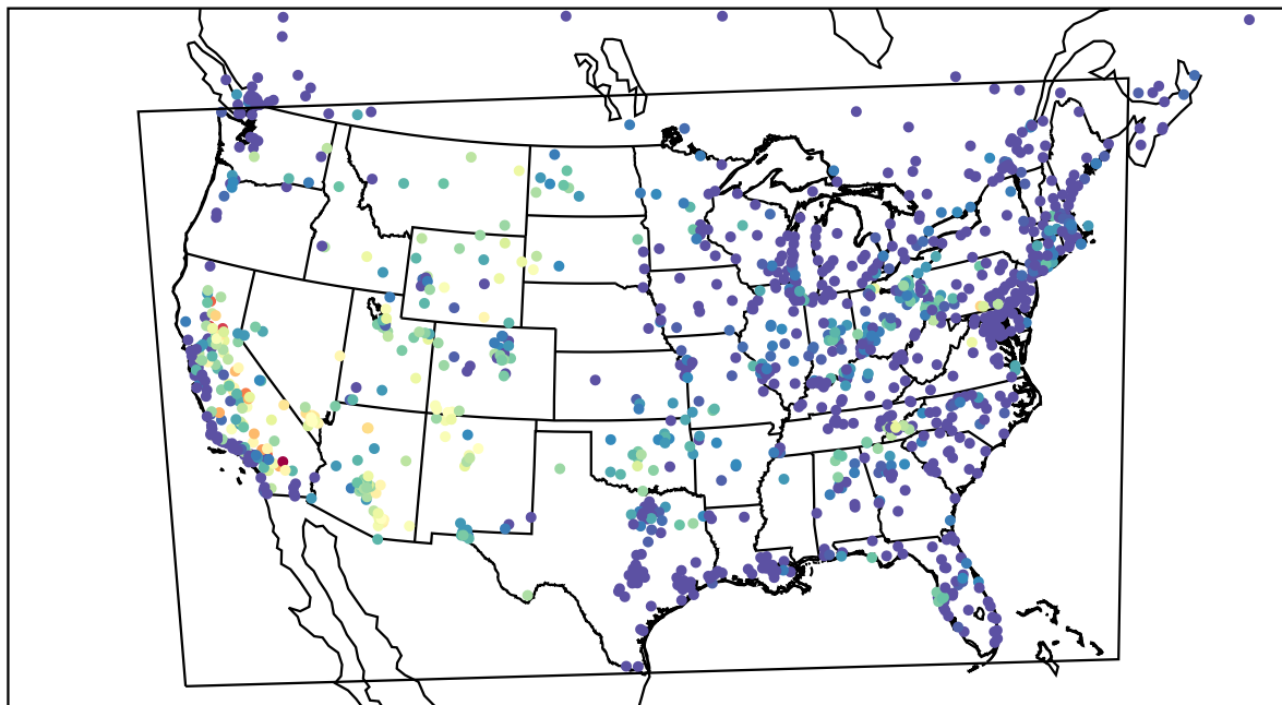
AirNOW (2022-08-17_07:00:00)
