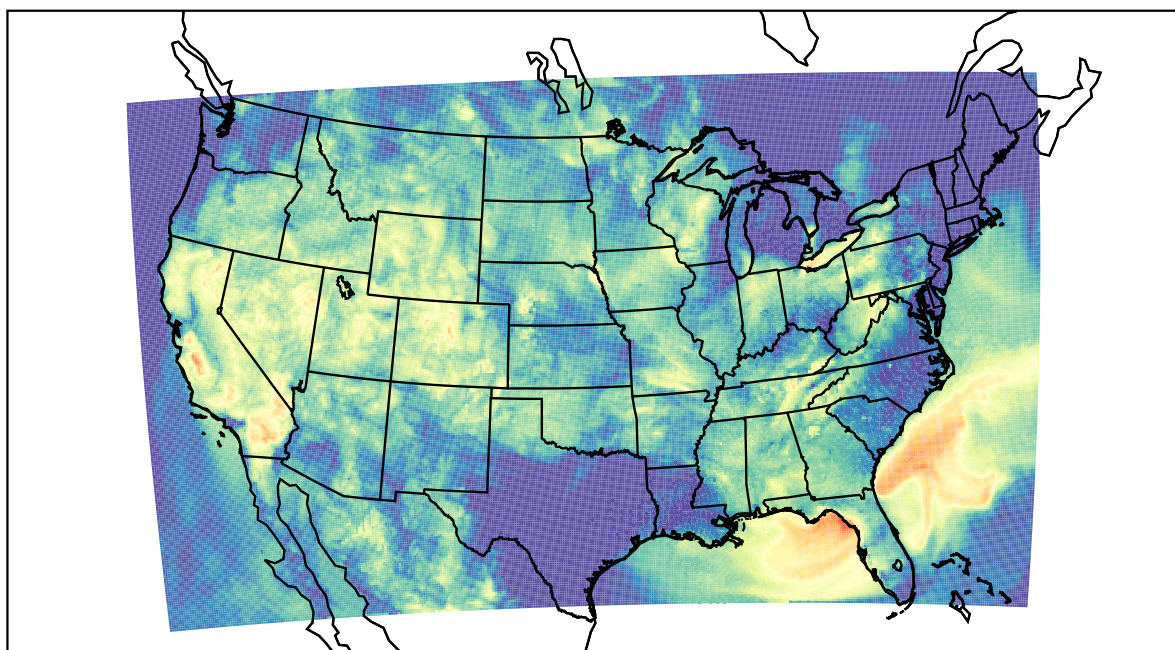
WRF (2022-08-17_11:00:00)
