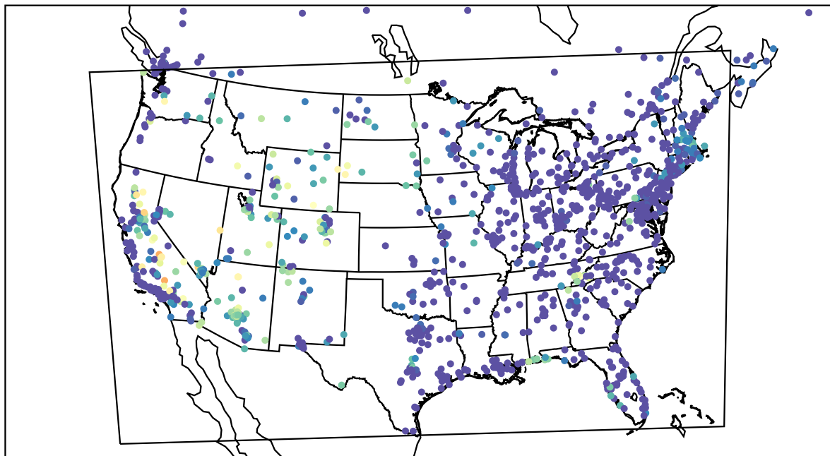
AirNOW (2022-08-18_11:00:00)
