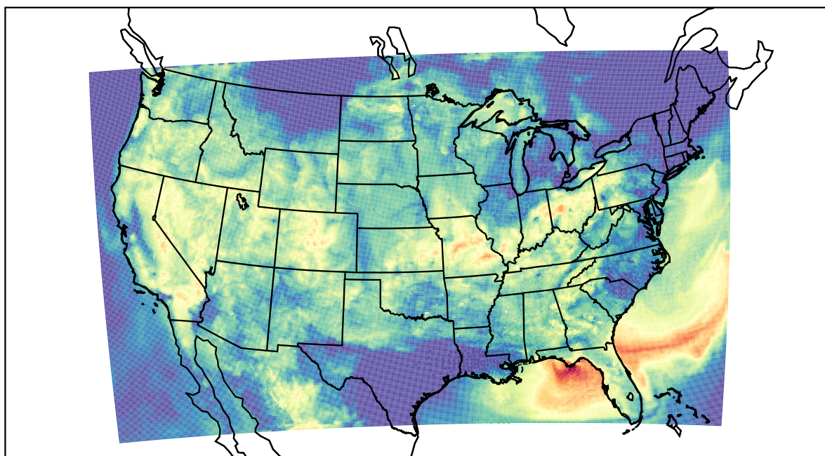
WRF (2022-08-18_11:00:00)
