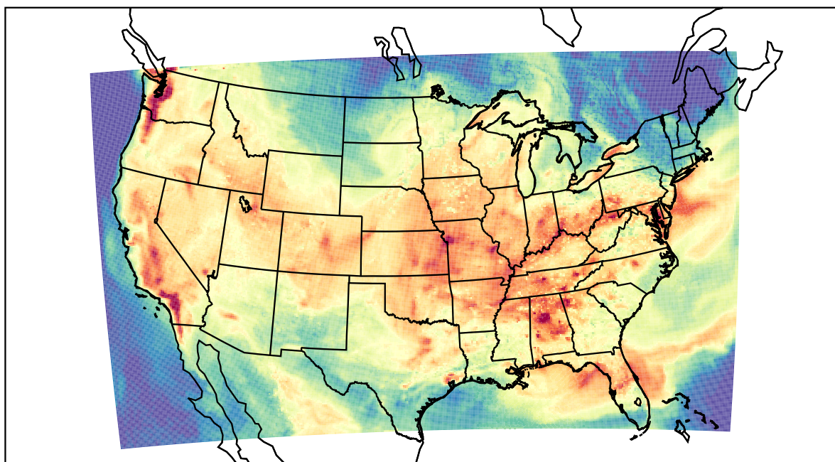
WRF (2022-08-18_21:00:00)
