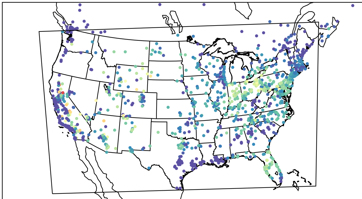
AirNOW (2022-08-17_14:00:00)
