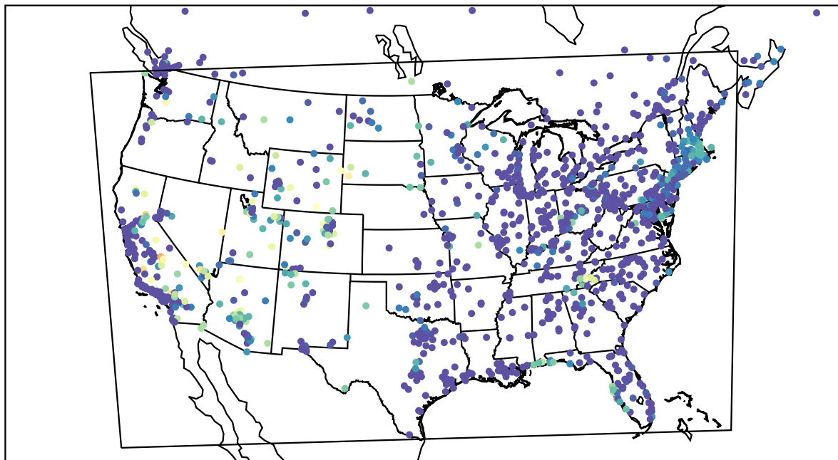
AirNOW (2022-08-18_12:00:00)
