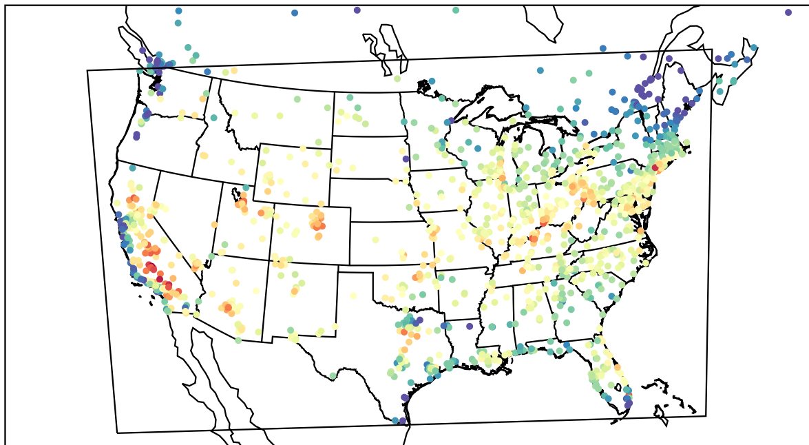
AirNOW (2022-08-18_18:00:00)
