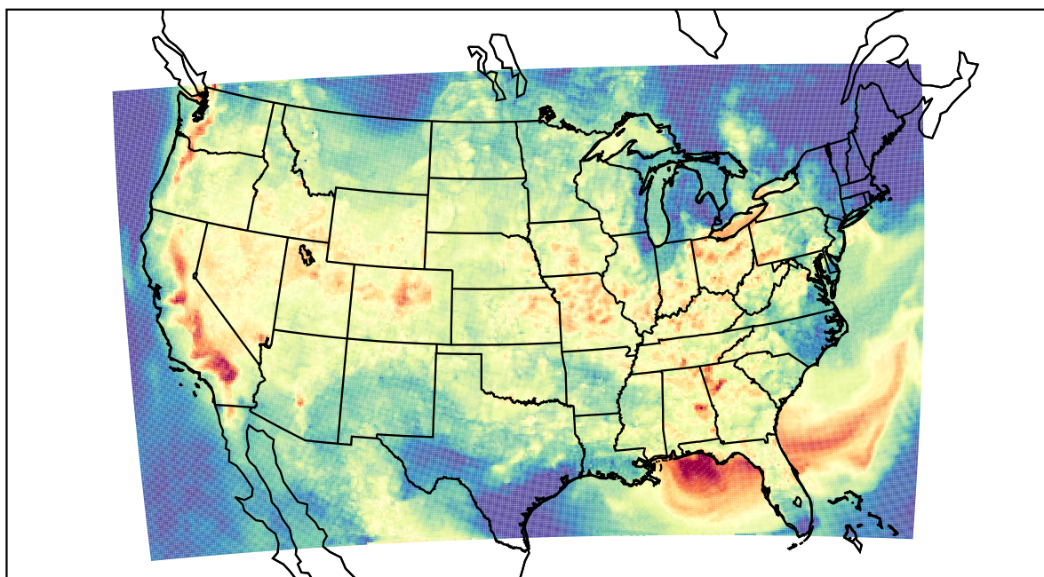
WRF (2022-08-18_02:00:00)
