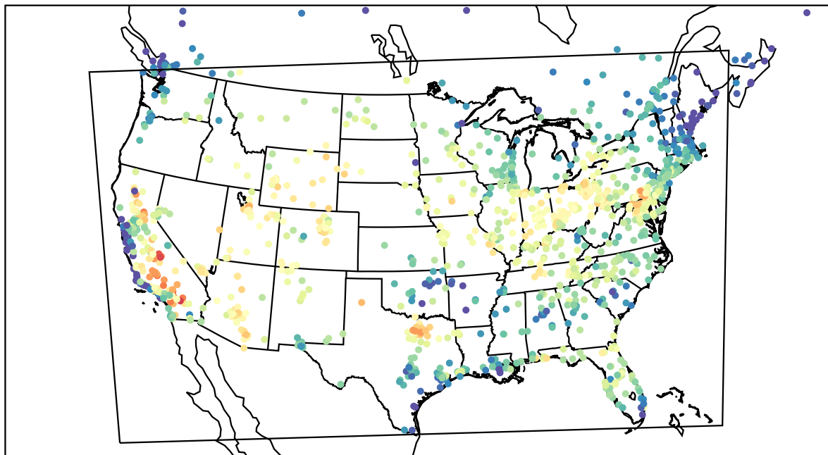
AirNOW (2022-08-17_17:00:00)
