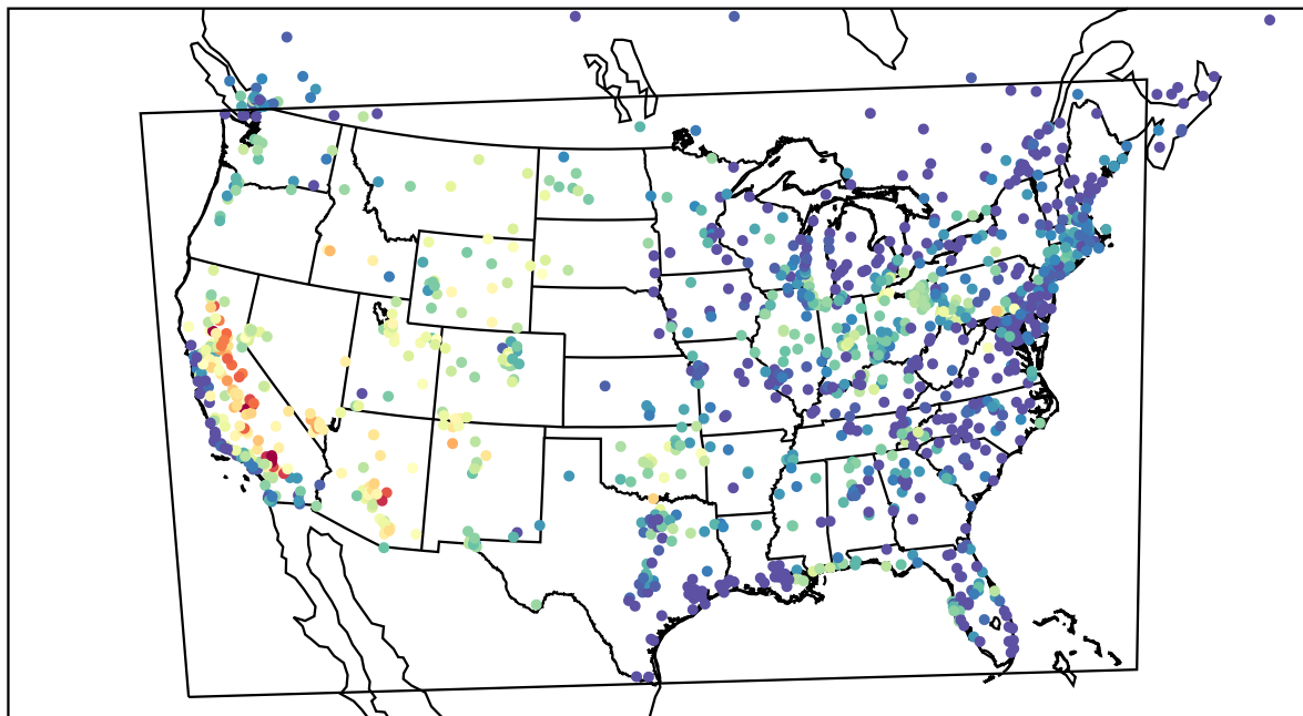
AirNOW (2022-08-17_03:00:00)
