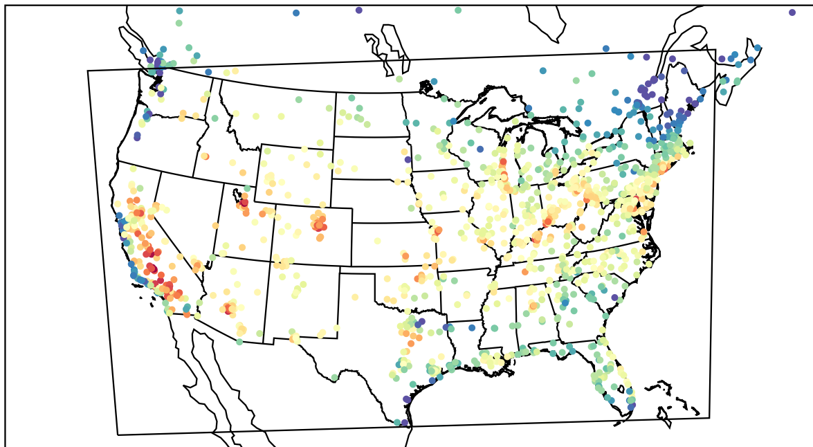
AirNOW (2022-08-18_19:00:00)
