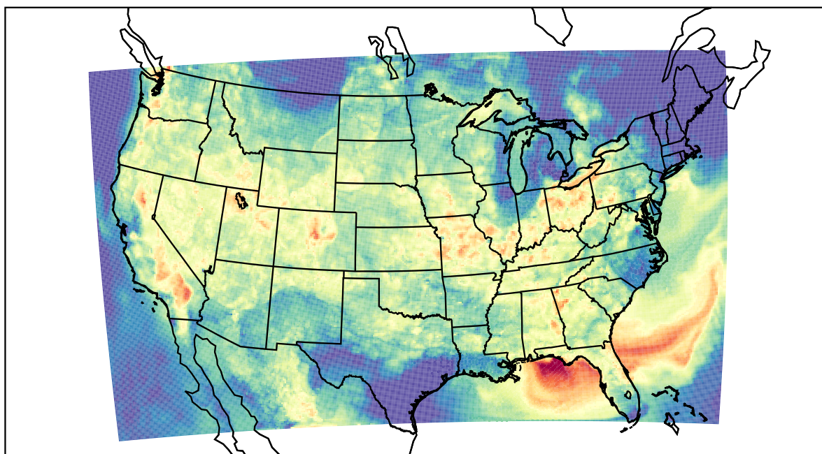
WRF (2022-08-18_04:00:00)
