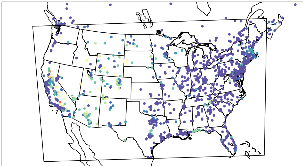
AirNOW (2022-08-18_10:00:00)
