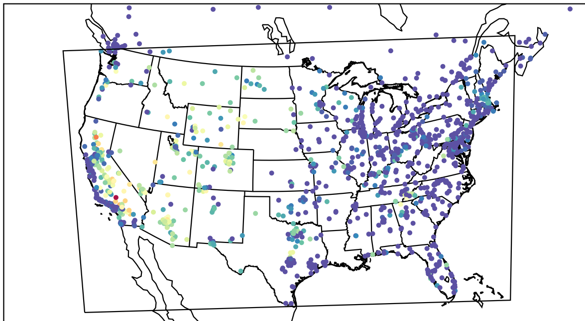
AirNOW (2022-08-18_07:00:00)
