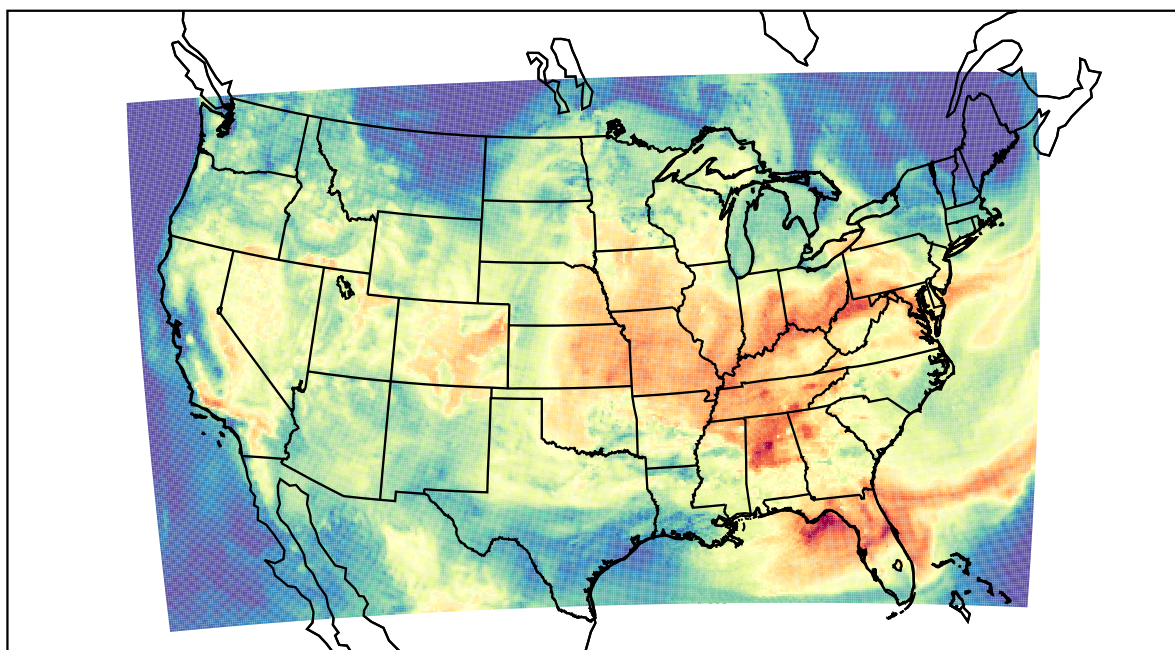
WRF (2022-08-18_16:00:00)
