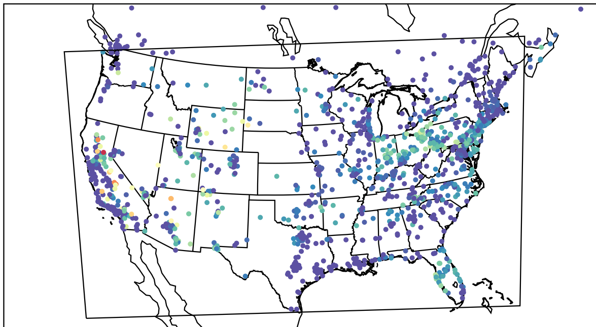
AirNOW (2022-08-17_13:00:00)
