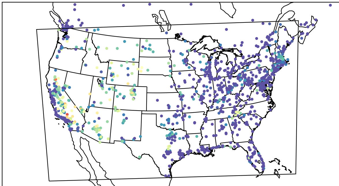
AirNOW (2022-08-18_08:00:00)
