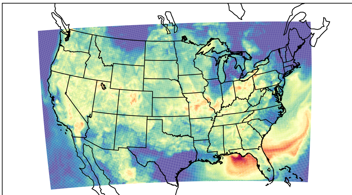
WRF (2022-08-18_06:00:00)
