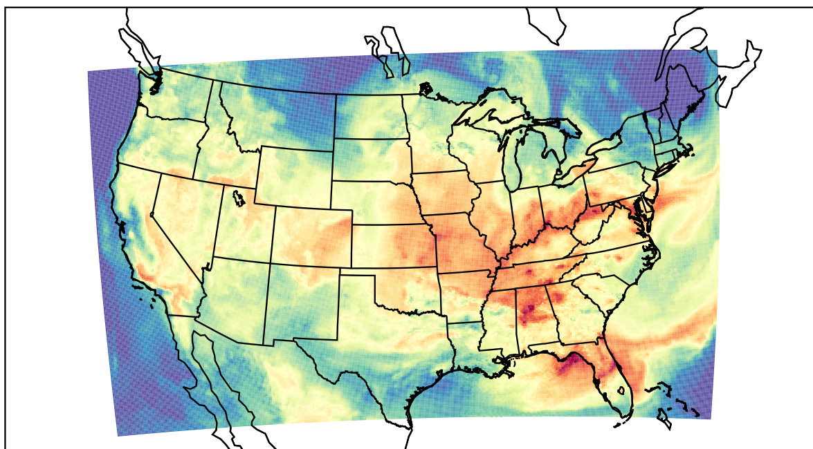
WRF (2022-08-18_17:00:00)
