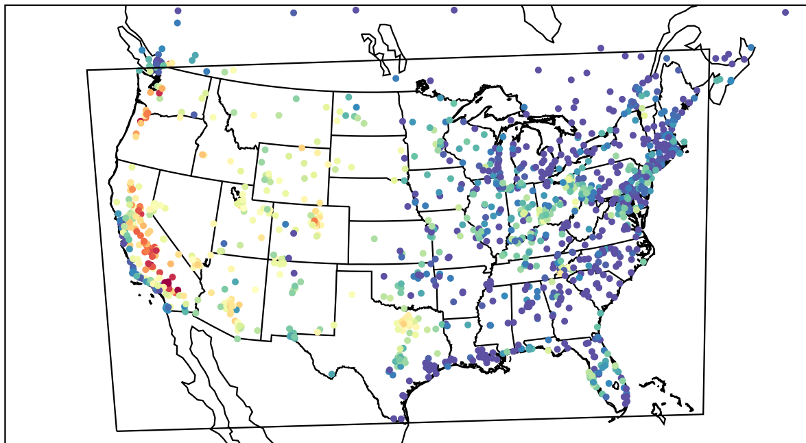
AirNOW (2022-08-18_02:00:00)
