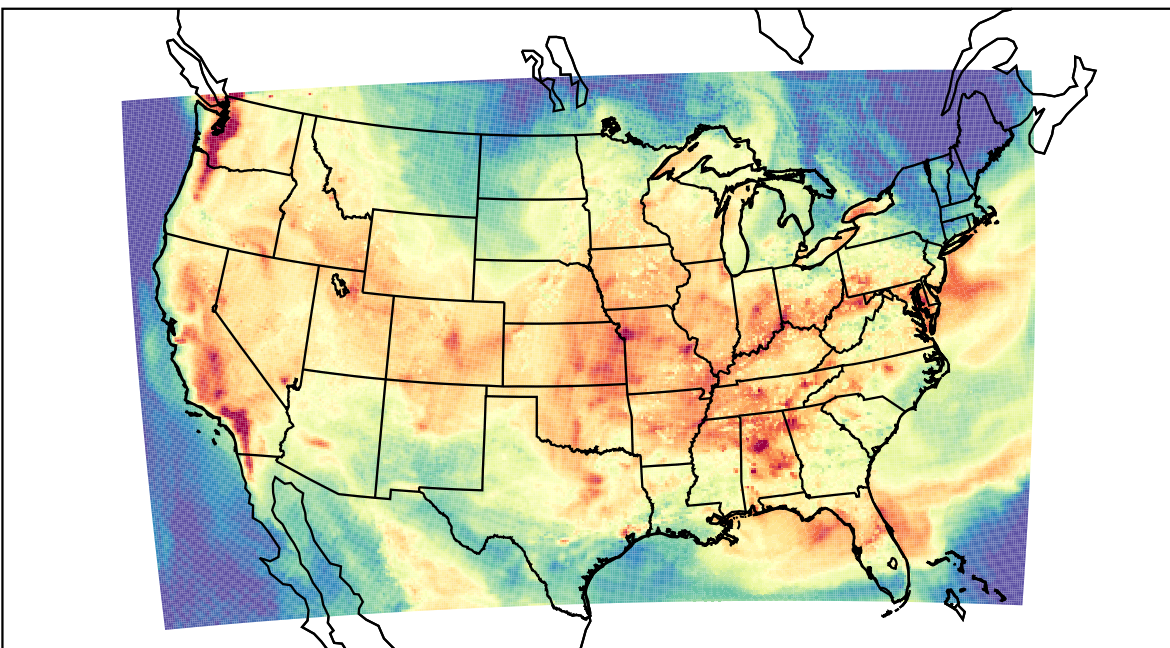
WRF (2022-08-18_22:00:00)
