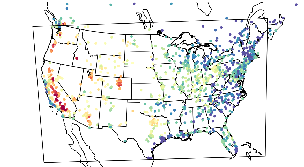
AirNOW (2022-08-18_00:00:00)
