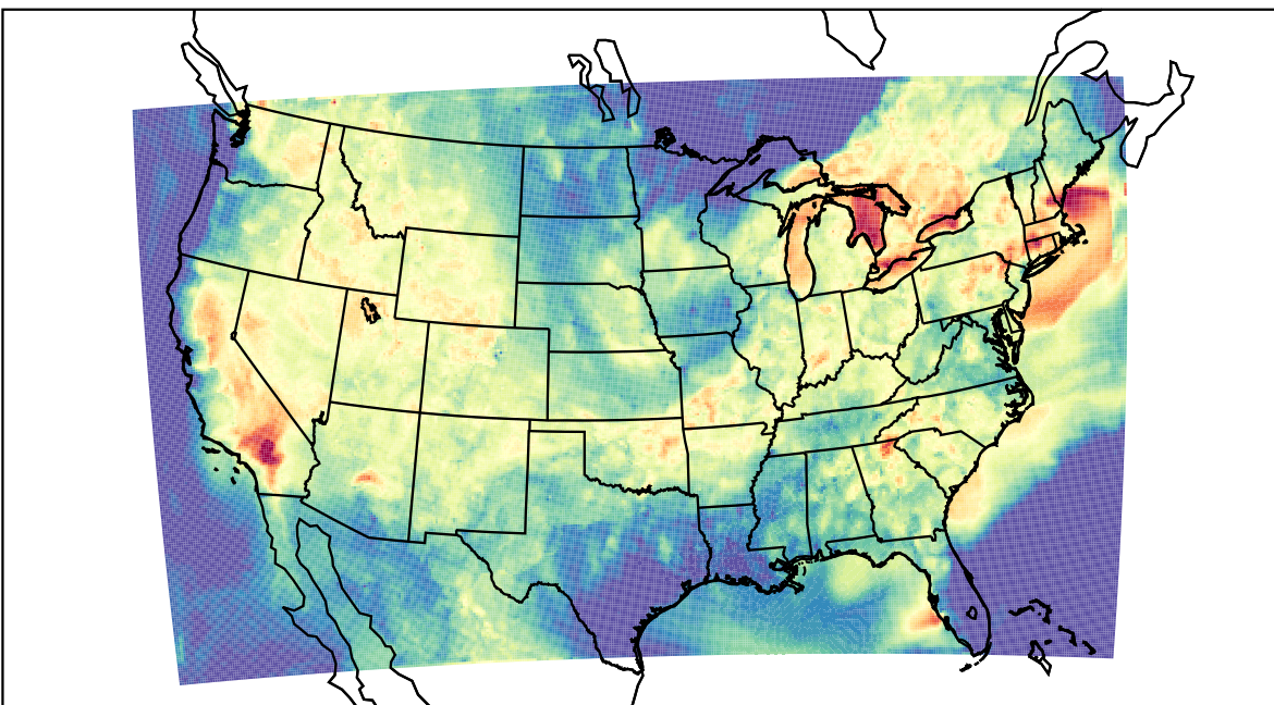
WRF (2022-08-21_02:00:00)
