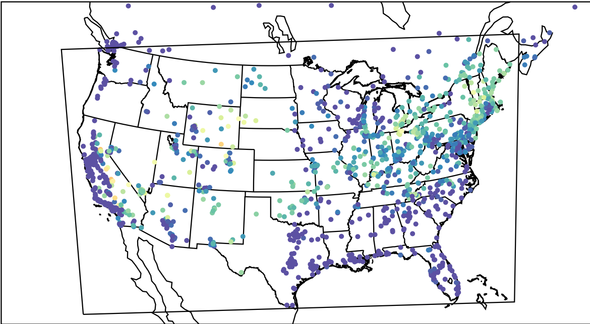
AirNOW (2022-08-22_14:00:00)
