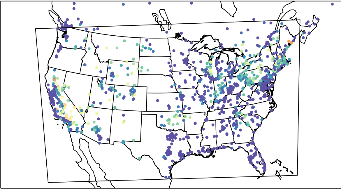
AirNOW (2022-08-21_08:00:00)
