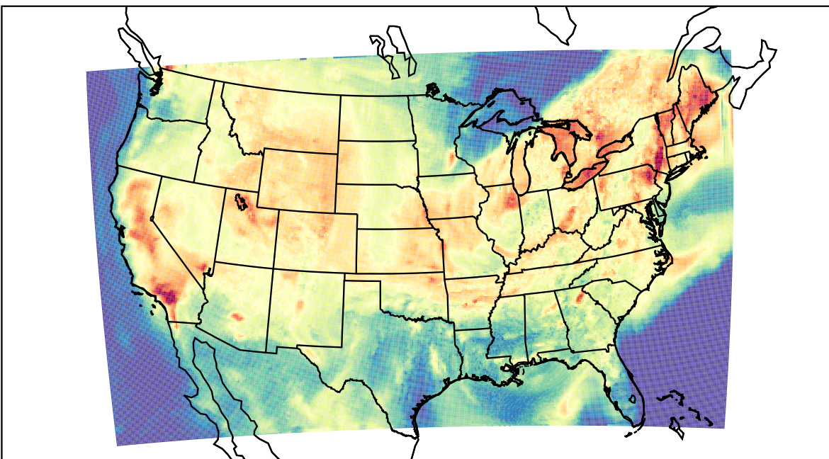
WRF (2022-08-21_22:00:00)
