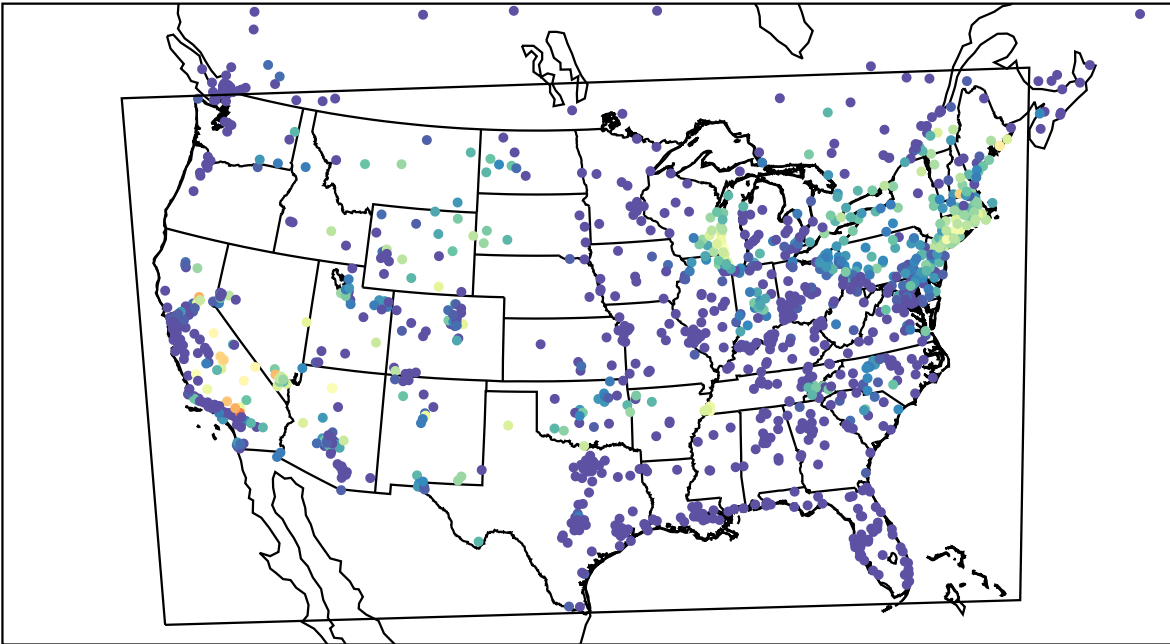
AirNOW (2022-08-21_12:00:00)
