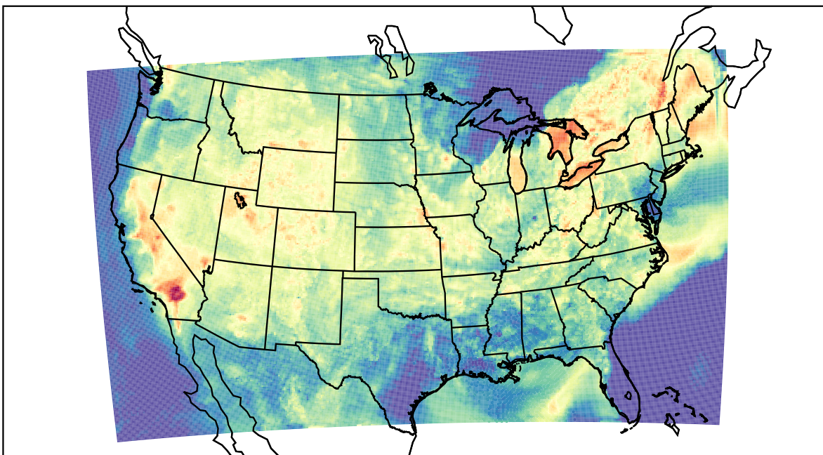
WRF (2022-08-22_02:00:00)
