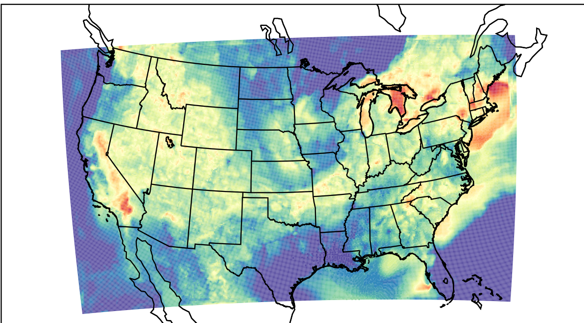
WRF (2022-08-21_04:00:00)
