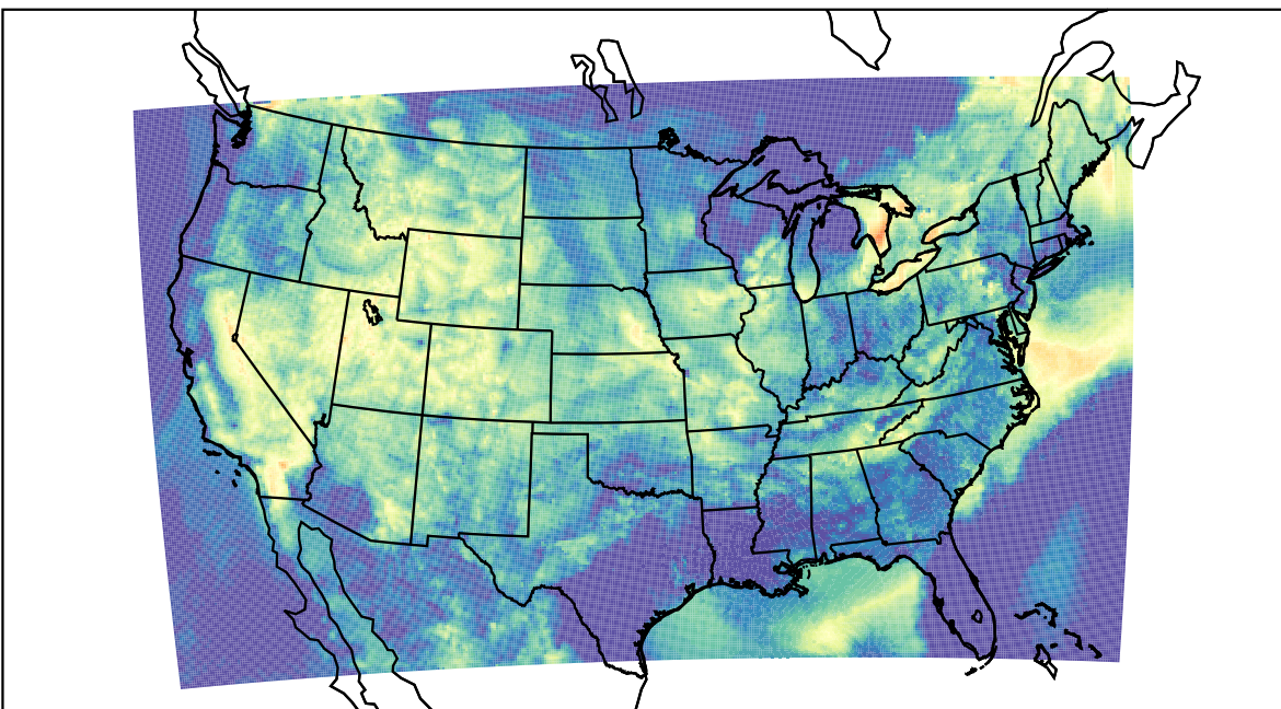
WRF (2022-08-22_11:00:00)
