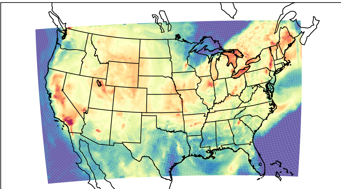
WRF (2022-08-21_23:00:00)
