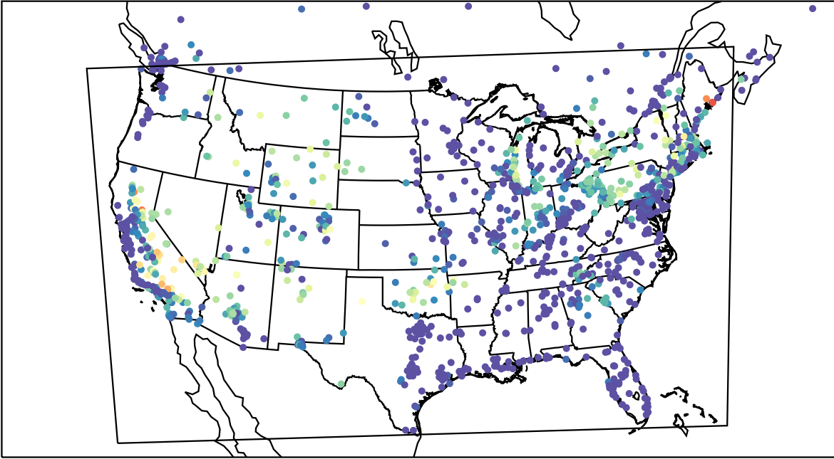
AirNOW (2022-08-21_07:00:00)
