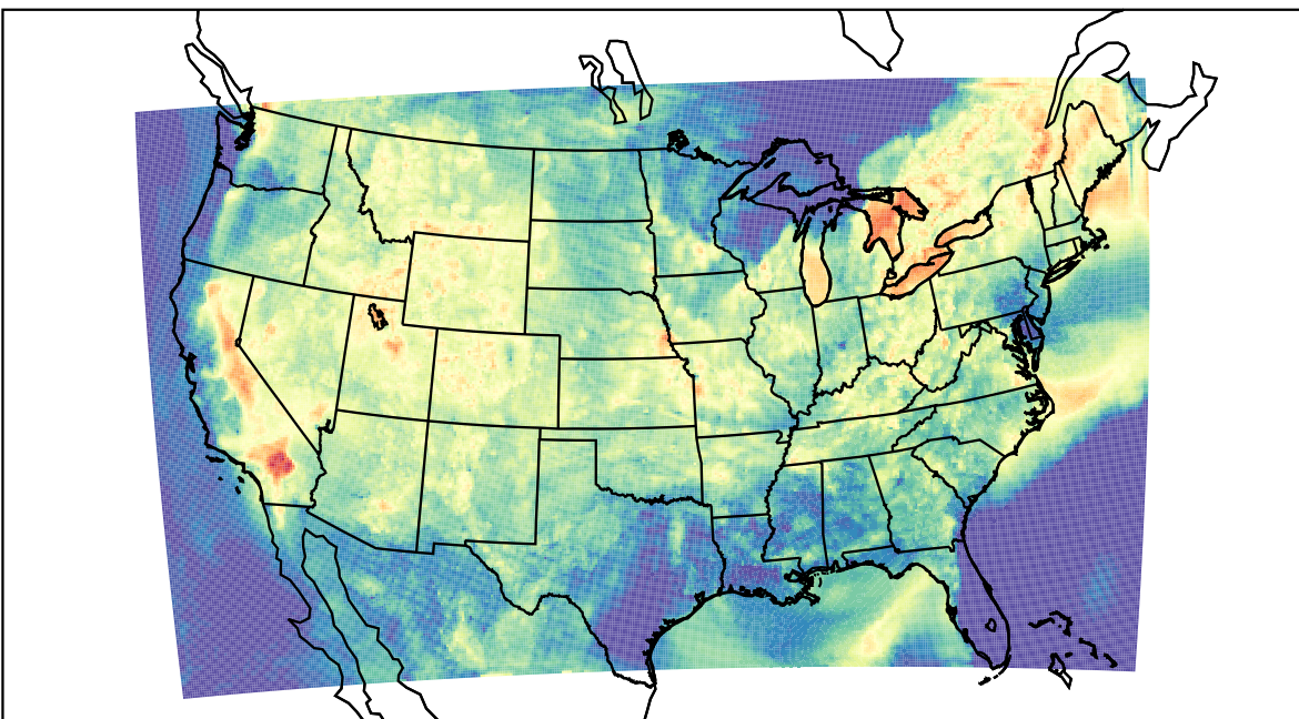
WRF (2022-08-22_03:00:00)
