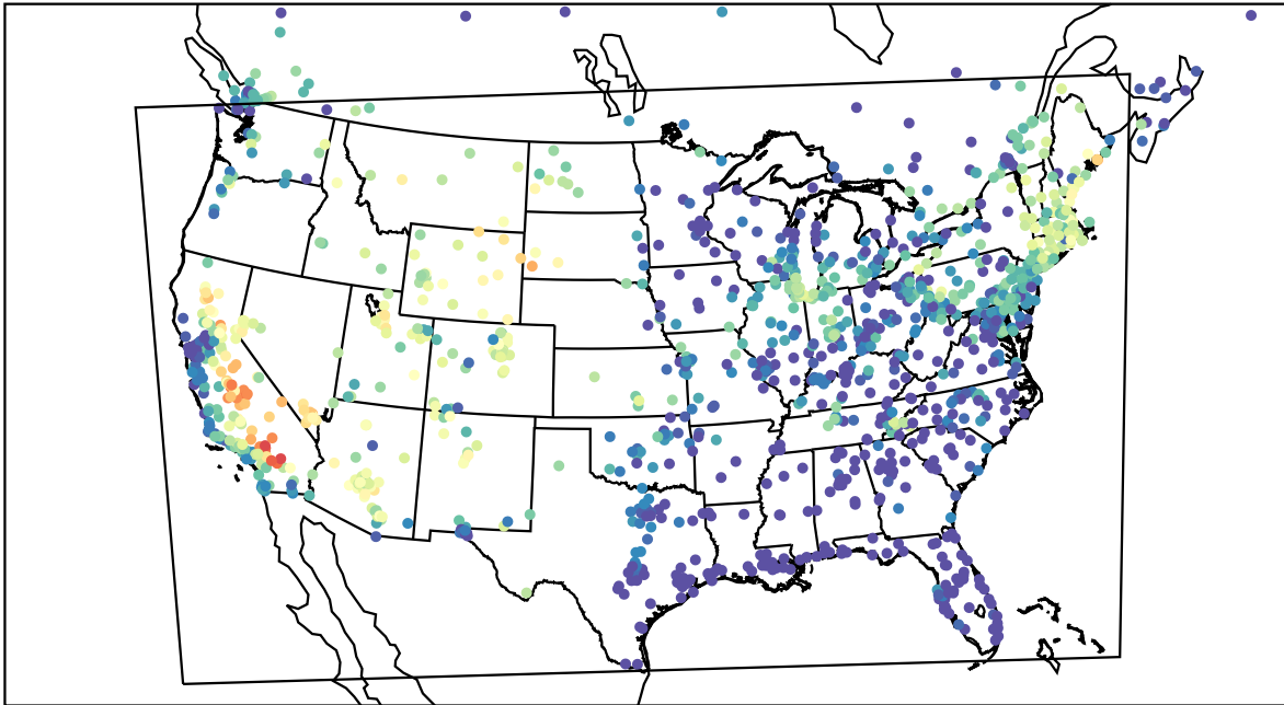
AirNOW (2022-08-22_02:00:00)
