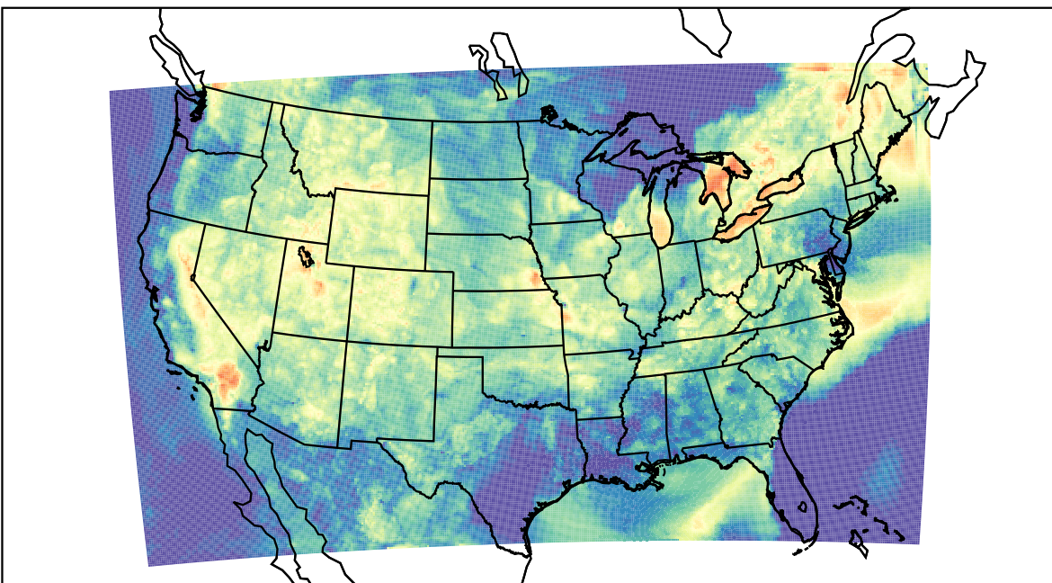
WRF (2022-08-22_05:00:00)
