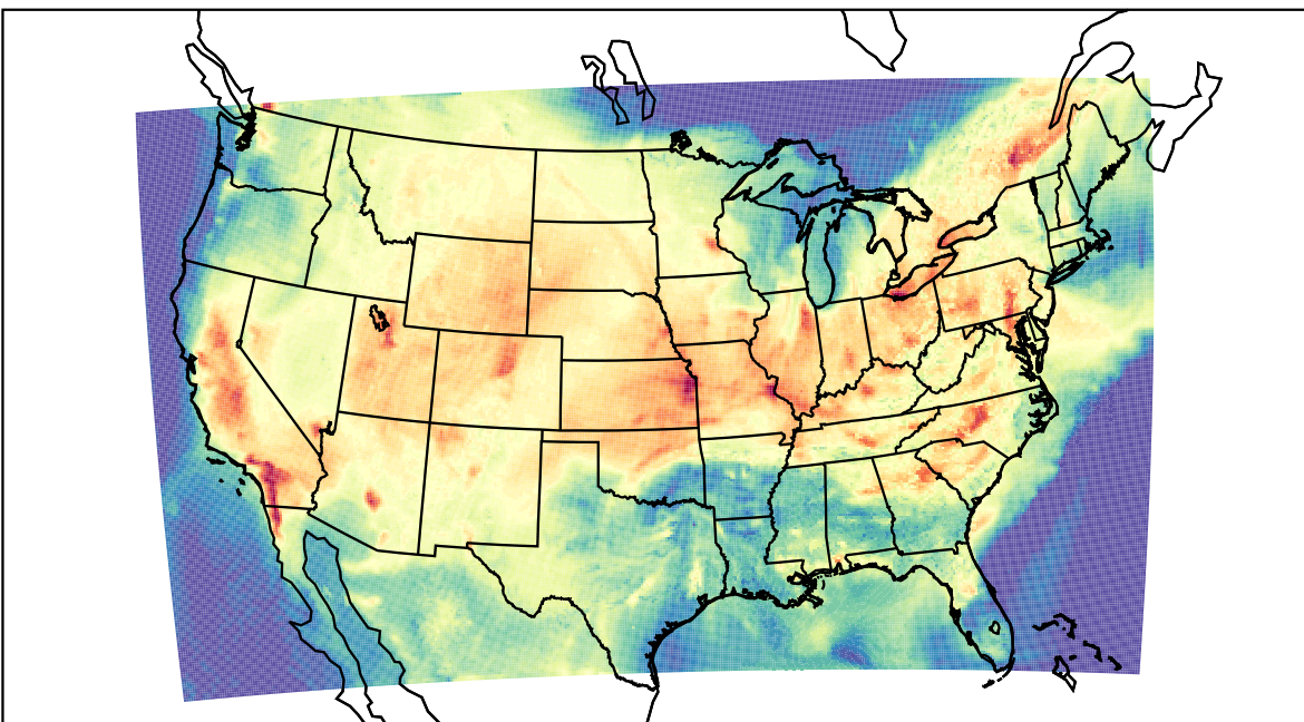
WRF (2022-08-22_21:00:00)
