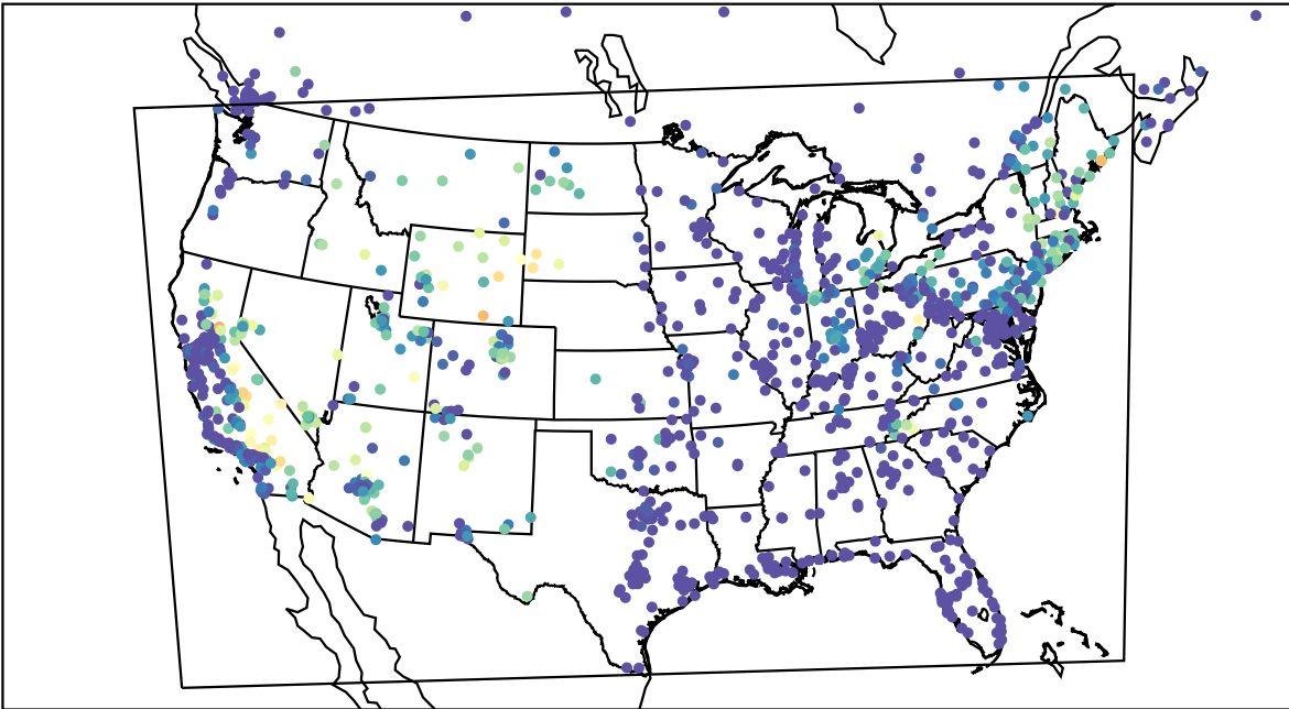
AirNOW (2022-08-22_08:00:00)
