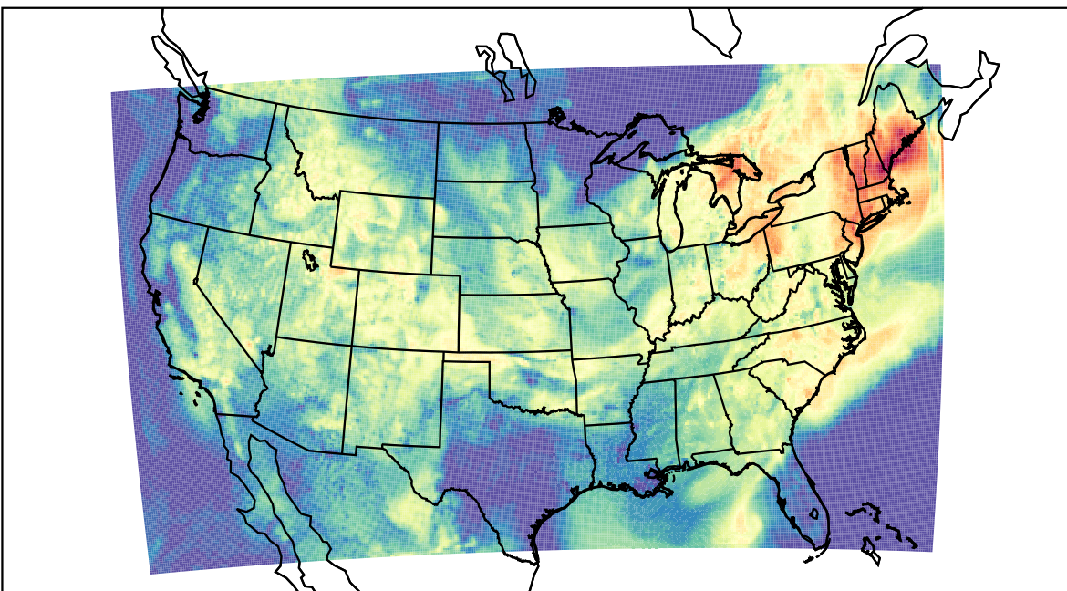
WRF (2022-08-21_15:00:00)
