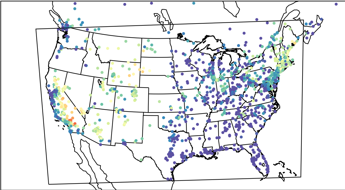
AirNOW (2022-08-22_03:00:00)
