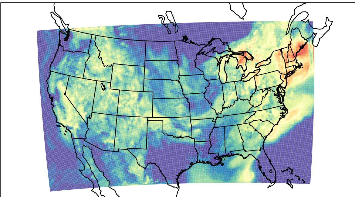
WRF (2022-08-21_14:00:00)
