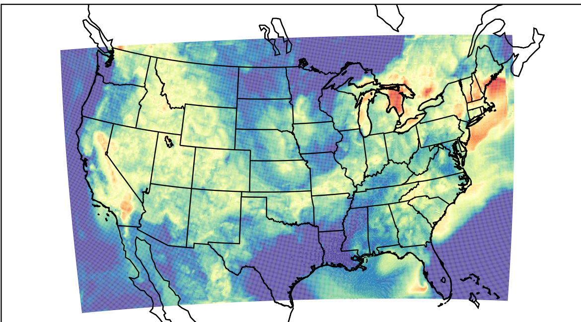
WRF (2022-08-21_06:00:00)
