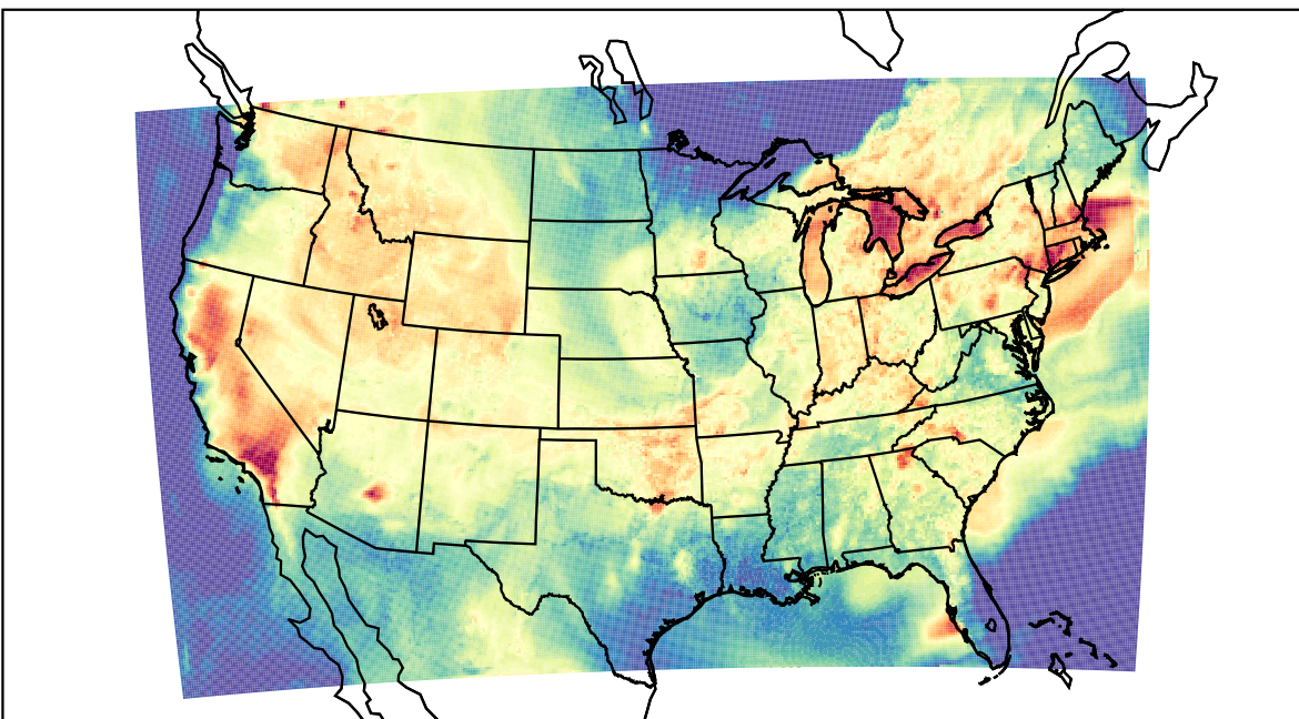
WRF (2022-08-21_00:00:00)
