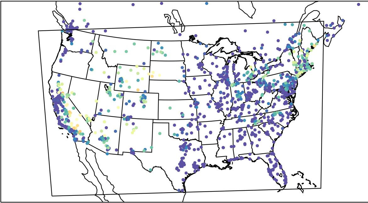
AirNOW (2022-08-22_07:00:00)
