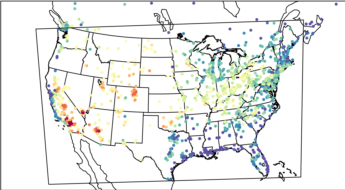
AirNOW (2022-08-22_22:00:00)
