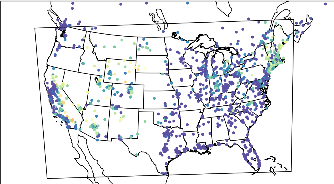
AirNOW (2022-08-22_06:00:00)
