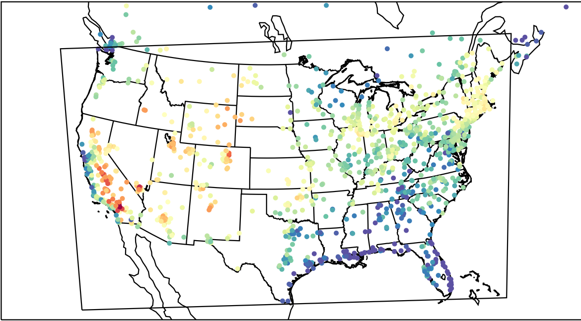
AirNOW (2022-08-21_21:00:00)
