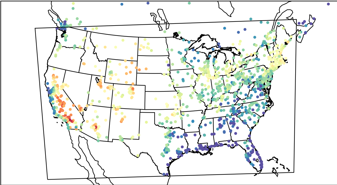
AirNOW (2022-08-21_22:00:00)
