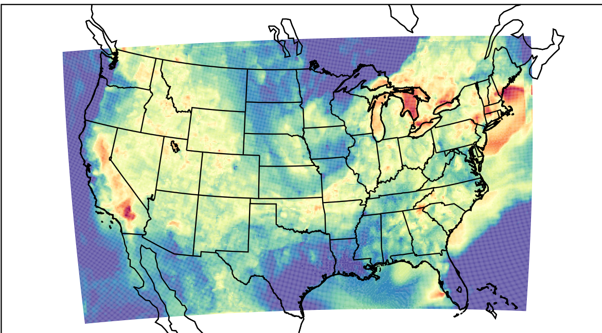
WRF (2022-08-21_03:00:00)
