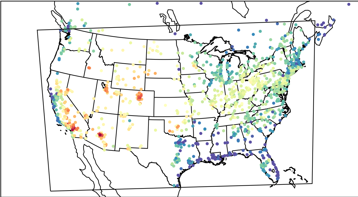
AirNOW (2022-08-22_20:00:00)
