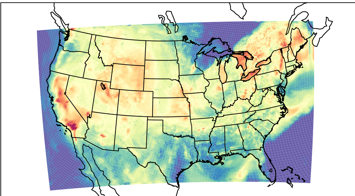
WRF (2022-08-22_00:00:00)
