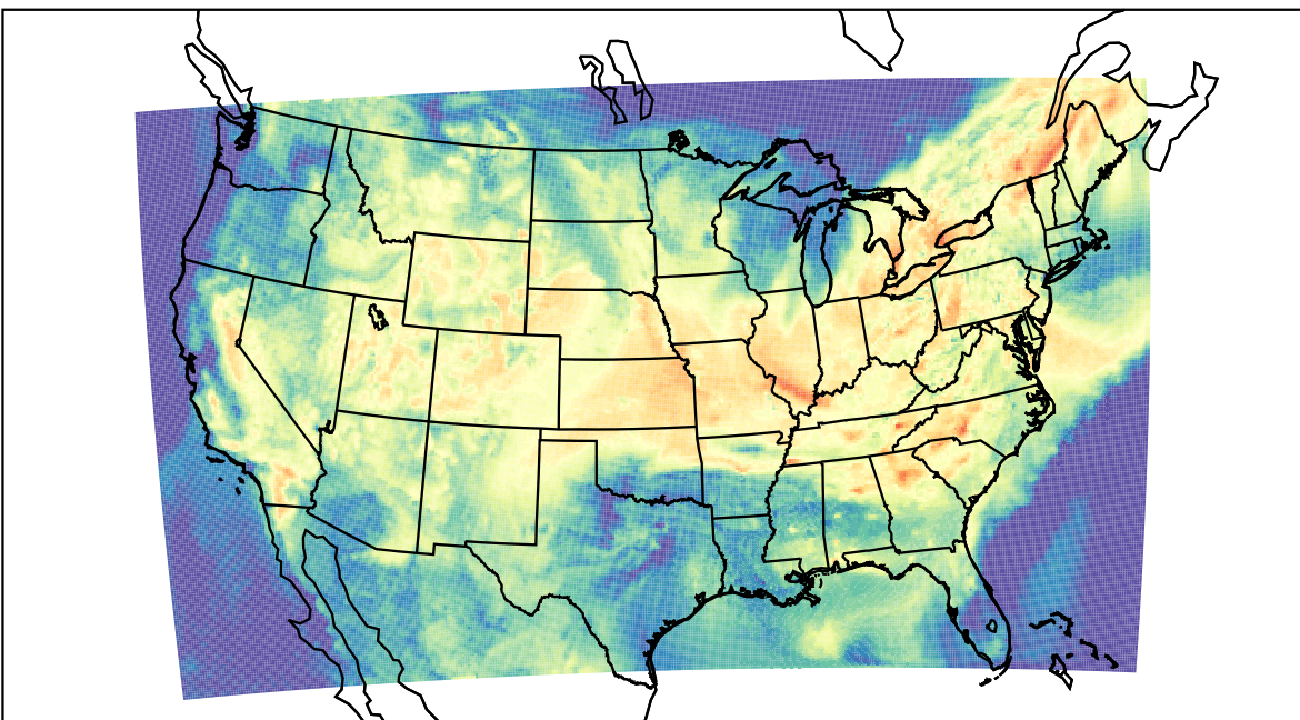
WRF (2022-08-22_16:00:00)
