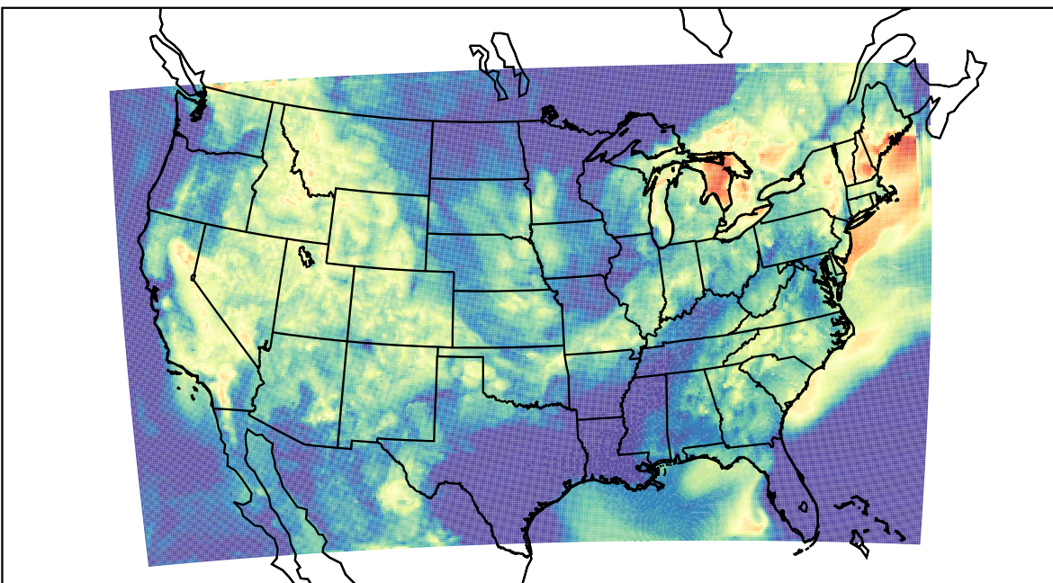
WRF (2022-08-21_09:00:00)
