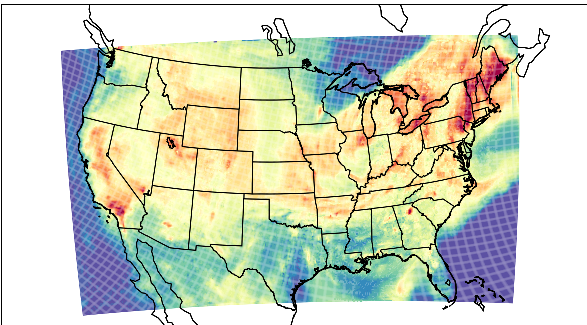
WRF (2022-08-21_21:00:00)
