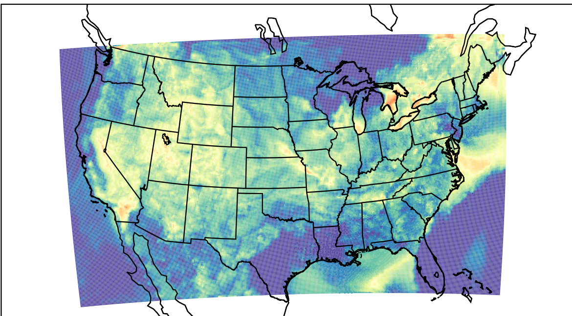
WRF (2022-08-22_08:00:00)
