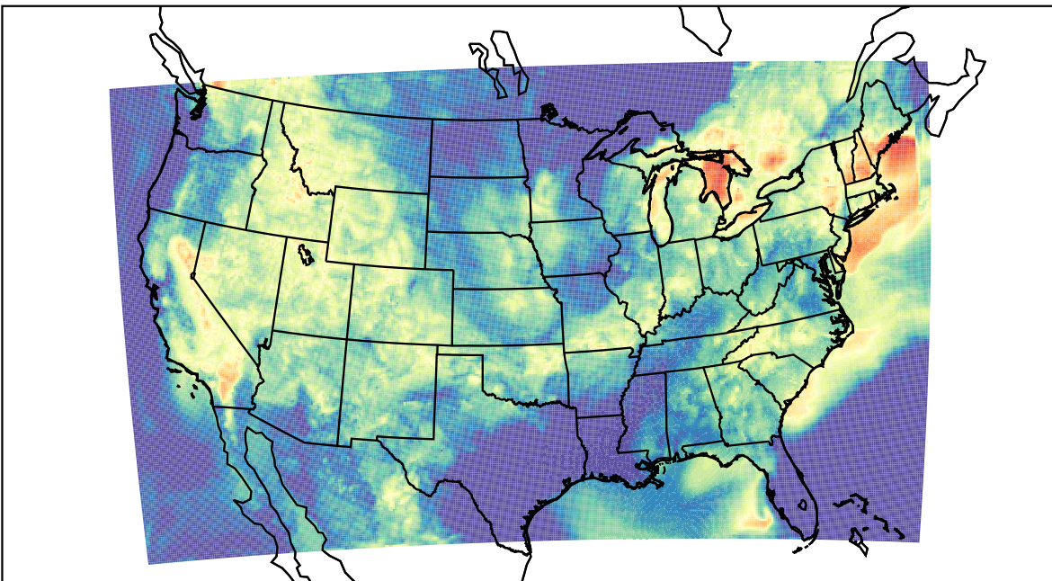
WRF (2022-08-21_07:00:00)
