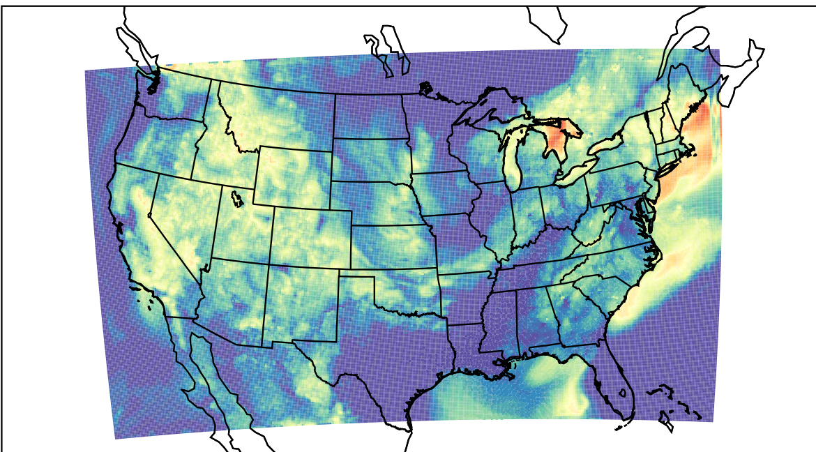
WRF (2022-08-21_12:00:00)
