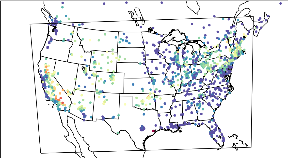
AirNOW (2022-08-21_04:00:00)
