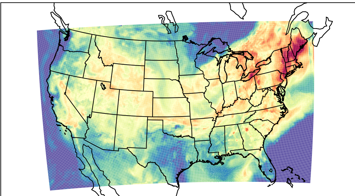
WRF (2022-08-21_17:00:00)
