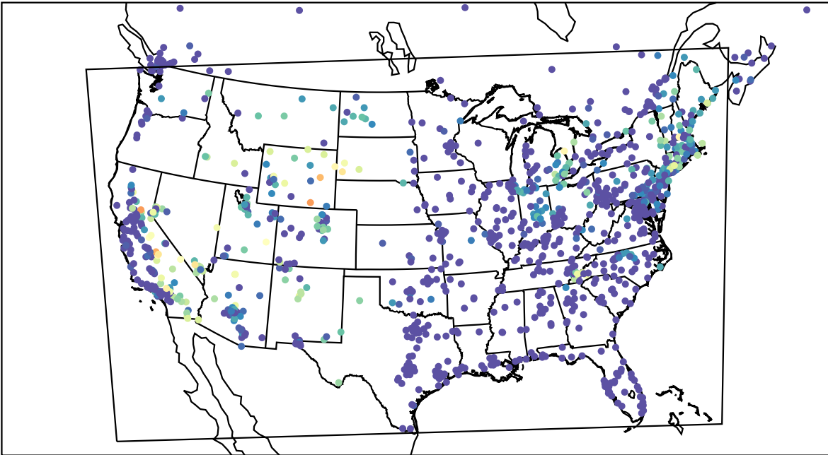
AirNOW (2022-08-22_10:00:00)
