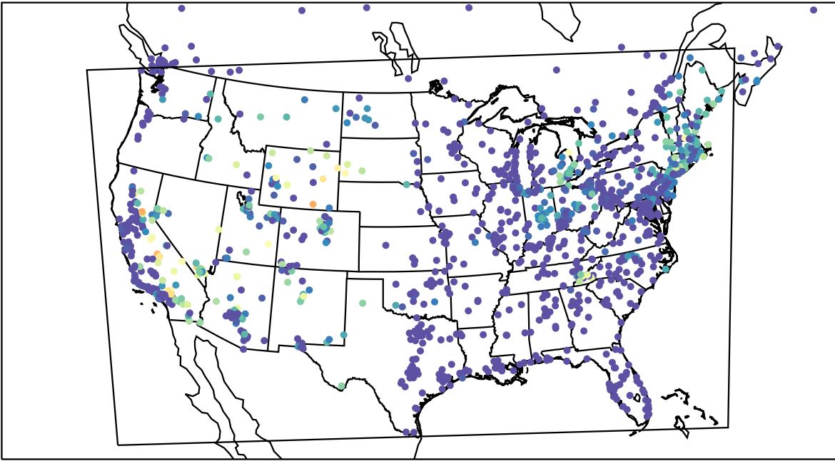
AirNOW (2022-08-22_11:00:00)
