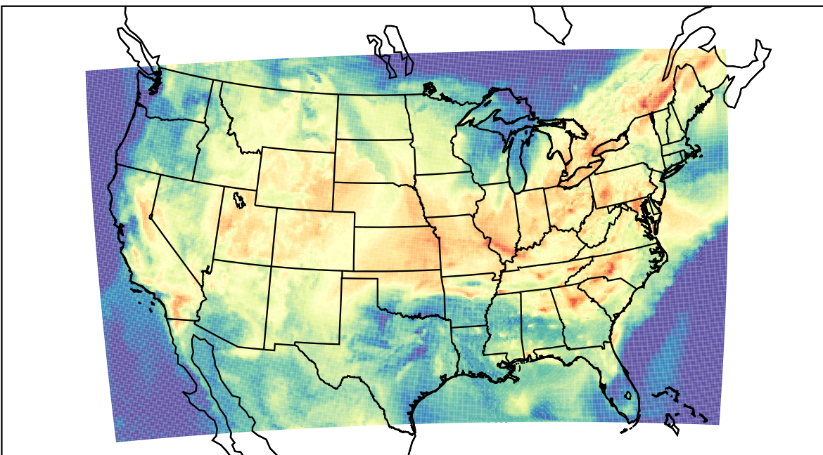
WRF (2022-08-22_17:00:00)
