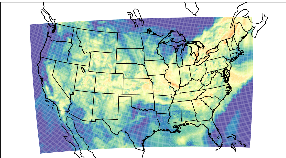
WRF (2022-08-22_15:00:00)
