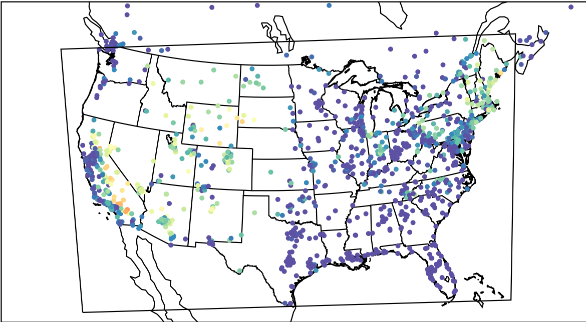
AirNOW (2022-08-22_05:00:00)
