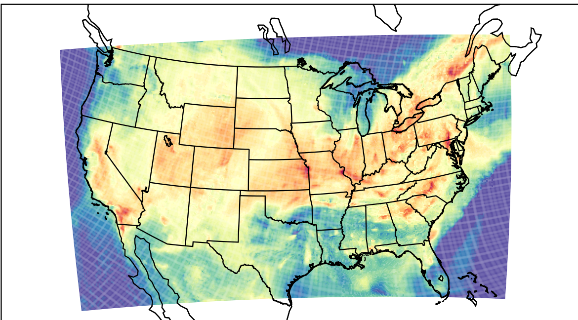
WRF (2022-08-22_19:00:00)
