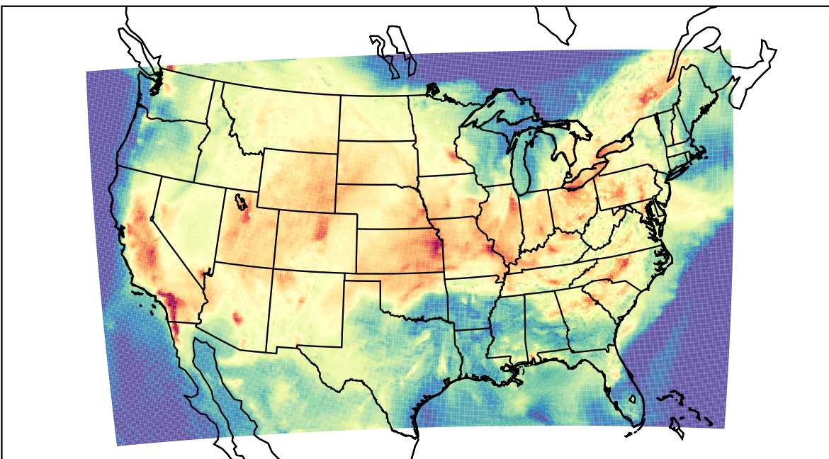
WRF (2022-08-22_22:00:00)
