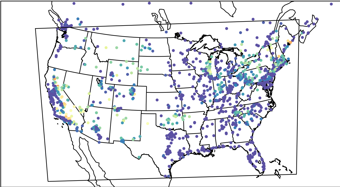
AirNOW (2022-08-21_09:00:00)
