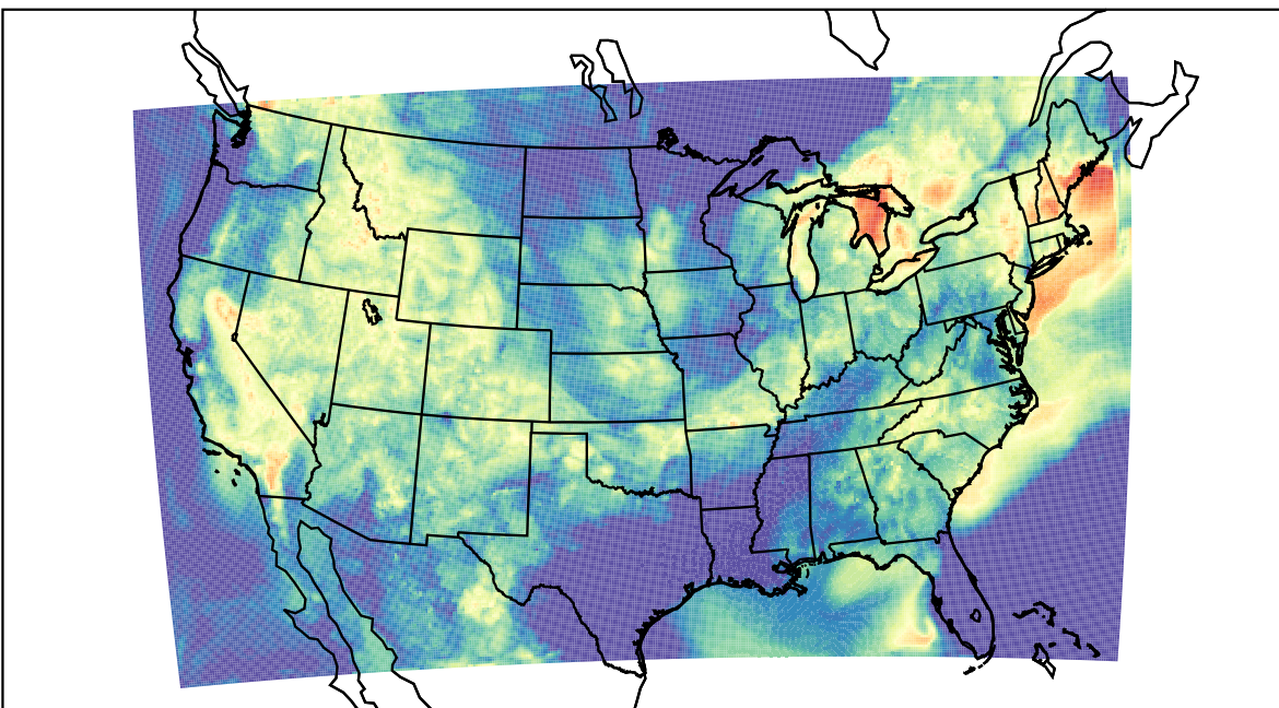
WRF (2022-08-21_08:00:00)
