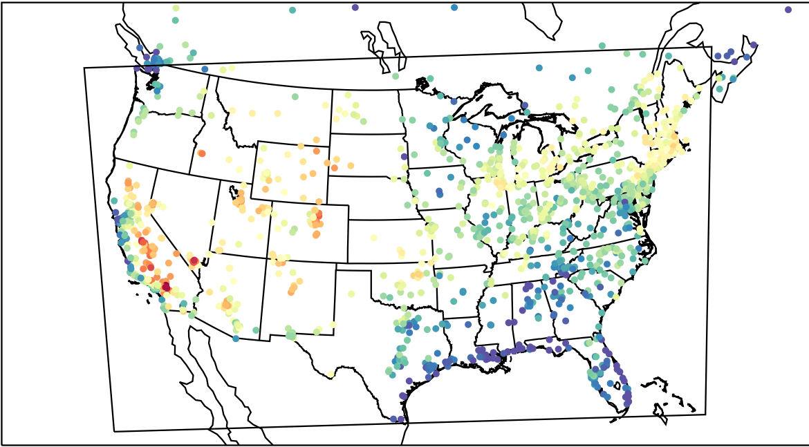
AirNOW (2022-08-21_20:00:00)
