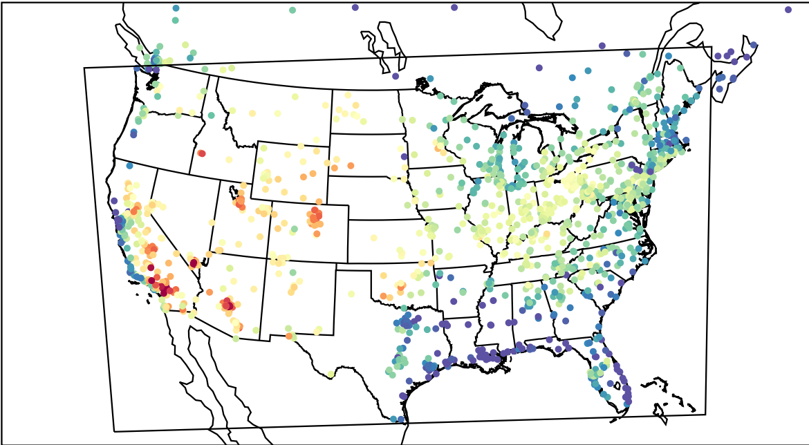
AirNOW (2022-08-22_21:00:00)
