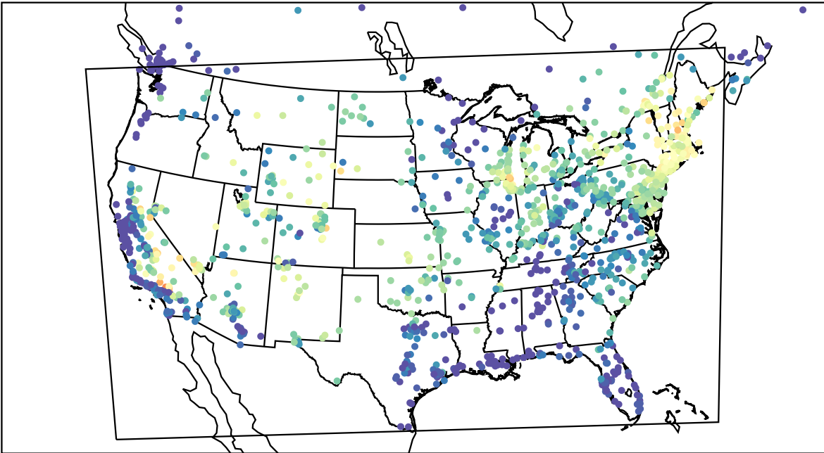
AirNOW (2022-08-21_15:00:00)
