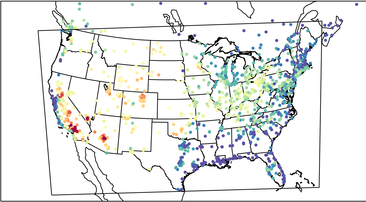
AirNOW (2022-08-22_23:00:00)
