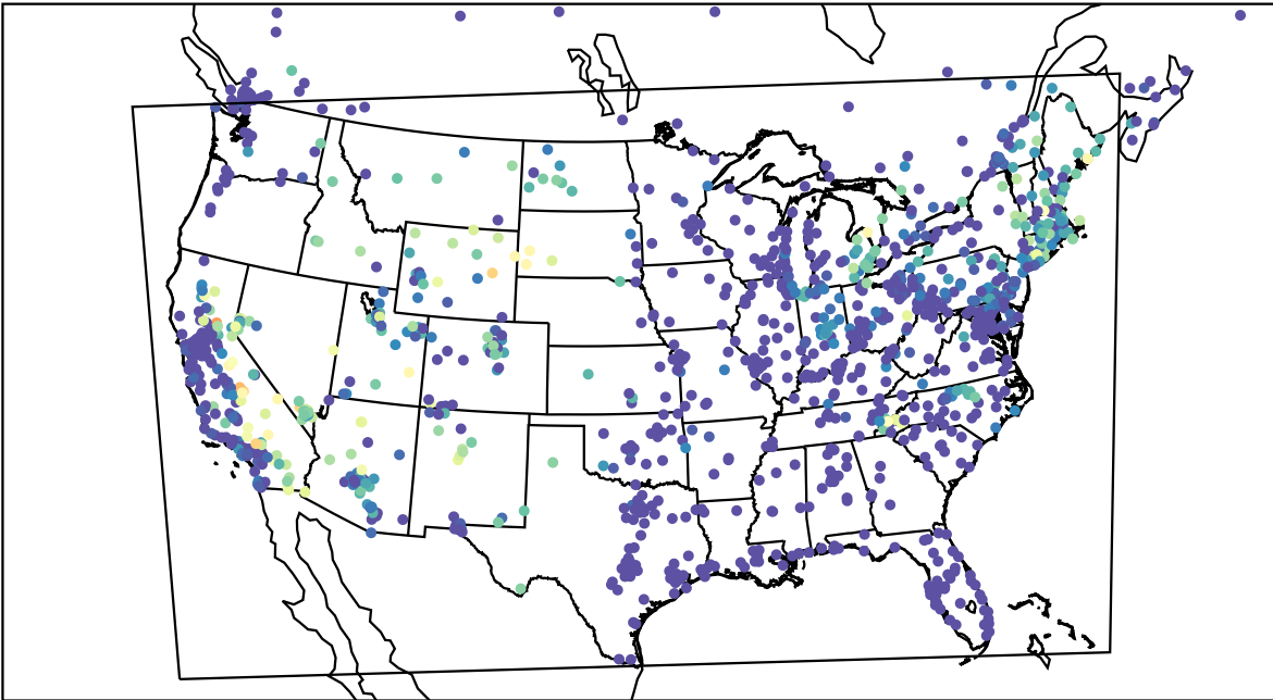
AirNOW (2022-08-22_09:00:00)
