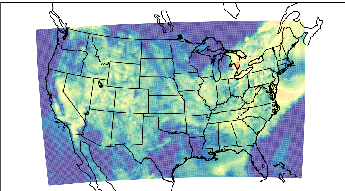
WRF (2022-08-22_14:00:00)
