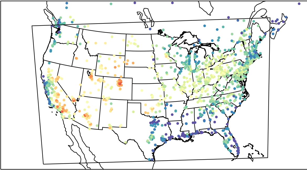
AirNOW (2022-08-22_19:00:00)
