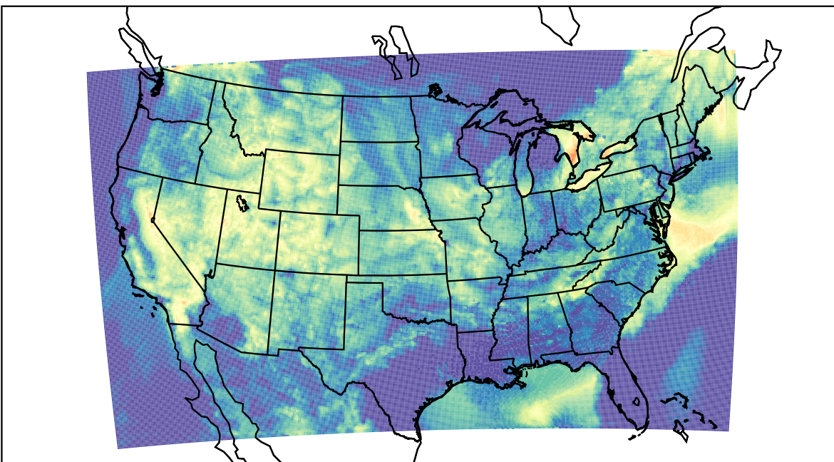
WRF (2022-08-22_12:00:00)
