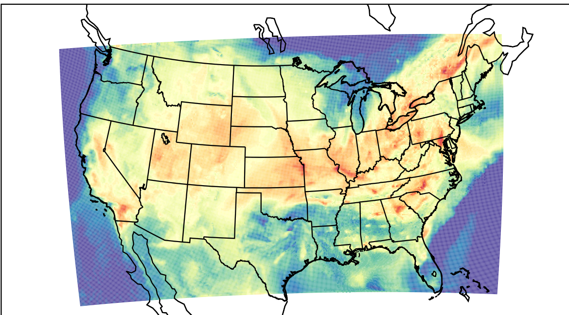
WRF (2022-08-22_18:00:00)
