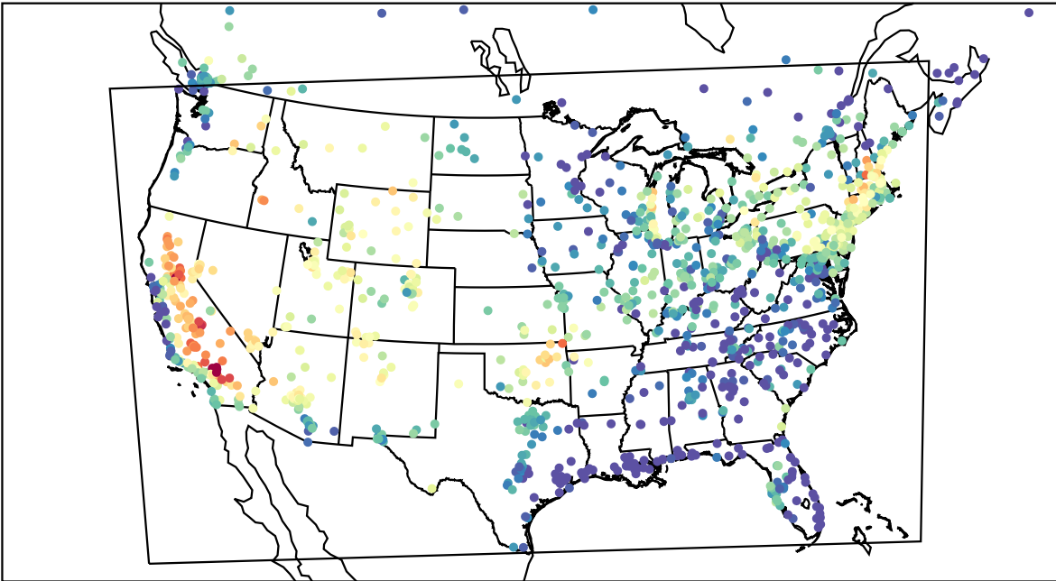
AirNOW (2022-08-21_01:00:00)
