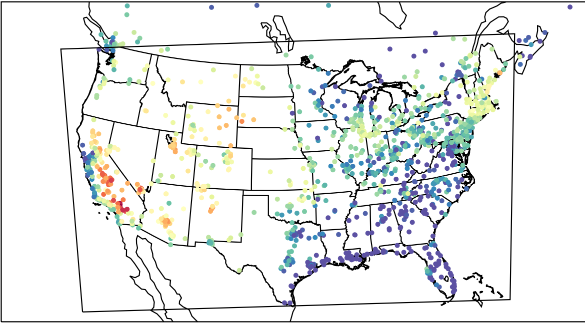
AirNOW (2022-08-22_00:00:00)
