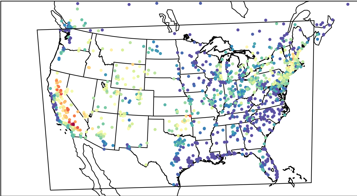
AirNOW (2022-08-21_02:00:00)
