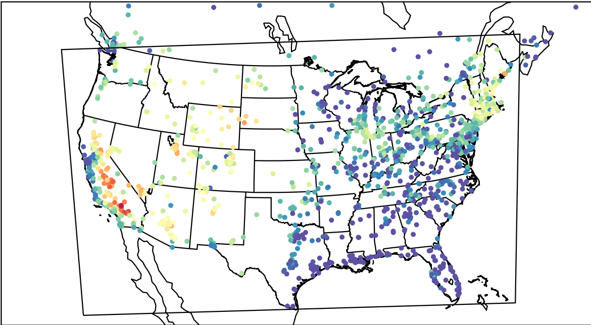
AirNOW (2022-08-22_01:00:00)
