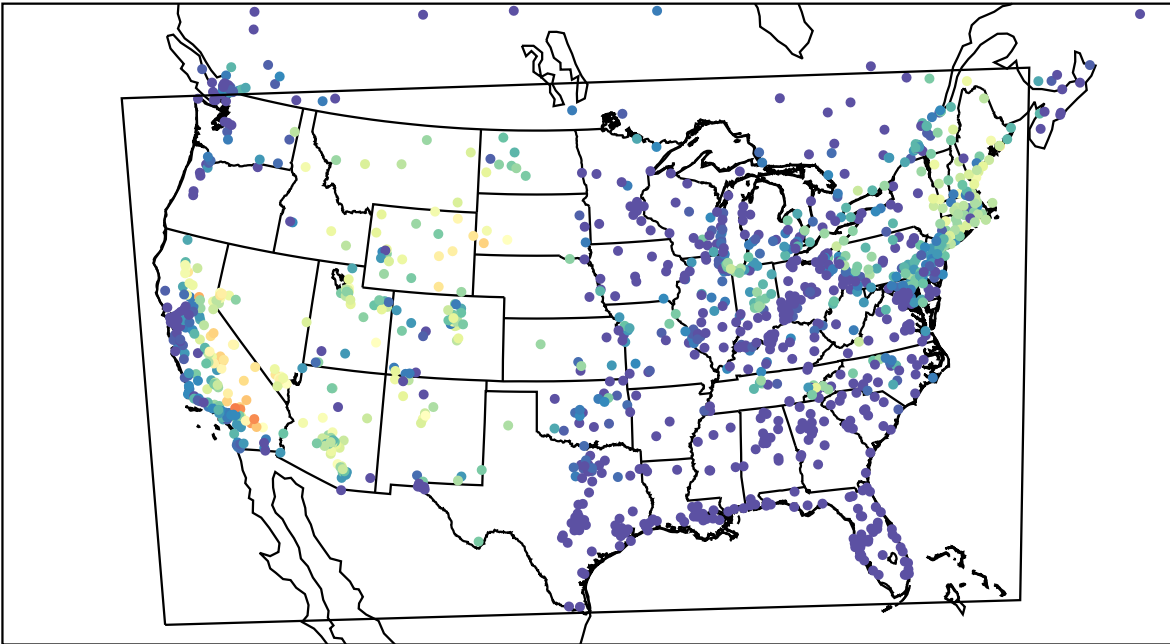
AirNOW (2022-08-22_04:00:00)
