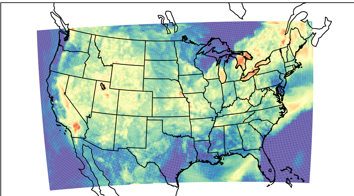
WRF (2022-08-22_04:00:00)
