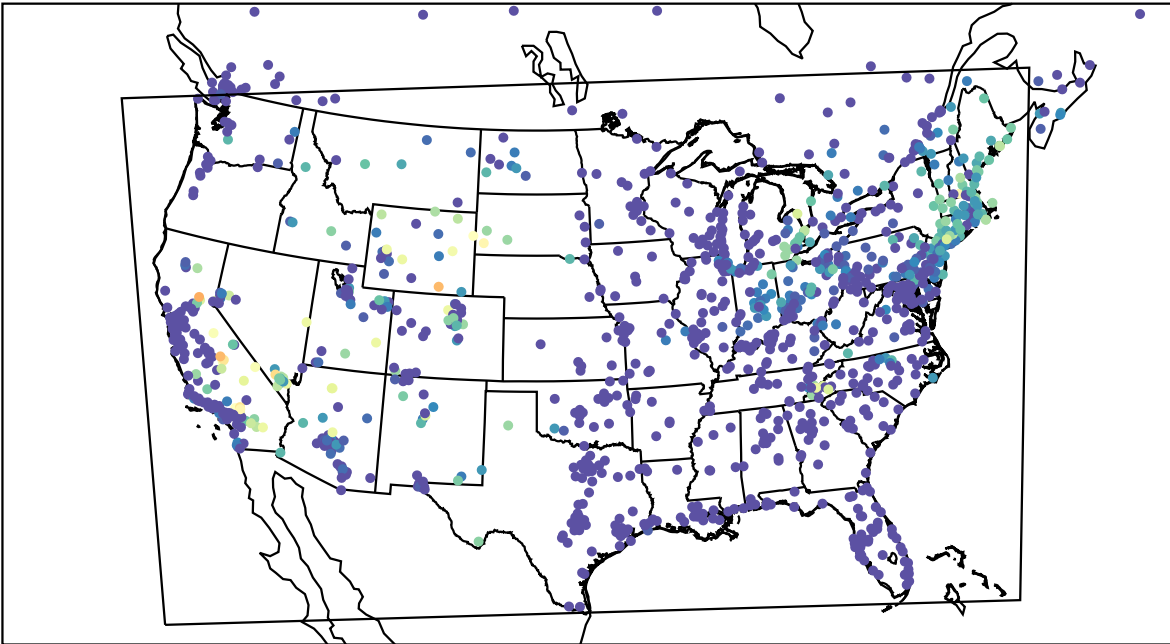
AirNOW (2022-08-22_12:00:00)
