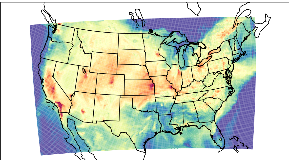
WRF (2022-08-22_23:00:00)
