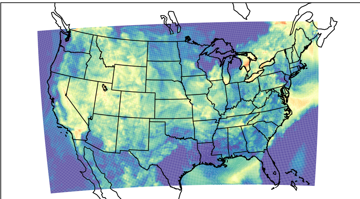
WRF (2022-08-22_09:00:00)
