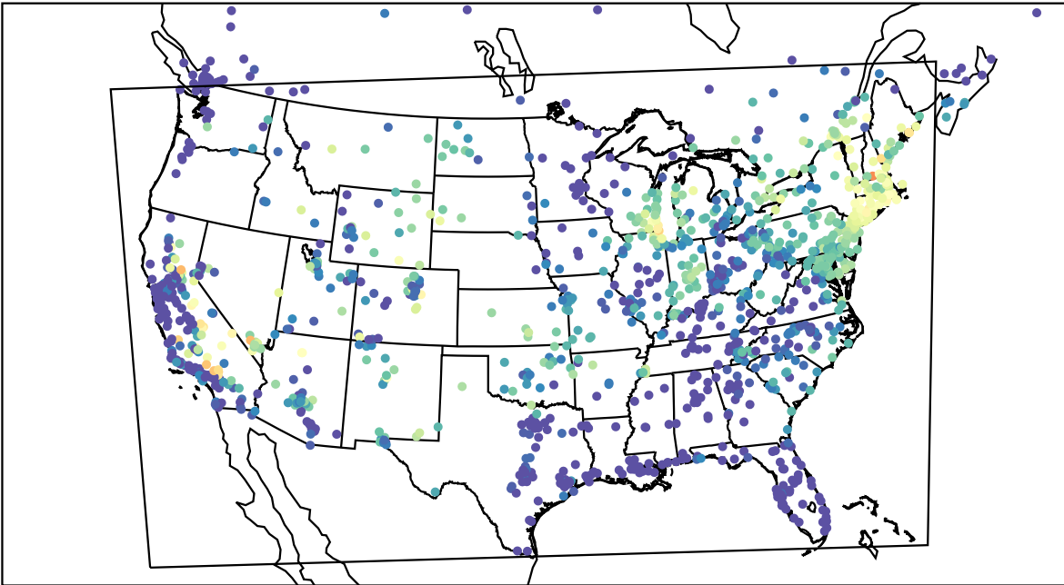
AirNOW (2022-08-21_14:00:00)
