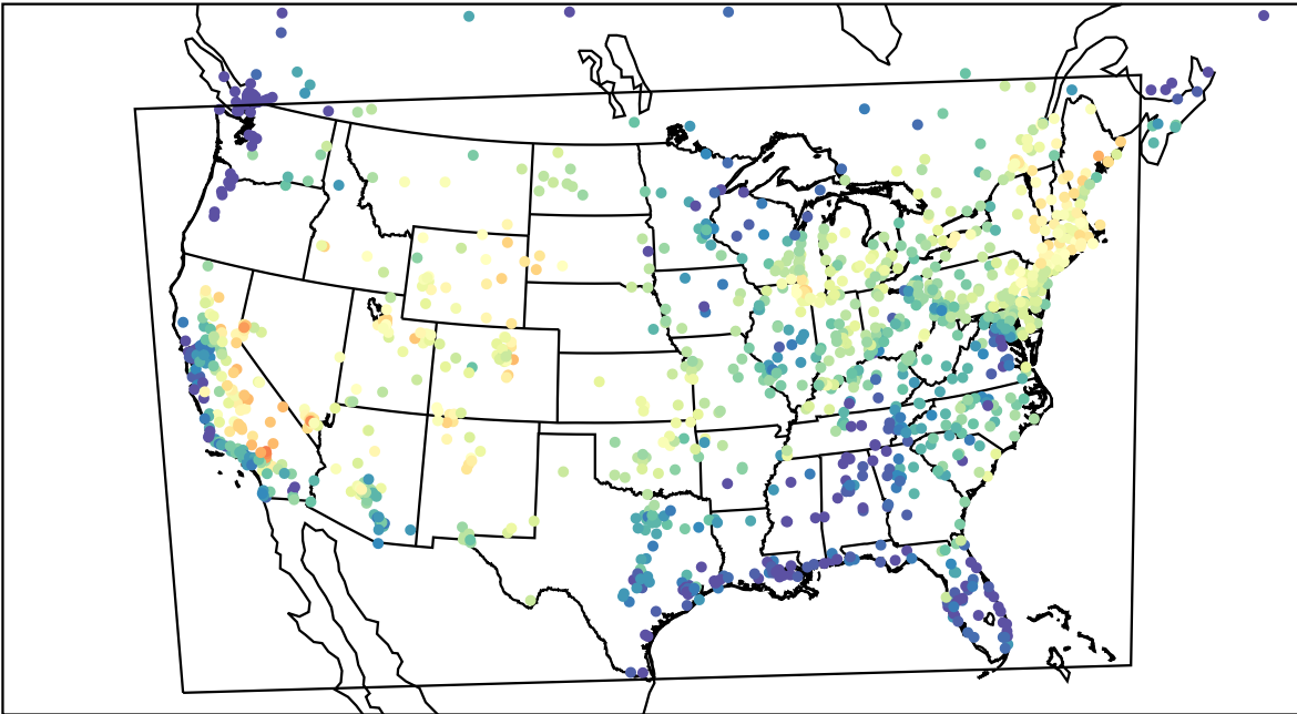
AirNOW (2022-08-21_17:00:00)
