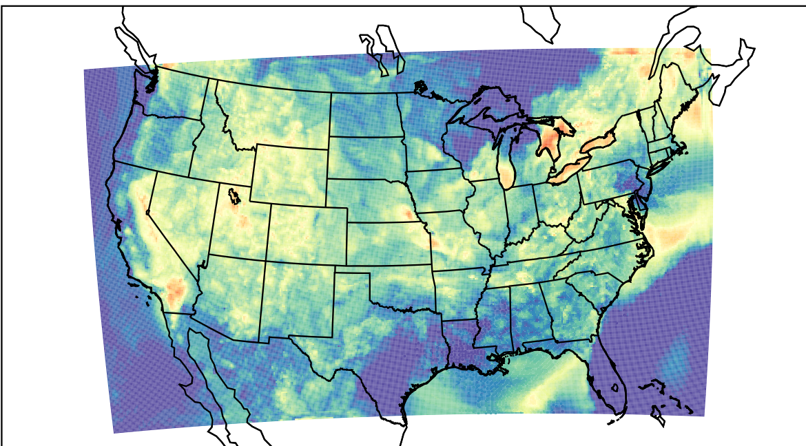
WRF (2022-08-22_06:00:00)
