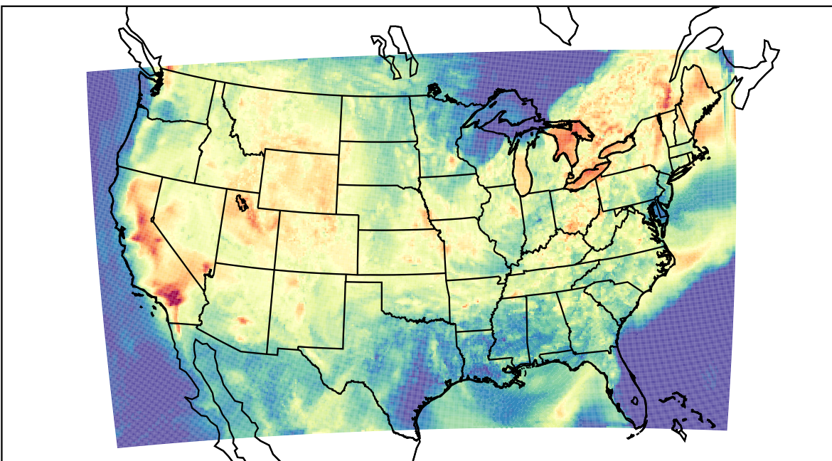
WRF (2022-08-22_01:00:00)
