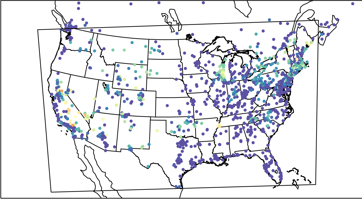
AirNOW (2022-08-21_11:00:00)
