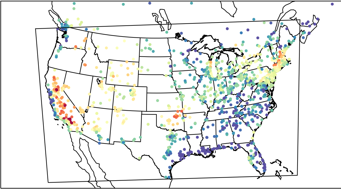
AirNOW (2022-08-21_00:00:00)
