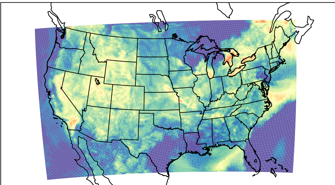
WRF (2022-08-22_07:00:00)
