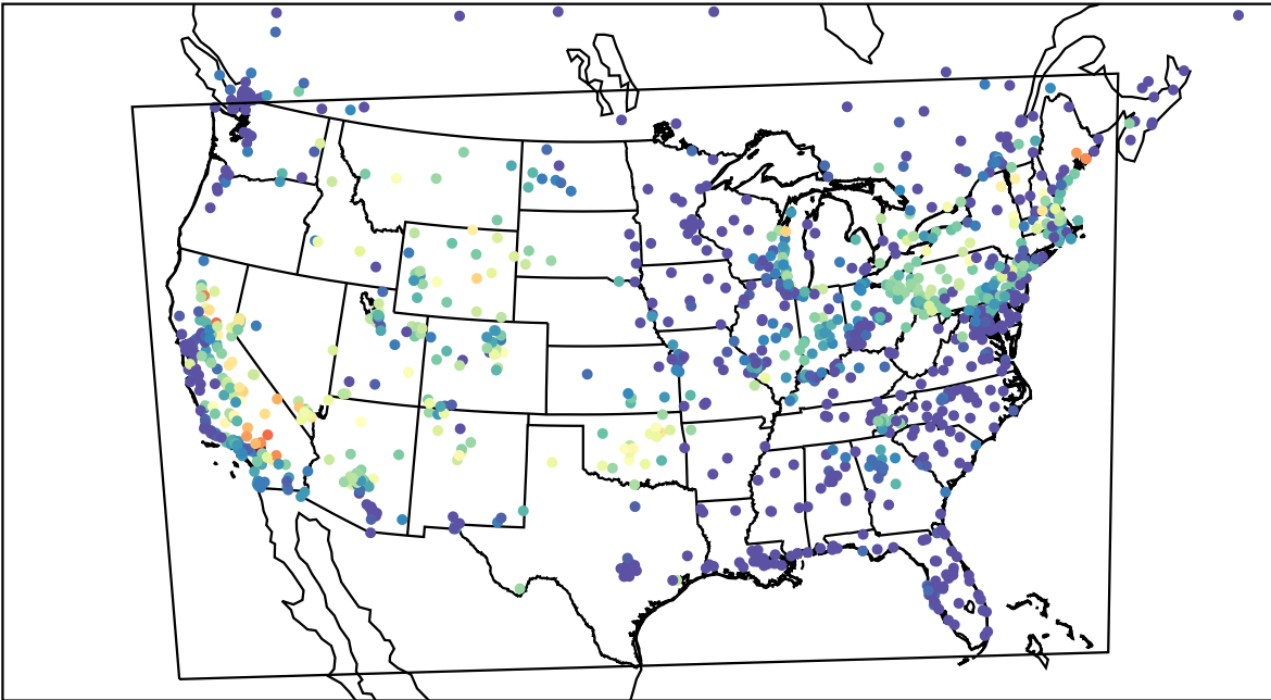
AirNOW (2022-08-21_05:00:00)
