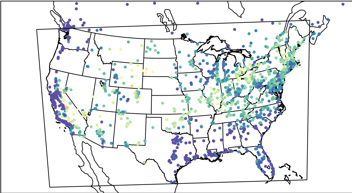
AirNOW (2022-08-22_15:00:00)
