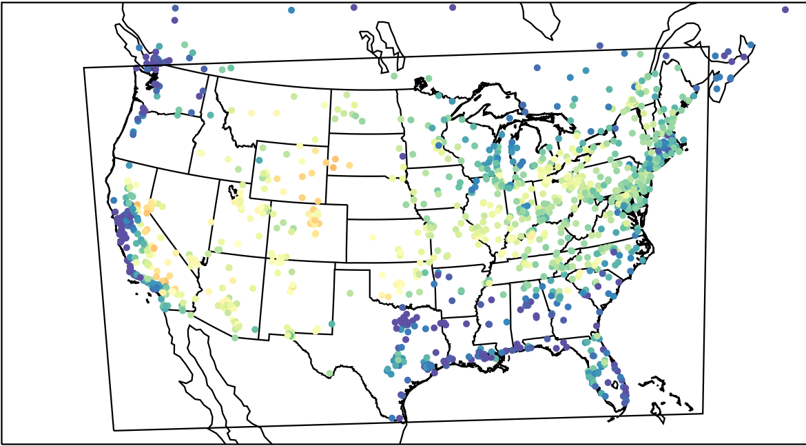
AirNOW (2022-08-22_17:00:00)
