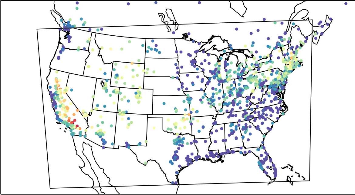
AirNOW (2022-08-21_03:00:00)
