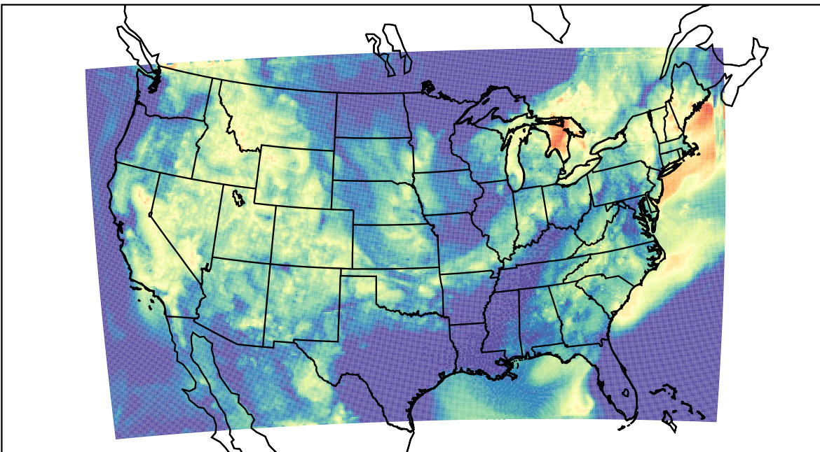
WRF (2022-08-21_11:00:00)
