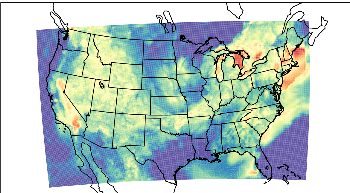
WRF (2022-08-21_05:00:00)
