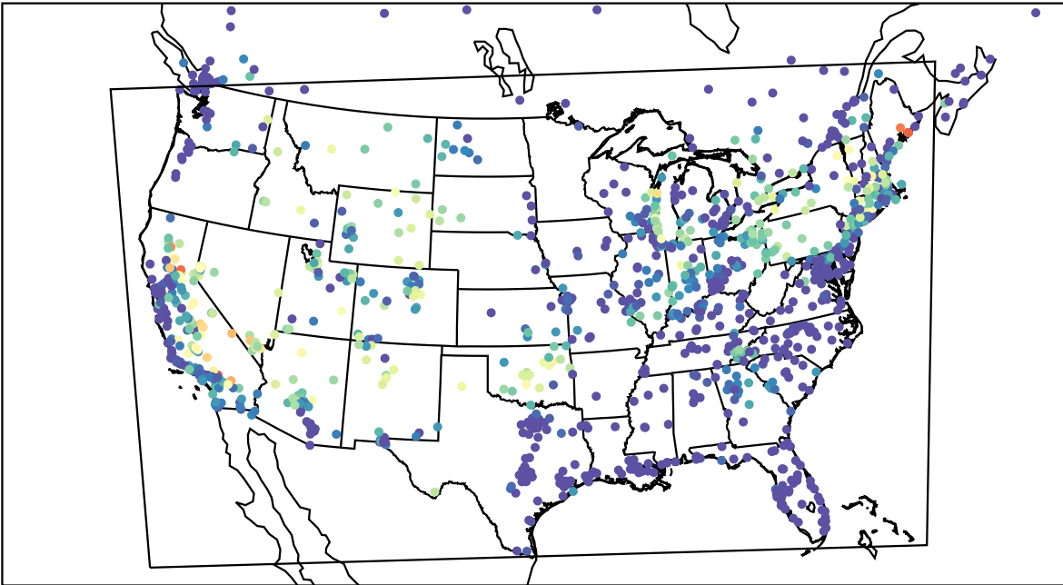
AirNOW (2022-08-21_06:00:00)
