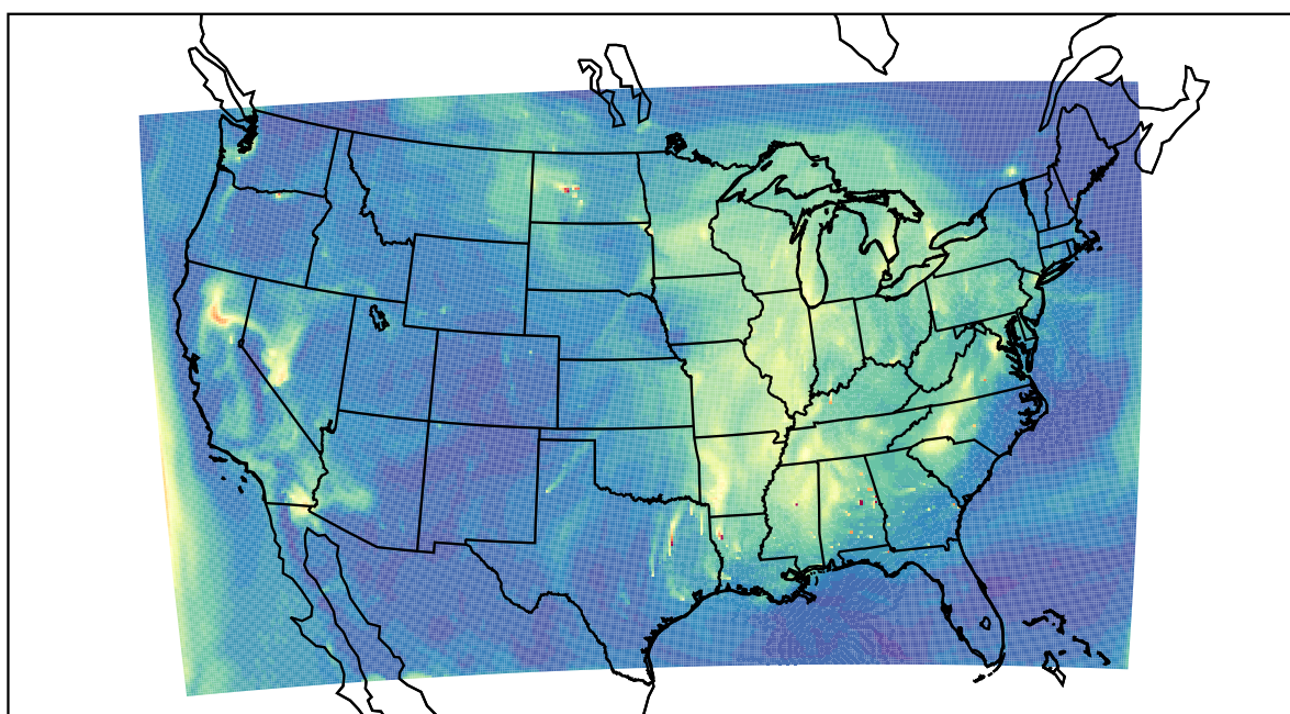
WRF 2022-09-17_17:00:00
